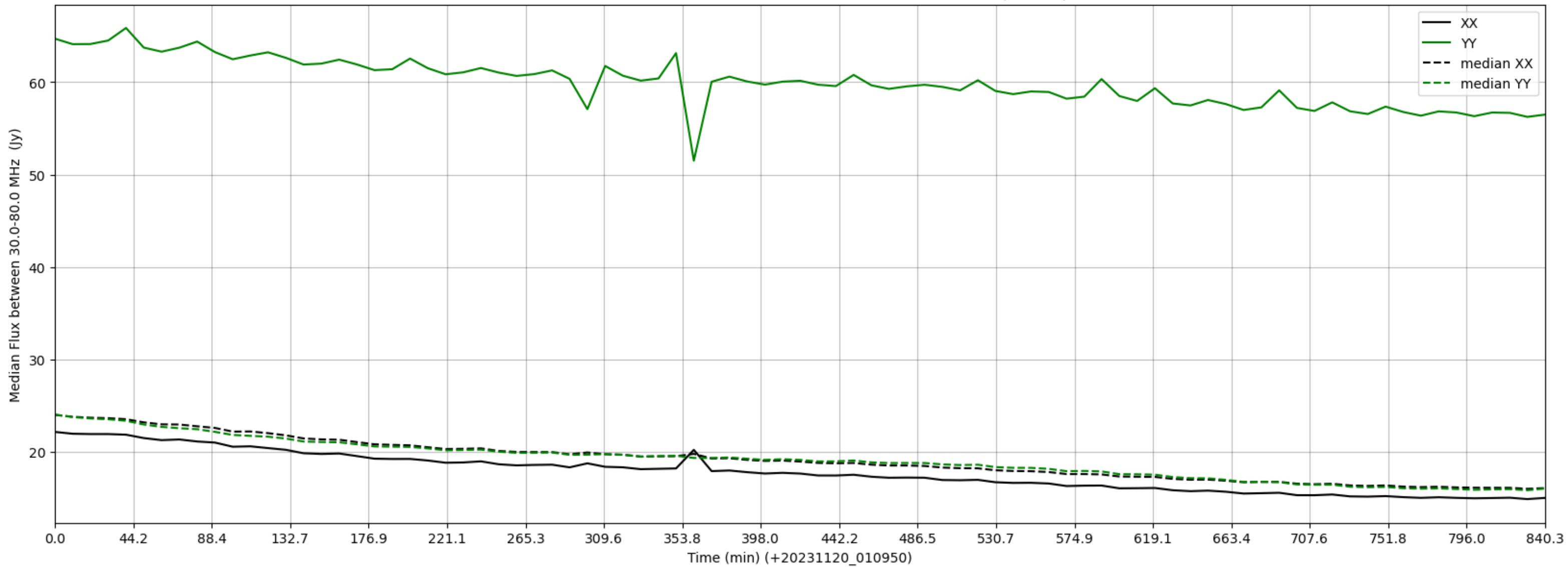
LWA169 - Correlator# 292 - XX FLAGS:Good - YY FLAGS:BadSpecShape
