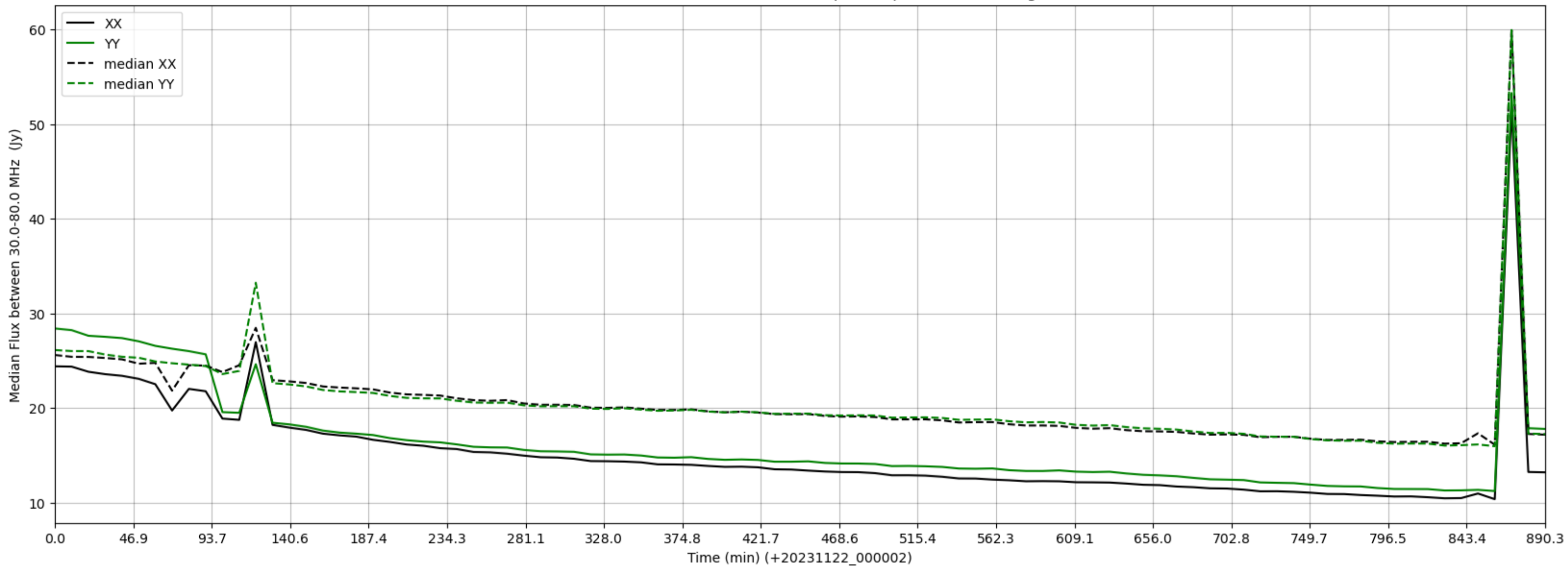
LWA335 - Correlator# 057 - XX FLAGS:BadSpecShape - YY FLAGS:HighTimeVar
