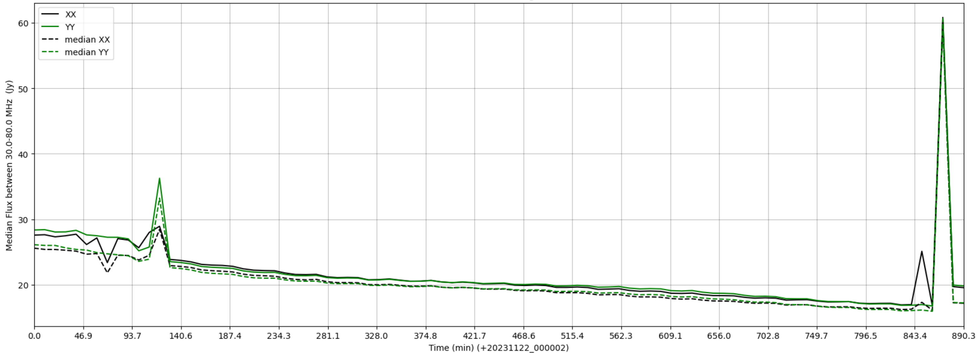
LWA001 - Correlator# 065 - XX FLAGS:HighTimeVar - YY FLAGS:Good
