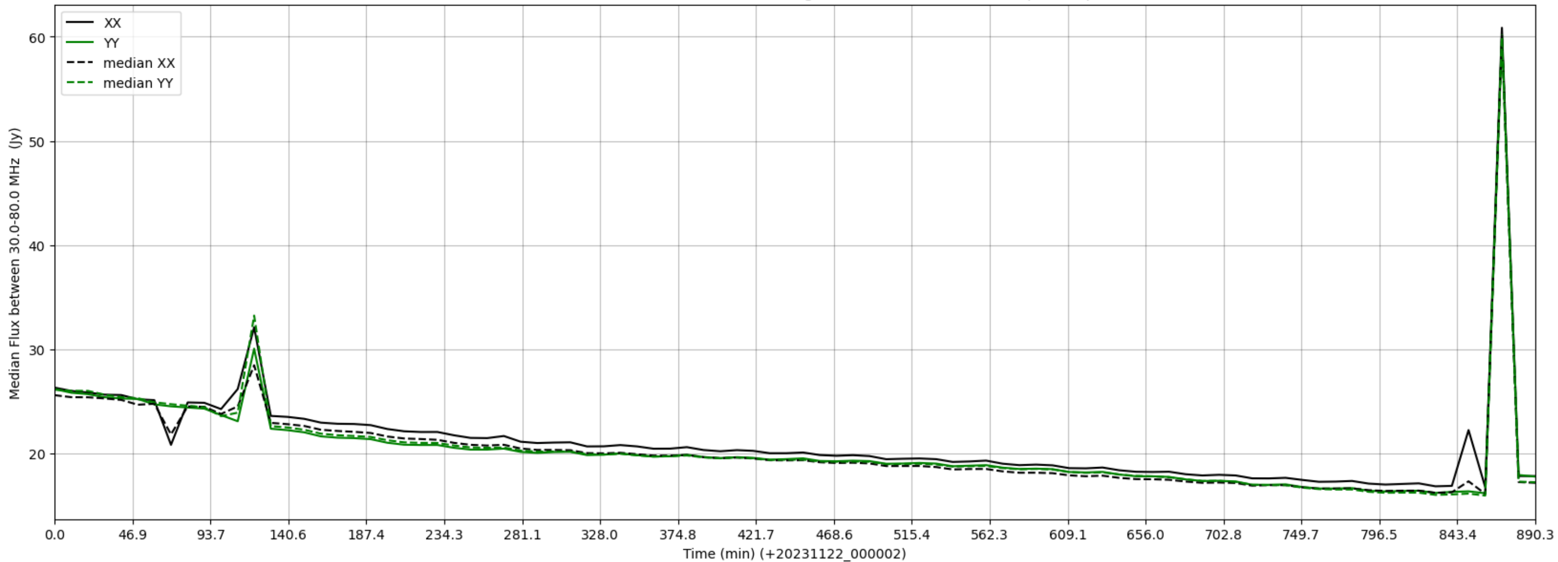
LWA237 - Correlator# 311 - XX FLAGS:HighTimeVar - YY FLAGS:BadSpecShape
