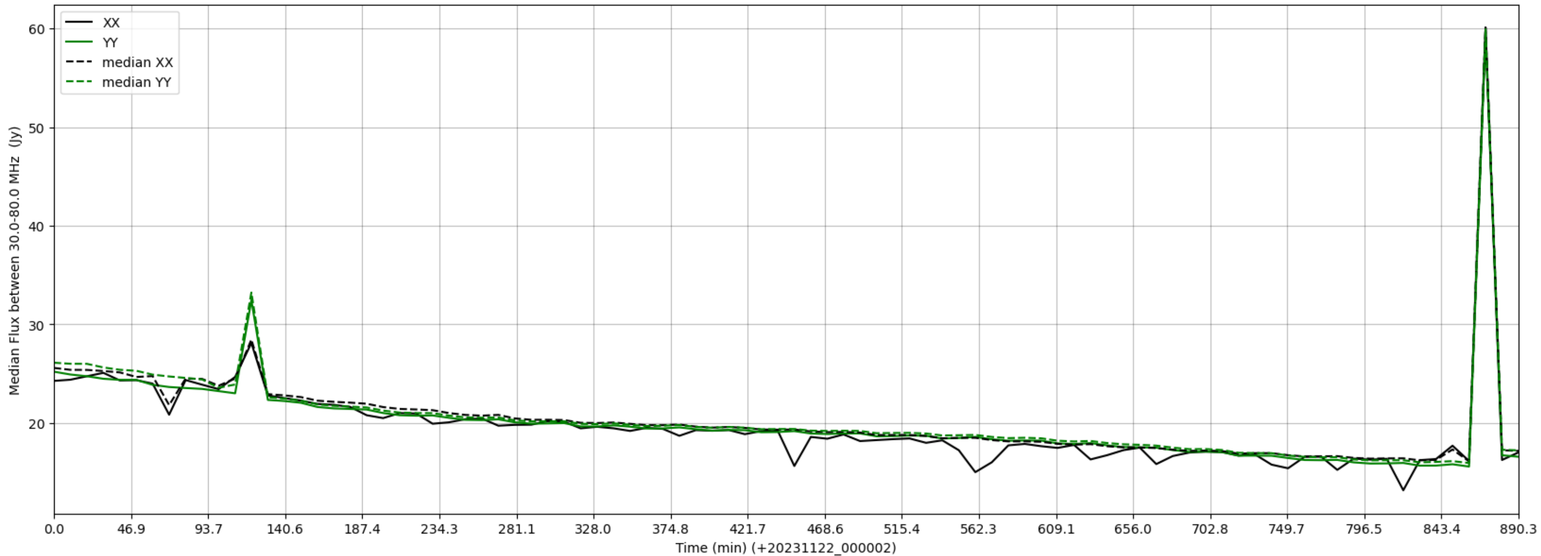
LWA209 - Correlator# 301 - XX FLAGS:Good - YY FLAGS:Good
