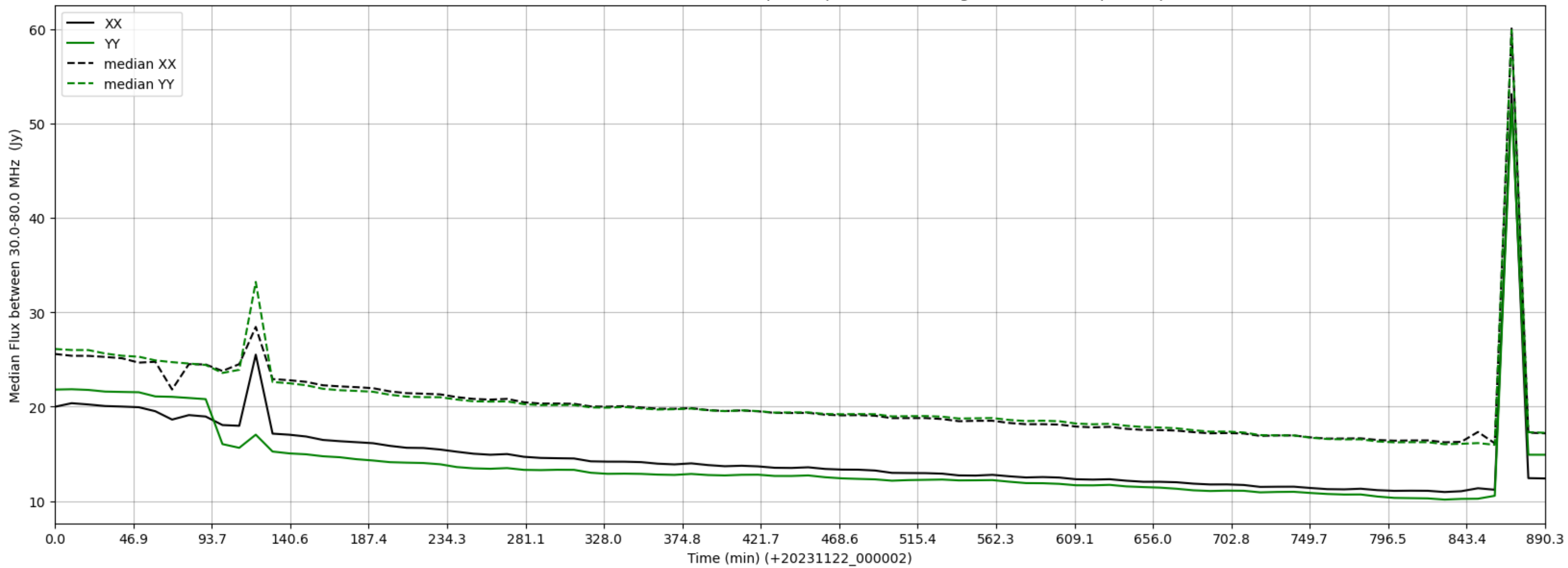
LWA302 - Correlator# 092 - XX FLAGS:BadSpecShape - YY FLAGS:HighTimeVar+BadSpecShape
