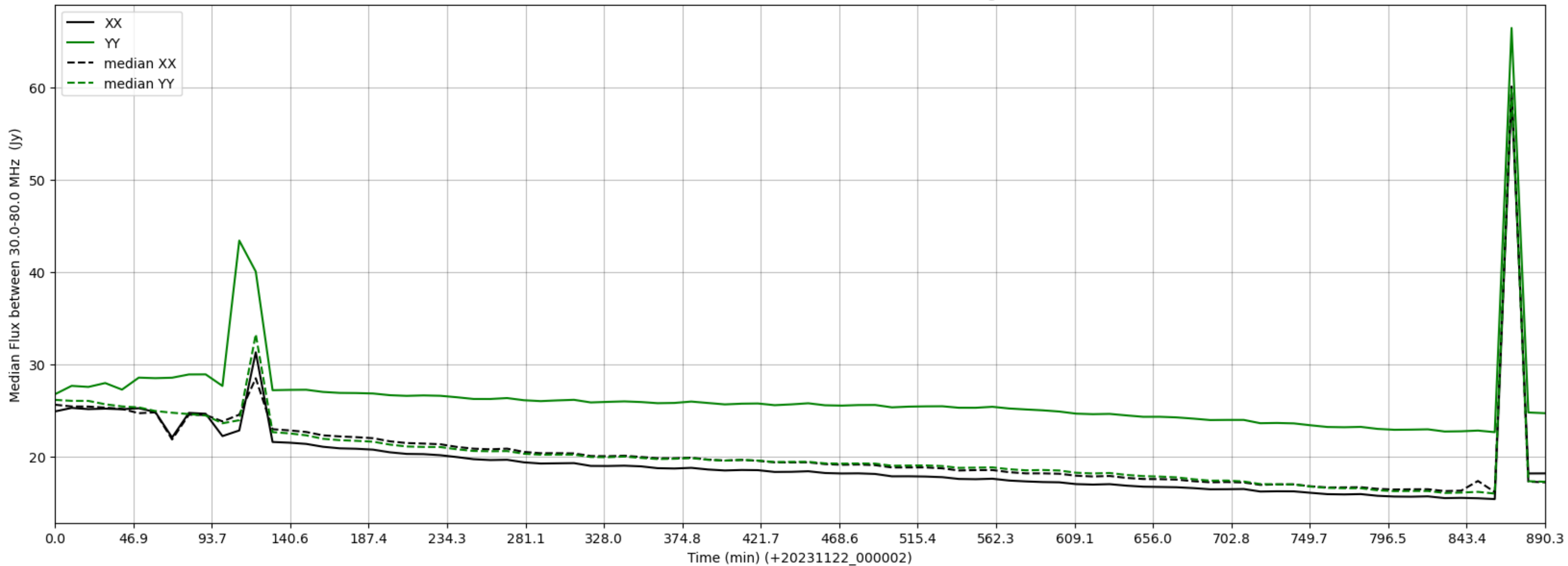
LWA316 - Correlator# 155 - XX FLAGS:Good - YY FLAGS:HighTimeVar
