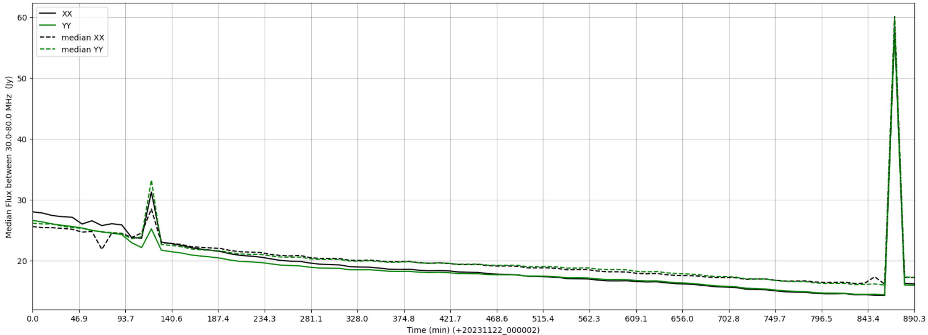
LWA349 - Correlator# 282 - XX FLAGS:Good - YY FLAGS:BadSpecShape
