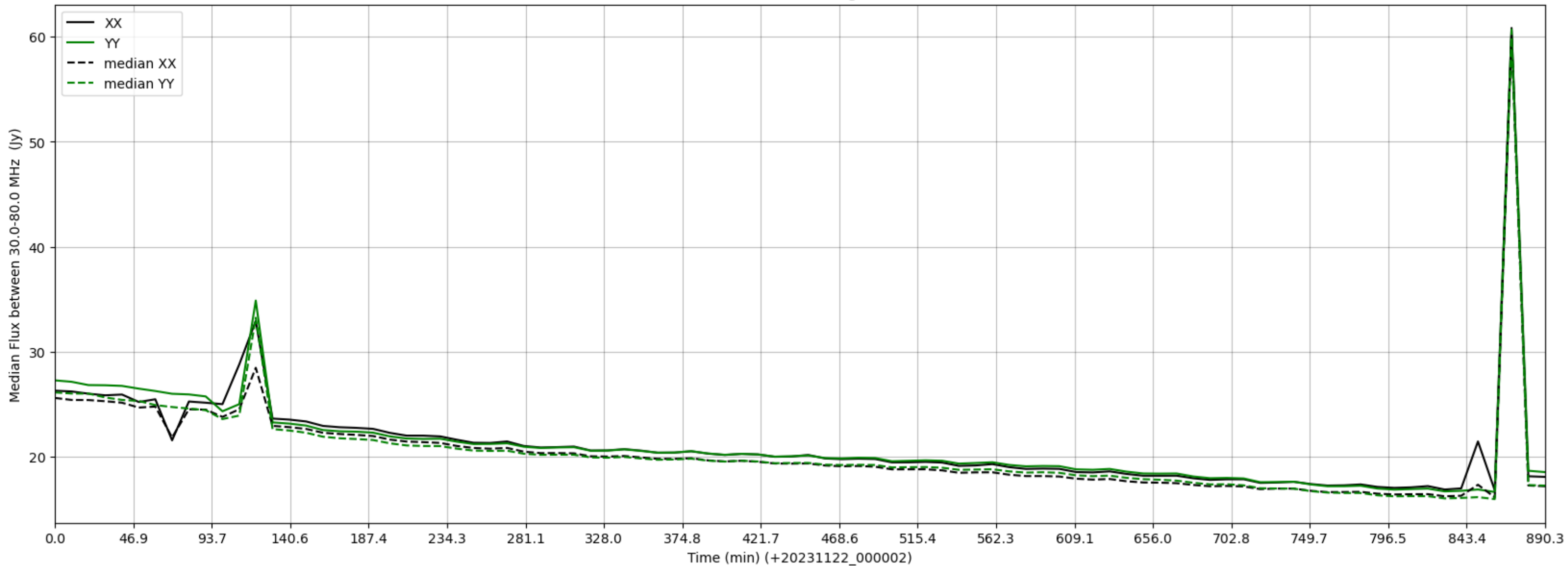
LWA228 - Correlator# 302 - XX FLAGS:HighTimeVar - YY FLAGS:Good
