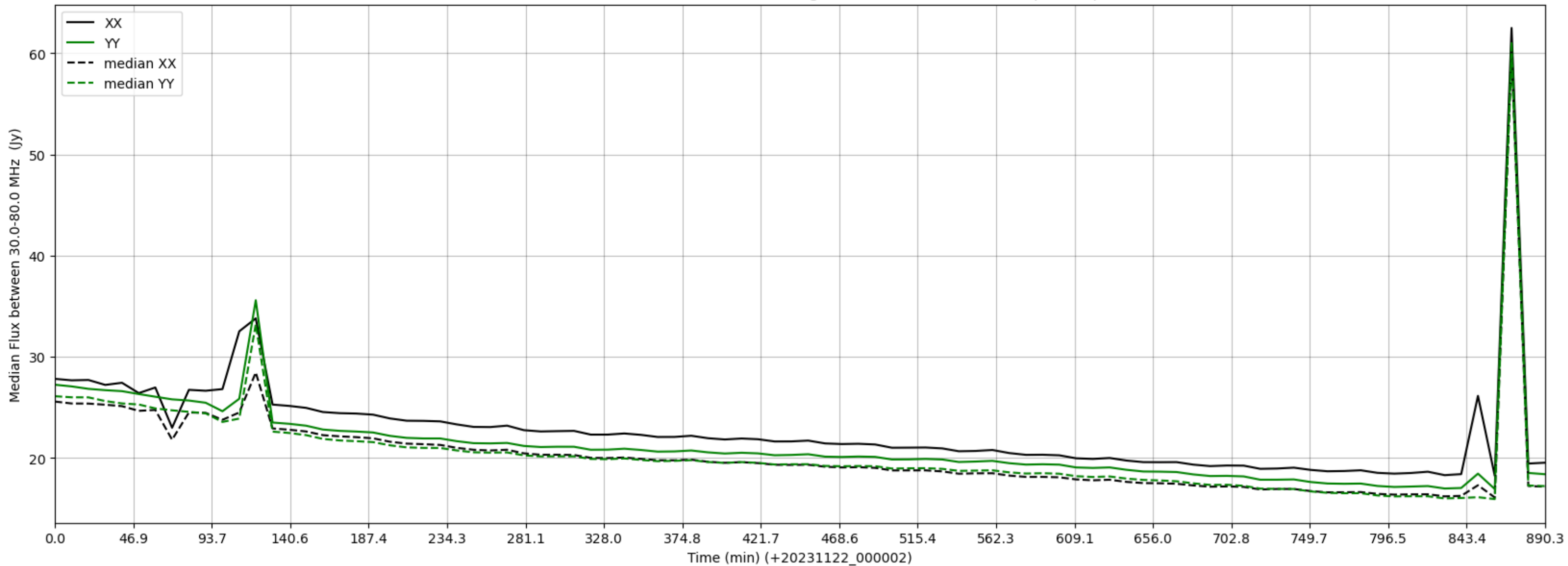
LWA229 - Correlator# 305 - XX FLAGS:HighTimeVar - YY FLAGS:BadSpecShape
