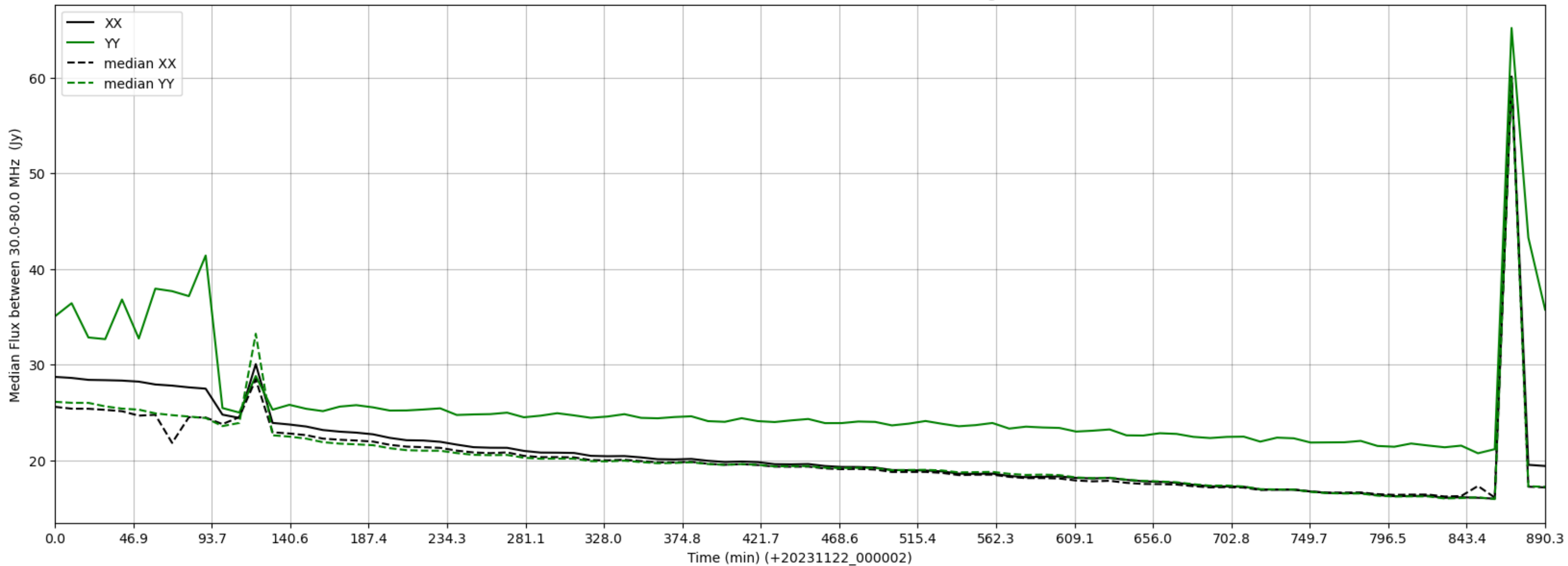
LWA288 - Correlator# 042 - XX FLAGS:Good - YY FLAGS:HighTimeVar
