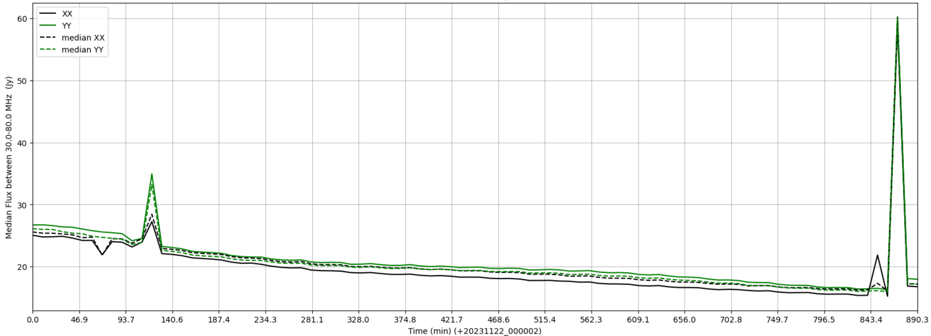
LWA011 - Correlator# 072 - XX FLAGS:HighTimeVar - YY FLAGS:Good
