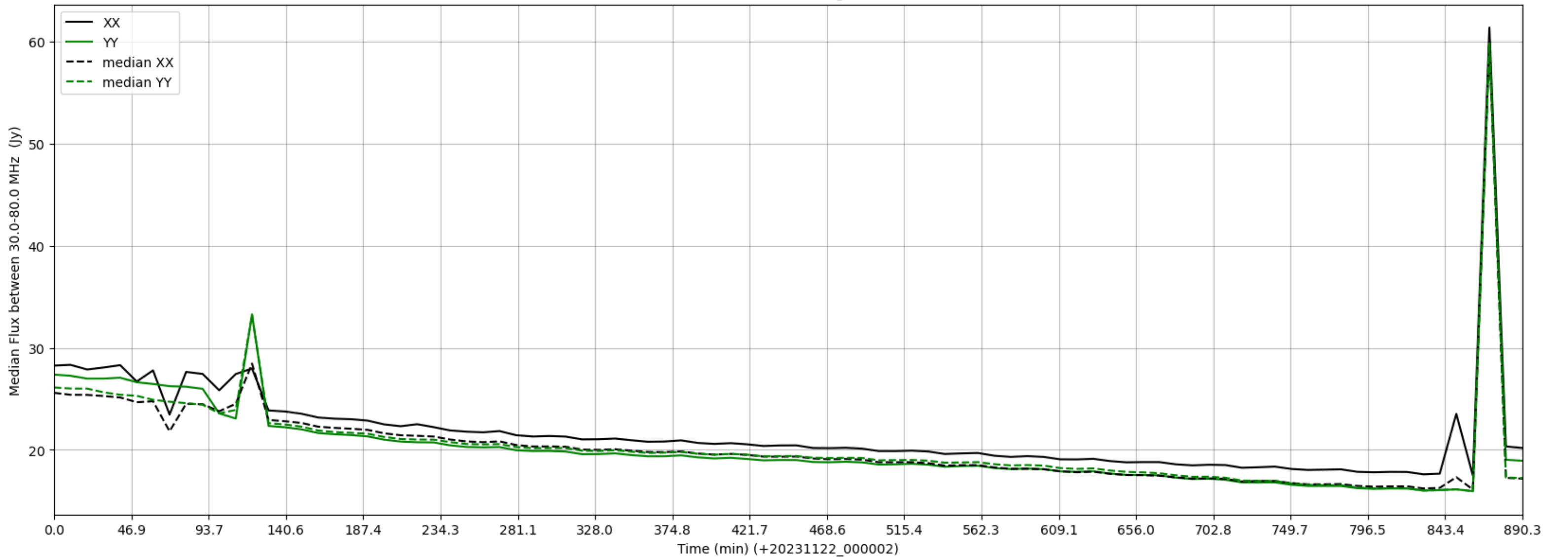
LWA066 - Correlator# 164 - XX FLAGS:HighTimeVar - YY FLAGS:Good
