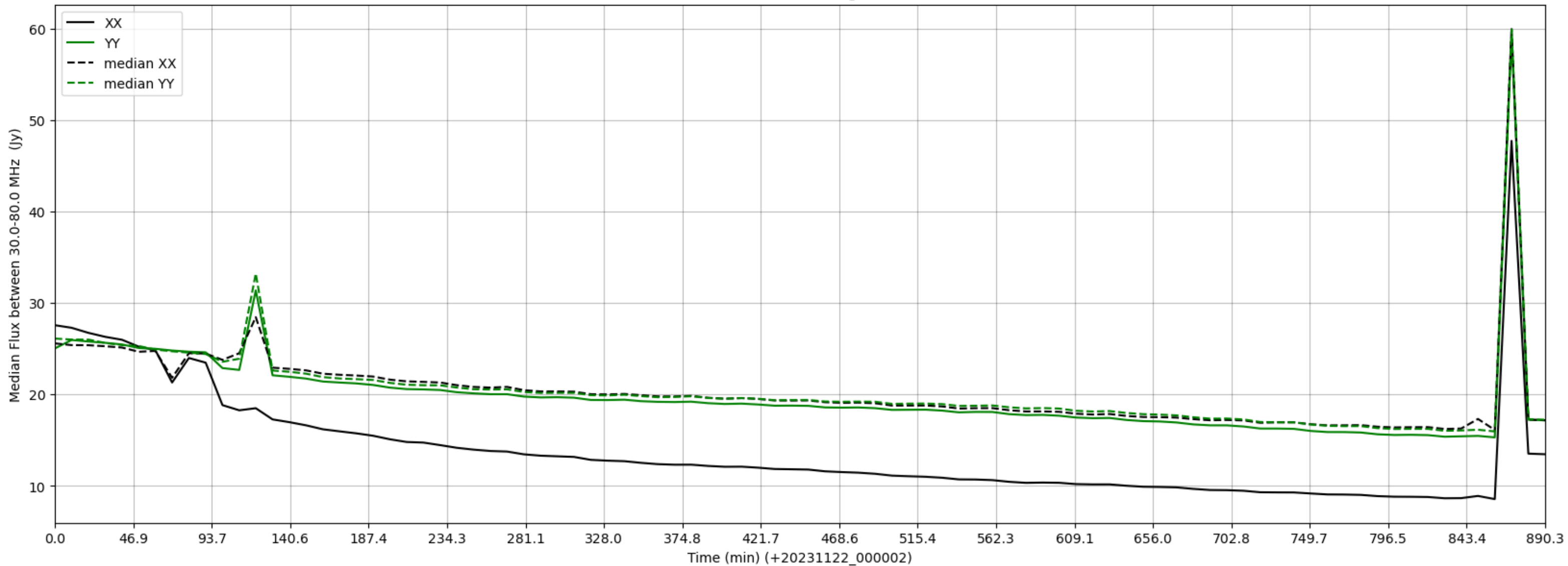
LWA357 - Correlator# 286 - XX FLAGS:HighTimeVar - YY FLAGS:Good
