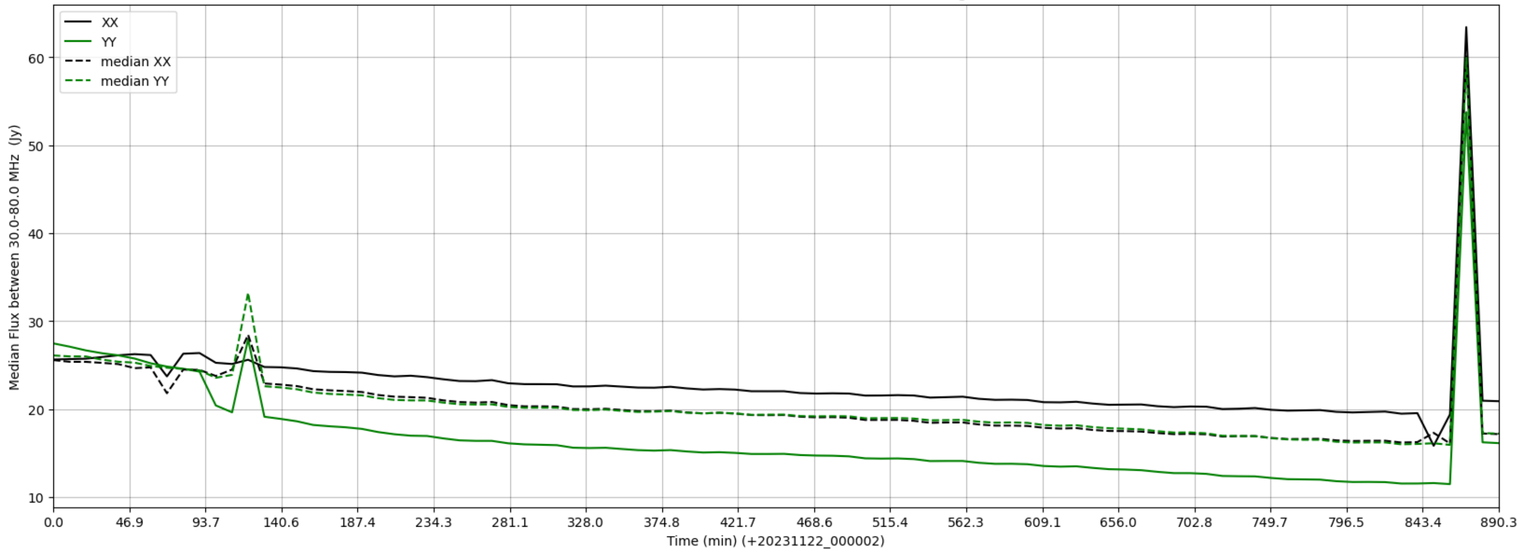
LWA269 - Correlator# 005 - XX FLAGS:Good - YY FLAGS:HighTimeVar
