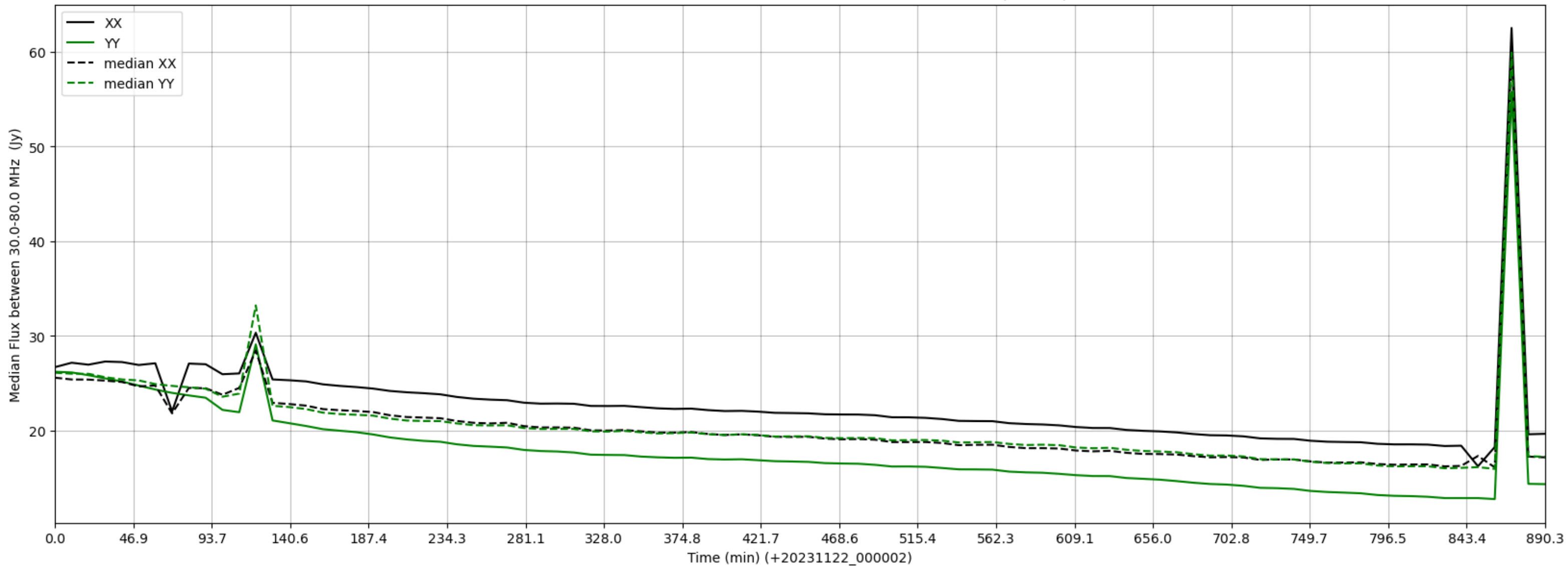
LWA304 - Correlator# 351 - XX FLAGS:Good - YY FLAGS:BadSpecShape
