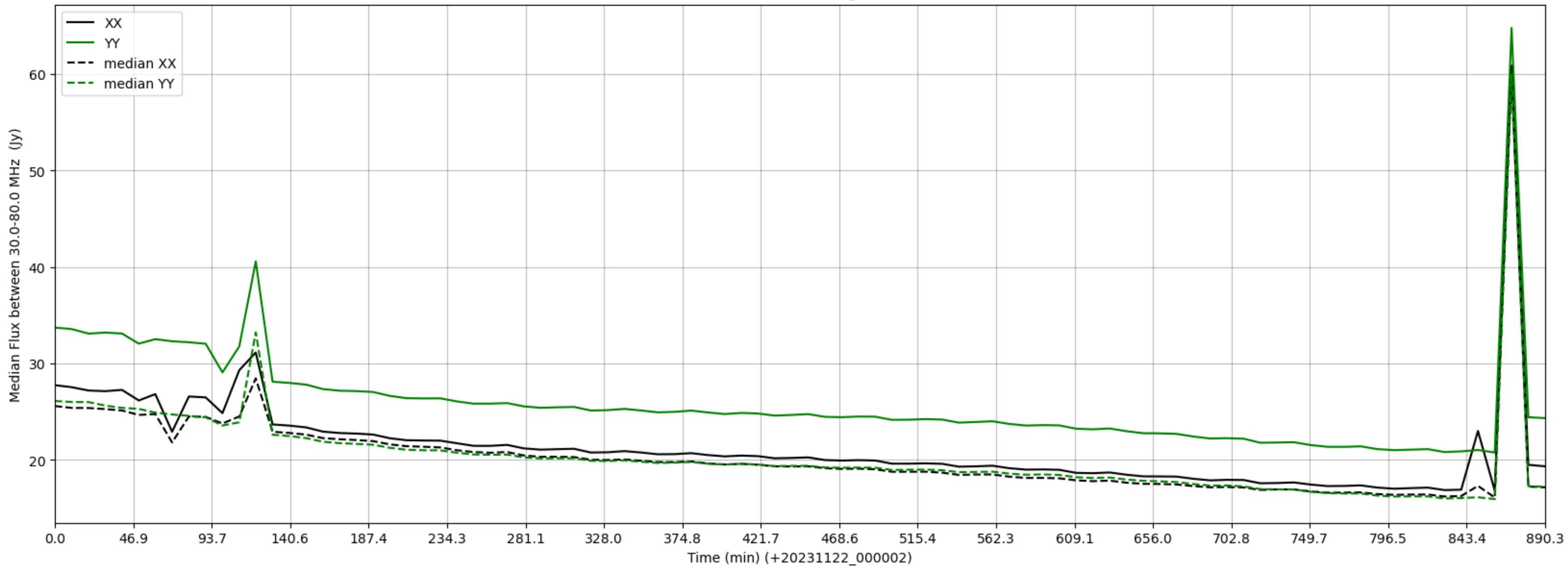
LWA197 - Correlator# 274 - XX FLAGS:HighTimeVar - YY FLAGS:Good
