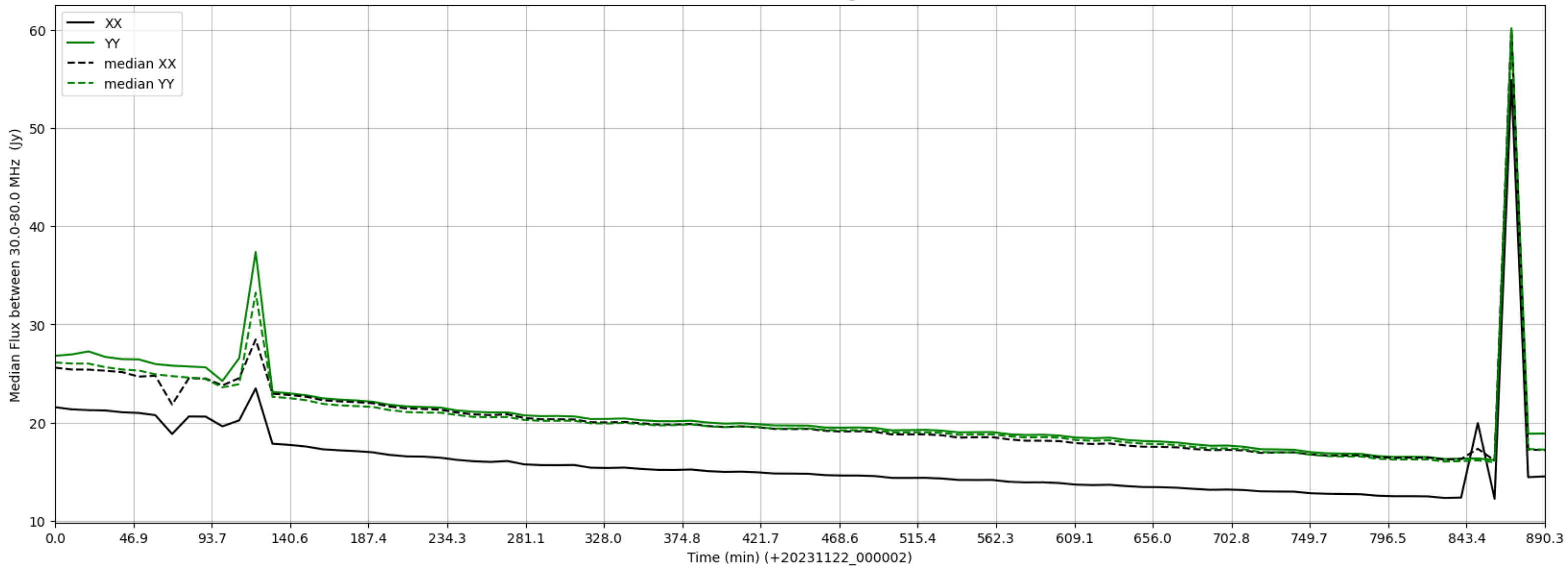
LWA038 - Correlator# 077 - XX FLAGS:HighTimeVar - YY FLAGS:Good
