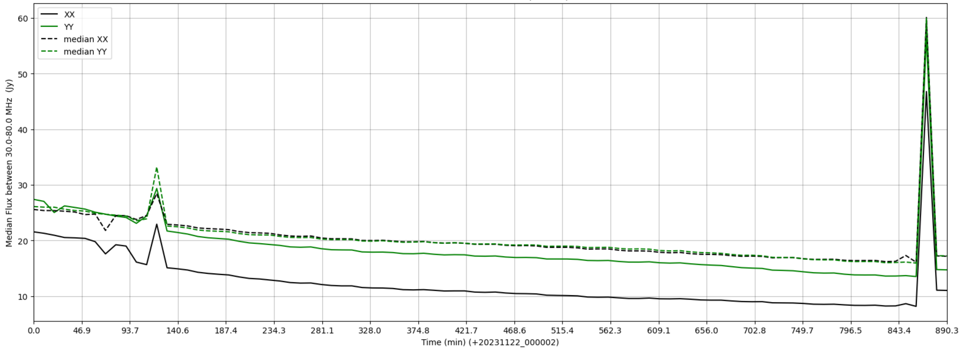
LWA283 - Correlator# 040 - XX FLAGS:BadSpecShape - YY FLAGS:Good
