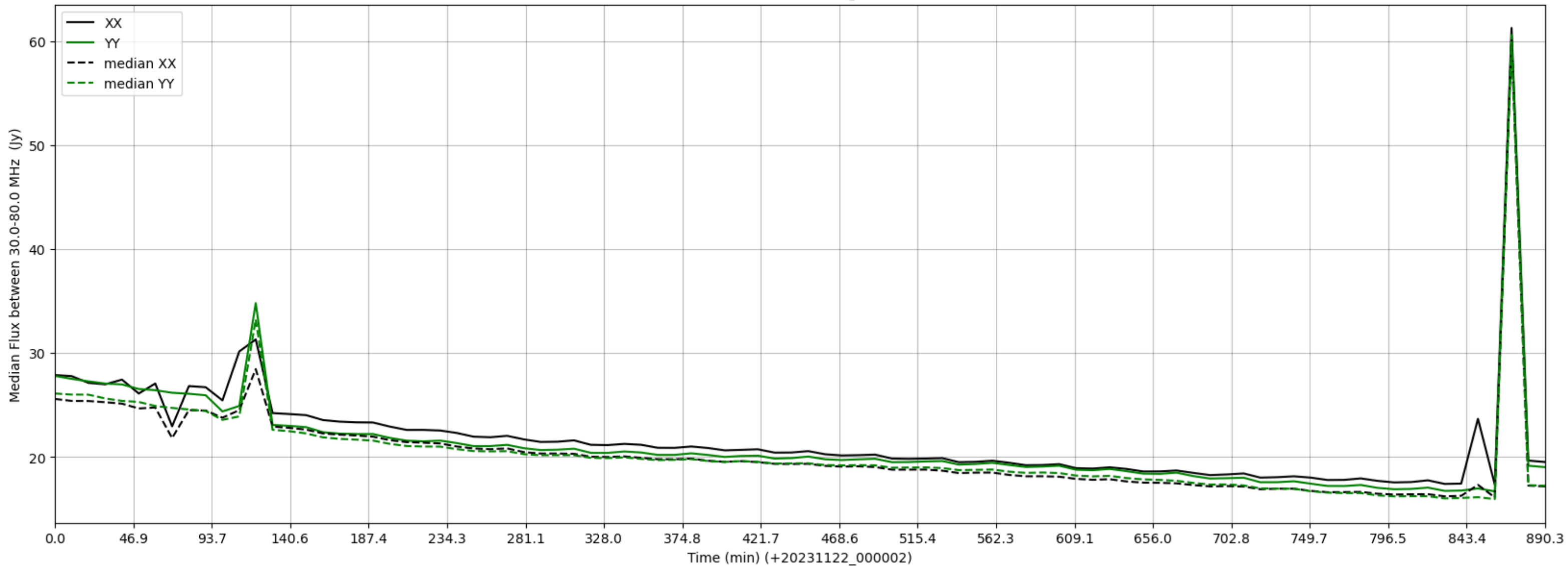
LWA198 - Correlator# 271 - XX FLAGS:HighTimeVar - YY FLAGS:Good
