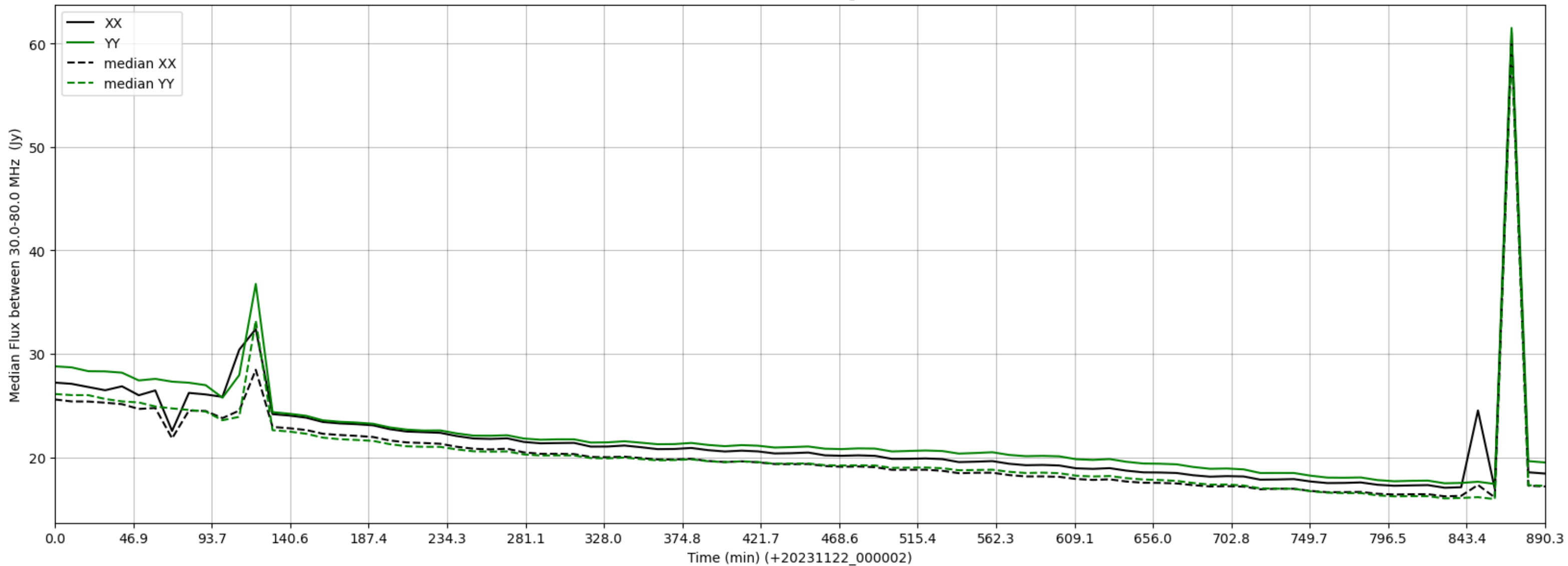
LWA203 - Correlator# 295 - XX FLAGS:HighTimeVar - YY FLAGS:Good
