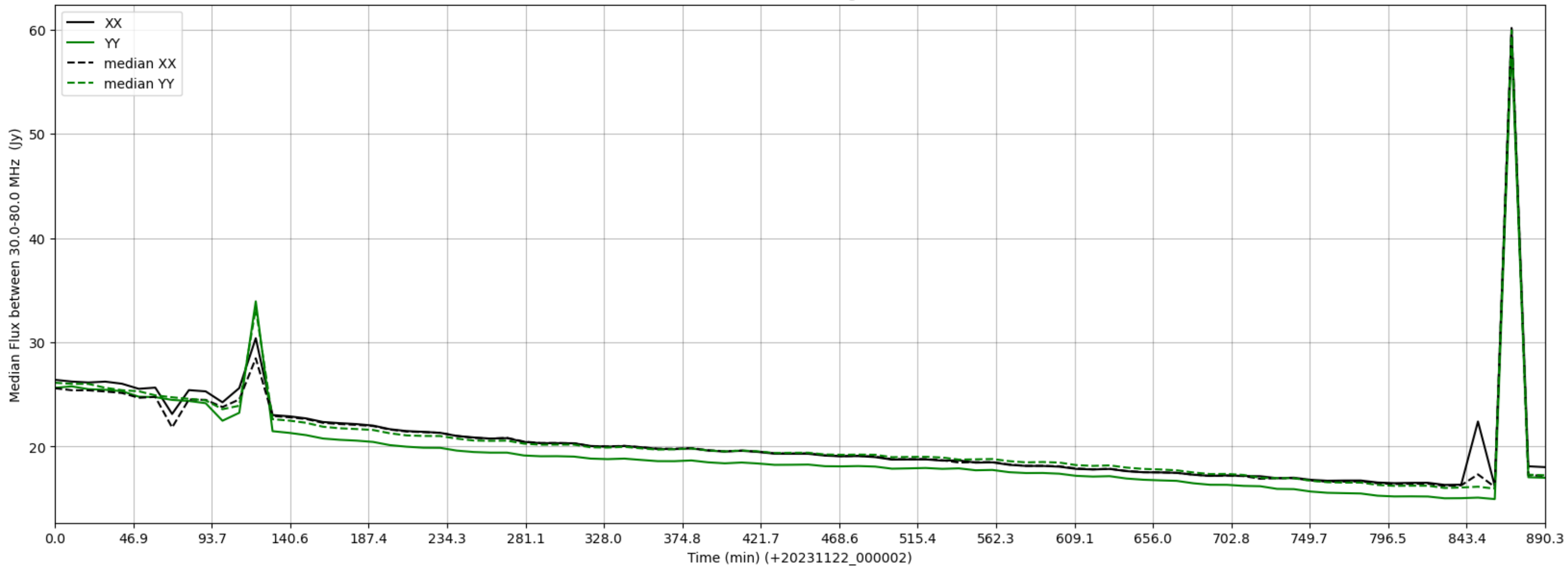
LWA008 - Correlator# 075 - XX FLAGS:HighTimeVar - YY FLAGS:Good
