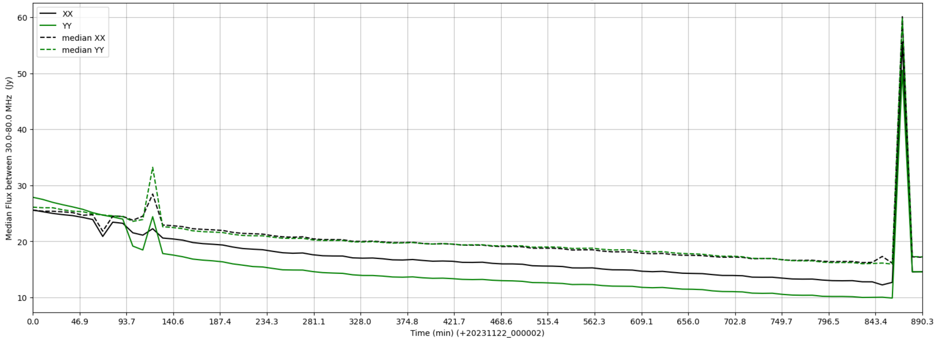
LWA294 - Correlator# 188 - XX FLAGS:Good - YY FLAGS:HighTimeVar
