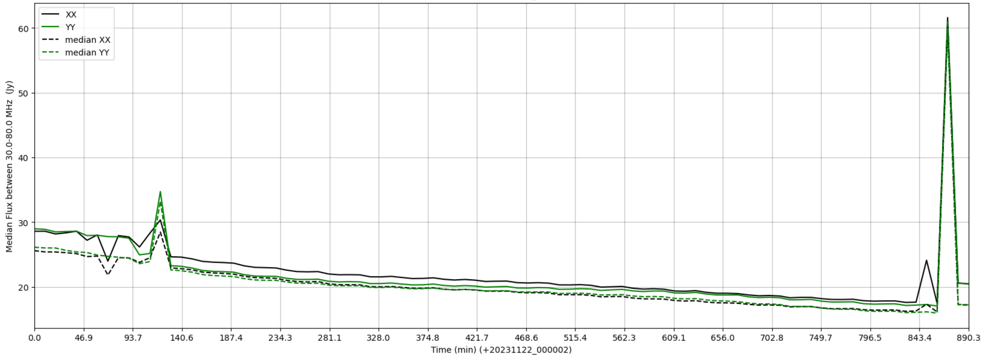
LWA097 - Correlator# 170 - XX FLAGS:HighTimeVar - YY FLAGS:Good
