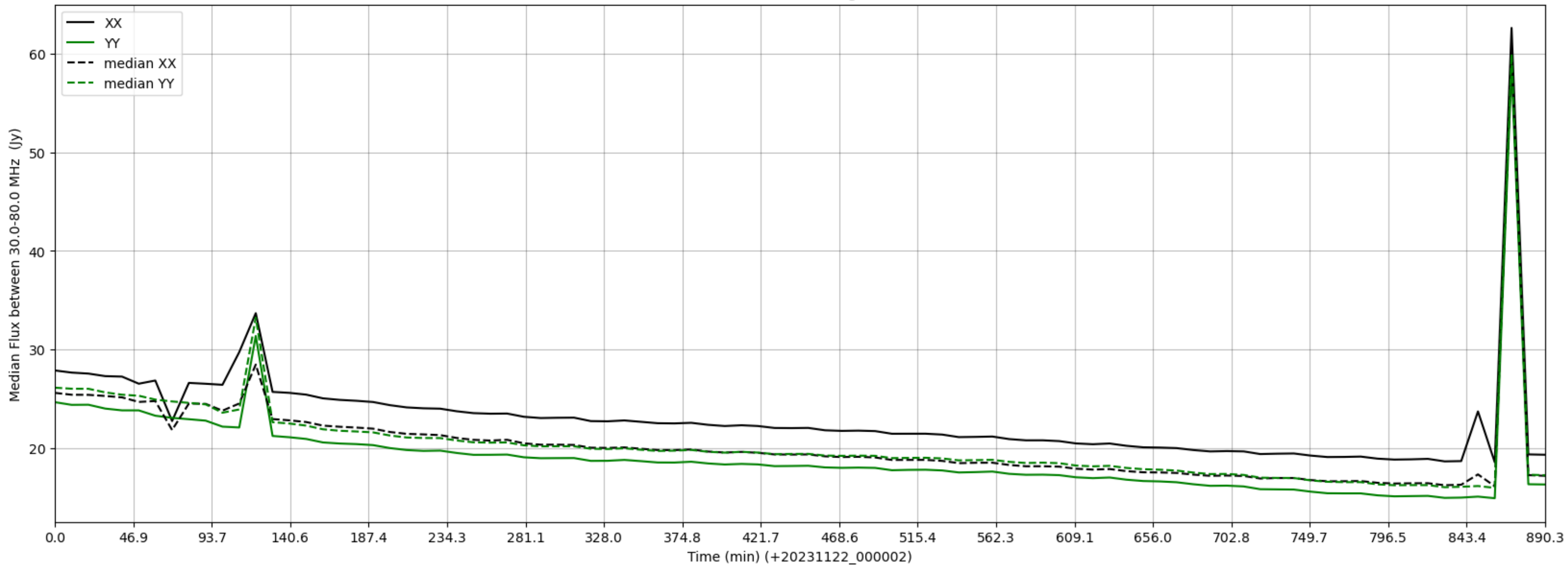
LWA207 - Correlator# 299 - XX FLAGS:HighTimeVar - YY FLAGS:Good
