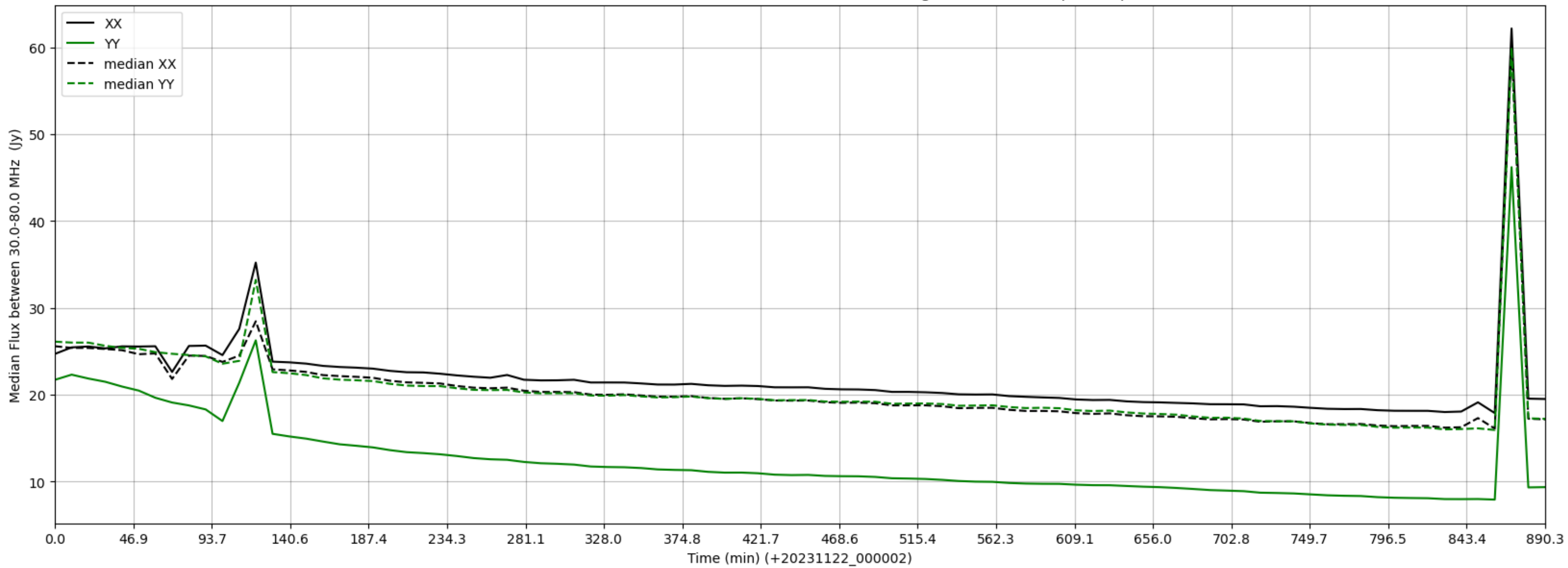
LWA347 - Correlator# 255 - XX FLAGS:Good - YY FLAGS:HighTimeVar+BadSpecShape
