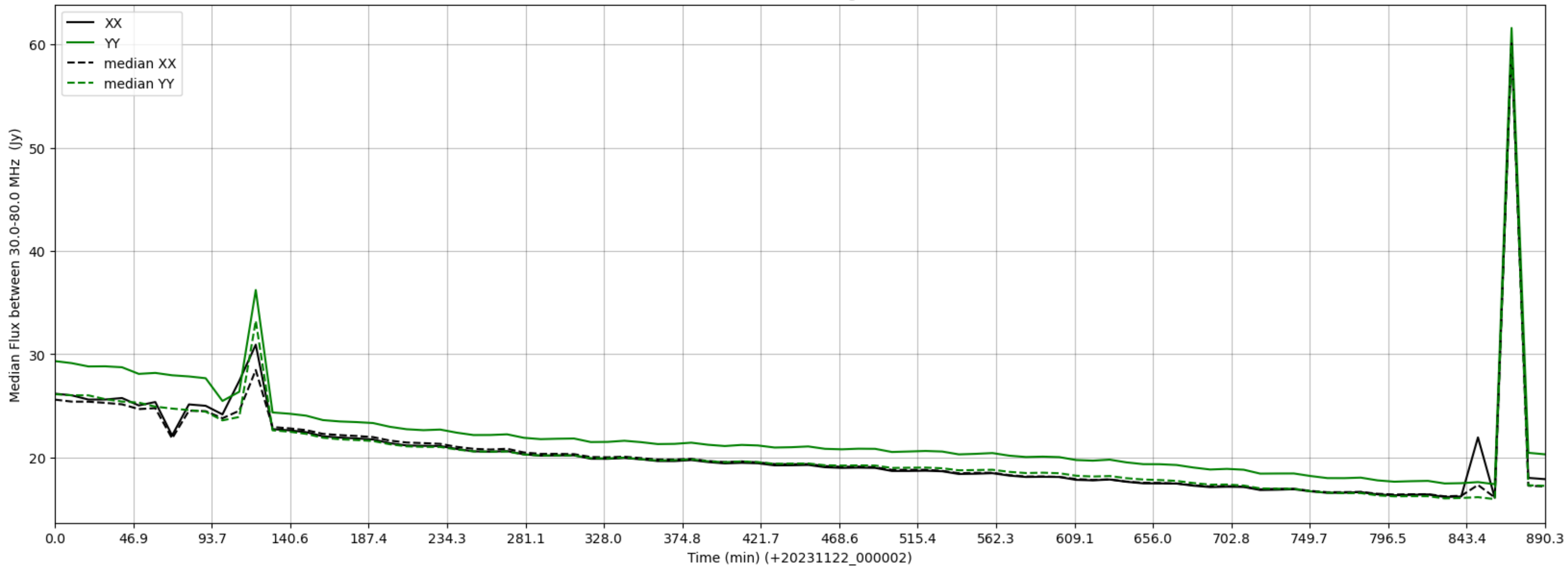
LWA196 - Correlator# 275 - XX FLAGS:HighTimeVar - YY FLAGS:Good
