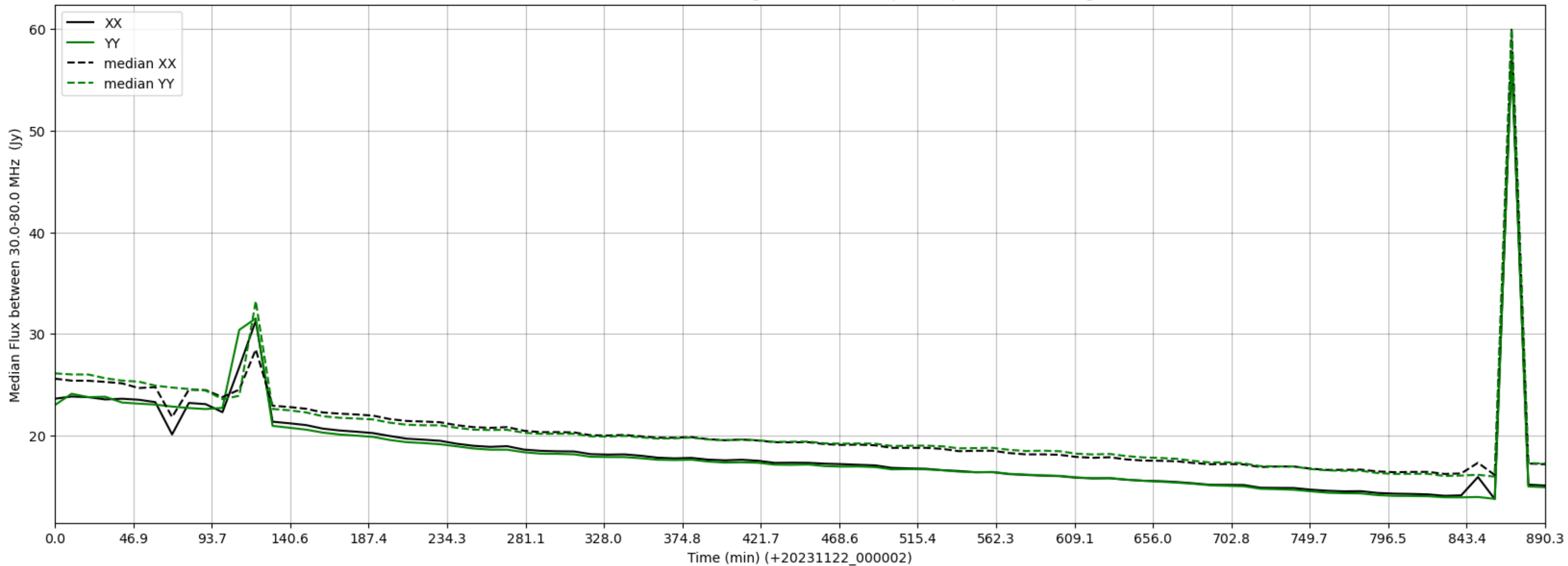
LWA341 - Correlator# 029 - XX FLAGS:HighTimeVar+BadSpecShape - YY FLAGS:HighTimeVar
