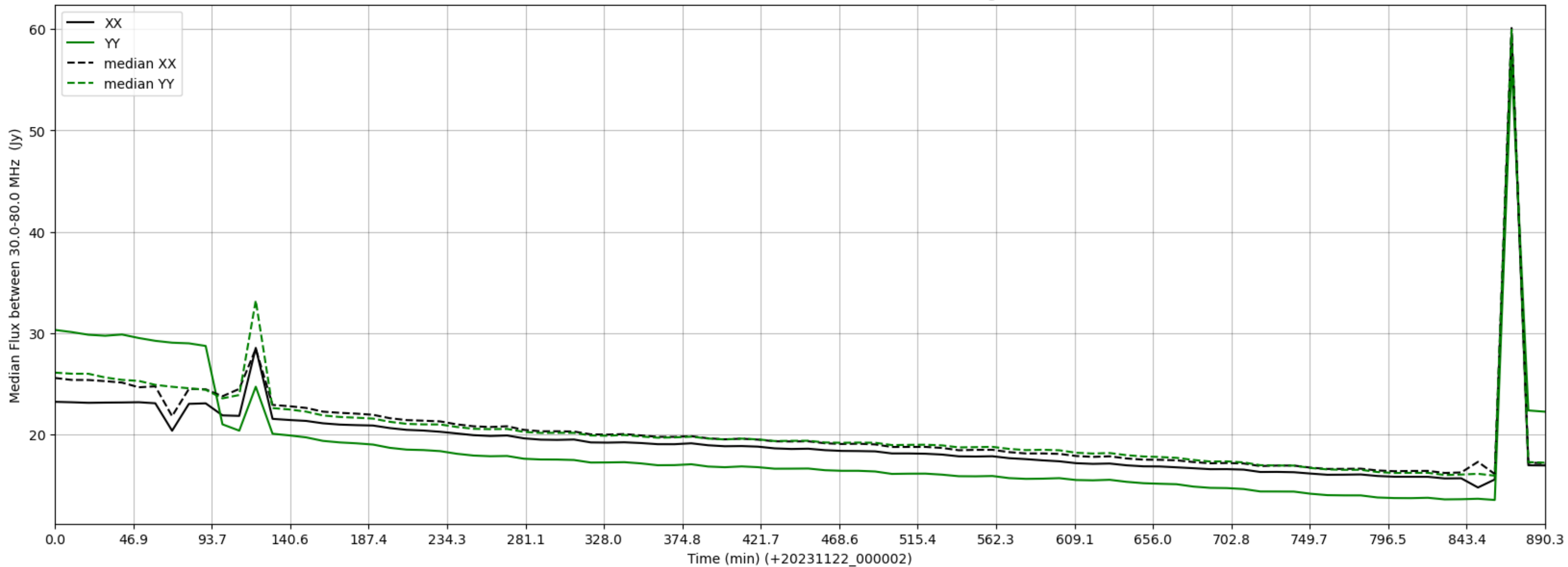
LWA354 - Correlator# 063 - XX FLAGS:Good - YY FLAGS:HighTimeVar
