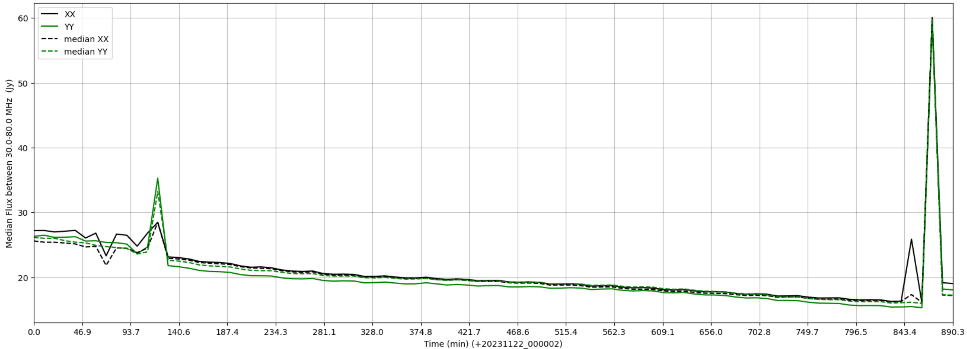
LWA034 - Correlator# 162 - XX FLAGS:HighTimeVar - YY FLAGS:Good
