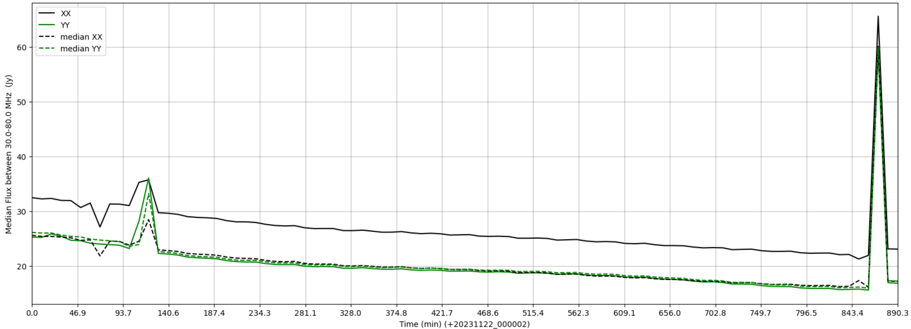
LWA075 - Correlator# 089 - XX FLAGS:Good - YY FLAGS:HighTimeVar
