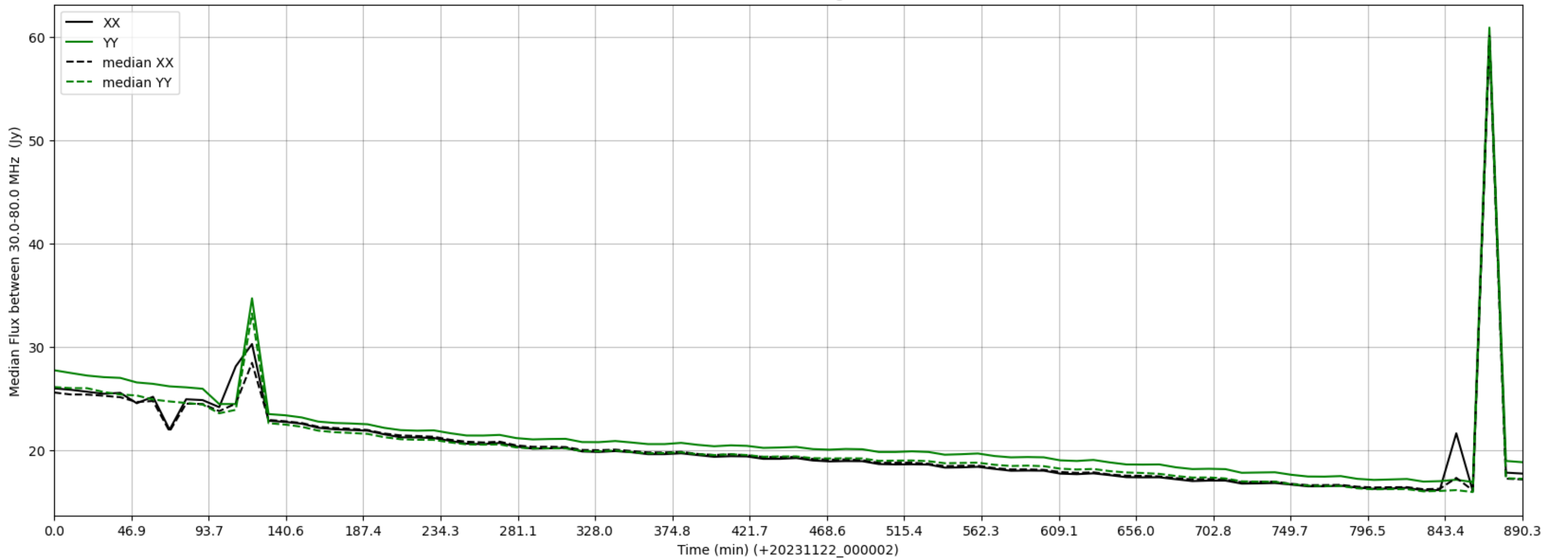
LWA134 - Correlator# 184 - XX FLAGS:HighTimeVar - YY FLAGS:Good
