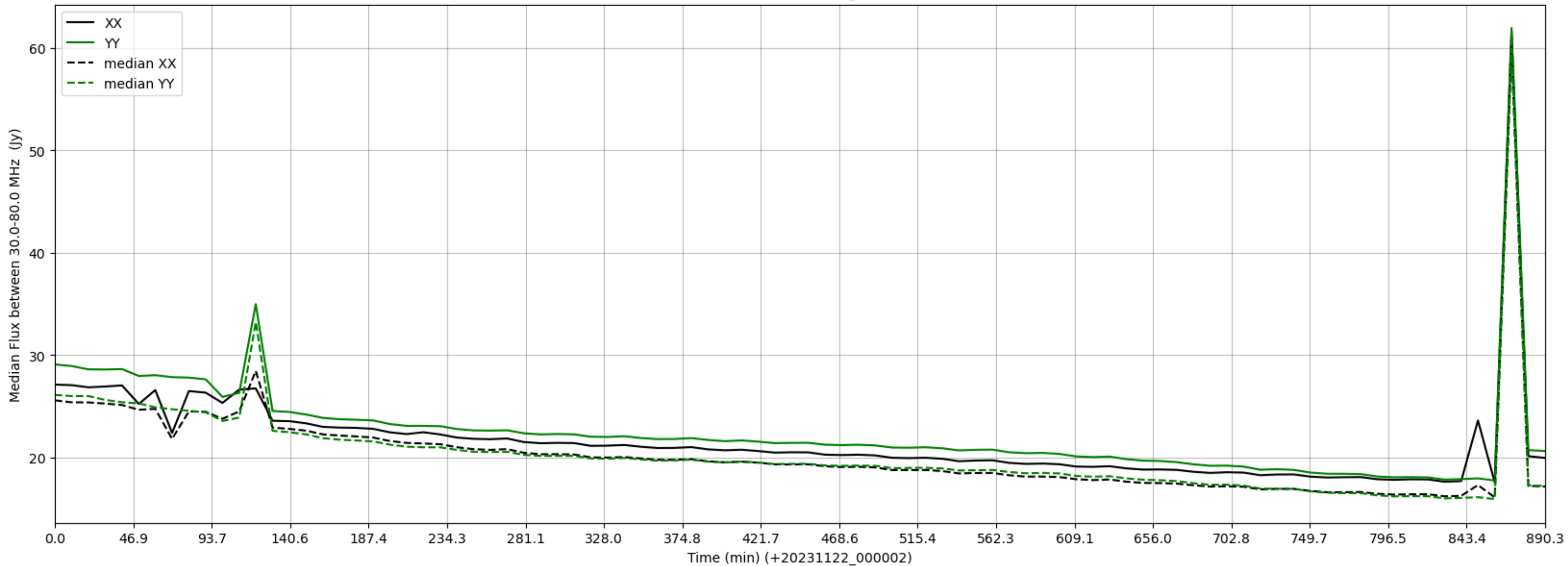
LWA129 - Correlator# 180 - XX FLAGS:HighTimeVar - YY FLAGS:Good
