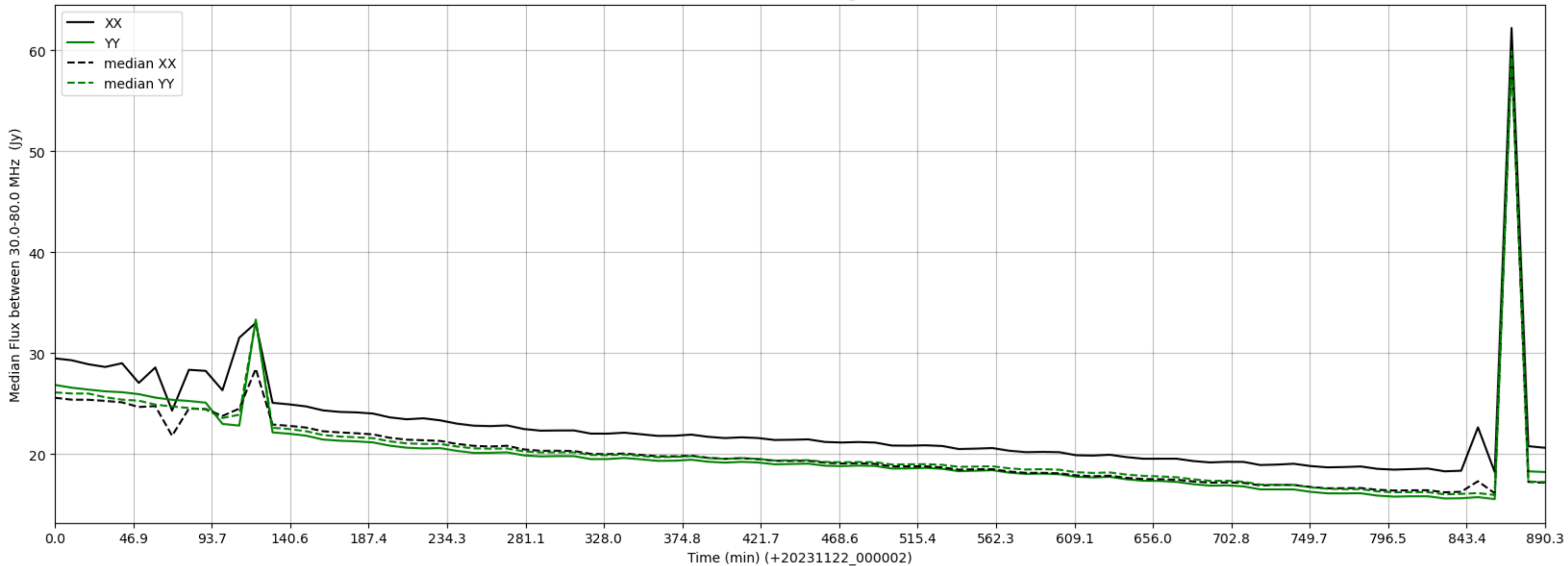
LWA133 - Correlator# 257 - XX FLAGS:HighTimeVar - YY FLAGS:Good
