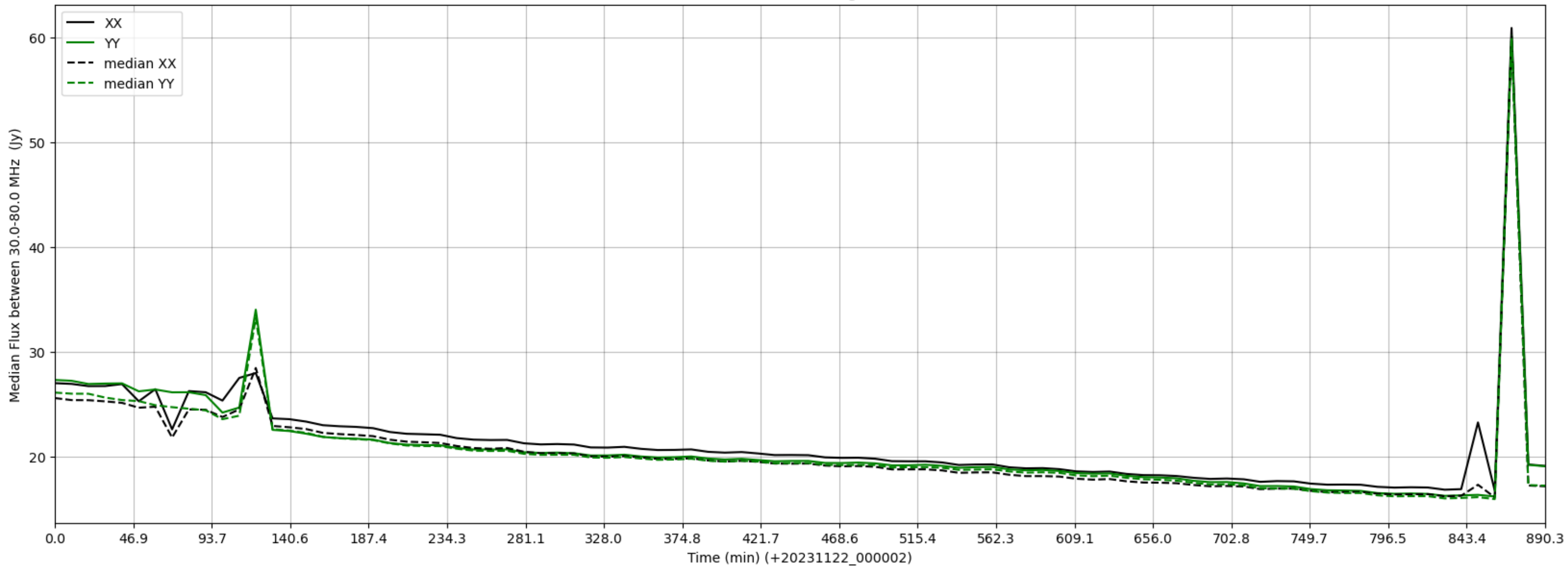
LWA130 - Correlator# 183 - XX FLAGS:HighTimeVar - YY FLAGS:Good
