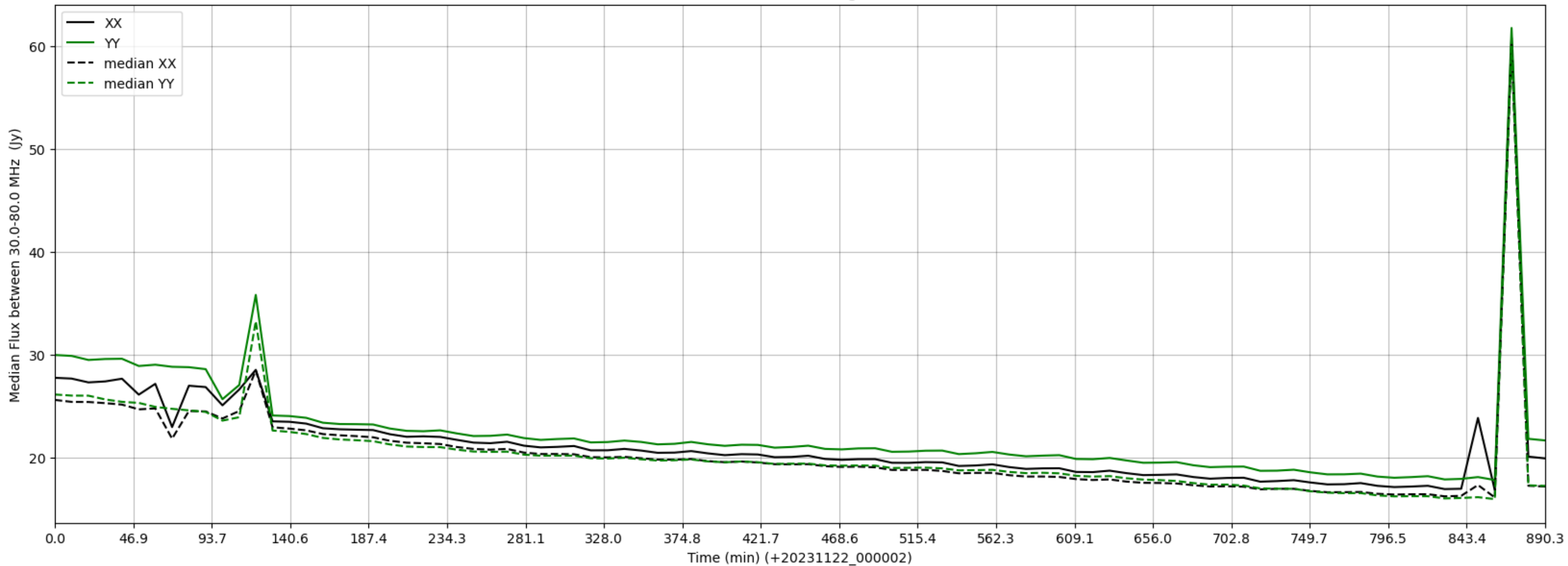
LWA161 - Correlator# 262 - XX FLAGS:HighTimeVar - YY FLAGS:Good
