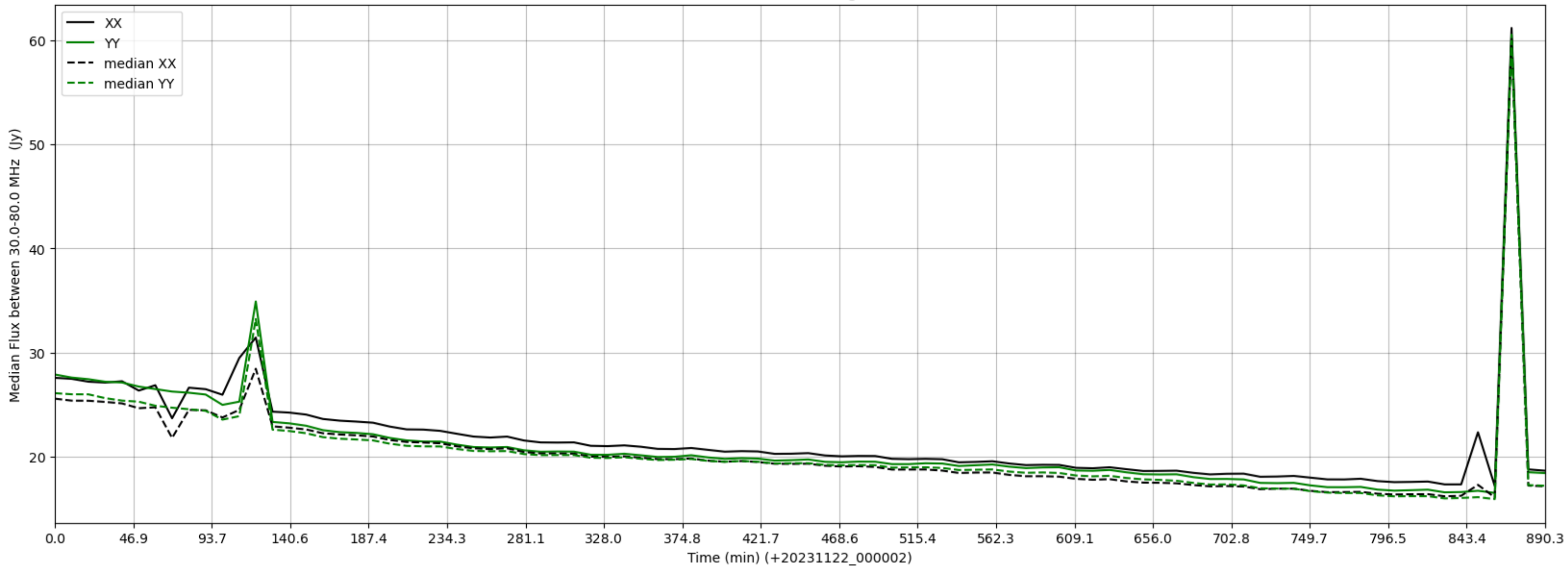
LWA070 - Correlator# 168 - XX FLAGS:HighTimeVar - YY FLAGS:Good
