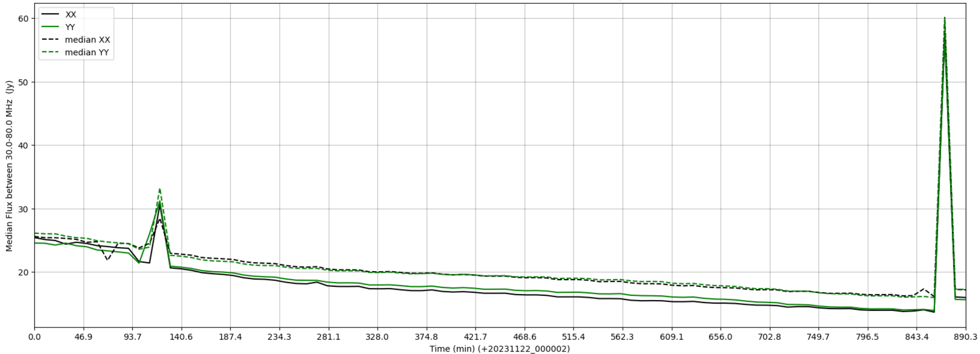
LWA320 - Correlator# 054 - XX FLAGS:Good - YY FLAGS:HighTimeVar
