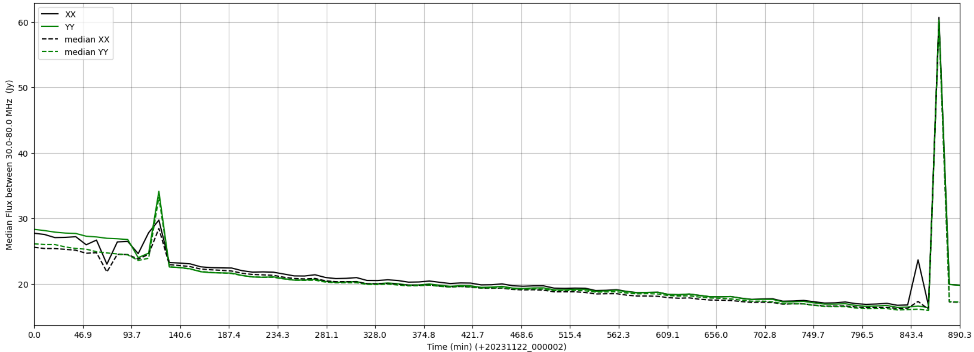
LWA193 - Correlator# 270 - XX FLAGS:HighTimeVar - YY FLAGS:Good
