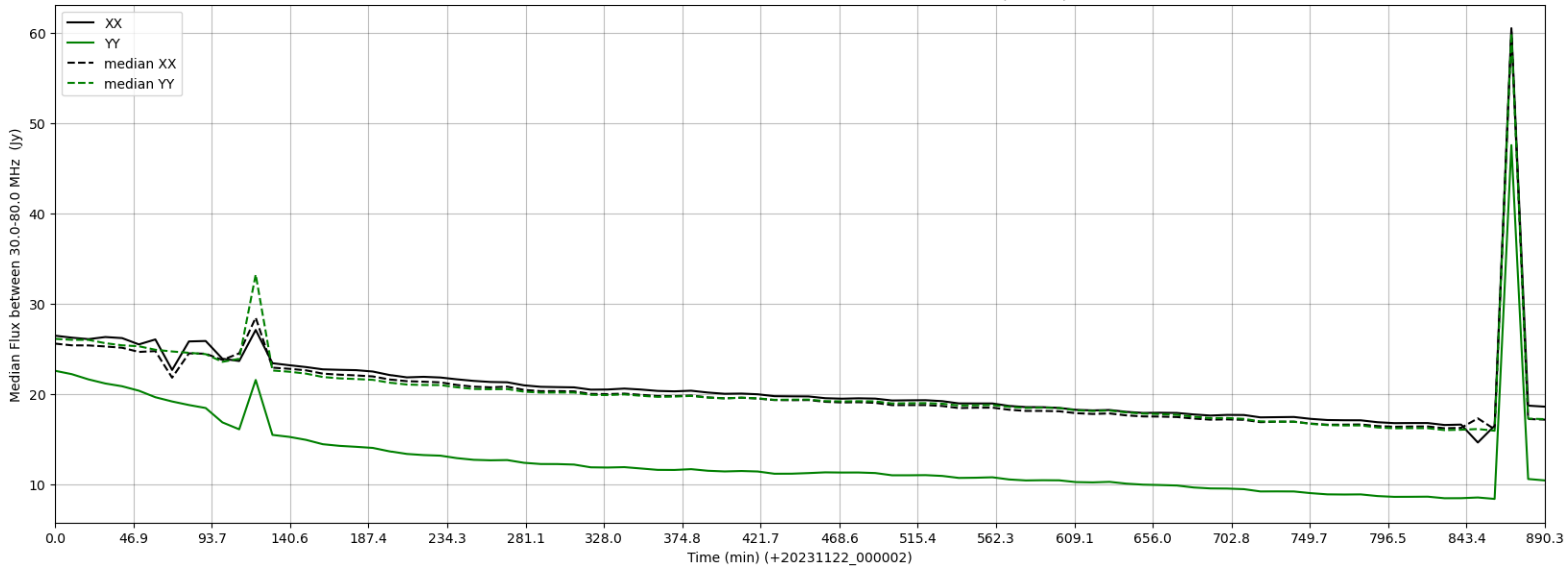
LWA358 - Correlator# 159 - XX FLAGS:Good - YY FLAGS:BadSpecShape
