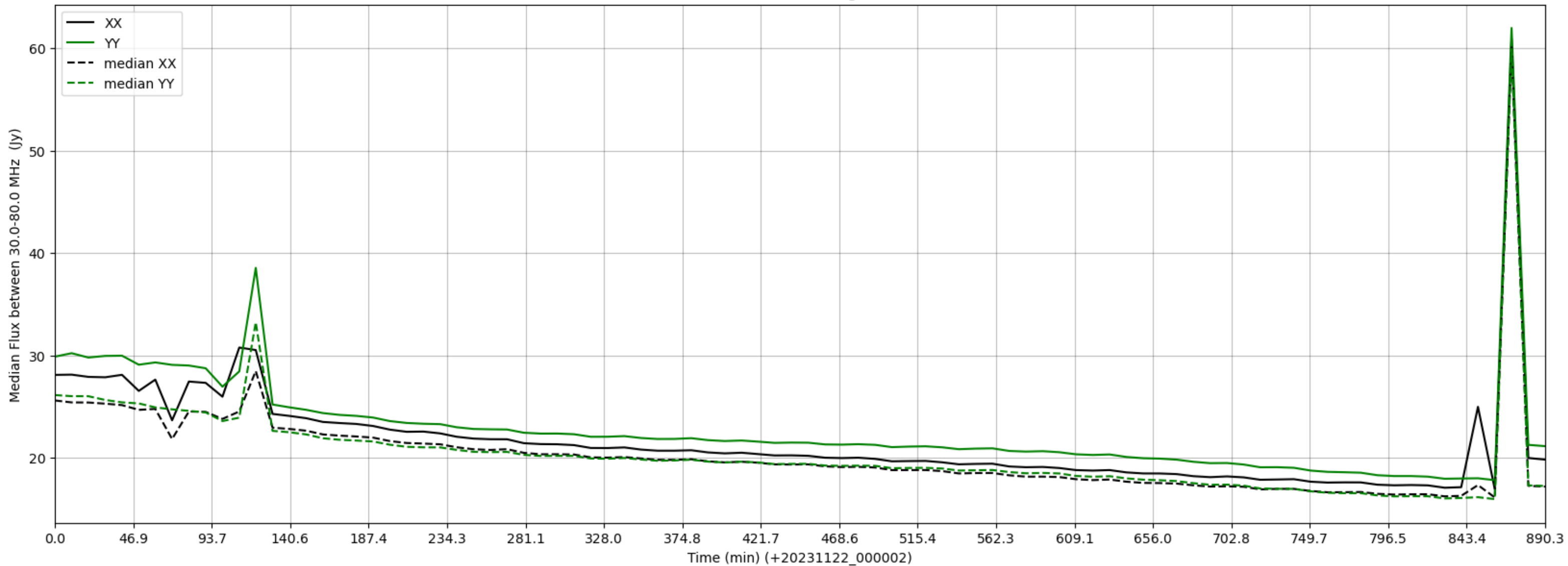
LWA033 - Correlator# 161 - XX FLAGS:HighTimeVar - YY FLAGS:Good
