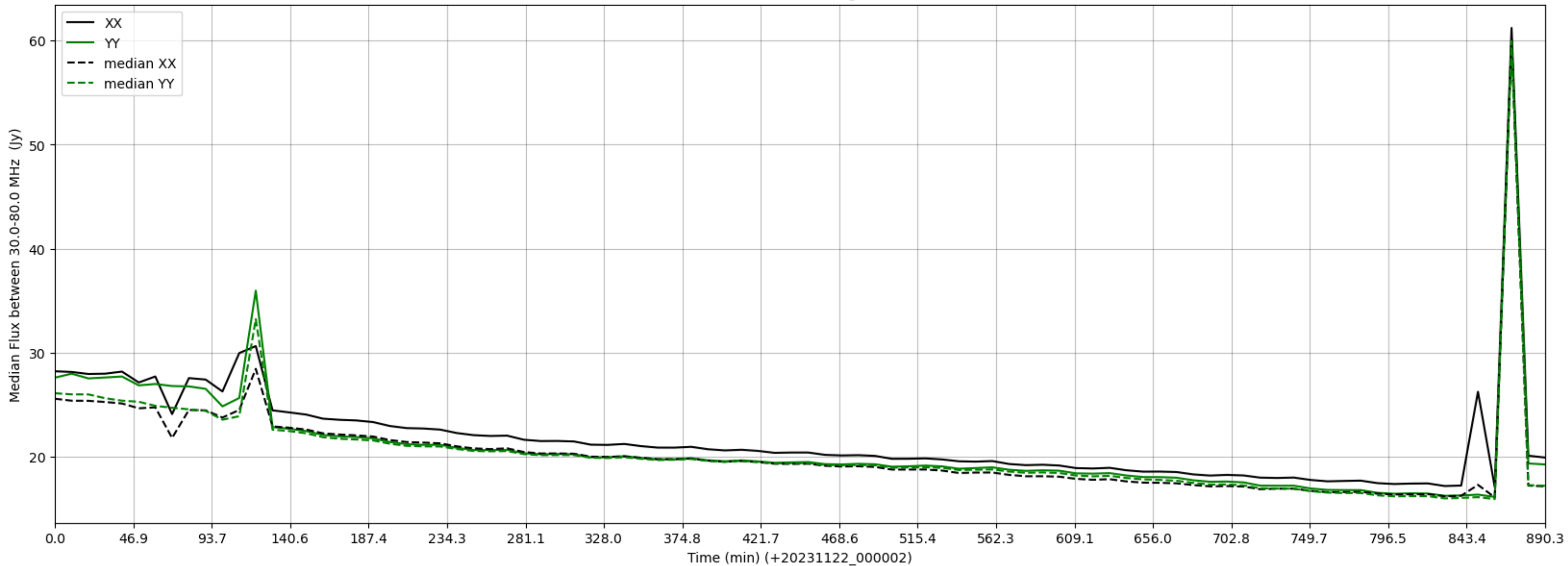
LWA002 - Correlator# 064 - XX FLAGS:HighTimeVar - YY FLAGS:Good
