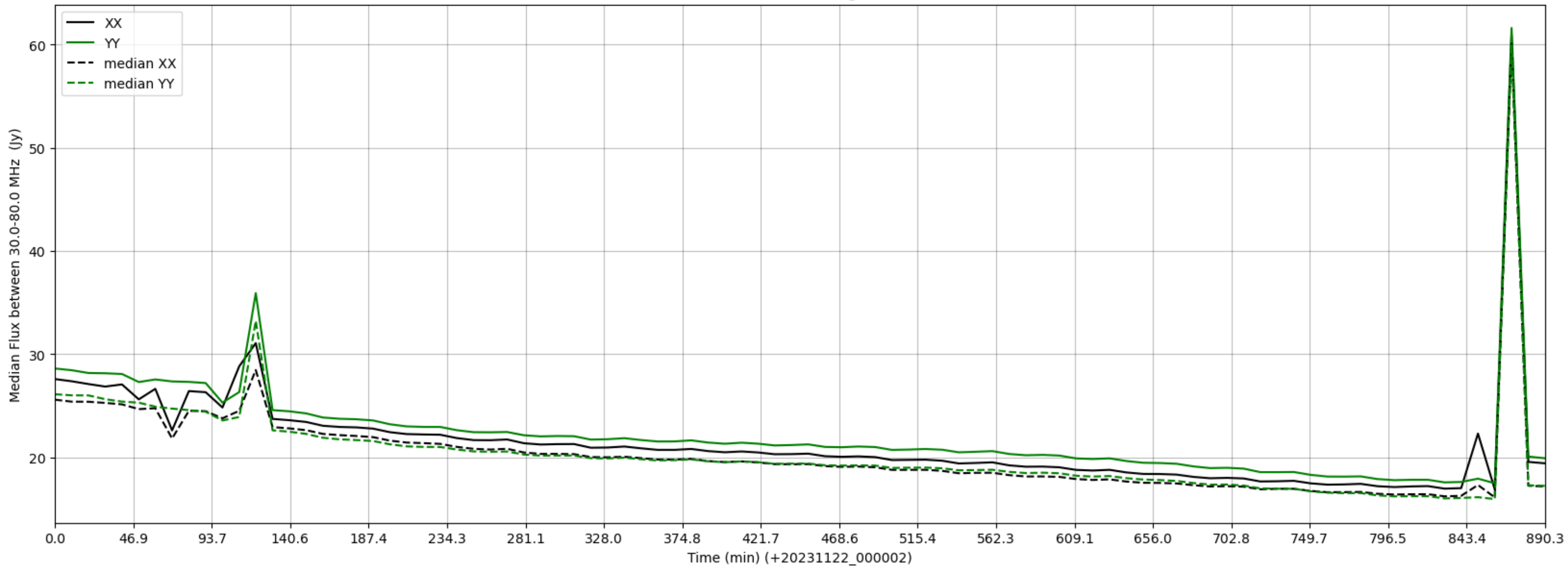
LWA199 - Correlator# 277 - XX FLAGS:HighTimeVar - YY FLAGS:Good
