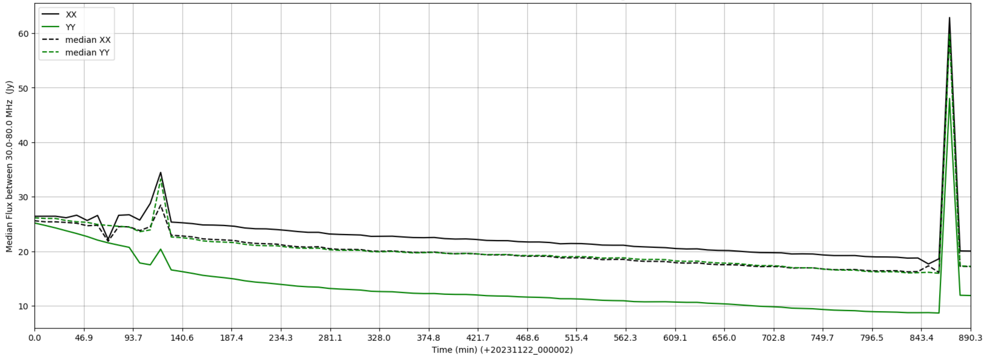
LWA290 - Correlator# 285 - XX FLAGS:Good - YY FLAGS:HighTimeVar
