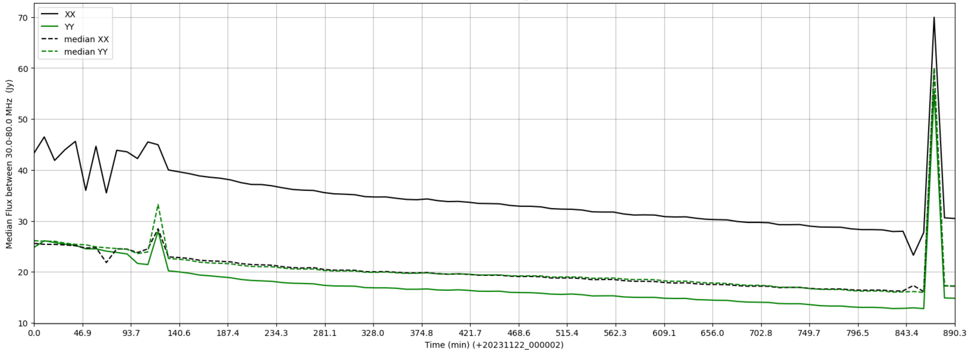
LWA362 - Correlator# 030 - XX FLAGS:HighTimeVar - YY FLAGS:Good
