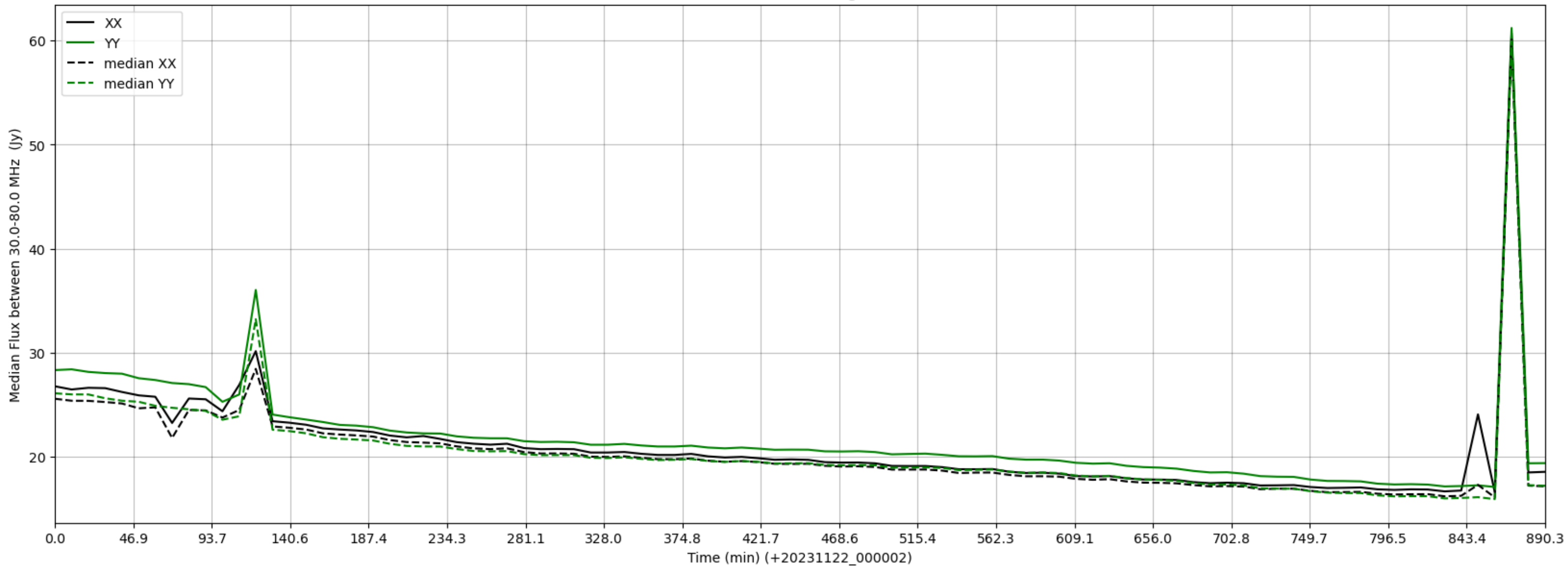
LWA006 - Correlator# 068 - XX FLAGS:HighTimeVar - YY FLAGS:Good
