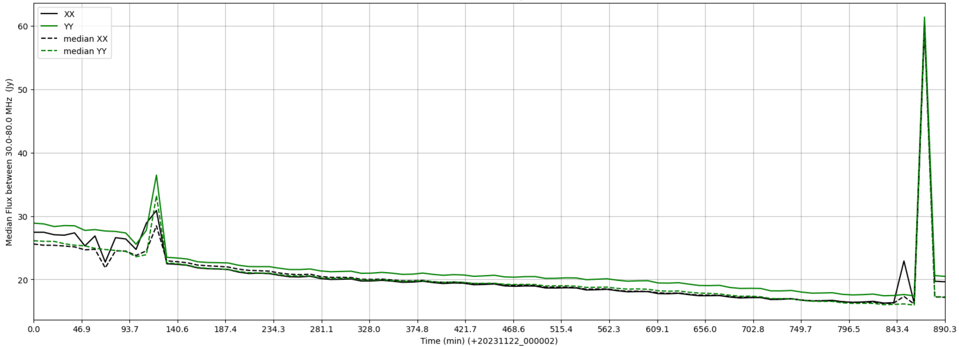
LWA225 - Correlator# 281 - XX FLAGS:HighTimeVar - YY FLAGS:Good
