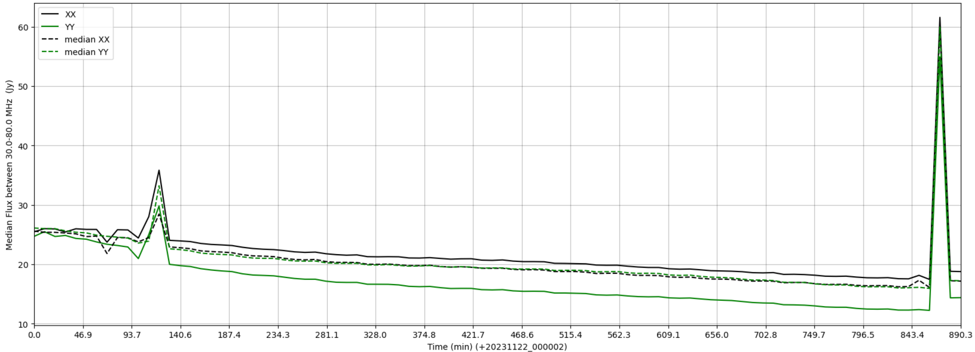
LWA348 - Correlator# 124 - XX FLAGS:Good - YY FLAGS:HighTimeVar
