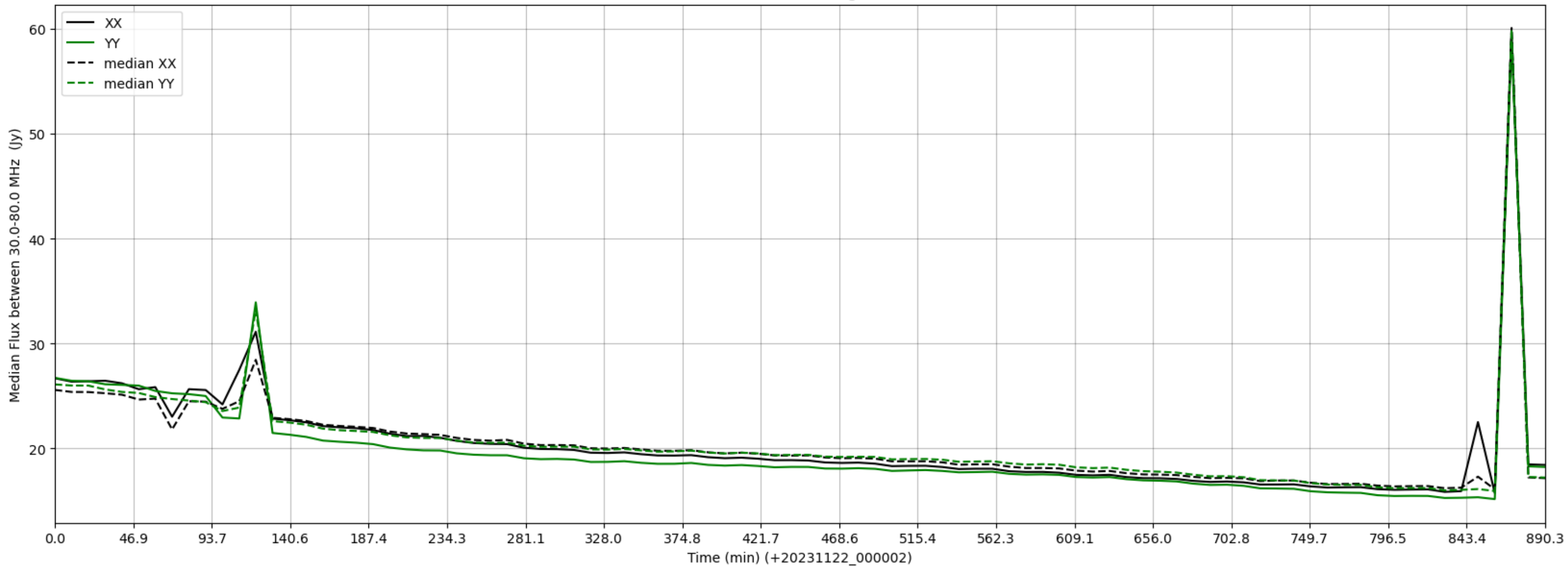
LWA005 - Correlator# 069 - XX FLAGS:HighTimeVar - YY FLAGS:Good
