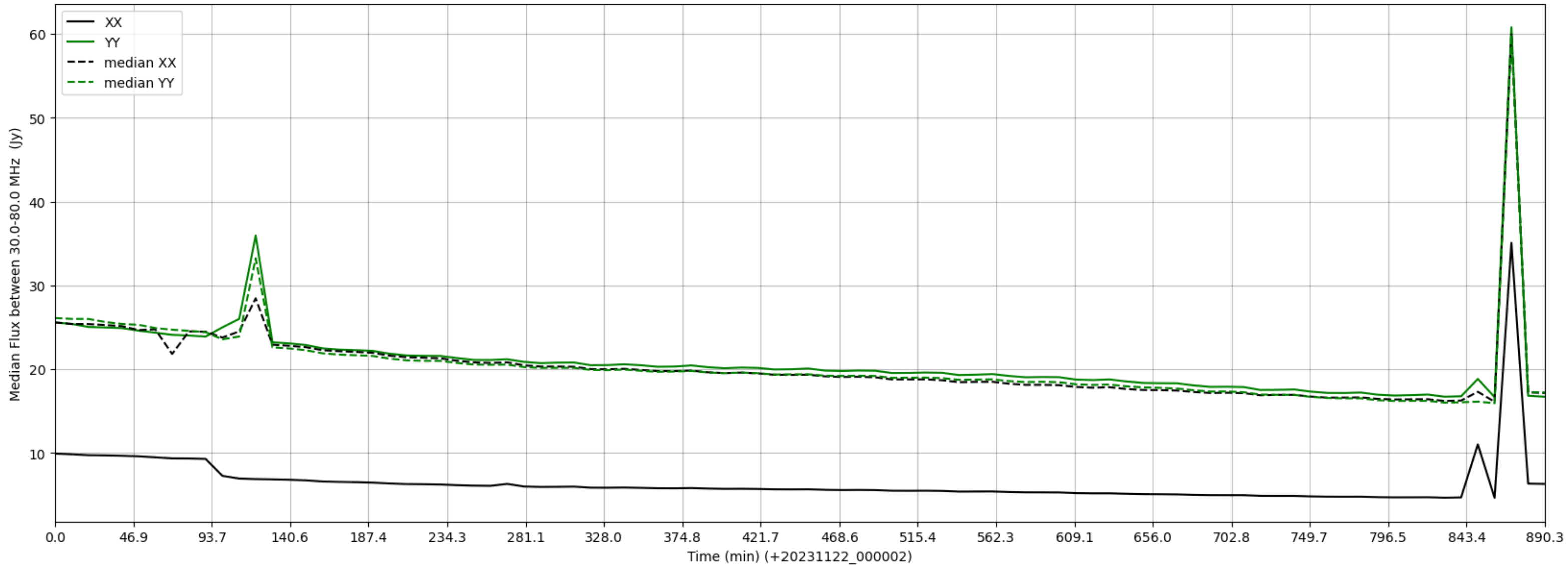
LWA232 - Correlator# 307 - XX FLAGS:HighTimeVar+BadSpecShape - YY FLAGS:BadSpecShape
