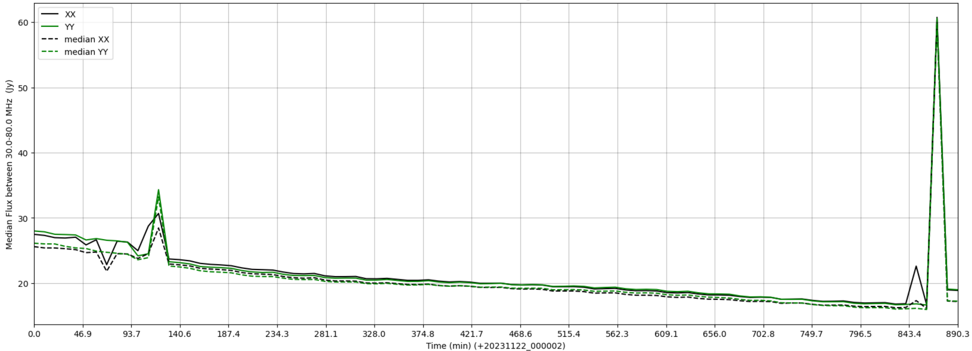
LWA164 - Correlator# 267 - XX FLAGS:HighTimeVar - YY FLAGS:Good
