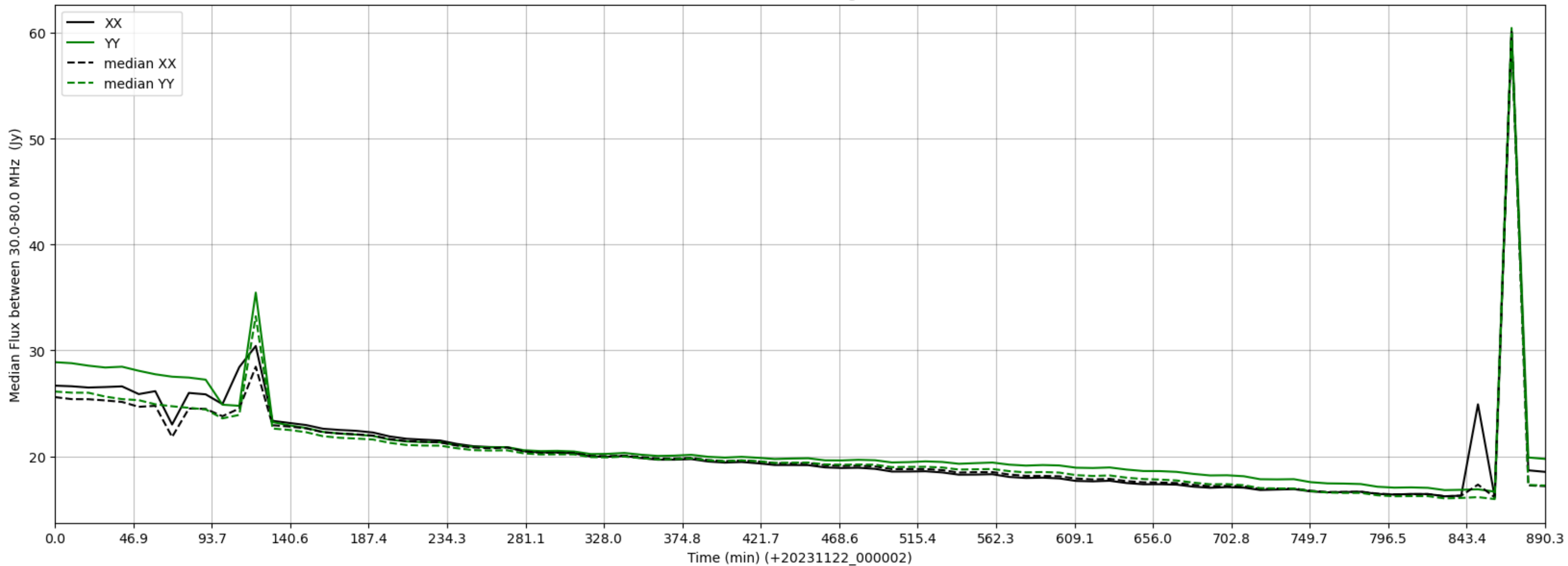
LWA003 - Correlator# 067 - XX FLAGS:HighTimeVar - YY FLAGS:Good
