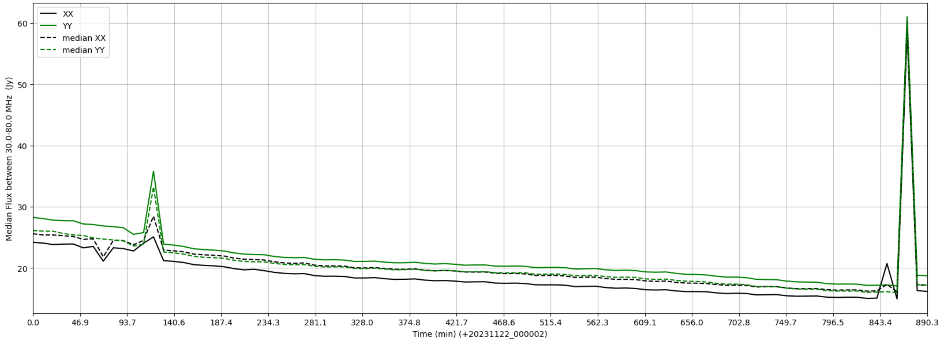
LWA100 - Correlator# 175 - XX FLAGS:HighTimeVar - YY FLAGS:Good
