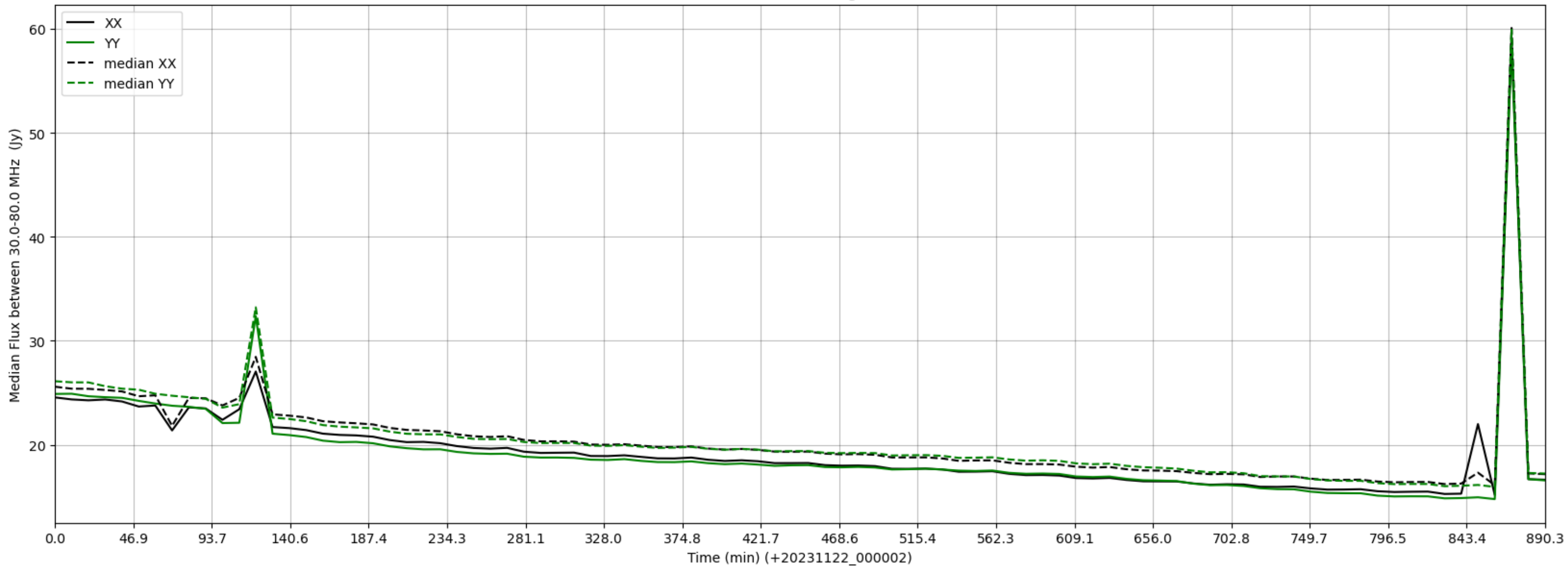
LWA010 - Correlator# 073 - XX FLAGS:HighTimeVar - YY FLAGS:Good
