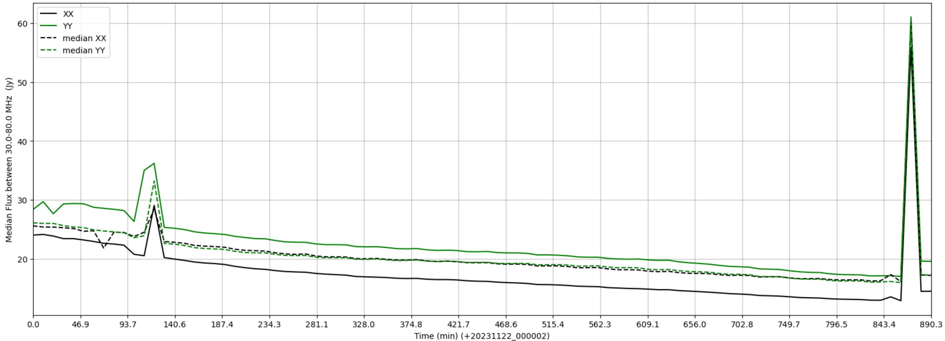
LWA291 - Correlator# 045 - XX FLAGS:Good - YY FLAGS:HighTimeVar
