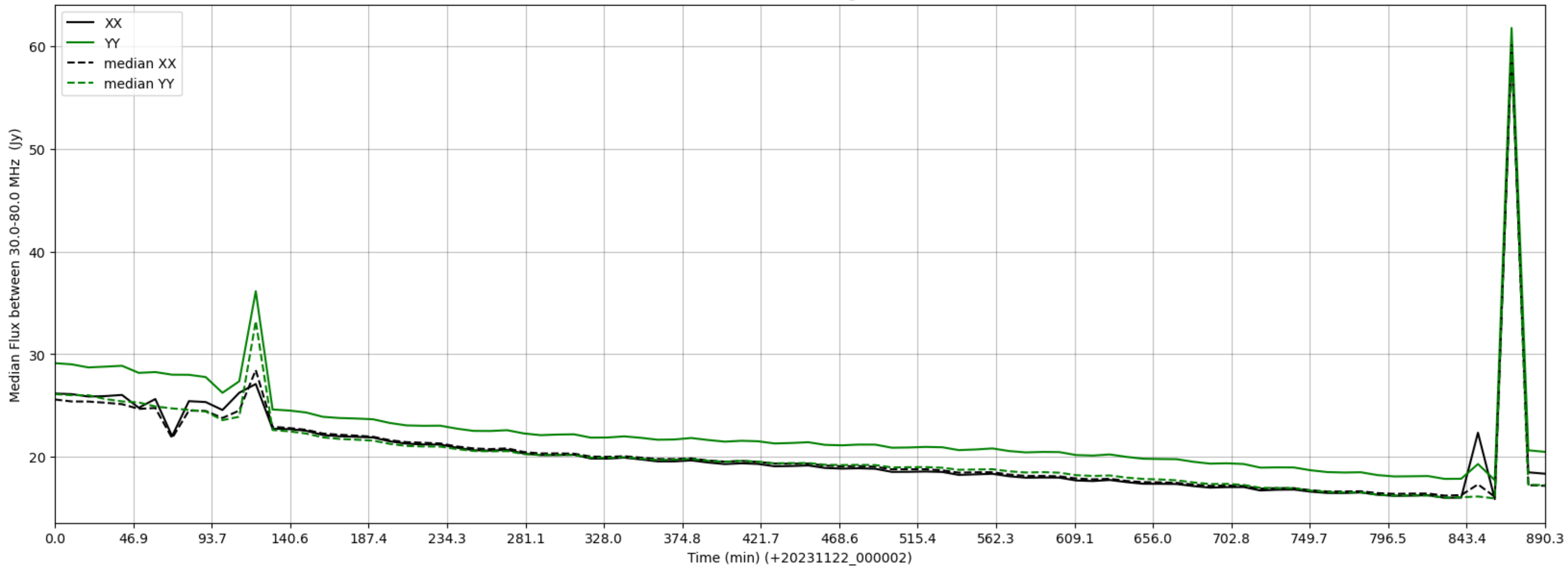
LWA194 - Correlator# 273 - XX FLAGS:HighTimeVar - YY FLAGS:Good
