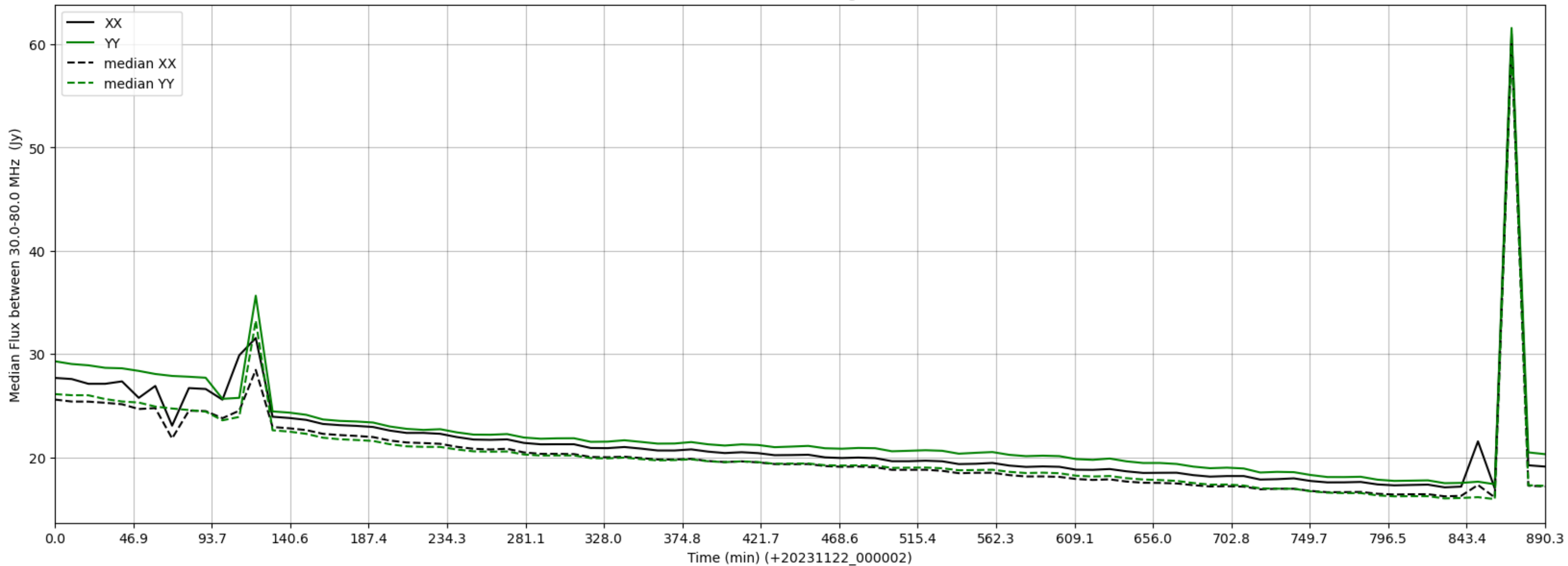
LWA163 - Correlator# 264 - XX FLAGS:HighTimeVar - YY FLAGS:Good
