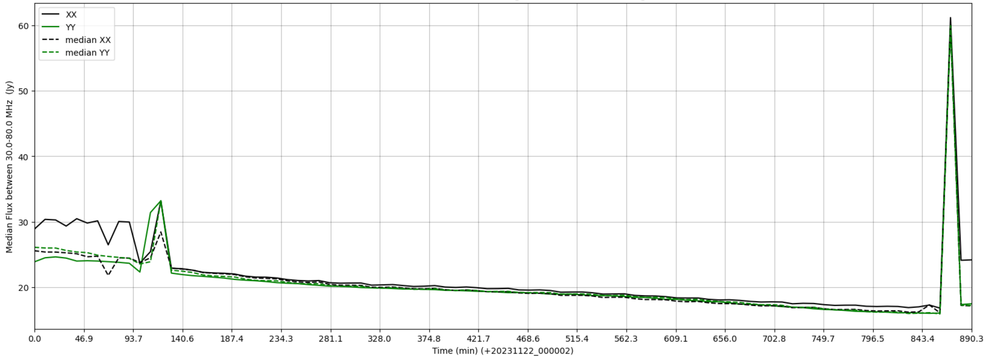
LWA315 - Correlator# 350 - XX FLAGS:HighTimeVar - YY FLAGS:HighTimeVar
