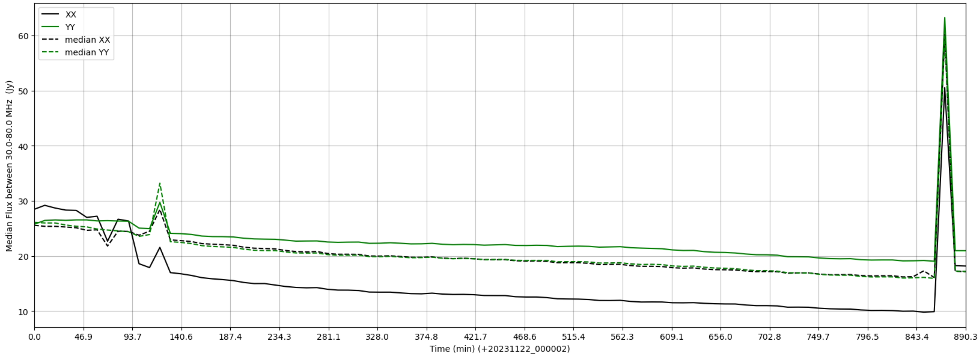
LWA317 - Correlator# 052 - XX FLAGS:HighTimeVar - YY FLAGS:Good
