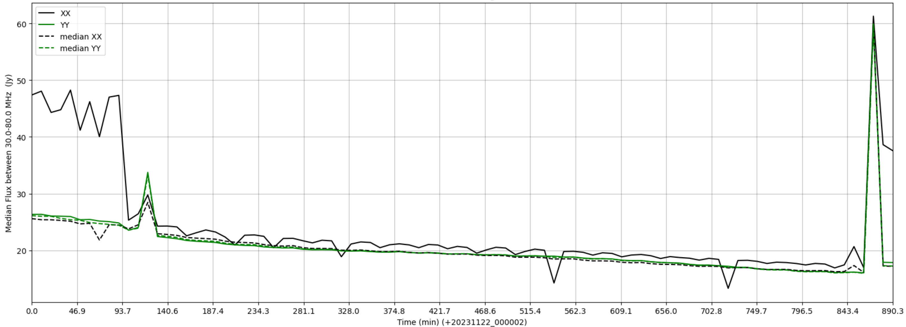
LWA041 - Correlator# 079 - XX FLAGS:HighTimeVar - YY FLAGS:Good
