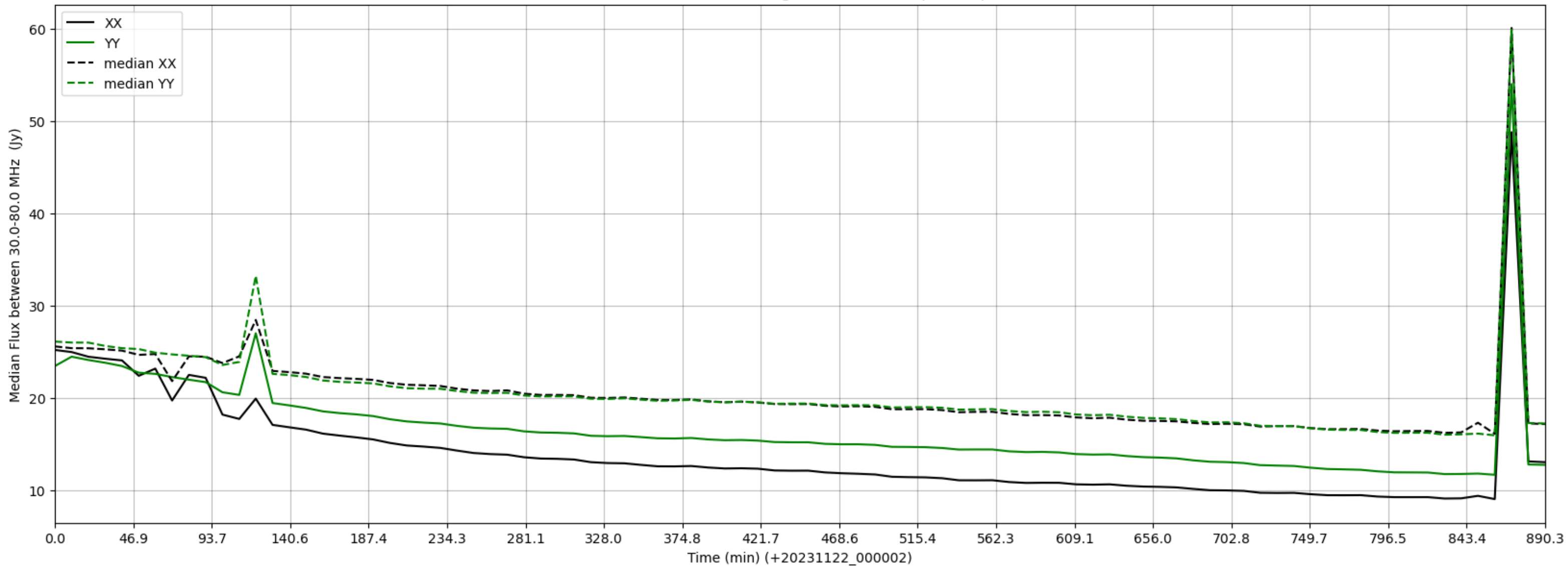
LWA363 - Correlator# 094 - XX FLAGS:HighTimeVar+BadSpecShape - YY FLAGS:Good
