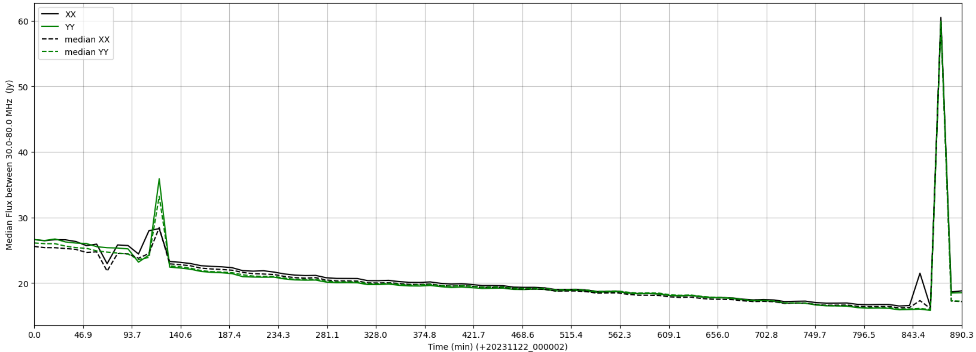
LWA004 - Correlator# 066 - XX FLAGS:HighTimeVar - YY FLAGS:Good
