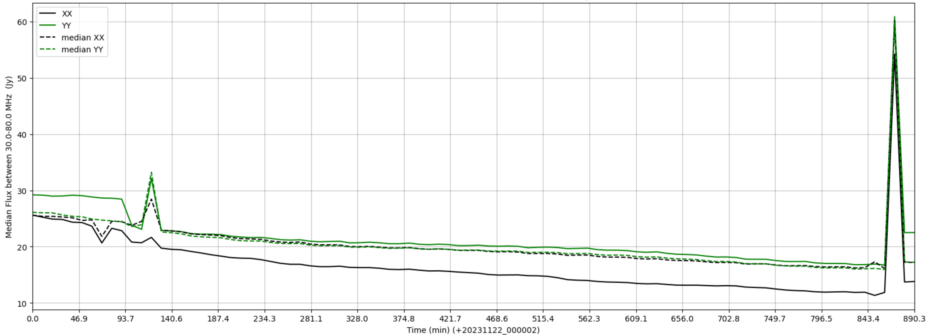
LWA328 - Correlator# 157 - XX FLAGS:Good - YY FLAGS:HighTimeVar
