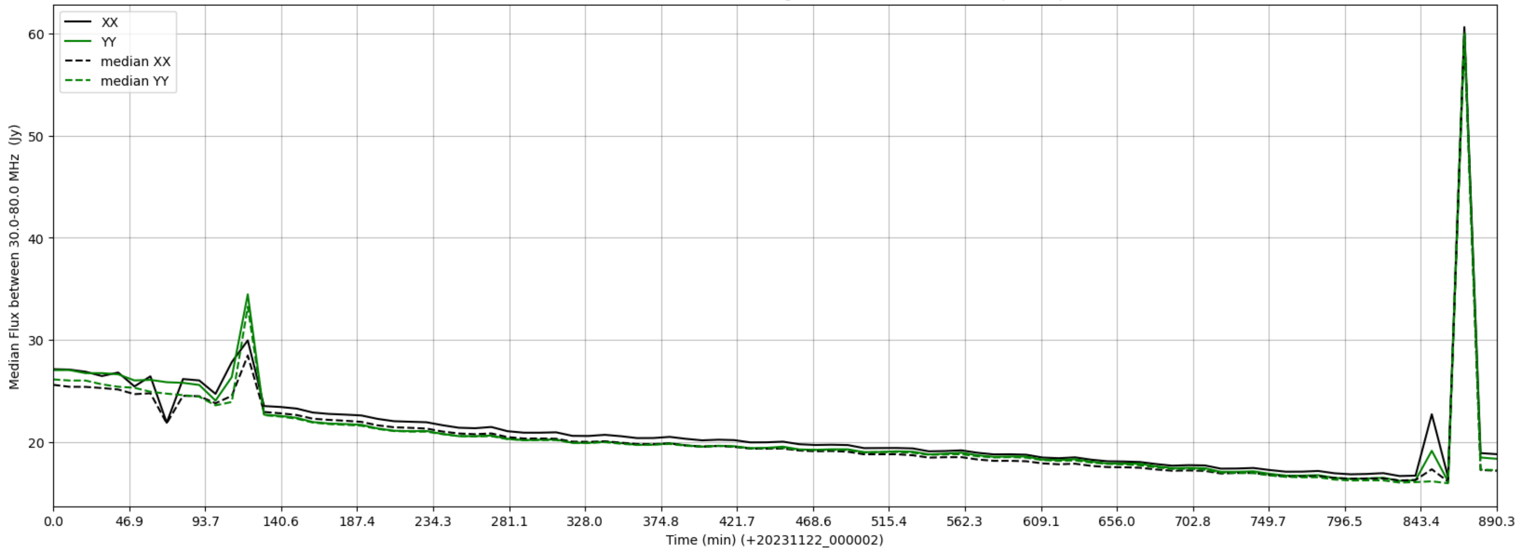
LWA230 - Correlator# 303 - XX FLAGS:HighTimeVar - YY FLAGS:BadSpecShape
