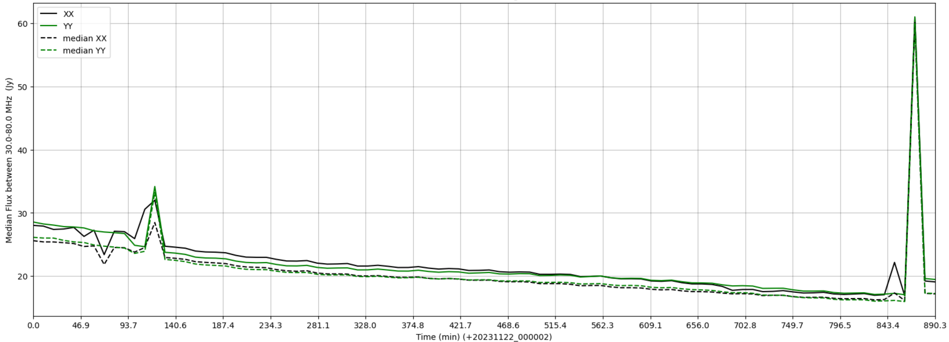
LWA162 - Correlator# 265 - XX FLAGS:HighTimeVar - YY FLAGS:Good
