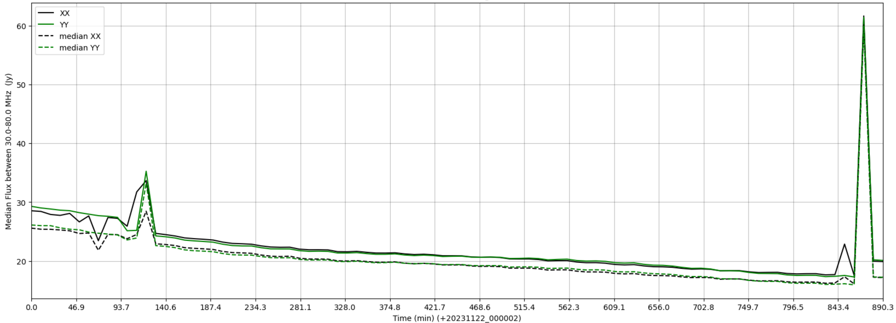
LWA132 - Correlator# 185 - XX FLAGS:HighTimeVar - YY FLAGS:Good
