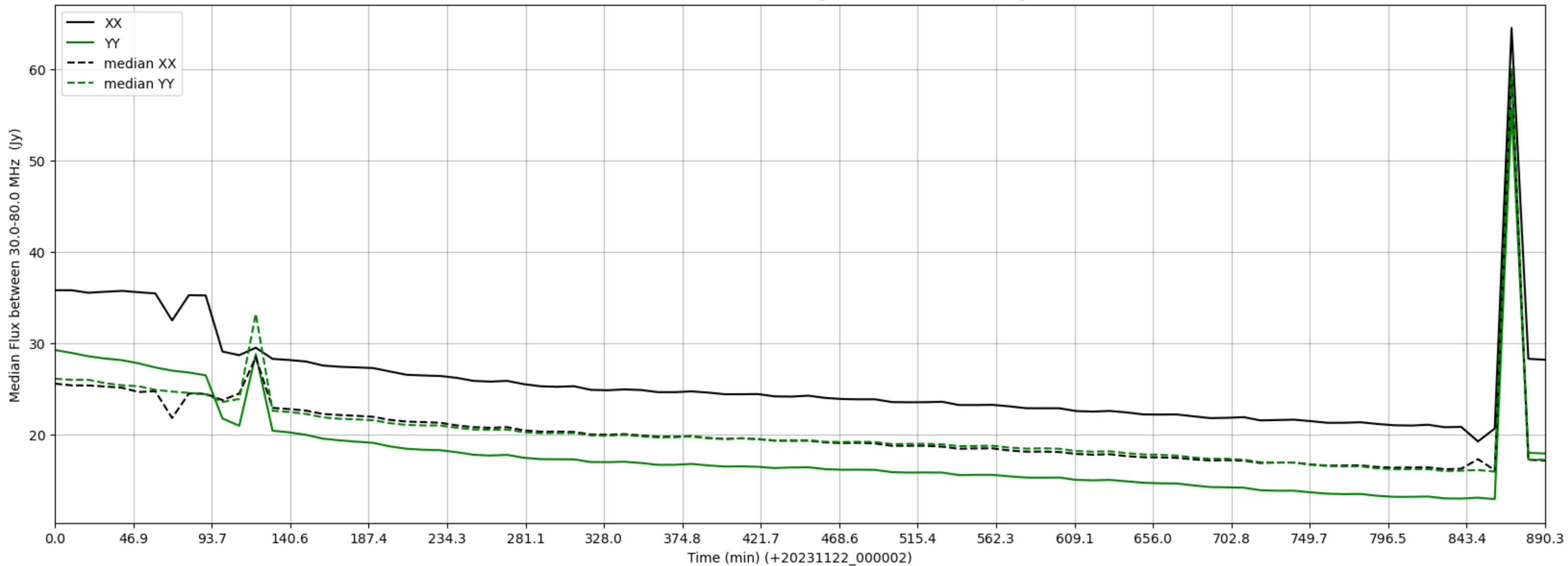
LWA277 - Correlator# 009 - XX FLAGS:HighTimeVar - YY FLAGS:HighTimeVar
