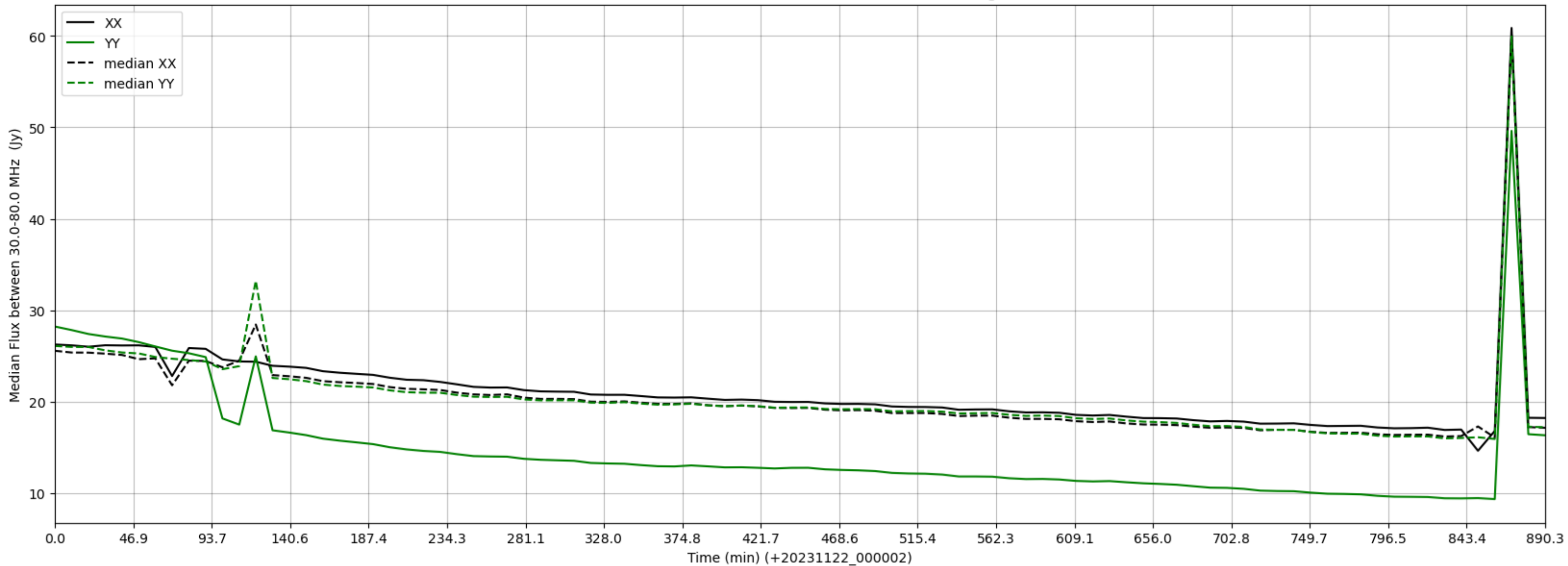
LWA326 - Correlator# 250 - XX FLAGS:Good - YY FLAGS:HighTimeVar
