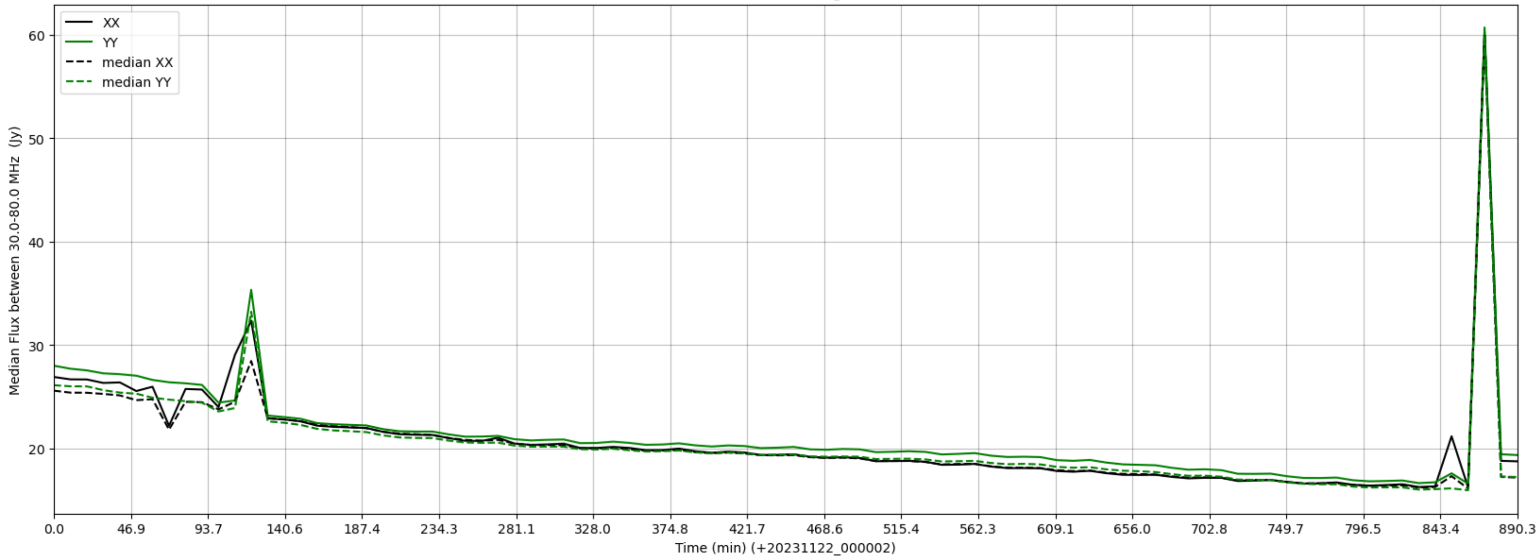
LWA227 - Correlator# 280 - XX FLAGS:HighTimeVar - YY FLAGS:Good
