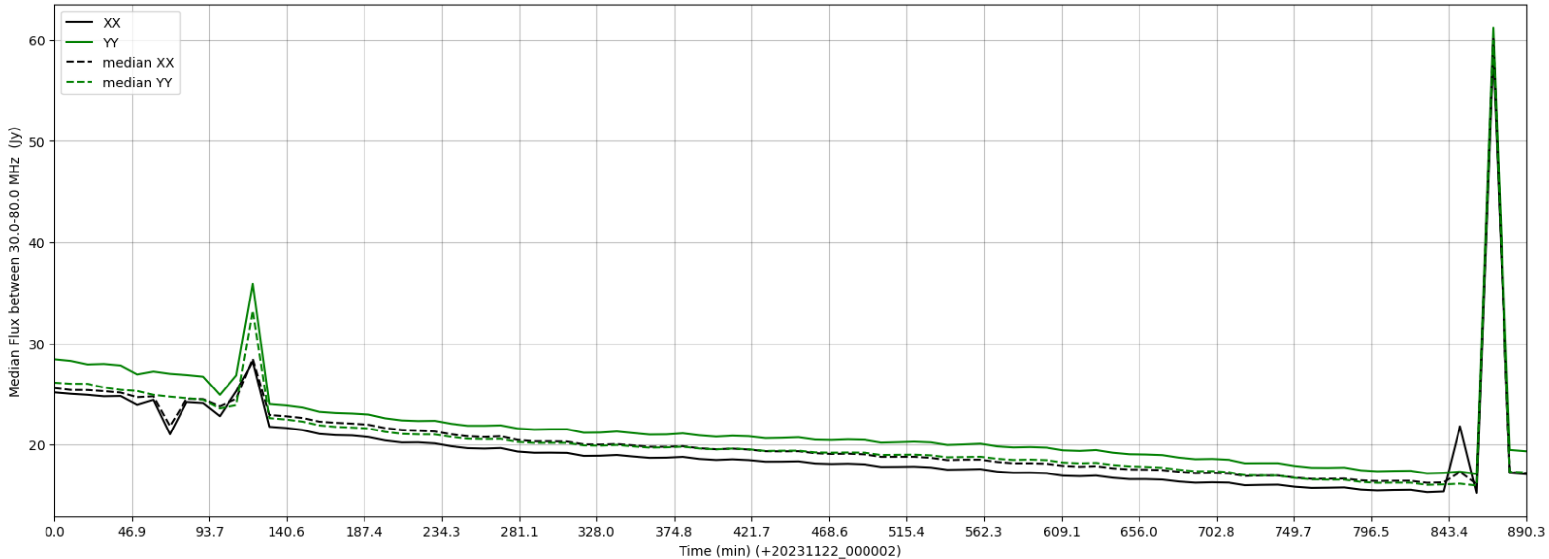
LWA200 - Correlator# 276 - XX FLAGS:HighTimeVar - YY FLAGS:Good
