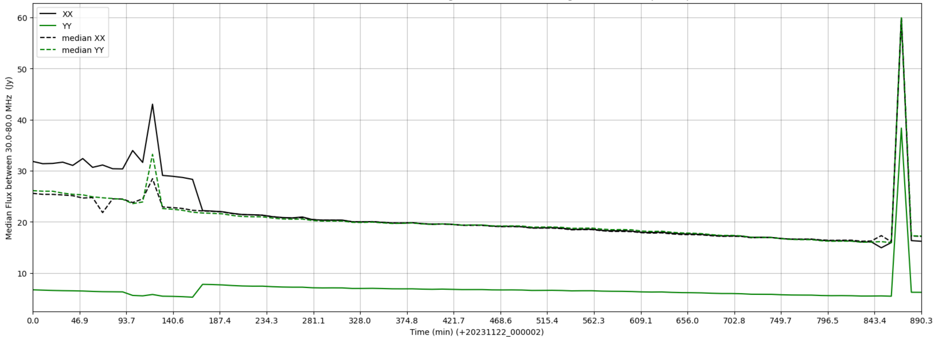
LWA058 - Correlator# 137 - XX FLAGS:HighTimeVar - YY FLAGS:HighTimeVar+BadSpecShape
