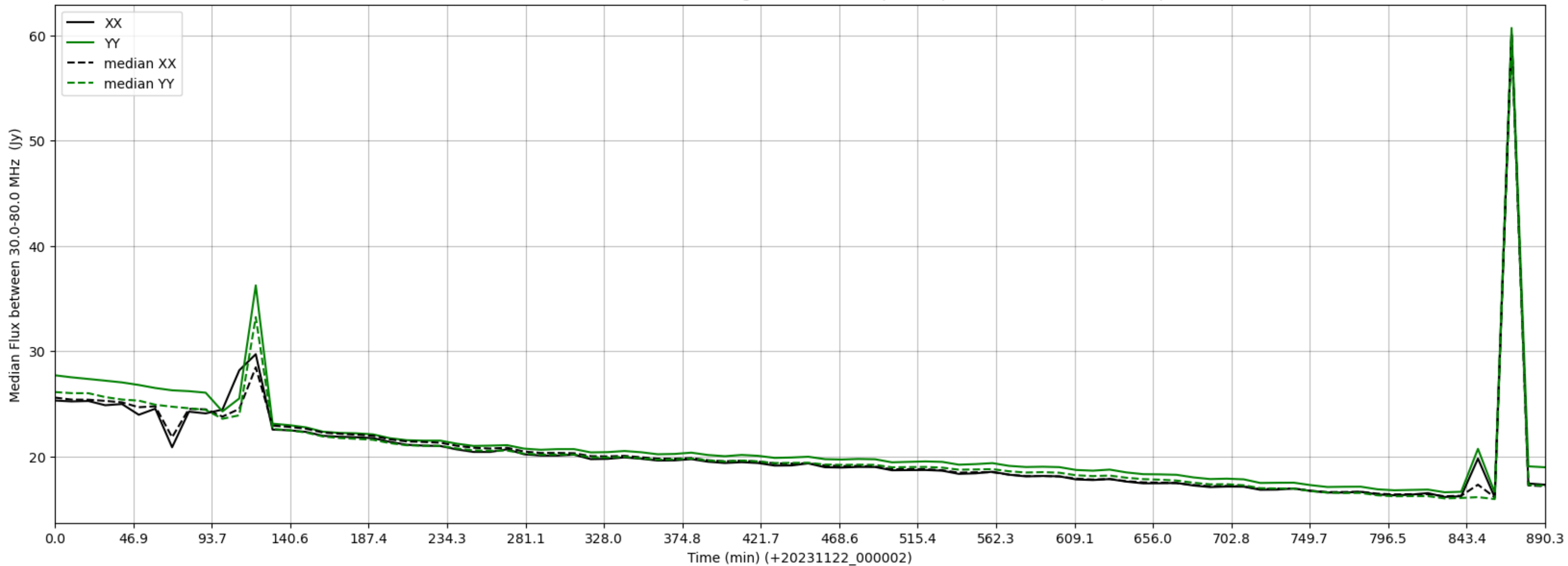
LWA226 - Correlator# 304 - XX FLAGS:HighTimeVar+BadSpecShape - YY FLAGS:BadSpecShape
