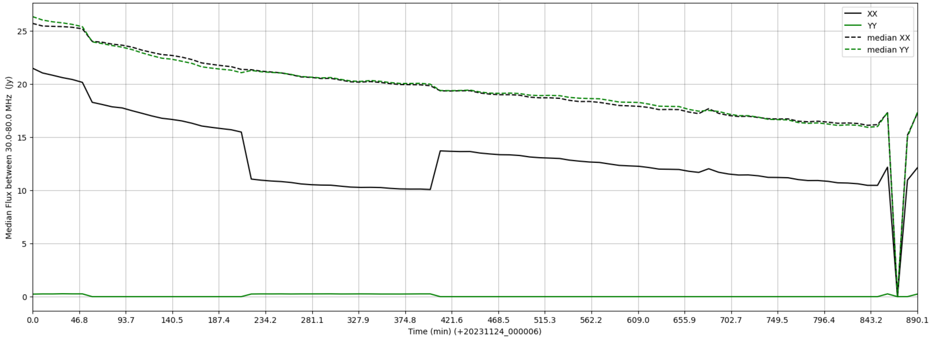
LWA292 - Correlator# 044 - XX FLAGS:HighTimeVar - YY FLAGS:LowFlux
