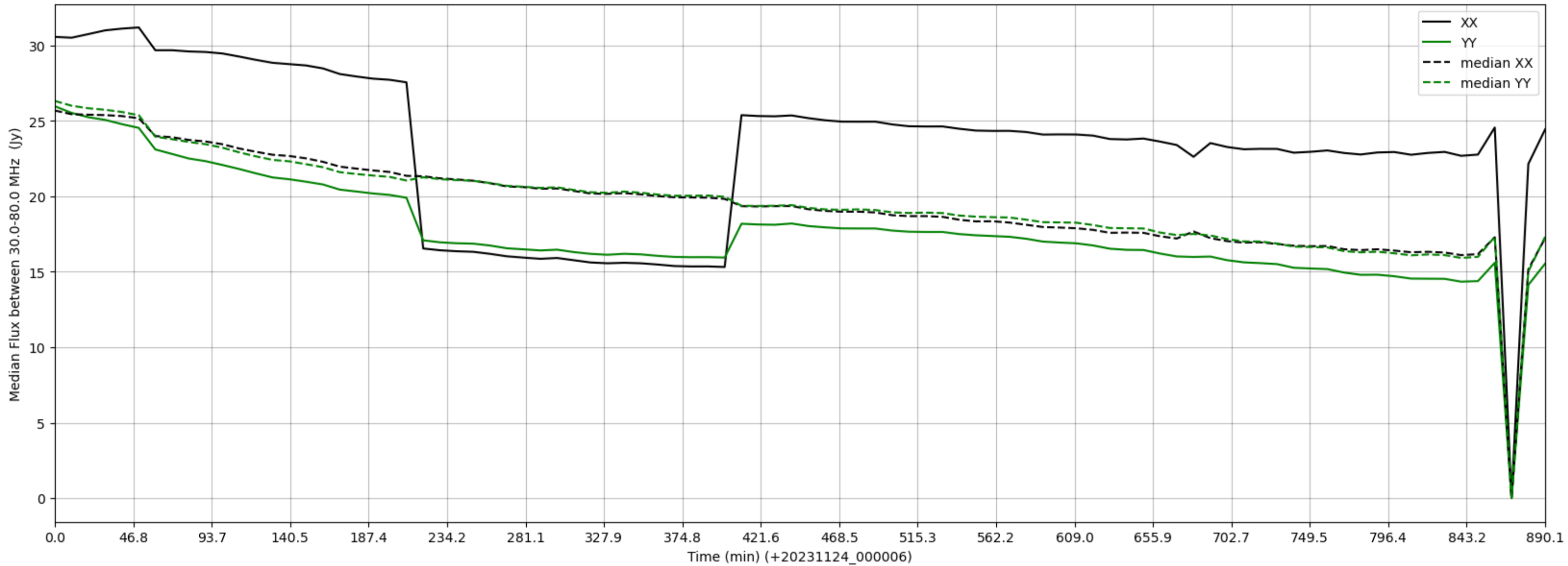
LWA301 - Correlator# 048 - XX FLAGS:HighTimeVar - YY FLAGS:BadSpecShape
