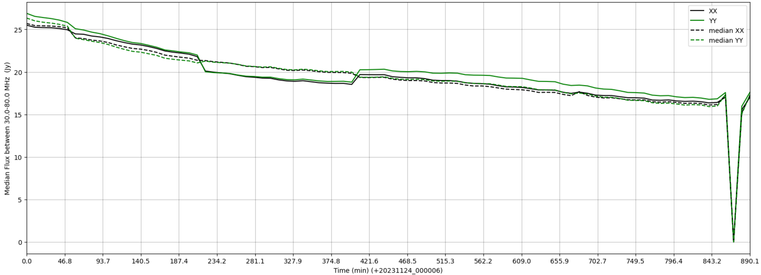
LWA054 - Correlator# 118 - XX FLAGS:BadSpecShape - YY FLAGS:BadSpecShape
