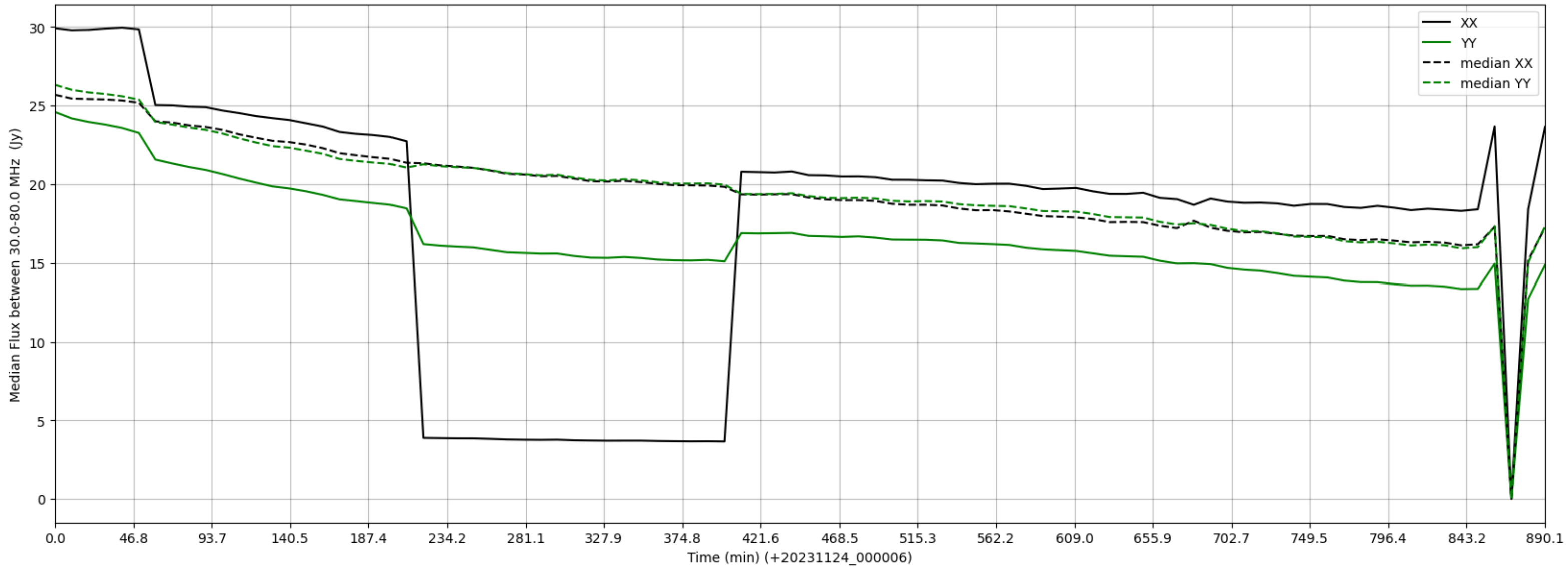
LWA318 - Correlator# 055 - XX FLAGS:HighTimeVar - YY FLAGS:BadSpecShape
