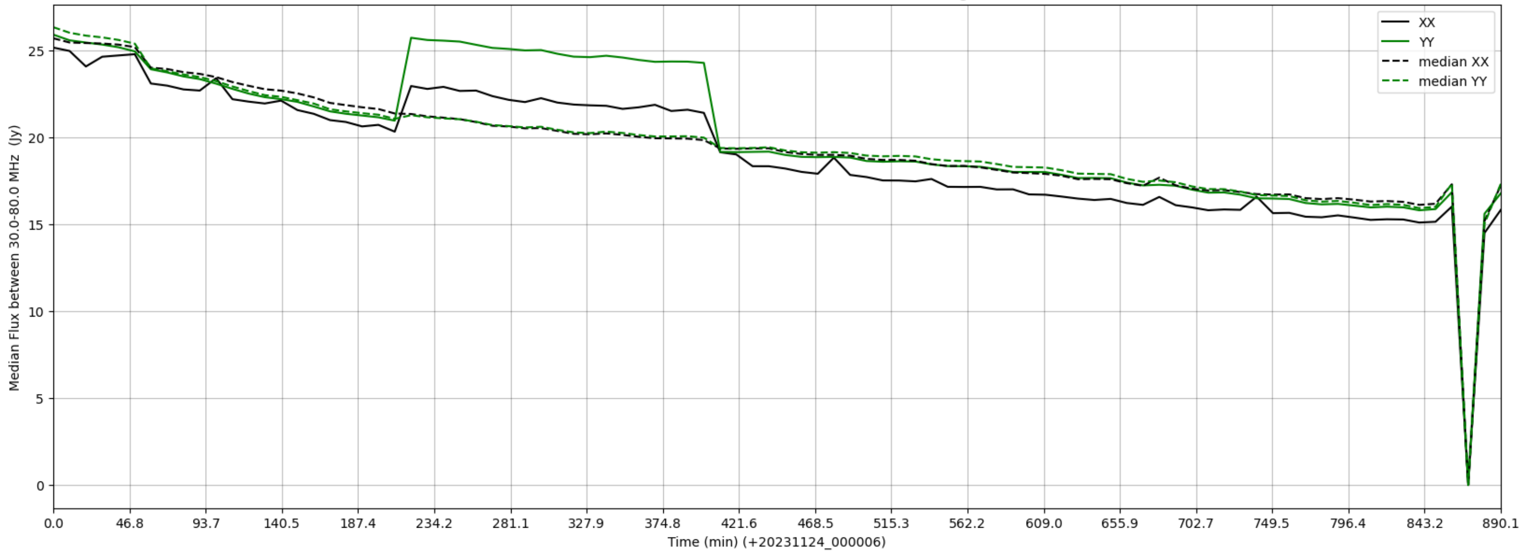
LWA215 - Correlator# 331 - XX FLAGS:Good - YY FLAGS:HighTimeVar
