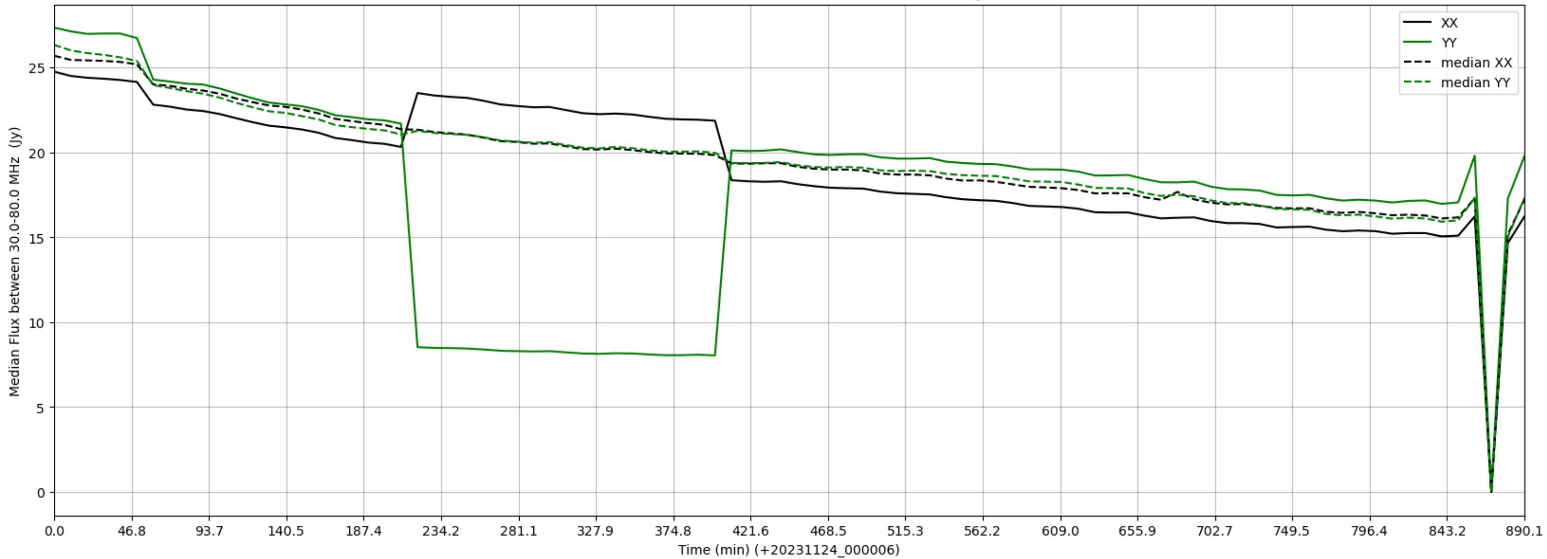
LWA257 - Correlator# 032 - XX FLAGS:Good - YY FLAGS:HighTimeVar
