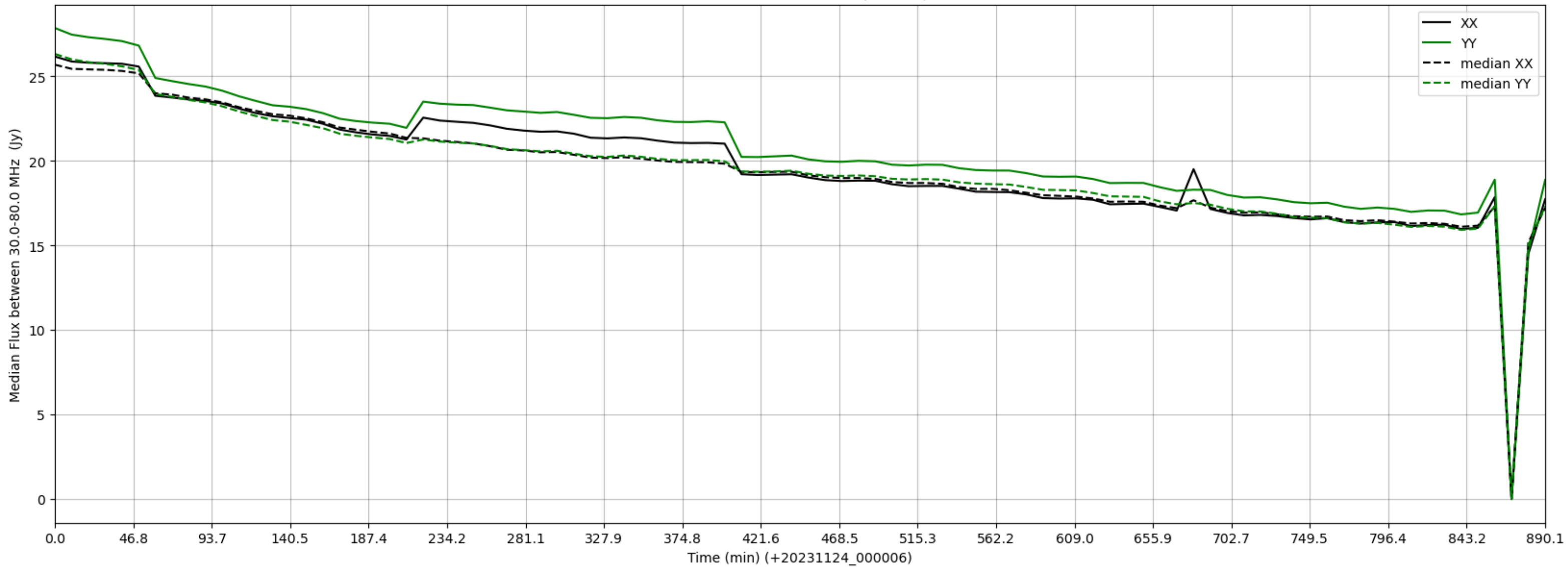
LWA134 - Correlator# 184 - XX FLAGS:BadSpecShape - YY FLAGS:Good
