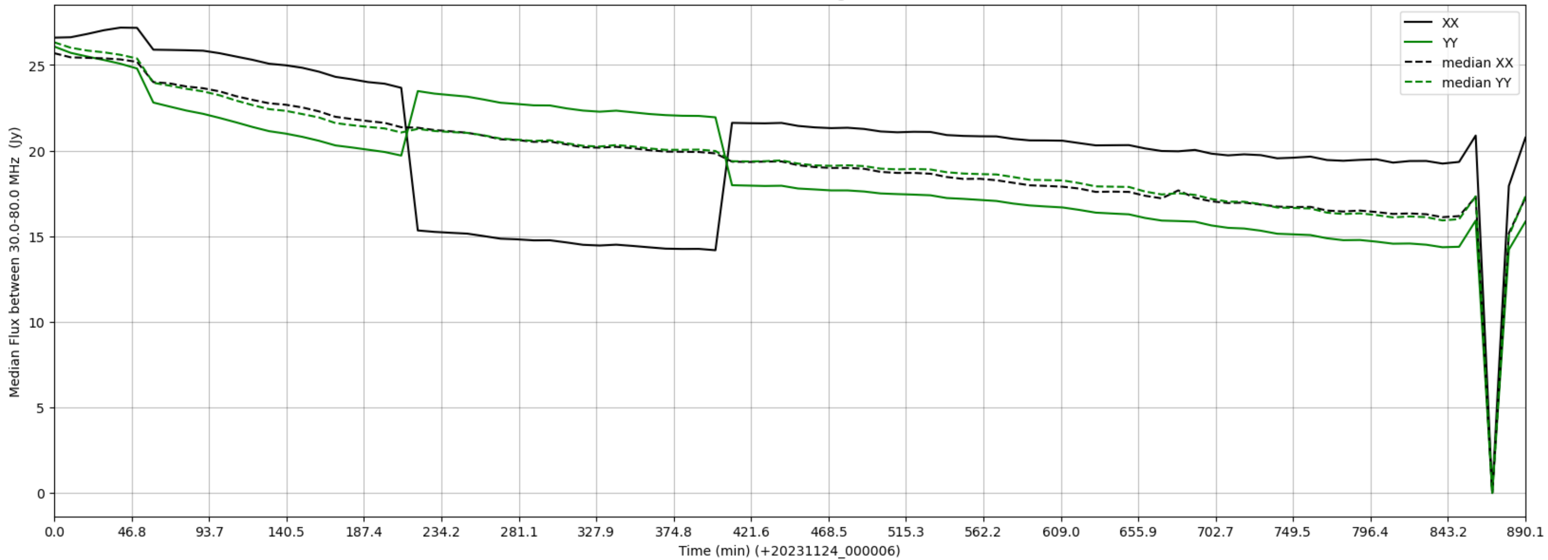
LWA306 - Correlator# 053 - XX FLAGS:HighTimeVar - YY FLAGS:Good
