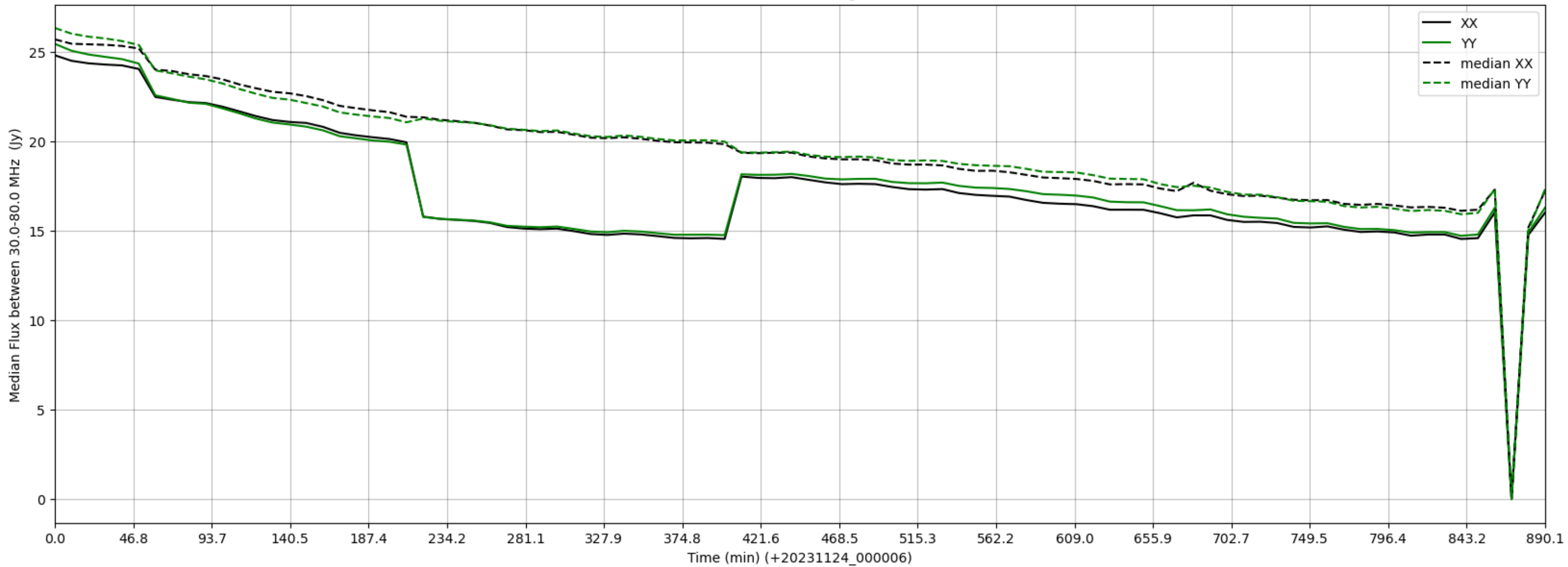
LWA336 - Correlator# 056 - XX FLAGS:HighTimeVar - YY FLAGS:Good
