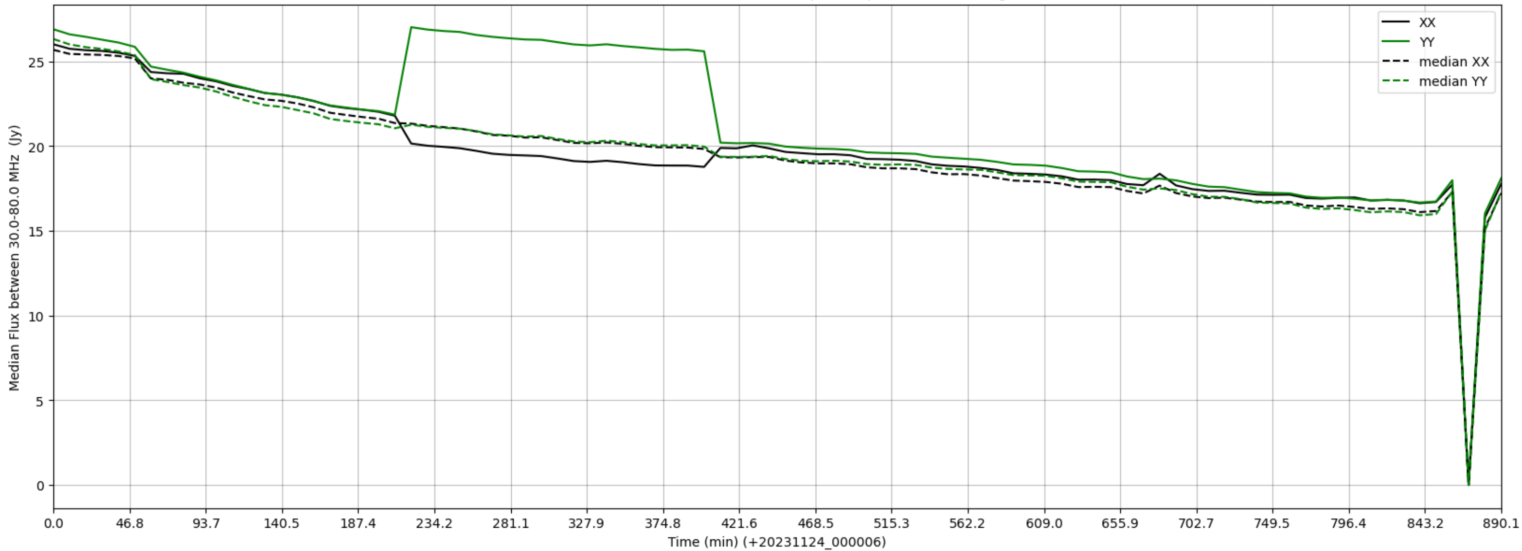
LWA142 - Correlator# 211 - XX FLAGS:BadSpecShape - YY FLAGS:HighTimeVar
