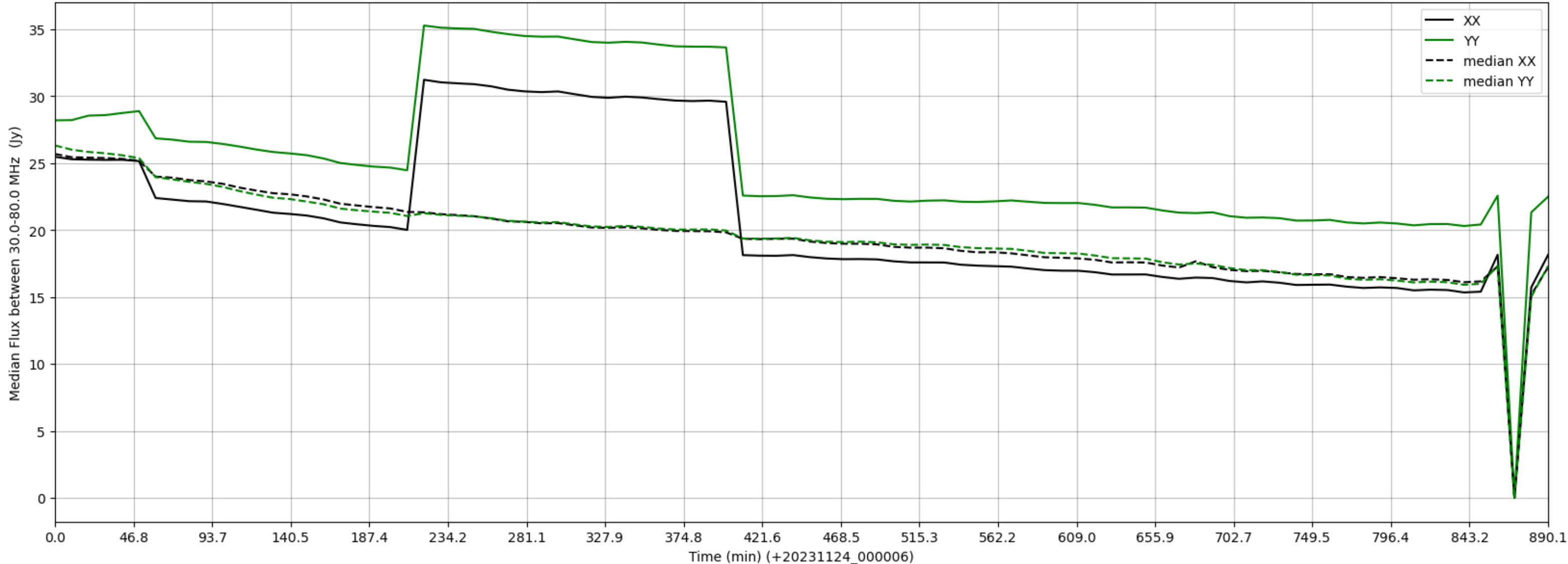
LWA316 - Correlator# 155 - XX FLAGS:HighTimeVar+BadSpecShape - YY FLAGS:HighTimeVar
