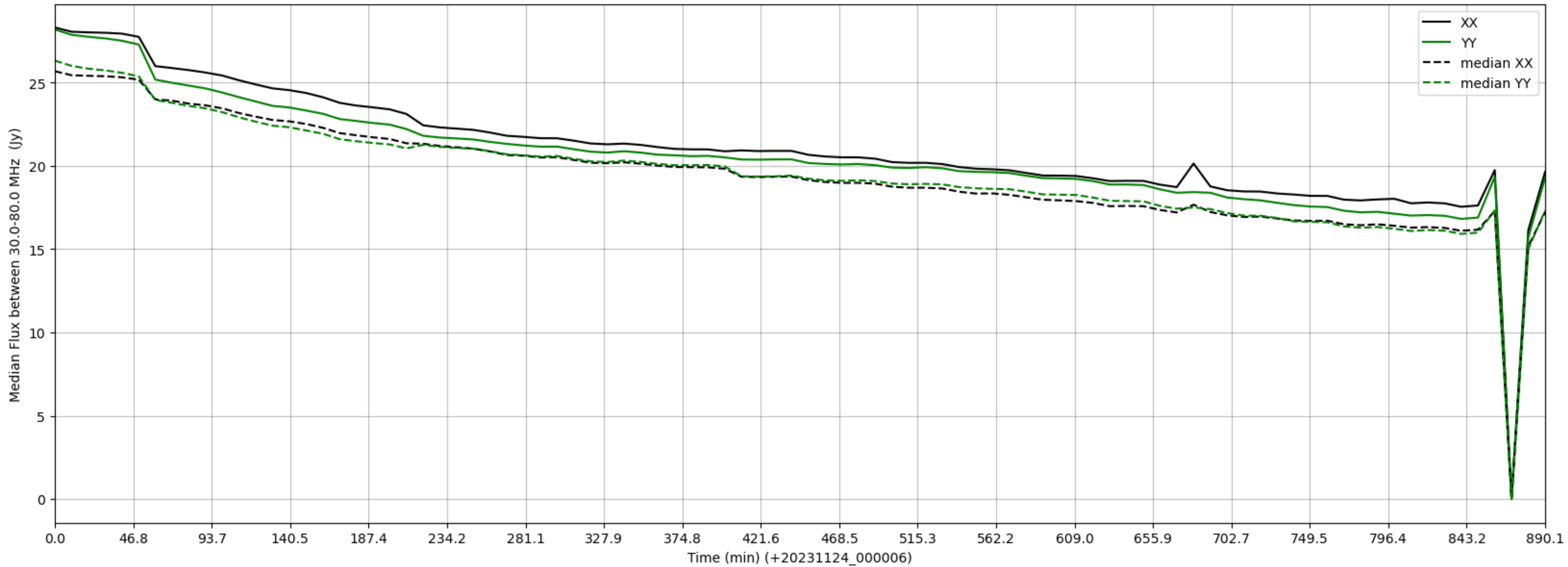
LWA069 - Correlator# 169 - XX FLAGS:BadSpecShape - YY FLAGS:BadSpecShape
