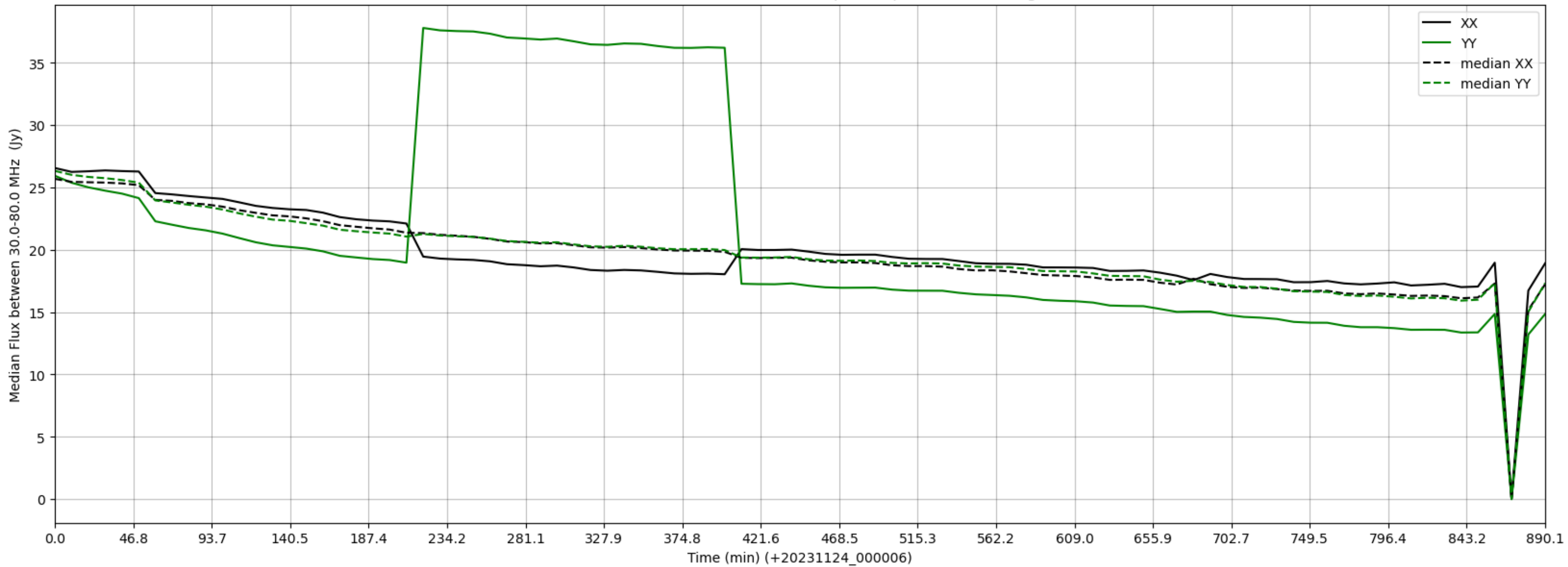
LWA361 - Correlator# 158 - XX FLAGS:BadSpecShape - YY FLAGS:HighTimeVar
