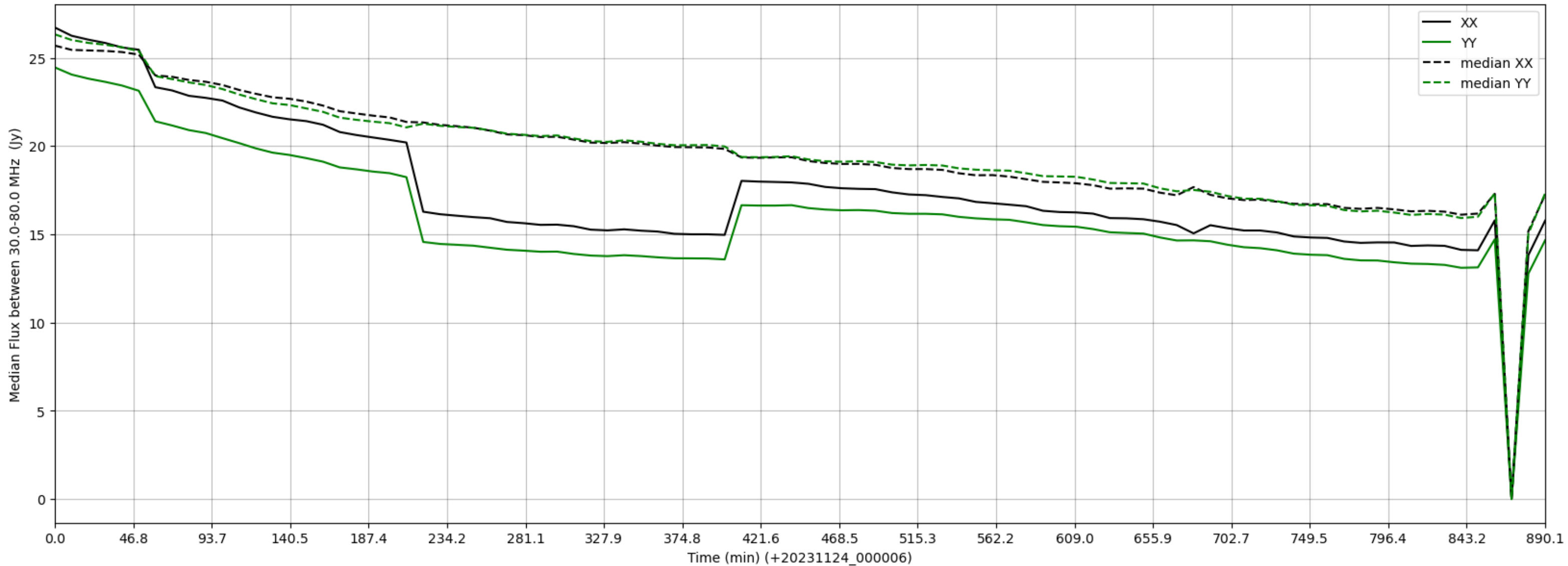
LWA299 - Correlator# 191 - XX FLAGS:HighTimeVar+BadSpecShape - YY FLAGS:BadSpecShape
