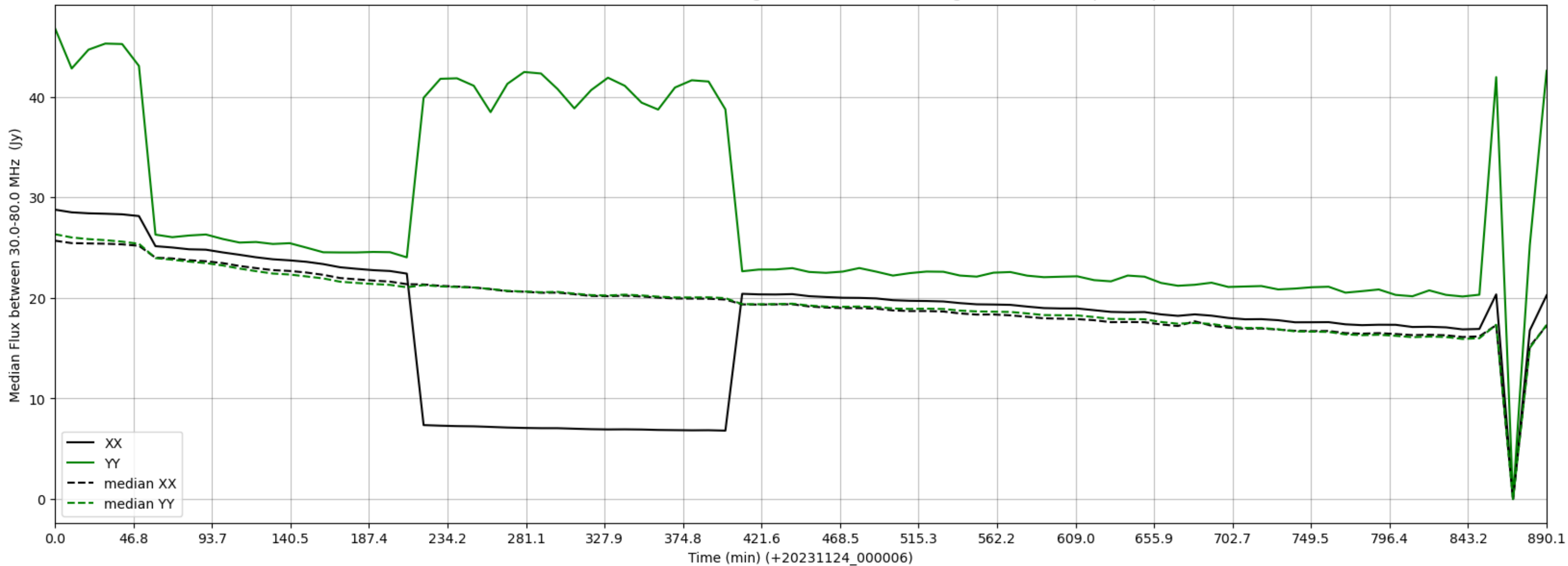
LWA288 - Correlator# 042 - XX FLAGS:HighTimeVar - YY FLAGS:HighTimeVar+BadSpecShape
