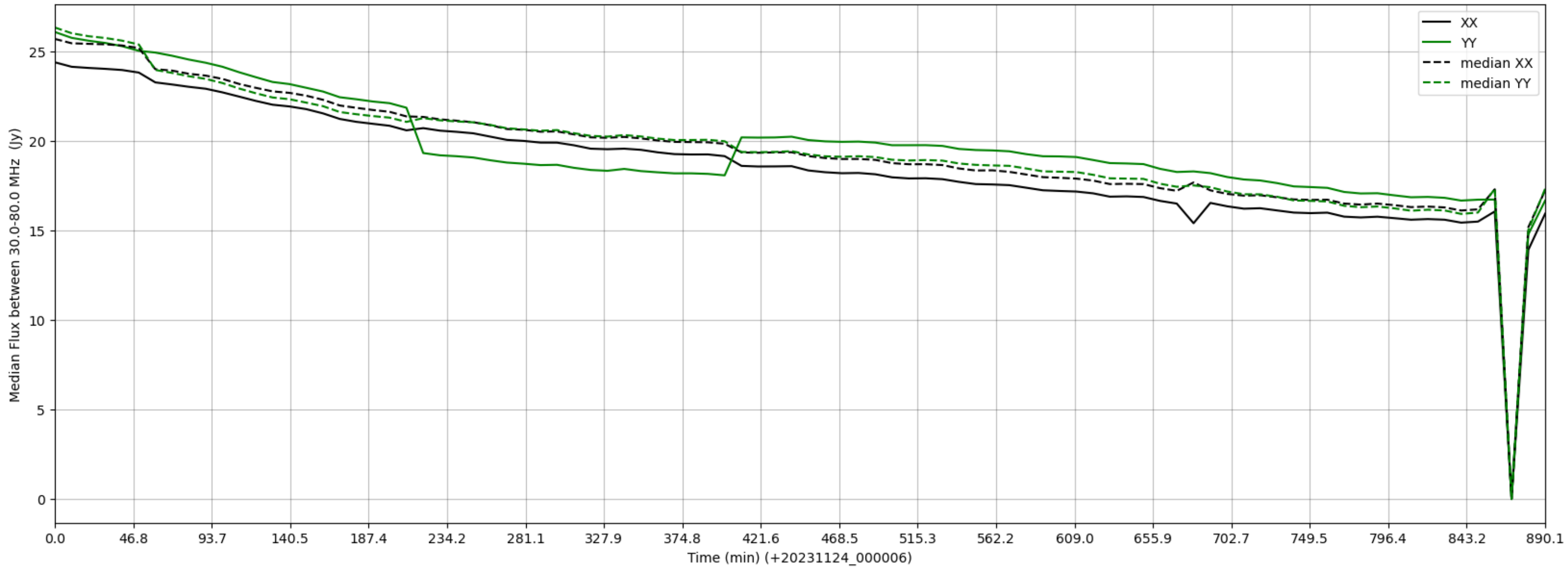
LWA092 - Correlator# 149 - XX FLAGS:Good - YY FLAGS:BadSpecShape
