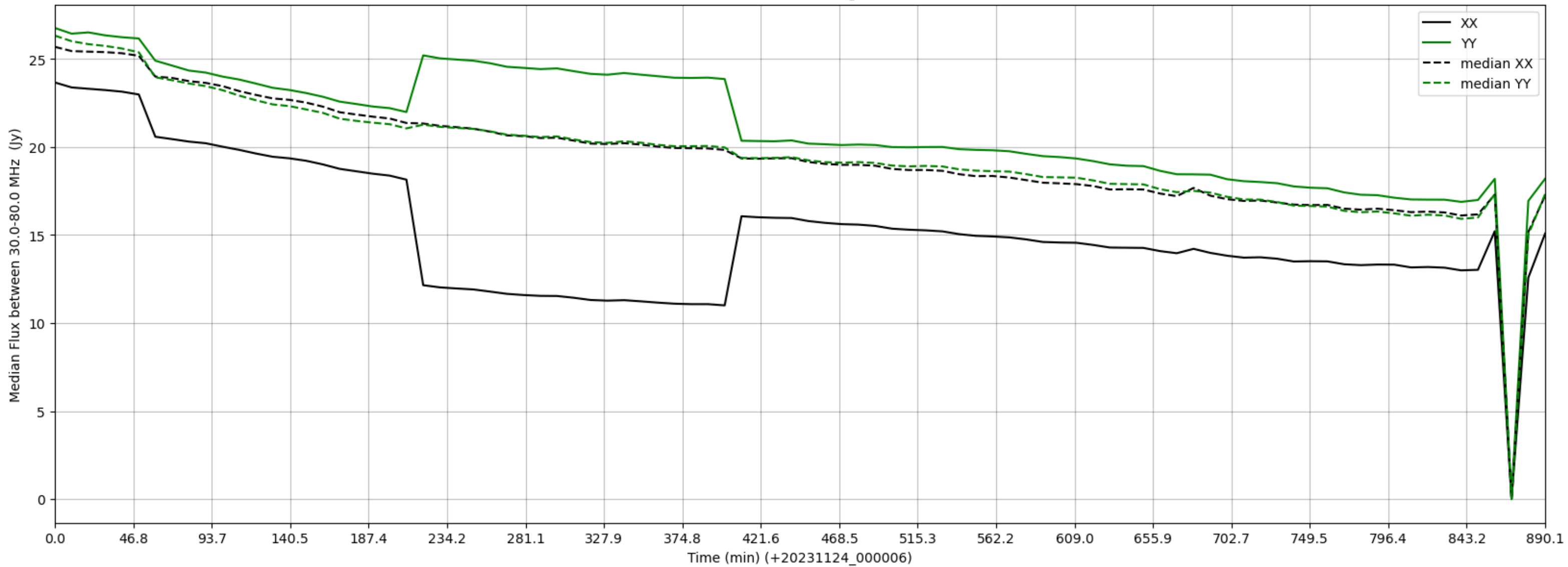
LWA285 - Correlator# 013 - XX FLAGS:HighTimeVar - YY FLAGS:Good
