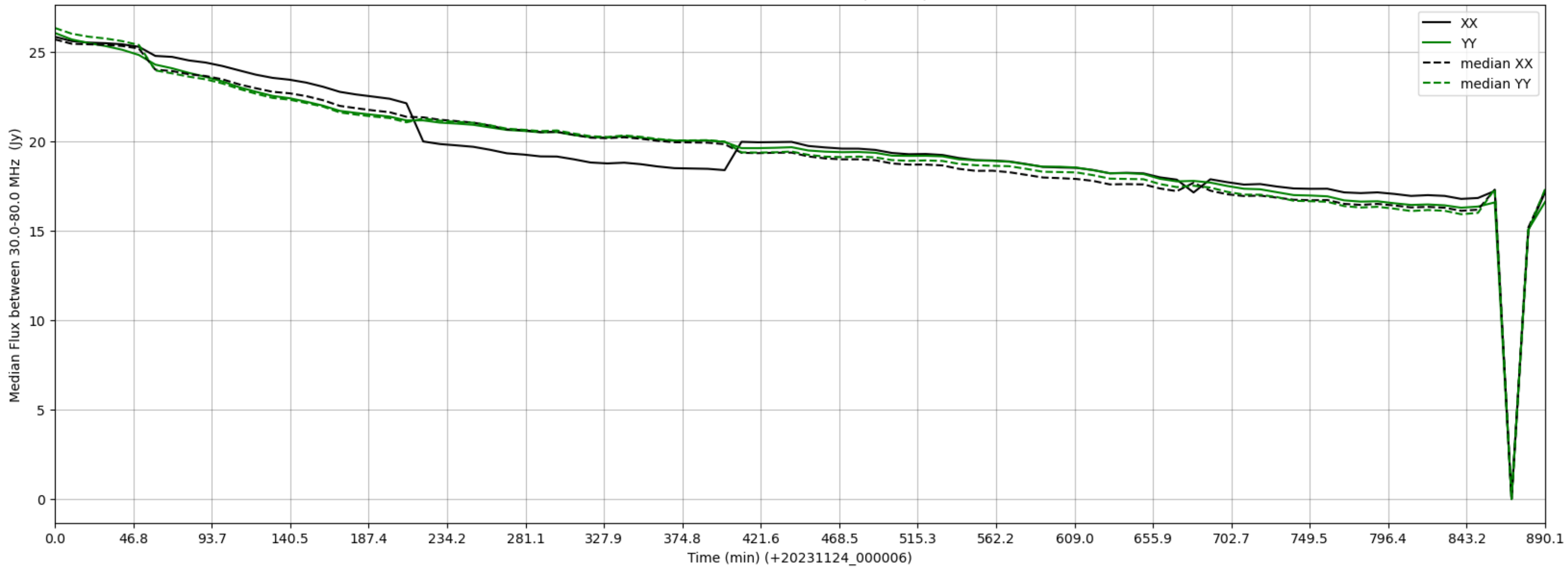
LWA156 - Correlator# 235 - XX FLAGS:BadSpecShape - YY FLAGS:Good
