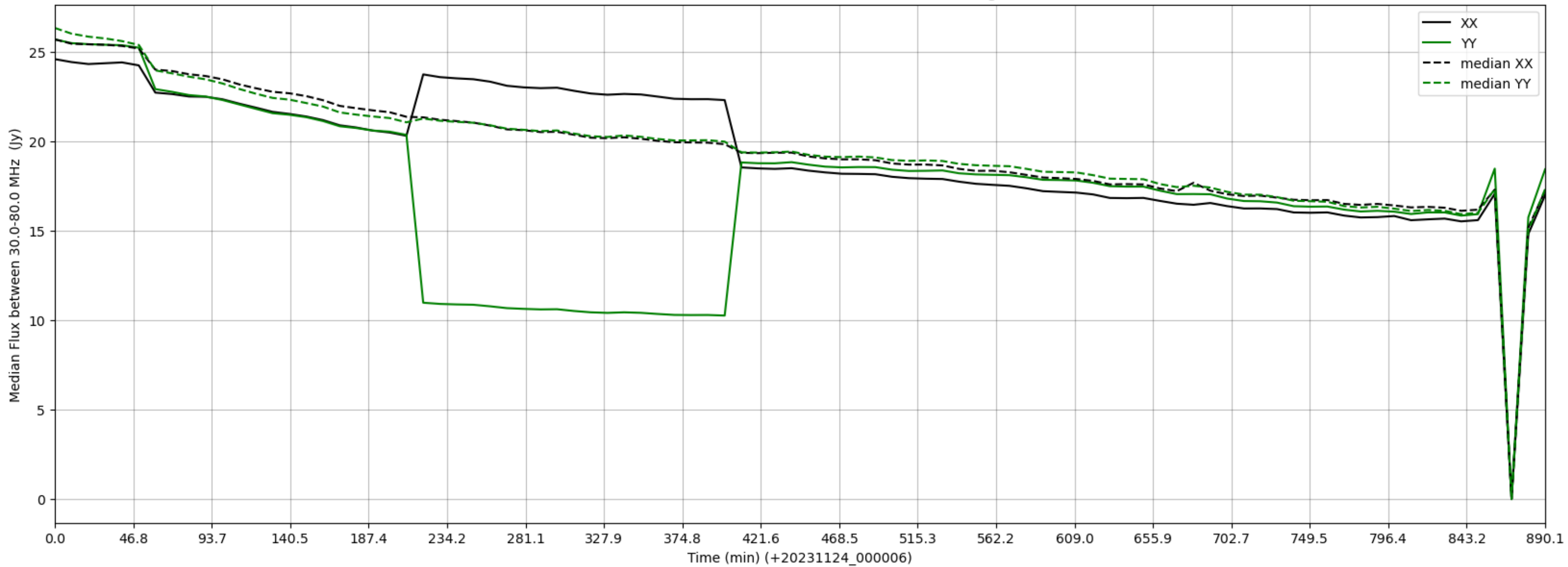
LWA289 - Correlator# 189 - XX FLAGS:Good - YY FLAGS:HighTimeVar
