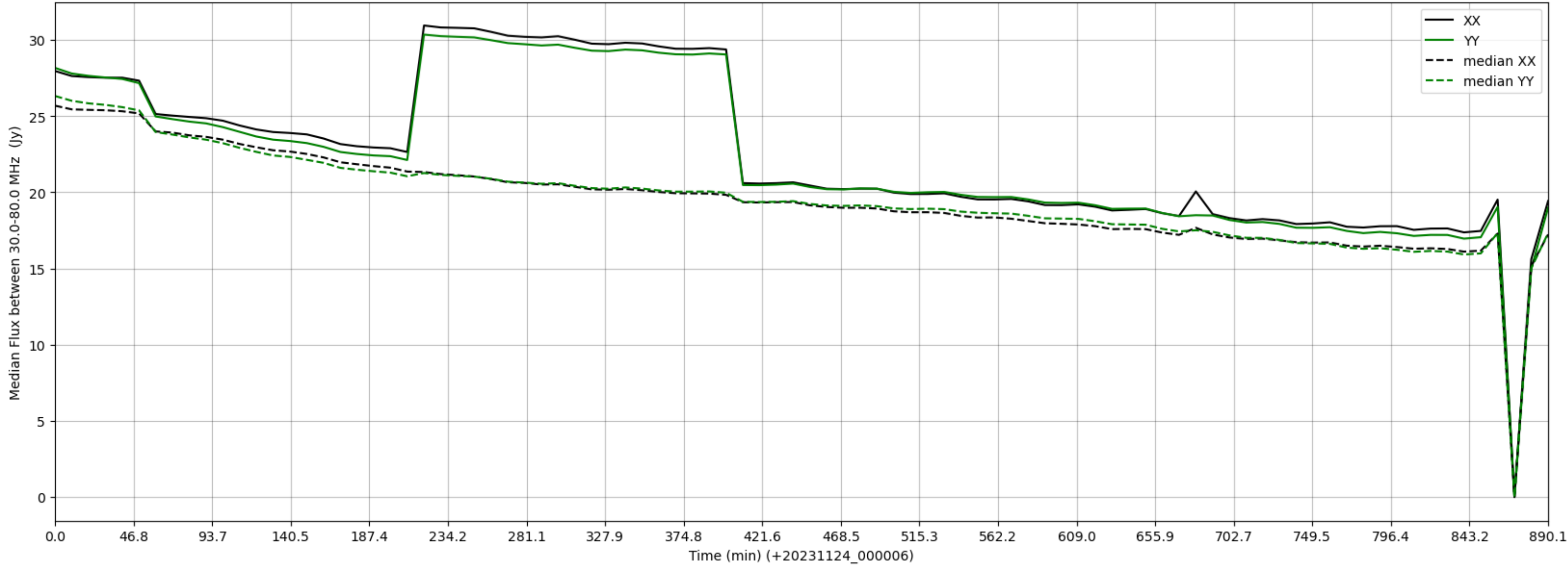
LWA202 - Correlator# 278 - XX FLAGS:HighTimeVar+BadSpecShape - YY FLAGS:HighTimeVar
