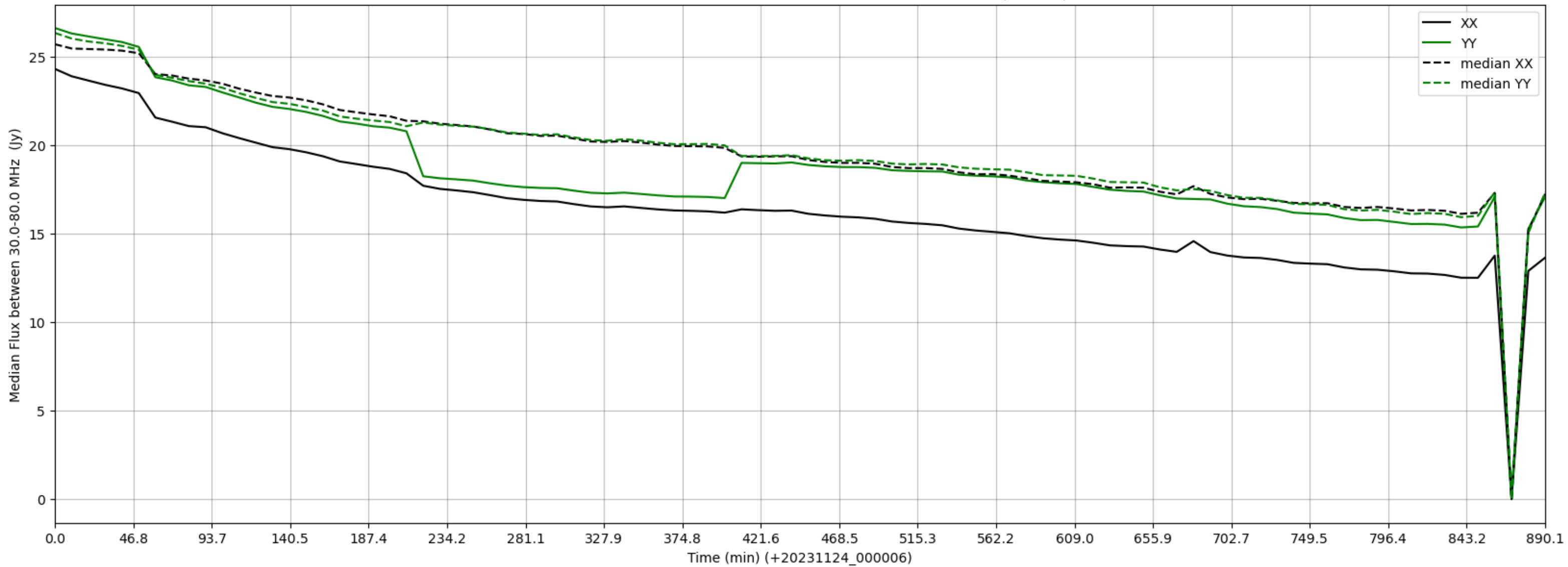
LWA258 - Correlator# 035 - XX FLAGS:Good - YY FLAGS:BadSpecShape
