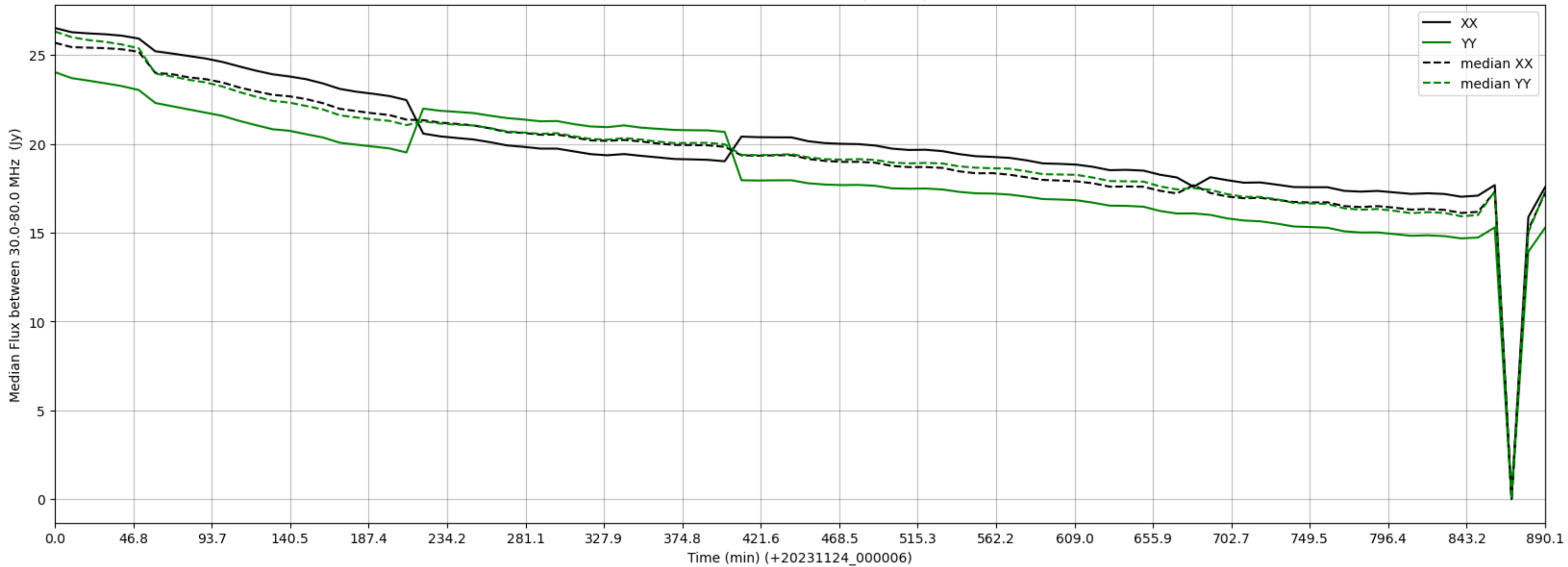
LWA121 - Correlator# 153 - XX FLAGS:BadSpecShape - YY FLAGS:Good
