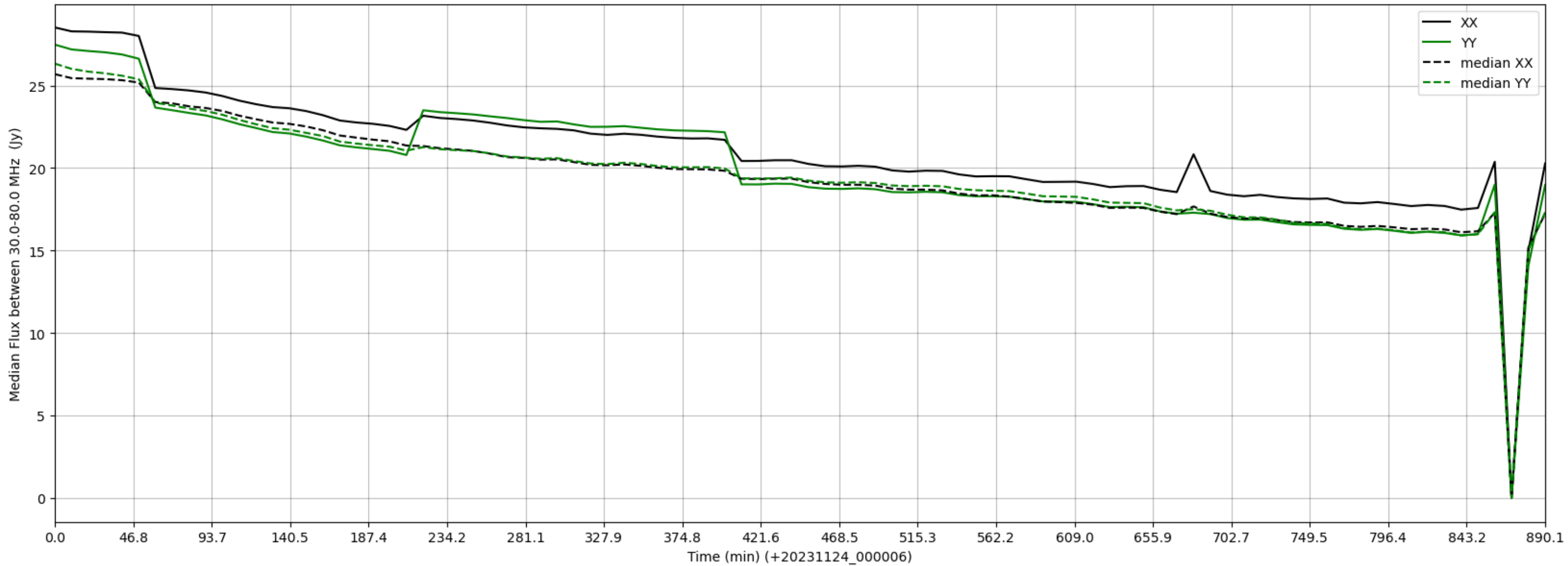
LWA066 - Correlator# 164 - XX FLAGS:BadSpecShape - YY FLAGS:BadSpecShape
