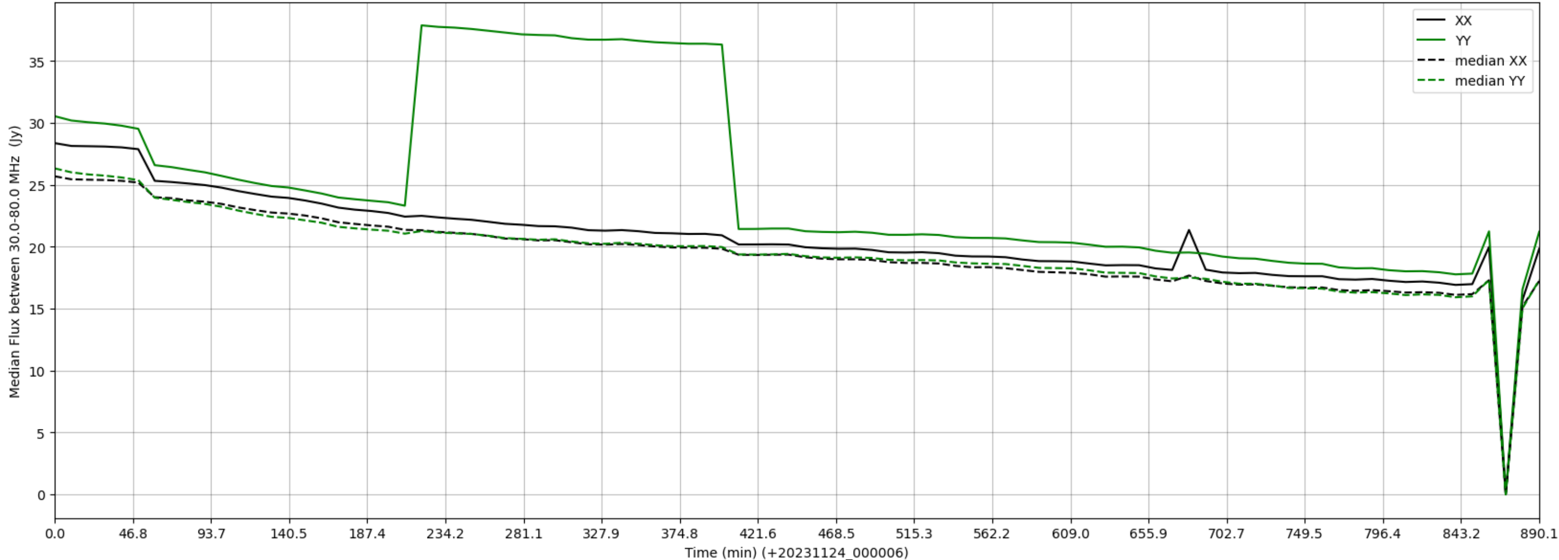
LWA033 - Correlator# 161 - XX FLAGS:BadSpecShape - YY FLAGS:HighTimeVar+BadSpecShape
