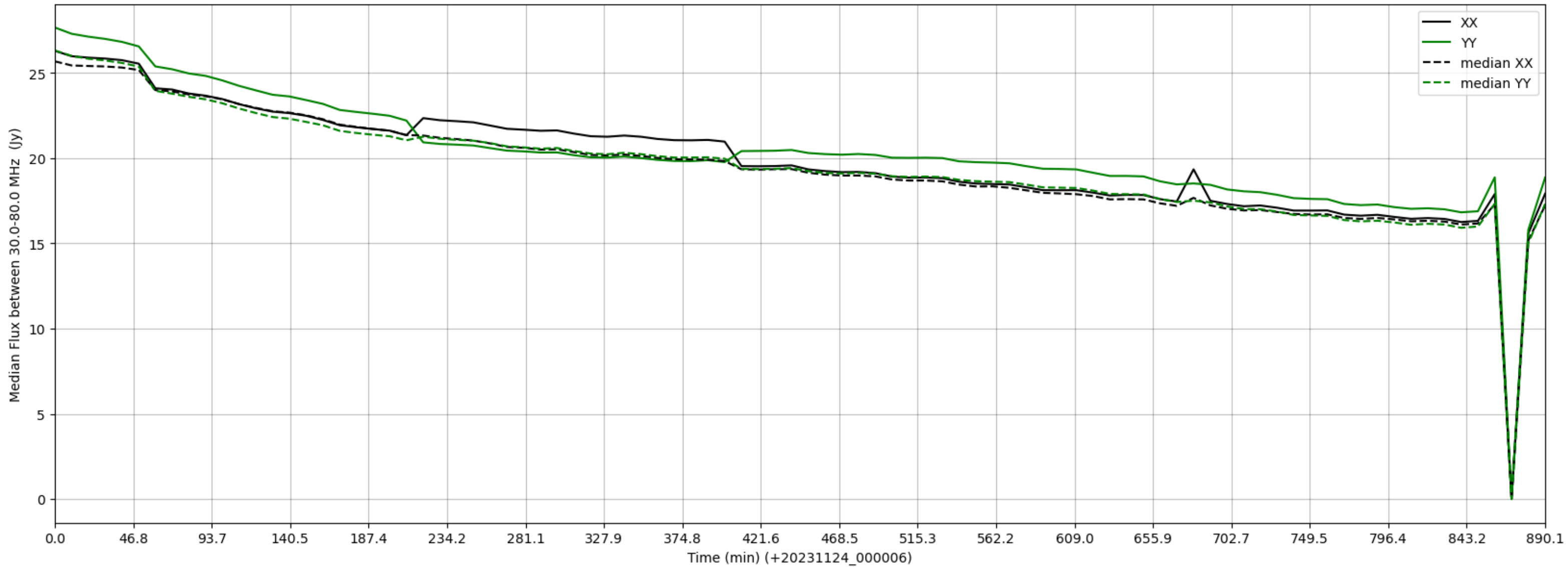
LWA136 - Correlator# 259 - XX FLAGS:Good - YY FLAGS:BadSpecShape
