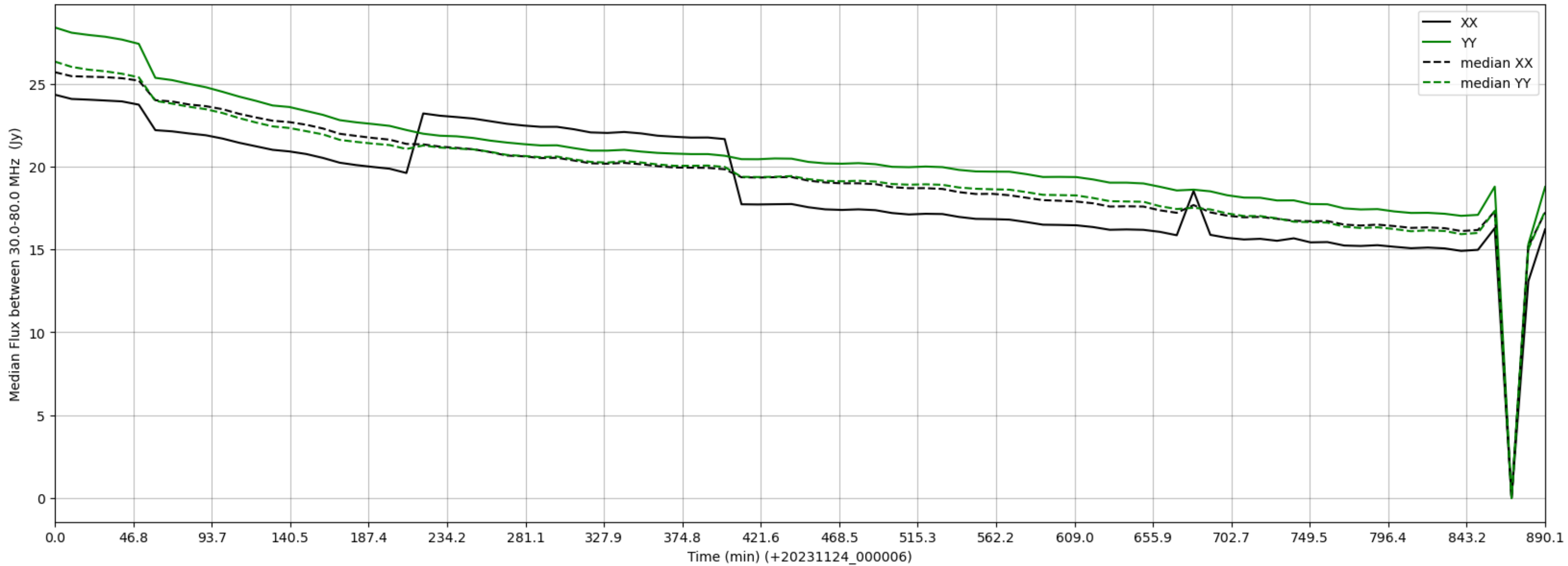
LWA100 - Correlator# 175 - XX FLAGS:HighTimeVar+BadSpecShape - YY FLAGS:BadSpecShape
