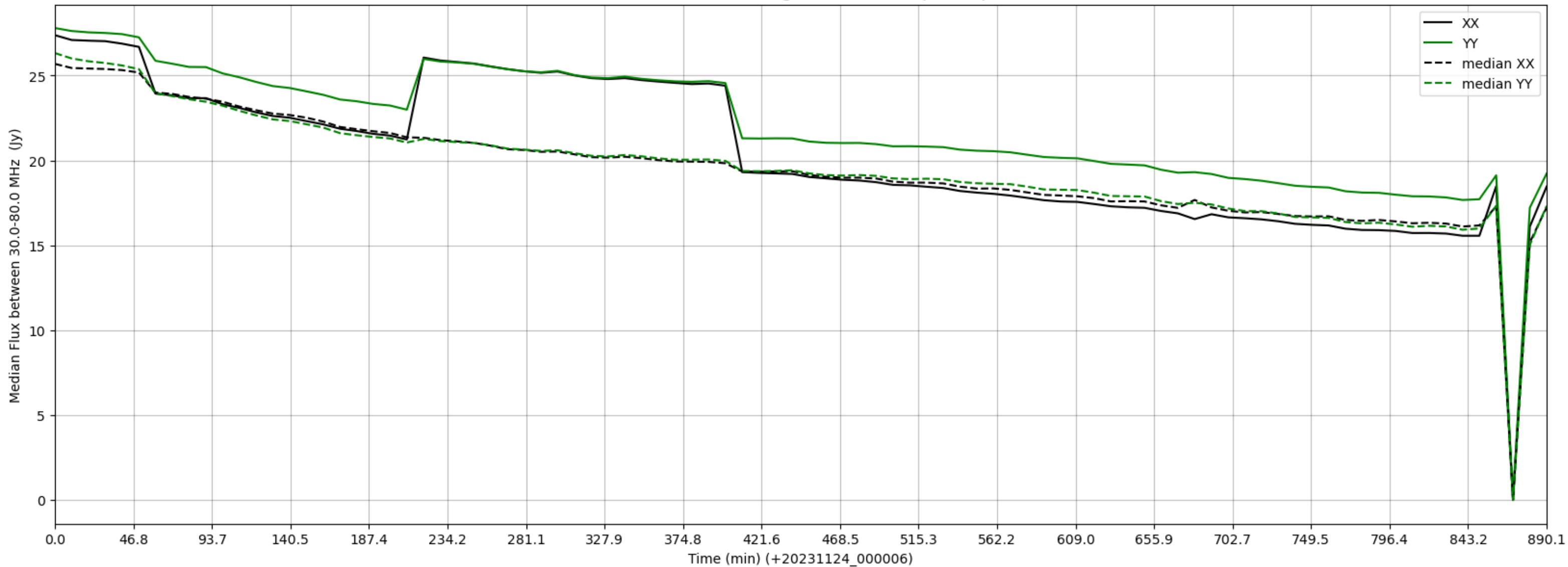
LWA329 - Correlator# 287 - XX FLAGS:HighTimeVar+BadSpecShape - YY FLAGS:Good
