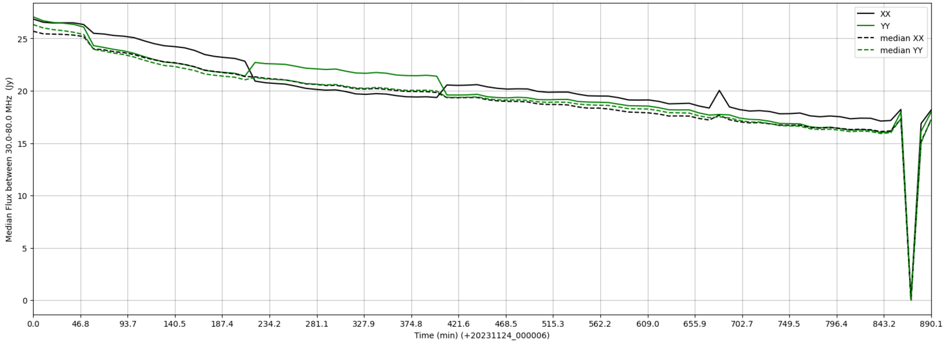
LWA018 - Correlator# 100 - XX FLAGS:BadSpecShape - YY FLAGS:Good
