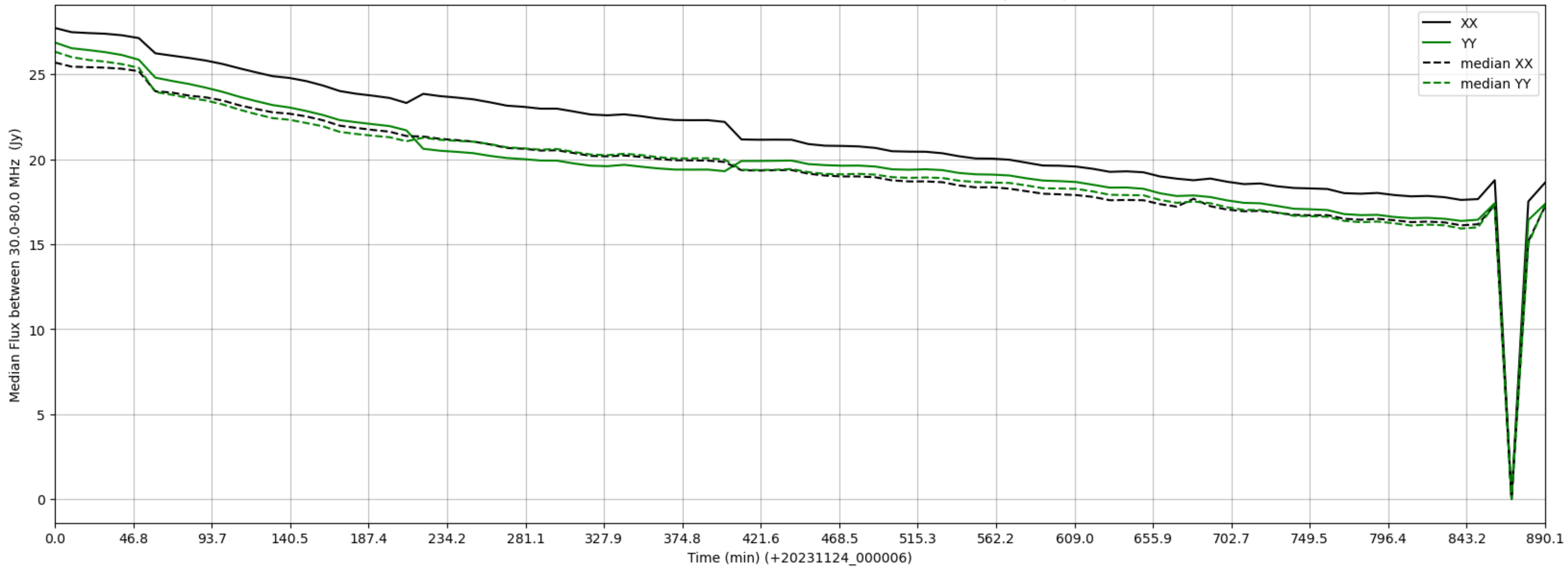
LWA024 - Correlator# 106 - XX FLAGS:Good - YY FLAGS:BadSpecShape
