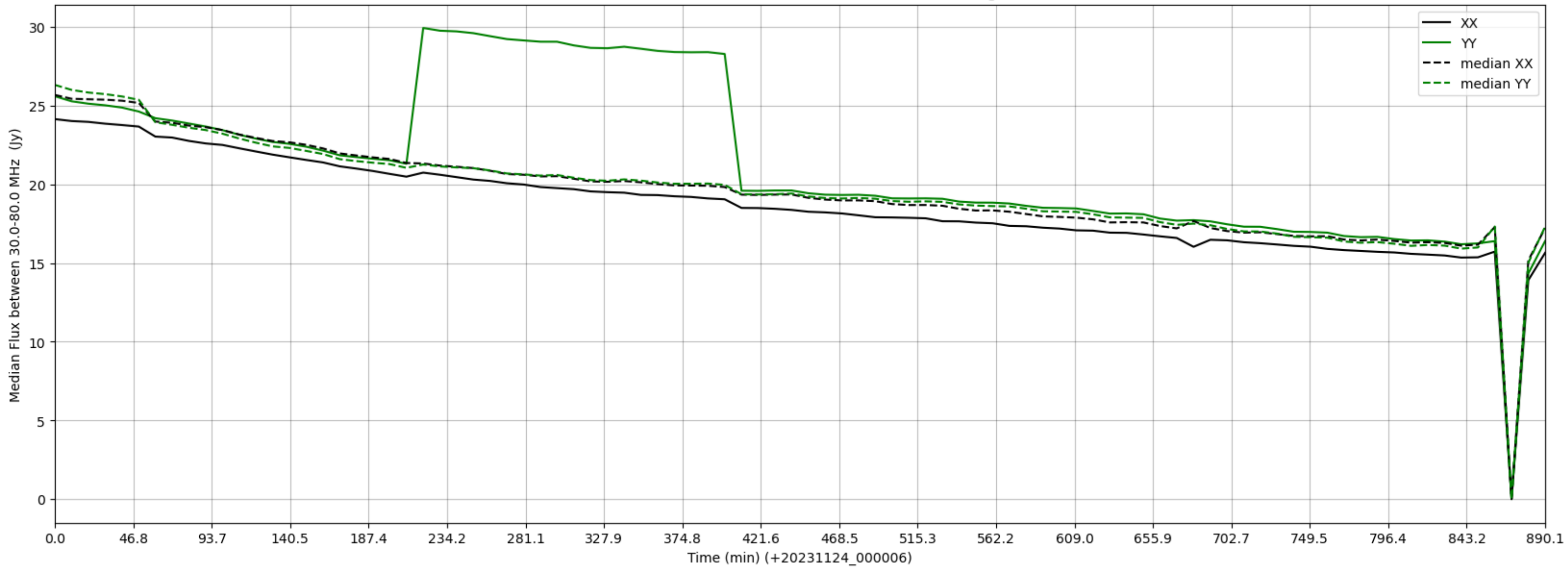
LWA128 - Correlator# 229 - XX FLAGS:Good - YY FLAGS:HighTimeVar
