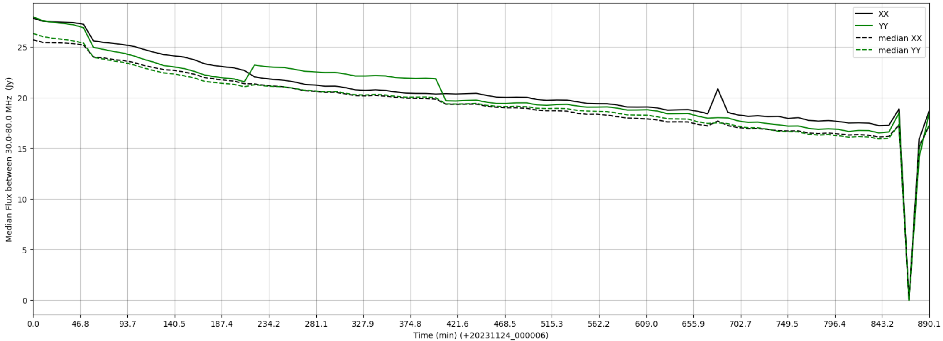
LWA070 - Correlator# 168 - XX FLAGS:BadSpecShape - YY FLAGS:Good
