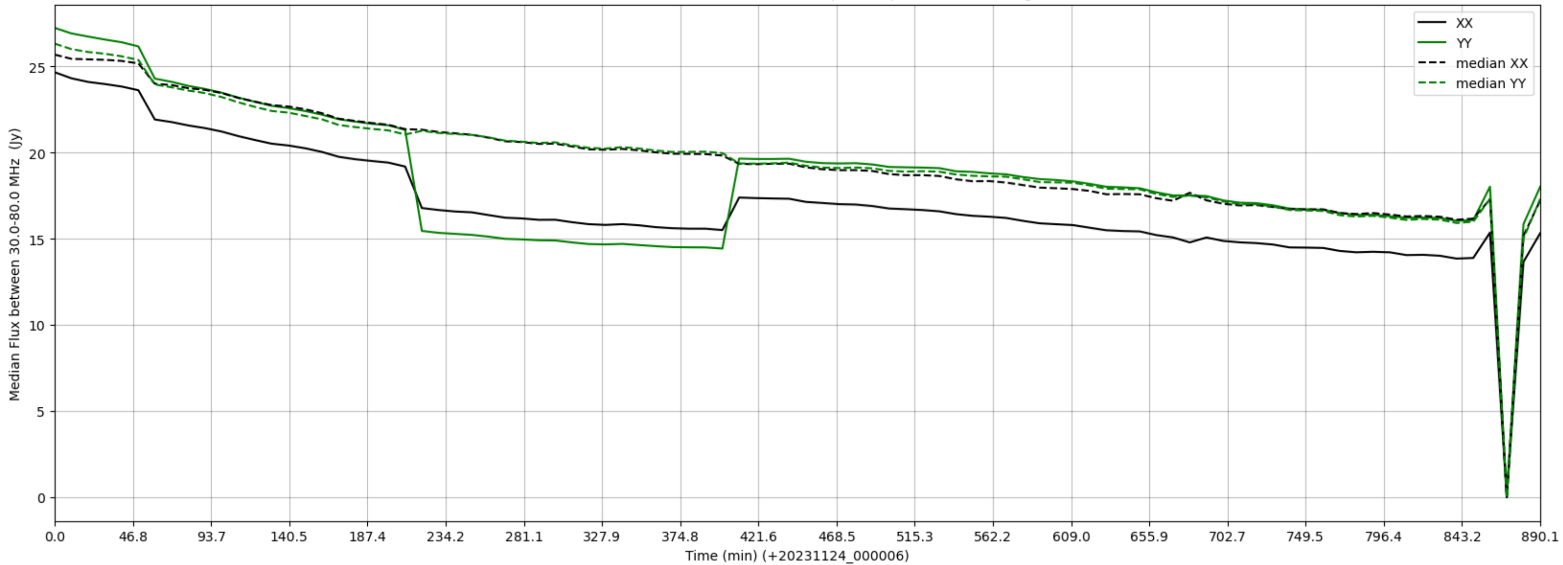
LWA265 - Correlator# 036 - XX FLAGS:BadSpecShape - YY FLAGS:HighTimeVar
