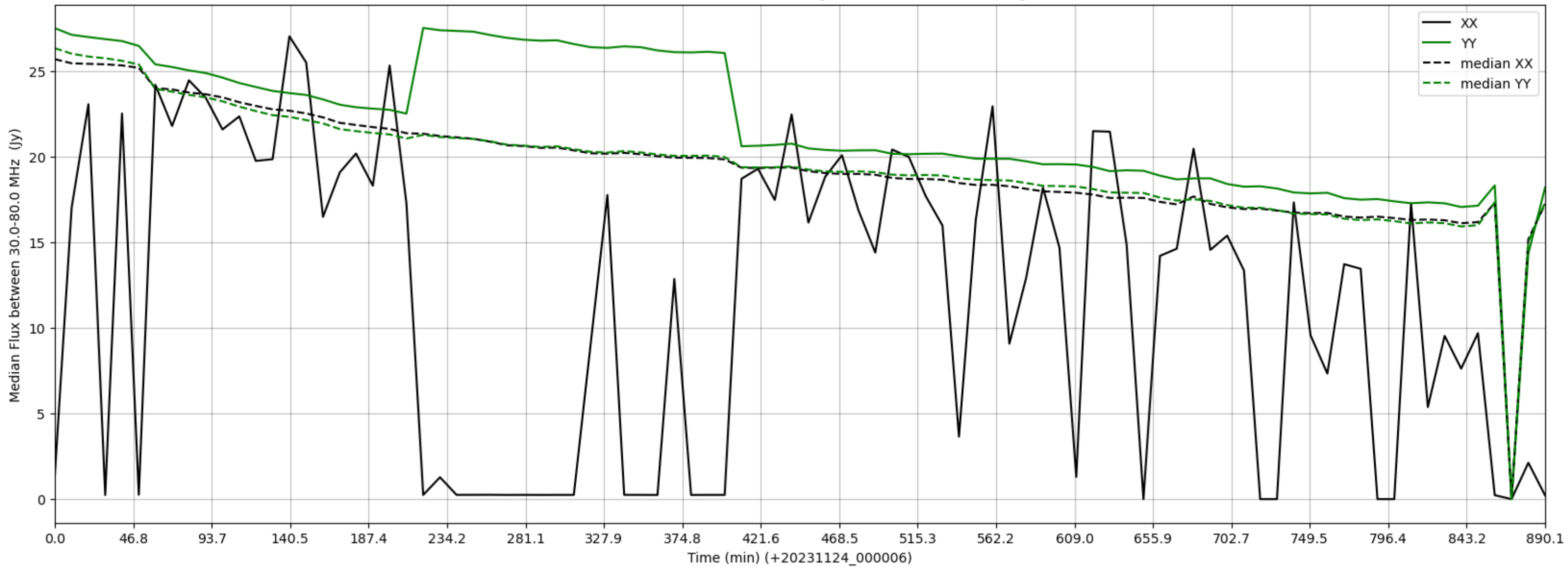
LWA255 - Correlator# 033 - XX FLAGS:HighTimeVar - YY FLAGS:HighTimeVar
