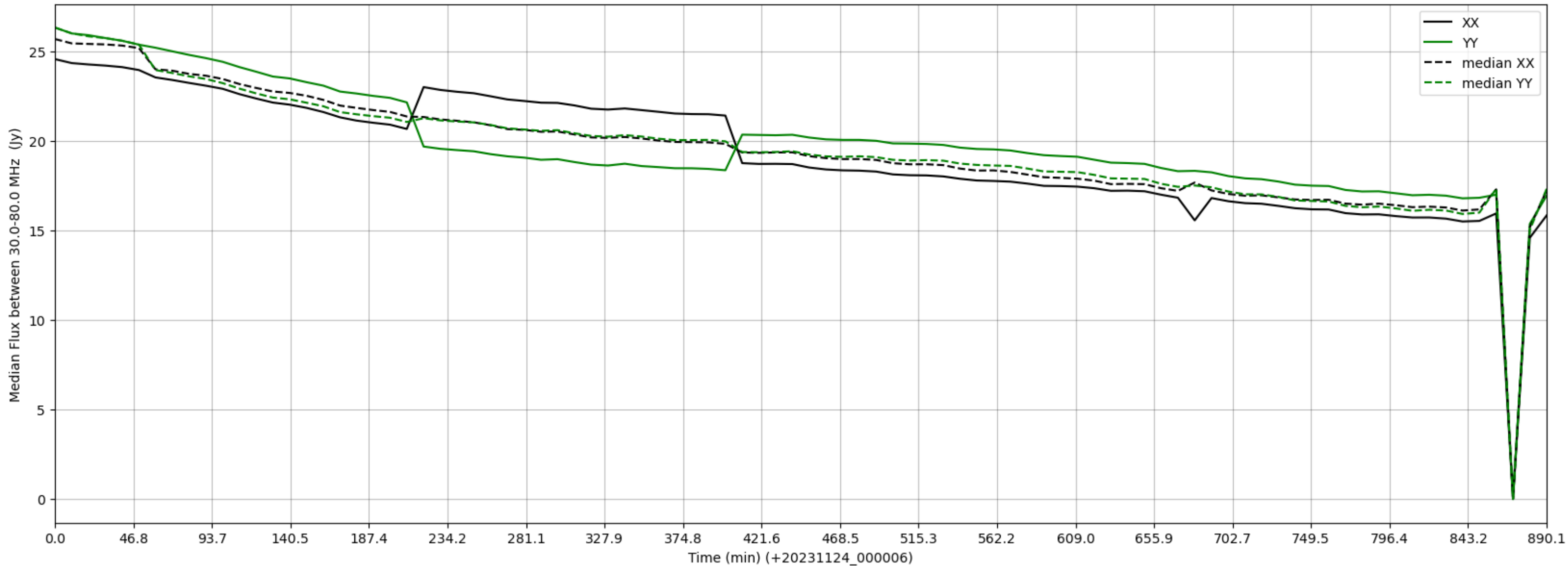
LWA064 - Correlator# 141 - XX FLAGS:Good - YY FLAGS:BadSpecShape
