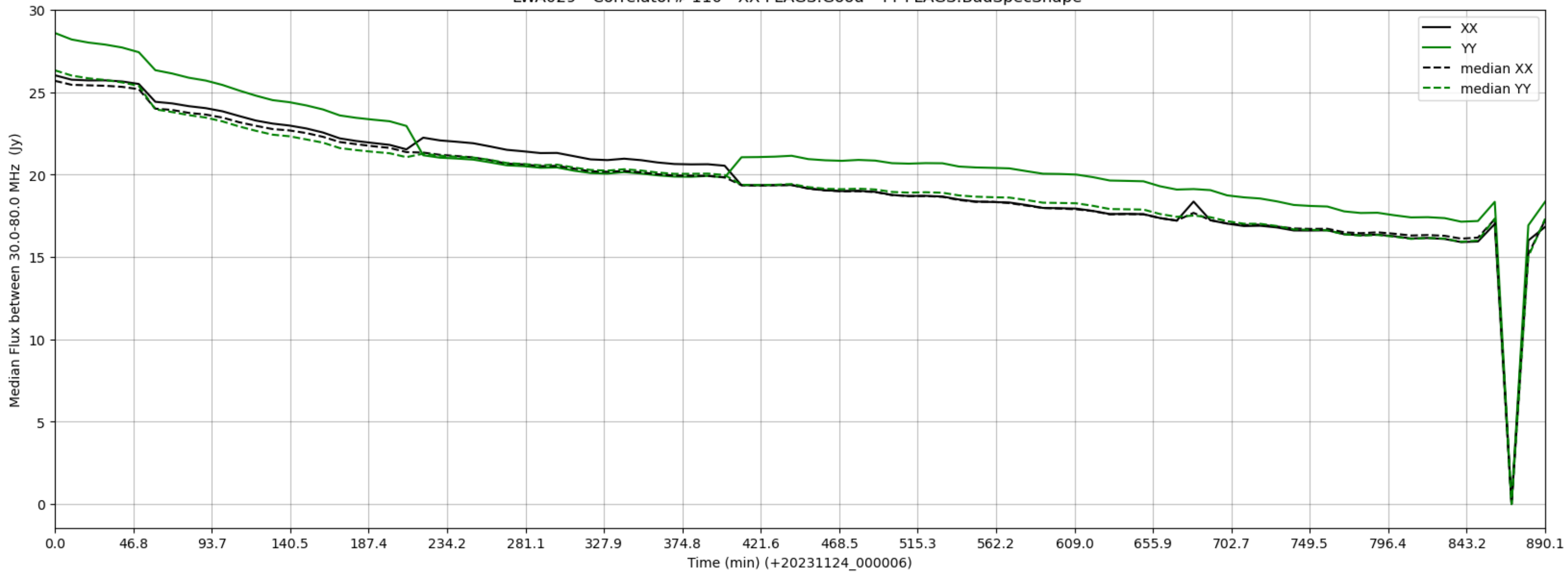
LWA029 - Correlator# 110 - XX FLAGS:Good - YY FLAGS:BadSpecShape
