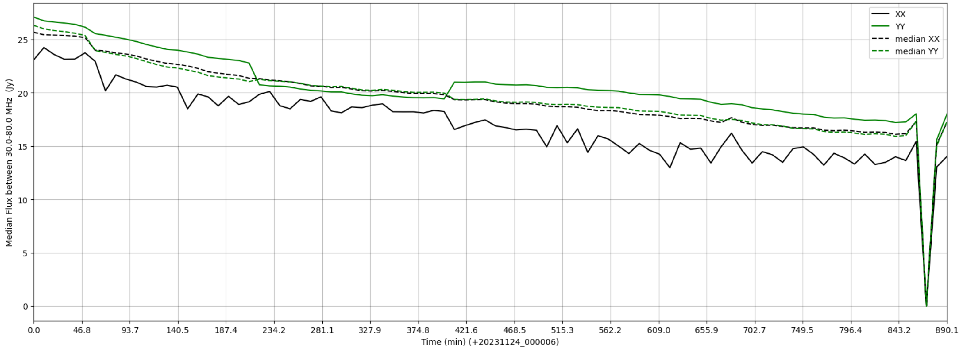
LWA111 - Correlator# 201 - XX FLAGS:Good - YY FLAGS:BadSpecShape
