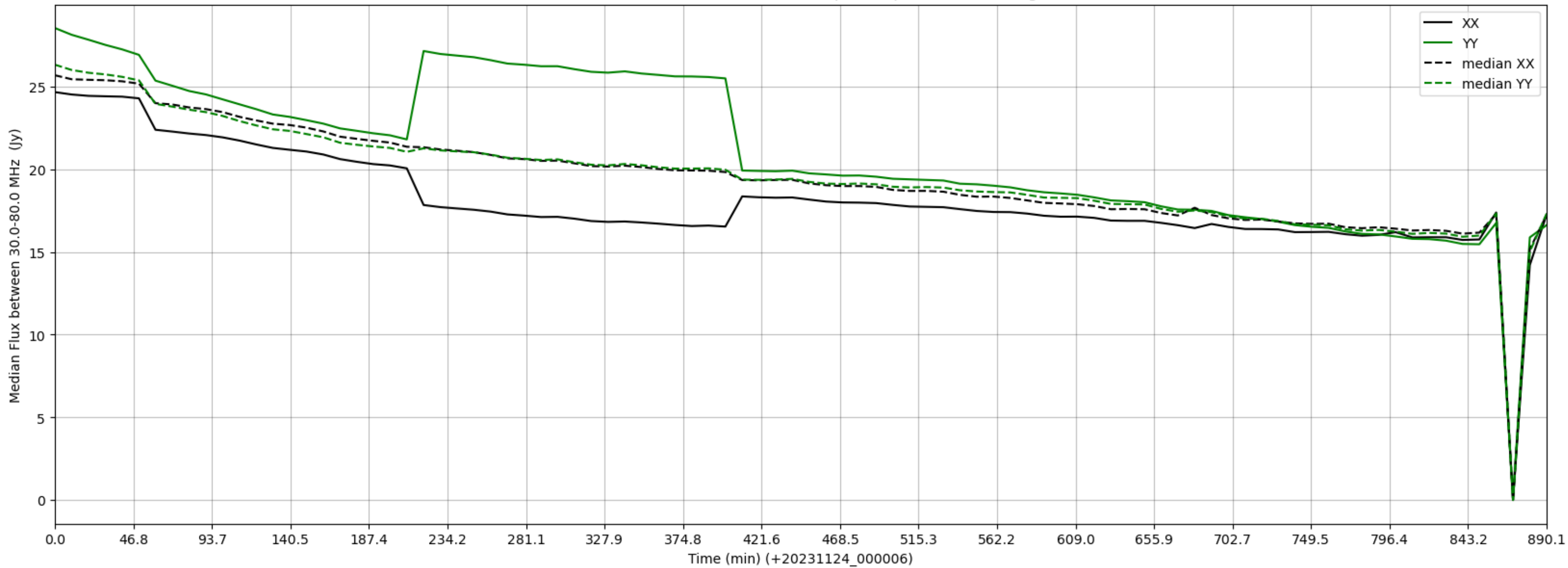
LWA284 - Correlator# 043 - XX FLAGS:BadSpecShape - YY FLAGS:HighTimeVar
