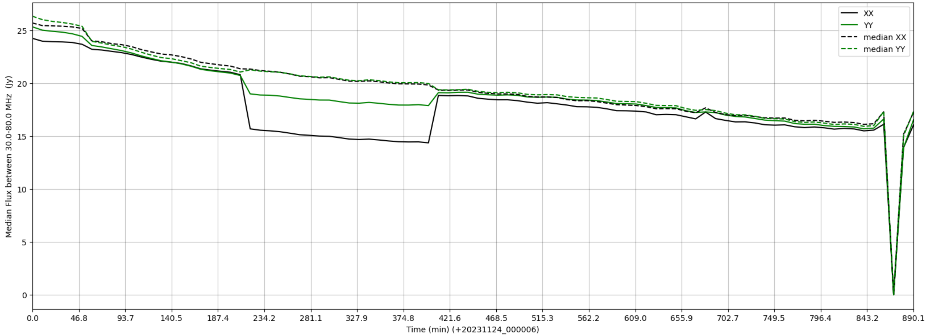
LWA112 - Correlator# 200 - XX FLAGS:HighTimeVar - YY FLAGS:BadSpecShape
