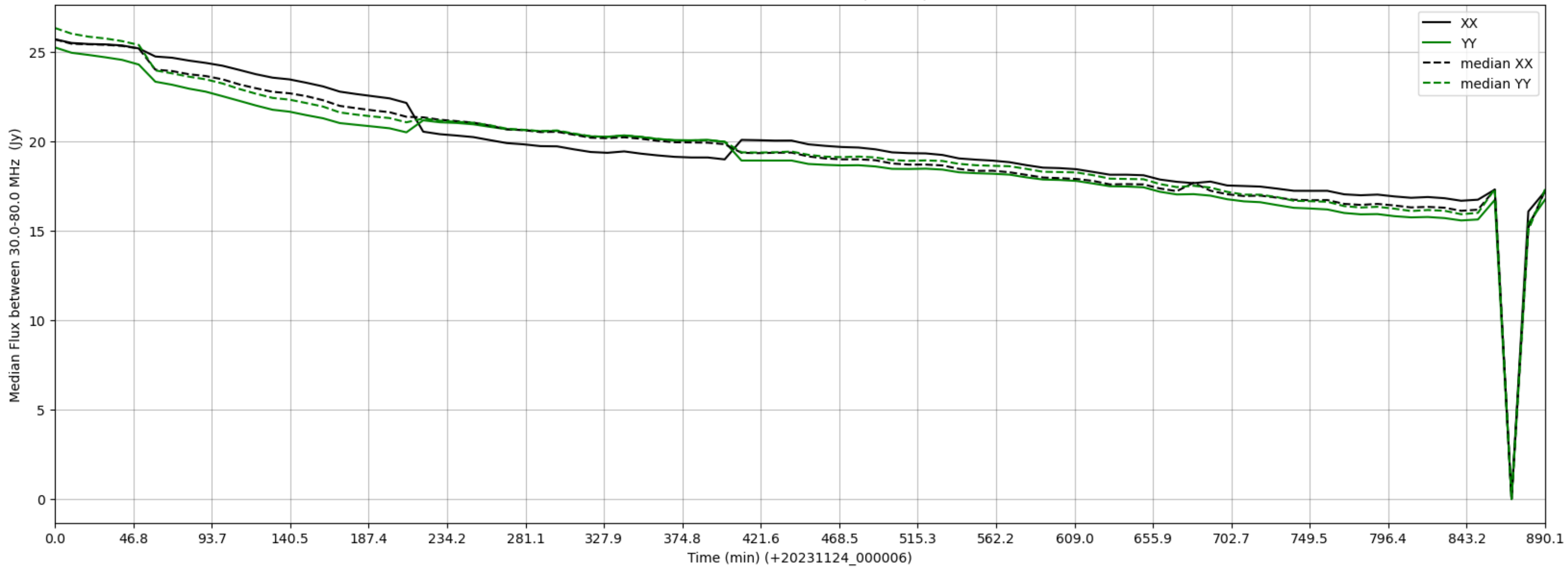
LWA051 - Correlator# 114 - XX FLAGS:BadSpecShape - YY FLAGS:Good
