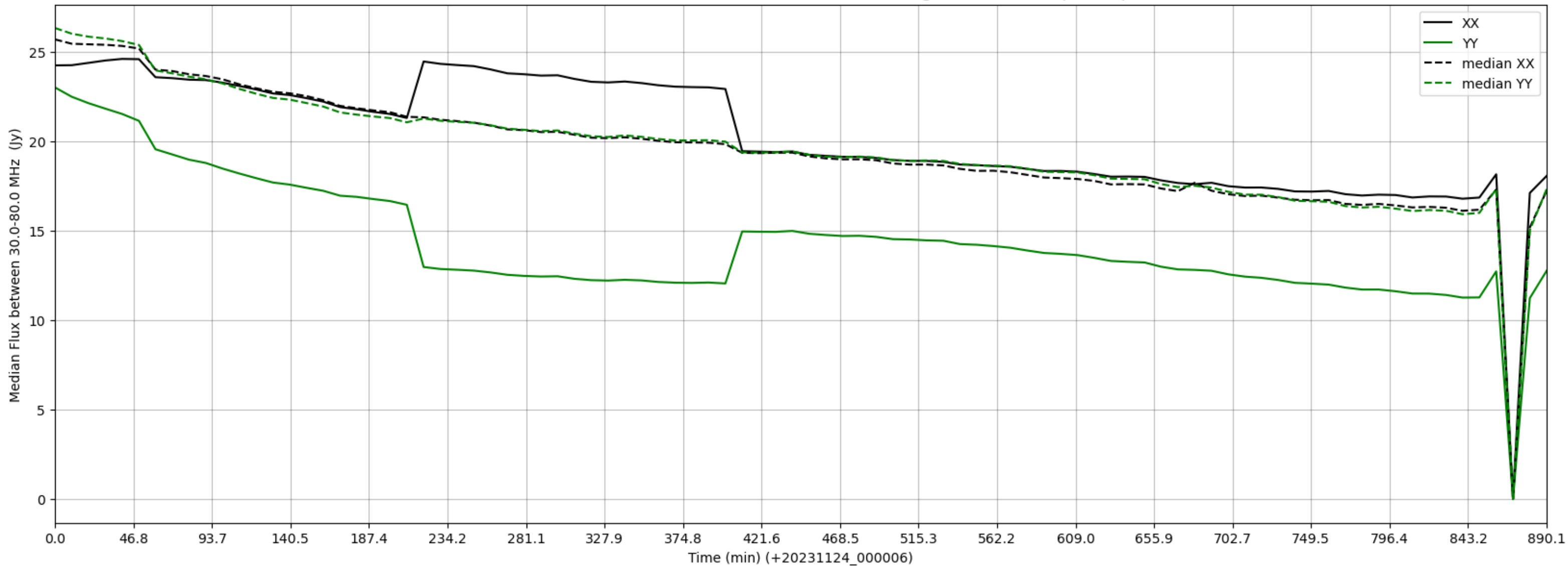
LWA263 - Correlator# 037 - XX FLAGS:Good - YY FLAGS:HighTimeVar+BadSpecShape
