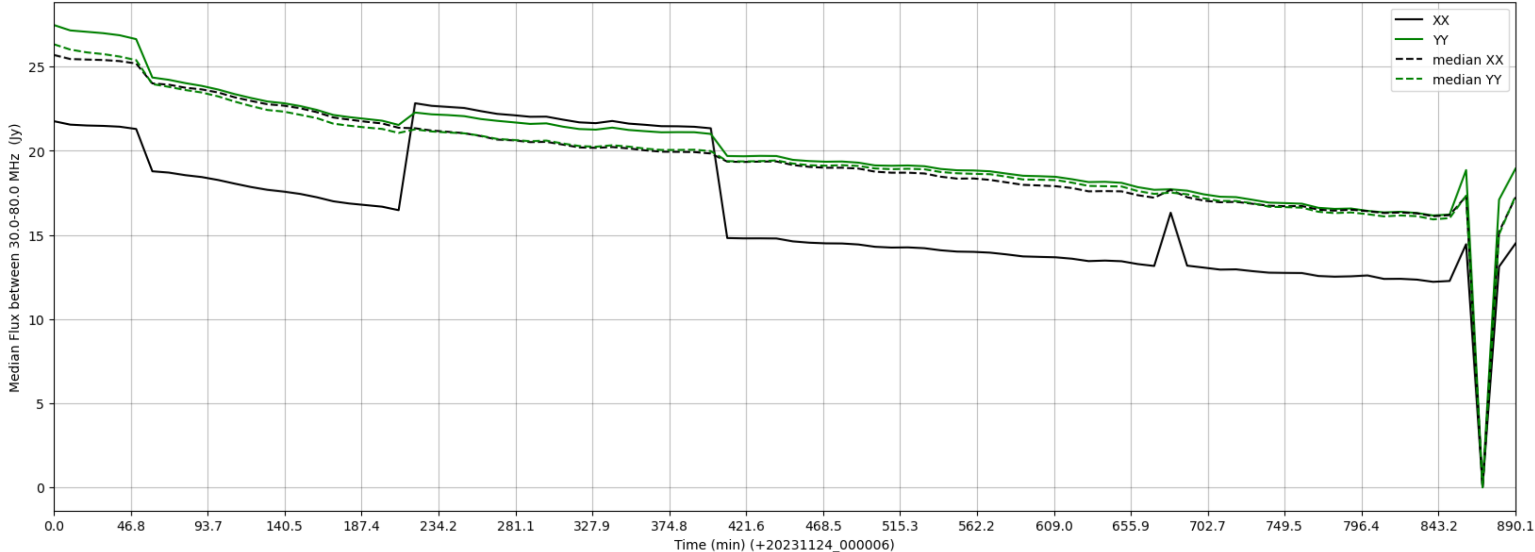
LWA038 - Correlator# 077 - XX FLAGS:HighTimeVar+BadSpecShape - YY FLAGS:BadSpecShape
