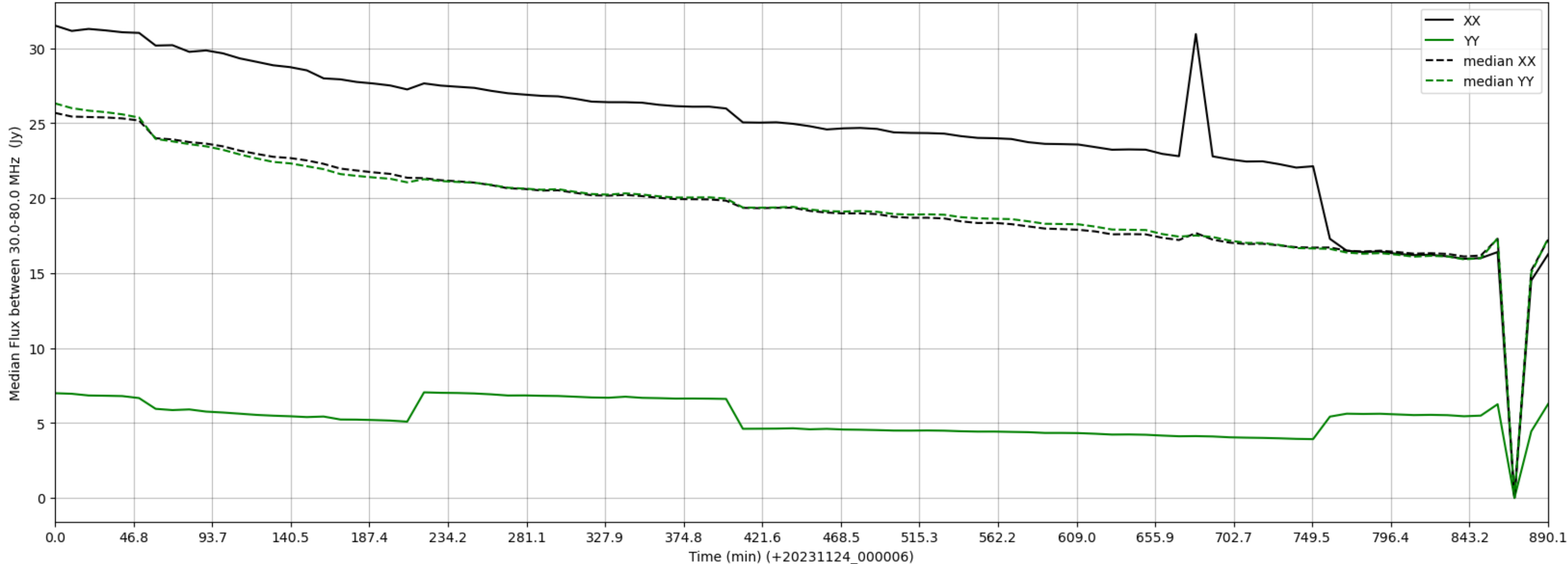
LWA058 - Correlator# 137 - XX FLAGS:BadSpecShape - YY FLAGS:HighTimeVar+BadSpecShape
