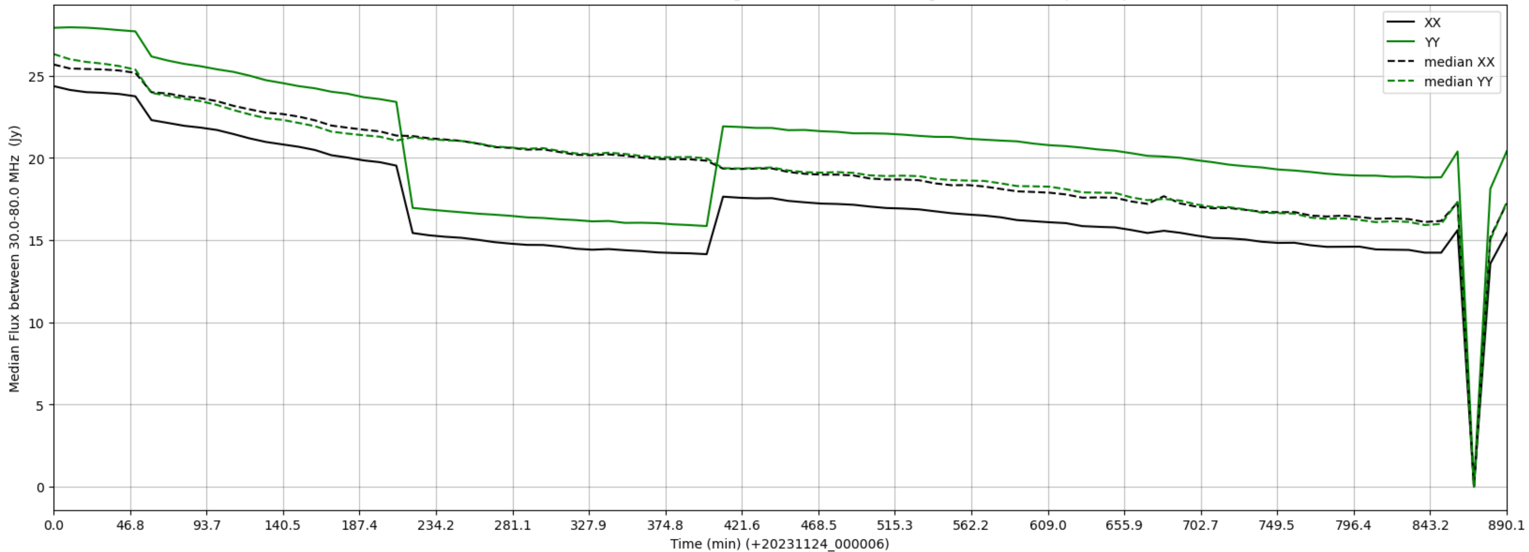
LWA364 - Correlator# 127 - XX FLAGS:HighTimeVar - YY FLAGS:HighTimeVar+BadSpecShape
