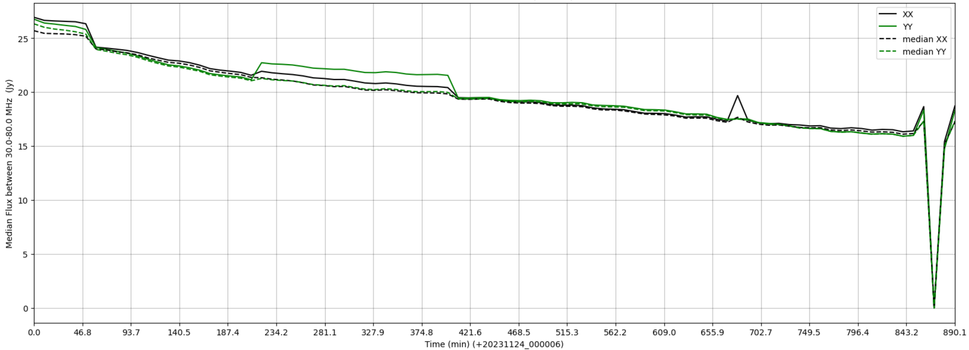
LWA098 - Correlator# 173 - XX FLAGS:BadSpecShape - YY FLAGS:Good
