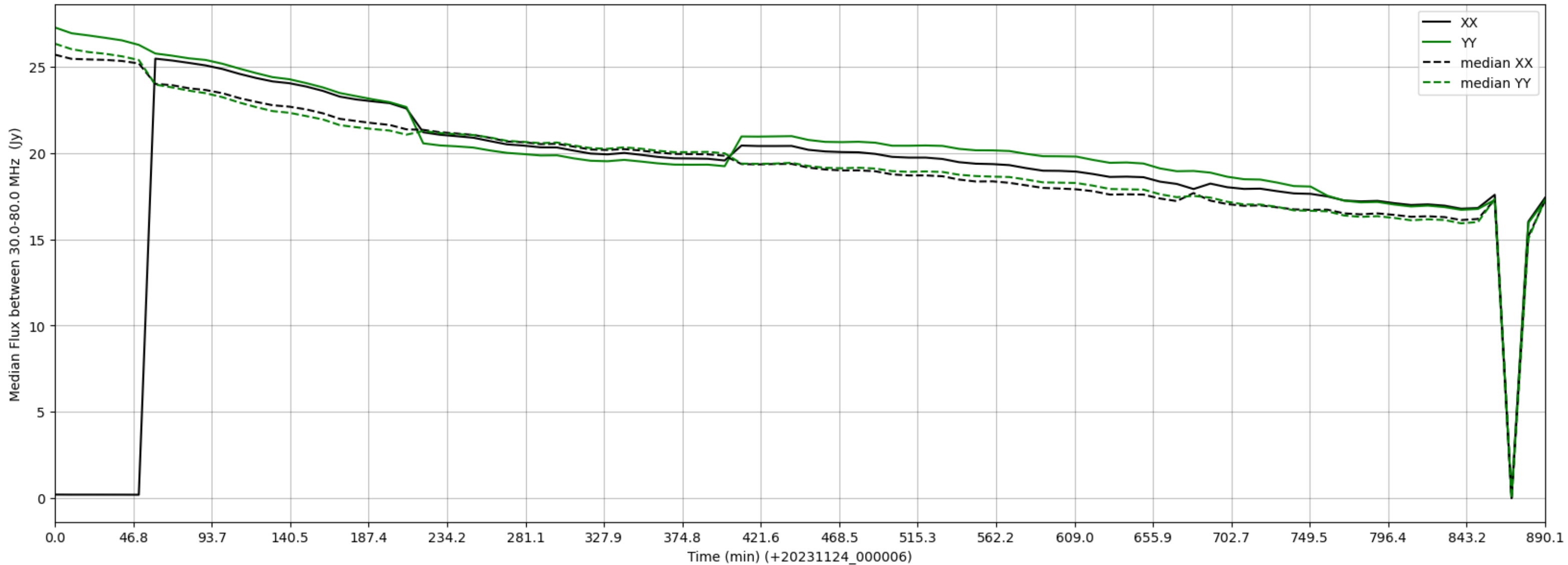
LWA057 - Correlator# 134 - XX FLAGS:HighTimeVar - YY FLAGS:BadSpecShape
