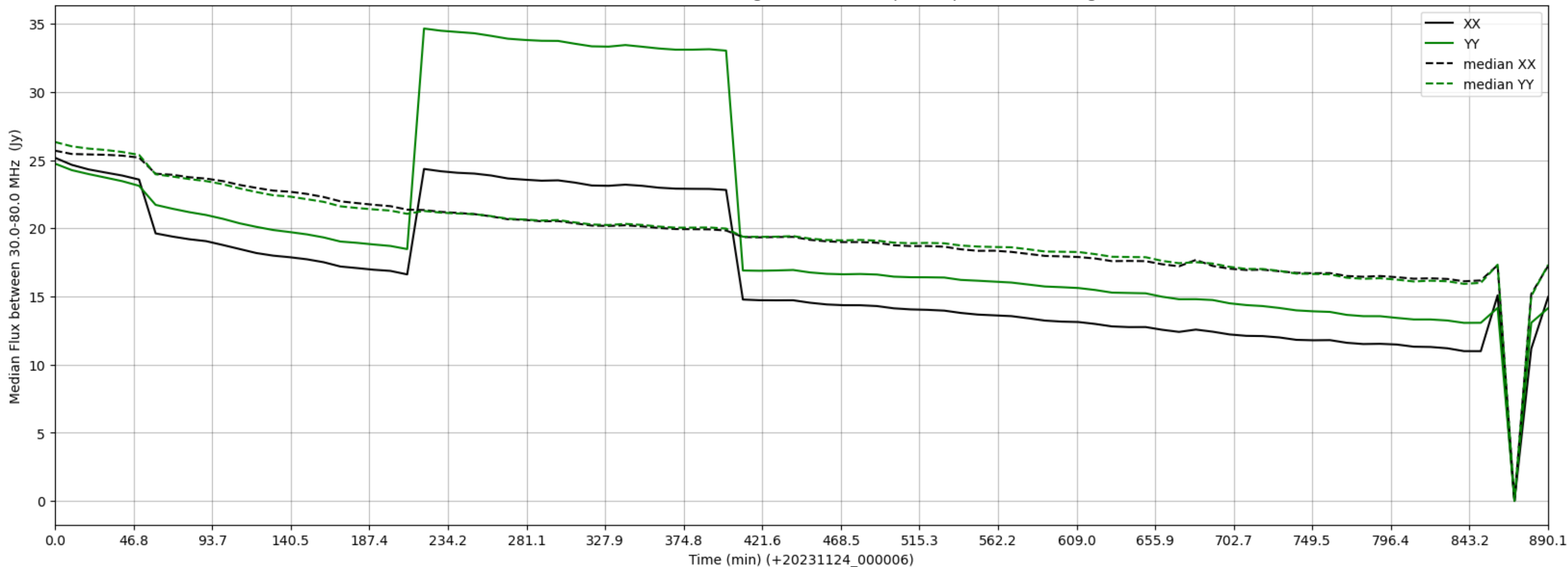
LWA363 - Correlator# 094 - XX FLAGS:HighTimeVar+BadSpecShape - YY FLAGS:HighTimeVar
