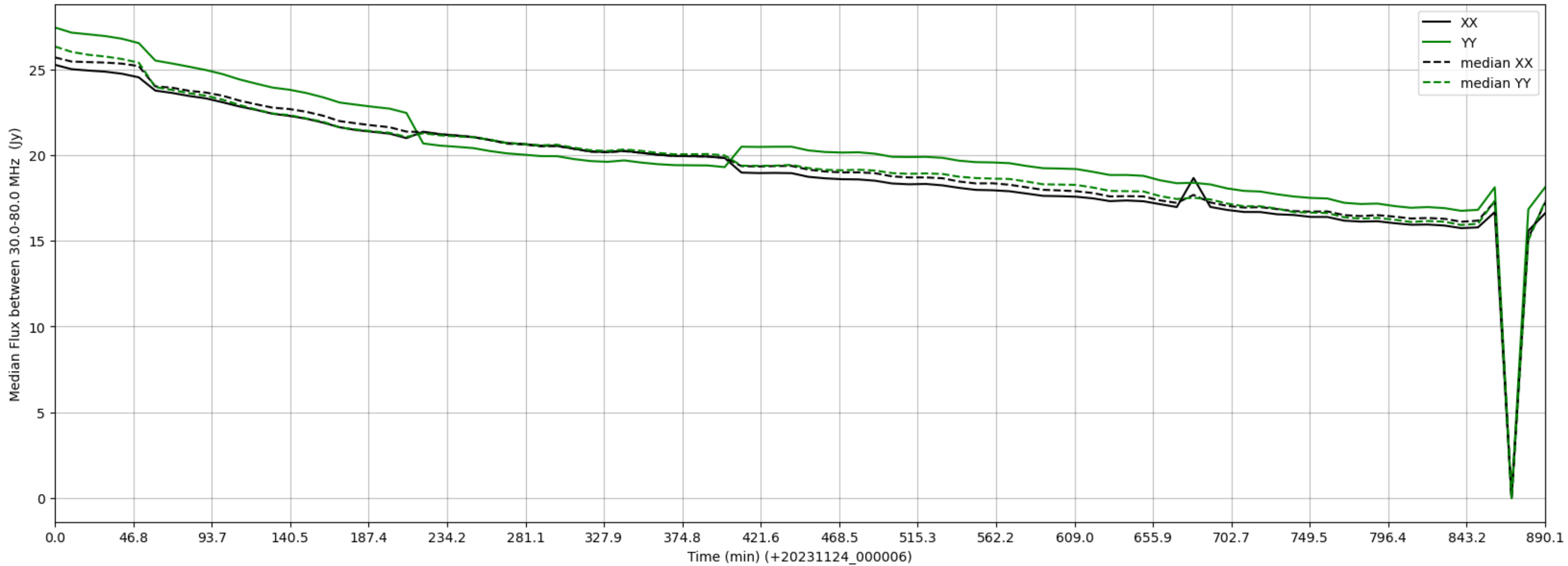
LWA101 - Correlator# 174 - XX FLAGS:Good - YY FLAGS:BadSpecShape
