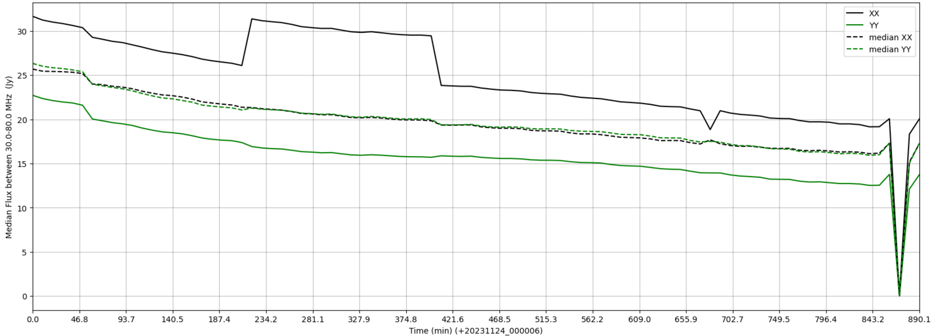
LWA295 - Correlator# 047 - XX FLAGS:HighTimeVar - YY FLAGS:BadSpecShape
