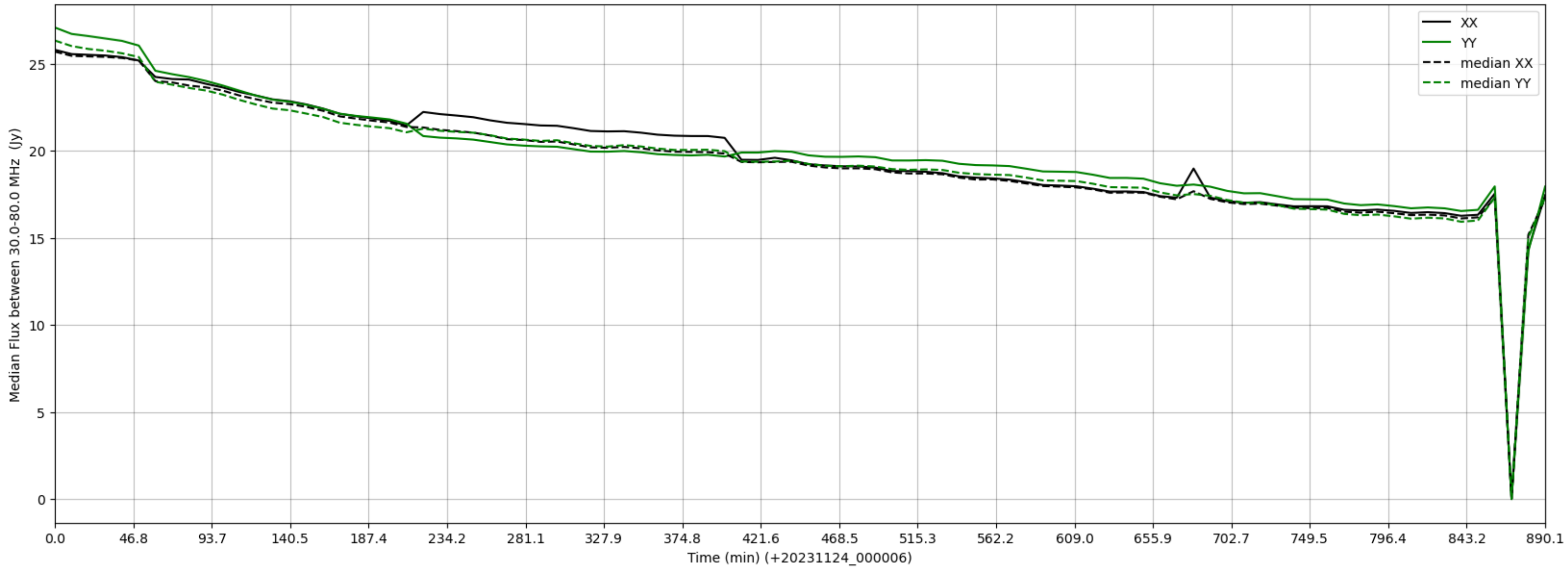
LWA144 - Correlator# 213 - XX FLAGS:Good - YY FLAGS:BadSpecShape
