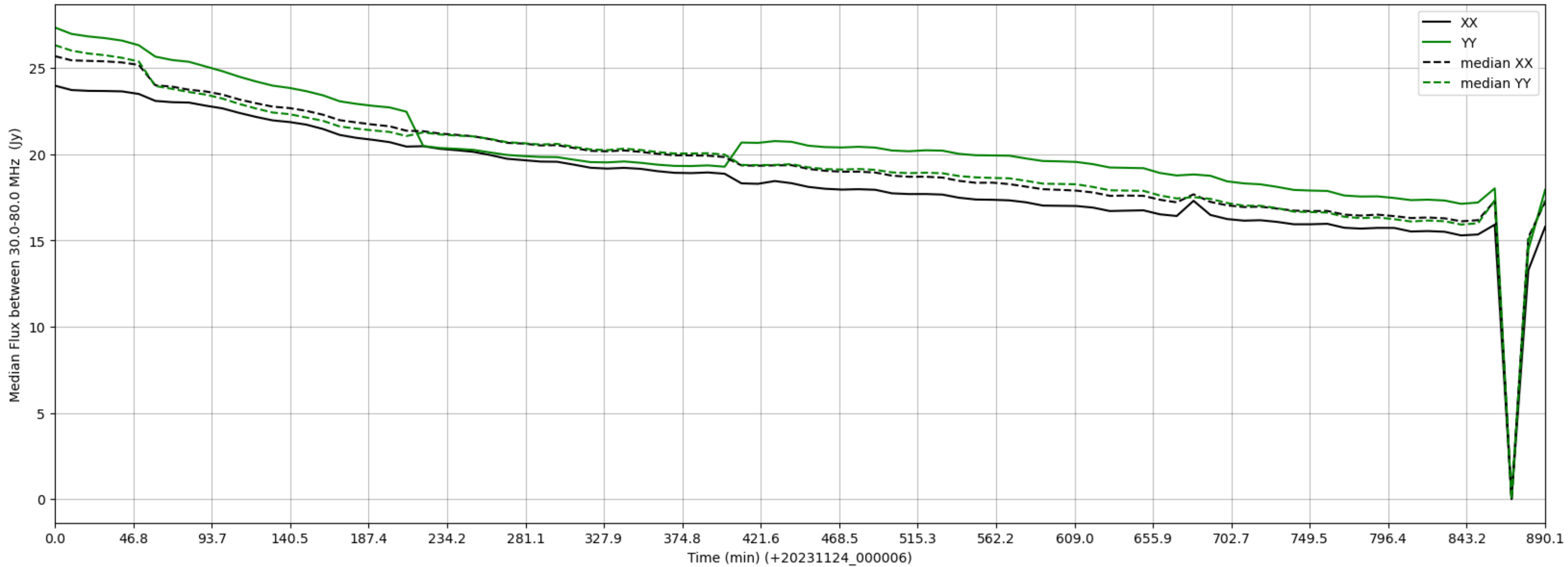
LWA118 - Correlator# 206 - XX FLAGS:Good - YY FLAGS:BadSpecShape
