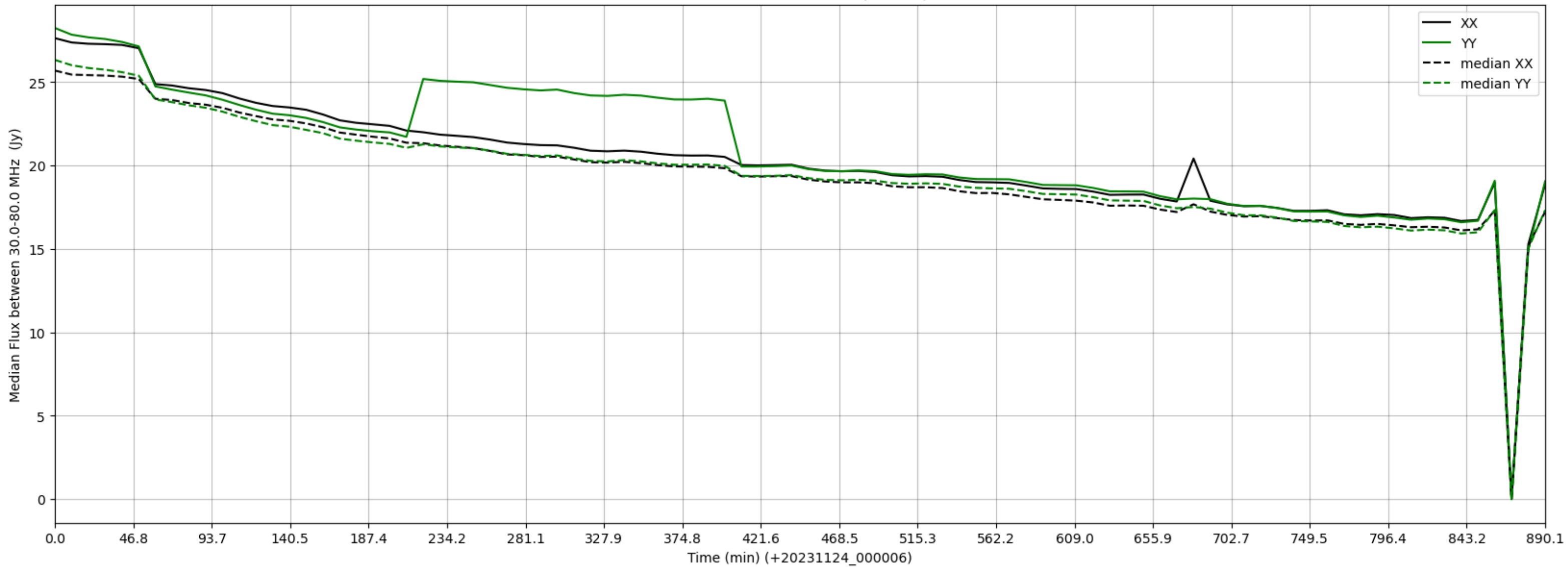
LWA164 - Correlator# 267 - XX FLAGS:BadSpecShape - YY FLAGS:Good
