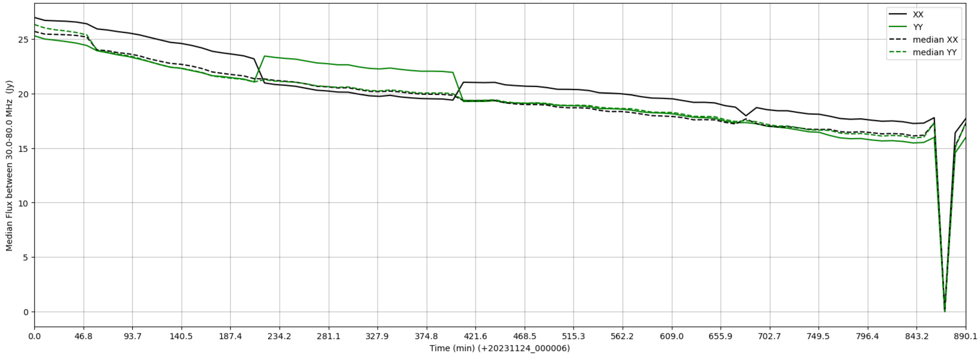
LWA059 - Correlator# 136 - XX FLAGS:BadSpecShape - YY FLAGS:Good
