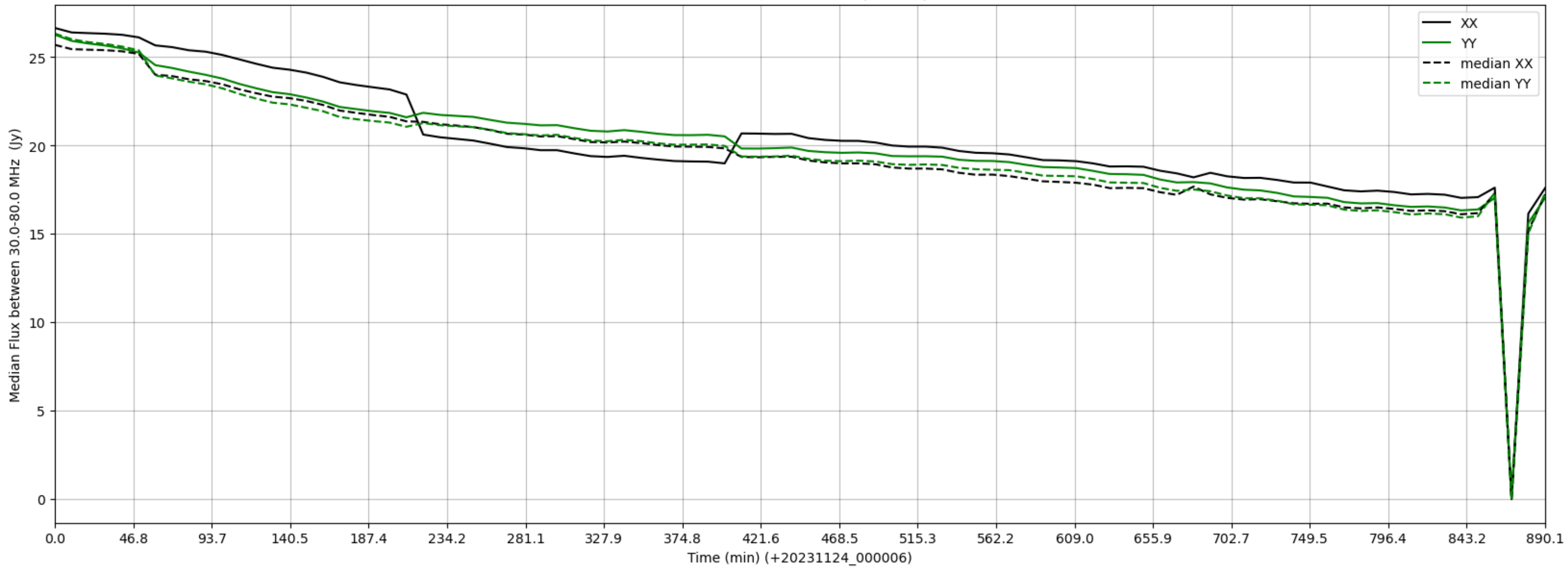
LWA055 - Correlator# 121 - XX FLAGS:BadSpecShape - YY FLAGS:Good
