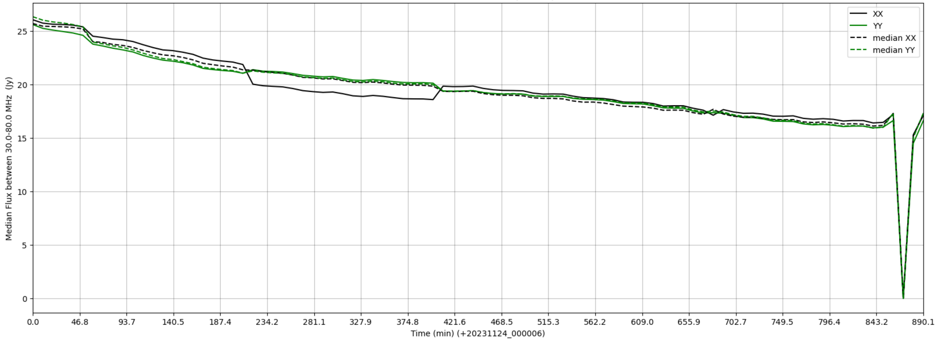
LWA184 - Correlator# 241 - XX FLAGS:BadSpecShape - YY FLAGS:Good
