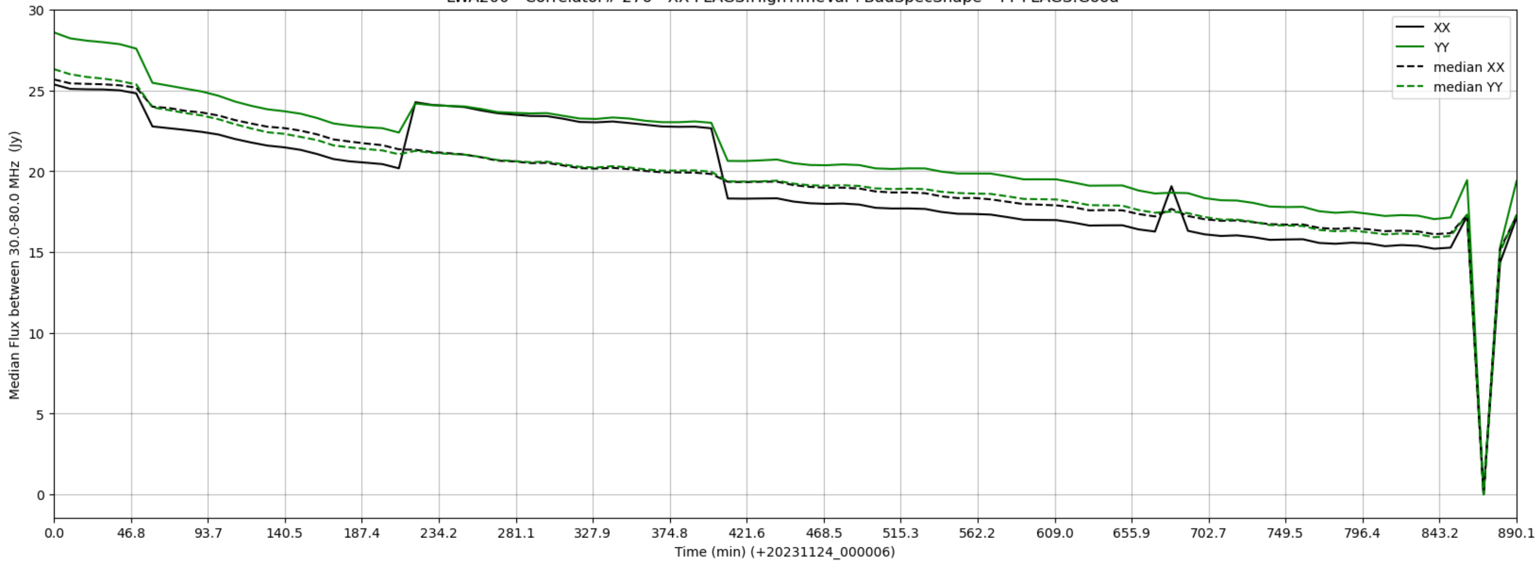
LWA200 - Correlator# 276 - XX FLAGS:HighTimeVar+BadSpecShape - YY FLAGS:Good
