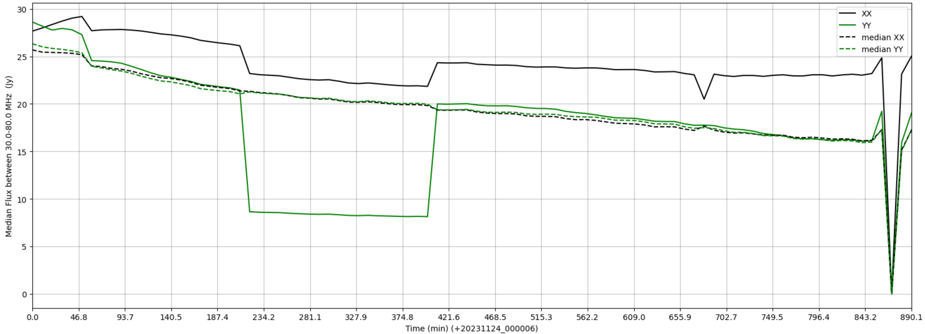
LWA308 - Correlator# 015 - XX FLAGS:Good - YY FLAGS:HighTimeVar
