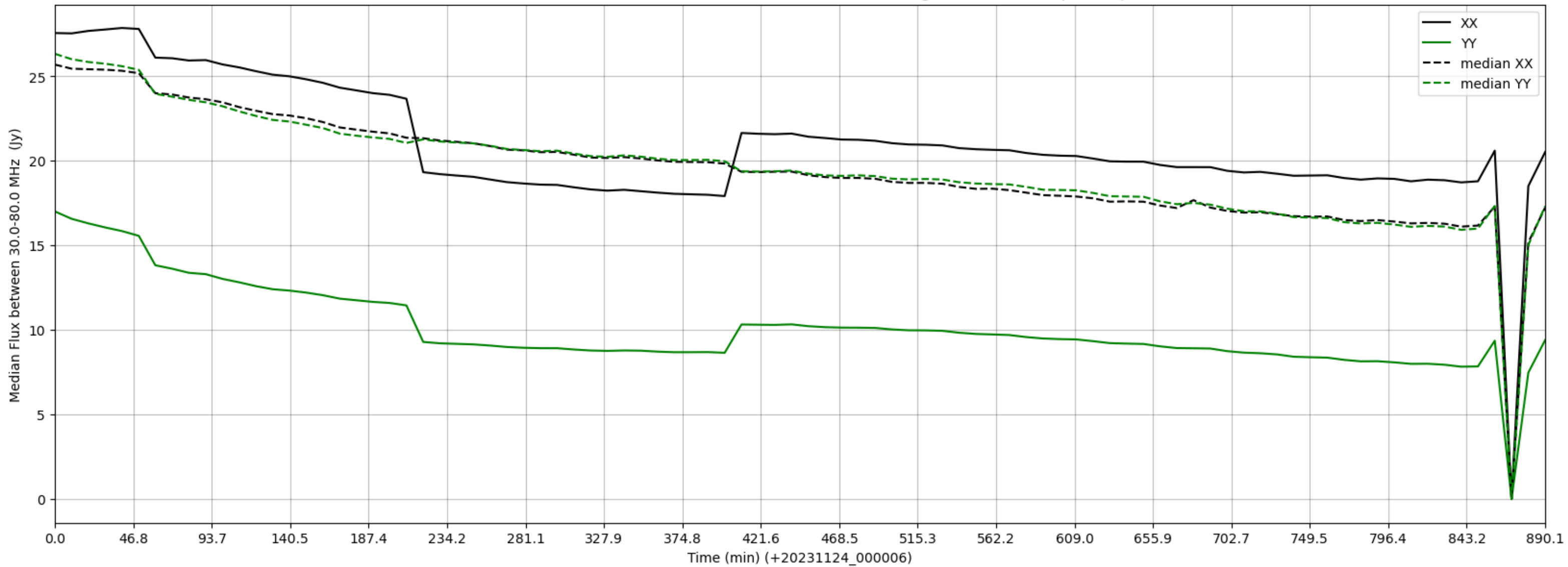
LWA319 - Correlator# 190 - XX FLAGS:Good - YY FLAGS:HighTimeVar+BadSpecShape
