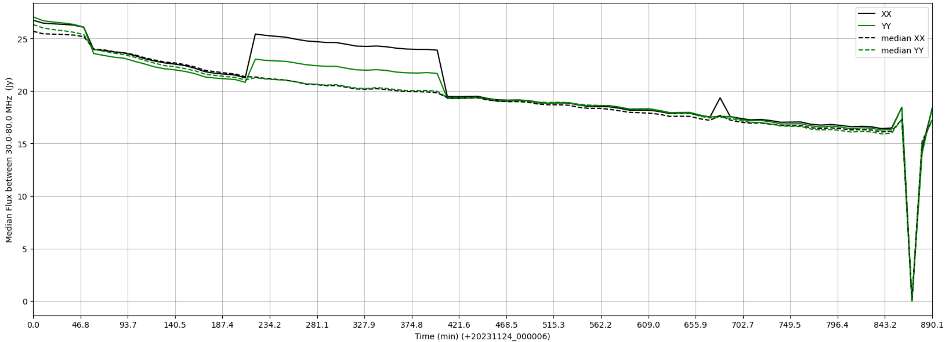
LWA135 - Correlator# 256 - XX FLAGS:HighTimeVar+BadSpecShape - YY FLAGS:Good
