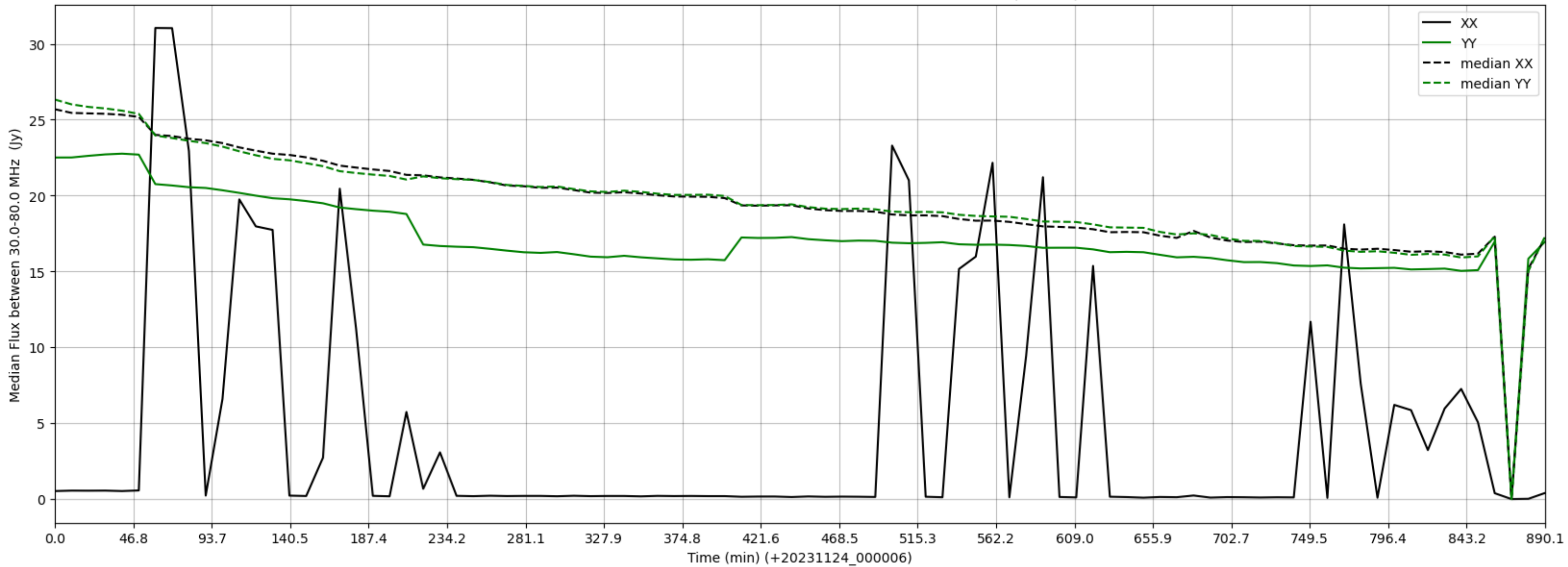
LWA310 - Correlator# 017 - XX FLAGS:LowFlux - YY FLAGS:BadSpecShape
