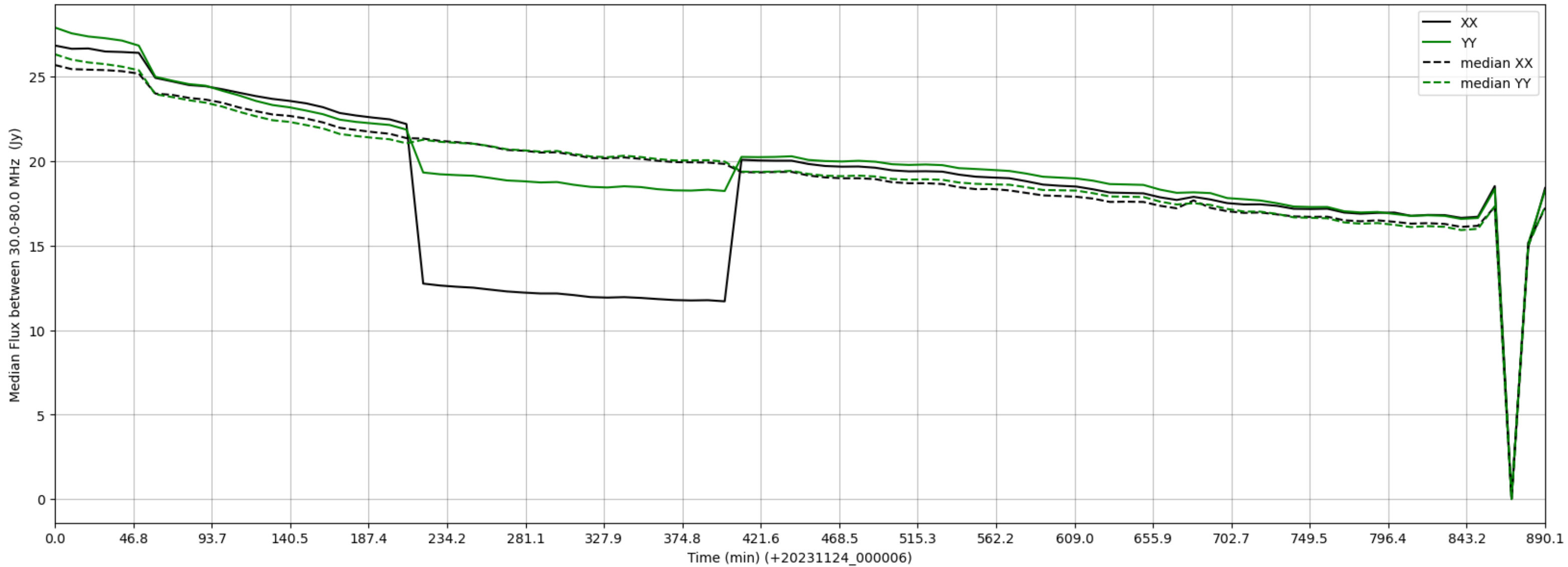
LWA324 - Correlator# 122 - XX FLAGS:HighTimeVar - YY FLAGS:BadSpecShape
