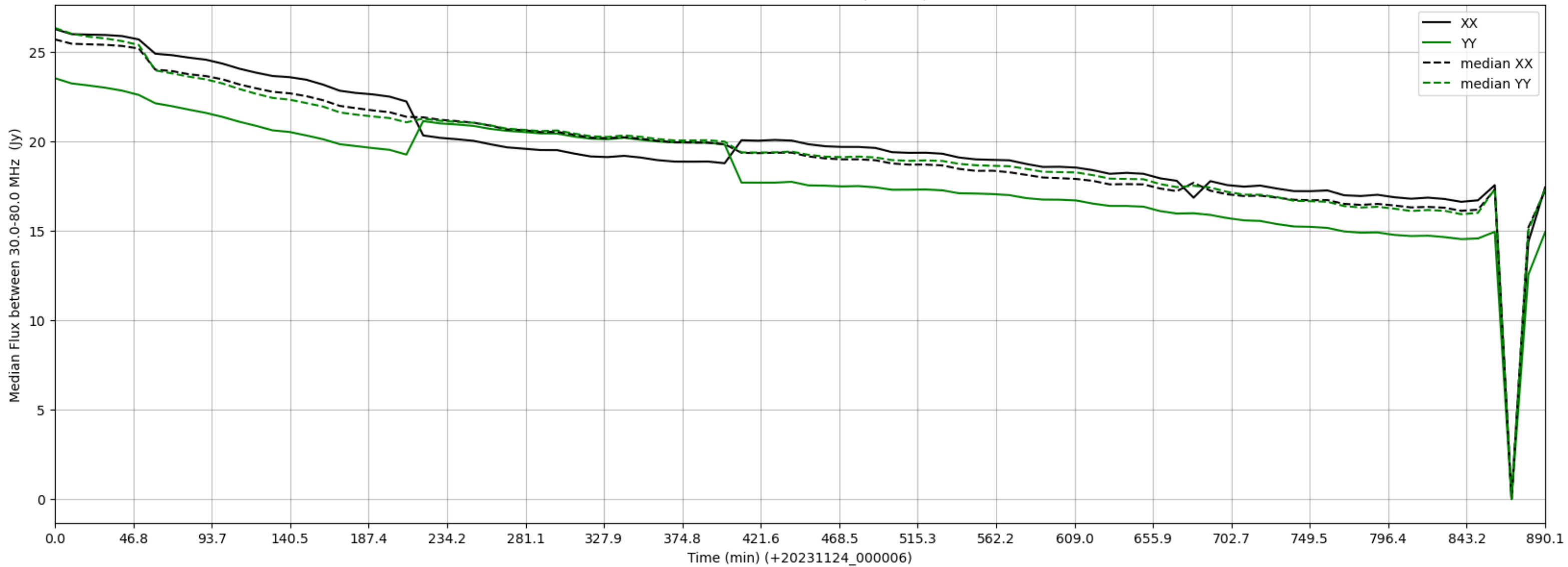
LWA125 - Correlator# 227 - XX FLAGS:BadSpecShape - YY FLAGS:Good
