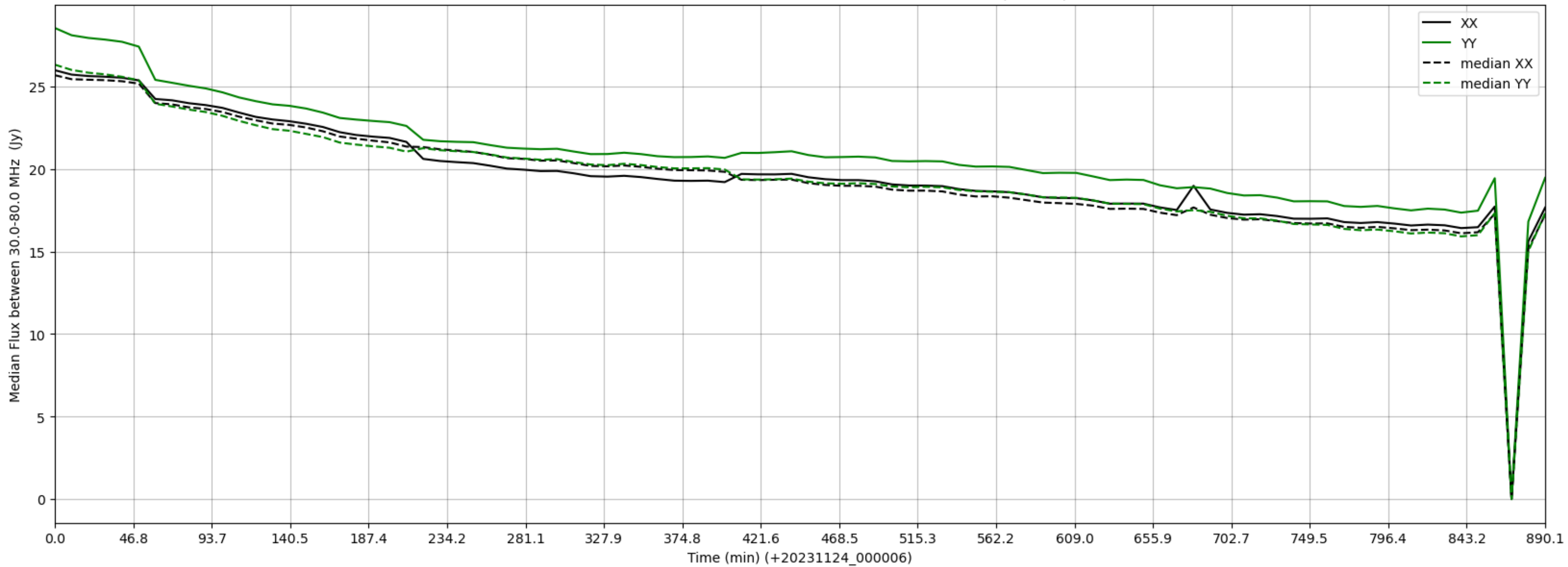
LWA166 - Correlator# 269 - XX FLAGS:Good - YY FLAGS:BadSpecShape
