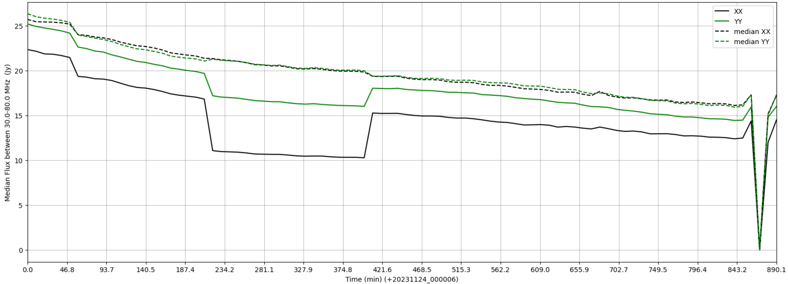
LWA351 - Correlator# 060 - XX FLAGS:HighTimeVar - YY FLAGS:BadSpecShape
