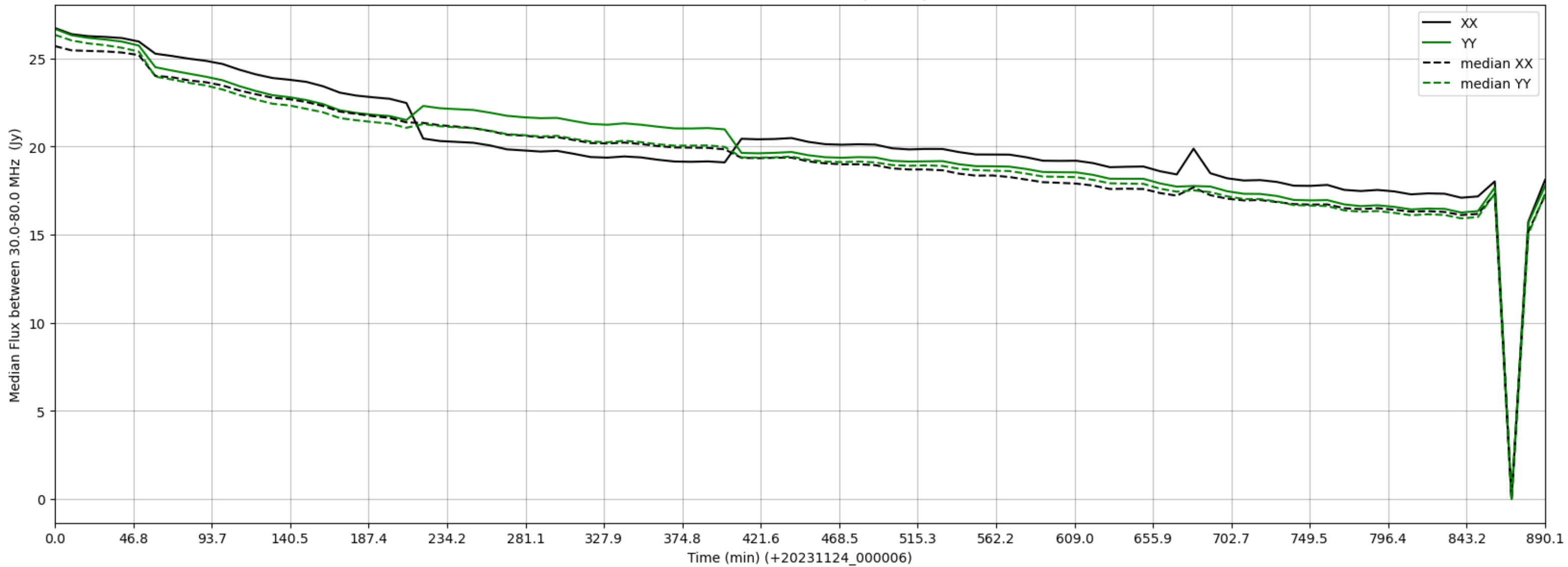
LWA242 - Correlator# 339 - XX FLAGS:BadSpecShape - YY FLAGS:Good
