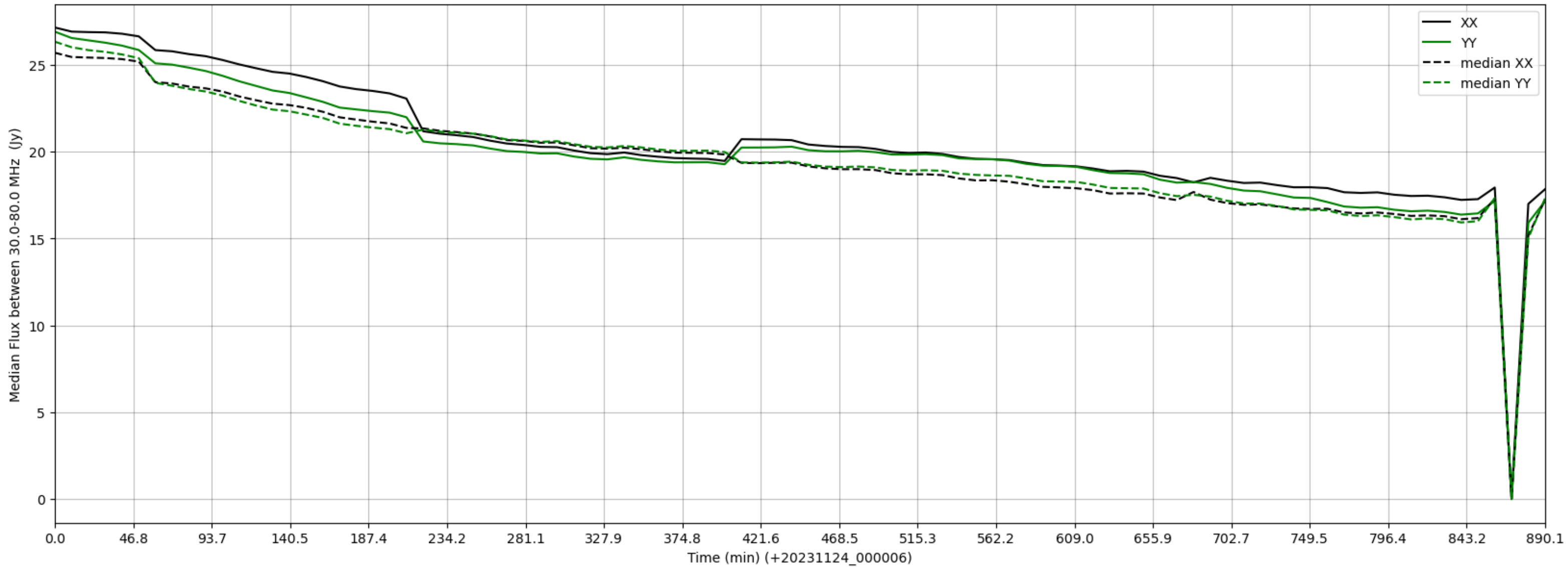
LWA031 - Correlator# 131 - XX FLAGS:BadSpecShape - YY FLAGS:BadSpecShape
