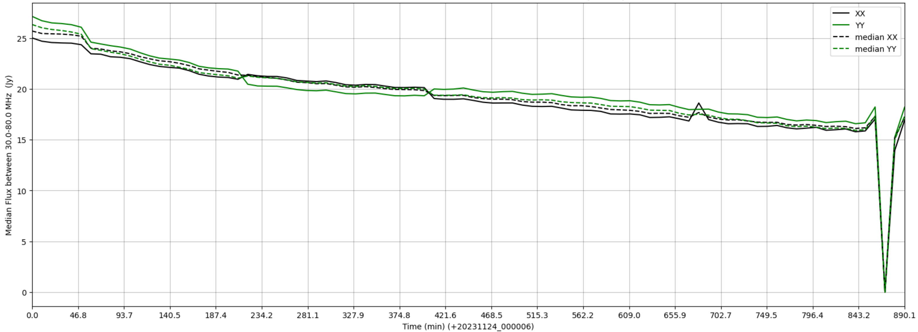
LWA141 - Correlator# 263 - XX FLAGS:Good - YY FLAGS:BadSpecShape
