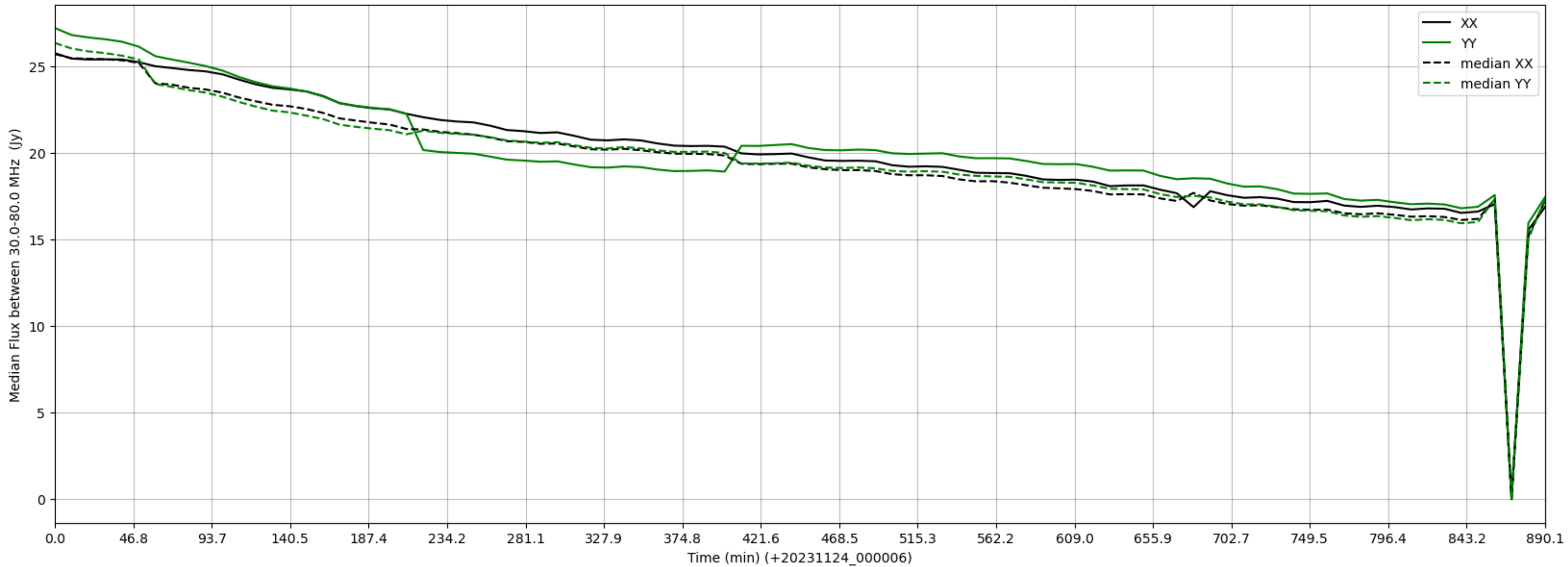
LWA032 - Correlator# 130 - XX FLAGS:Good - YY FLAGS:BadSpecShape
