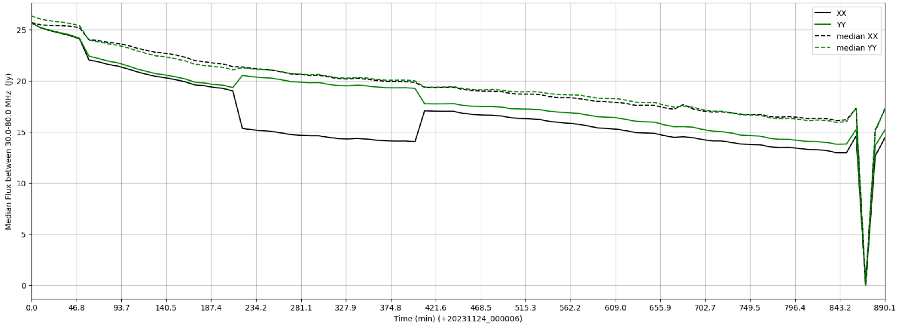
LWA360 - Correlator# 062 - XX FLAGS:HighTimeVar+BadSpecShape - YY FLAGS:Good
