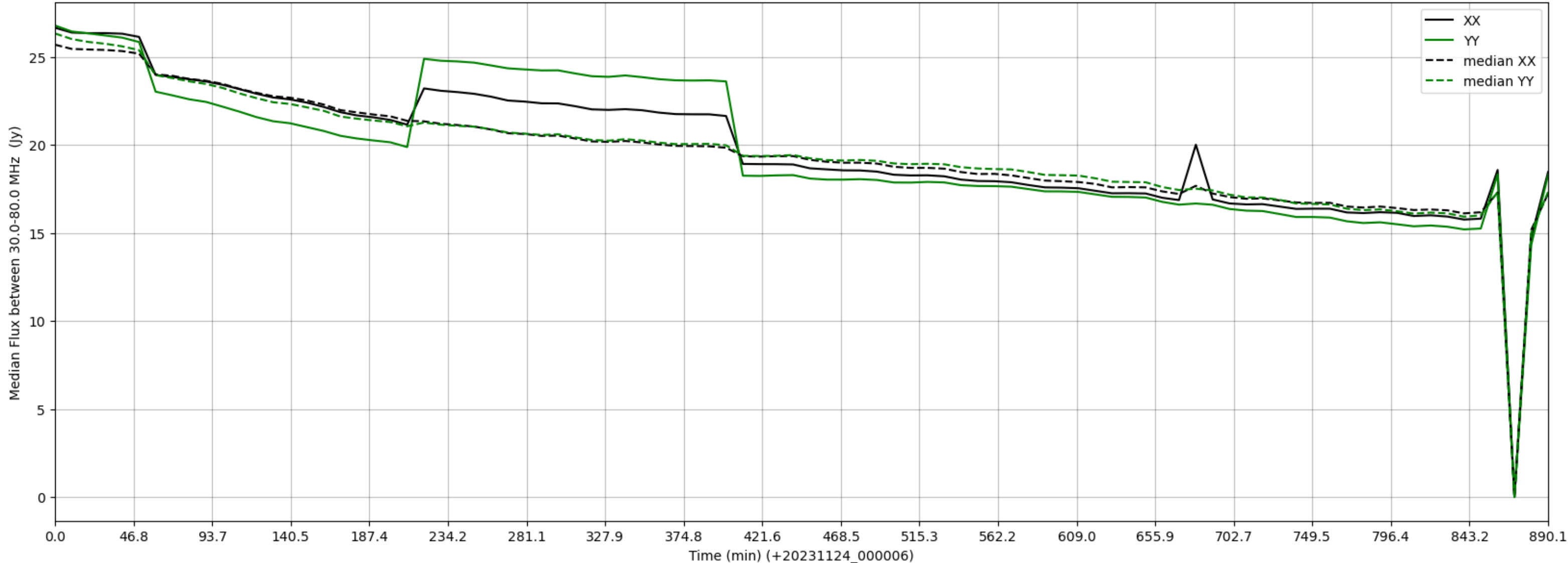
LWA005 - Correlator# 069 - XX FLAGS:BadSpecShape - YY FLAGS:HighTimeVar+BadSpecShape
