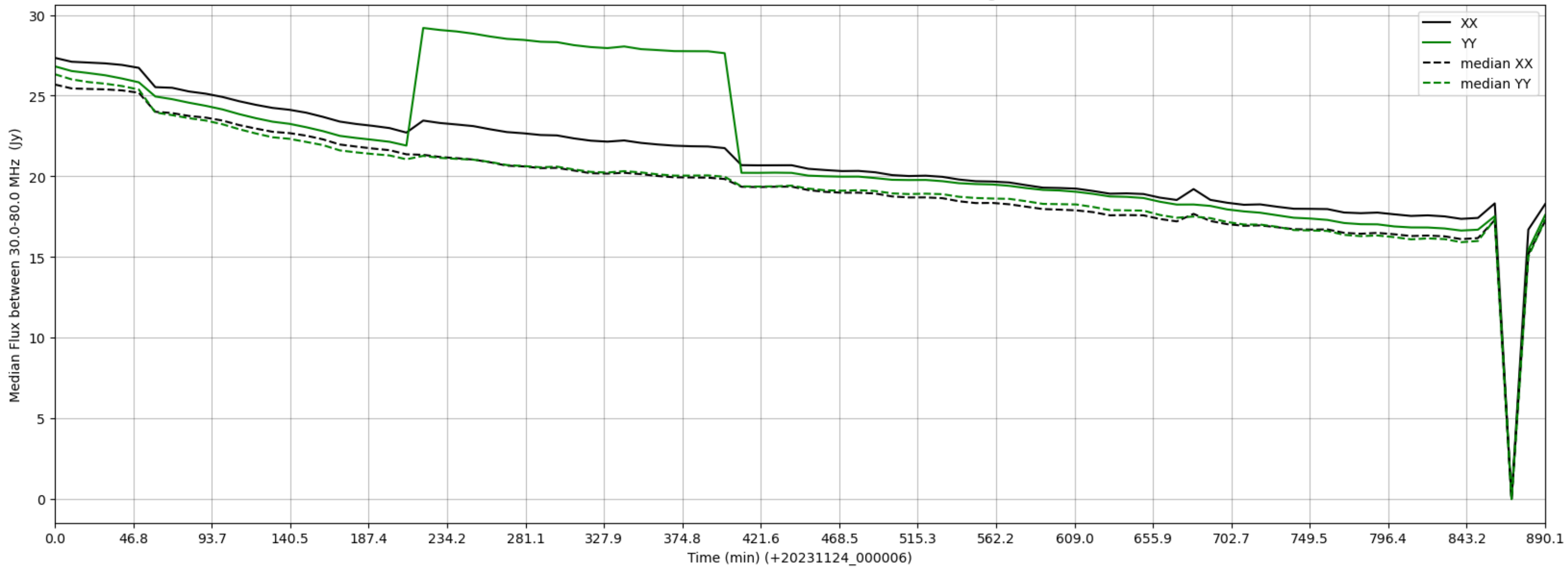
LWA211 - Correlator# 327 - XX FLAGS:Good - YY FLAGS:HighTimeVar
