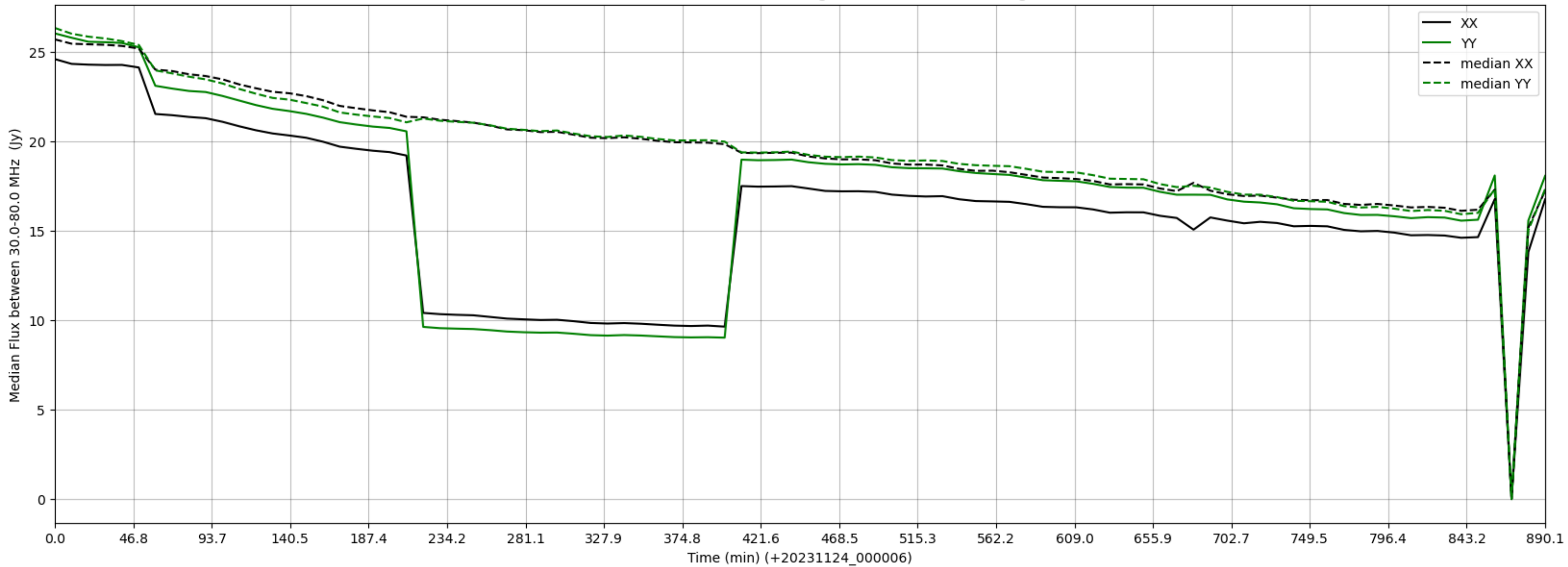
LWA312 - Correlator# 019 - XX FLAGS:HighTimeVar - YY FLAGS:HighTimeVar
