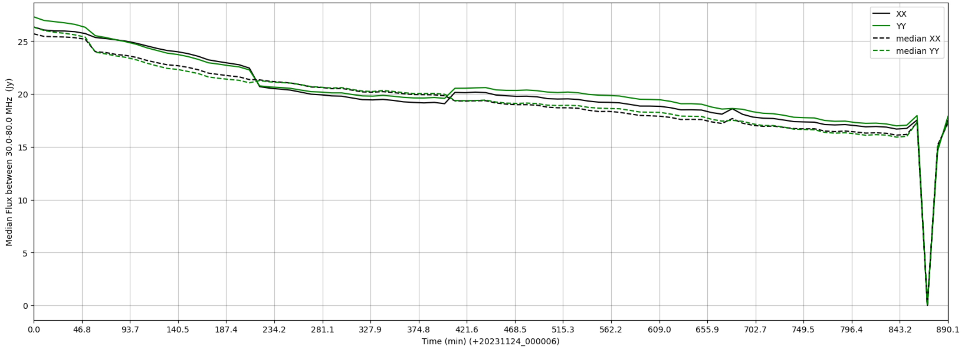
LWA114 - Correlator# 202 - XX FLAGS:Good - YY FLAGS:BadSpecShape
