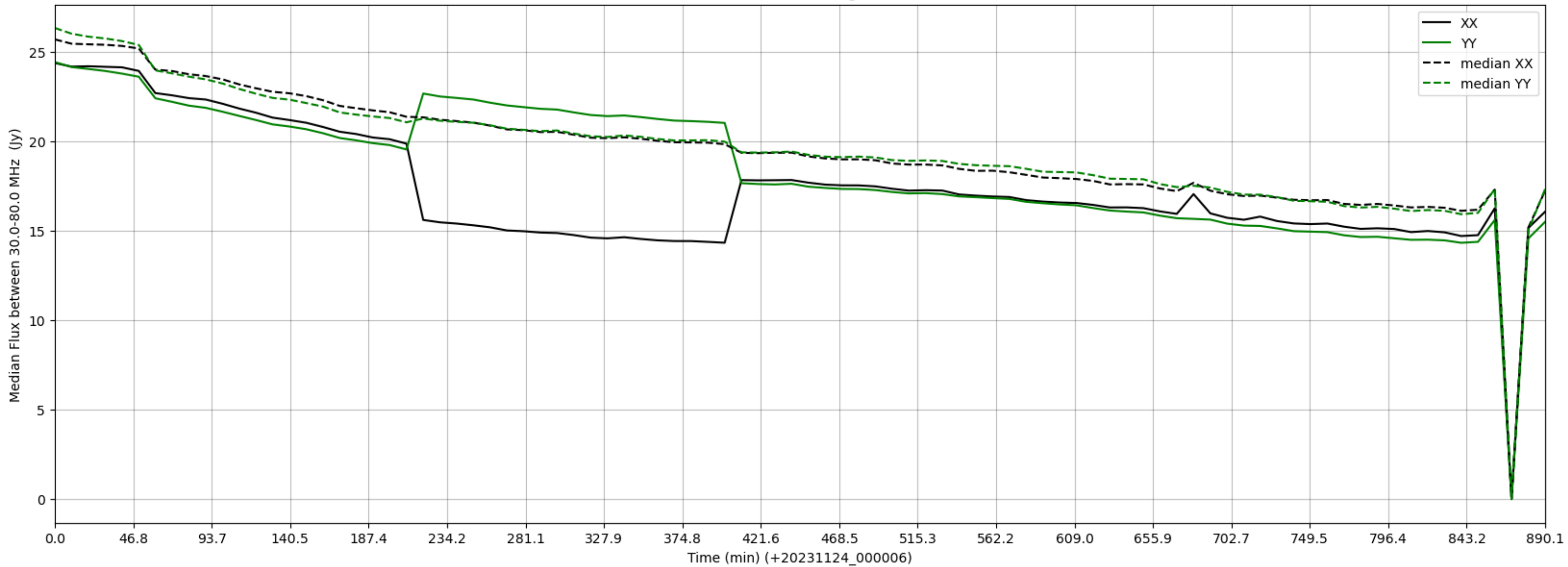
LWA341 - Correlator# 029 - XX FLAGS:HighTimeVar - YY FLAGS:Good
