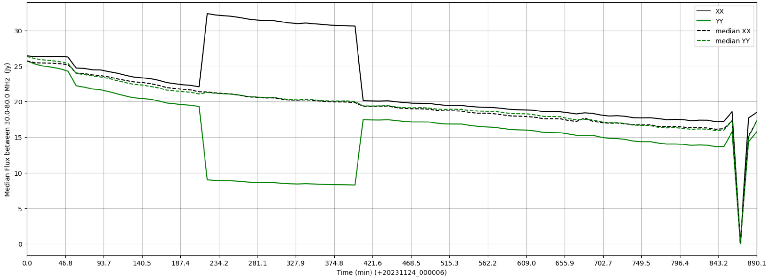
LWA348 - Correlator# 124 - XX FLAGS:HighTimeVar - YY FLAGS:HighTimeVar
