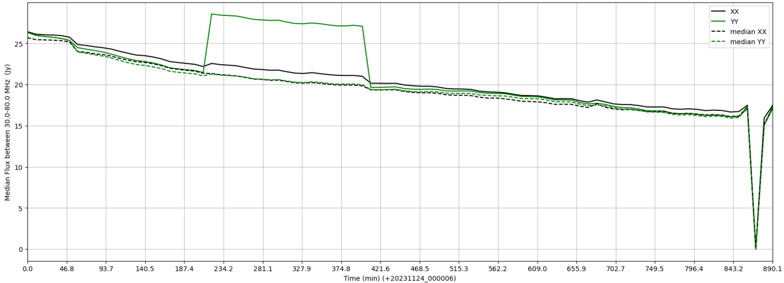
LWA217 - Correlator# 333 - XX FLAGS:Good - YY FLAGS:HighTimeVar
