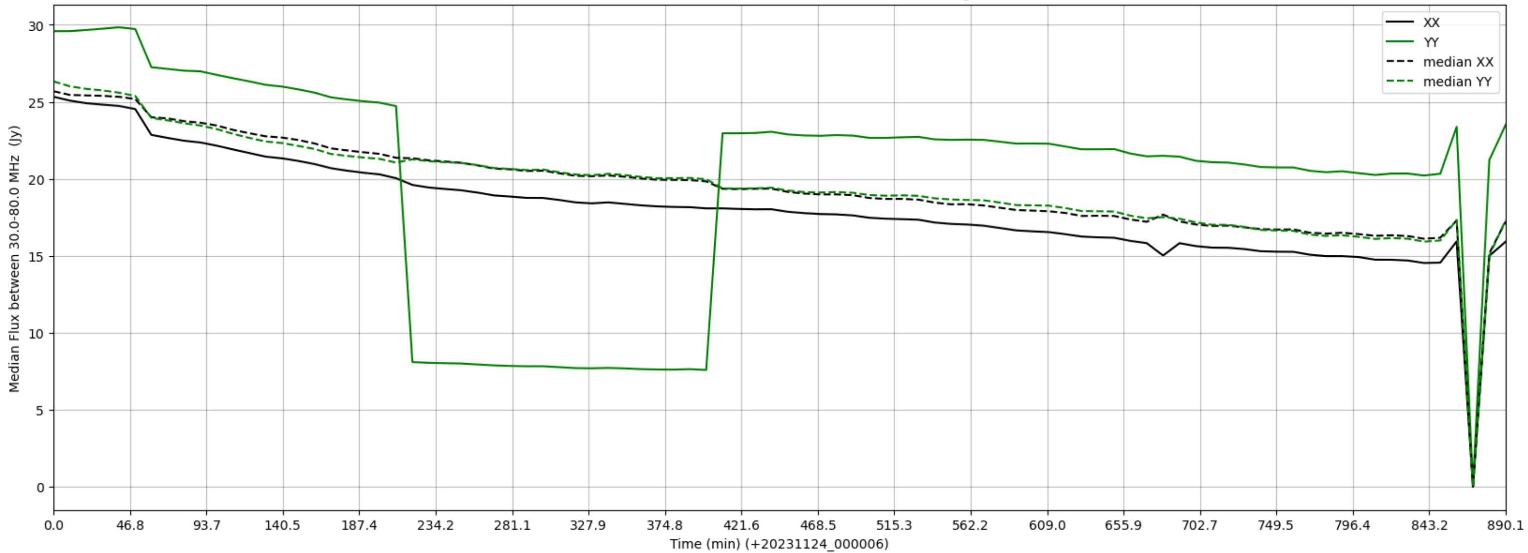
LWA311 - Correlator# 016 - XX FLAGS:Good - YY FLAGS:HighTimeVar
