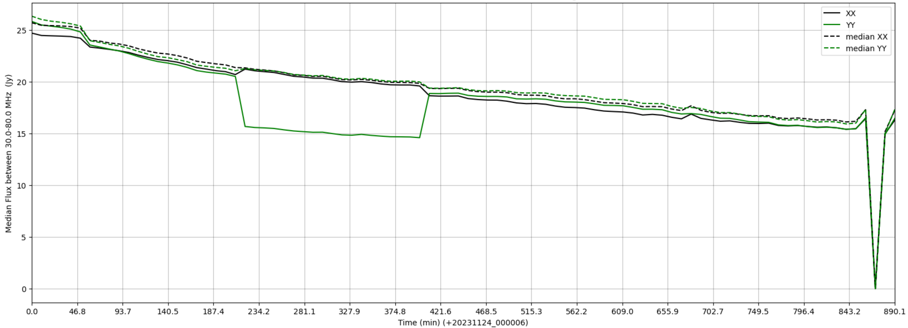
LWA022 - Correlator# 104 - XX FLAGS:Good - YY FLAGS:HighTimeVar
