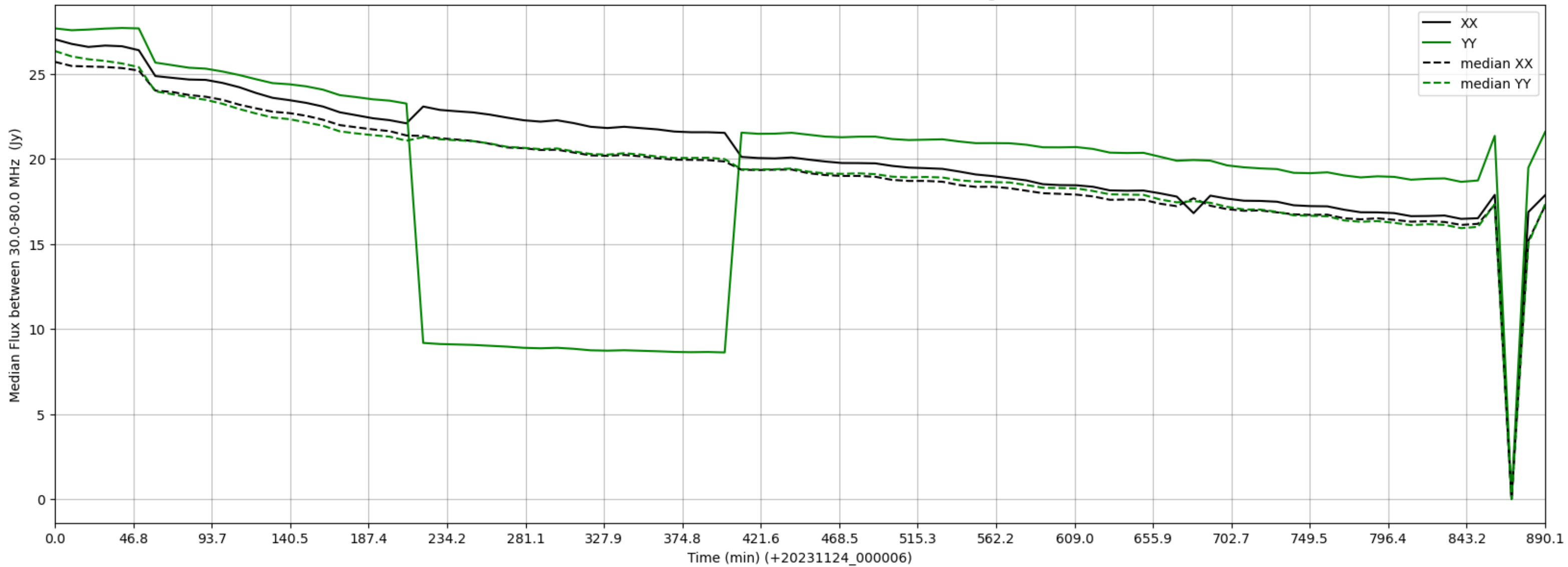
LWA332 - Correlator# 025 - XX FLAGS:Good - YY FLAGS:HighTimeVar
