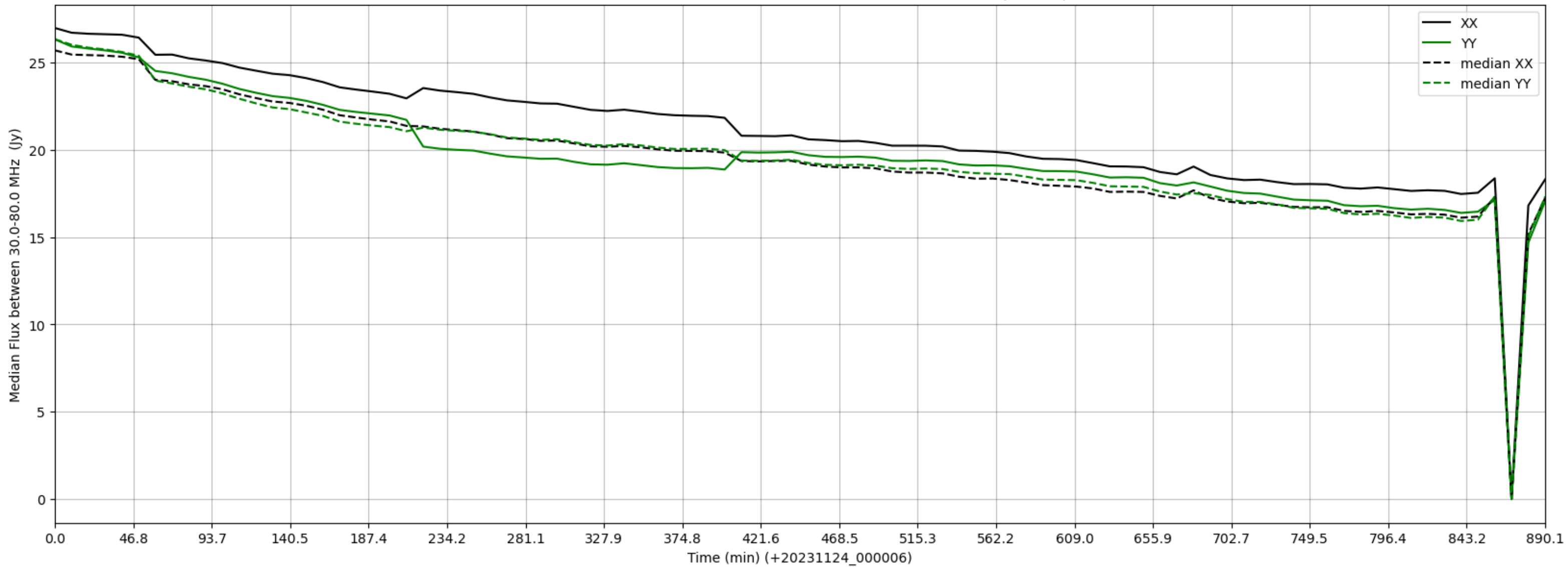
LWA147 - Correlator# 214 - XX FLAGS:Good - YY FLAGS:BadSpecShape
