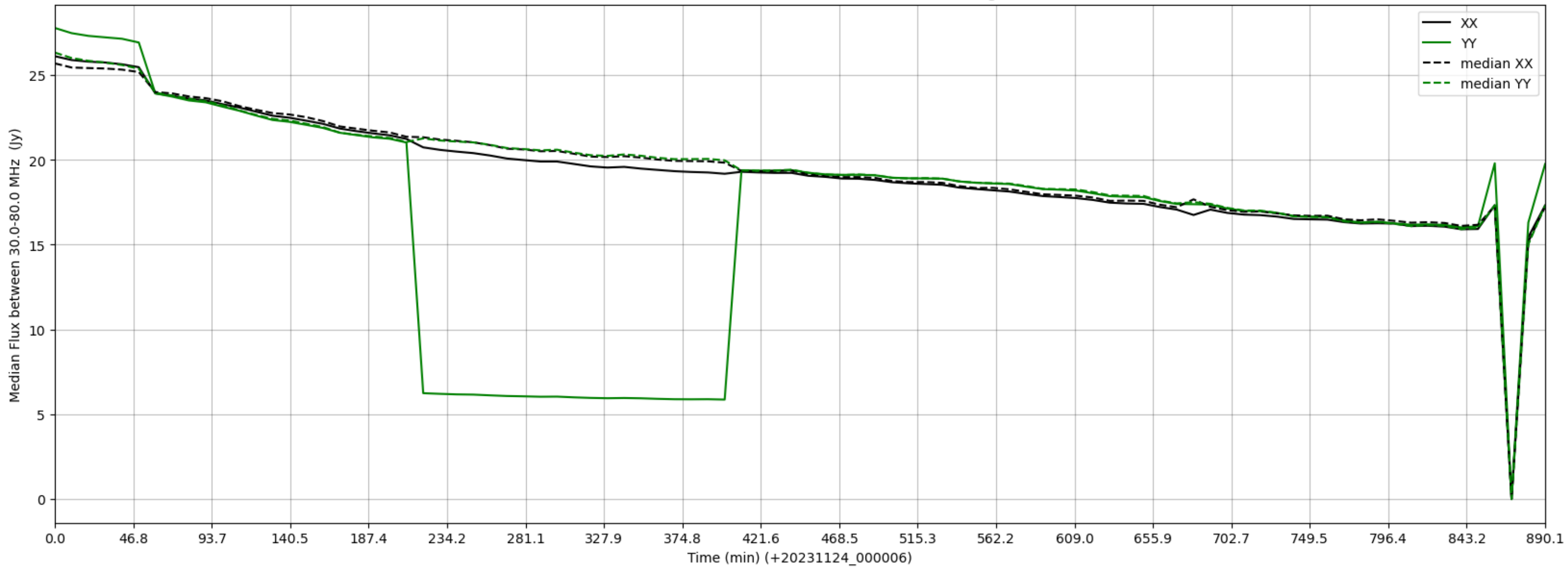
LWA344 - Correlator# 061 - XX FLAGS:Good - YY FLAGS:HighTimeVar
