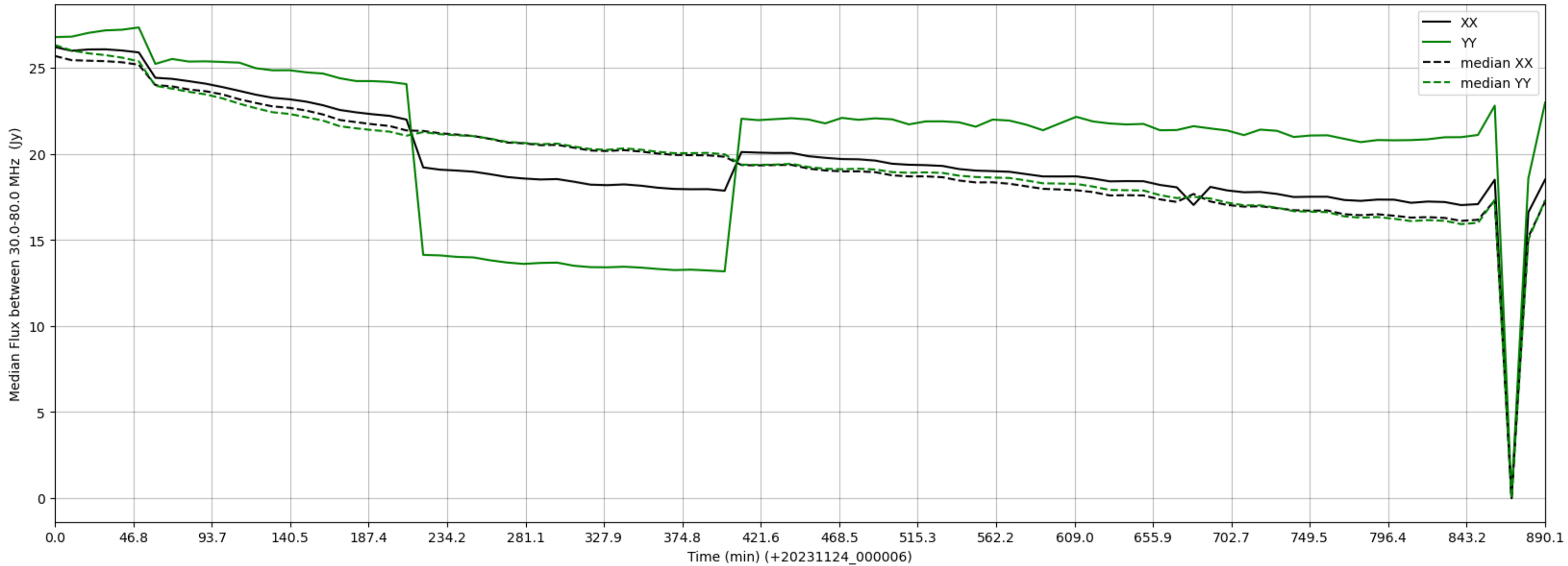
LWA282 - Correlator# 010 - XX FLAGS:BadSpecShape - YY FLAGS:HighTimeVar
