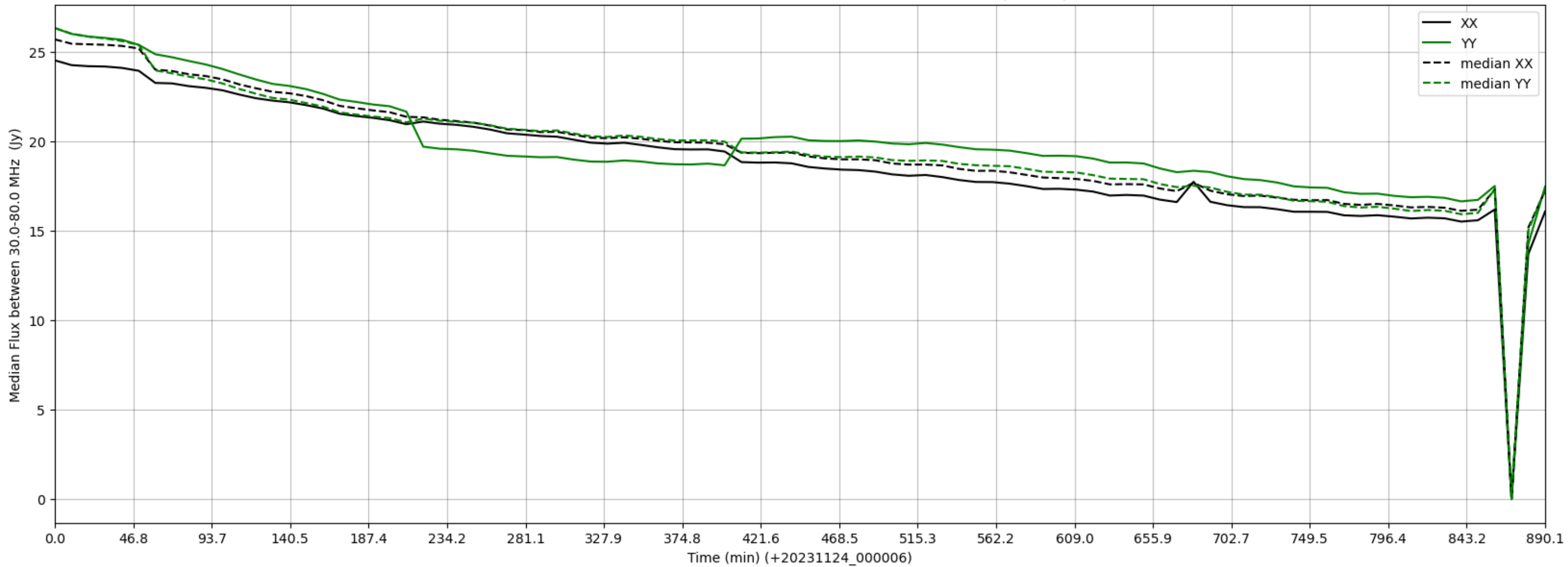
LWA113 - Correlator# 203 - XX FLAGS:Good - YY FLAGS:BadSpecShape
