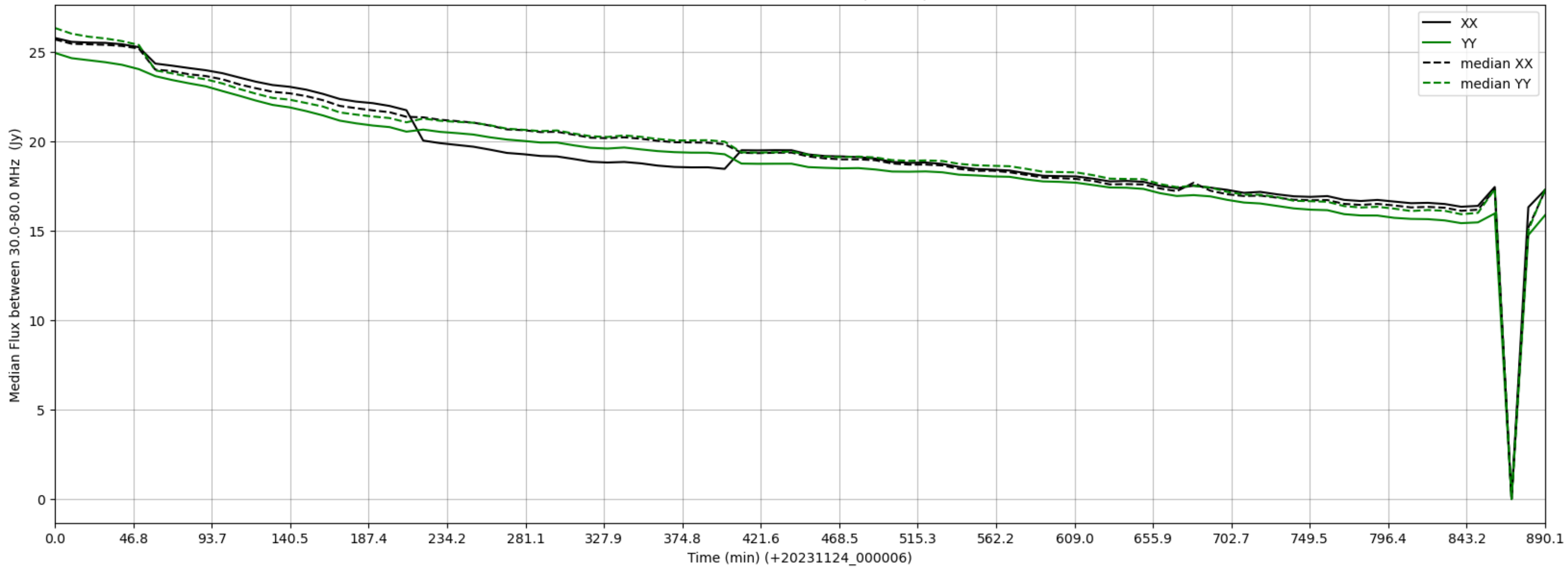
LWA023 - Correlator# 107 - XX FLAGS:BadSpecShape - YY FLAGS:Good
