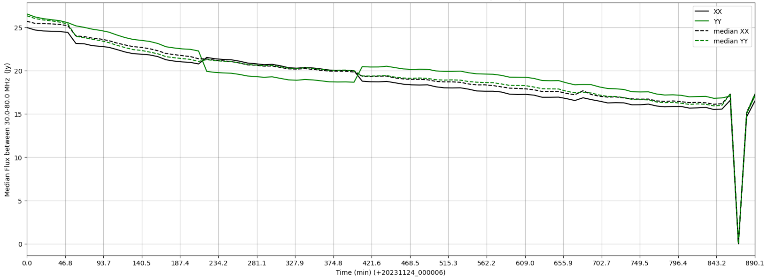
LWA223 - Correlator# 337 - XX FLAGS:Good - YY FLAGS:BadSpecShape
