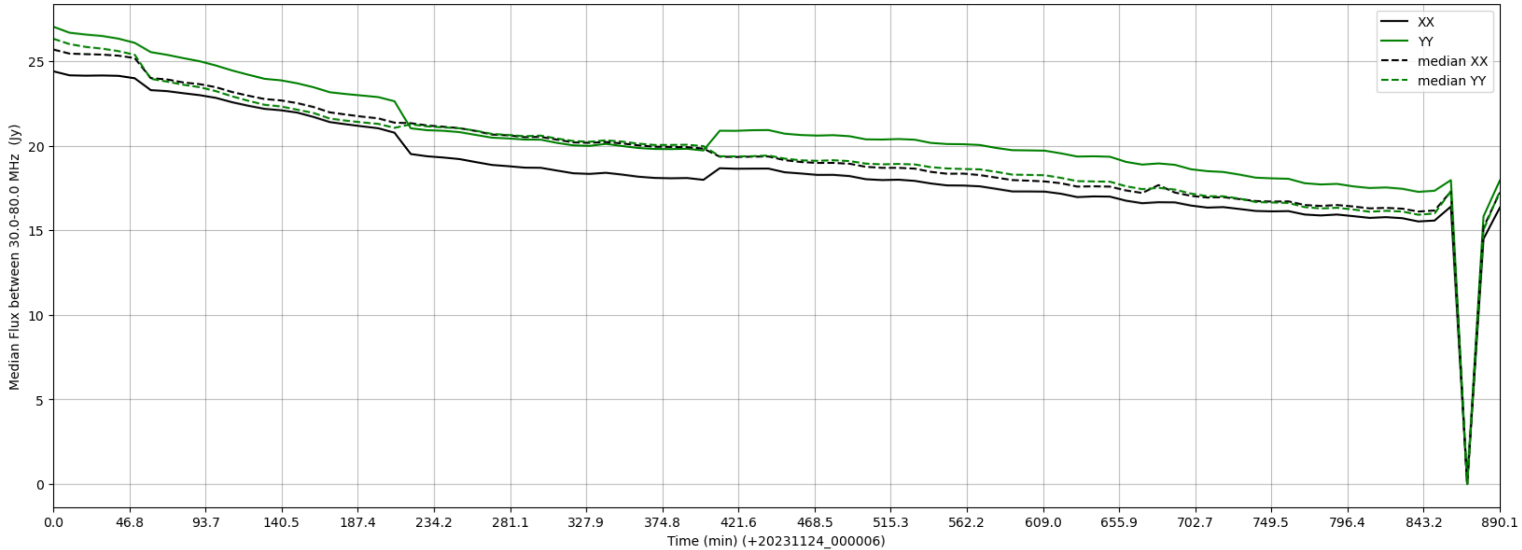
LWA110 - Correlator# 198 - XX FLAGS:Good - YY FLAGS:BadSpecShape
