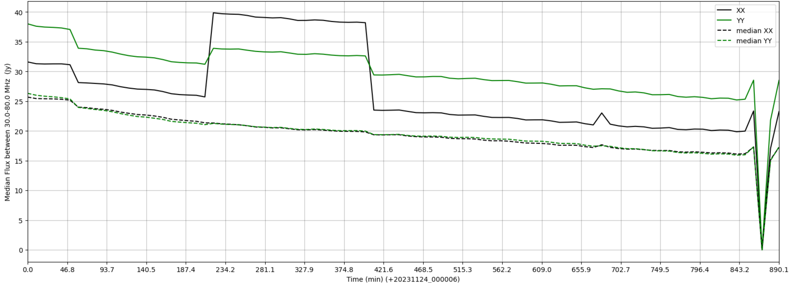
LWA195 - Correlator# 272 - XX FLAGS:HighTimeVar+BadSpecShape - YY FLAGS:BadSpecShape
