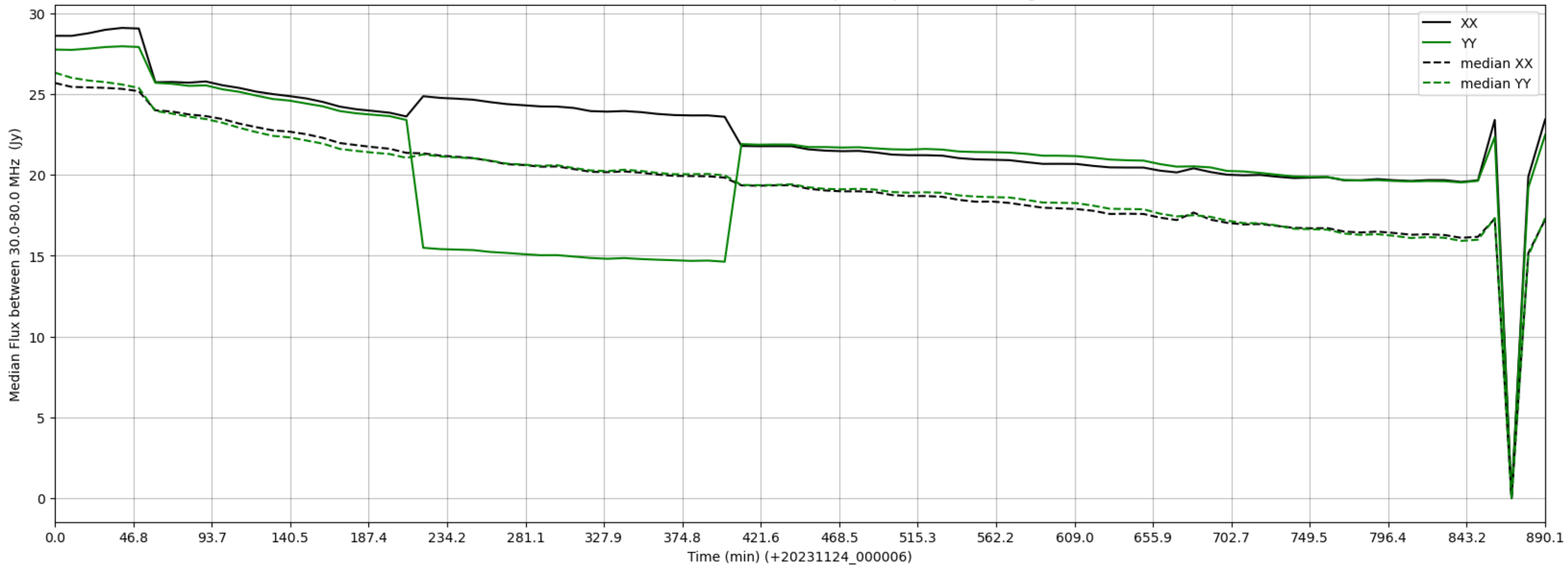
LWA333 - Correlator# 253 - XX FLAGS:BadSpecShape - YY FLAGS:HighTimeVar
