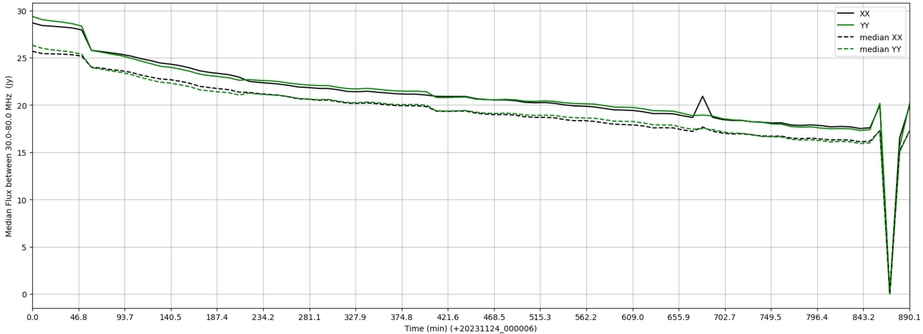
LWA132 - Correlator# 185 - XX FLAGS:BadSpecShape - YY FLAGS:BadSpecShape
