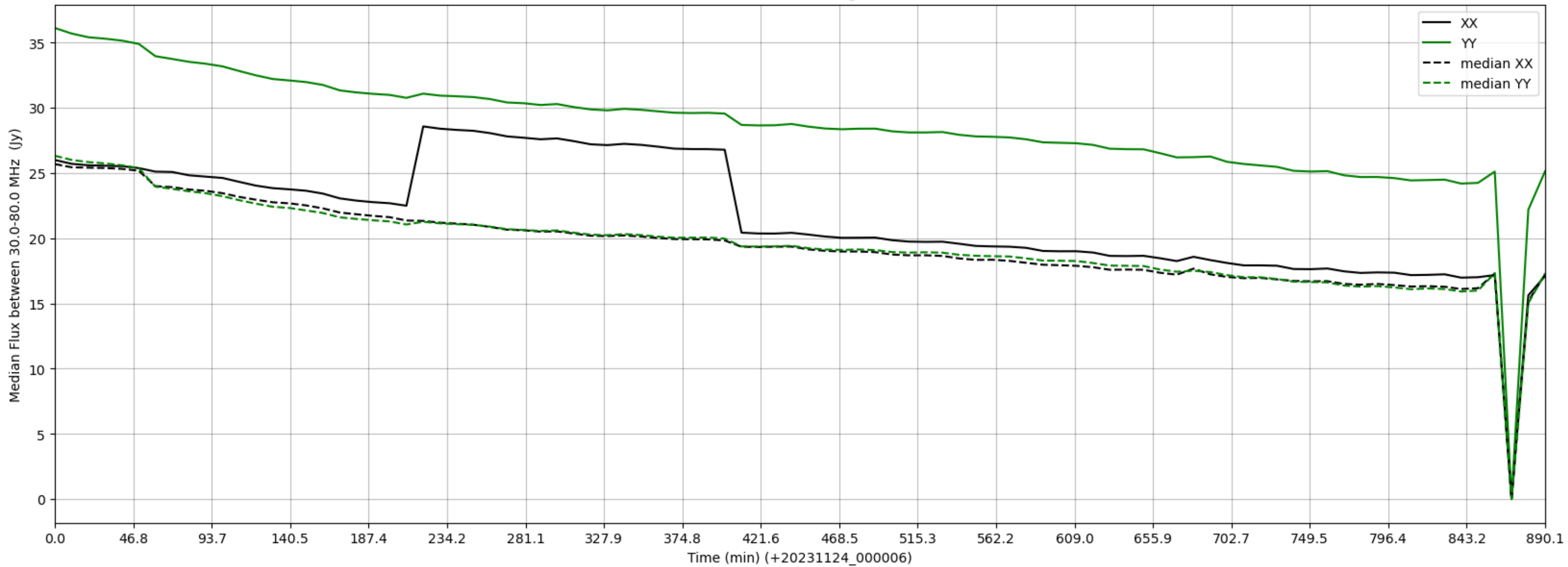
LWA222 - Correlator# 249 - XX FLAGS:HighTimeVar - YY FLAGS:Good
