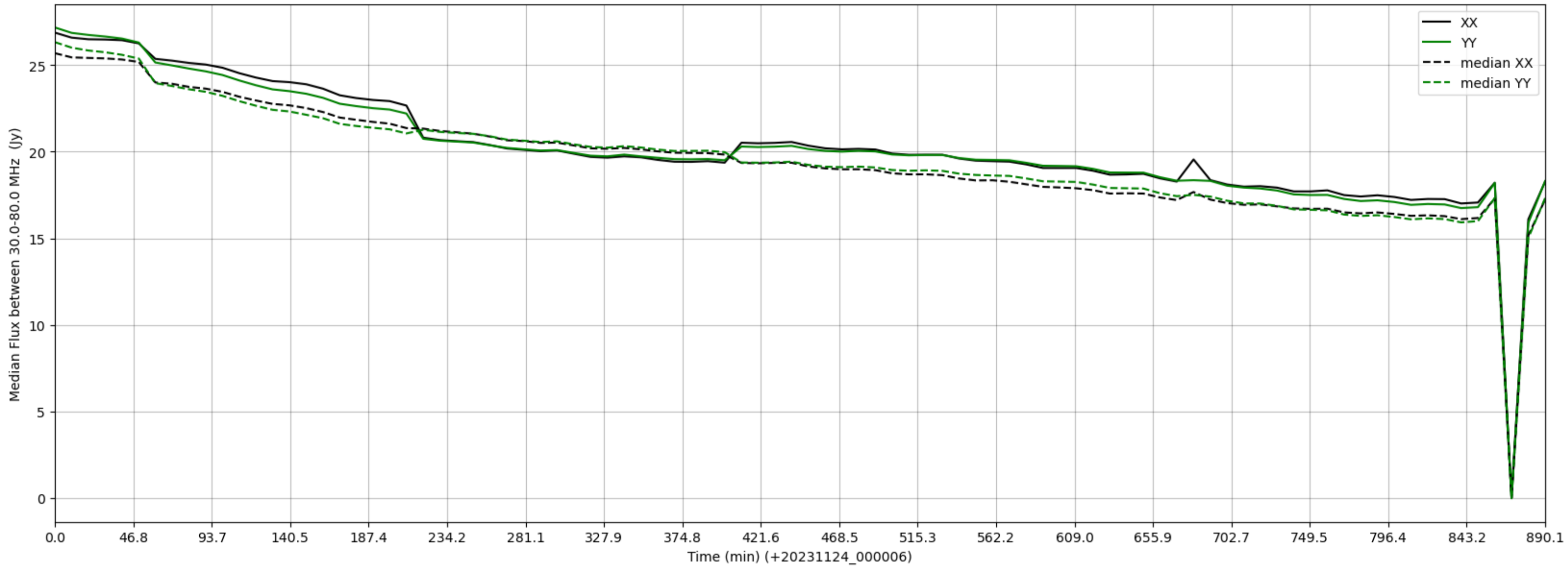
LWA235 - Correlator# 309 - XX FLAGS:BadSpecShape - YY FLAGS:BadSpecShape
