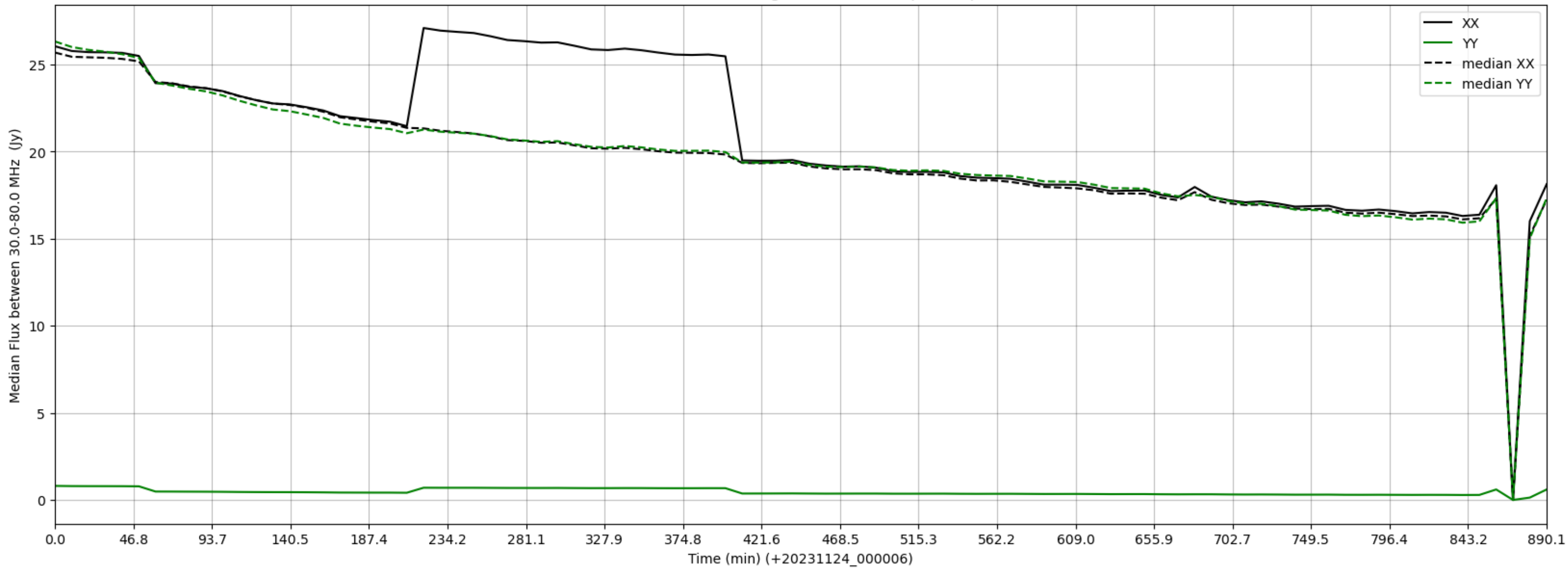
LWA204 - Correlator# 294 - XX FLAGS:HighTimeVar+BadSpecShape - YY FLAGS:LowFlux
