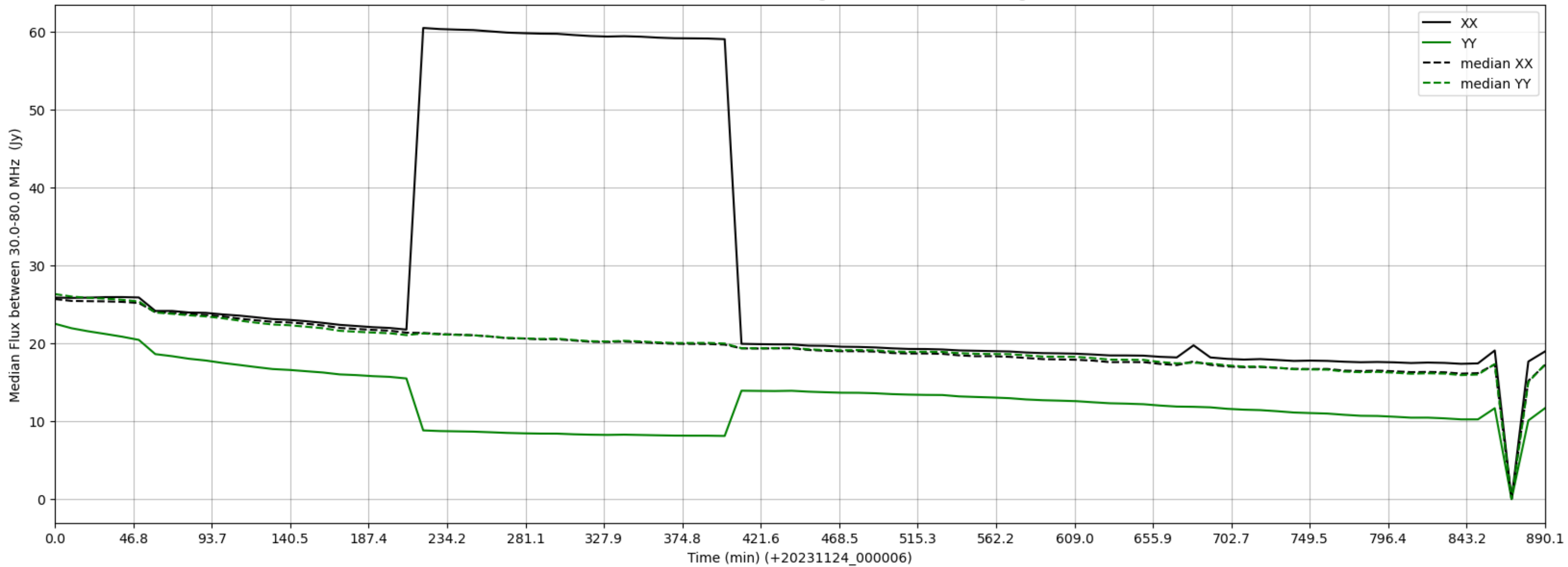
LWA347 - Correlator# 255 - XX FLAGS:HighTimeVar - YY FLAGS:HighTimeVar
