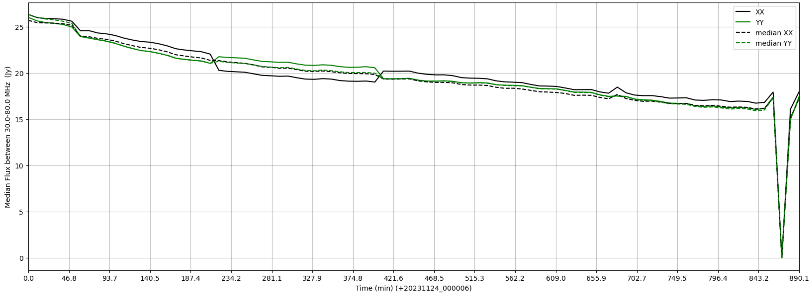
LWA080 - Correlator# 119 - XX FLAGS:BadSpecShape - YY FLAGS:Good
