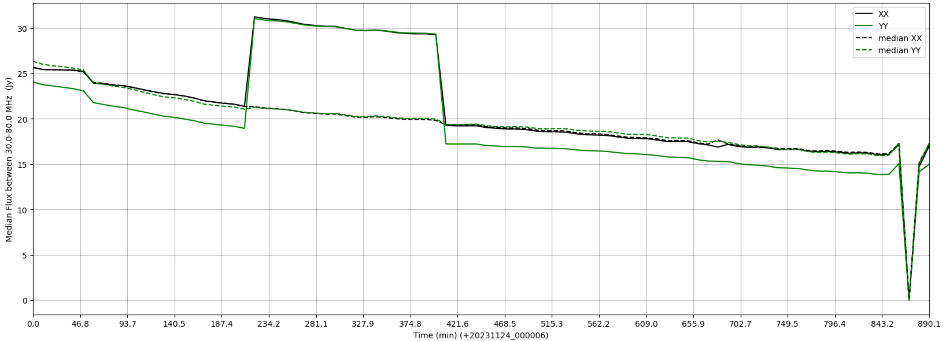
LWA260 - Correlator# 034 - XX FLAGS:HighTimeVar - YY FLAGS:HighTimeVar
