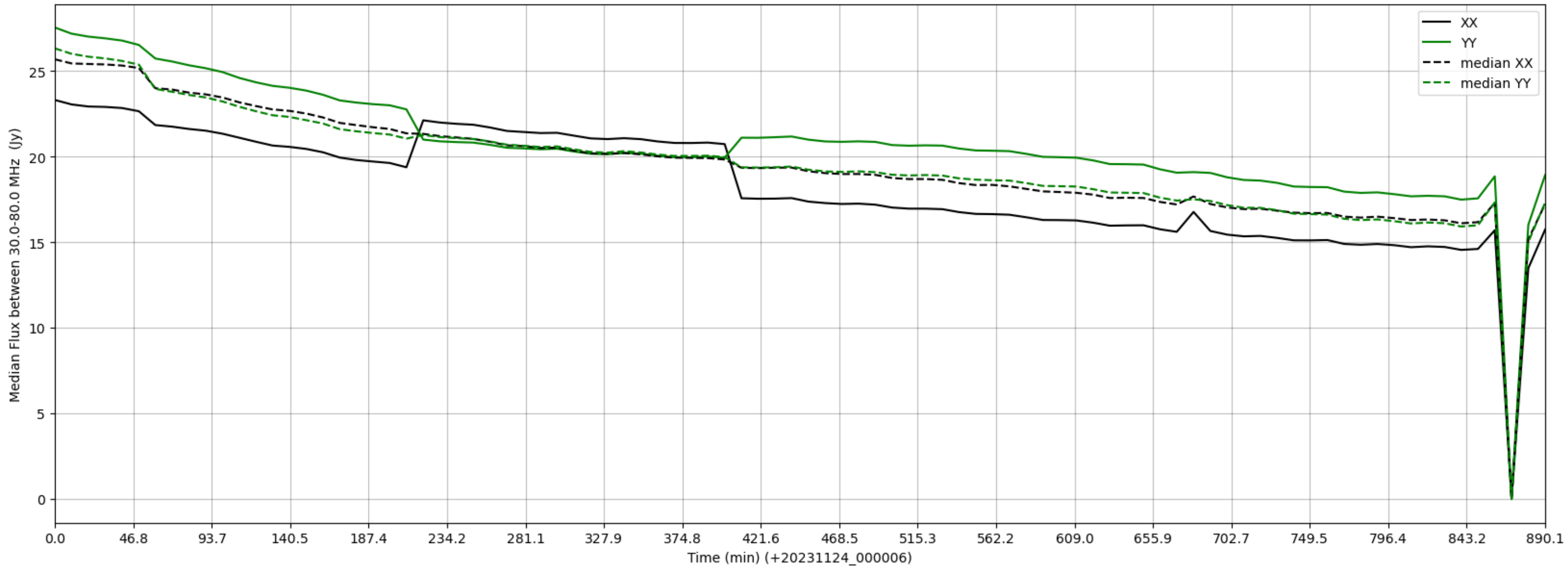
LWA206 - Correlator# 296 - XX FLAGS:Good - YY FLAGS:BadSpecShape
