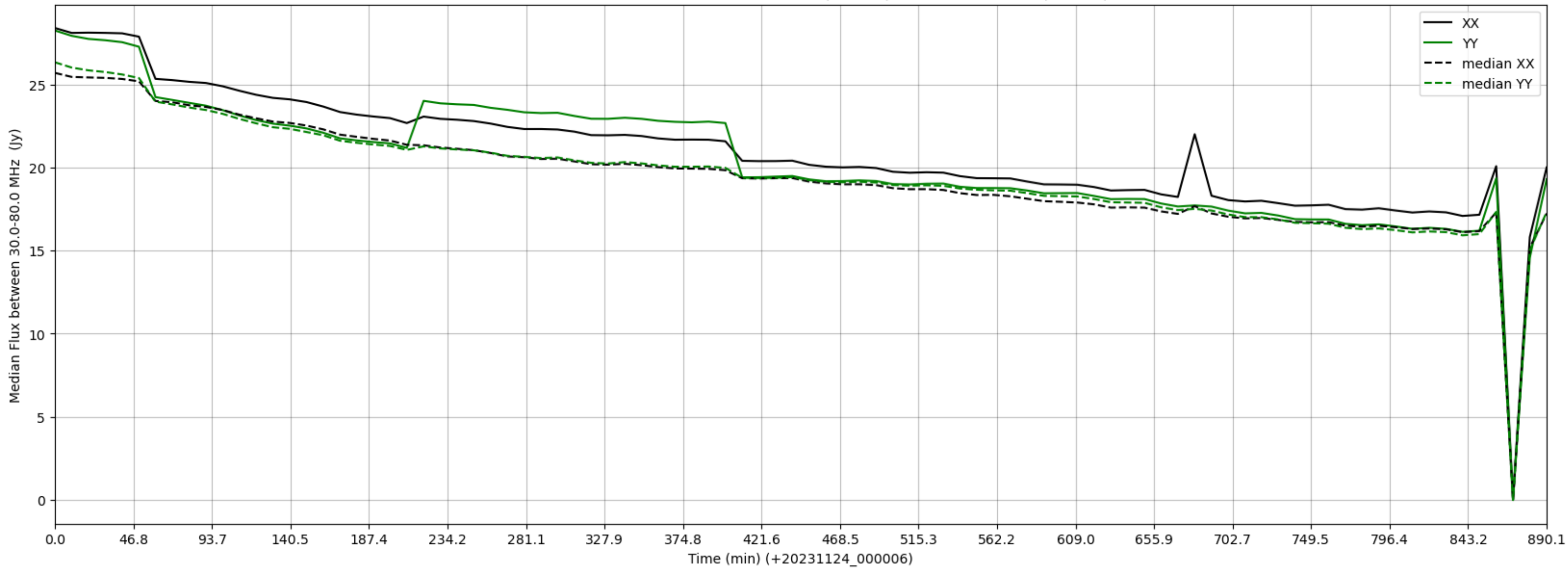
LWA002 - Correlator# 064 - XX FLAGS:BadSpecShape - YY FLAGS:BadSpecShape
