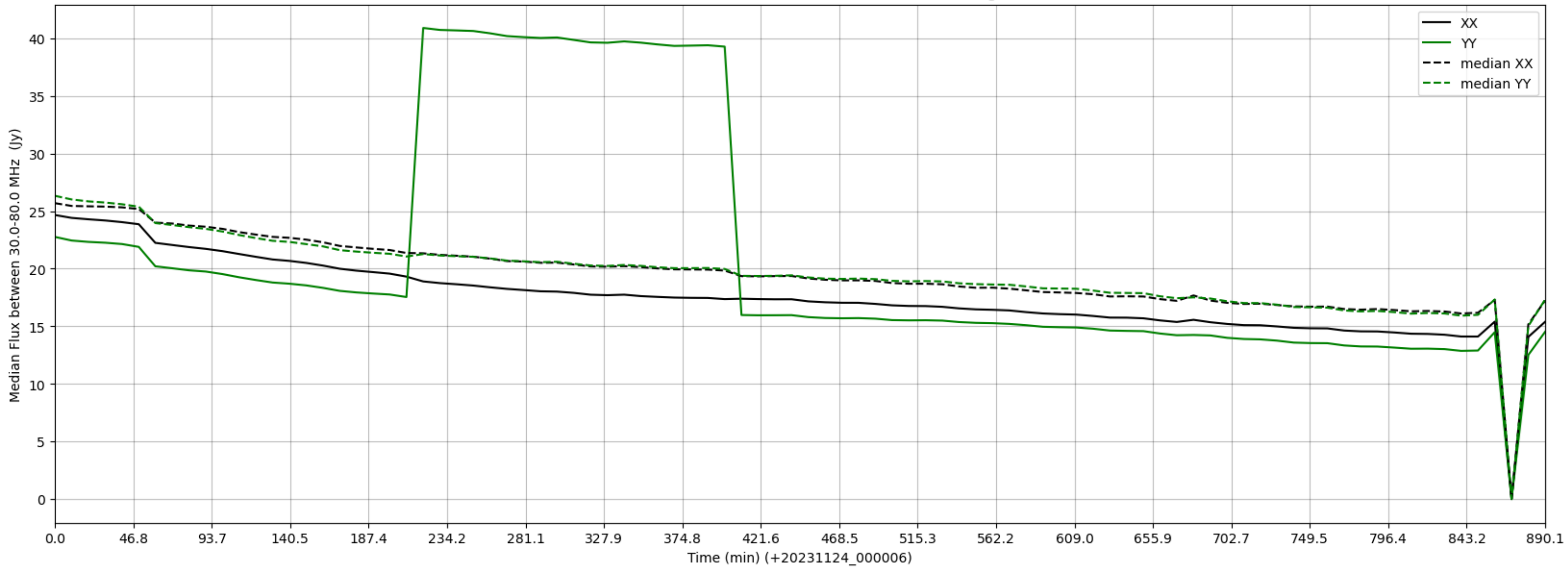
LWA274 - Correlator# 091 - XX FLAGS:Good - YY FLAGS:HighTimeVar
