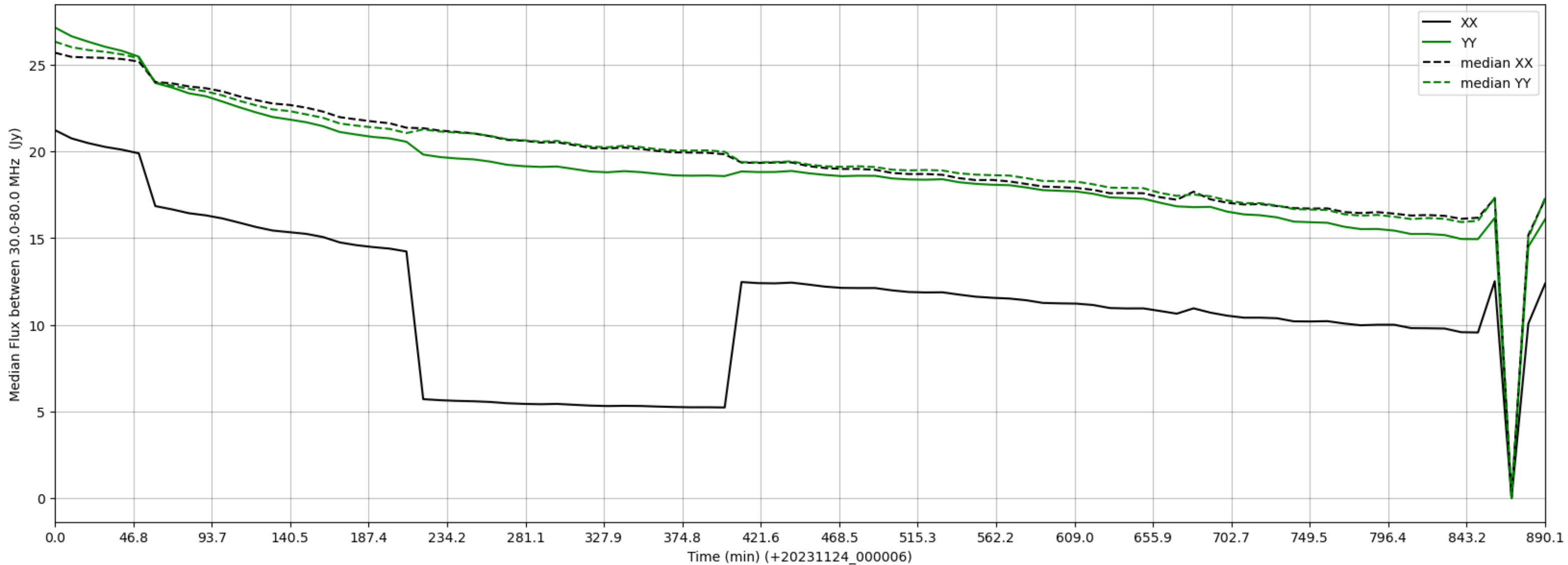
LWA283 - Correlator# 040 - XX FLAGS:HighTimeVar - YY FLAGS:BadSpecShape
