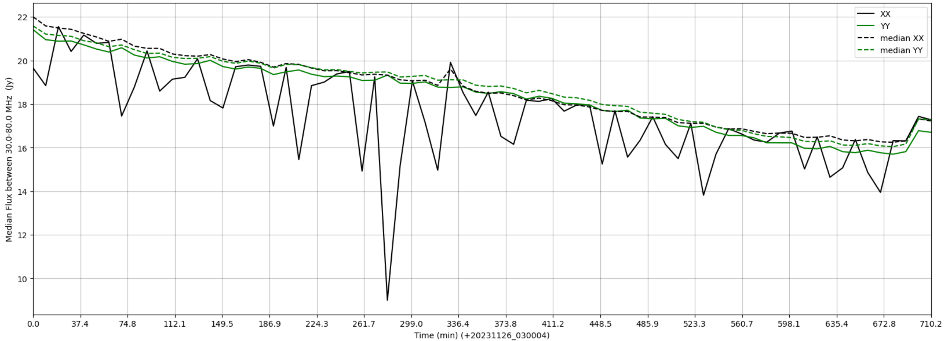
LWA209 - Correlator# 301 - XX FLAGS:HighTimeVar - YY FLAGS:Good
