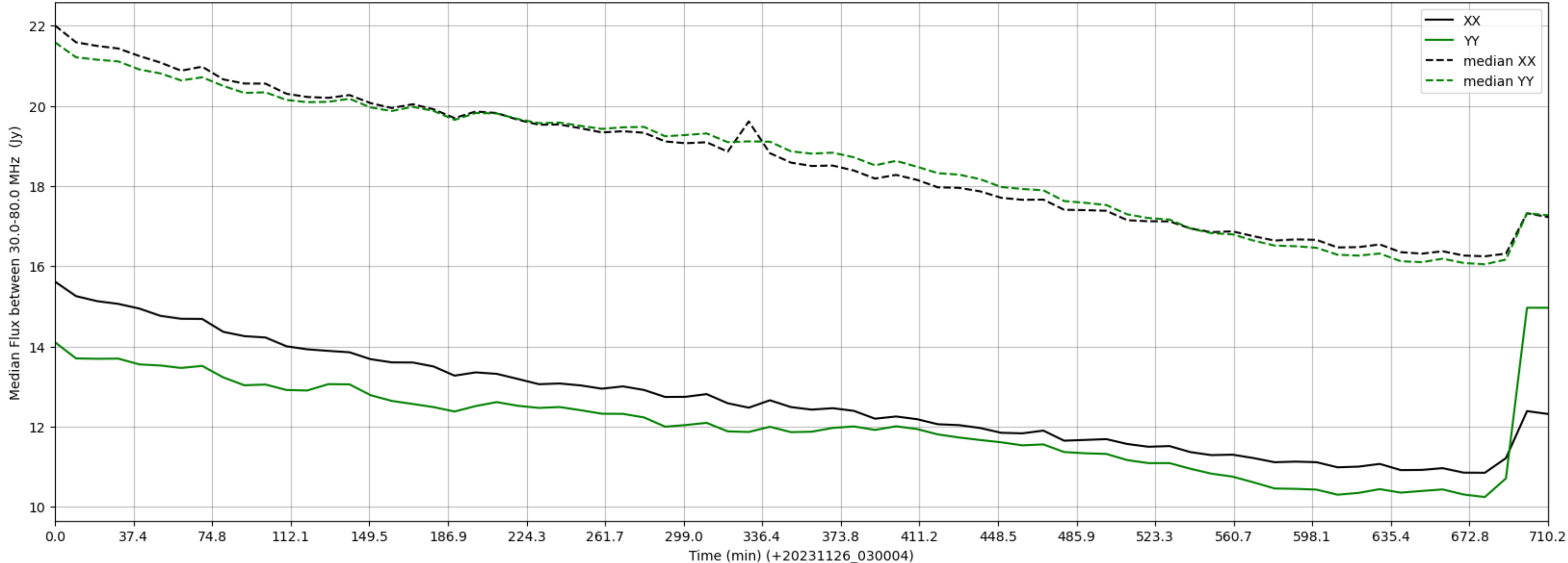
LWA302 - Correlator# 092 - XX FLAGS:BadSpecShape - YY FLAGS:HighTimeVar+BadSpecShape
