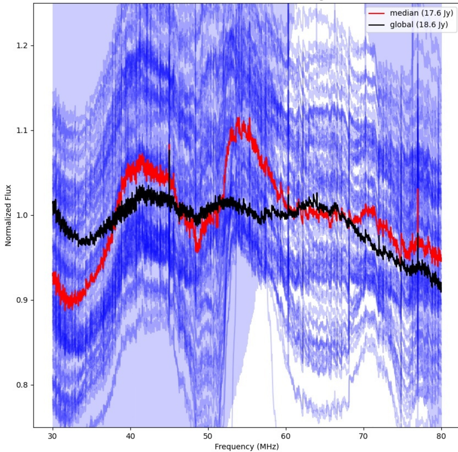
LWA209 - Correlator# 301 - XX - FLAGS:HighTimeVar
