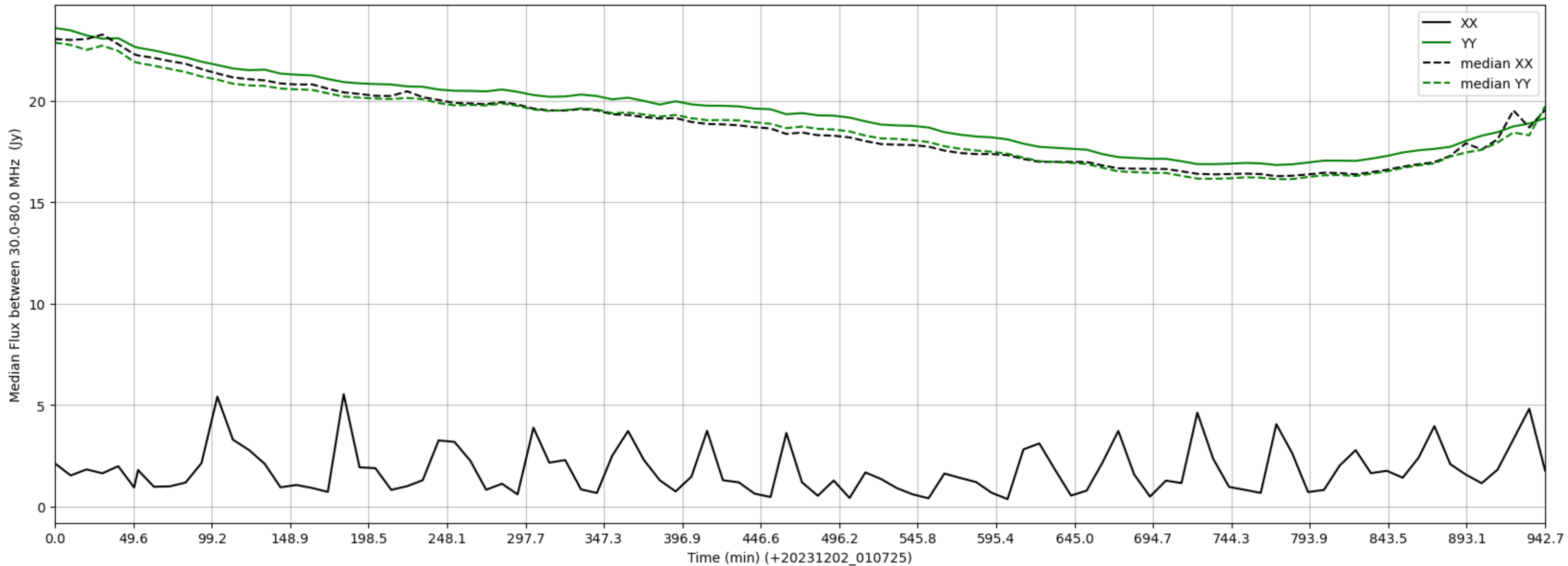
LWA124 - Correlator# 224 - XX FLAGS:LowFlux - YY FLAGS:Good
