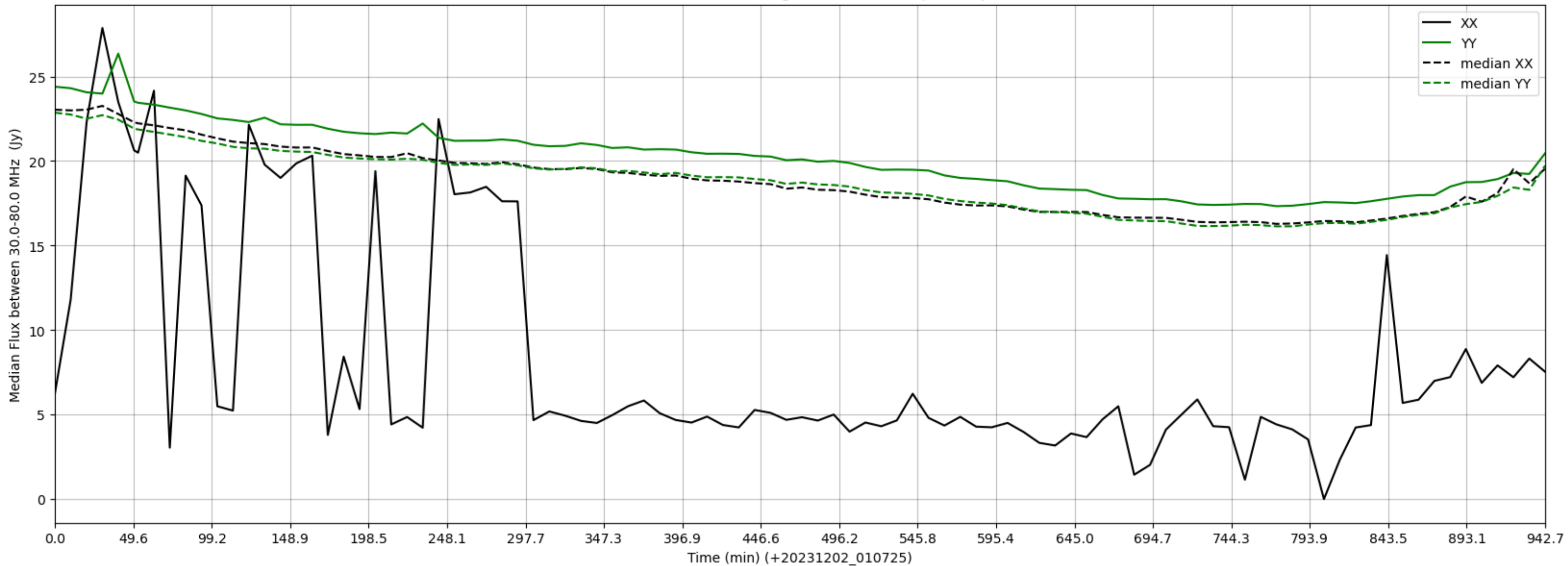
LWA255 - Correlator# 033 - XX FLAGS:HighTimeVar+BadSpecShape - YY FLAGS:Good
