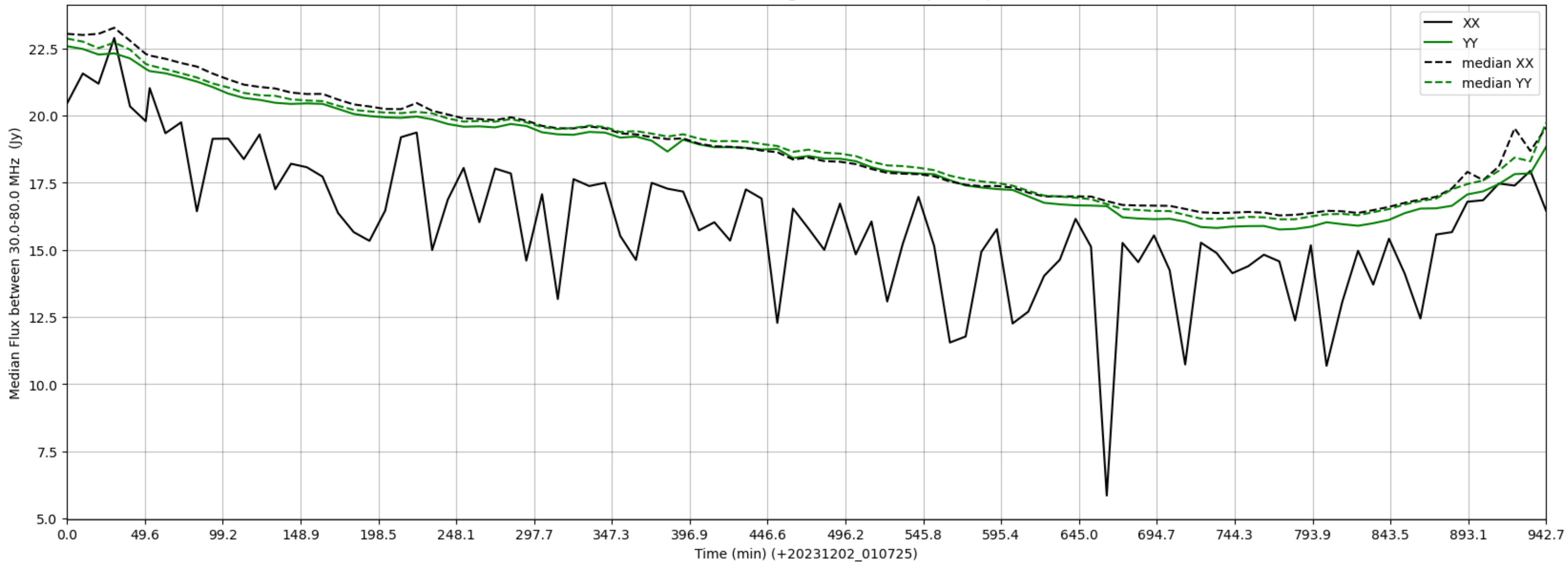
LWA209 - Correlator# 301 - XX FLAGS:HighTimeVar+BadSpecShape - YY FLAGS:Good
