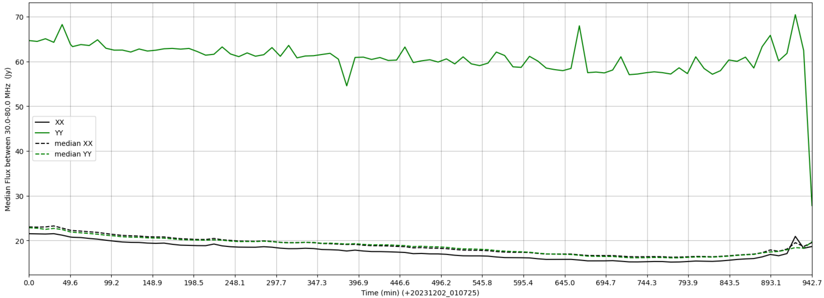
LWA169 - Correlator# 292 - XX FLAGS:Good - YY FLAGS:HighTimeVar+BadSpecShape
