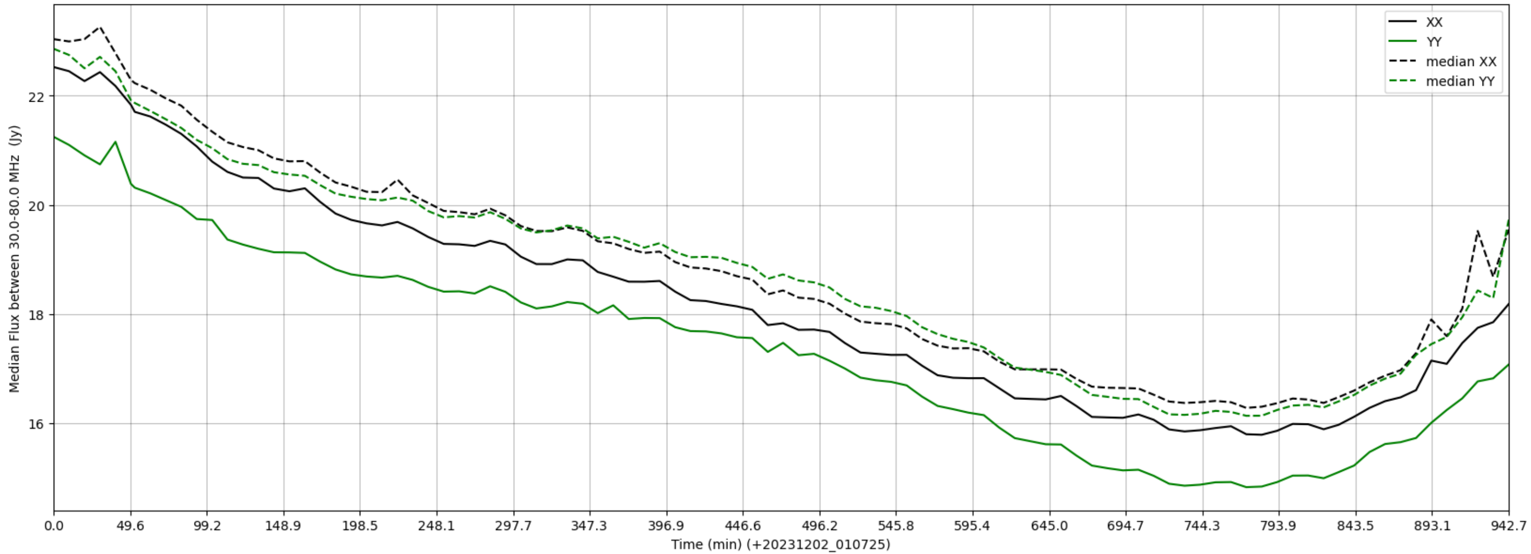
LWA091 - Correlator# 146 - XX FLAGS:BadSpecShape - YY FLAGS:Good
