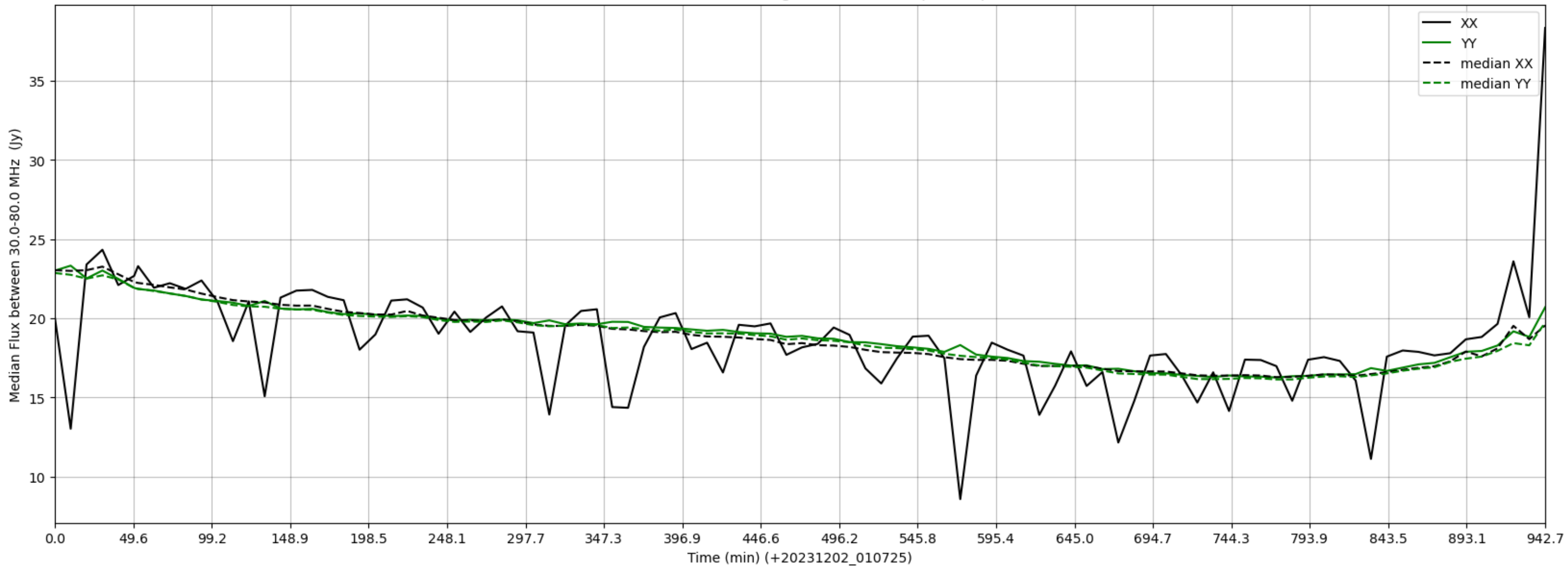
LWA041 - Correlator# 079 - XX FLAGS:HighTimeVar+BadSpecShape - YY FLAGS:Good
