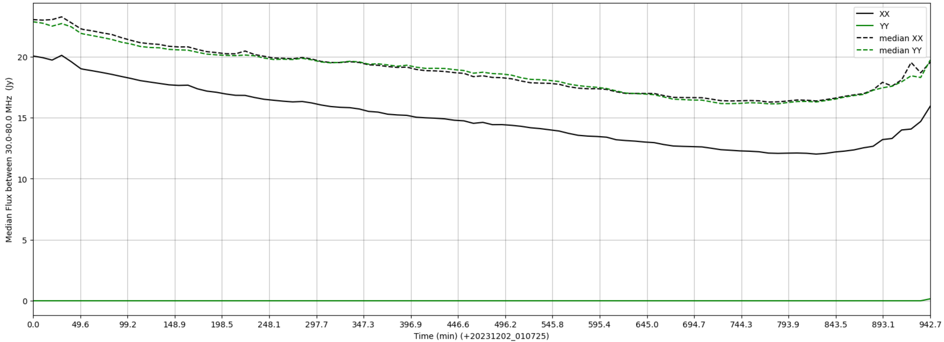
LWA314 - Correlator# 021 - XX FLAGS:Good - YY FLAGS:LowFlux
