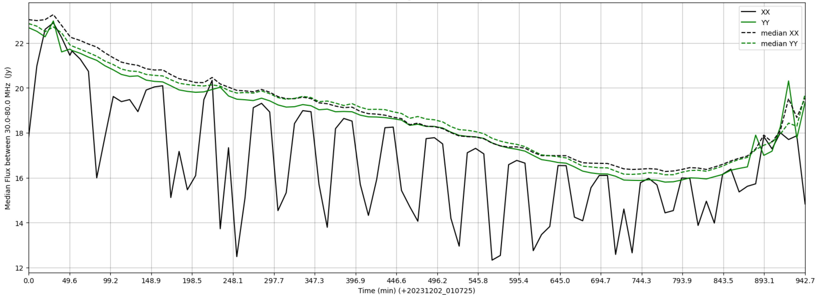
LWA105 - Correlator# 178 - XX FLAGS:HighTimeVar+BadSpecShape - YY FLAGS:Good
