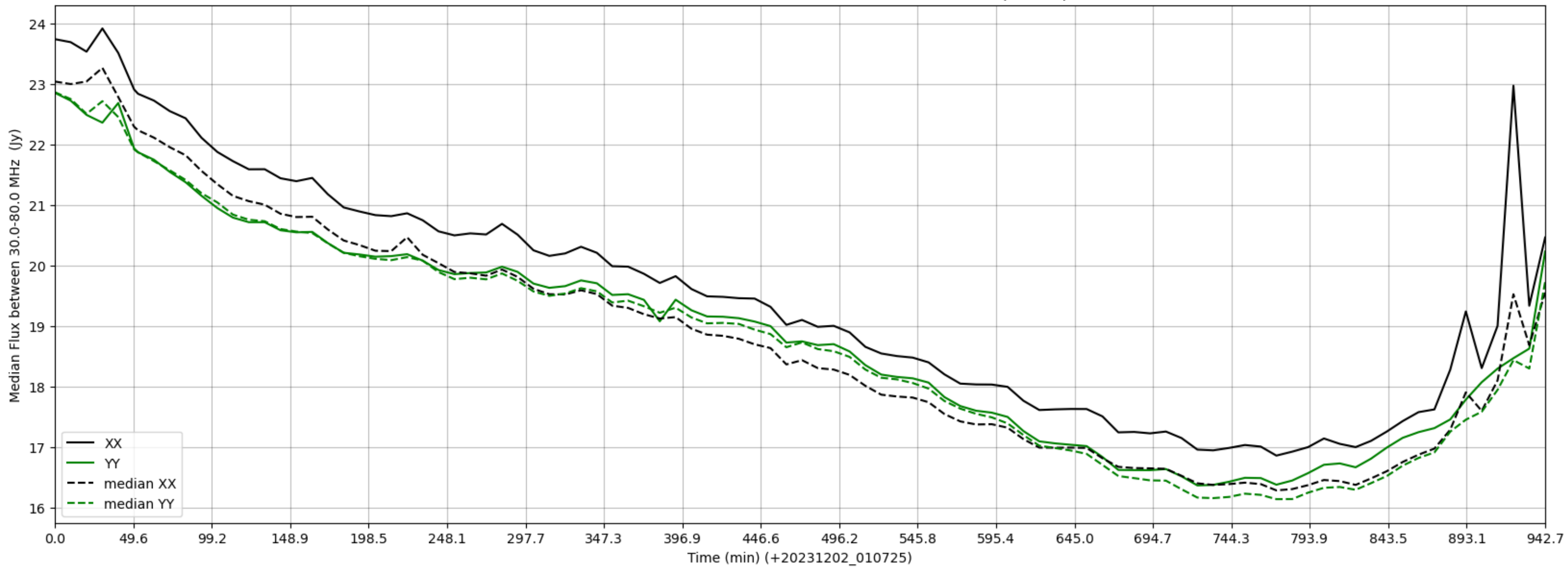
LWA237 - Correlator# 311 - XX FLAGS:Good - YY FLAGS:BadSpecShape
