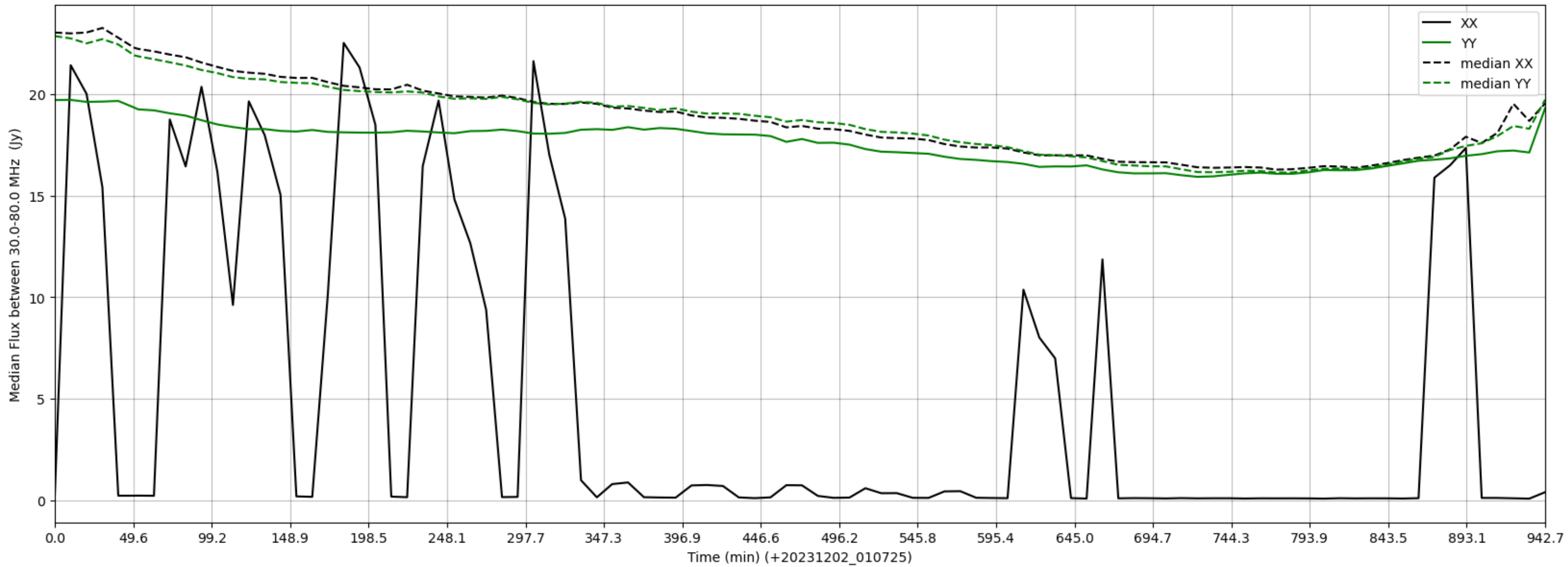
LWA310 - Correlator# 017 - XX FLAGS:LowFlux - YY FLAGS:Good
