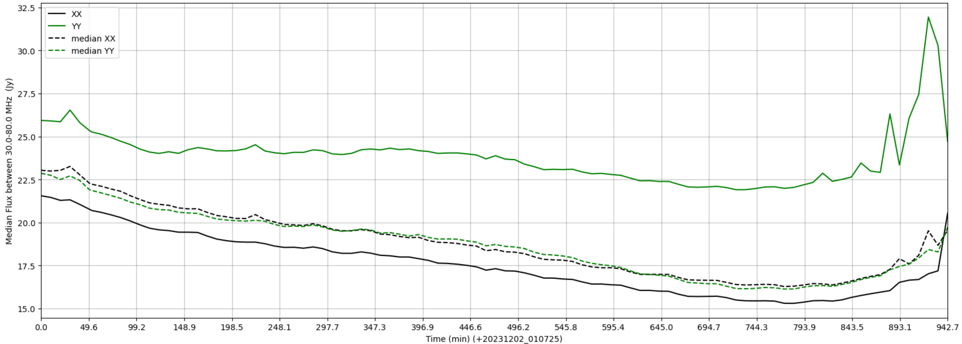
LWA316 - Correlator# 155 - XX FLAGS:Good - YY FLAGS:HighTimeVar
