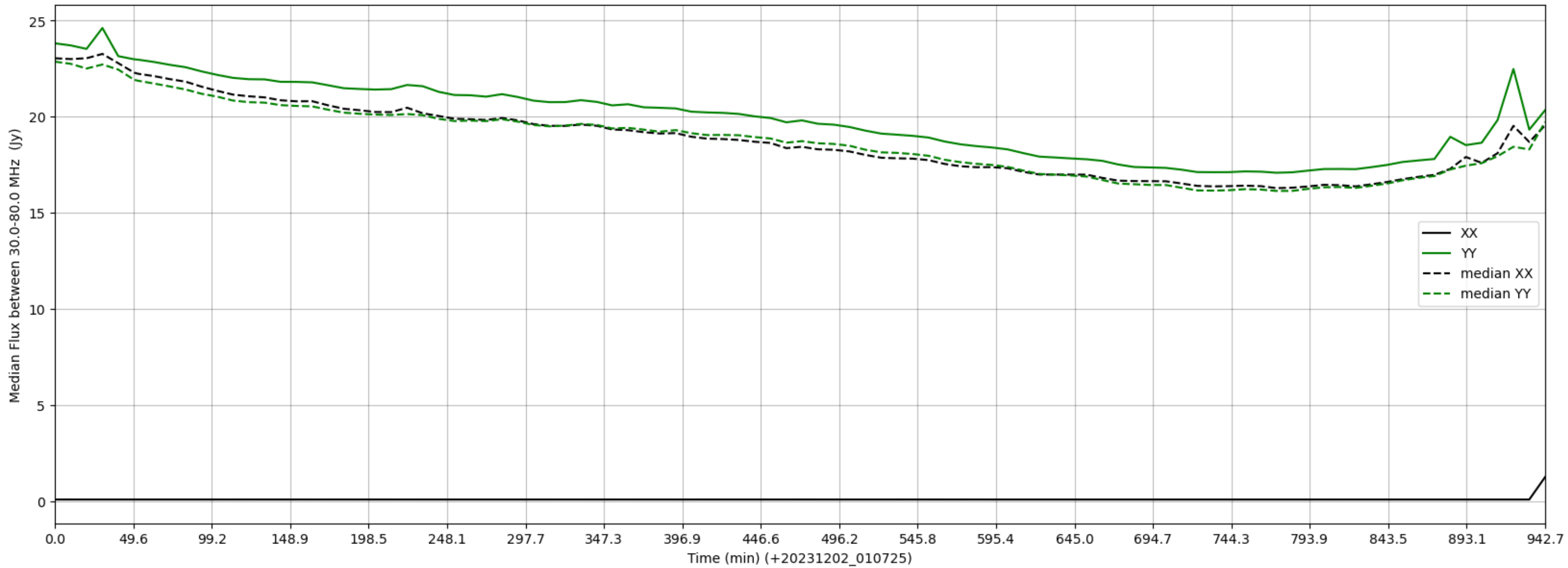
LWA076 - Correlator# 193 - XX FLAGS:LowFlux - YY FLAGS:Good
