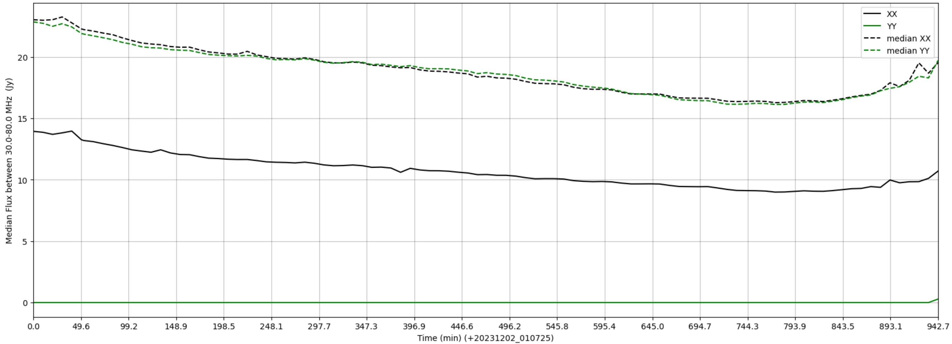
LWA150 - Correlator# 215 - XX FLAGS:Good - YY FLAGS:LowFlux
