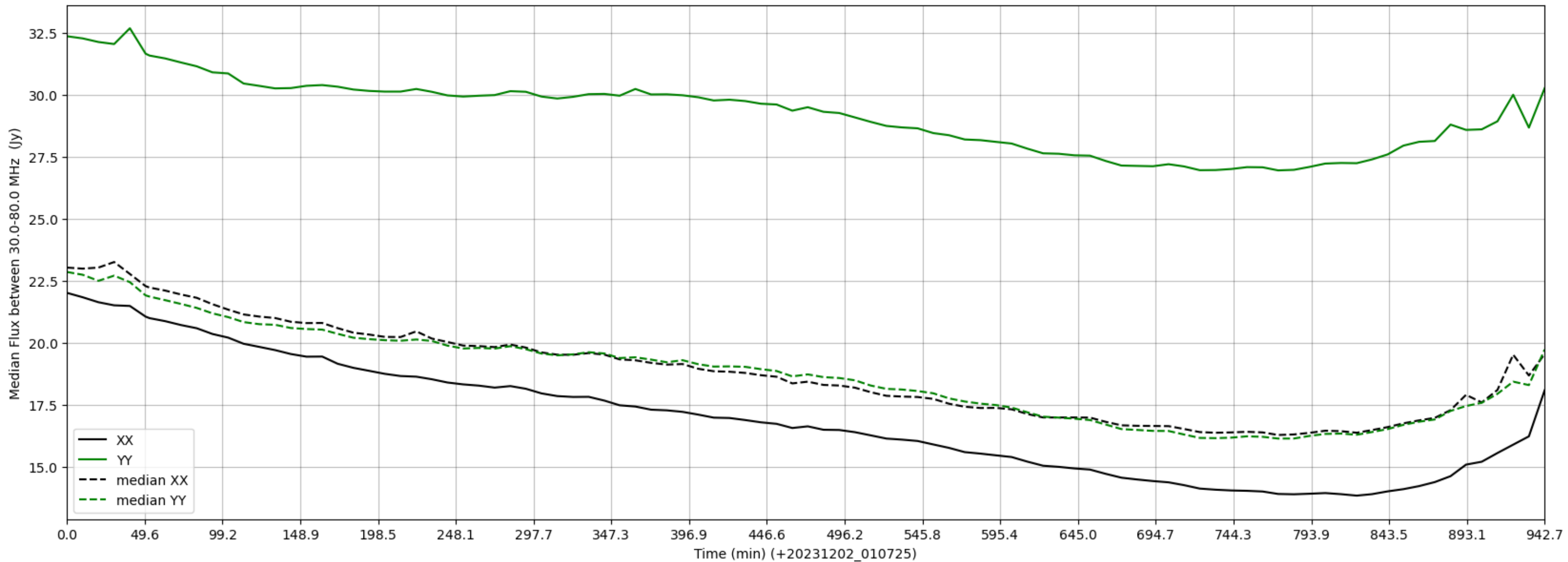
LWA296 - Correlator# 046 - XX FLAGS:Good - YY FLAGS:Good
