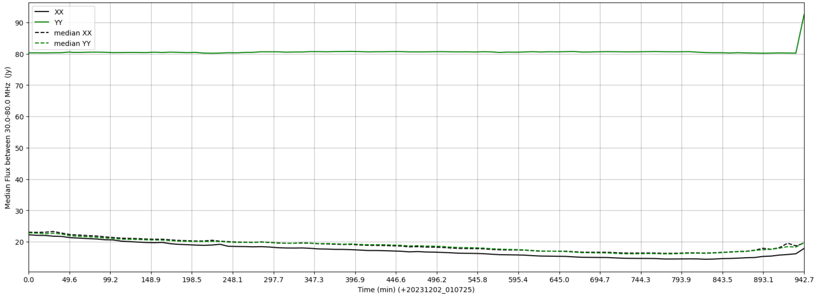
LWA280 - Correlator# 041 - XX FLAGS:Good - YY FLAGS:BadSpecShape
