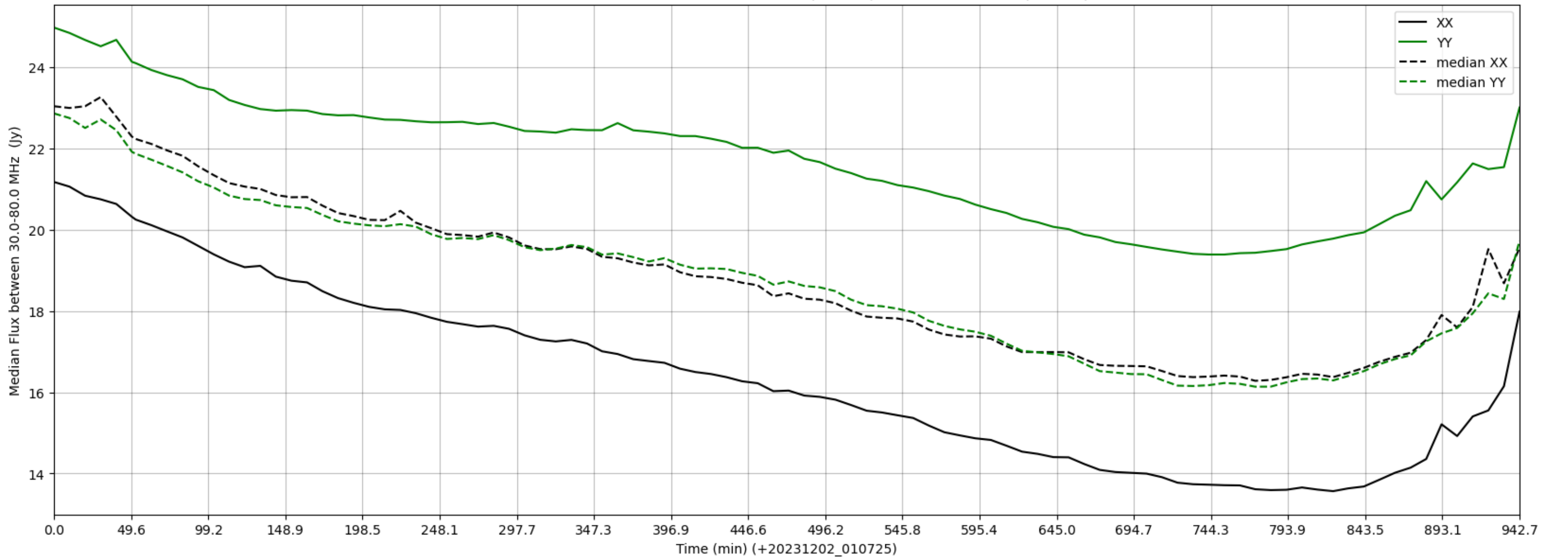
LWA364 - Correlator# 127 - XX FLAGS:BadSpecShape - YY FLAGS:BadSpecShape
