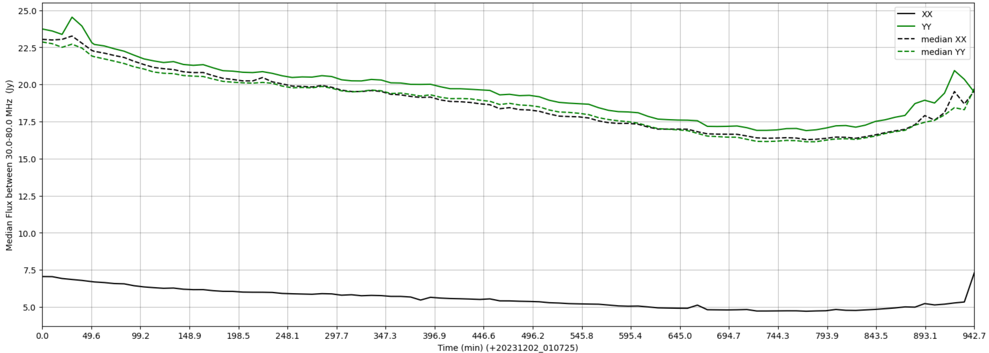
LWA232 - Correlator# 307 - XX FLAGS:BadSpecShape - YY FLAGS:BadSpecShape
