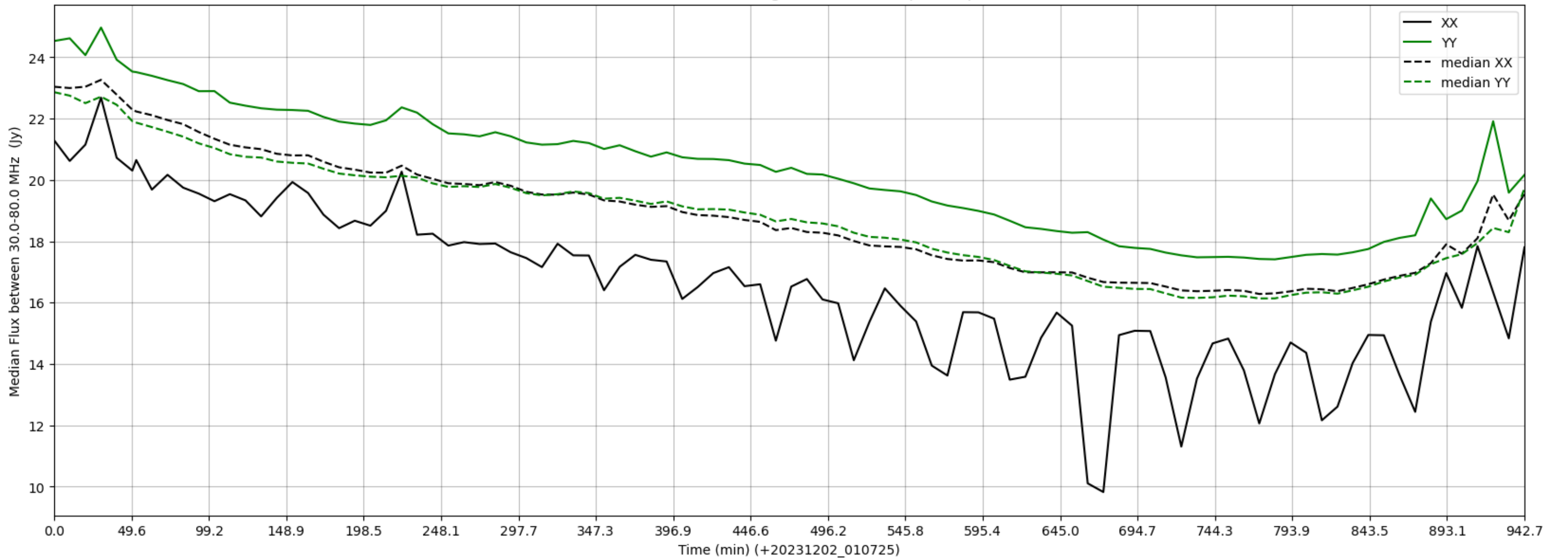
LWA111 - Correlator# 201 - XX FLAGS:HighTimeVar+BadSpecShape - YY FLAGS:Good
