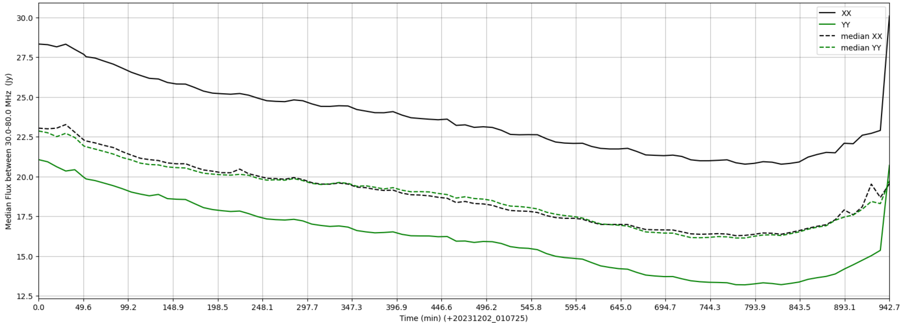
LWA277 - Correlator# 009 - XX FLAGS:Good - YY FLAGS:Good
