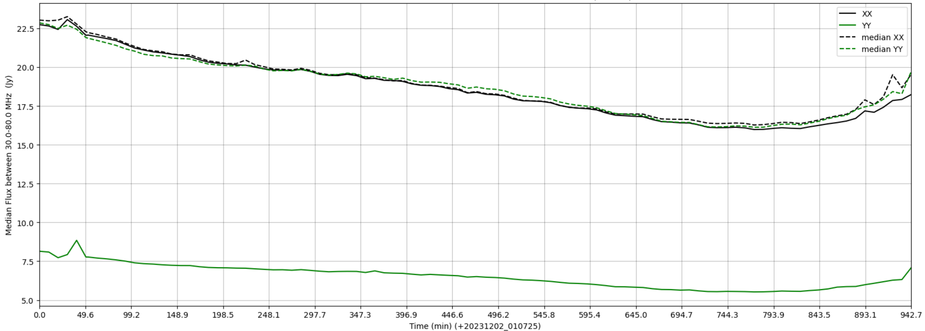
LWA058 - Correlator# 137 - XX FLAGS:Good - YY FLAGS:BadSpecShape
