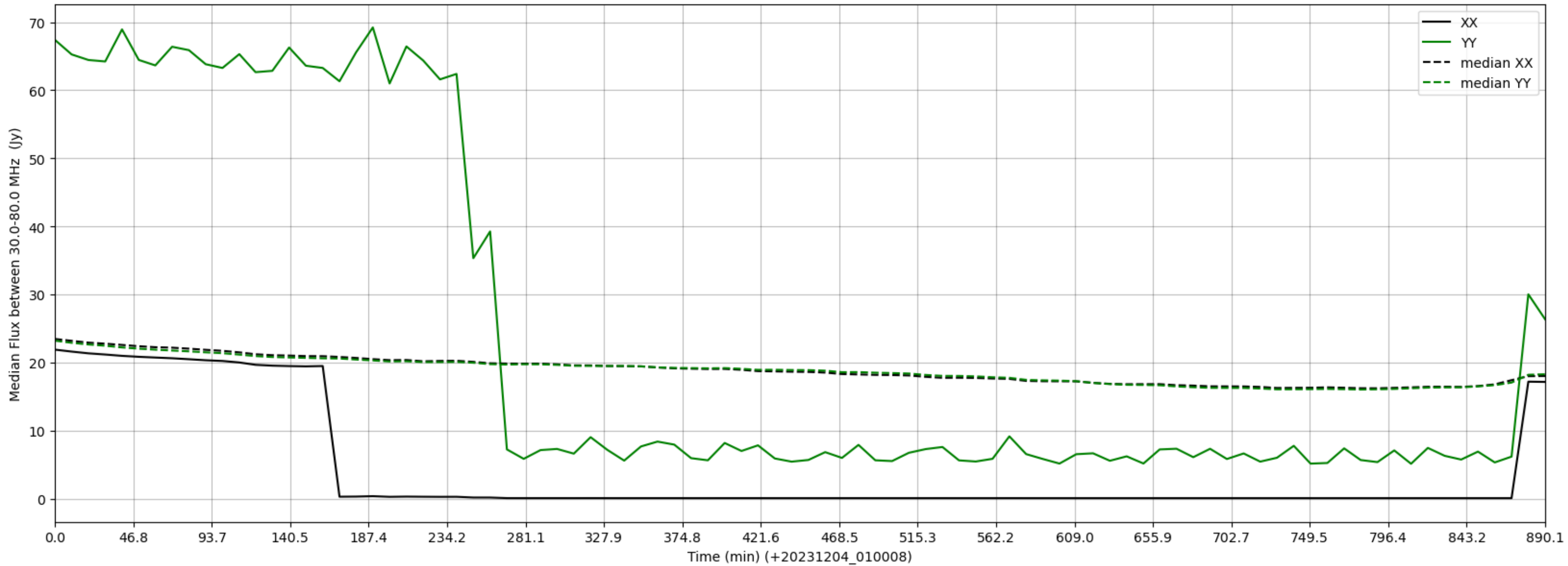
LWA169 - Correlator# 292 - XX FLAGS:LowFlux - YY FLAGS:HighTimeVar+BadSpecShape
