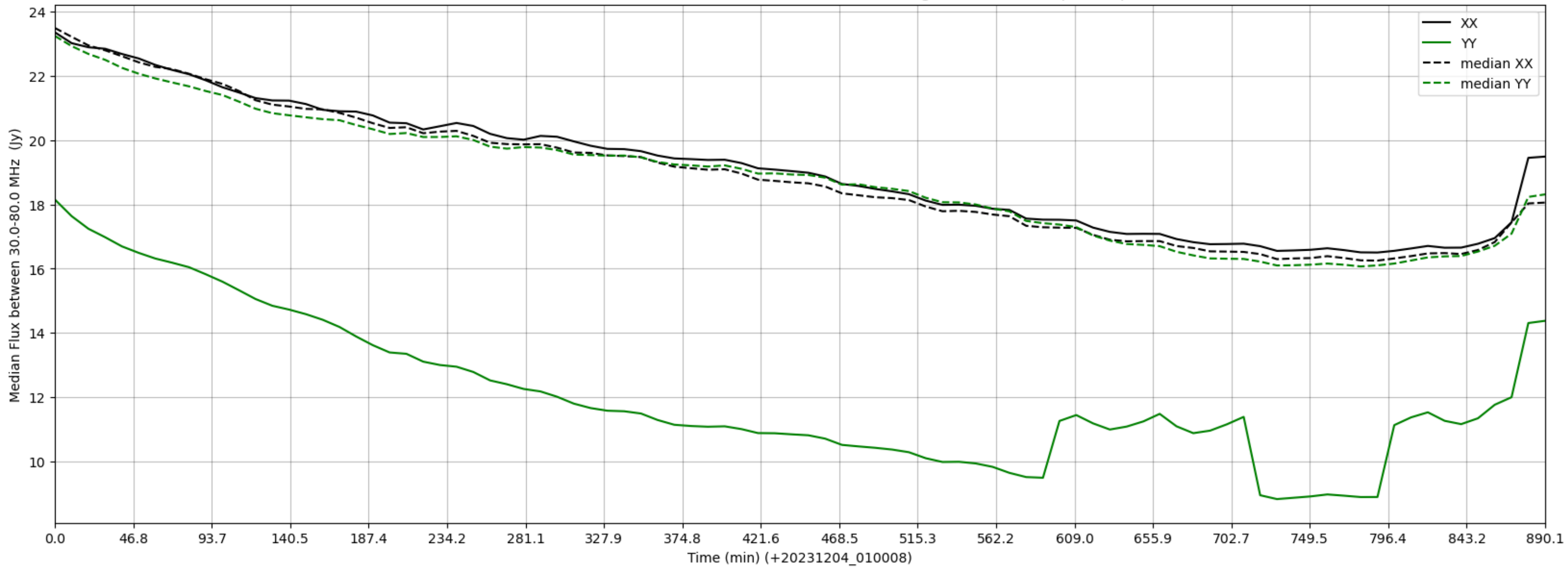
LWA358 - Correlator# 159 - XX FLAGS:Good - YY FLAGS:HighTimeVar+BadSpecShape
