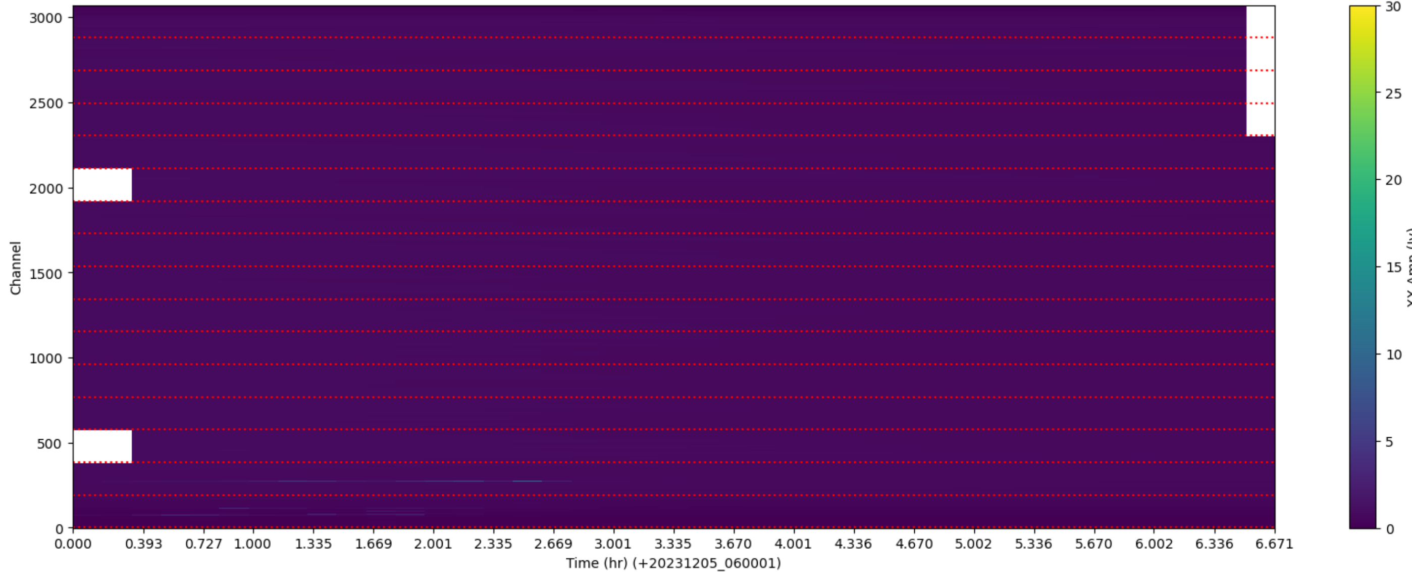
LWA205 - Correlator# 297 - XX - FLAGS: LowFlux
