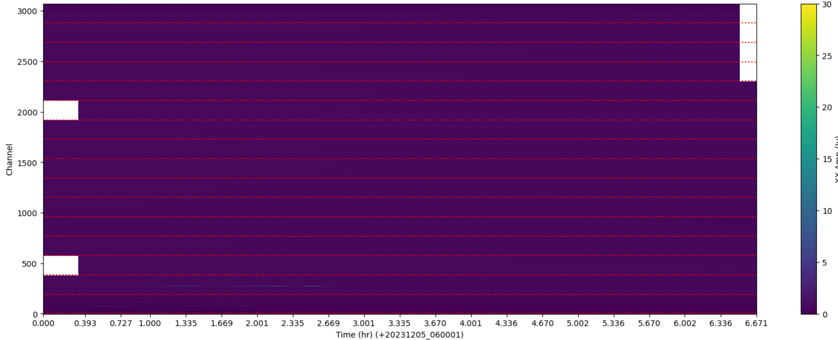
LWA206 - Correlator# 296 - XX - FLAGS: LowFlux
