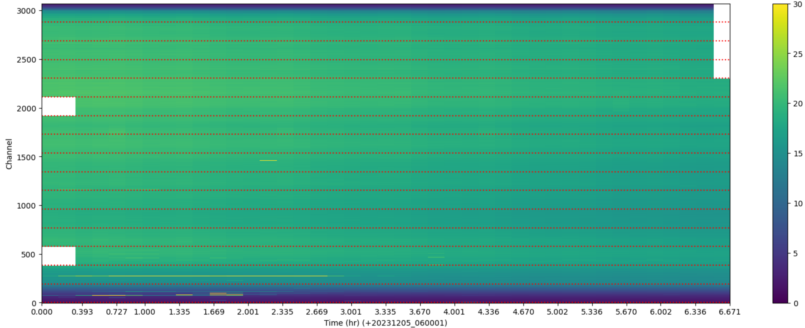
LWA161 - Correlator# 262 - XX - FLAGS: Good
