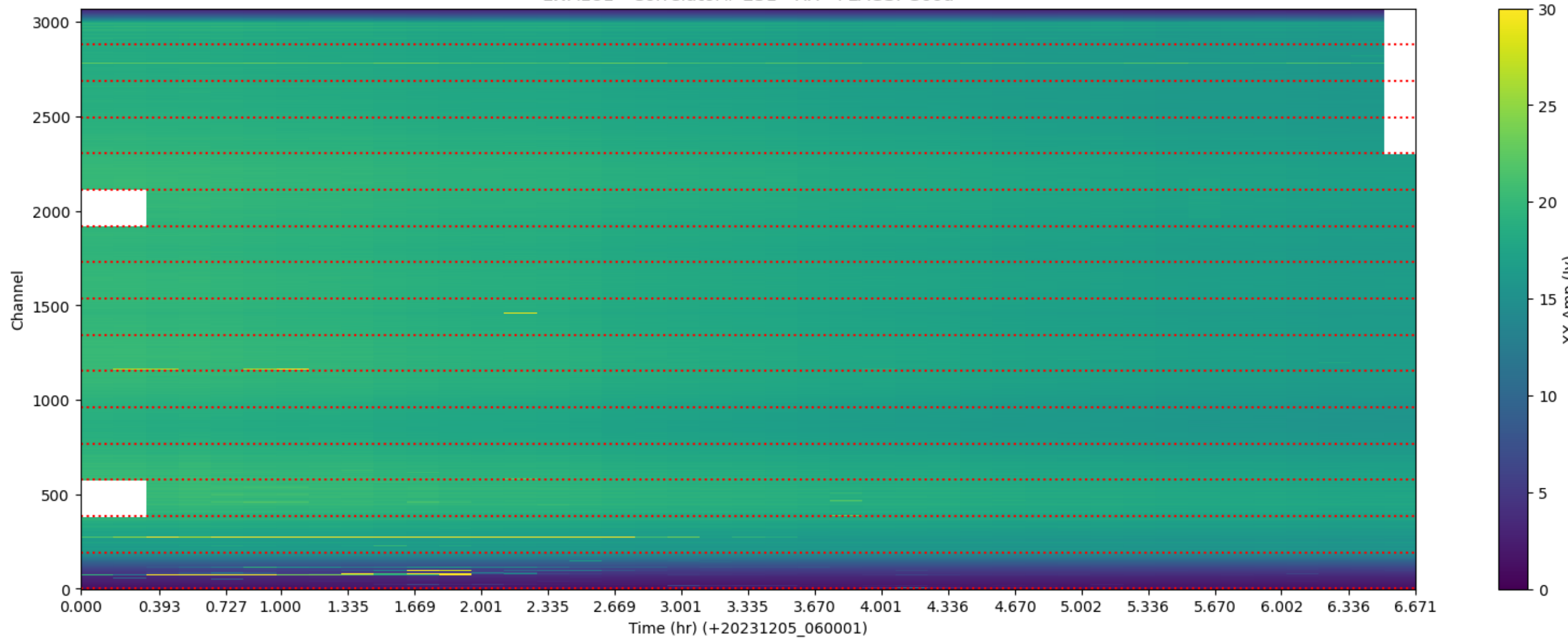
LWA181 - Correlator# 231 - XX - FLAGS: Good
