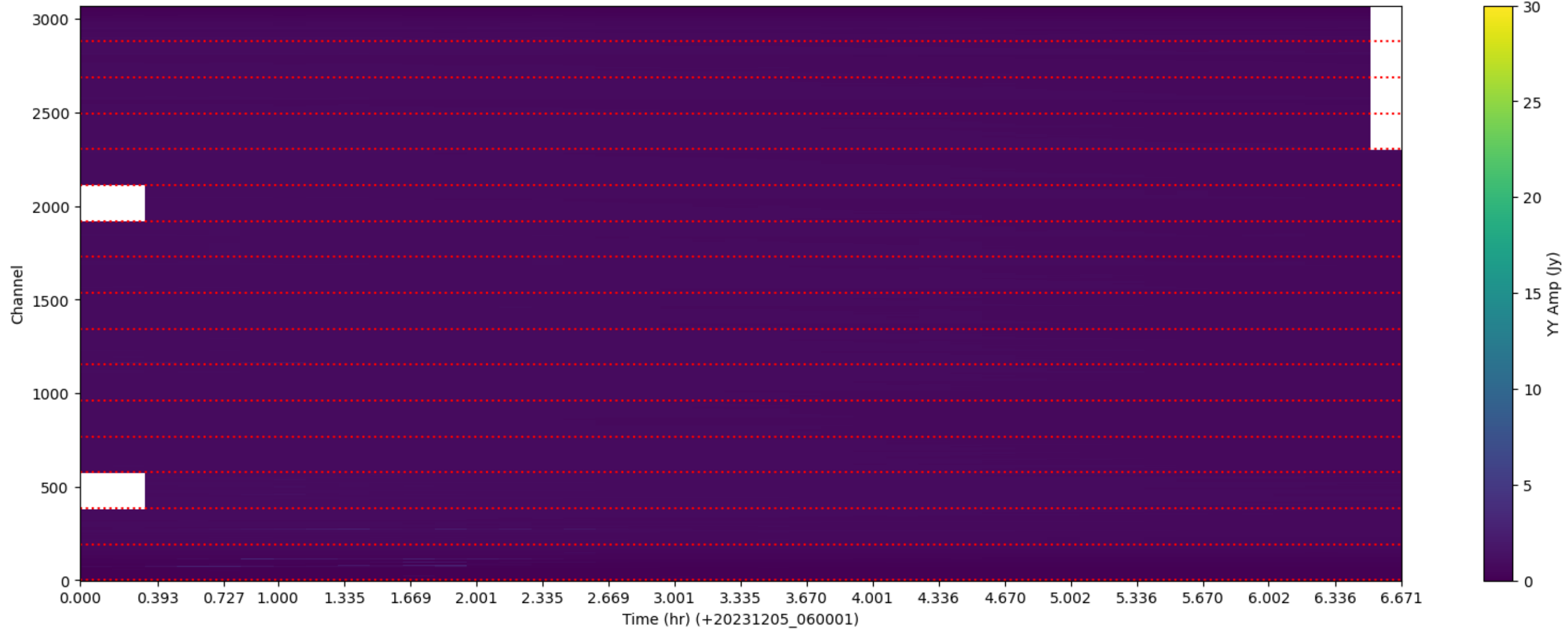
LWA173 - Correlator# 290 - YY - FLAGS: LowFlux
