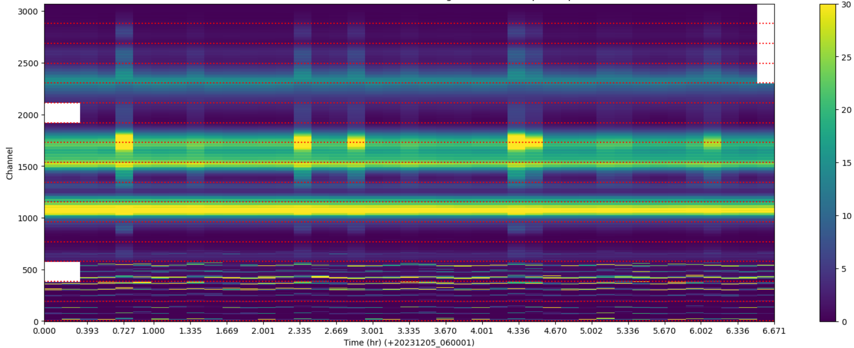
LWA169 - Correlator# 292 - YY - FLAGS: HighTimeVar+BadSpecShape
