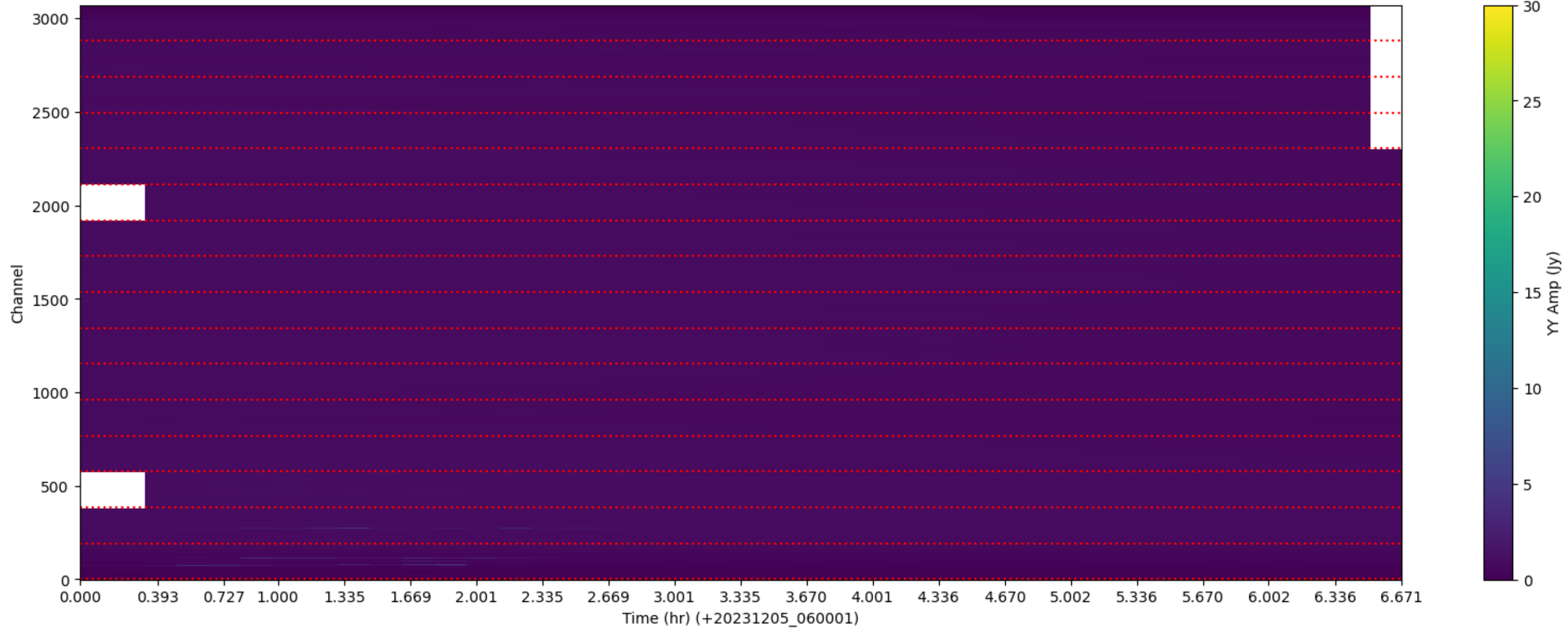
LWA206 - Correlator# 296 - YY - FLAGS: LowFlux
