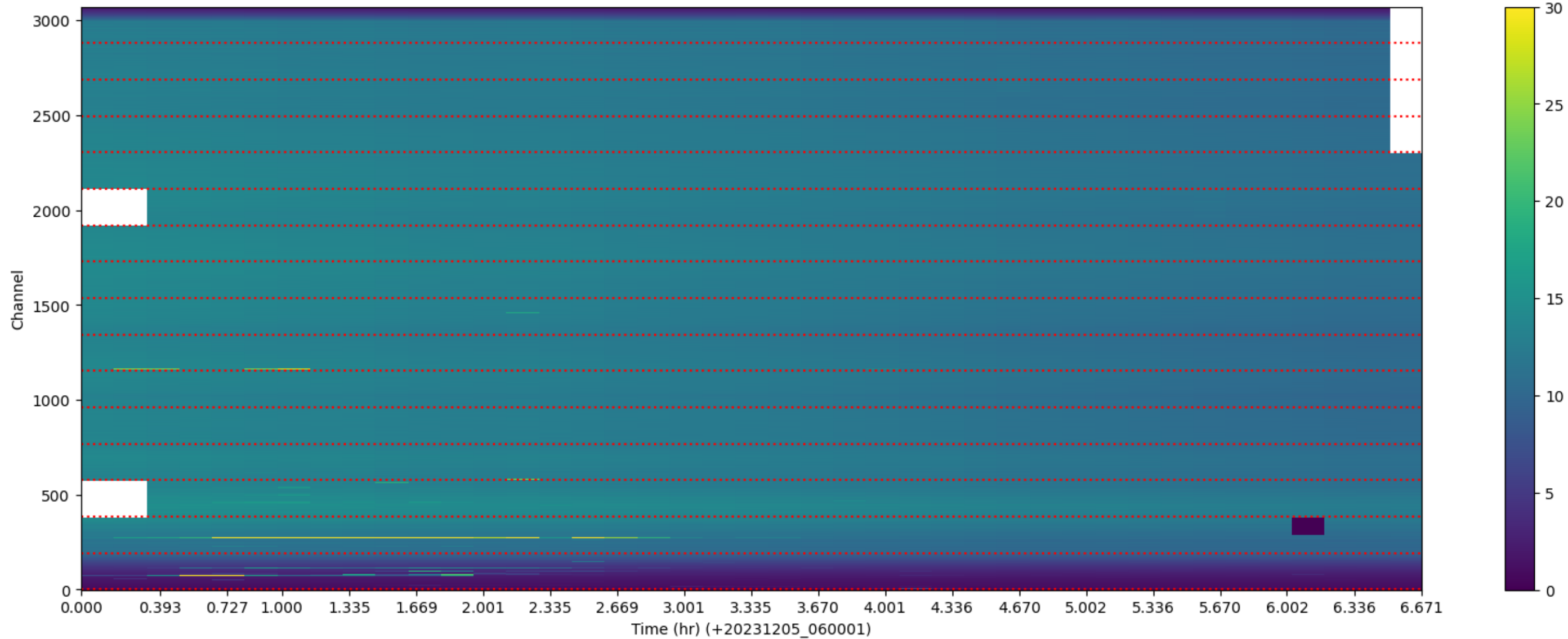
LWA263 - Correlator# 037 - YY - FLAGS: Good
