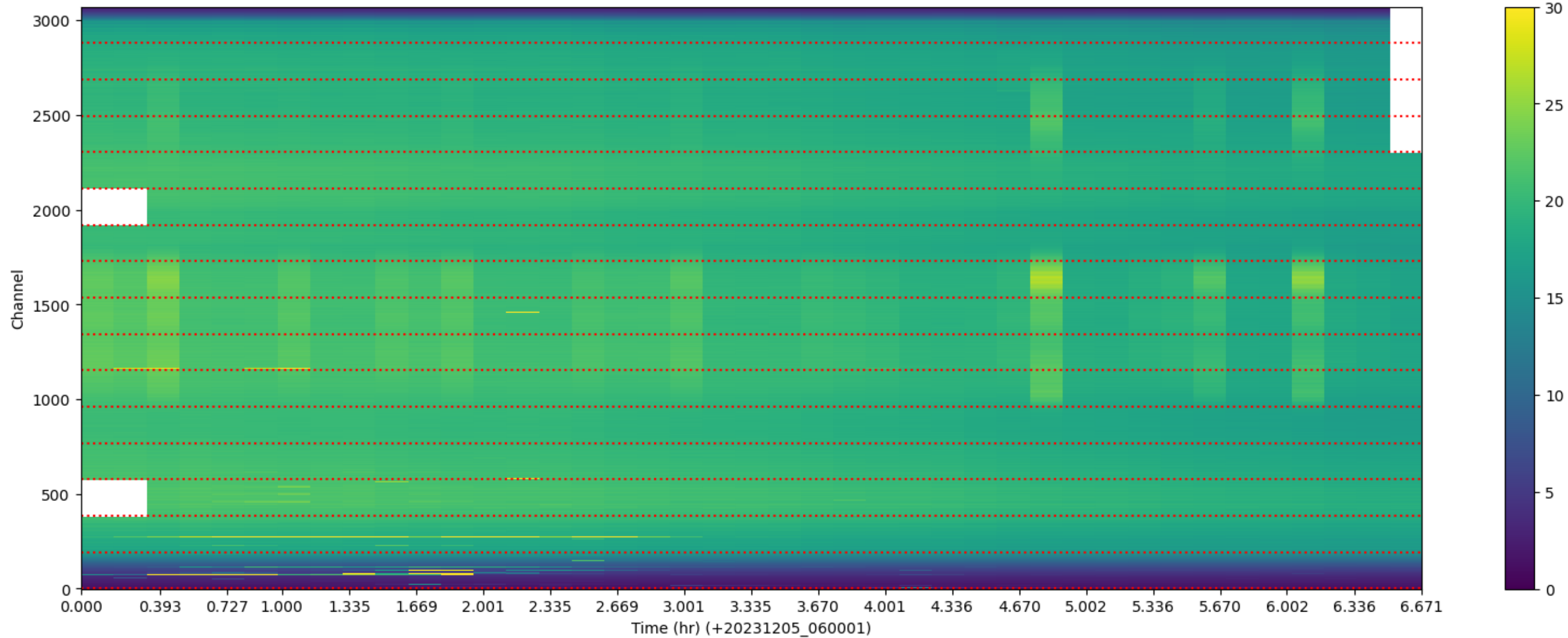
LWA037 - Correlator# 181 - YY - FLAGS: Good
