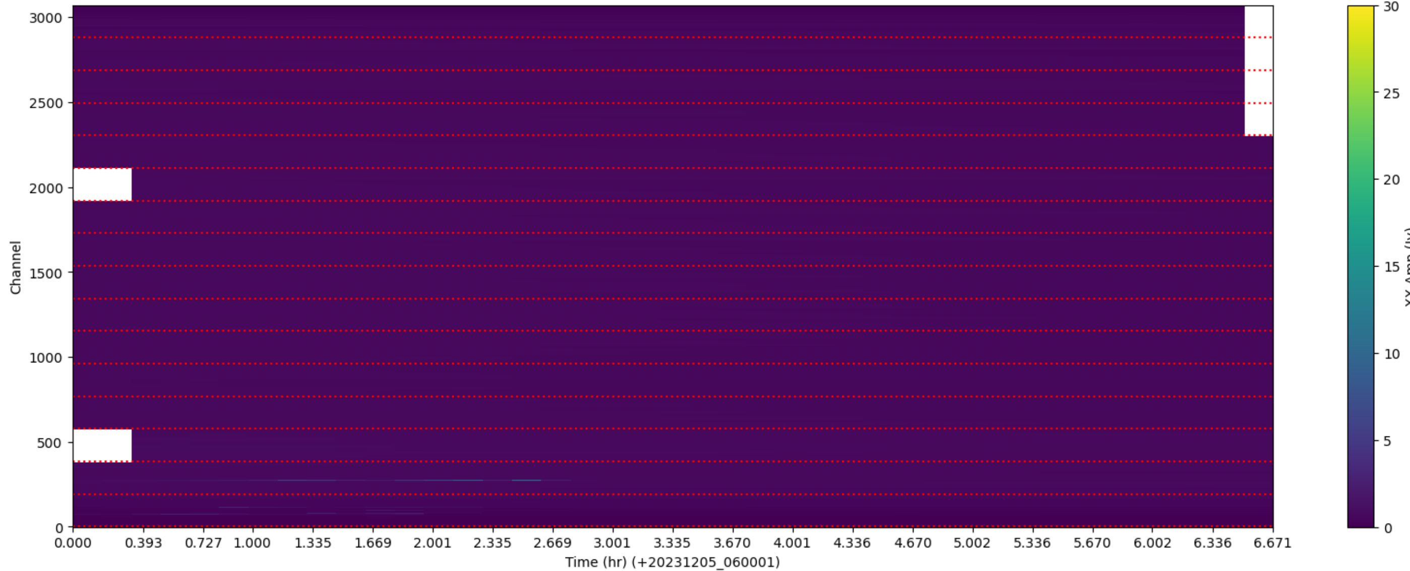
LWA169 - Correlator# 292 - XX - FLAGS: LowFlux
