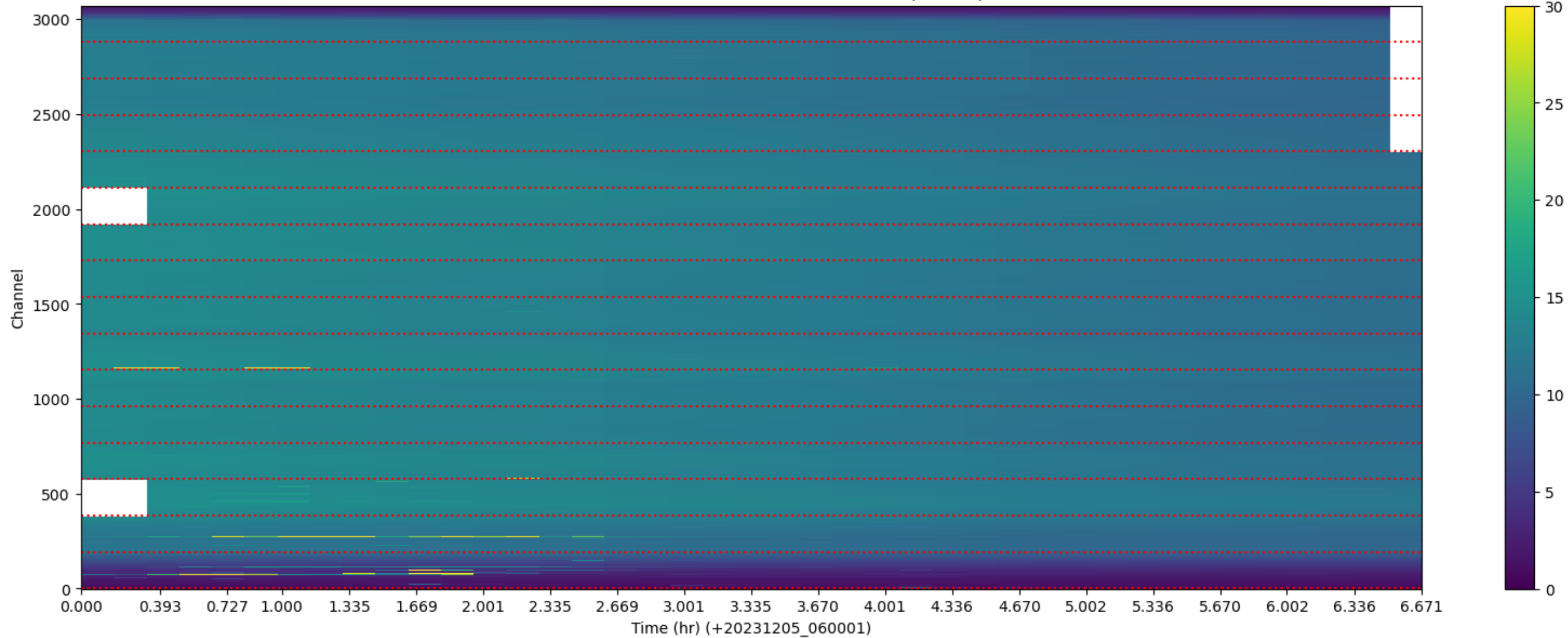
LWA293 - Correlator# 284 - YY - FLAGS: BadSpecShape
