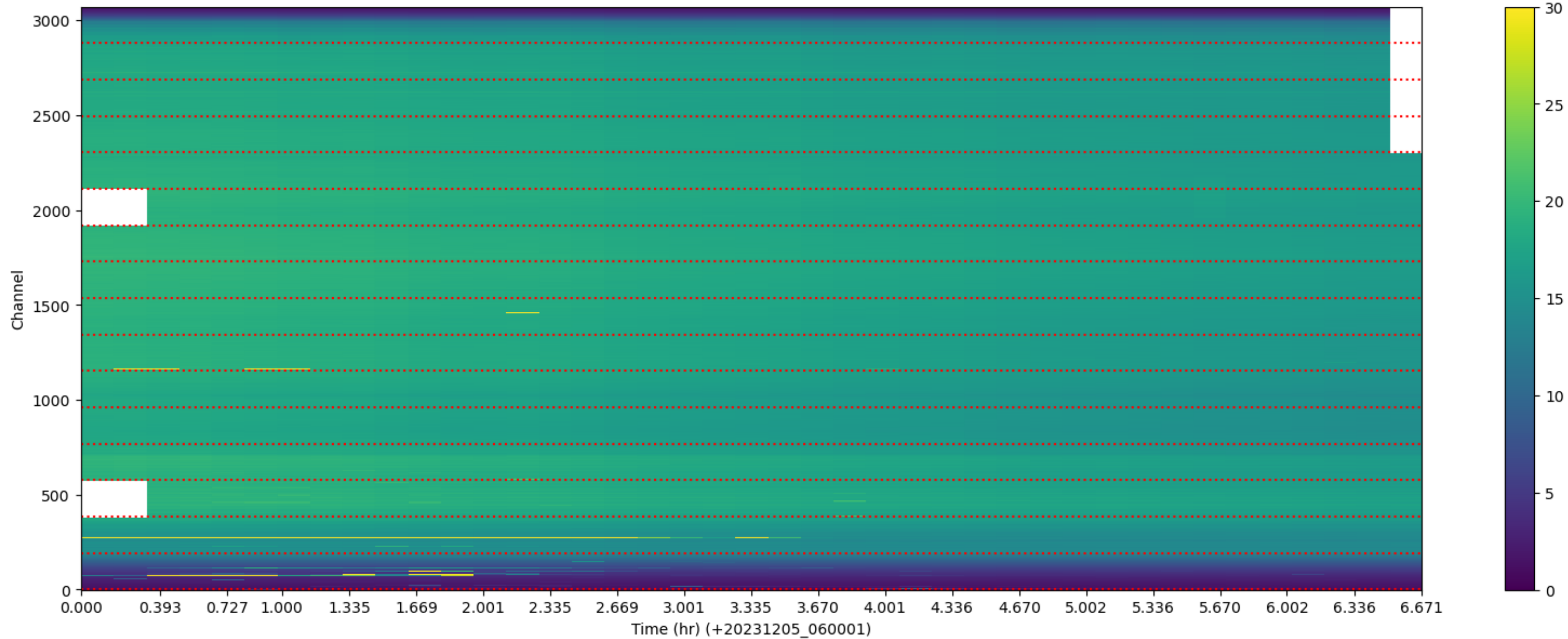
LWA289 - Correlator# 189 - XX - FLAGS: Good
