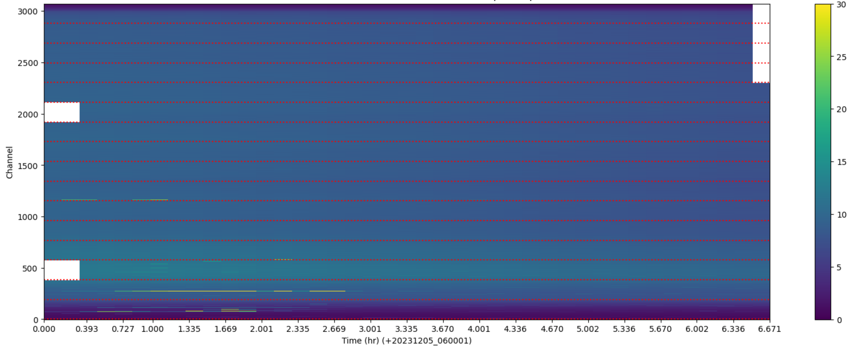
LWA319 - Correlator# 190 - YY - FLAGS: BadSpecShape
