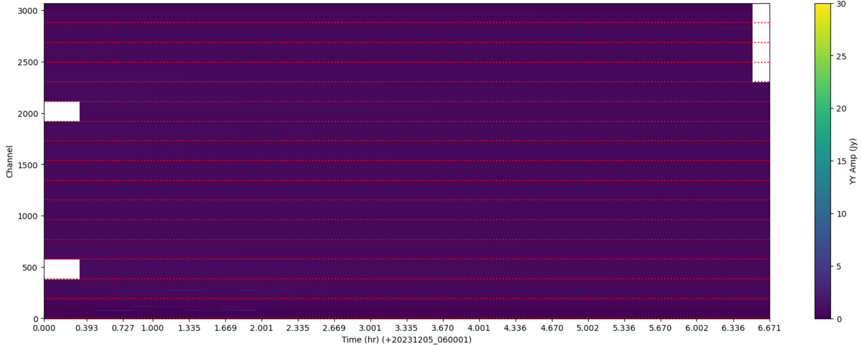
LWA207 - Correlator# 299 - YY - FLAGS: LowFlux
