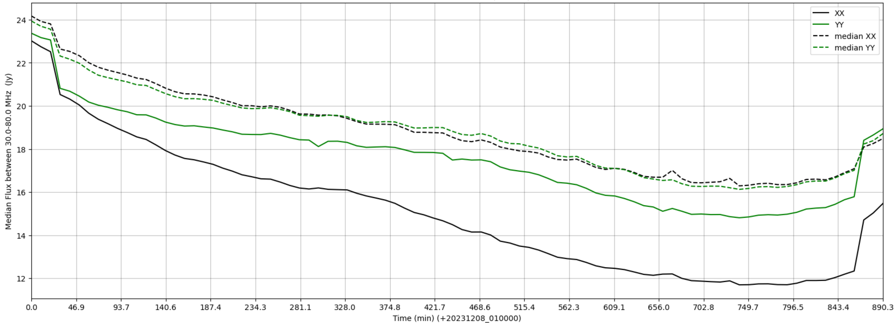
LWA276 - Correlator# 006 - XX FLAGS:BadSpecShape - YY FLAGS:Good
