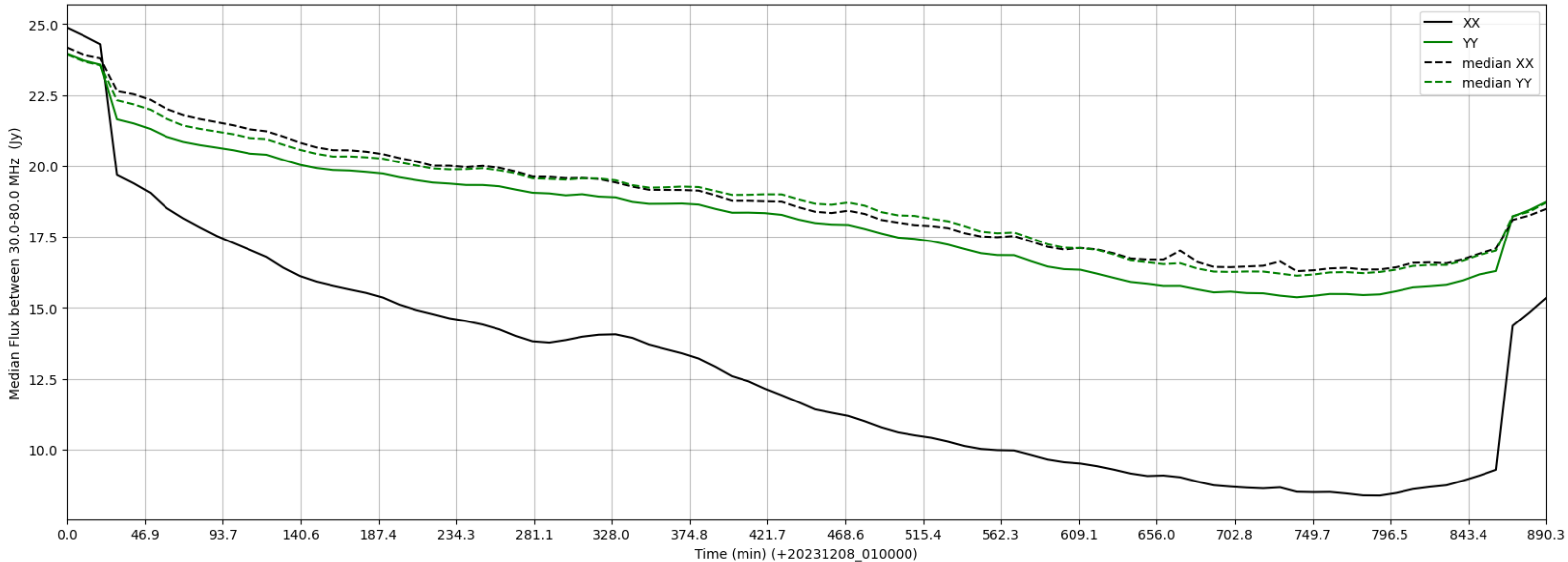
LWA357 - Correlator# 286 - XX FLAGS:HighTimeVar+BadSpecShape - YY FLAGS:Good
