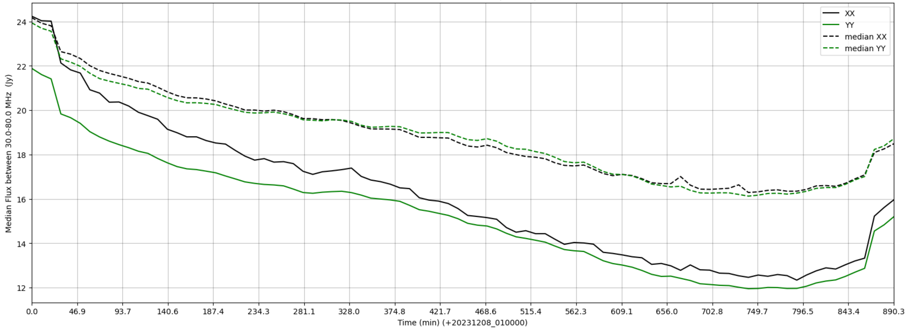
LWA299 - Correlator# 191 - XX FLAGS:BadSpecShape - YY FLAGS:Good
