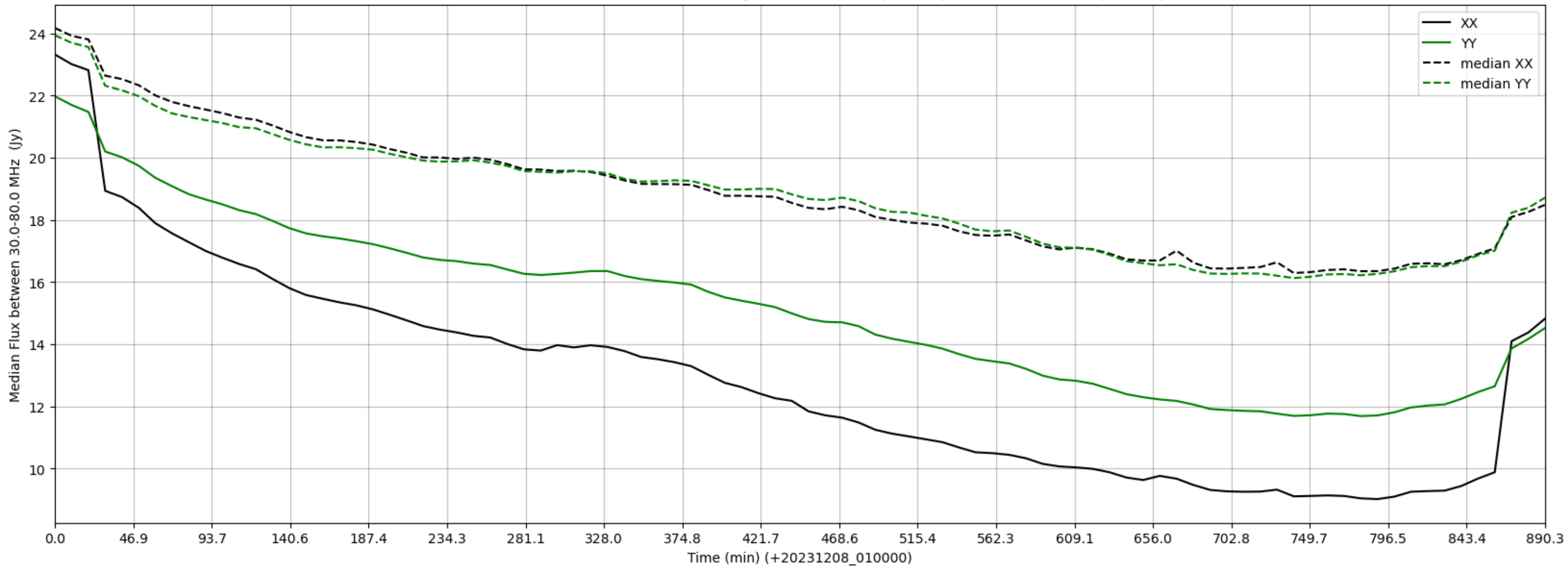
LWA363 - Correlator# 094 - XX FLAGS:HighTimeVar+BadSpecShape - YY FLAGS:BadSpecShape
