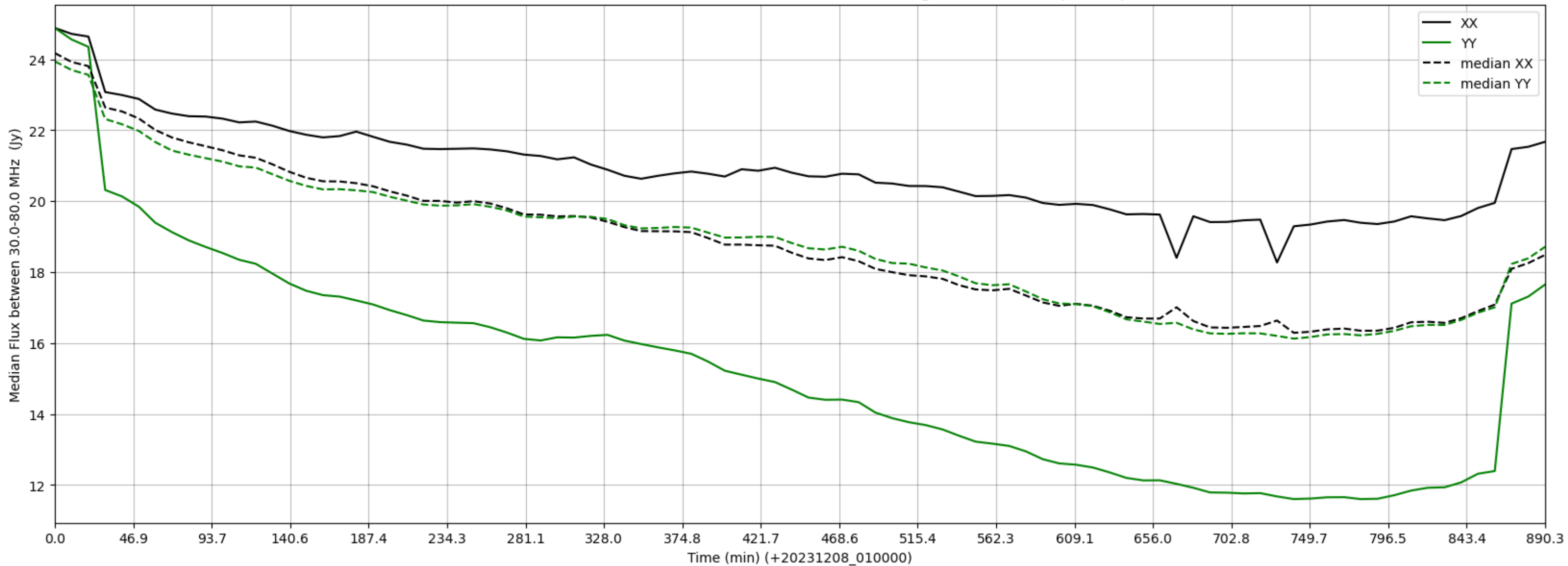
LWA269 - Correlator# 005 - XX FLAGS:Good - YY FLAGS:HighTimeVar+BadSpecShape
