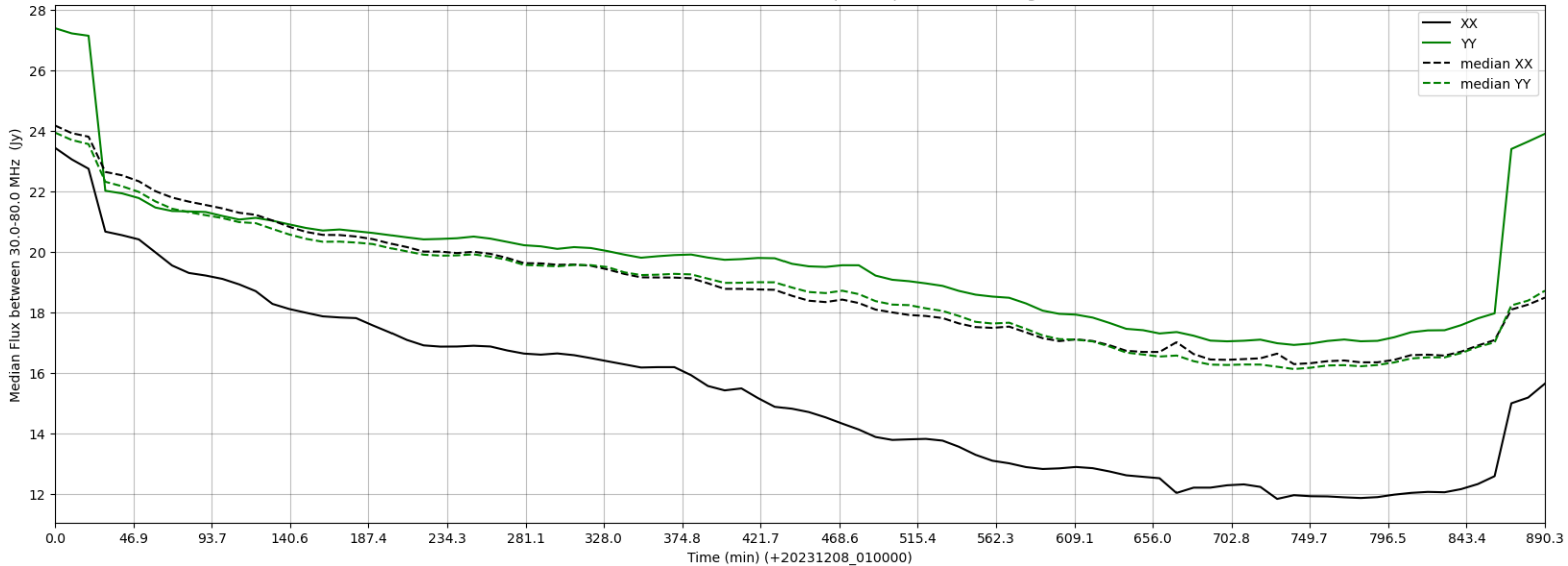
LWA328 - Correlator# 157 - XX FLAGS:BadSpecShape - YY FLAGS:HighTimeVar
