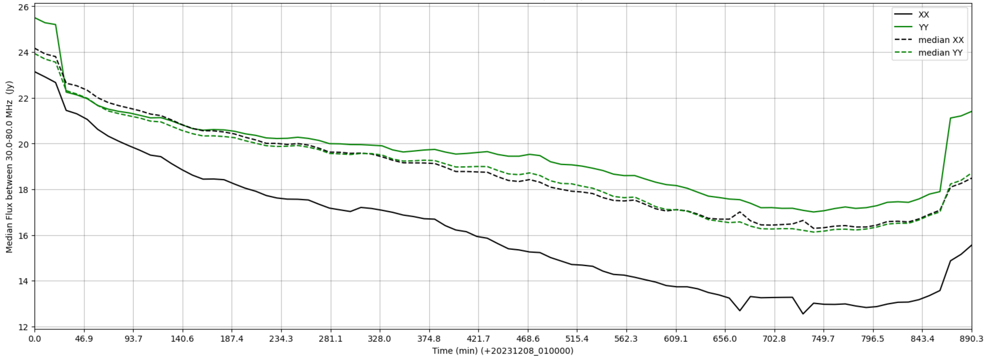
LWA259 - Correlator# 001 - XX FLAGS:BadSpecShape - YY FLAGS:Good
