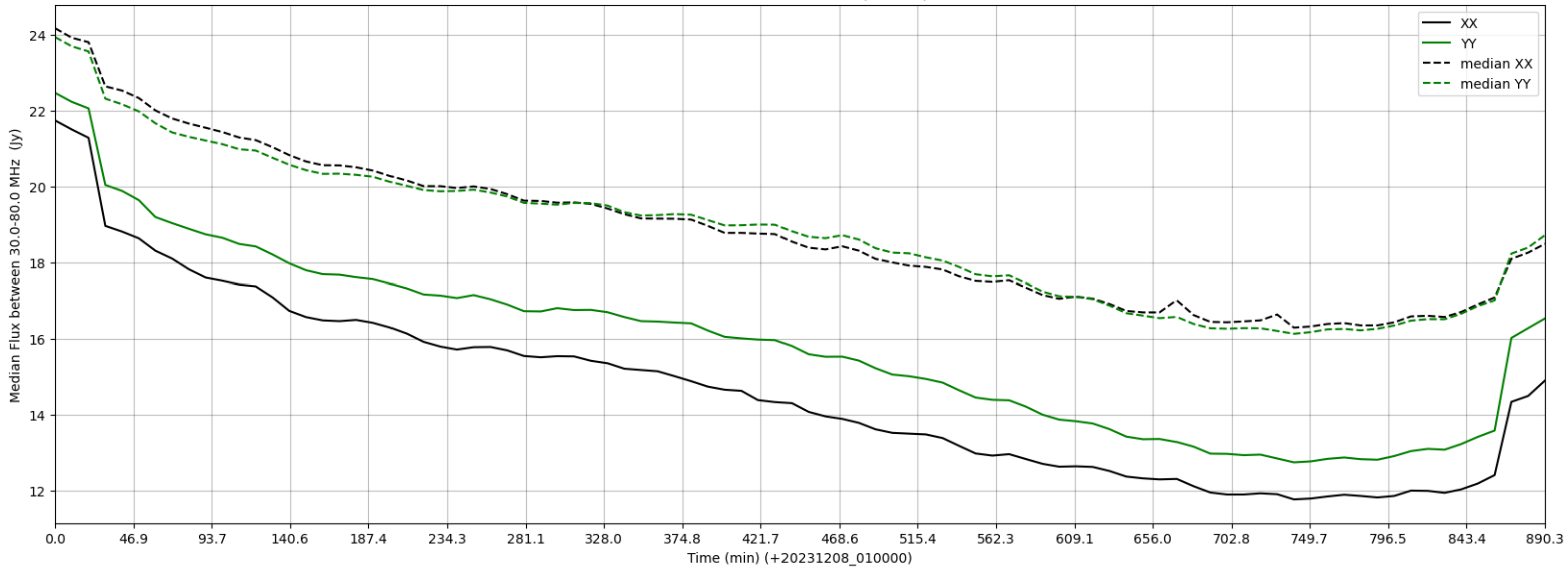
LWA337 - Correlator# 059 - XX FLAGS:BadSpecShape - YY FLAGS:Good
