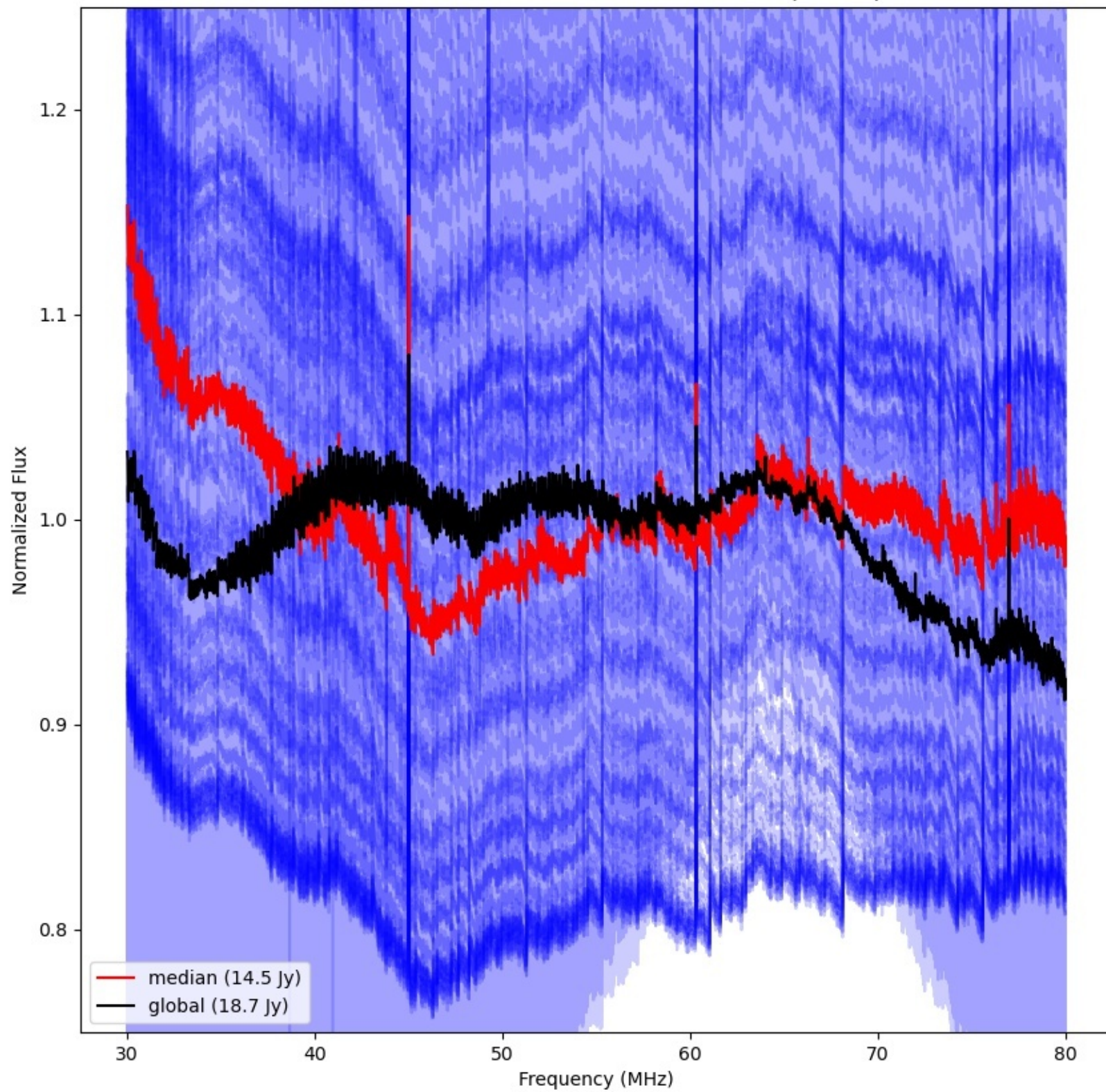
LWA337 - Correlator# 059 - XX - FLAGS:BadSpecShape
