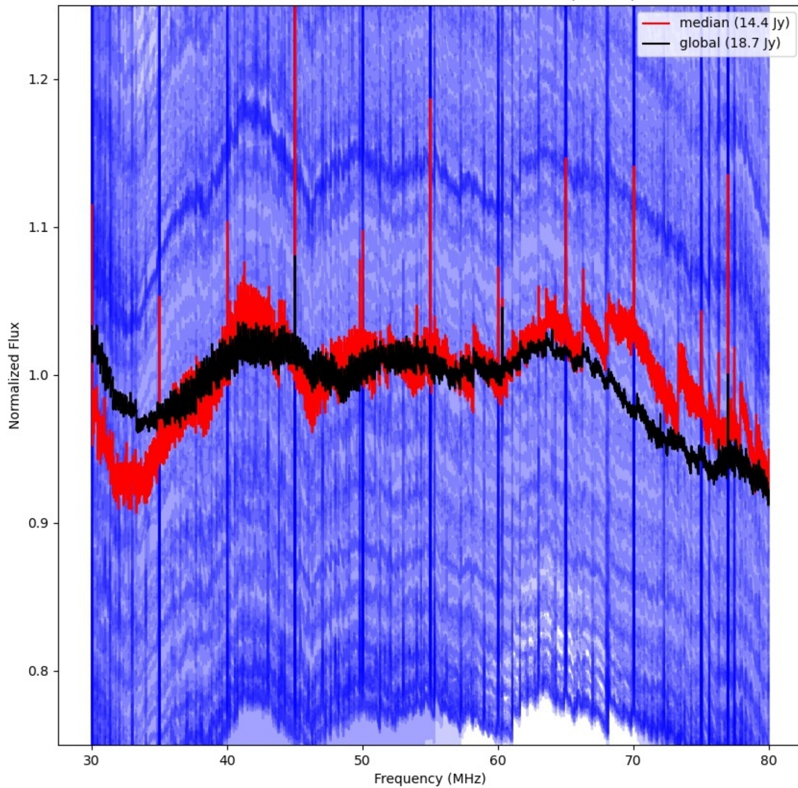
LWA360 - Correlator# 062 - XX - FLAGS:BadSpecShape
