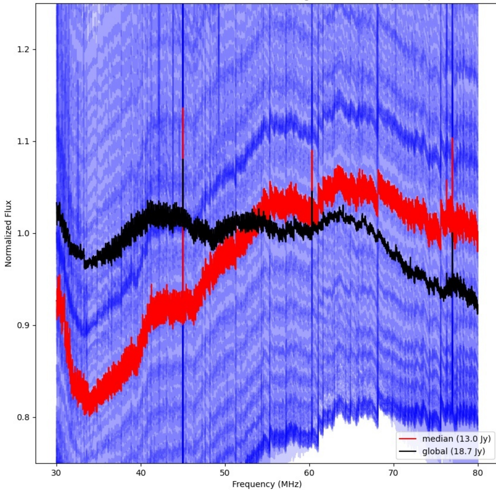
LWA317 - Correlator# 052 - XX - FLAGS:HighTimeVar+BadSpecShape
