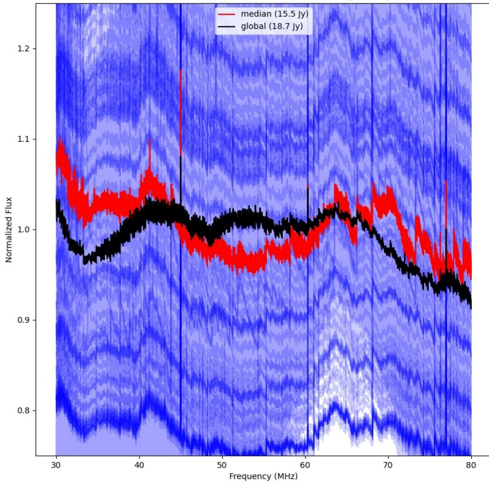
LWA334 - Correlator# 156 - XX - FLAGS:BadSpecShape
