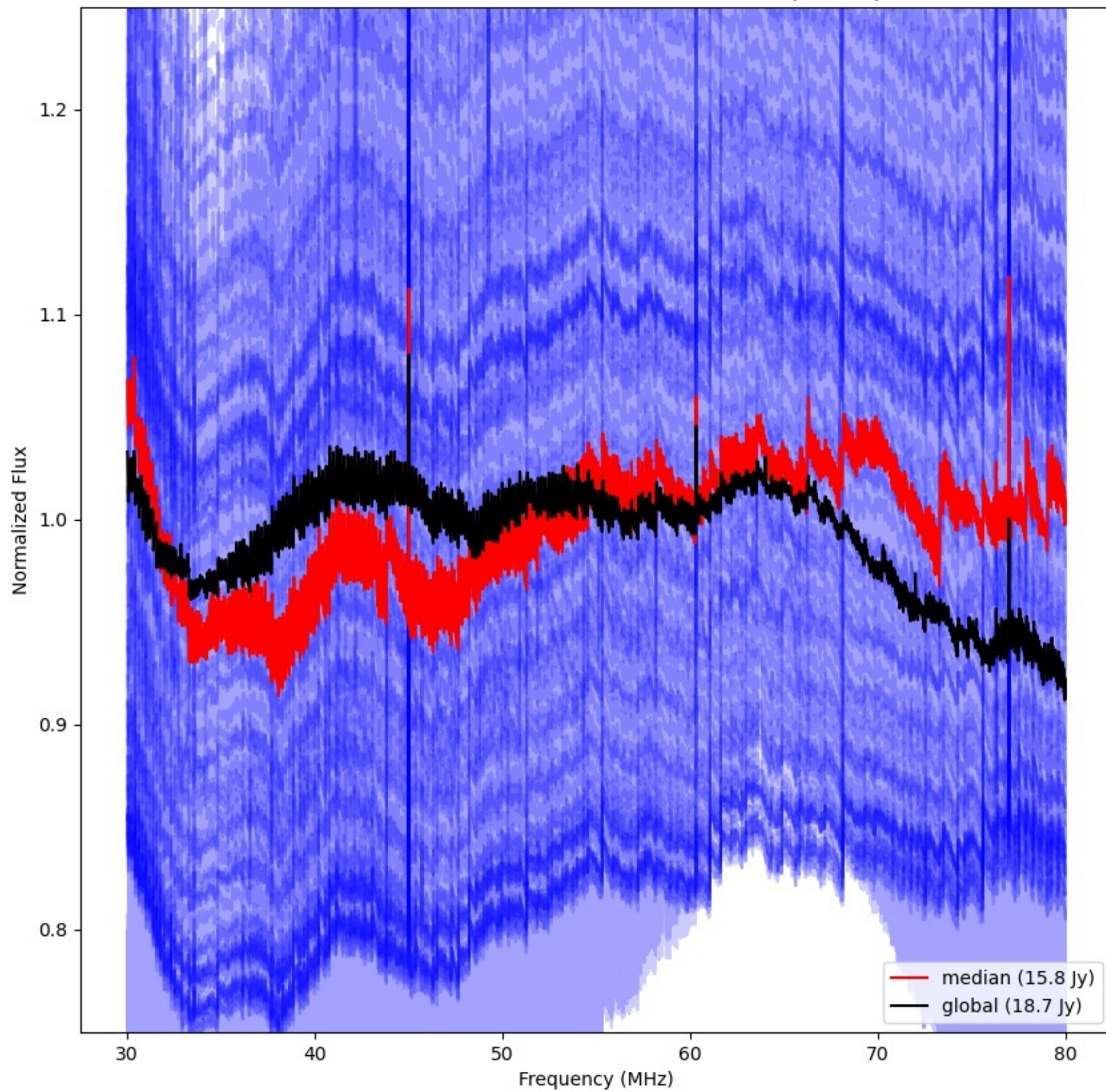
LWA259 - Correlator# 001 - XX - FLAGS:BadSpecShape
