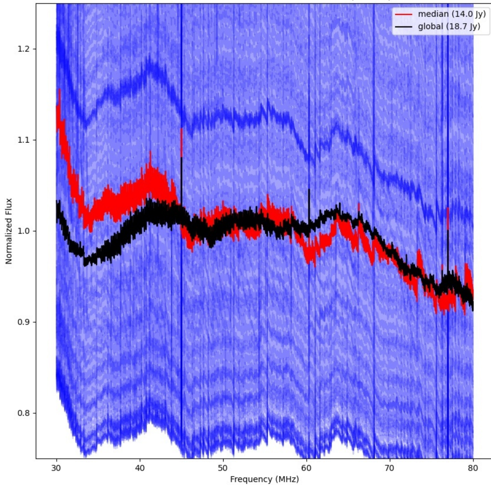
LWA258 - Correlator# 035 - XX - FLAGS:BadSpecShape
