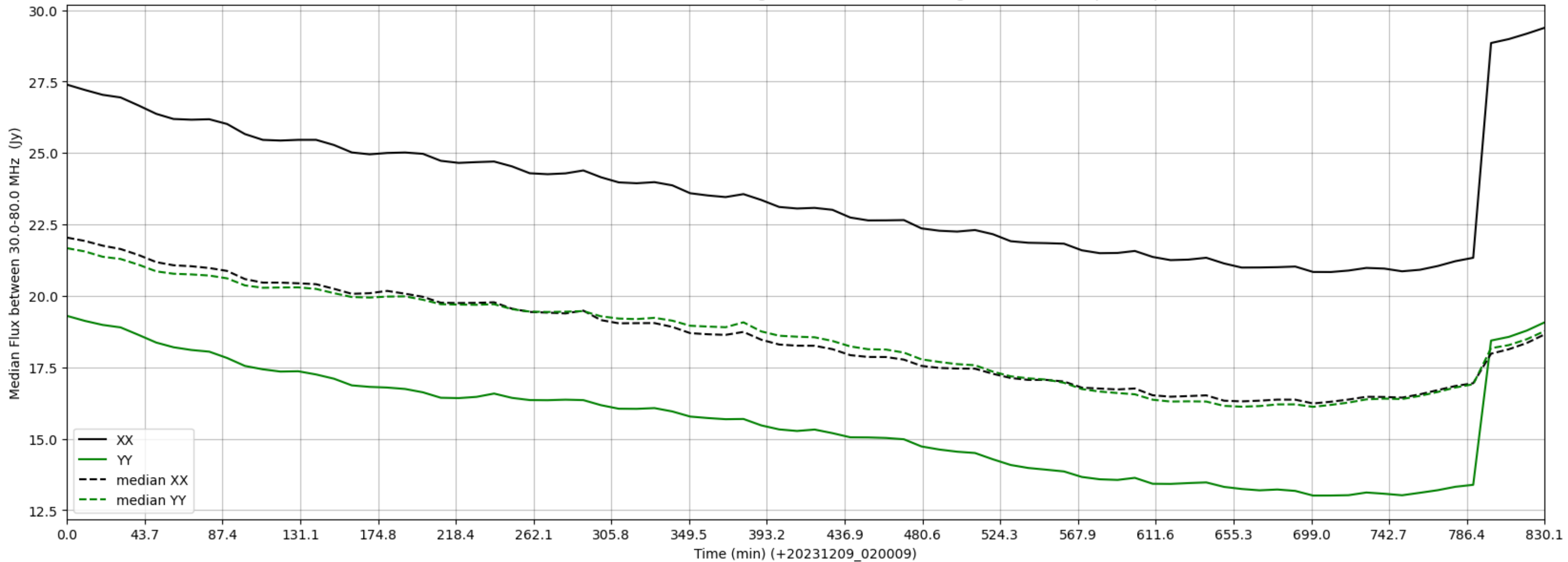
LWA277 - Correlator# 009 - XX FLAGS:HighTimeVar - YY FLAGS:HighTimeVar+BadSpecShape
