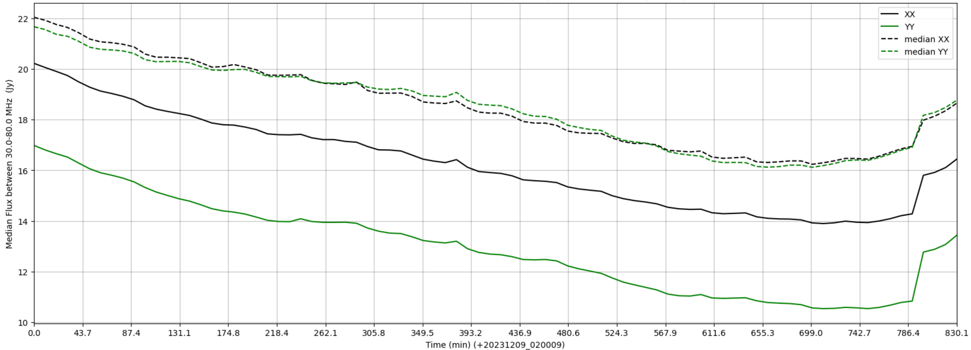
LWA262 - Correlator# 123 - XX FLAGS:BadSpecShape - YY FLAGS:BadSpecShape
