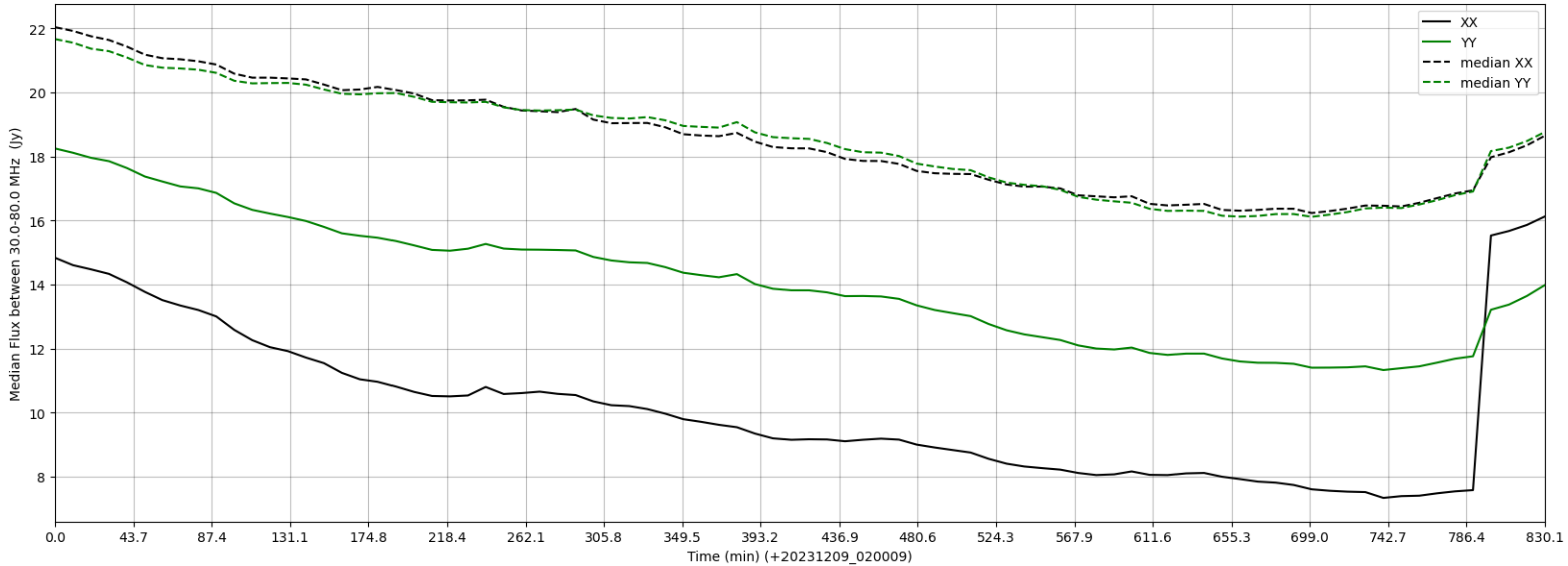
LWA313 - Correlator# 018 - XX FLAGS:HighTimeVar - YY FLAGS:BadSpecShape
