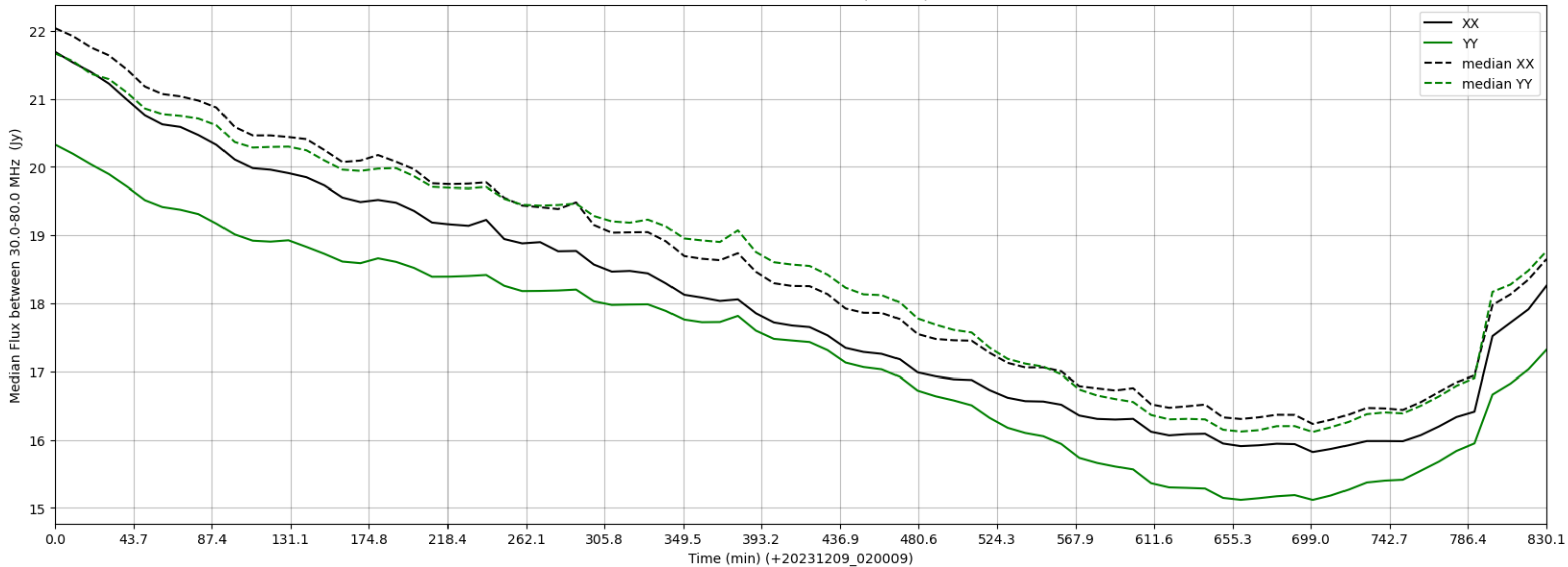
LWA086 - Correlator# 143 - XX FLAGS:BadSpecShape - YY FLAGS:Good
