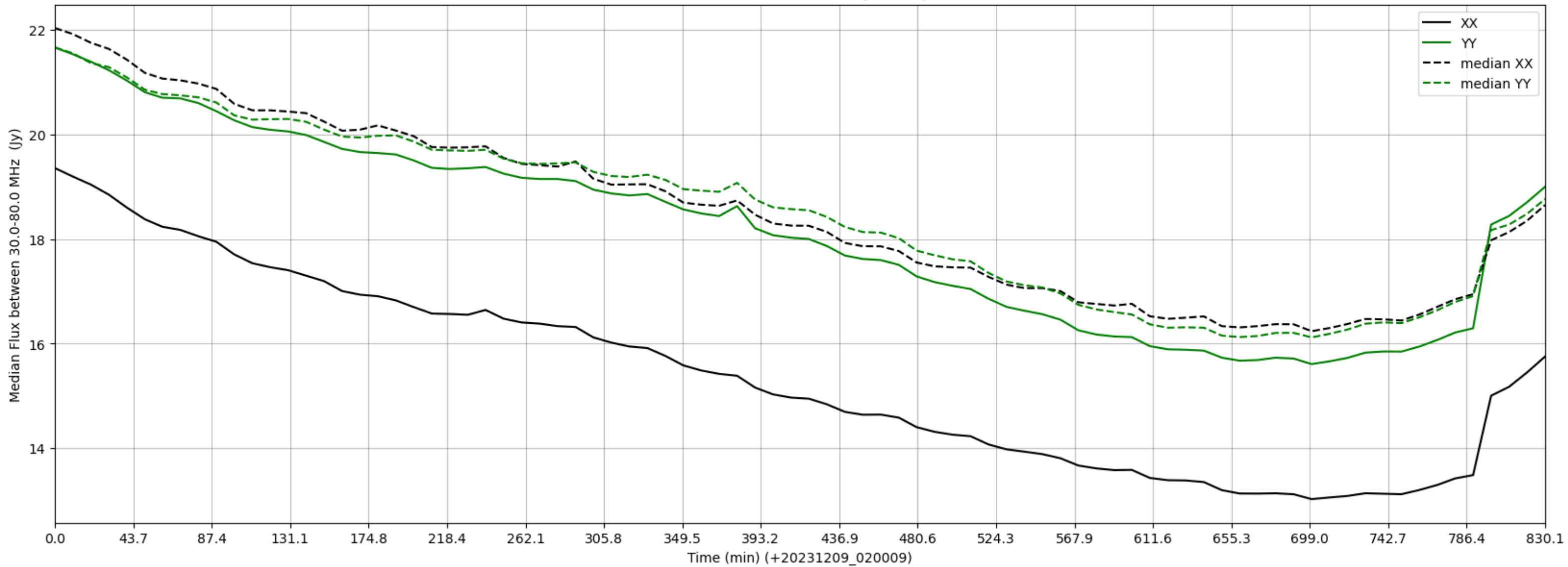
LWA265 - Correlator# 036 - XX FLAGS:BadSpecShape - YY FLAGS:Good
