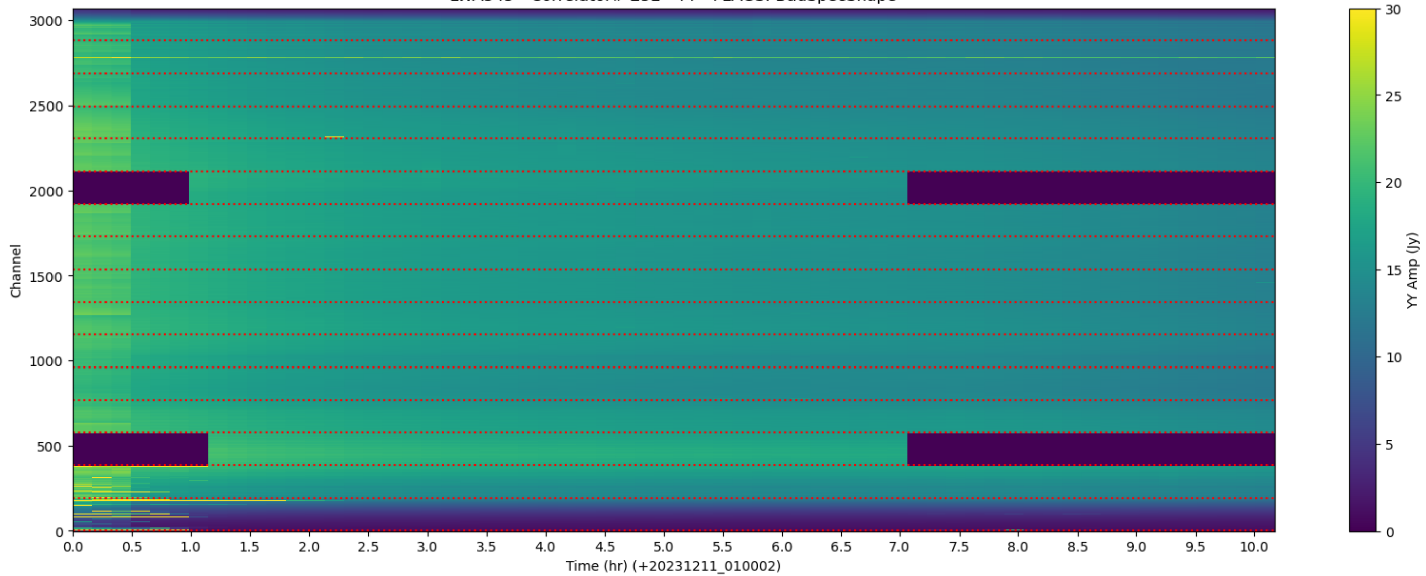
LWA345 - Correlator# 252 - YY - FLAGS: BadSpecShape
