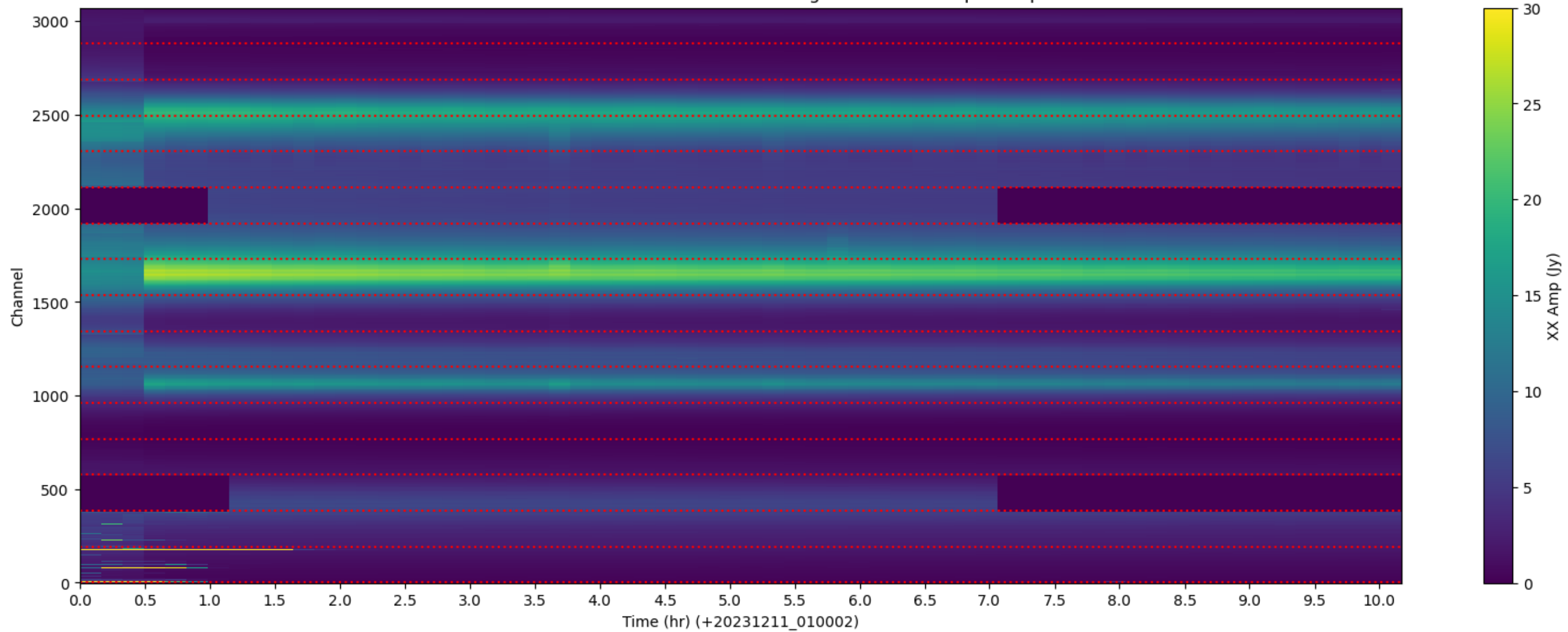
LWA232 - Correlator# 307 - XX - FLAGS: HighTimeVar+BadSpecShape
