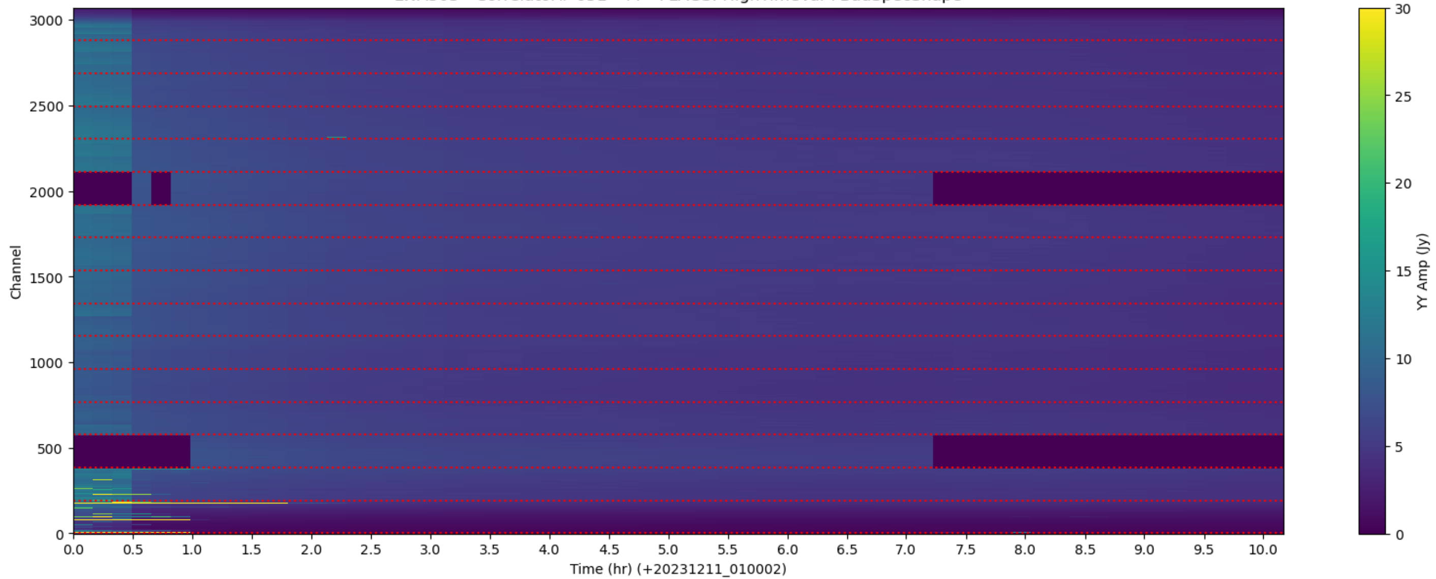
LWA303 - Correlator# 051 - YY - FLAGS: HighTimeVar+BadSpecShape
