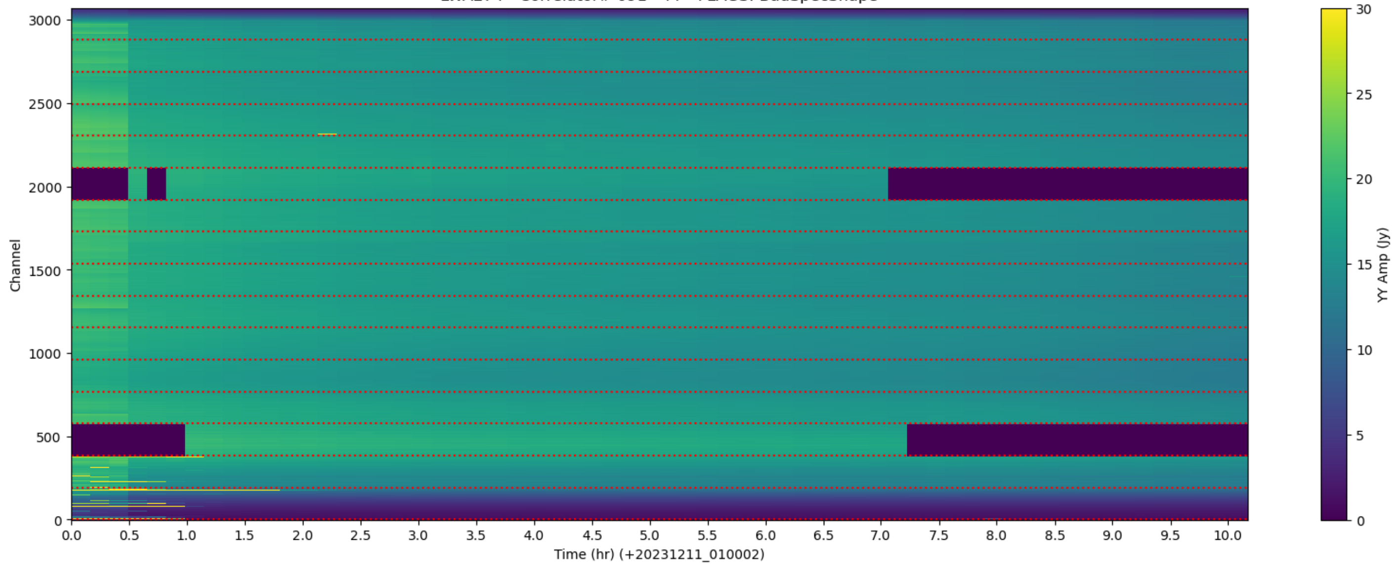
LWA274 - Correlator# 091 - YY - FLAGS: BadSpecShape
