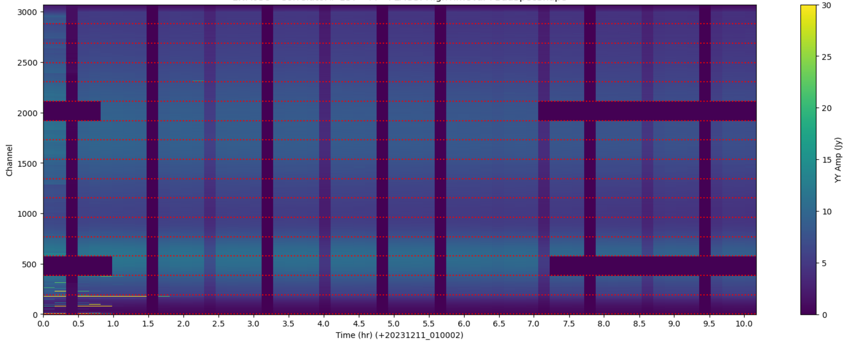
LWA058 - Correlator# 137 - YY - FLAGS: HighTimeVar+BadSpecShape
