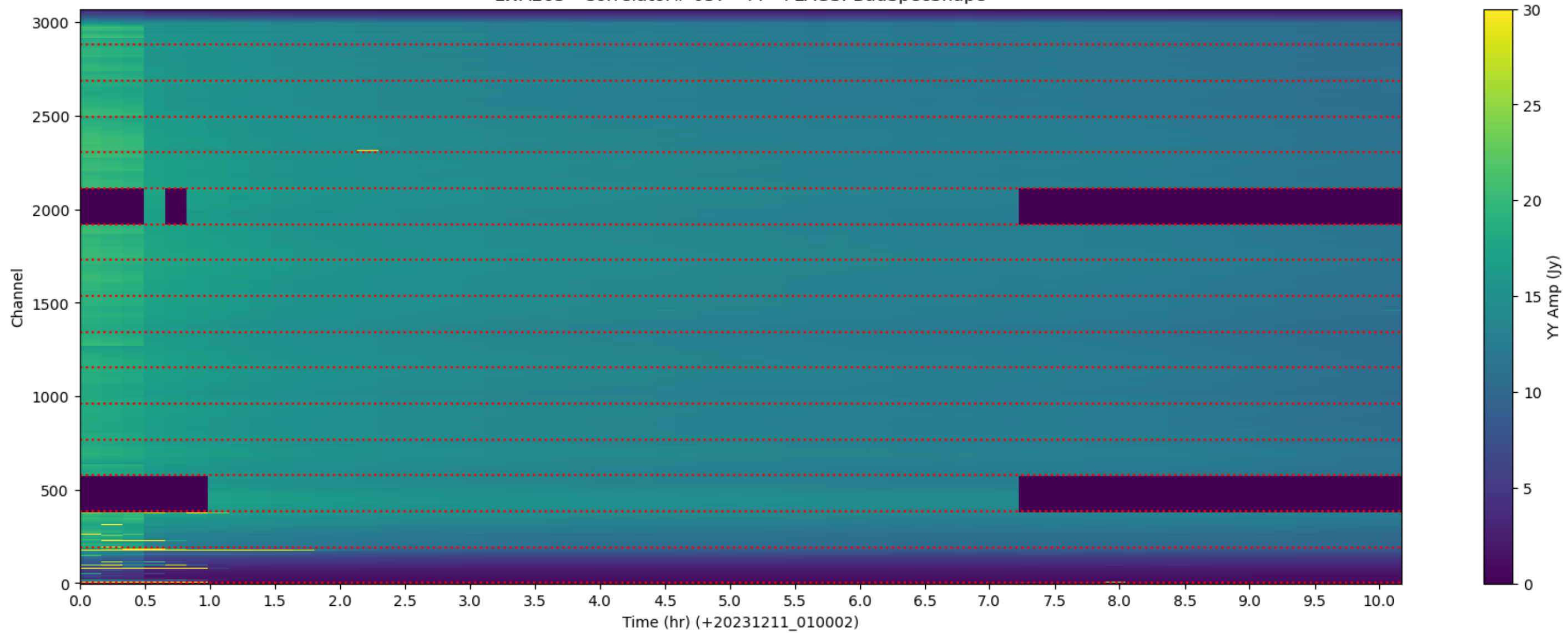
LWA263 - Correlator# 037 - YY - FLAGS: BadSpecShape
