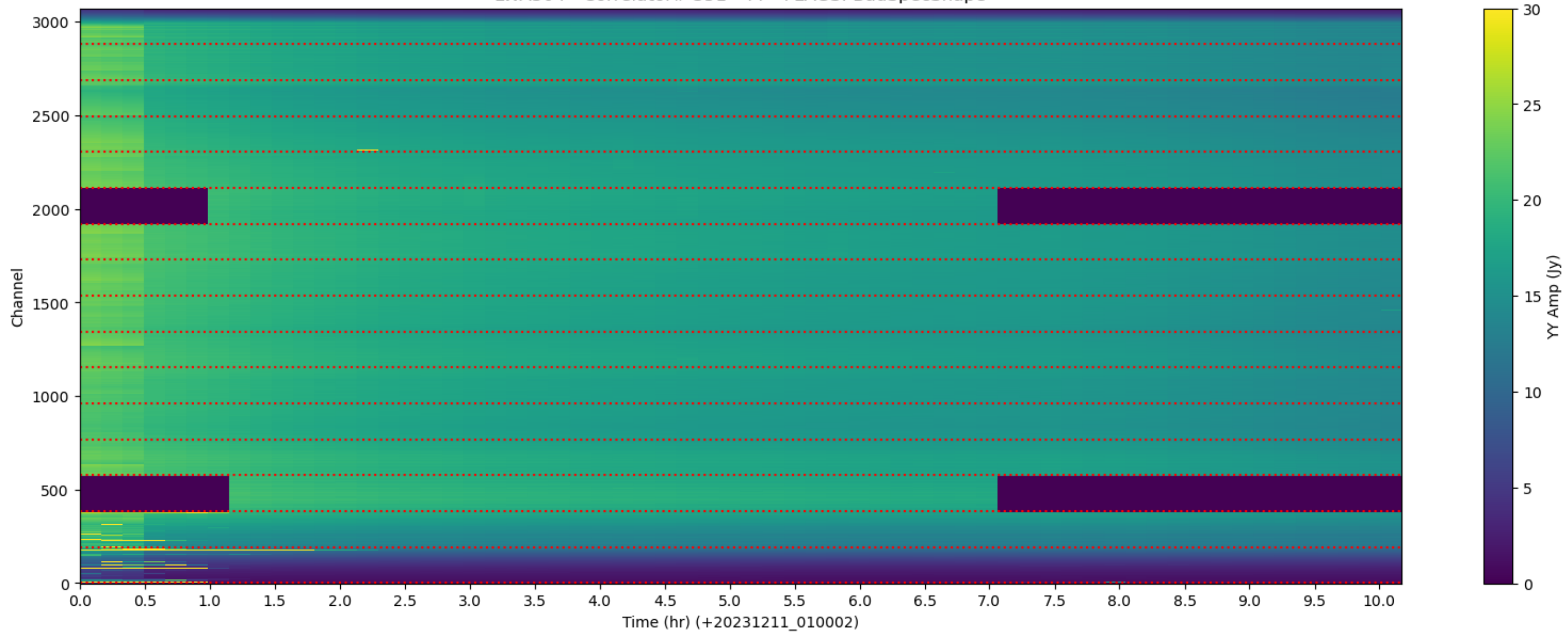
LWA304 - Correlator# 351 - YY - FLAGS: BadSpecShape
