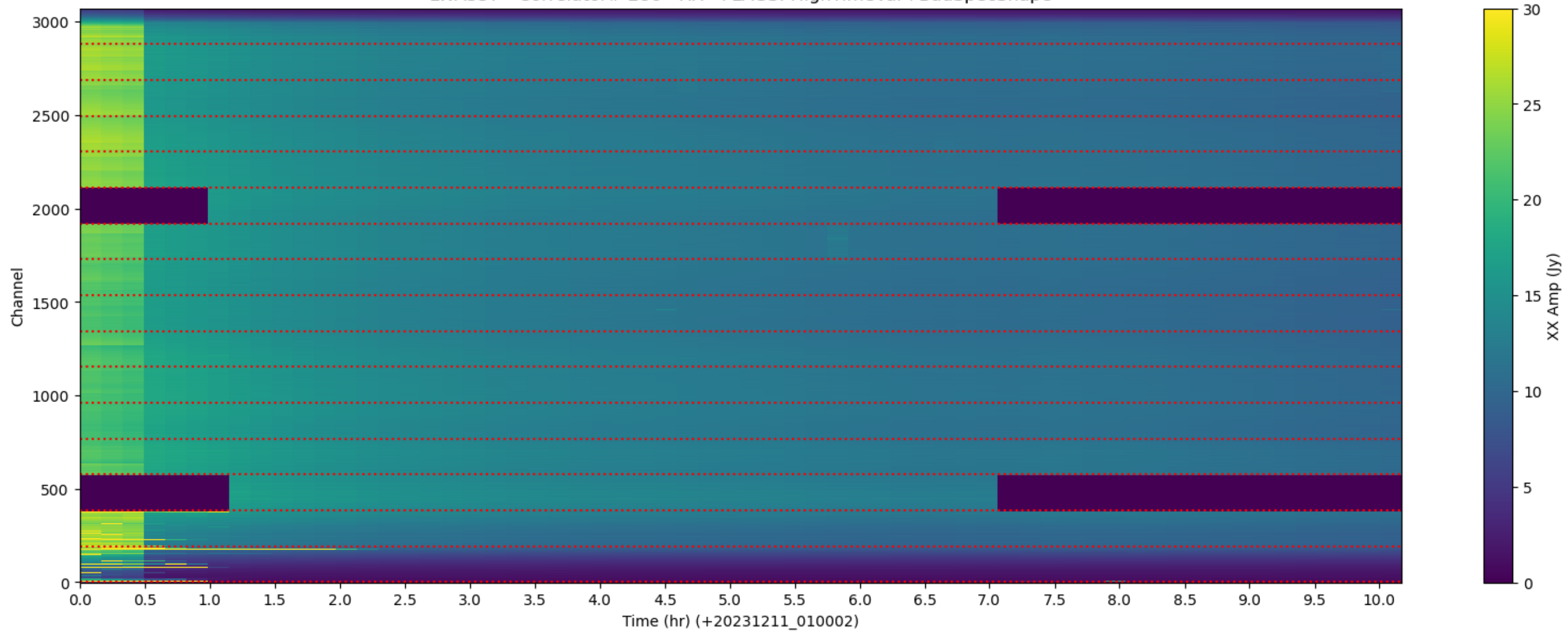
LWA357 - Correlator# 286 - XX - FLAGS: HighTimeVar+BadSpecShape
