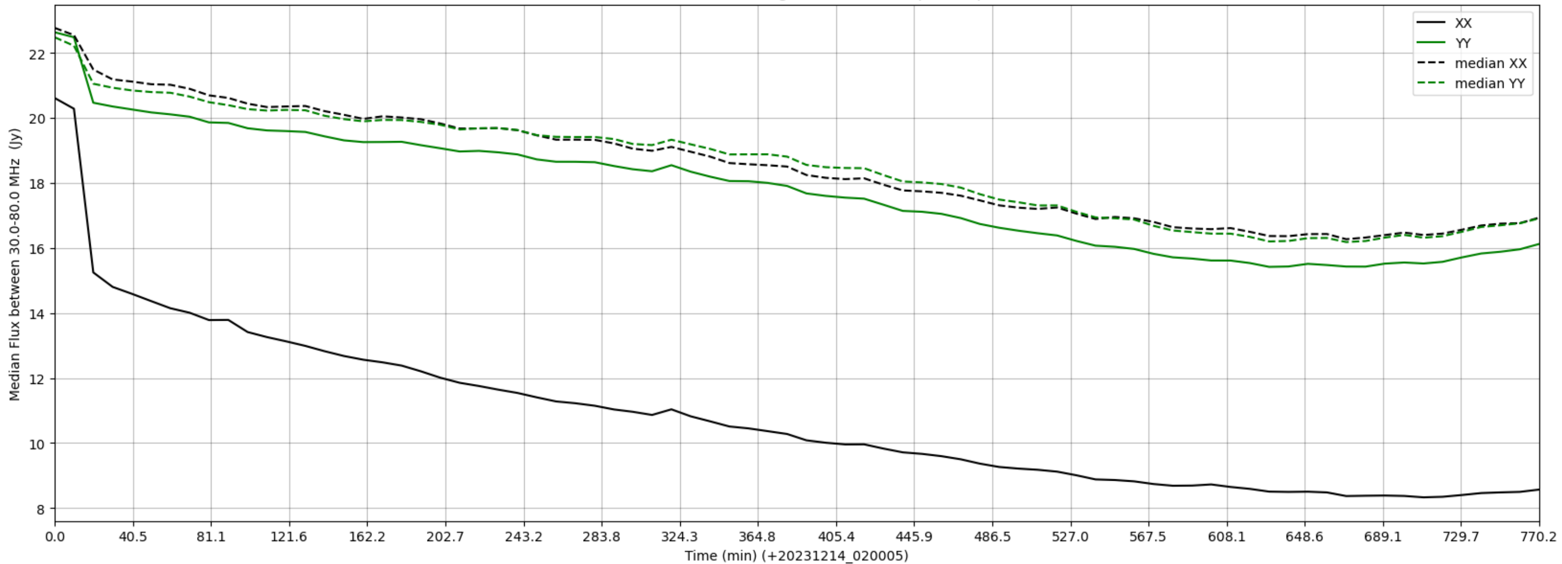
LWA357 - Correlator# 286 - XX FLAGS:HighTimeVar+BadSpecShape - YY FLAGS:Good
