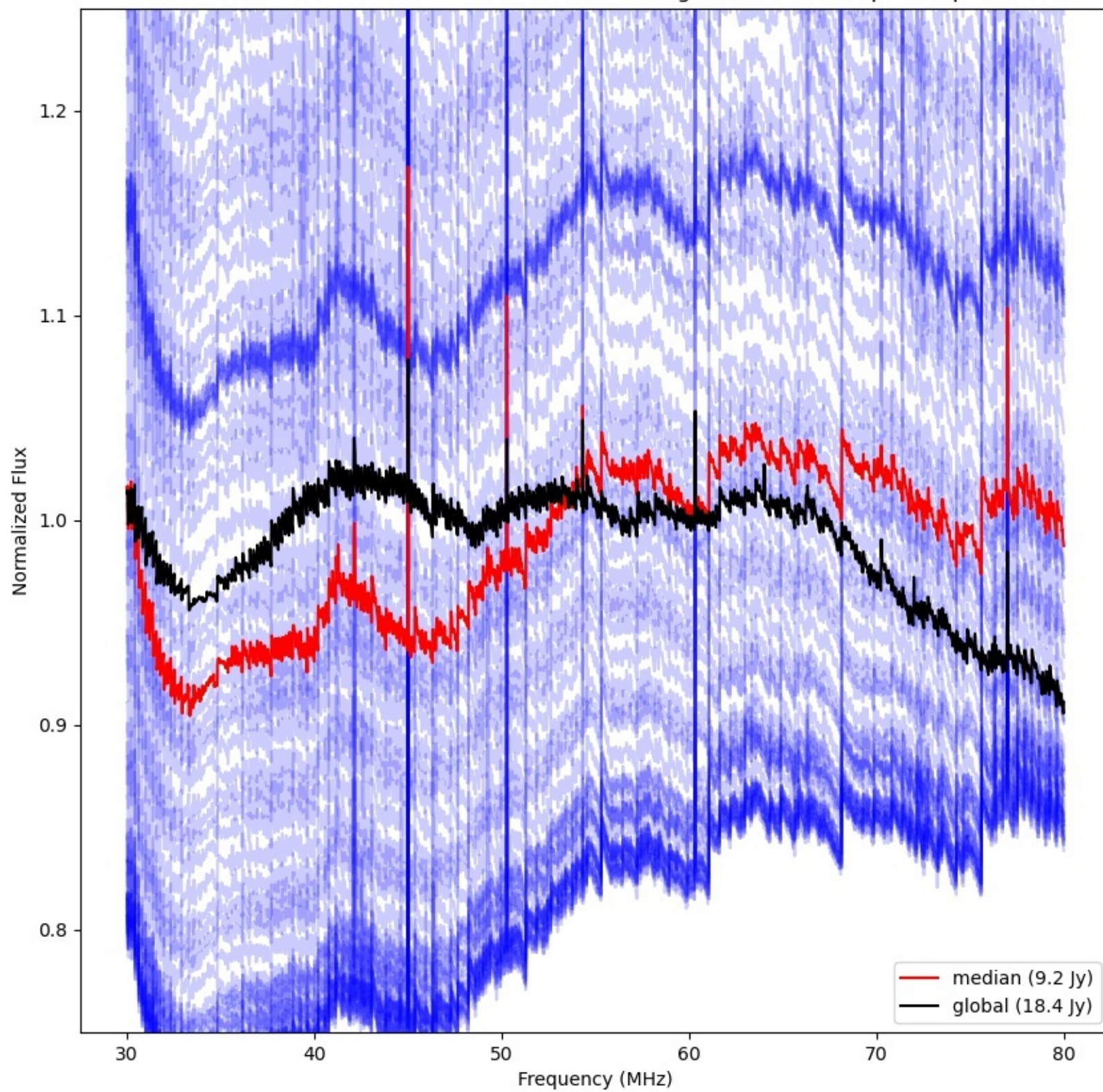
LWA313 - Correlator# 018 - XX - FLAGS:HighTimeVar+BadSpecShape
