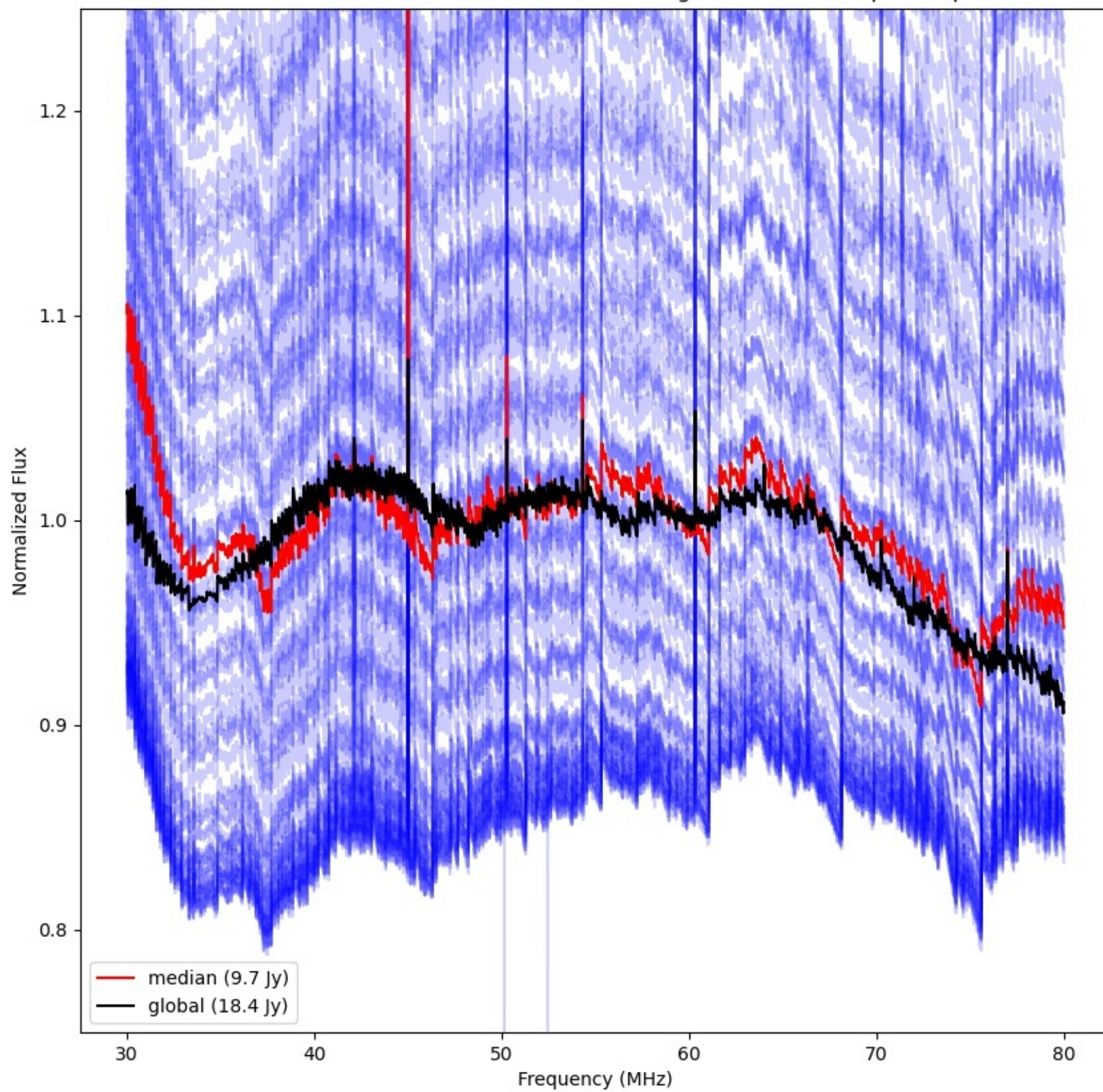
LWA283 - Correlator# 040 - XX - FLAGS:HighTimeVar+BadSpecShape
