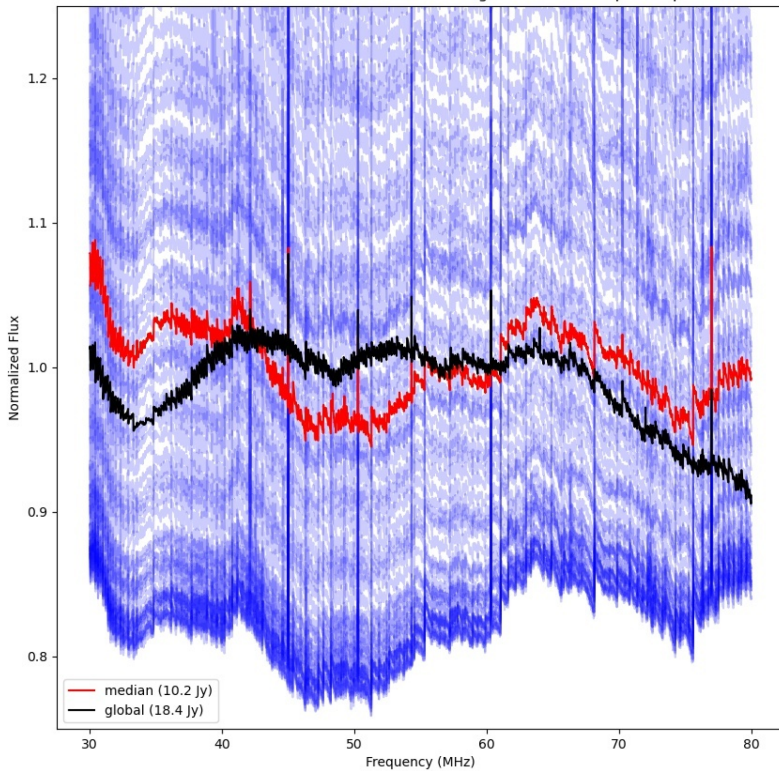
LWA357 - Correlator# 286 - XX - FLAGS:HighTimeVar+BadSpecShape
