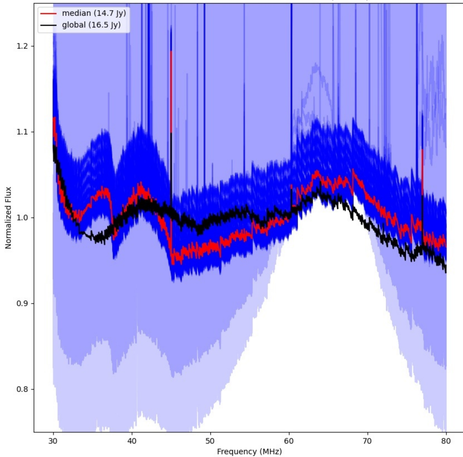
LWA262 - Correlator# 123 - XX - FLAGS:BadSpecShape
