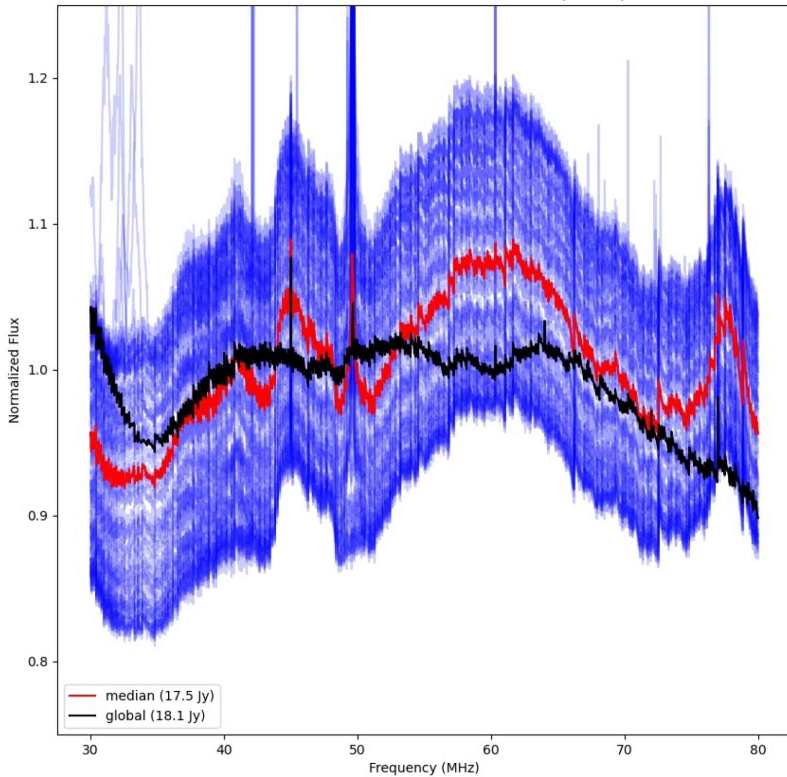
LWA005 - Correlator# 069 - YY - FLAGS:BadSpecShape
