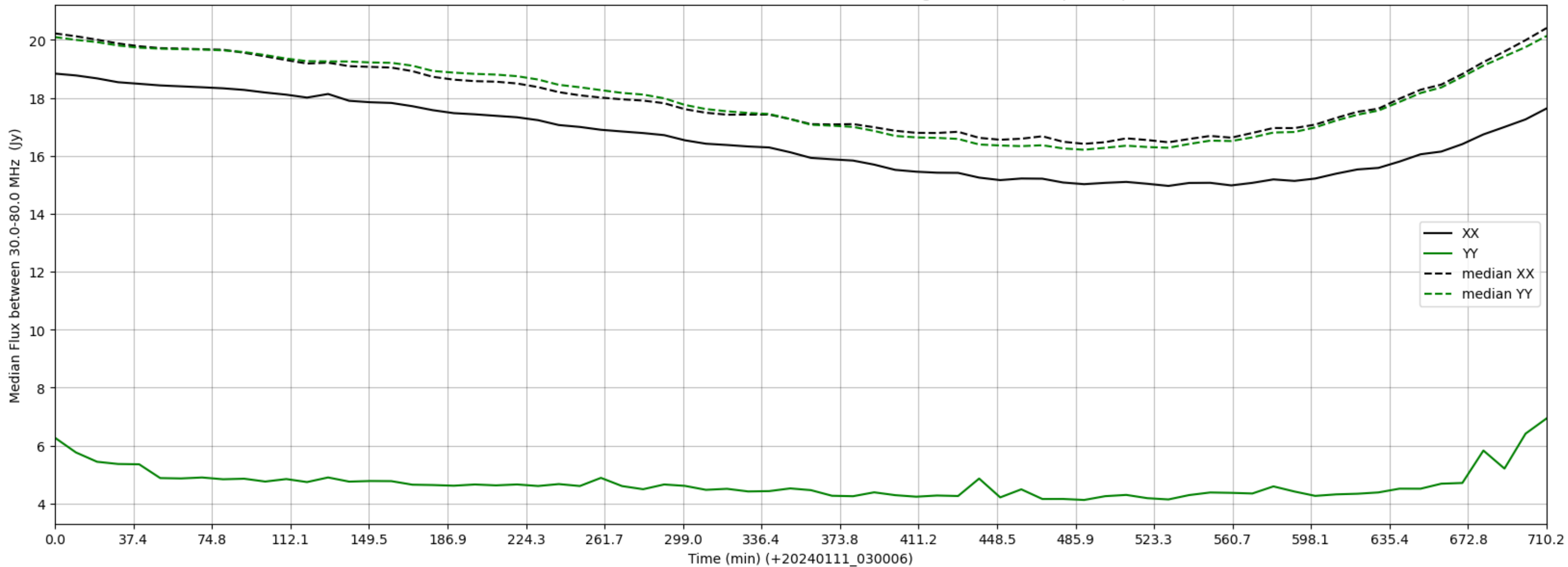
LWA280 - Correlator# 041 - XX FLAGS:Good - YY FLAGS:HighTimeVar+BadSpecShape
