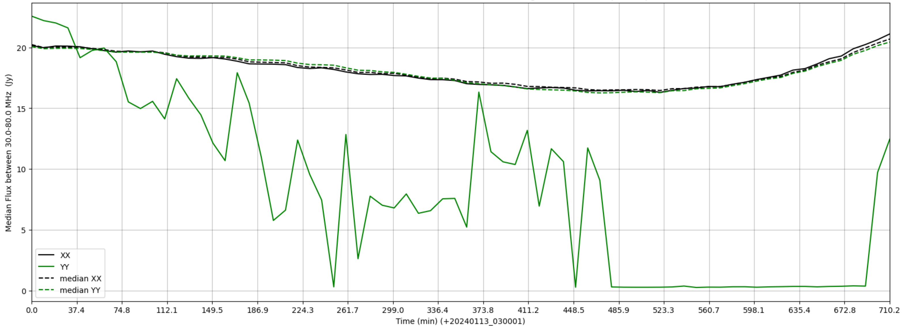
LWA044 - Correlator# 080 - XX FLAGS:Good - YY FLAGS:HighTimeVar+BadSpecShape
