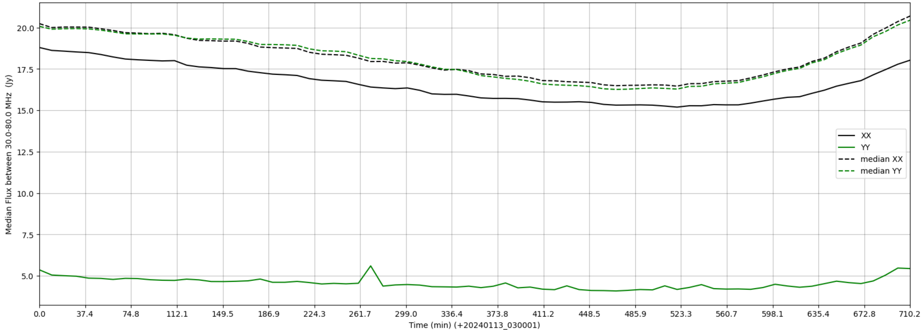
LWA280 - Correlator# 041 - XX FLAGS:BadSpecShape - YY FLAGS:BadSpecShape
