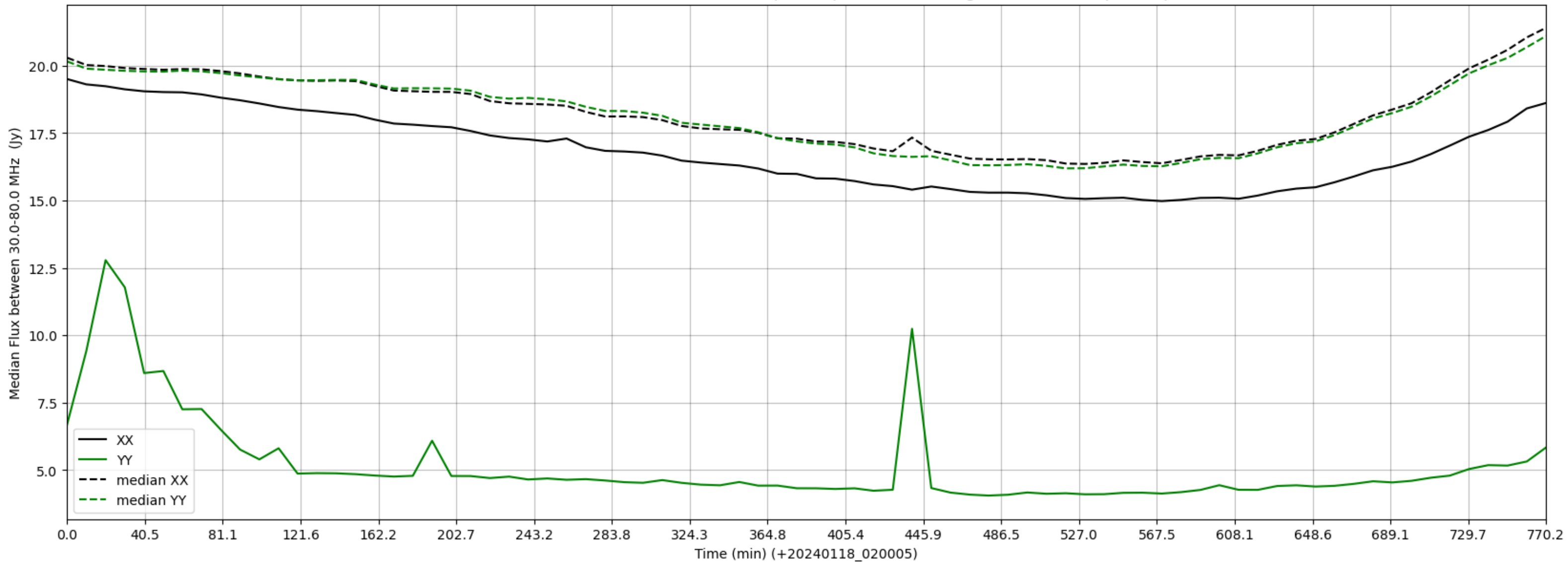
LWA280 - Correlator# 041 - XX FLAGS:BadSpecShape - YY FLAGS:HighTimeVar+BadSpecShape
