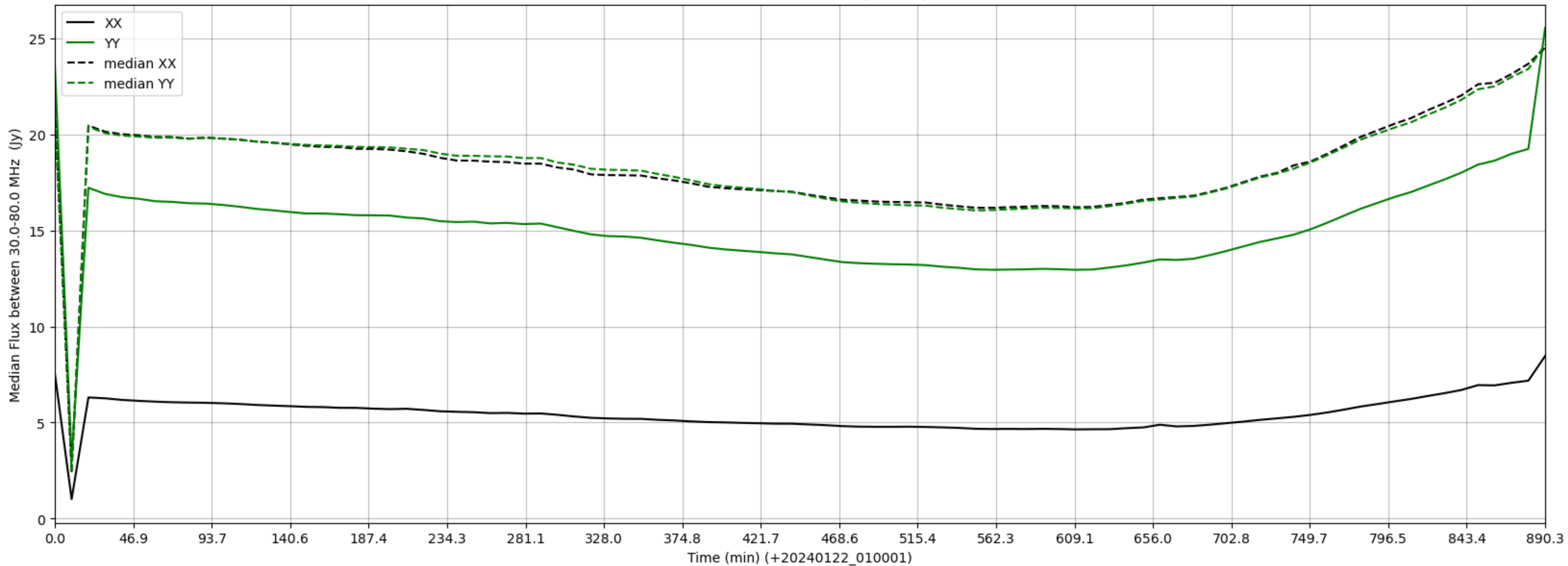
LWA335 - Correlator# 057 - XX FLAGS:BadSpecShape - YY FLAGS:Good
