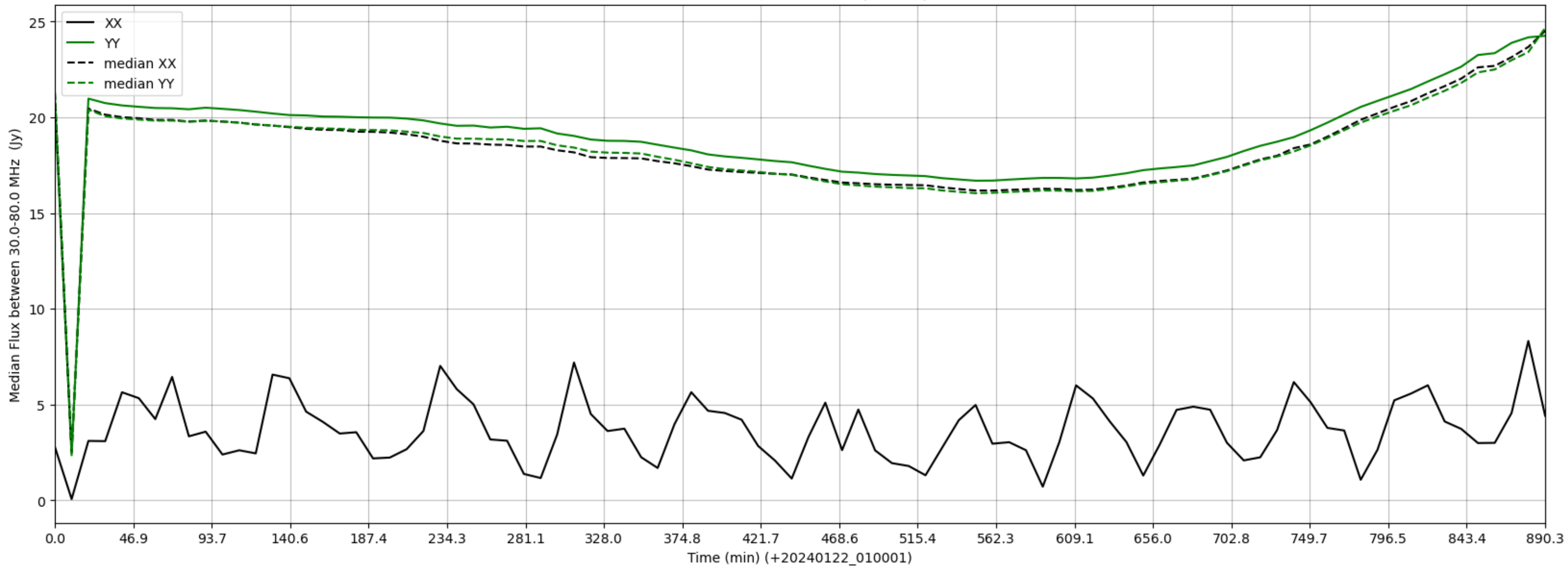
LWA124 - Correlator# 224 - XX FLAGS:BadSpecShape - YY FLAGS:Good
