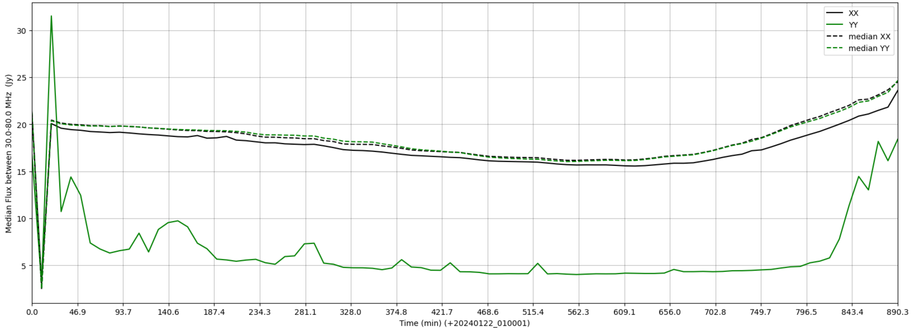
LWA280 - Correlator# 041 - XX FLAGS:BadSpecShape - YY FLAGS:HighTimeVar+BadSpecShape
