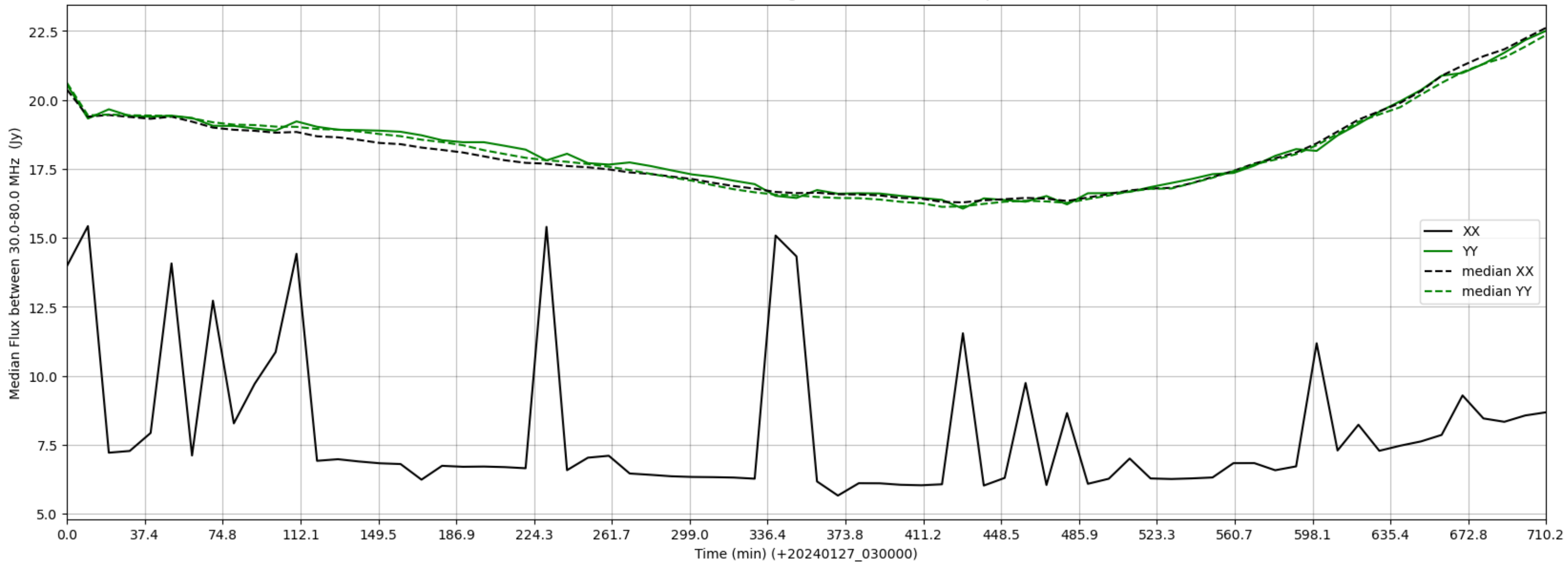
LWA105 - Correlator# 178 - XX FLAGS:HighTimeVar+BadSpecShape - YY FLAGS:Good
