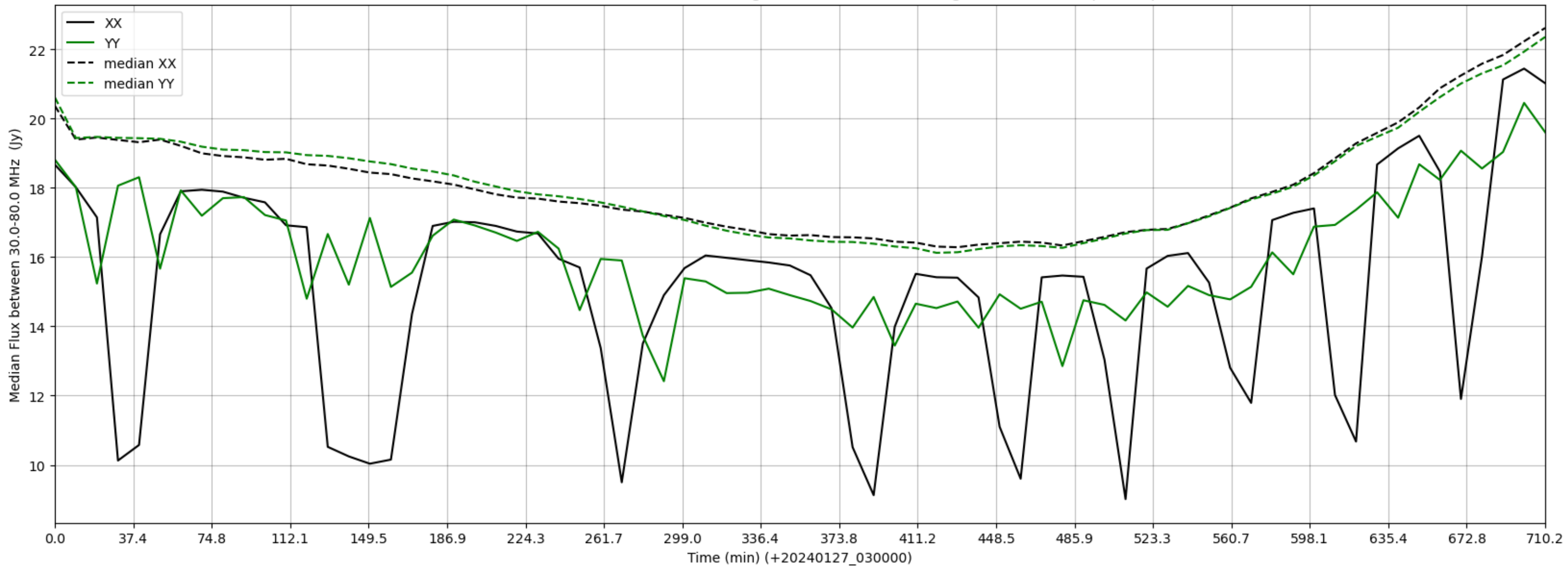
LWA120 - Correlator# 208 - XX FLAGS:HighTimeVar - YY FLAGS:HighTimeVar+BadSpecShape
