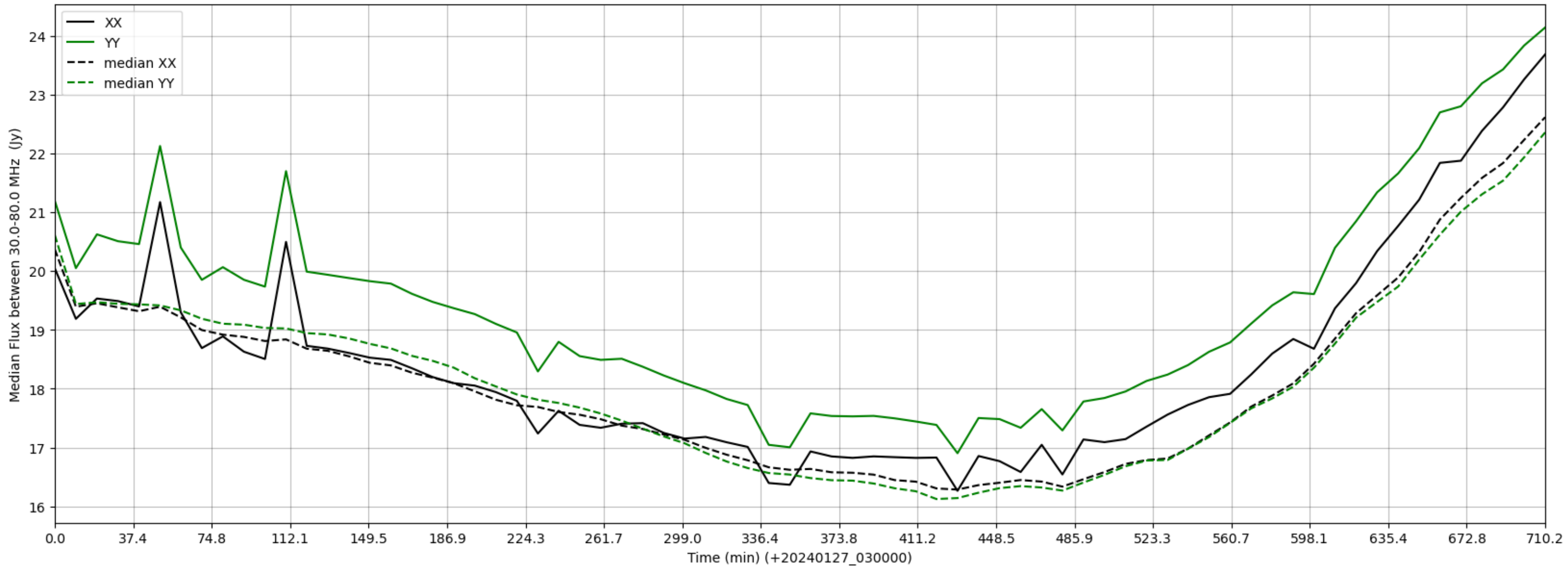
LWA103 - Correlator# 176 - XX FLAGS:Good - YY FLAGS:BadSpecShape
