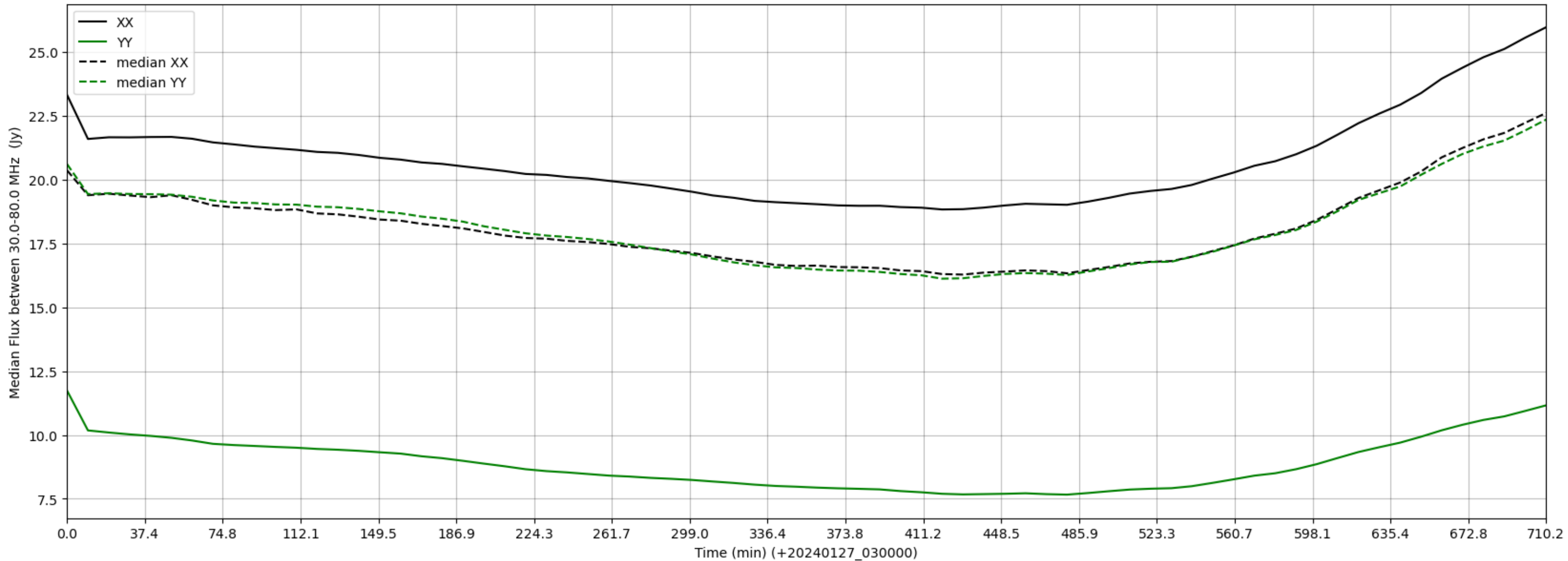
LWA319 - Correlator# 190 - XX FLAGS:Good - YY FLAGS:BadSpecShape
