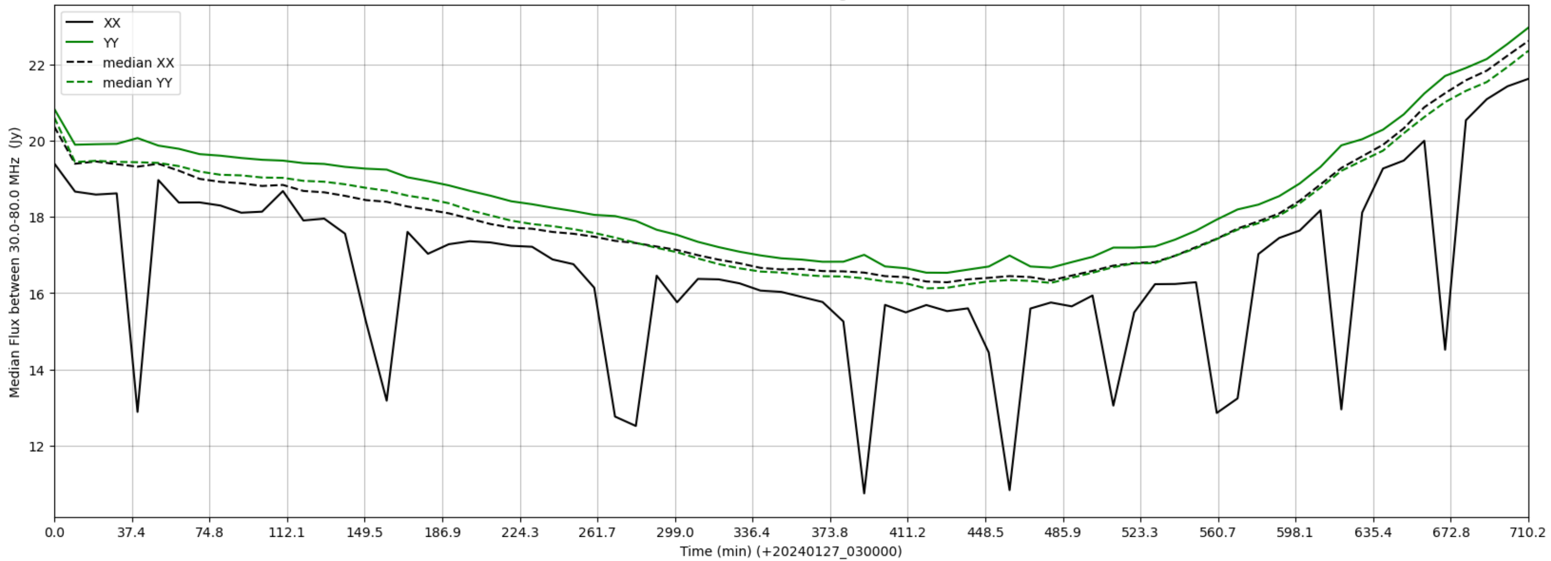
LWA151 - Correlator# 218 - XX FLAGS:HighTimeVar - YY FLAGS:Good
