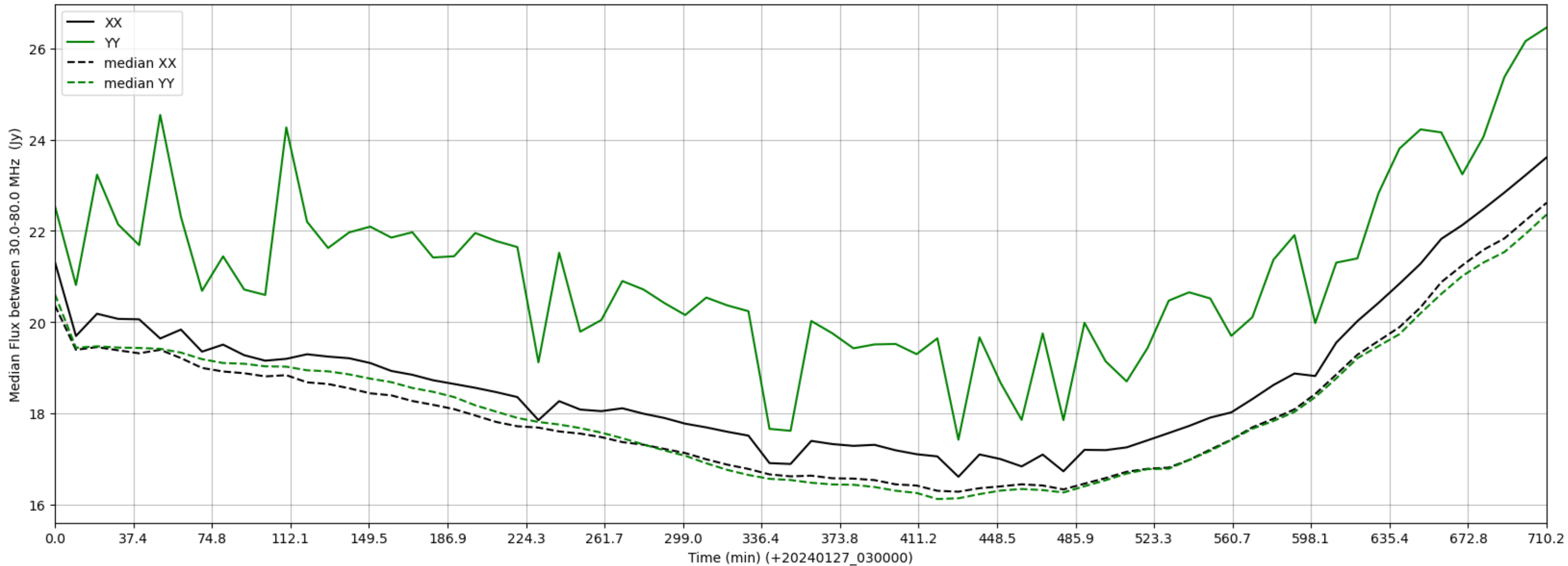
LWA037 - Correlator# 181 - XX FLAGS:BadSpecShape - YY FLAGS:HighTimeVar+BadSpecShape
