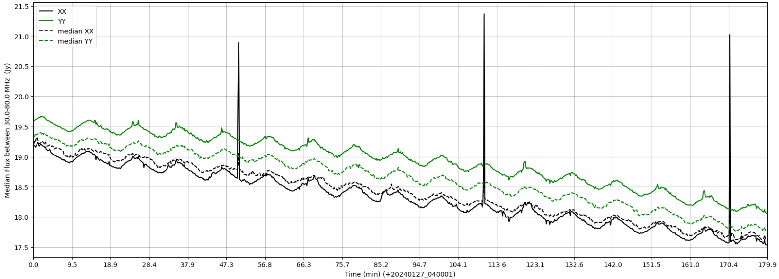
LWA042 - Correlator# 078 - XX FLAGS:HighTimeVar - YY FLAGS:Good
