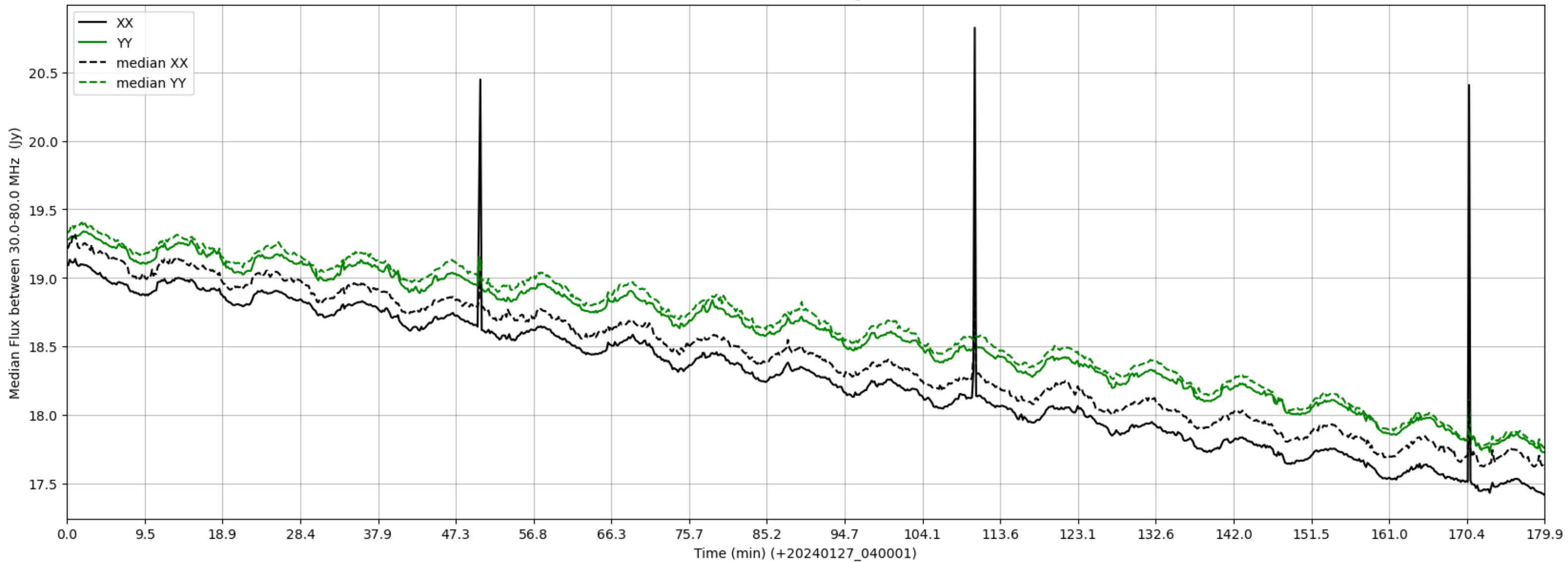
LWA243 - Correlator# 330 - XX FLAGS:HighTimeVar - YY FLAGS:Good
