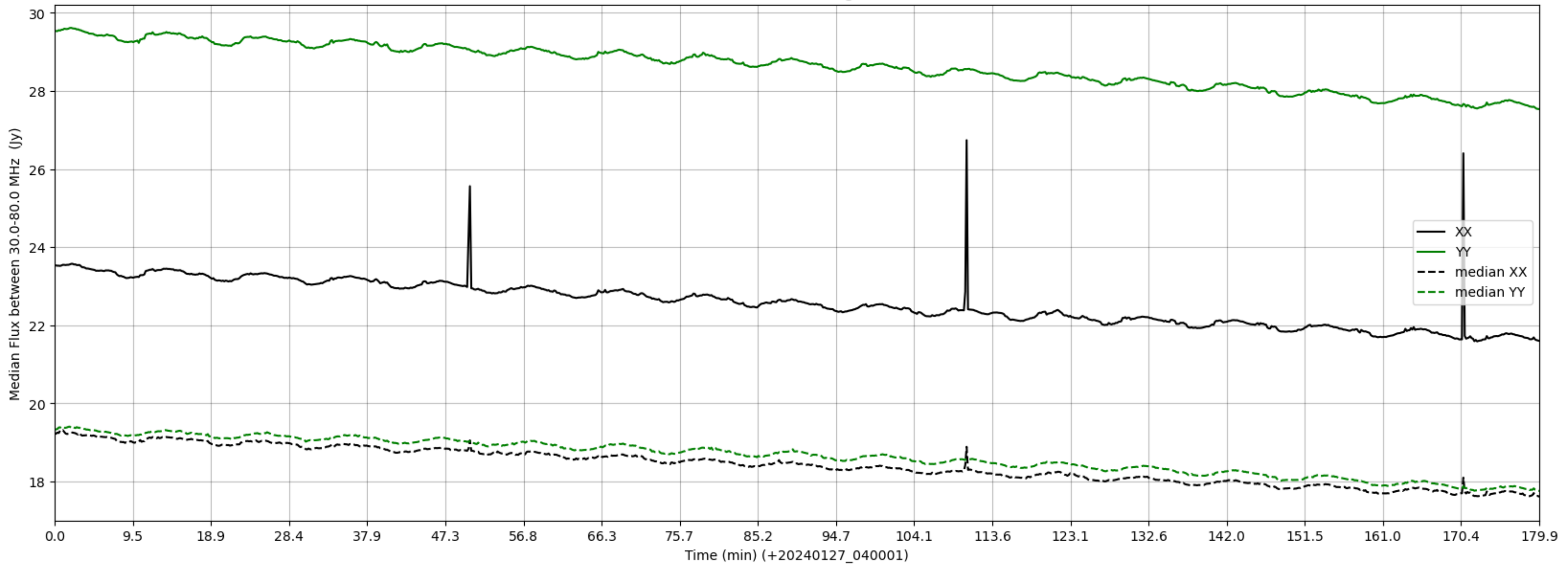
LWA195 - Correlator# 272 - XX FLAGS:HighTimeVar - YY FLAGS:Good
