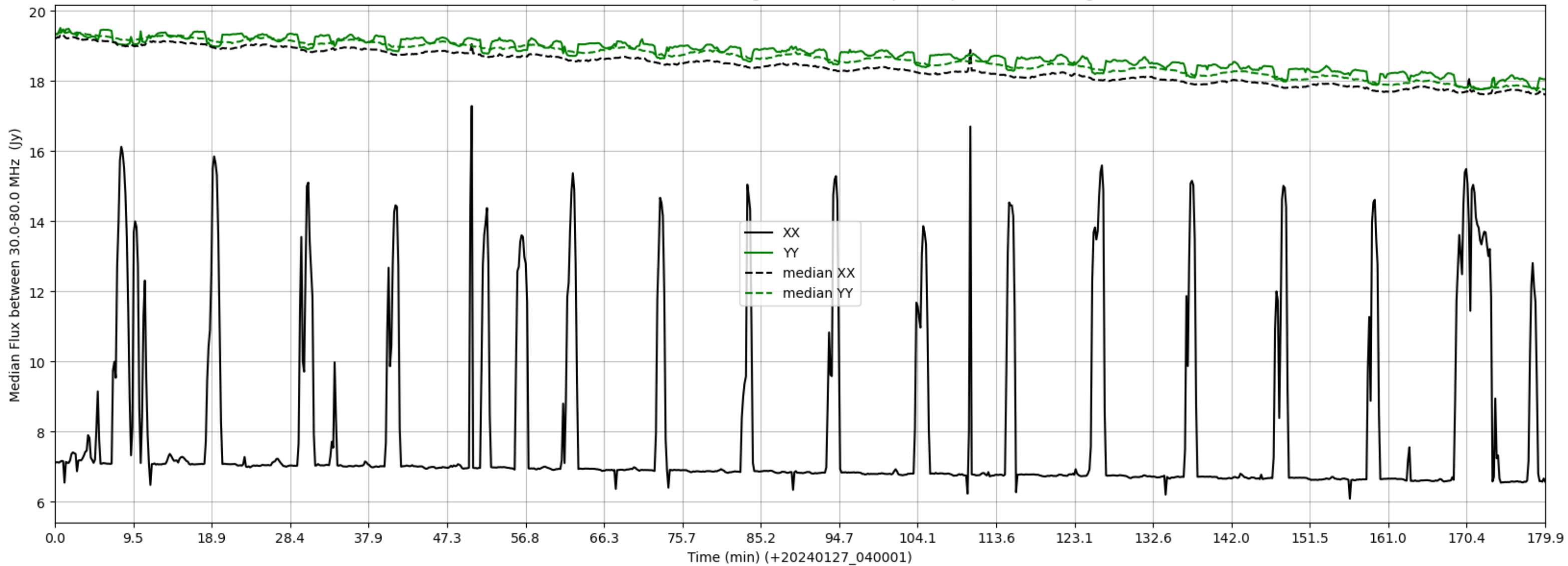
LWA105 - Correlator# 178 - XX FLAGS:HighTimeVar+BadSpecShape - YY FLAGS:HighTimeVar
