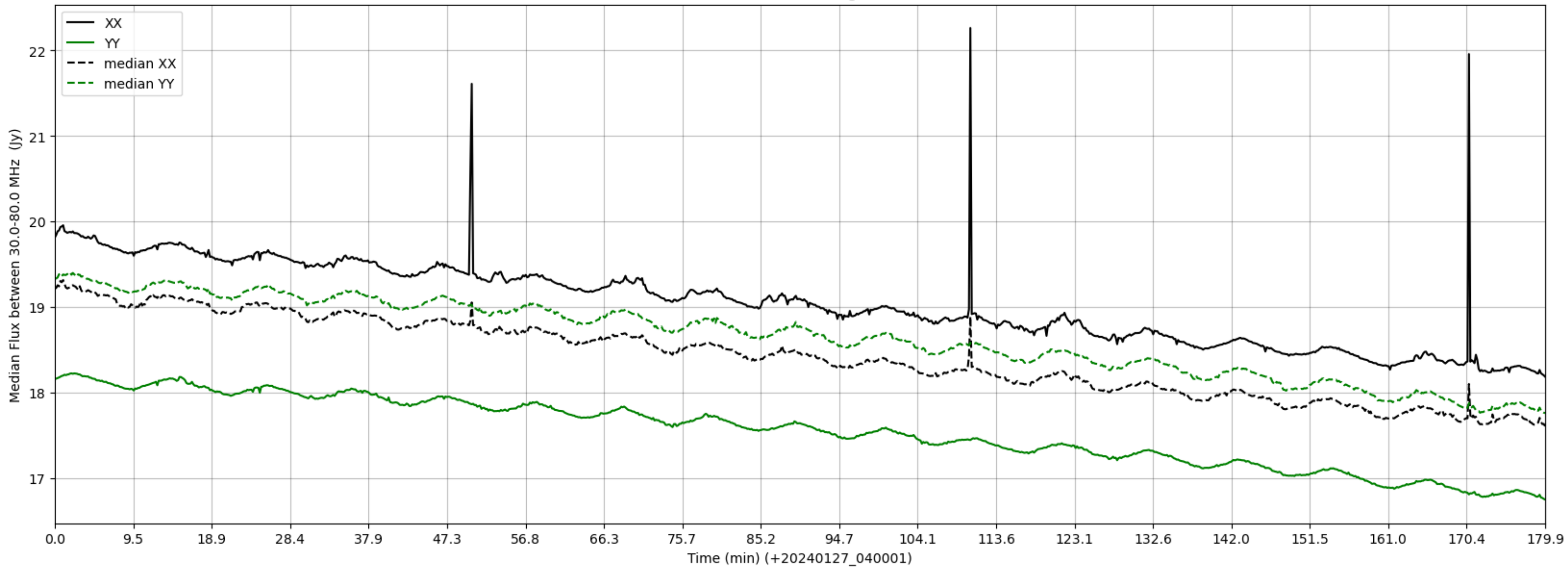
LWA021 - Correlator# 105 - XX FLAGS:HighTimeVar - YY FLAGS:Good
