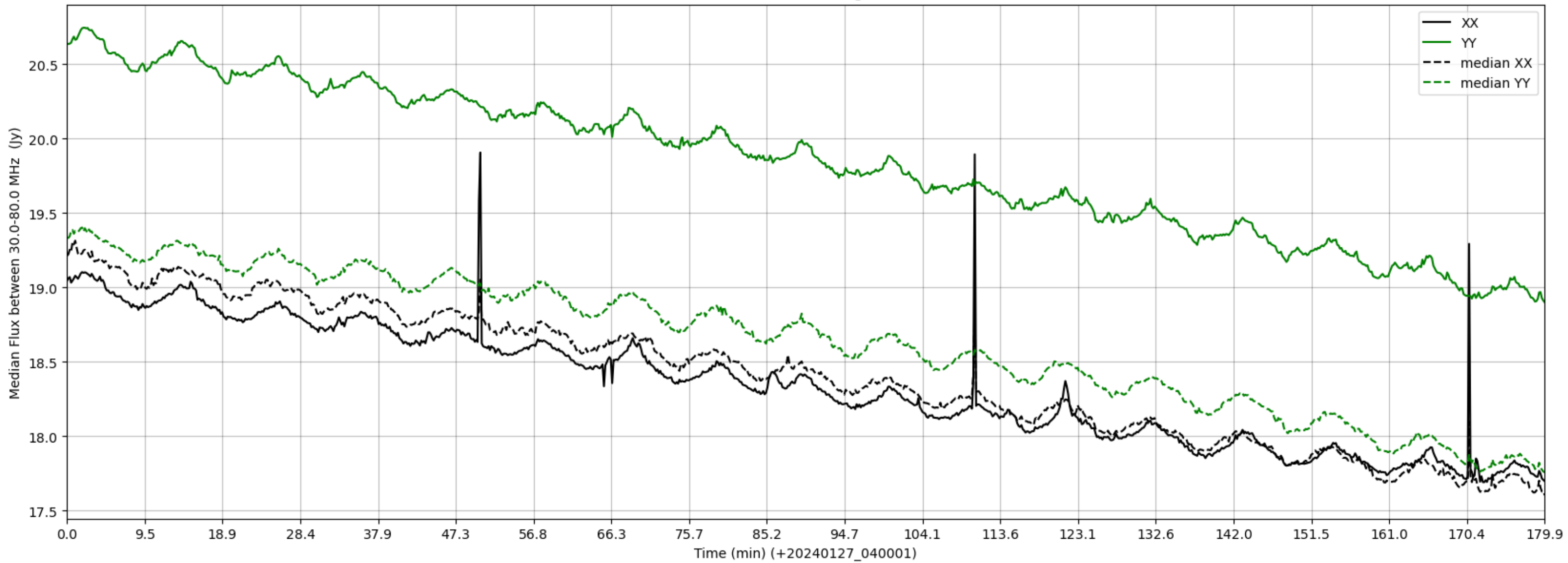
LWA107 - Correlator# 197 - XX FLAGS:HighTimeVar - YY FLAGS:Good
