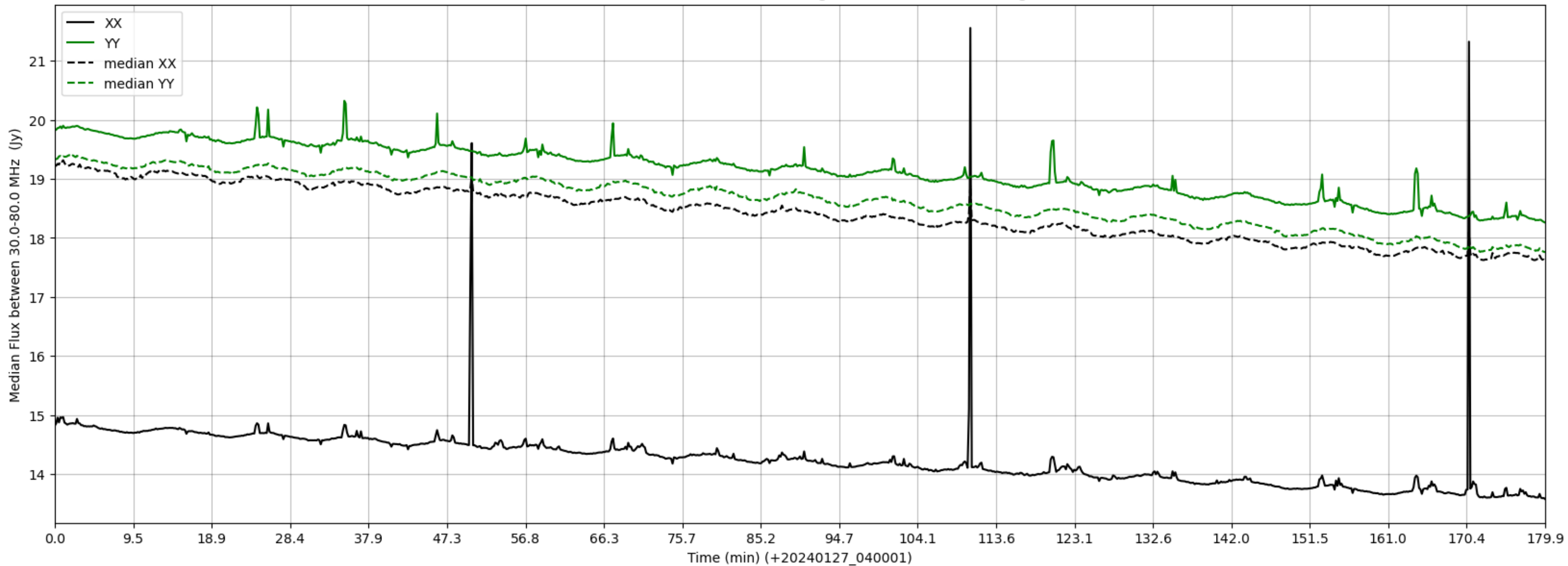
LWA038 - Correlator# 077 - XX FLAGS:HighTimeVar - YY FLAGS:HighTimeVar
