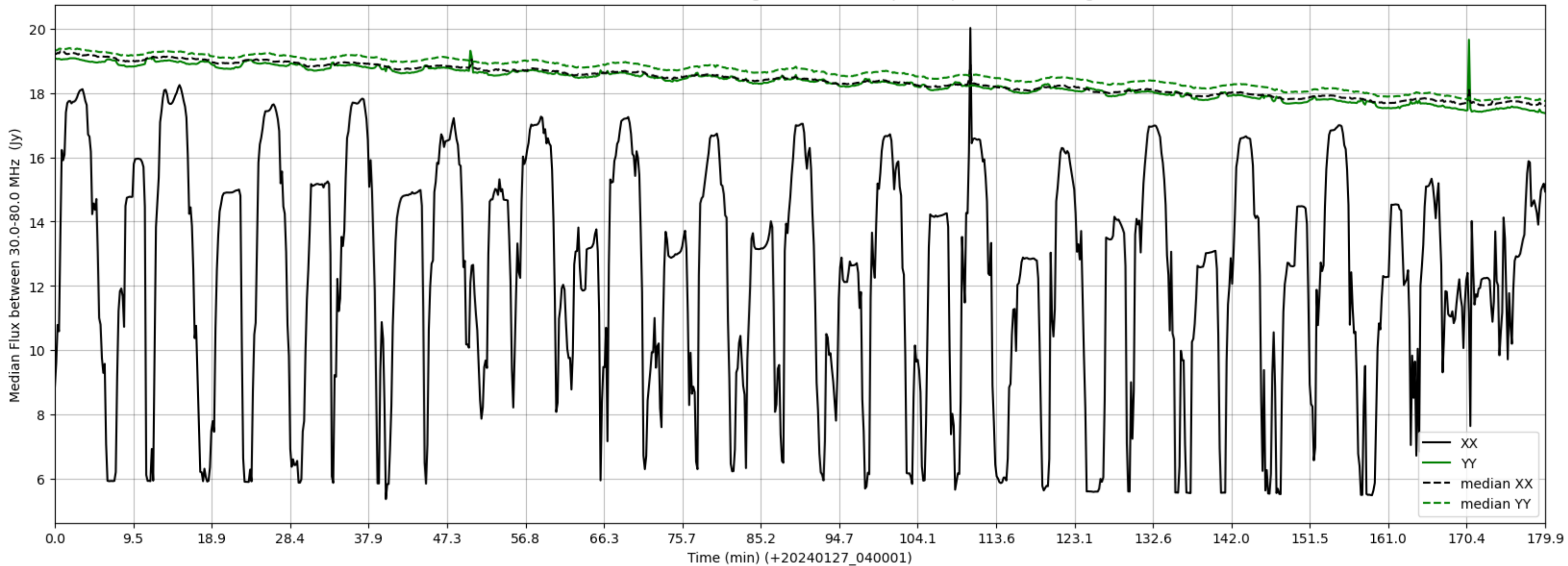
LWA209 - Correlator# 301 - XX FLAGS:HighTimeVar+BadSpecShape - YY FLAGS:HighTimeVar
