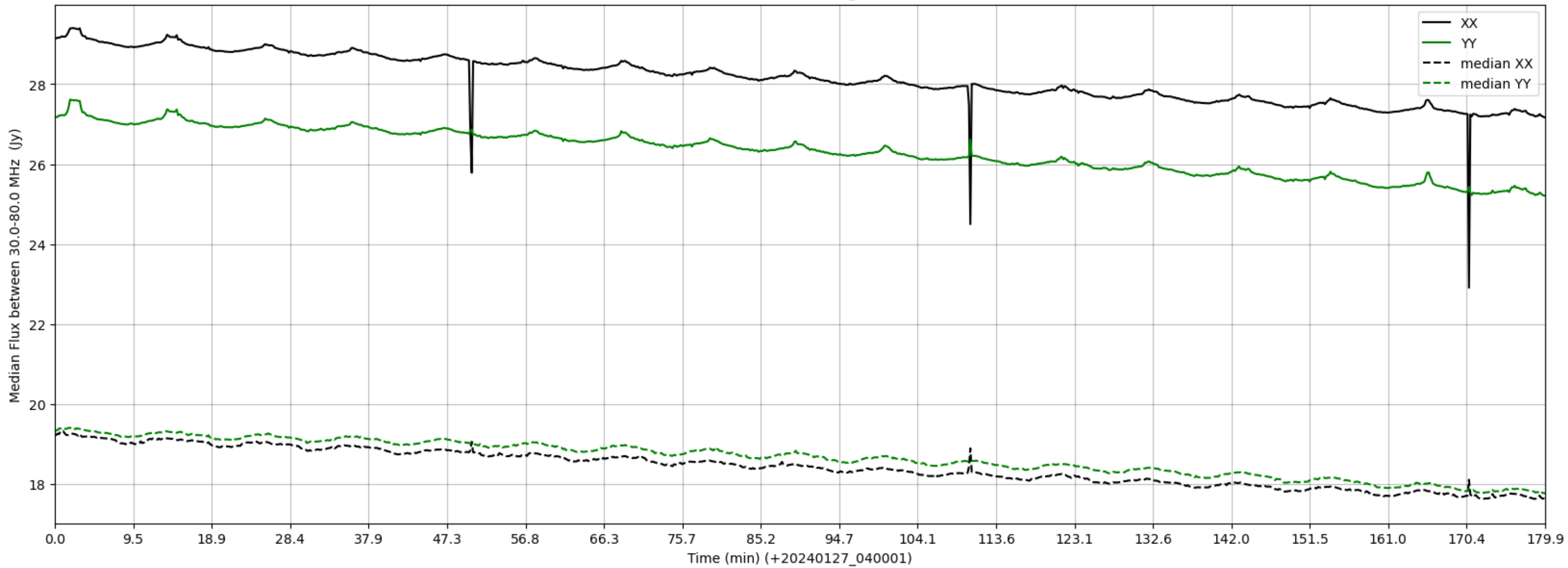
LWA178 - Correlator# 221 - XX FLAGS:HighTimeVar - YY FLAGS:Good
