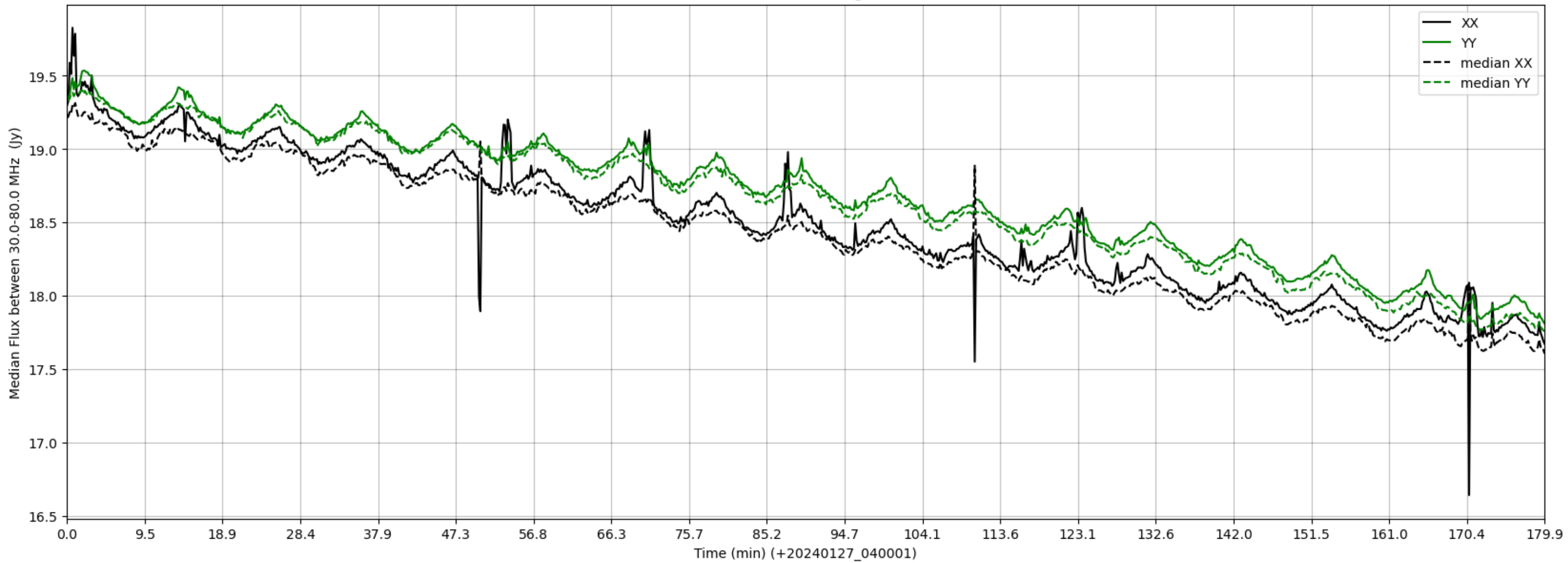
LWA145 - Correlator# 212 - XX FLAGS:HighTimeVar - YY FLAGS:Good
