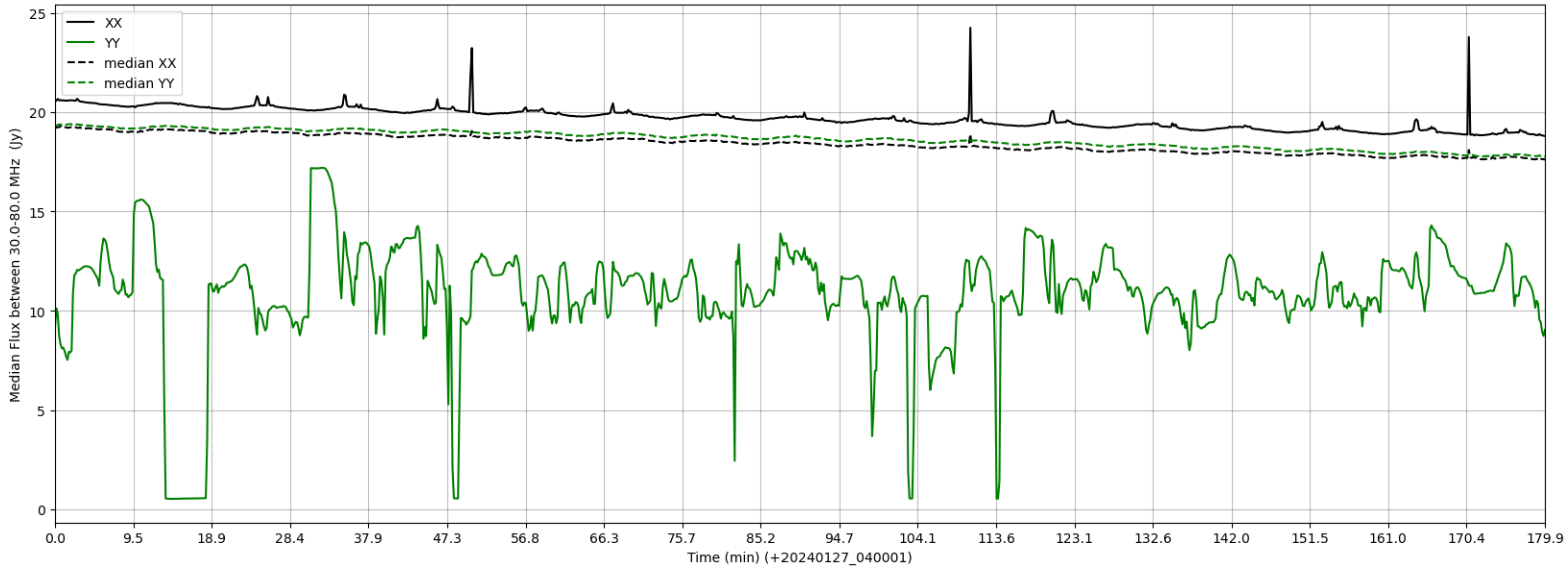
LWA009 - Correlator# 070 - XX FLAGS:HighTimeVar - YY FLAGS:HighTimeVar+BadSpecShape
