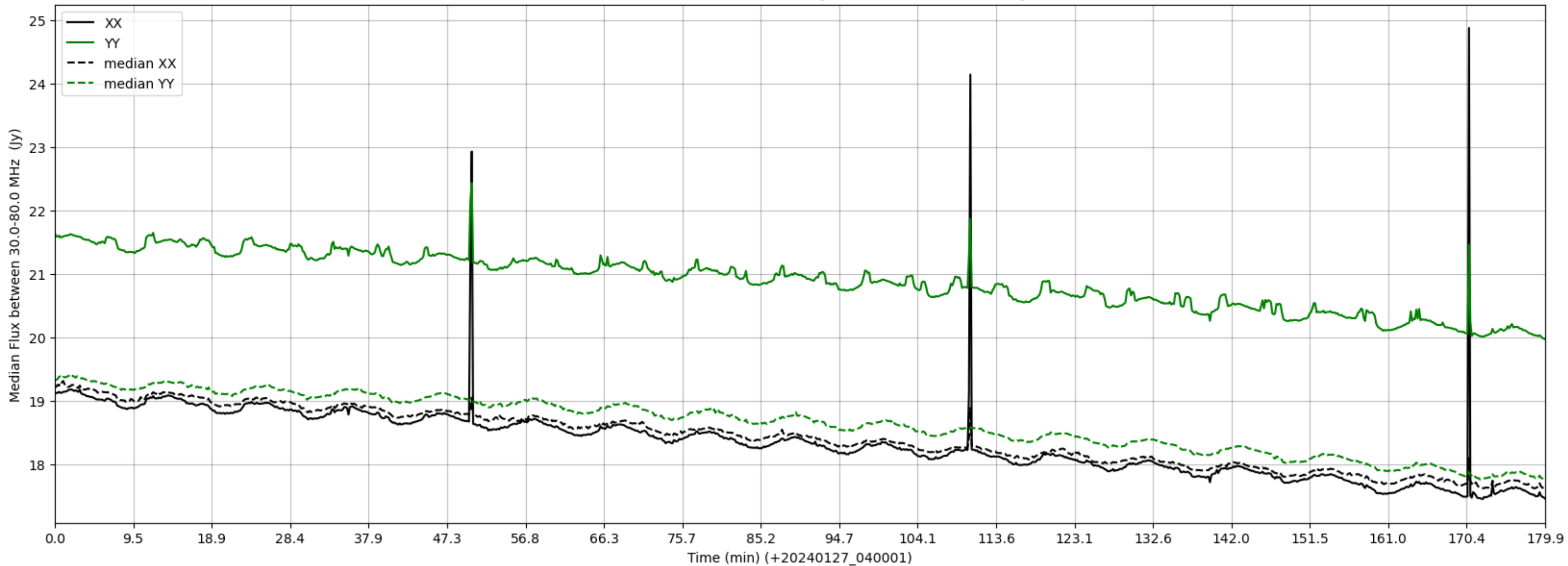
LWA194 - Correlator# 273 - XX FLAGS:HighTimeVar - YY FLAGS:HighTimeVar
