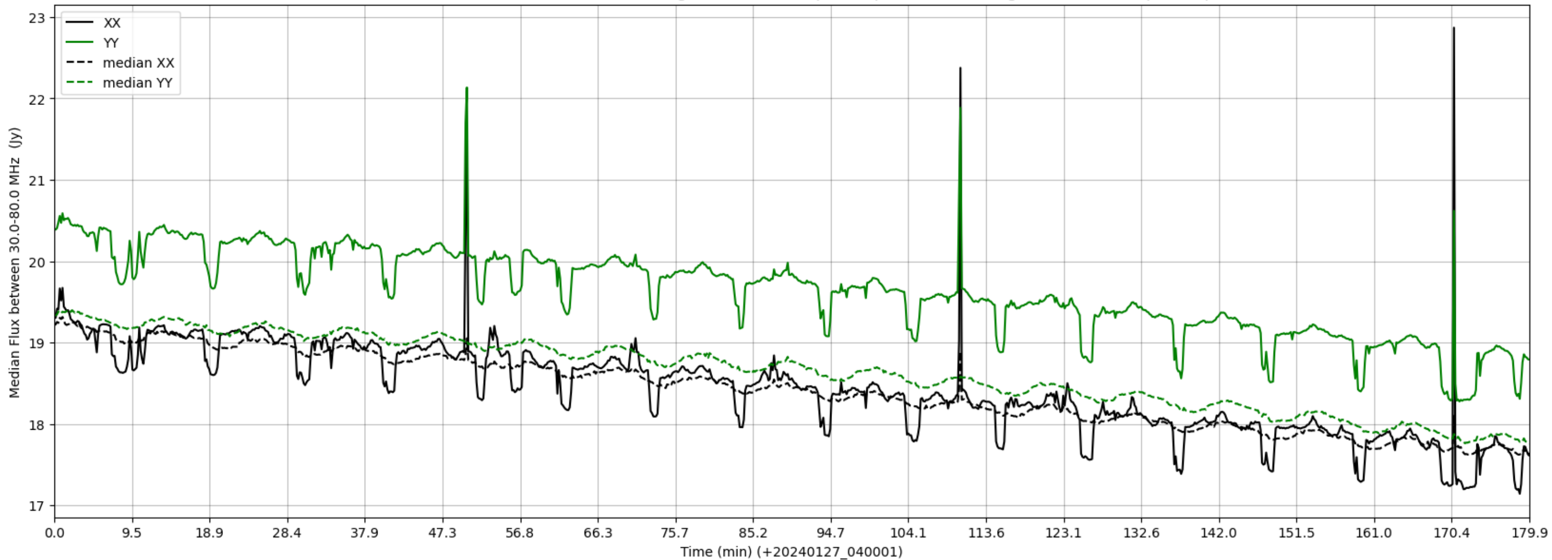
LWA103 - Correlator# 176 - XX FLAGS:HighTimeVar+BadSpecShape - YY FLAGS:HighTimeVar+BadSpecShape
