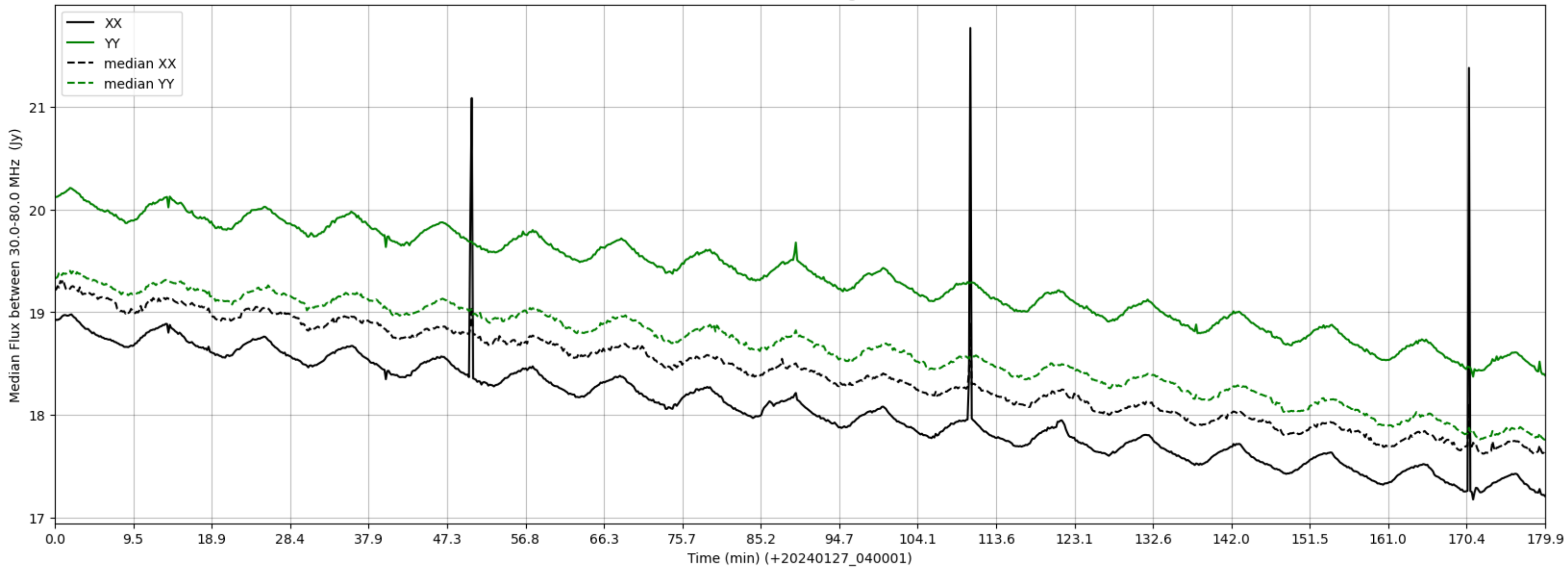
LWA141 - Correlator# 263 - XX FLAGS:HighTimeVar - YY FLAGS:Good
