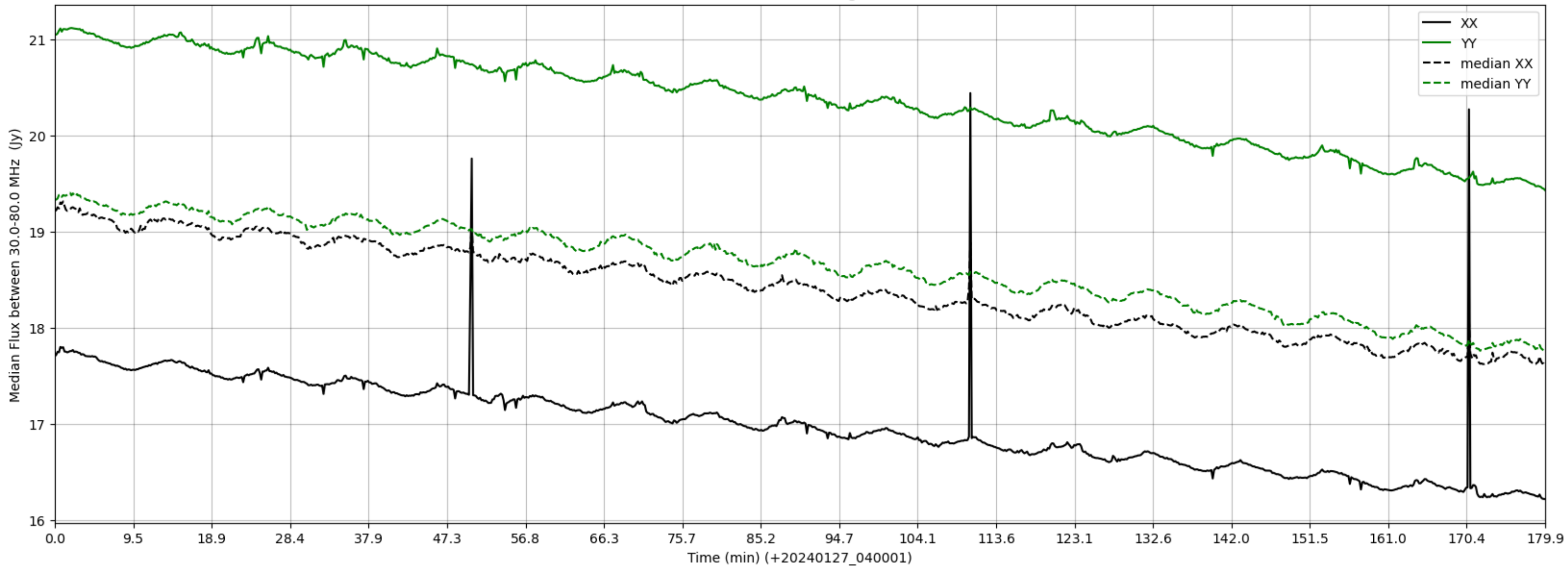
LWA045 - Correlator# 083 - XX FLAGS:HighTimeVar - YY FLAGS:Good
