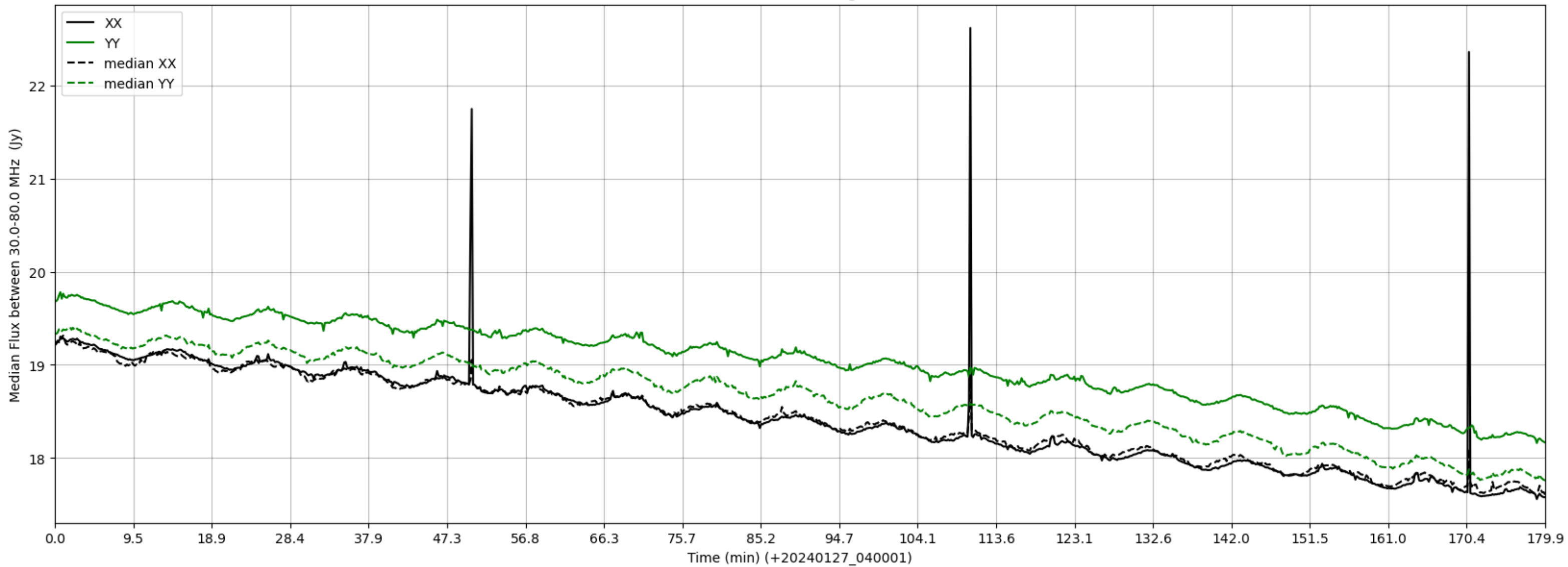
LWA016 - Correlator# 097 - XX FLAGS:HighTimeVar - YY FLAGS:Good
