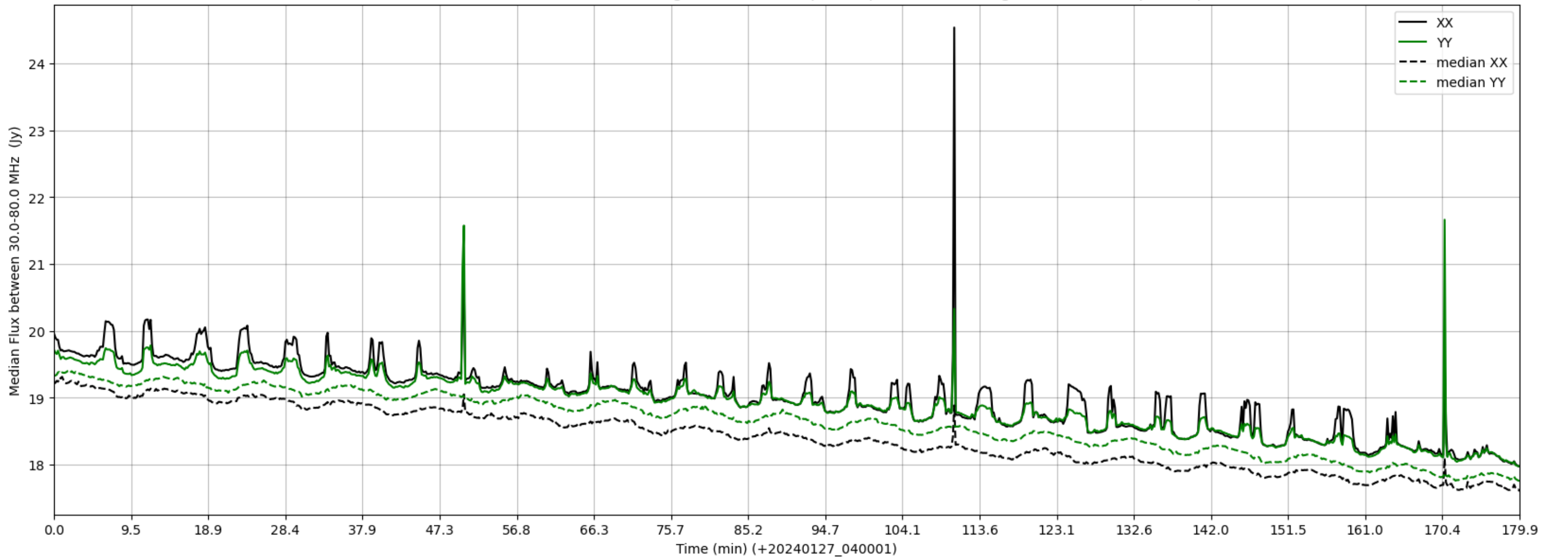
LWA230 - Correlator# 303 - XX FLAGS:HighTimeVar+BadSpecShape - YY FLAGS:HighTimeVar+BadSpecShape
