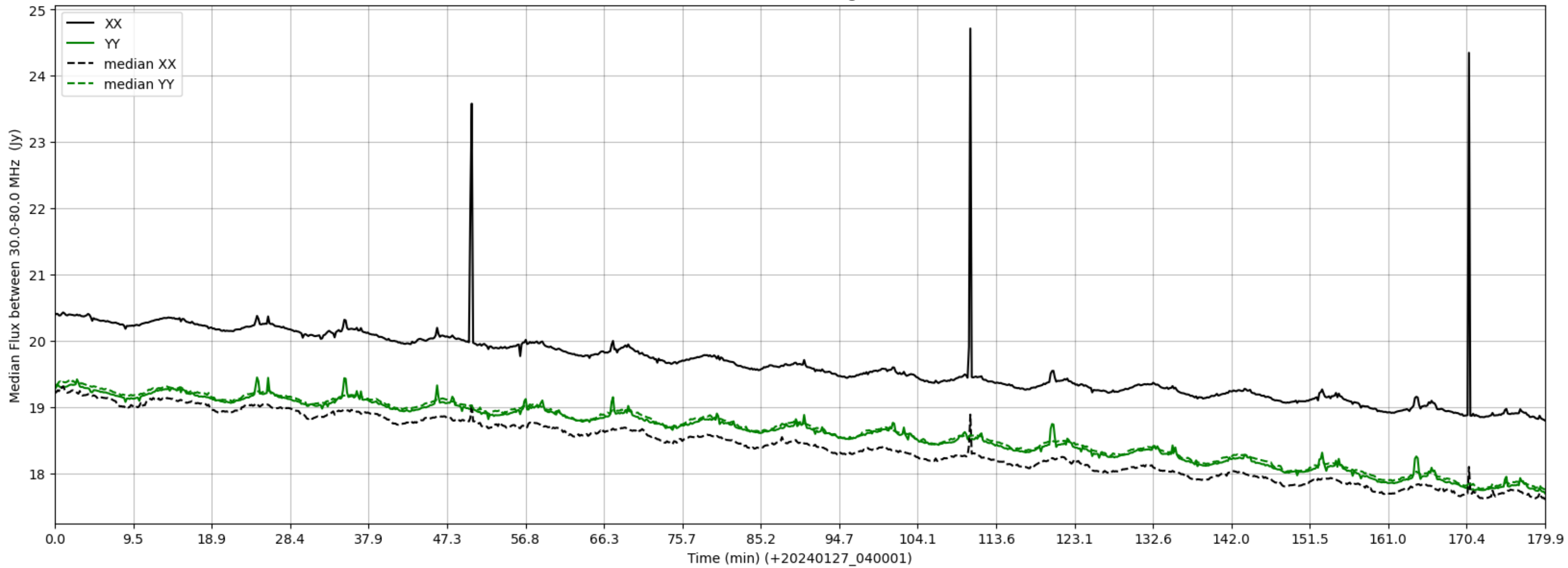
LWA007 - Correlator# 071 - XX FLAGS:HighTimeVar - YY FLAGS:Good
