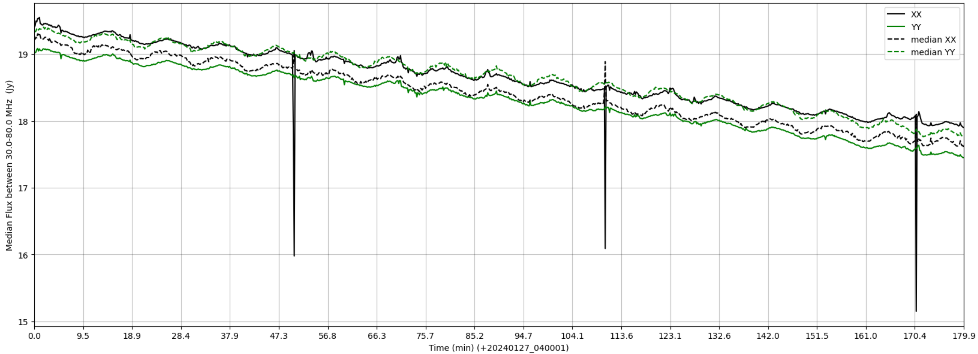
LWA192 - Correlator# 247 - XX FLAGS:HighTimeVar - YY FLAGS:Good
