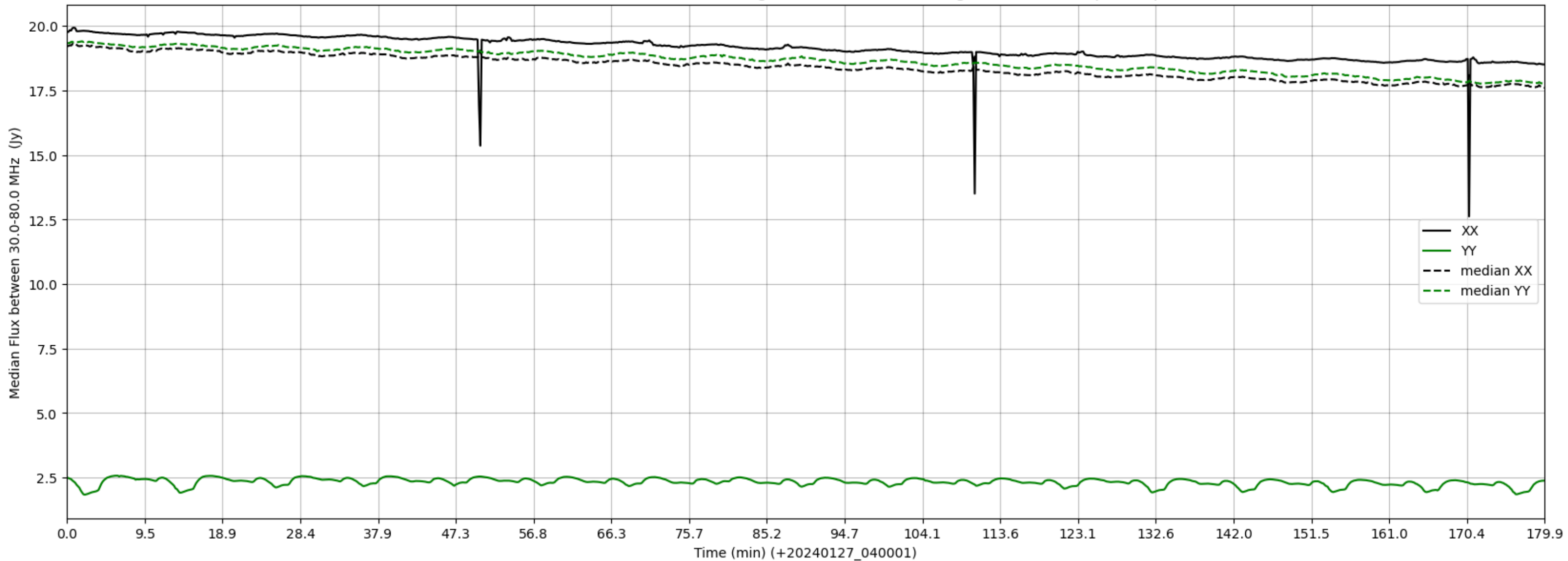
LWA307 - Correlator# 012 - XX FLAGS:HighTimeVar - YY FLAGS:HighTimeVar+BadSpecShape
