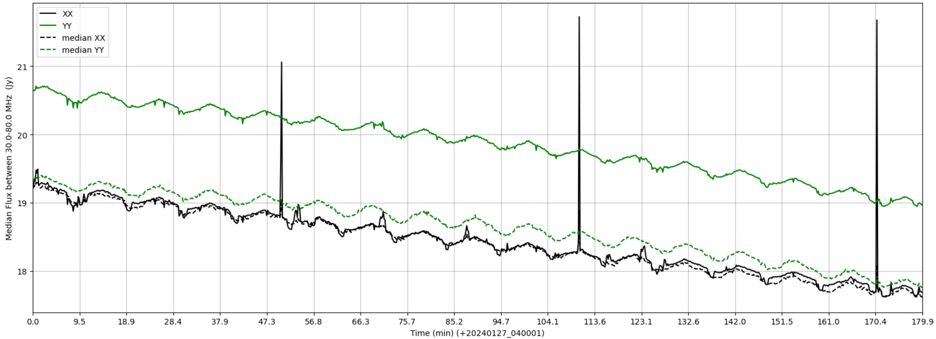
LWA101 - Correlator# 174 - XX FLAGS:HighTimeVar - YY FLAGS:Good
