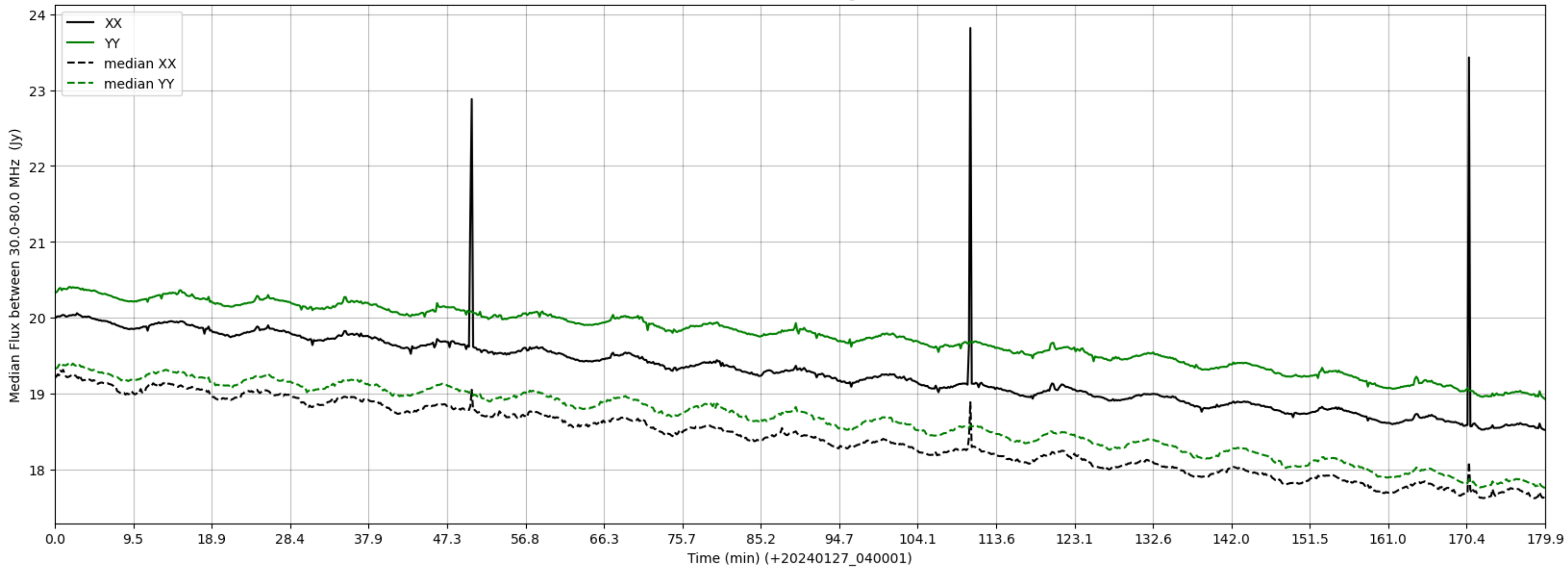
LWA015 - Correlator# 098 - XX FLAGS:HighTimeVar - YY FLAGS:Good
