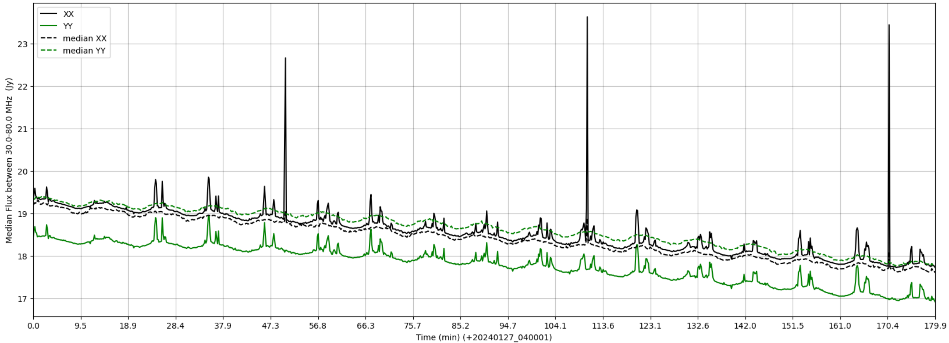
LWA008 - Correlator# 075 - XX FLAGS:HighTimeVar - YY FLAGS:HighTimeVar
