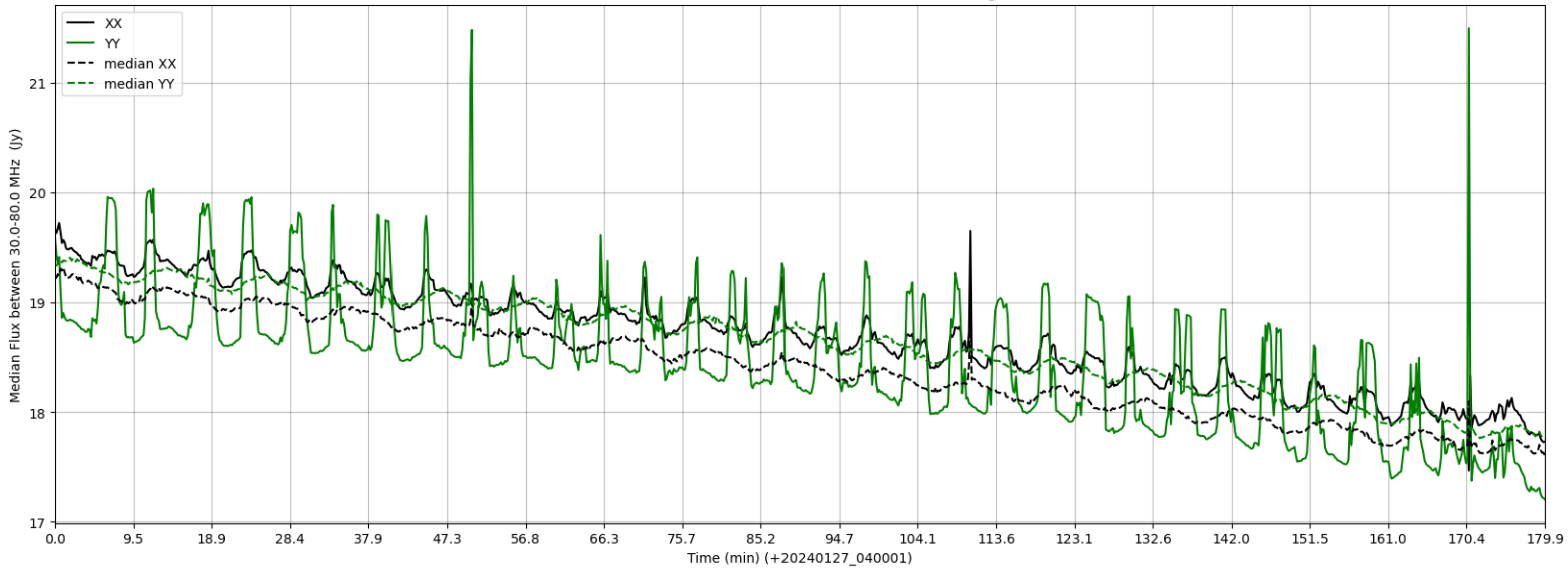
LWA208 - Correlator# 298 - XX FLAGS:Good - YY FLAGS:HighTimeVar
