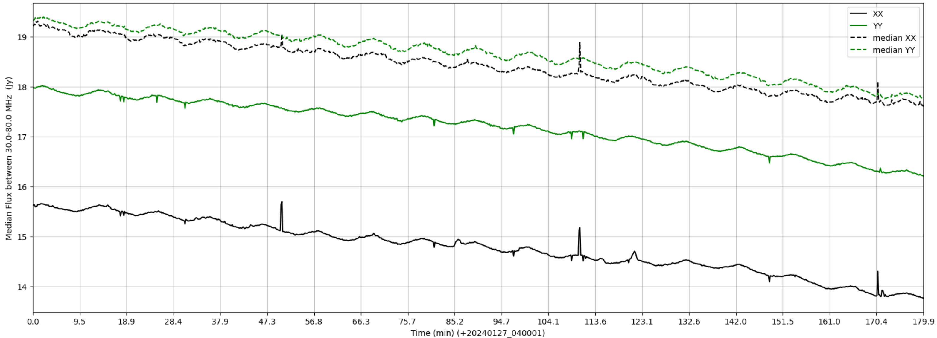
LWA305 - Correlator# 050 - XX FLAGS:HighTimeVar - YY FLAGS:Good
