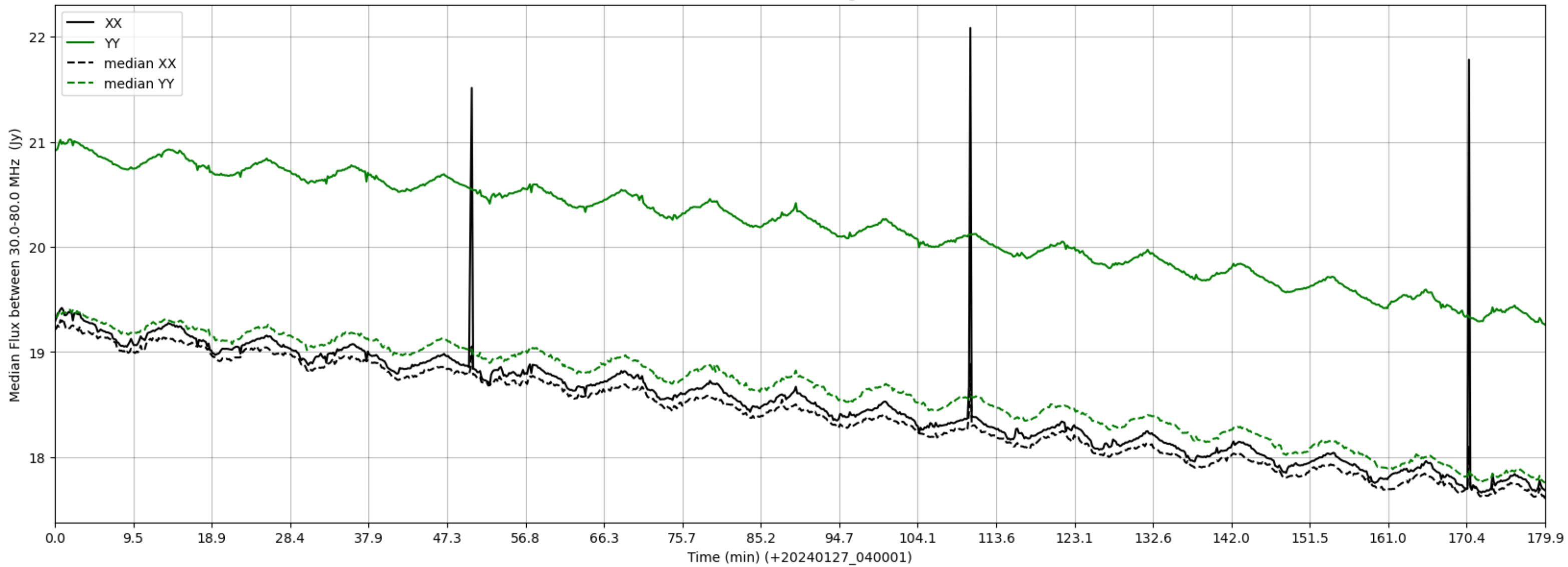
LWA139 - Correlator# 187 - XX FLAGS:HighTimeVar - YY FLAGS:Good
