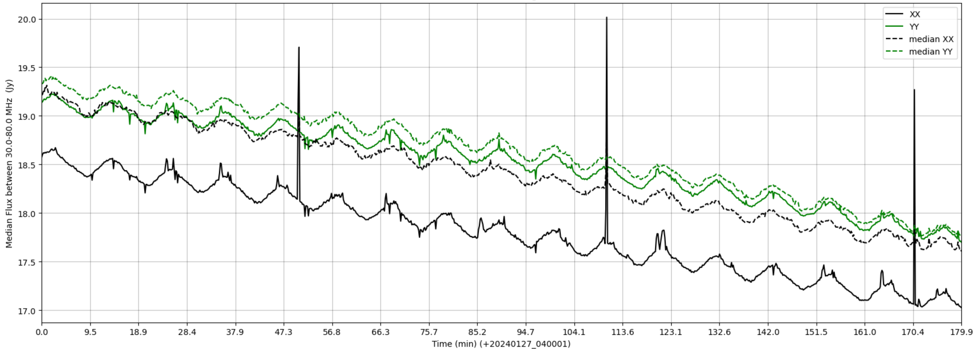
LWA074 - Correlator# 086 - XX FLAGS:HighTimeVar - YY FLAGS:Good
