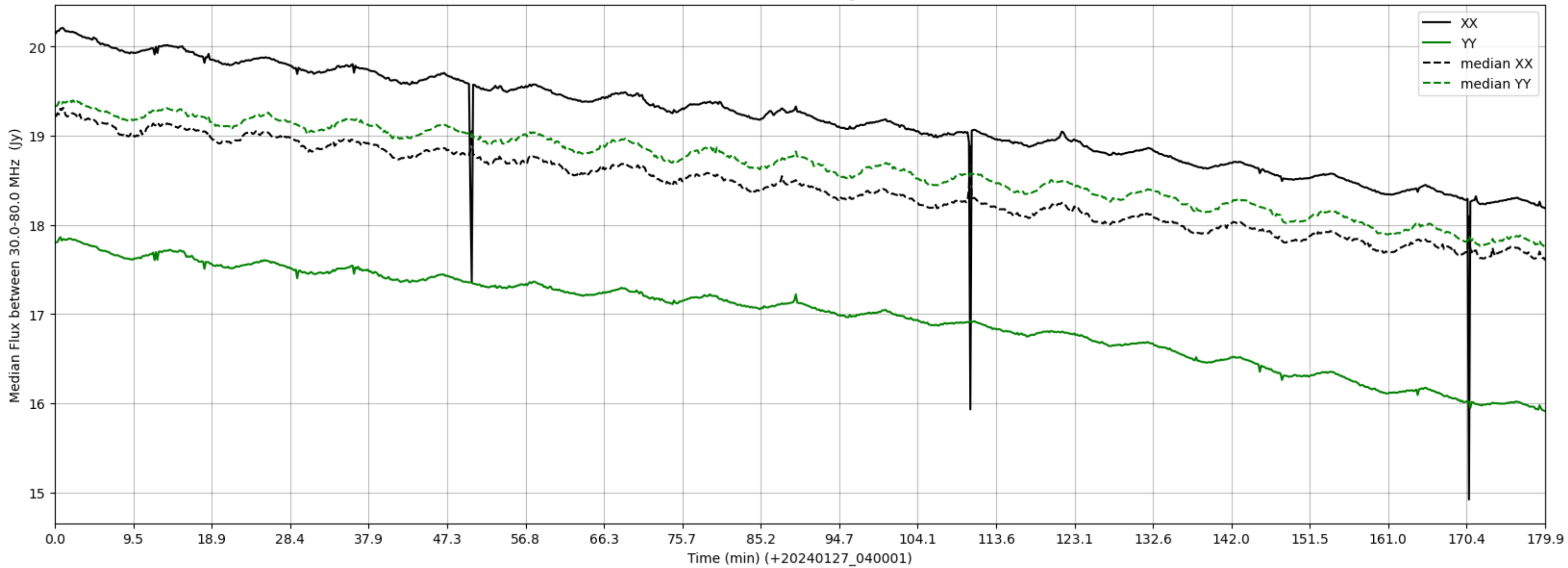
LWA268 - Correlator# 002 - XX FLAGS:HighTimeVar - YY FLAGS:Good
