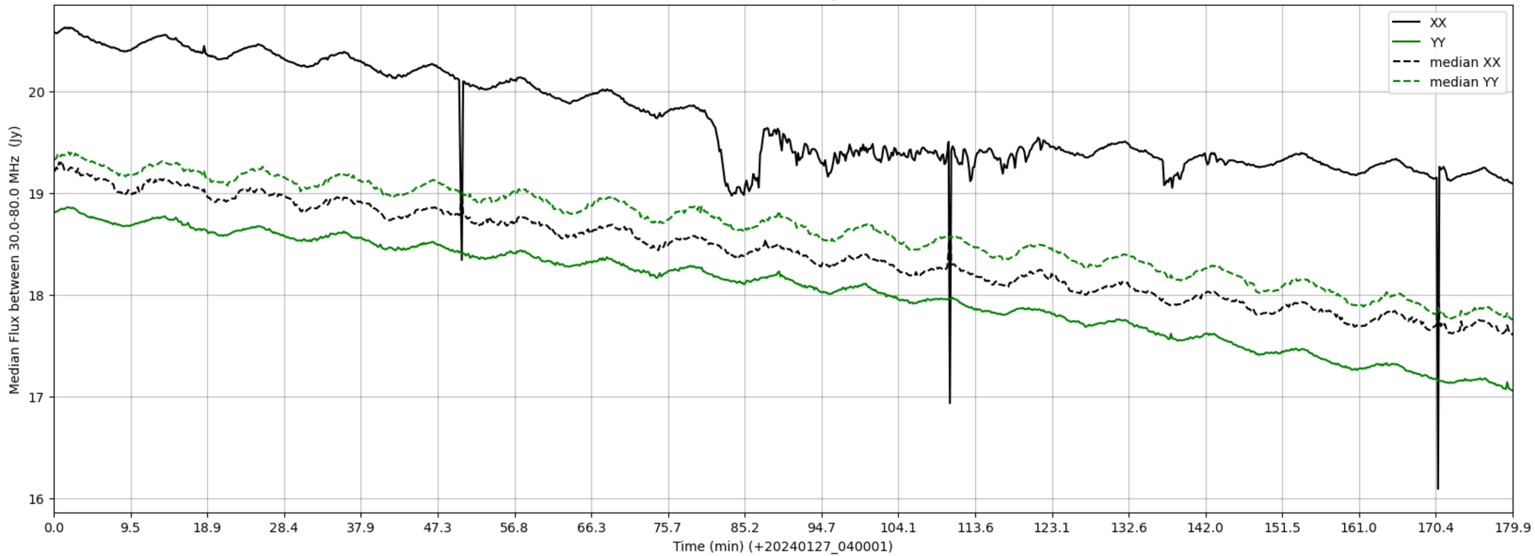
LWA261 - Correlator# 346 - XX FLAGS:HighTimeVar - YY FLAGS:Good
