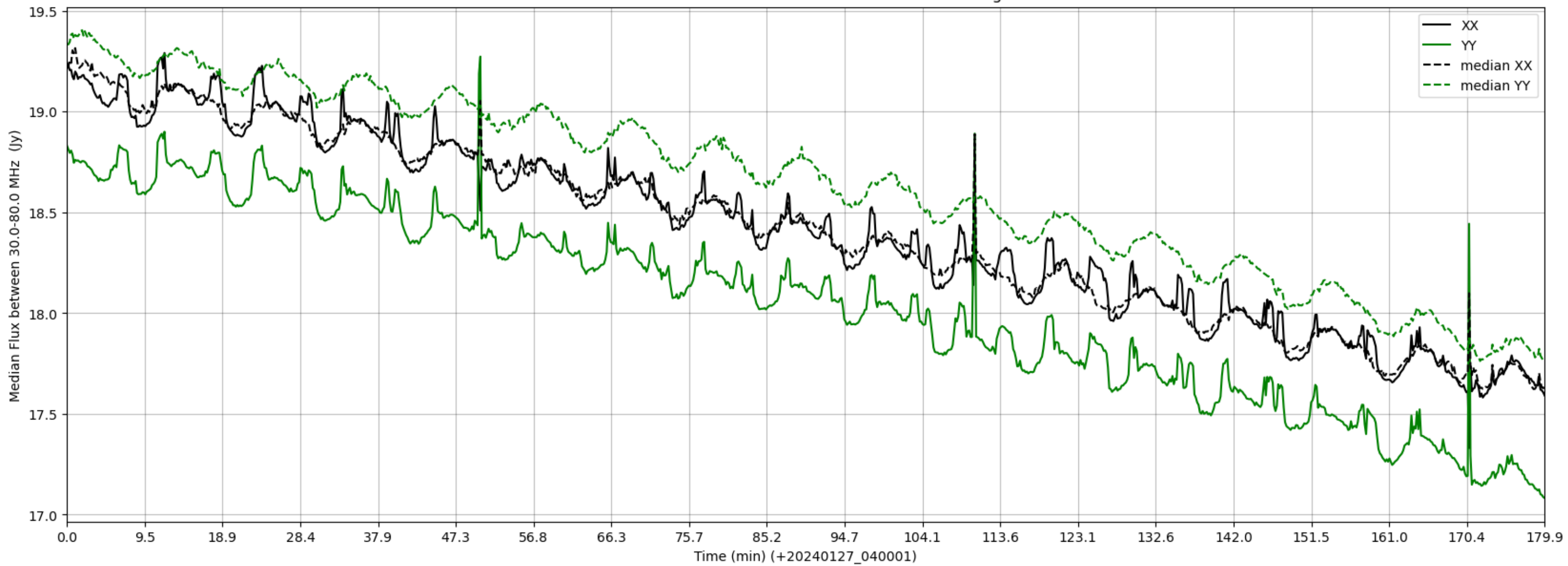
LWA210 - Correlator# 300 - XX FLAGS:Good - YY FLAGS:HighTimeVar
