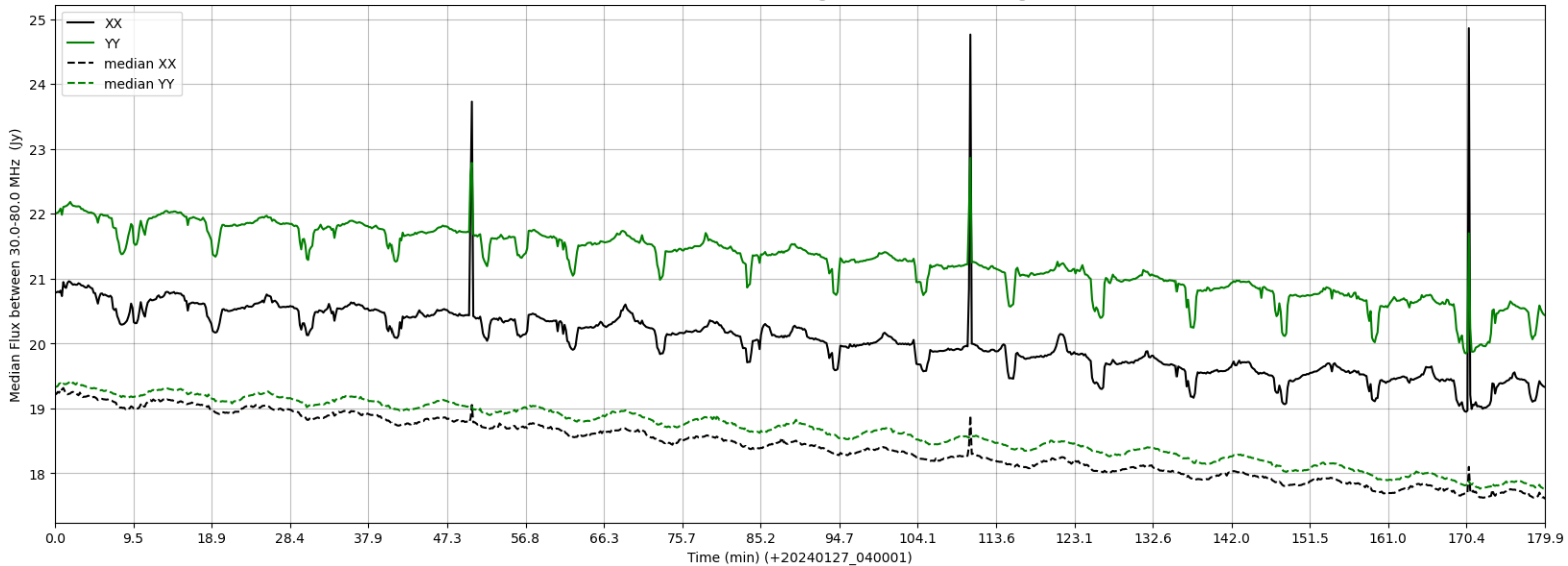
LWA129 - Correlator# 180 - XX FLAGS:HighTimeVar - YY FLAGS:HighTimeVar
