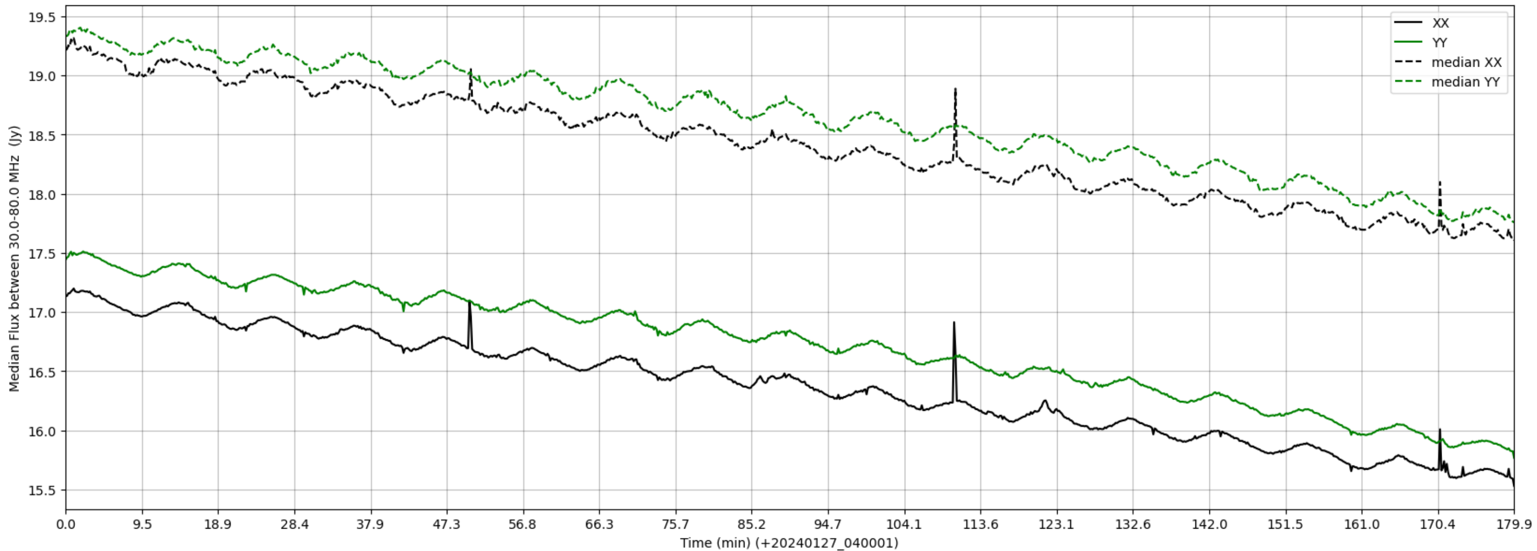
LWA320 - Correlator# 054 - XX FLAGS:Good - YY FLAGS:Good
