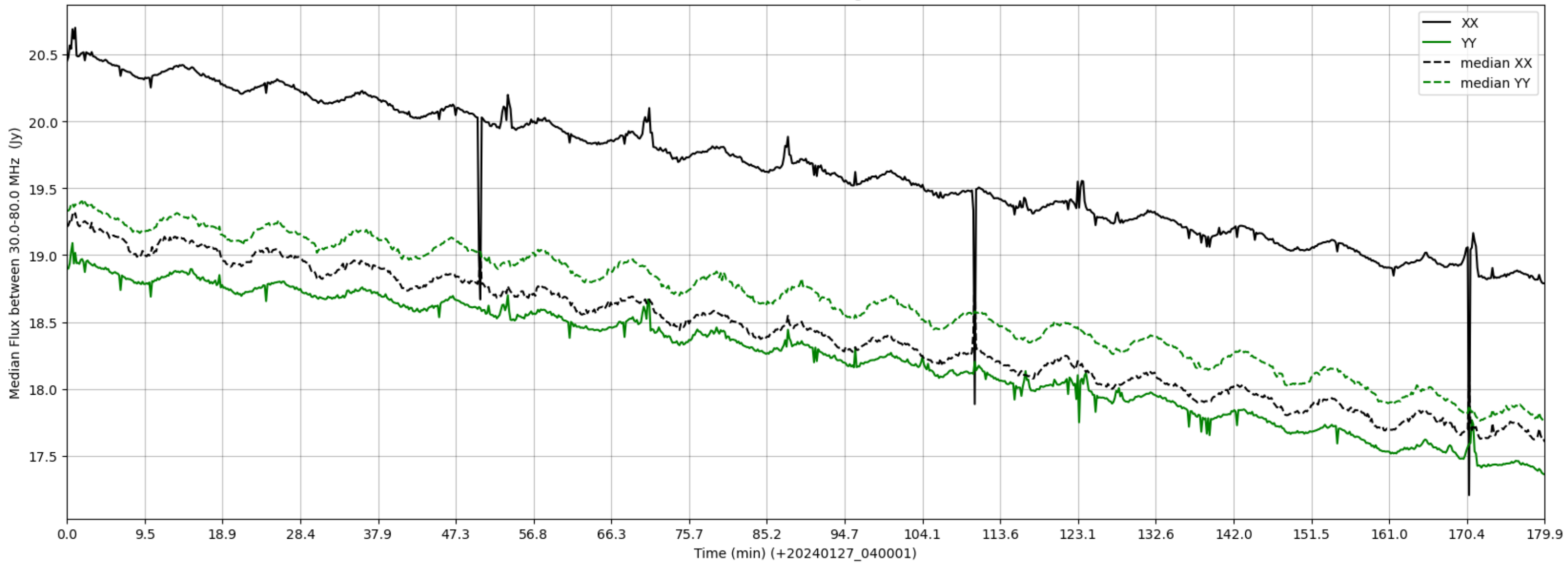
LWA059 - Correlator# 136 - XX FLAGS:HighTimeVar - YY FLAGS:Good
