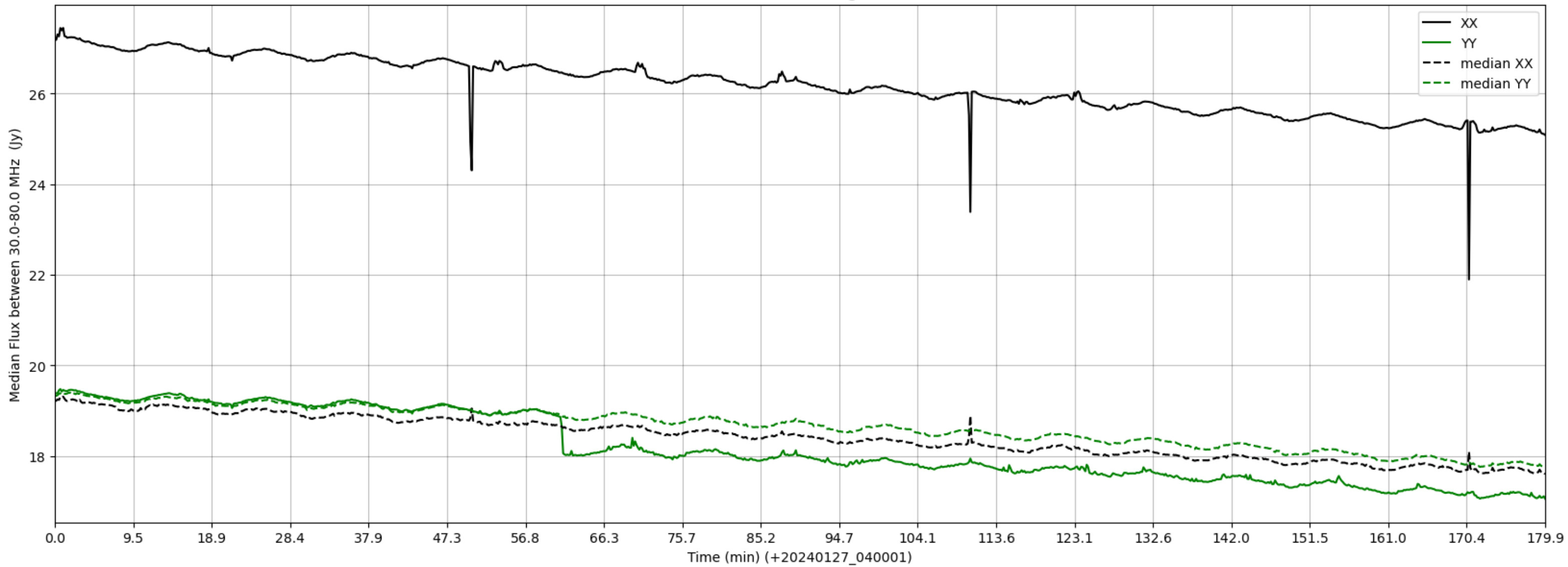
LWA214 - Correlator# 328 - XX FLAGS:HighTimeVar - YY FLAGS:Good
