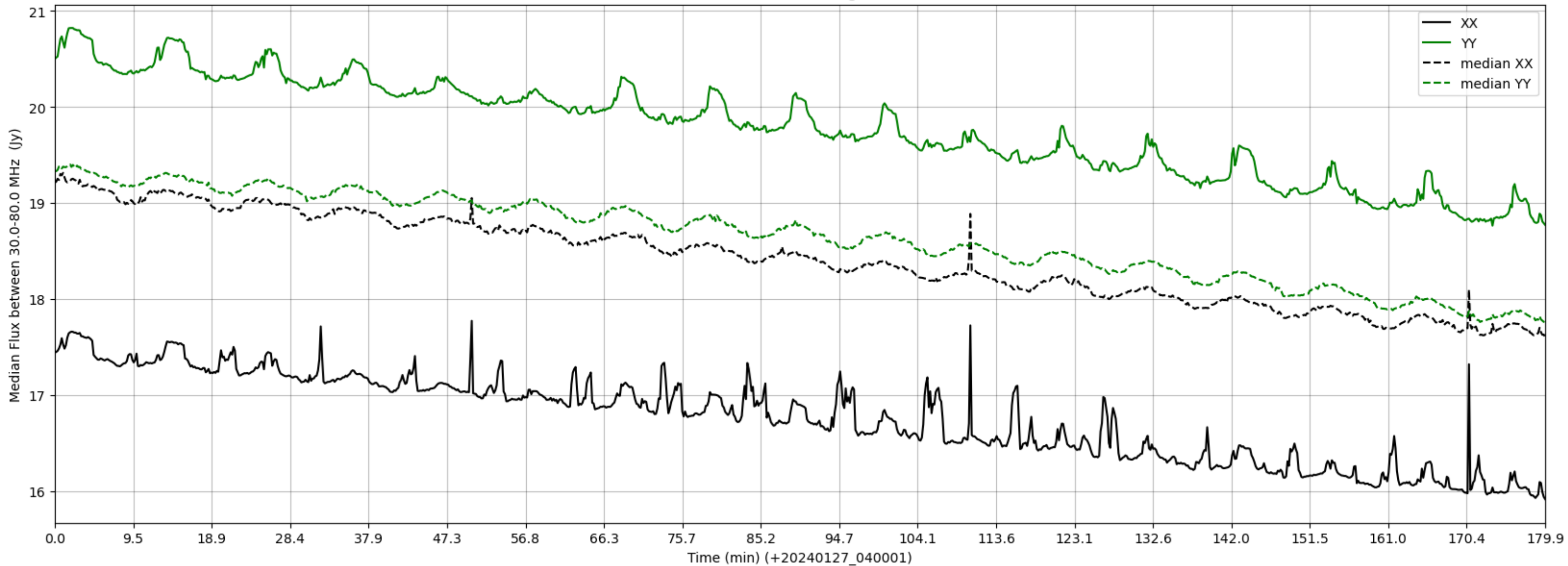
LWA143 - Correlator# 210 - XX FLAGS:HighTimeVar - YY FLAGS:Good
