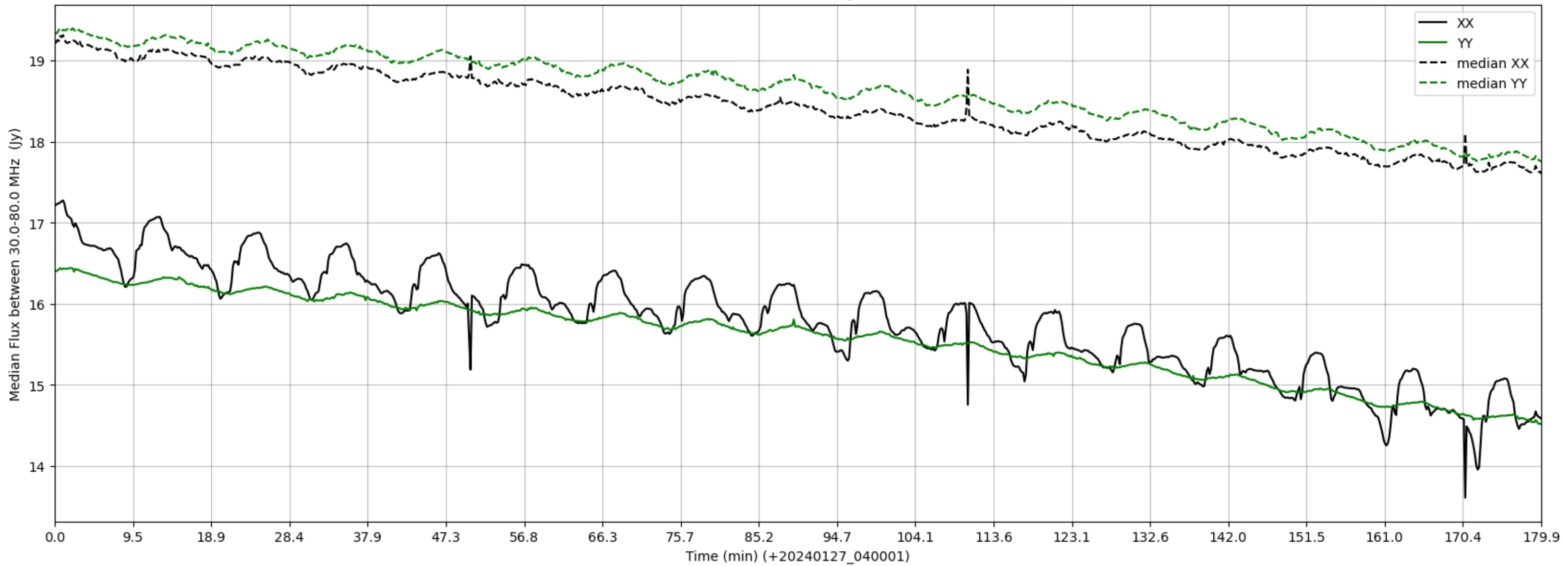
LWA299 - Correlator# 191 - XX FLAGS:HighTimeVar - YY FLAGS:Good
