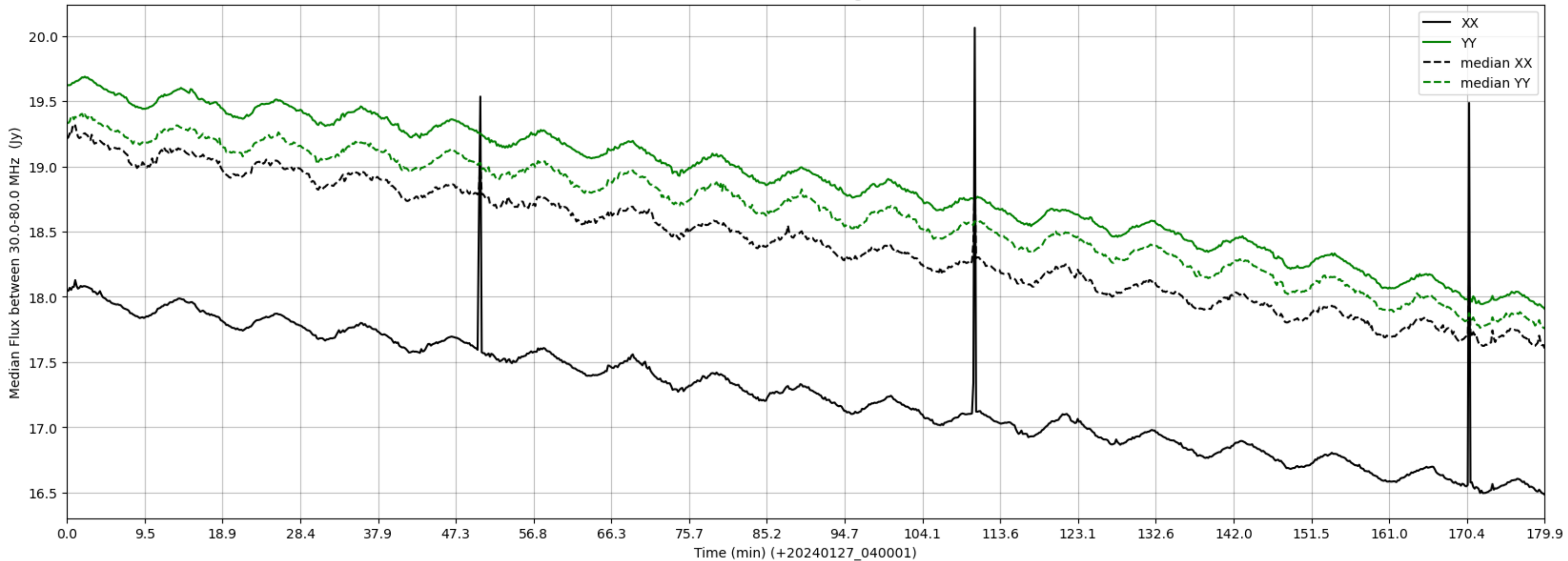
LWA245 - Correlator# 341 - XX FLAGS:HighTimeVar - YY FLAGS:Good
