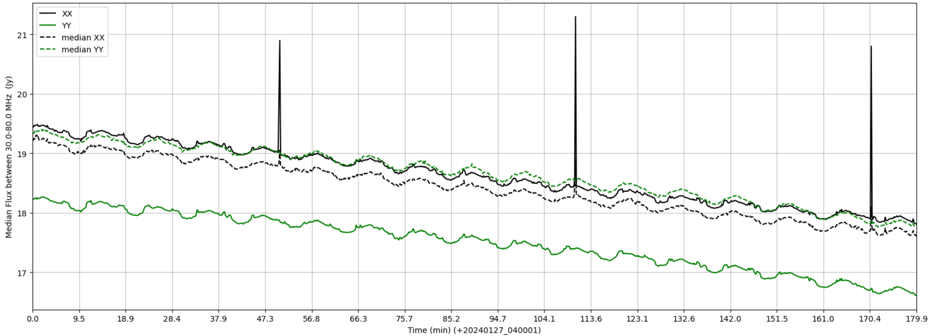
LWA171 - Correlator# 291 - XX FLAGS:HighTimeVar - YY FLAGS:Good
