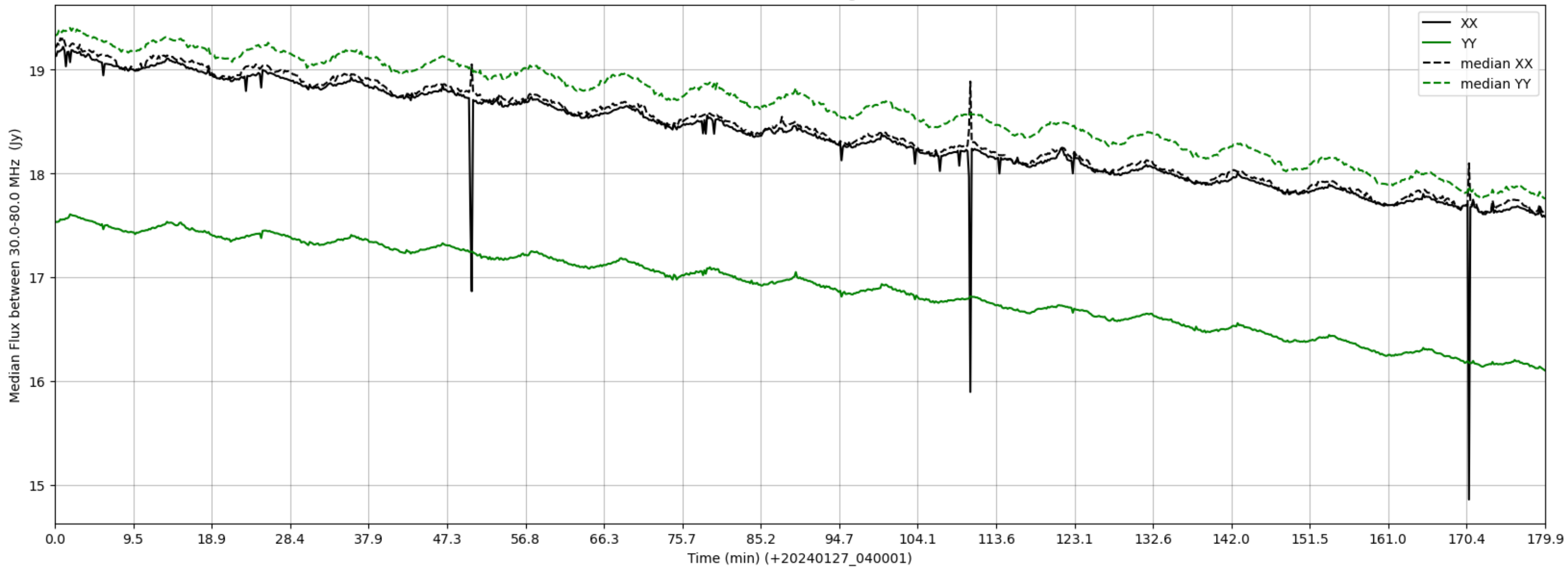
LWA160 - Correlator# 239 - XX FLAGS:HighTimeVar - YY FLAGS:Good
