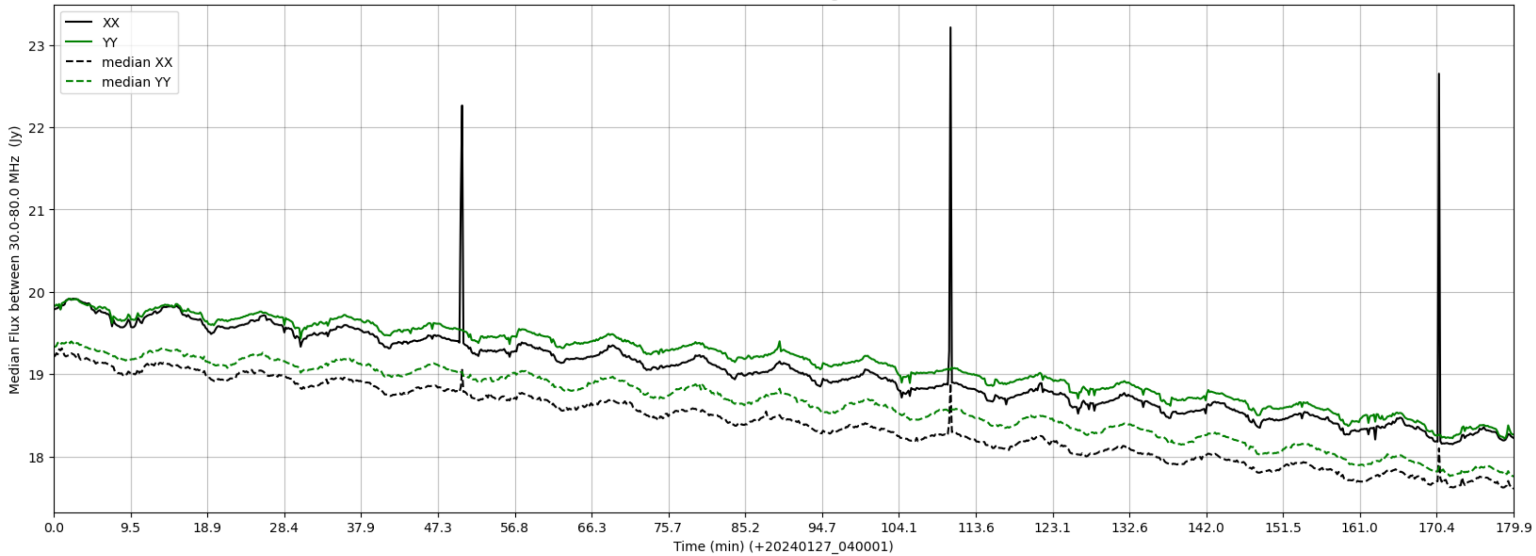
LWA068 - Correlator# 166 - XX FLAGS:HighTimeVar - YY FLAGS:Good
