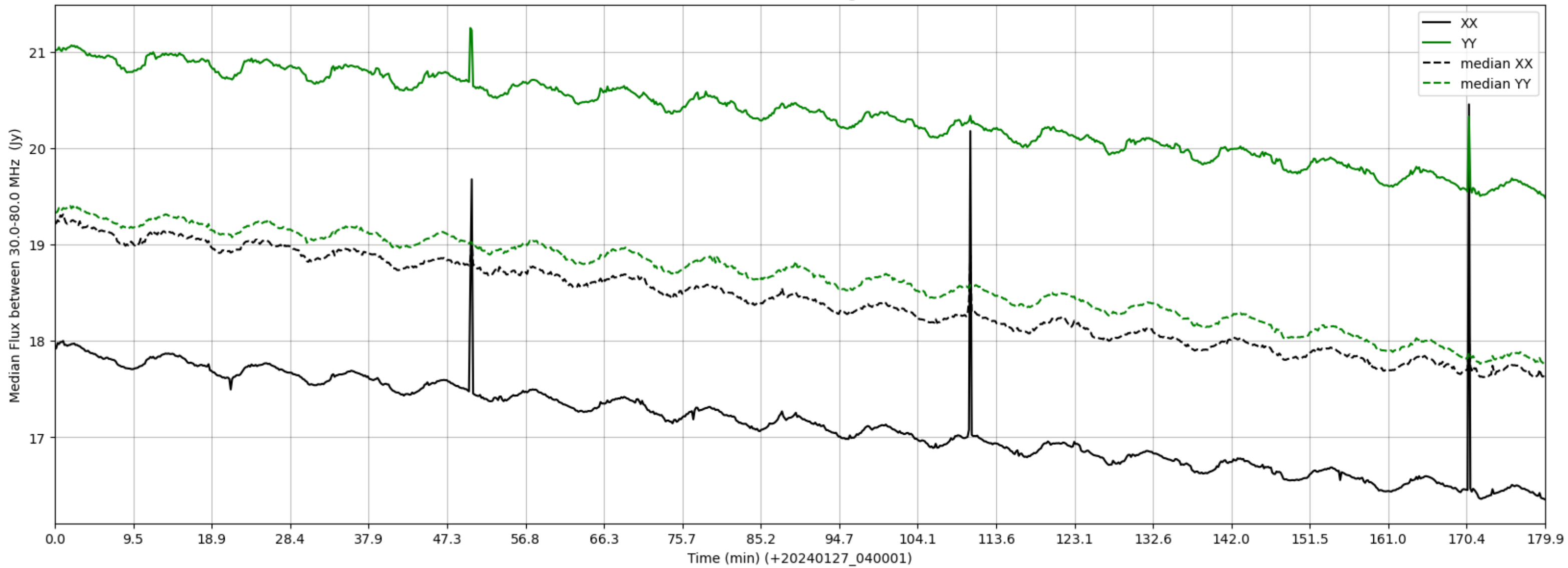
LWA169 - Correlator# 292 - XX FLAGS:HighTimeVar - YY FLAGS:Good
