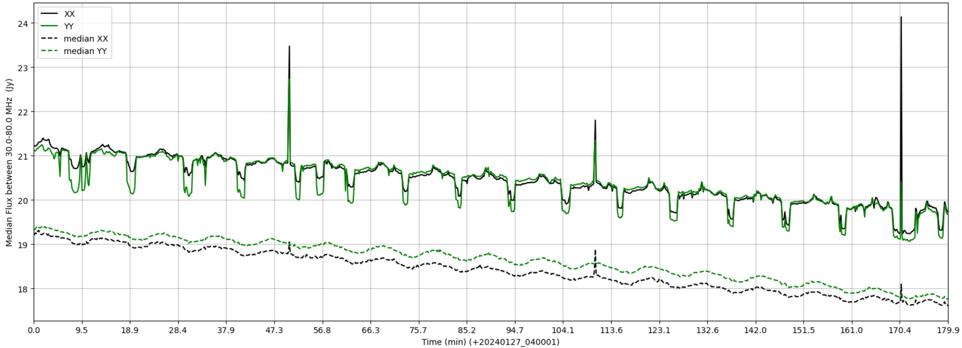
LWA097 - Correlator# 170 - XX FLAGS:HighTimeVar - YY FLAGS:HighTimeVar+BadSpecShape
