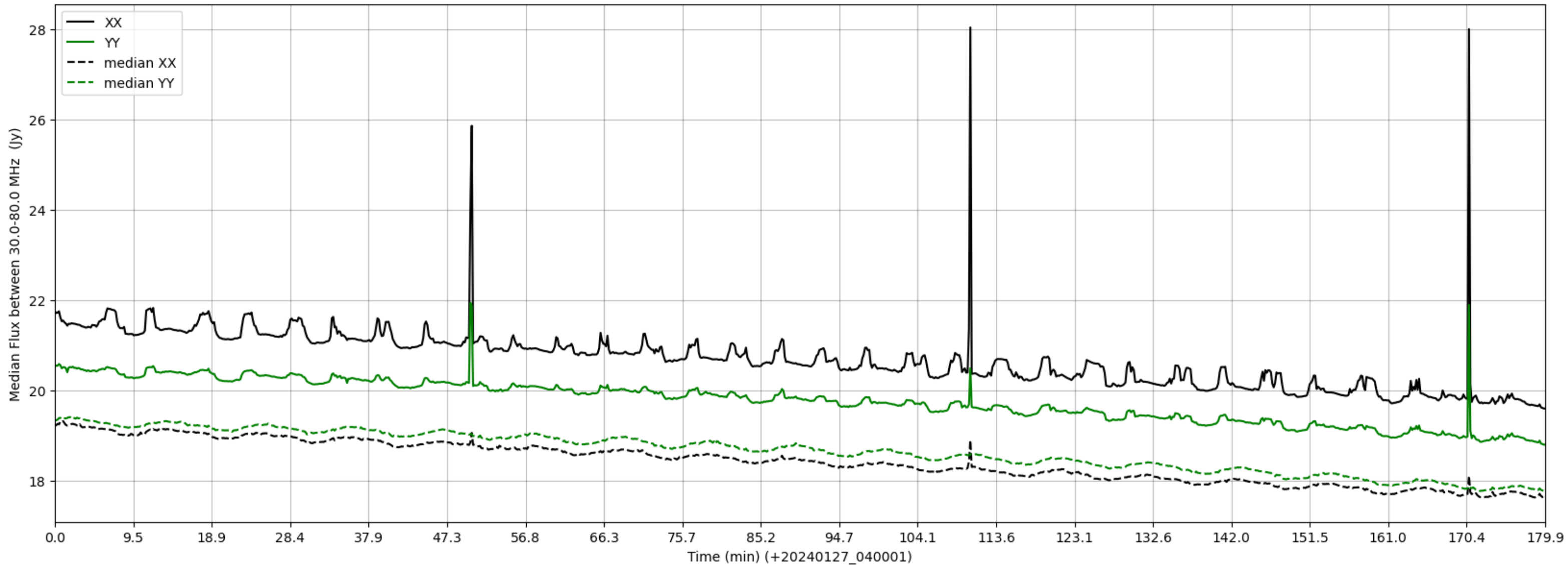
LWA229 - Correlator# 305 - XX FLAGS:HighTimeVar - YY FLAGS:HighTimeVar+BadSpecShape
