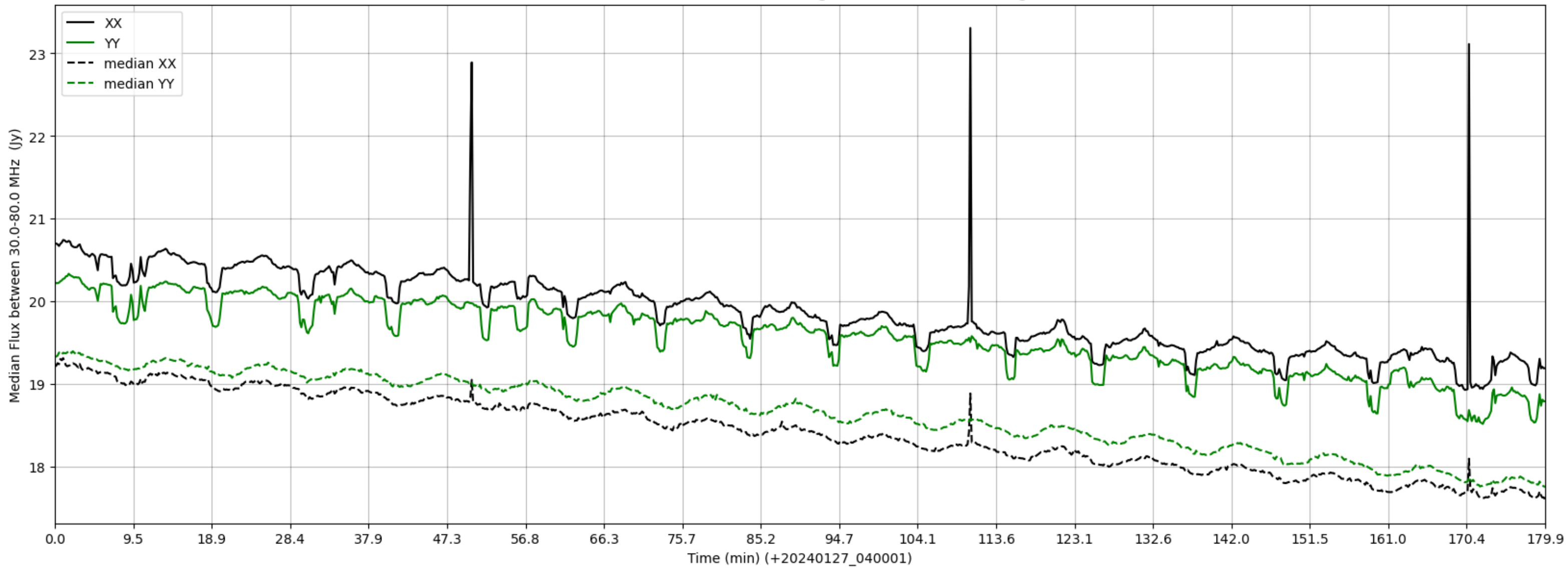
LWA070 - Correlator# 168 - XX FLAGS:HighTimeVar - YY FLAGS:HighTimeVar
