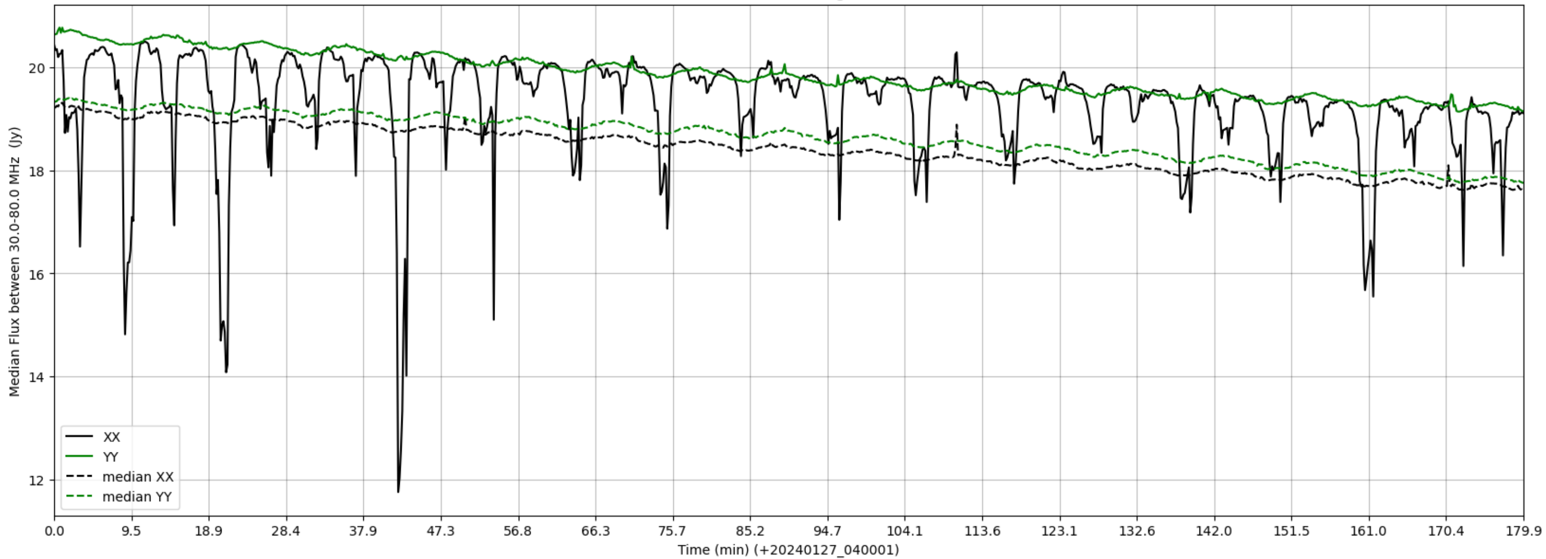
LWA256 - Correlator# 347 - XX FLAGS:HighTimeVar - YY FLAGS:Good
