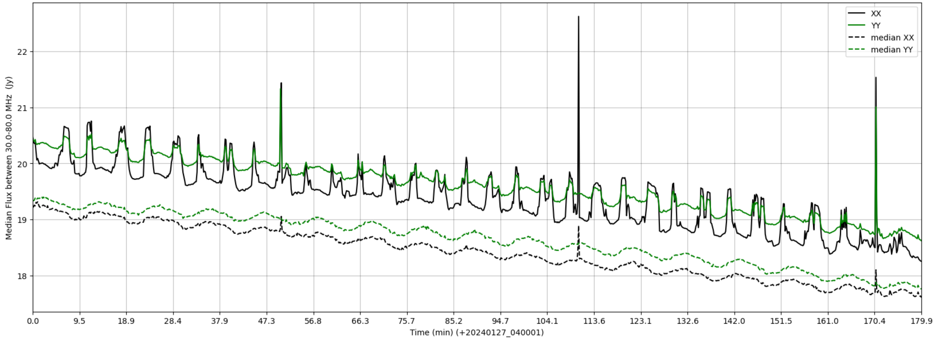
LWA228 - Correlator# 302 - XX FLAGS:HighTimeVar - YY FLAGS:HighTimeVar+BadSpecShape
