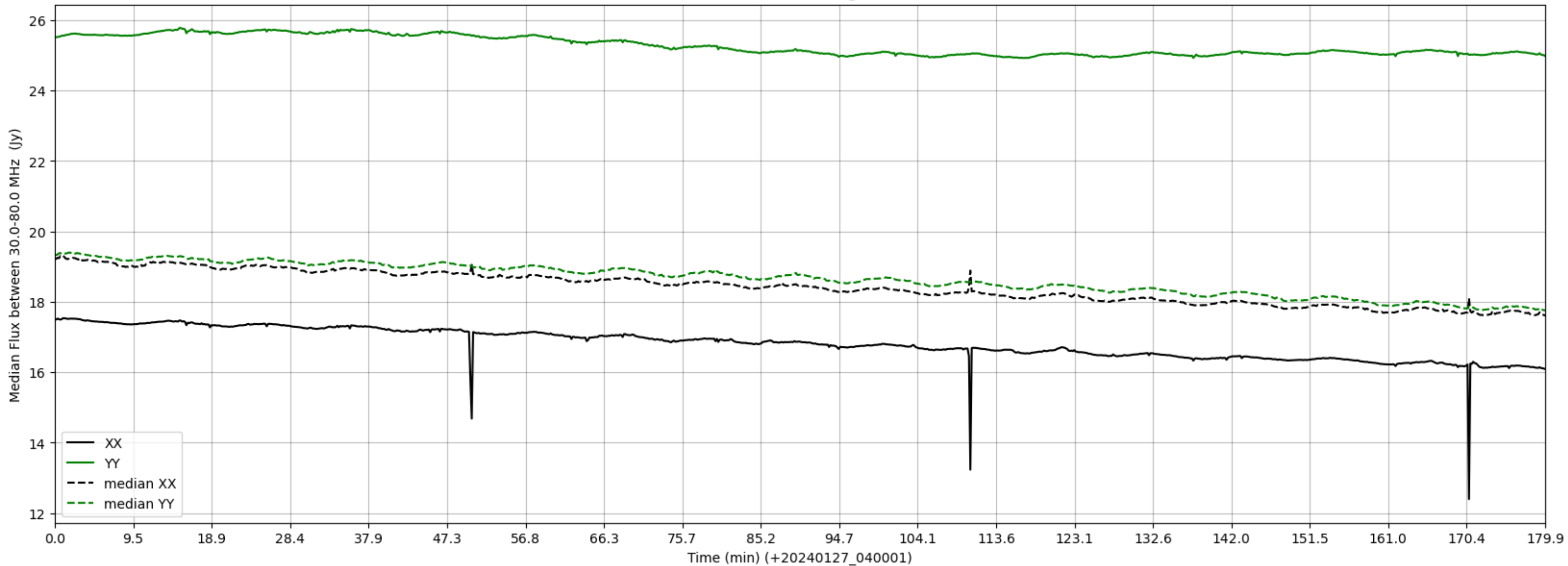
LWA331 - Correlator# 125 - XX FLAGS:HighTimeVar - YY FLAGS:Good
