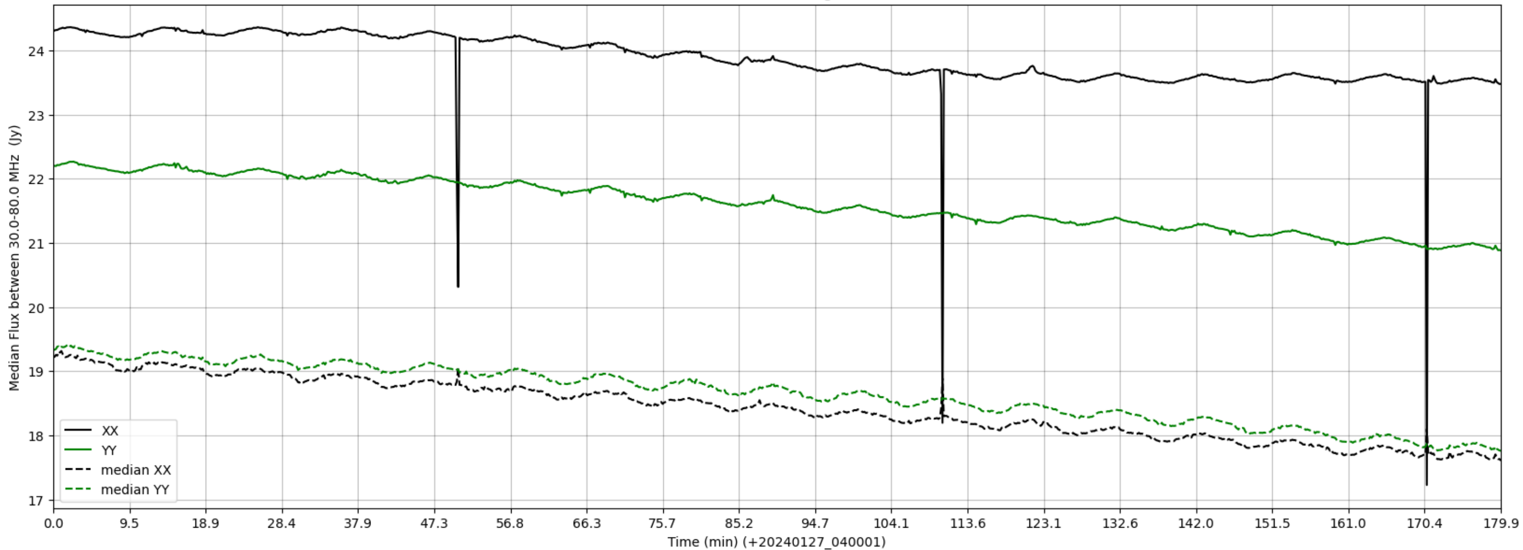
LWA281 - Correlator# 011 - XX FLAGS:HighTimeVar - YY FLAGS:Good
