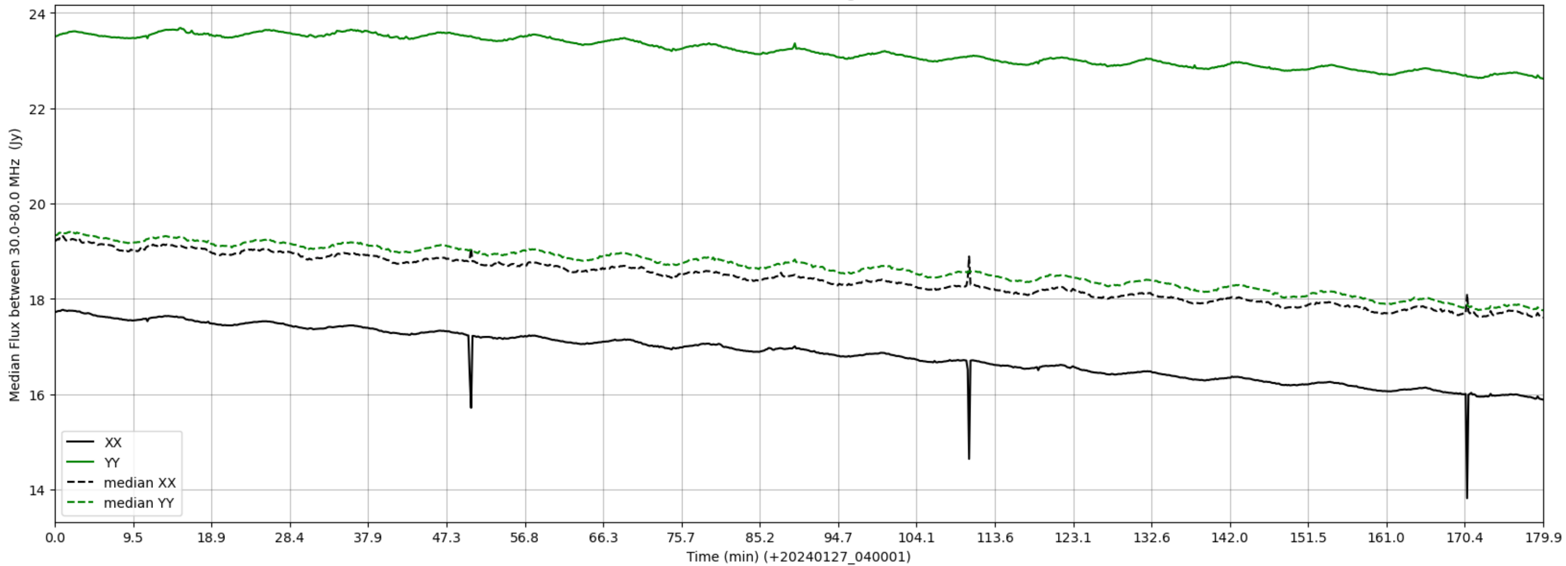
LWA311 - Correlator# 016 - XX FLAGS:HighTimeVar - YY FLAGS:Good
