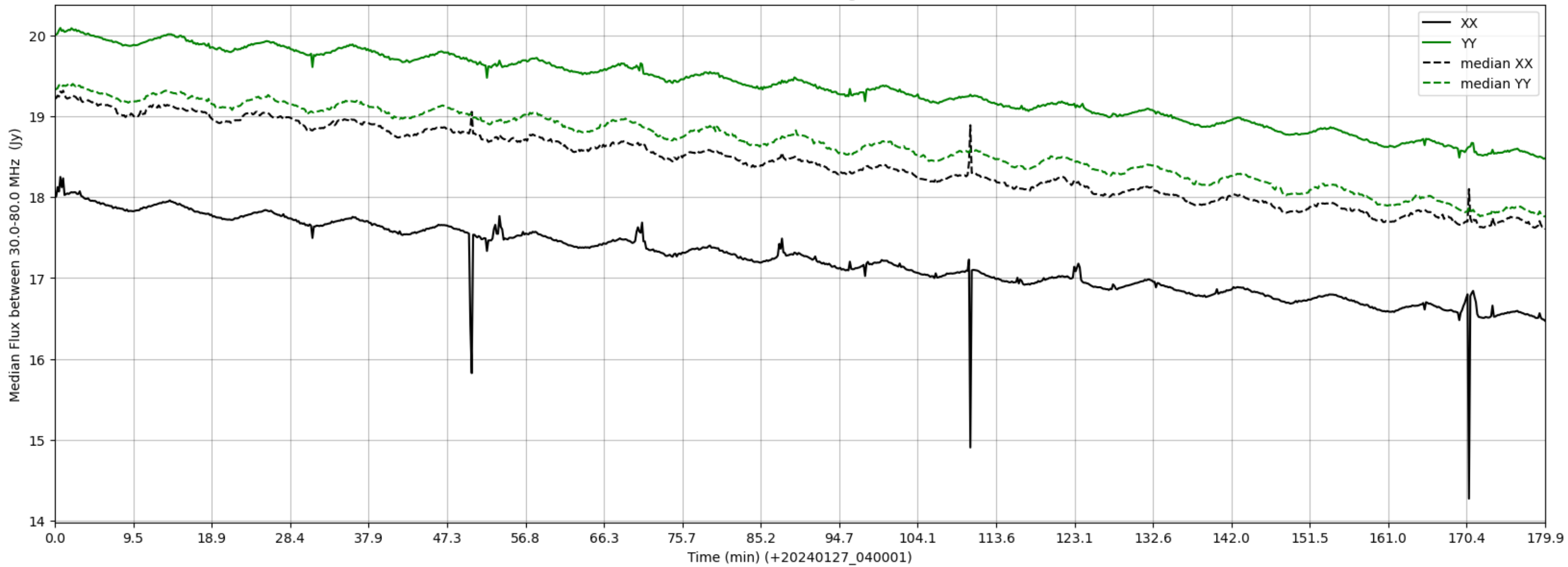
LWA092 - Correlator# 149 - XX FLAGS:HighTimeVar - YY FLAGS:Good
