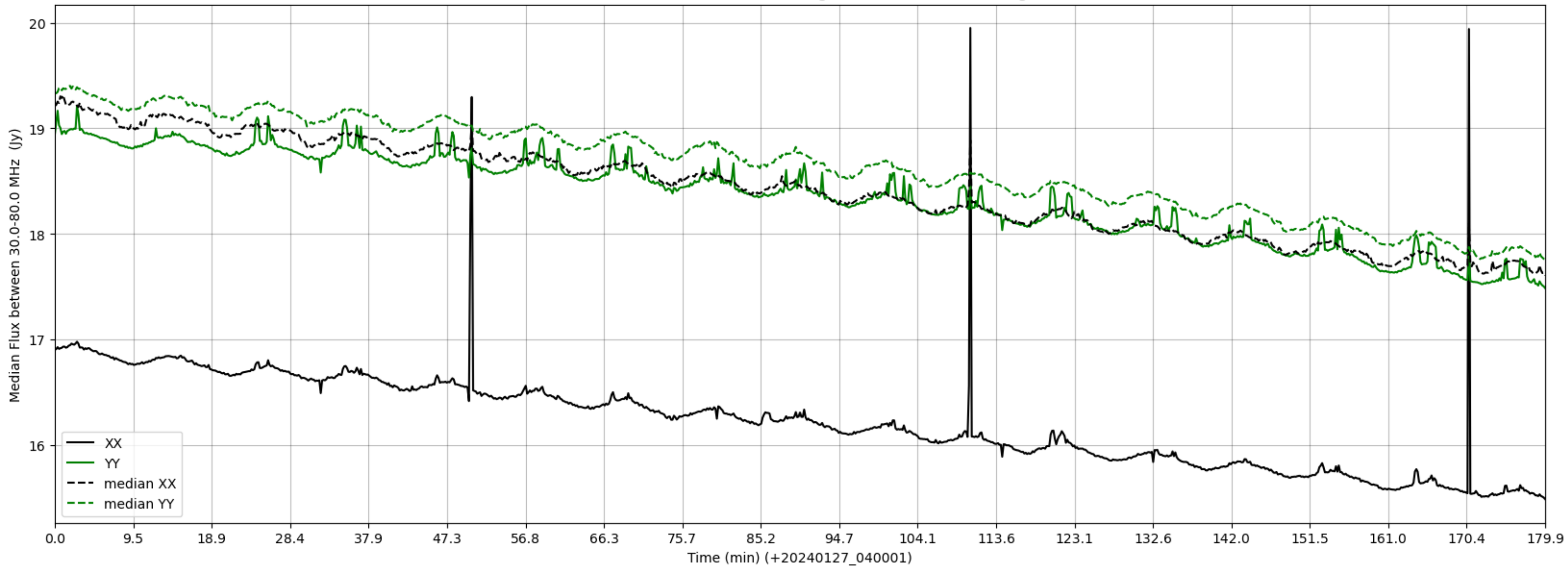
LWA071 - Correlator# 084 - XX FLAGS:HighTimeVar - YY FLAGS:HighTimeVar
