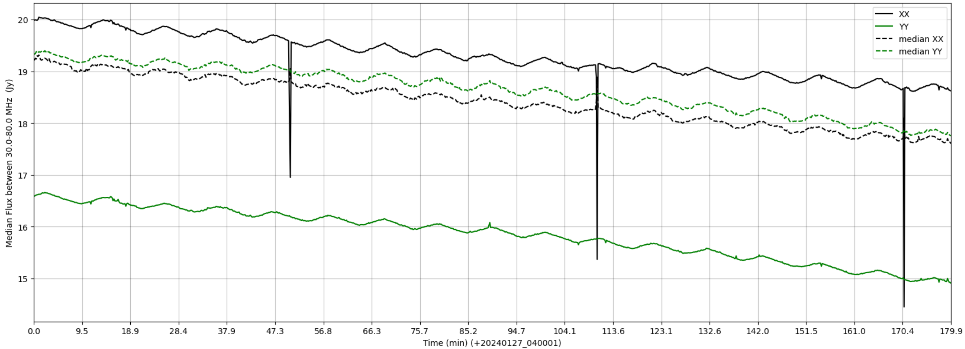
LWA321 - Correlator# 020 - XX FLAGS:HighTimeVar - YY FLAGS:Good
