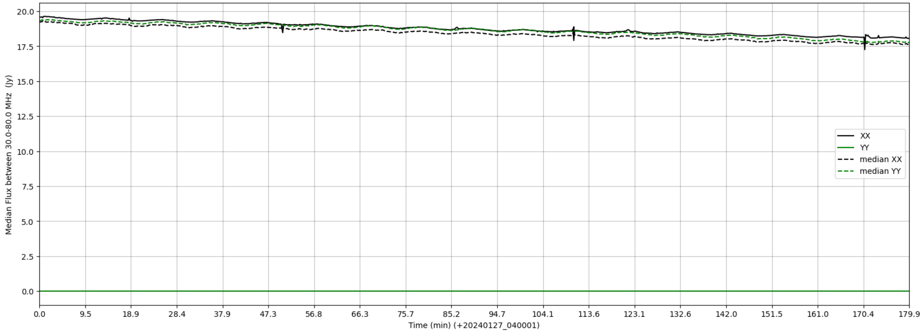
LWA325 - Correlator# 154 - XX FLAGS:Good - YY FLAGS:LowFlux
