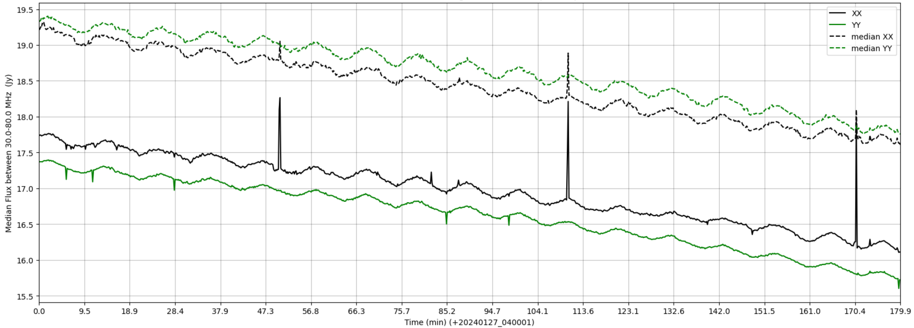
LWA341 - Correlator# 029 - XX FLAGS:HighTimeVar+BadSpecShape - YY FLAGS:Good
