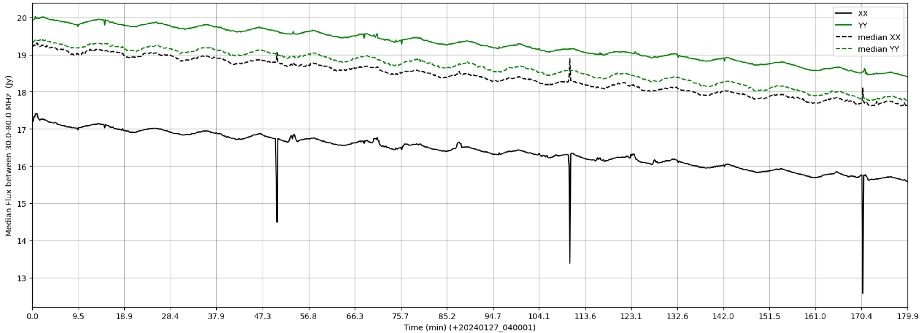
LWA278 - Correlator# 008 - XX FLAGS:HighTimeVar - YY FLAGS:Good
