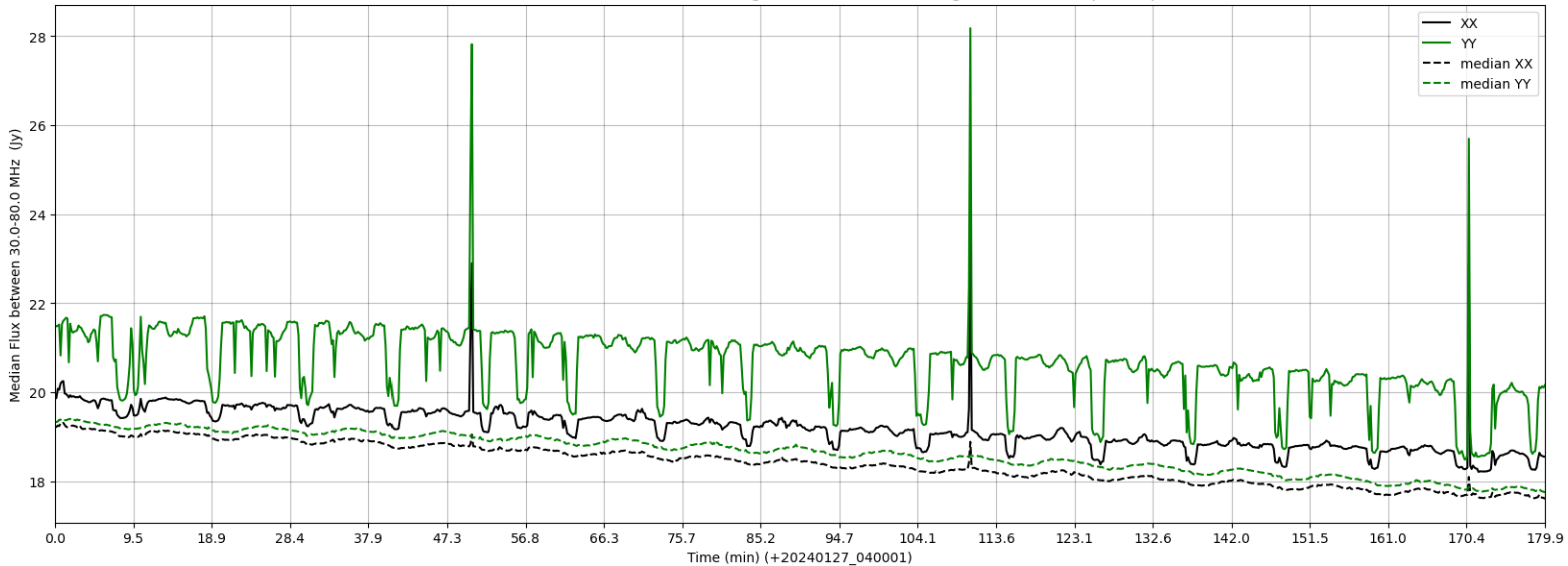
LWA104 - Correlator# 179 - XX FLAGS:HighTimeVar - YY FLAGS:HighTimeVar+BadSpecShape
