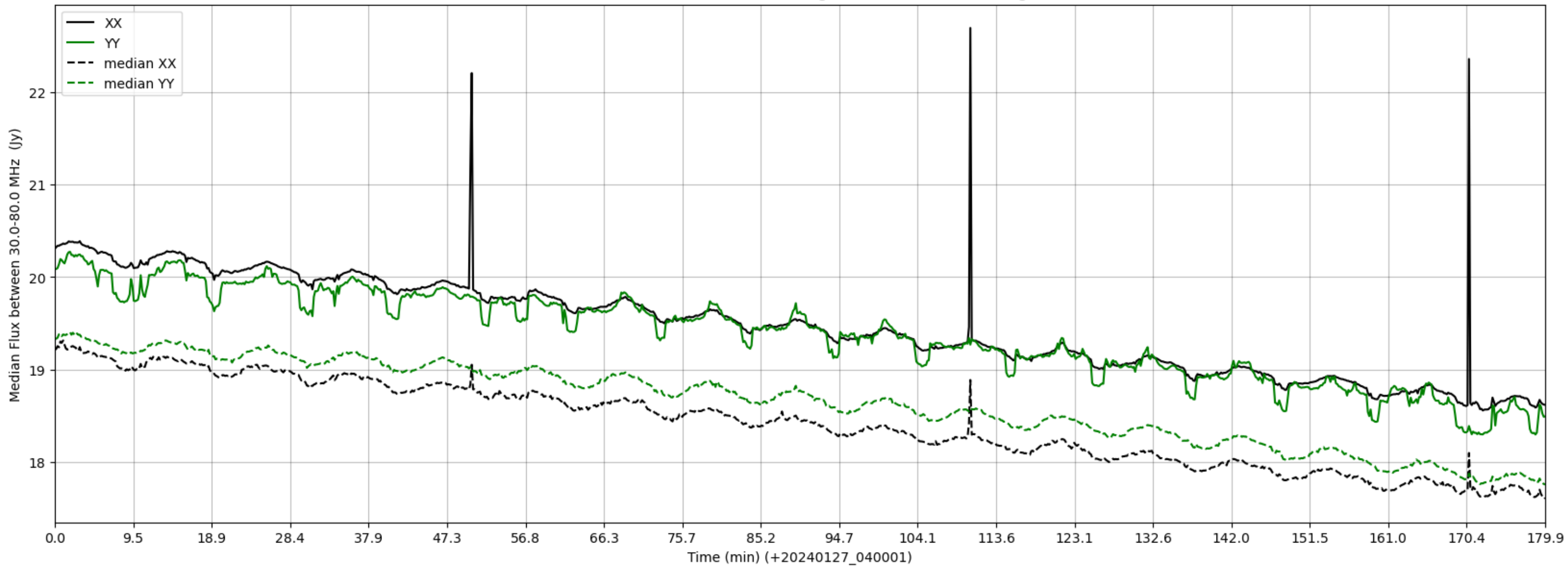
LWA131 - Correlator# 182 - XX FLAGS:HighTimeVar - YY FLAGS:HighTimeVar
