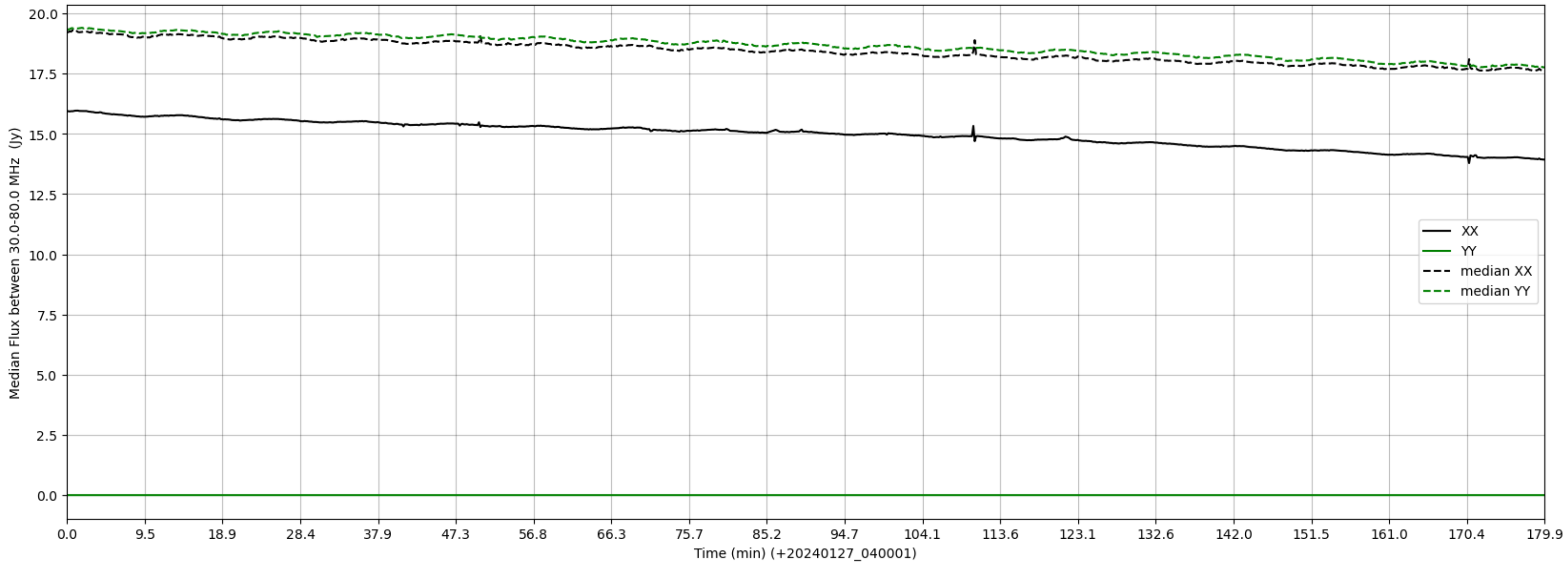
LWA314 - Correlator# 021 - XX FLAGS:Good - YY FLAGS:LowFlux
