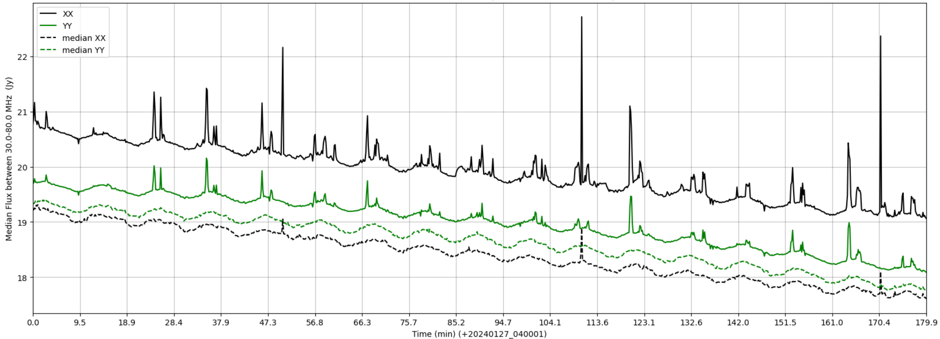
LWA040 - Correlator# 076 - XX FLAGS:HighTimeVar - YY FLAGS:HighTimeVar
