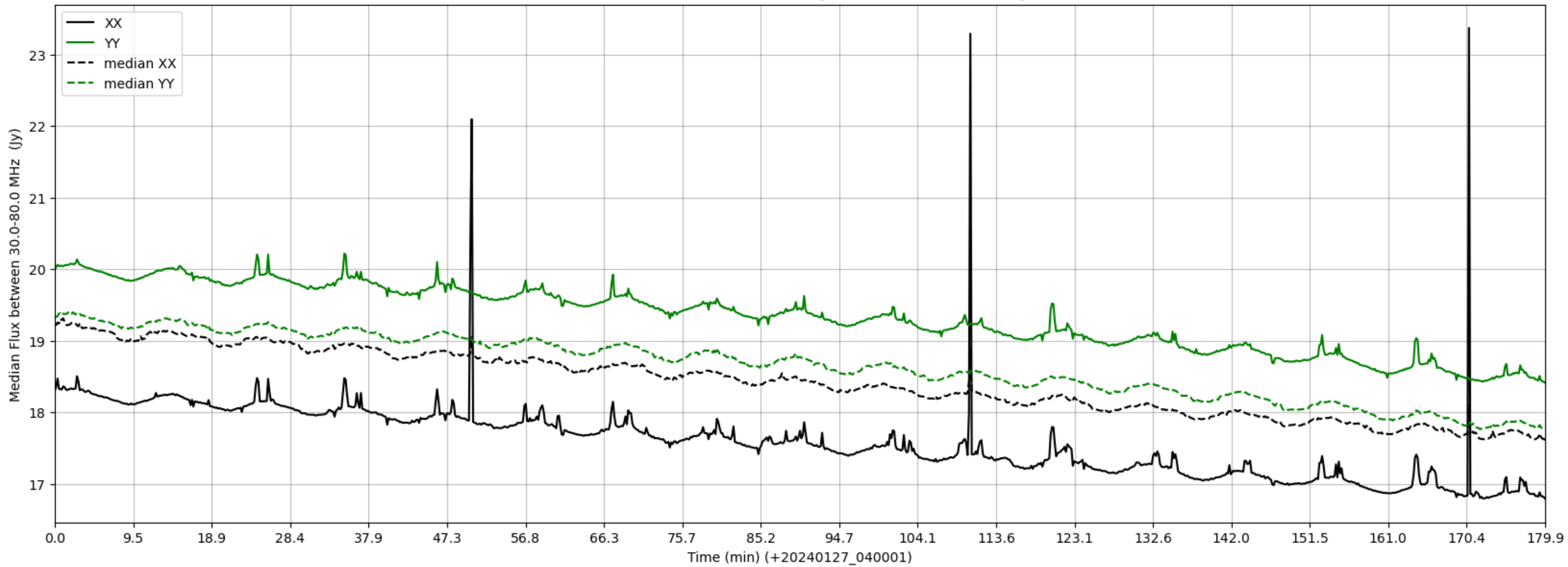
LWA011 - Correlator# 072 - XX FLAGS:HighTimeVar - YY FLAGS:HighTimeVar
