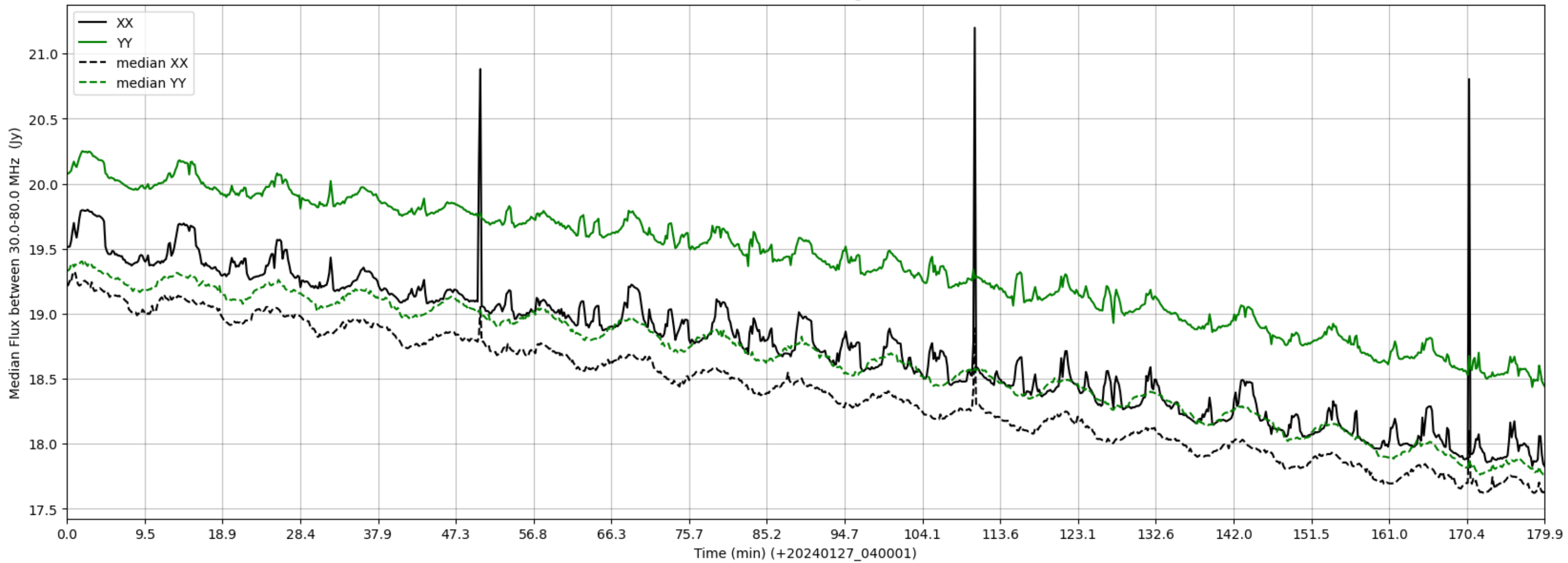
LWA144 - Correlator# 213 - XX FLAGS:HighTimeVar - YY FLAGS:Good
