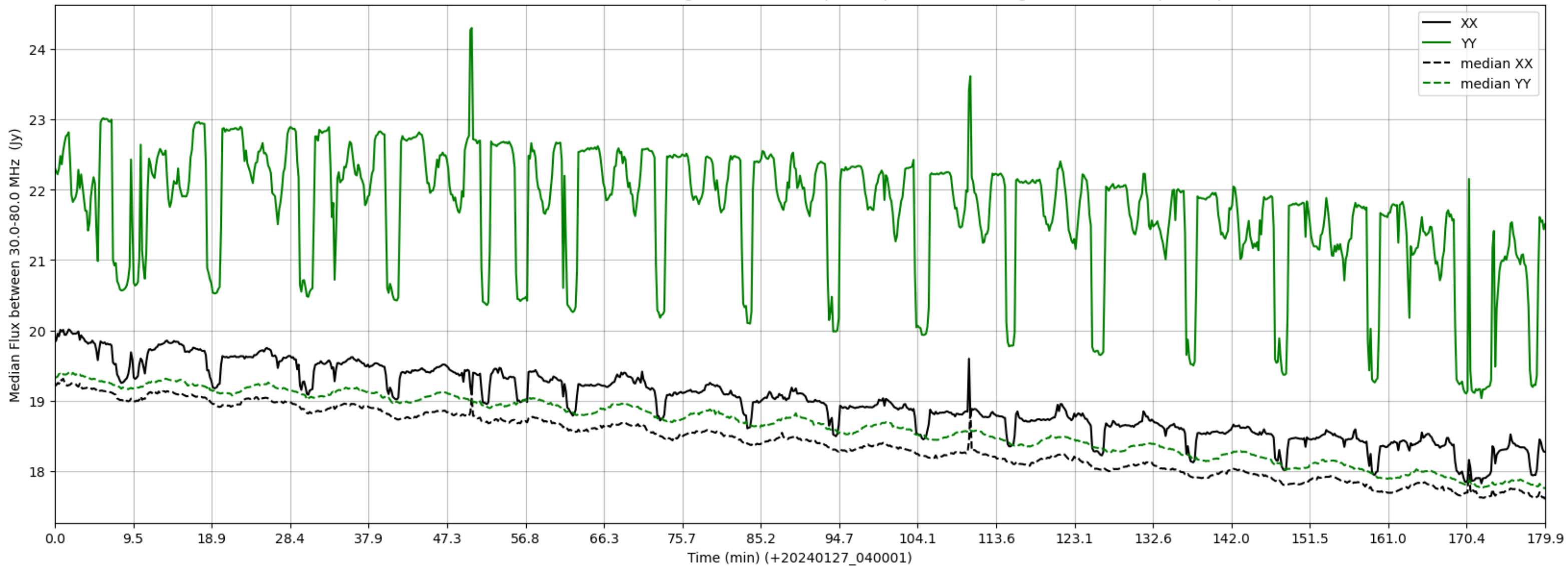
LWA037 - Correlator# 181 - XX FLAGS:HighTimeVar+BadSpecShape - YY FLAGS:HighTimeVar+BadSpecShape
