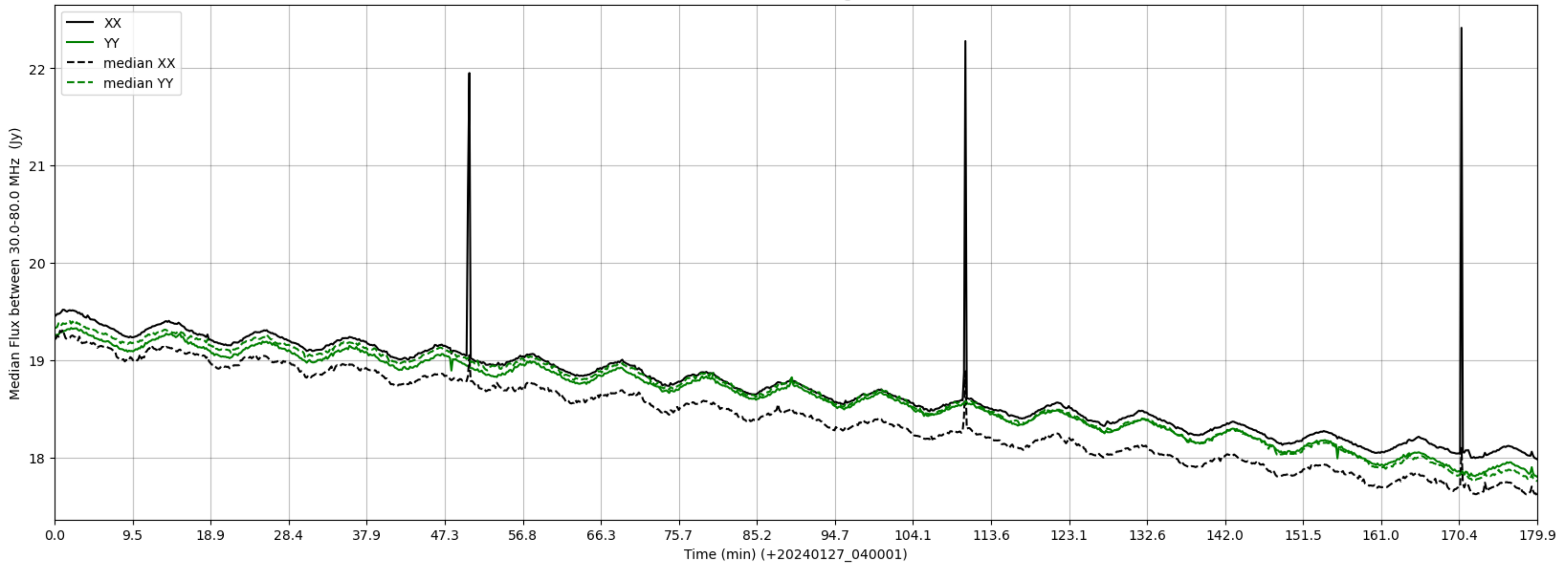
LWA135 - Correlator# 256 - XX FLAGS:HighTimeVar - YY FLAGS:Good
