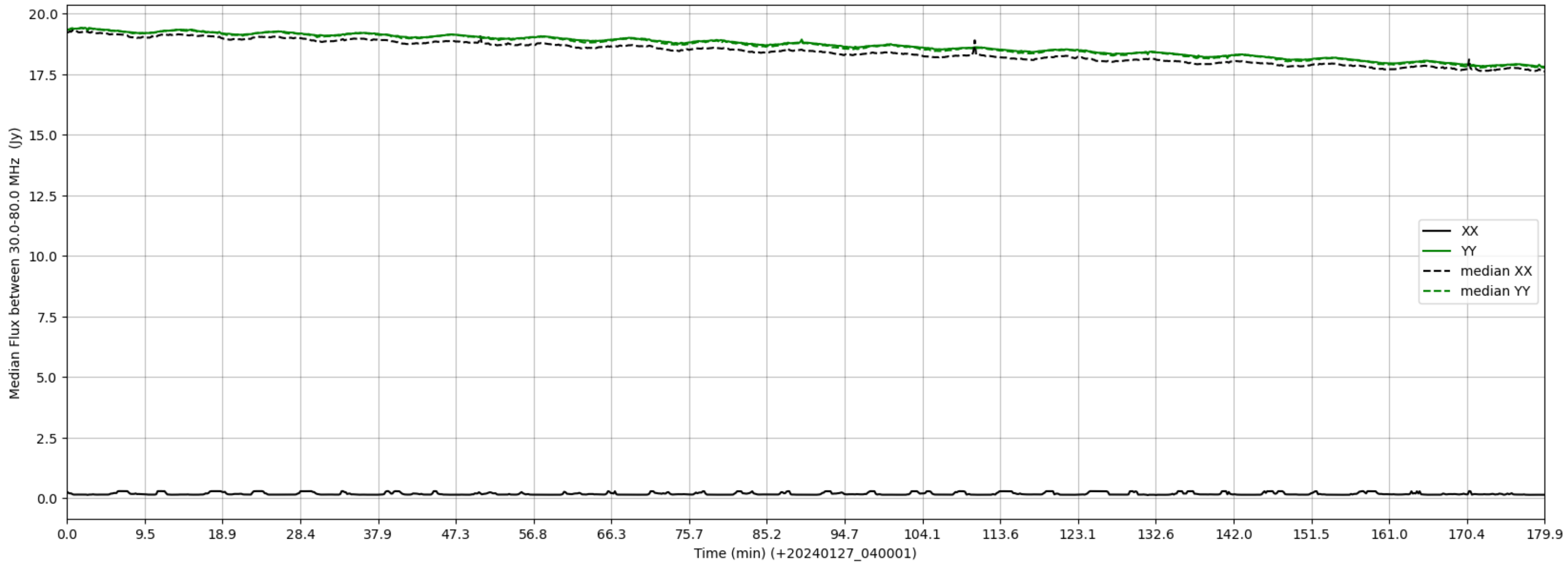
LWA138 - Correlator# 261 - XX FLAGS:LowFlux - YY FLAGS:Good
