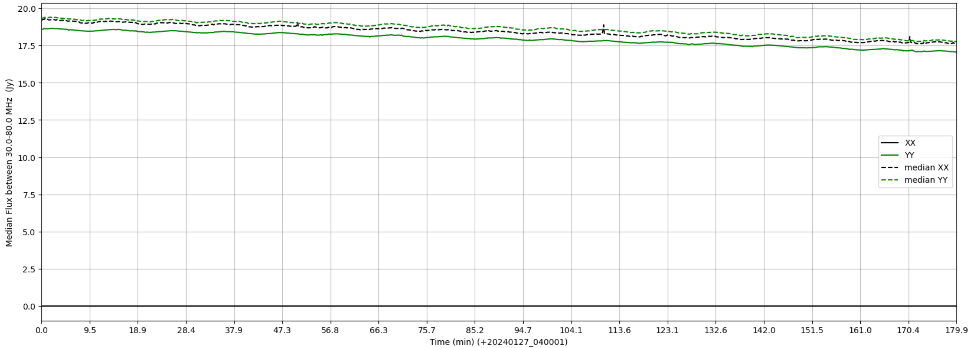
LWA095 - Correlator# 150 - XX FLAGS:LowFlux - YY FLAGS:Good
