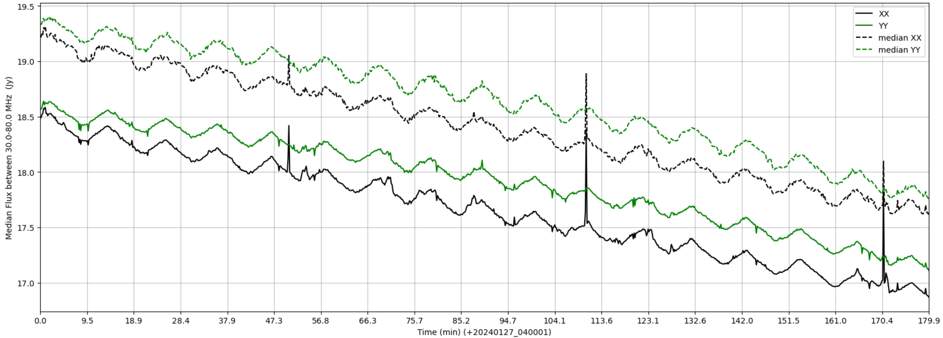
LWA186 - Correlator# 243 - XX FLAGS:Good - YY FLAGS:Good
