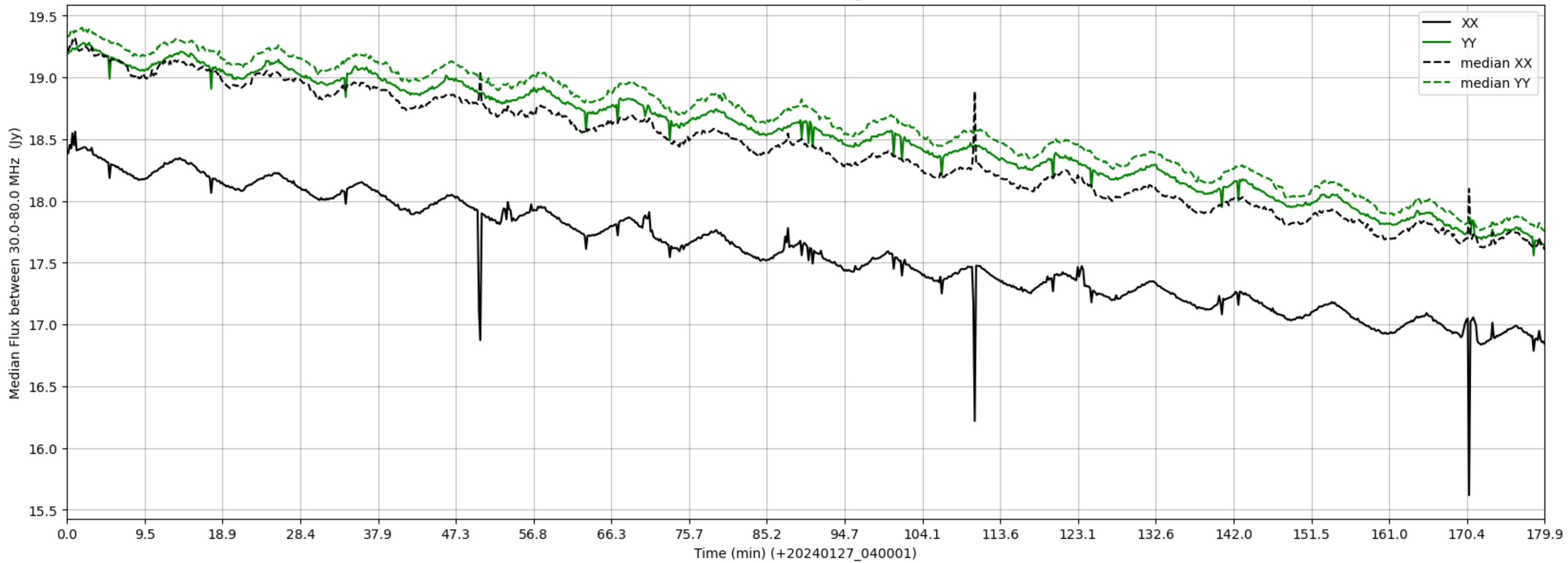
LWA062 - Correlator# 138 - XX FLAGS:HighTimeVar - YY FLAGS:Good
