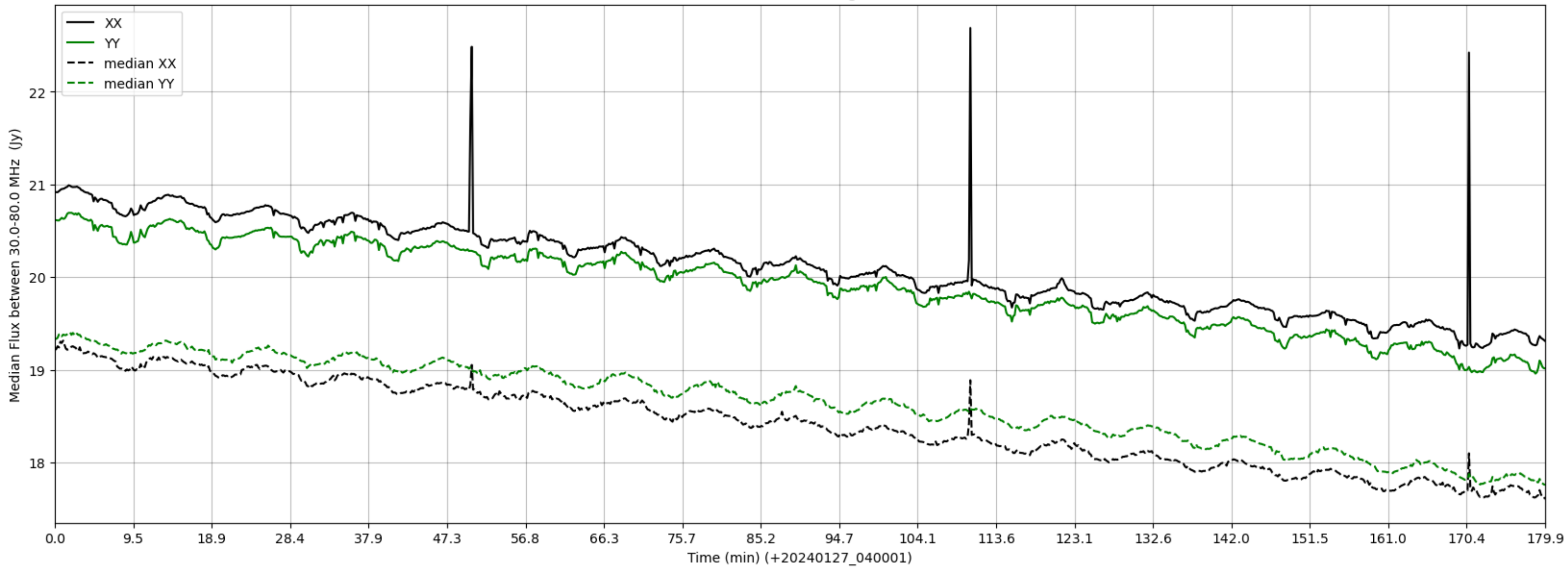
LWA069 - Correlator# 169 - XX FLAGS:HighTimeVar - YY FLAGS:Good
