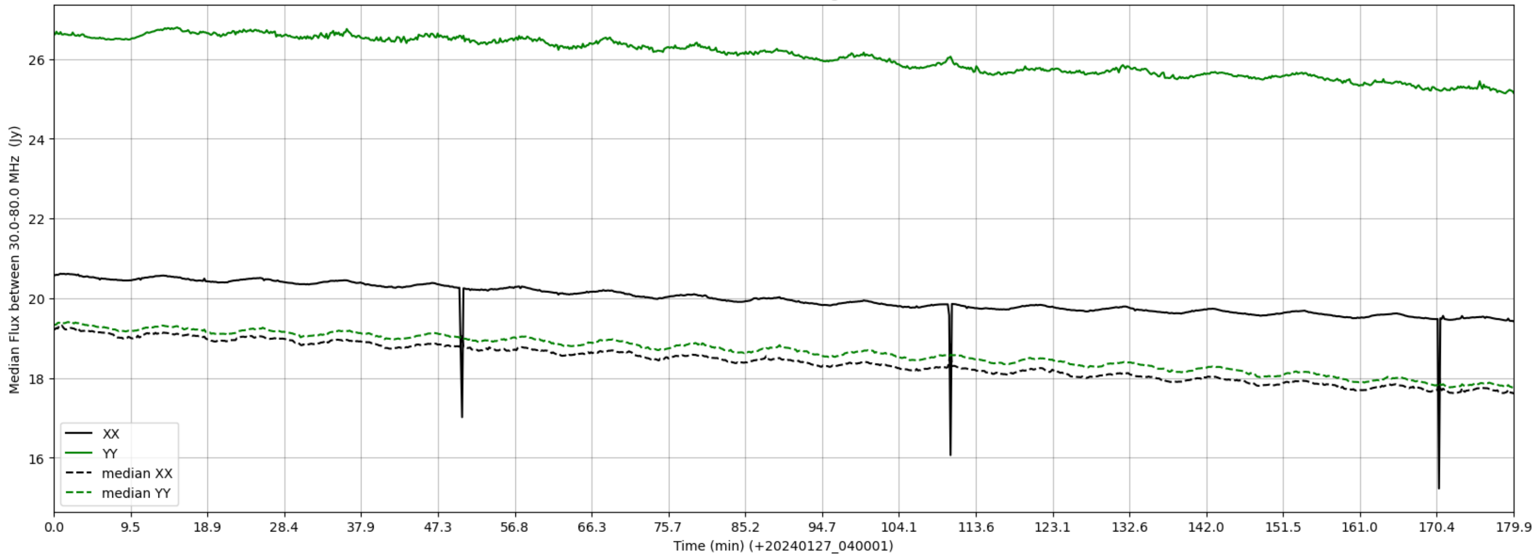
LWA322 - Correlator# 251 - XX FLAGS:HighTimeVar - YY FLAGS:Good
