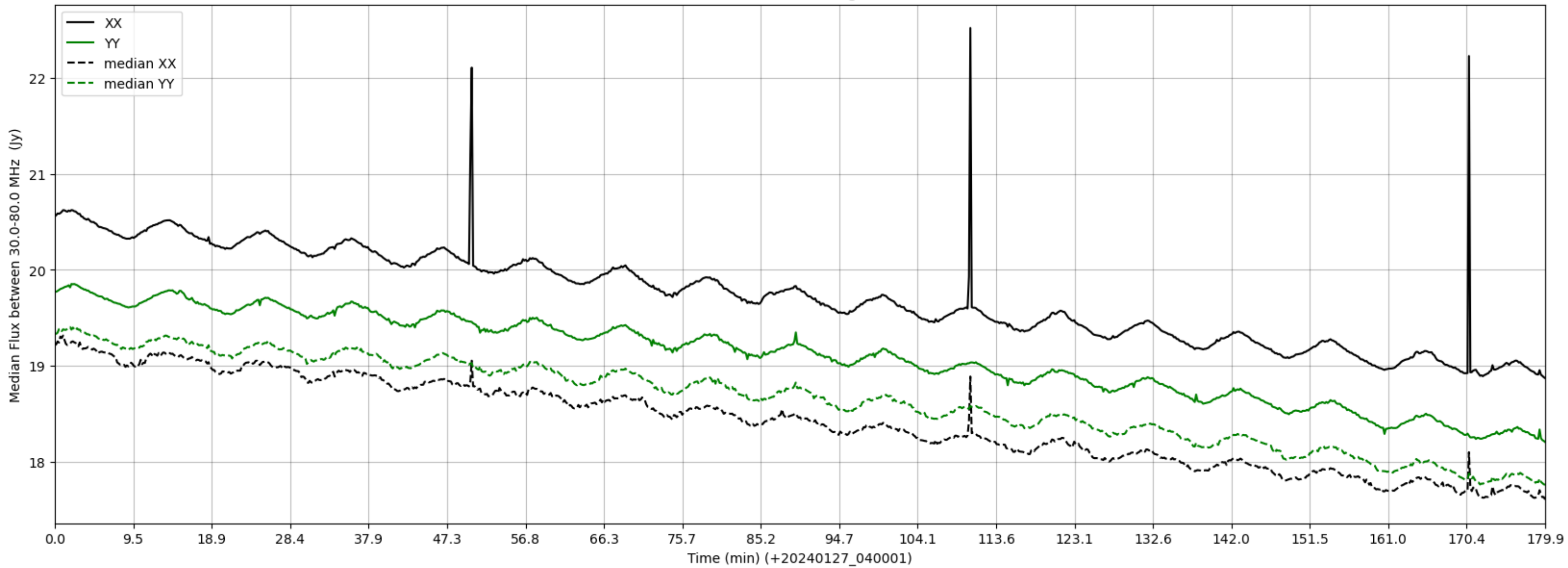
LWA018 - Correlator# 100 - XX FLAGS:HighTimeVar - YY FLAGS:Good
