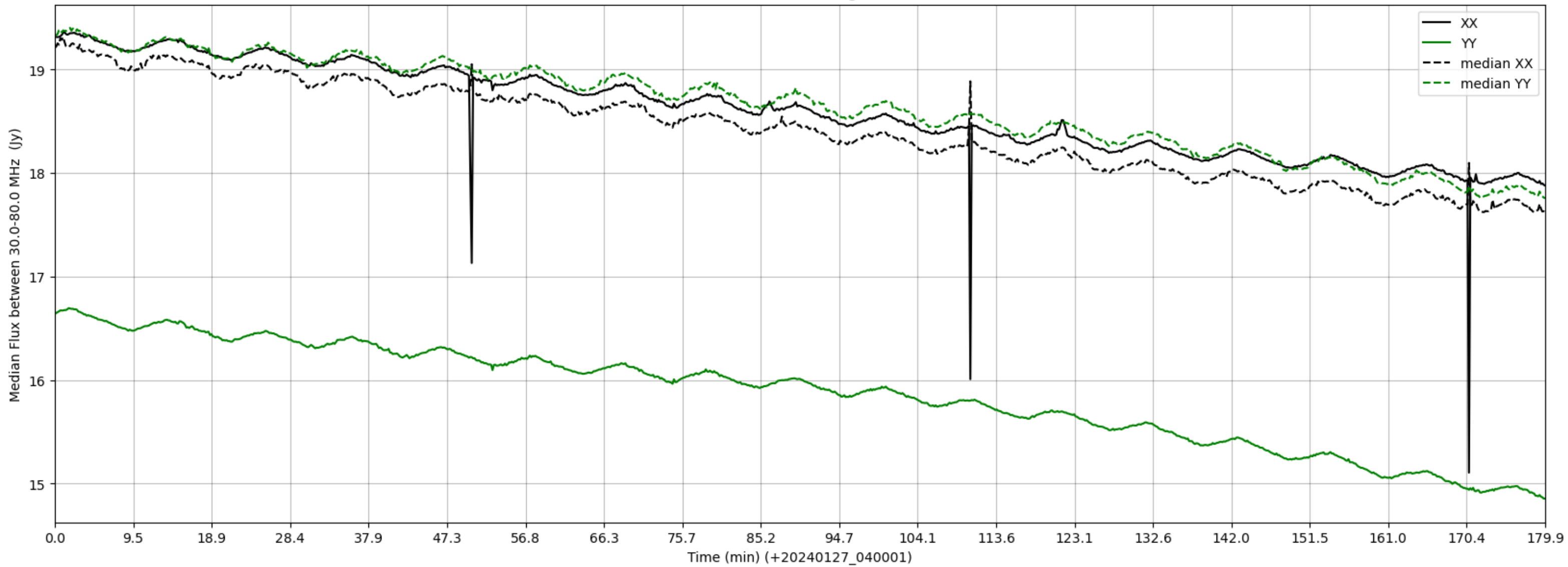
LWA266 - Correlator# 000 - XX FLAGS:HighTimeVar - YY FLAGS:Good
