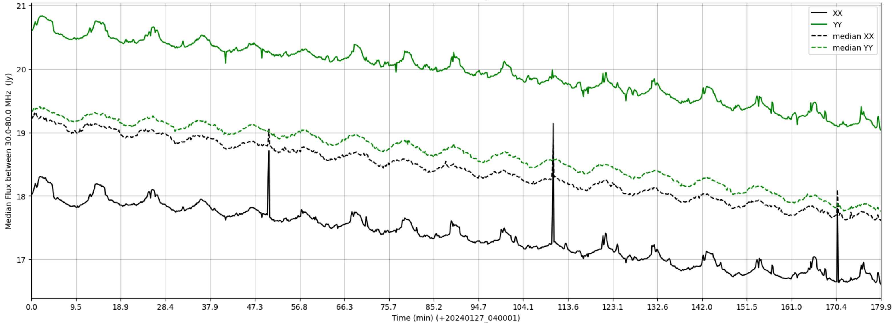
LWA118 - Correlator# 206 - XX FLAGS:HighTimeVar - YY FLAGS:Good
