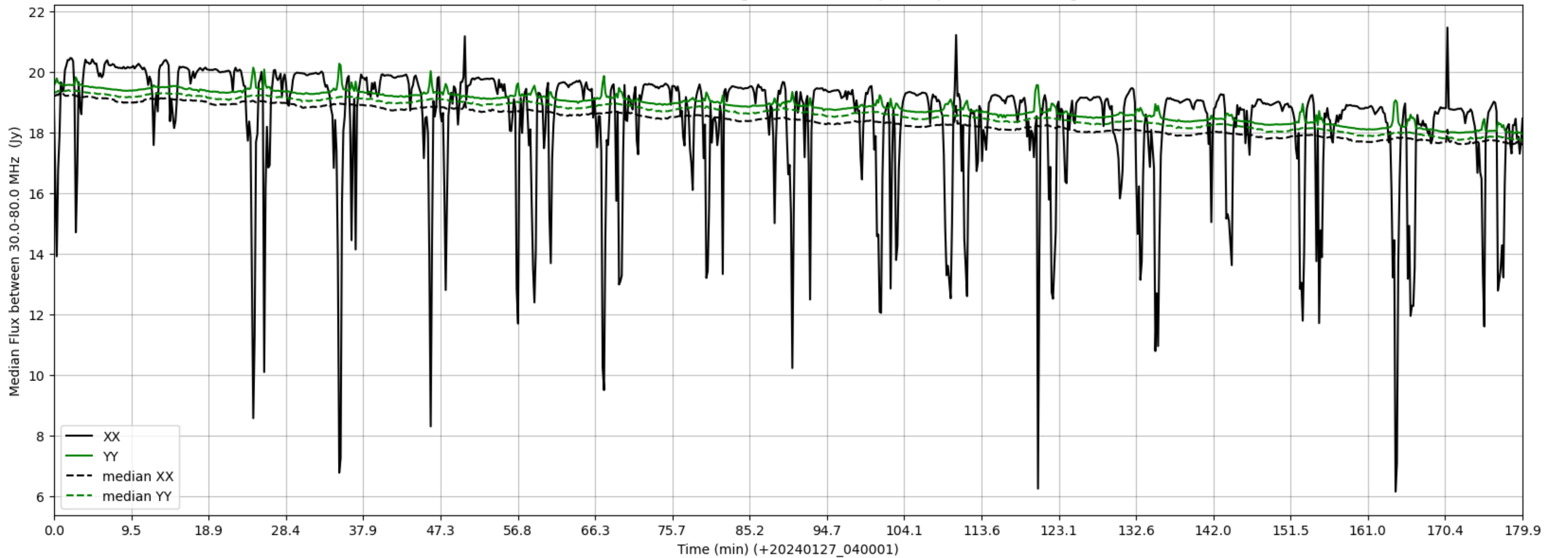
LWA041 - Correlator# 079 - XX FLAGS:HighTimeVar+BadSpecShape - YY FLAGS:HighTimeVar
