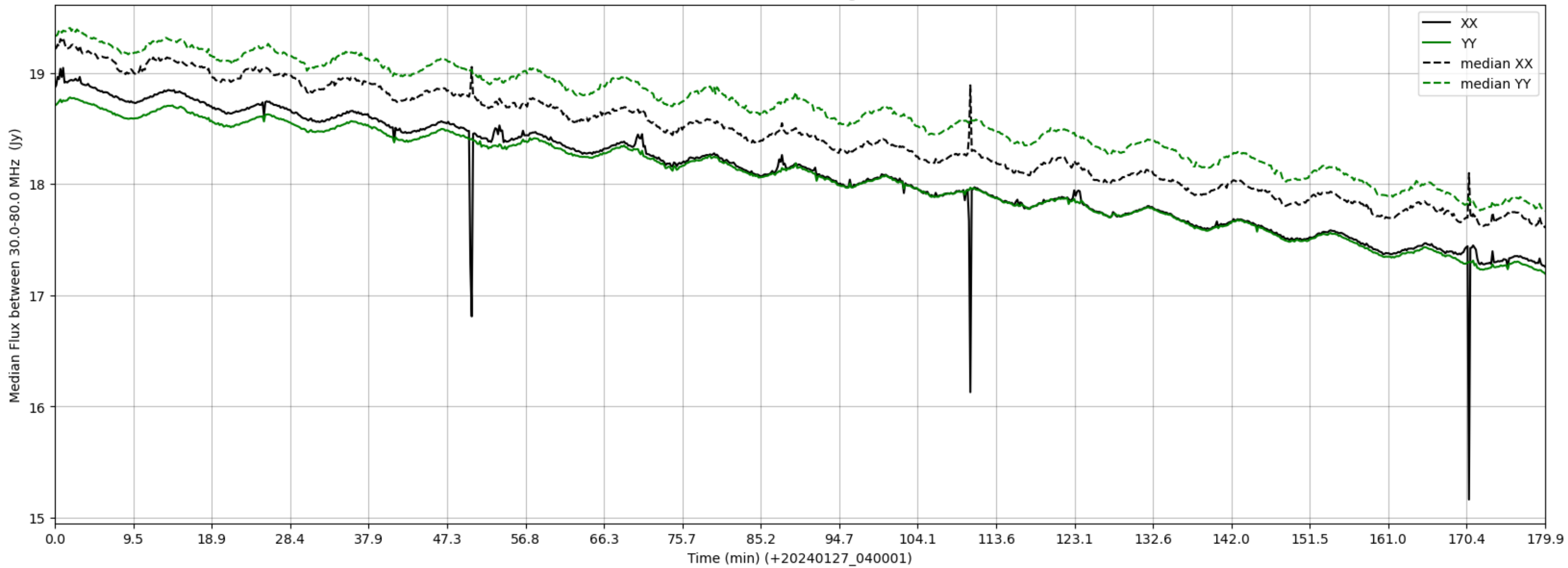
LWA094 - Correlator# 151 - XX FLAGS:HighTimeVar - YY FLAGS:Good
