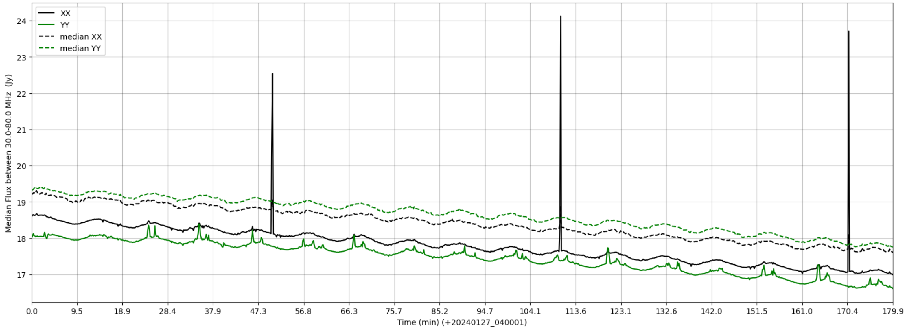
LWA010 - Correlator# 073 - XX FLAGS:HighTimeVar - YY FLAGS:HighTimeVar
