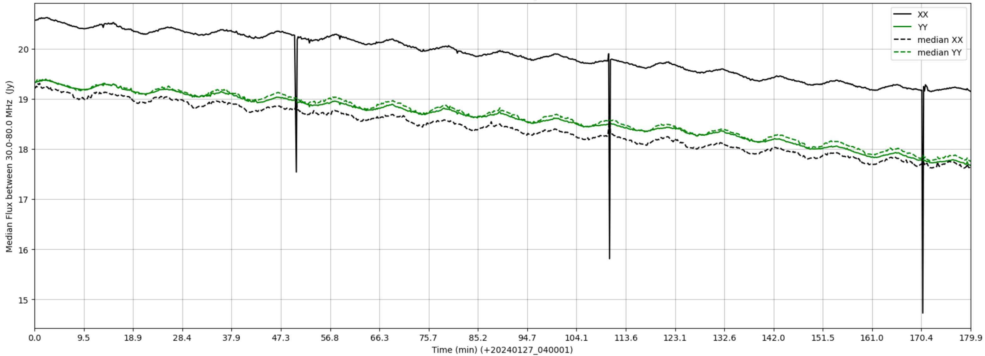
LWA327 - Correlator# 023 - XX FLAGS:HighTimeVar - YY FLAGS:Good
