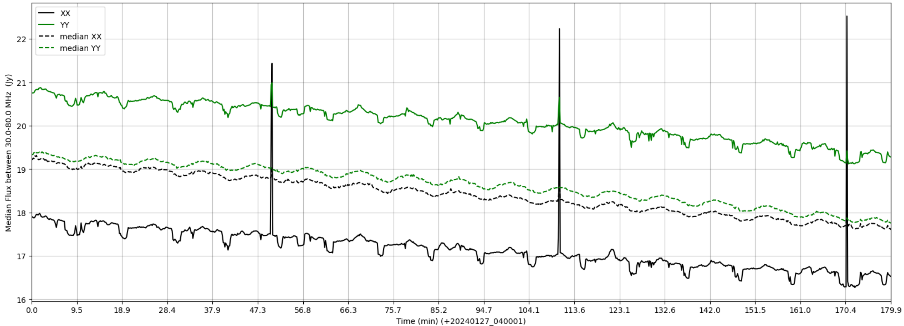
LWA100 - Correlator# 175 - XX FLAGS:HighTimeVar - YY FLAGS:HighTimeVar
