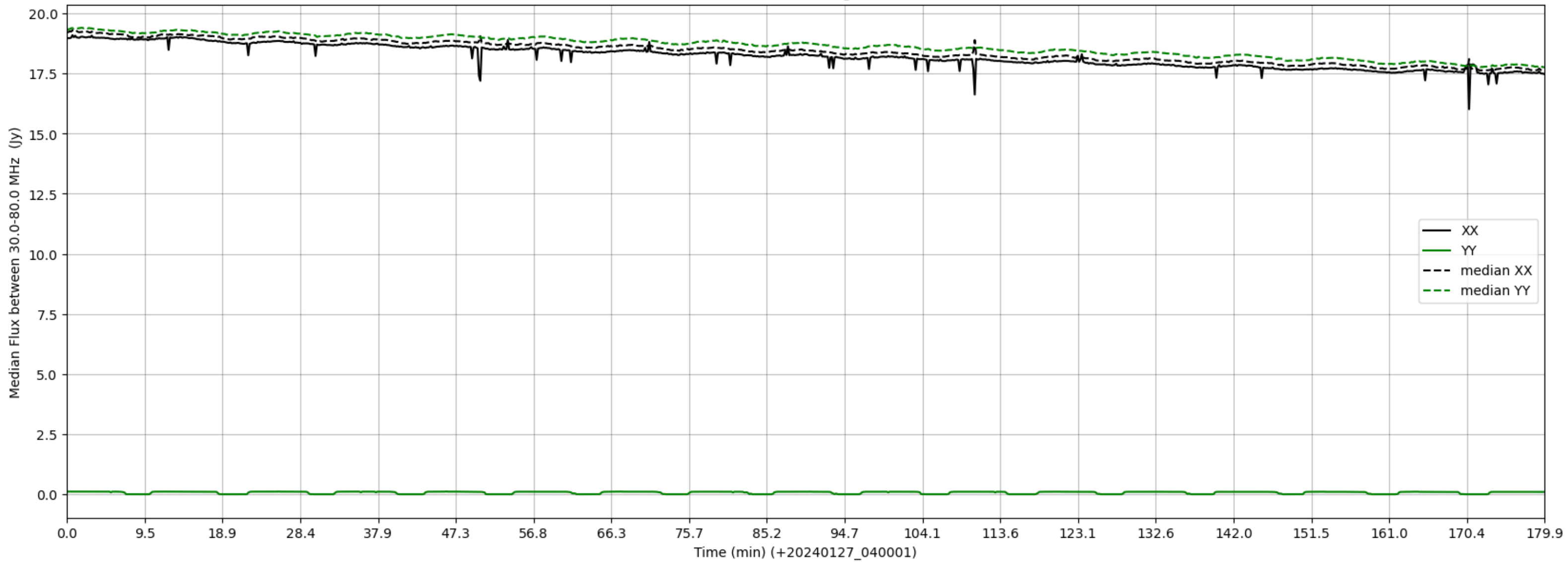
LWA058 - Correlator# 137 - XX FLAGS:HighTimeVar - YY FLAGS:LowFlux
