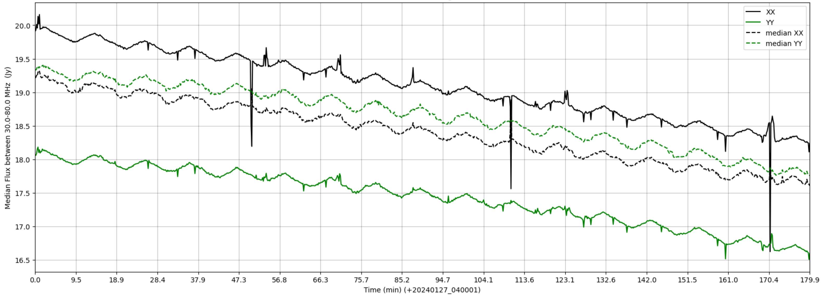
LWA060 - Correlator# 133 - XX FLAGS:HighTimeVar - YY FLAGS:Good
