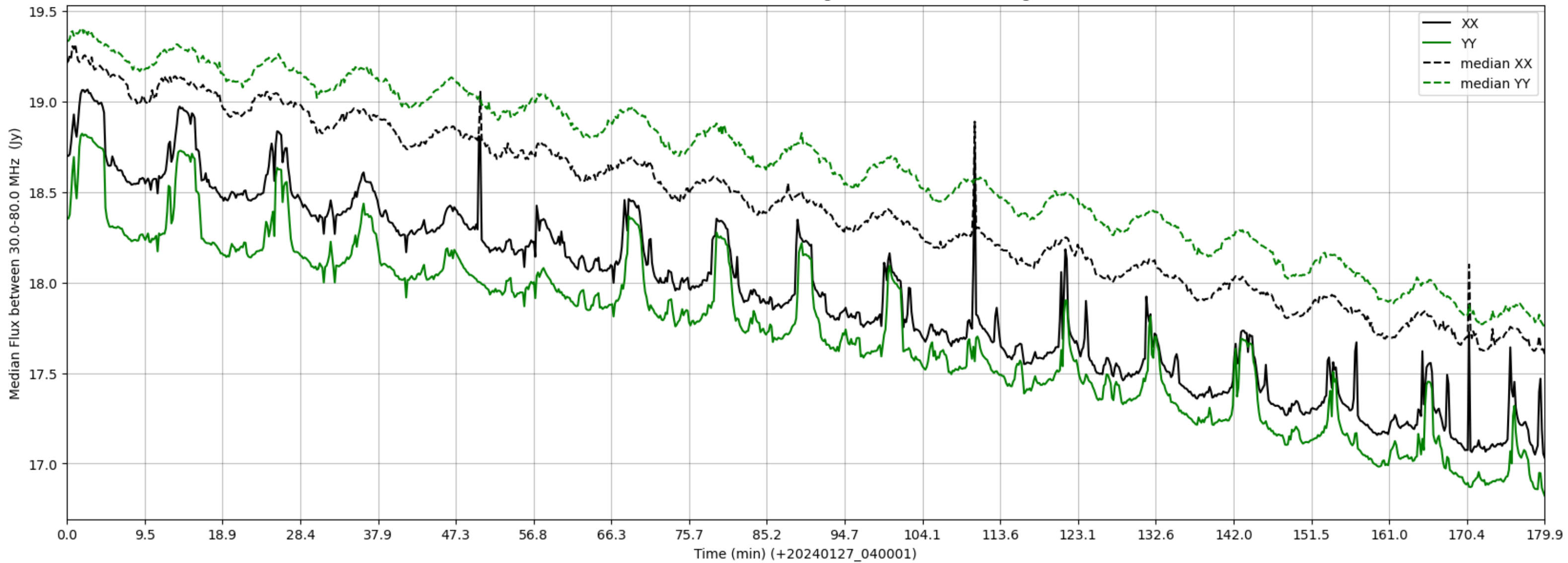
LWA082 - Correlator# 209 - XX FLAGS:HighTimeVar - YY FLAGS:HighTimeVar
