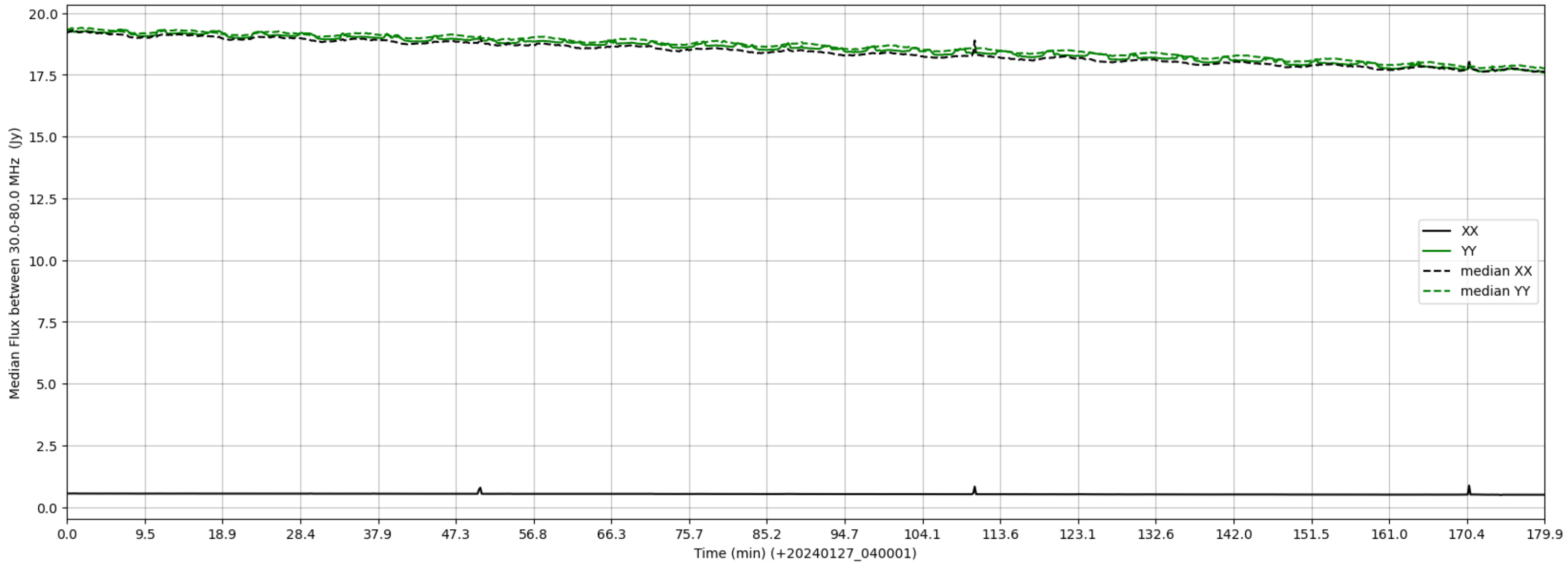
LWA234 - Correlator# 289 - XX FLAGS:LowFlux - YY FLAGS:Good
