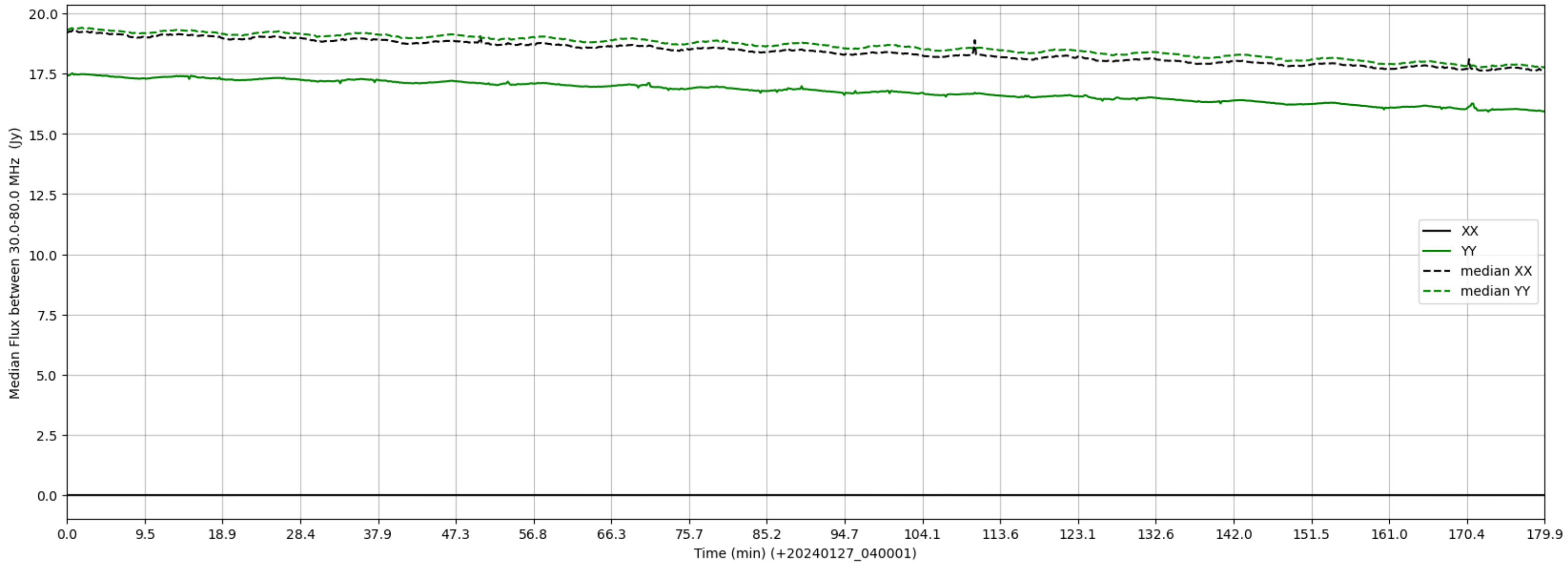
LWA159 - Correlator# 236 - XX FLAGS:LowFlux - YY FLAGS:Good
