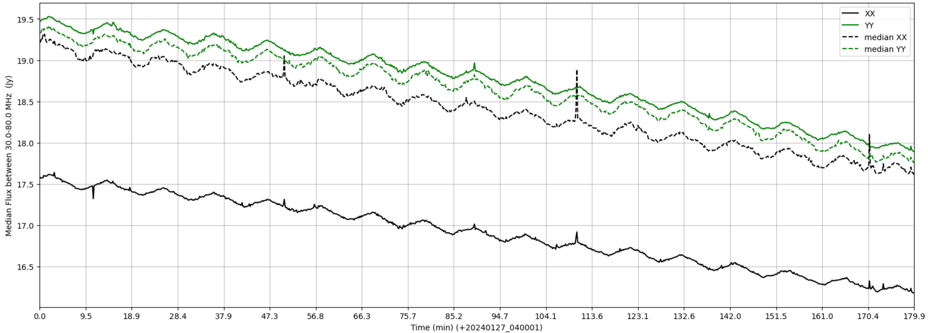
LWA300 - Correlator# 348 - XX FLAGS:Good - YY FLAGS:Good
