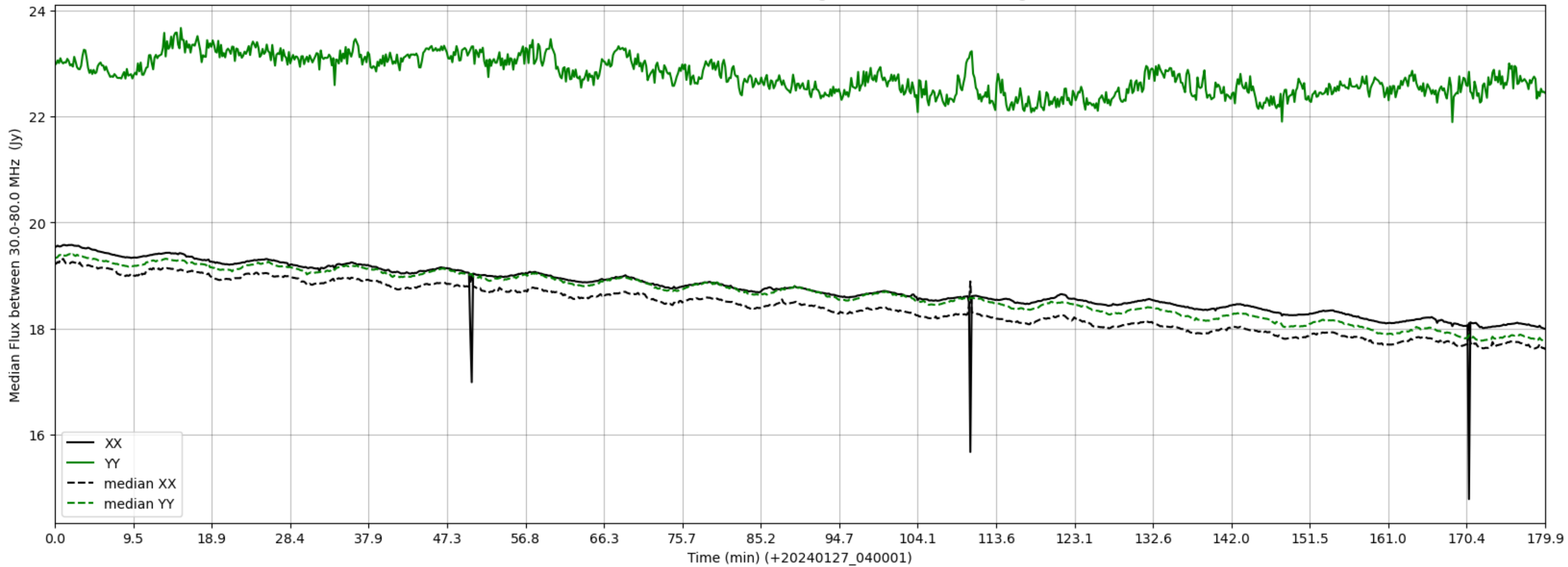
LWA282 - Correlator# 010 - XX FLAGS:HighTimeVar - YY FLAGS:HighTimeVar
