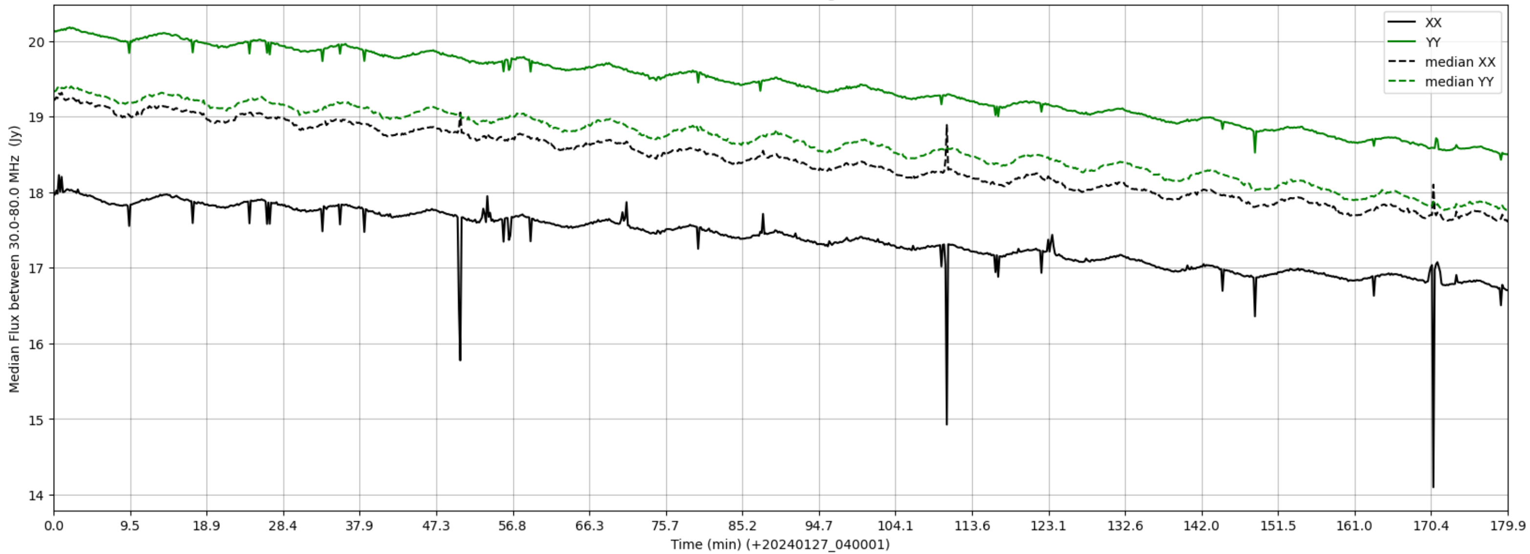
LWA064 - Correlator# 141 - XX FLAGS:HighTimeVar - YY FLAGS:Good
