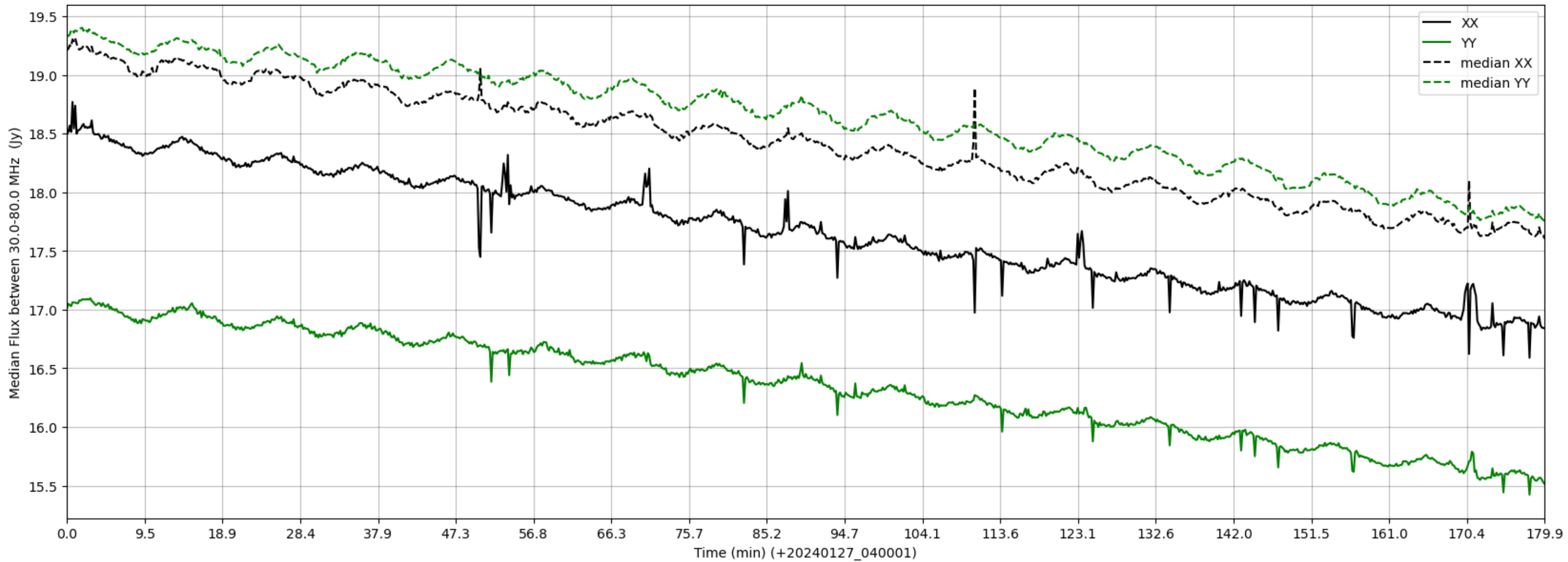
LWA190 - Correlator# 244 - XX FLAGS:Good - YY FLAGS:Good
