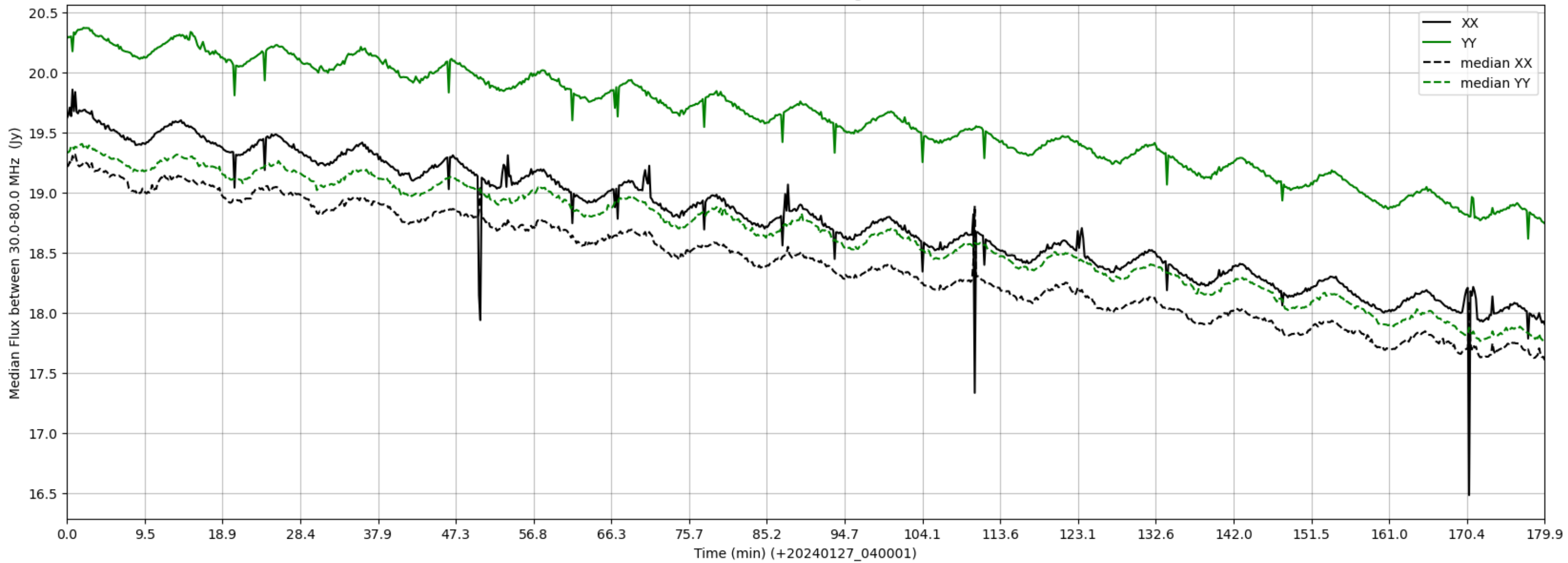
LWA032 - Correlator# 130 - XX FLAGS:HighTimeVar - YY FLAGS:Good
