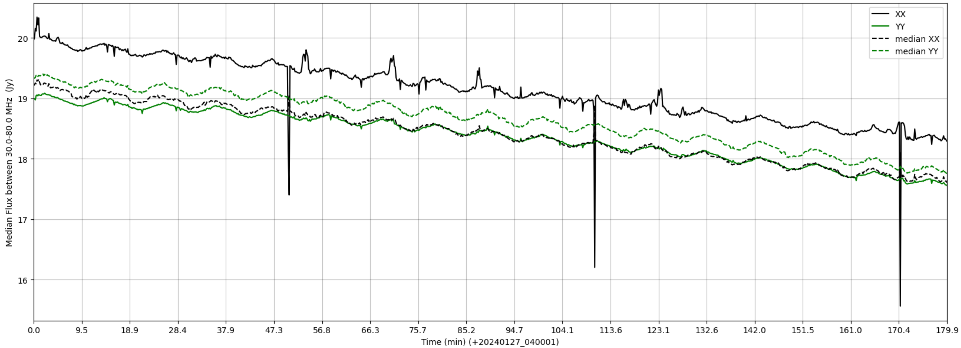
LWA126 - Correlator# 226 - XX FLAGS:HighTimeVar - YY FLAGS:Good
