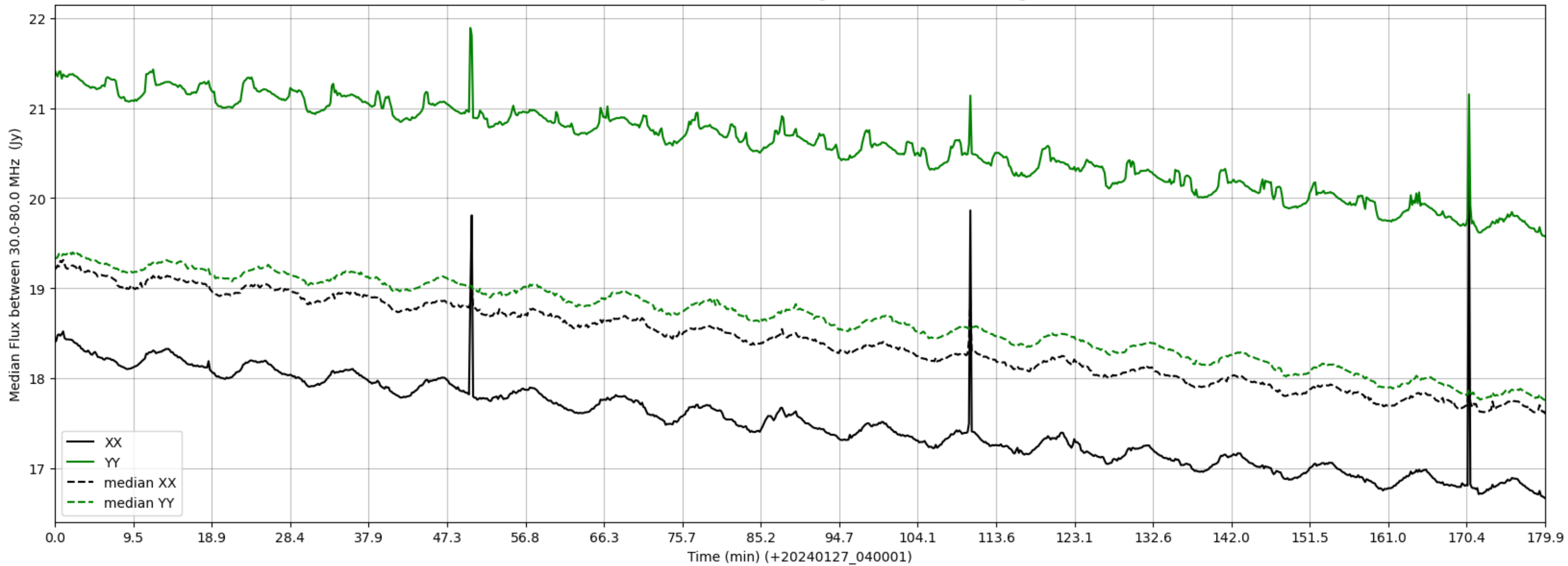
LWA173 - Correlator# 290 - XX FLAGS:HighTimeVar - YY FLAGS:HighTimeVar
