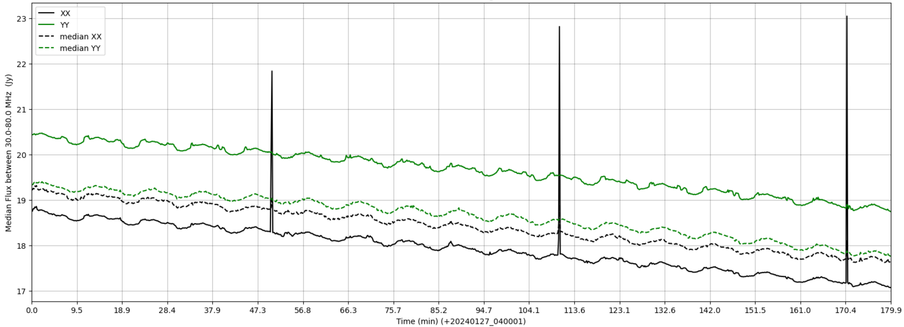
LWA240 - Correlator# 312 - XX FLAGS:HighTimeVar - YY FLAGS:Good
