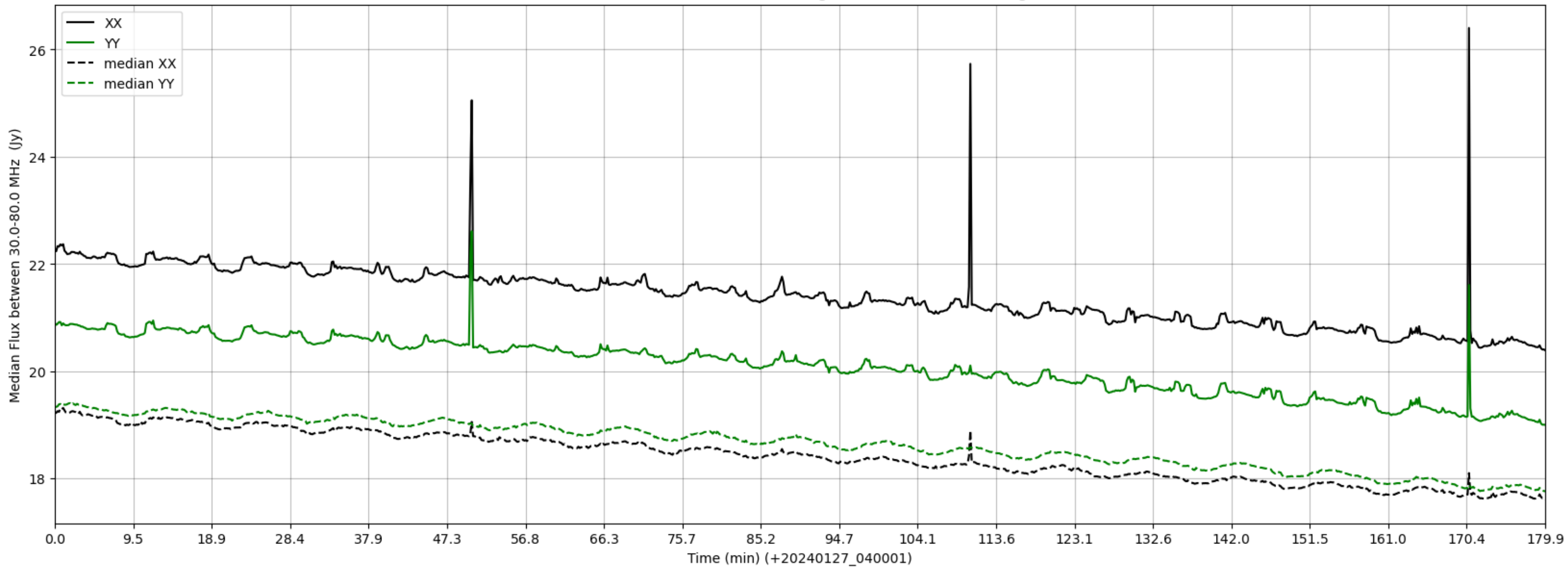
LWA254 - Correlator# 315 - XX FLAGS:HighTimeVar - YY FLAGS:HighTimeVar
