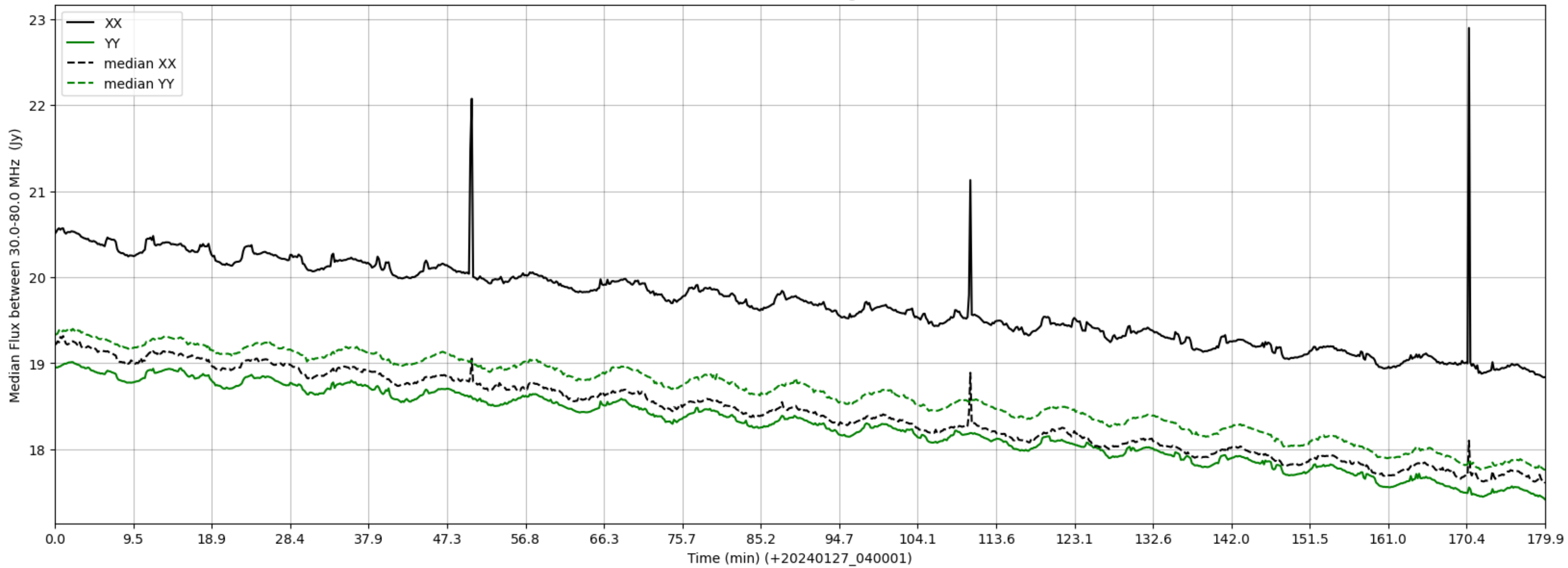
LWA239 - Correlator# 313 - XX FLAGS:HighTimeVar - YY FLAGS:Good
