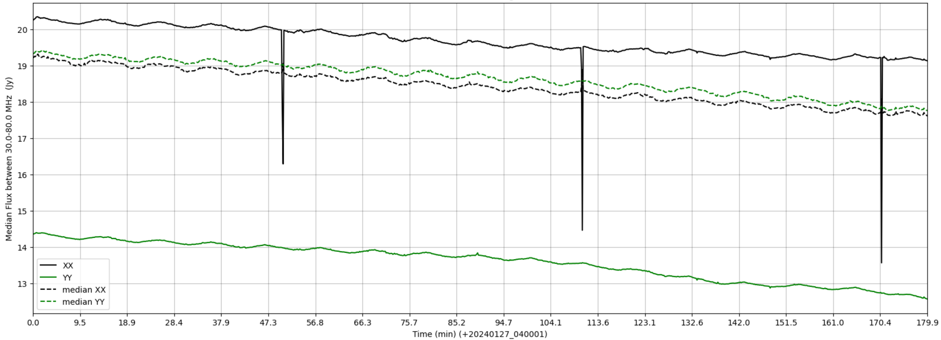
LWA271 - Correlator# 004 - XX FLAGS:HighTimeVar - YY FLAGS:Good
