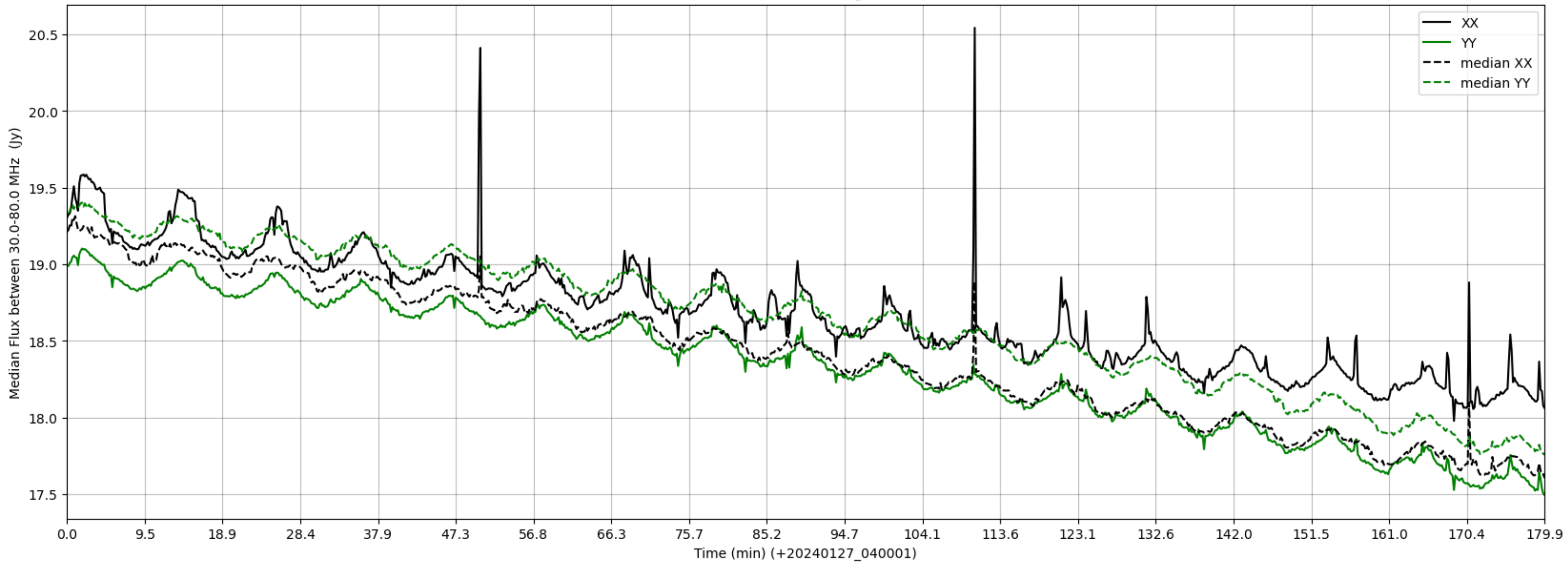
LWA117 - Correlator# 207 - XX FLAGS:HighTimeVar - YY FLAGS:Good
