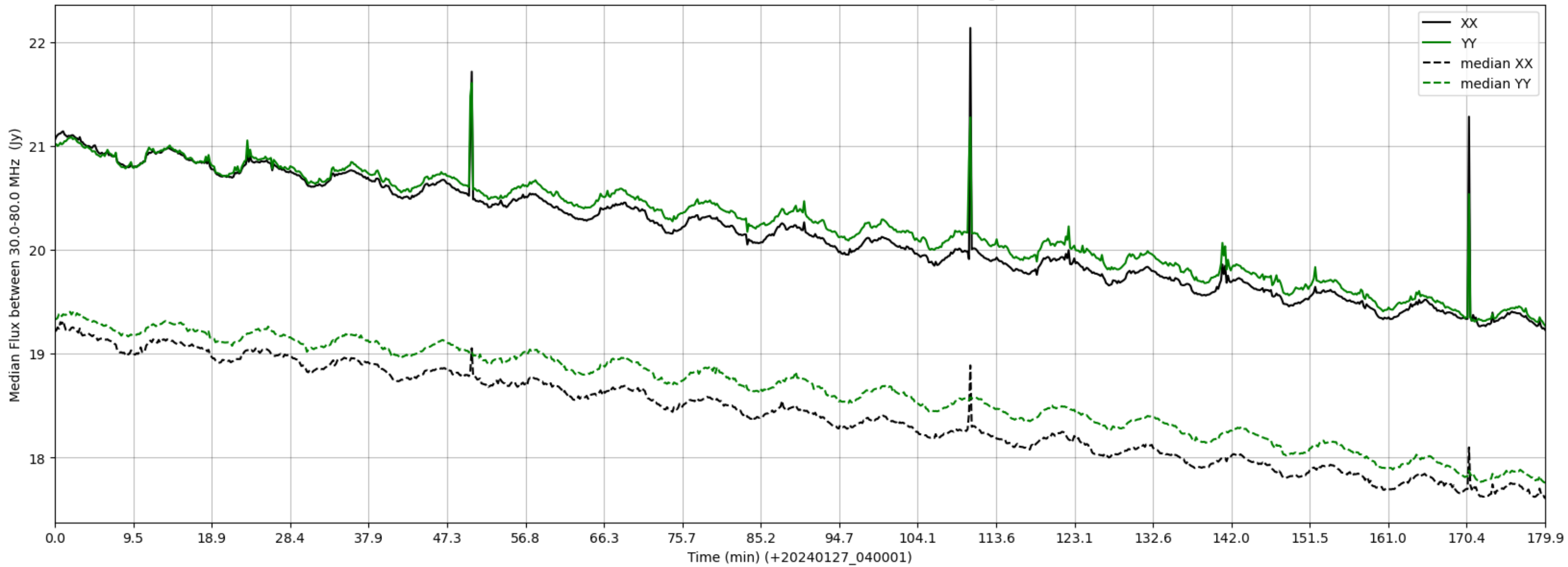
LWA253 - Correlator# 283 - XX FLAGS:Good - YY FLAGS:HighTimeVar
