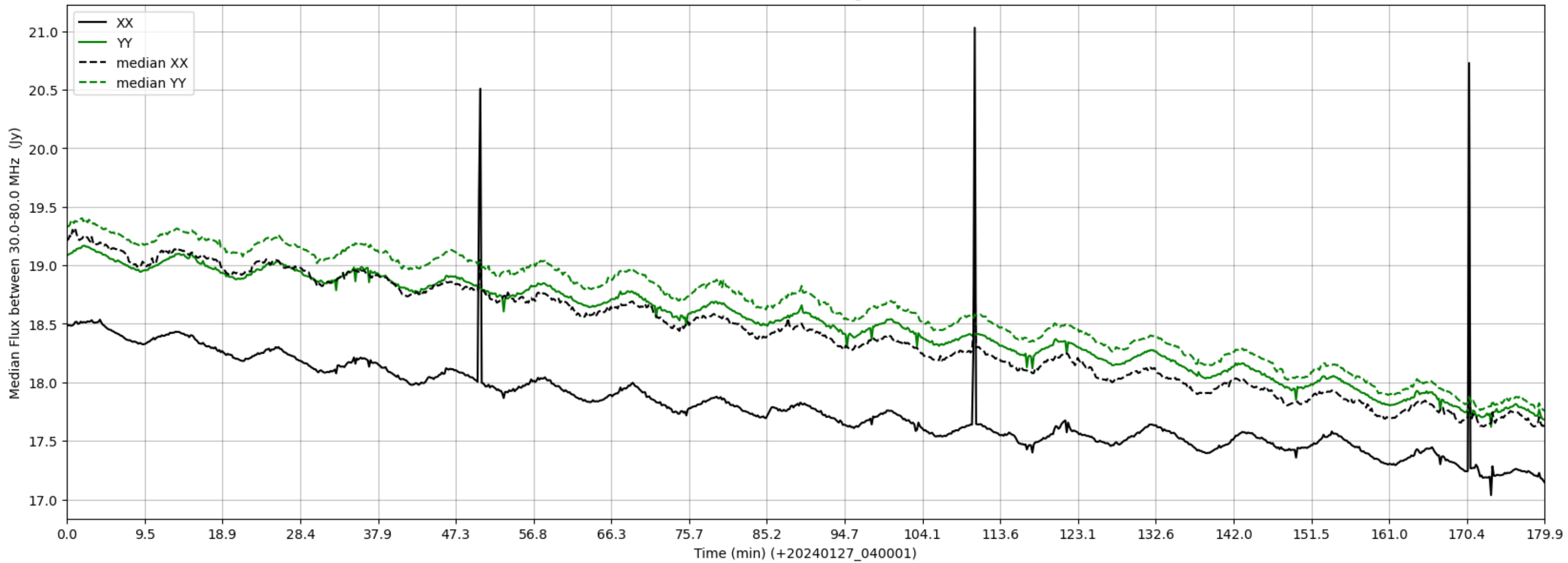
LWA077 - Correlator# 088 - XX FLAGS:HighTimeVar - YY FLAGS:Good
