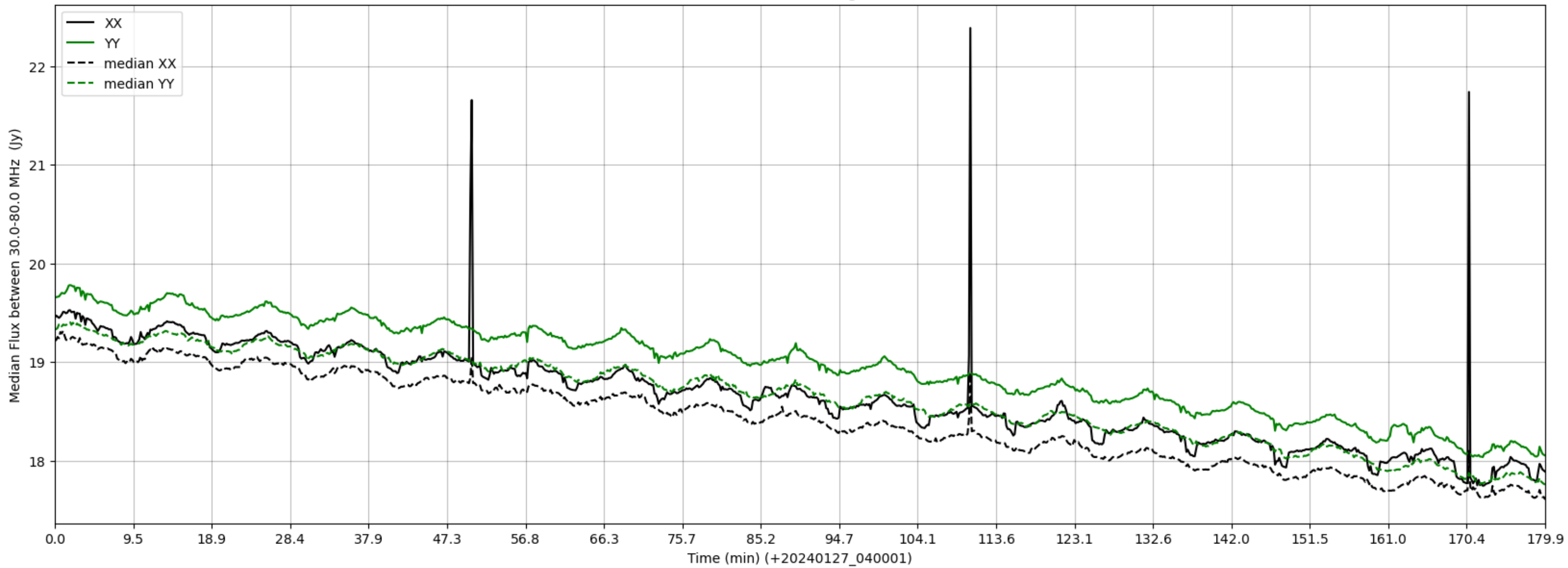
LWA098 - Correlator# 173 - XX FLAGS:HighTimeVar - YY FLAGS:Good
