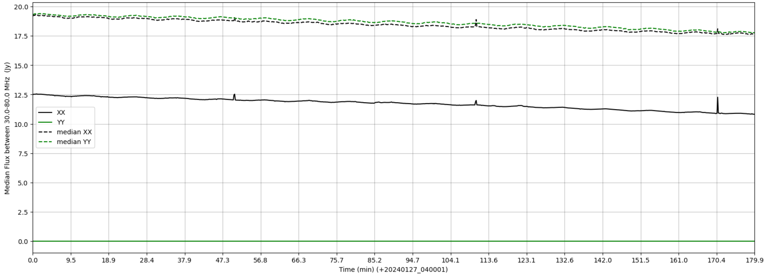
LWA292 - Correlator# 044 - XX FLAGS:Good - YY FLAGS:LowFlux
