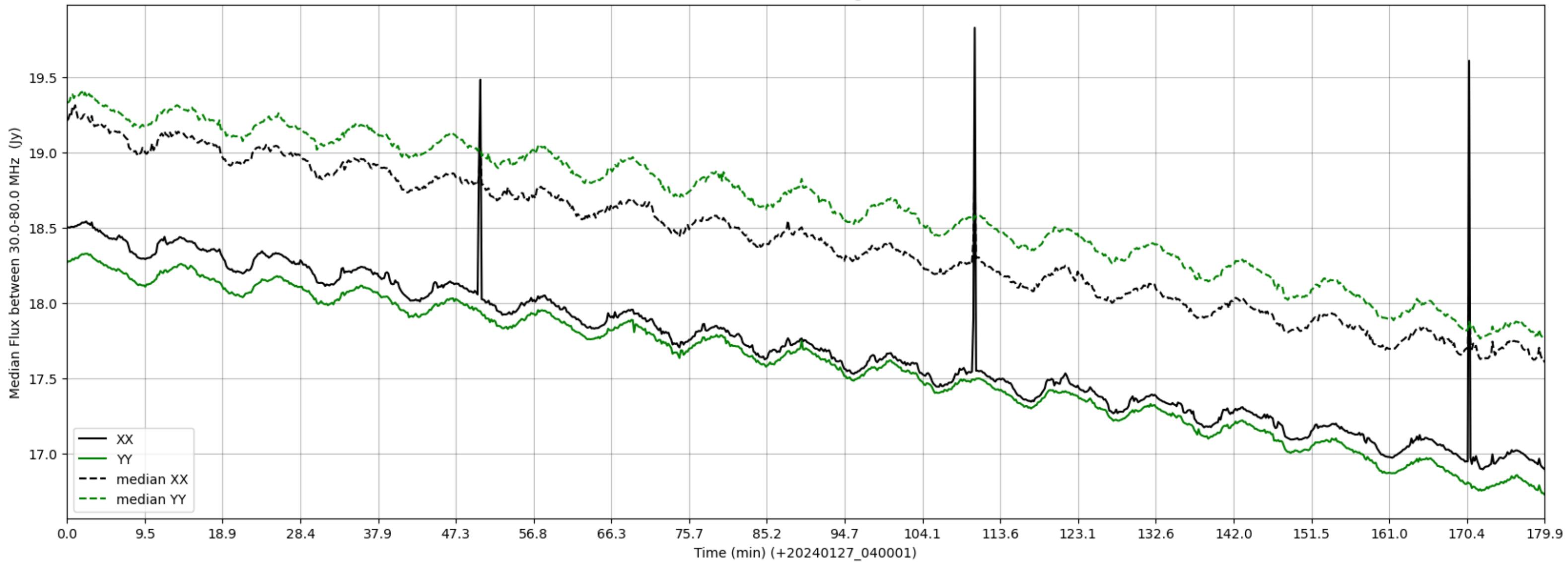
LWA170 - Correlator# 288 - XX FLAGS:HighTimeVar - YY FLAGS:Good
