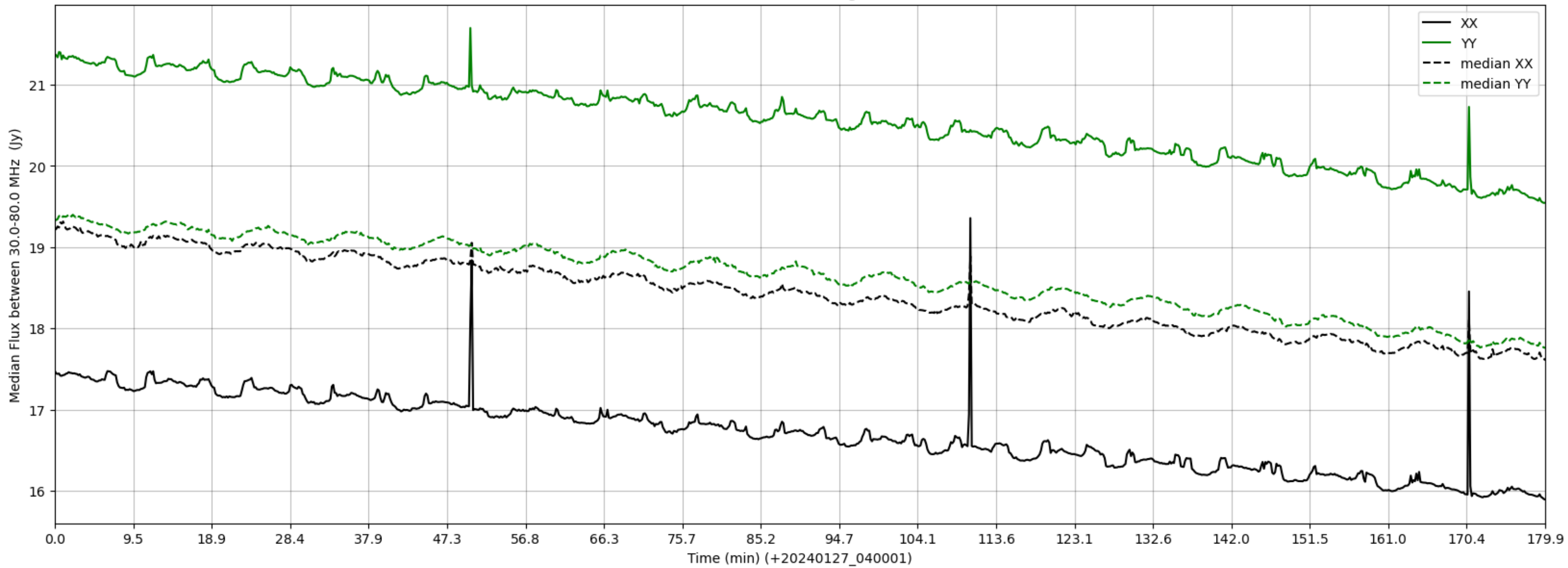
LWA206 - Correlator# 296 - XX FLAGS:HighTimeVar - YY FLAGS:Good
