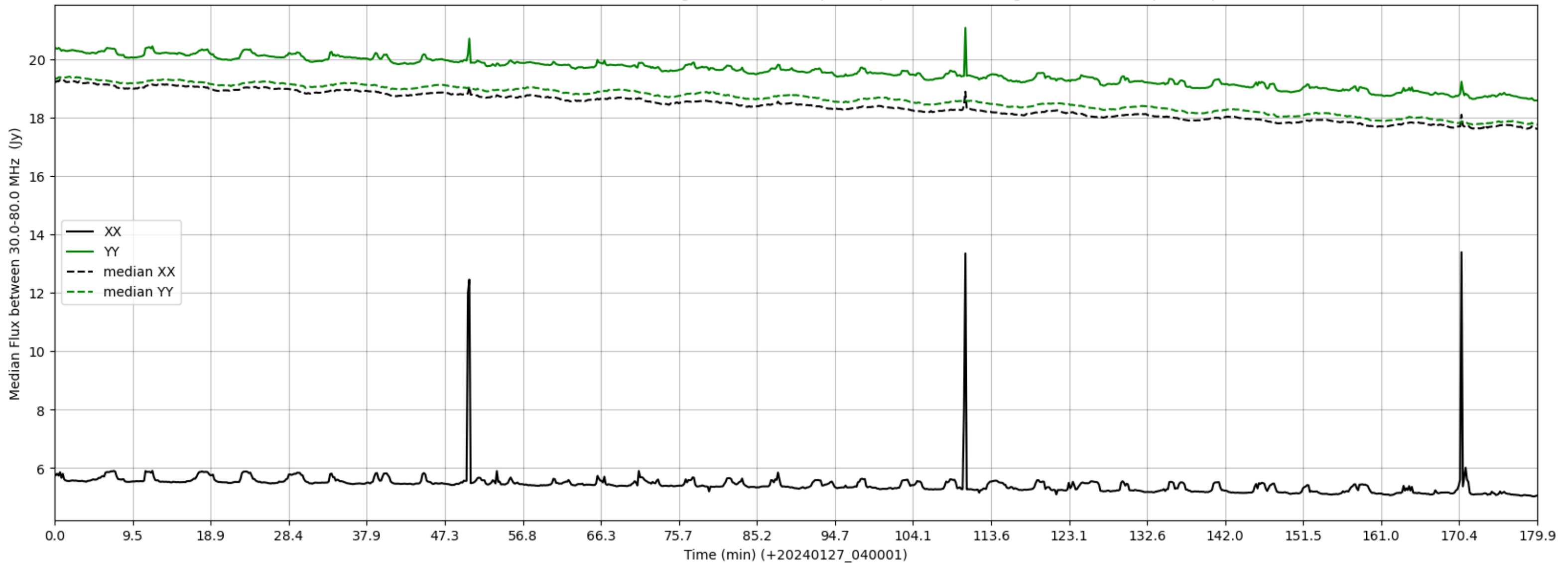
LWA232 - Correlator# 307 - XX FLAGS:HighTimeVar+BadSpecShape - YY FLAGS:HighTimeVar+BadSpecShape
