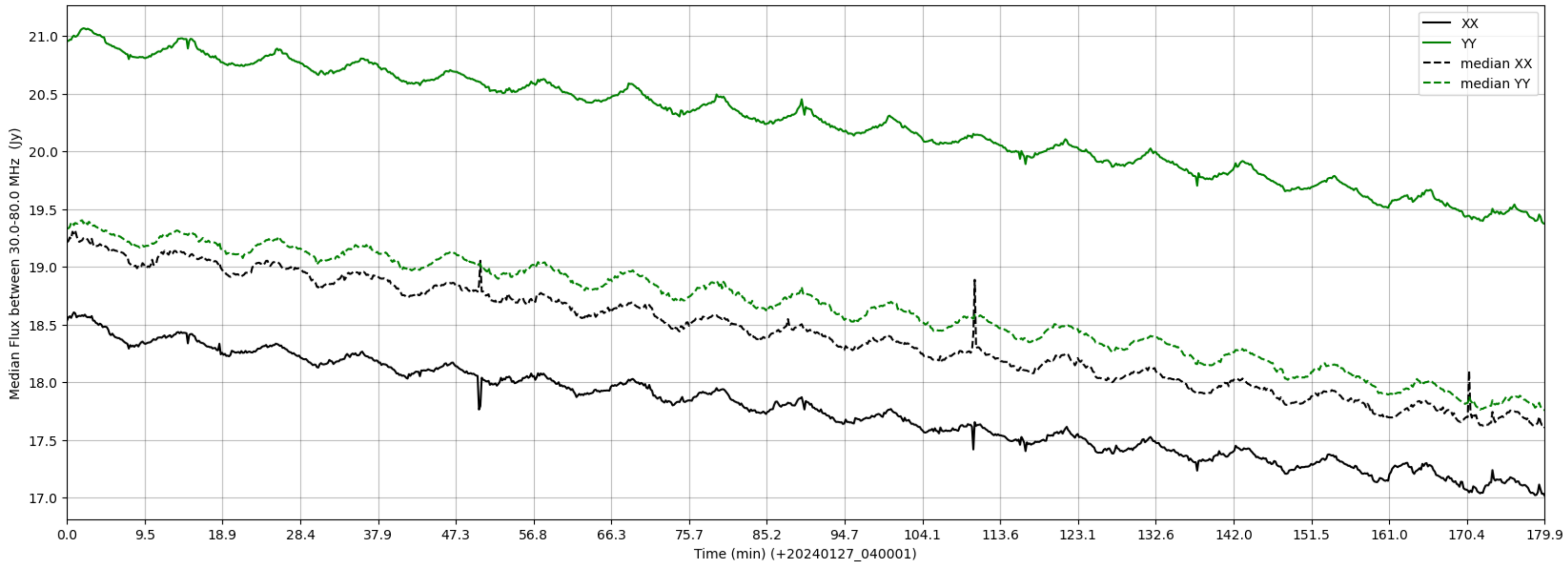
LWA110 - Correlator# 198 - XX FLAGS:Good - YY FLAGS:Good
