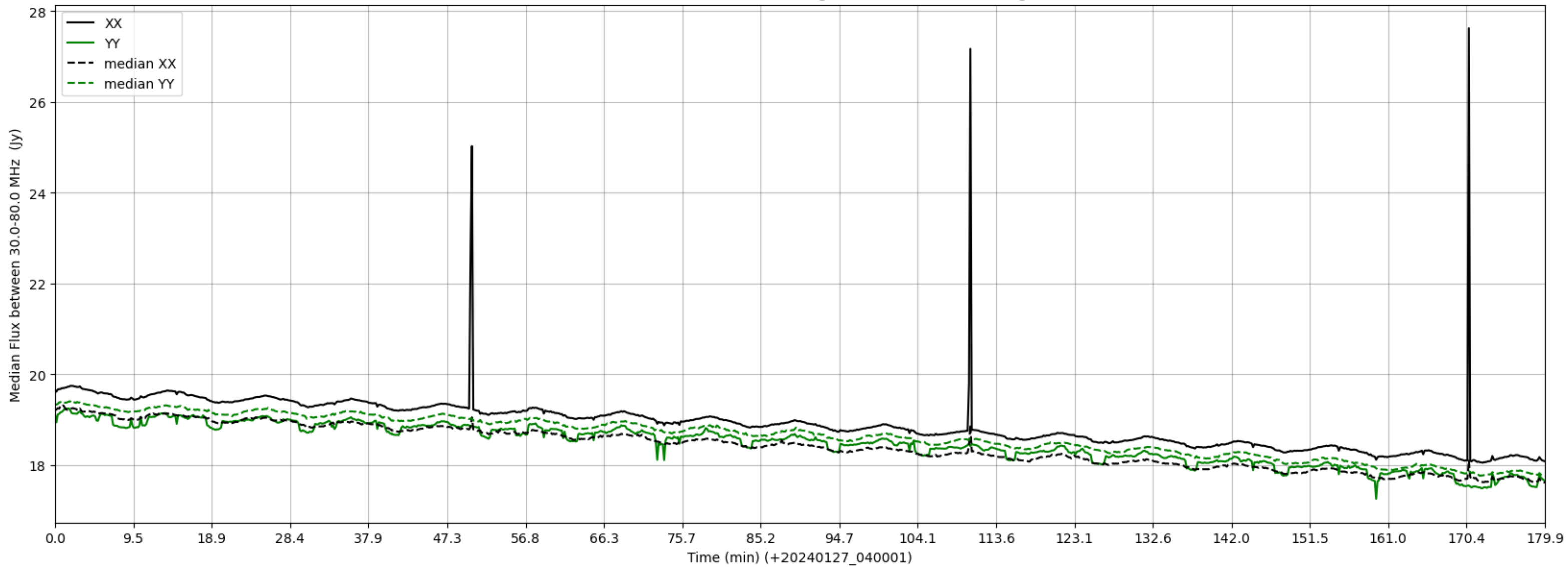
LWA034 - Correlator# 162 - XX FLAGS:HighTimeVar - YY FLAGS:HighTimeVar
