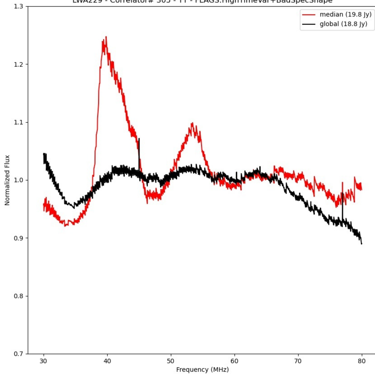
LWA229 - Correlator# 305 - YY - FLAGS:HighTimeVar+BadSpecShape
