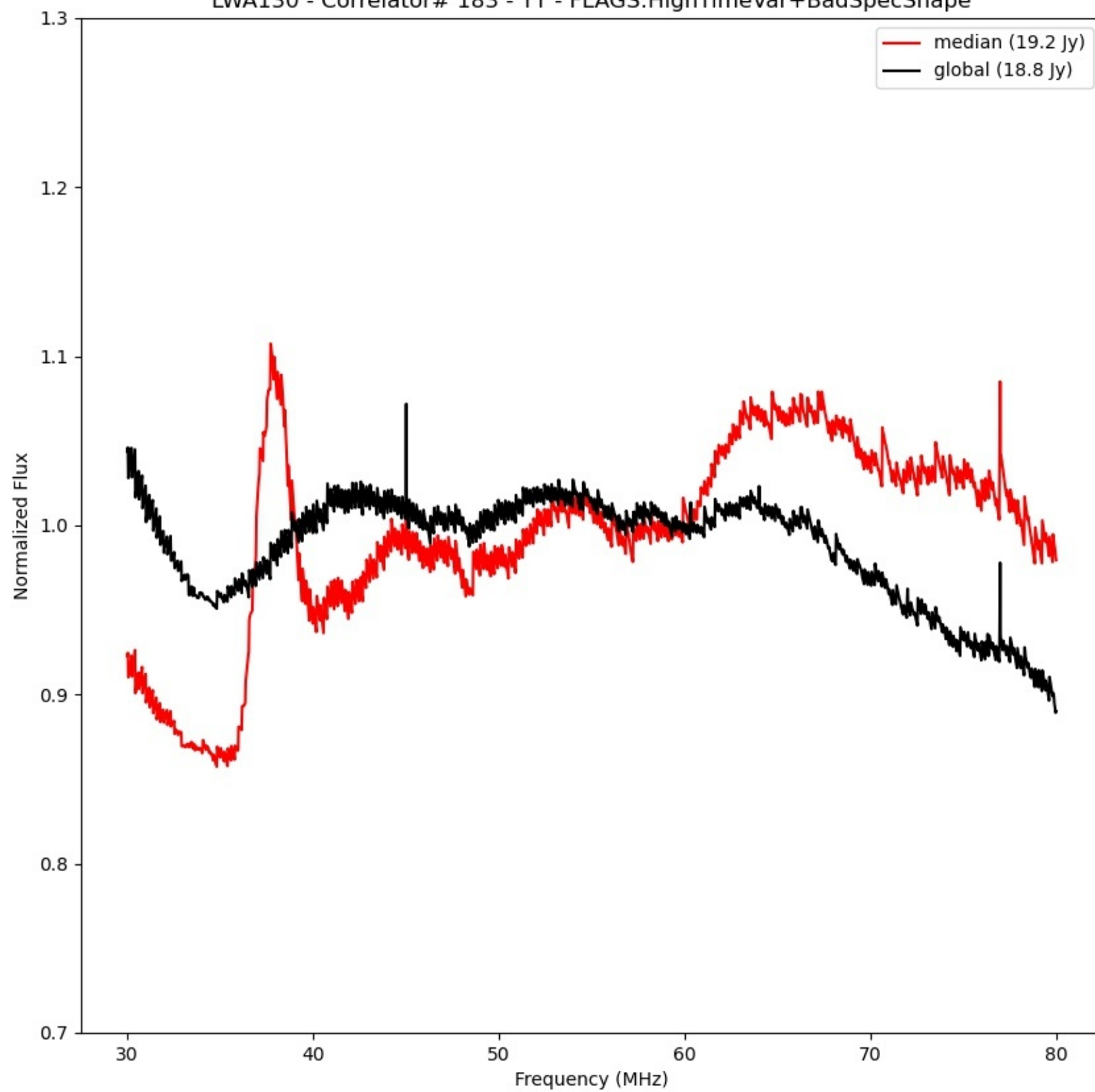
LWA130 - Correlator# 183 - YY - FLAGS:HighTimeVar+BadSpecShape
