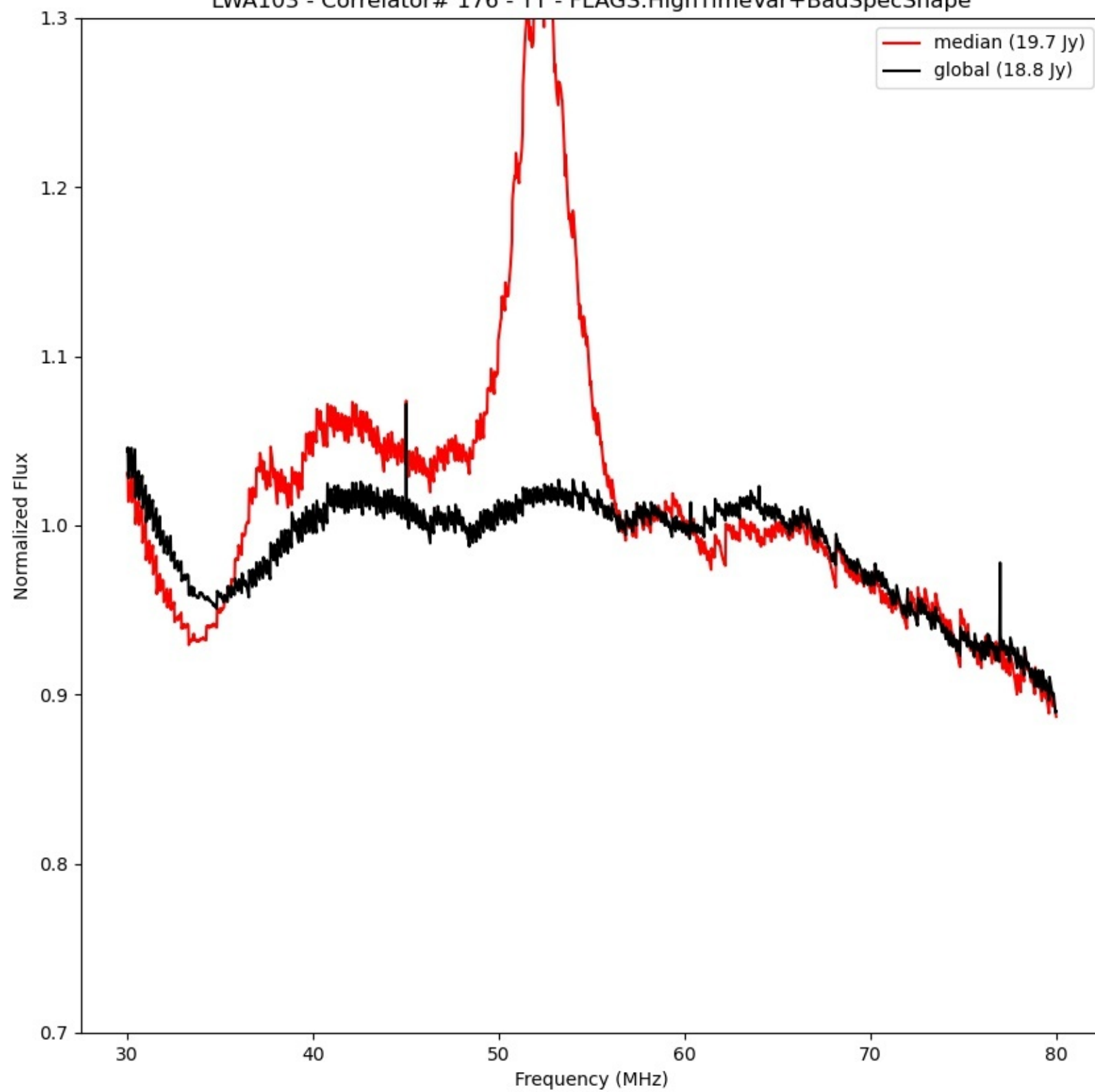
LWA103 - Correlator# 176 - YY - FLAGS:HighTimeVar+BadSpecShape
