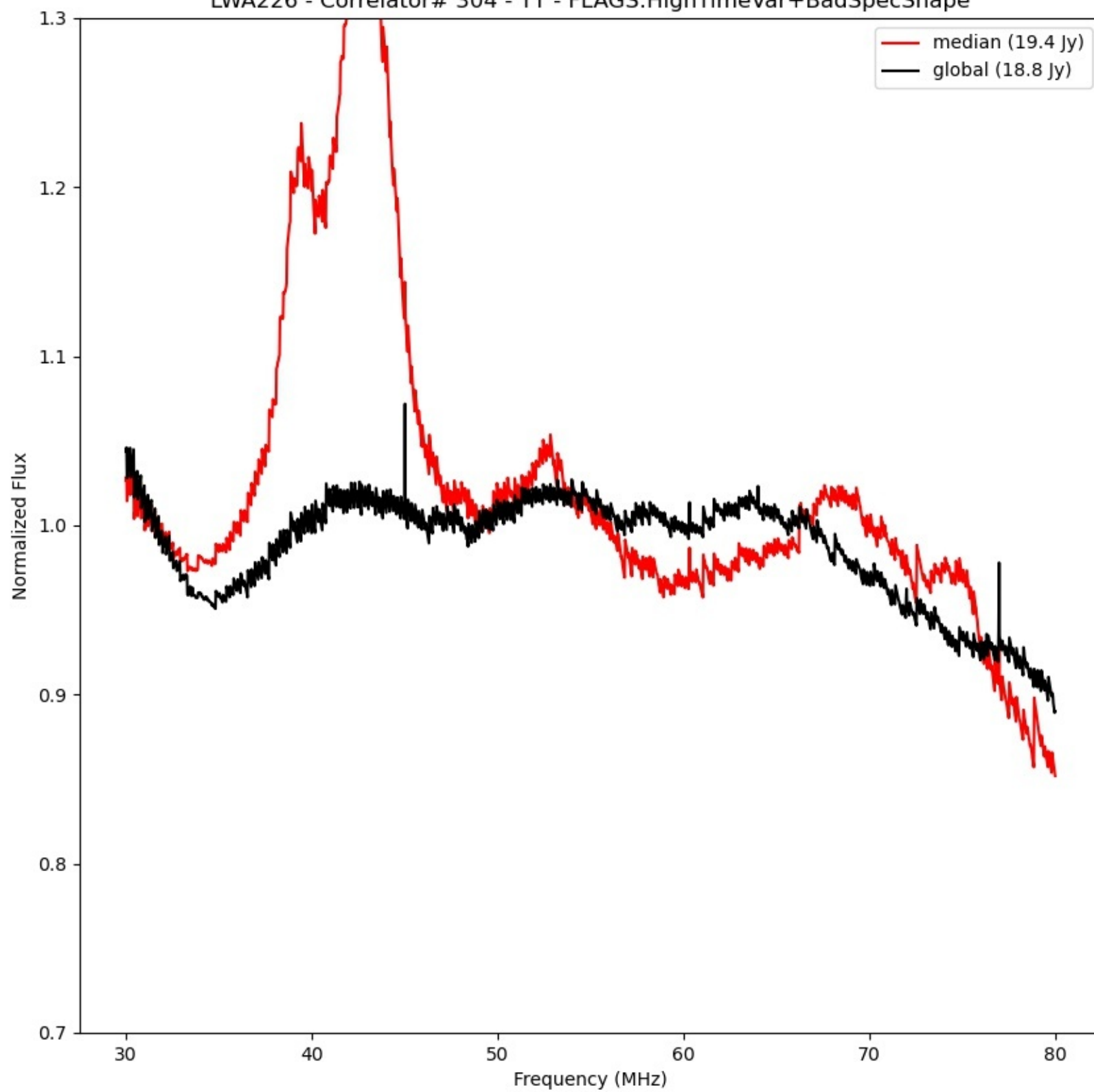
LWA226 - Correlator# 304 - YY - FLAGS:HighTimeVar+BadSpecShape
