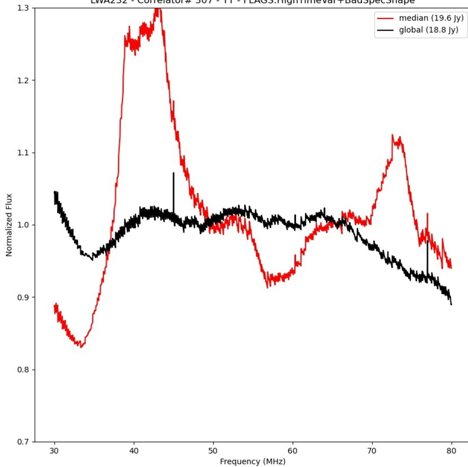
LWA232 - Correlator# 307 - YY - FLAGS:HighTimeVar+BadSpecShape
