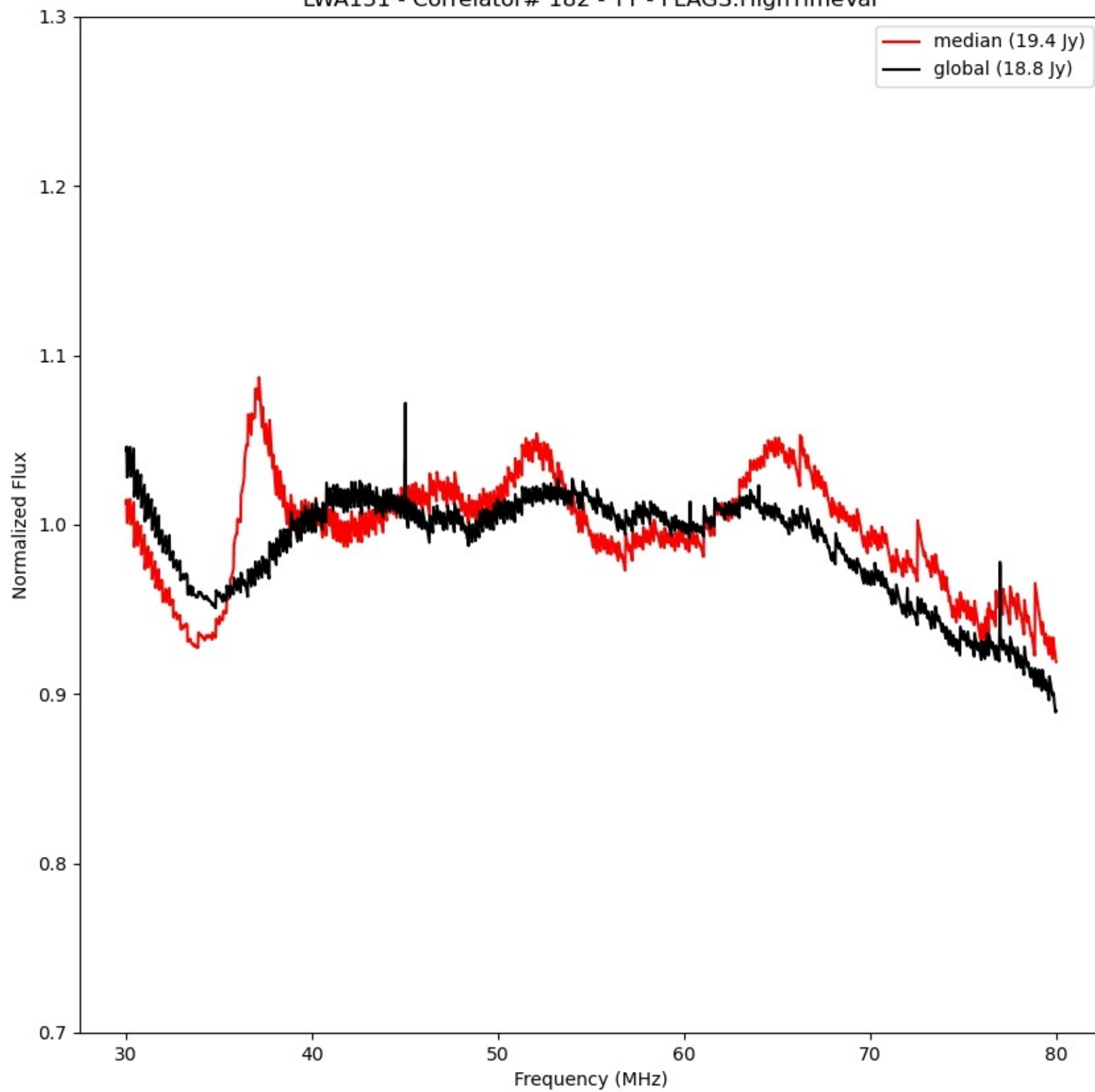
LWA131 - Correlator# 182 - YY - FLAGS:HighTimeVar
