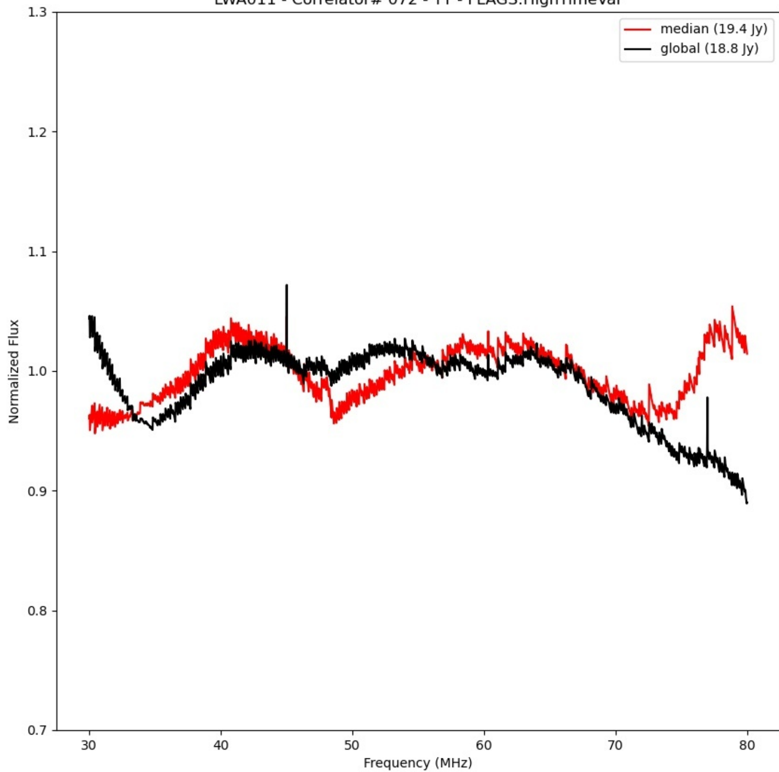
LWA011 - Correlator# 072 - YY - FLAGS:HighTimeVar
