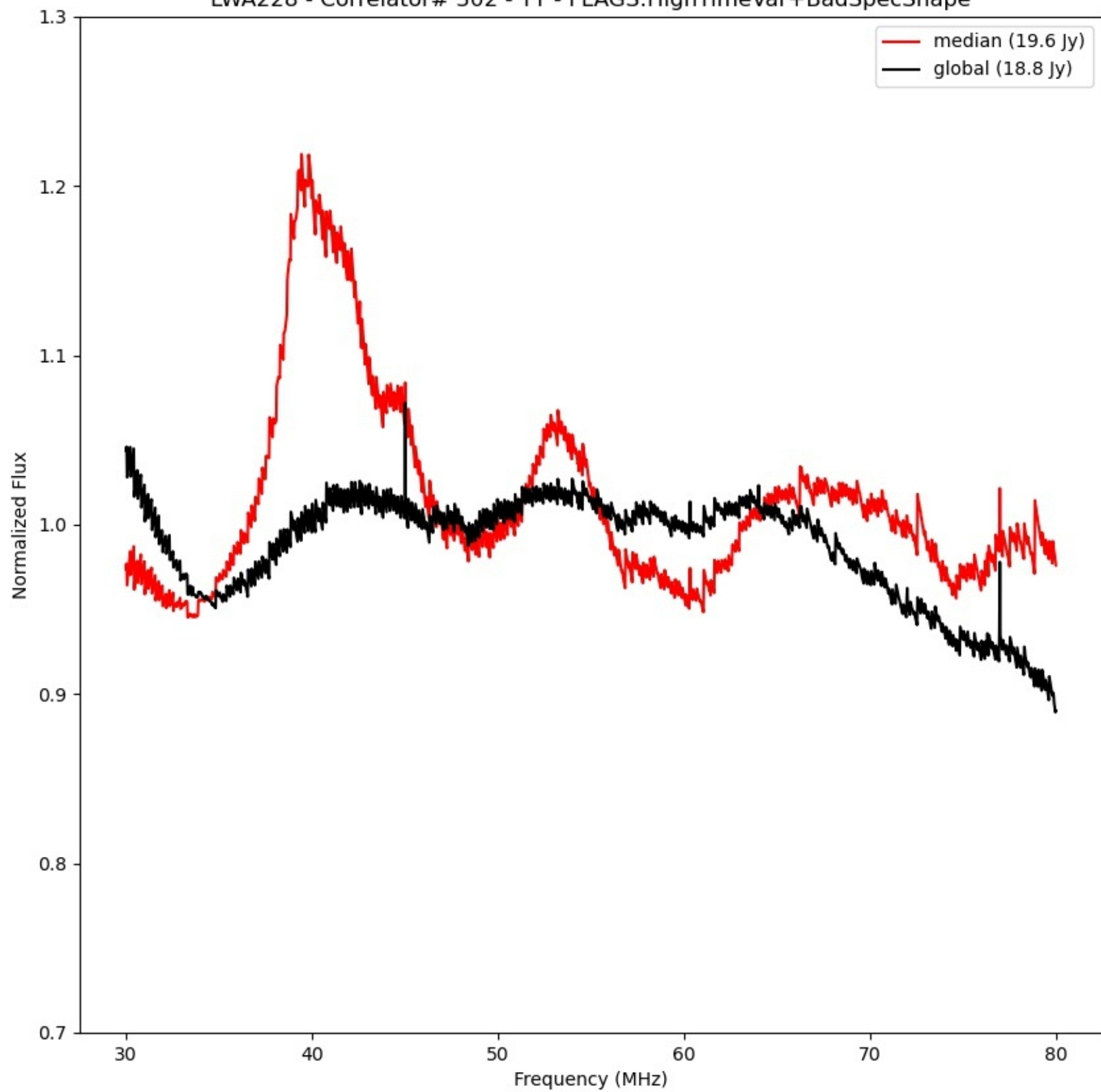
LWA228 - Correlator# 302 - YY - FLAGS:HighTimeVar+BadSpecShape
