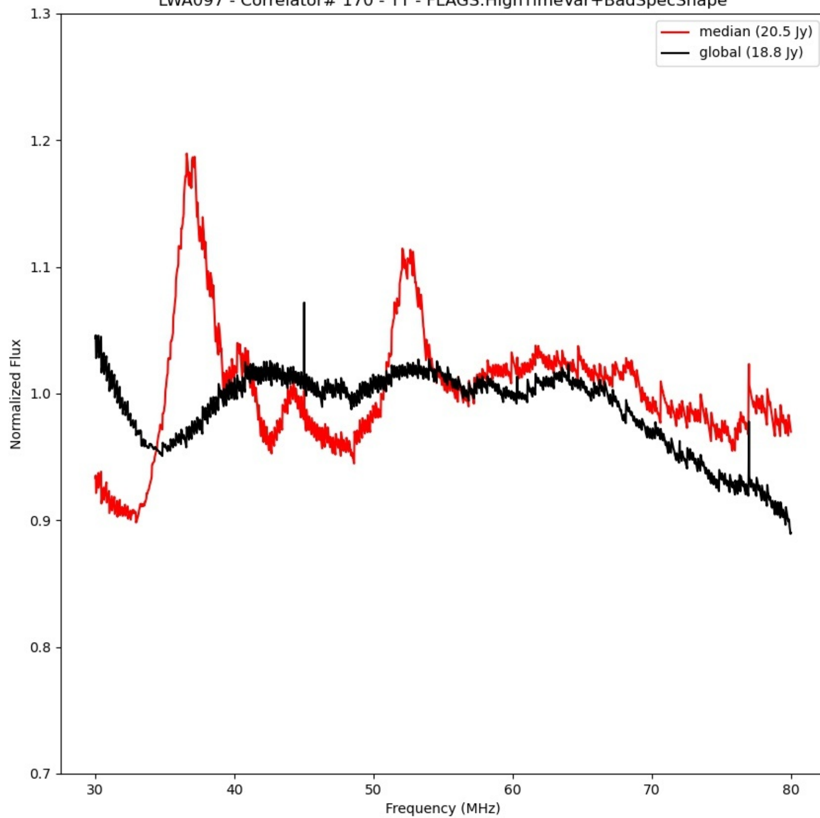
LWA097 - Correlator# 170 - YY - FLAGS:HighTimeVar+BadSpecShape
