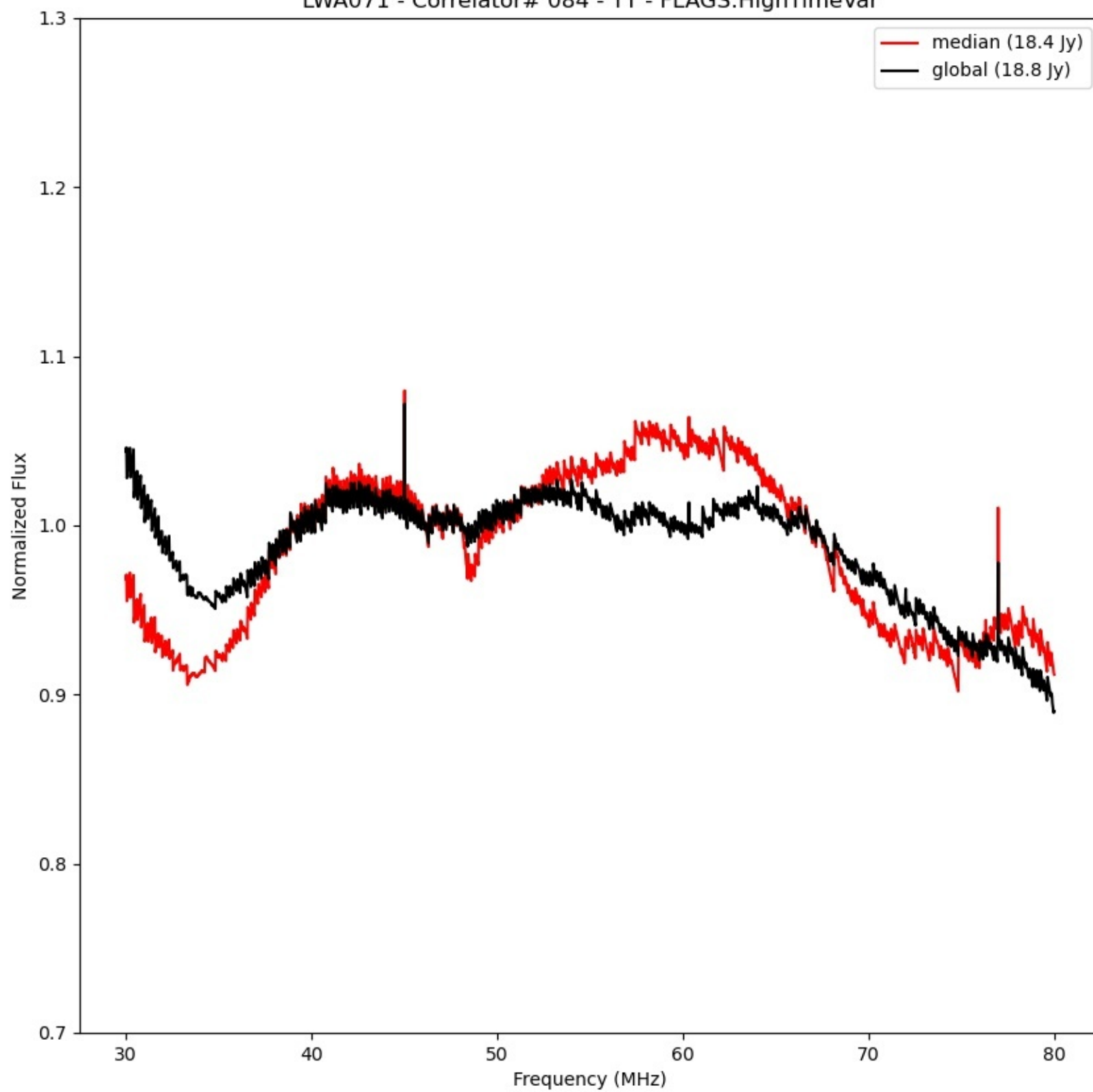
LWA071 - Correlator# 084 - YY - FLAGS:HighTimeVar
