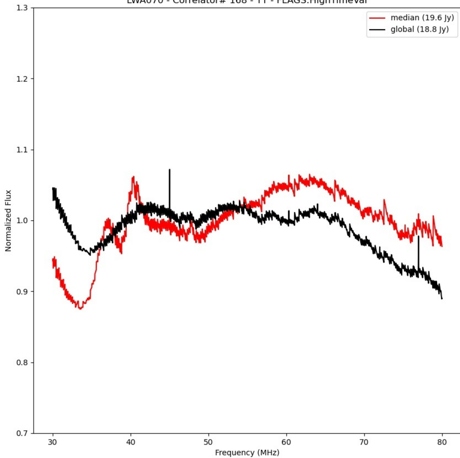
LWA070 - Correlator# 168 - YY - FLAGS:HighTimeVar
