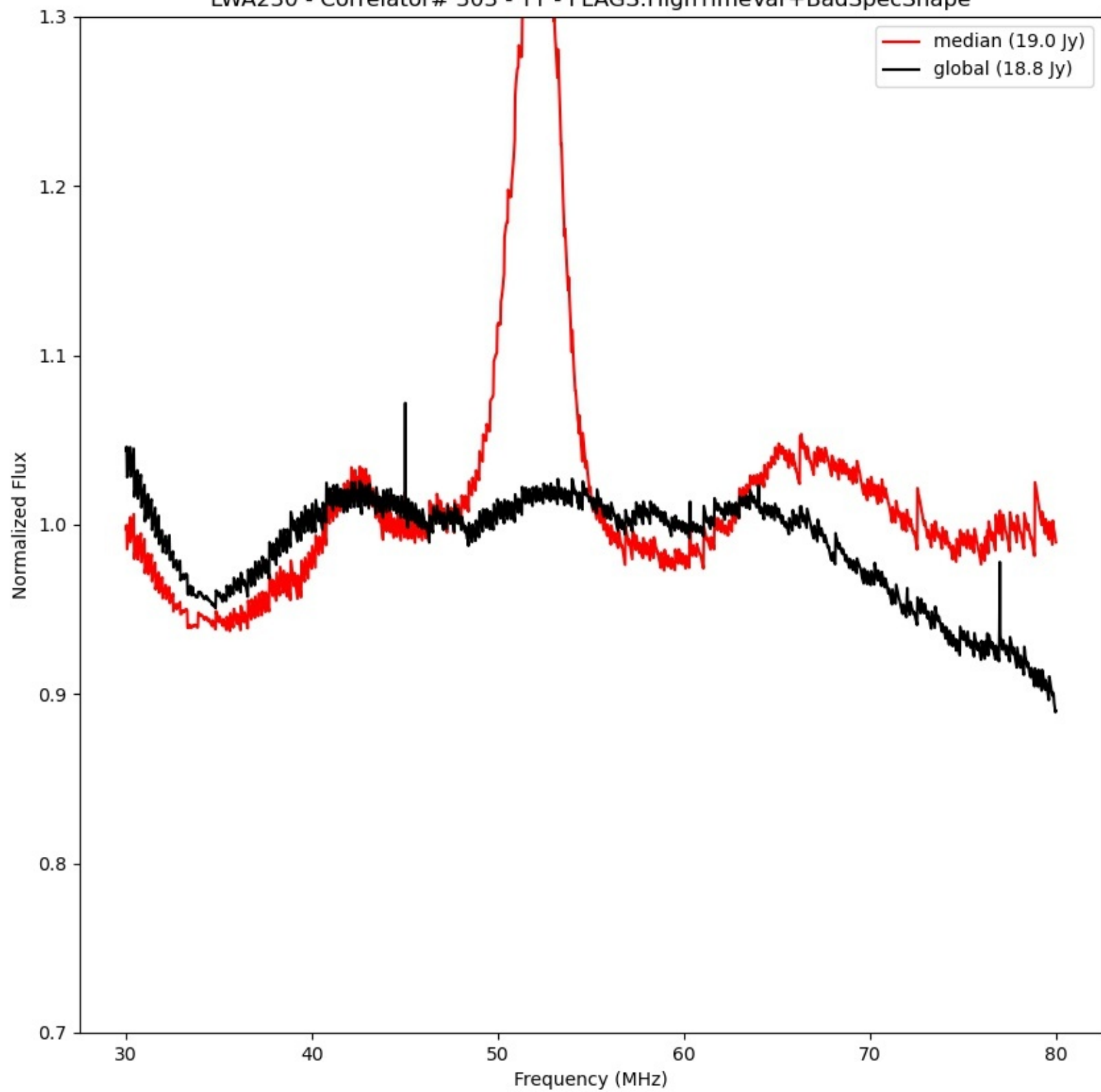
LWA230 - Correlator# 303 - YY - FLAGS:HighTimeVar+BadSpecShape
