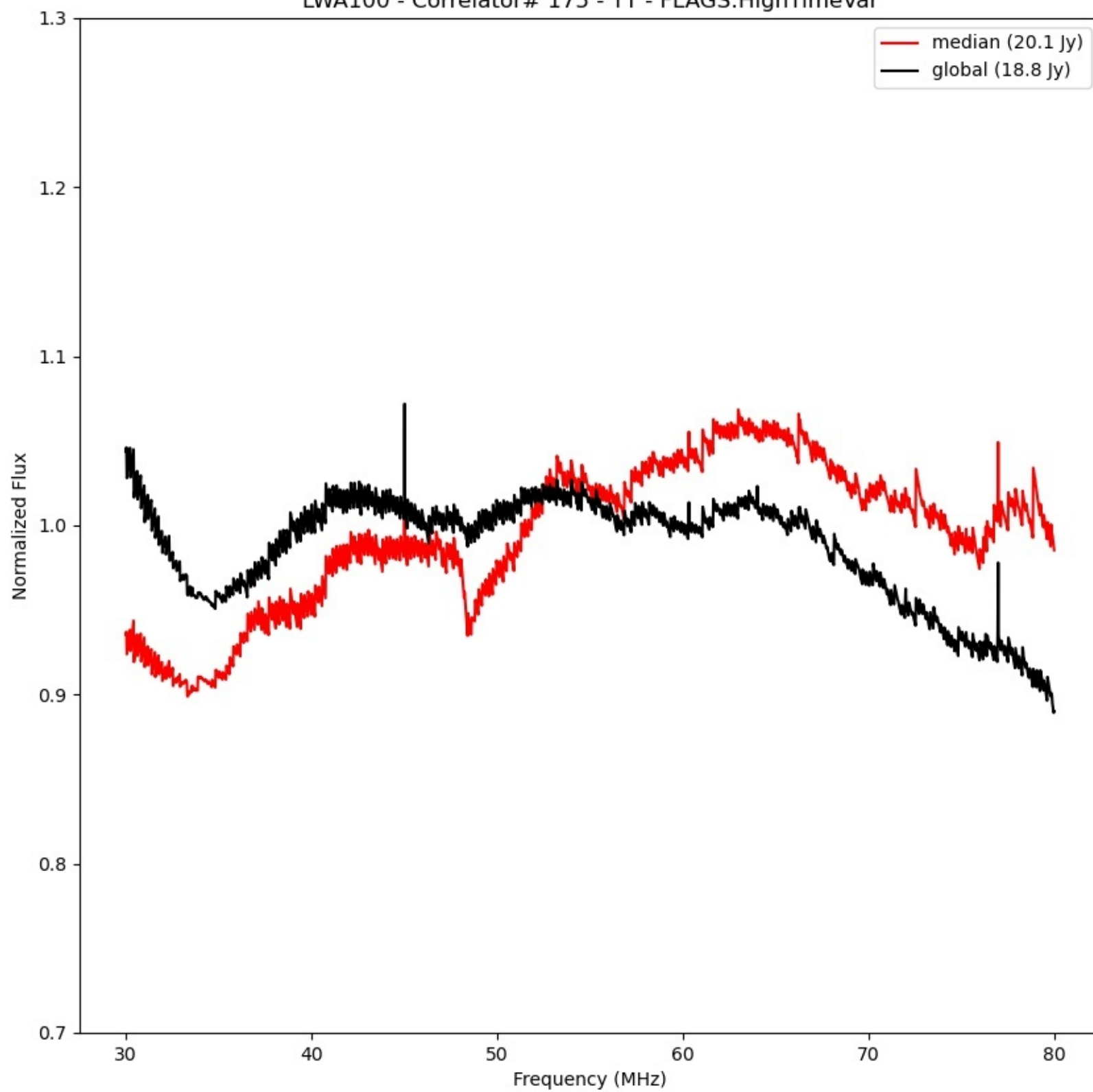
LWA100 - Correlator# 175 - YY - FLAGS:HighTimeVar
