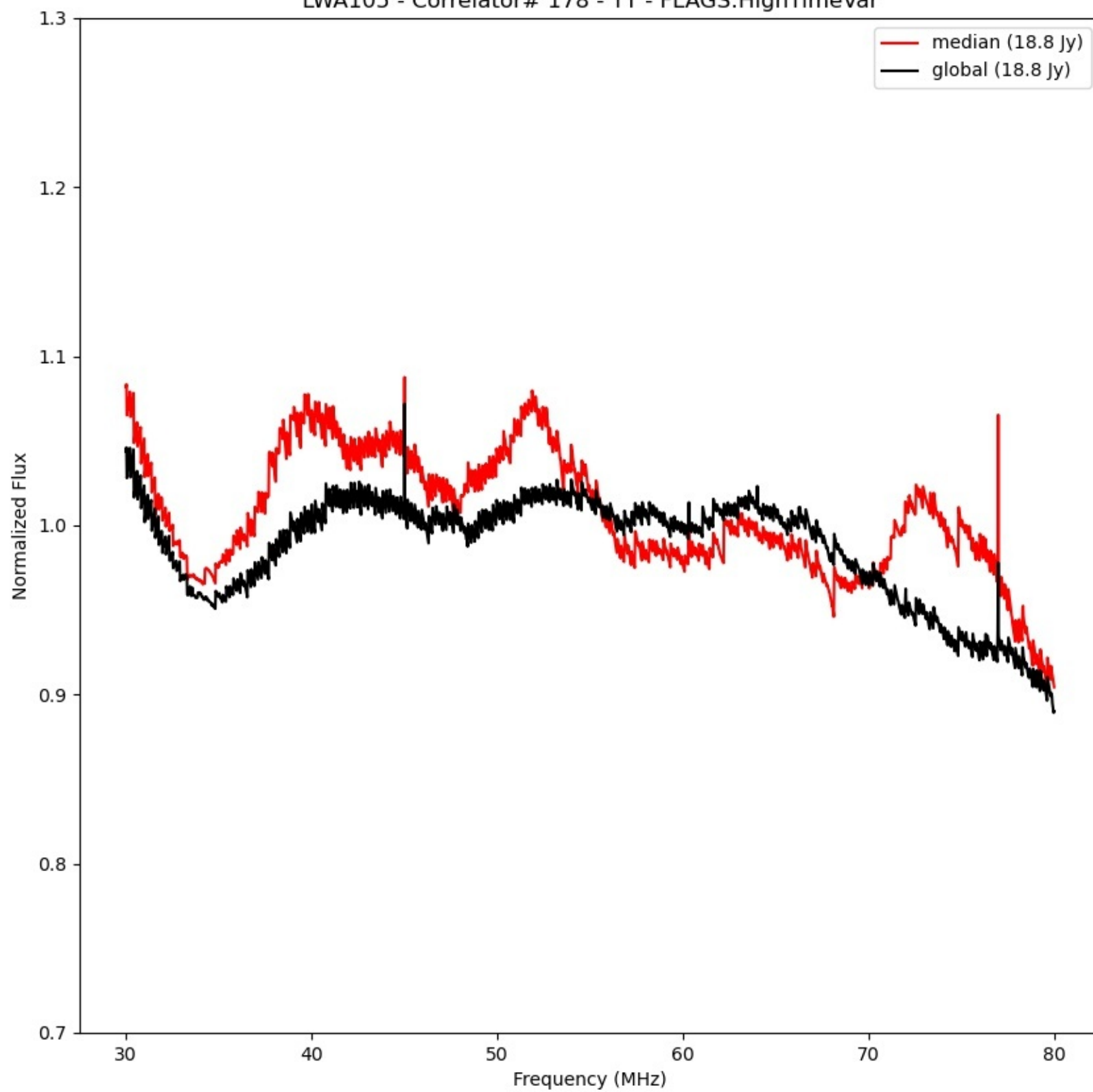
LWA105 - Correlator# 178 - YY - FLAGS:HighTimeVar
