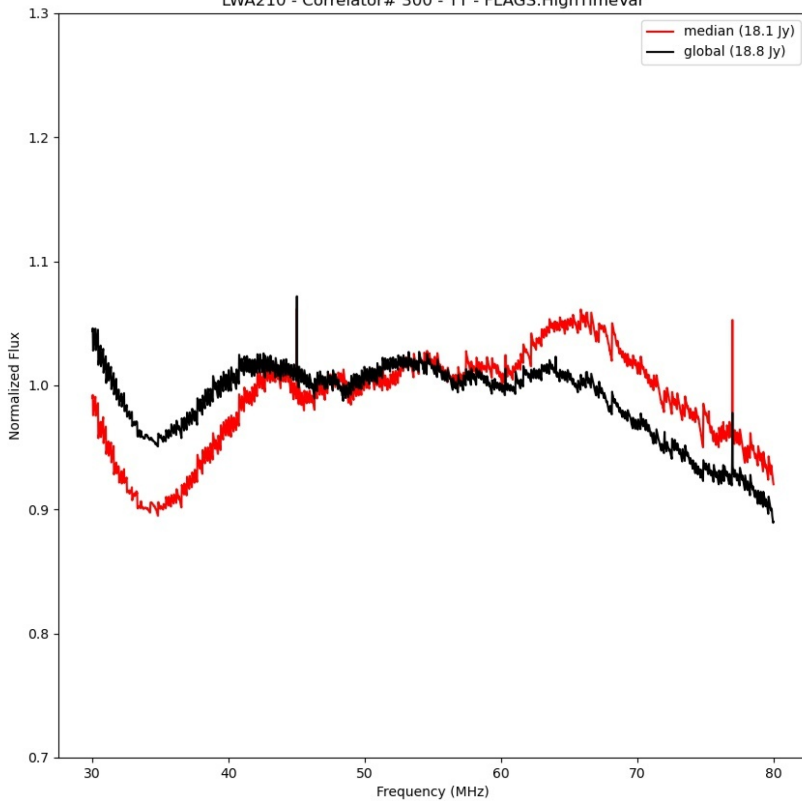
LWA210 - Correlator# 300 - YY - FLAGS:HighTimeVar
