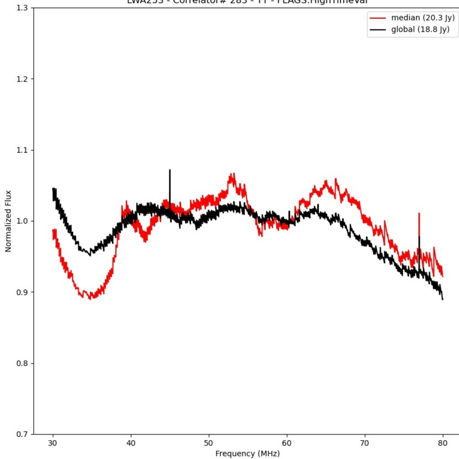
LWA253 - Correlator# 283 - YY - FLAGS:HighTimeVar
