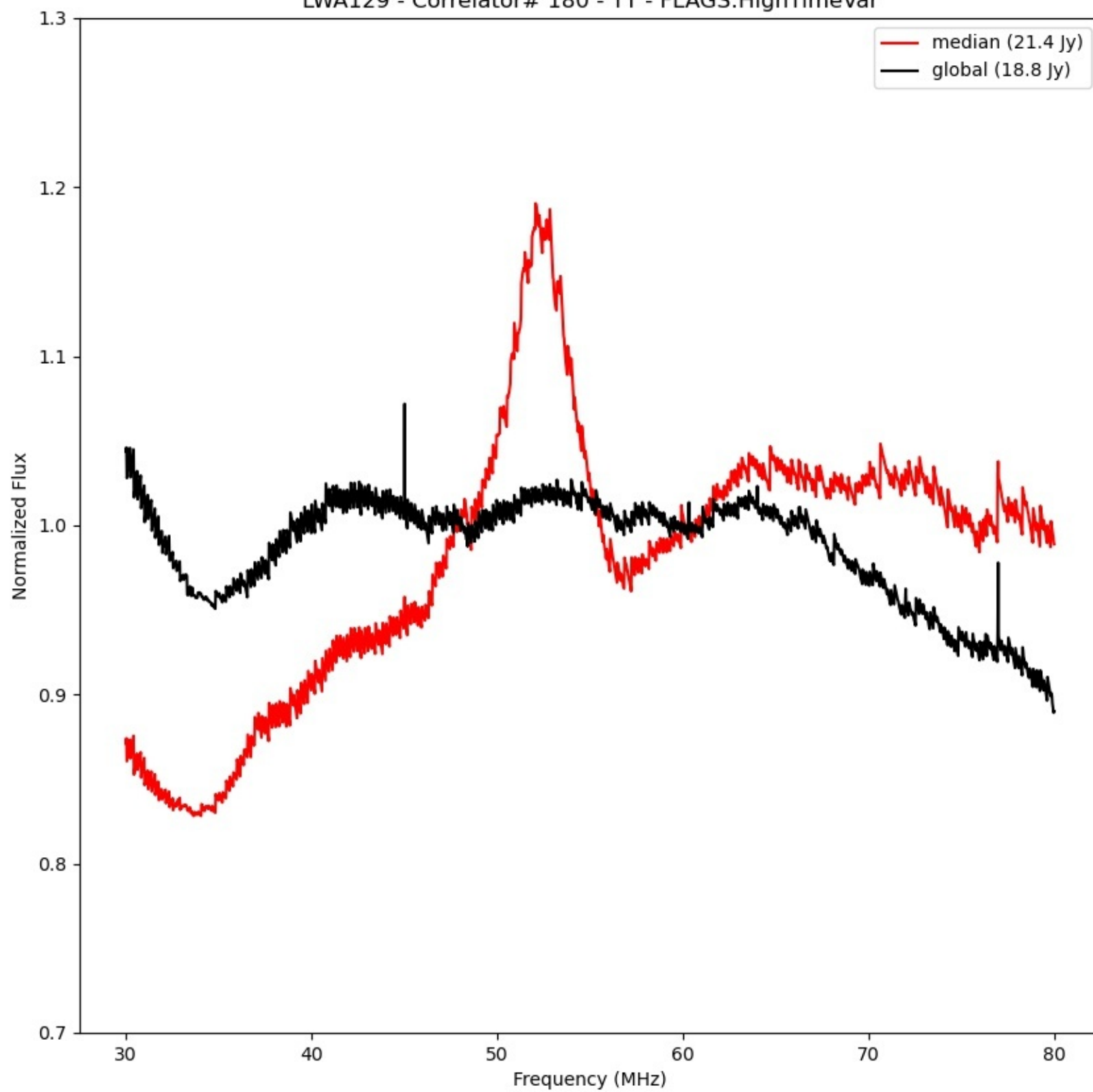
LWA129 - Correlator# 180 - YY - FLAGS:HighTimeVar
