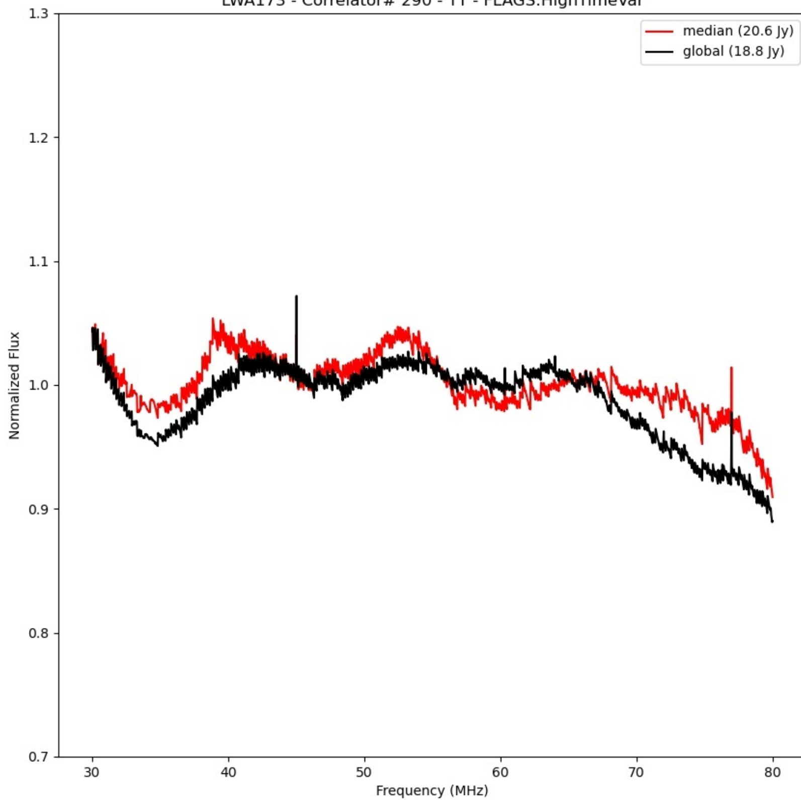
LWA173 - Correlator# 290 - YY - FLAGS:HighTimeVar
