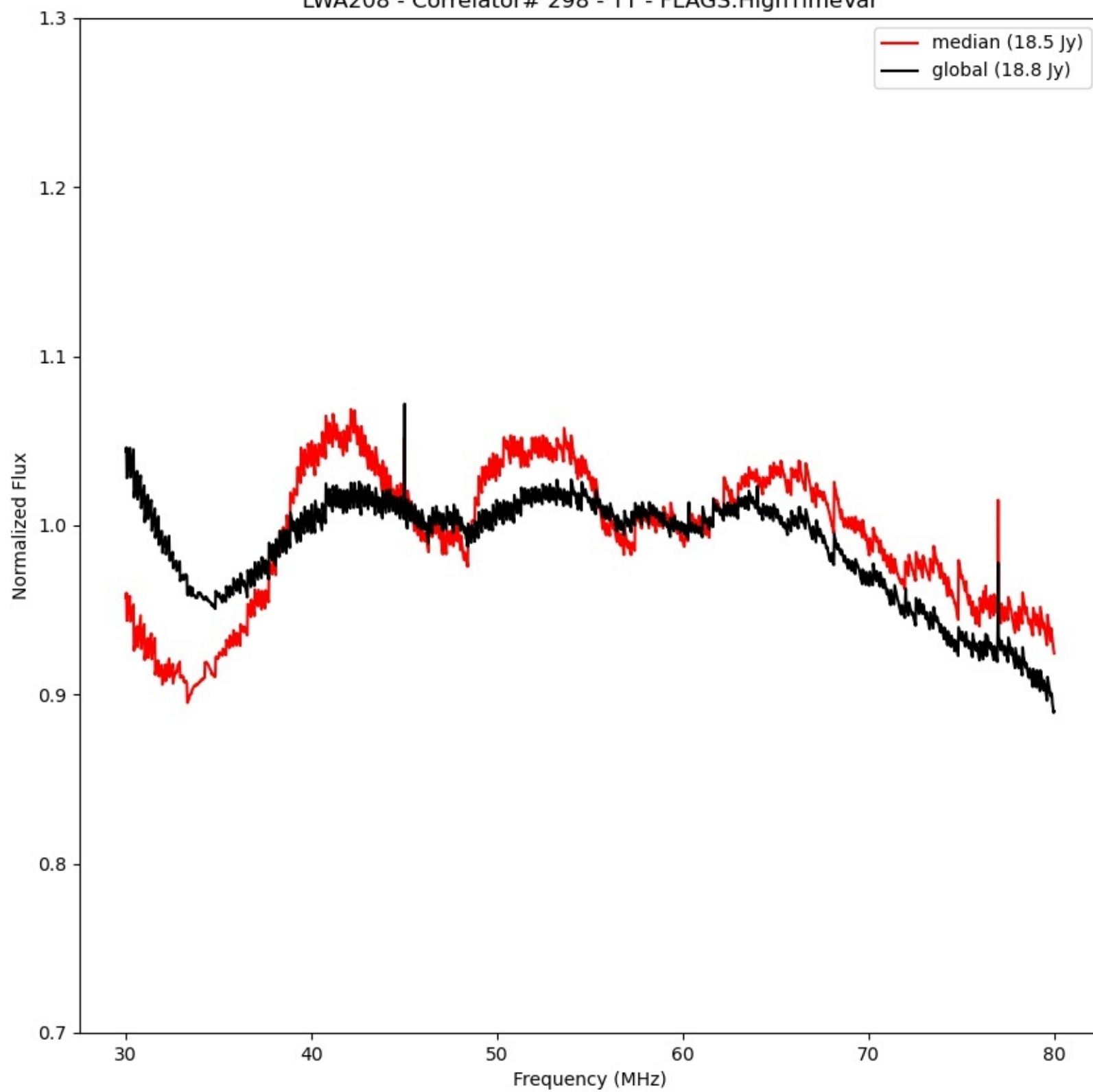
LWA208 - Correlator# 298 - YY - FLAGS:HighTimeVar
