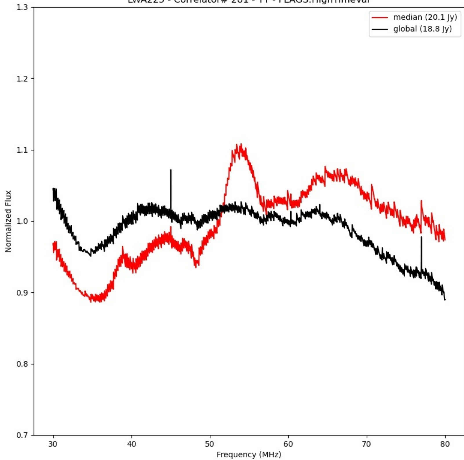
LWA225 - Correlator# 281 - YY - FLAGS:HighTimeVar
