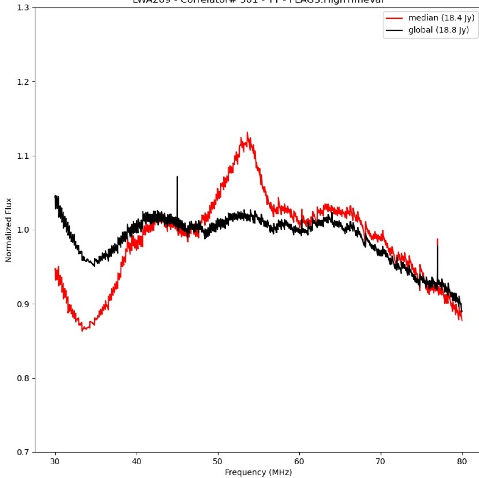
LWA209 - Correlator# 301 - YY - FLAGS:HighTimeVar
