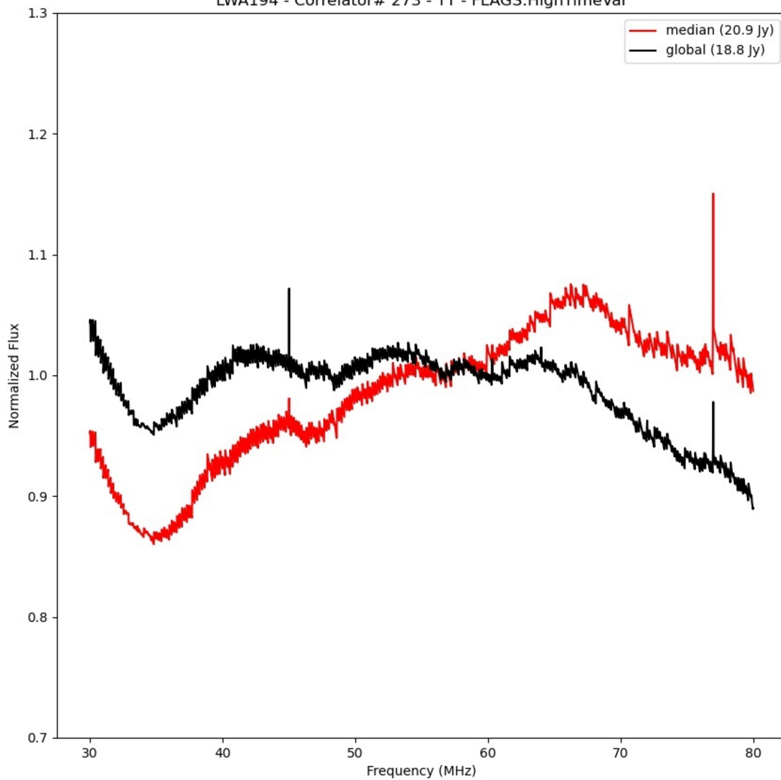
LWA194 - Correlator# 273 - YY - FLAGS:HighTimeVar
