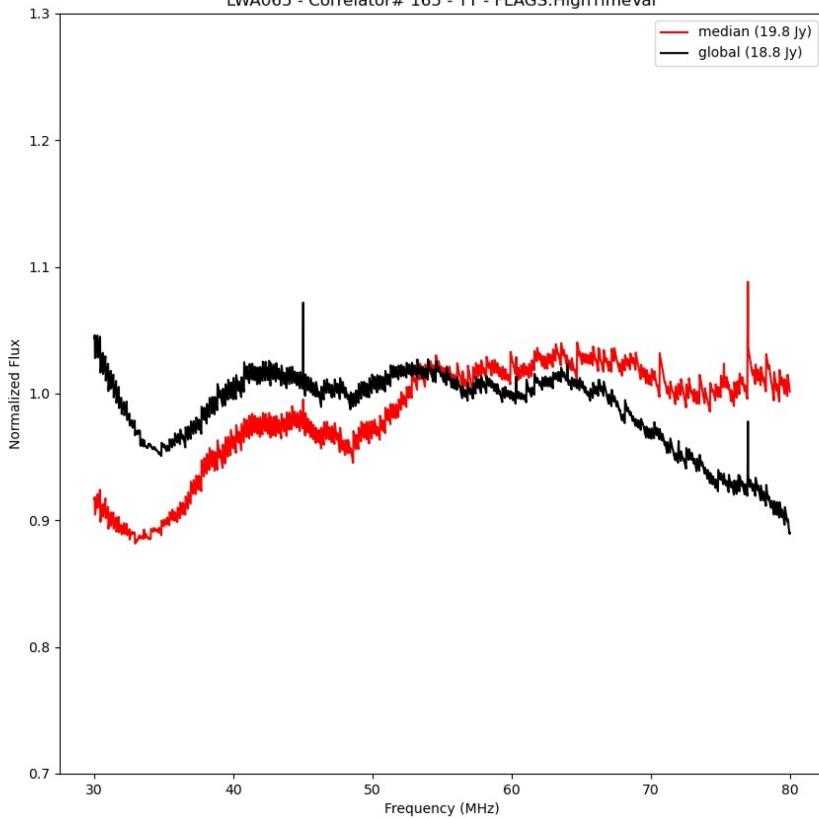
LWA065 - Correlator# 165 - YY - FLAGS:HighTimeVar
