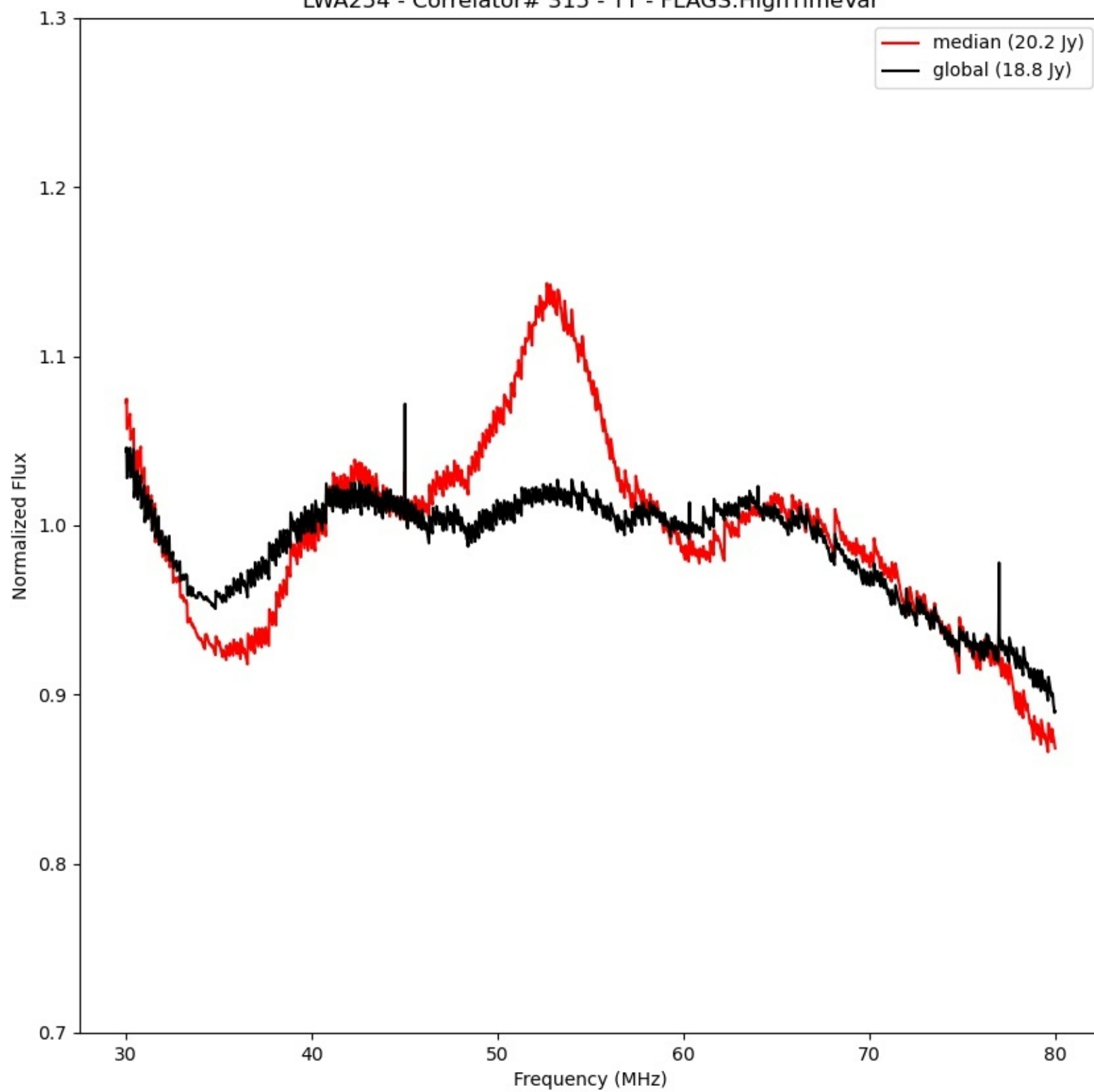
LWA254 - Correlator# 315 - YY - FLAGS:HighTimeVar
