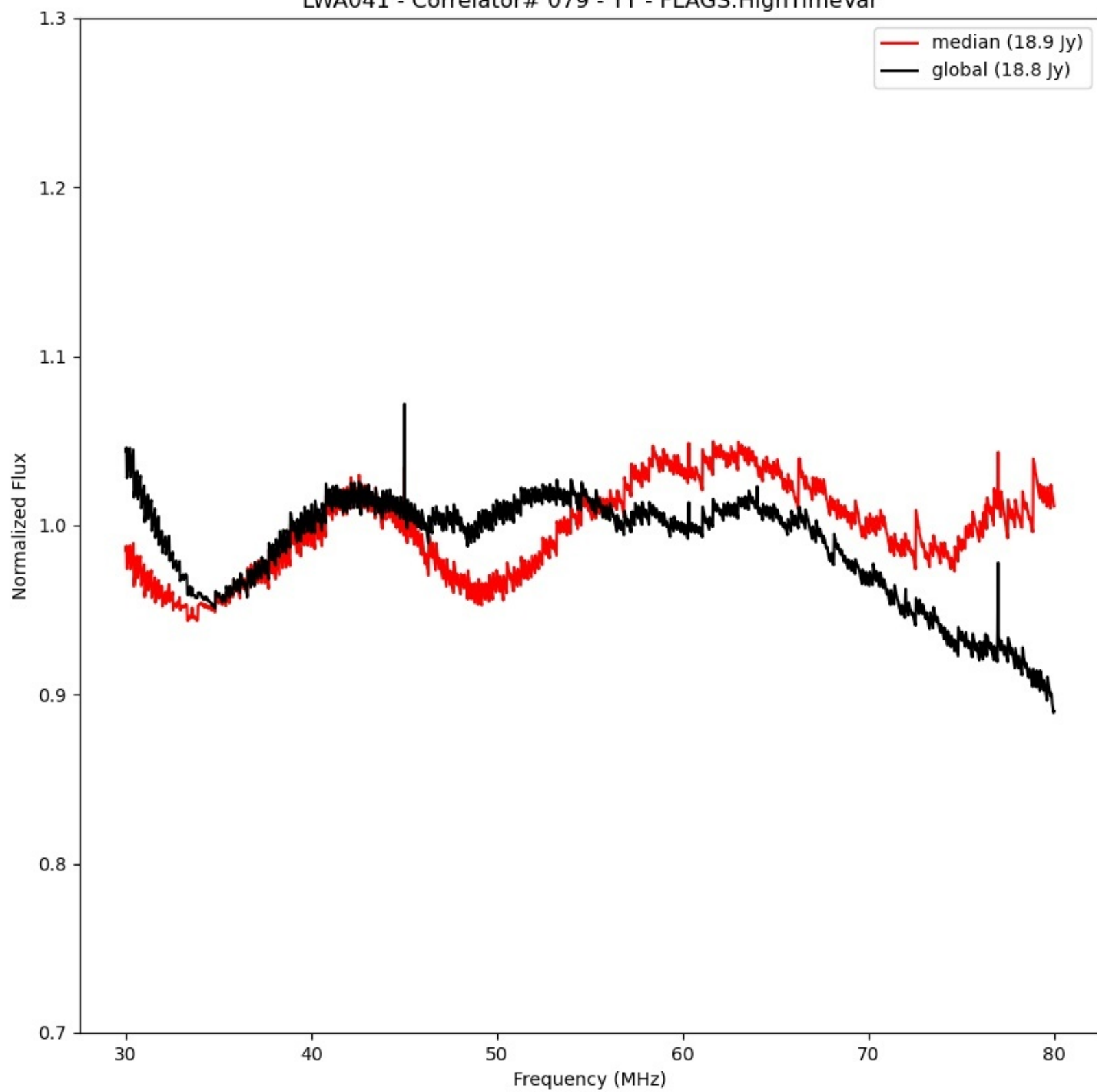
LWA041 - Correlator# 079 - YY - FLAGS:HighTimeVar
