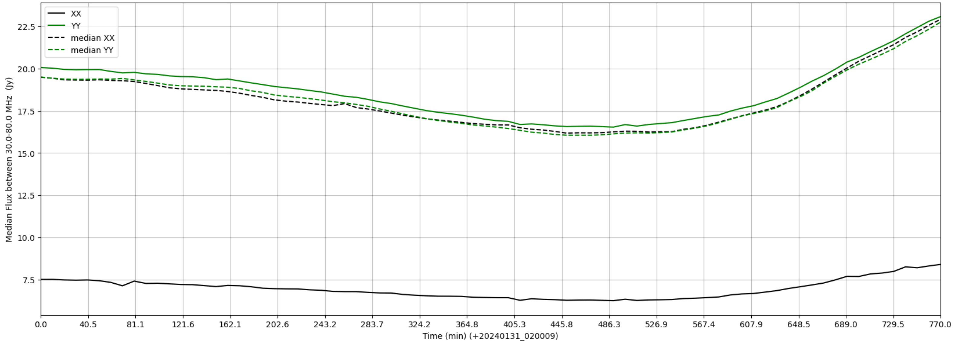
LWA130 - Correlator# 183 - XX FLAGS:BadSpecShape - YY FLAGS:BadSpecShape
