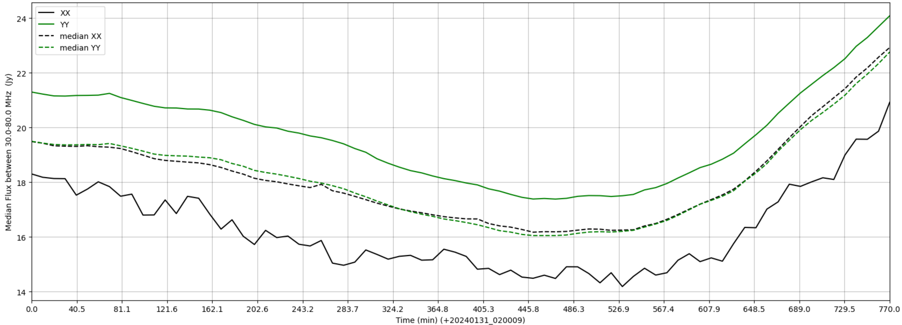
LWA111 - Correlator# 201 - XX FLAGS:BadSpecShape - YY FLAGS:Good
