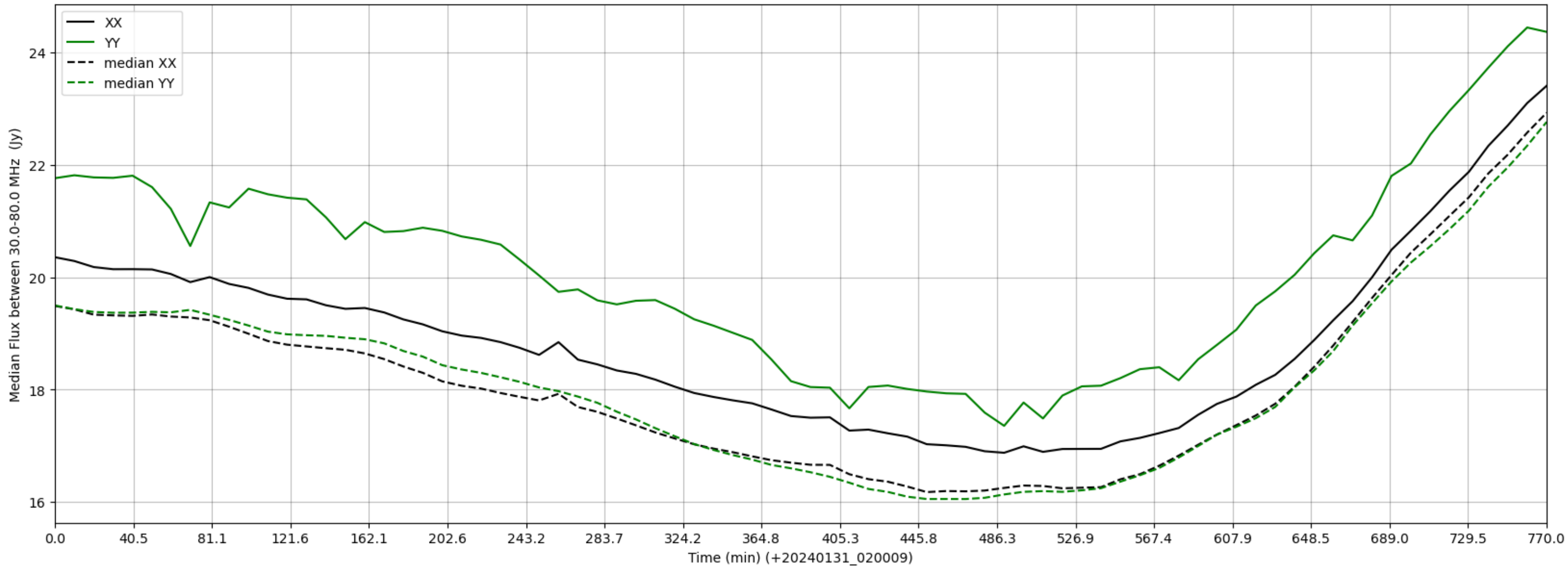
LWA104 - Correlator# 179 - XX FLAGS:Good - YY FLAGS:BadSpecShape
