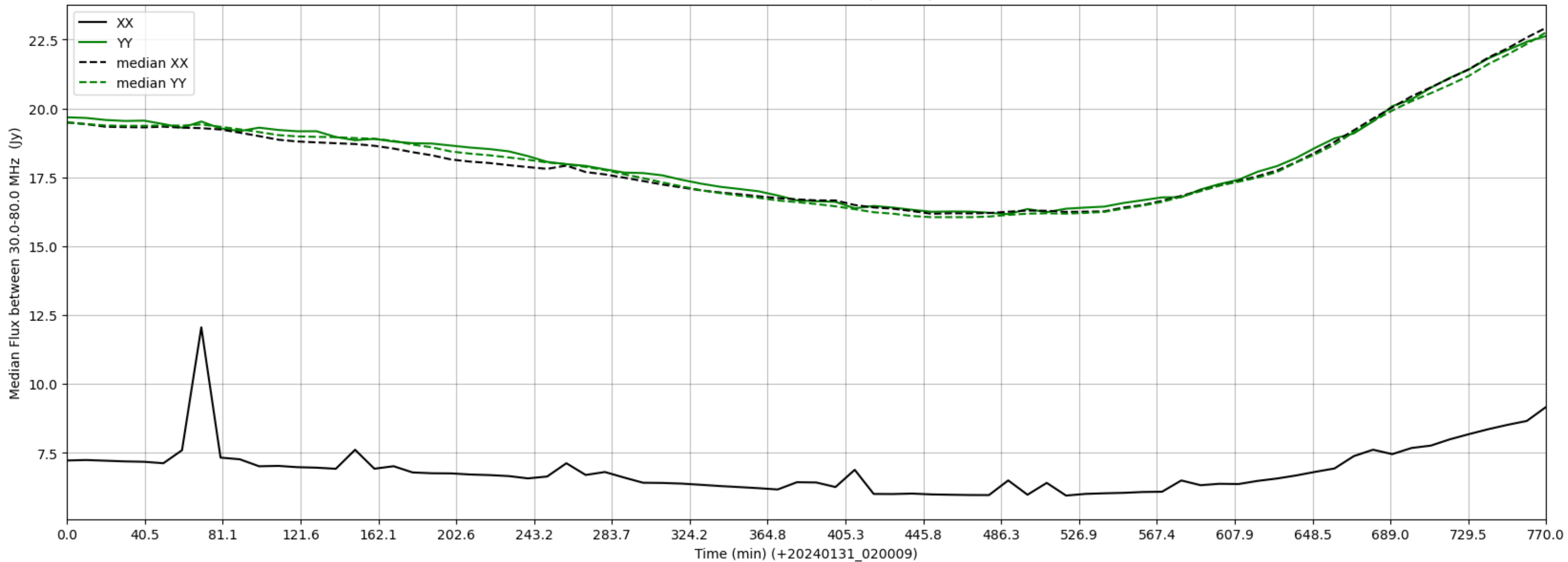
LWA105 - Correlator# 178 - XX FLAGS:BadSpecShape - YY FLAGS:Good
