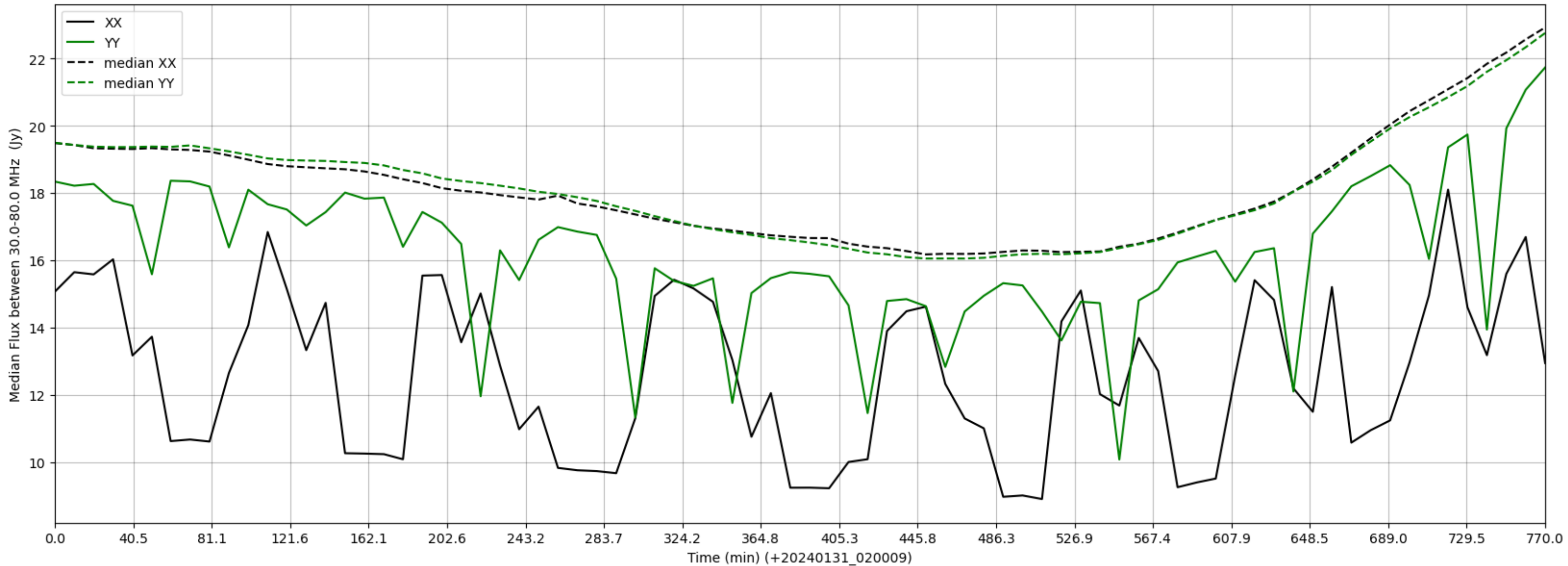
LWA120 - Correlator# 208 - XX FLAGS:HighTimeVar+BadSpecShape - YY FLAGS:BadSpecShape
