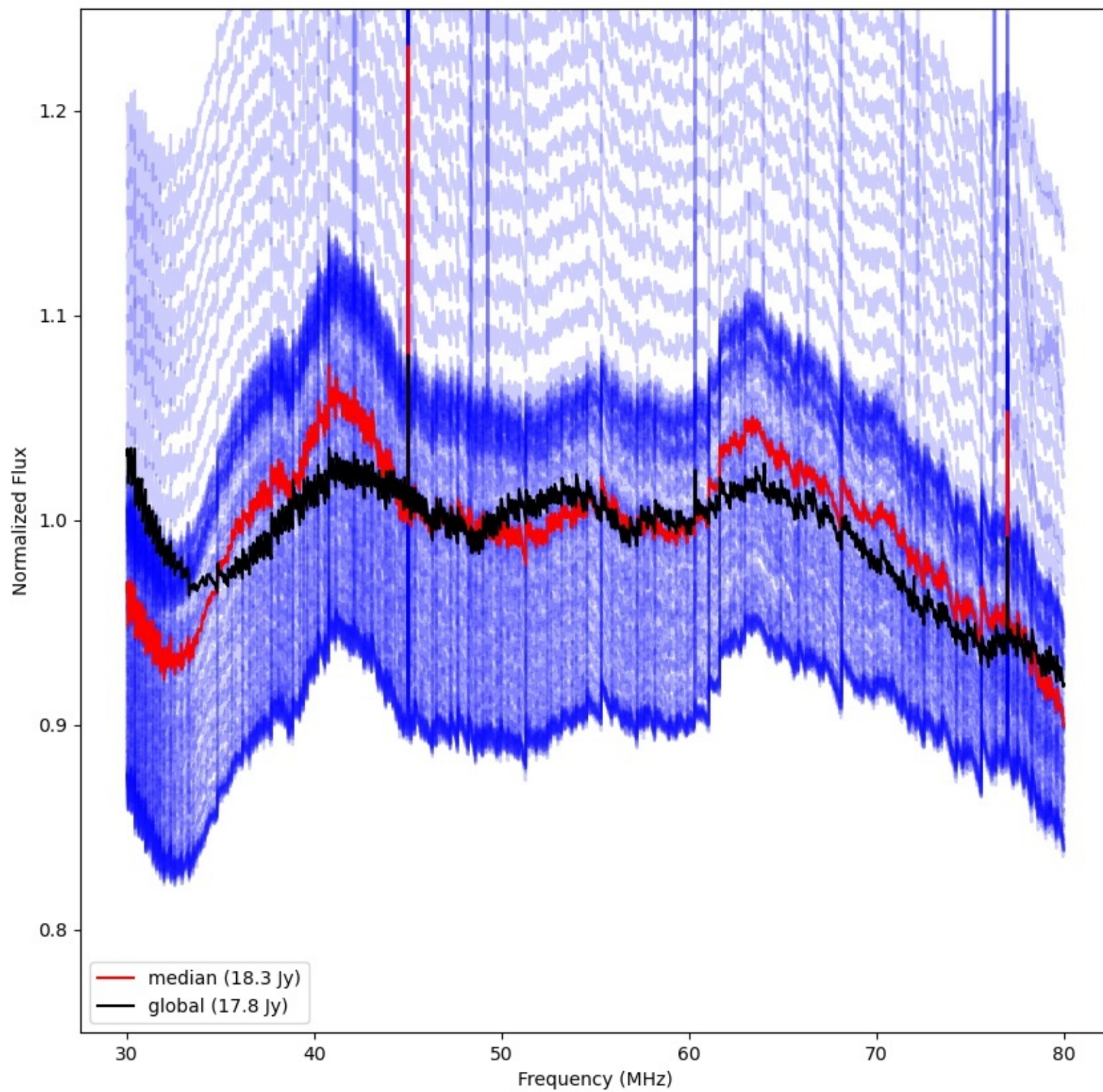
LWA322 - Correlator# 251 - XX - FLAGS:Good
