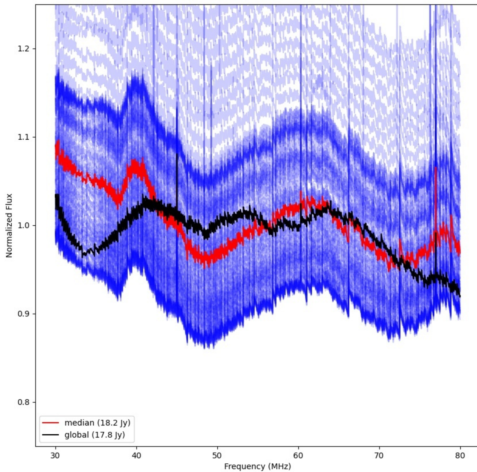
LWA004 - Correlator# 066 - XX - FLAGS:Good
