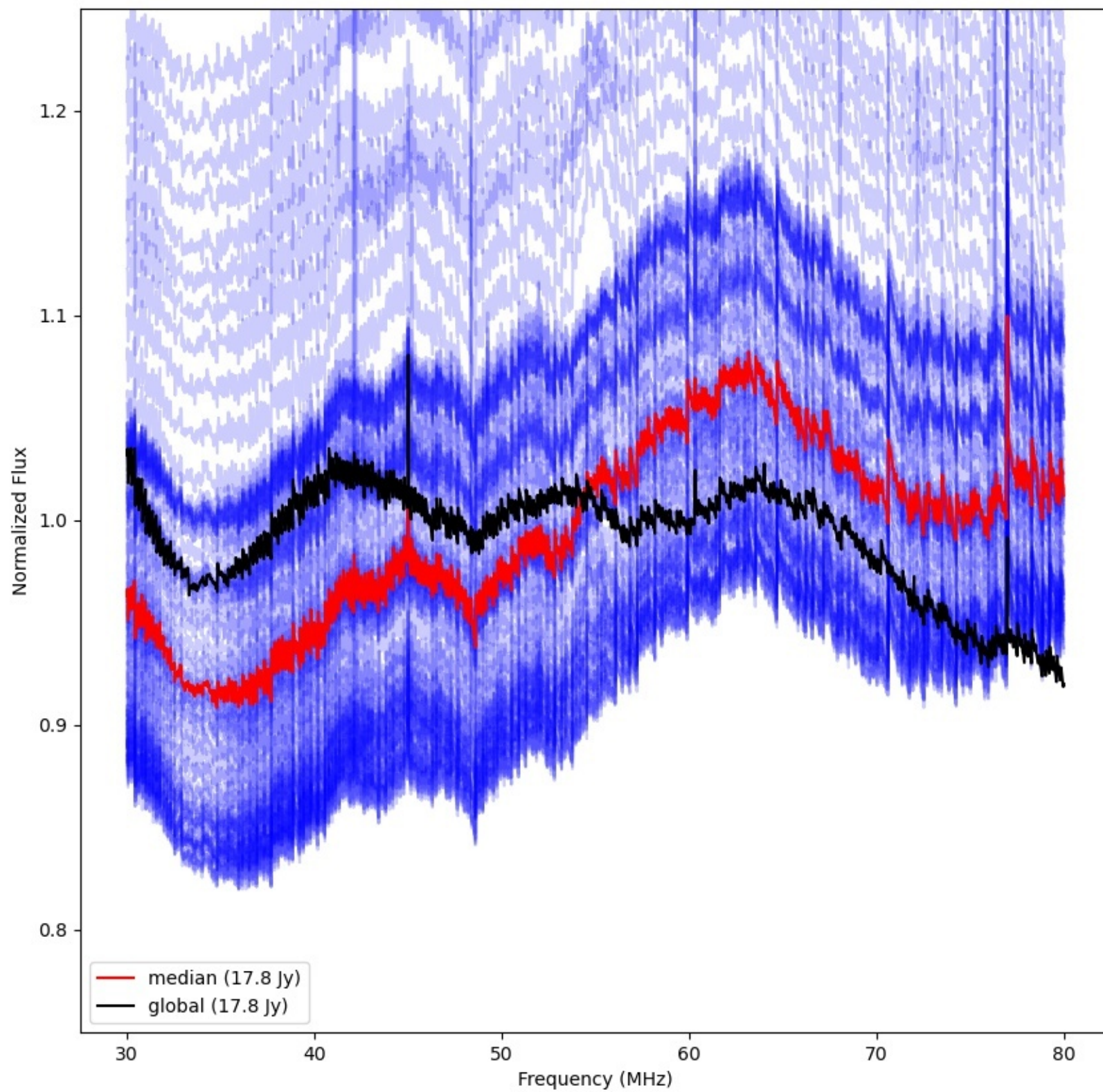
LWA225 - Correlator# 281 - XX - FLAGS:Good
