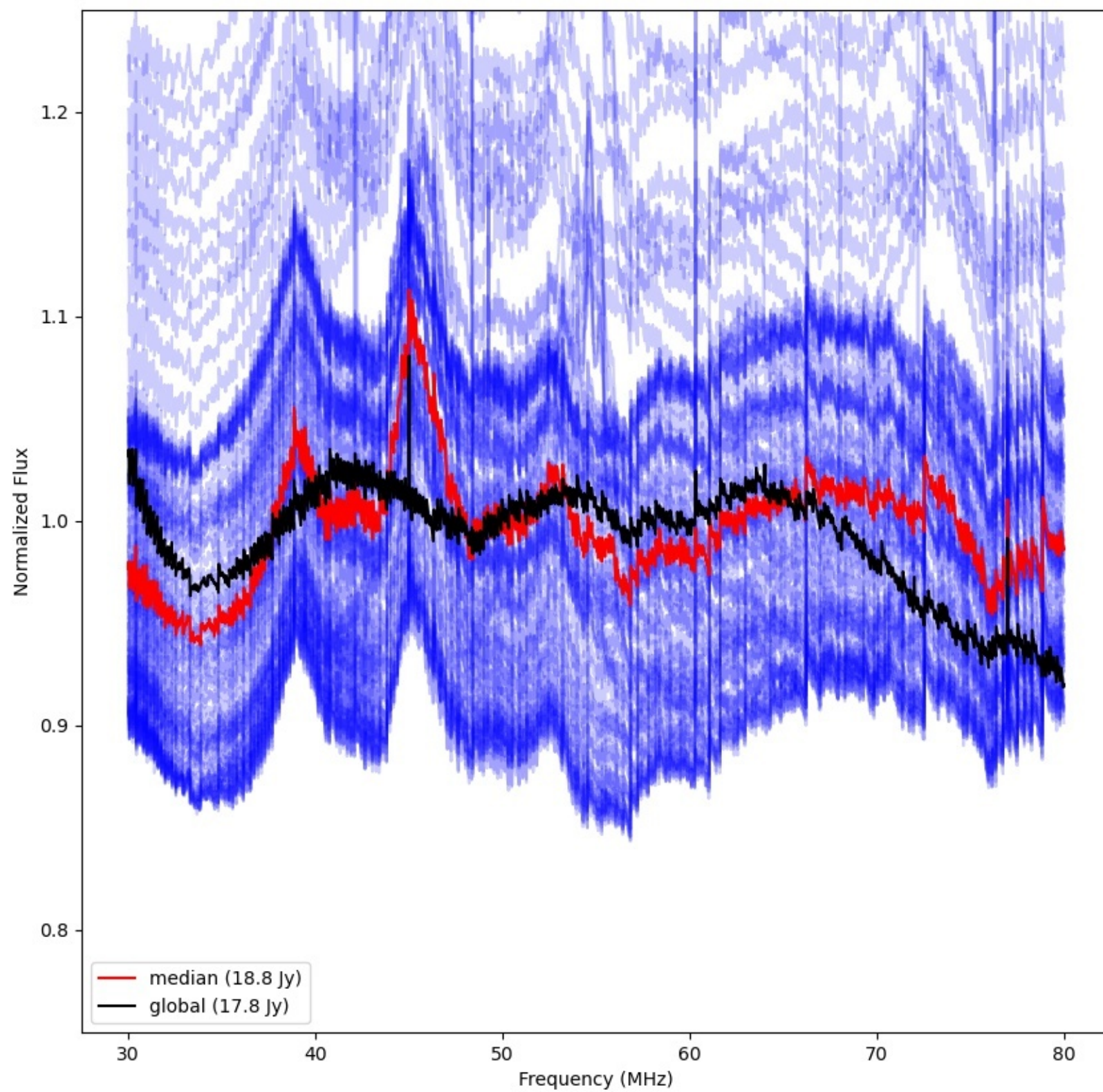
LWA228 - Correlator# 302 - XX - FLAGS:Good
