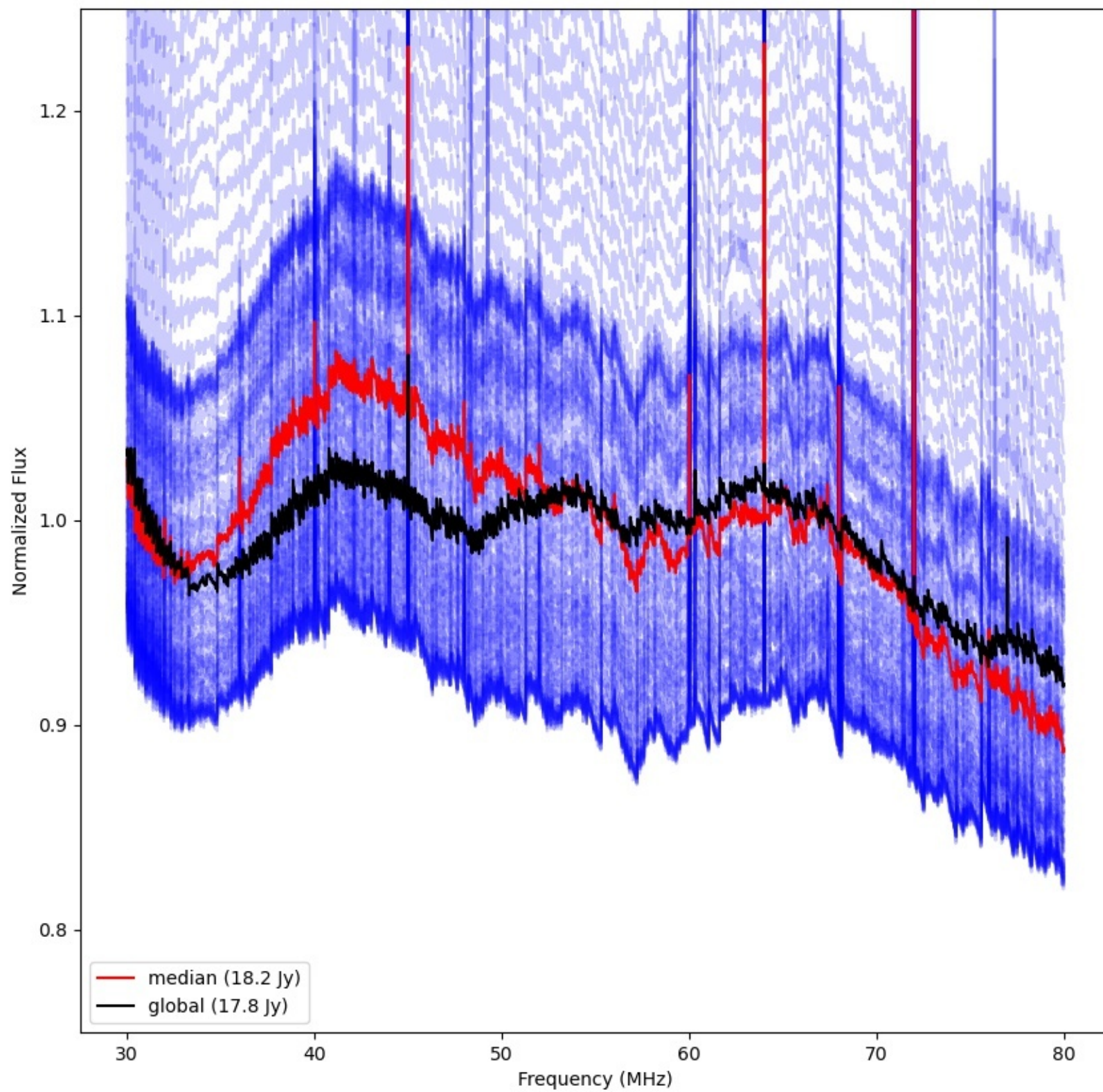
LWA192 - Correlator# 247 - XX - FLAGS:Good
