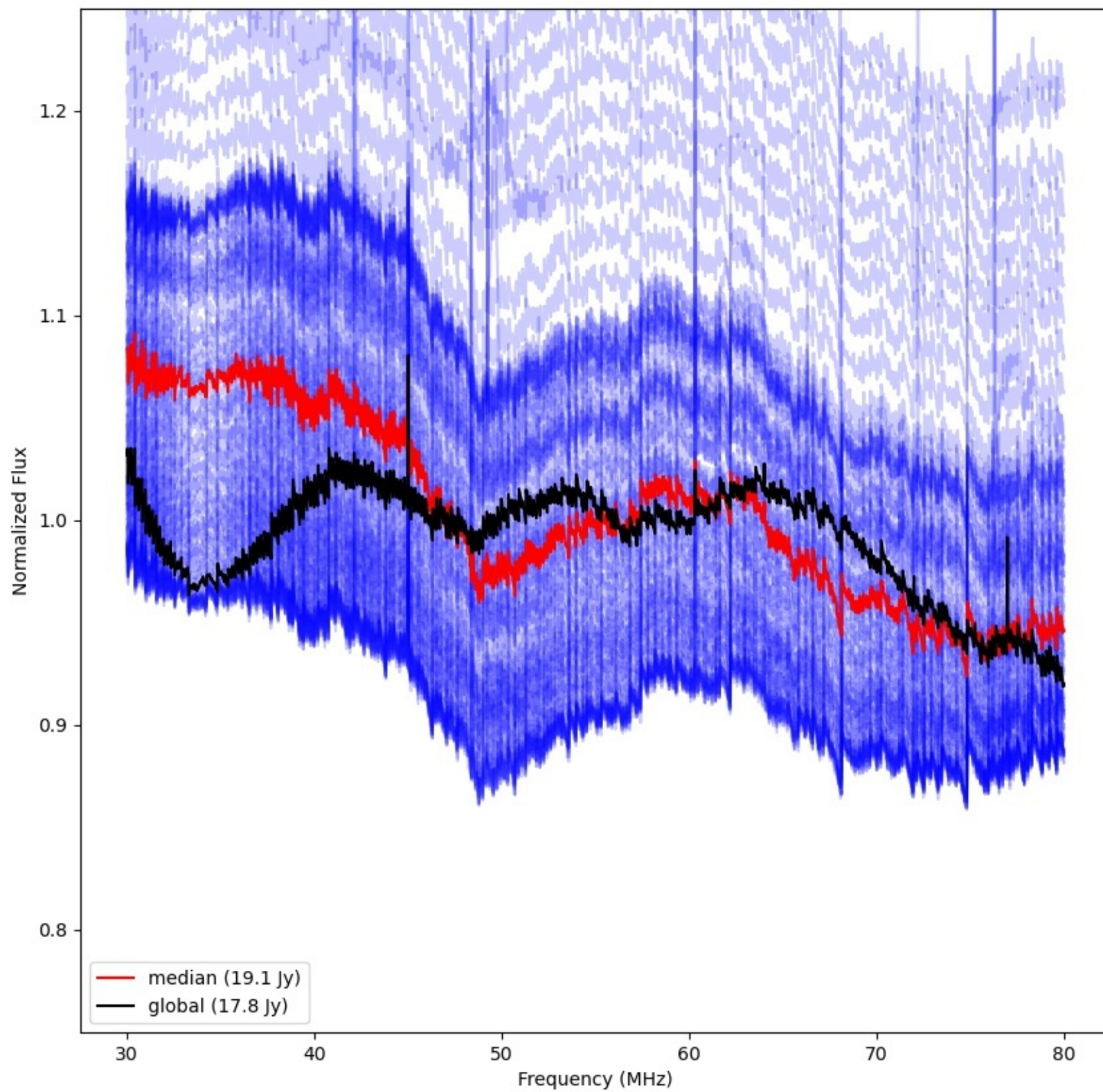
LWA012 - Correlator# 074 - XX - FLAGS:Good
