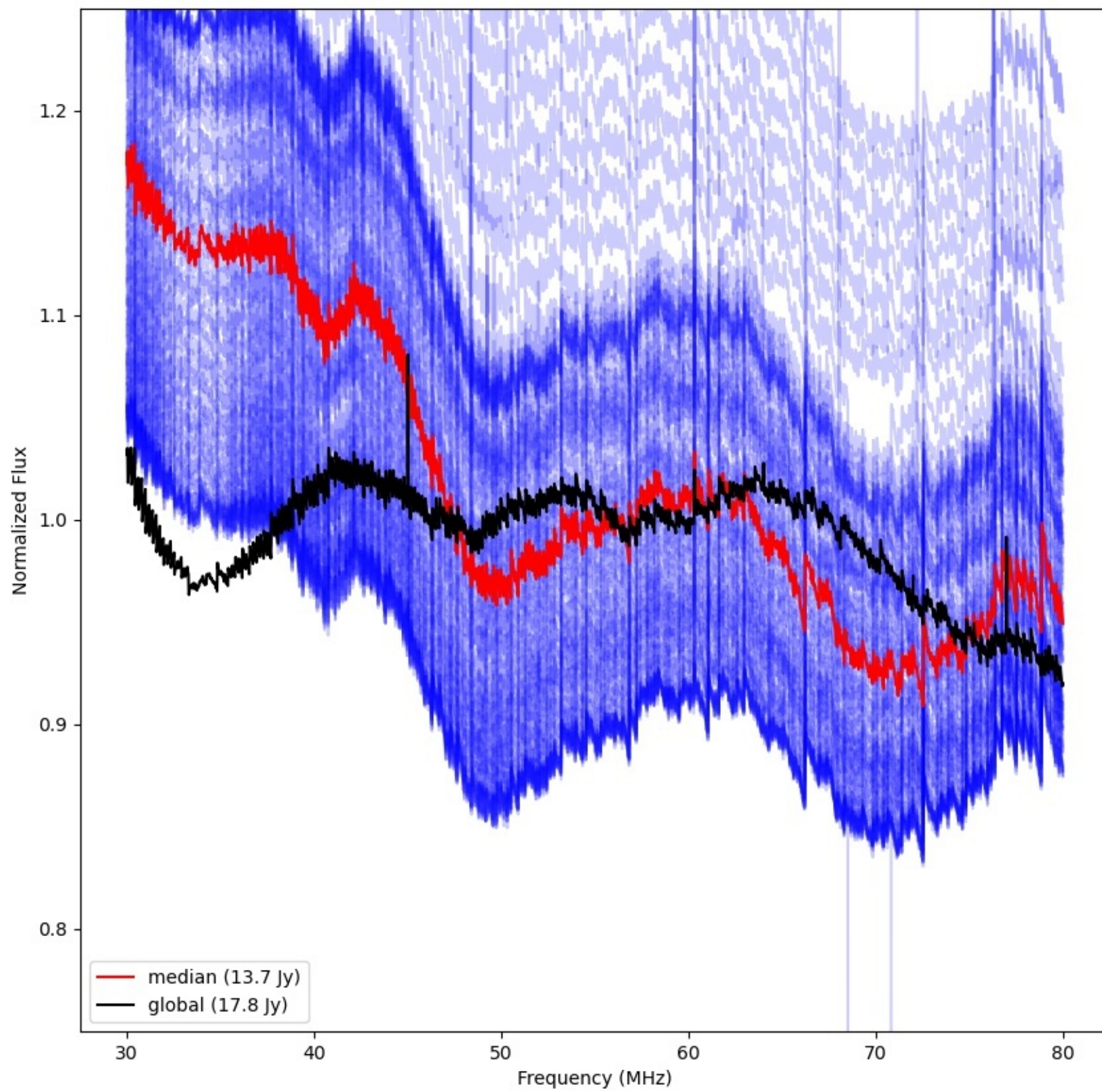
LWA038 - Correlator# 077 - XX - FLAGS:Good
