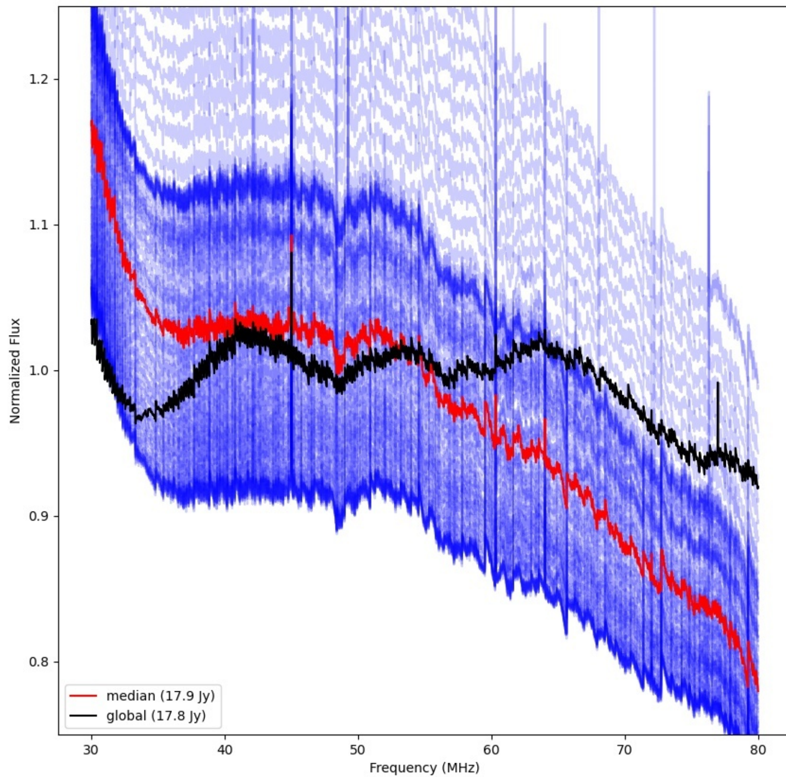
LWA058 - Correlator# 137 - XX - FLAGS:Good
