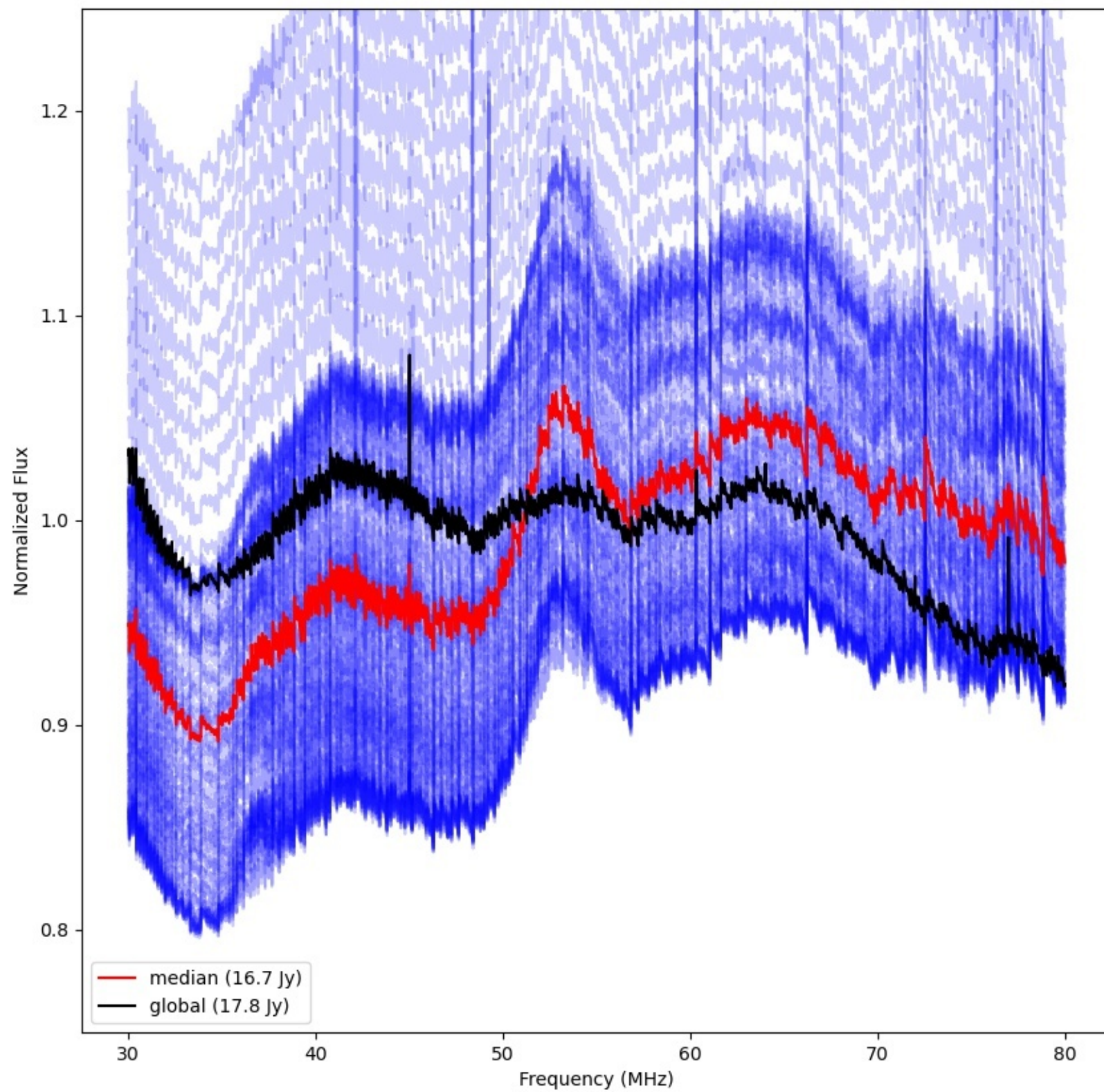
LWA100 - Correlator# 175 - XX - FLAGS:Good
