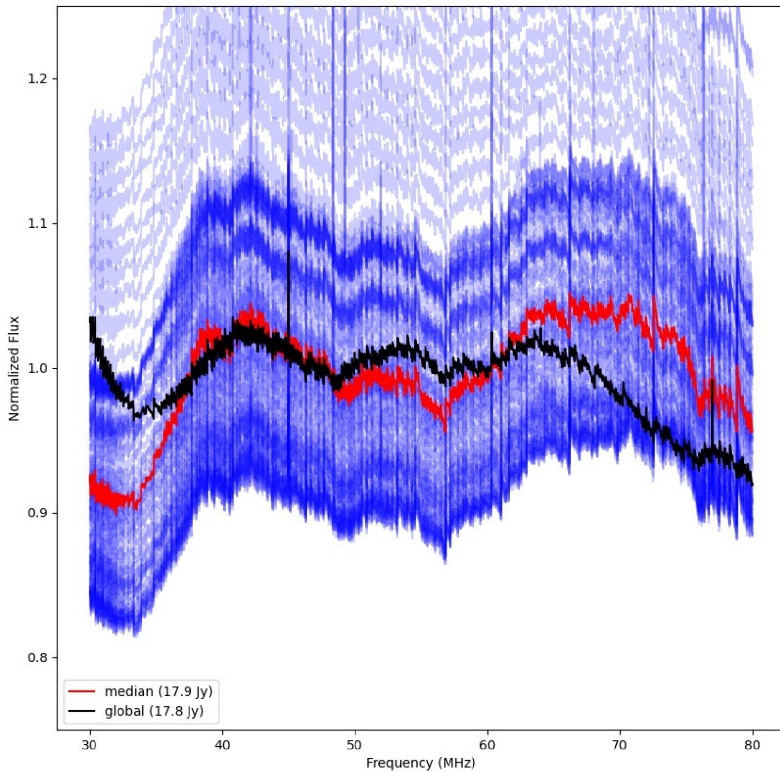
LWA134 - Correlator# 184 - XX - FLAGS:Good
