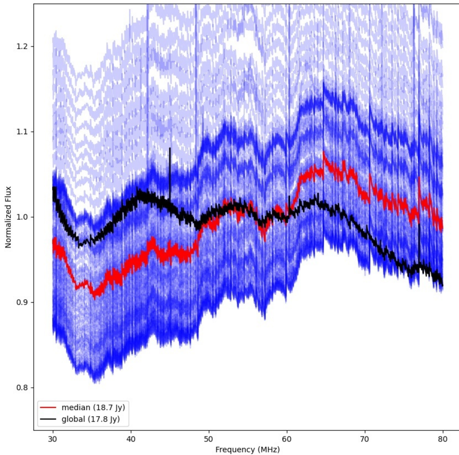
LWA161 - Correlator# 262 - XX - FLAGS:Good
