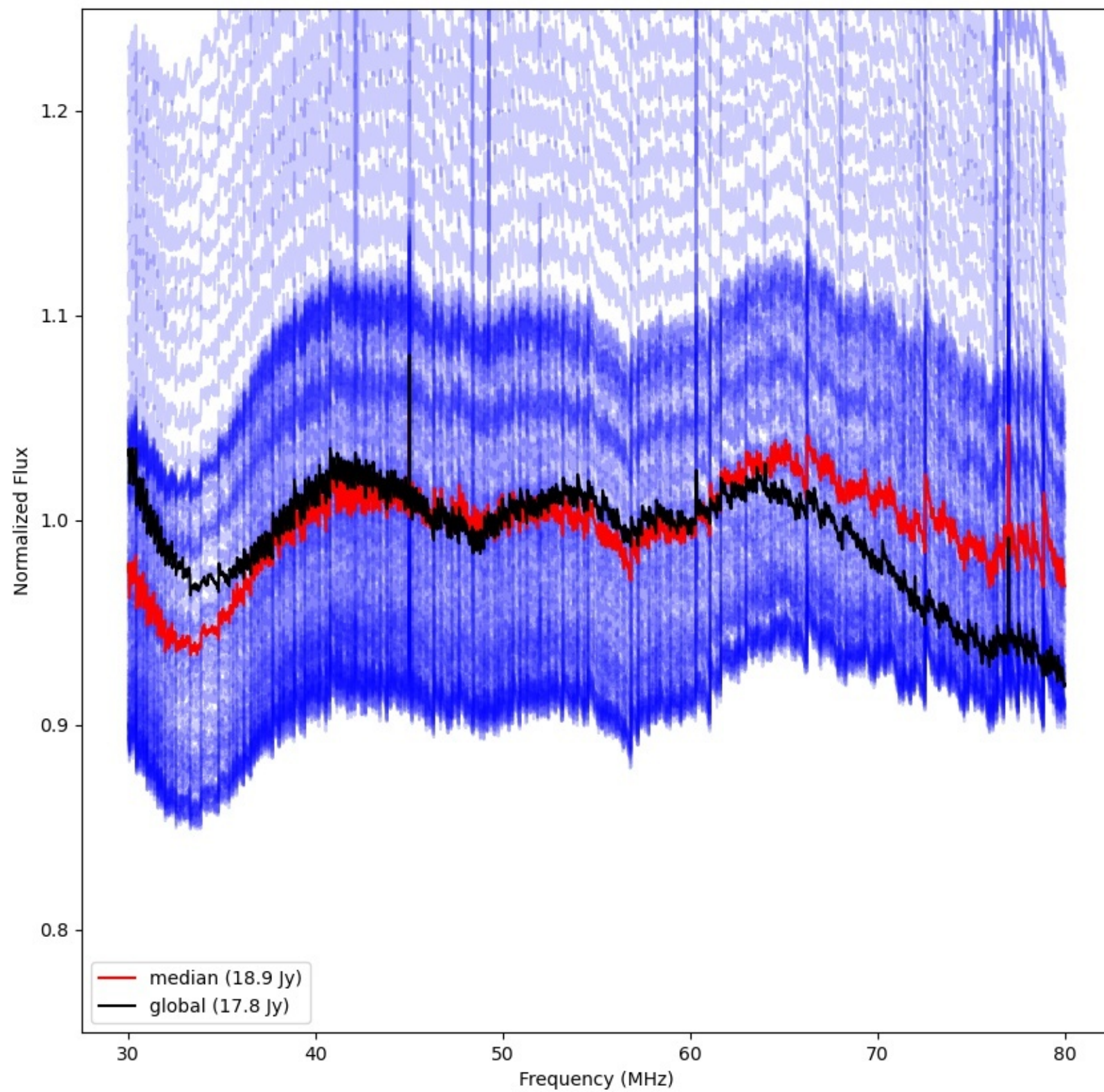
LWA131 - Correlator# 182 - XX - FLAGS:Good
