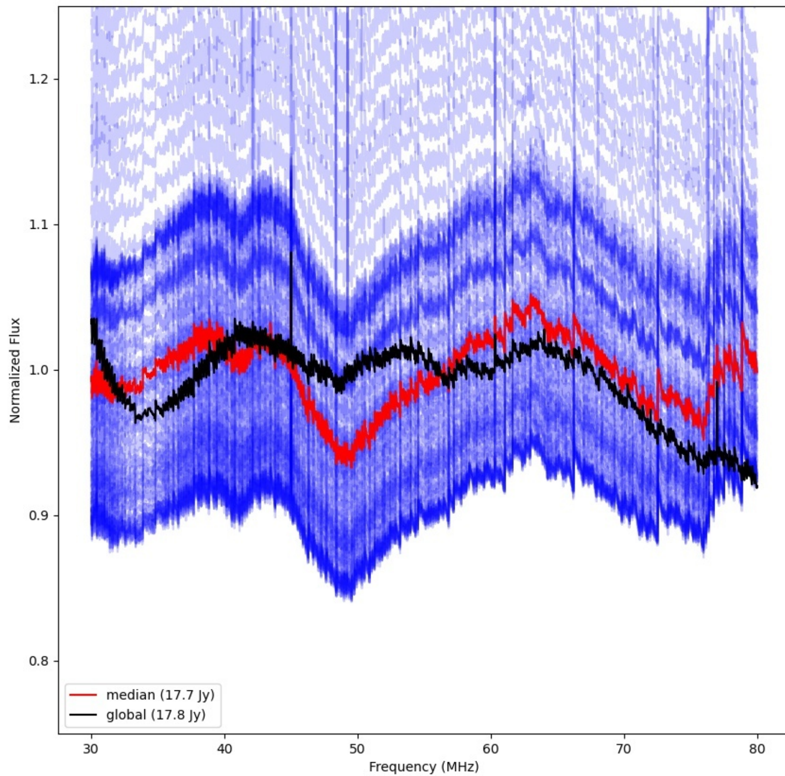
LWA042 - Correlator# 078 - XX - FLAGS:Good
