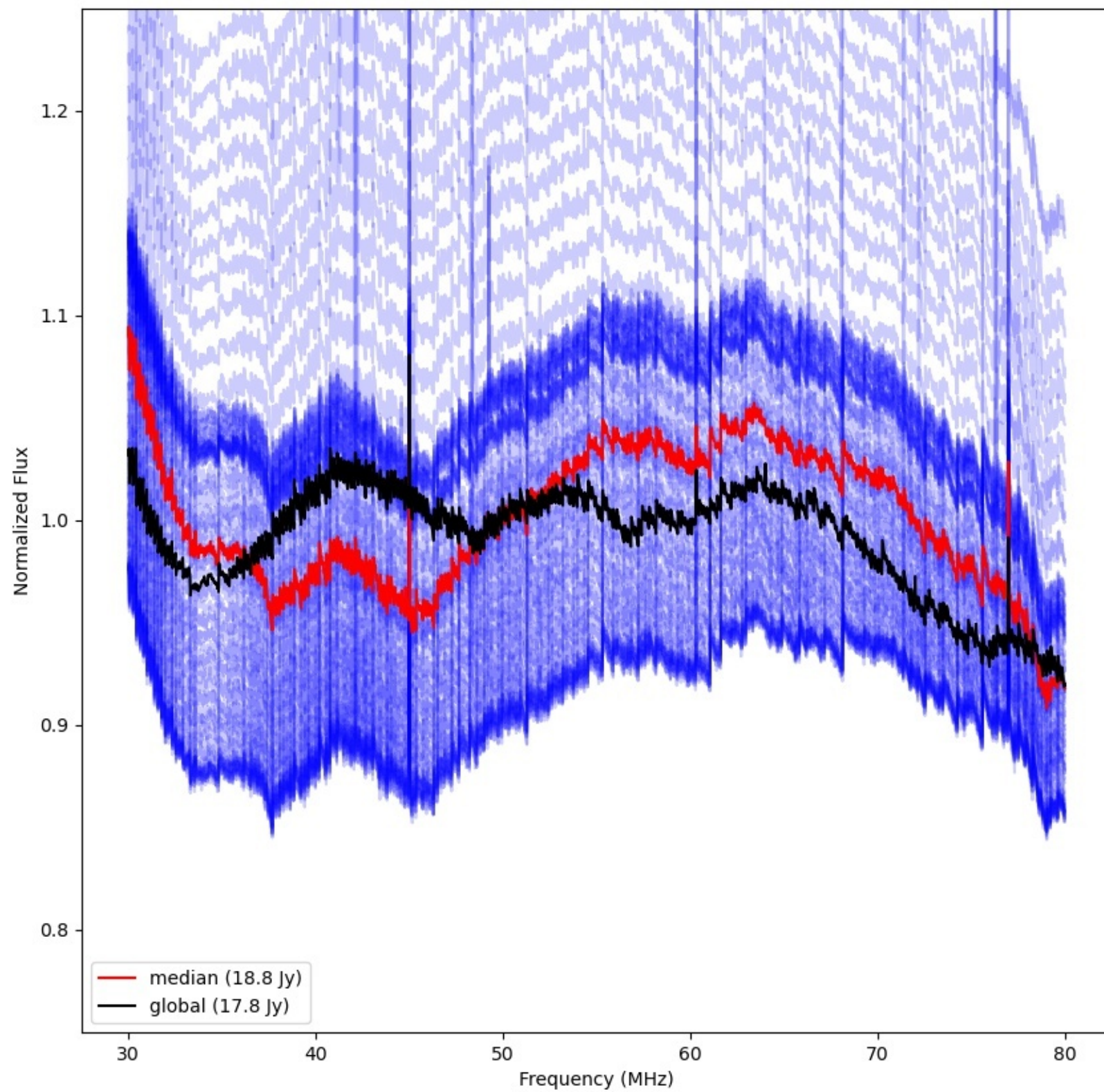
LWA327 - Correlator# 023 - XX - FLAGS:Good
