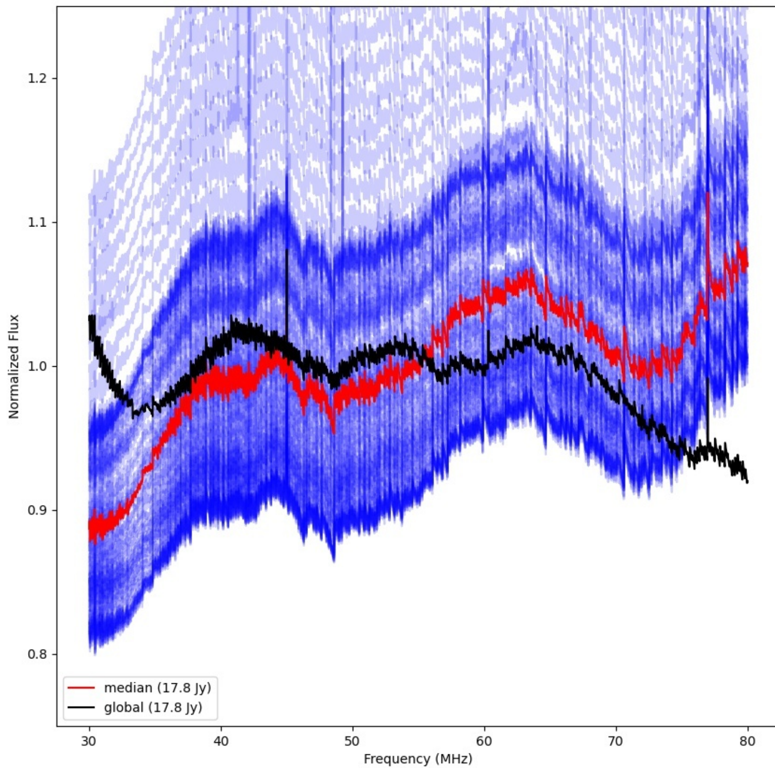
LWA003 - Correlator# 067 - XX - FLAGS:Good
