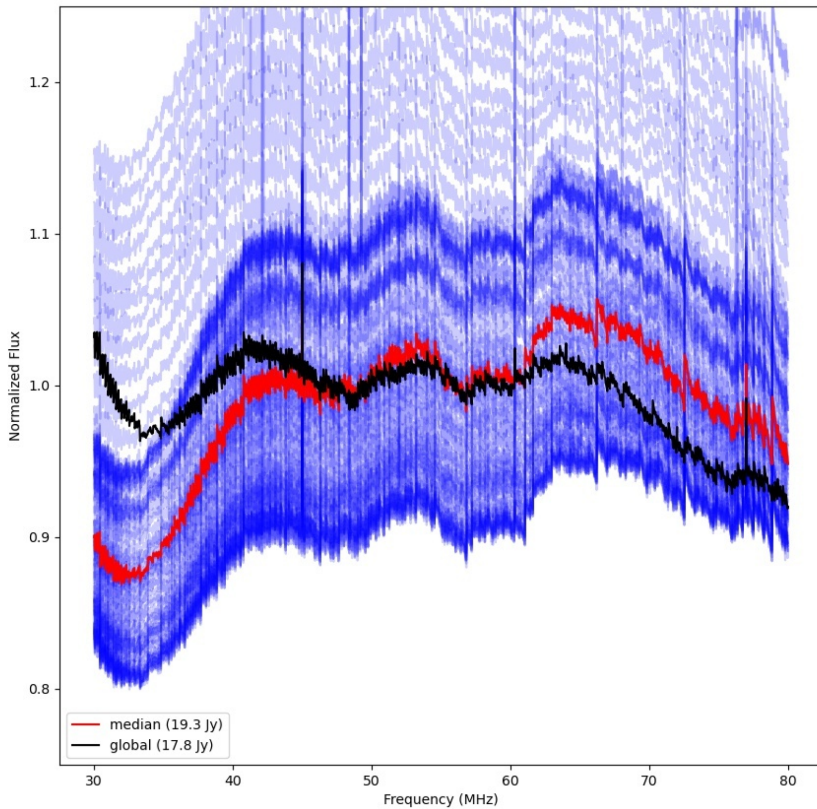
LWA162 - Correlator# 265 - XX - FLAGS:Good
