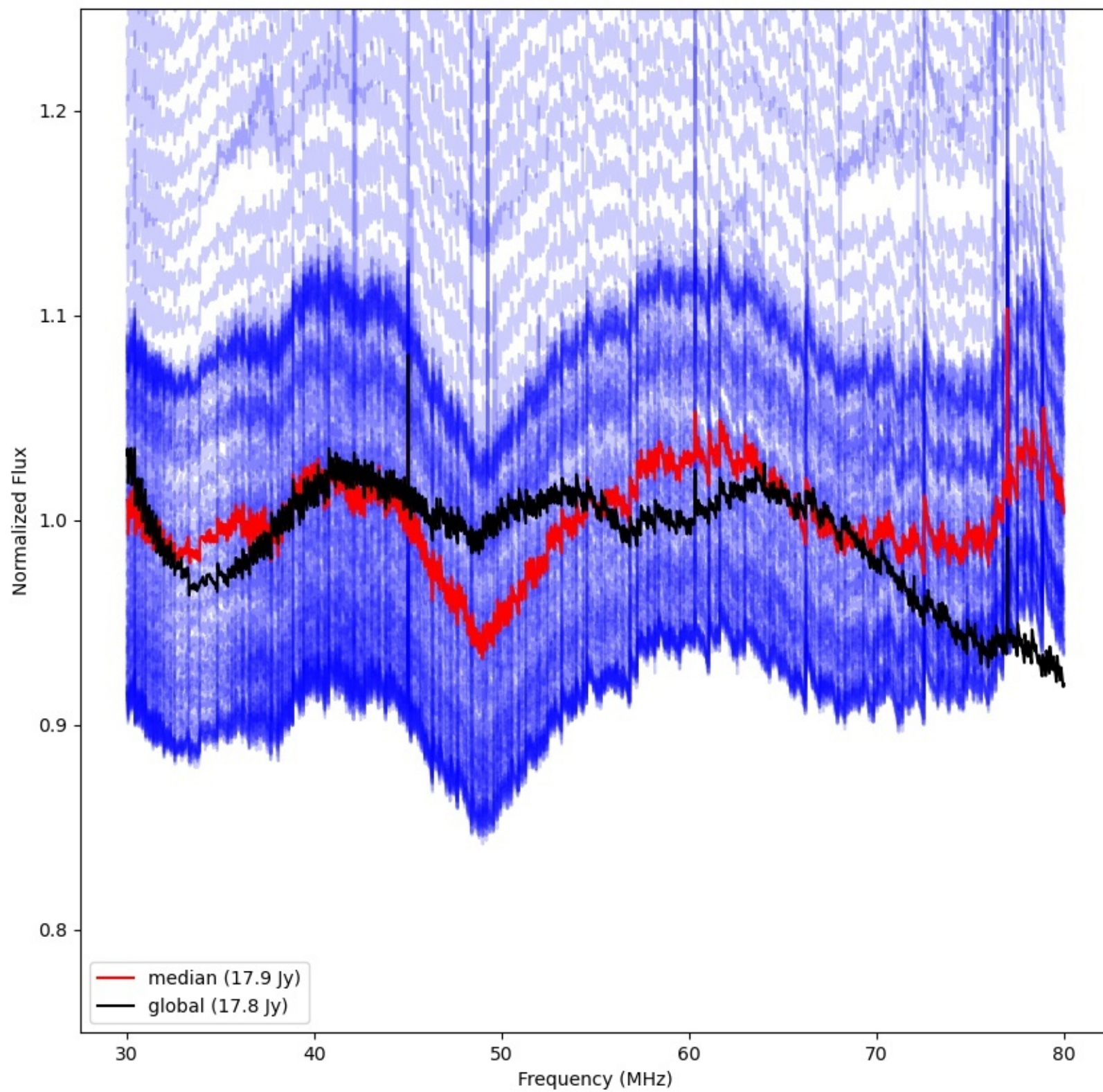
LWA008 - Correlator# 075 - XX - FLAGS:Good
