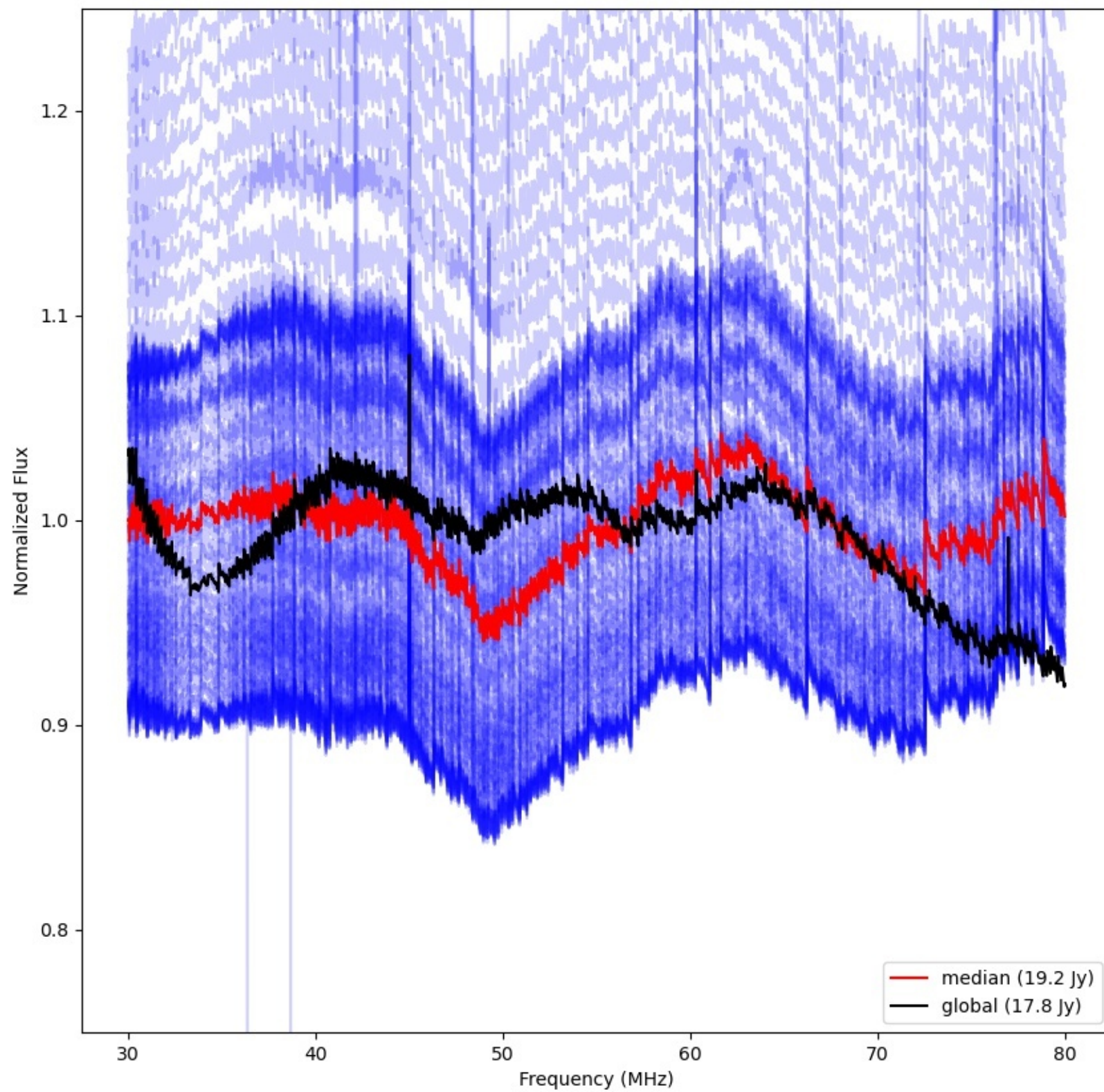
LWA007 - Correlator# 071 - XX - FLAGS:Good
