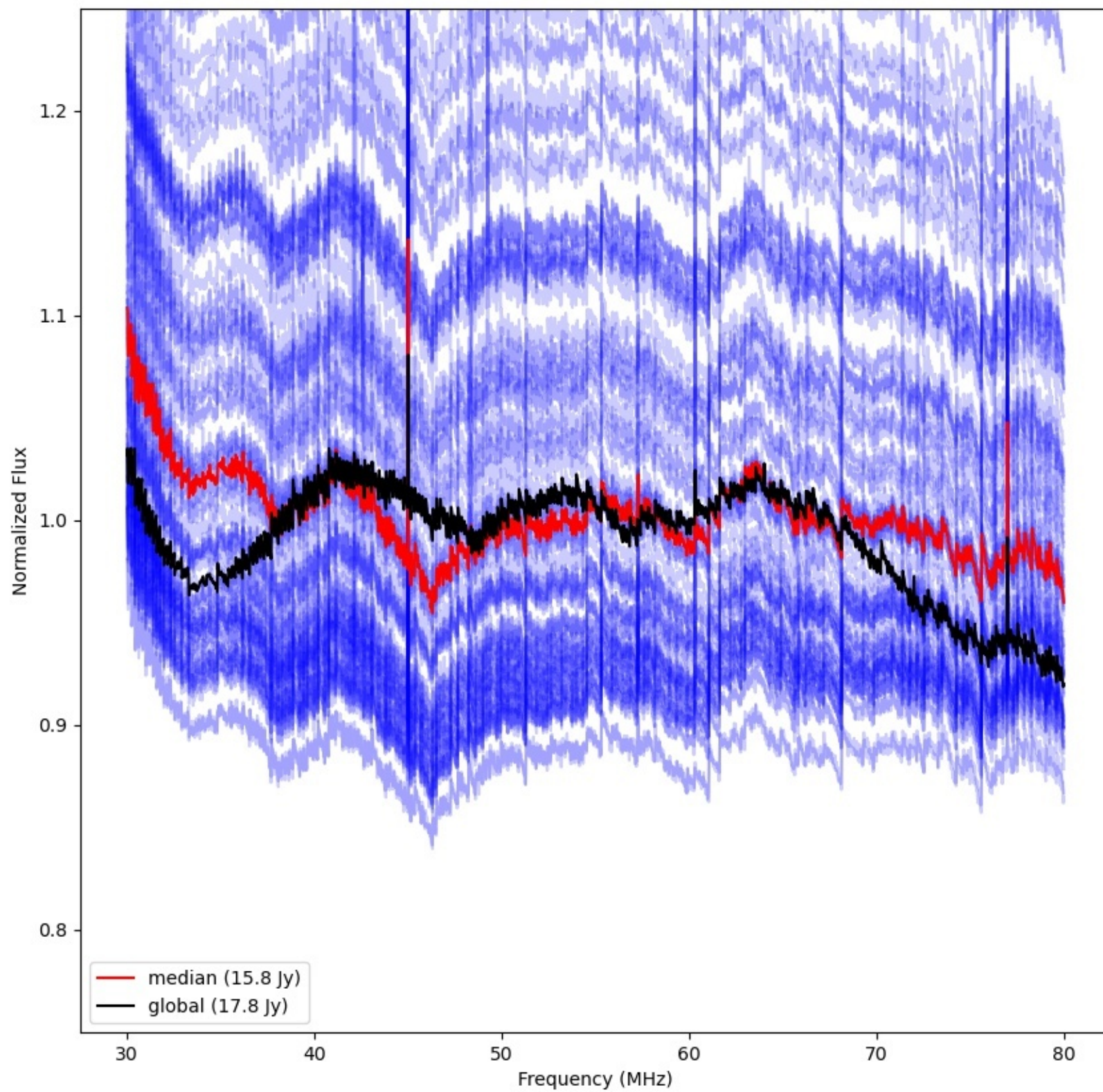
LWA299 - Correlator# 191 - XX - FLAGS:Good
