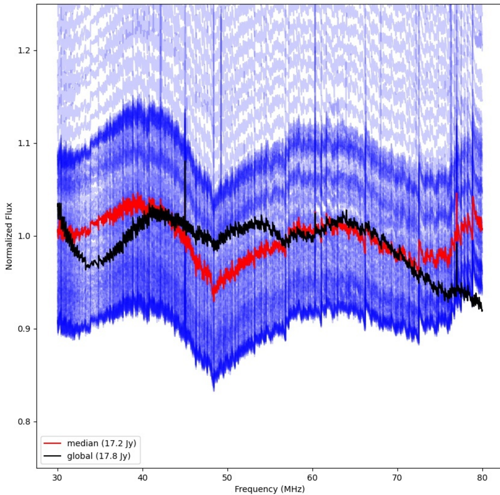
LWA010 - Correlator# 073 - XX - FLAGS:Good
