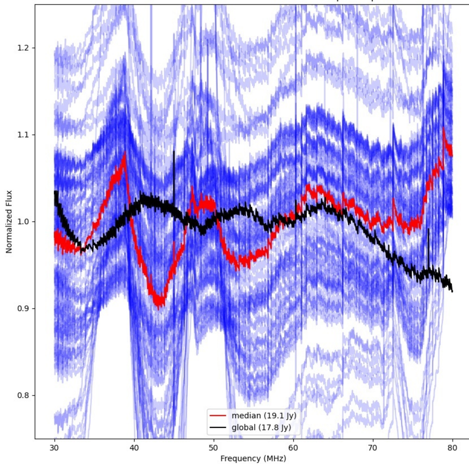
LWA041 - Correlator# 079 - XX - FLAGS:BadSpecShape
