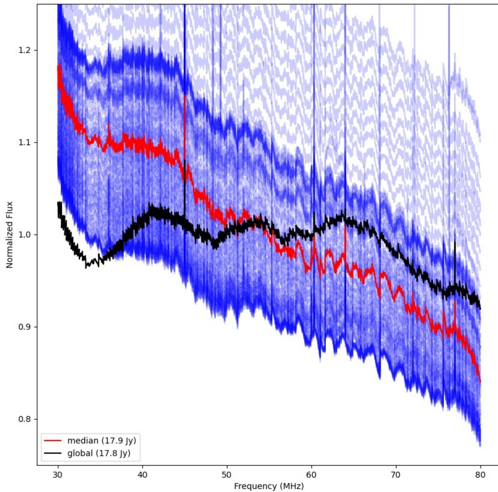
LWA063 - Correlator# 132 - XX - FLAGS:Good
