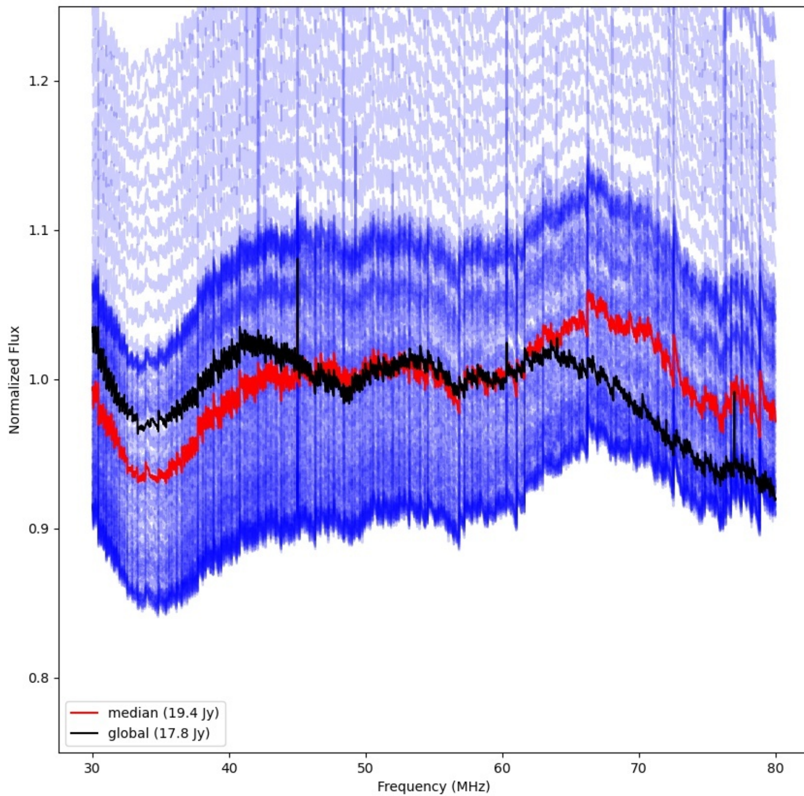
LWA132 - Correlator# 185 - XX - FLAGS:Good
