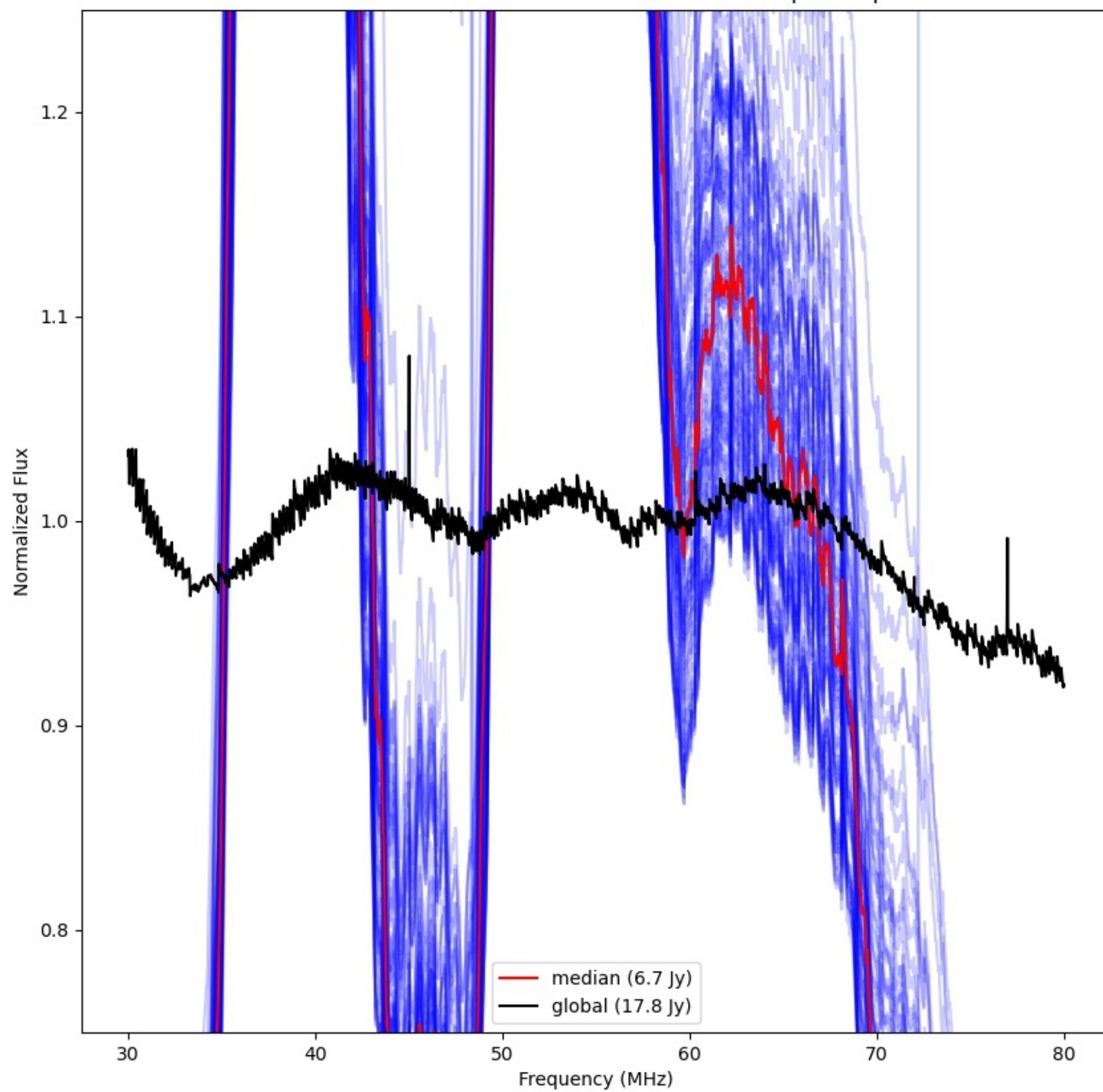
LWA105 - Correlator# 178 - XX - FLAGS:BadSpecShape
