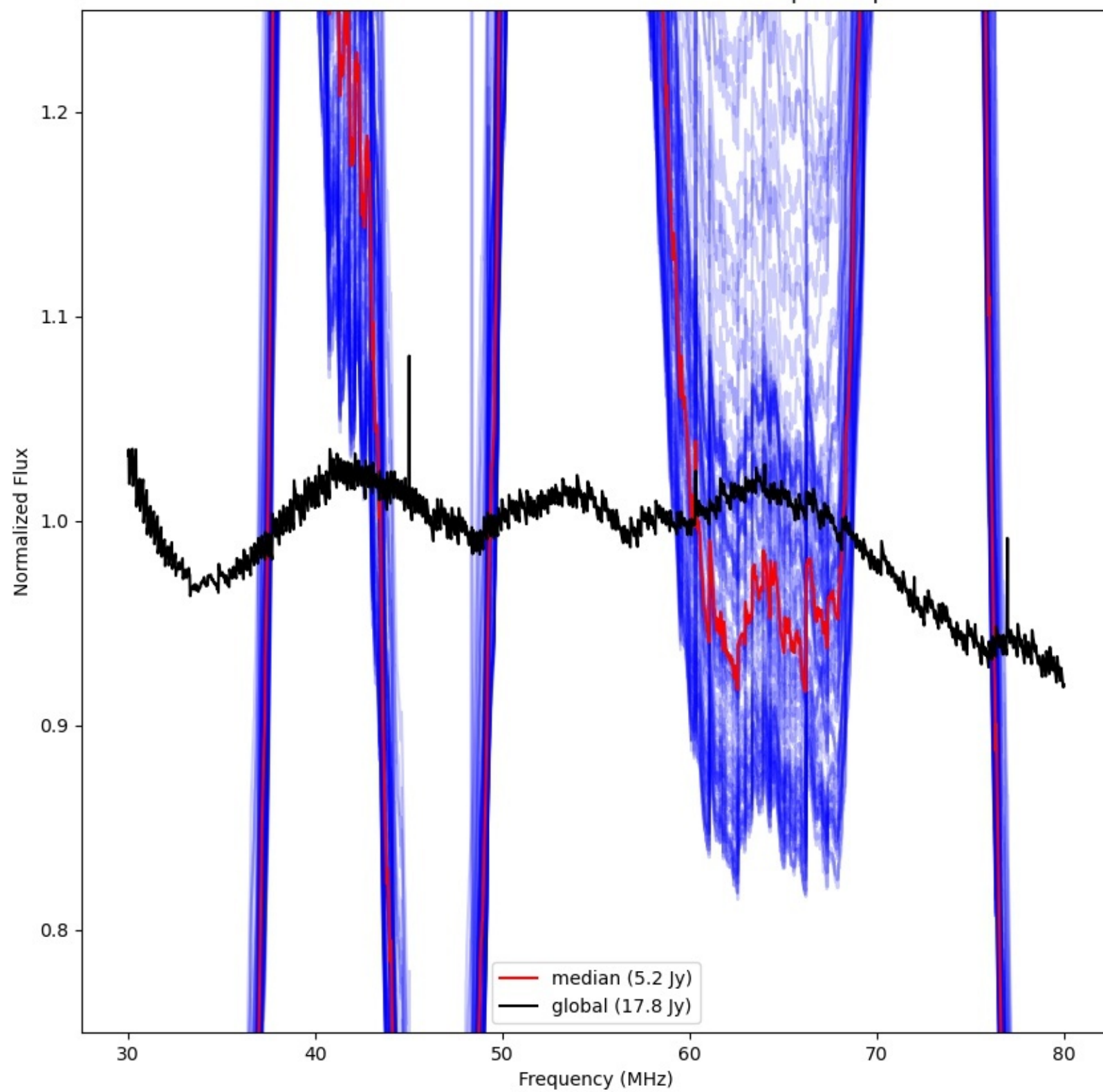
LWA232 - Correlator# 307 - XX - FLAGS:BadSpecShape
