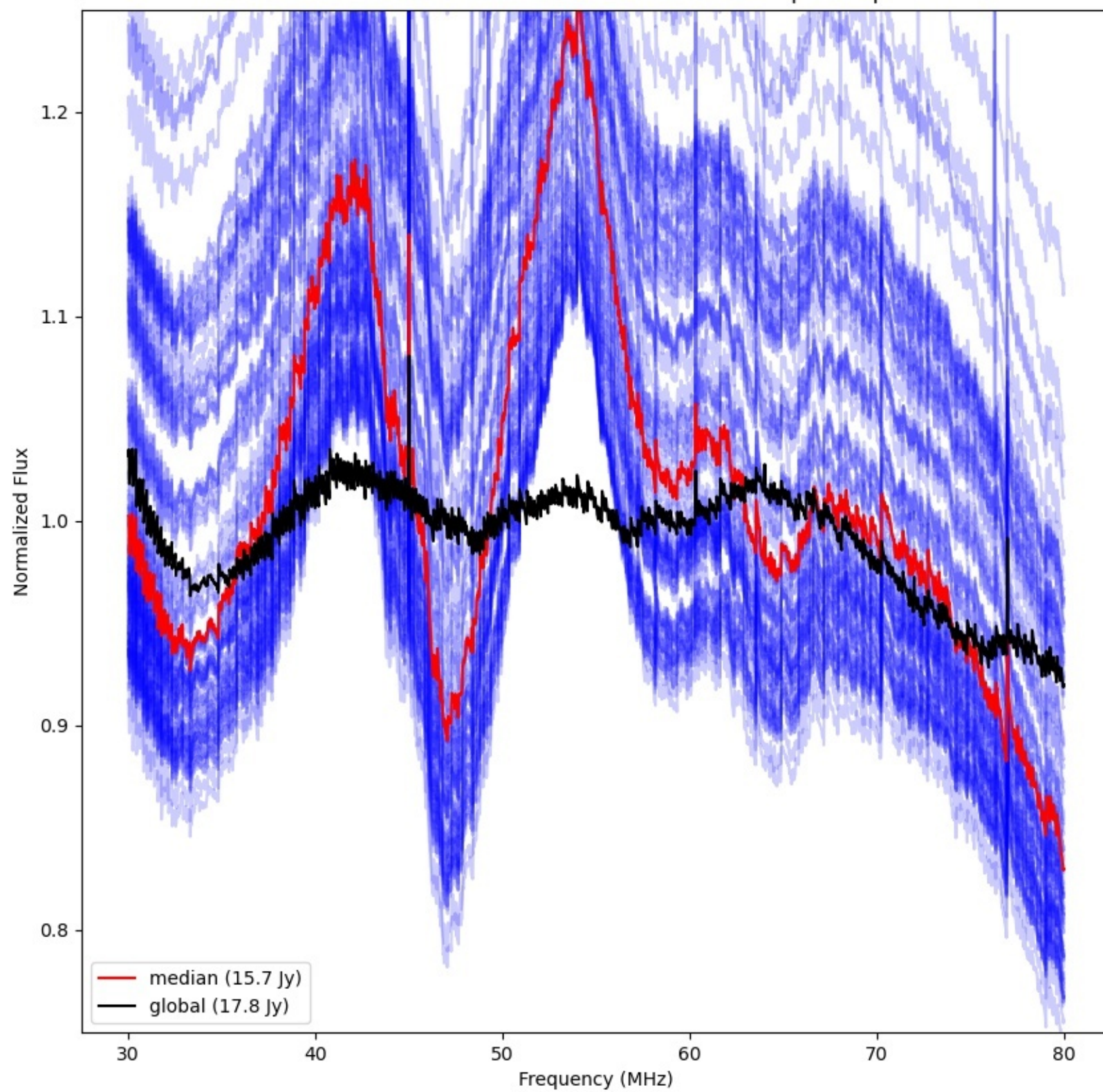
LWA111 - Correlator# 201 - XX - FLAGS:BadSpecShape
