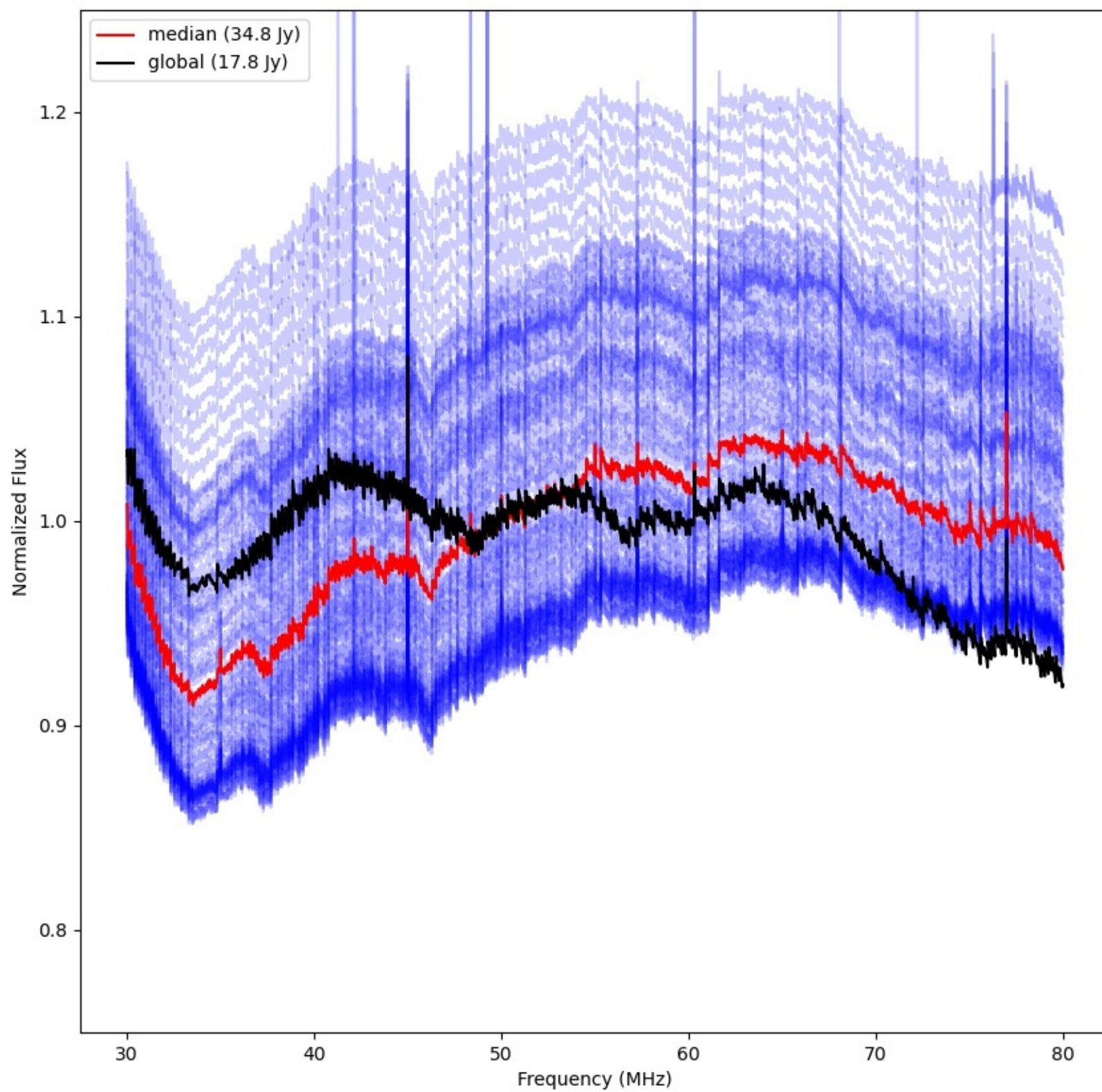
LWA362 - Correlator# 030 - XX - FLAGS:Good
