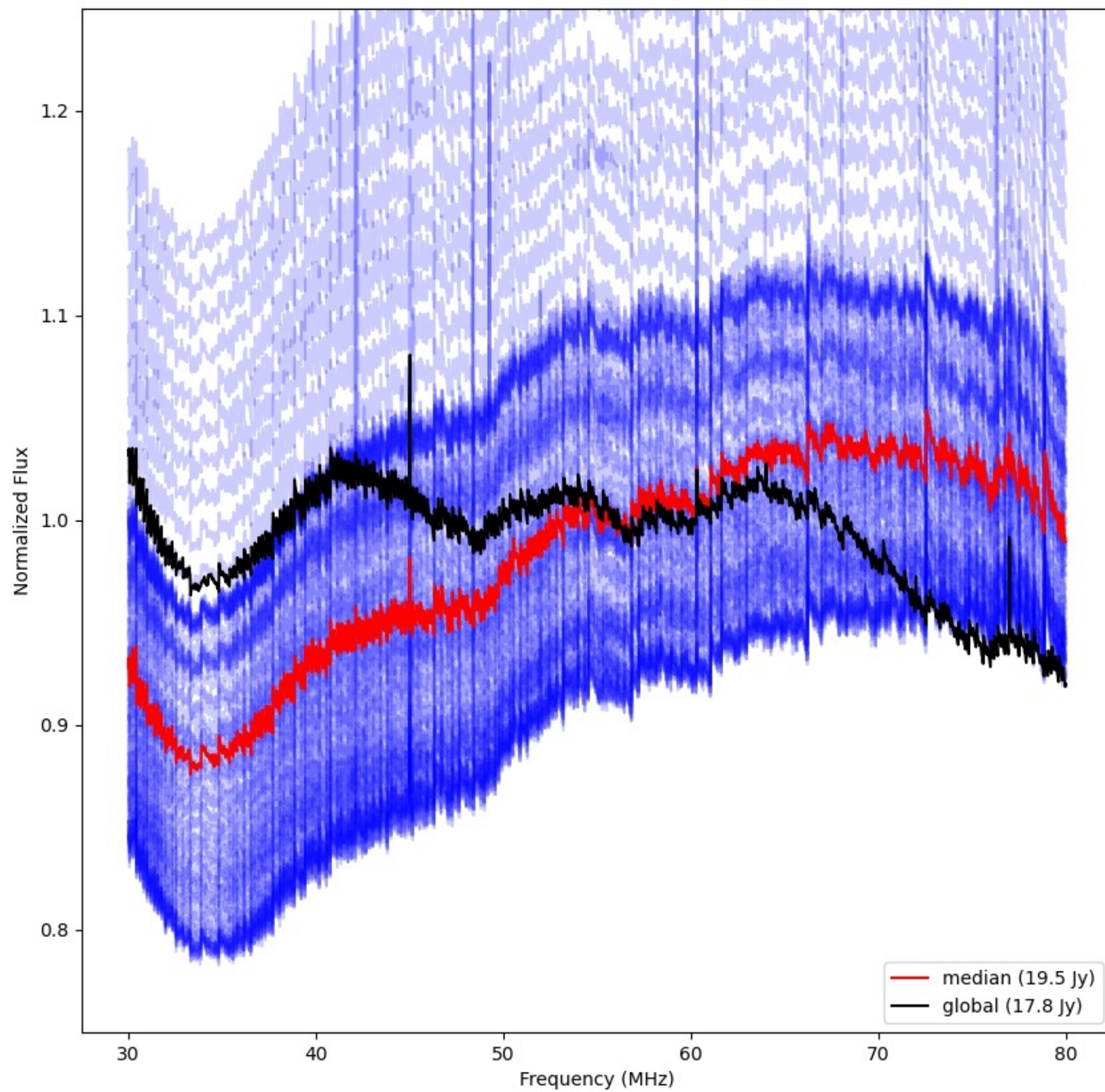
LWA137 - Correlator# 258 - XX - FLAGS:Good
