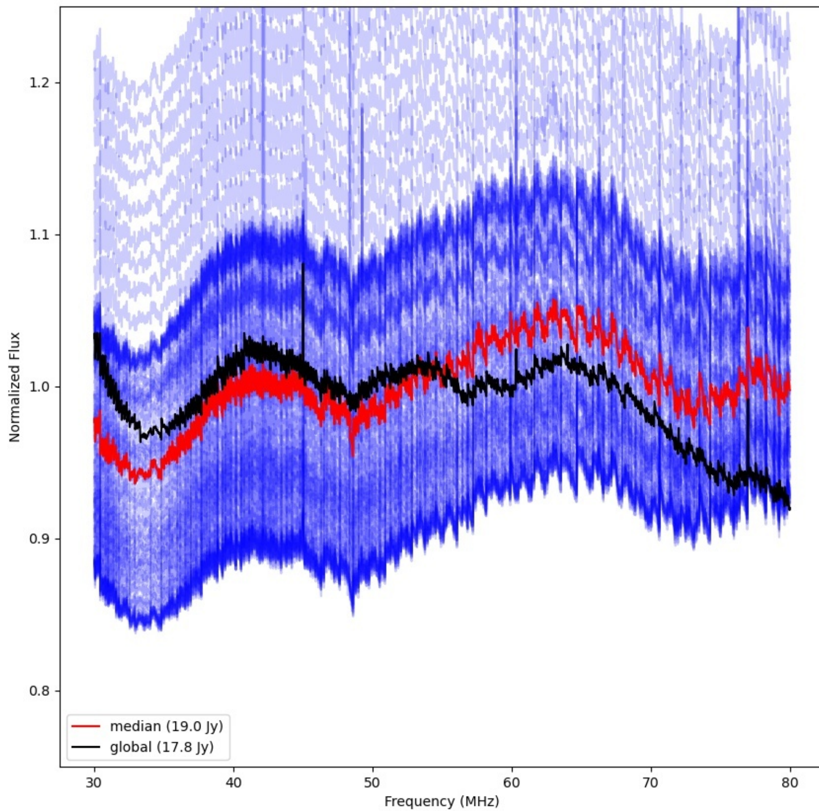
LWA033 - Correlator# 161 - XX - FLAGS:Good
