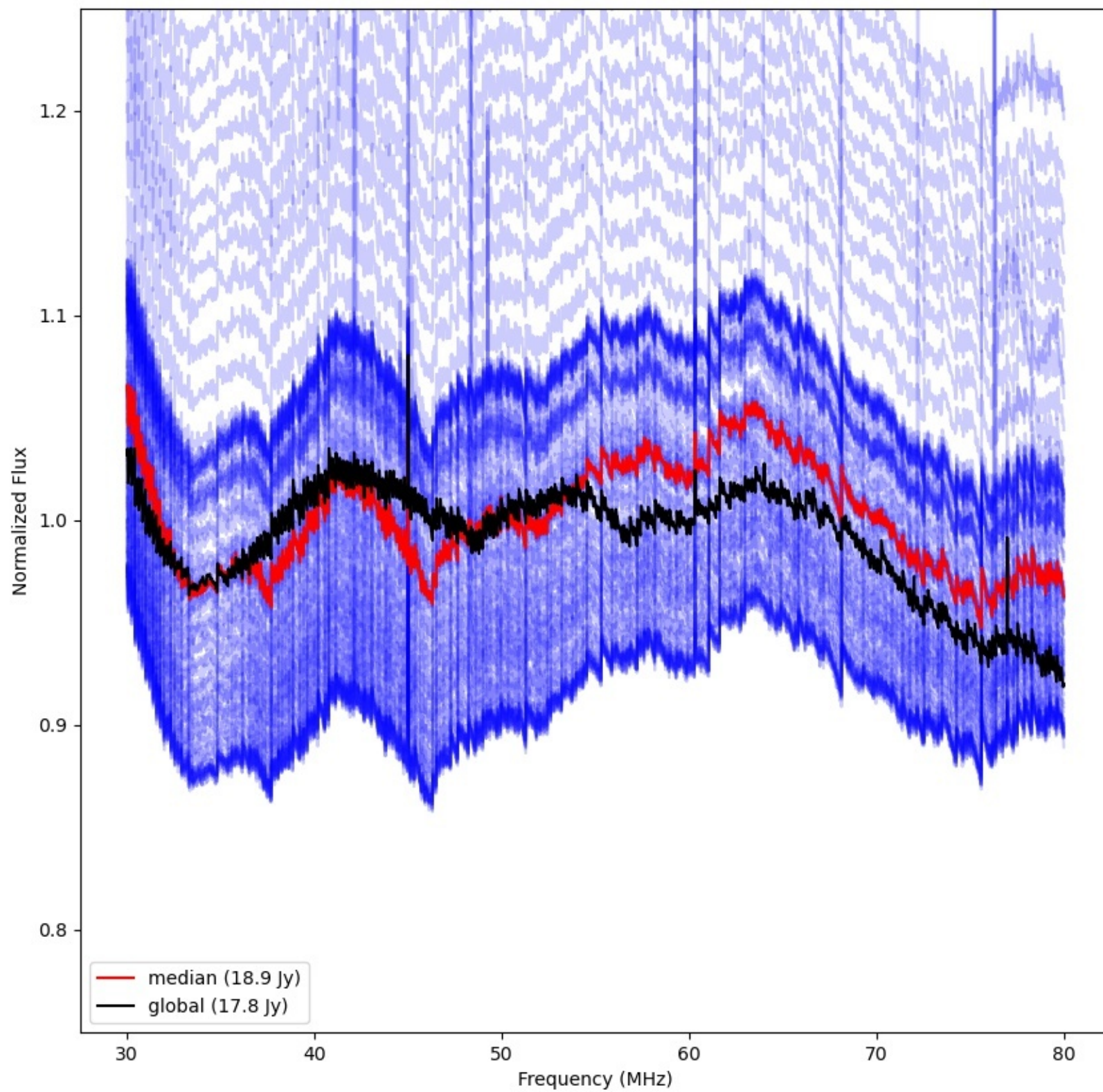
LWA261 - Correlator# 346 - XX - FLAGS:Good
