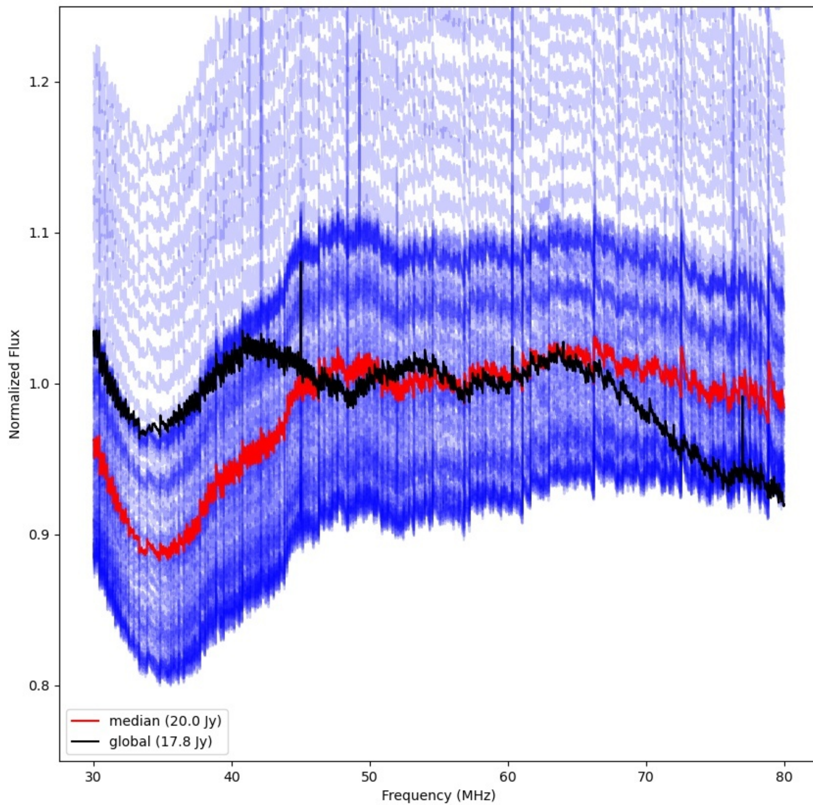
LWA133 - Correlator# 257 - XX - FLAGS:Good
