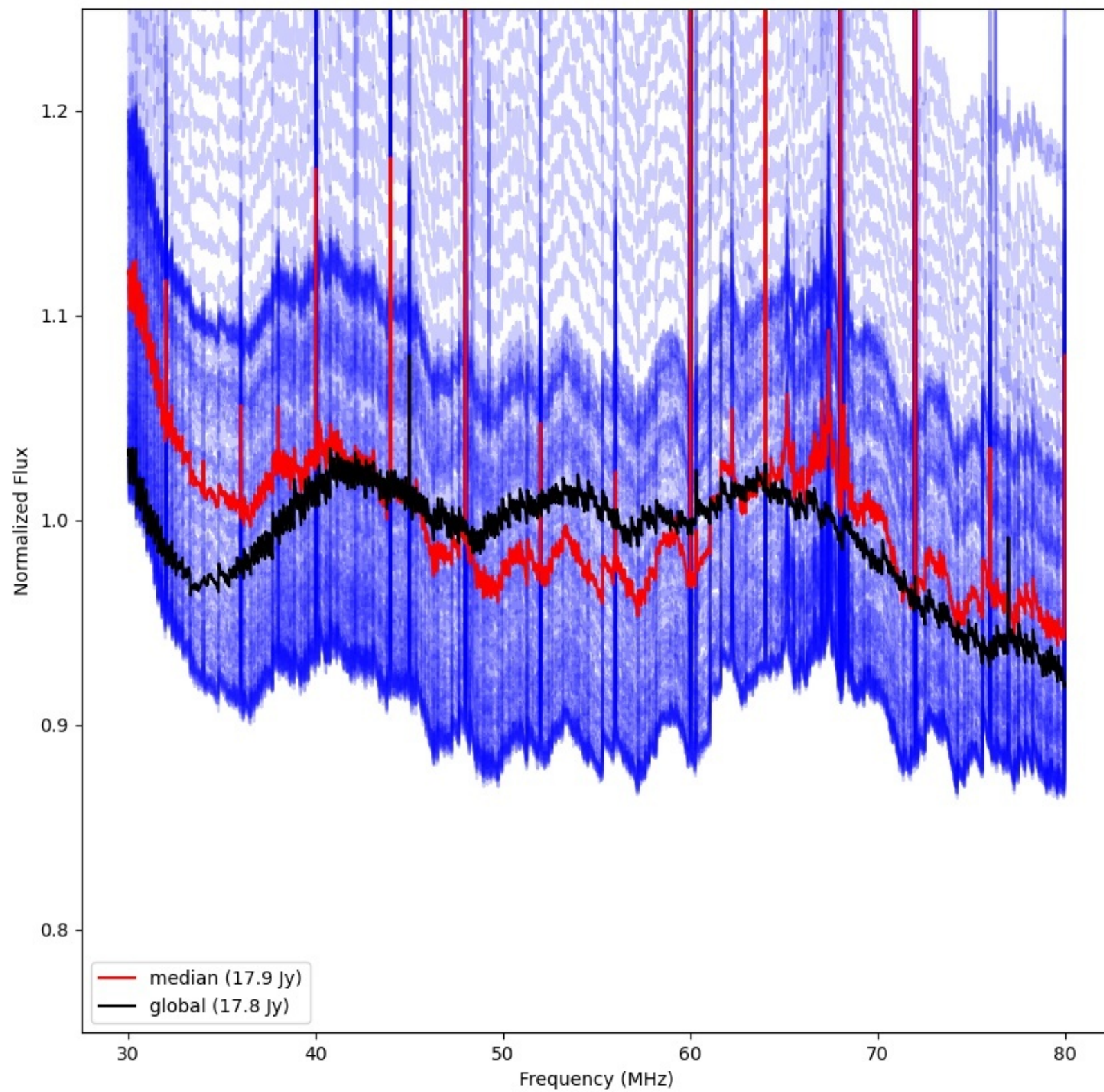
LWA160 - Correlator# 239 - XX - FLAGS:Good
