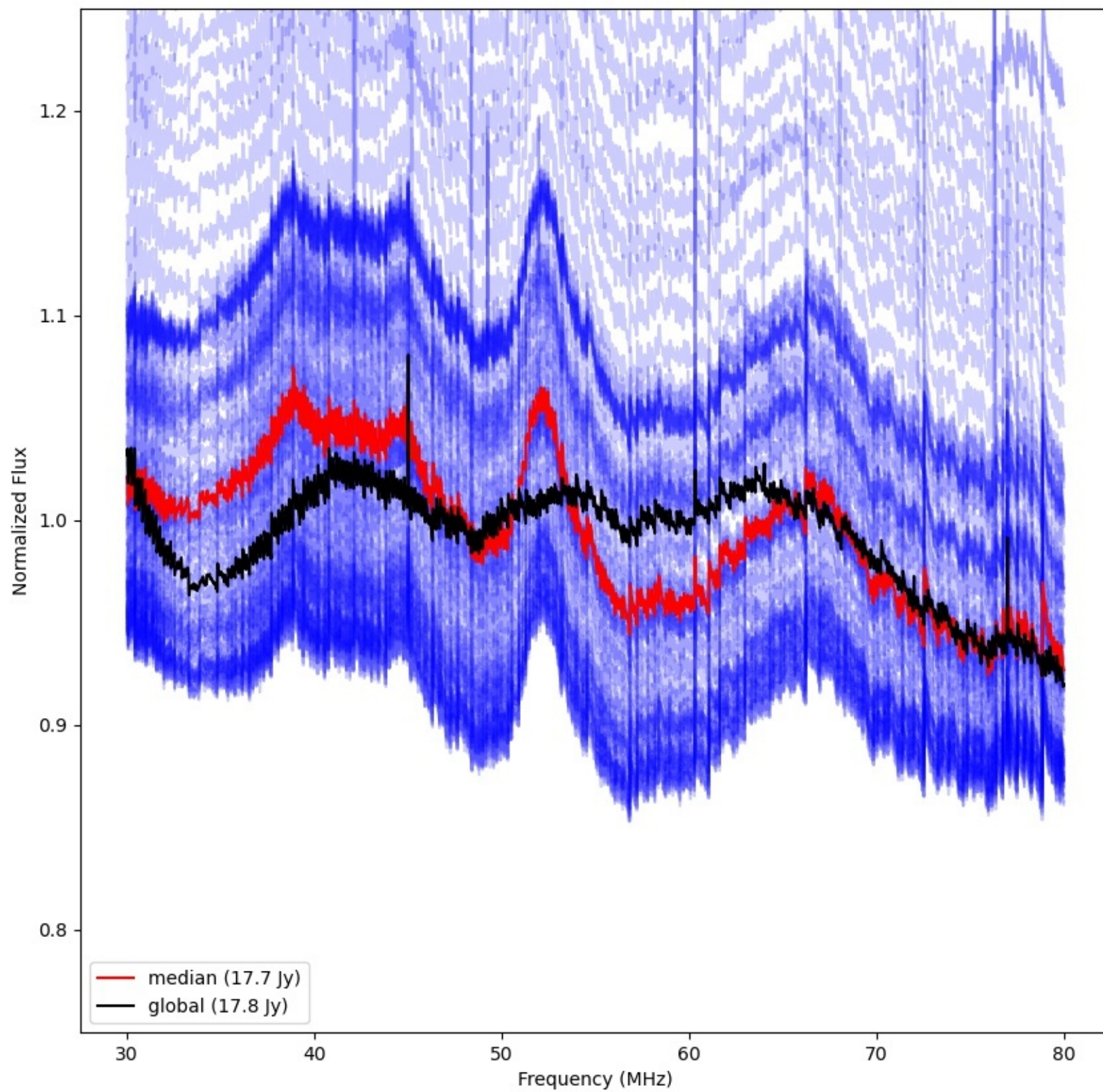
LWA227 - Correlator# 280 - XX - FLAGS:Good
