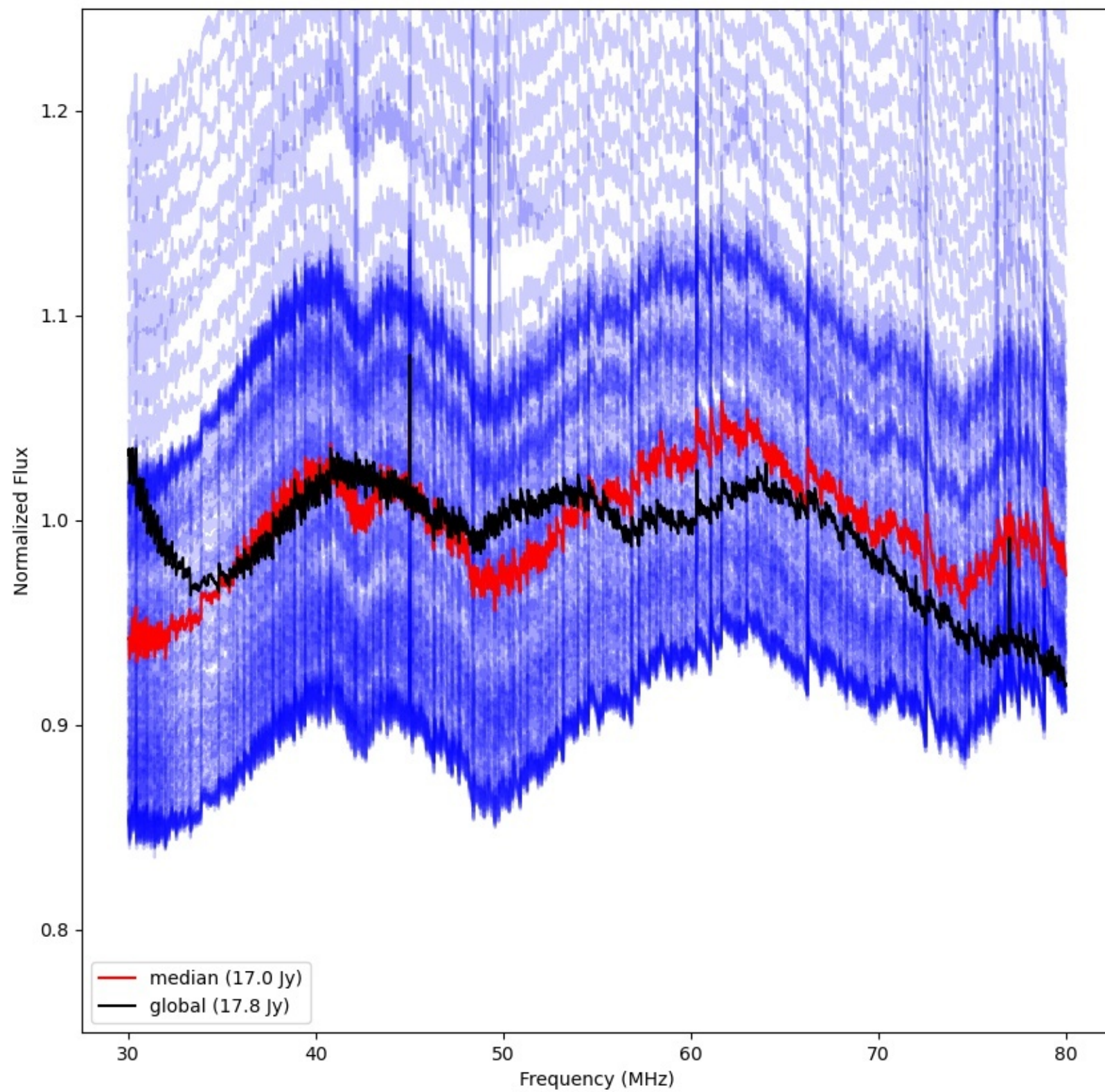
LWA011 - Correlator# 072 - XX - FLAGS:Good
