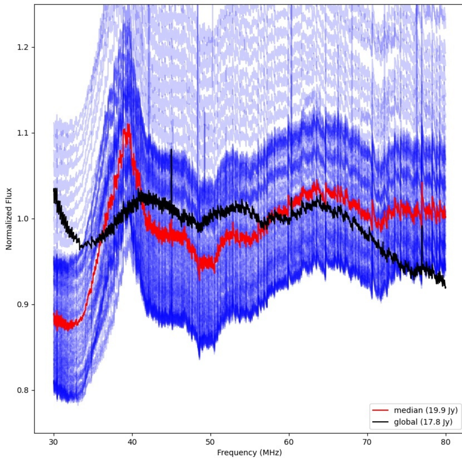
LWA097 - Correlator# 170 - XX - FLAGS:Good
