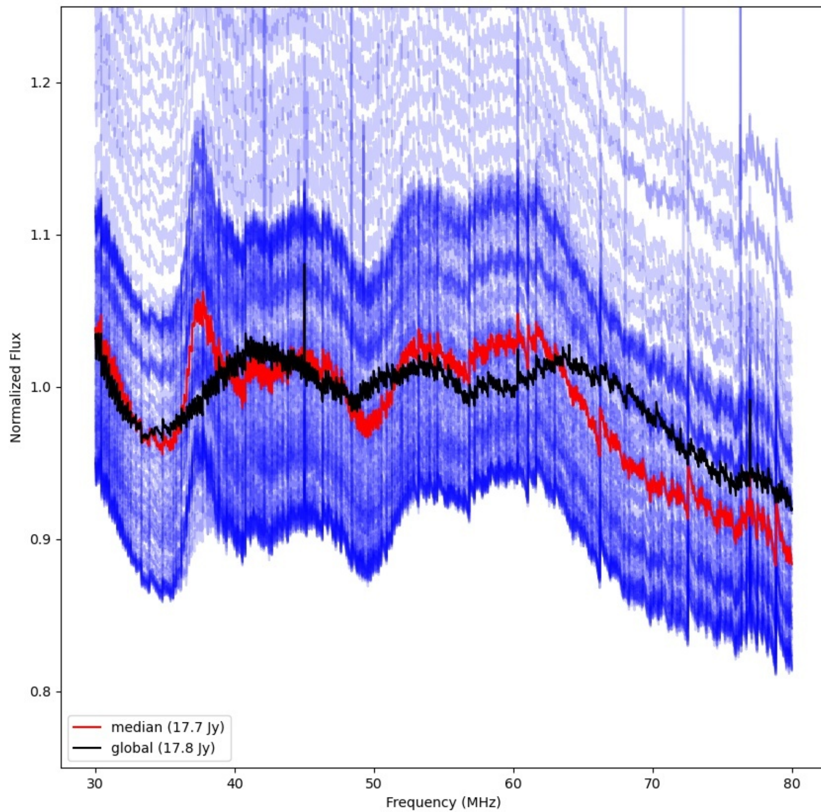
LWA036 - Correlator# 163 - XX - FLAGS:Good
