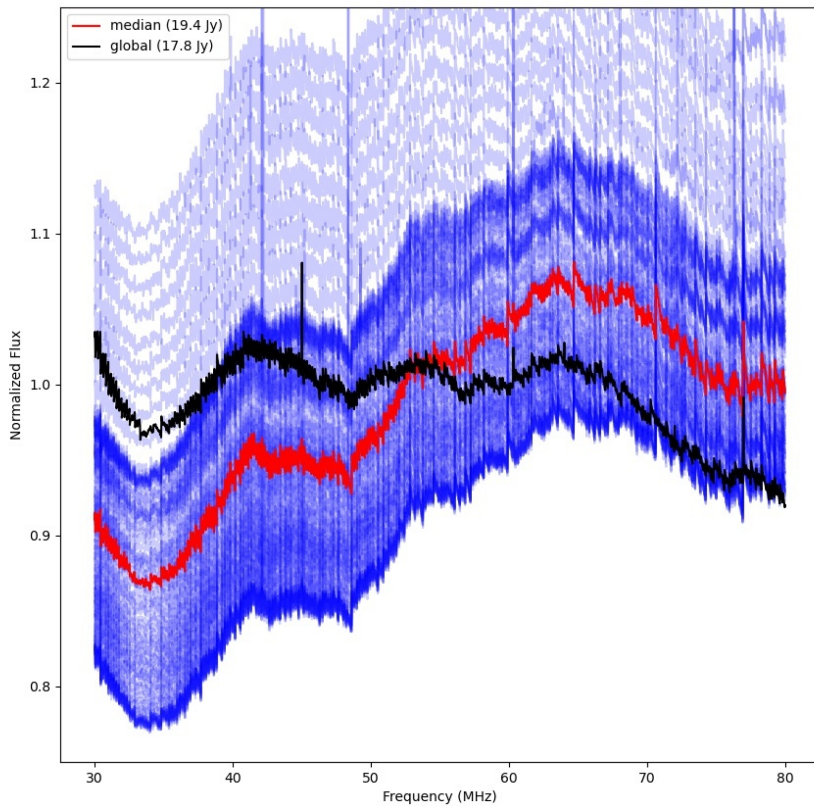
LWA066 - Correlator# 164 - XX - FLAGS:Good
