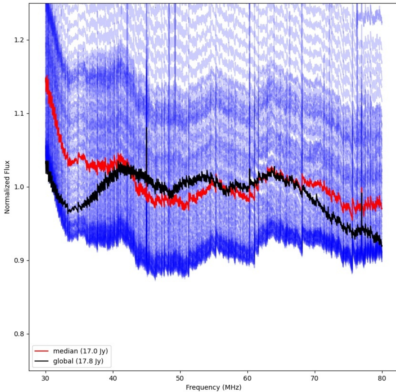
LWA287 - Correlator# 223 - XX - FLAGS:Good
