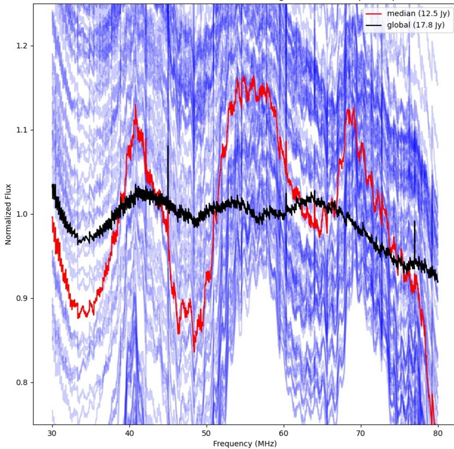
LWA120 - Correlator# 208 - XX - FLAGS:HighTimeVar+BadSpecShape
