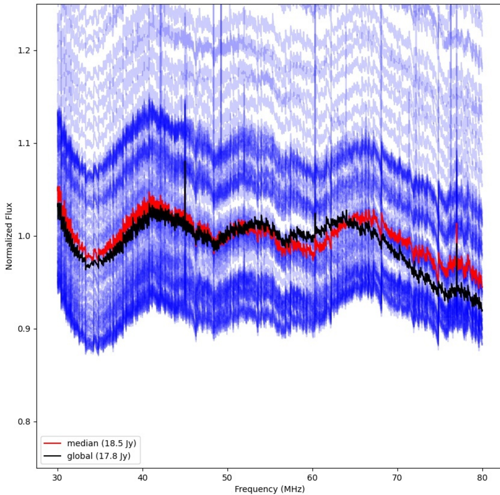
LWA142 - Correlator# 211 - XX - FLAGS:Good
