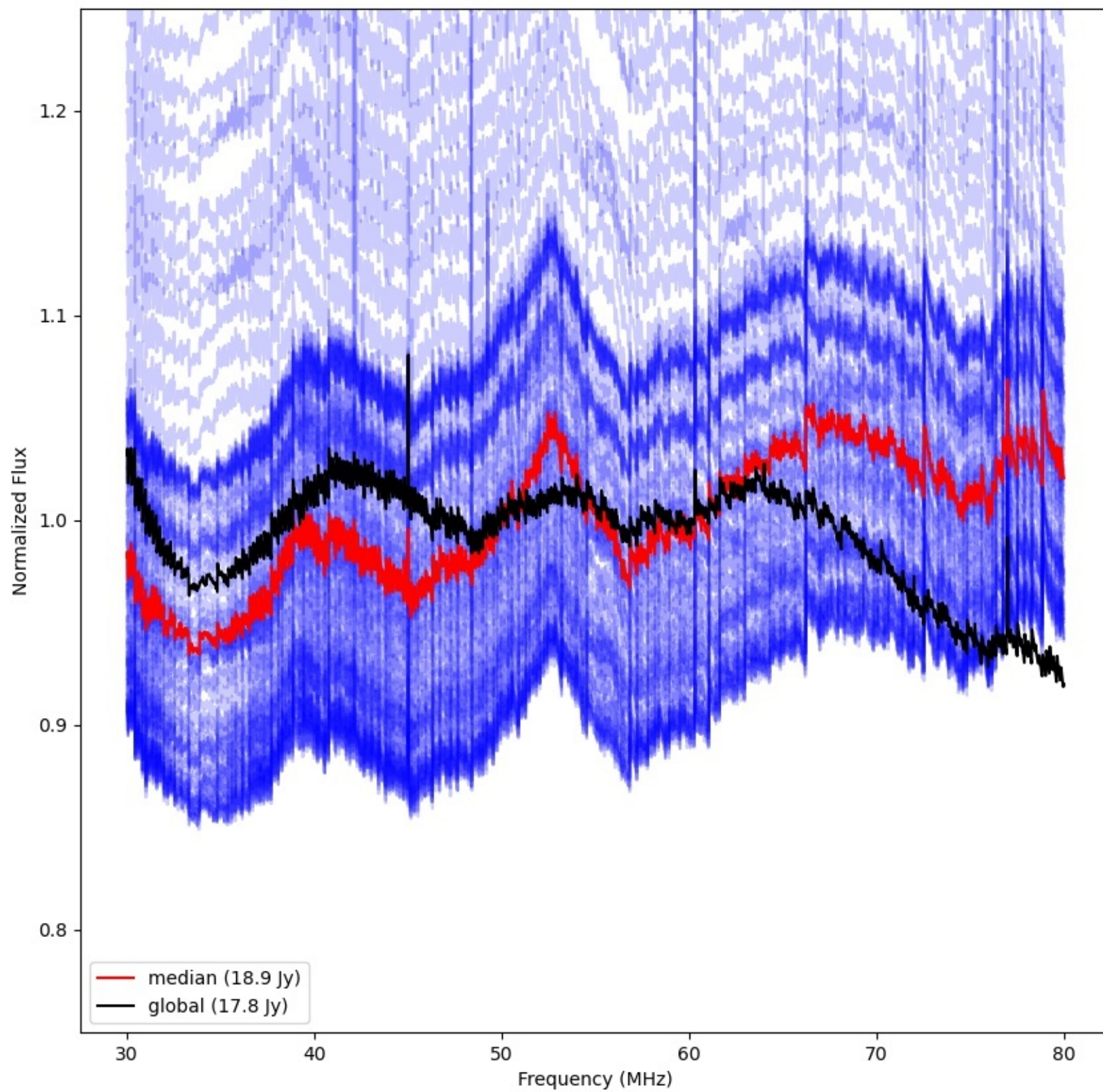
LWA203 - Correlator# 295 - XX - FLAGS:Good
