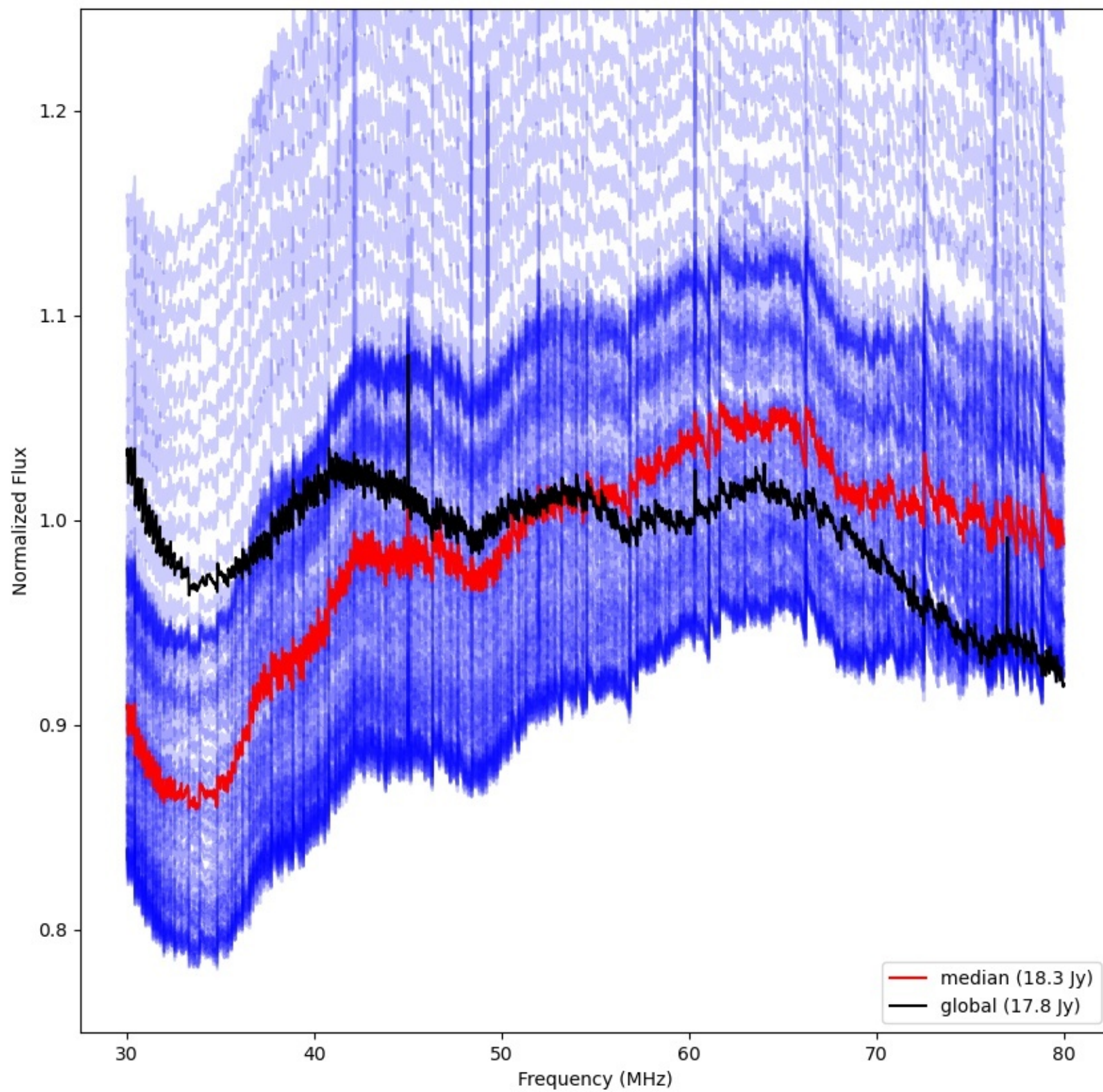
LWA099 - Correlator# 172 - XX - FLAGS:Good
