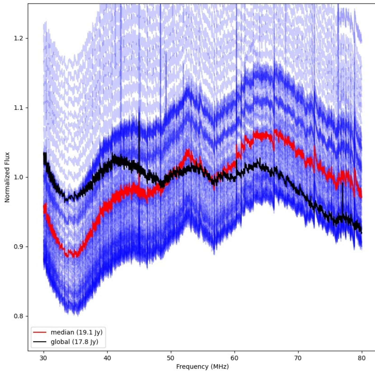
LWA202 - Correlator# 278 - XX - FLAGS:Good
