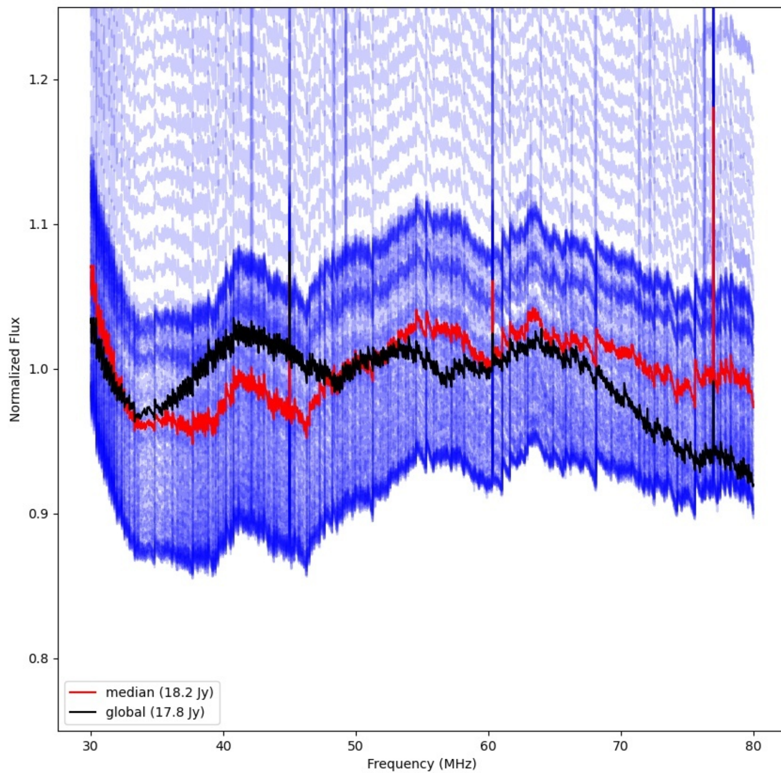
LWA282 - Correlator# 010 - XX - FLAGS:Good
