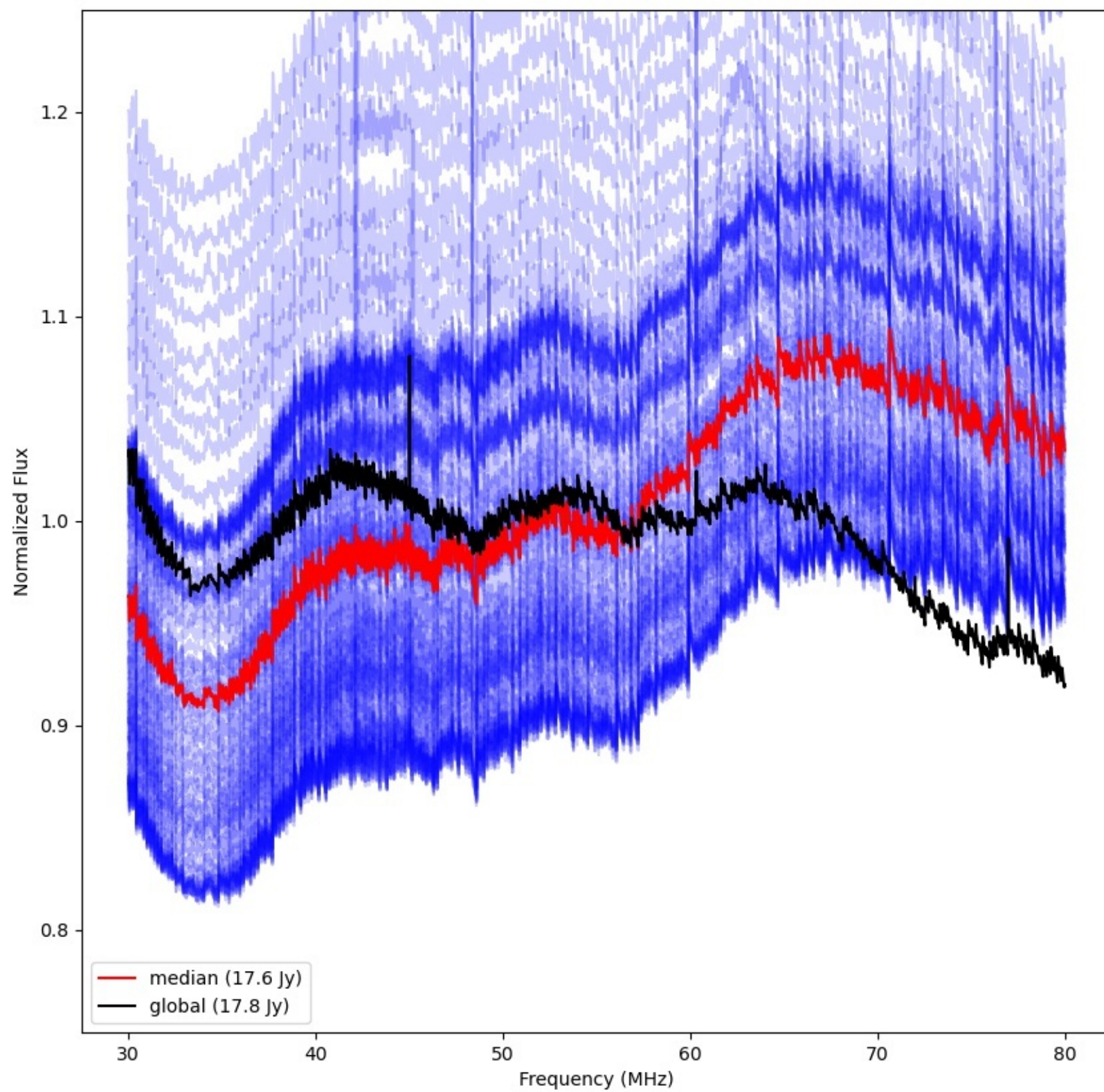
LWA194 - Correlator# 273 - XX - FLAGS:Good
