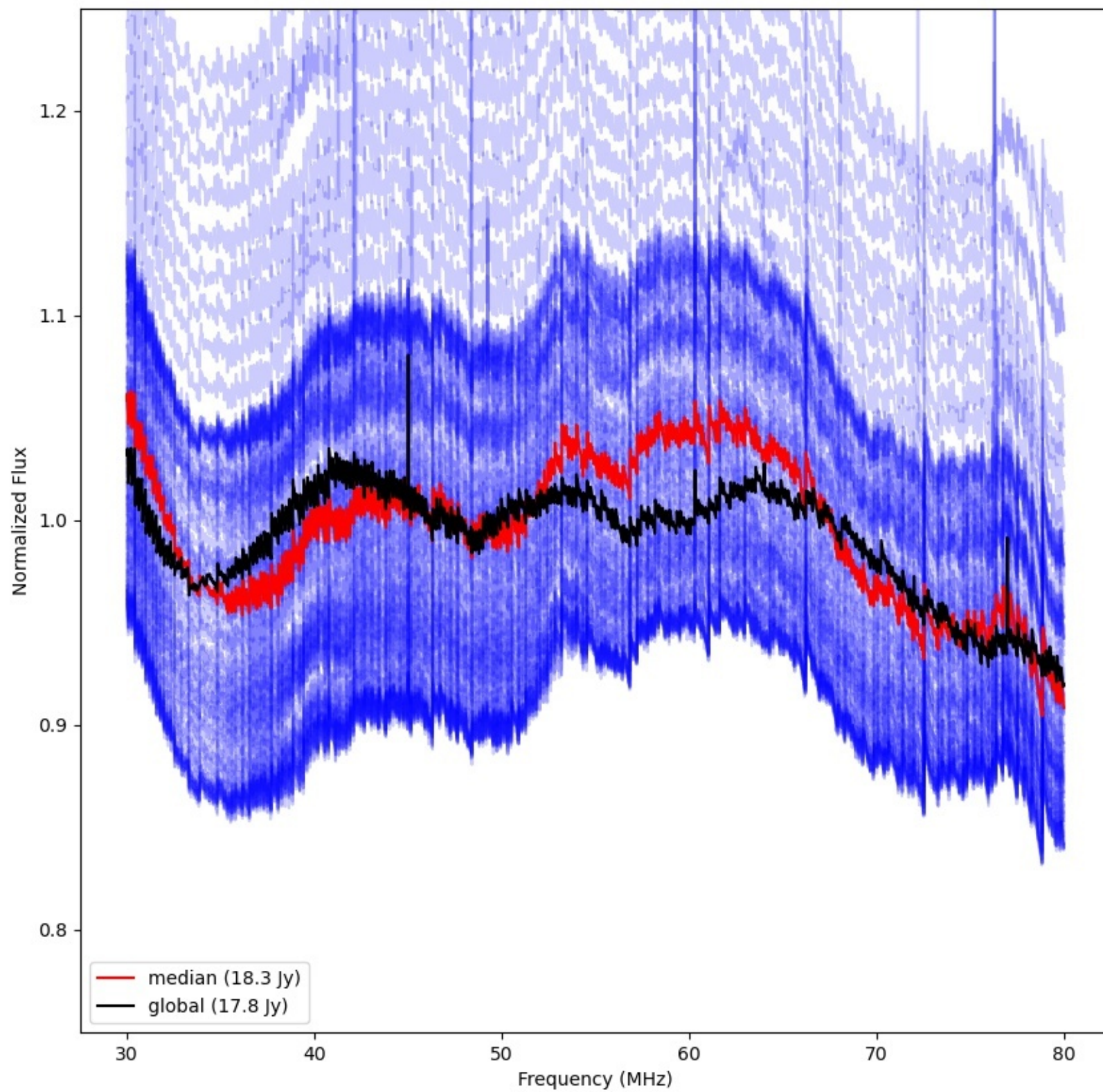
LWA068 - Correlator# 166 - XX - FLAGS:Good
