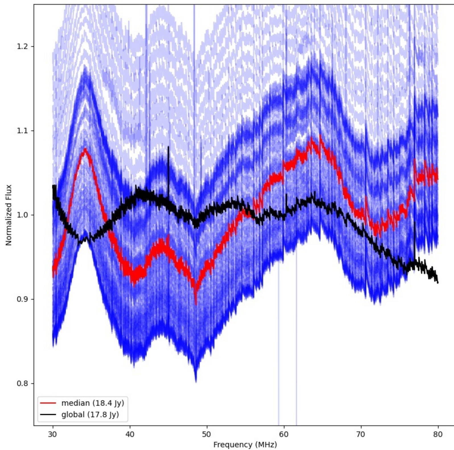
LWA001 - Correlator# 065 - XX - FLAGS:Good
