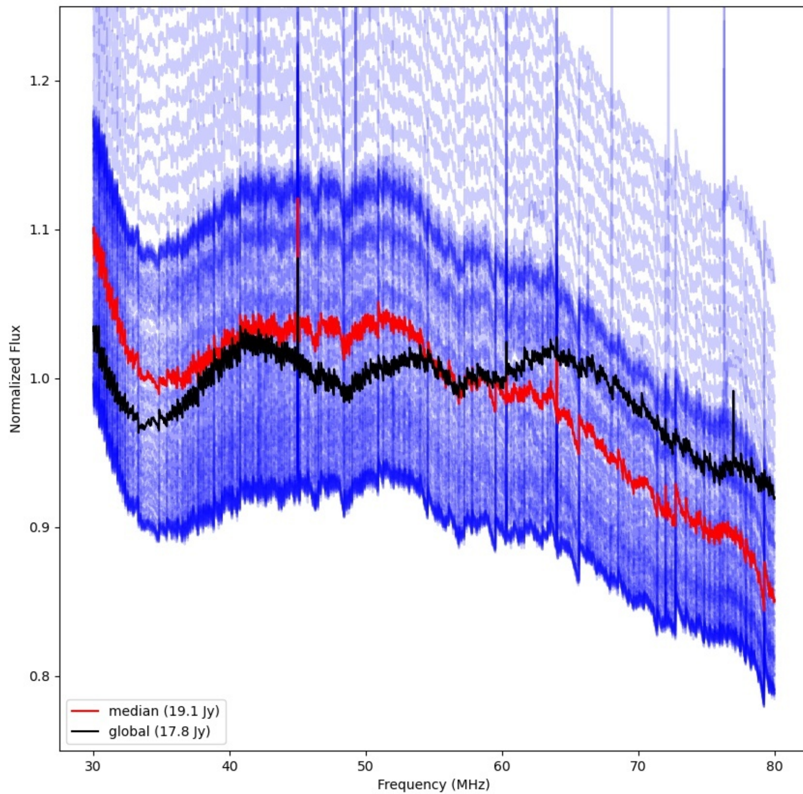
LWA059 - Correlator# 136 - XX - FLAGS:Good
