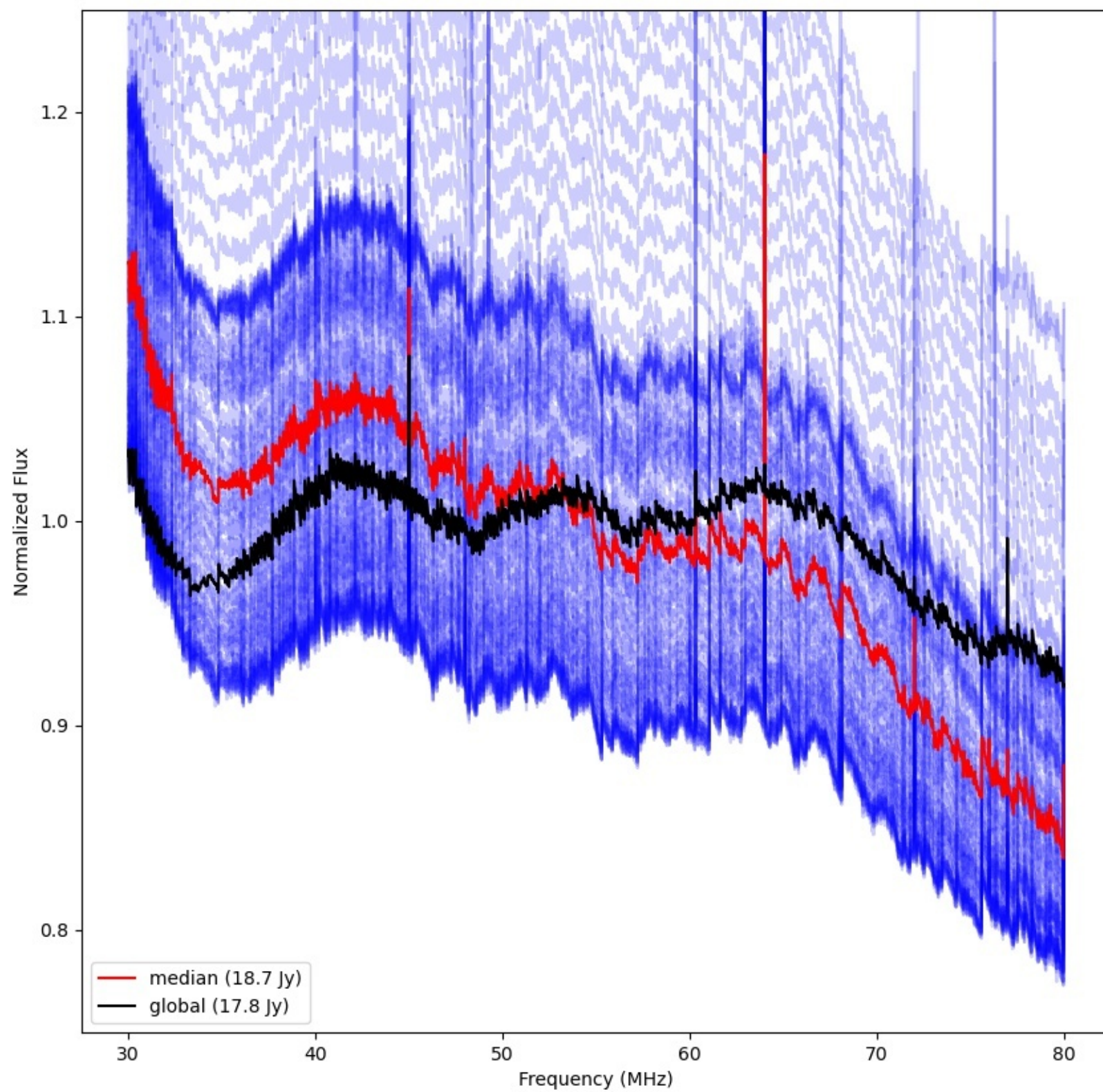
LWA126 - Correlator# 226 - XX - FLAGS:Good
