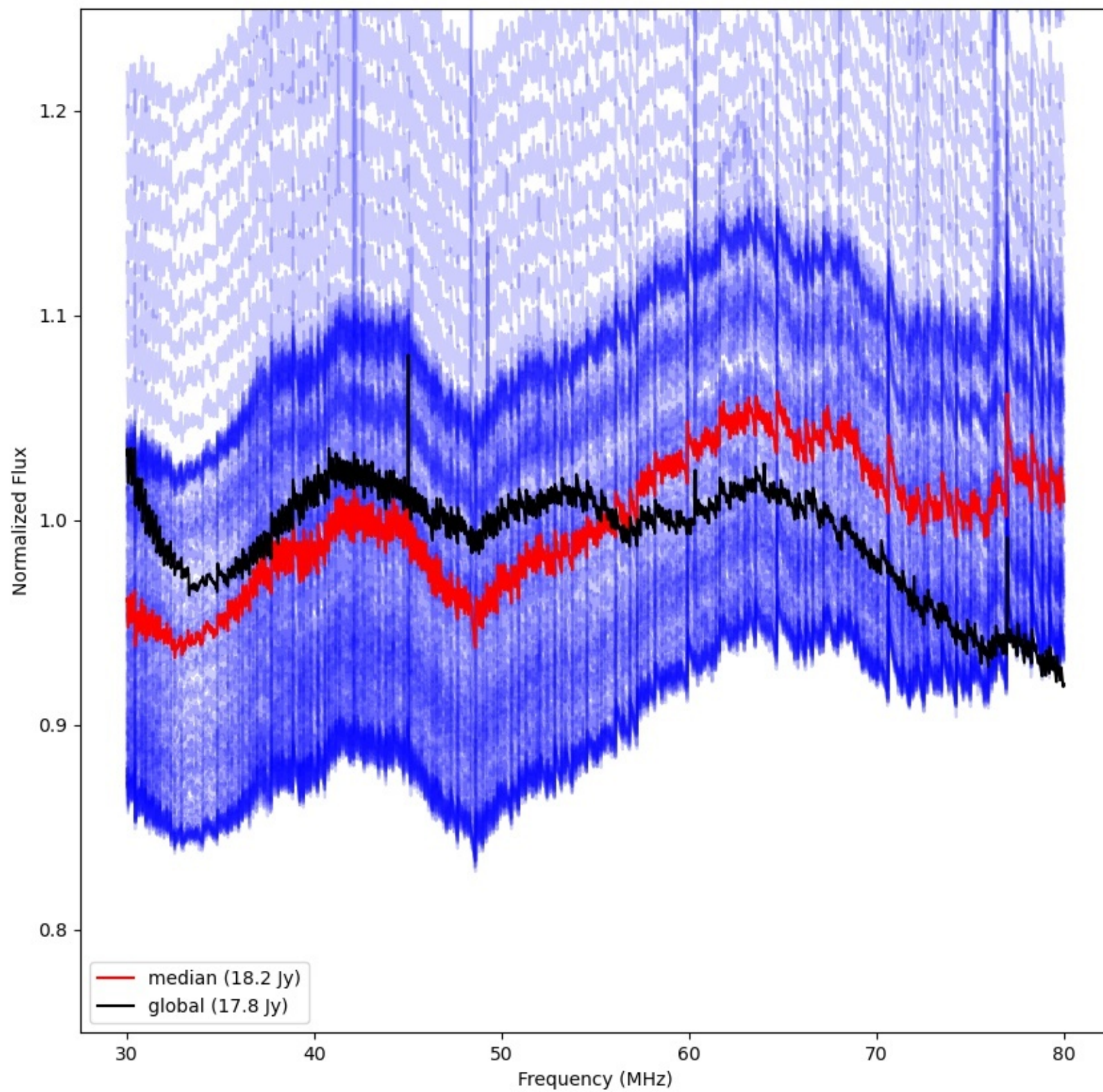
LWA034 - Correlator# 162 - XX - FLAGS:Good
