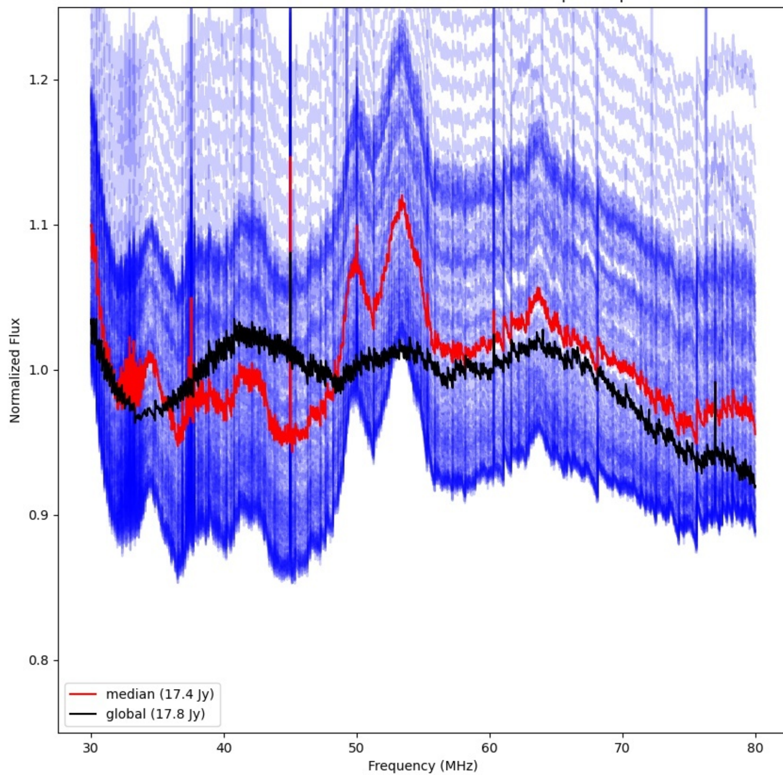
LWA280 - Correlator# 041 - XX - FLAGS:BadSpecShape
