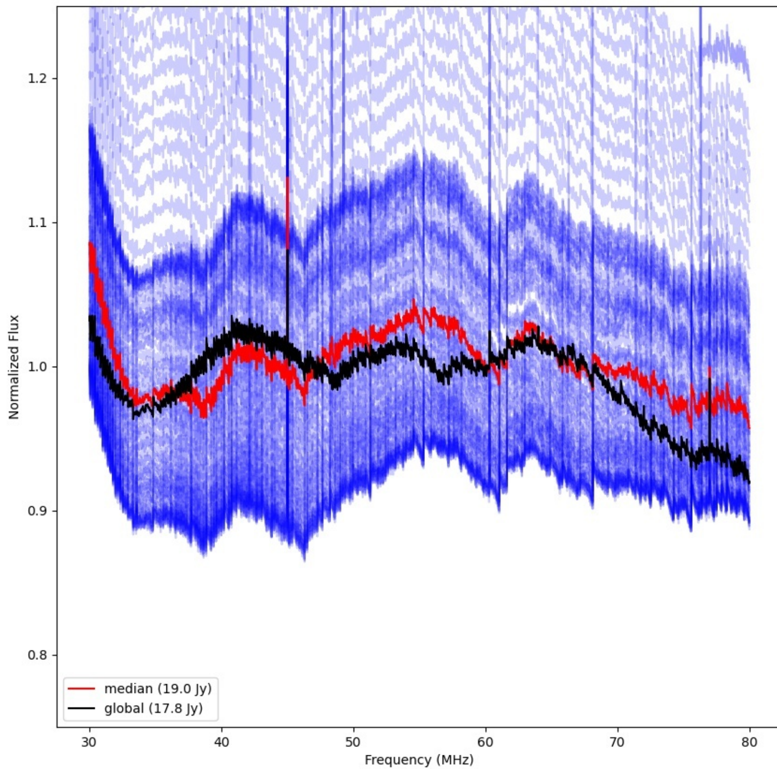
LWA268 - Correlator# 002 - XX - FLAGS:Good
