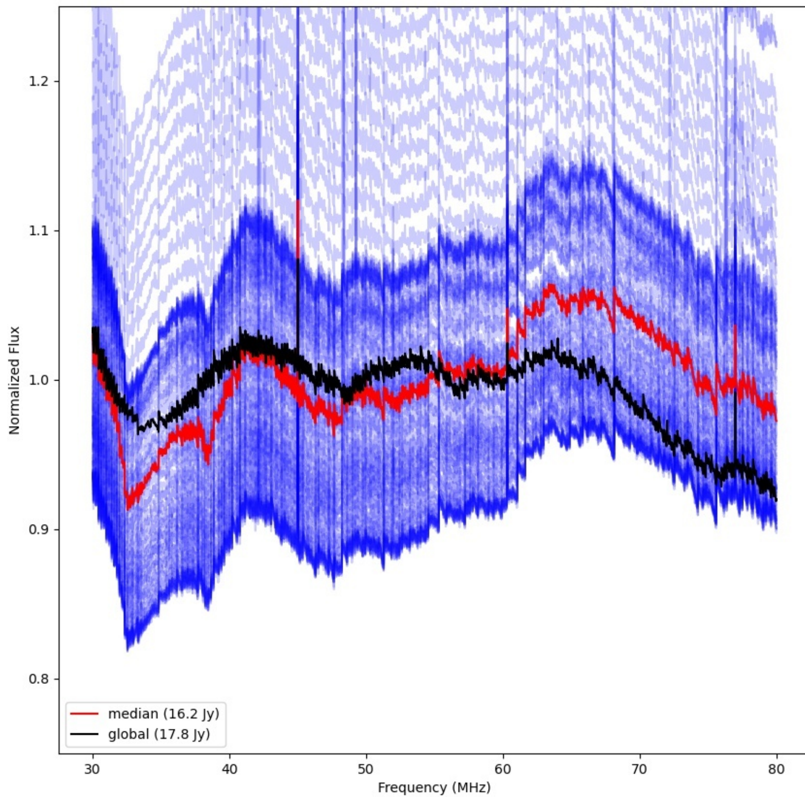
LWA331 - Correlator# 125 - XX - FLAGS:Good
