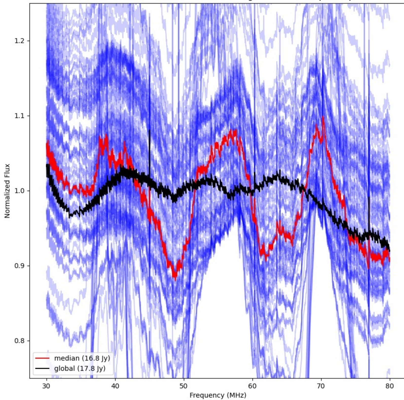
LWA151 - Correlator# 218 - XX - FLAGS:HighTimeVar+BadSpecShape
