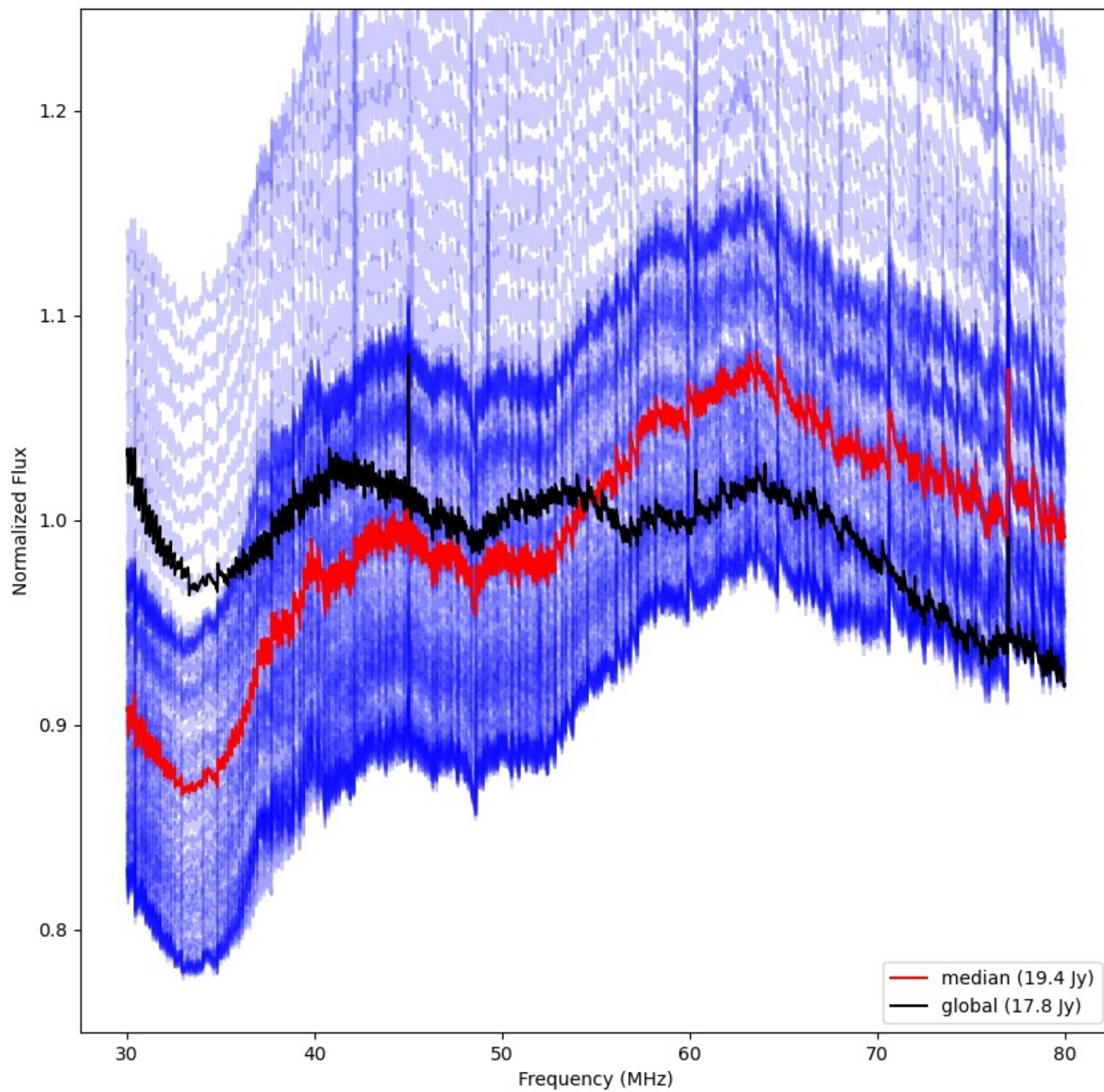
LWA065 - Correlator# 165 - XX - FLAGS:Good
