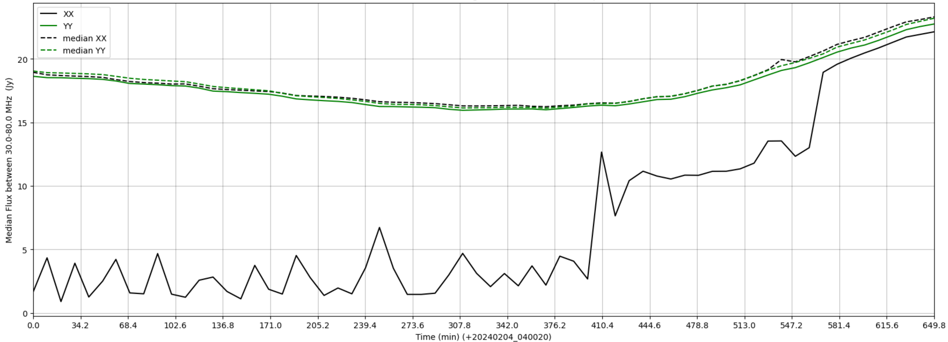
LWA353 - Correlator# 031 - XX FLAGS:HighTimeVar+BadSpecShape - YY FLAGS:Good
