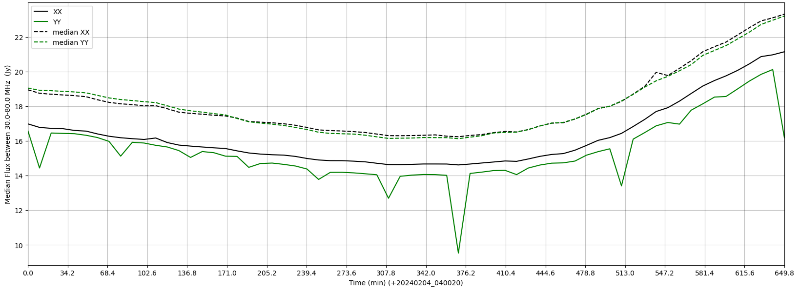
LWA323 - Correlator# 095 - XX FLAGS:Good - YY FLAGS:HighTimeVar
