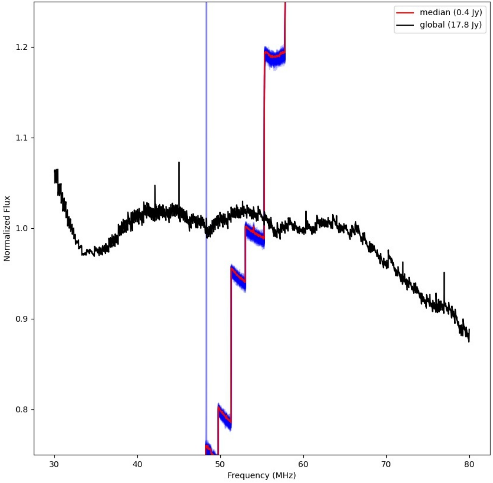
LWA316 - Correlator# 155 - XX - FLAGS:LowFlux
