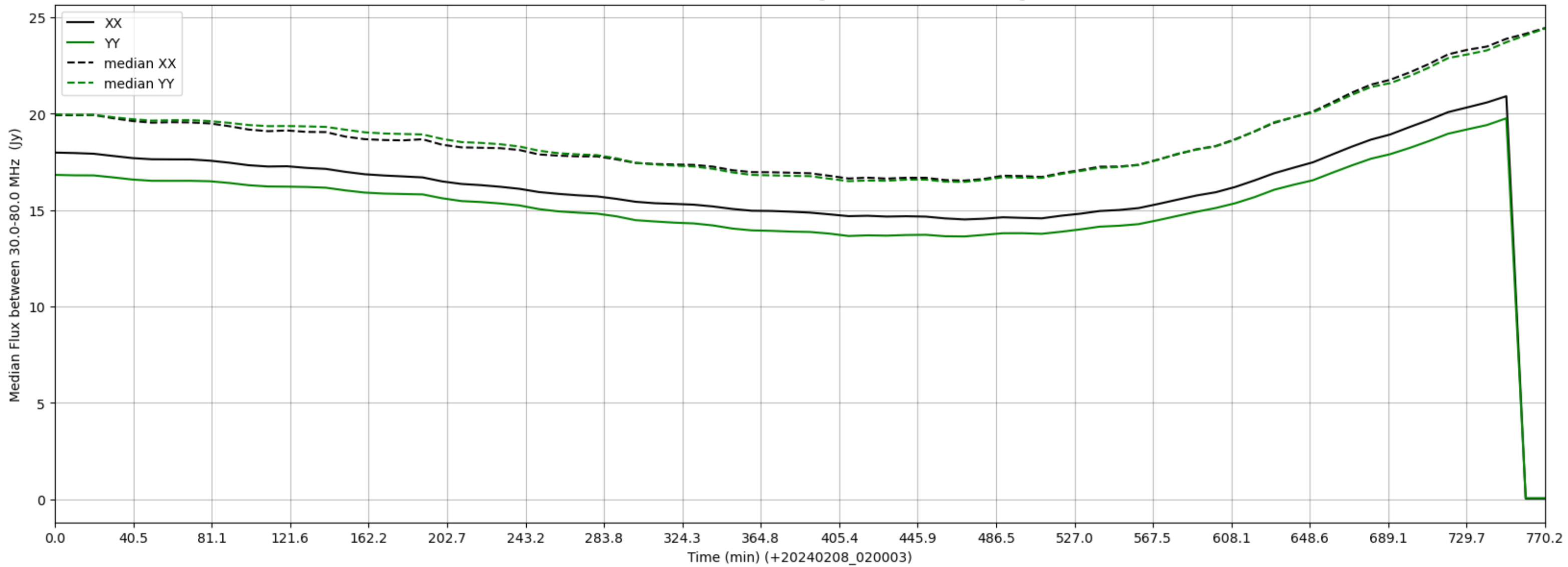
LWA274 - Correlator# 091 - XX FLAGS:HighTimeVar - YY FLAGS:HighTimeVar
