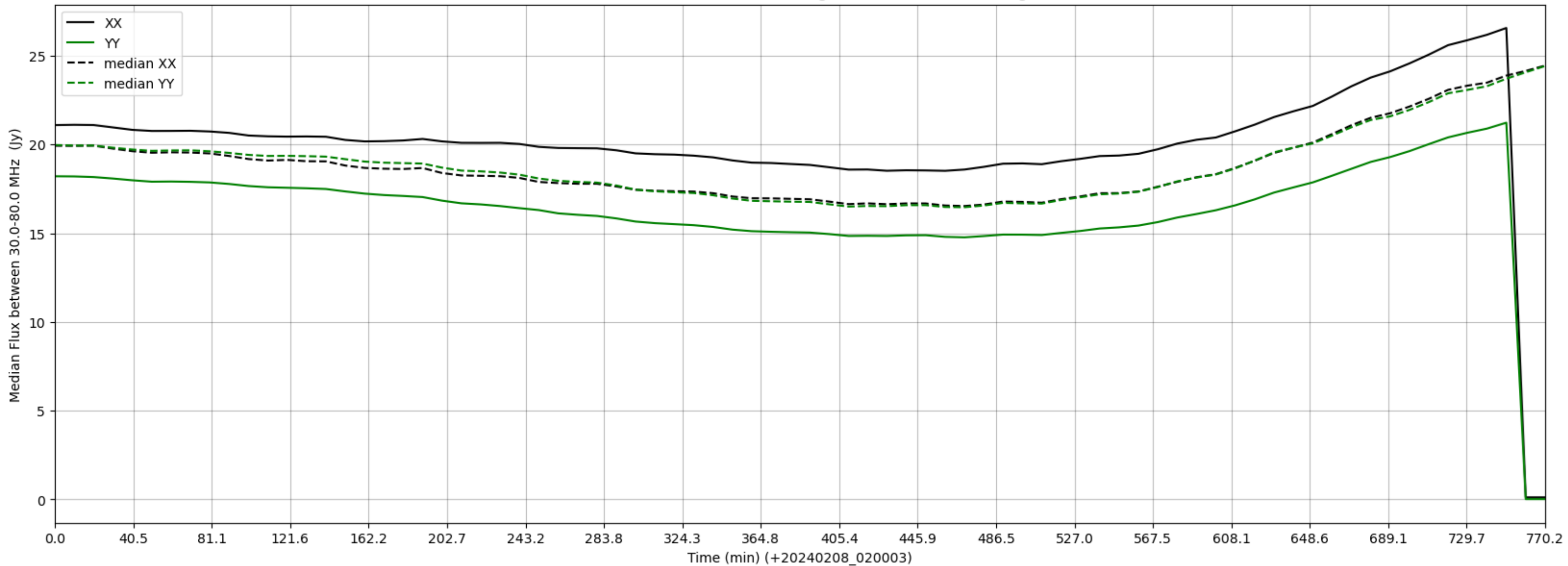
LWA306 - Correlator# 053 - XX FLAGS:HighTimeVar - YY FLAGS:HighTimeVar
