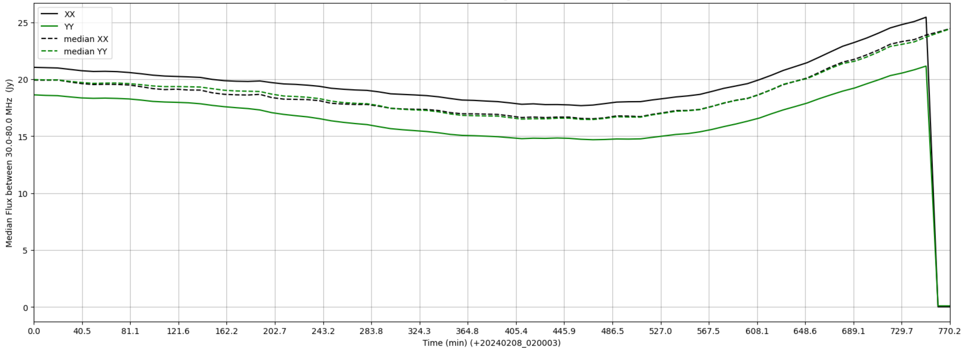
LWA304 - Correlator# 351 - XX FLAGS:HighTimeVar - YY FLAGS:HighTimeVar
