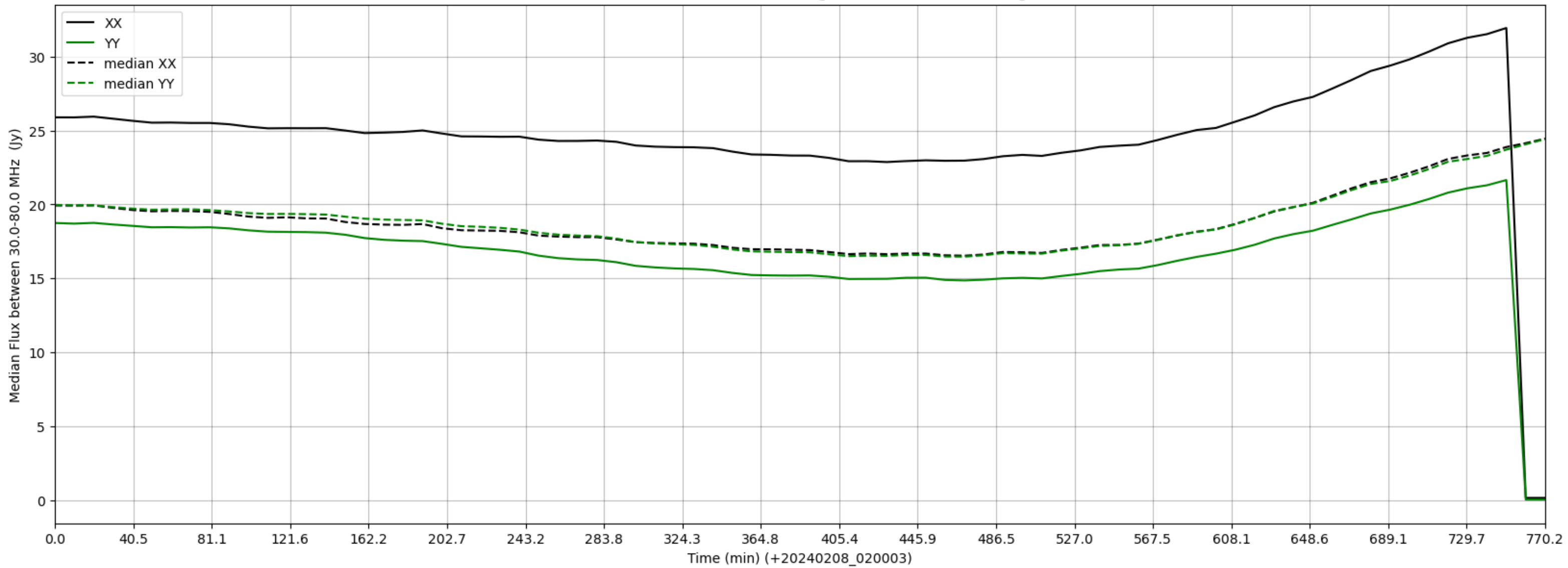
LWA301 - Correlator# 048 - XX FLAGS:HighTimeVar - YY FLAGS:HighTimeVar
