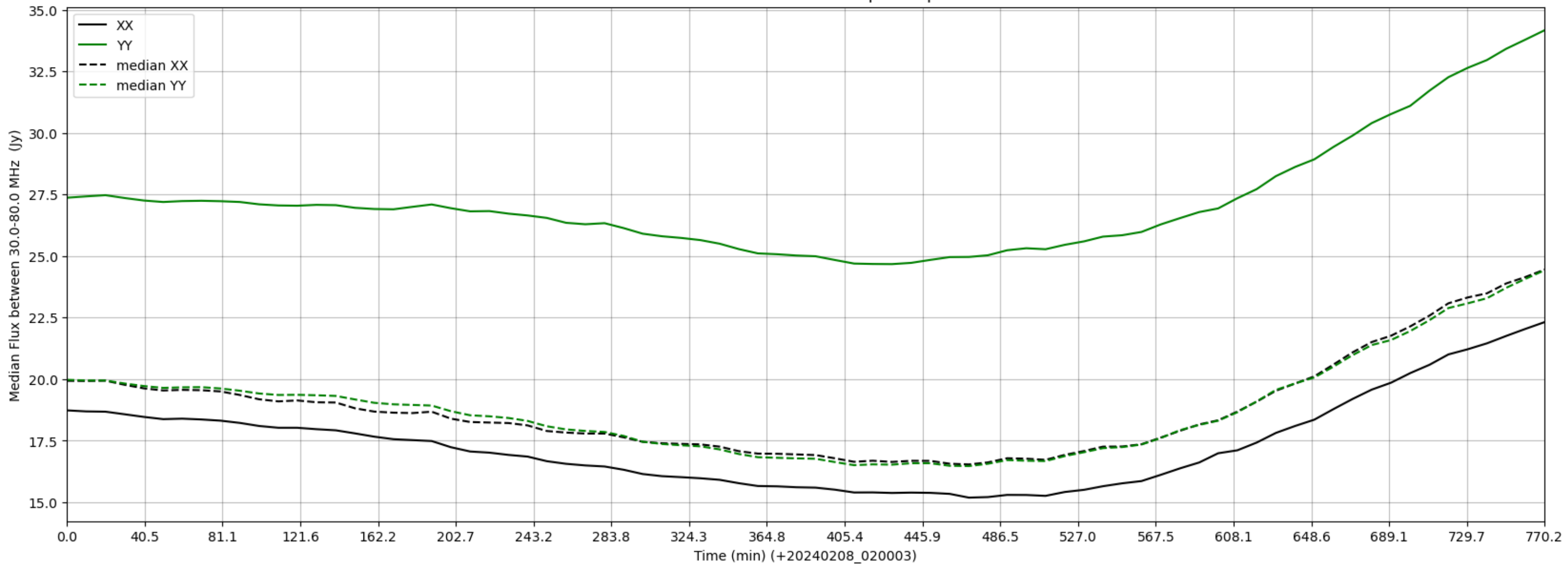
LWA296 - Correlator# 046 - XX FLAGS:BadSpecShape - YY FLAGS:Good
