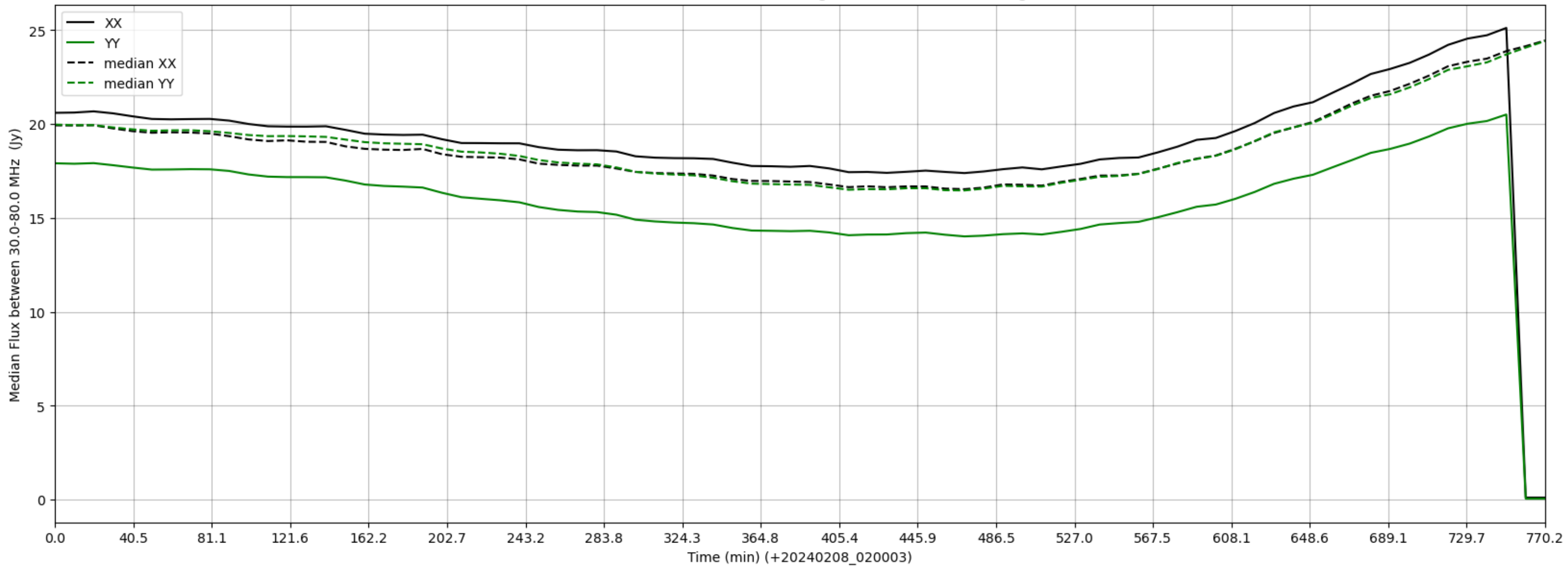
LWA361 - Correlator# 158 - XX FLAGS:HighTimeVar - YY FLAGS:HighTimeVar
