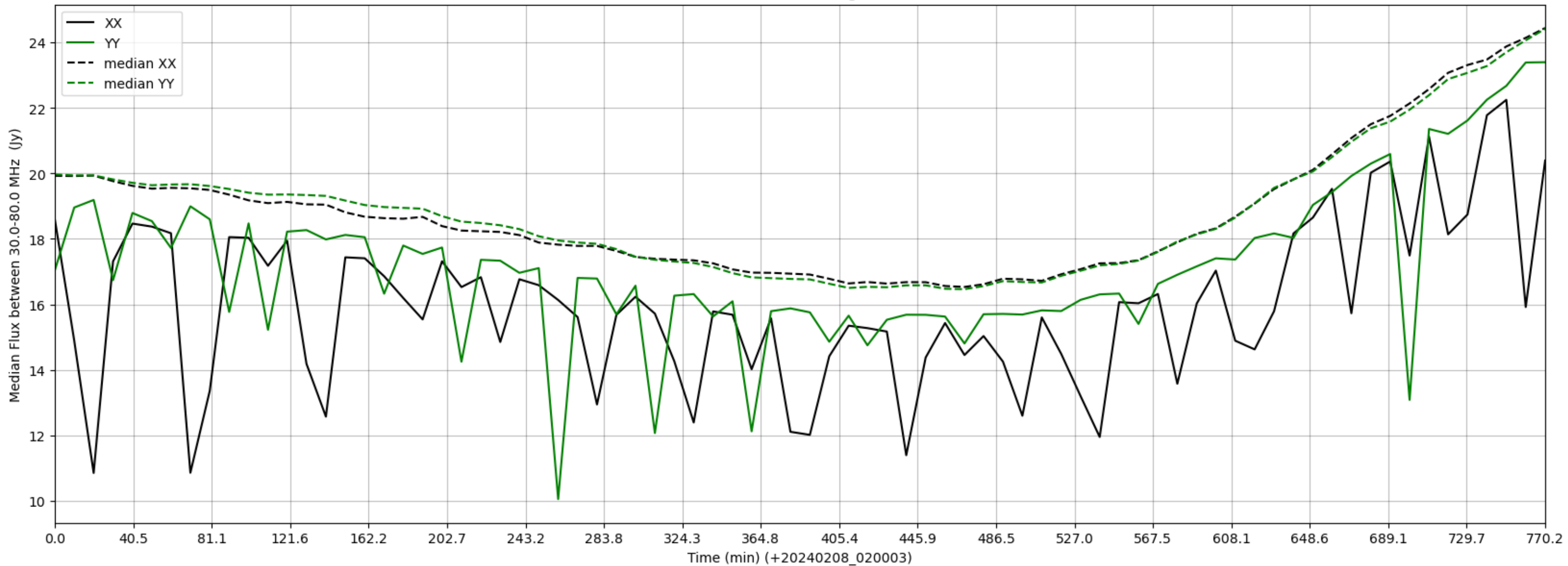
LWA120 - Correlator# 208 - XX FLAGS:HighTimeVar - YY FLAGS:Good
