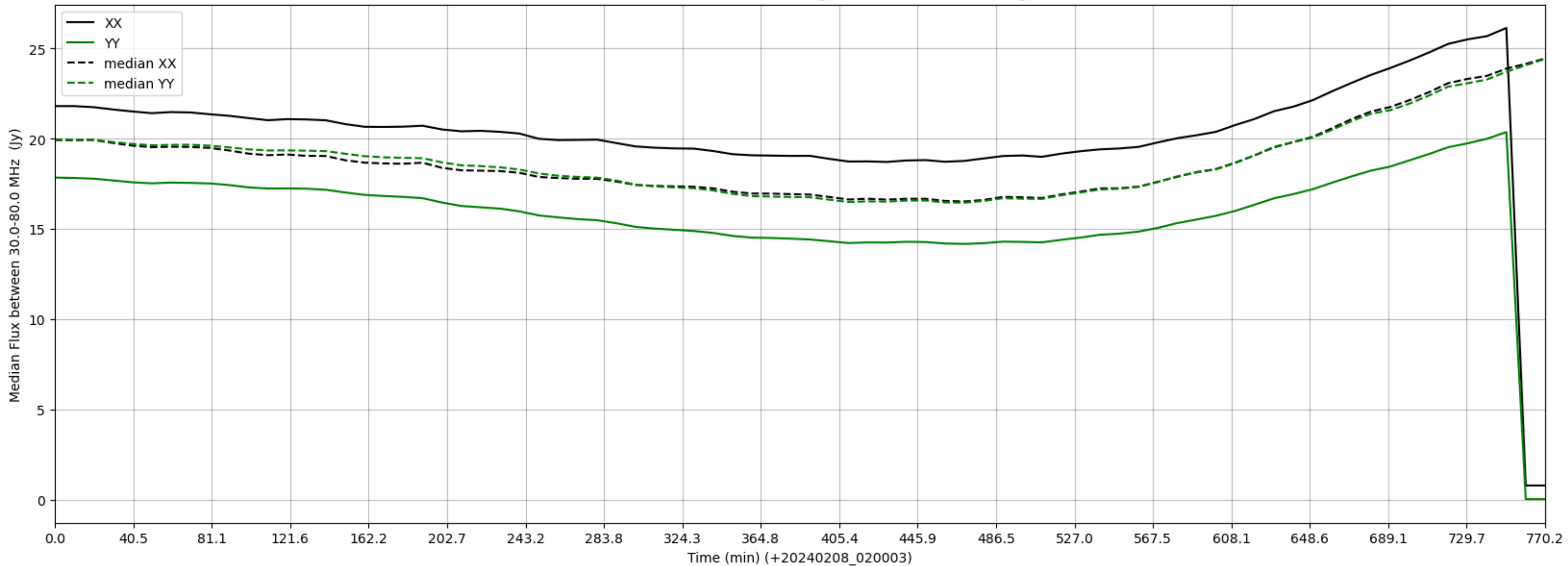
LWA318 - Correlator# 055 - XX FLAGS:HighTimeVar - YY FLAGS:HighTimeVar
