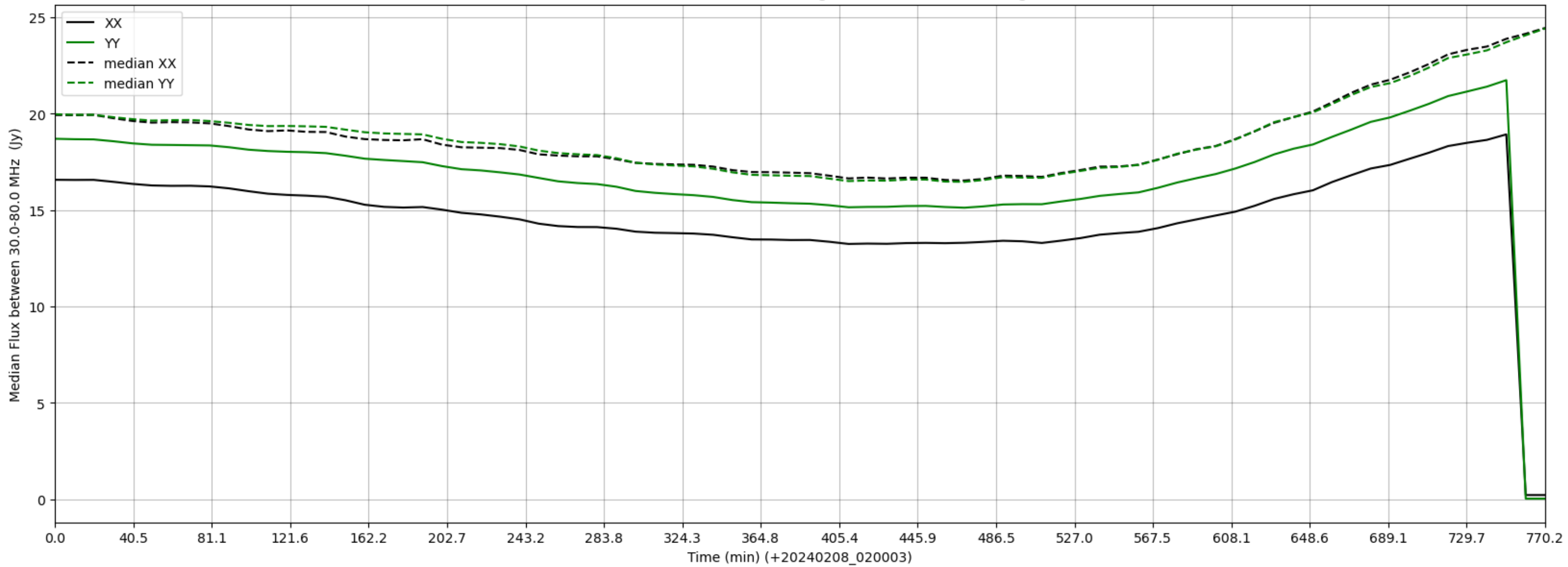
LWA305 - Correlator# 050 - XX FLAGS:HighTimeVar - YY FLAGS:HighTimeVar
