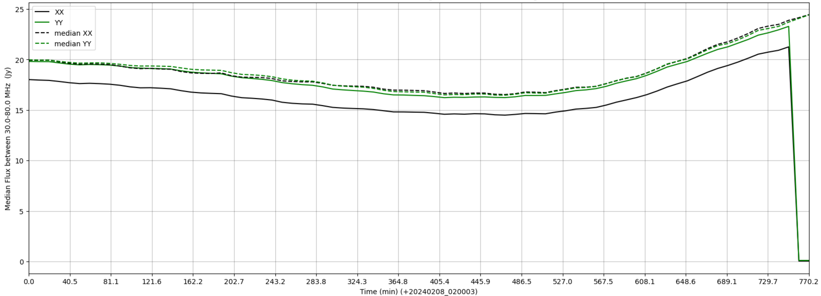
LWA265 - Correlator# 036 - XX FLAGS:HighTimeVar - YY FLAGS:HighTimeVar
