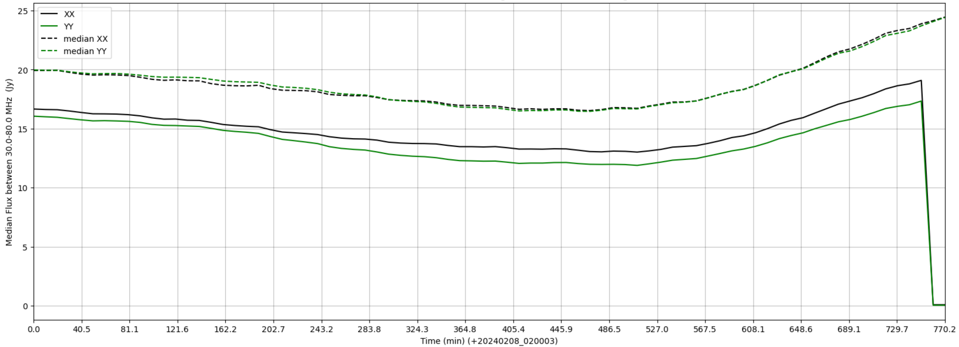
LWA293 - Correlator# 284 - XX FLAGS:HighTimeVar - YY FLAGS:HighTimeVar
