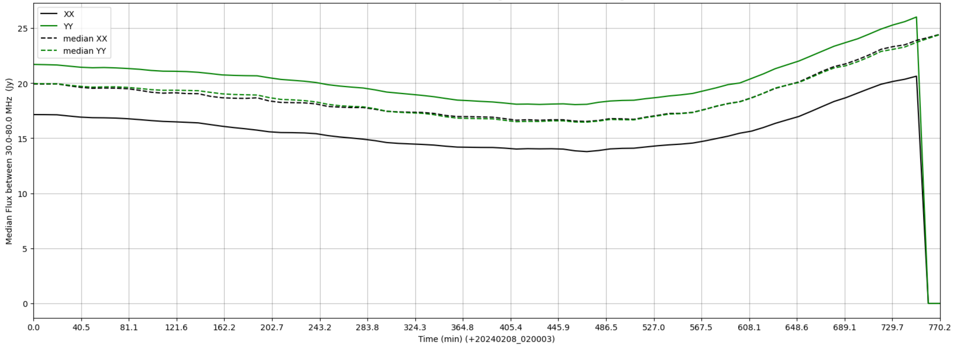
LWA346 - Correlator# 316 - XX FLAGS:HighTimeVar - YY FLAGS:HighTimeVar
