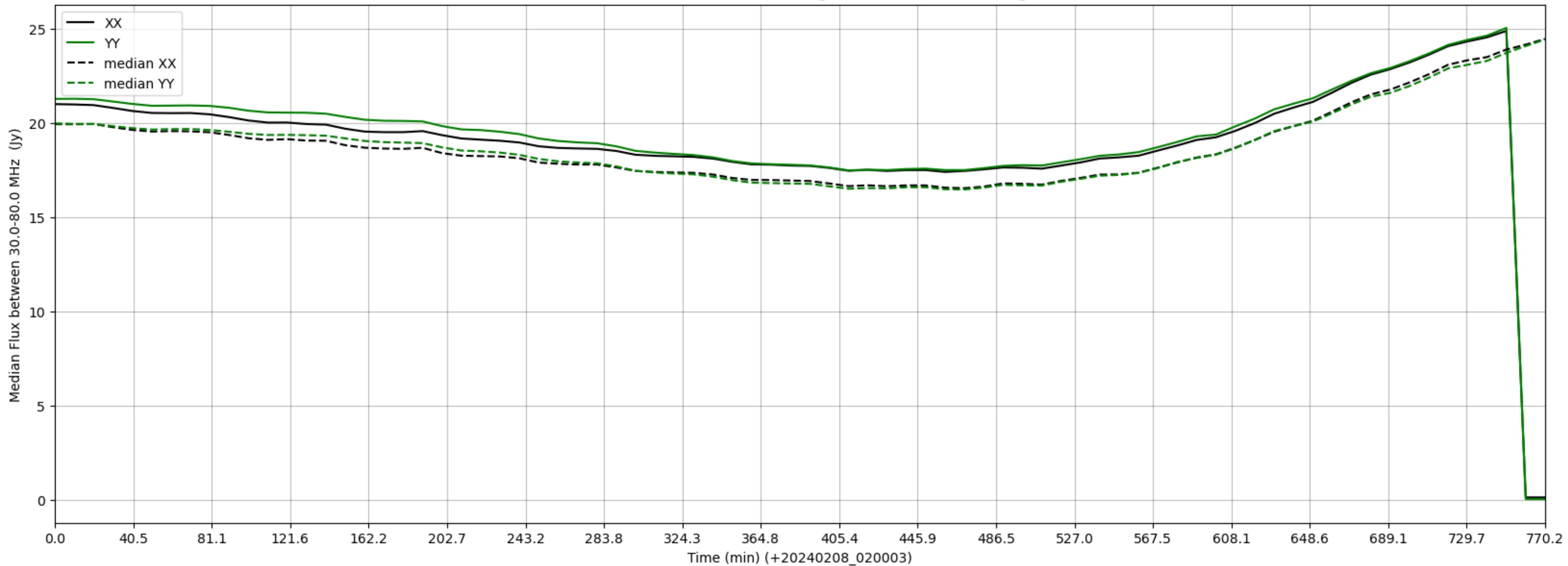
LWA324 - Correlator# 122 - XX FLAGS:HighTimeVar - YY FLAGS:HighTimeVar
