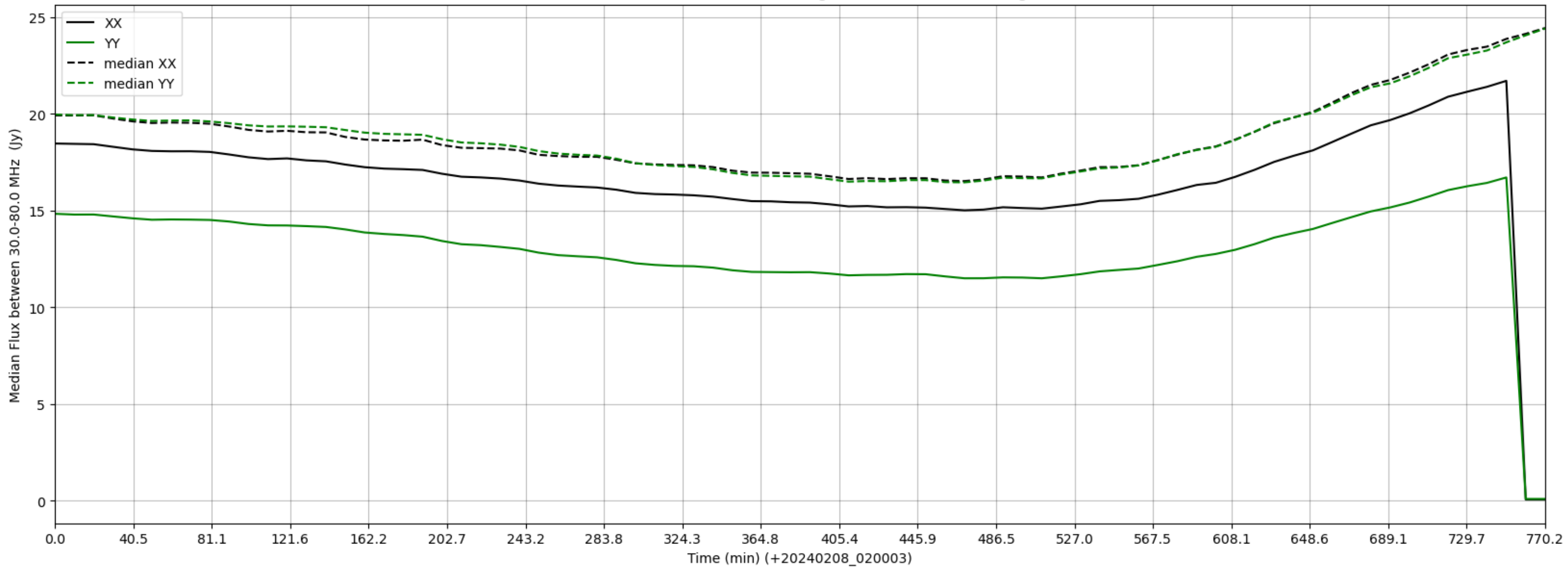
LWA262 - Correlator# 123 - XX FLAGS:HighTimeVar - YY FLAGS:HighTimeVar
