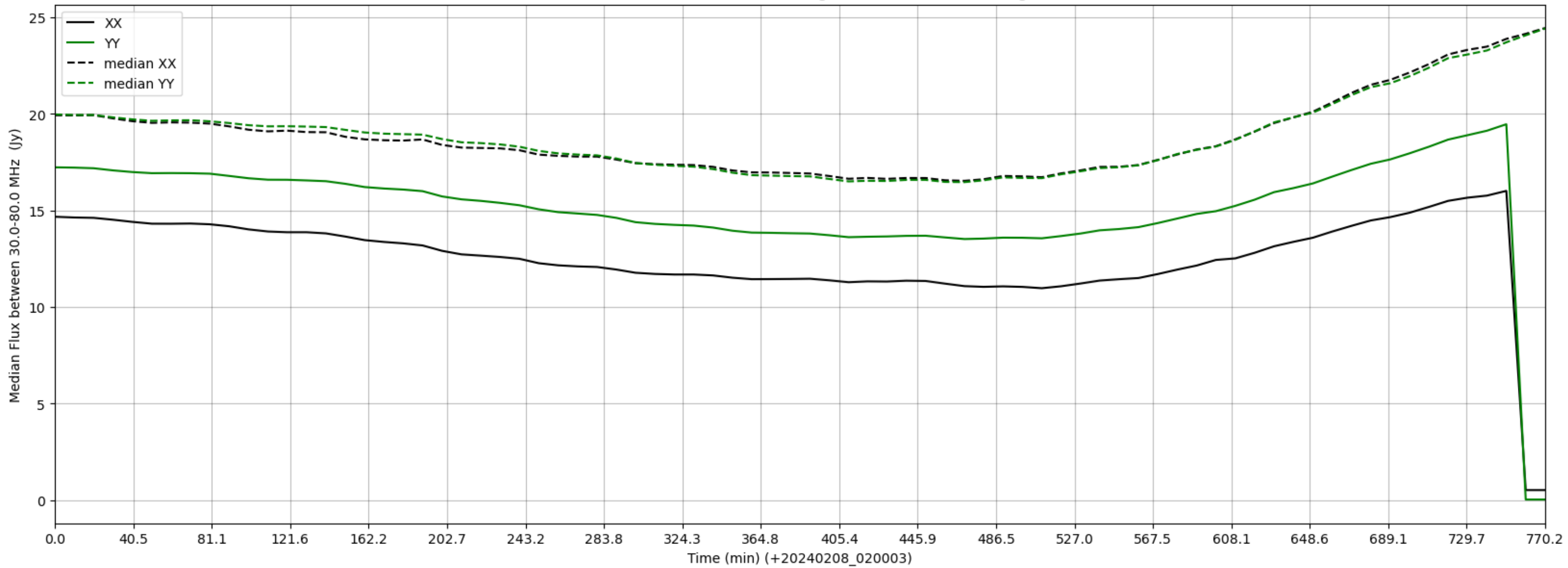
LWA363 - Correlator# 094 - XX FLAGS:HighTimeVar - YY FLAGS:HighTimeVar
