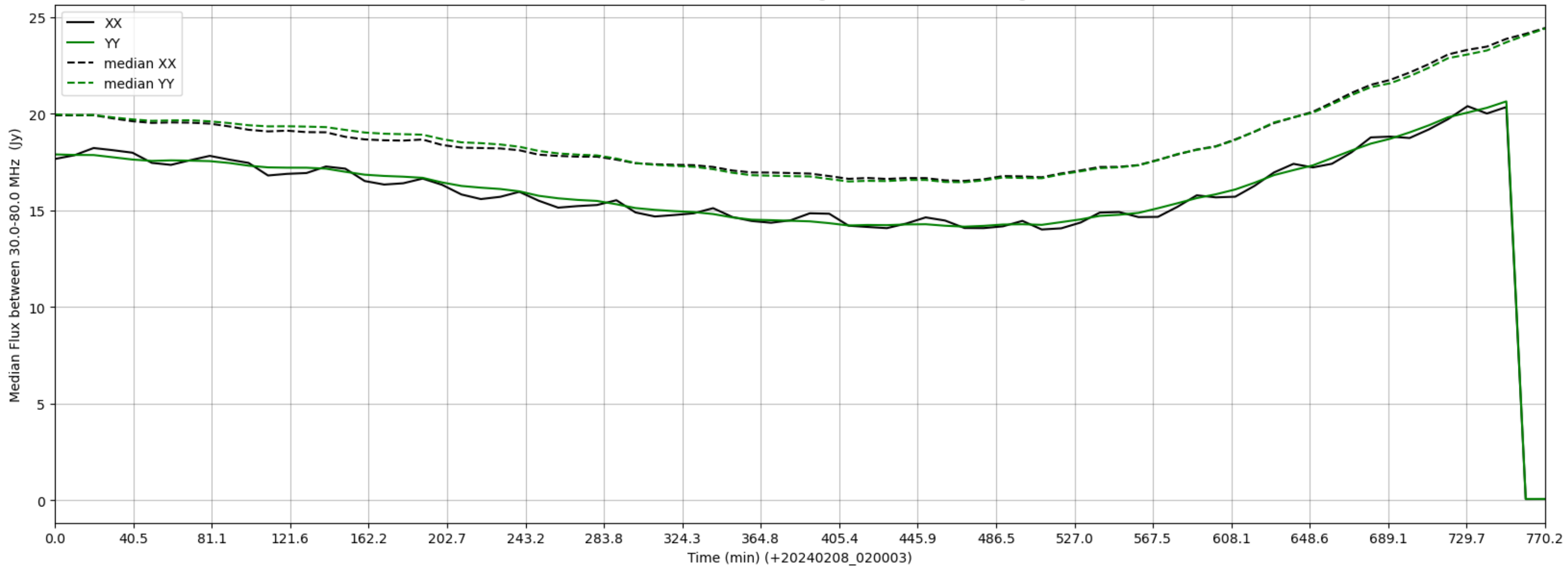
LWA299 - Correlator# 191 - XX FLAGS:HighTimeVar - YY FLAGS:HighTimeVar
