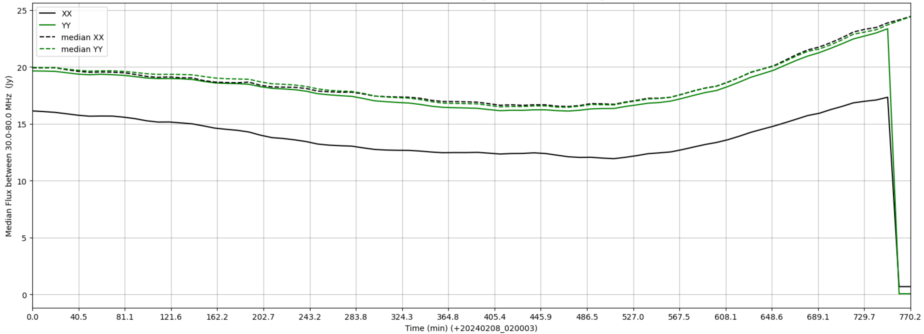
LWA357 - Correlator# 286 - XX FLAGS:HighTimeVar - YY FLAGS:HighTimeVar
