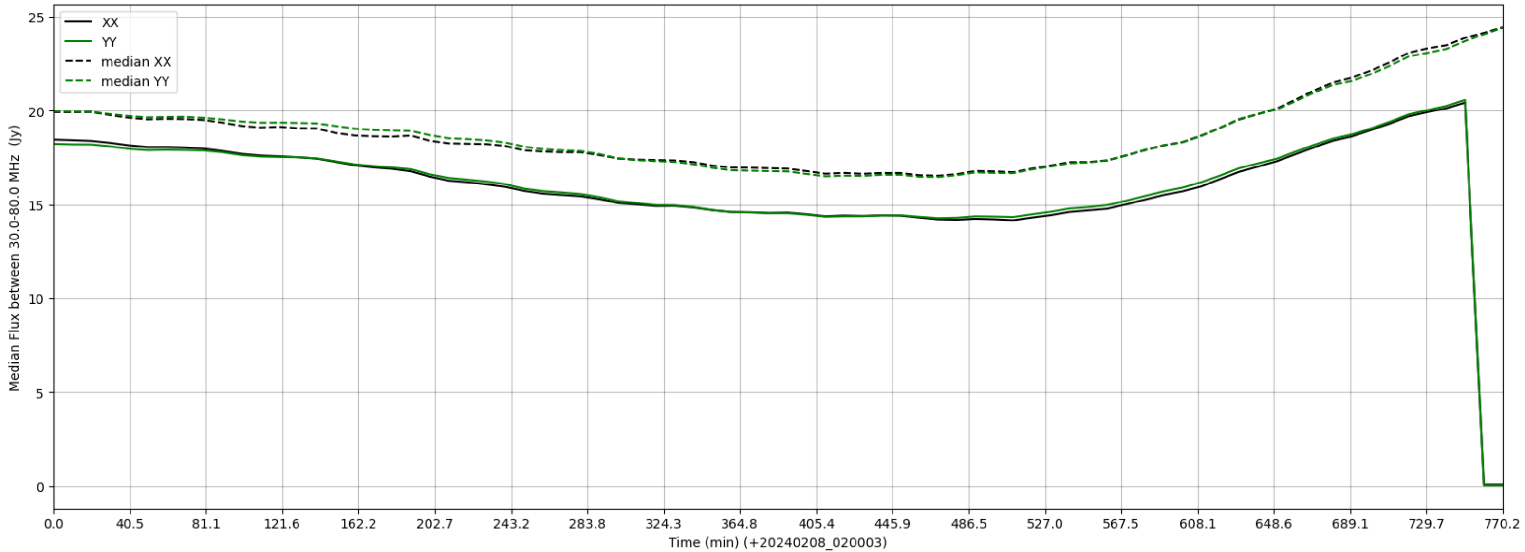
LWA360 - Correlator# 062 - XX FLAGS:HighTimeVar - YY FLAGS:HighTimeVar
