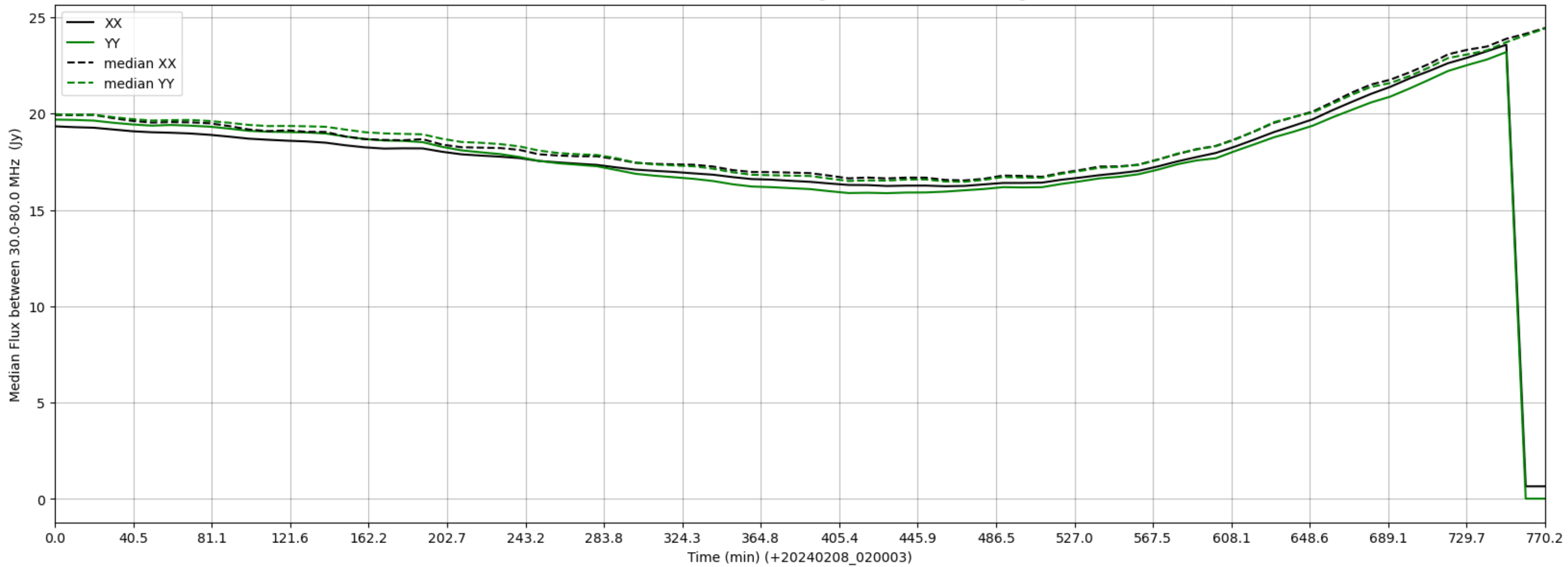
LWA356 - Correlator# 318 - XX FLAGS:HighTimeVar - YY FLAGS:HighTimeVar
