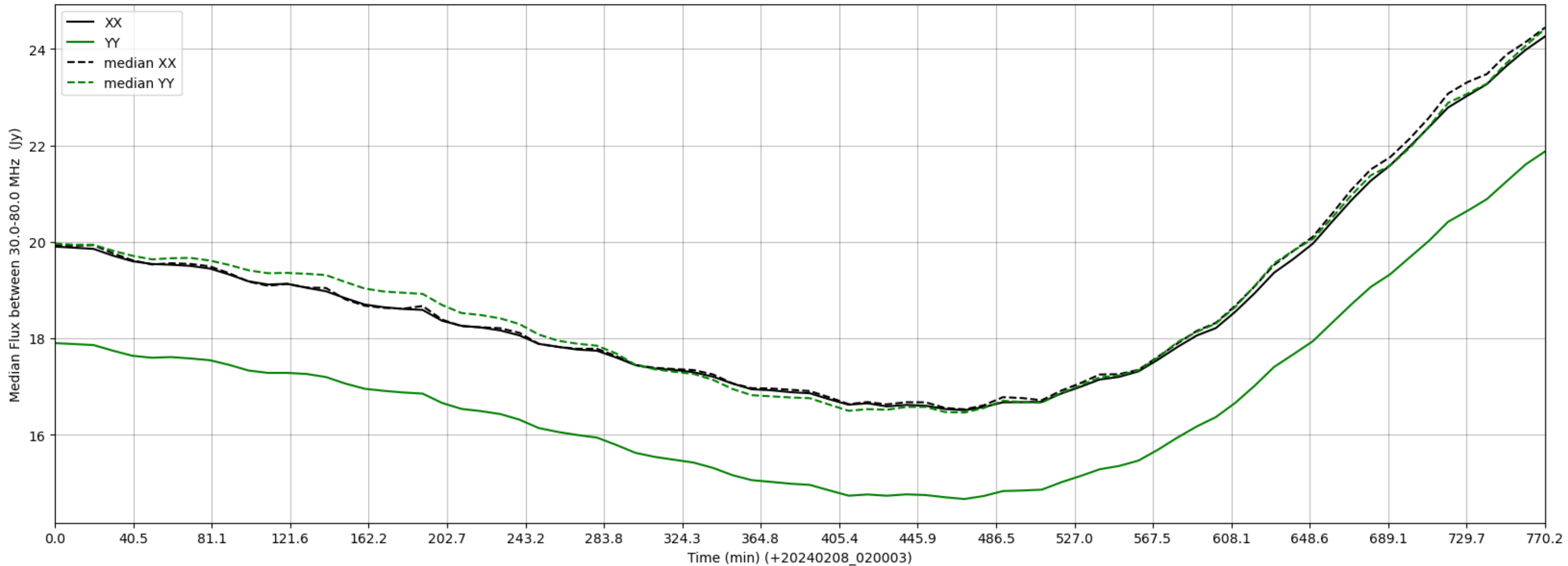
LWA160 - Correlator# 239 - XX FLAGS:BadSpecShape - YY FLAGS:Good
