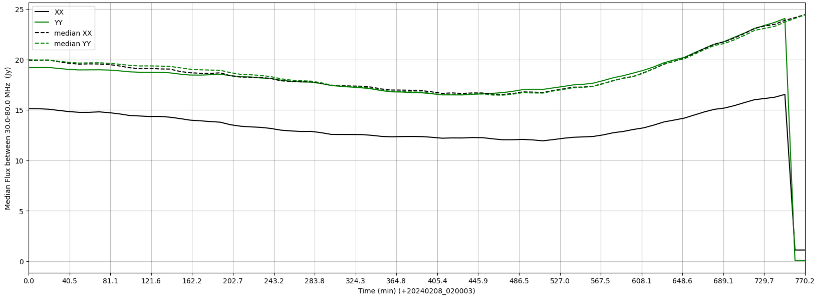
LWA317 - Correlator# 052 - XX FLAGS:HighTimeVar - YY FLAGS:HighTimeVar
