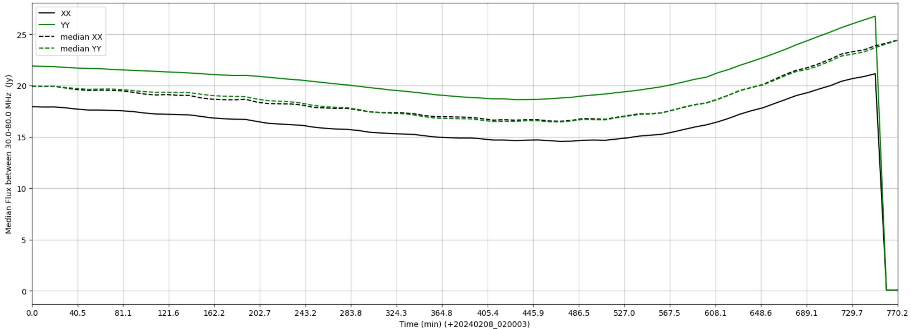
LWA364 - Correlator# 127 - XX FLAGS:HighTimeVar - YY FLAGS:HighTimeVar
