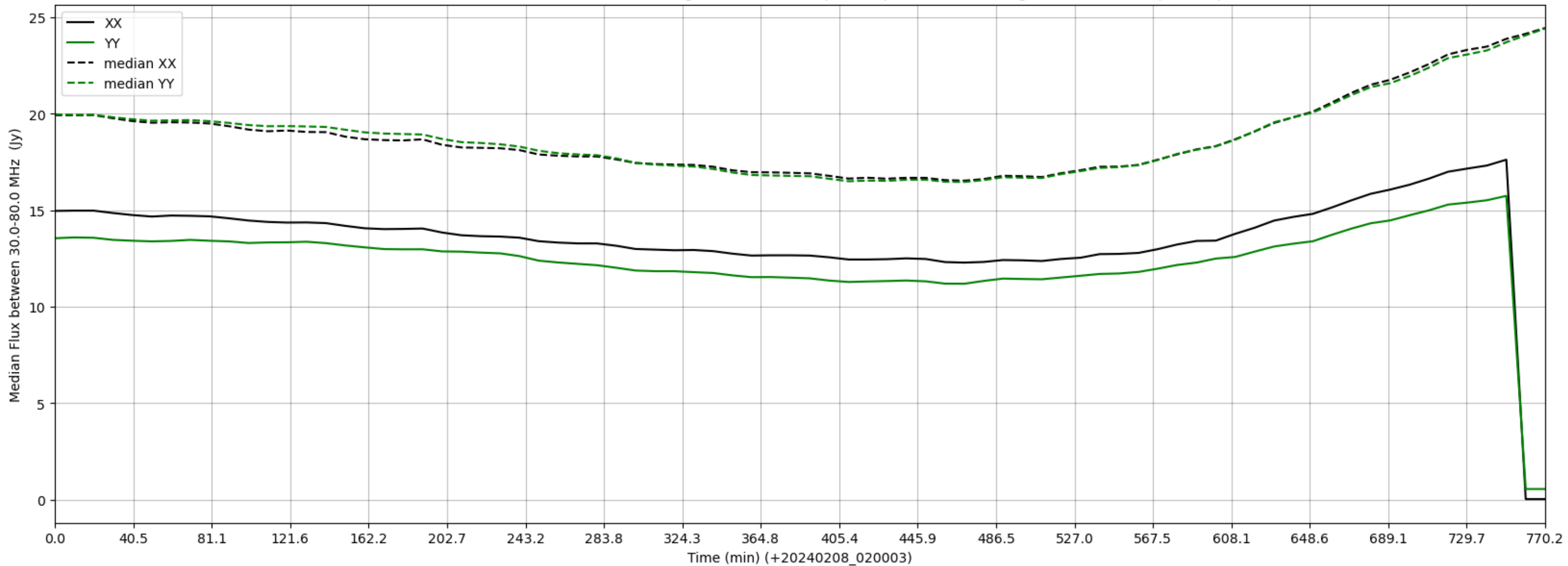
LWA302 - Correlator# 092 - XX FLAGS:HighTimeVar+BadSpecShape - YY FLAGS:HighTimeVar+BadSpecShape
