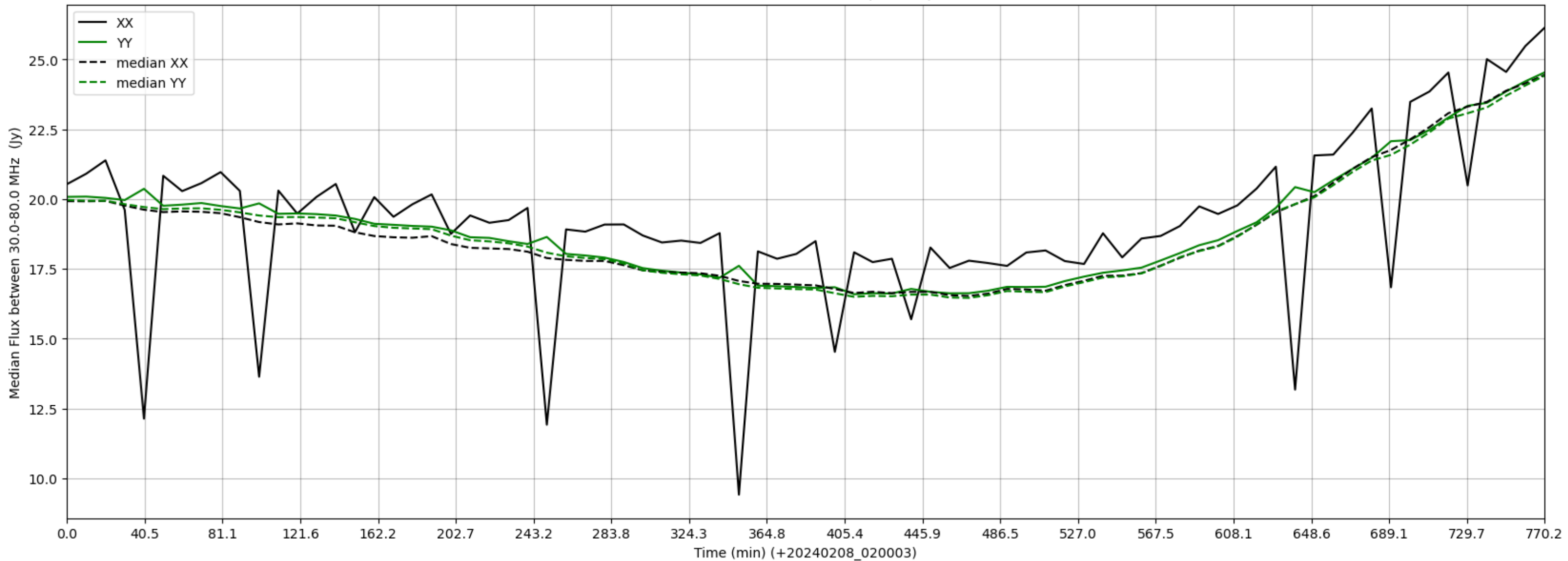
LWA041 - Correlator# 079 - XX FLAGS:BadSpecShape - YY FLAGS:Good
