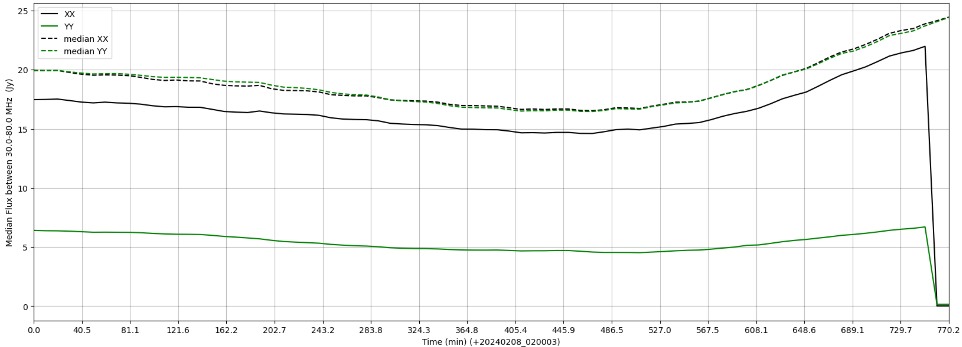
LWA303 - Correlator# 051 - XX FLAGS:HighTimeVar - YY FLAGS:HighTimeVar+BadSpecShape
