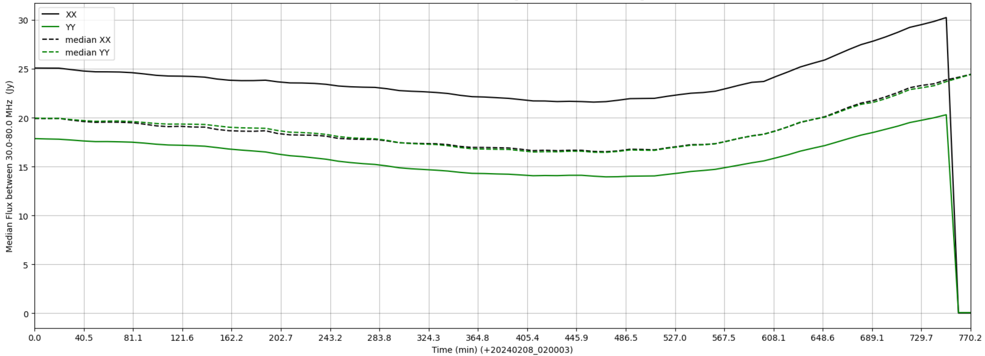
LWA345 - Correlator# 252 - XX FLAGS:HighTimeVar - YY FLAGS:HighTimeVar
