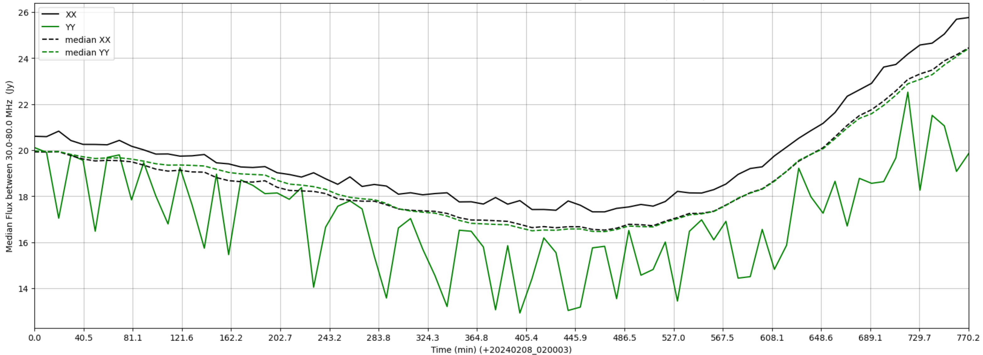
LWA142 - Correlator# 211 - XX FLAGS:Good - YY FLAGS:HighTimeVar+BadSpecShape
