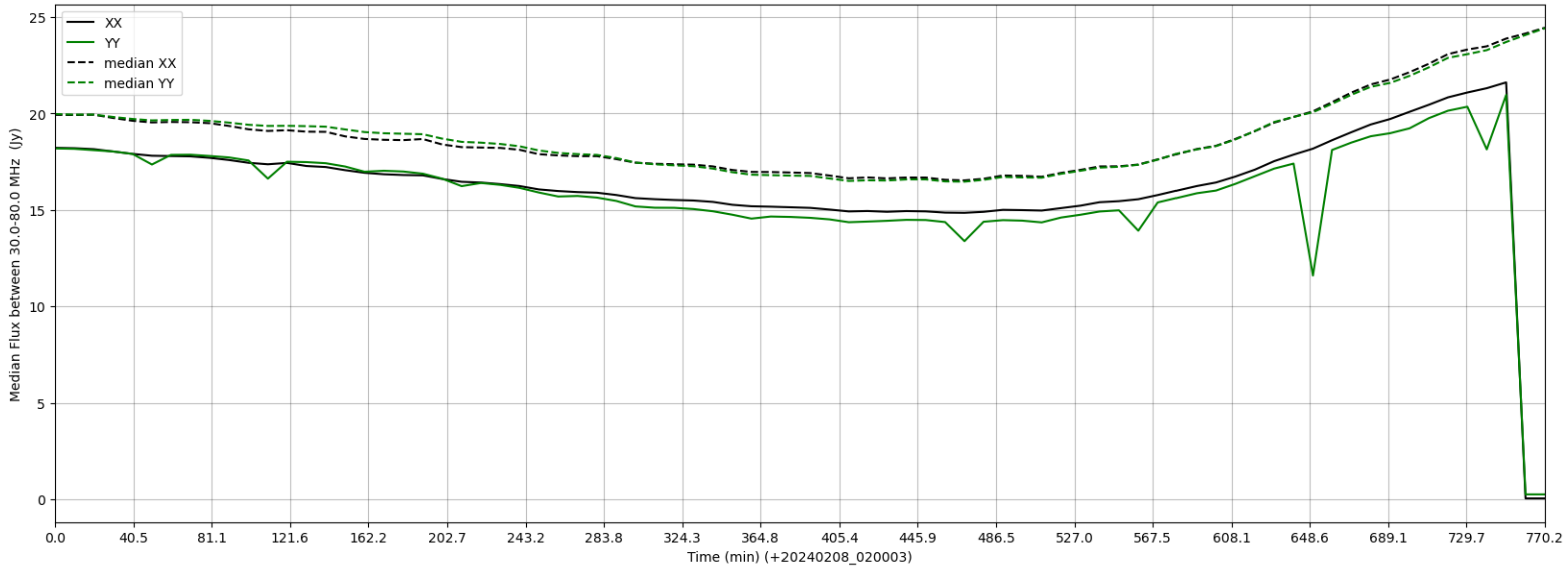
LWA323 - Correlator# 095 - XX FLAGS:HighTimeVar - YY FLAGS:HighTimeVar
