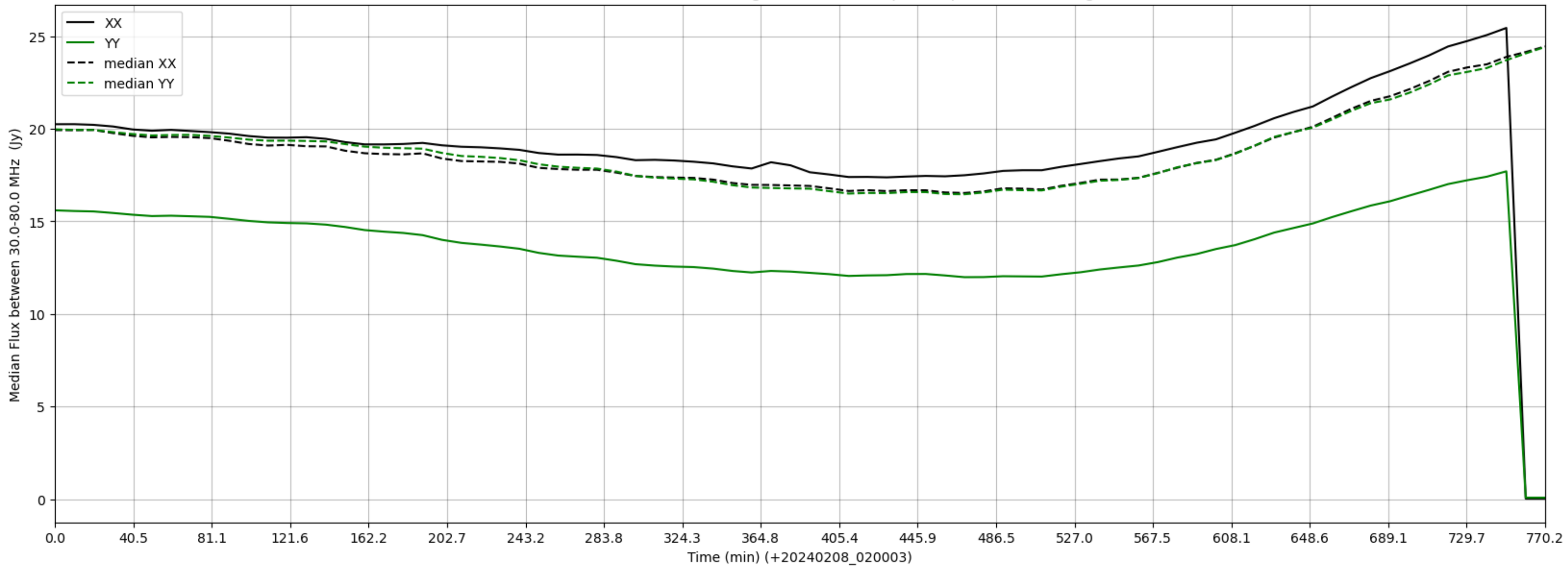
LWA263 - Correlator# 037 - XX FLAGS:HighTimeVar+BadSpecShape - YY FLAGS:HighTimeVar
