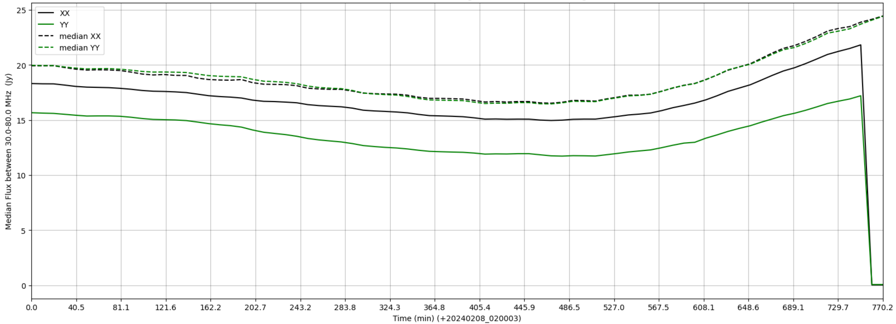
LWA359 - Correlator# 254 - XX FLAGS:HighTimeVar - YY FLAGS:HighTimeVar
