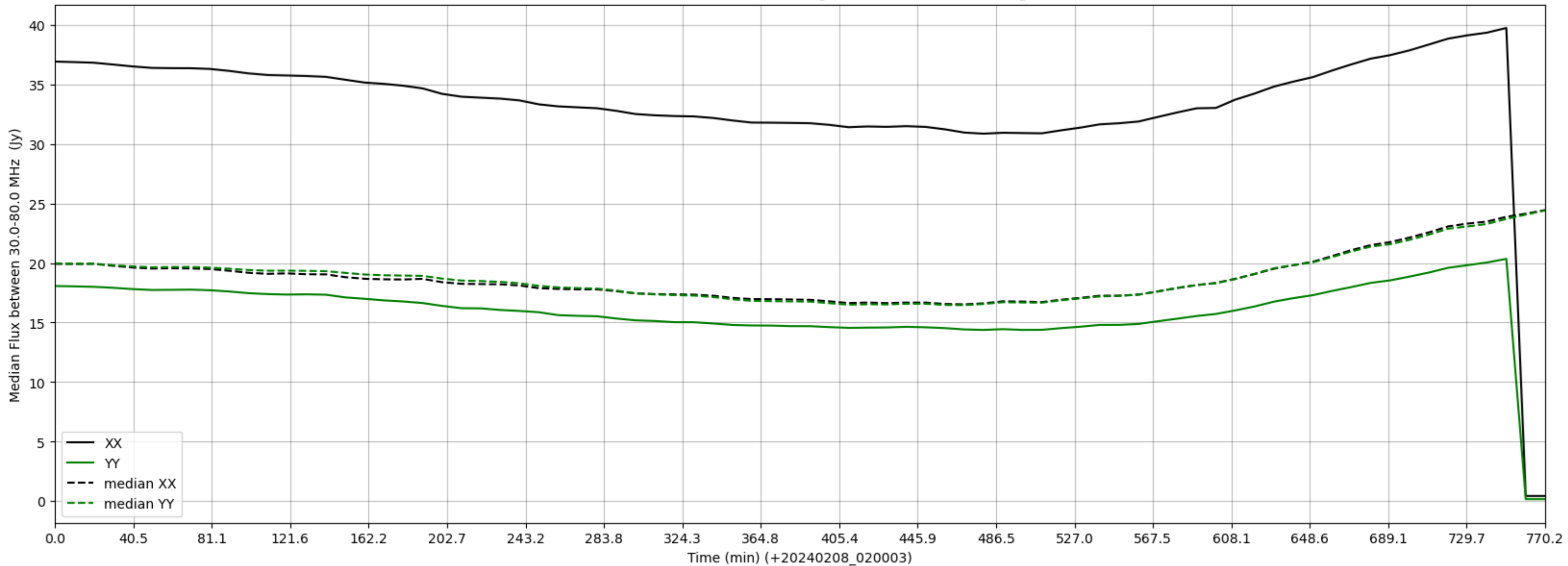
LWA362 - Correlator# 030 - XX FLAGS:HighTimeVar - YY FLAGS:HighTimeVar
