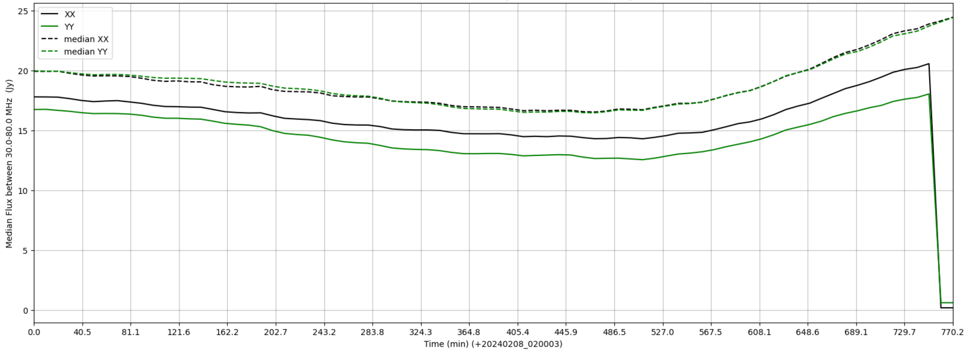
LWA294 - Correlator# 188 - XX FLAGS:HighTimeVar - YY FLAGS:HighTimeVar
