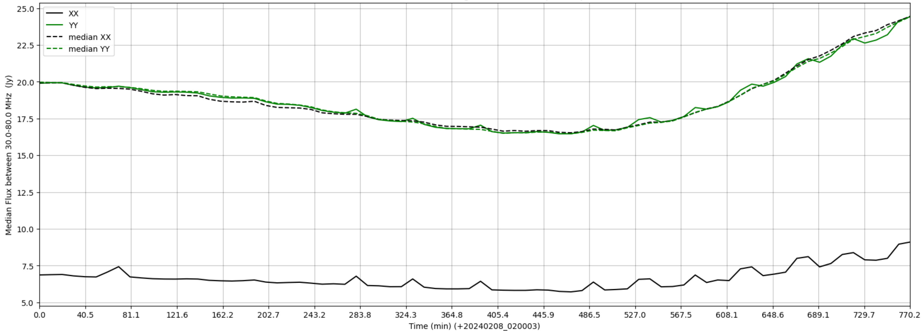
LWA130 - Correlator# 183 - XX FLAGS:HighTimeVar+BadSpecShape - YY FLAGS:Good
