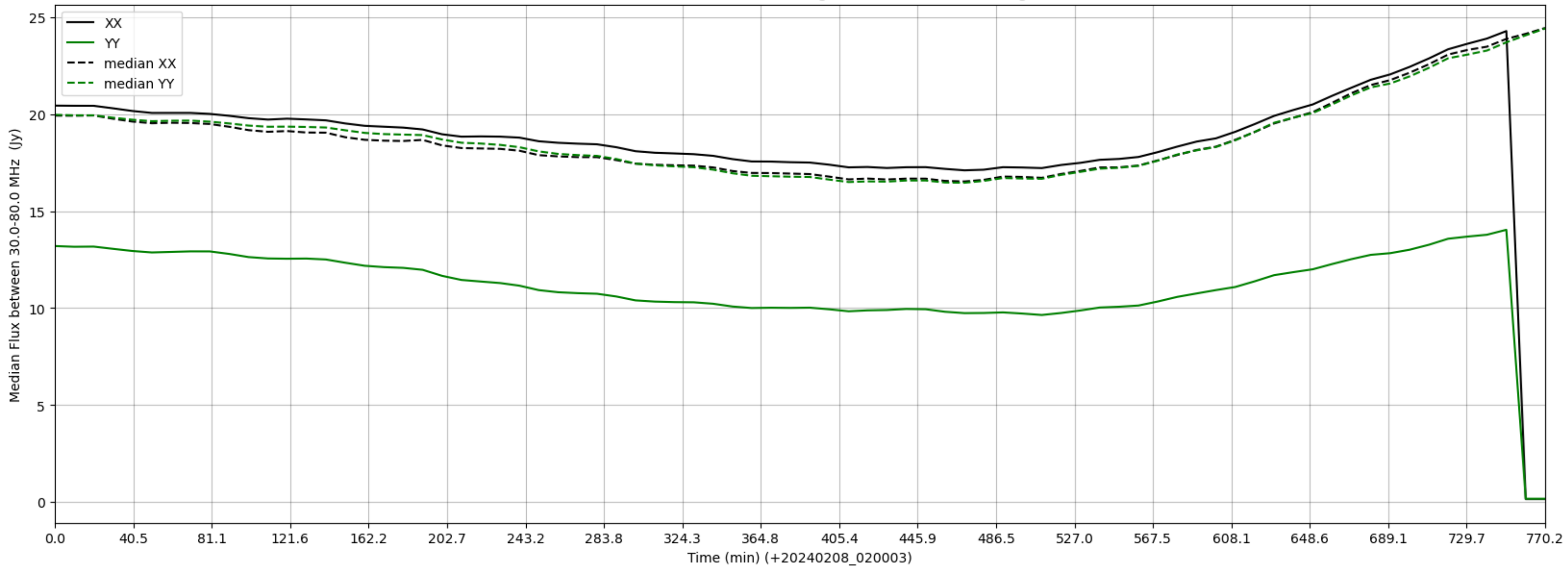
LWA358 - Correlator# 159 - XX FLAGS:HighTimeVar - YY FLAGS:HighTimeVar
