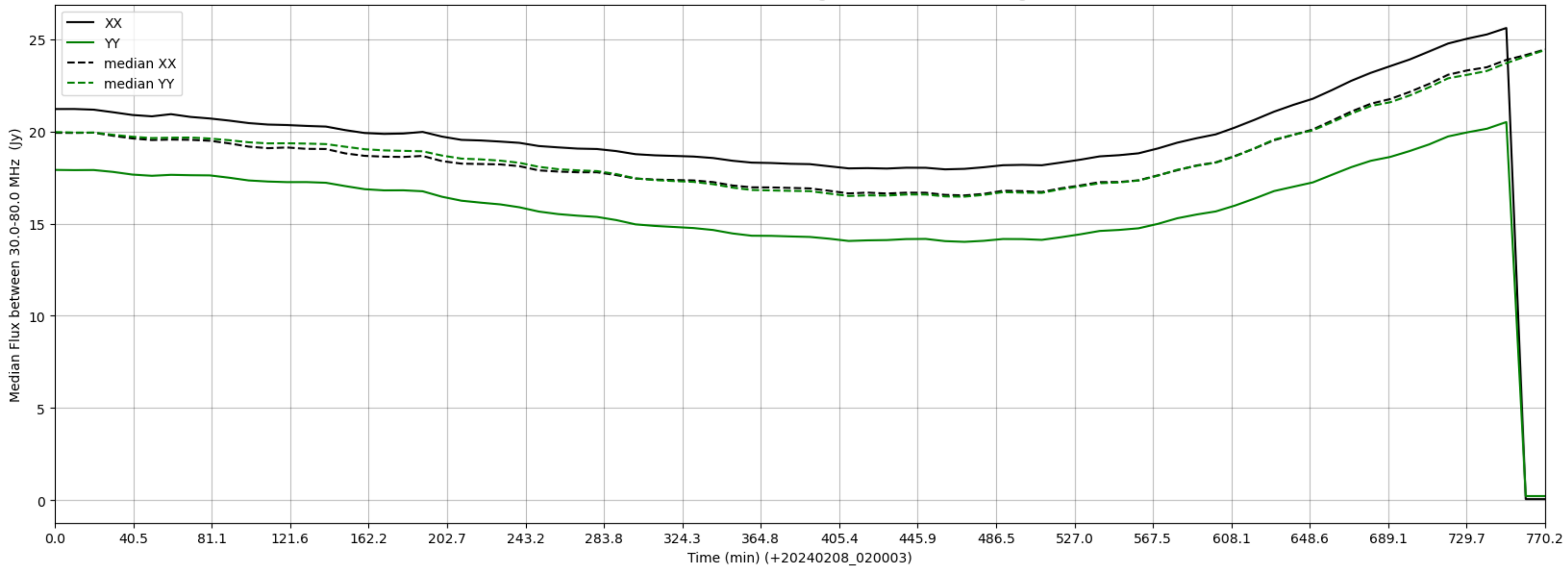
LWA355 - Correlator# 222 - XX FLAGS:HighTimeVar - YY FLAGS:HighTimeVar
