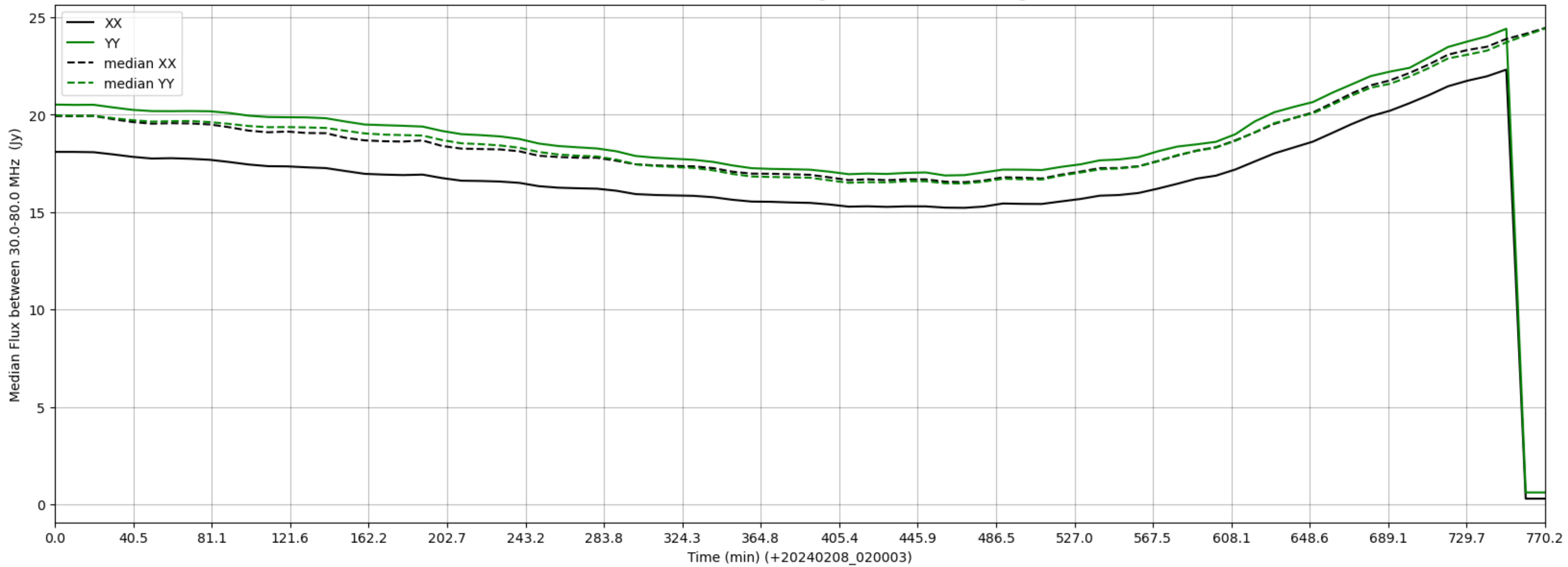
LWA300 - Correlator# 348 - XX FLAGS:HighTimeVar - YY FLAGS:HighTimeVar
