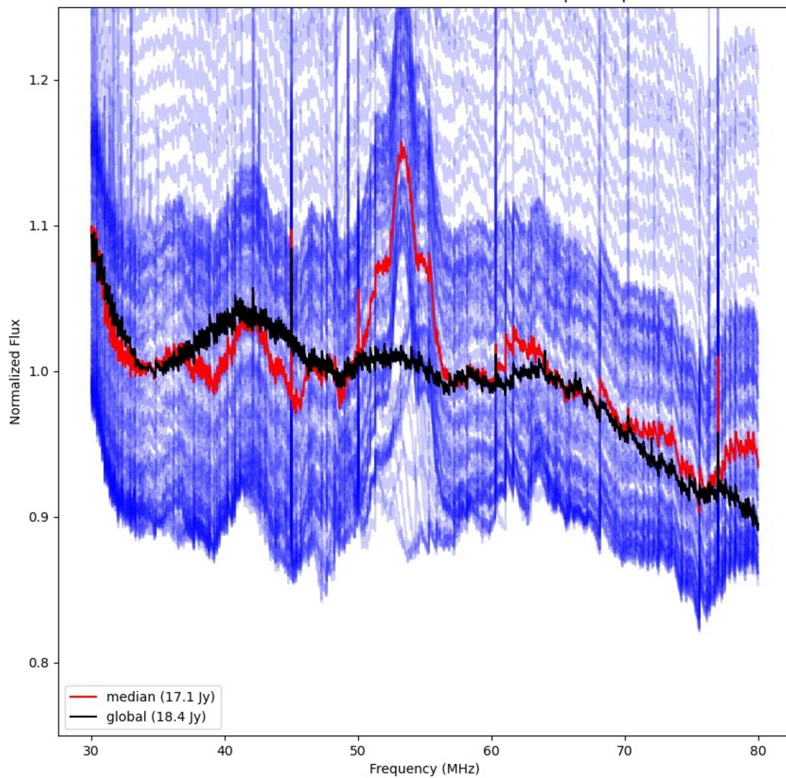
LWA296 - Correlator# 046 - XX - FLAGS:BadSpecShape
