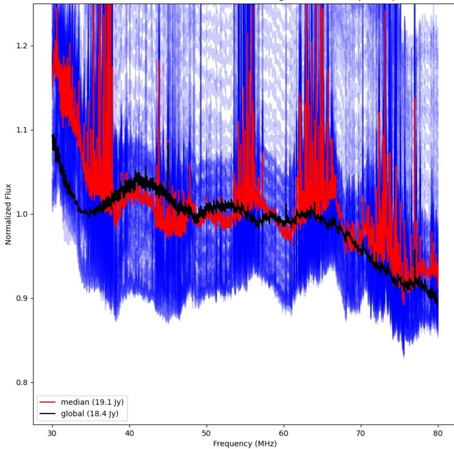
LWA263 - Correlator# 037 - XX - FLAGS:HighTimeVar+BadSpecShape
