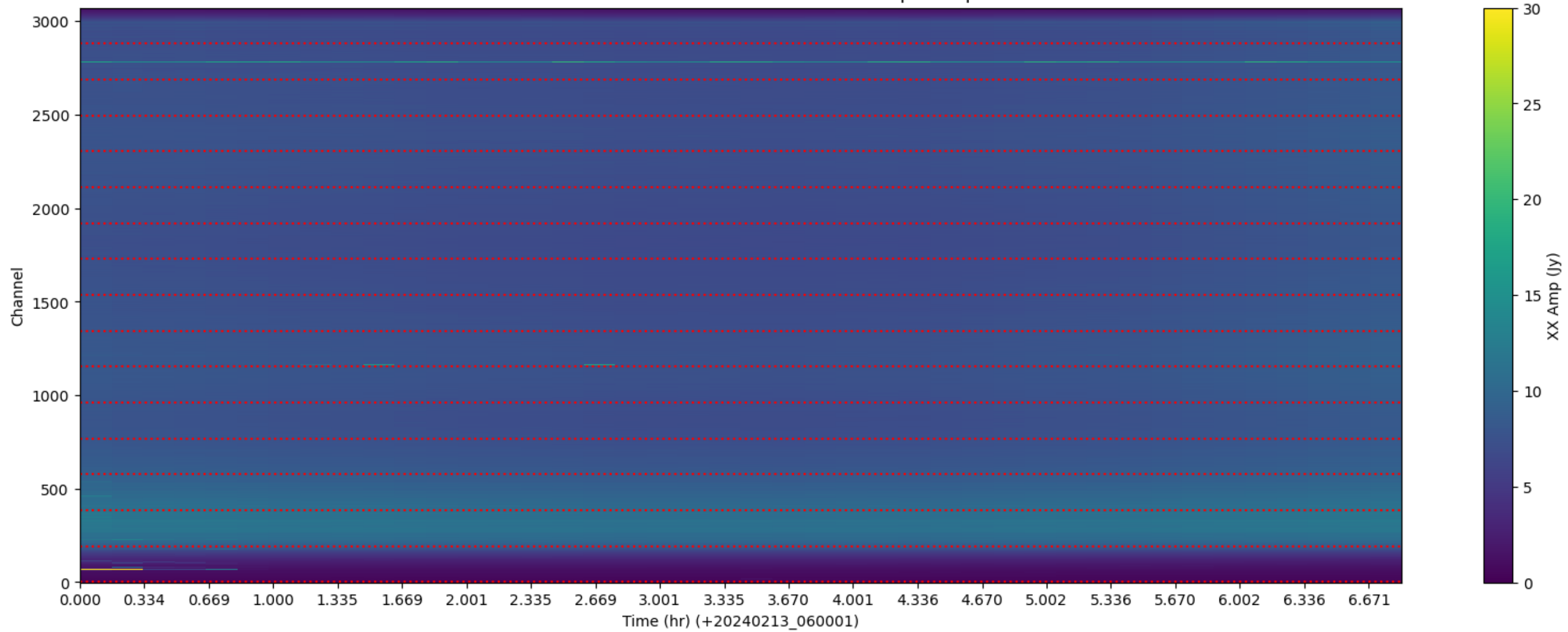
LWA153 - Correlator# 230 - XX - FLAGS: BadSpecShape
