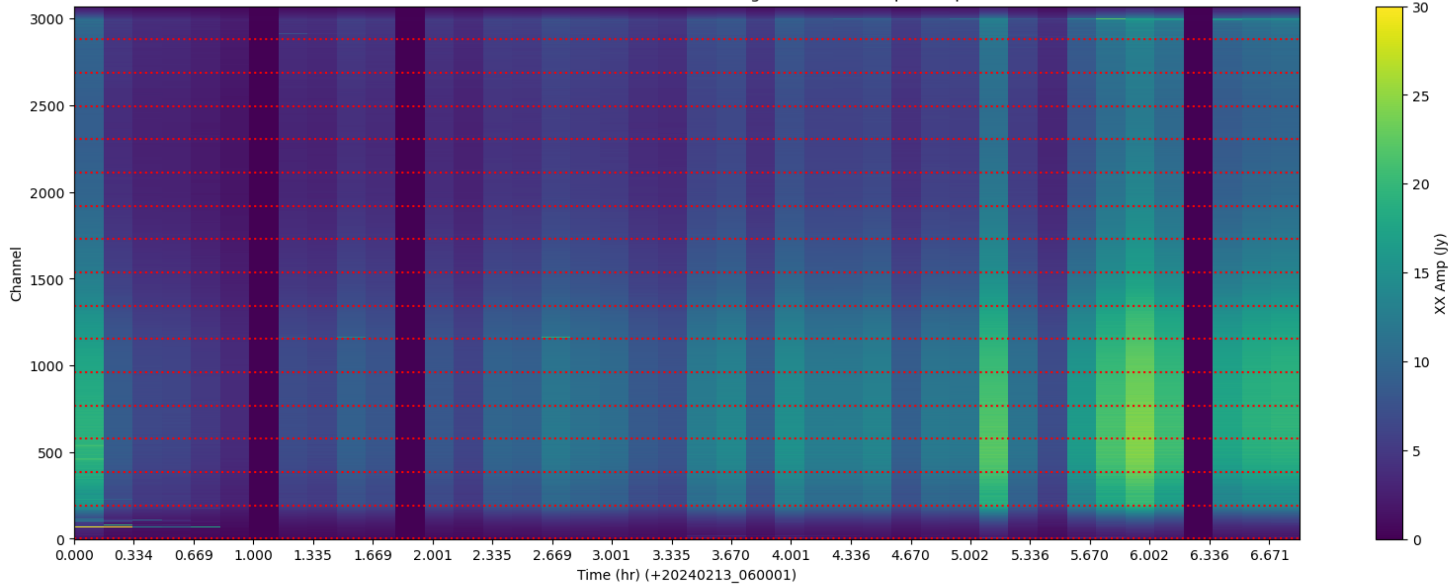
LWA255 - Correlator# 033 - XX - FLAGS: HighTimeVar+BadSpecShape
