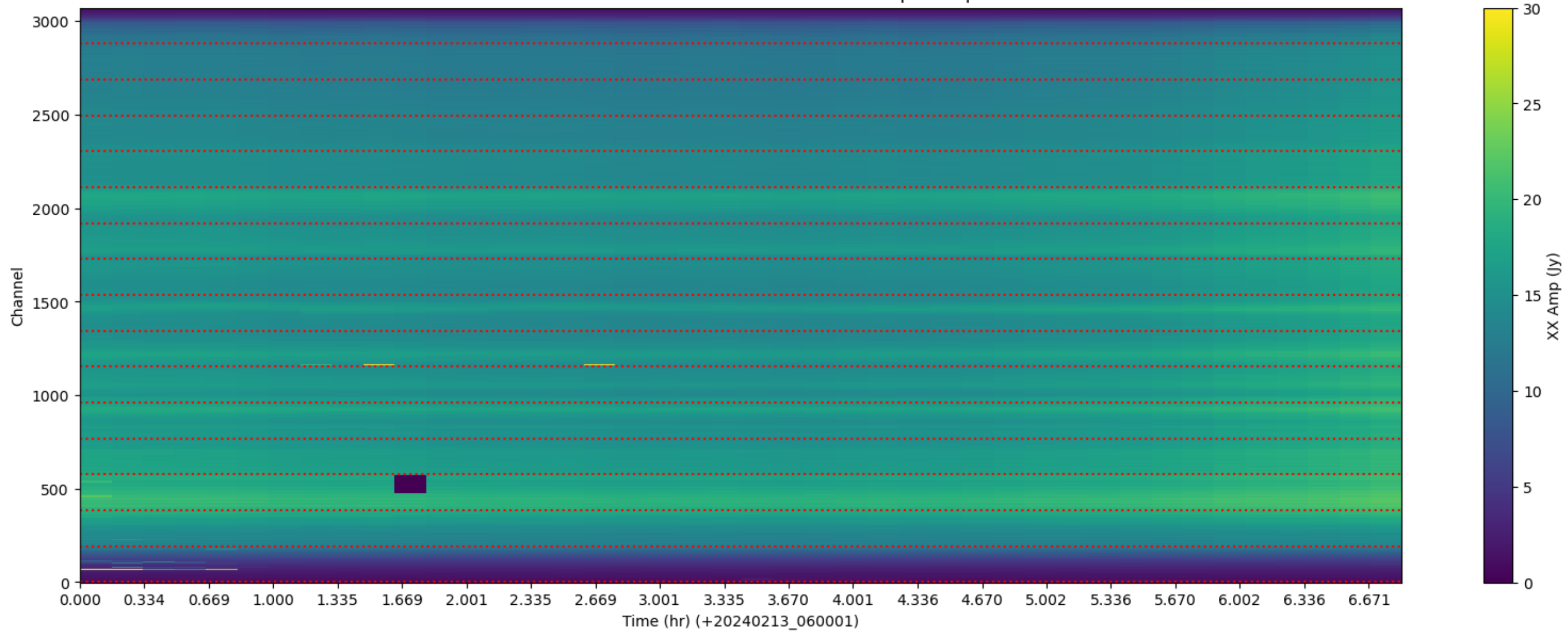
LWA336 - Correlator# 056 - XX - FLAGS: BadSpecShape
