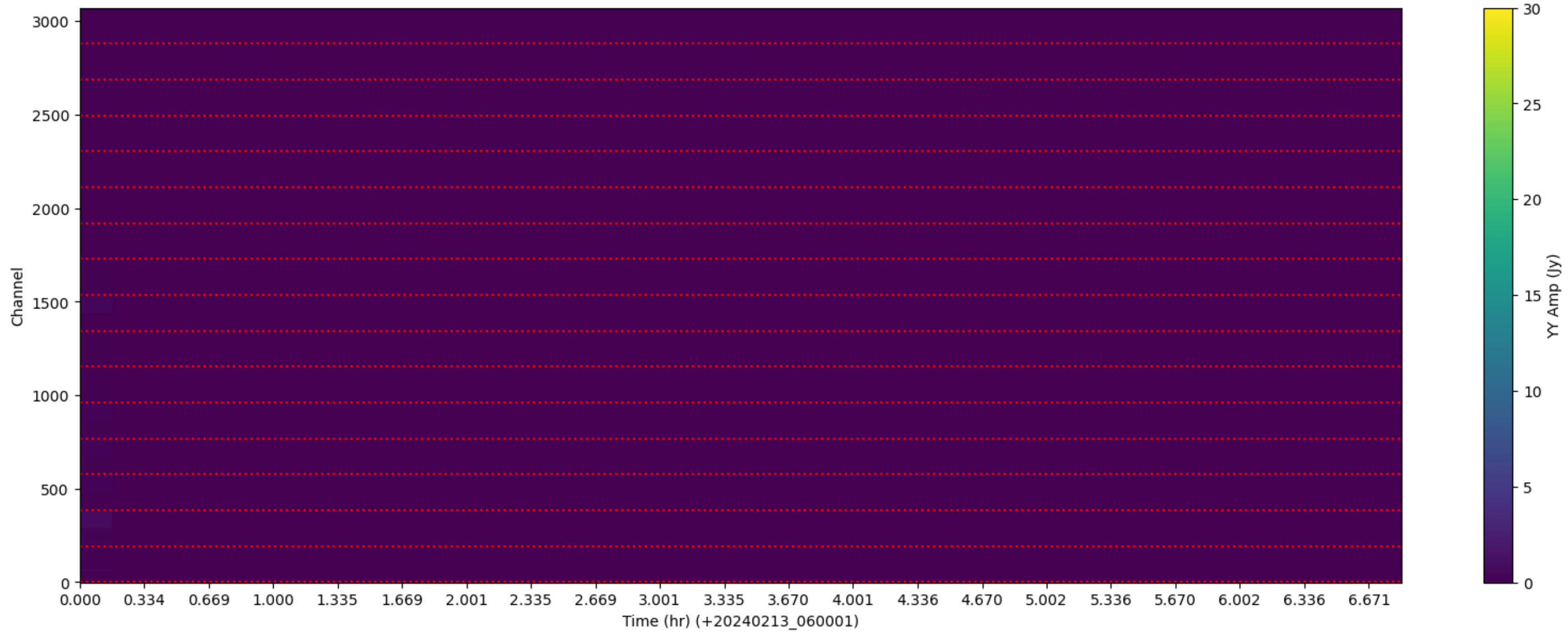
LWA161 - Correlator# 262 - YY - FLAGS: LowFlux
