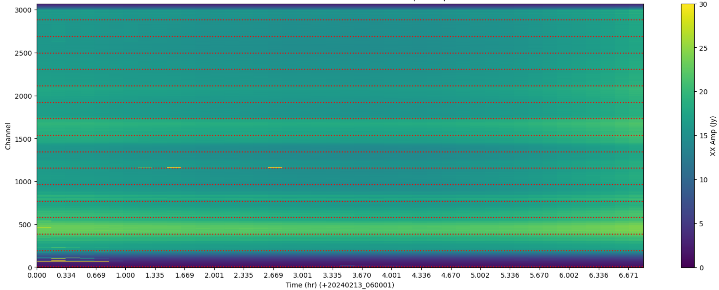
LWA280 - Correlator# 041 - XX - FLAGS: BadSpecShape
