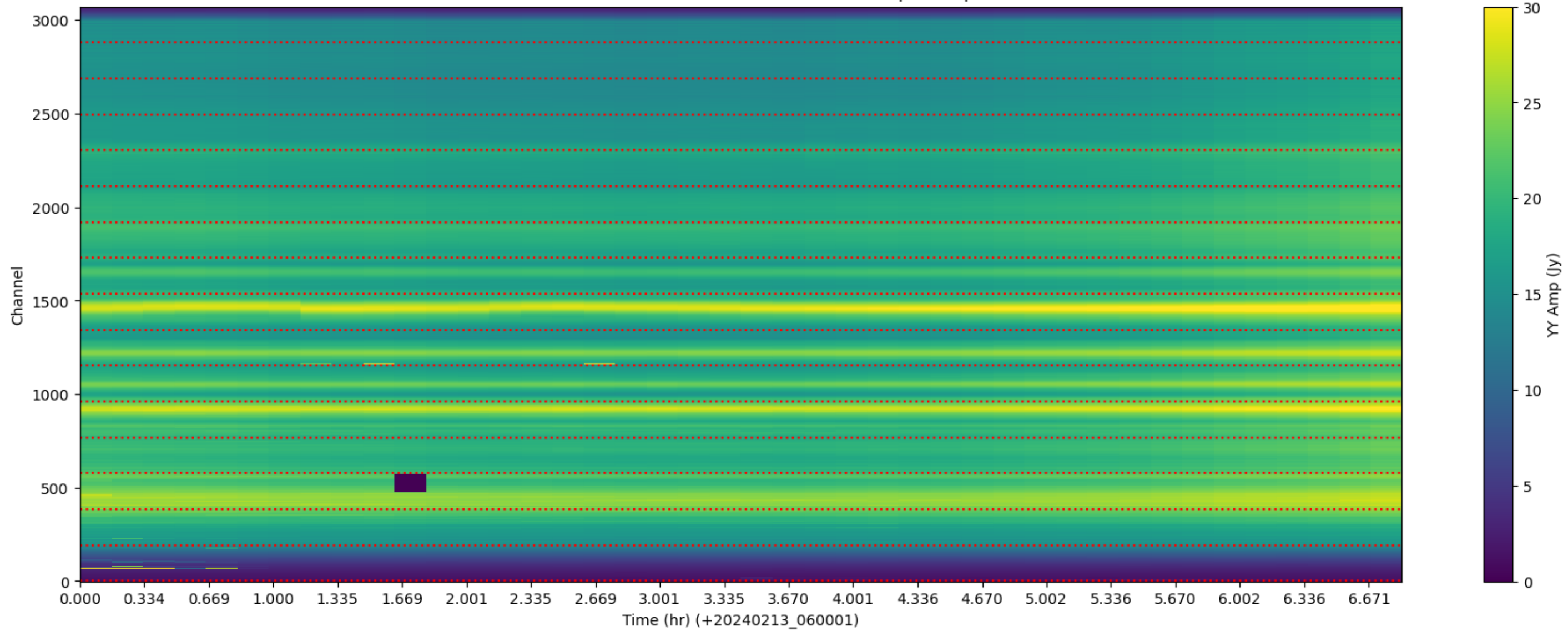
LWA336 - Correlator# 056 - YY - FLAGS: BadSpecShape
