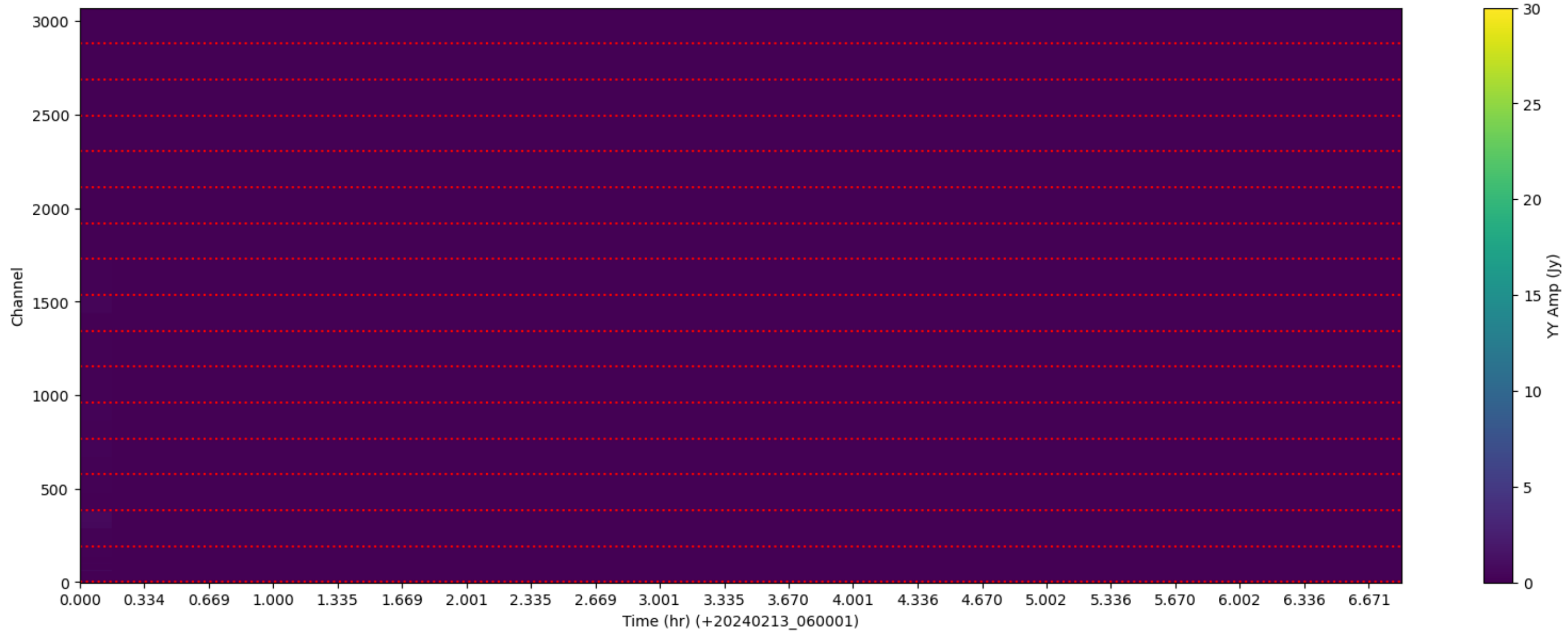
LWA198 - Correlator# 271 - YY - FLAGS: LowFlux
