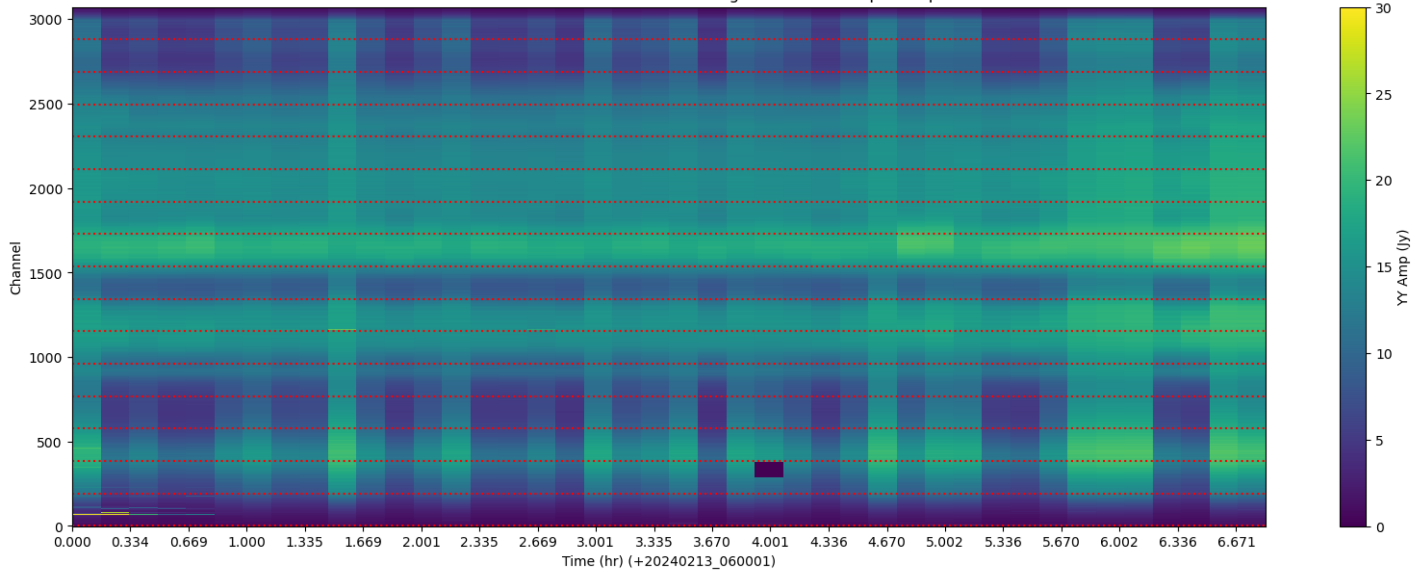
LWA142 - Correlator# 211 - YY - FLAGS: HighTimeVar+BadSpecShape
