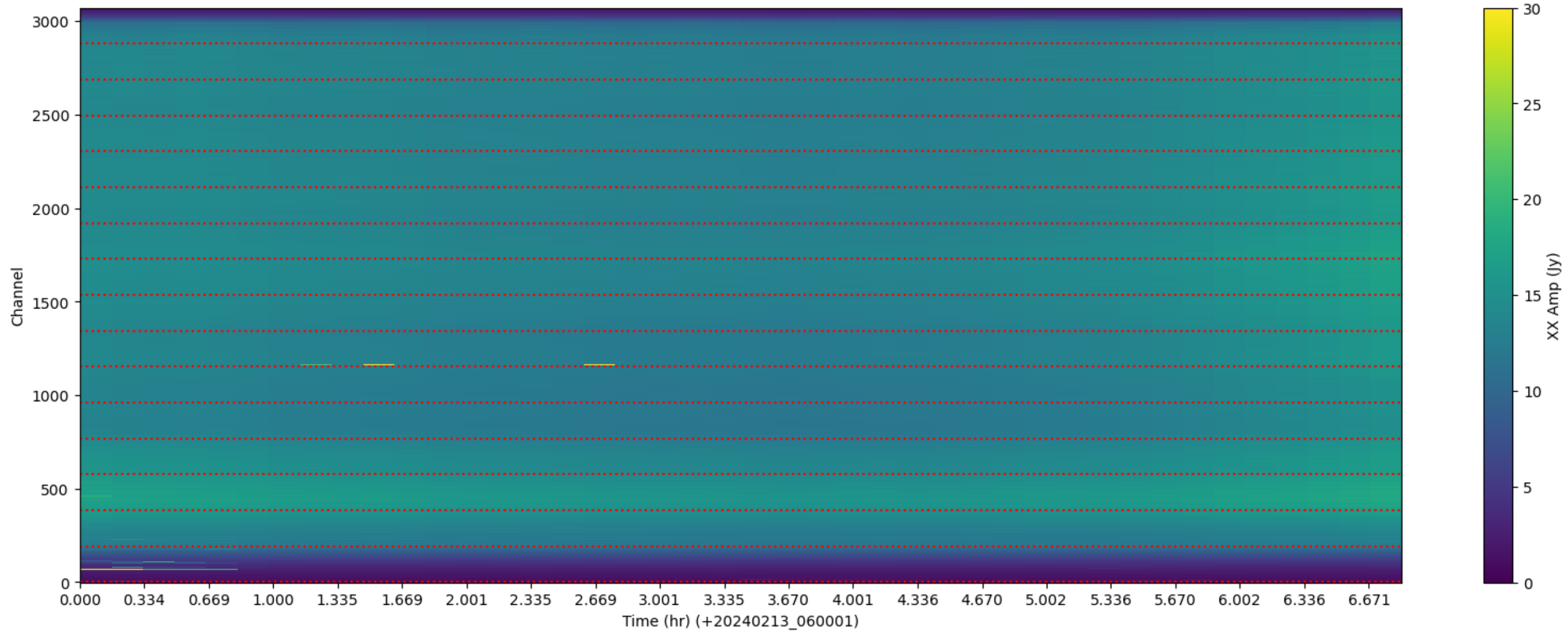
LWA339 - Correlator# 027 - XX - FLAGS: Good
