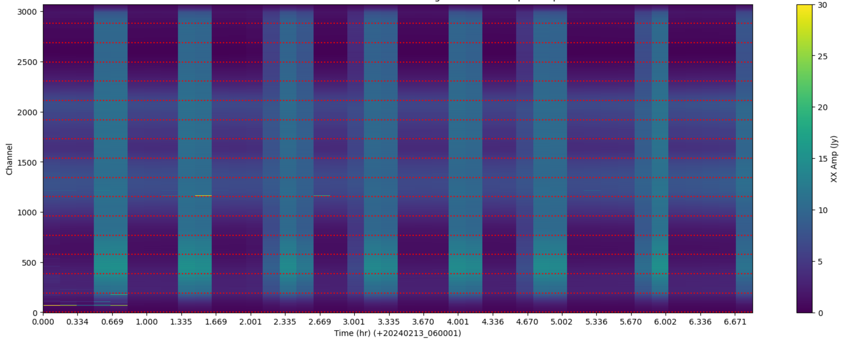
LWA335 - Correlator# 057 - XX - FLAGS: HighTimeVar+BadSpecShape
