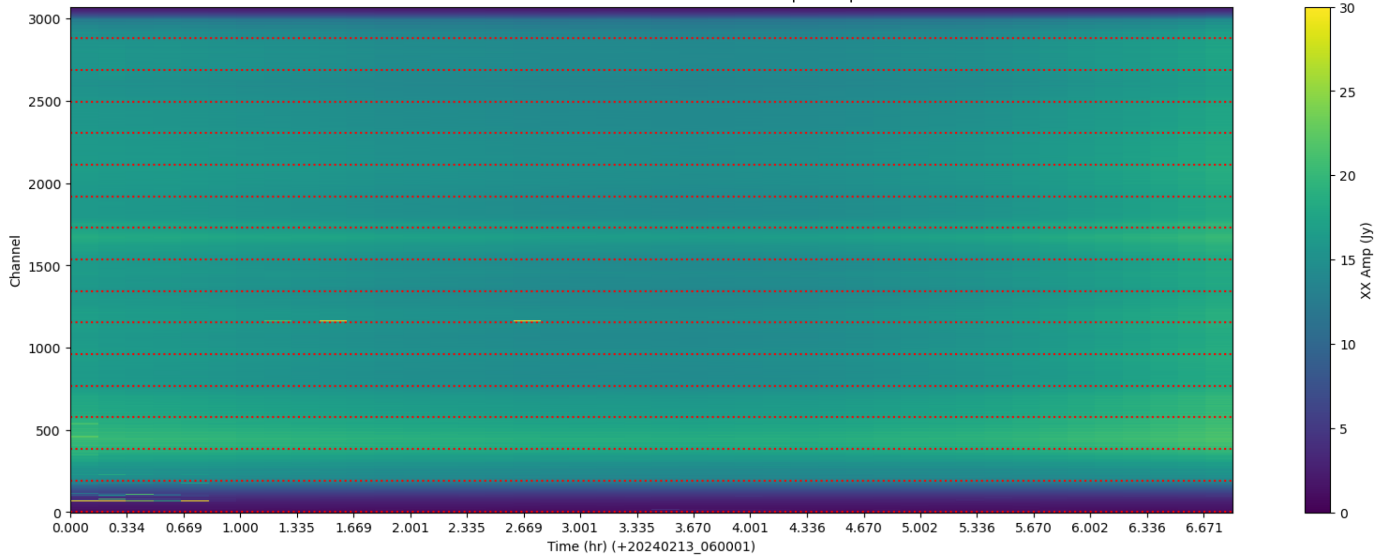
LWA296 - Correlator# 046 - XX - FLAGS: BadSpecShape
