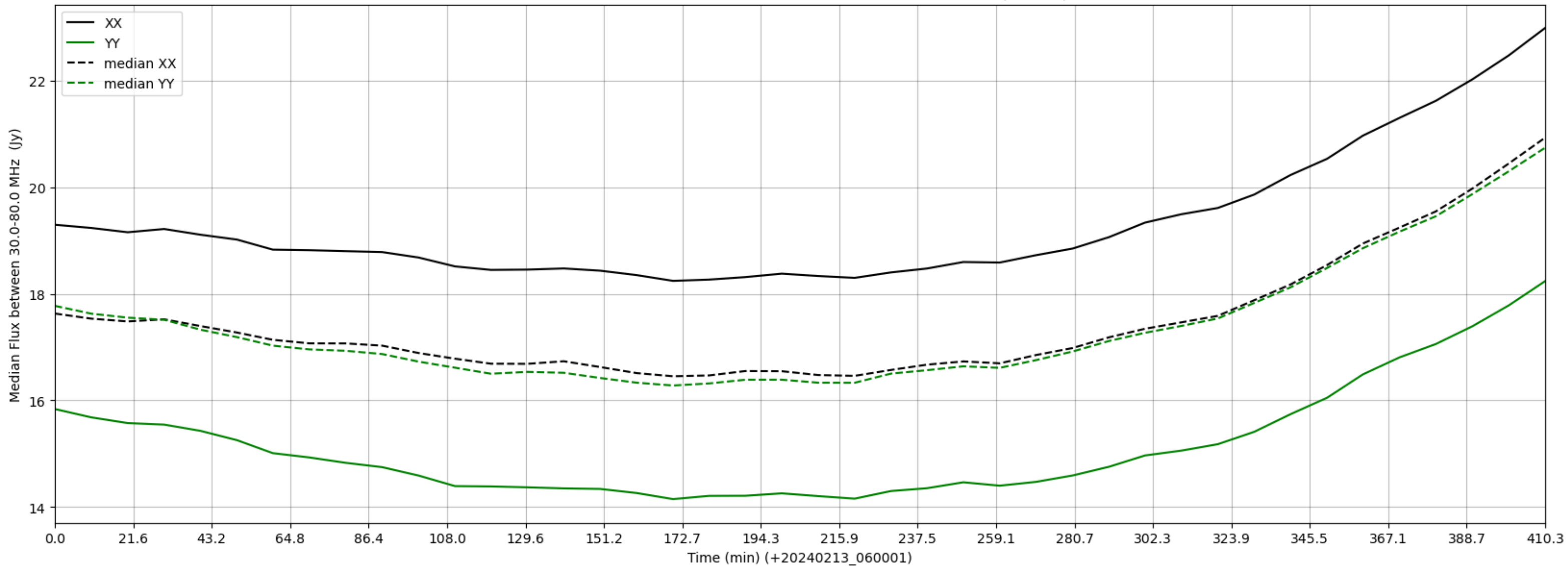
LWA348 - Correlator# 124 - XX FLAGS:Good - YY FLAGS:BadSpecShape
