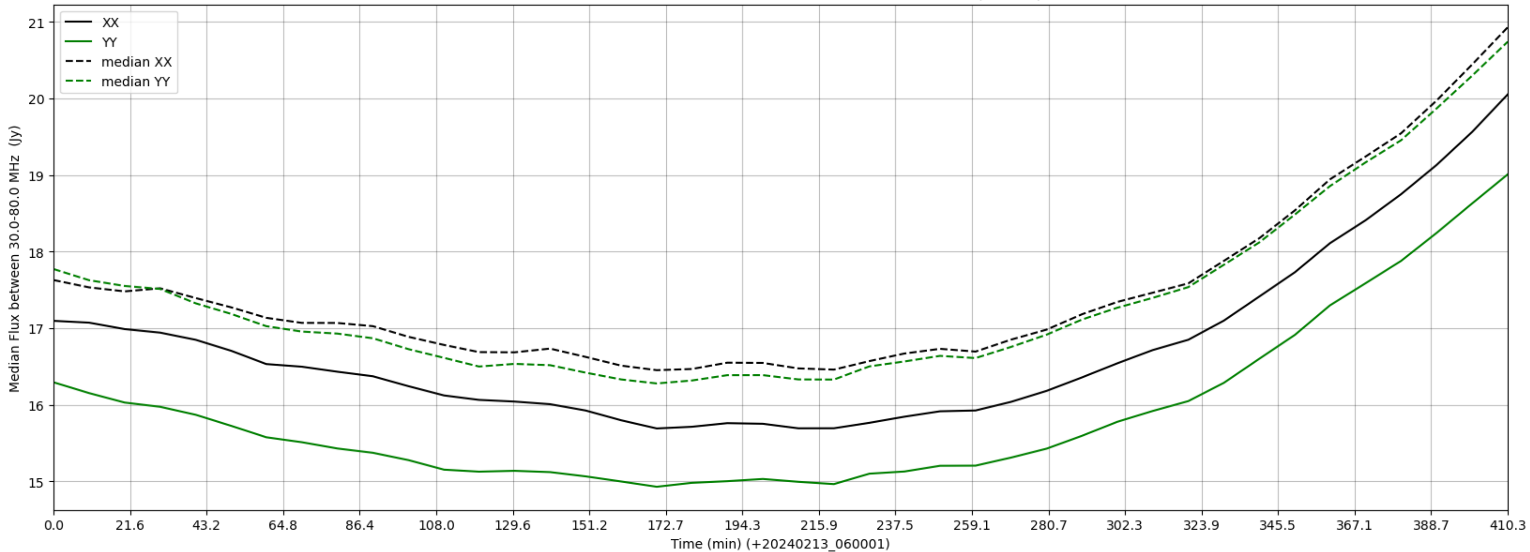
LWA341 - Correlator# 029 - XX FLAGS:Good - YY FLAGS:BadSpecShape
