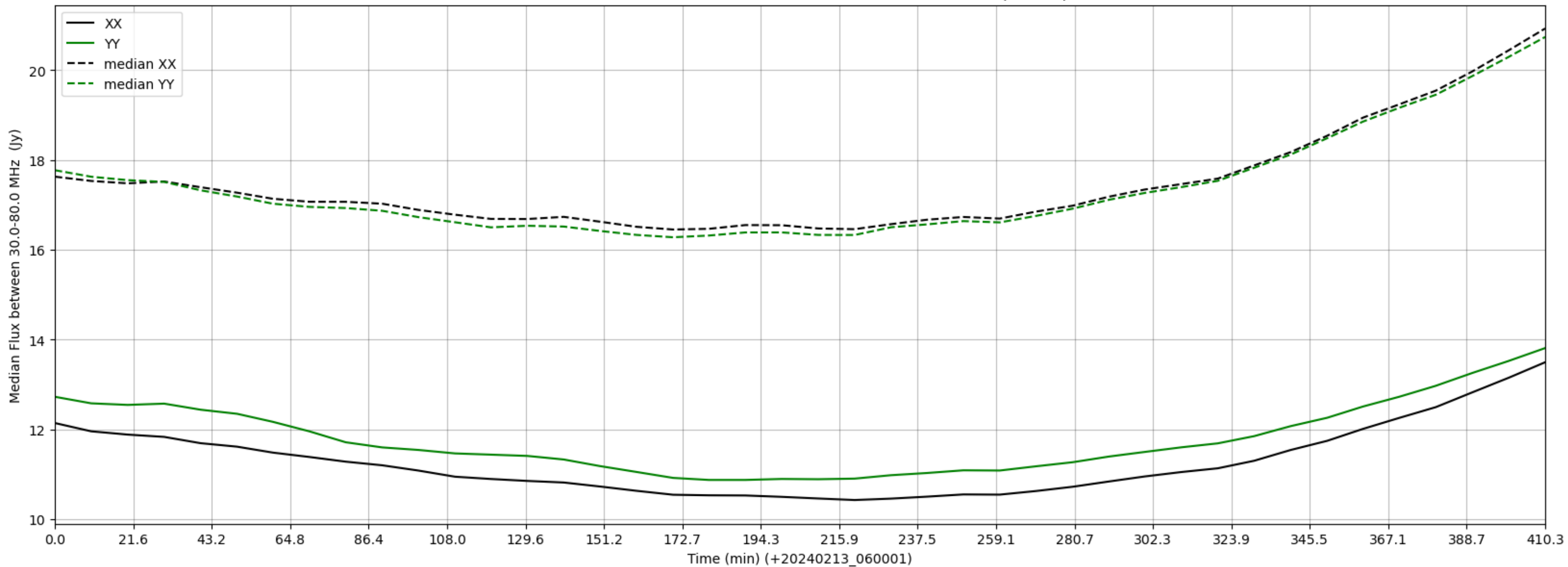
LWA297 - Correlator# 314 - XX FLAGS:Good - YY FLAGS:BadSpecShape
