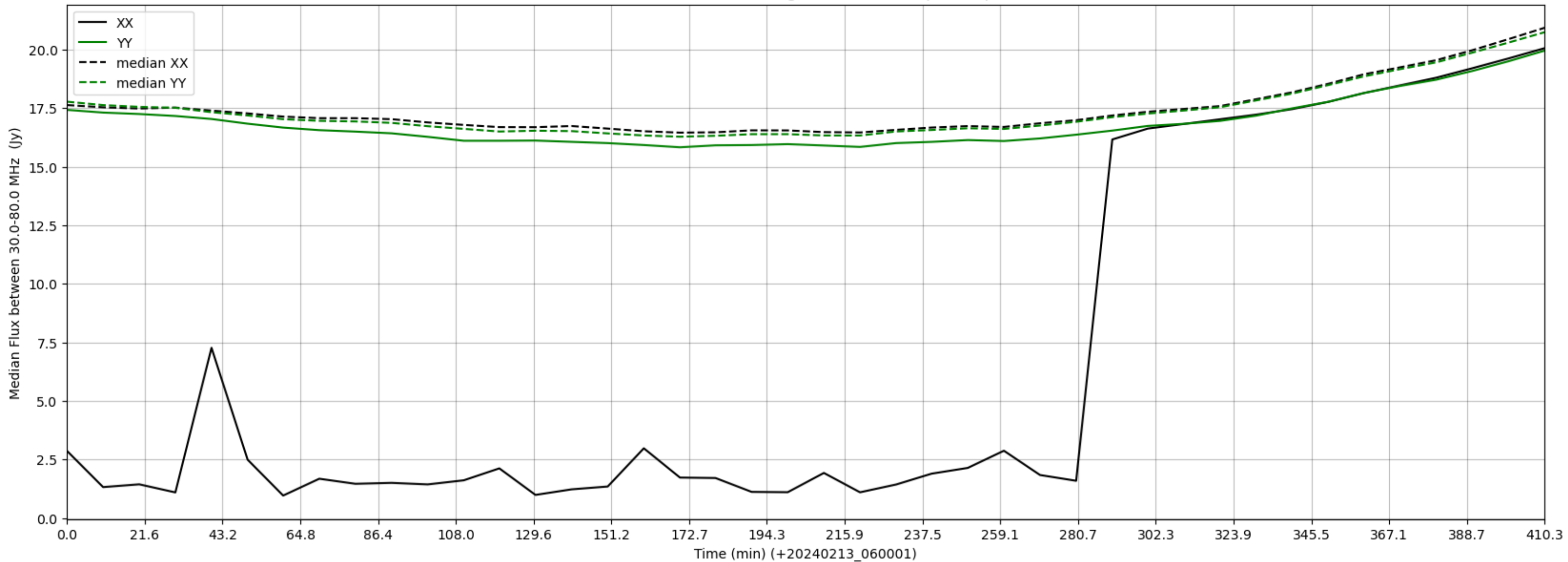
LWA353 - Correlator# 031 - XX FLAGS:HighTimeVar+BadSpecShape - YY FLAGS:Good
