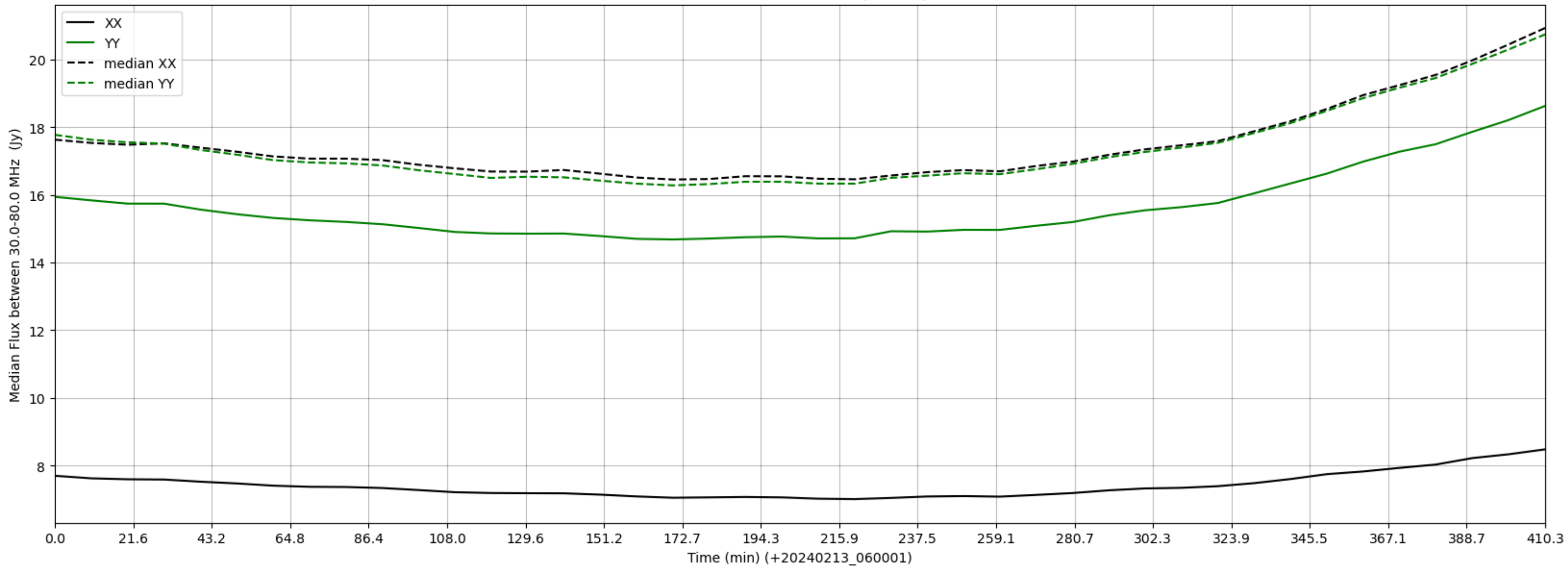
LWA153 - Correlator# 230 - XX FLAGS:BadSpecShape - YY FLAGS:Good
