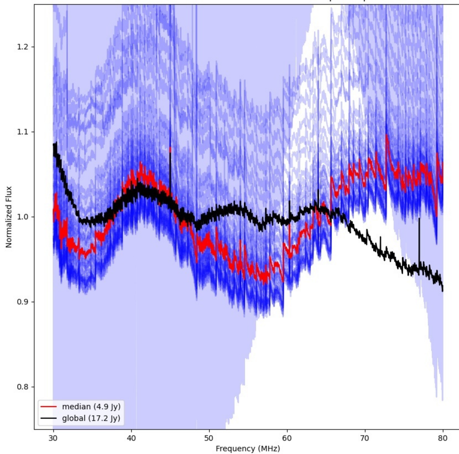
LWA153 - Correlator# 230 - XX - FLAGS:BadSpecShape
