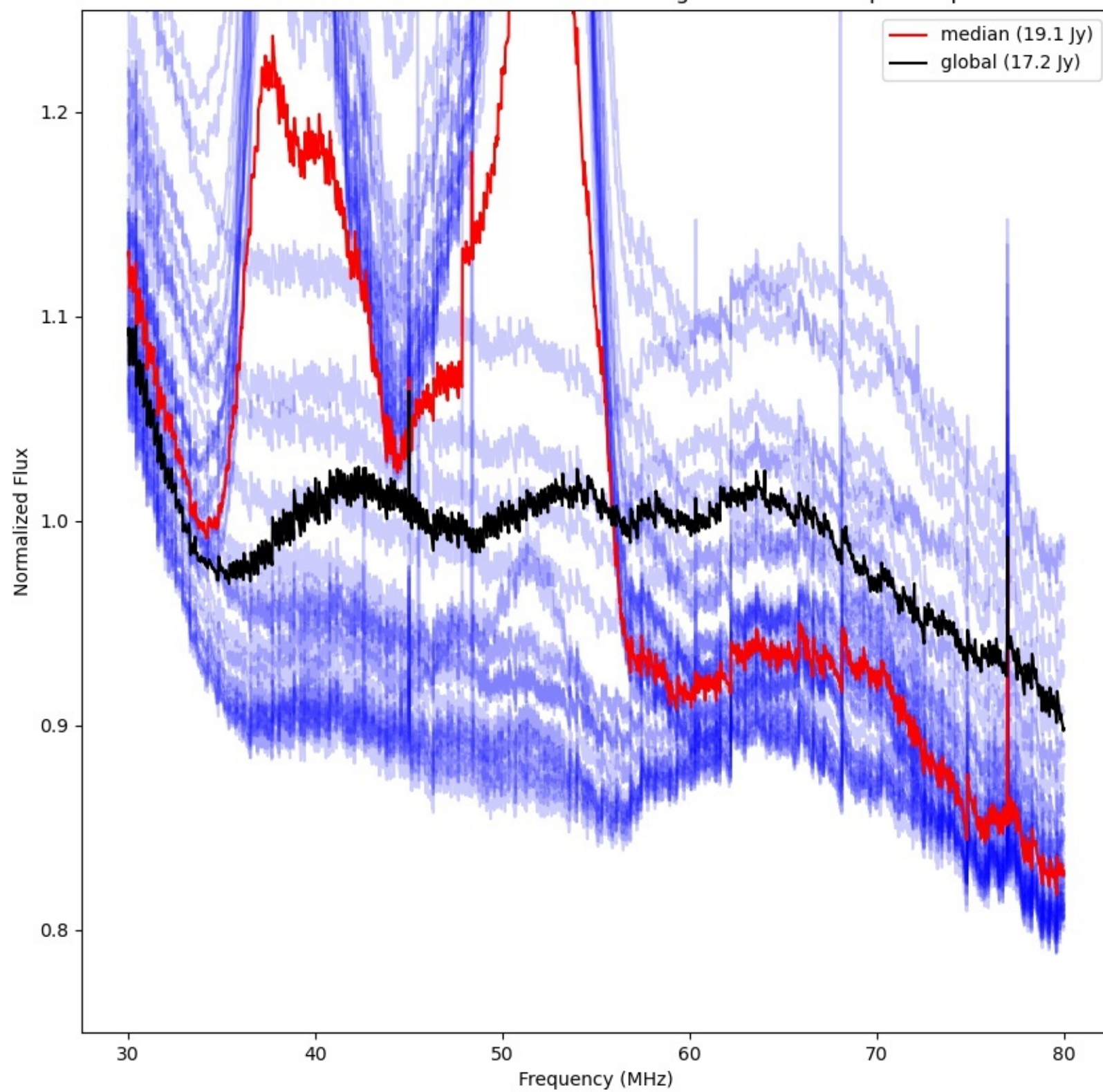
LWA104 - Correlator# 179 - YY - FLAGS:HighTimeVar+BadSpecShape
