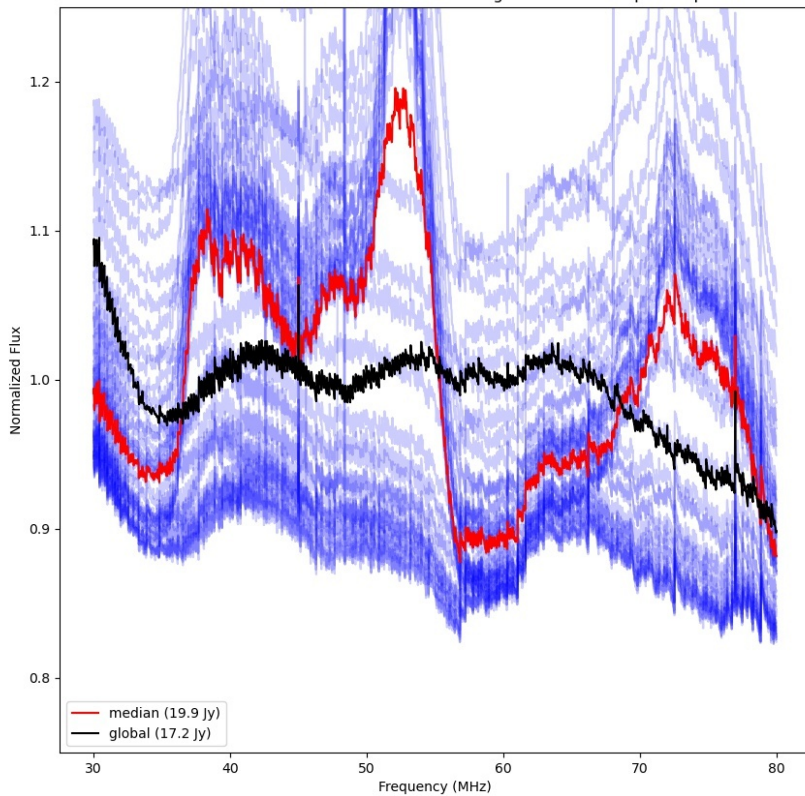
LWA037 - Correlator# 181 - YY - FLAGS:HighTimeVar+BadSpecShape
