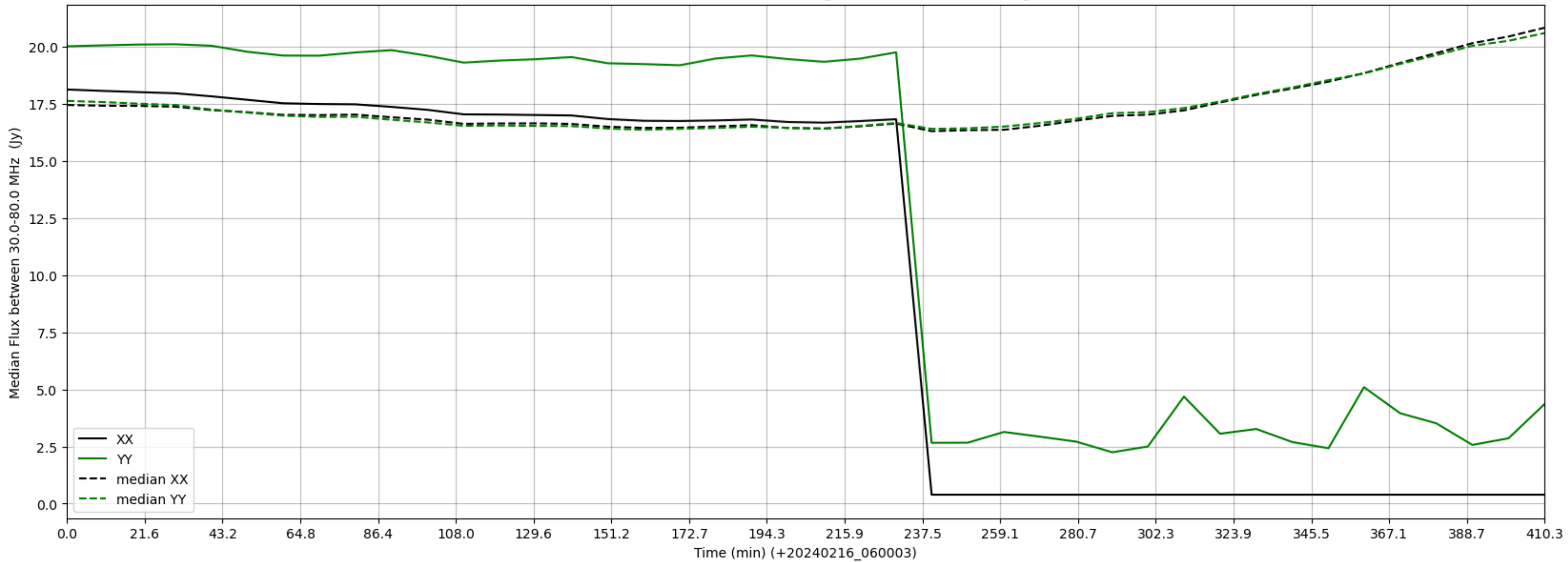
LWA288 - Correlator# 042 - XX FLAGS:HighTimeVar - YY FLAGS:HighTimeVar
