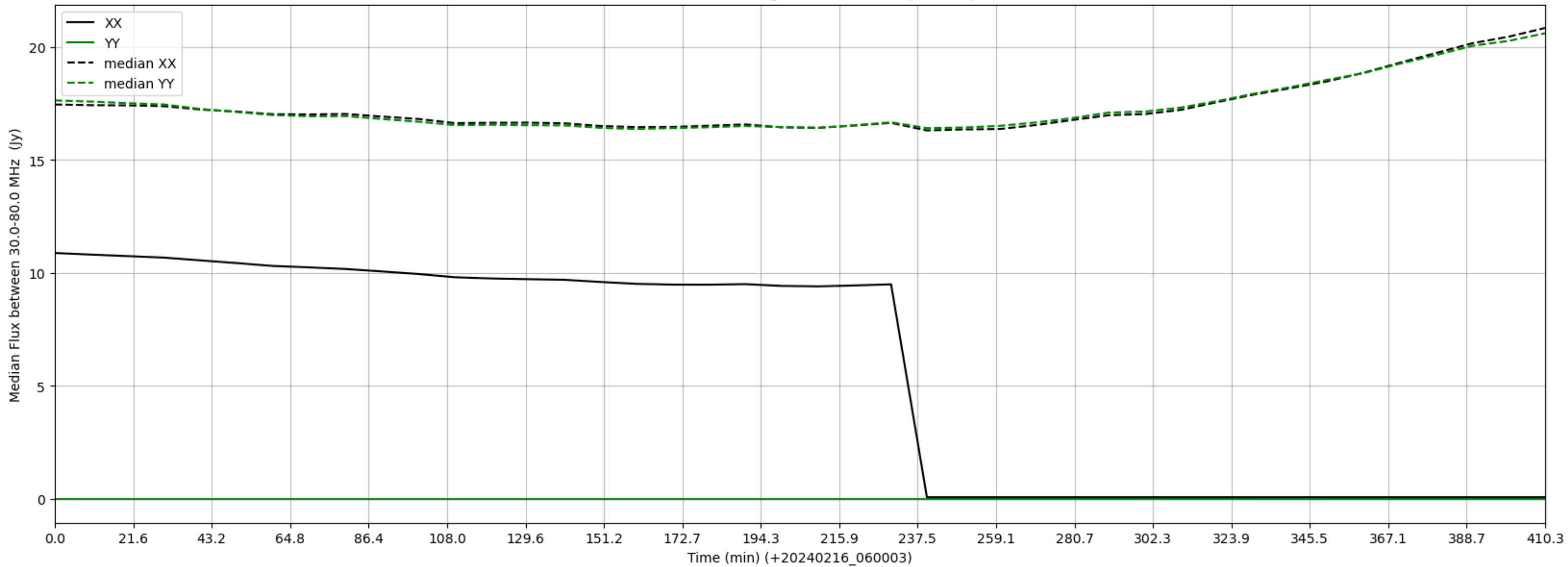
LWA292 - Correlator# 044 - XX FLAGS:HighTimeVar+BadSpecShape - YY FLAGS:LowFlux
