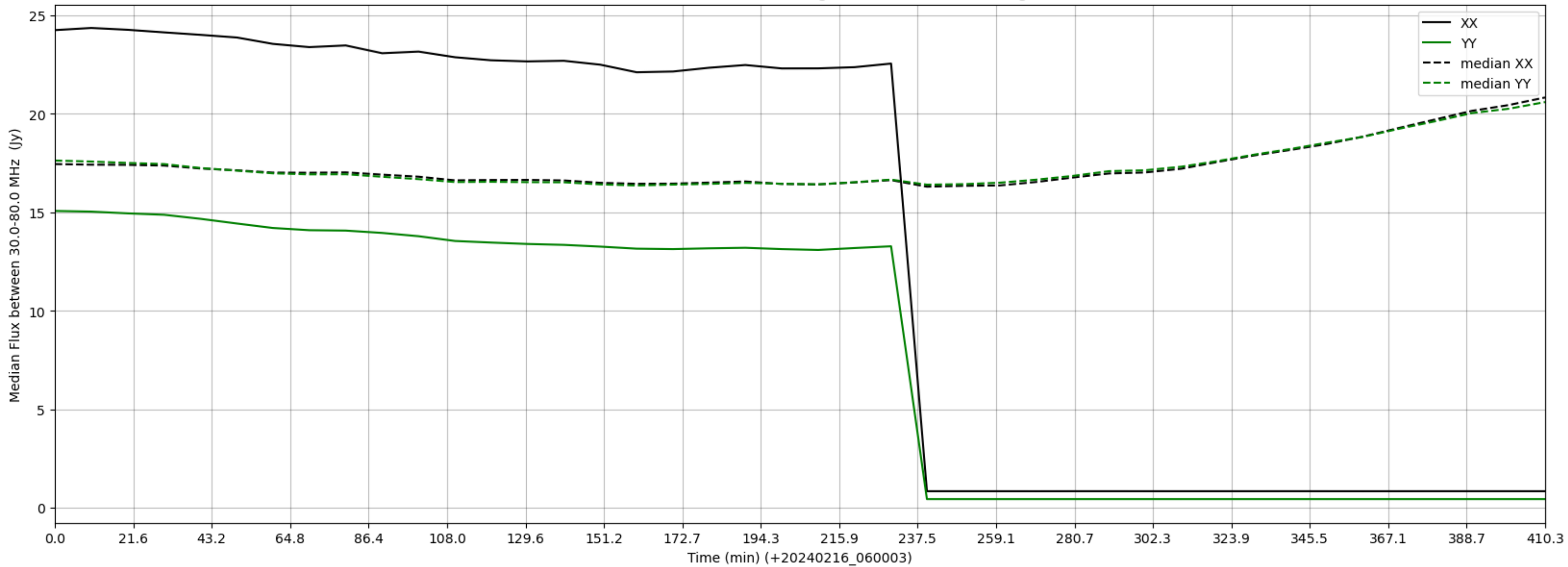
LWA286 - Correlator# 093 - XX FLAGS:HighTimeVar - YY FLAGS:HighTimeVar
