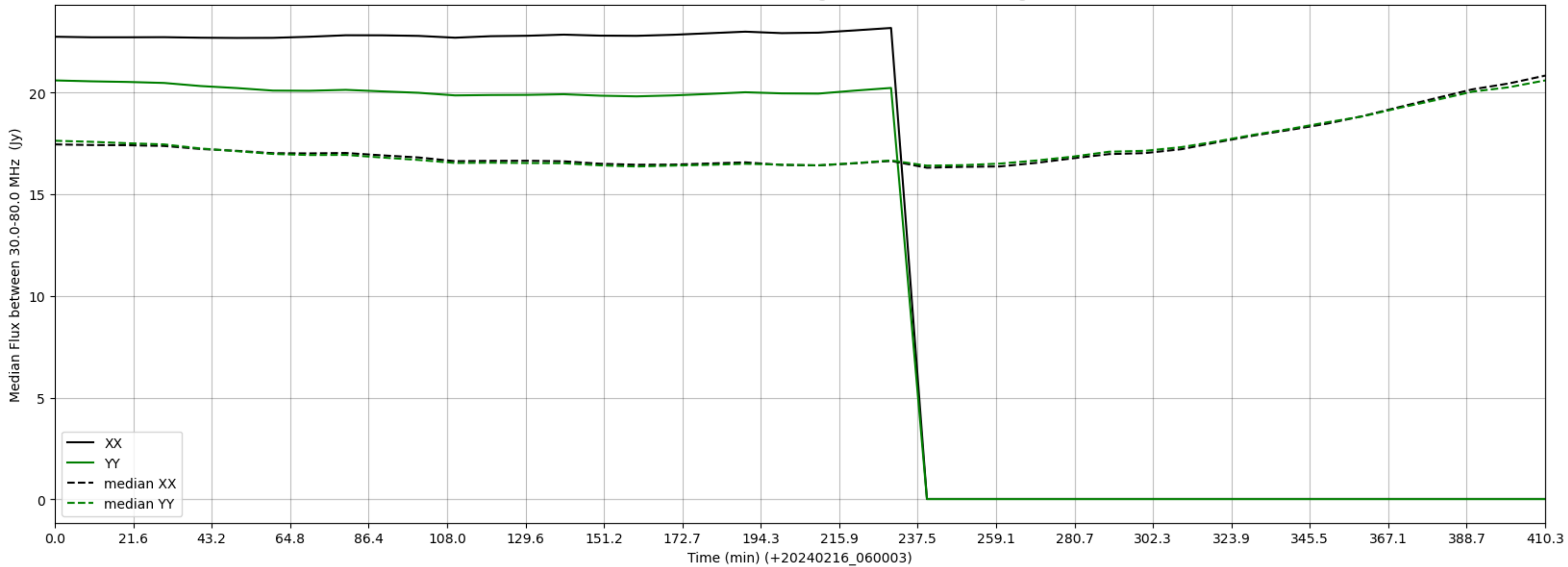
LWA281 - Correlator# 011 - XX FLAGS:HighTimeVar - YY FLAGS:HighTimeVar
