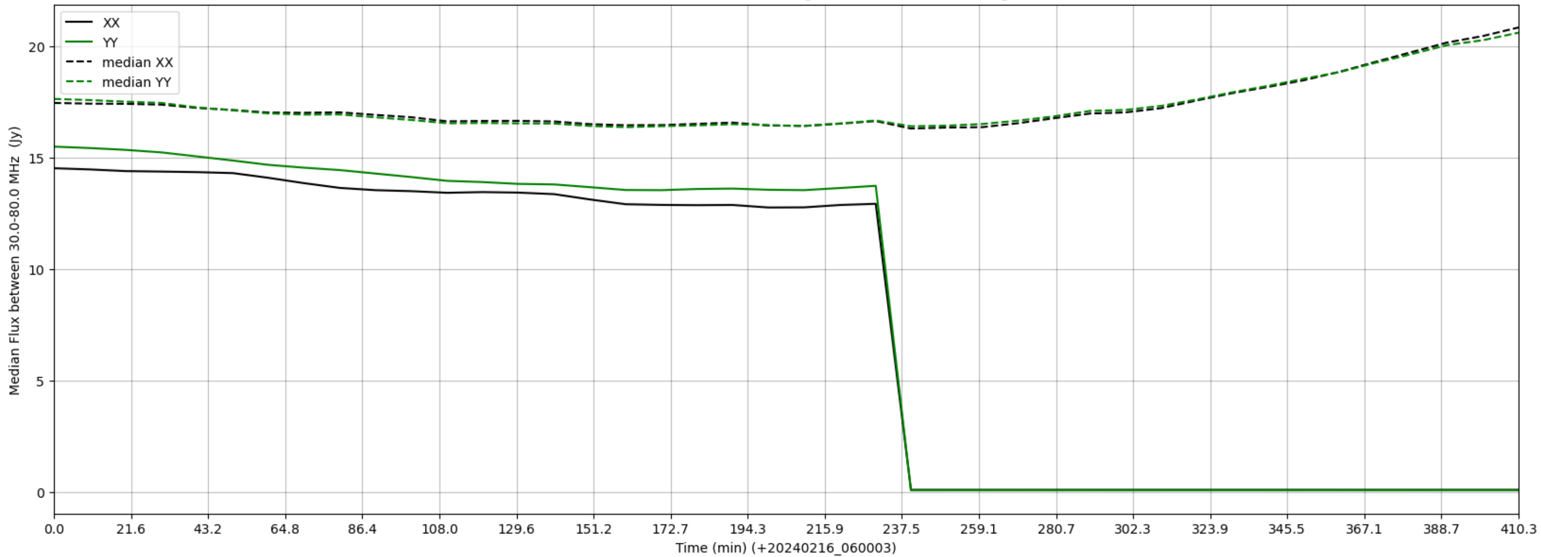
LWA334 - Correlator# 156 - XX FLAGS:HighTimeVar - YY FLAGS:HighTimeVar
