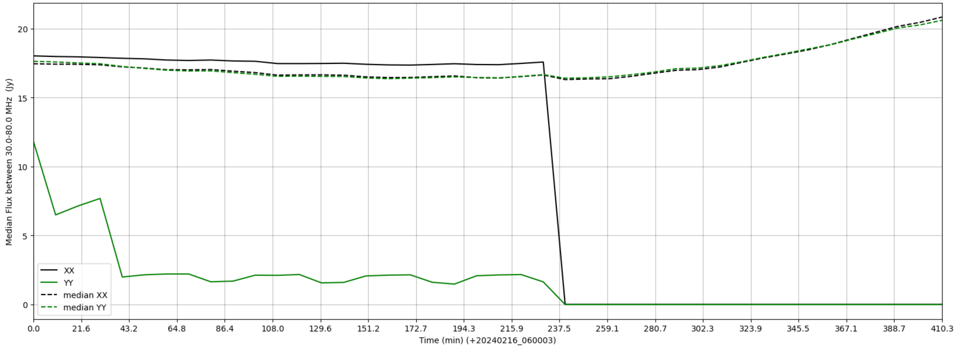
LWA307 - Correlator# 012 - XX FLAGS:HighTimeVar - YY FLAGS:LowFlux
