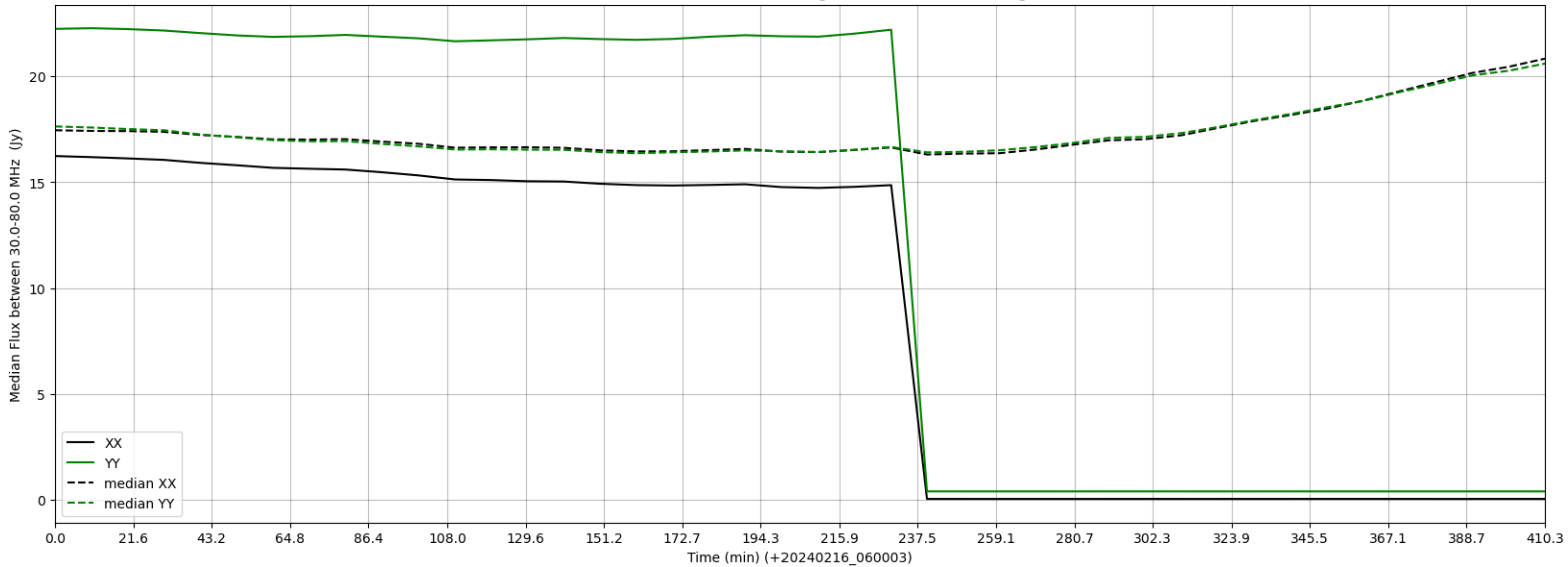
LWA311 - Correlator# 016 - XX FLAGS:HighTimeVar - YY FLAGS:HighTimeVar
