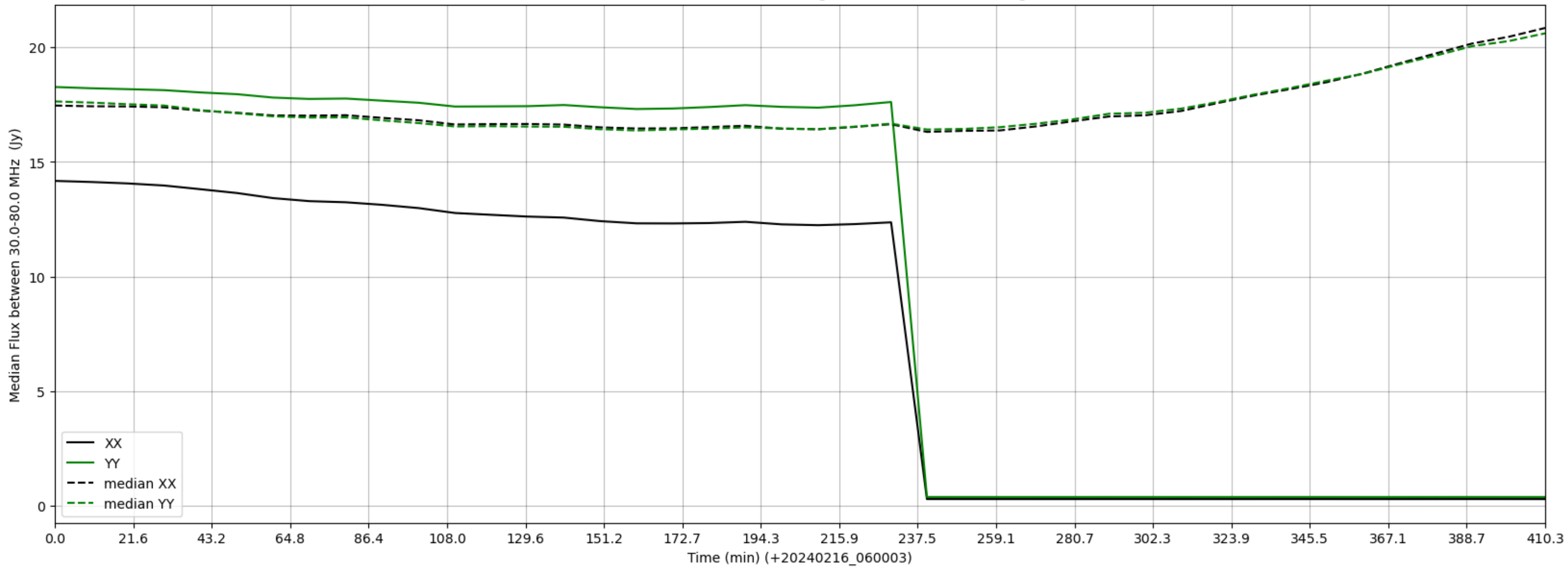
LWA338 - Correlator# 024 - XX FLAGS:HighTimeVar - YY FLAGS:HighTimeVar
