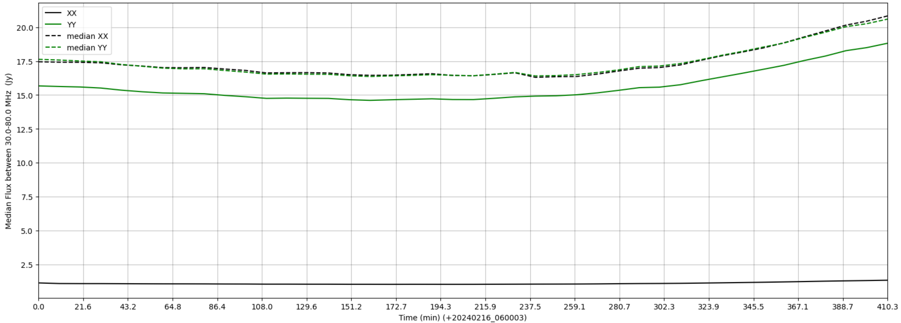
LWA153 - Correlator# 230 - XX FLAGS:LowFlux - YY FLAGS:Good
