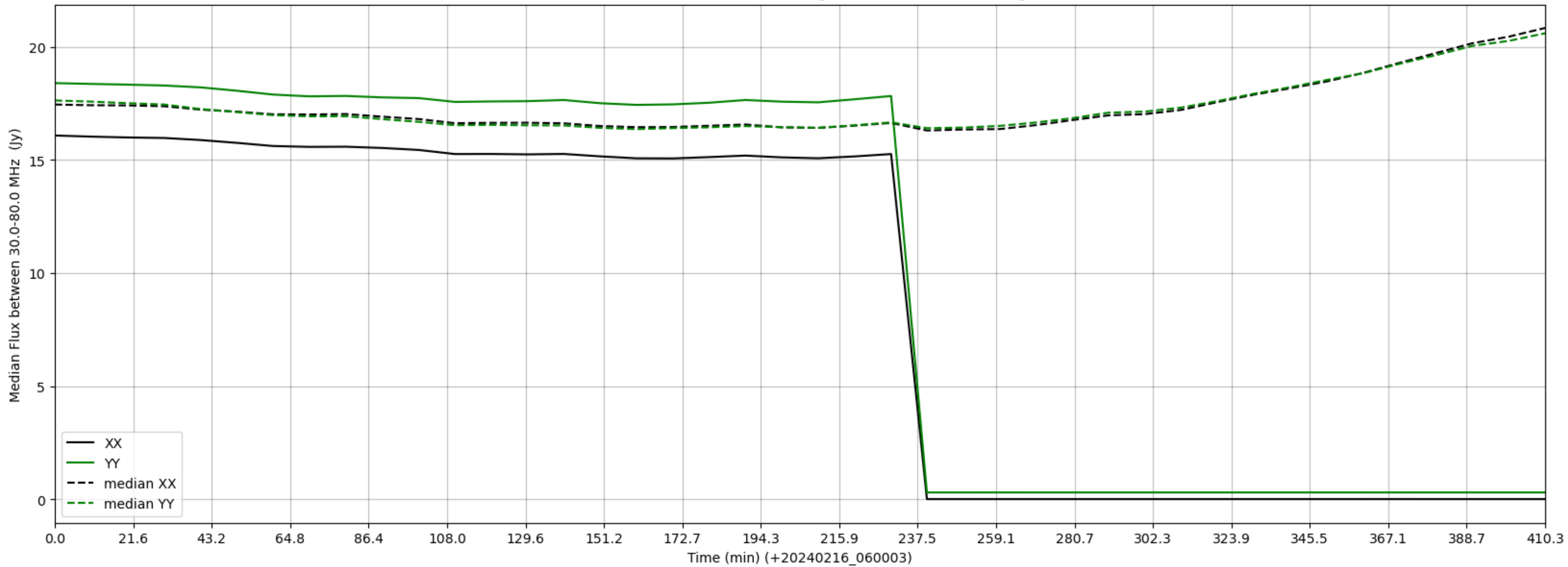
LWA257 - Correlator# 032 - XX FLAGS:HighTimeVar - YY FLAGS:HighTimeVar
