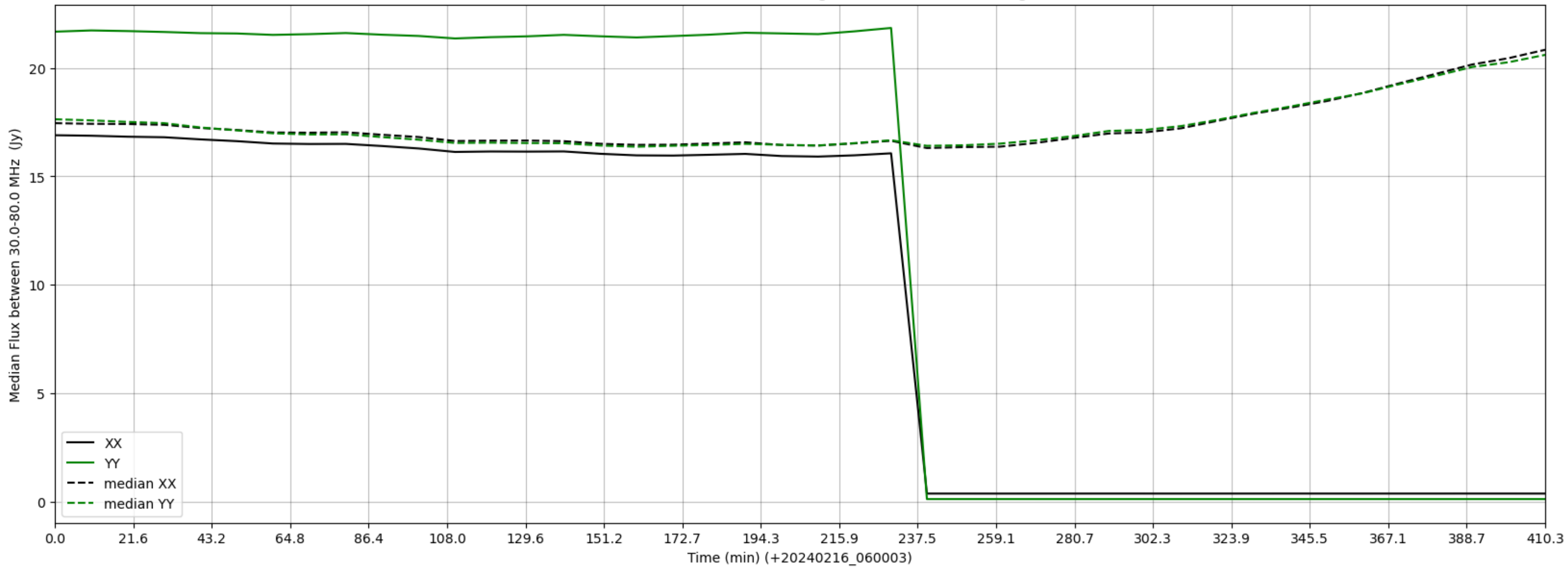
LWA316 - Correlator# 155 - XX FLAGS:HighTimeVar - YY FLAGS:HighTimeVar
