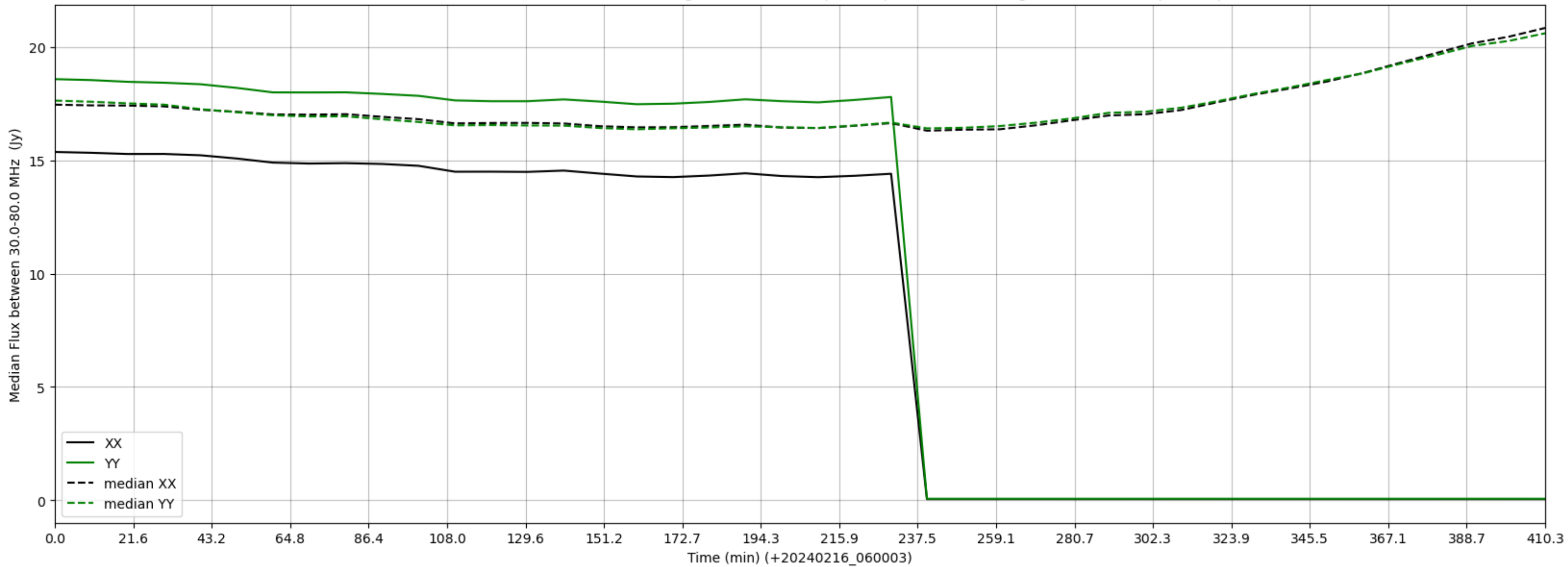
LWA336 - Correlator# 056 - XX FLAGS:HighTimeVar+BadSpecShape - YY FLAGS:HighTimeVar+BadSpecShape
