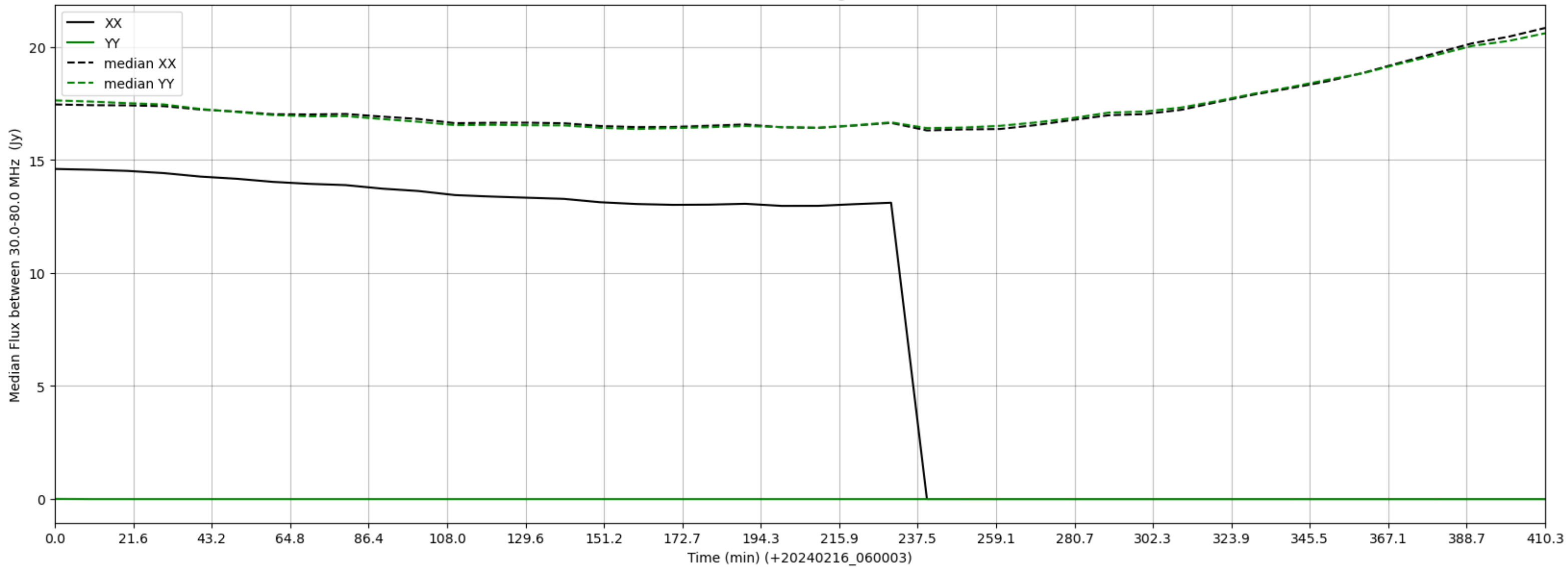
LWA314 - Correlator# 021 - XX FLAGS:HighTimeVar - YY FLAGS:LowFlux
