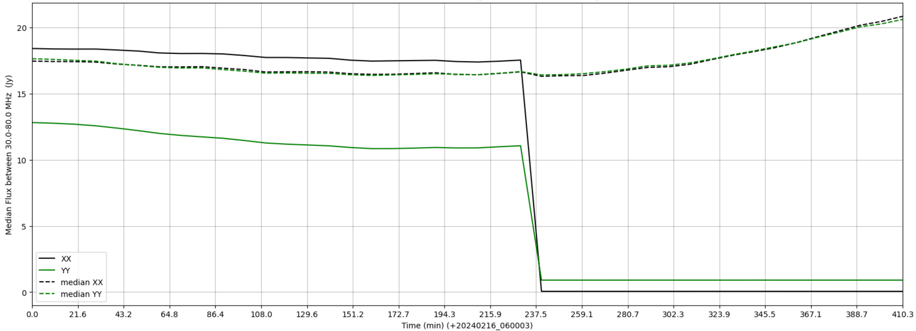
LWA326 - Correlator# 250 - XX FLAGS:HighTimeVar - YY FLAGS:HighTimeVar
