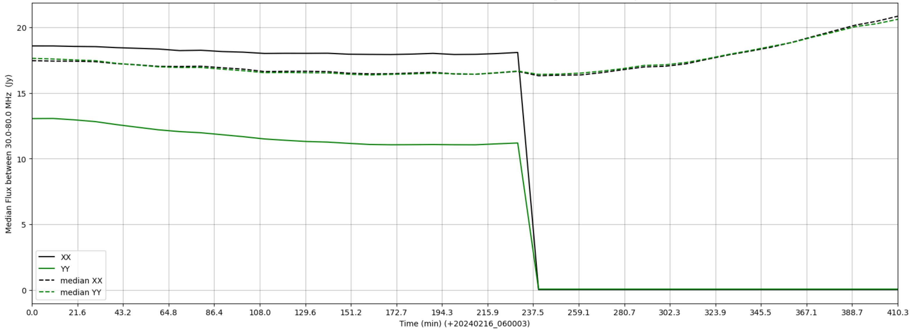
LWA347 - Correlator# 255 - XX FLAGS:HighTimeVar - YY FLAGS:HighTimeVar+BadSpecShape
