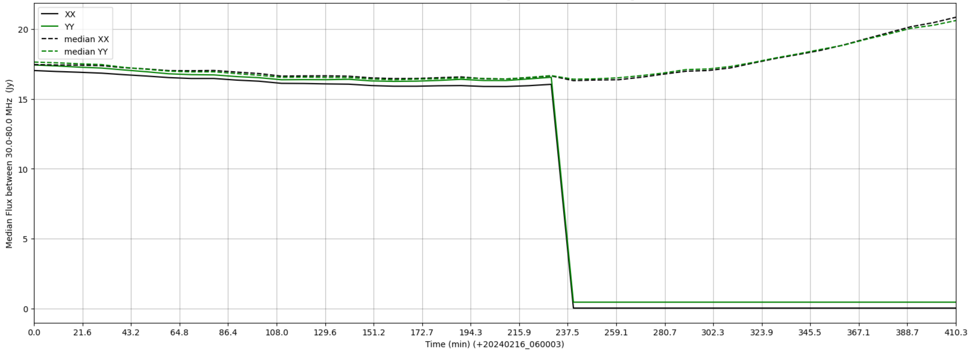
LWA344 - Correlator# 061 - XX FLAGS:HighTimeVar - YY FLAGS:HighTimeVar
