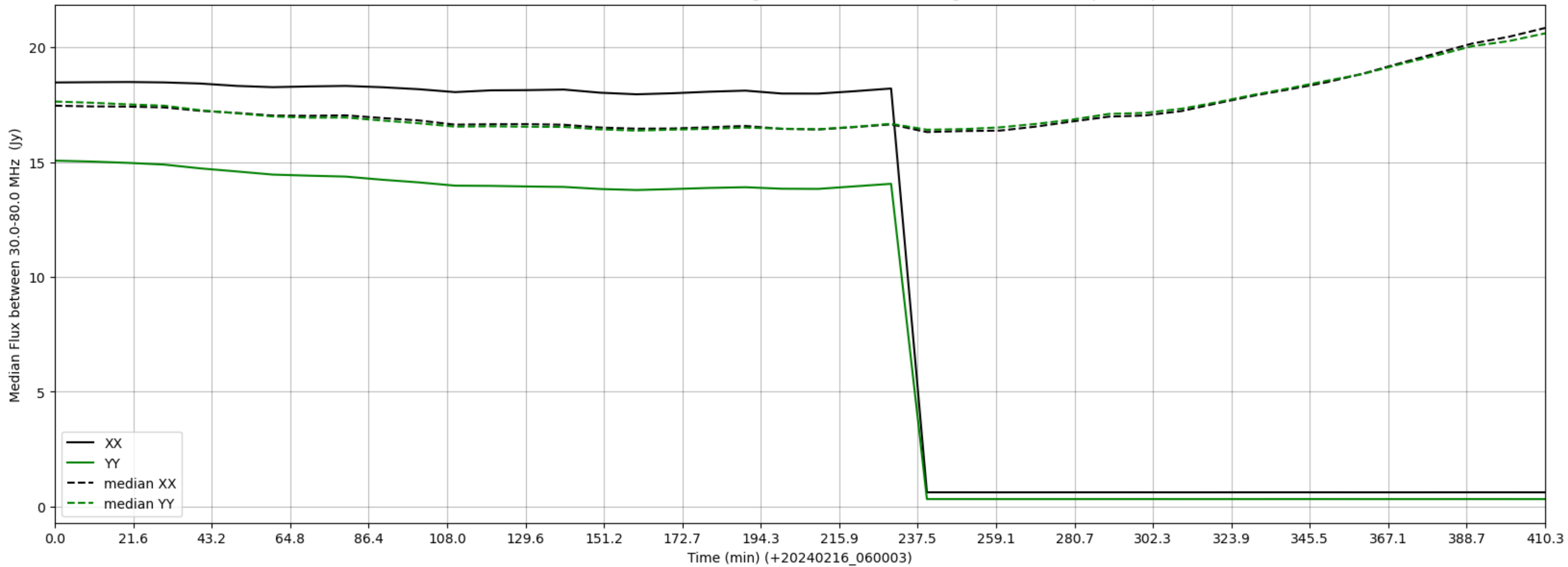
LWA321 - Correlator# 020 - XX FLAGS:HighTimeVar - YY FLAGS:HighTimeVar+BadSpecShape
