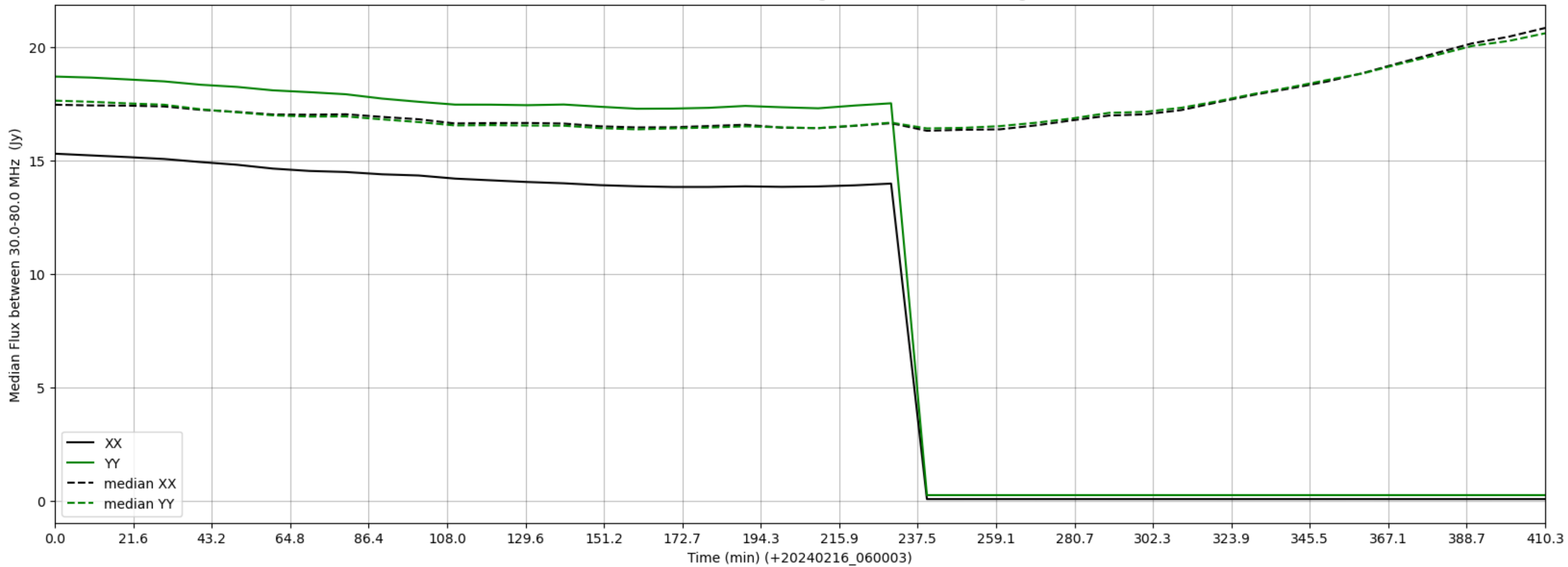
LWA291 - Correlator# 045 - XX FLAGS:HighTimeVar - YY FLAGS:HighTimeVar
