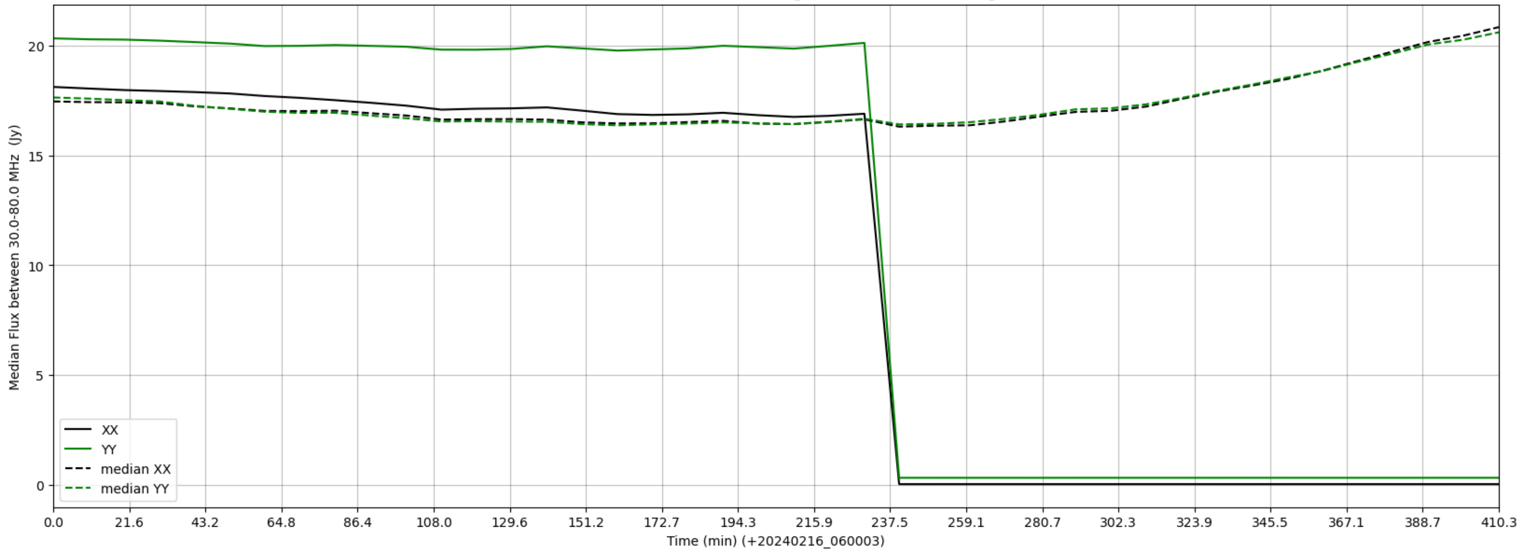
LWA332 - Correlator# 025 - XX FLAGS:HighTimeVar - YY FLAGS:HighTimeVar
