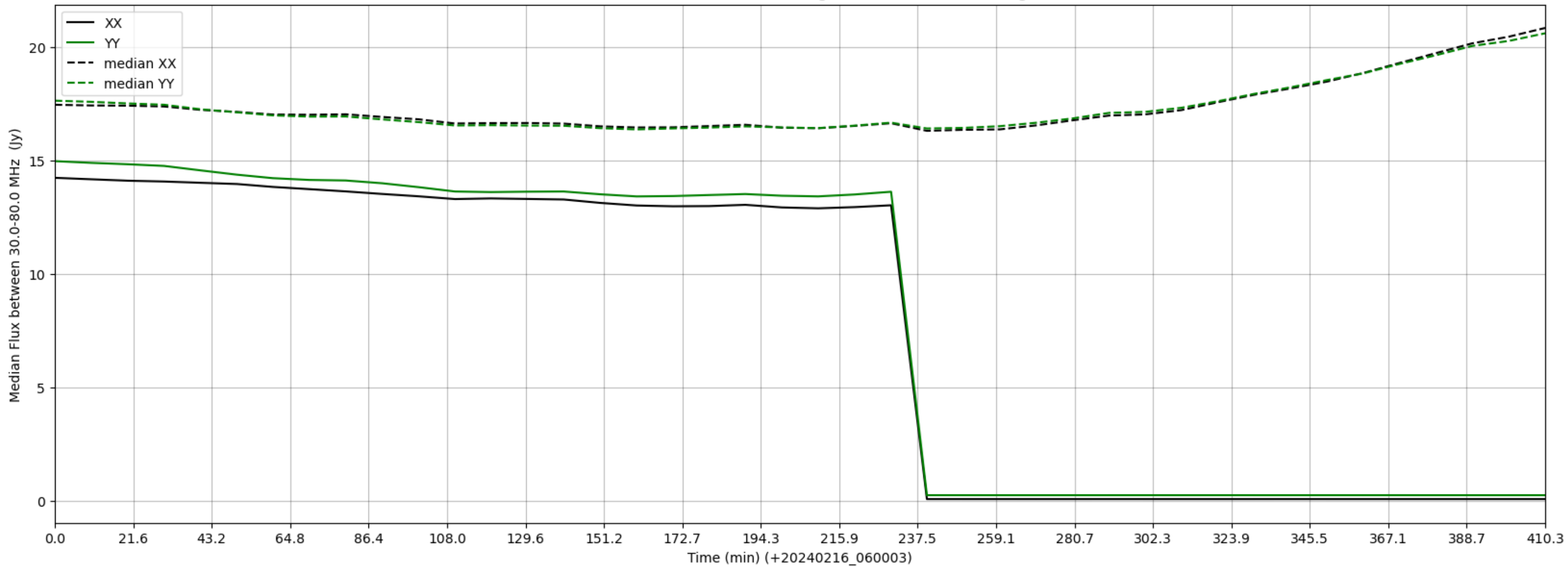
LWA337 - Correlator# 059 - XX FLAGS:HighTimeVar - YY FLAGS:HighTimeVar
