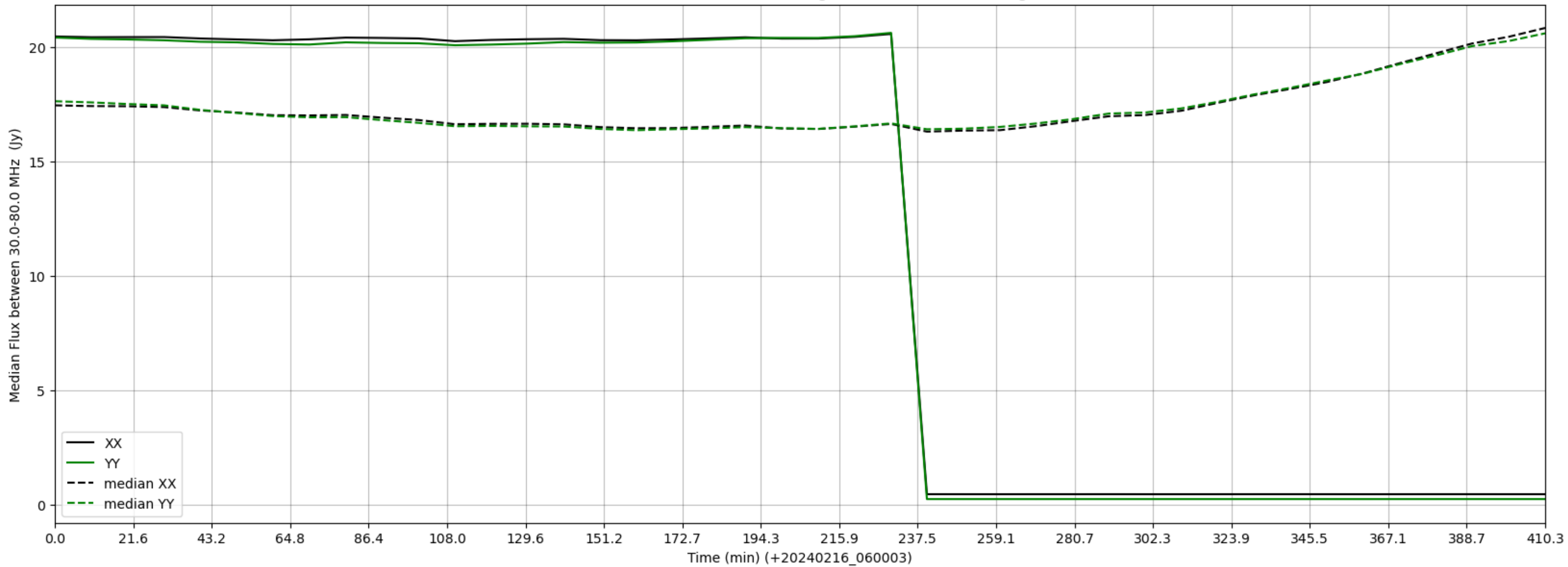
LWA333 - Correlator# 253 - XX FLAGS:HighTimeVar - YY FLAGS:HighTimeVar
