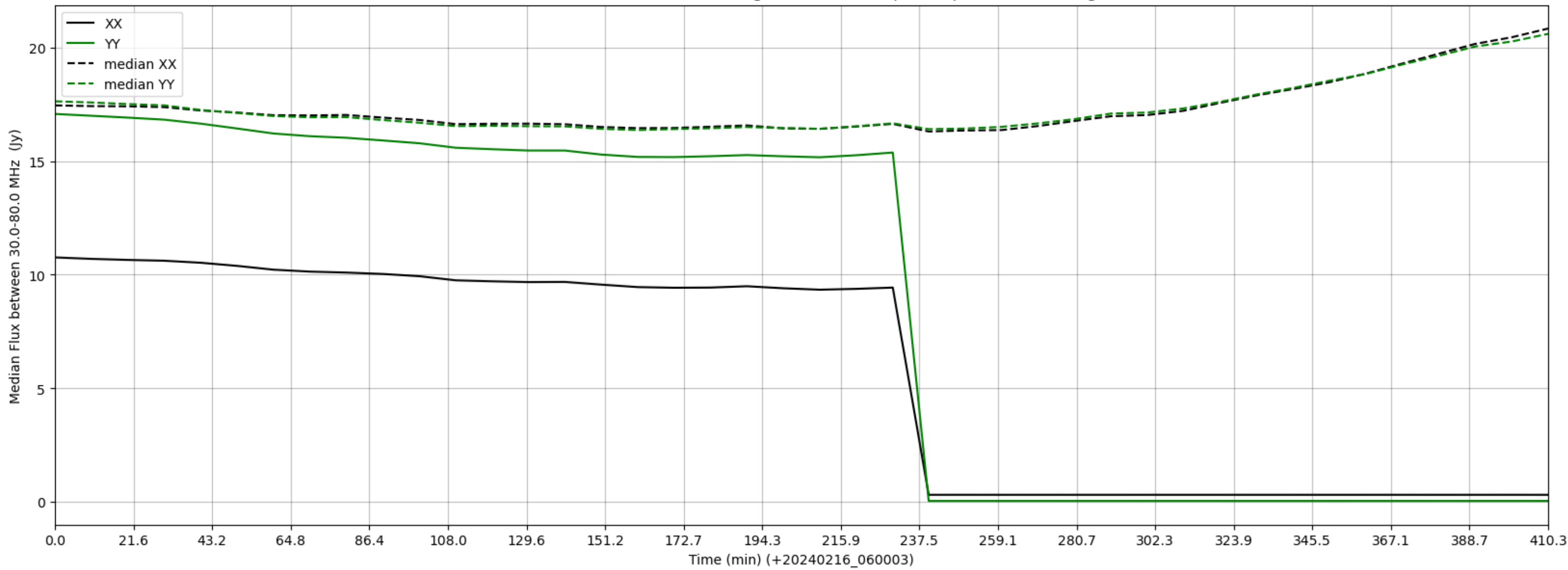
LWA283 - Correlator# 040 - XX FLAGS:HighTimeVar+BadSpecShape - YY FLAGS:HighTimeVar
