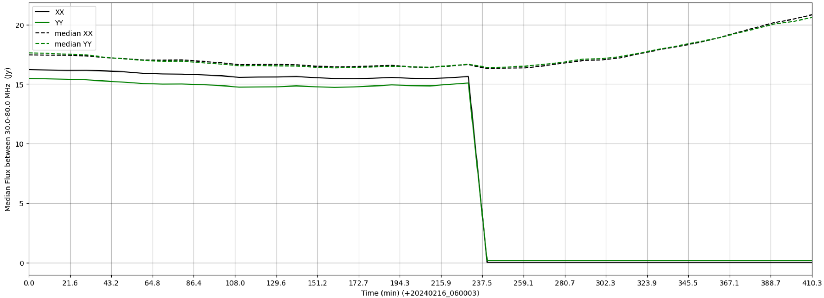
LWA289 - Correlator# 189 - XX FLAGS:HighTimeVar - YY FLAGS:HighTimeVar+BadSpecShape
