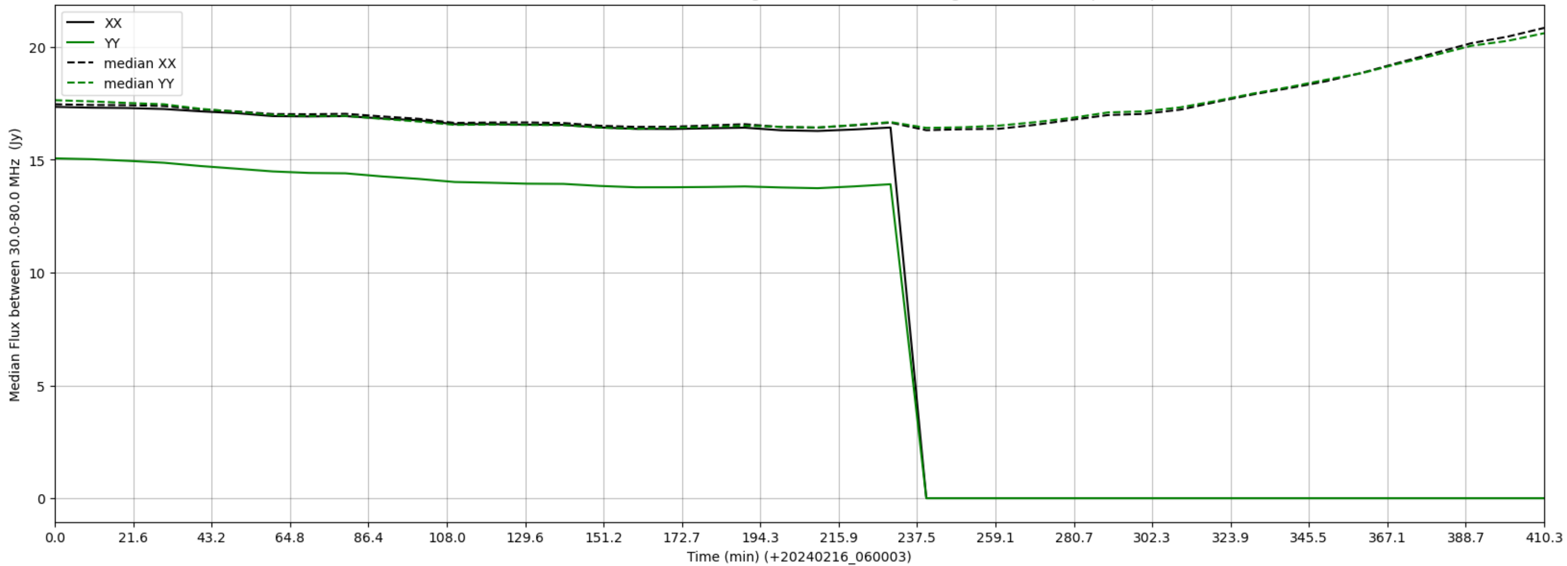
LWA260 - Correlator# 034 - XX FLAGS:HighTimeVar - YY FLAGS:HighTimeVar+BadSpecShape
