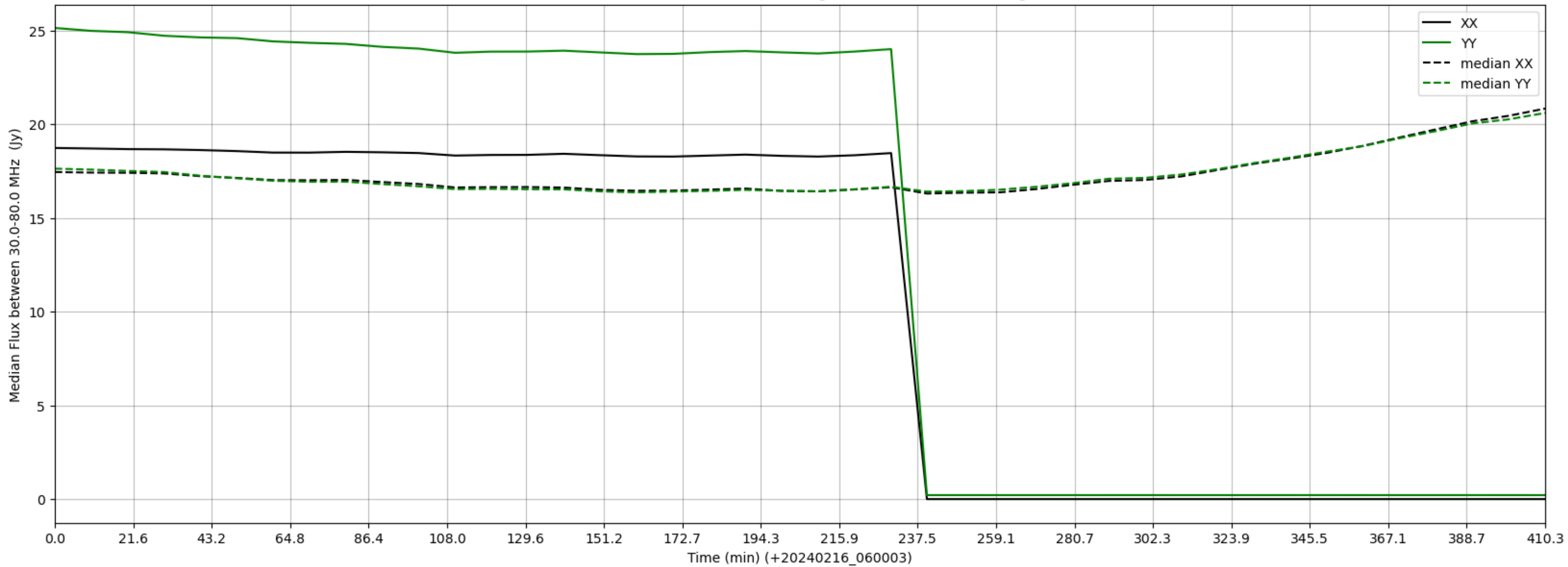
LWA322 - Correlator# 251 - XX FLAGS:HighTimeVar - YY FLAGS:HighTimeVar
