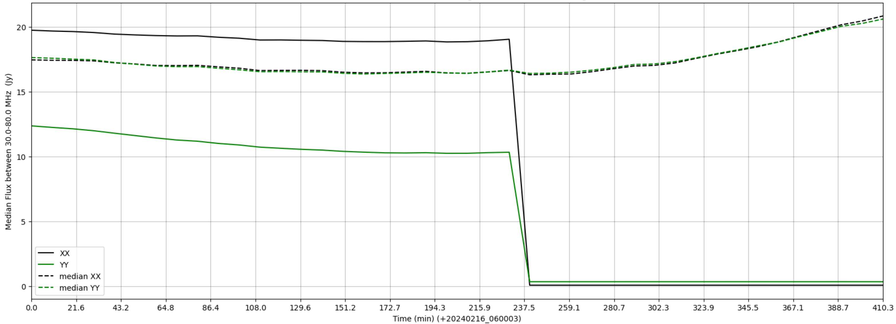
LWA290 - Correlator# 285 - XX FLAGS:HighTimeVar - YY FLAGS:HighTimeVar
