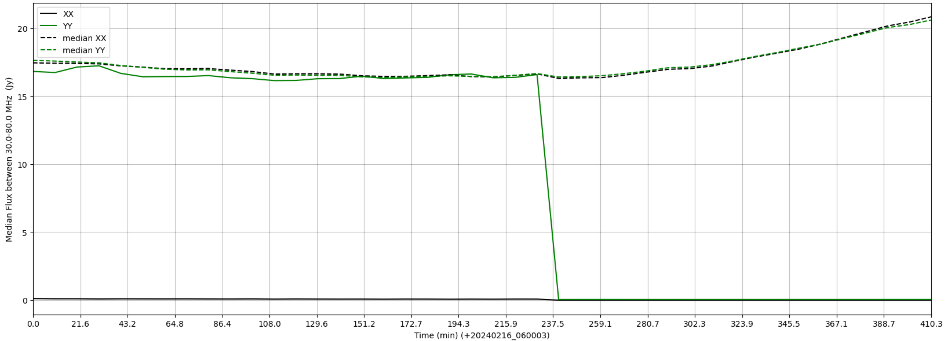
LWA310 - Correlator# 017 - XX FLAGS:LowFlux - YY FLAGS:HighTimeVar
