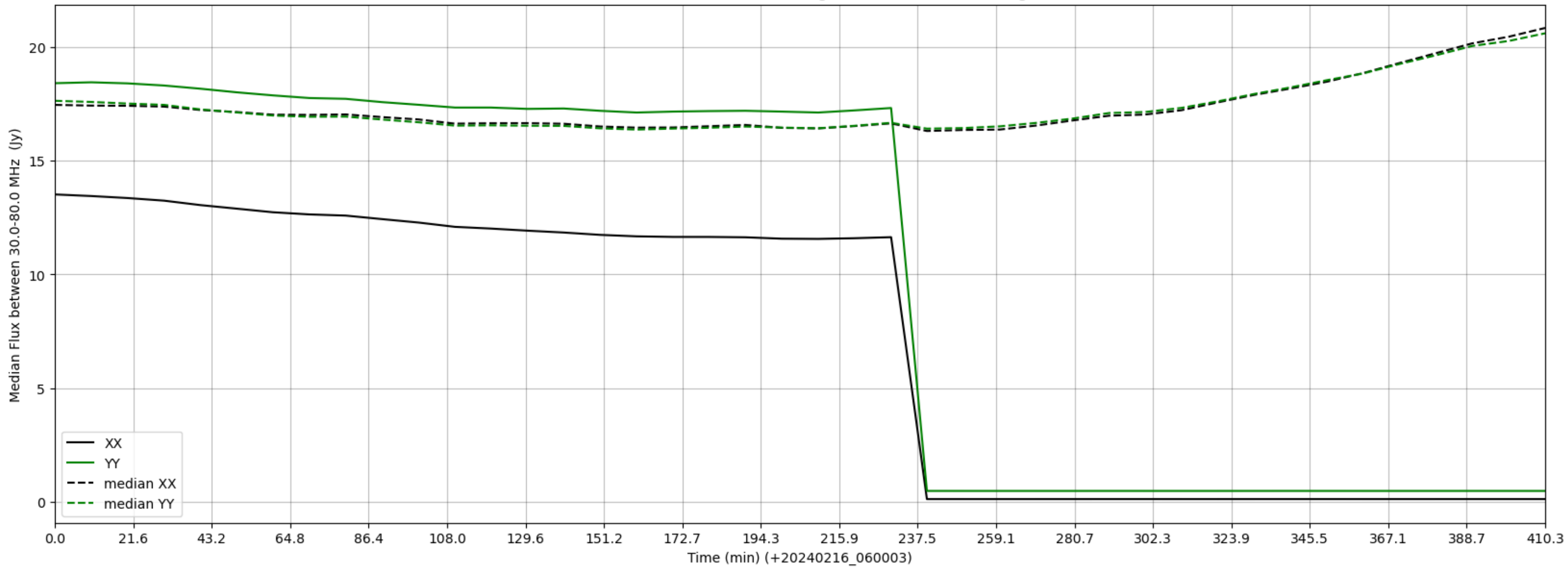
LWA342 - Correlator# 317 - XX FLAGS:HighTimeVar - YY FLAGS:HighTimeVar
