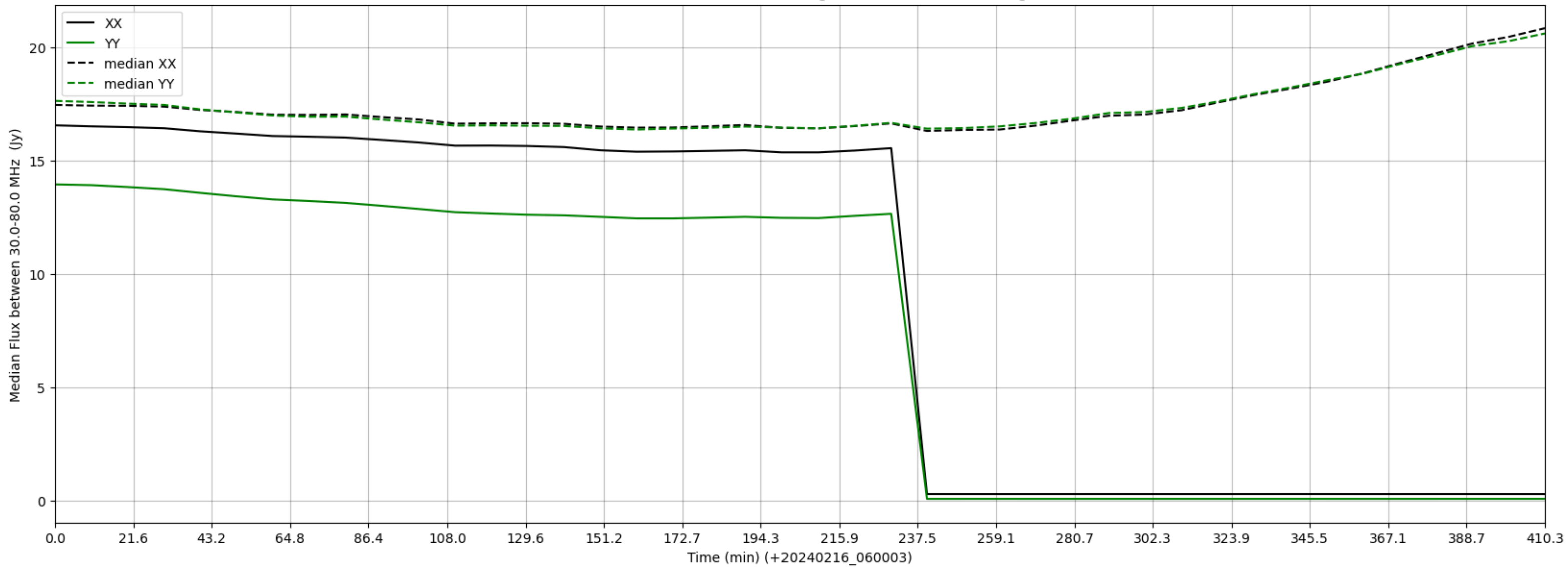
LWA330 - Correlator# 022 - XX FLAGS:HighTimeVar - YY FLAGS:HighTimeVar
