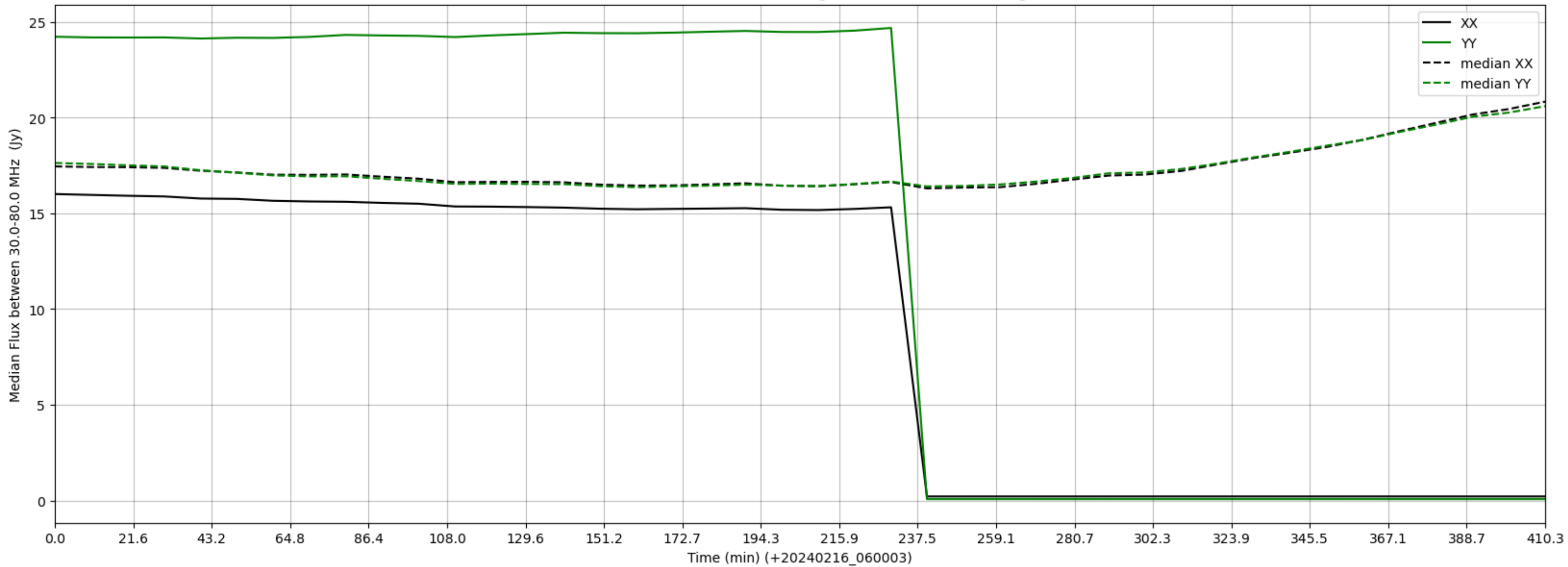
LWA331 - Correlator# 125 - XX FLAGS:HighTimeVar - YY FLAGS:HighTimeVar
