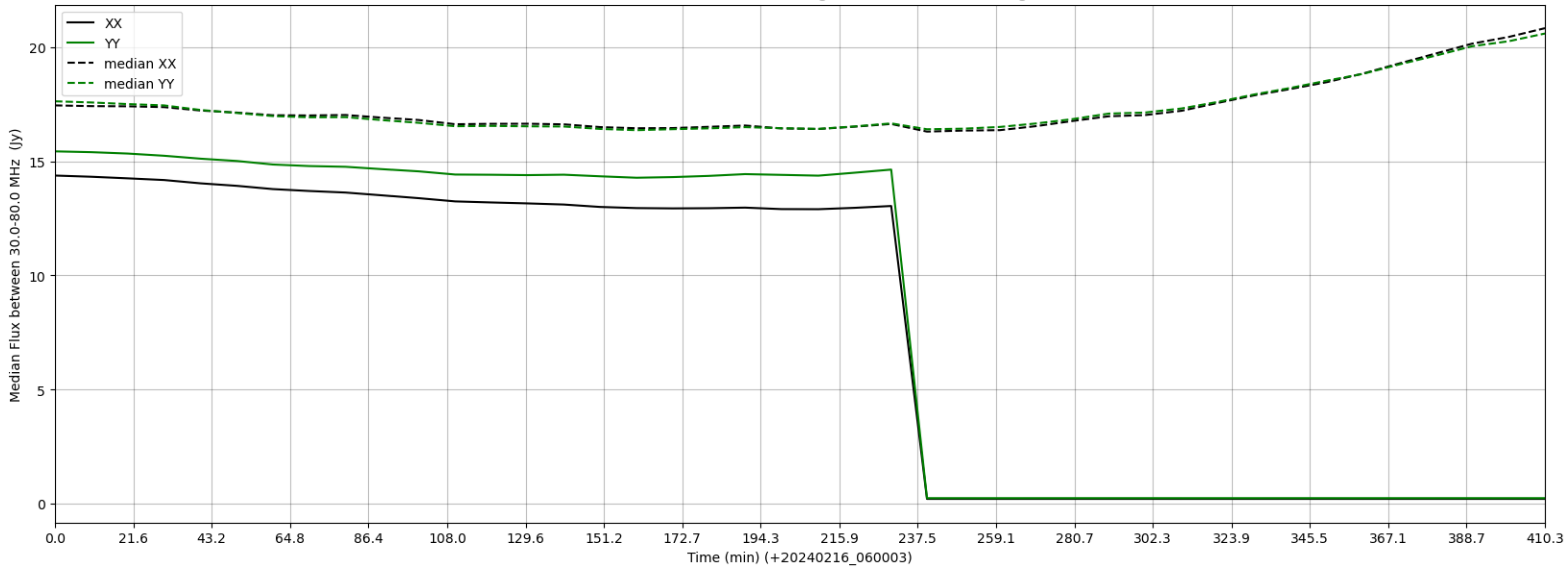
LWA276 - Correlator# 006 - XX FLAGS:HighTimeVar - YY FLAGS:HighTimeVar
