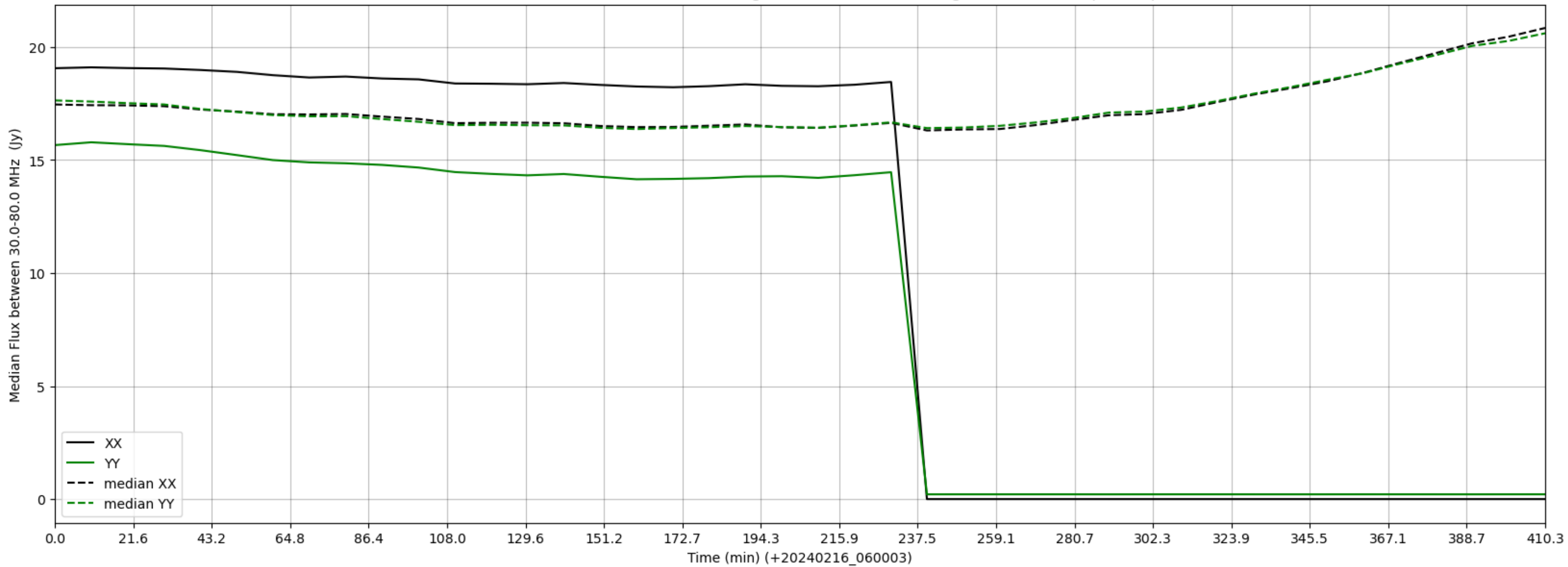
LWA348 - Correlator# 124 - XX FLAGS:HighTimeVar - YY FLAGS:HighTimeVar+BadSpecShape
