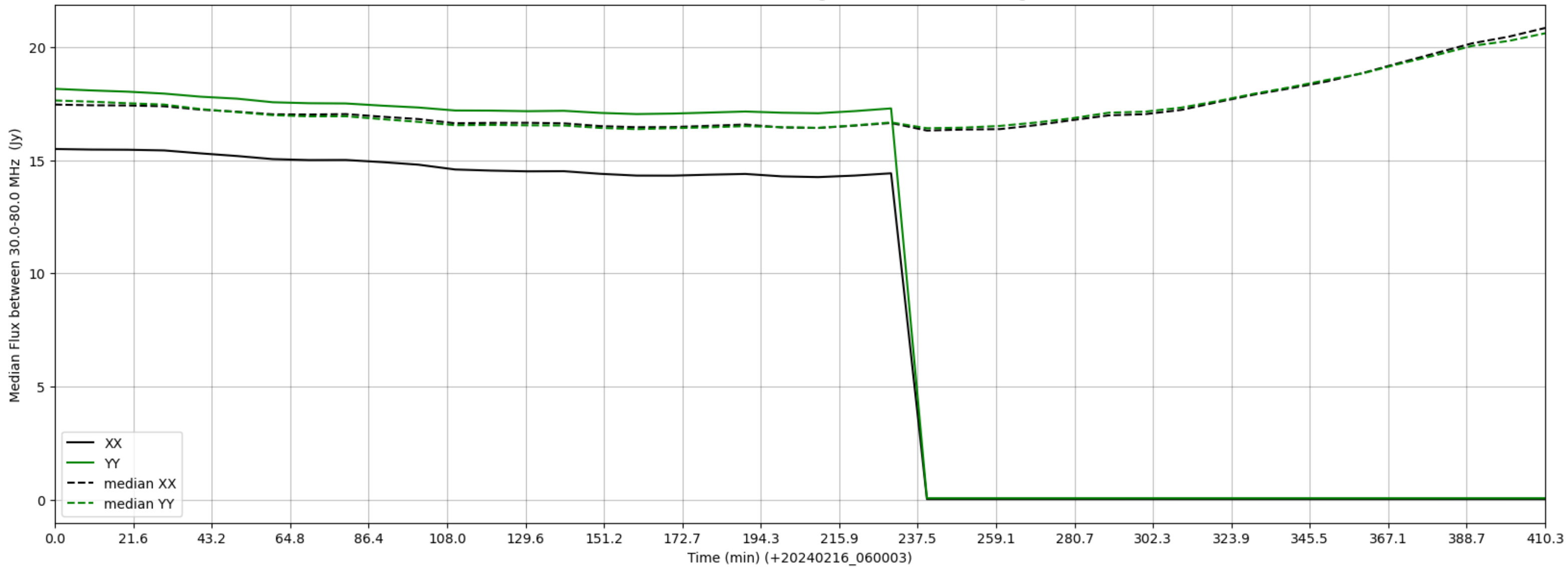
LWA278 - Correlator# 008 - XX FLAGS:HighTimeVar - YY FLAGS:HighTimeVar
