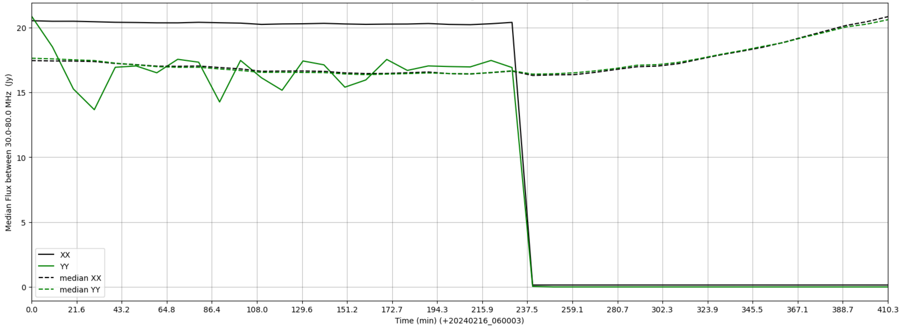
LWA309 - Correlator# 014 - XX FLAGS:HighTimeVar - YY FLAGS:HighTimeVar
