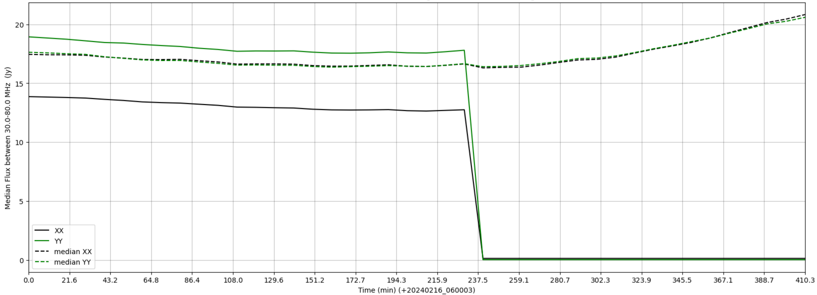
LWA285 - Correlator# 013 - XX FLAGS:HighTimeVar - YY FLAGS:HighTimeVar
