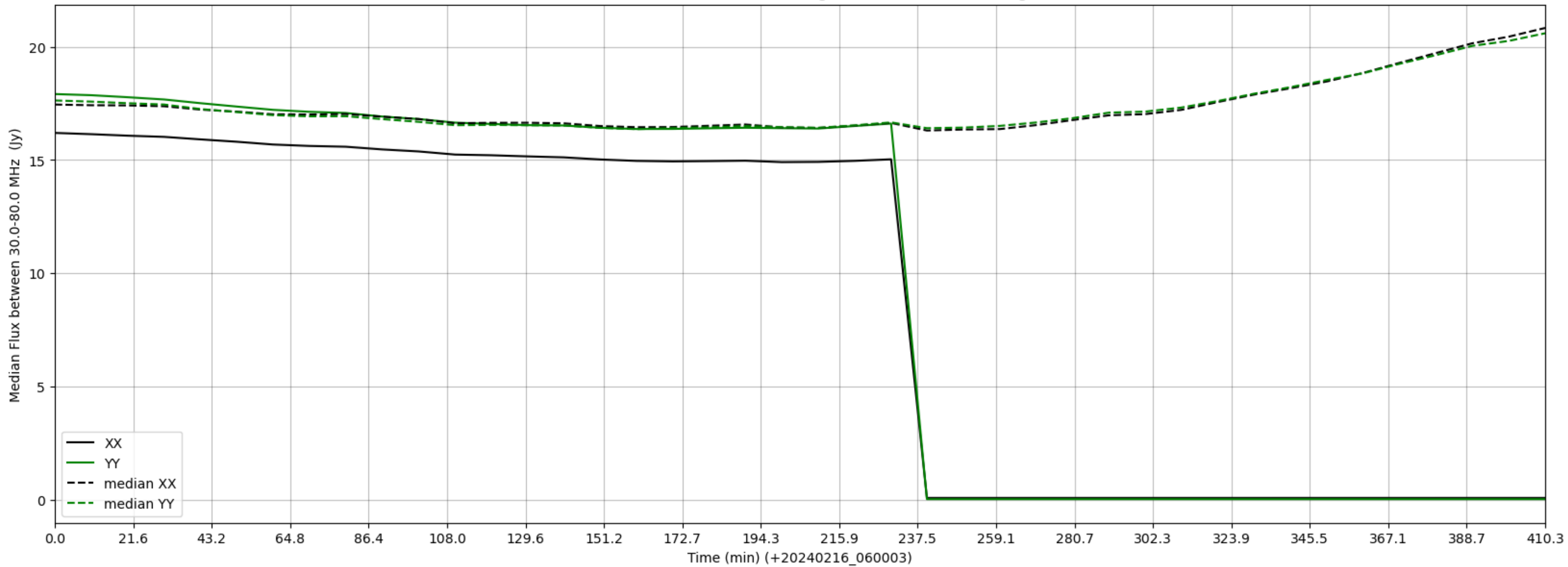
LWA273 - Correlator# 007 - XX FLAGS:HighTimeVar - YY FLAGS:HighTimeVar
