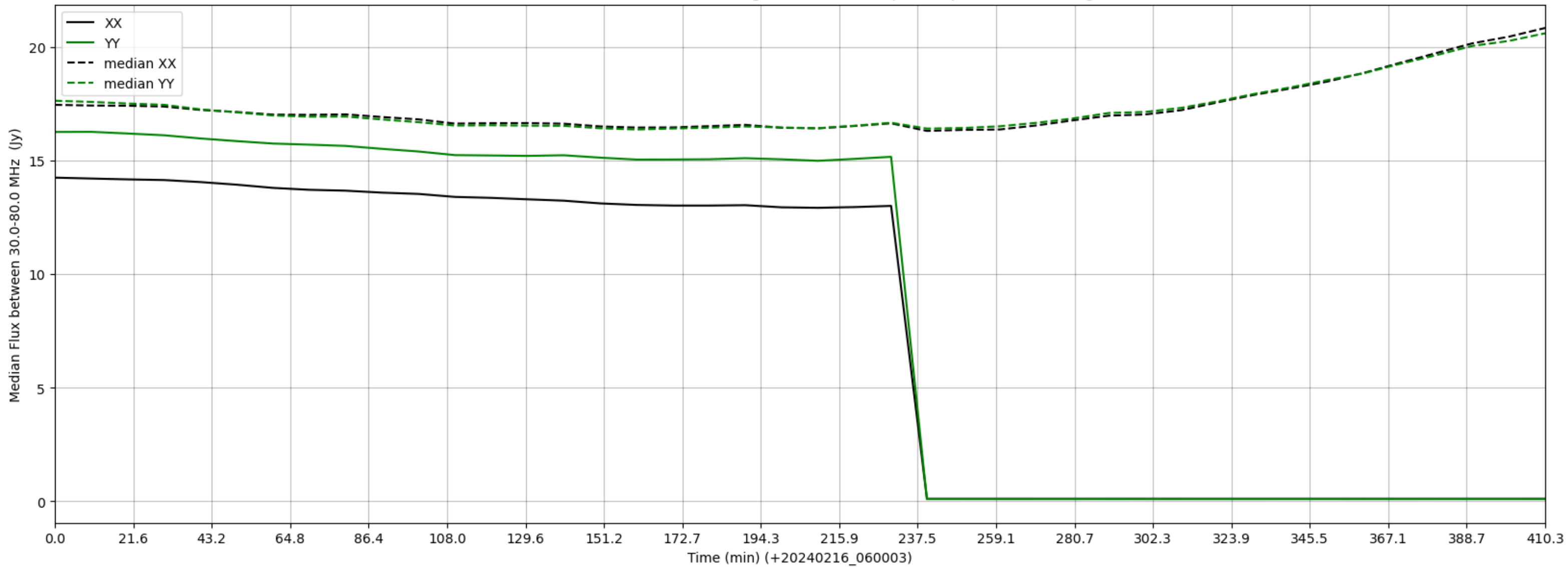
LWA340 - Correlator# 026 - XX FLAGS:HighTimeVar+BadSpecShape - YY FLAGS:HighTimeVar
