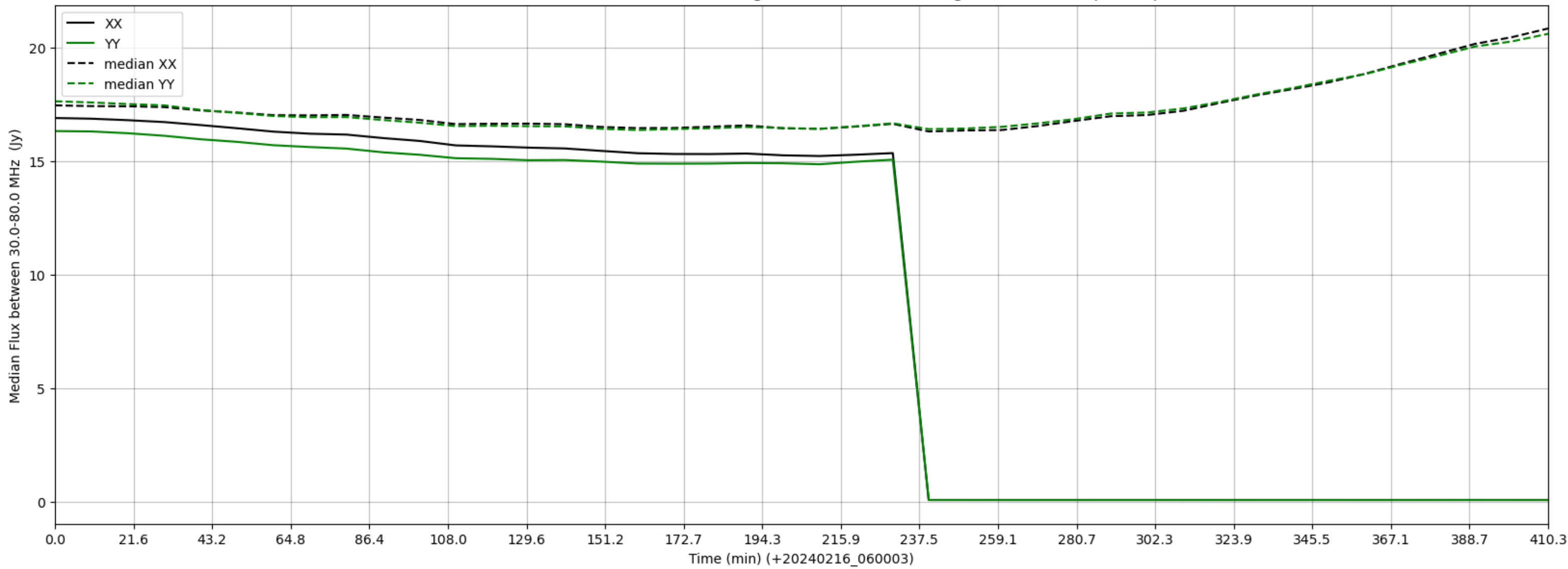
LWA349 - Correlator# 282 - XX FLAGS:HighTimeVar - YY FLAGS:HighTimeVar+BadSpecShape
