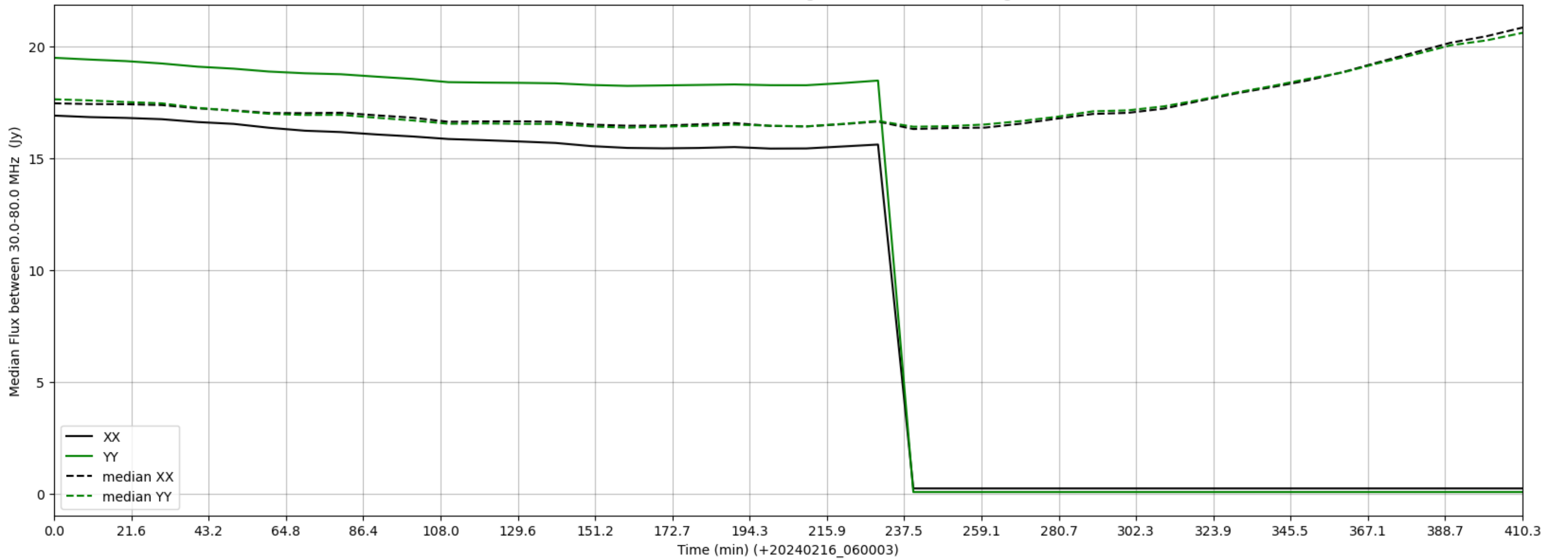
LWA329 - Correlator# 287 - XX FLAGS:HighTimeVar - YY FLAGS:HighTimeVar
