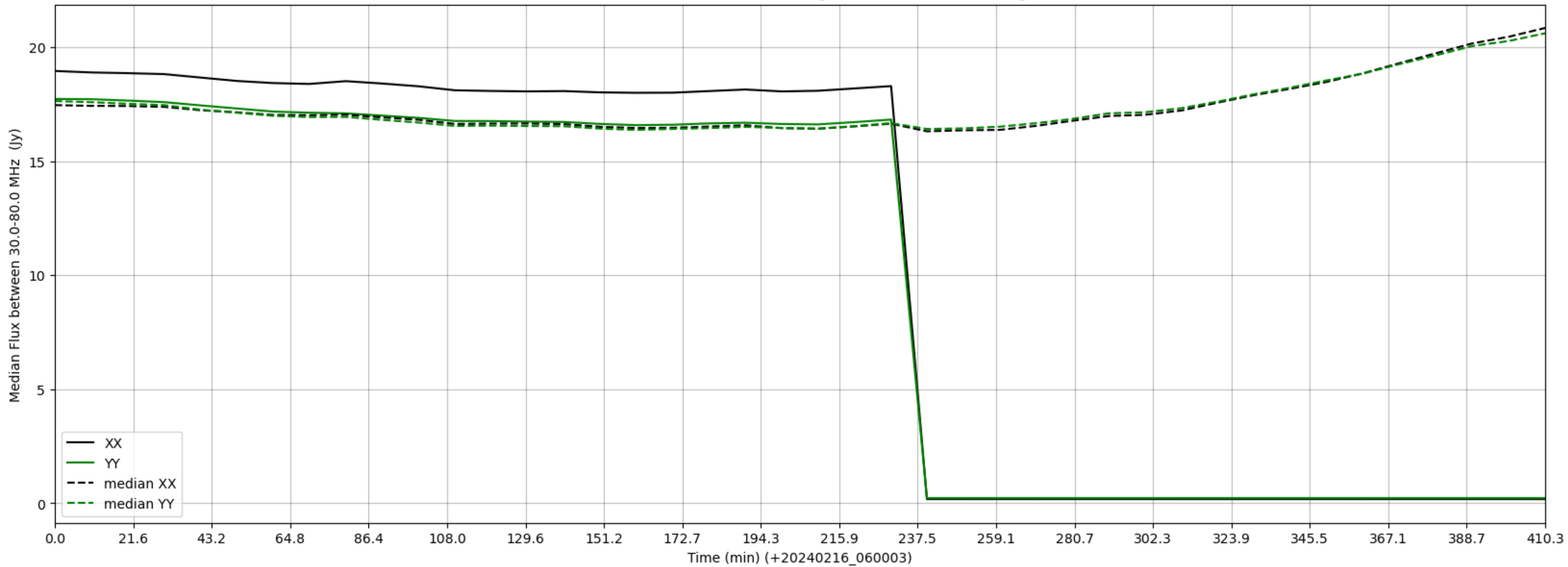
LWA327 - Correlator# 023 - XX FLAGS:HighTimeVar - YY FLAGS:HighTimeVar
