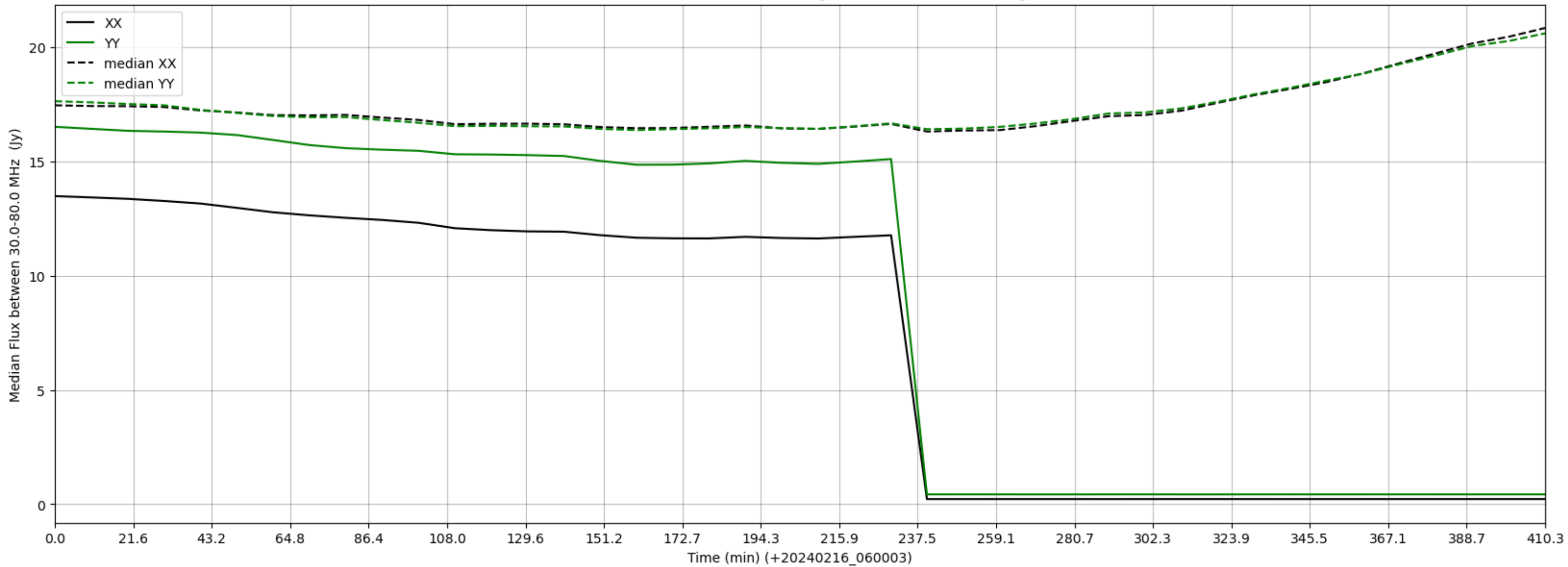
LWA275 - Correlator# 090 - XX FLAGS:HighTimeVar - YY FLAGS:HighTimeVar
