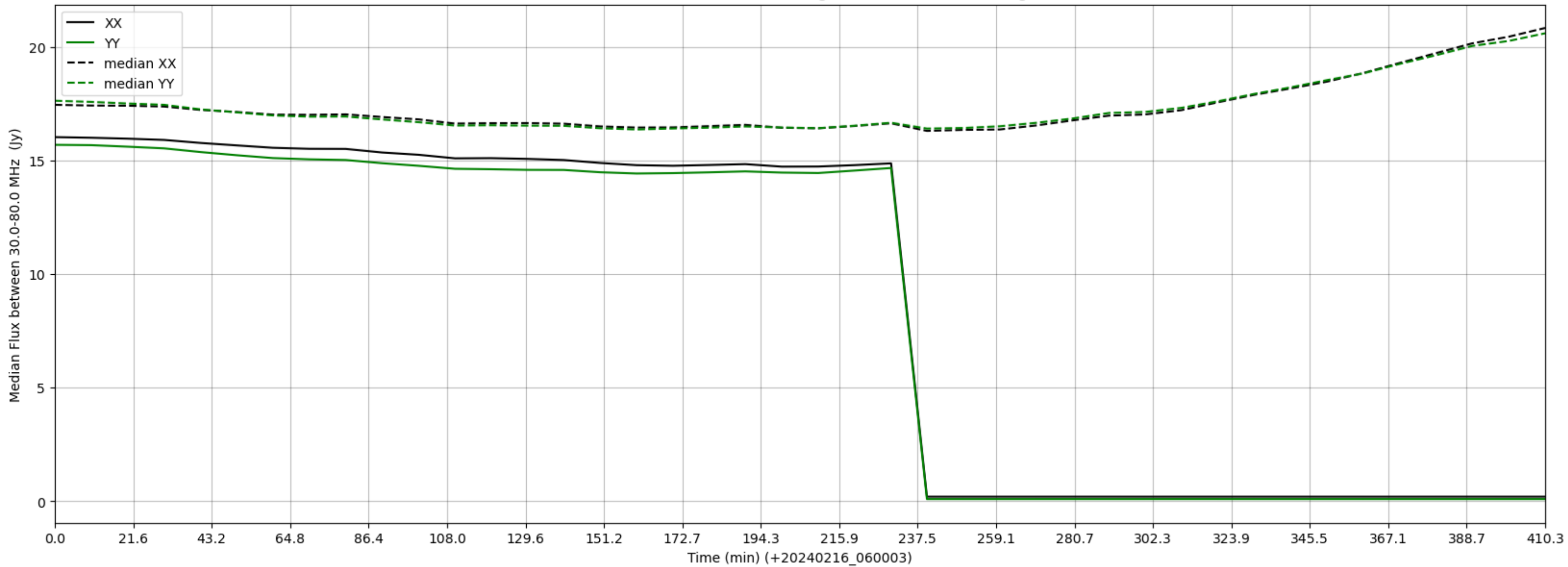
LWA320 - Correlator# 054 - XX FLAGS:HighTimeVar - YY FLAGS:HighTimeVar
