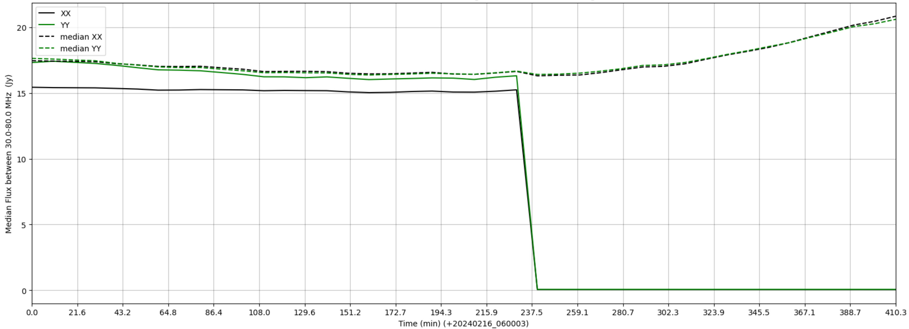
LWA353 - Correlator# 031 - XX FLAGS:HighTimeVar - YY FLAGS:HighTimeVar
