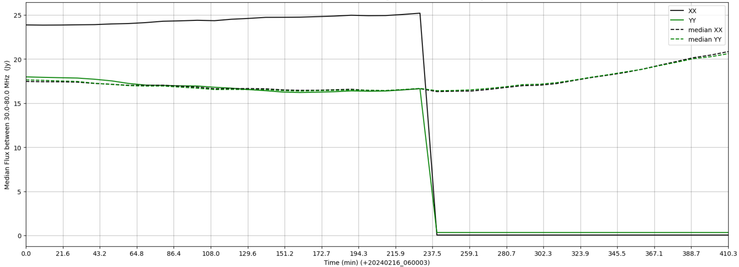
LWA308 - Correlator# 015 - XX FLAGS:HighTimeVar - YY FLAGS:HighTimeVar
