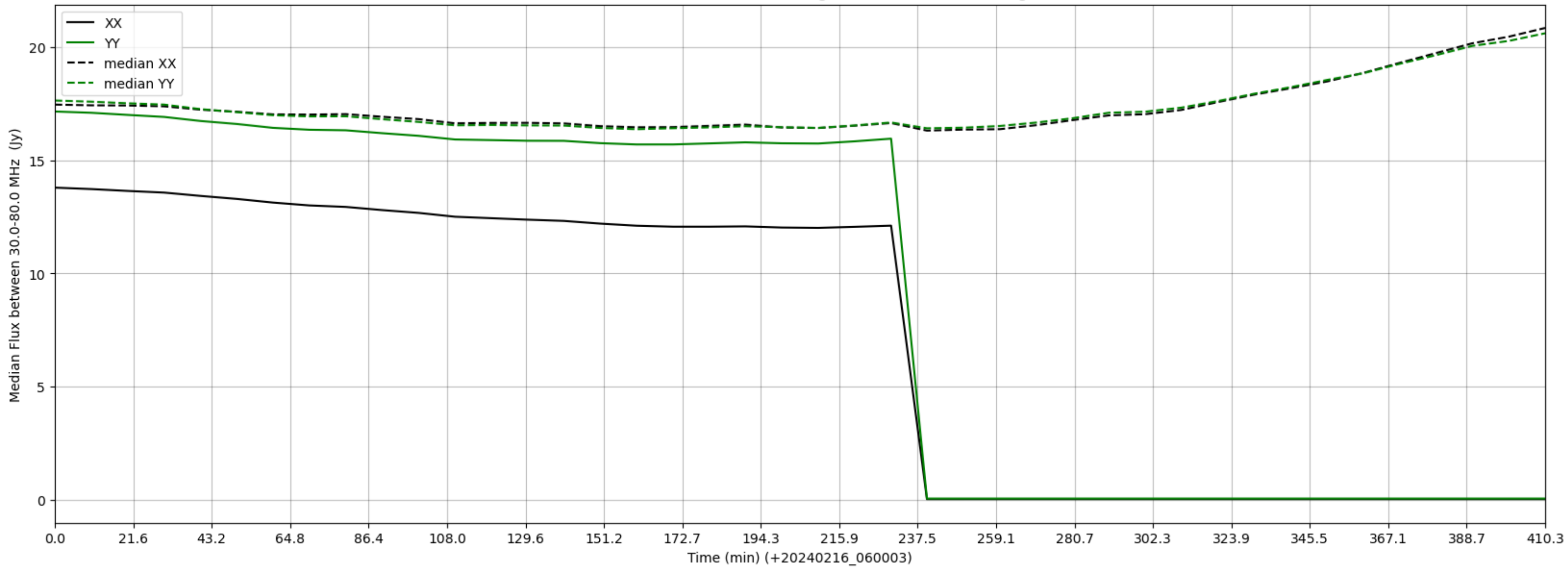
LWA258 - Correlator# 035 - XX FLAGS:HighTimeVar - YY FLAGS:HighTimeVar
