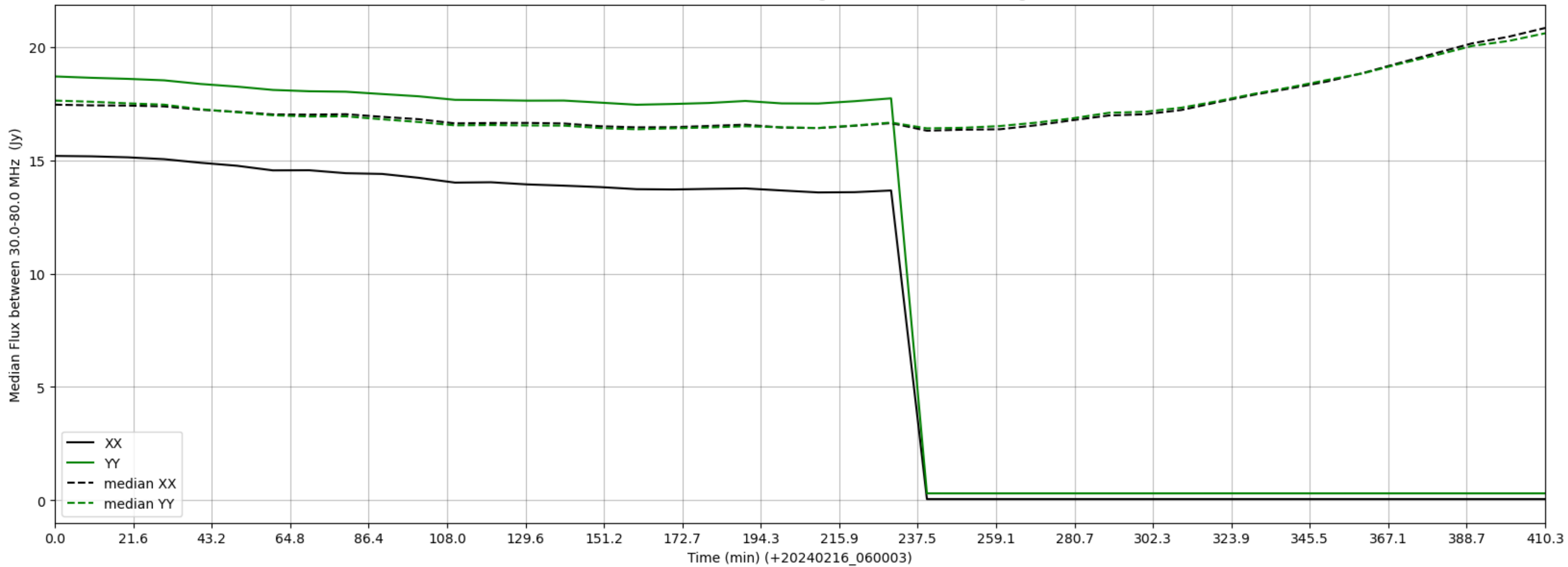
LWA259 - Correlator# 001 - XX FLAGS:HighTimeVar - YY FLAGS:HighTimeVar
