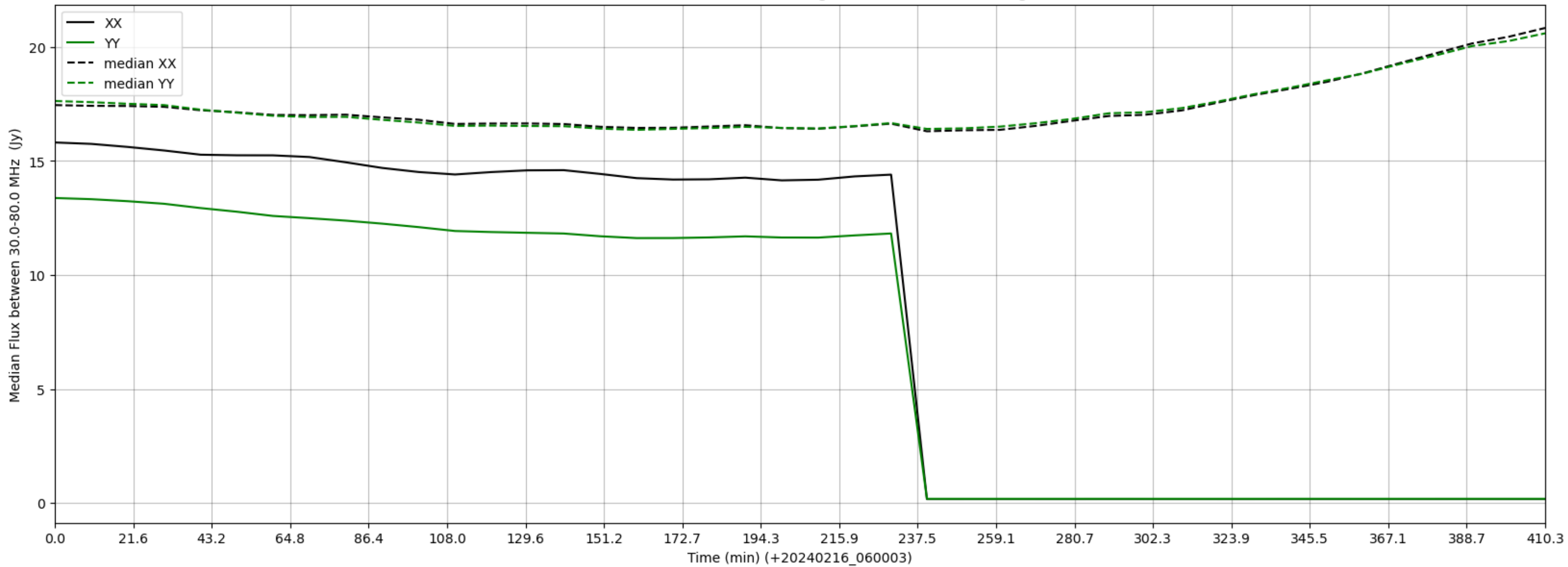
LWA279 - Correlator# 220 - XX FLAGS:HighTimeVar - YY FLAGS:HighTimeVar
