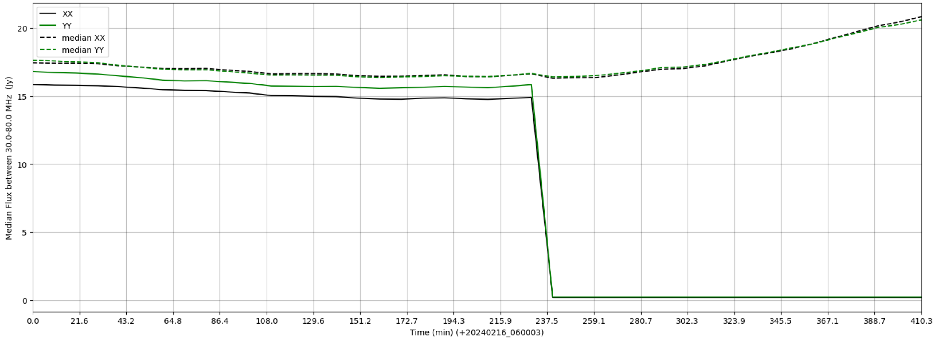
LWA312 - Correlator# 019 - XX FLAGS:HighTimeVar+BadSpecShape - YY FLAGS:HighTimeVar
