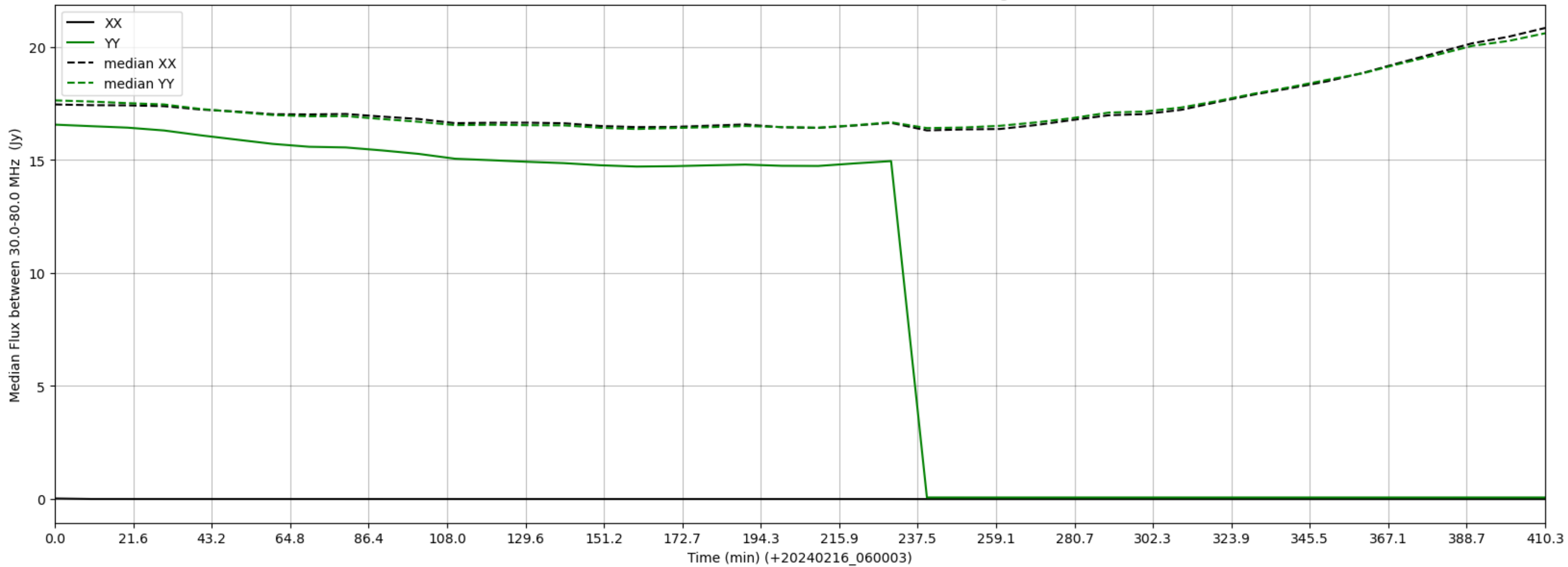
LWA267 - Correlator# 003 - XX FLAGS:LowFlux - YY FLAGS:HighTimeVar
