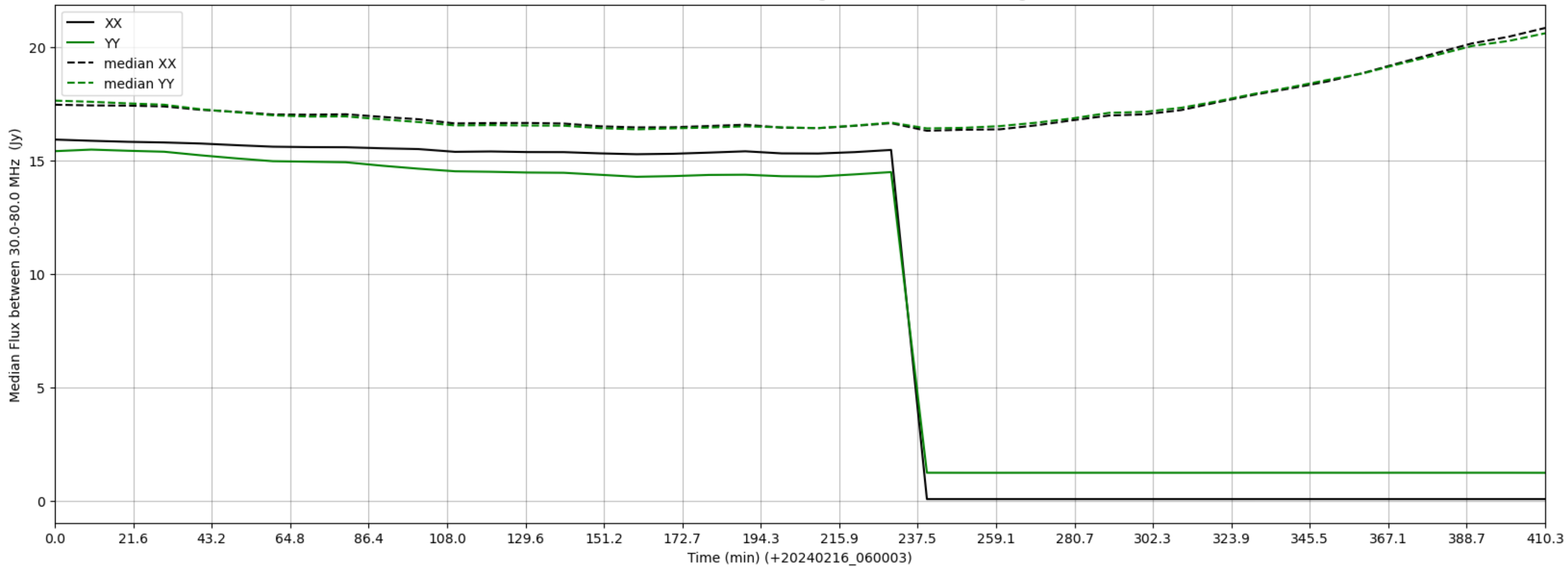
LWA354 - Correlator# 063 - XX FLAGS:HighTimeVar - YY FLAGS:HighTimeVar
