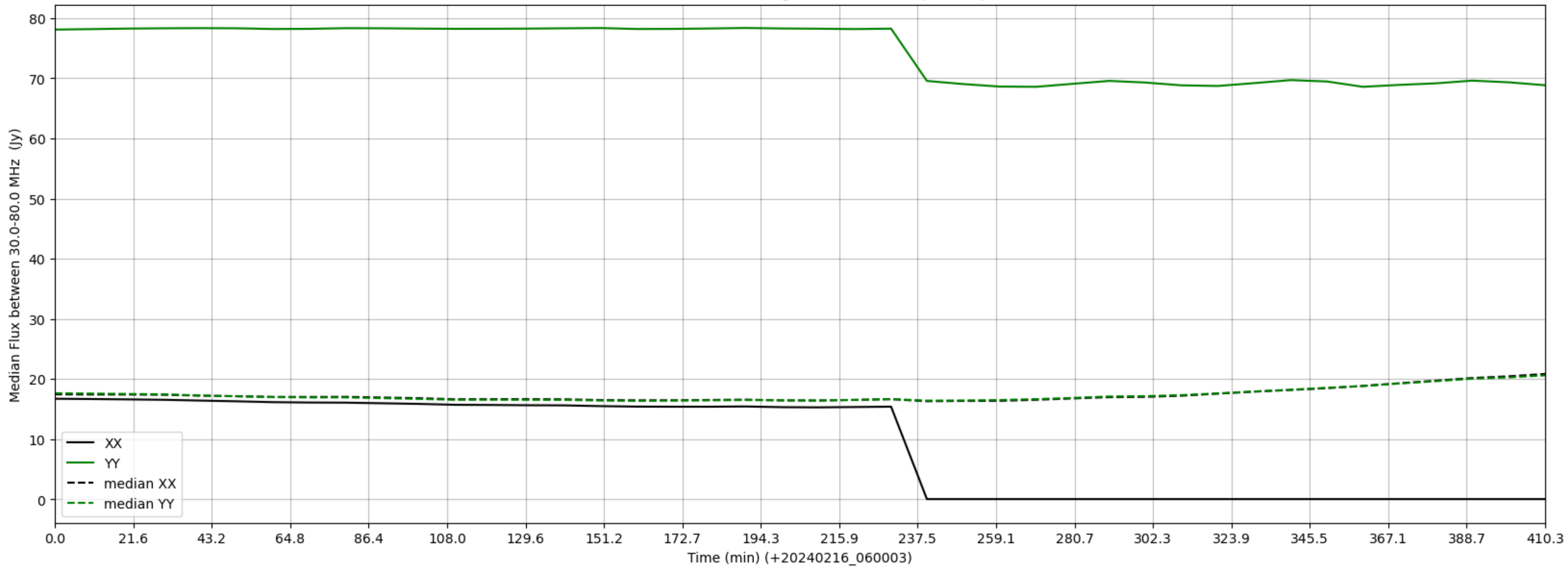
LWA280 - Correlator# 041 - XX FLAGS:HighTimeVar+BadSpecShape - YY FLAGS:Good
