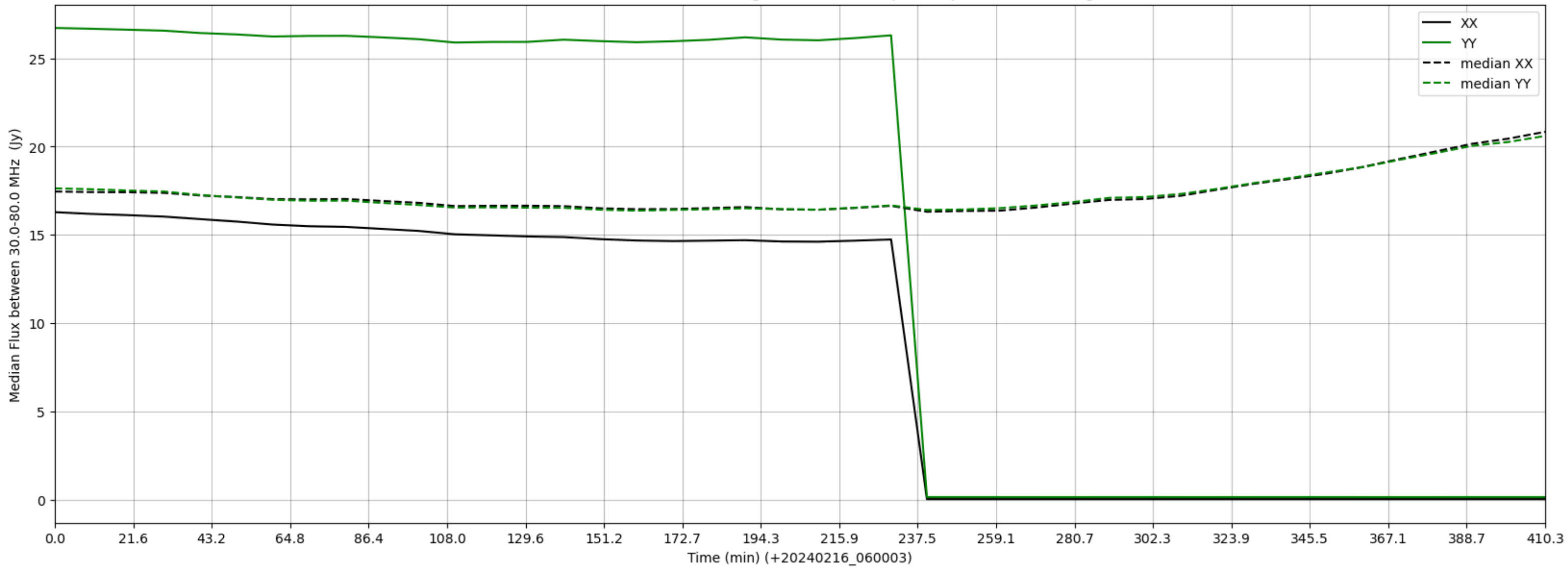
LWA296 - Correlator# 046 - XX FLAGS:HighTimeVar+BadSpecShape - YY FLAGS:HighTimeVar
