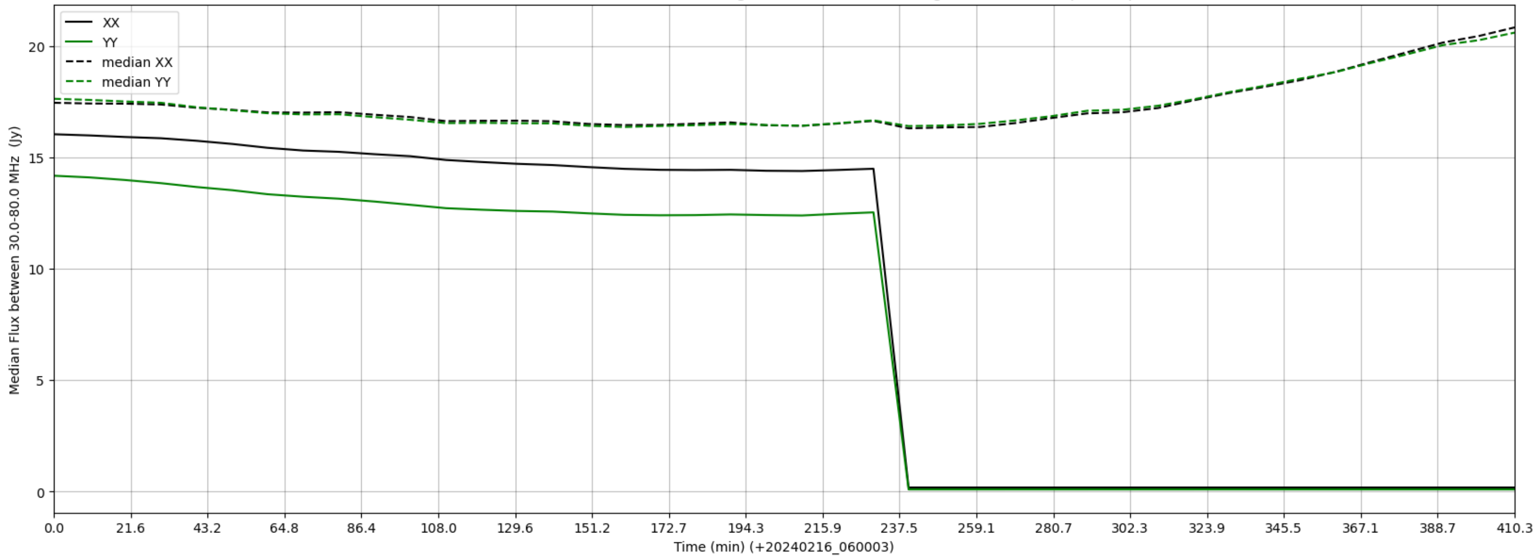
LWA287 - Correlator# 223 - XX FLAGS:HighTimeVar - YY FLAGS:HighTimeVar+BadSpecShape
