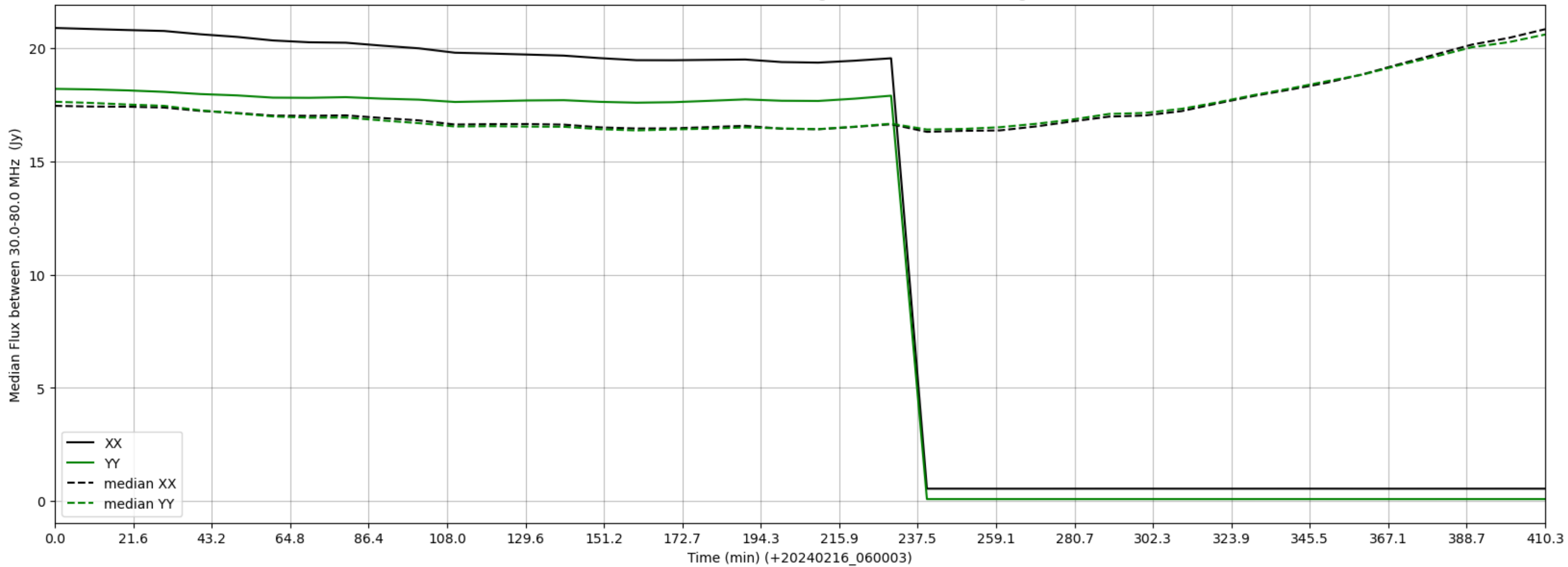
LWA264 - Correlator# 349 - XX FLAGS:HighTimeVar - YY FLAGS:HighTimeVar
