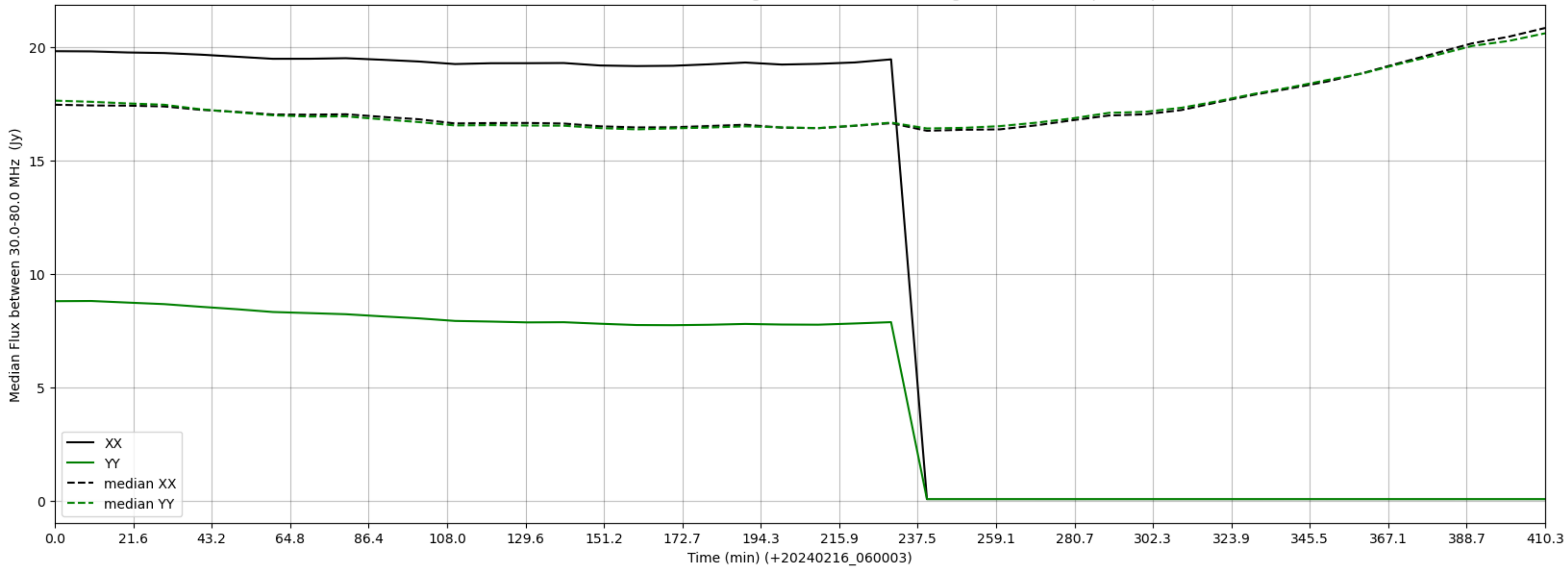
LWA319 - Correlator# 190 - XX FLAGS:HighTimeVar - YY FLAGS:HighTimeVar+BadSpecShape
