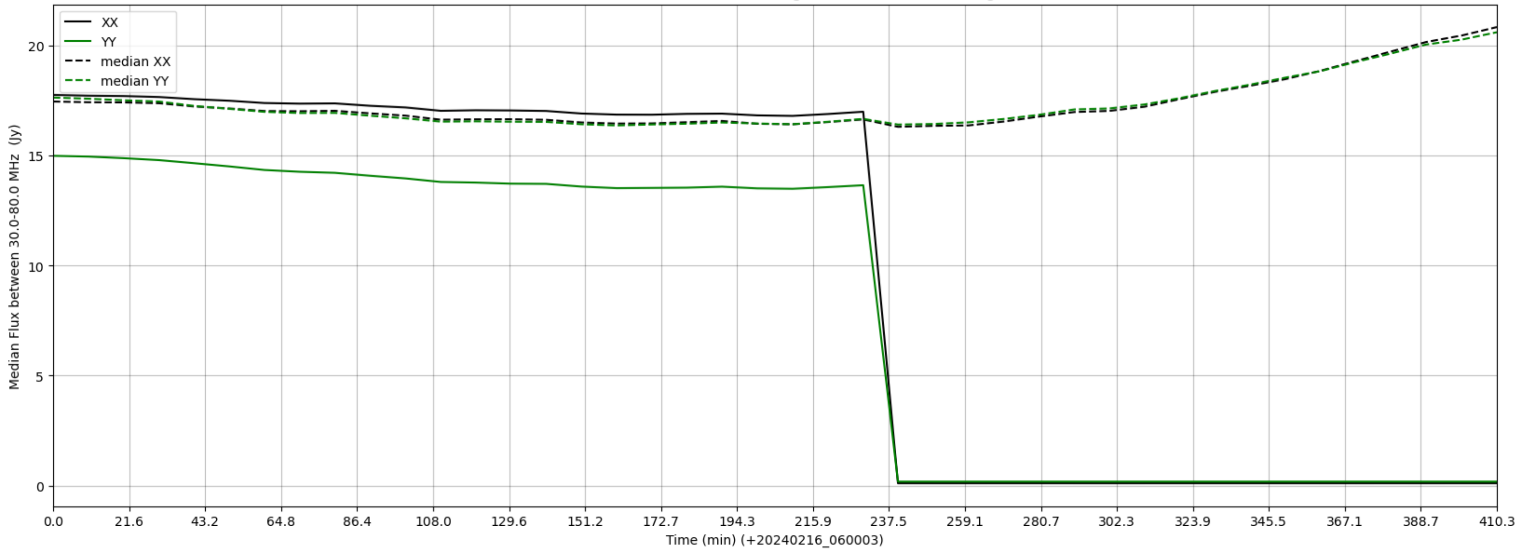
LWA266 - Correlator# 000 - XX FLAGS:HighTimeVar - YY FLAGS:HighTimeVar
