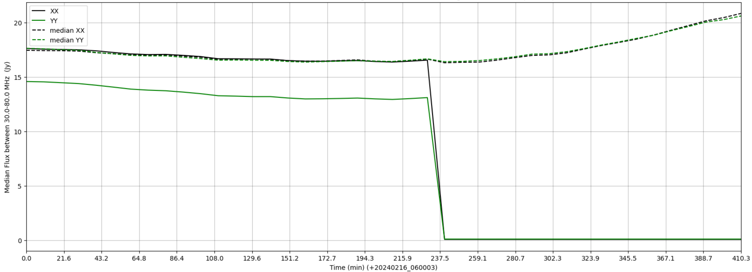
LWA343 - Correlator# 058 - XX FLAGS:HighTimeVar - YY FLAGS:HighTimeVar+BadSpecShape
