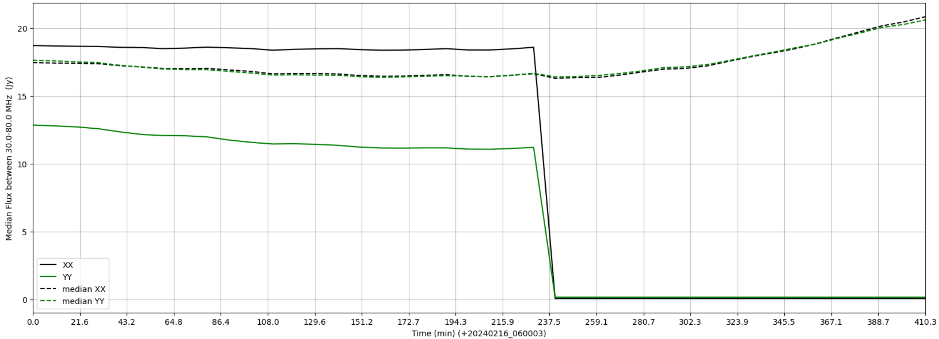
LWA271 - Correlator# 004 - XX FLAGS:HighTimeVar - YY FLAGS:HighTimeVar
