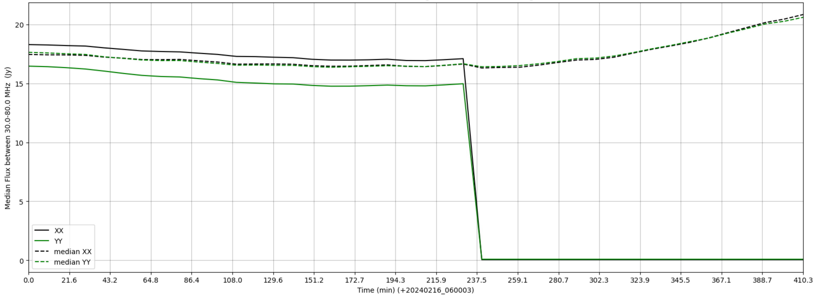
LWA268 - Correlator# 002 - XX FLAGS:HighTimeVar - YY FLAGS:HighTimeVar
