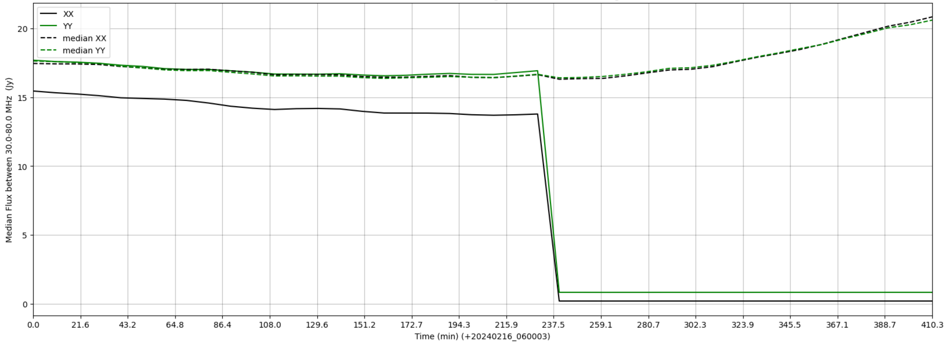
LWA328 - Correlator# 157 - XX FLAGS:HighTimeVar - YY FLAGS:HighTimeVar
