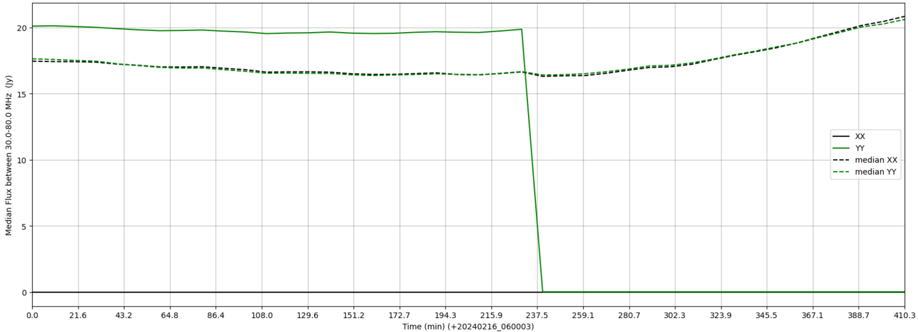
LWA352 - Correlator# 028 - XX FLAGS:LowFlux - YY FLAGS:HighTimeVar
