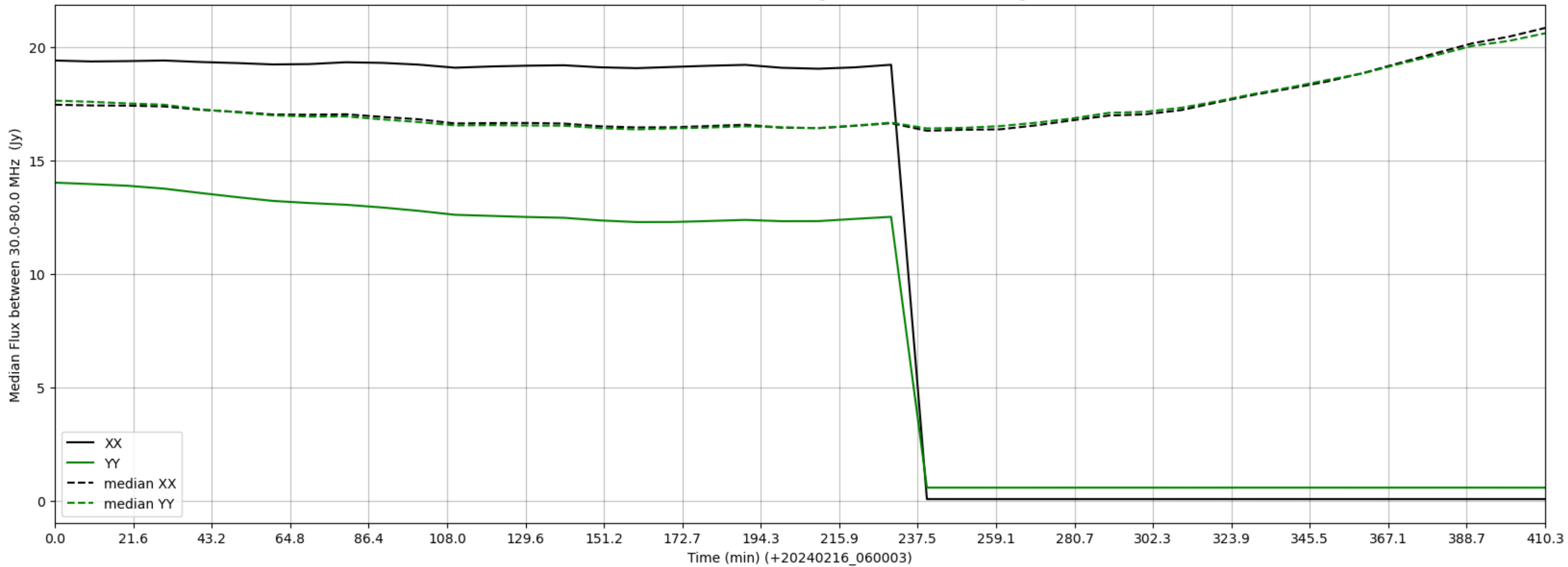
LWA269 - Correlator# 005 - XX FLAGS:HighTimeVar - YY FLAGS:HighTimeVar
