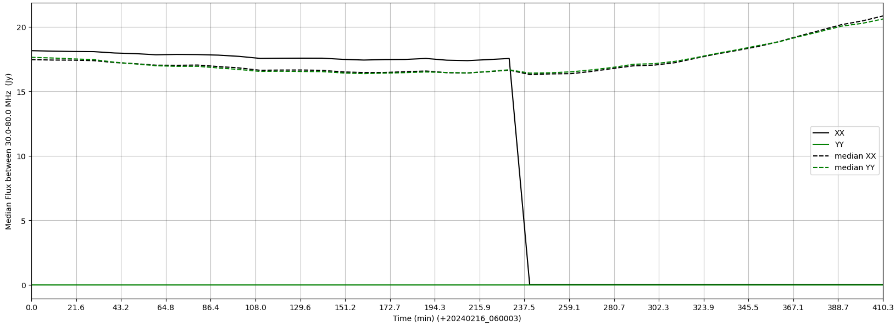
LWA325 - Correlator# 154 - XX FLAGS:HighTimeVar - YY FLAGS:LowFlux
