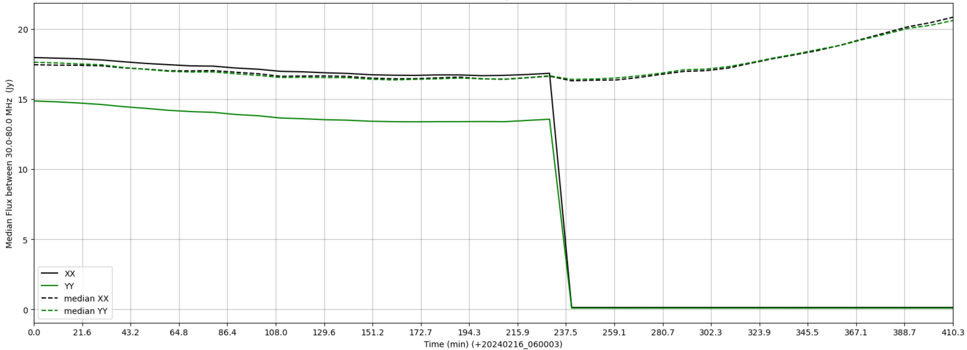
LWA350 - Correlator# 319 - XX FLAGS:HighTimeVar - YY FLAGS:HighTimeVar
