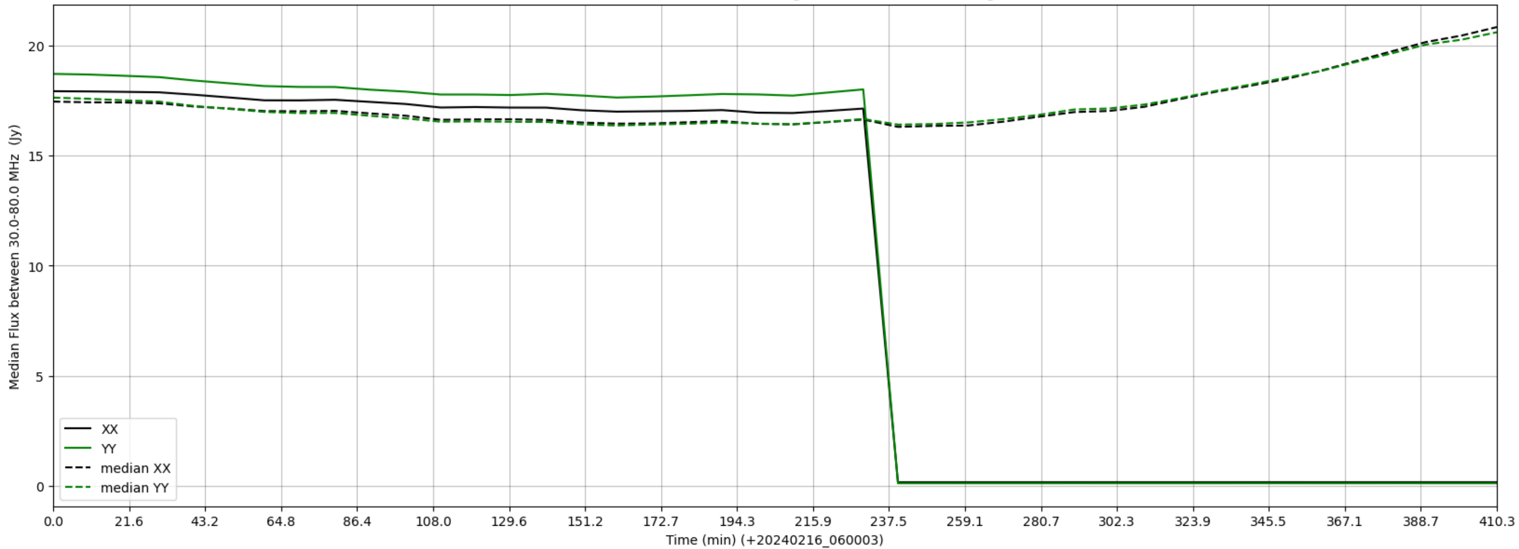
LWA270 - Correlator# 039 - XX FLAGS:HighTimeVar - YY FLAGS:HighTimeVar
