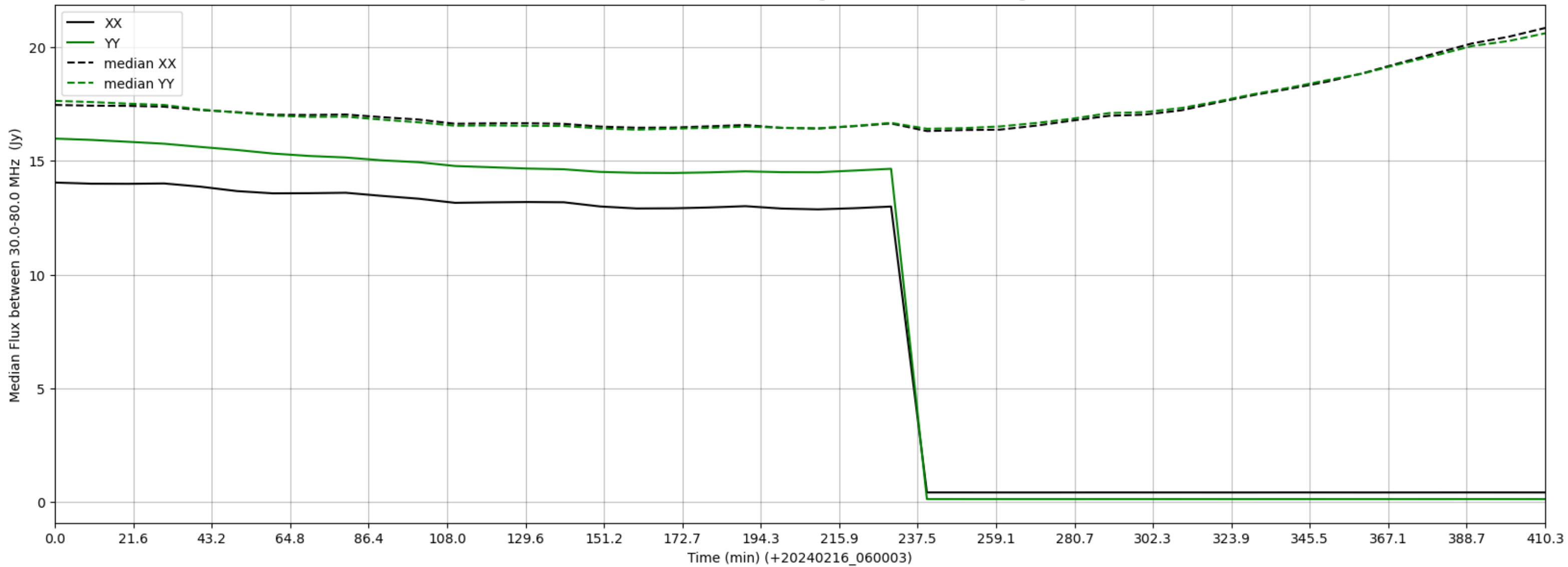
LWA339 - Correlator# 027 - XX FLAGS:HighTimeVar - YY FLAGS:HighTimeVar
