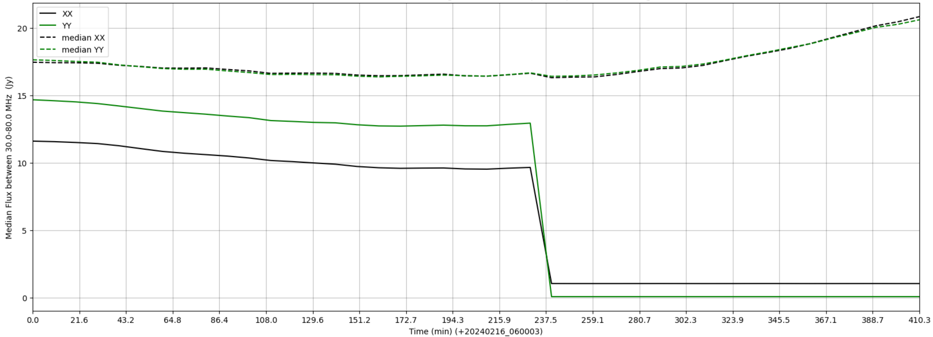
LWA313 - Correlator# 018 - XX FLAGS:HighTimeVar+BadSpecShape - YY FLAGS:HighTimeVar
