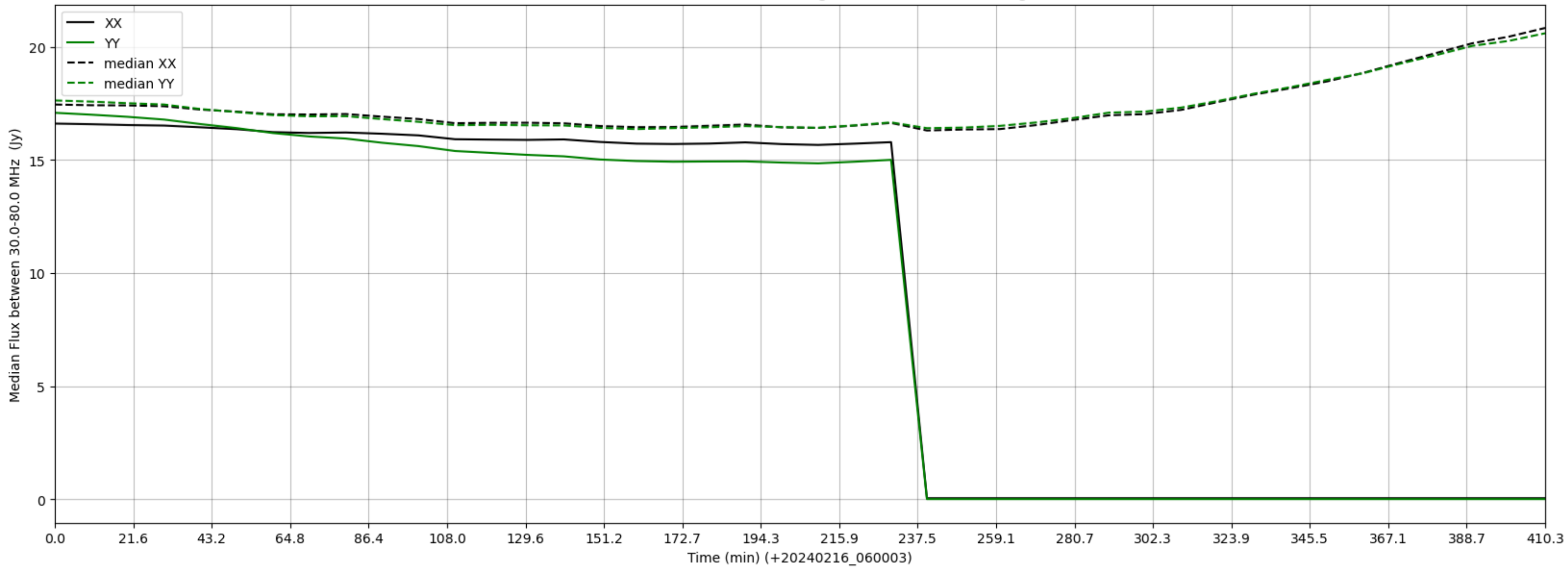
LWA284 - Correlator# 043 - XX FLAGS:HighTimeVar - YY FLAGS:HighTimeVar
