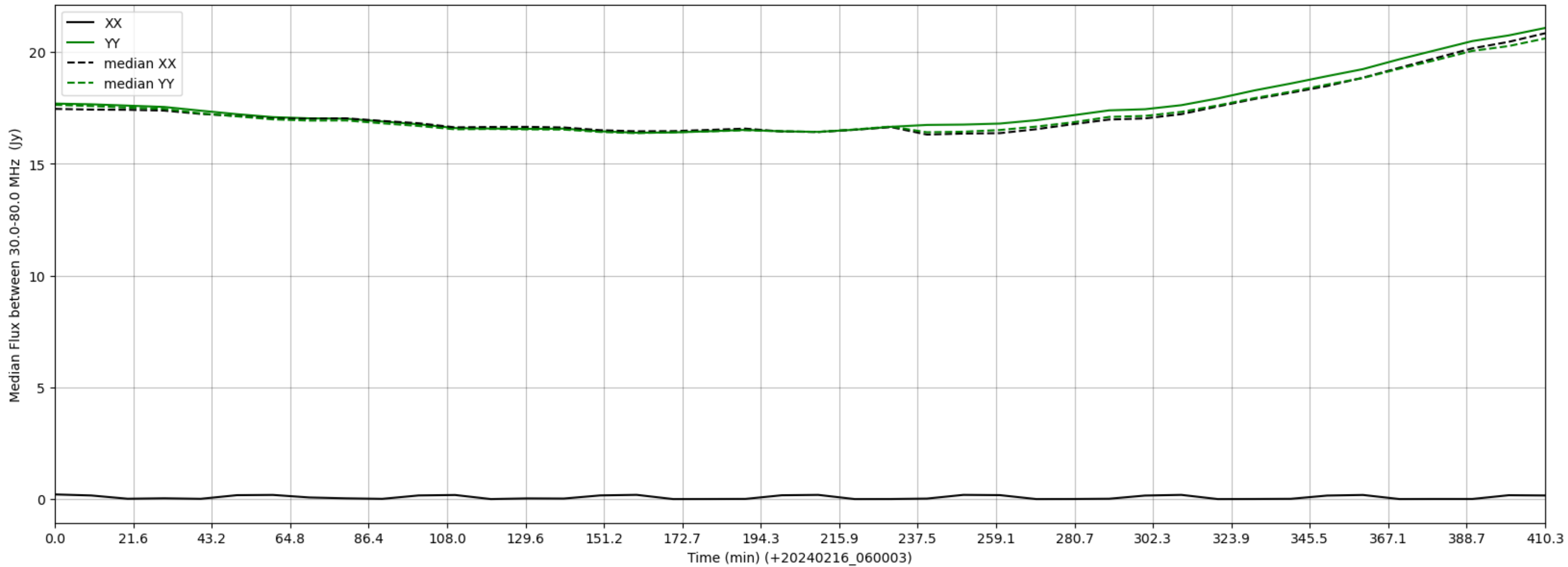
LWA105 - Correlator# 178 - XX FLAGS:LowFlux - YY FLAGS:Good
