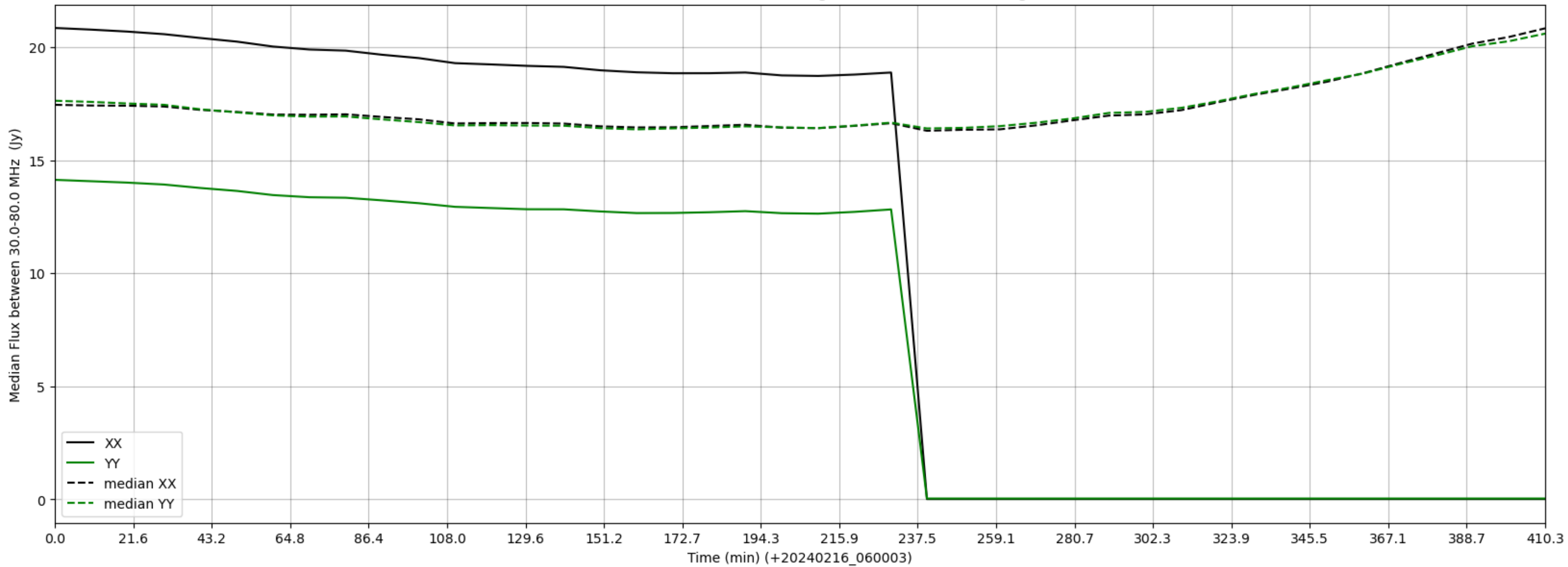
LWA295 - Correlator# 047 - XX FLAGS:HighTimeVar - YY FLAGS:HighTimeVar
