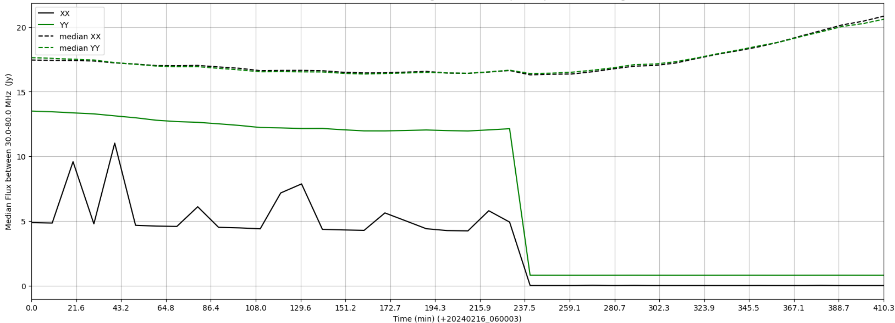
LWA335 - Correlator# 057 - XX FLAGS:HighTimeVar+BadSpecShape - YY FLAGS:HighTimeVar
