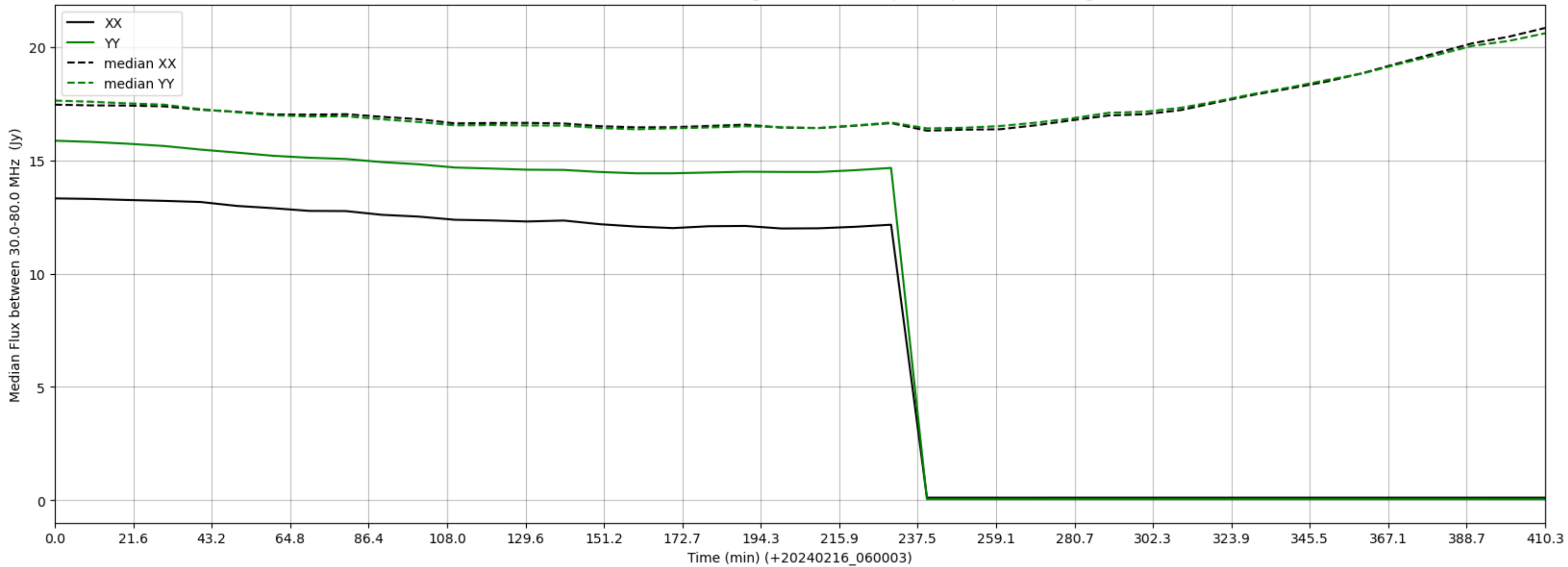
LWA351 - Correlator# 060 - XX FLAGS:HighTimeVar+BadSpecShape - YY FLAGS:HighTimeVar
