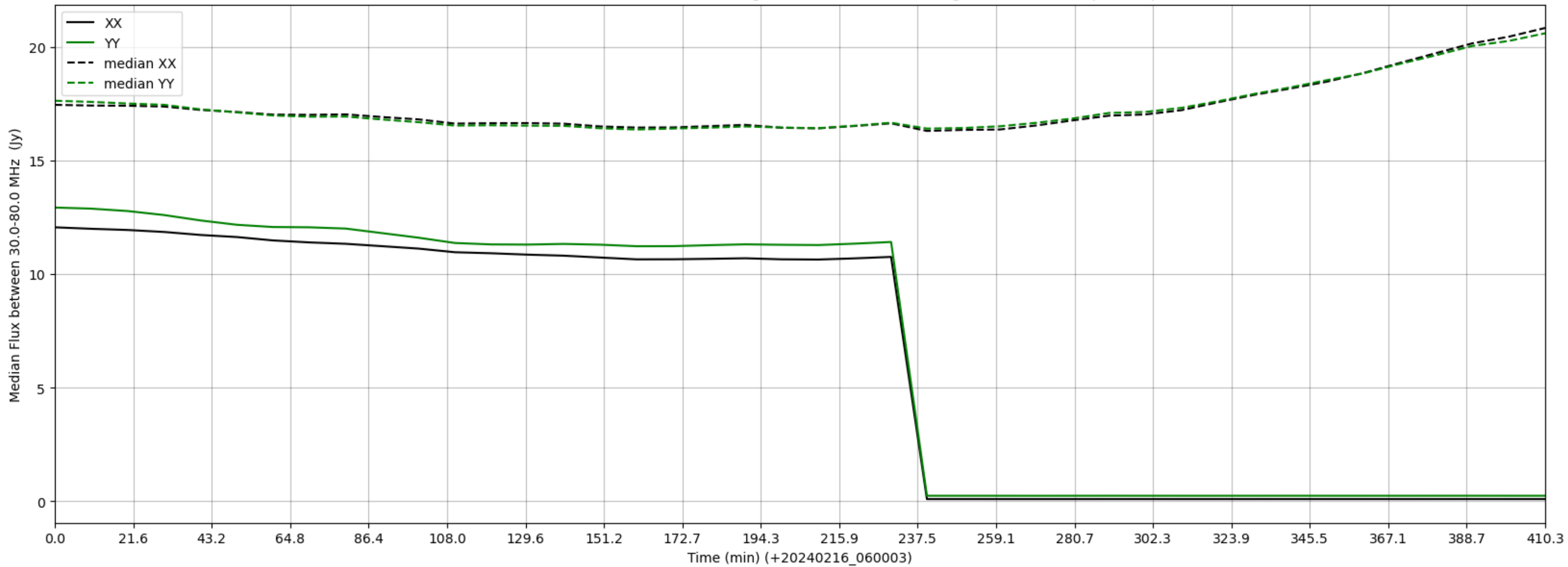
LWA297 - Correlator# 314 - XX FLAGS:HighTimeVar - YY FLAGS:HighTimeVar+BadSpecShape
