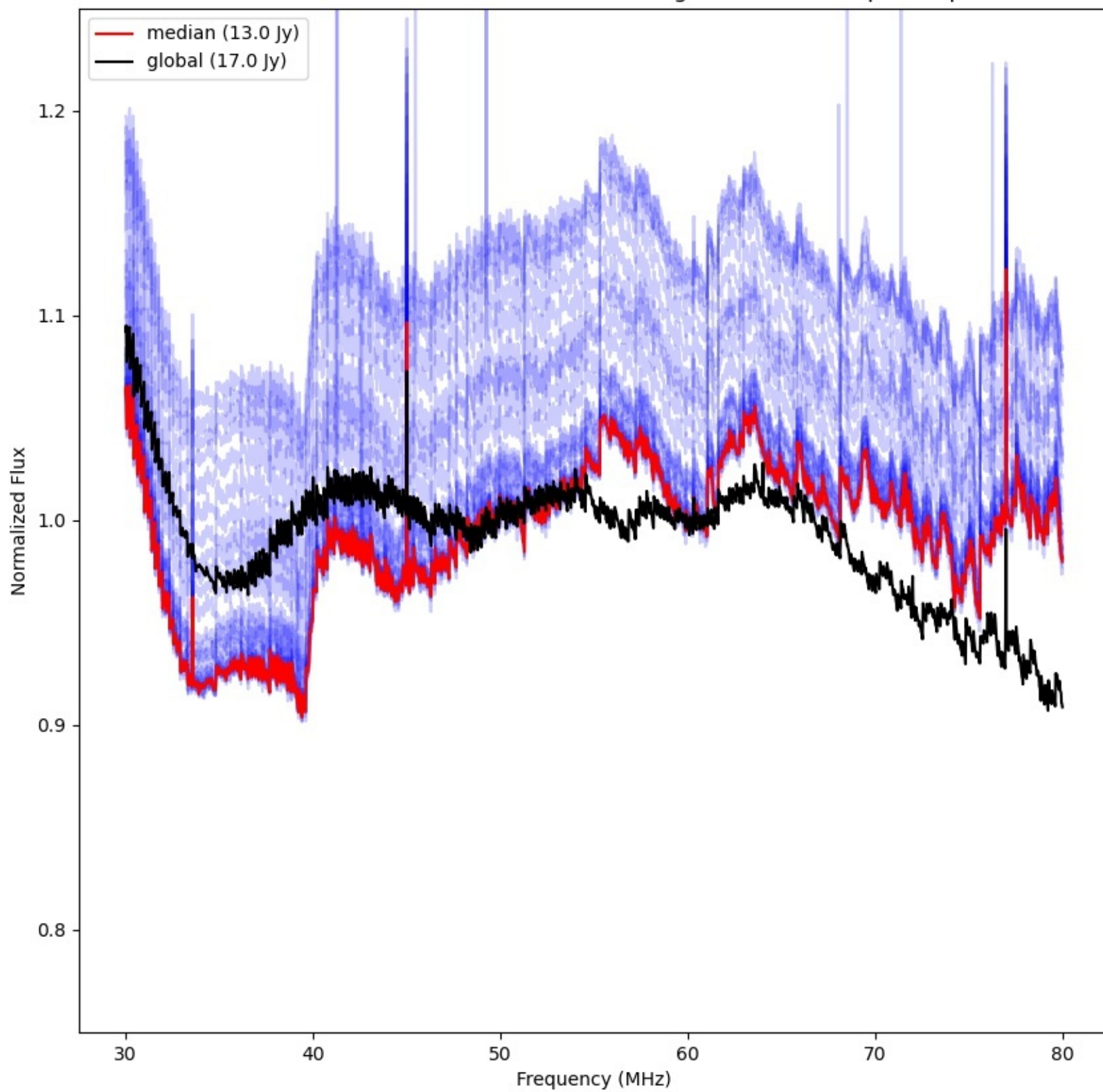
LWA343 - Correlator# 058 - YY - FLAGS:HighTimeVar+BadSpecShape
