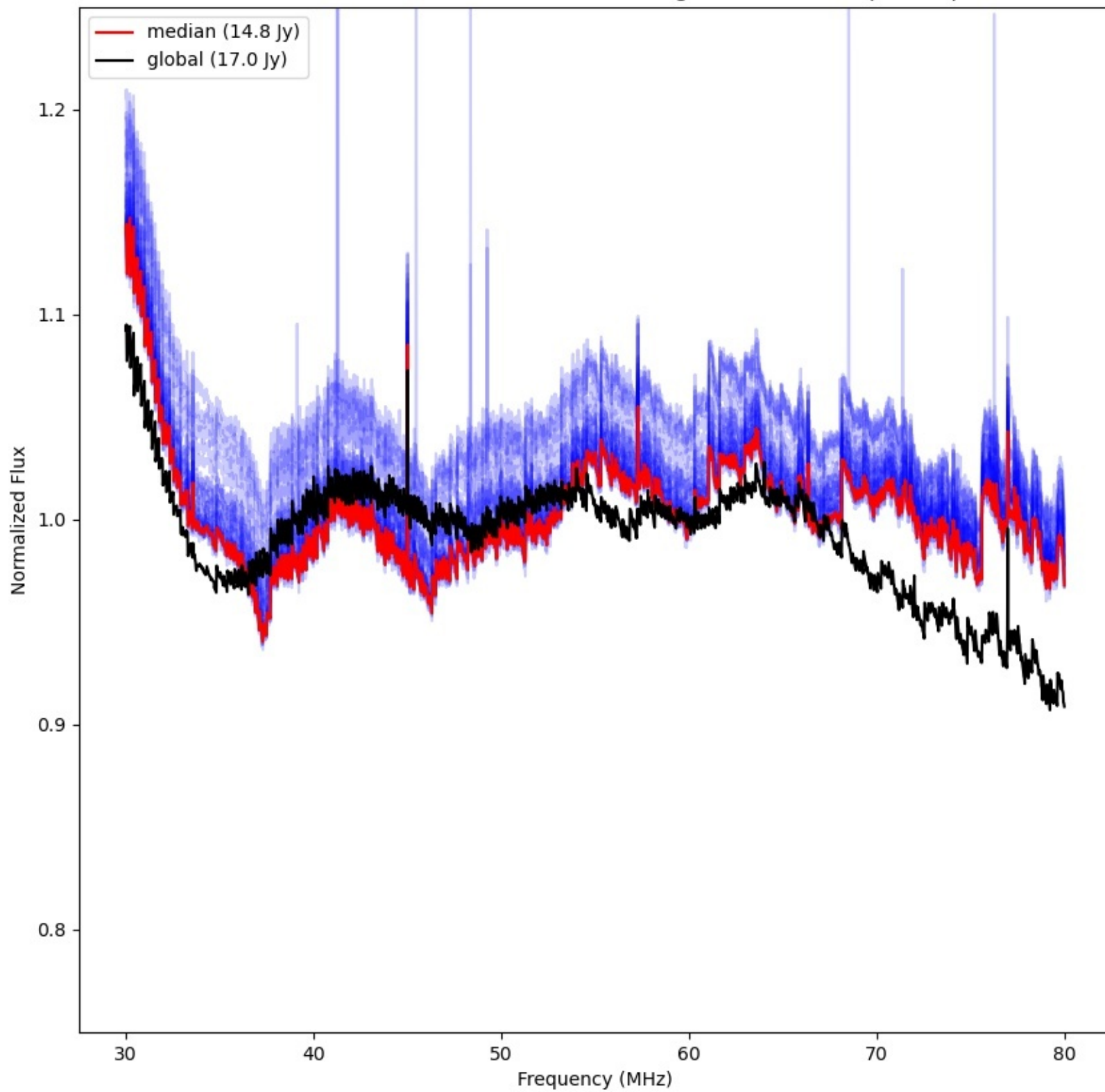
LWA289 - Correlator# 189 - YY - FLAGS:HighTimeVar+BadSpecShape
