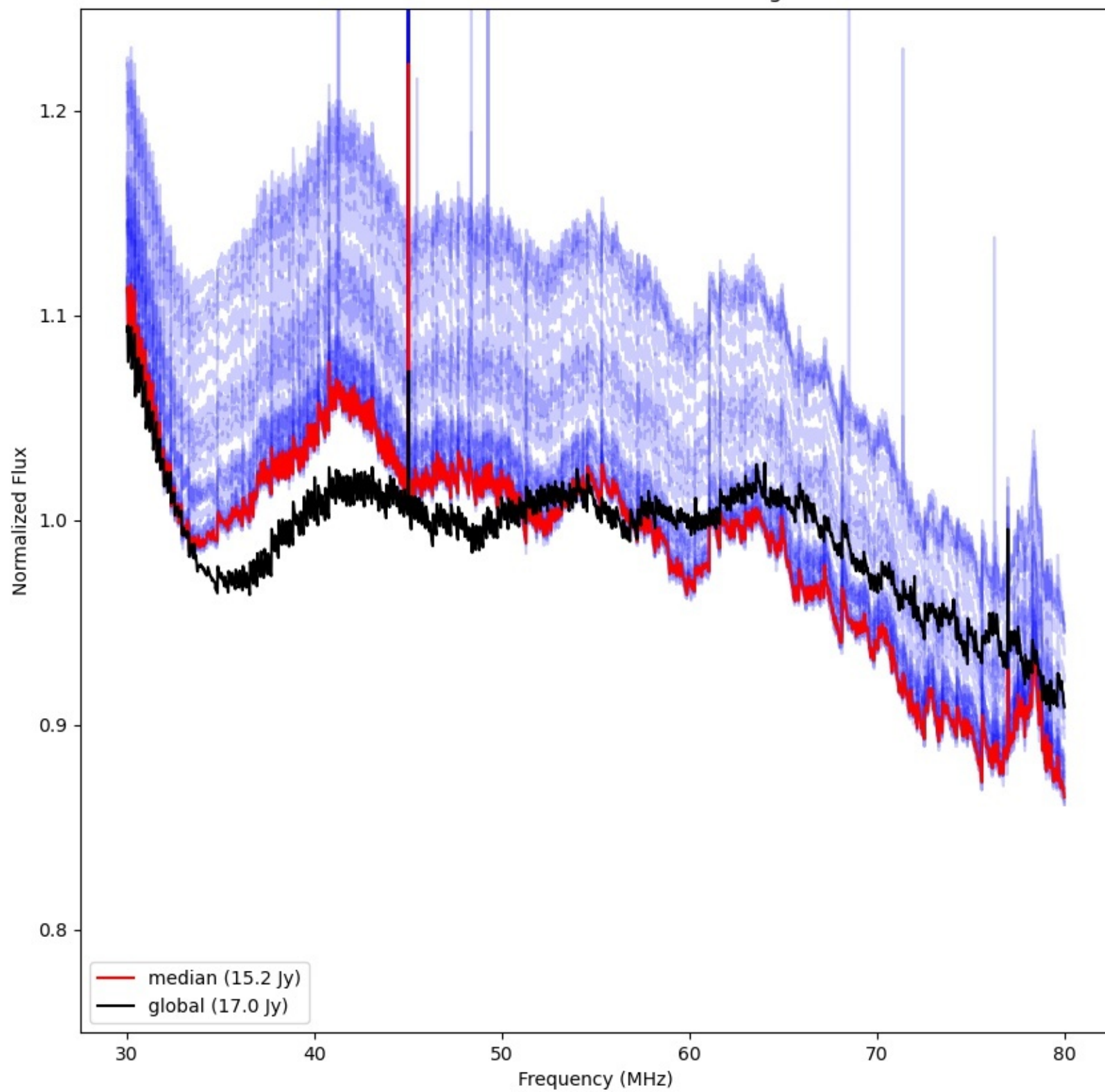
LWA283 - Correlator# 040 - YY - FLAGS:HighTimeVar
