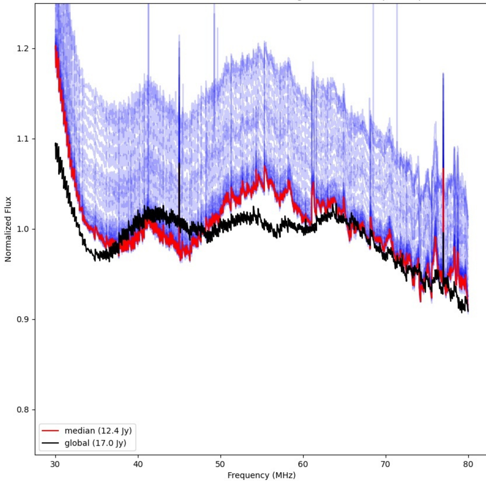
LWA287 - Correlator# 223 - YY - FLAGS:HighTimeVar+BadSpecShape
