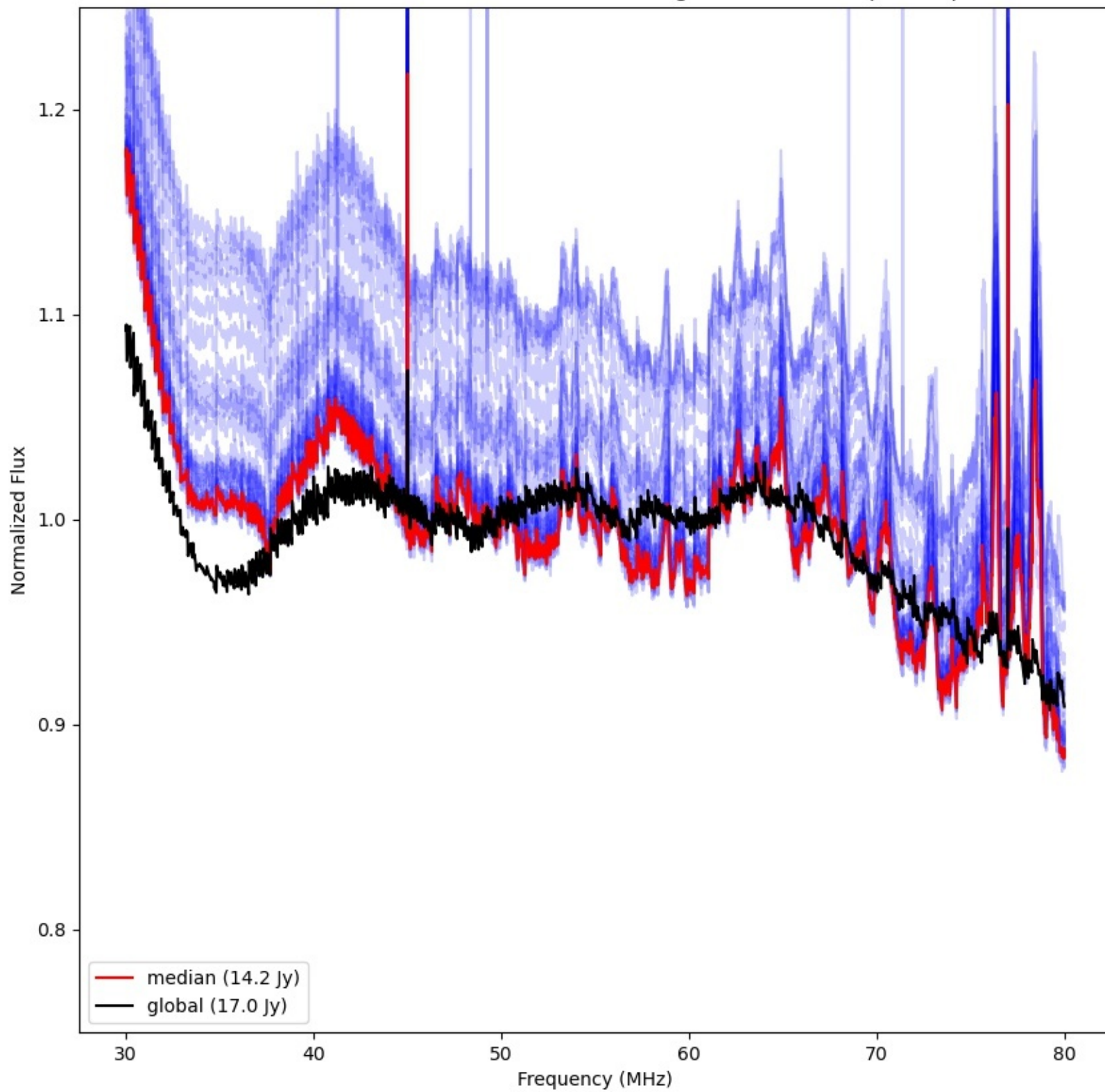
LWA348 - Correlator# 124 - YY - FLAGS:HighTimeVar+BadSpecShape
