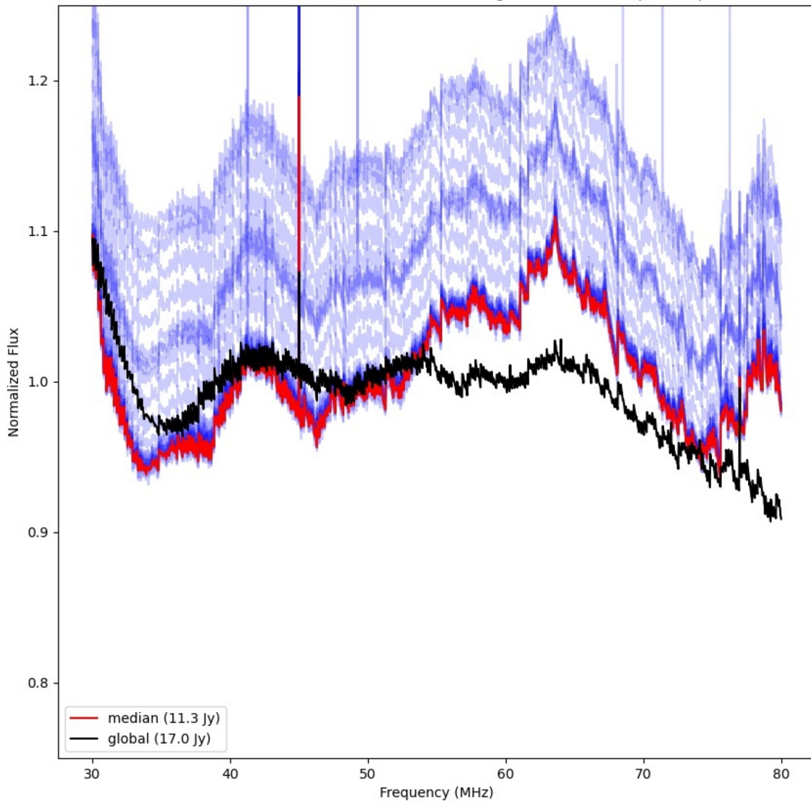
LWA297 - Correlator# 314 - YY - FLAGS:HighTimeVar+BadSpecShape
