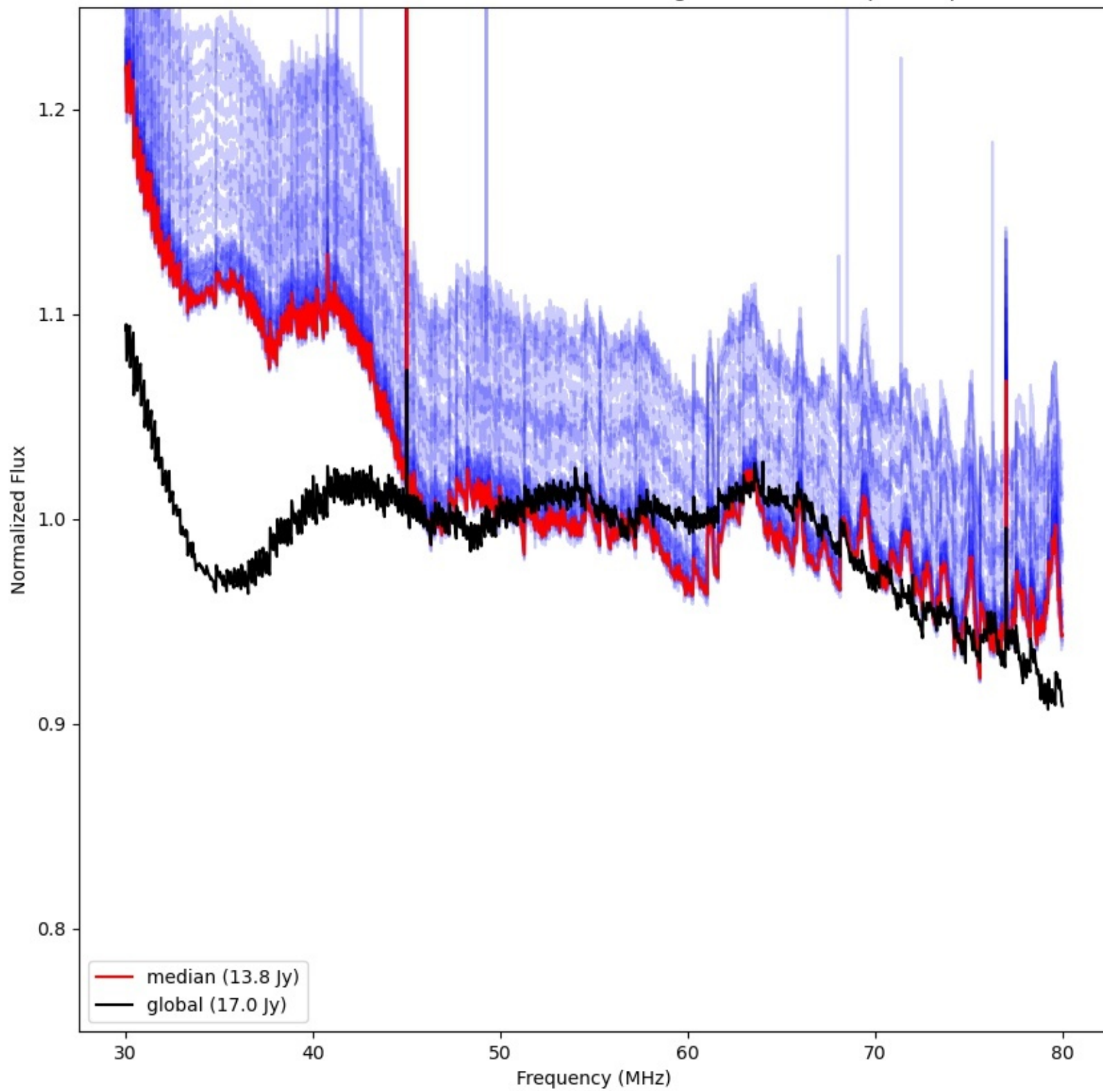
LWA260 - Correlator# 034 - YY - FLAGS:HighTimeVar+BadSpecShape
