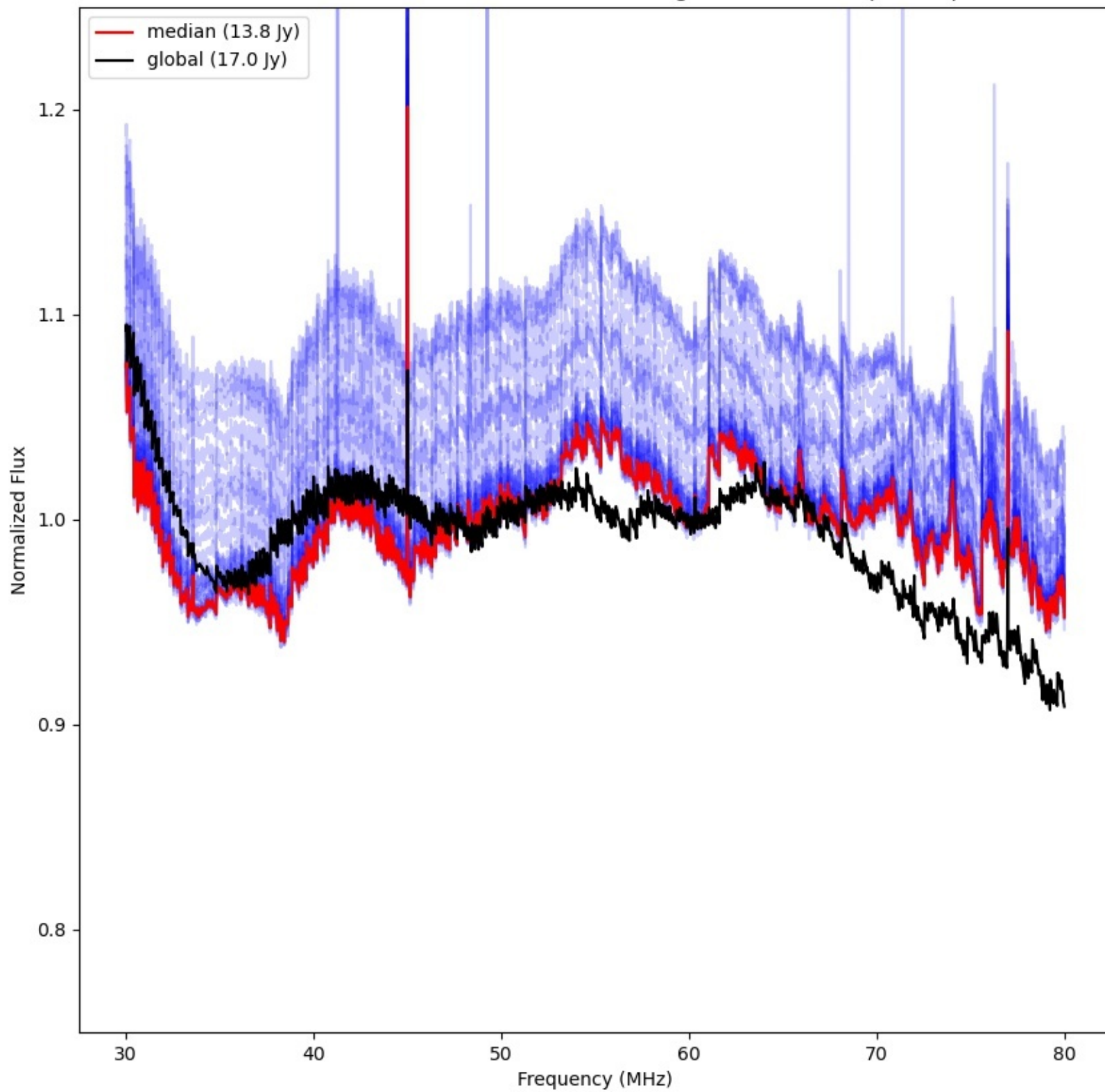
LWA321 - Correlator# 020 - YY - FLAGS:HighTimeVar+BadSpecShape
