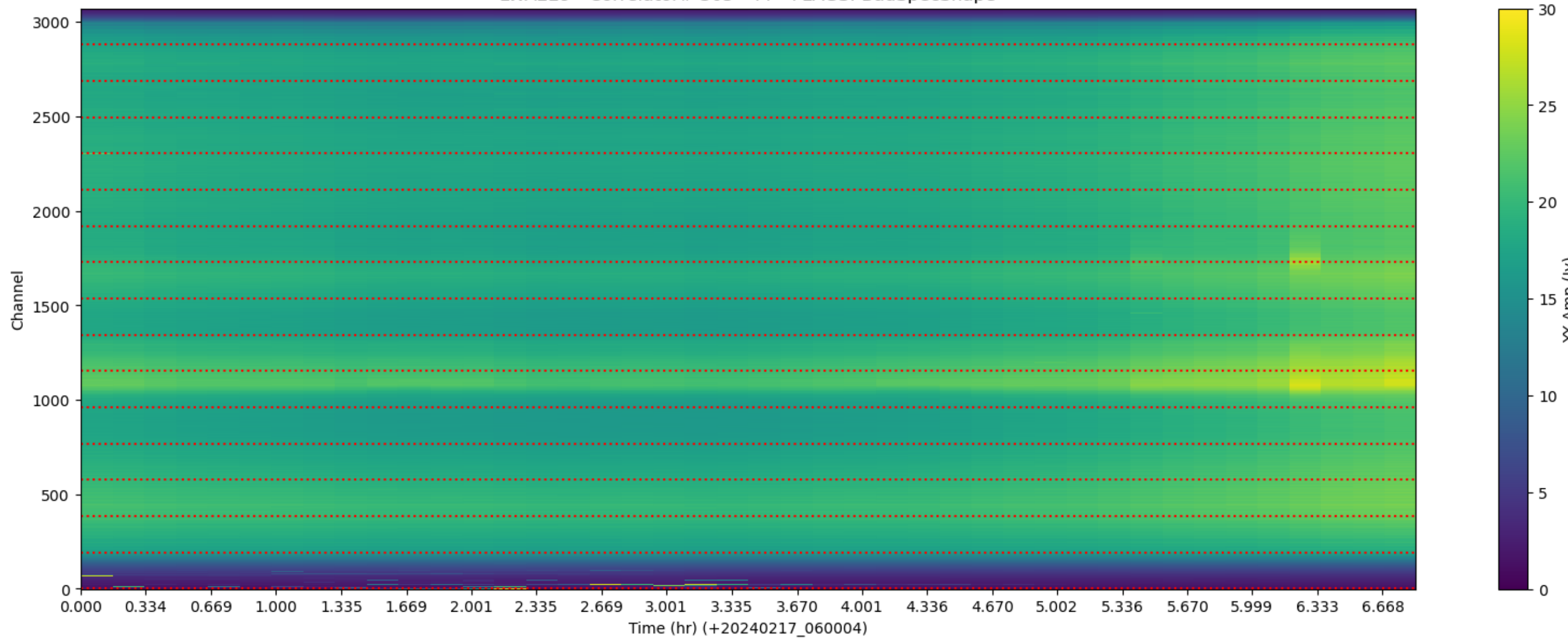
LWA229 - Correlator# 305 - YY - FLAGS: BadSpecShape
