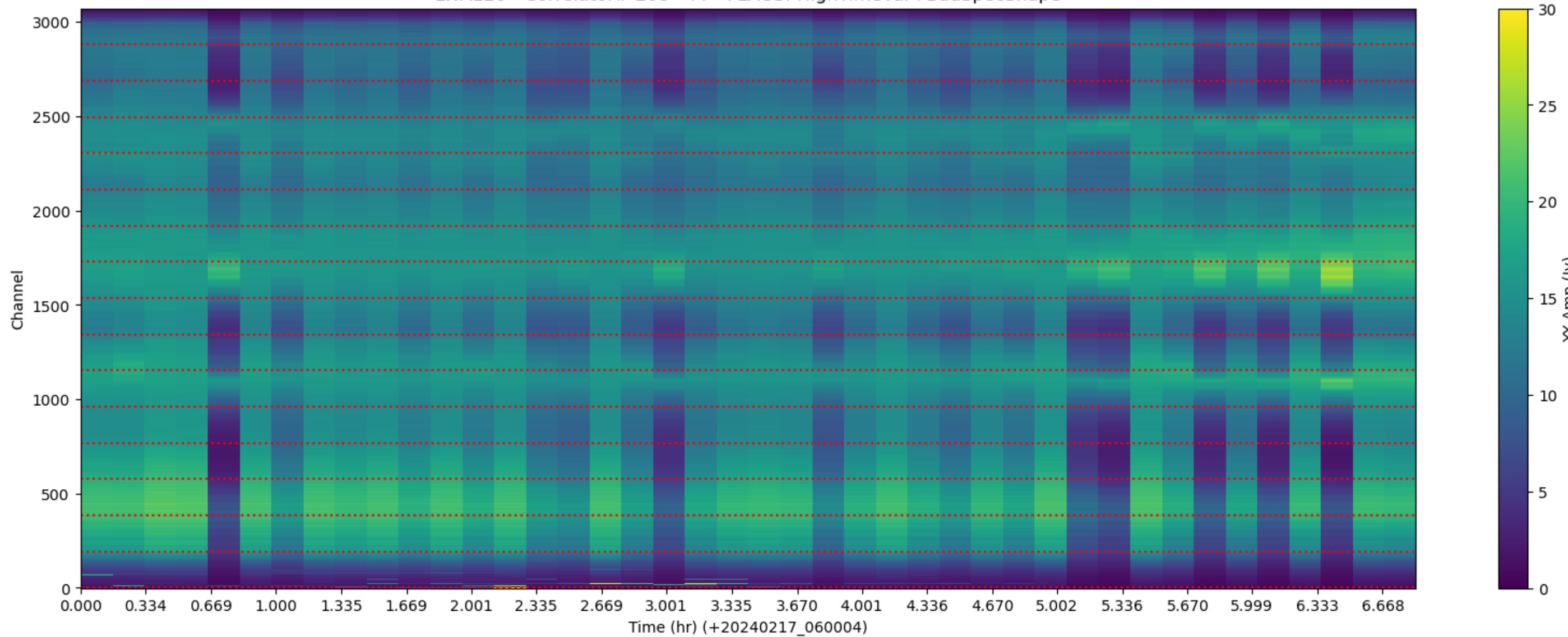
LWA120 - Correlator# 208 - YY - FLAGS: HighTimeVar+BadSpecShape
