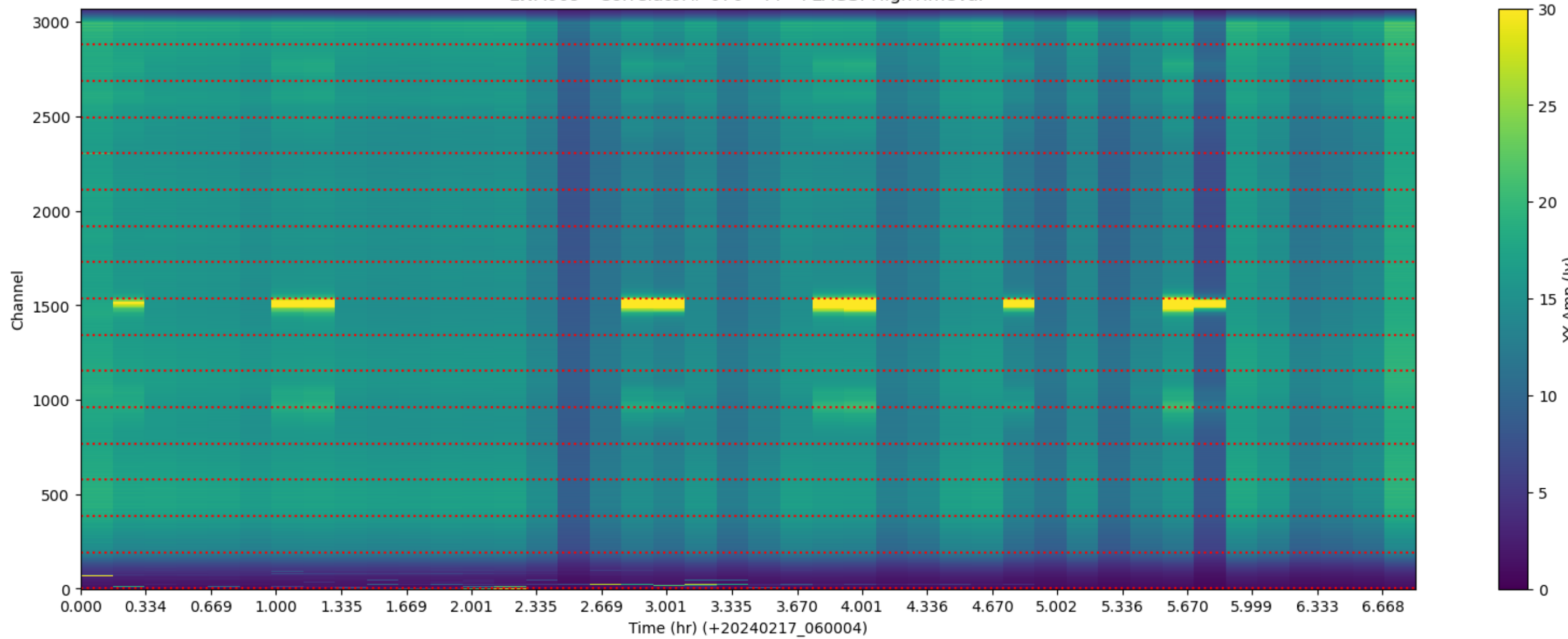
LWA009 - Correlator# 070 - YY - FLAGS: HighTimeVar
