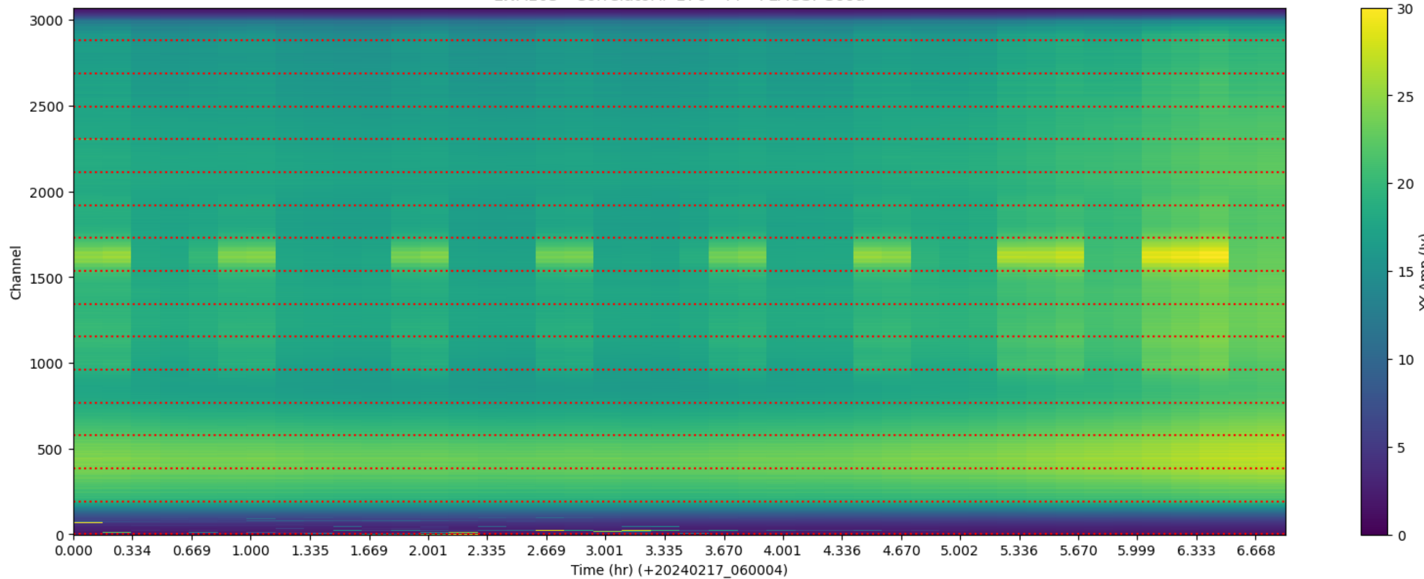
LWA103 - Correlator# 176 - YY - FLAGS: Good
