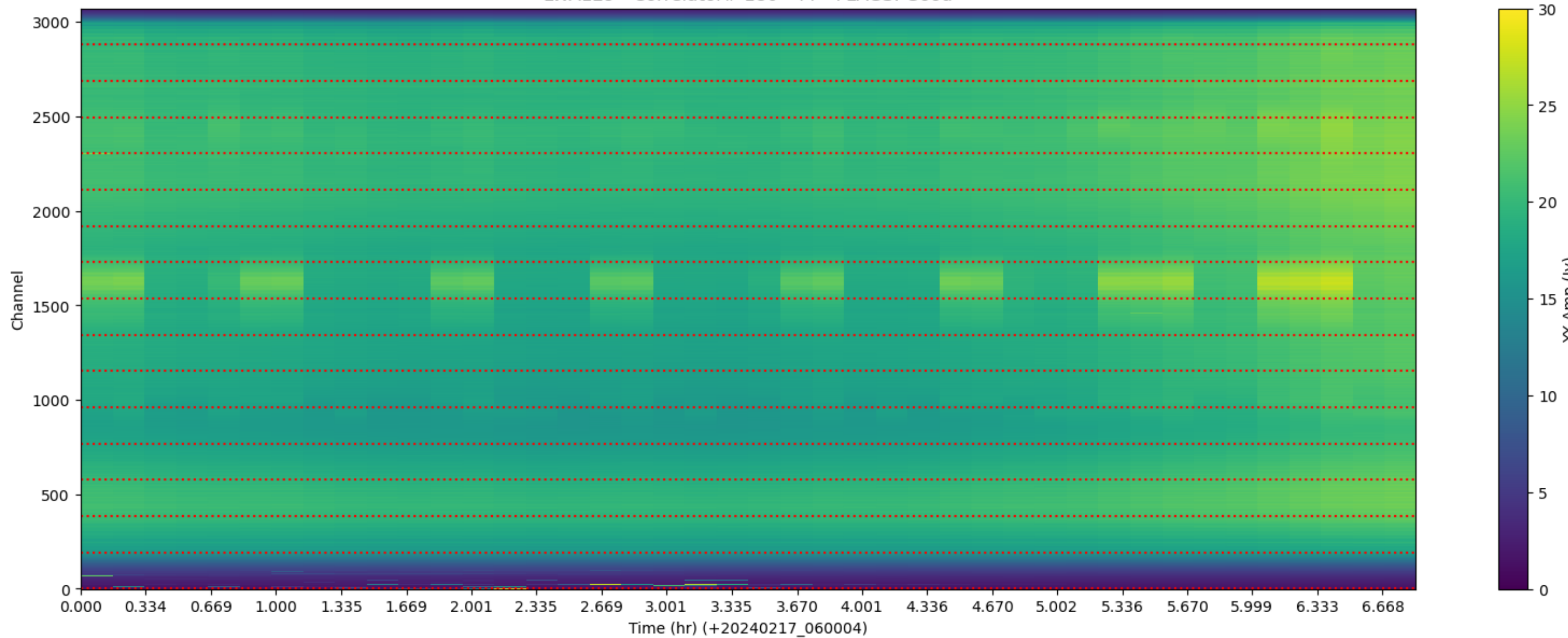
LWA129 - Correlator# 180 - YY - FLAGS: Good
