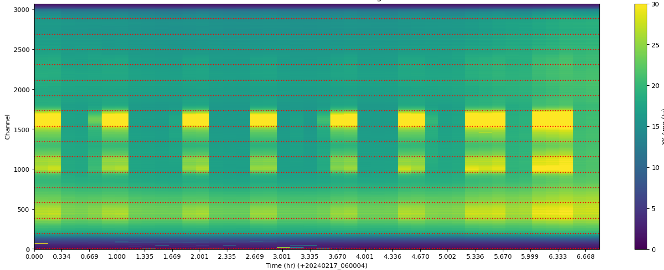
LWA104 - Correlator# 179 - YY - FLAGS: HighTimeVar
