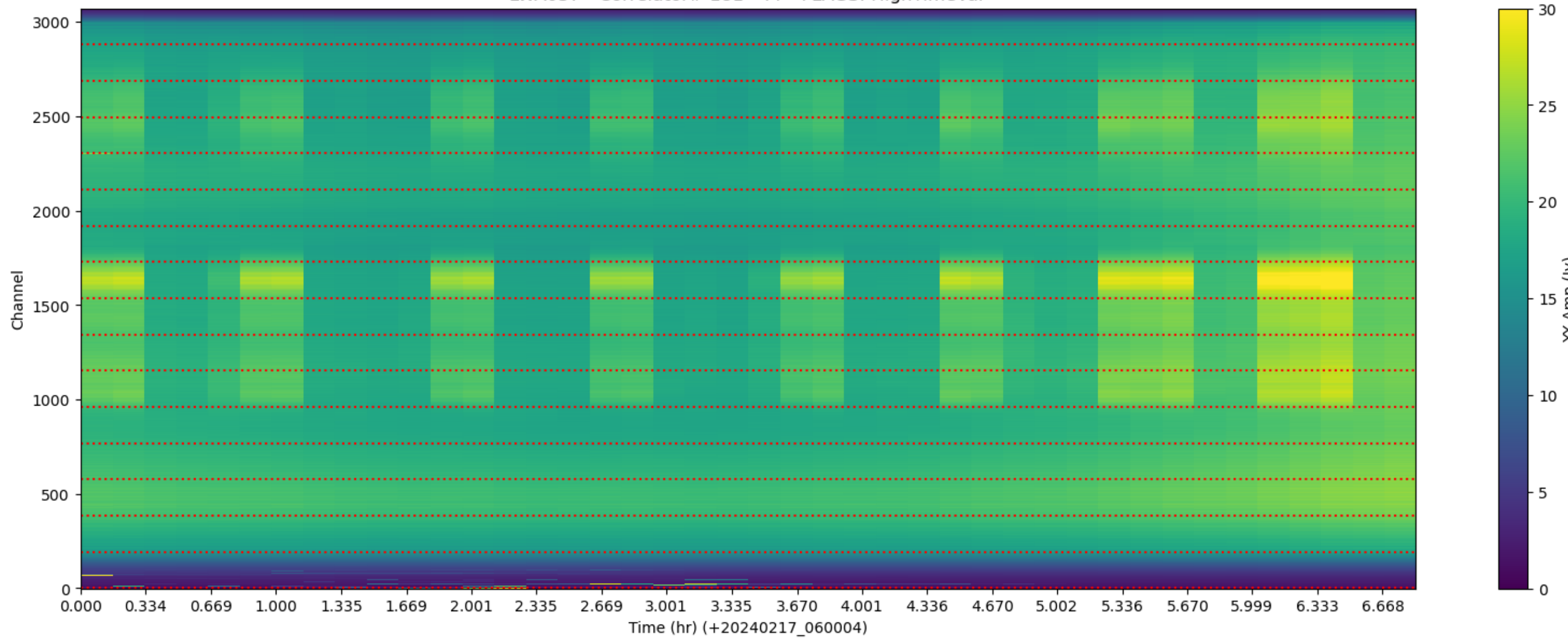
LWA037 - Correlator# 181 - YY - FLAGS: HighTimeVar
