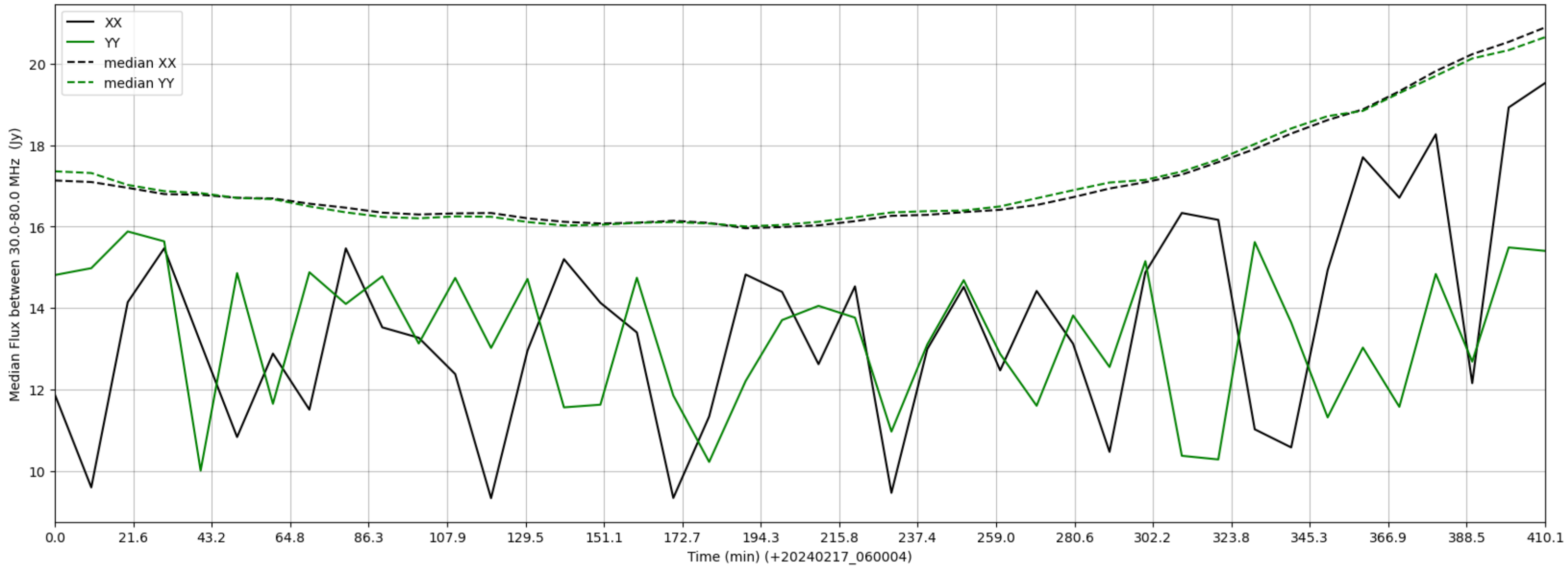
LWA120 - Correlator# 208 - XX FLAGS:HighTimeVar+BadSpecShape - YY FLAGS:HighTimeVar+BadSpecShape
