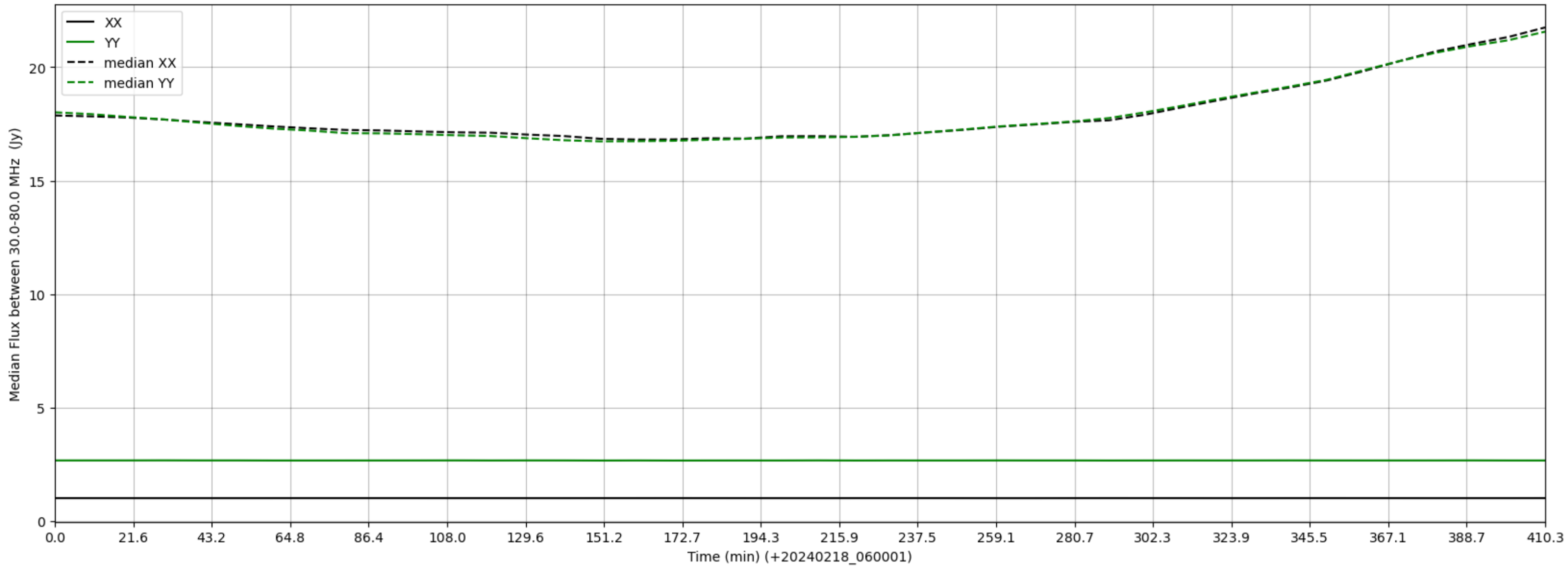
LWA257 - Correlator# 032 - XX FLAGS:LowFlux - YY FLAGS:BadSpecShape
