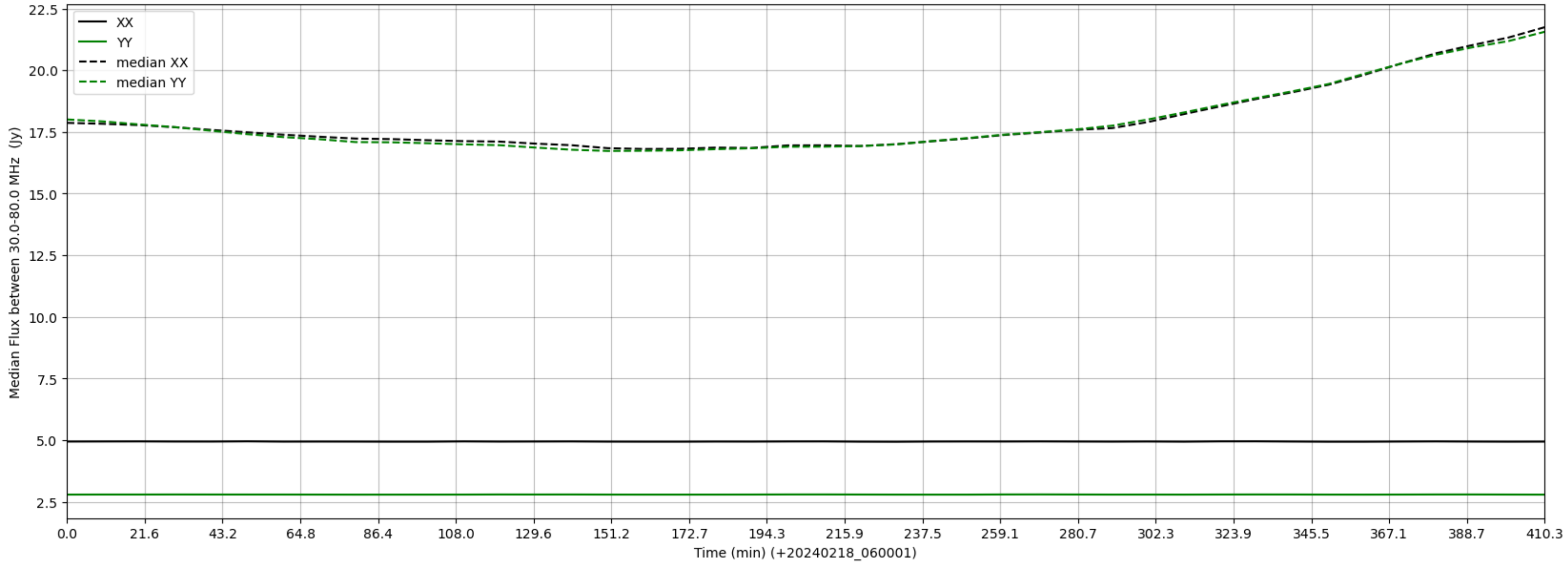
LWA321 - Correlator# 020 - XX FLAGS:BadSpecShape - YY FLAGS:BadSpecShape
