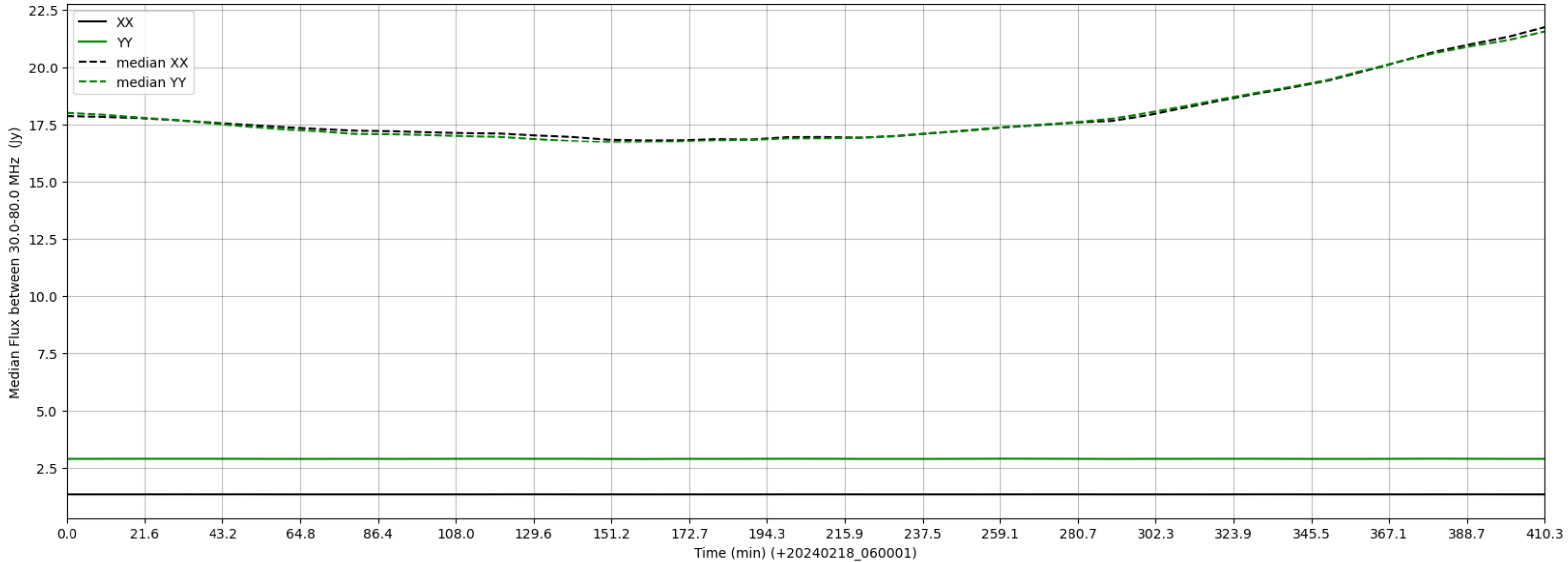
LWA308 - Correlator# 015 - XX FLAGS:LowFlux - YY FLAGS:BadSpecShape
