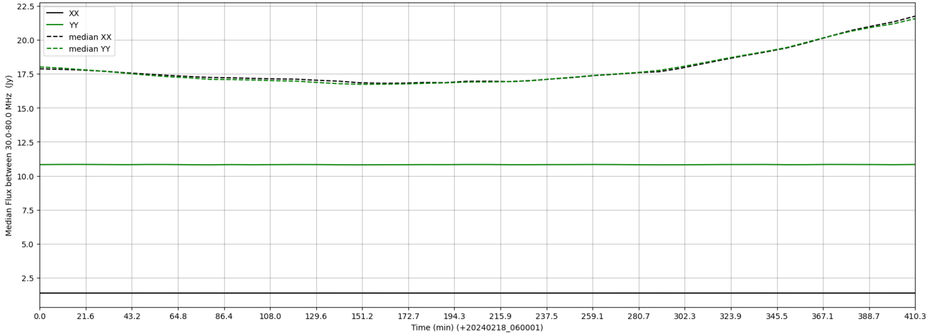
LWA354 - Correlator# 063 - XX FLAGS:LowFlux - YY FLAGS:BadSpecShape
