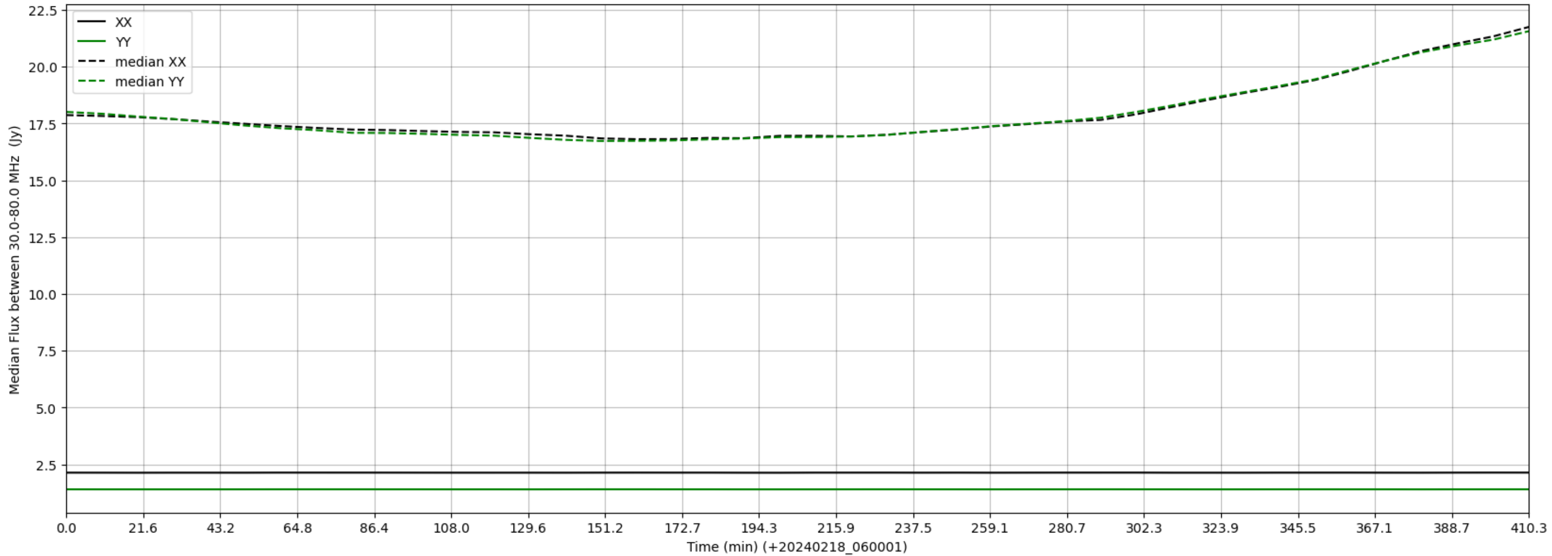
LWA331 - Correlator# 125 - XX FLAGS:BadSpecShape - YY FLAGS:LowFlux
