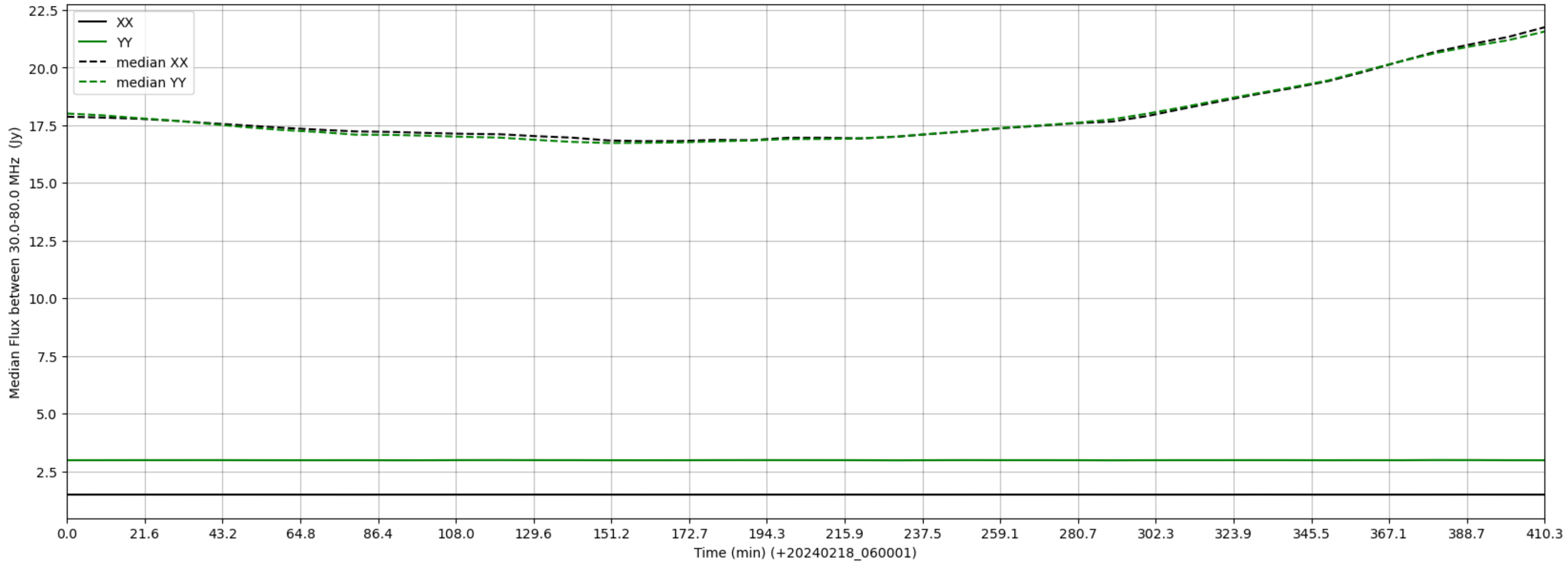
LWA290 - Correlator# 285 - XX FLAGS:LowFlux - YY FLAGS:BadSpecShape
