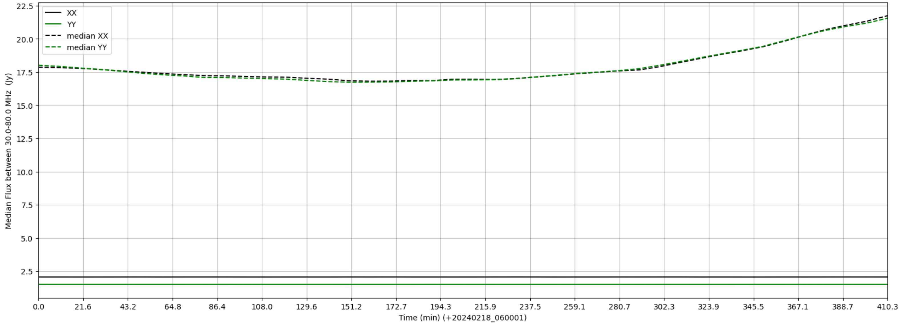
LWA320 - Correlator# 054 - XX FLAGS:BadSpecShape - YY FLAGS:LowFlux
