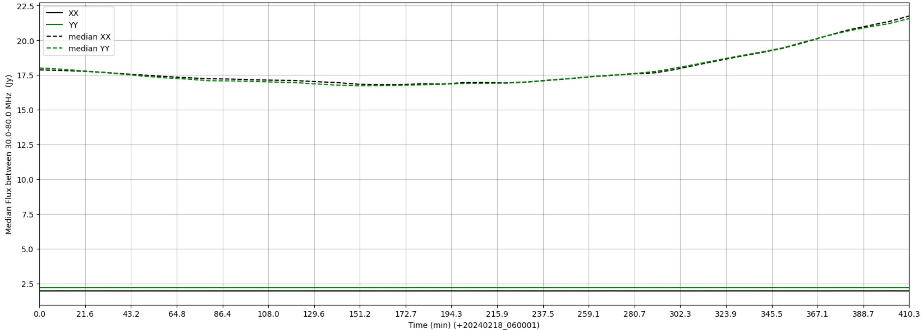
LWA327 - Correlator# 023 - XX FLAGS:BadSpecShape - YY FLAGS:BadSpecShape
