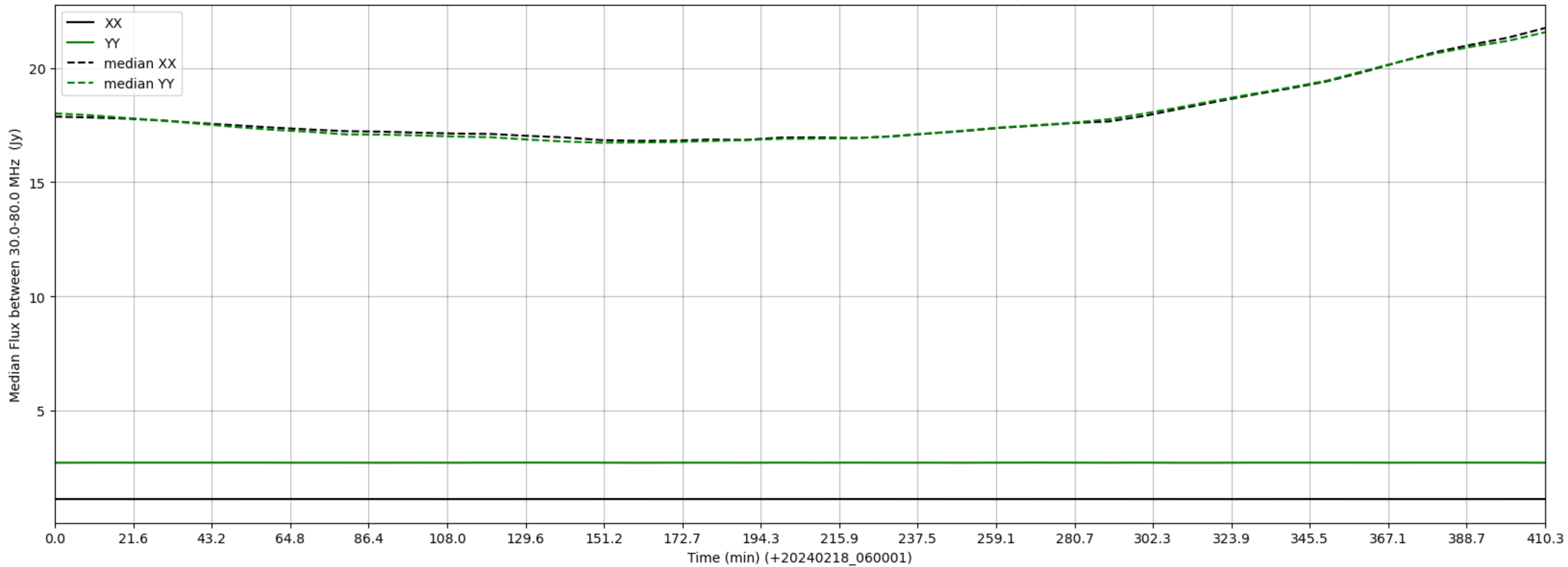
LWA332 - Correlator# 025 - XX FLAGS:LowFlux - YY FLAGS:BadSpecShape
