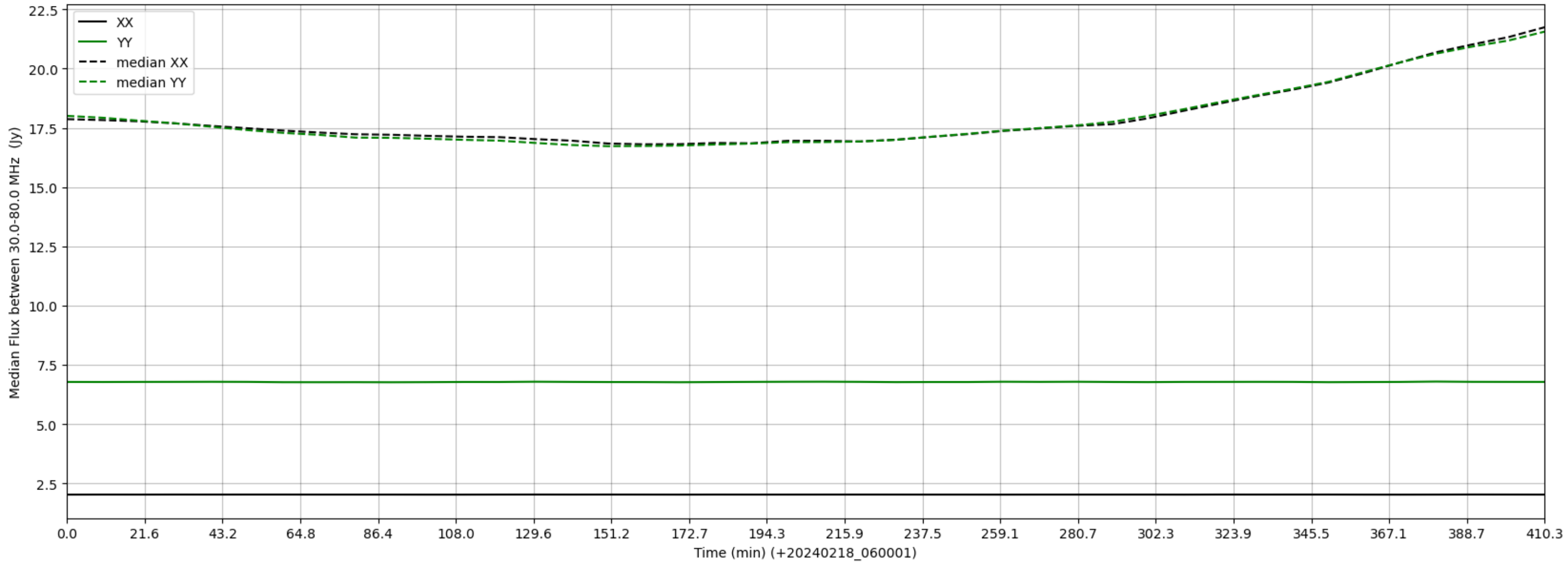
LWA328 - Correlator# 157 - XX FLAGS:BadSpecShape - YY FLAGS:BadSpecShape
