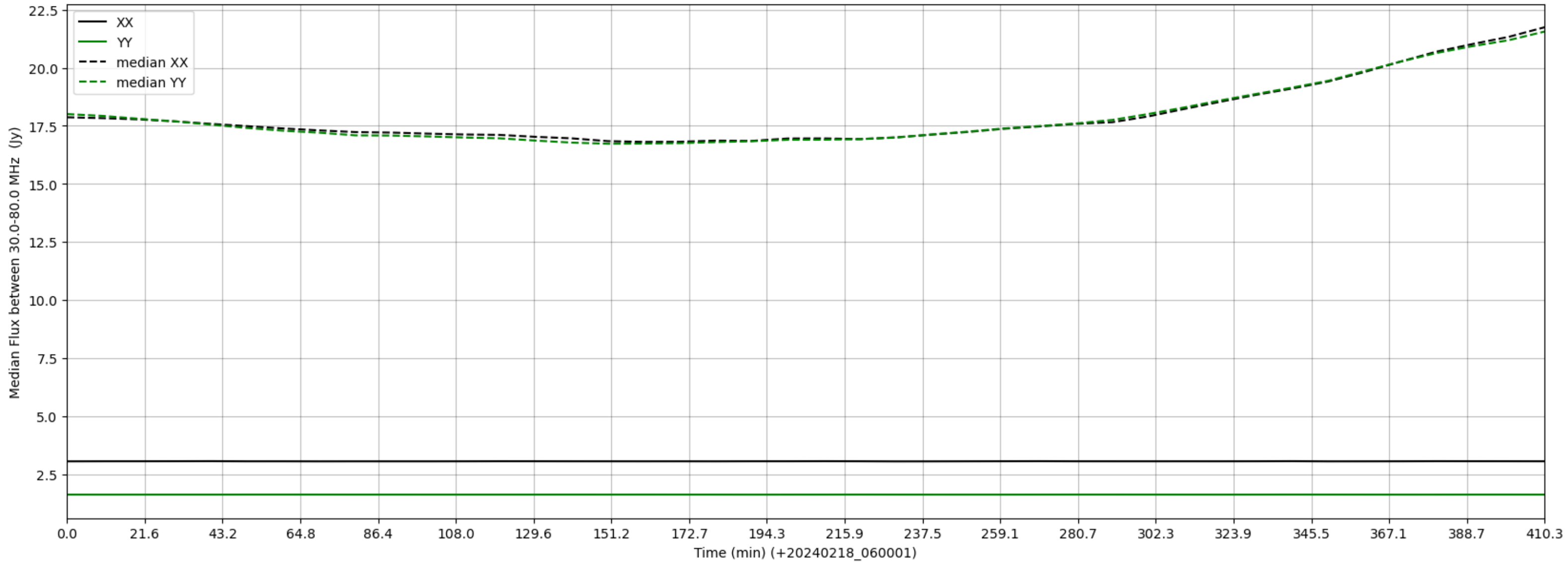
LWA316 - Correlator# 155 - XX FLAGS:BadSpecShape - YY FLAGS:LowFlux
