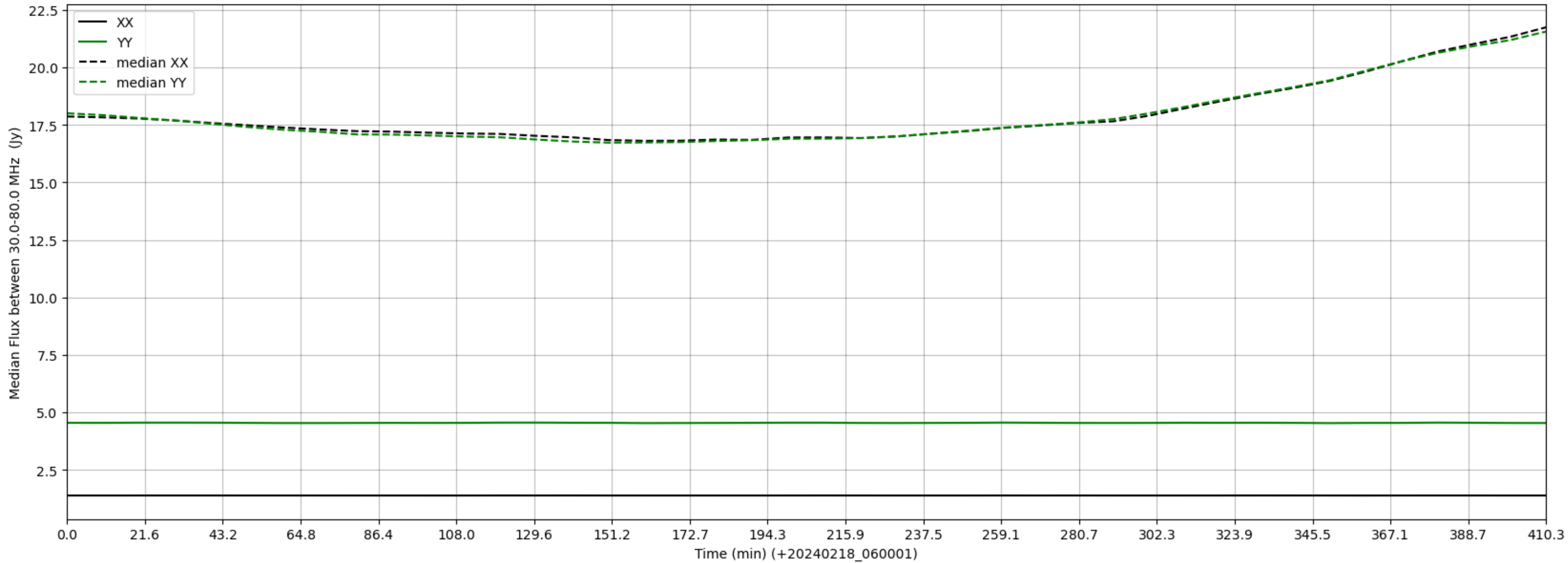
LWA269 - Correlator# 005 - XX FLAGS:LowFlux - YY FLAGS:BadSpecShape
