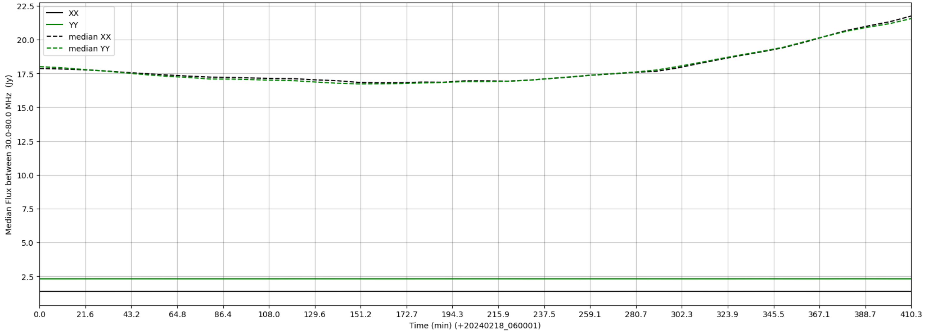
LWA291 - Correlator# 045 - XX FLAGS:LowFlux - YY FLAGS:BadSpecShape
