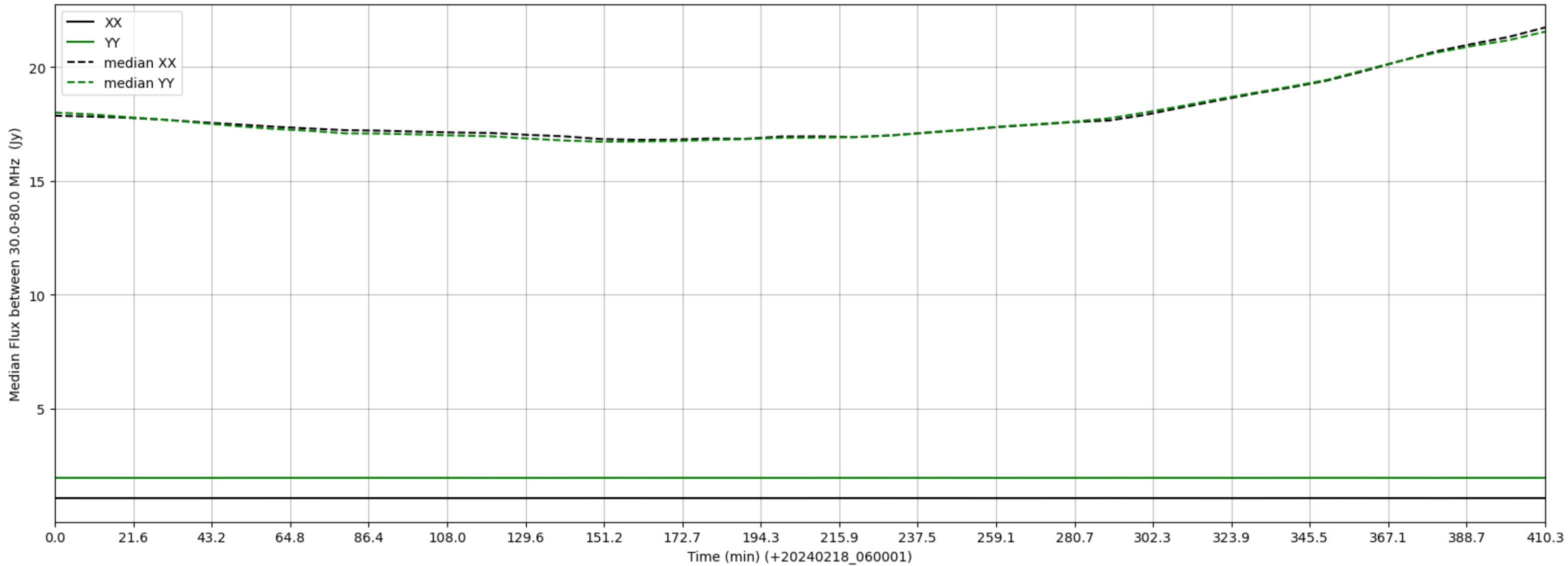
LWA289 - Correlator# 189 - XX FLAGS:LowFlux - YY FLAGS:BadSpecShape
