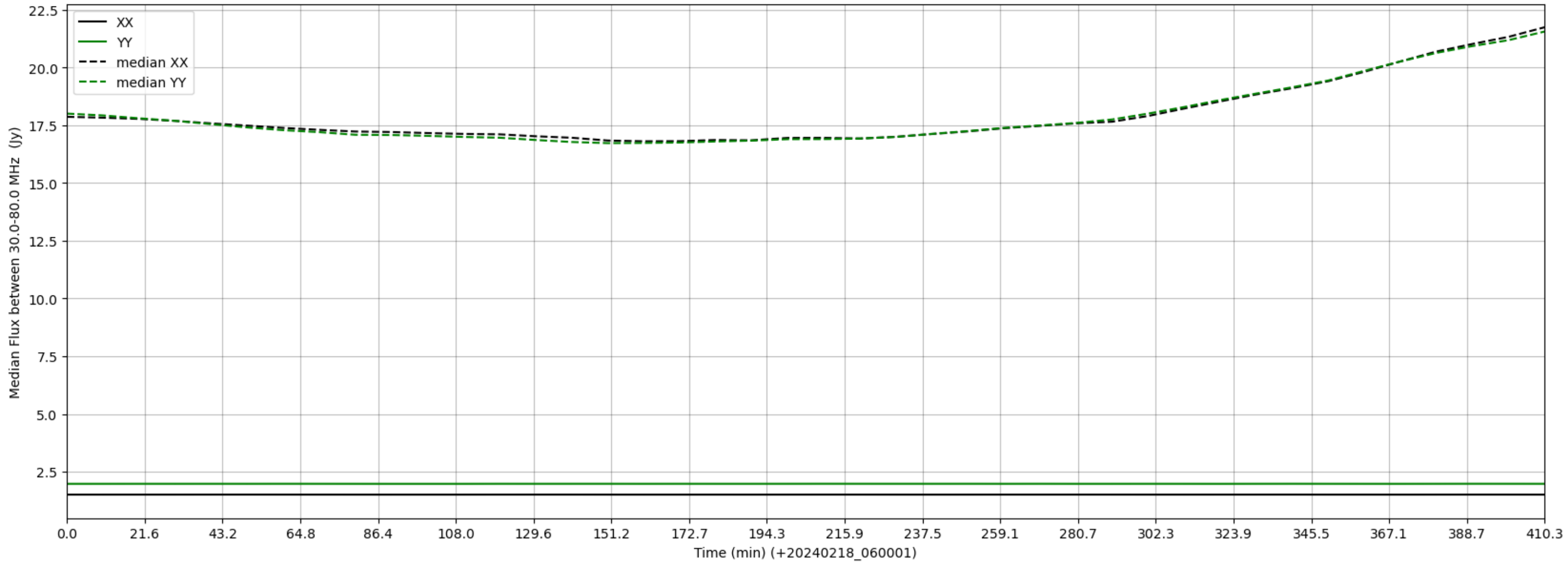
LWA298 - Correlator# 049 - XX FLAGS:LowFlux - YY FLAGS:BadSpecShape
