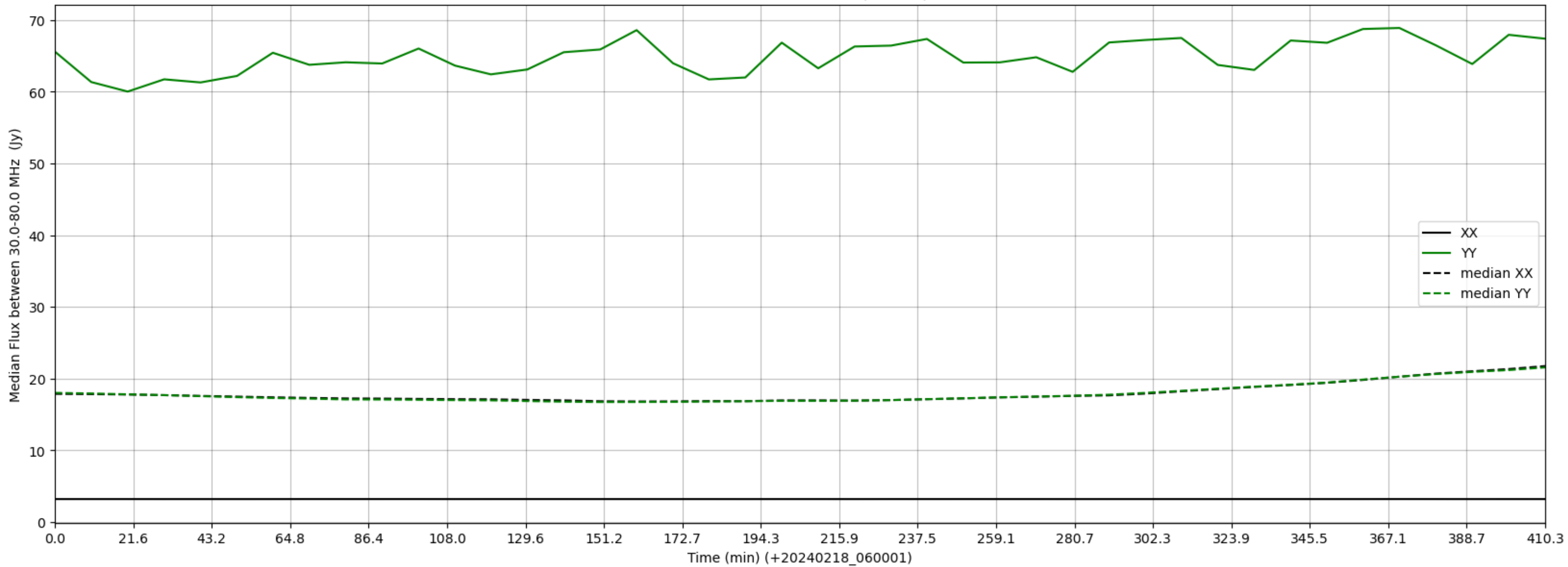
LWA288 - Correlator# 042 - XX FLAGS:BadSpecShape - YY FLAGS:Good
