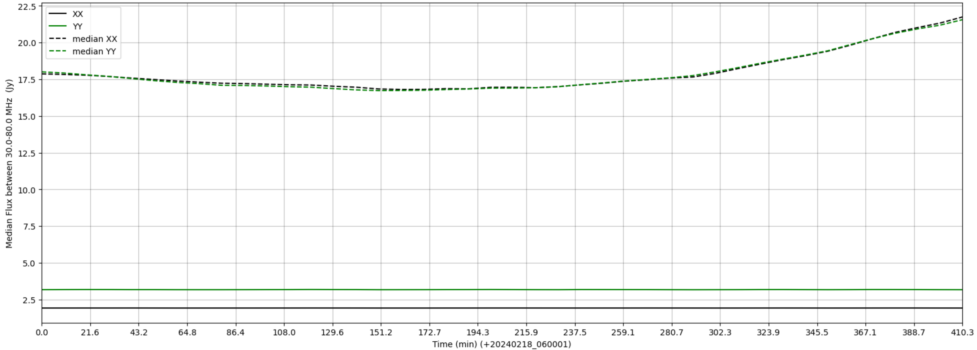
LWA272 - Correlator# 038 - XX FLAGS:BadSpecShape - YY FLAGS:BadSpecShape
