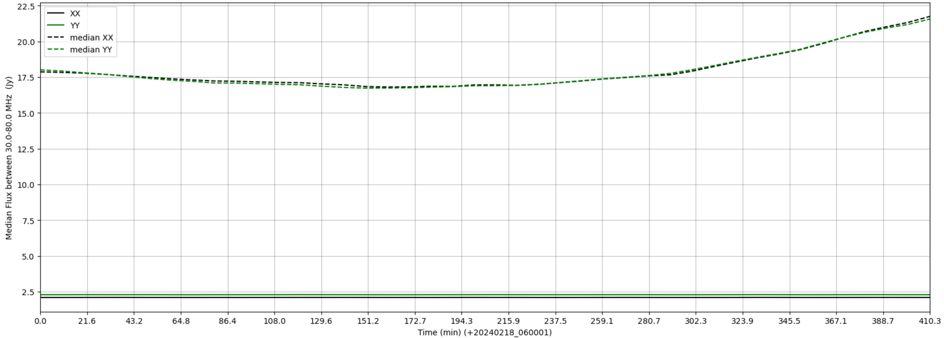
LWA312 - Correlator# 019 - XX FLAGS:BadSpecShape - YY FLAGS:BadSpecShape
