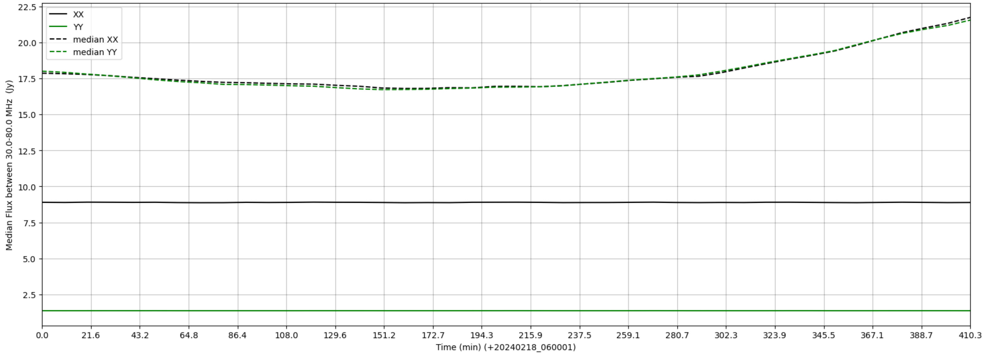
LWA313 - Correlator# 018 - XX FLAGS:BadSpecShape - YY FLAGS:LowFlux
