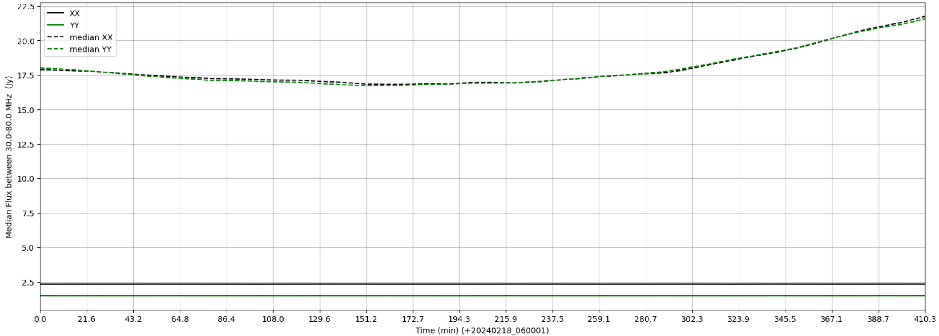
LWA329 - Correlator# 287 - XX FLAGS:BadSpecShape - YY FLAGS:LowFlux
