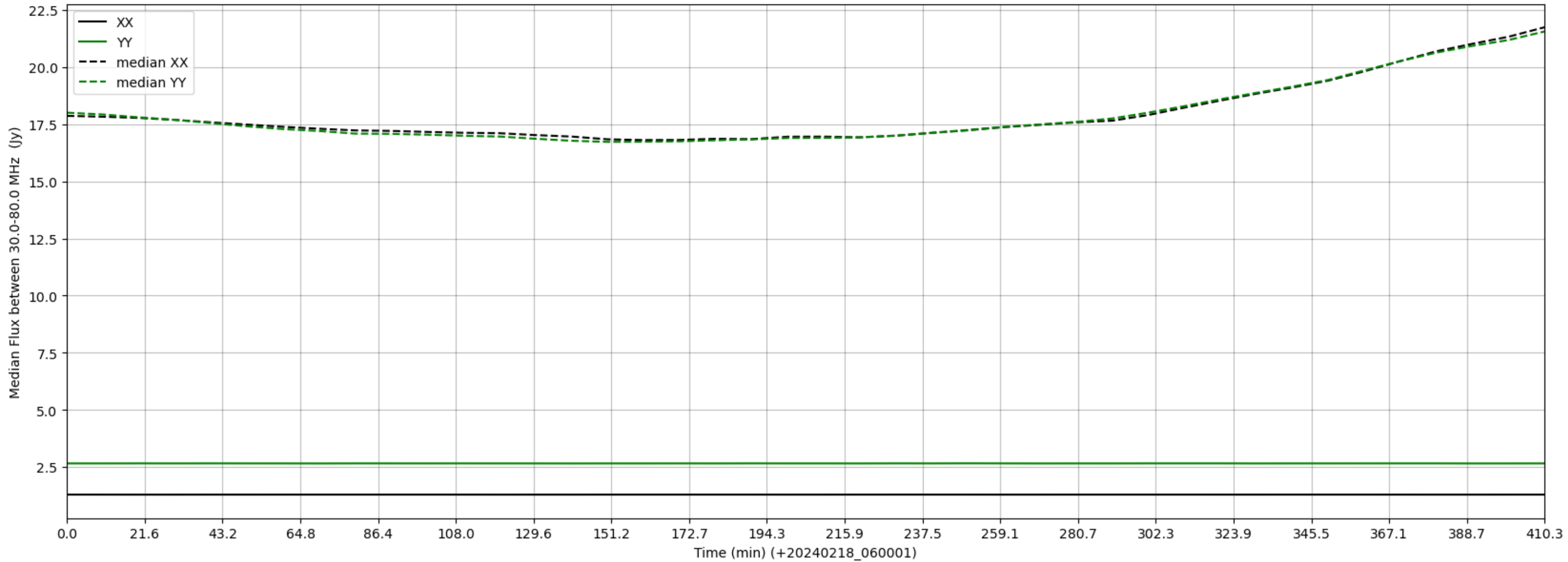
LWA259 - Correlator# 001 - XX FLAGS:LowFlux - YY FLAGS:BadSpecShape
