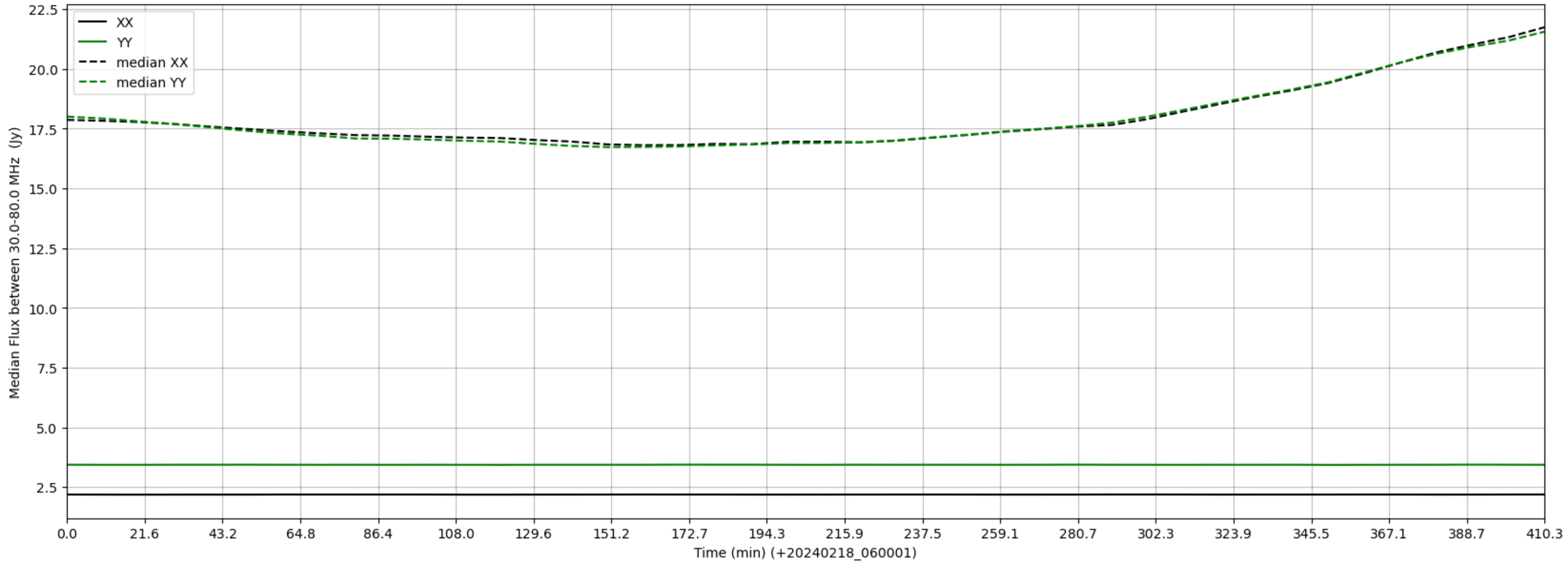
LWA275 - Correlator# 090 - XX FLAGS:BadSpecShape - YY FLAGS:BadSpecShape
