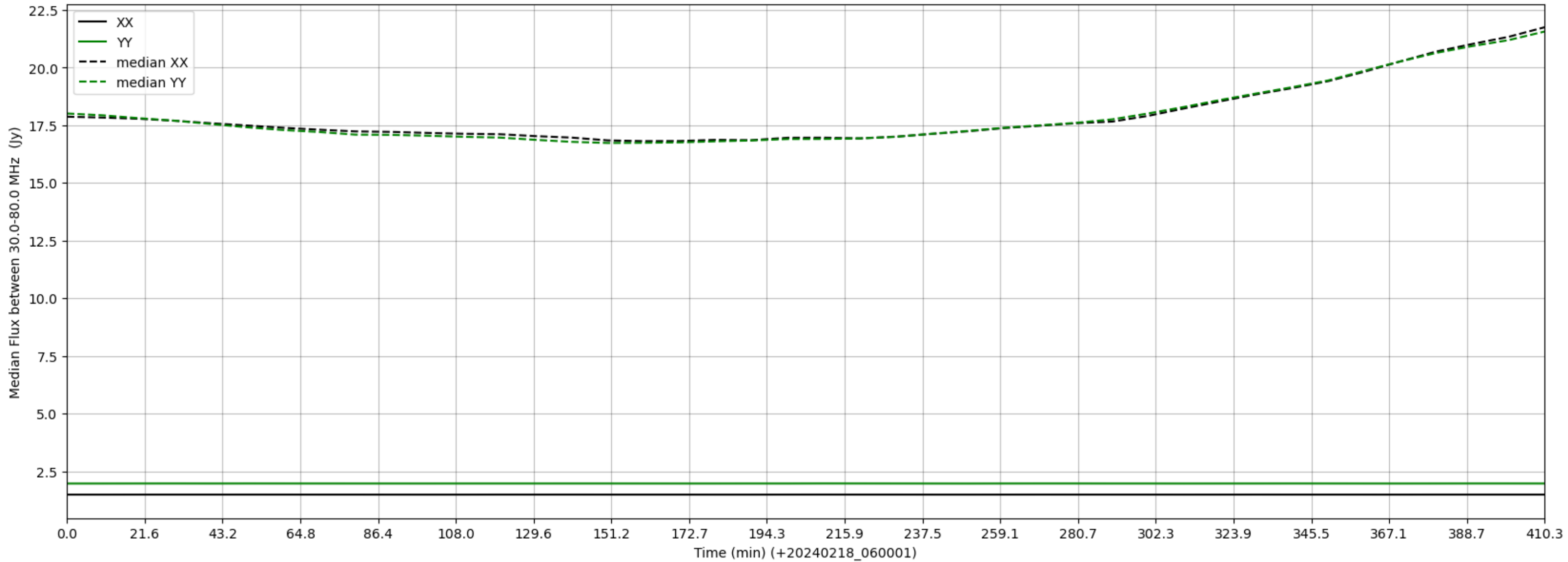
LWA271 - Correlator# 004 - XX FLAGS:LowFlux - YY FLAGS:BadSpecShape
