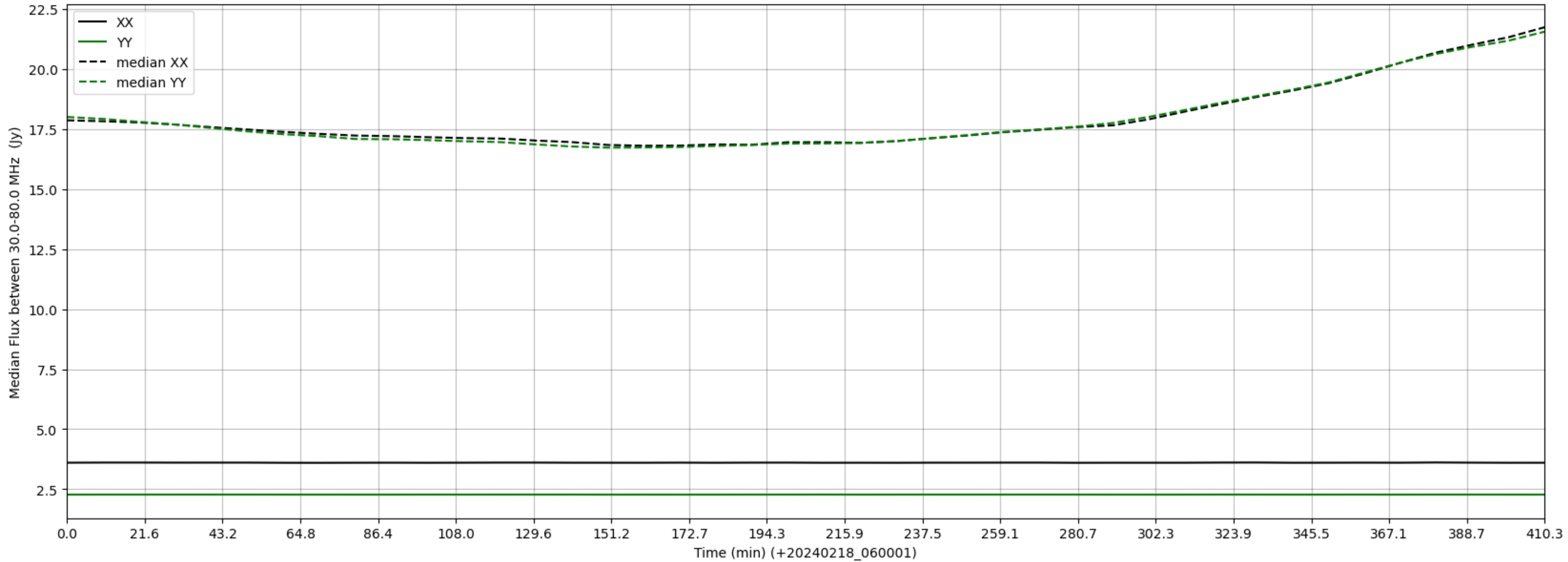
LWA333 - Correlator# 253 - XX FLAGS:BadSpecShape - YY FLAGS:BadSpecShape
