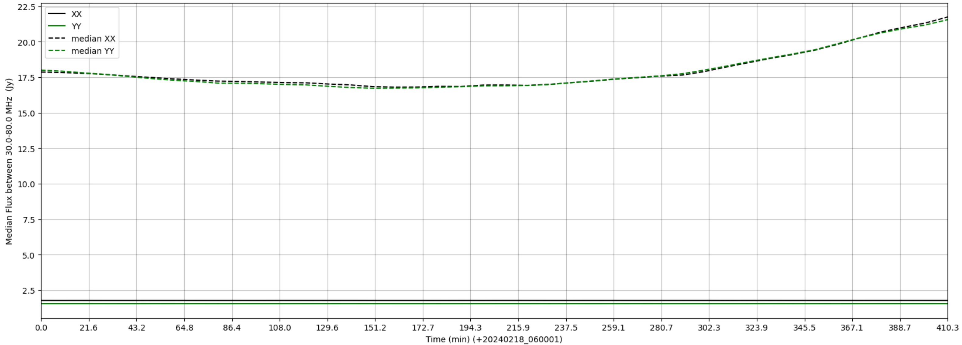
LWA350 - Correlator# 319 - XX FLAGS:BadSpecShape - YY FLAGS:LowFlux
