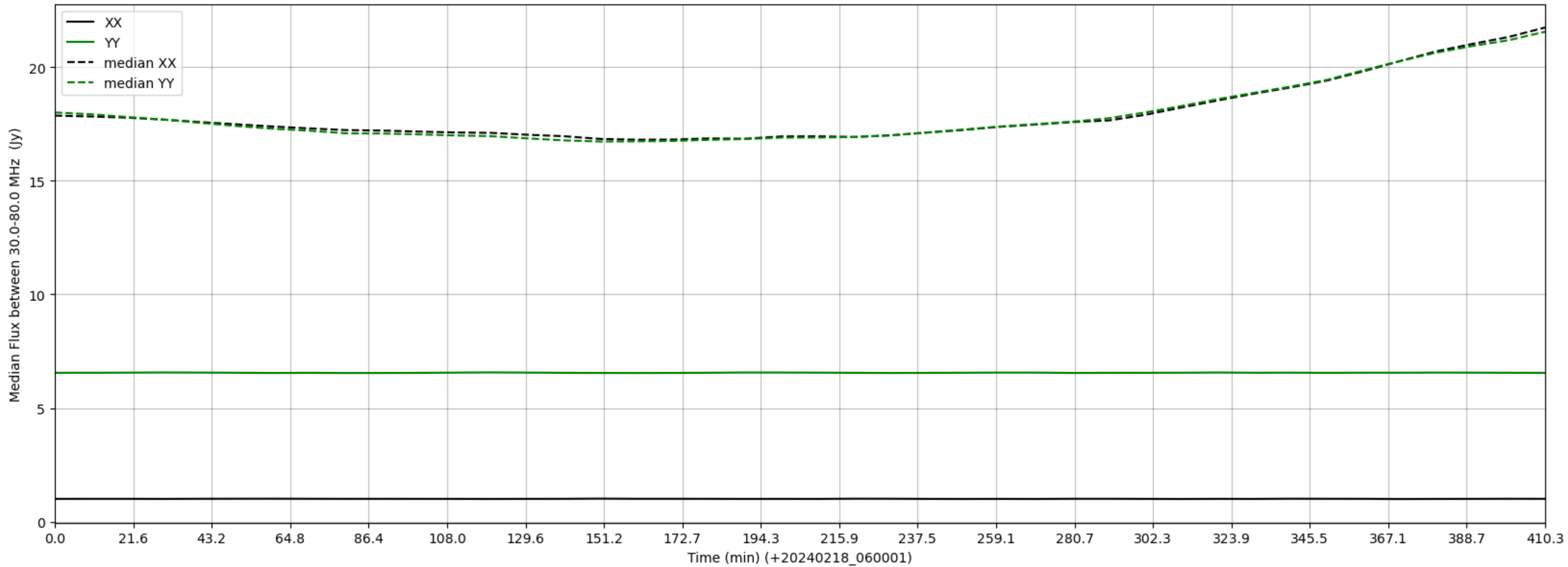
LWA335 - Correlator# 057 - XX FLAGS:LowFlux - YY FLAGS:BadSpecShape
