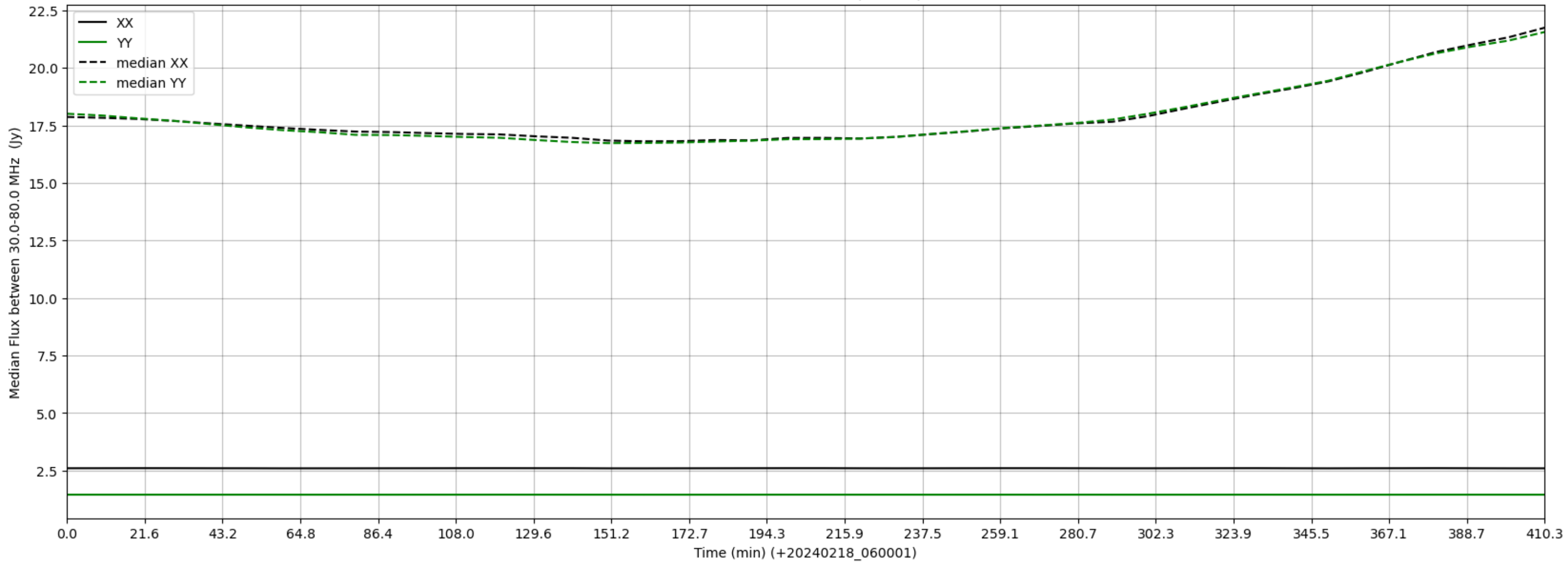
LWA330 - Correlator# 022 - XX FLAGS:BadSpecShape - YY FLAGS:LowFlux
