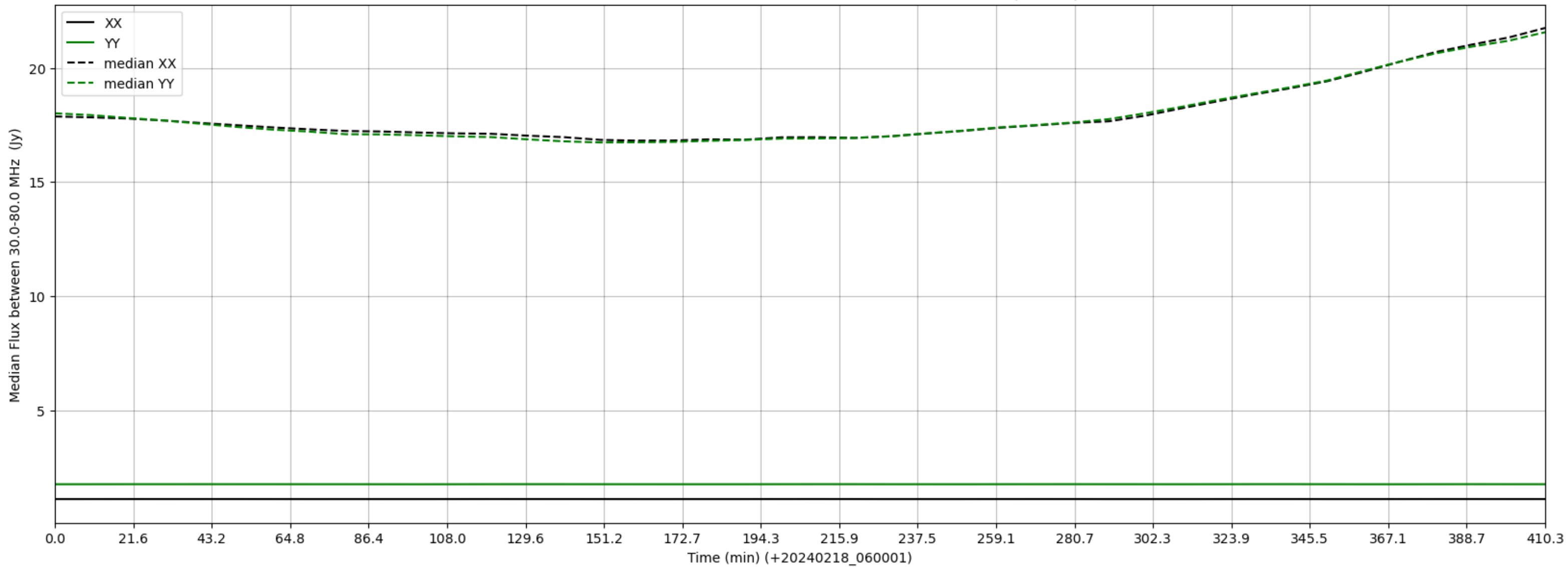
LWA296 - Correlator# 046 - XX FLAGS:LowFlux - YY FLAGS:BadSpecShape
