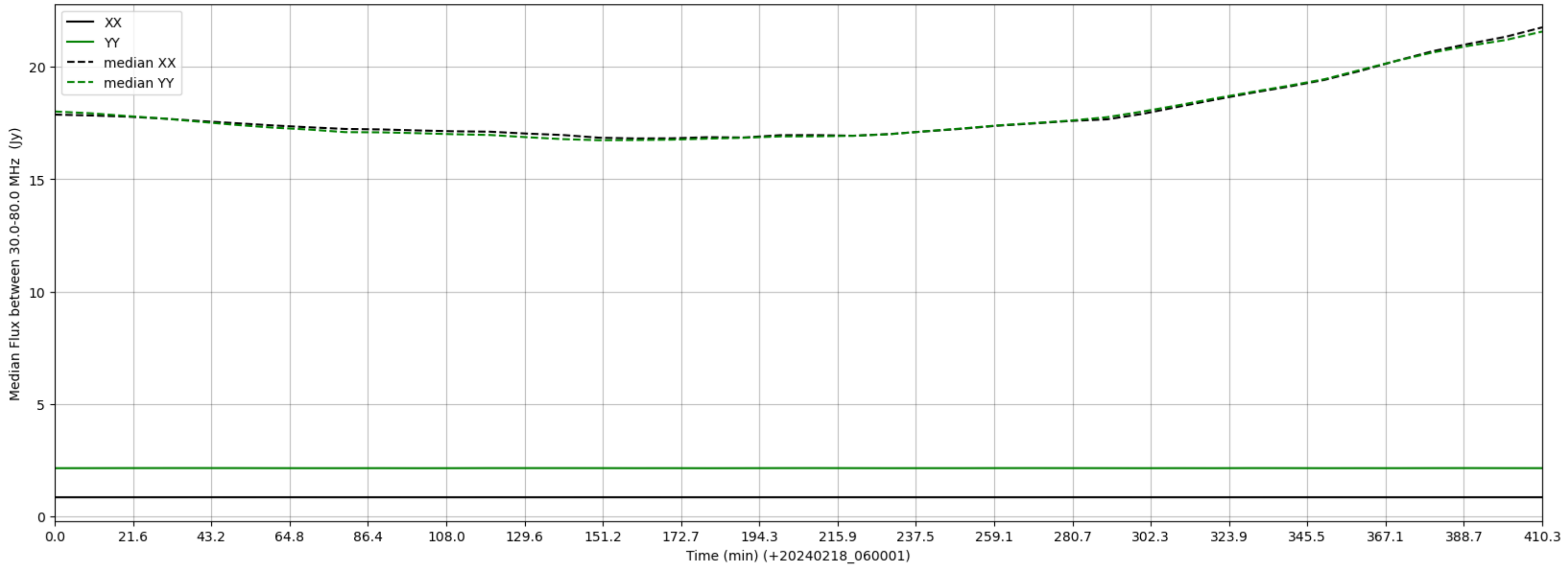
LWA322 - Correlator# 251 - XX FLAGS:LowFlux - YY FLAGS:BadSpecShape
