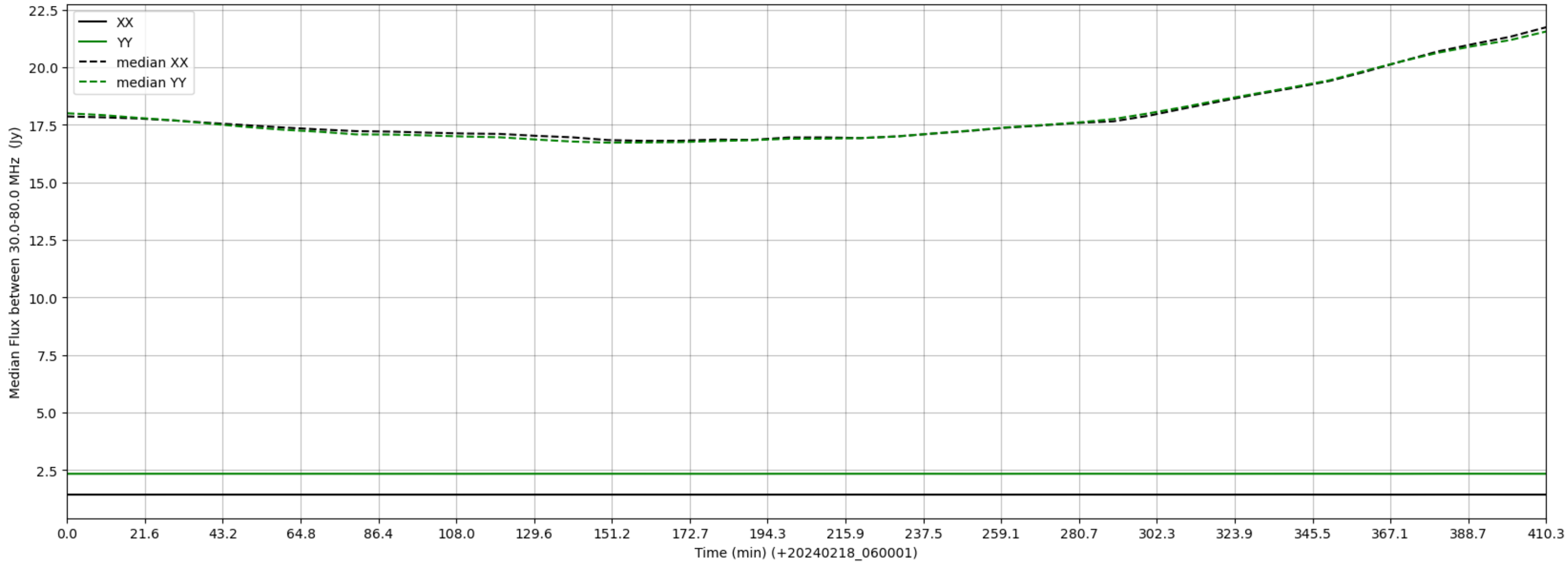
LWA337 - Correlator# 059 - XX FLAGS:LowFlux - YY FLAGS:BadSpecShape
