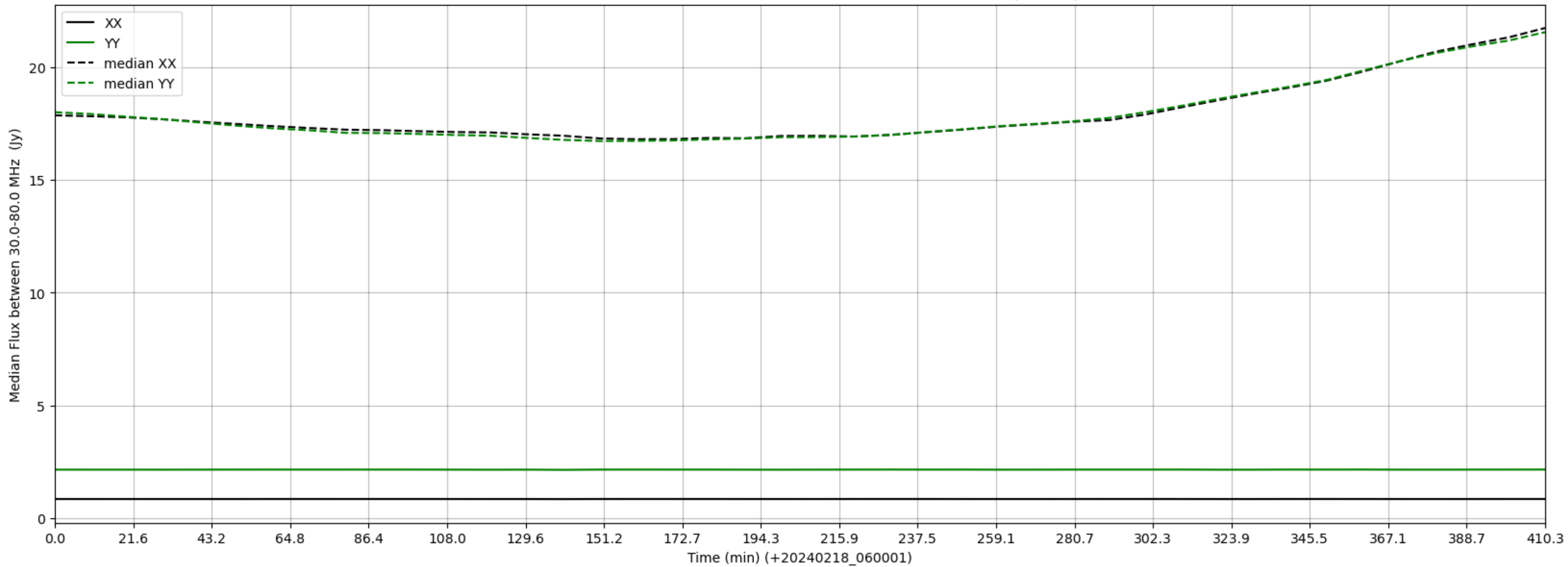
LWA348 - Correlator# 124 - XX FLAGS:LowFlux - YY FLAGS:BadSpecShape
