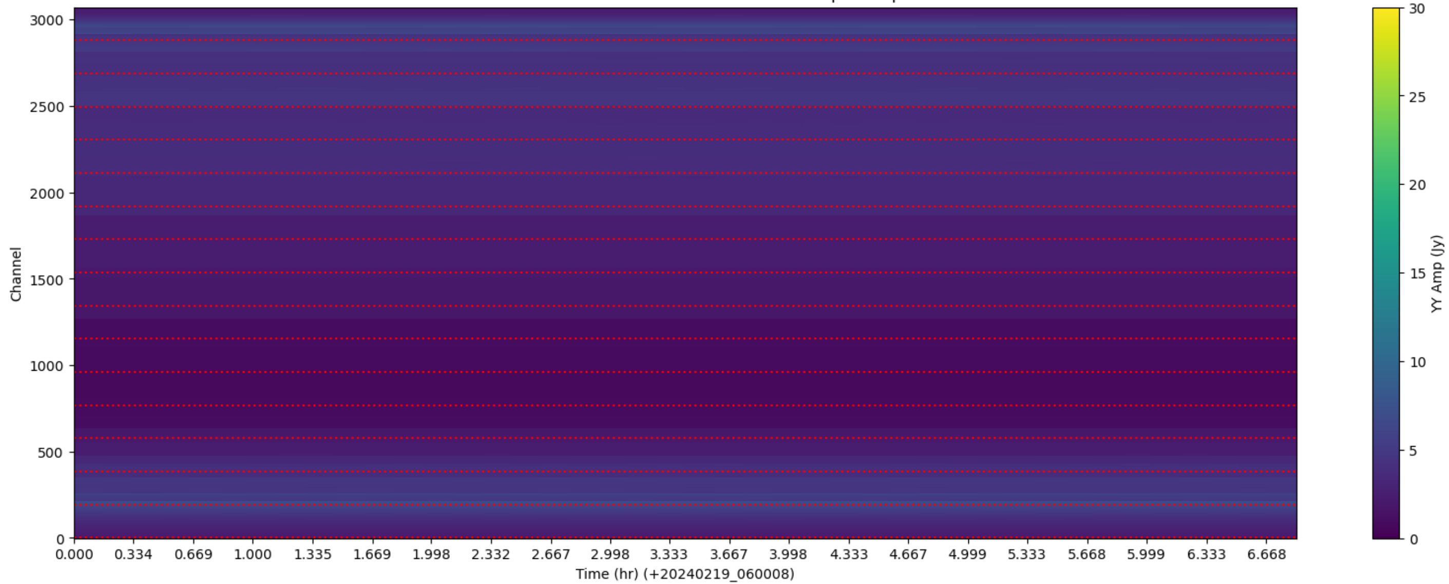
LWA312 - Correlator# 019 - YY - FLAGS: BadSpecShape
