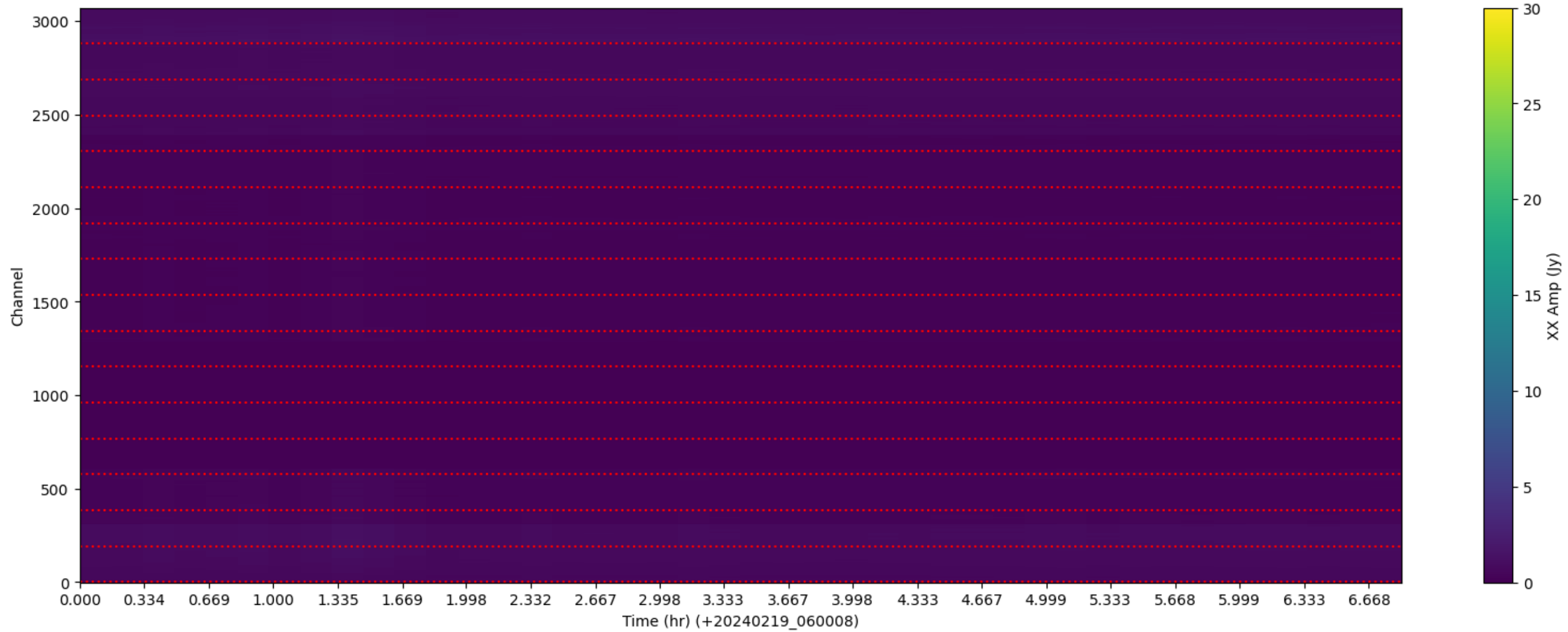
LWA187 - Correlator# 242 - XX - FLAGS: LowFlux
