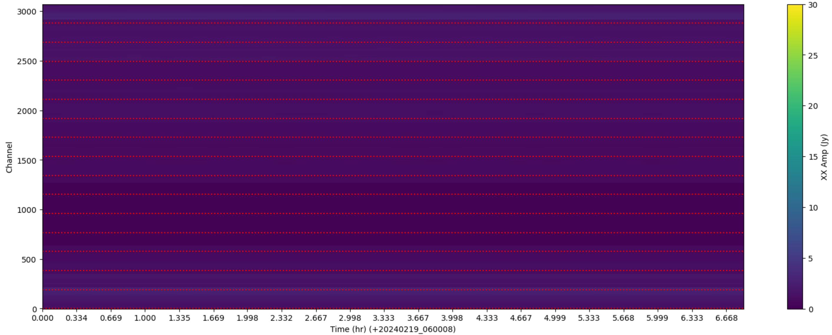
LWA348 - Correlator# 124 - XX - FLAGS: LowFlux
