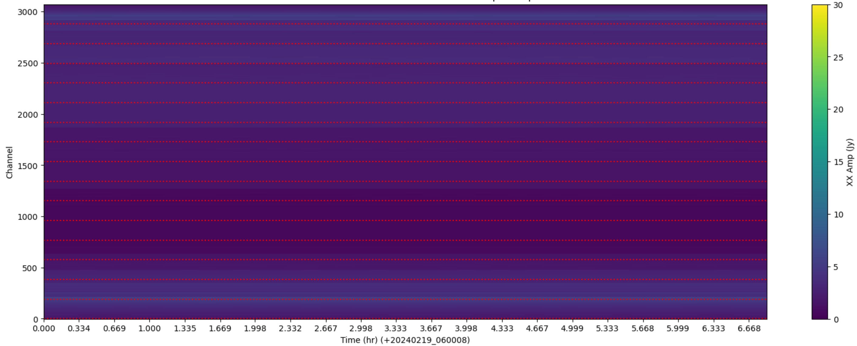
LWA309 - Correlator# 014 - XX - FLAGS: BadSpecShape
