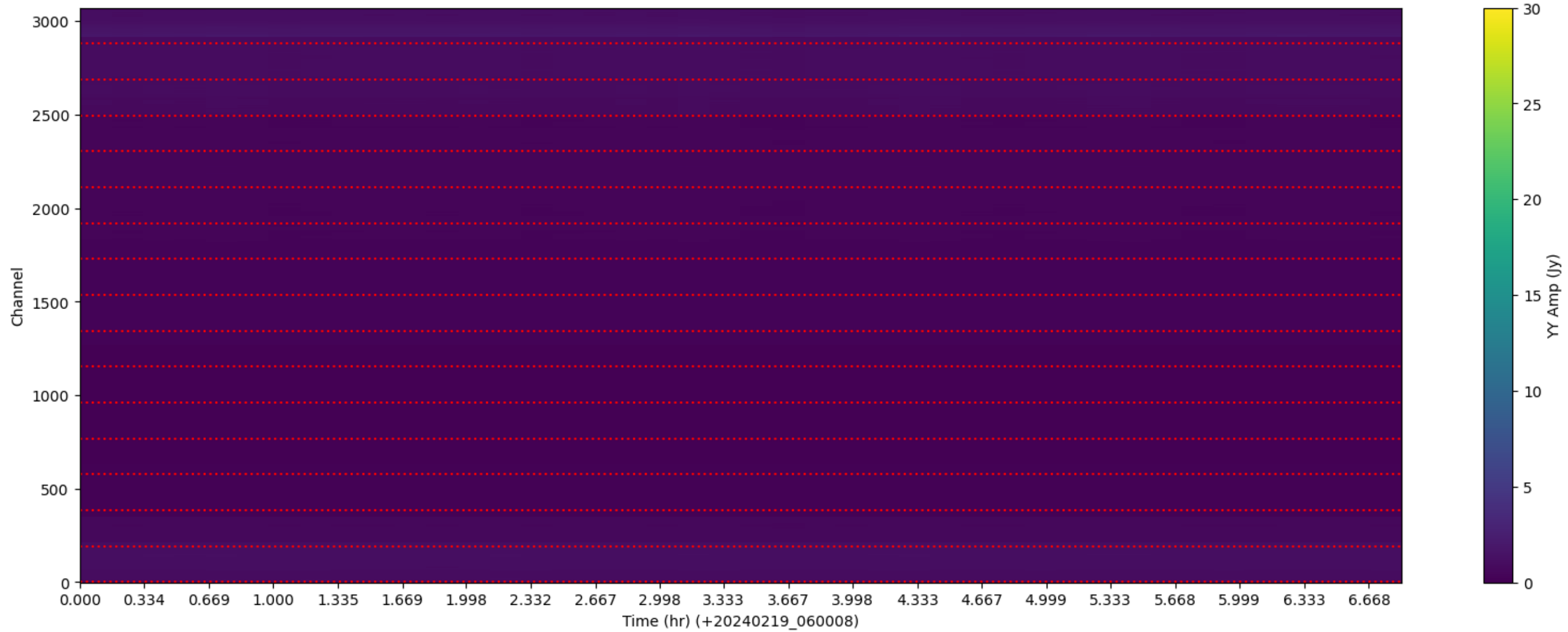
LWA307 - Correlator# 012 - YY - FLAGS: LowFlux
