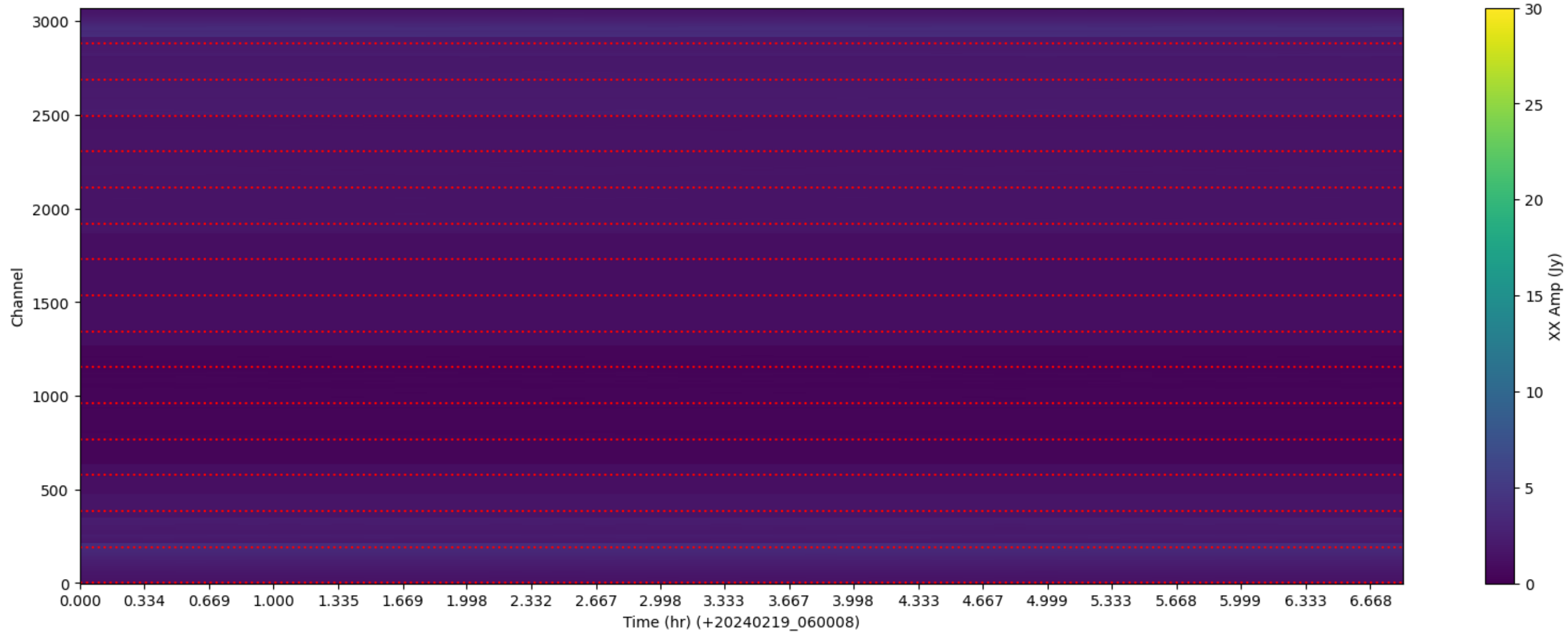
LWA332 - Correlator# 025 - XX - FLAGS: LowFlux
