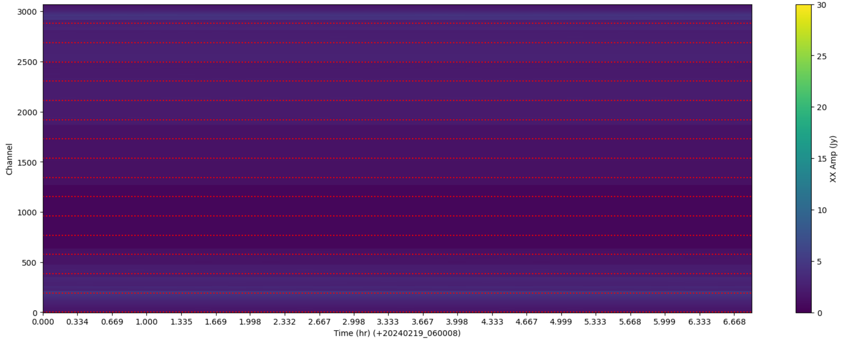
LWA271 - Correlator# 004 - XX - FLAGS: LowFlux
