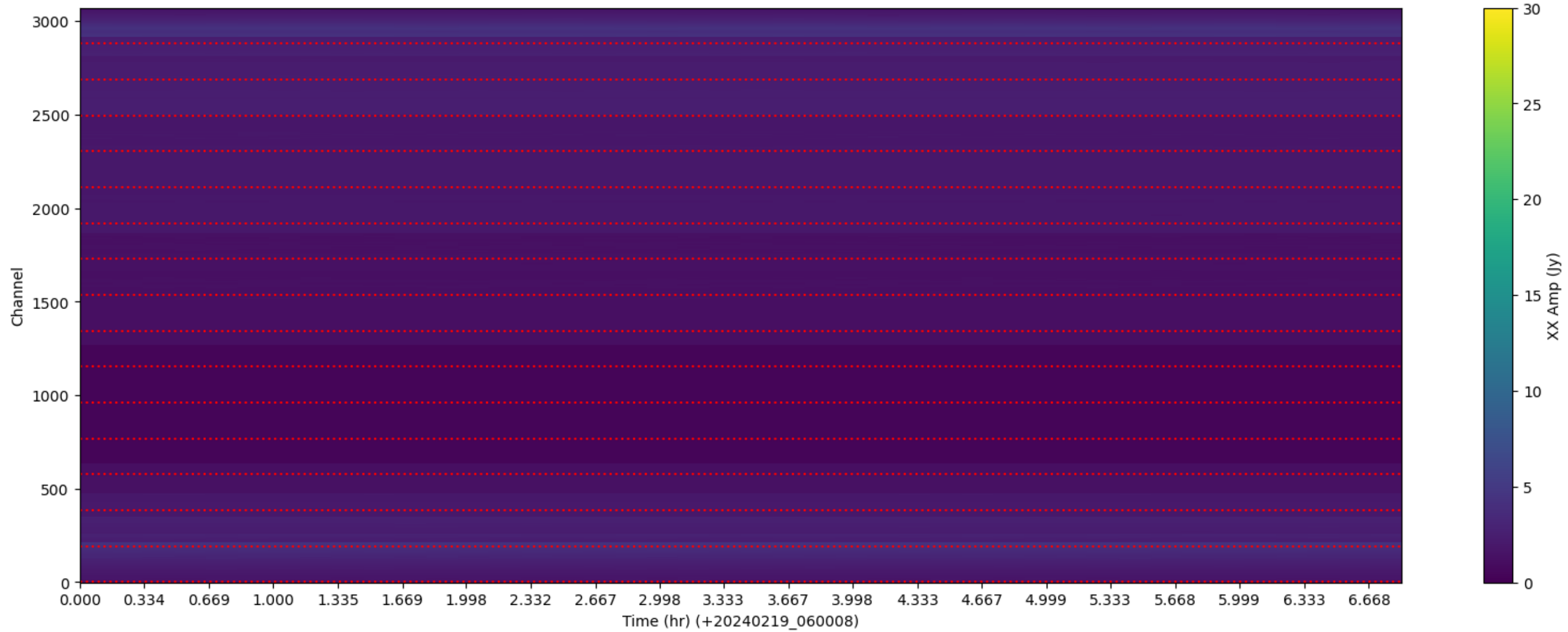
LWA259 - Correlator# 001 - XX - FLAGS: LowFlux
