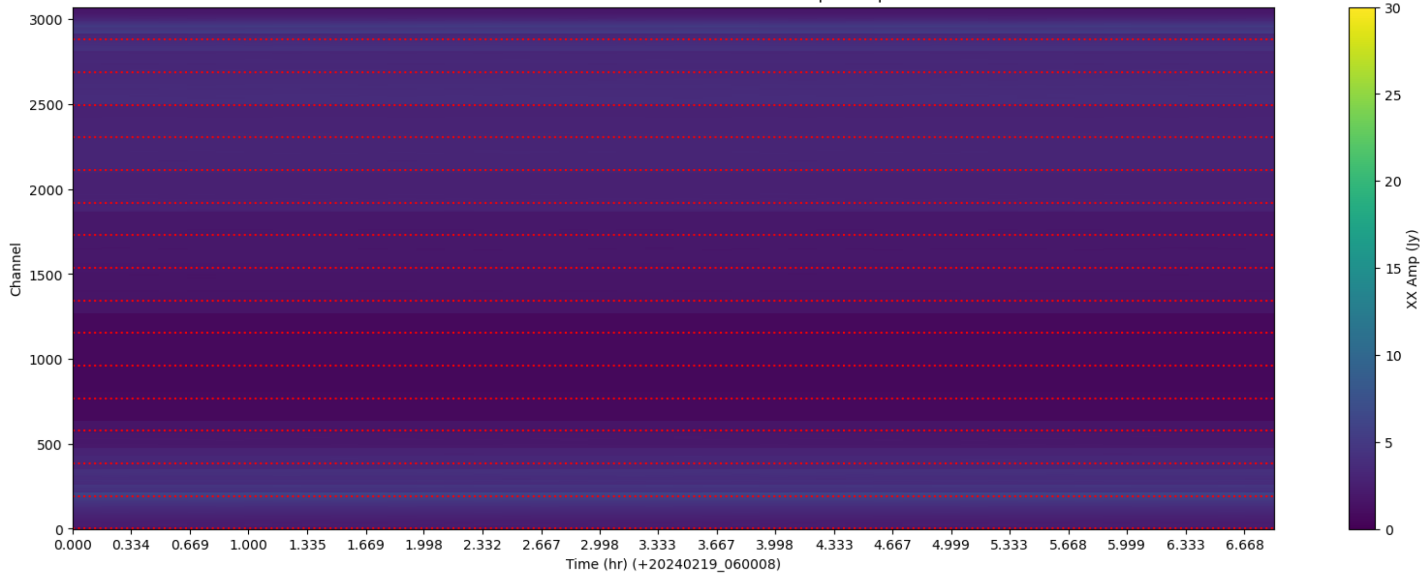
LWA279 - Correlator# 220 - XX - FLAGS: BadSpecShape
