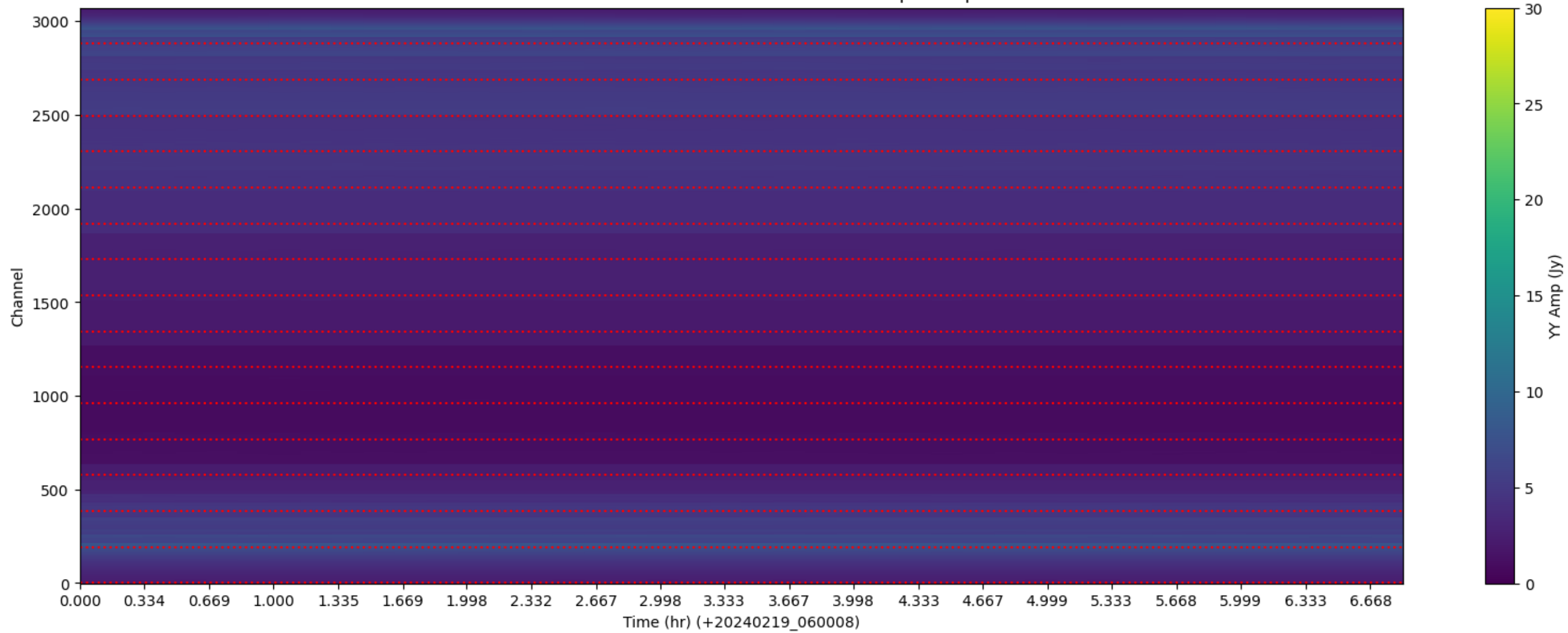
LWA257 - Correlator# 032 - YY - FLAGS: BadSpecShape
