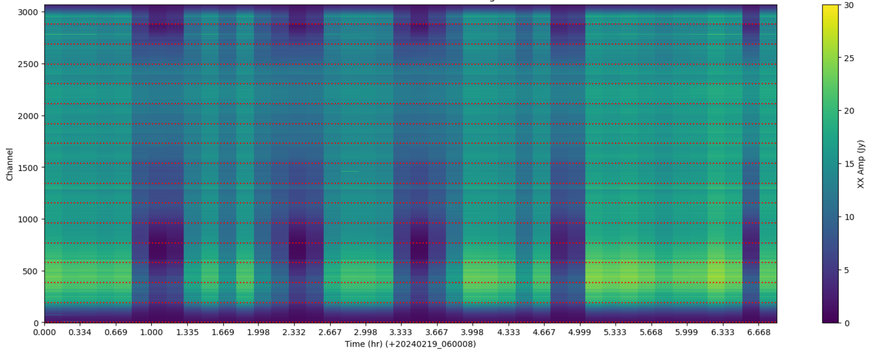
LWA120 - Correlator# 208 - XX - FLAGS: HighTimeVar
