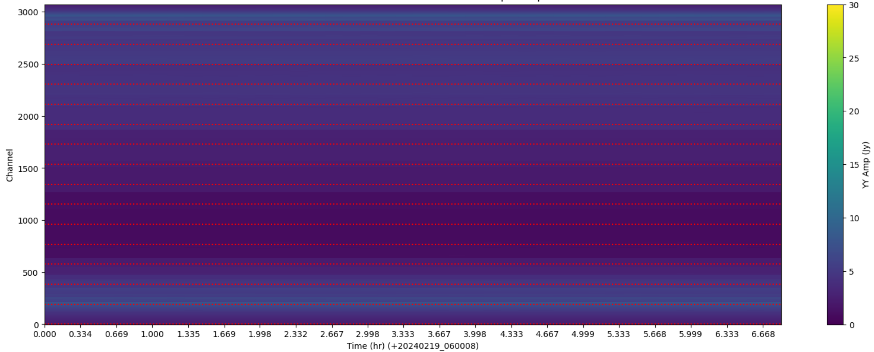
LWA259 - Correlator# 001 - YY - FLAGS: BadSpecShape
