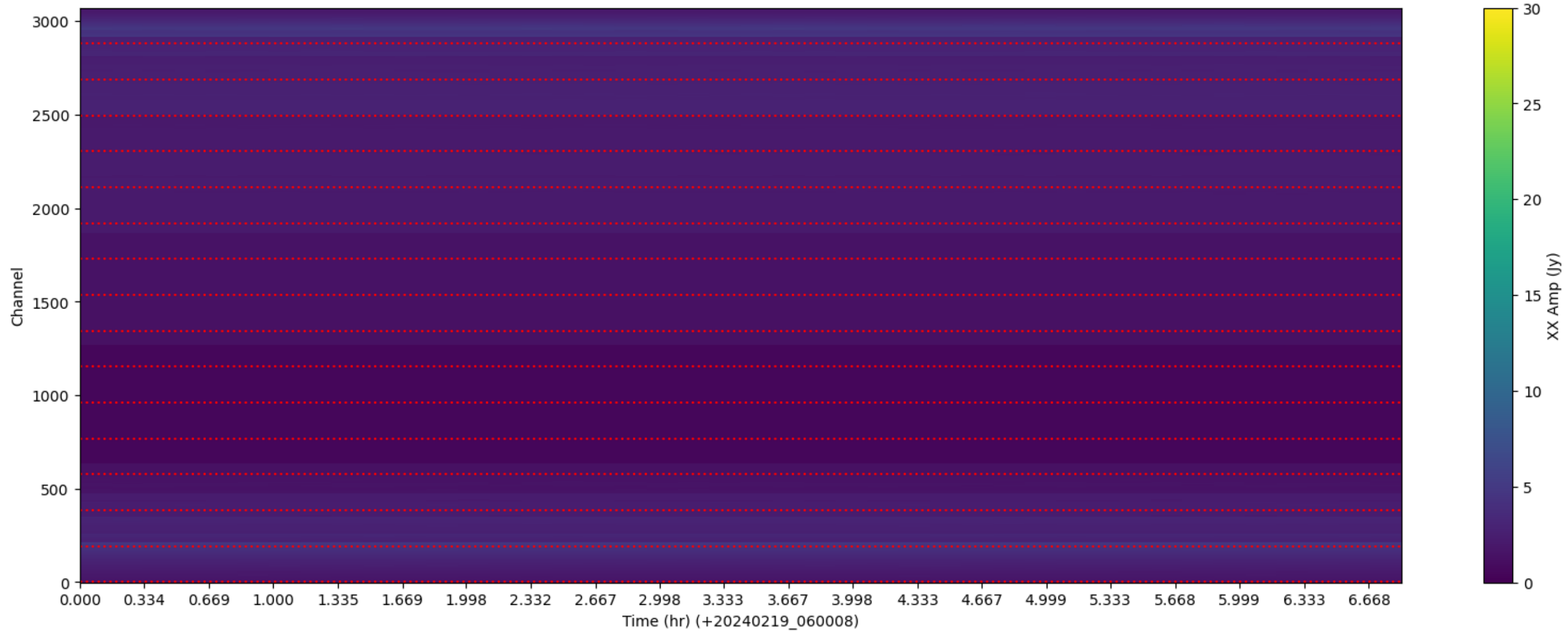
LWA292 - Correlator# 044 - XX - FLAGS: LowFlux
