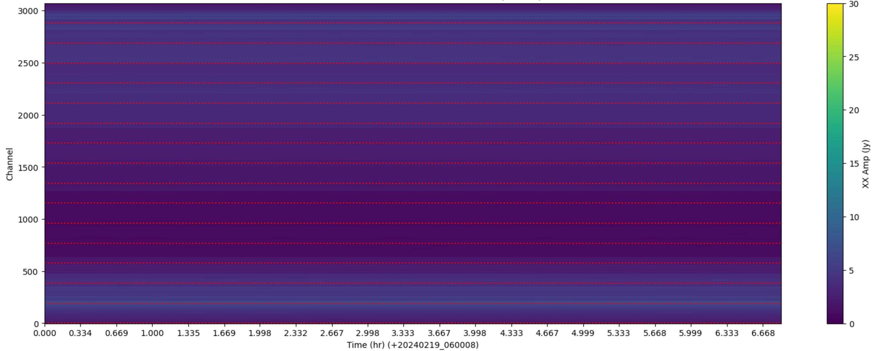
LWA329 - Correlator# 287 - XX - FLAGS: BadSpecShape
