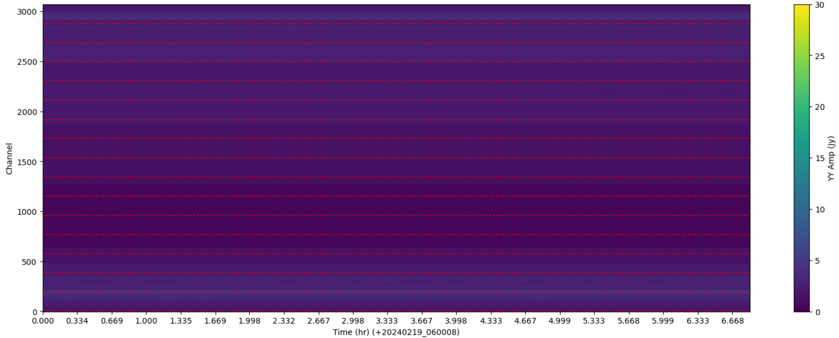
LWA313 - Correlator# 018 - YY - FLAGS: LowFlux
