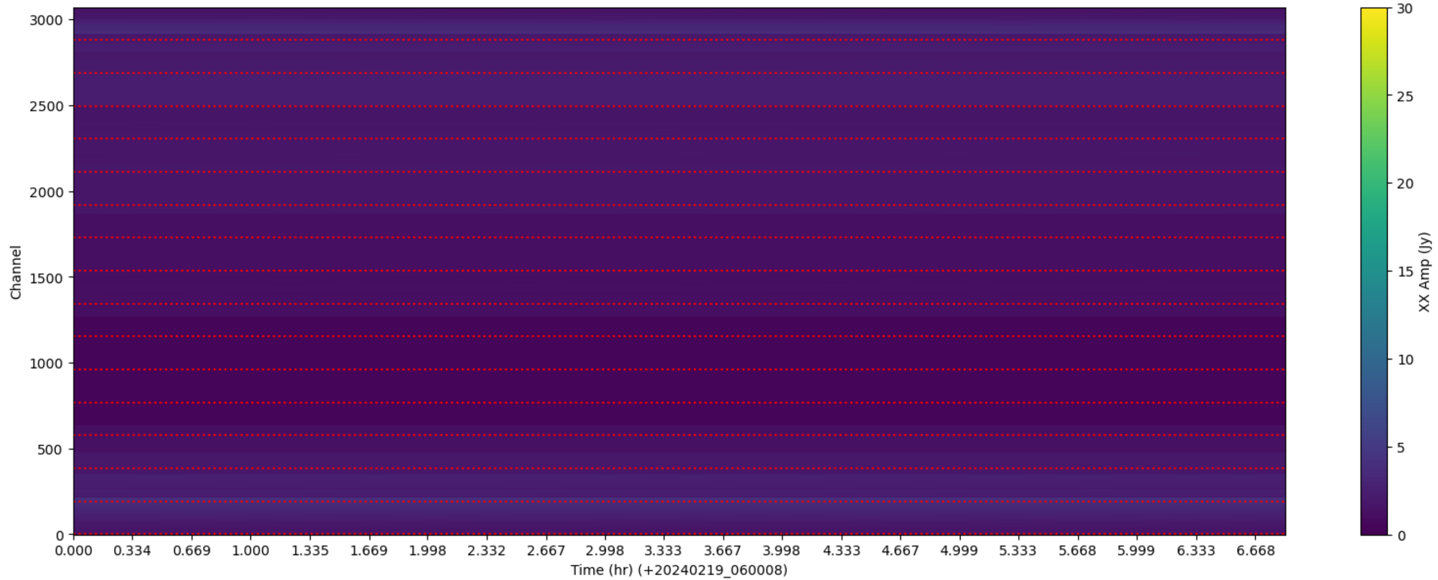
LWA282 - Correlator# 010 - XX - FLAGS: LowFlux
