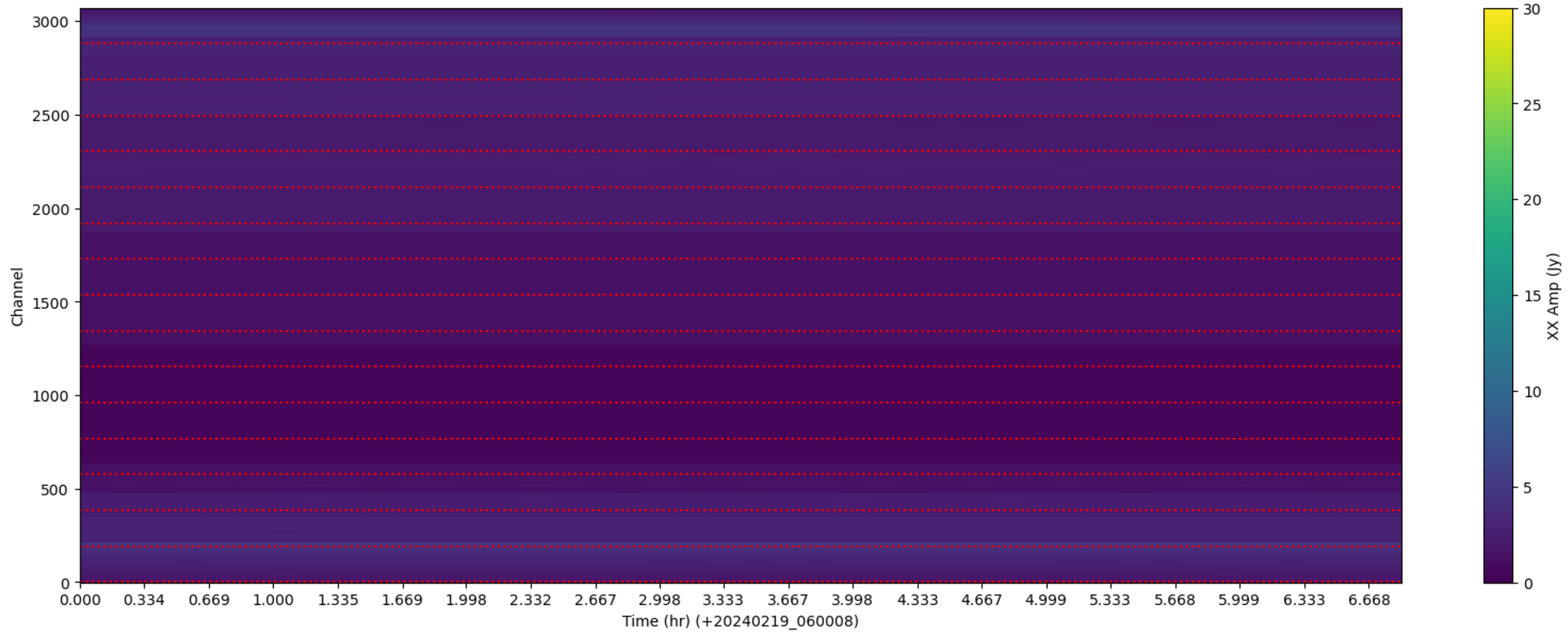
LWA341 - Correlator# 029 - XX - FLAGS: LowFlux
