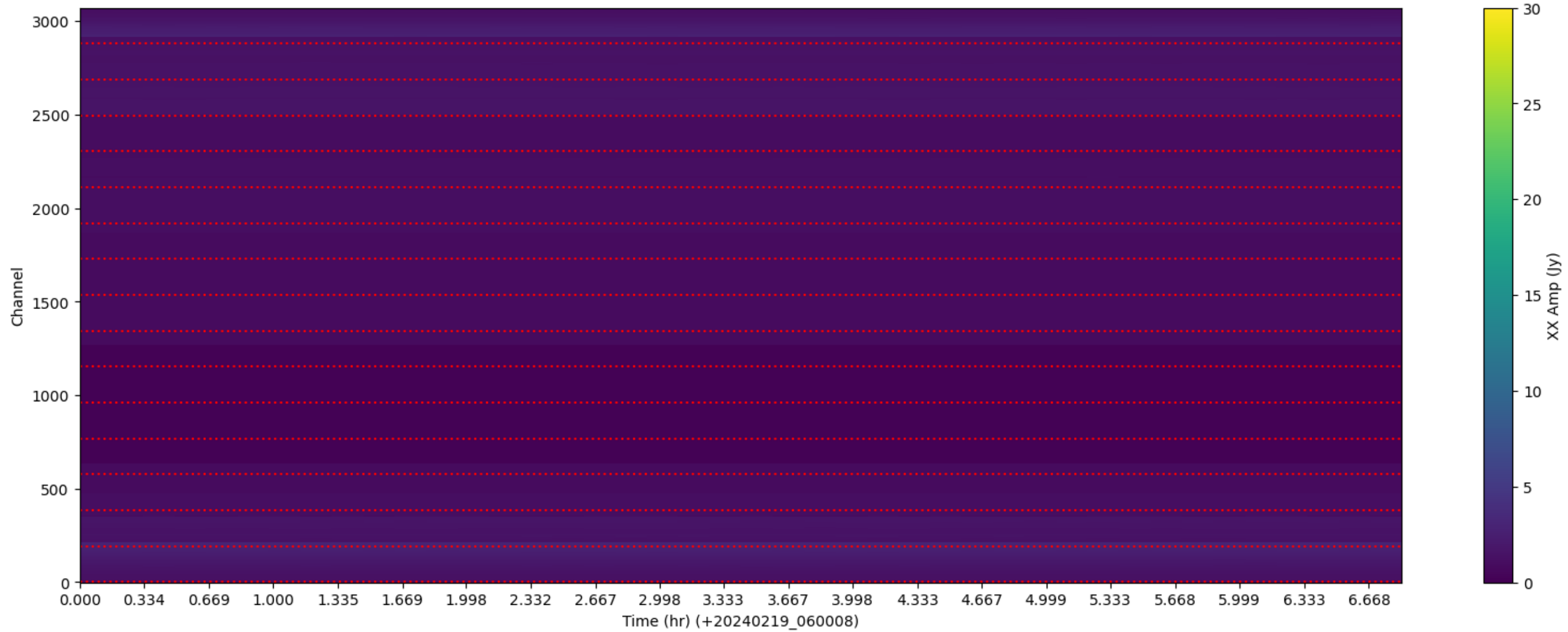
LWA260 - Correlator# 034 - XX - FLAGS: LowFlux
