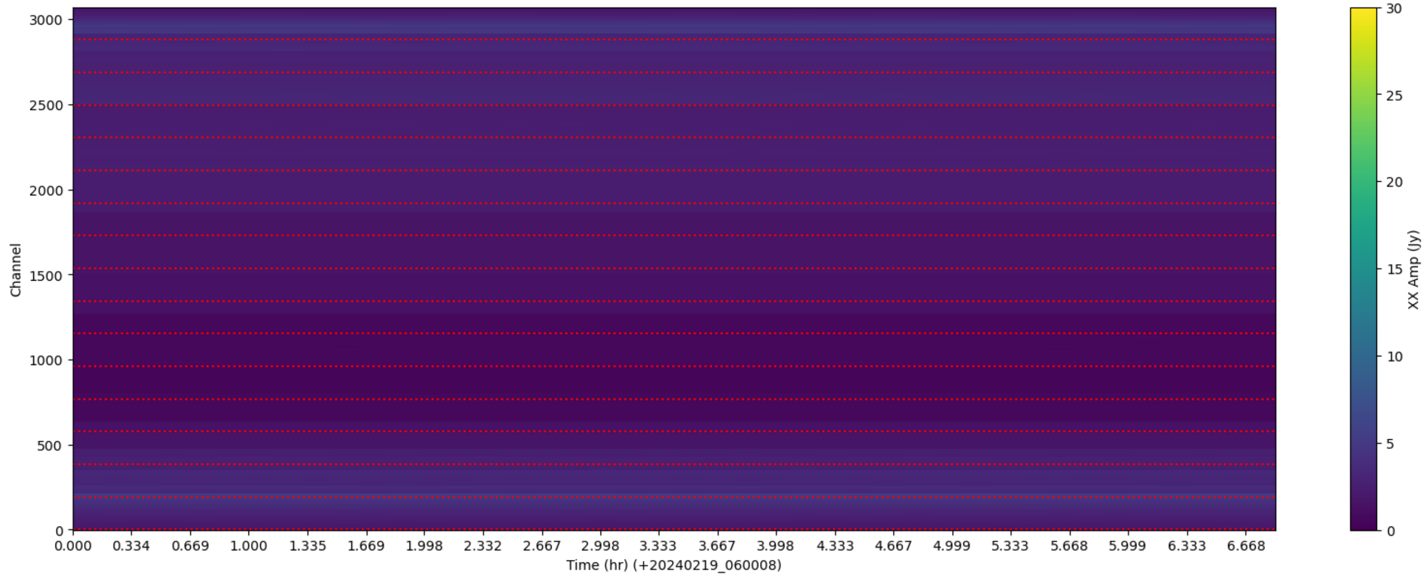
LWA266 - Correlator# 000 - XX - FLAGS: LowFlux
