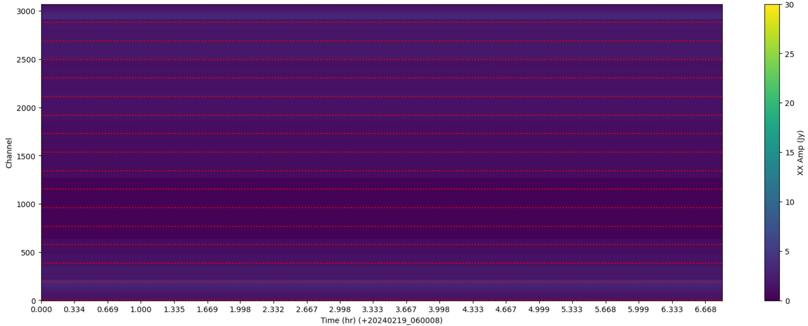
LWA365 - Correlator# 126 - XX - FLAGS: LowFlux
