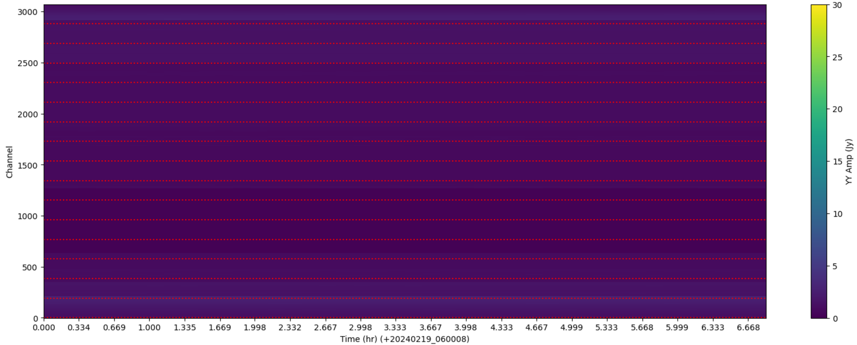
LWA260 - Correlator# 034 - YY - FLAGS: LowFlux
