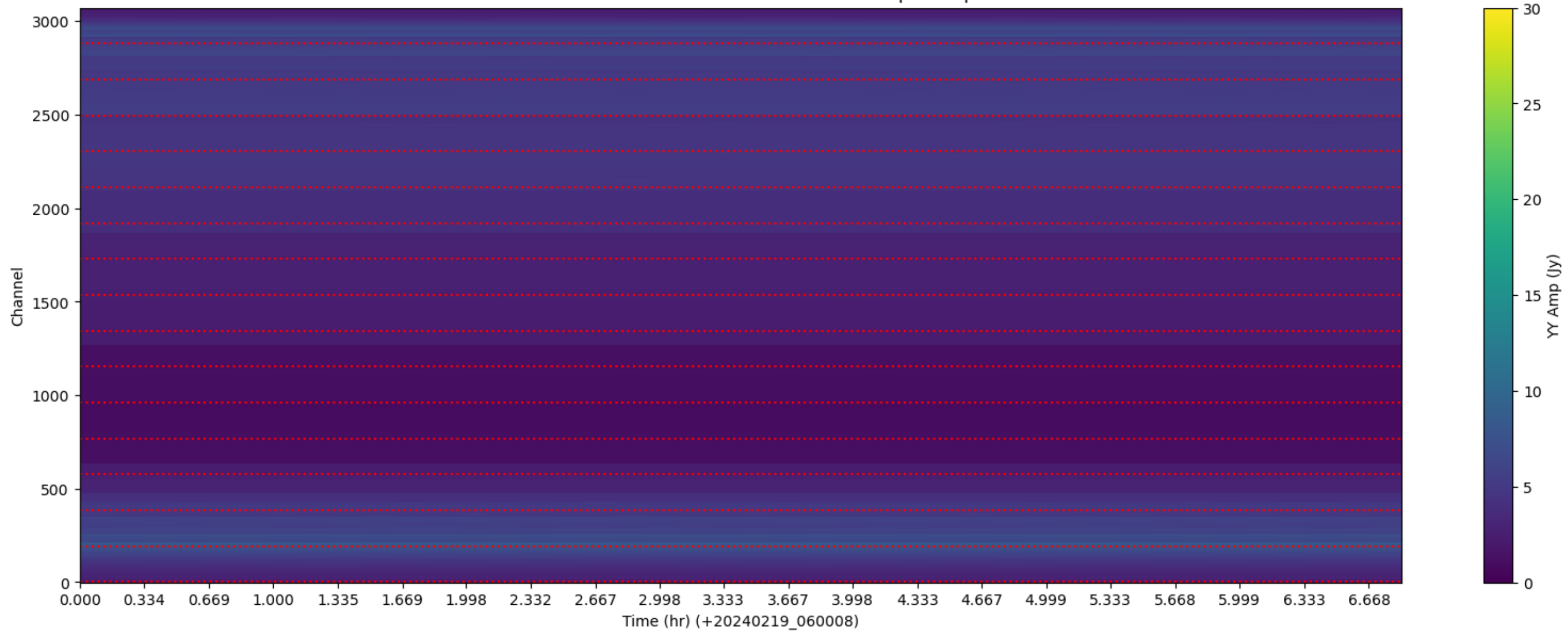
LWA321 - Correlator# 020 - YY - FLAGS: BadSpecShape
