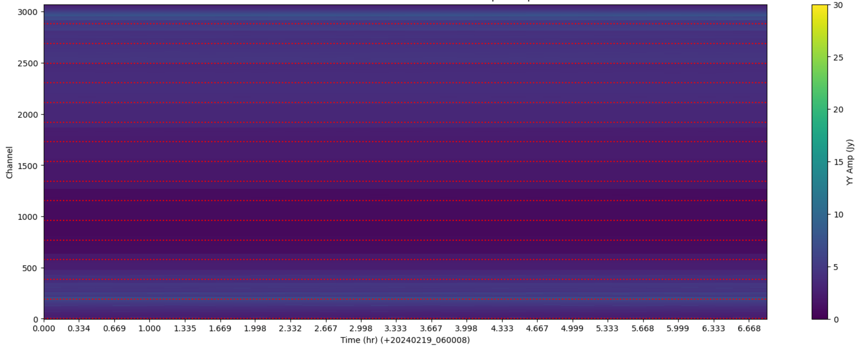
LWA276 - Correlator# 006 - YY - FLAGS: BadSpecShape
