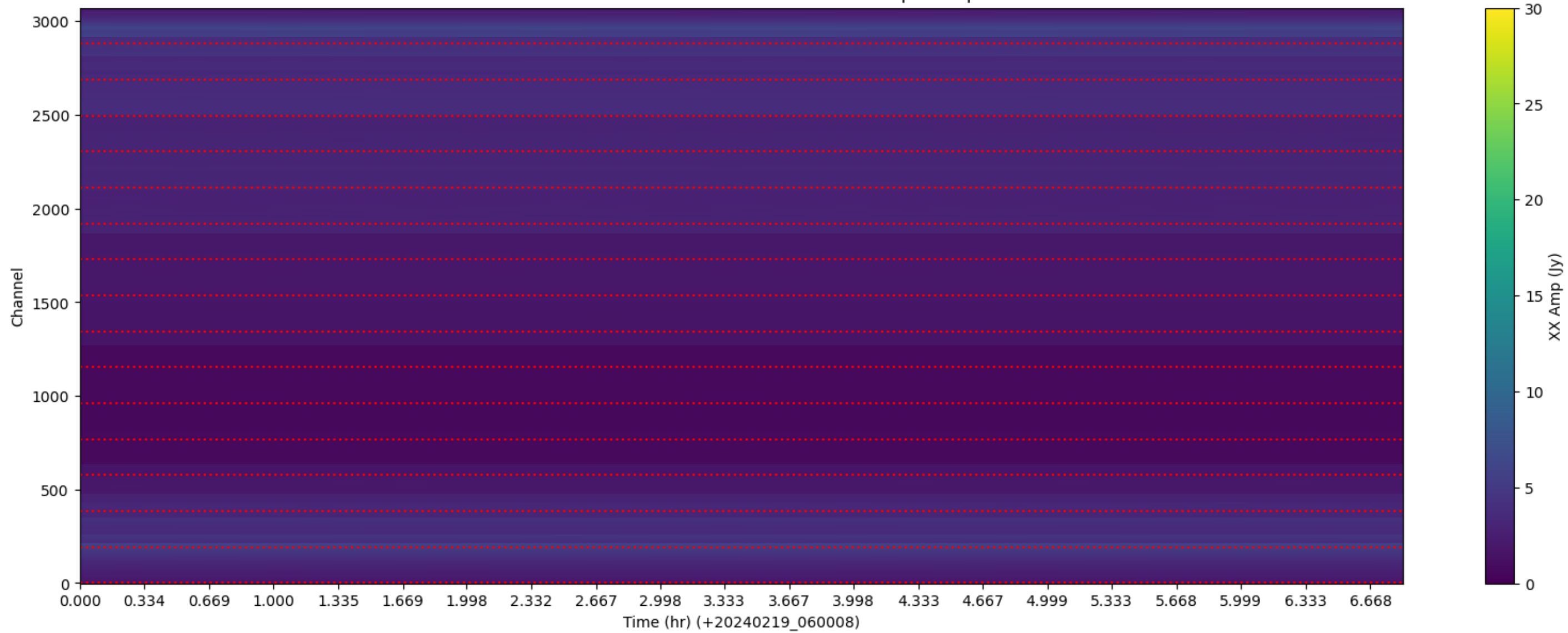
LWA270 - Correlator# 039 - XX - FLAGS: BadSpecShape
