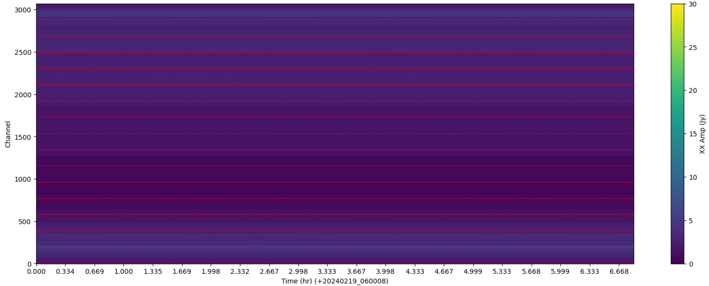
LWA334 - Correlator# 156 - XX - FLAGS: LowFlux
