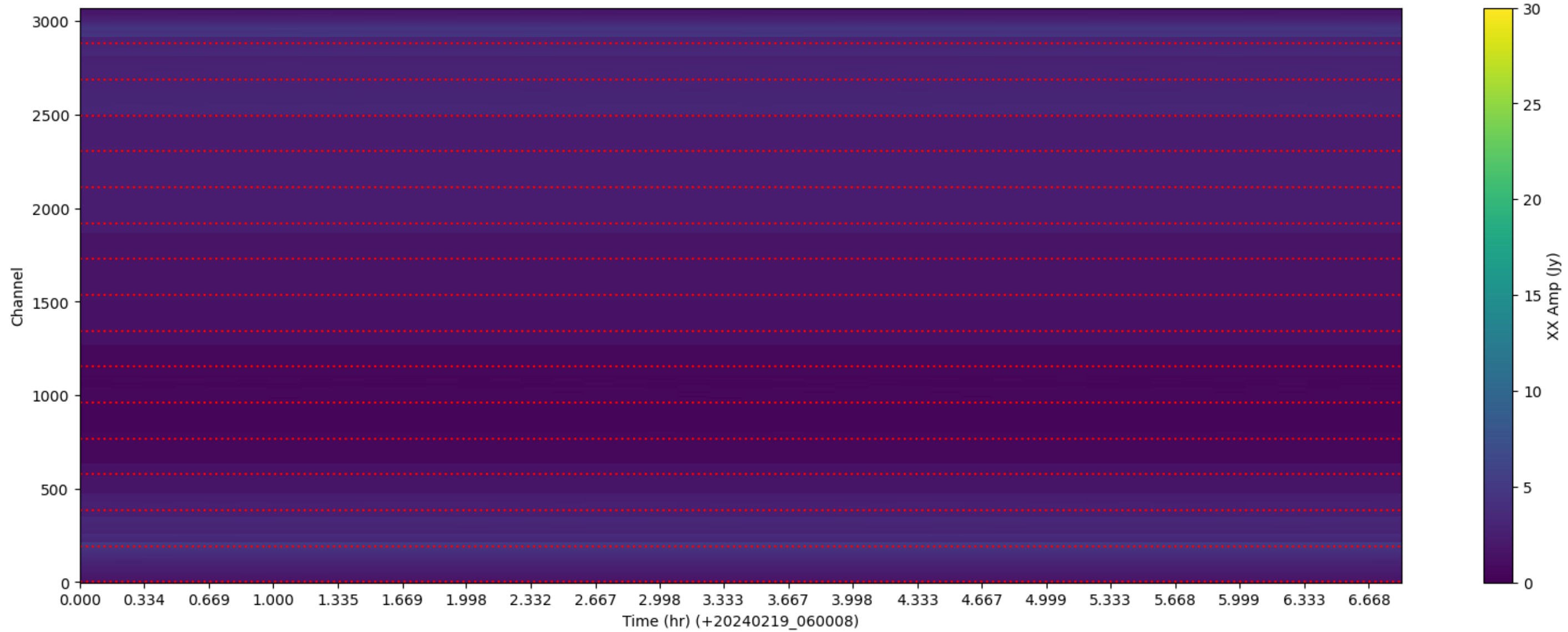
LWA351 - Correlator# 060 - XX - FLAGS: LowFlux
