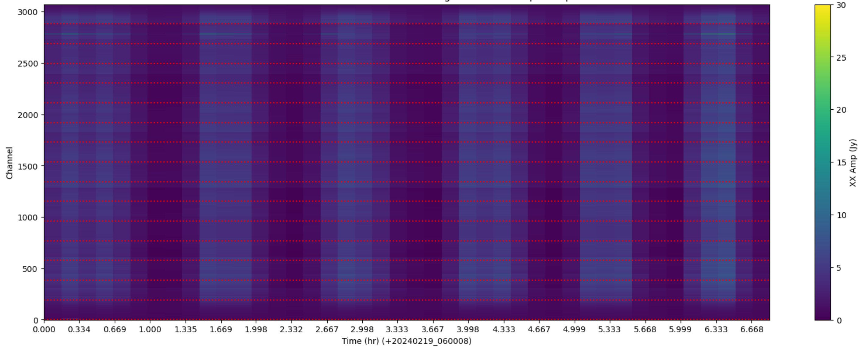
LWA124 - Correlator# 224 - XX - FLAGS: HighTimeVar+BadSpecShape
