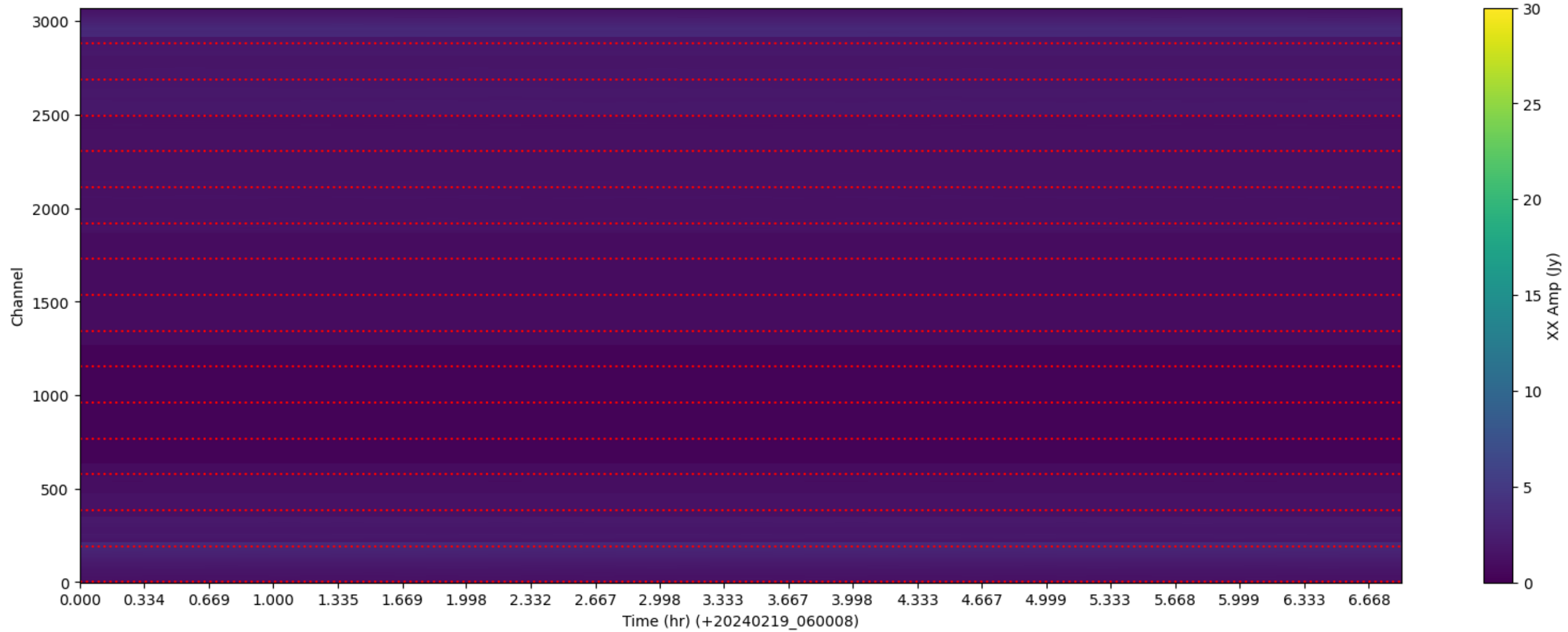
LWA257 - Correlator# 032 - XX - FLAGS: LowFlux
