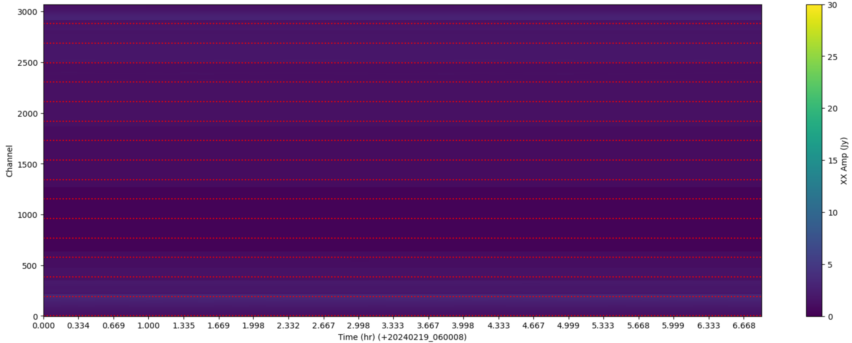
LWA307 - Correlator# 012 - XX - FLAGS: LowFlux
