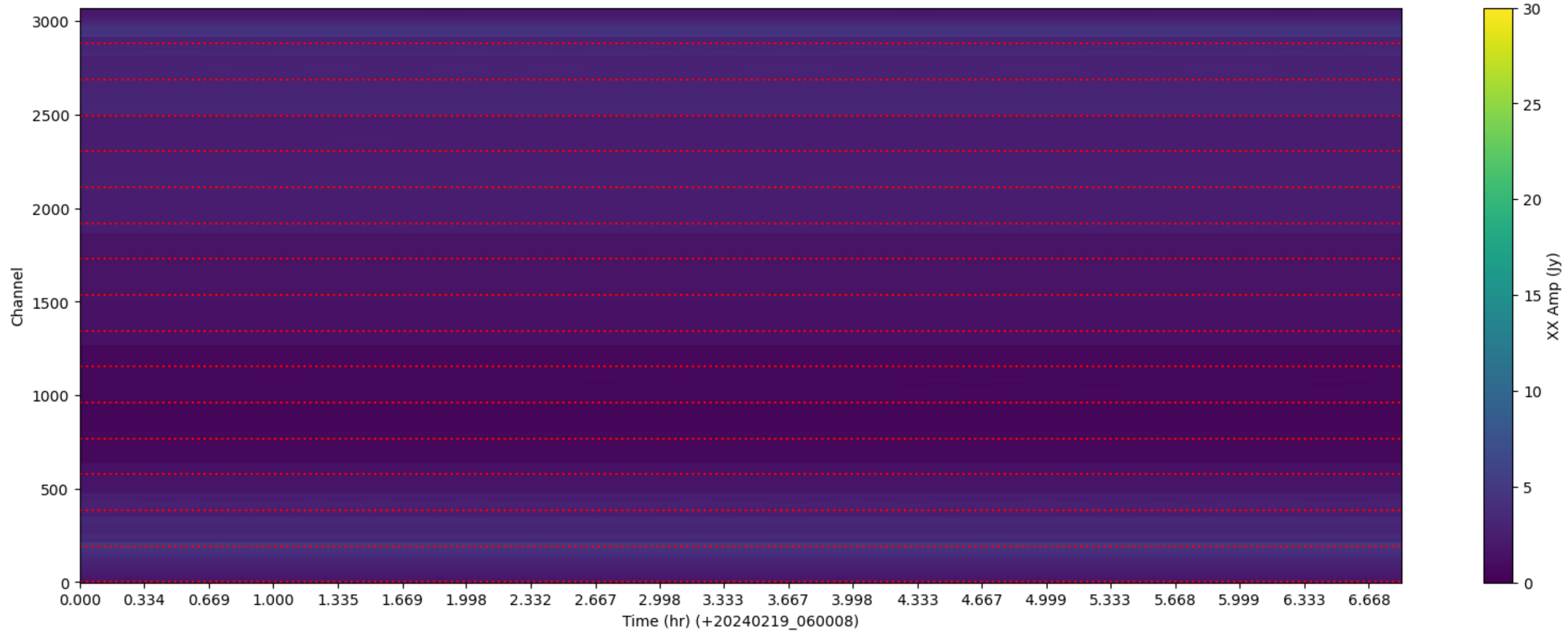
LWA340 - Correlator# 026 - XX - FLAGS: LowFlux
