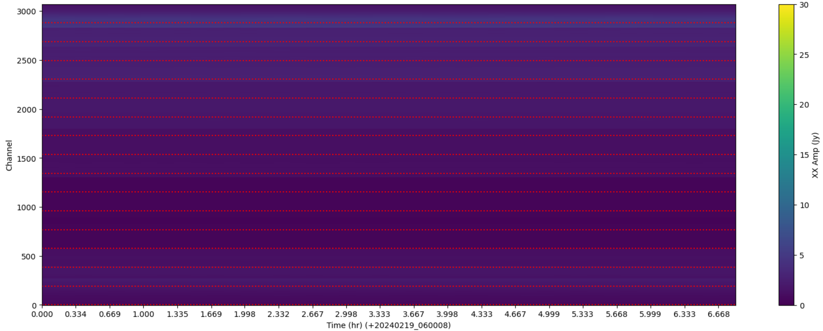
LWA076 - Correlator# 193 - XX - FLAGS: LowFlux
