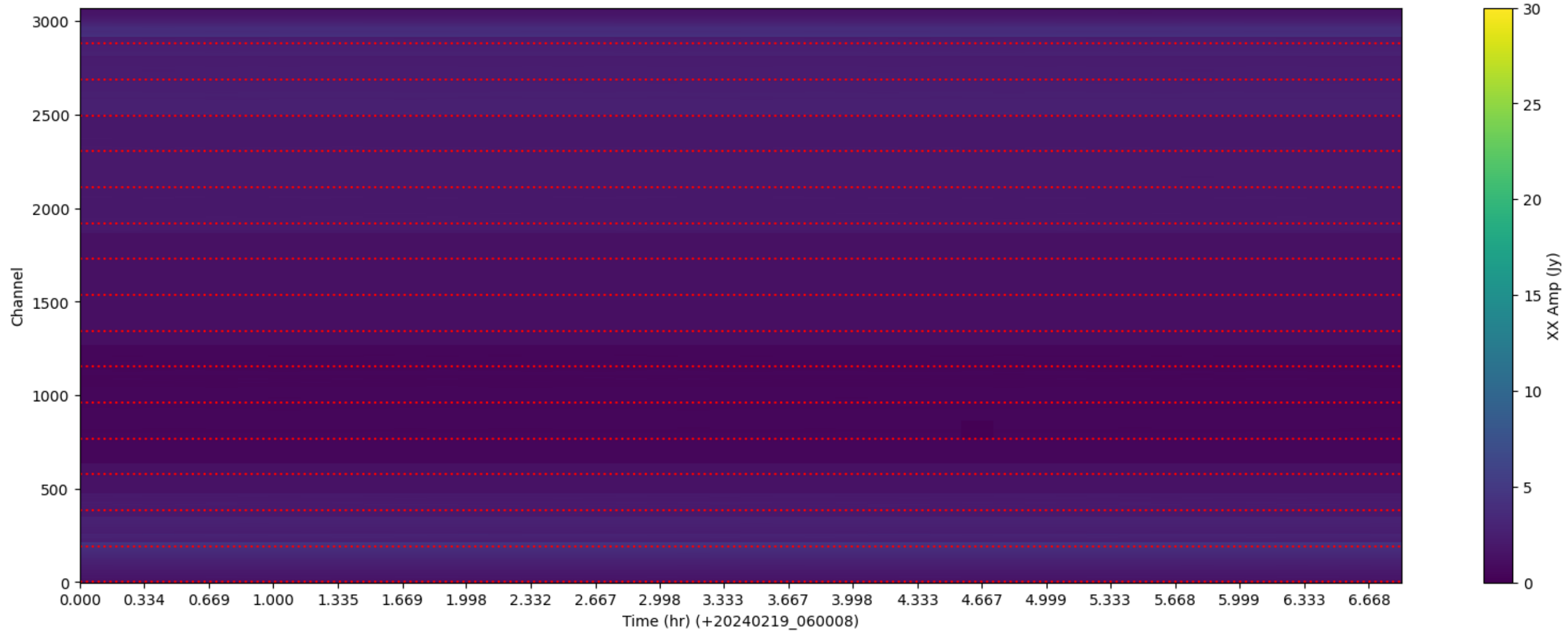
LWA319 - Correlator# 190 - XX - FLAGS: LowFlux
