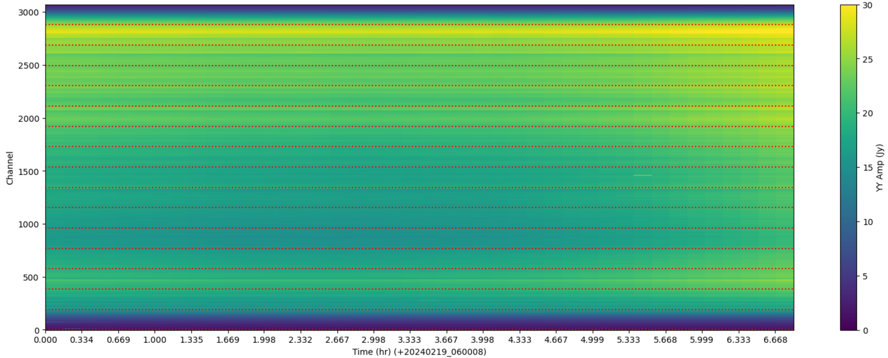
LWA066 - Correlator# 164 - YY - FLAGS: Good
