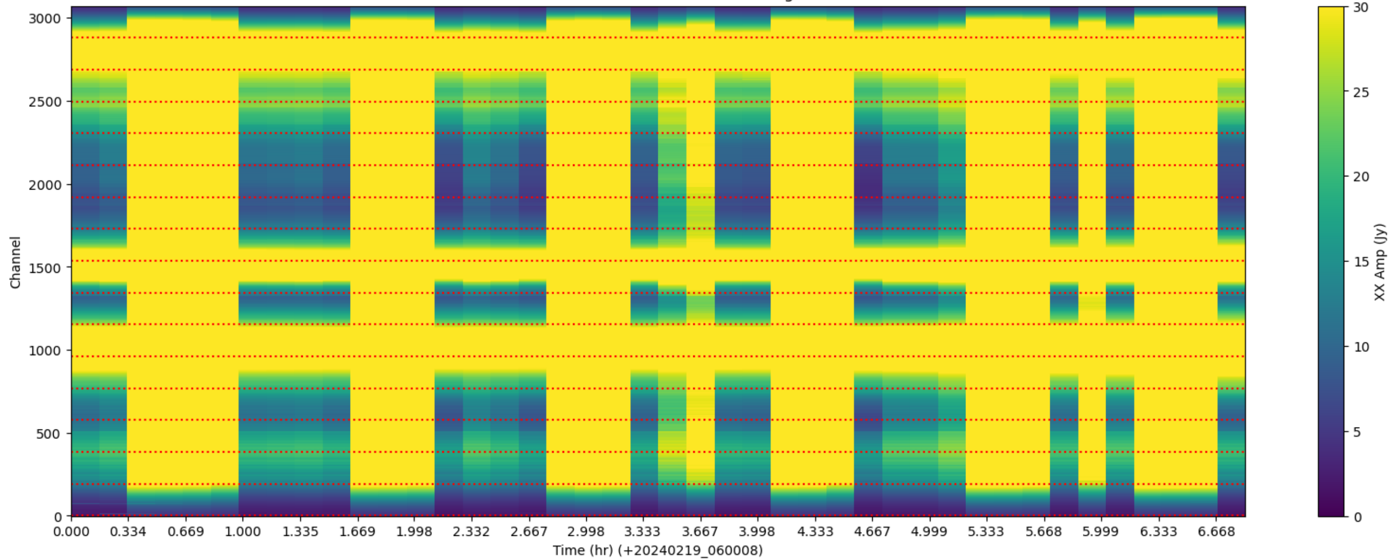
LWA041 - Correlator# 079 - XX - FLAGS: HighTimeVar
