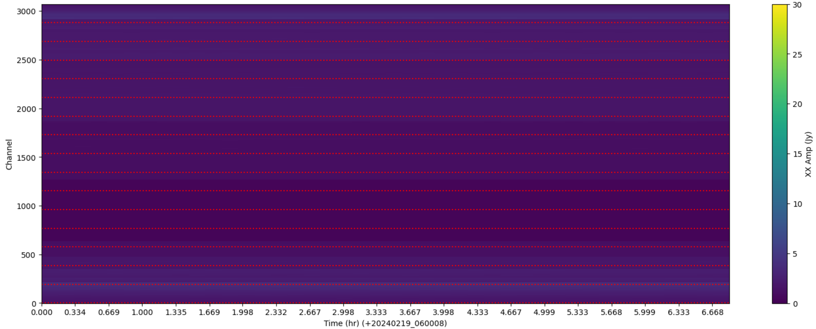
LWA325 - Correlator# 154 - XX - FLAGS: LowFlux
