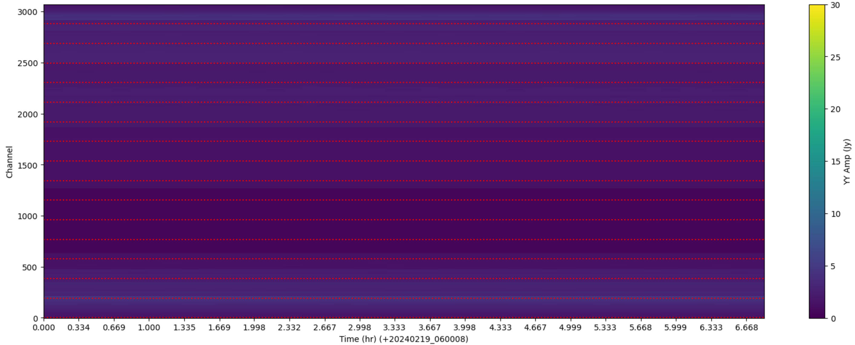
LWA330 - Correlator# 022 - YY - FLAGS: LowFlux
