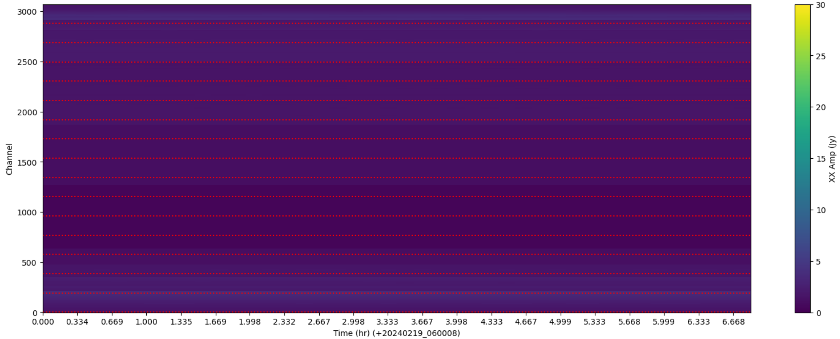
LWA311 - Correlator# 016 - XX - FLAGS: LowFlux
