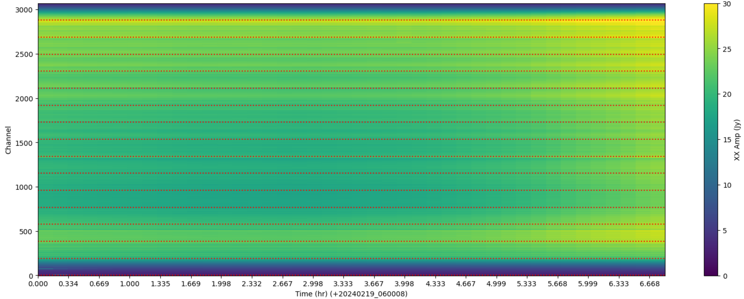
LWA131 - Correlator# 182 - XX - FLAGS: Good
