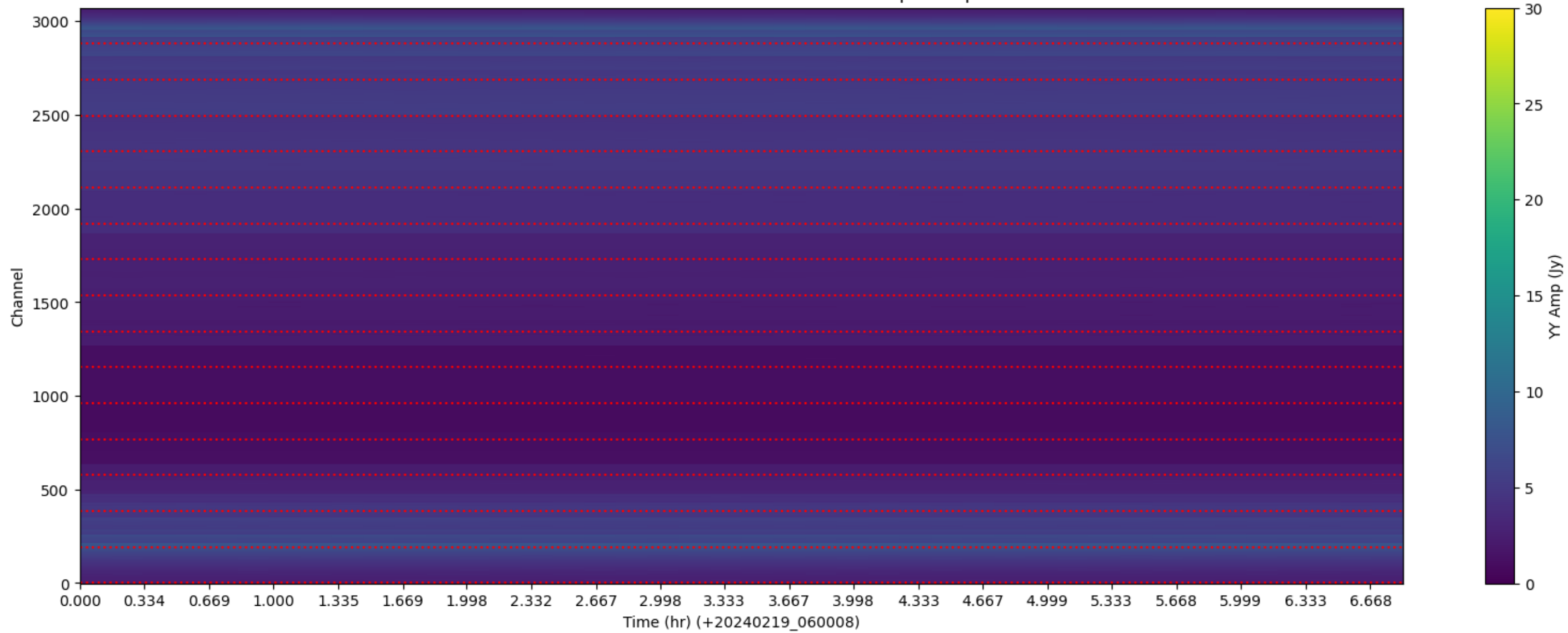
LWA332 - Correlator# 025 - YY - FLAGS: BadSpecShape
