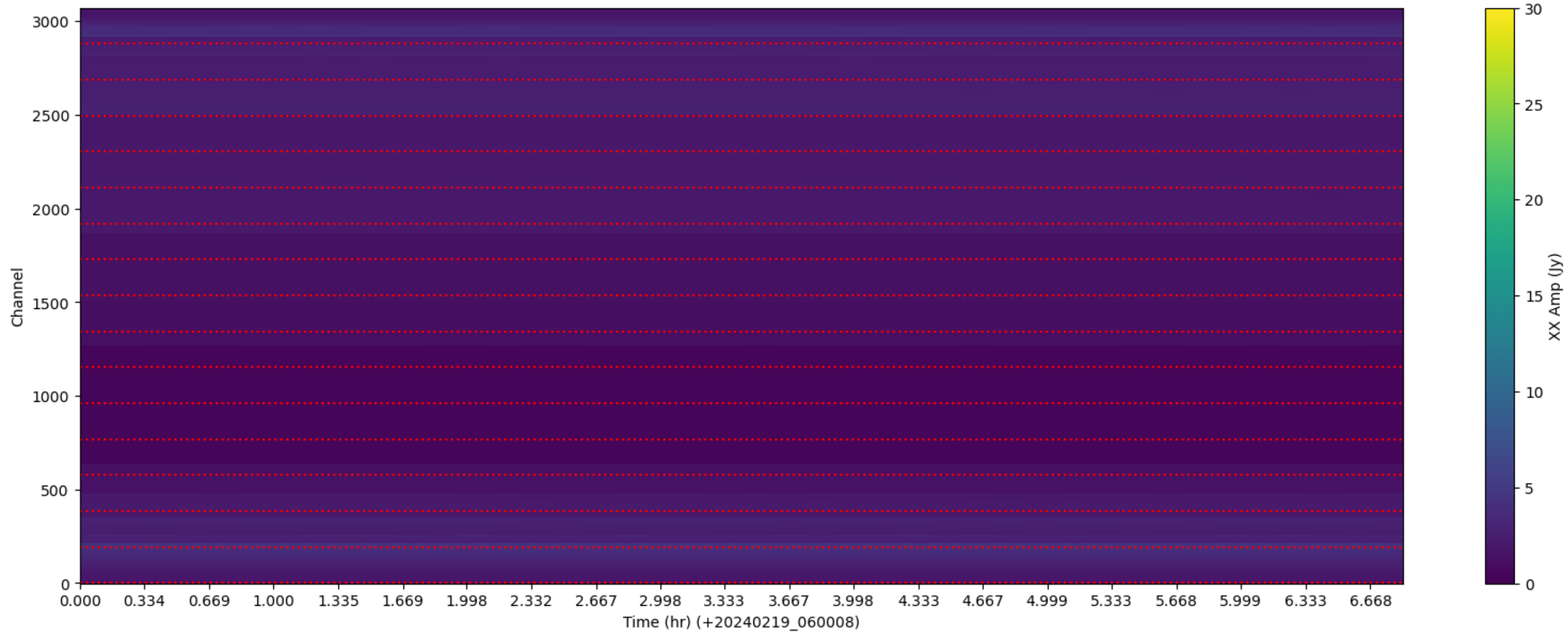
LWA354 - Correlator# 063 - XX - FLAGS: LowFlux
