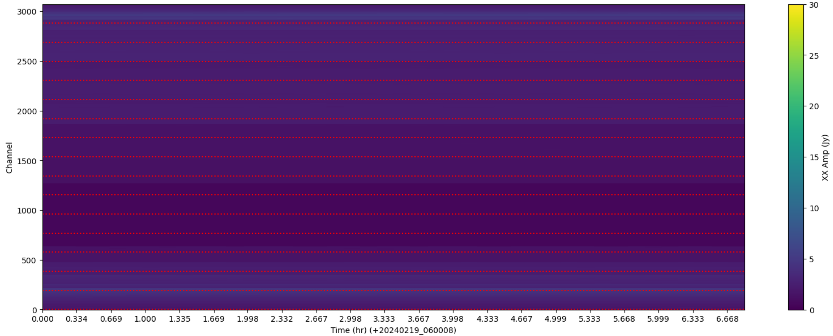
LWA298 - Correlator# 049 - XX - FLAGS: LowFlux
