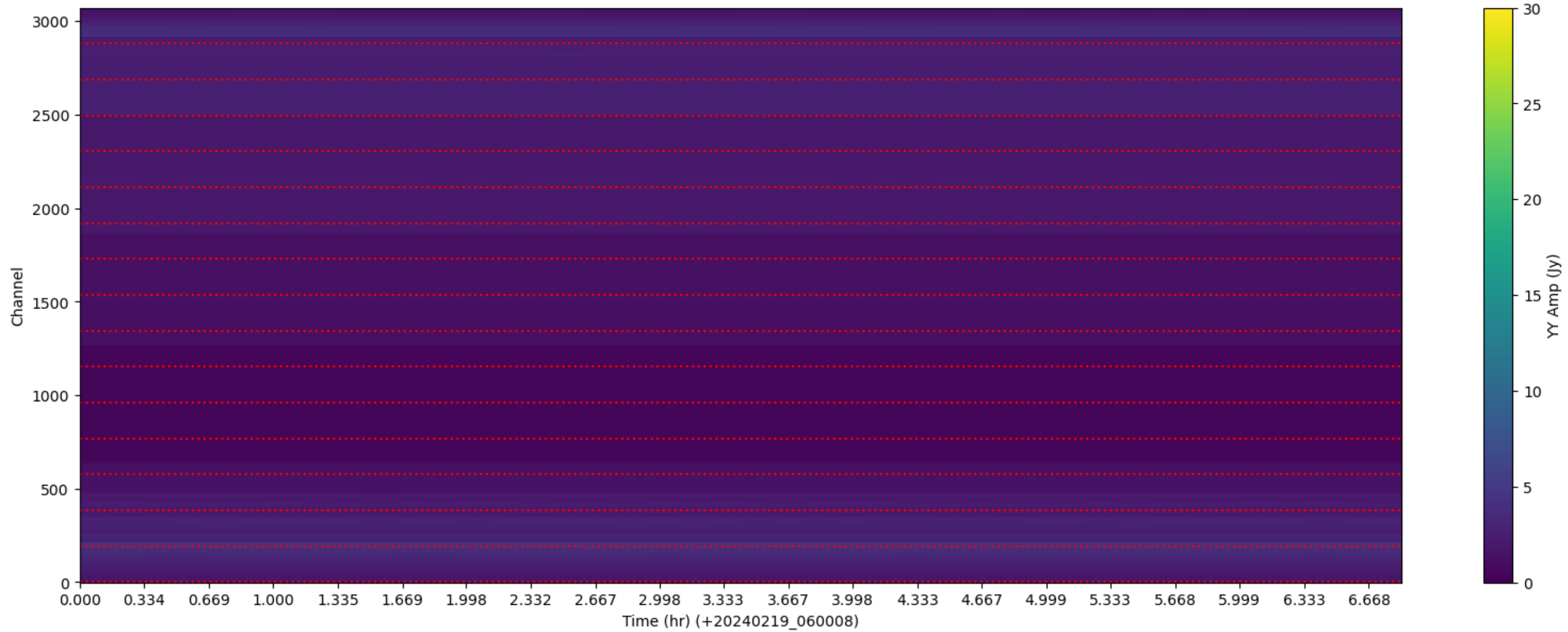
LWA353 - Correlator# 031 - YY - FLAGS: LowFlux
