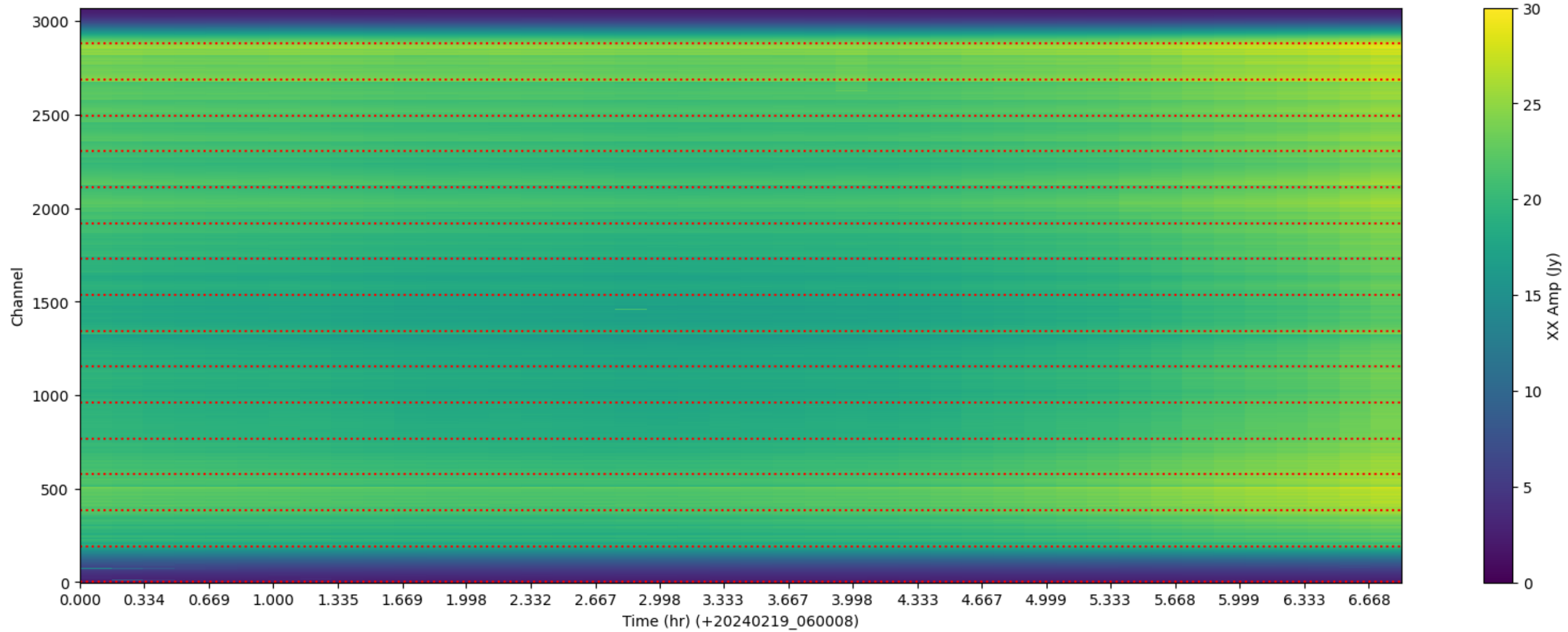
LWA004 - Correlator# 066 - XX - FLAGS: Good
