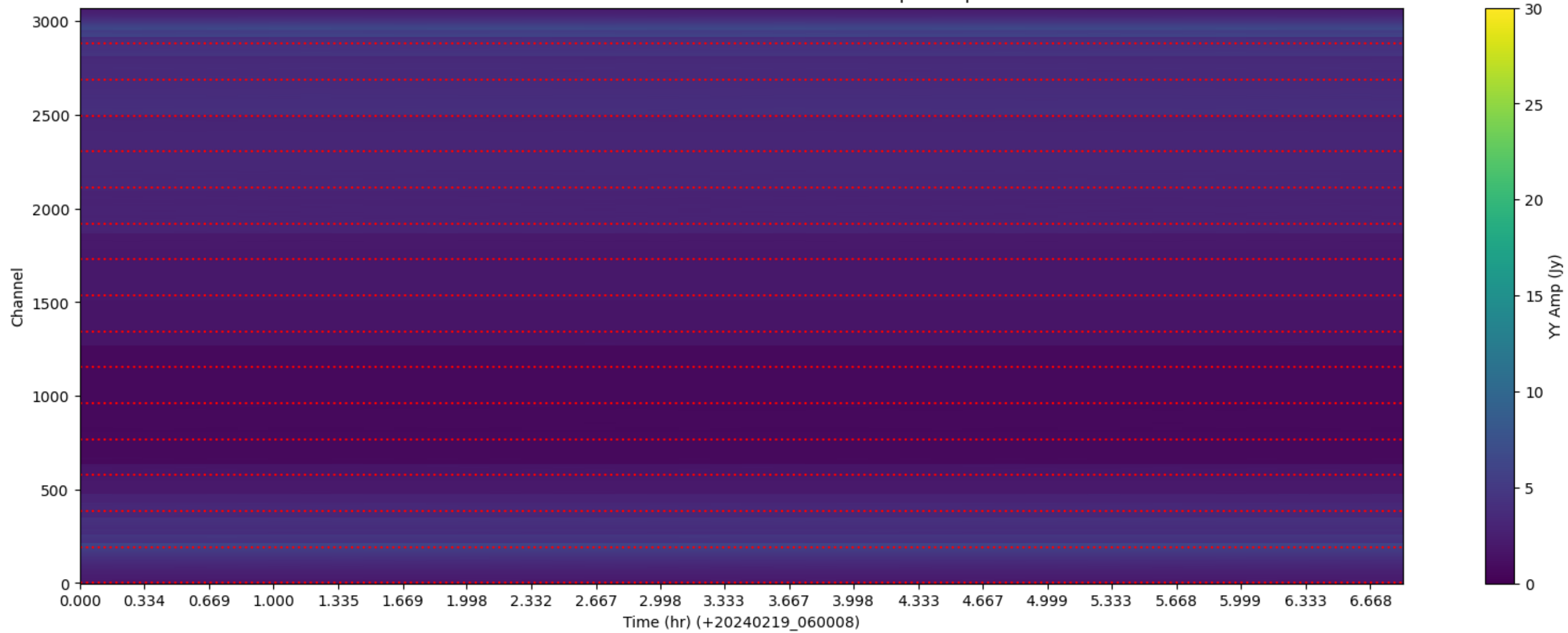
LWA298 - Correlator# 049 - YY - FLAGS: BadSpecShape
