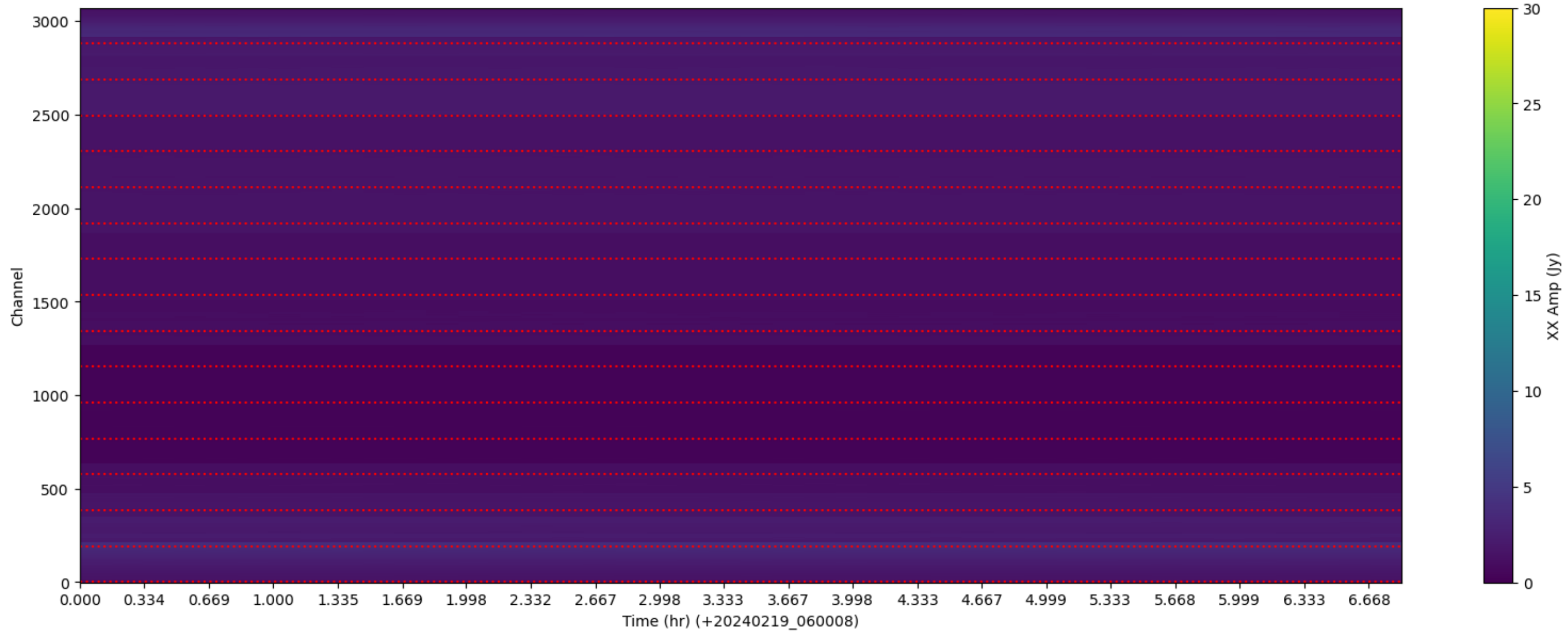
LWA278 - Correlator# 008 - XX - FLAGS: LowFlux
