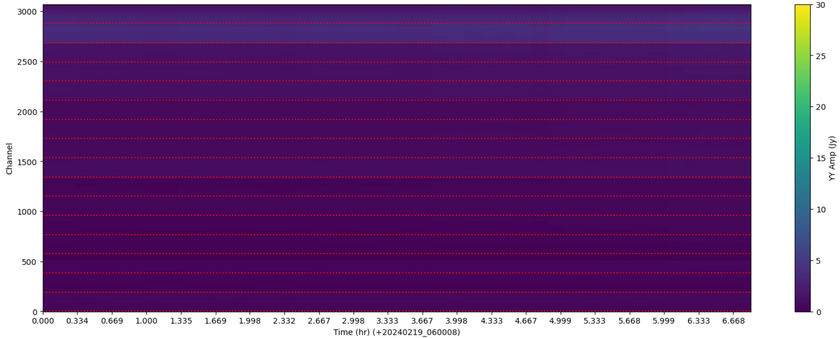
LWA009 - Correlator# 070 - YY - FLAGS: LowFlux
