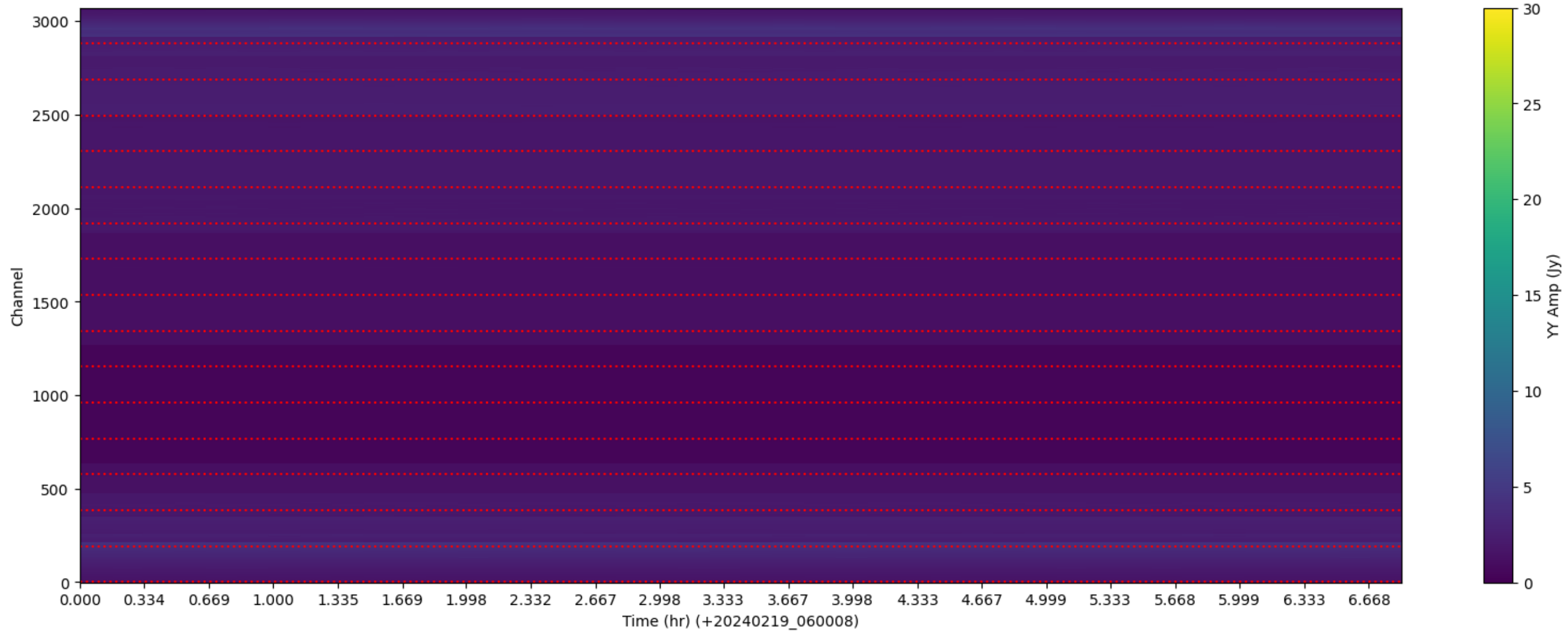
LWA310 - Correlator# 017 - YY - FLAGS: LowFlux
