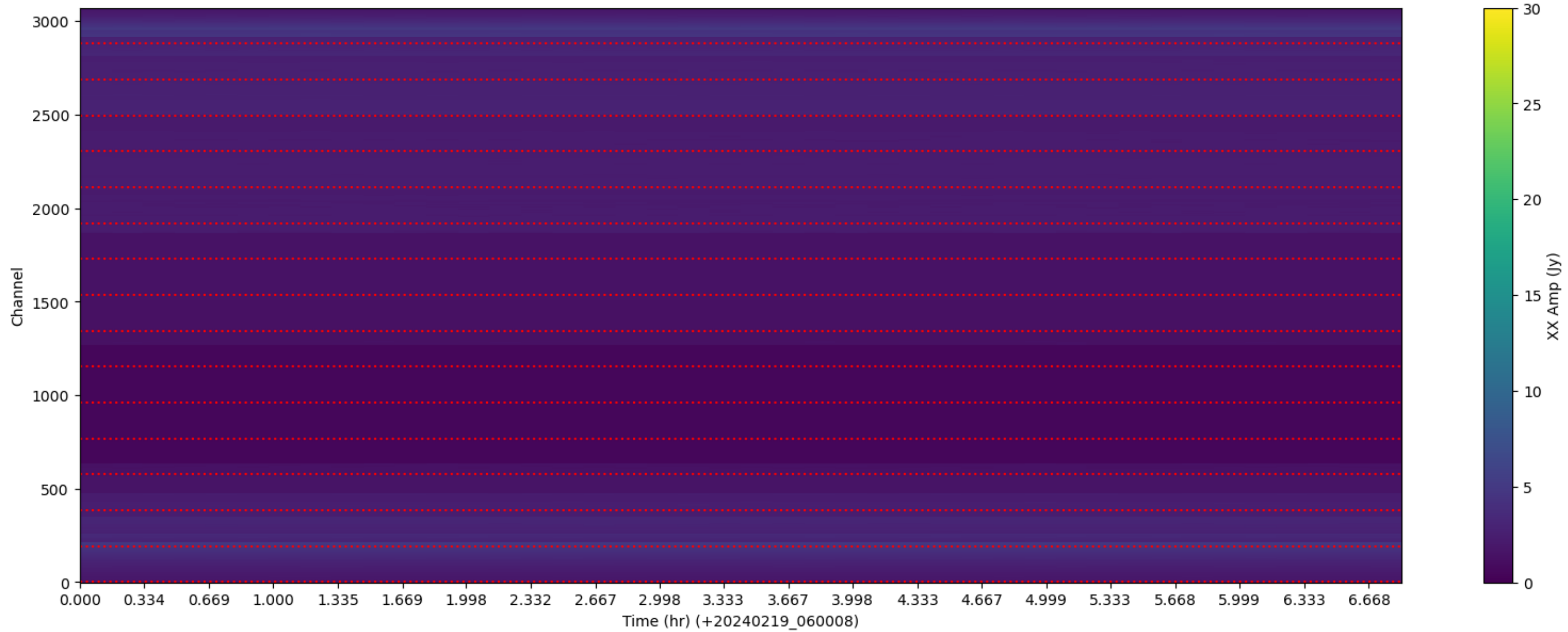
LWA290 - Correlator# 285 - XX - FLAGS: LowFlux
