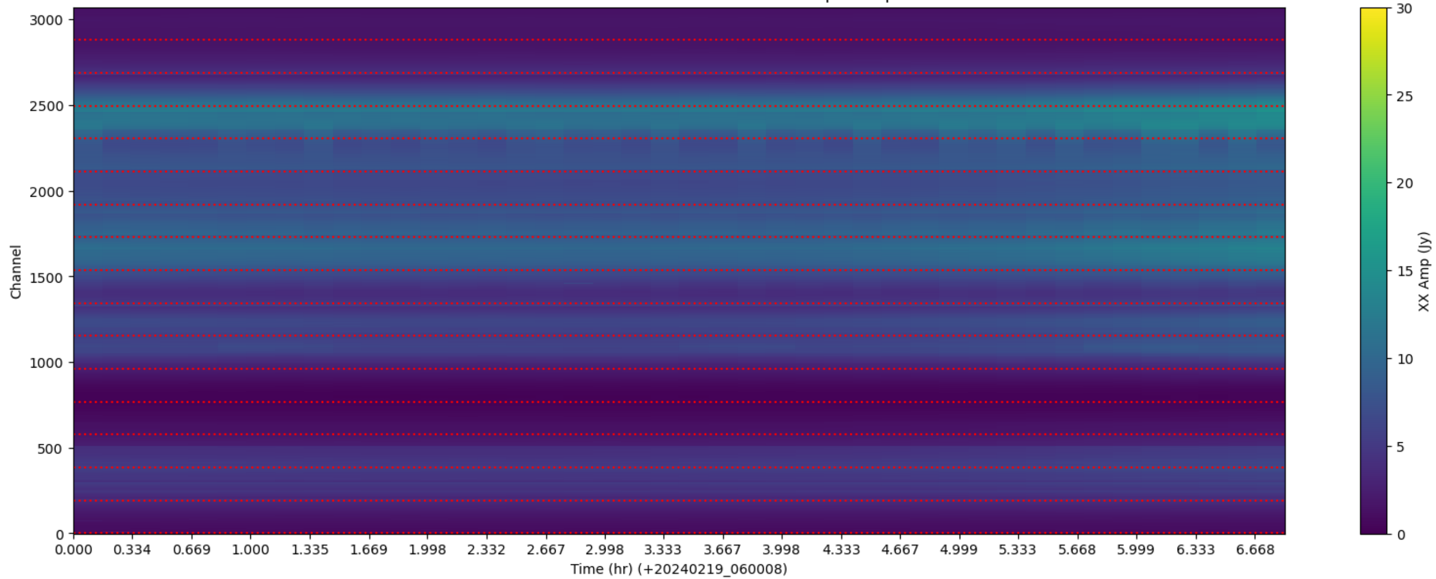
LWA232 - Correlator# 307 - XX - FLAGS: BadSpecShape
