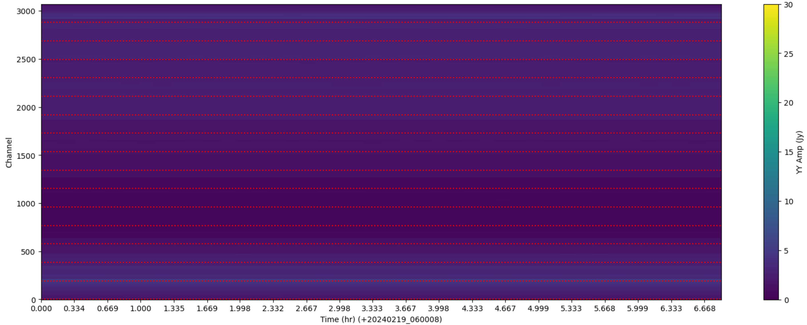
LWA350 - Correlator# 319 - YY - FLAGS: LowFlux
