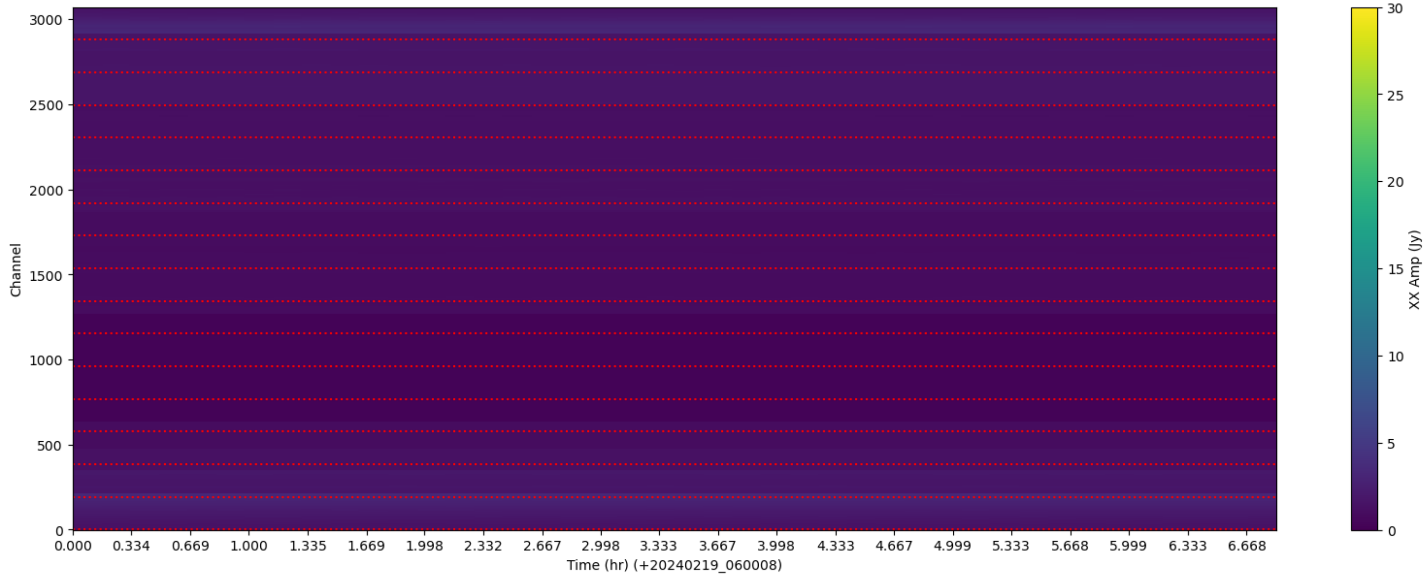
LWA261 - Correlator# 346 - XX - FLAGS: LowFlux
