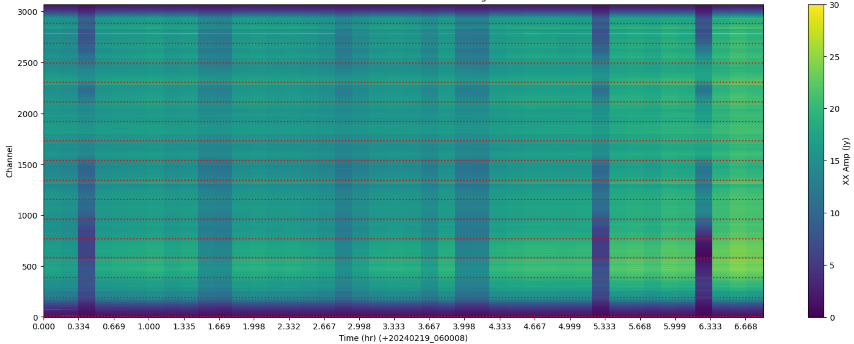
LWA151 - Correlator# 218 - XX - FLAGS: HighTimeVar
