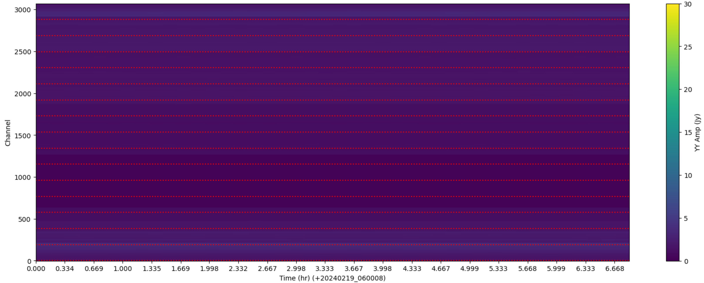
LWA365 - Correlator# 126 - YY - FLAGS: LowFlux
