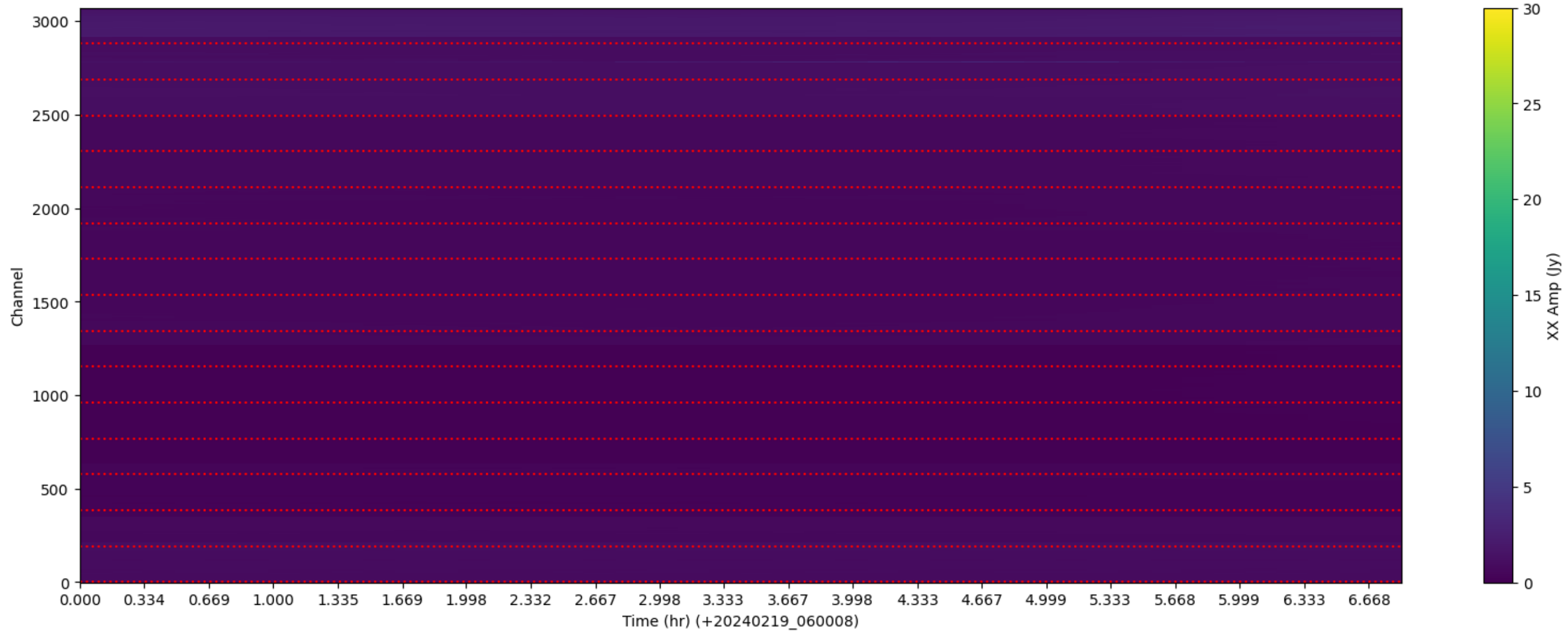
LWA191 - Correlator# 246 - XX - FLAGS: LowFlux
