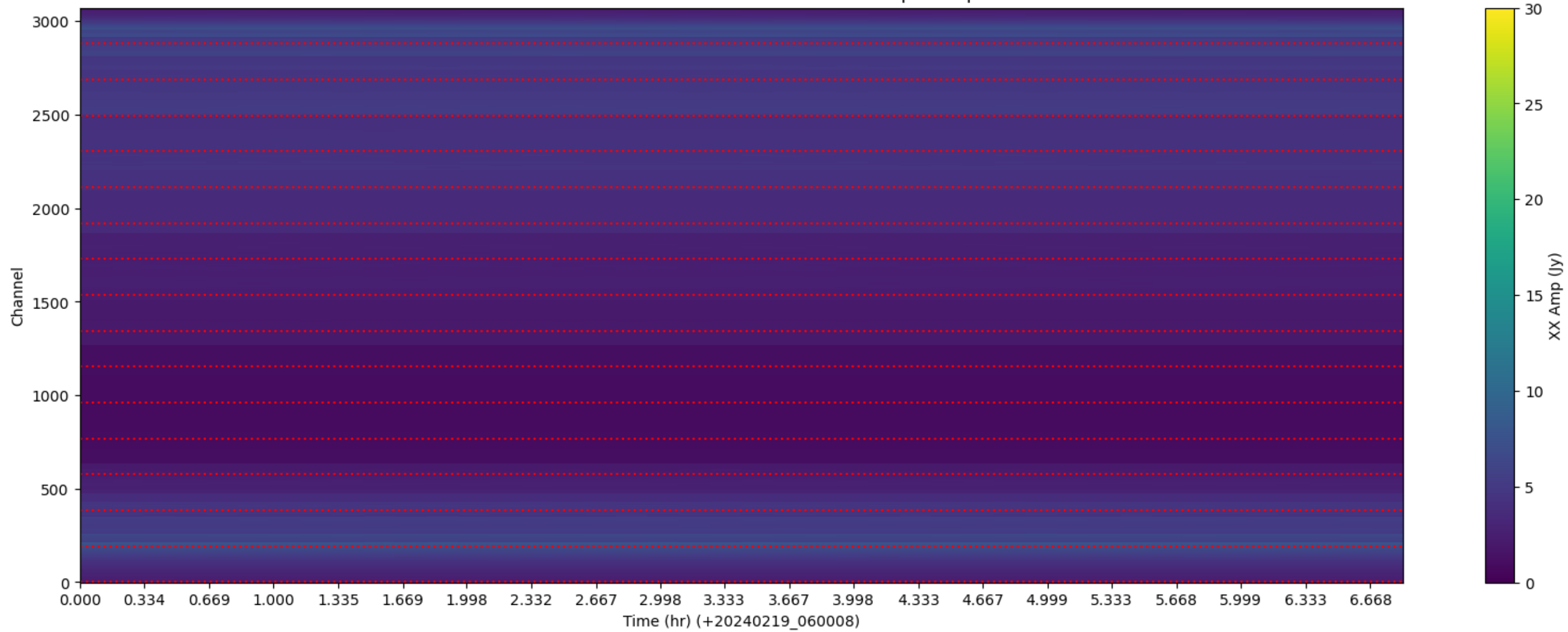
LWA330 - Correlator# 022 - XX - FLAGS: BadSpecShape
