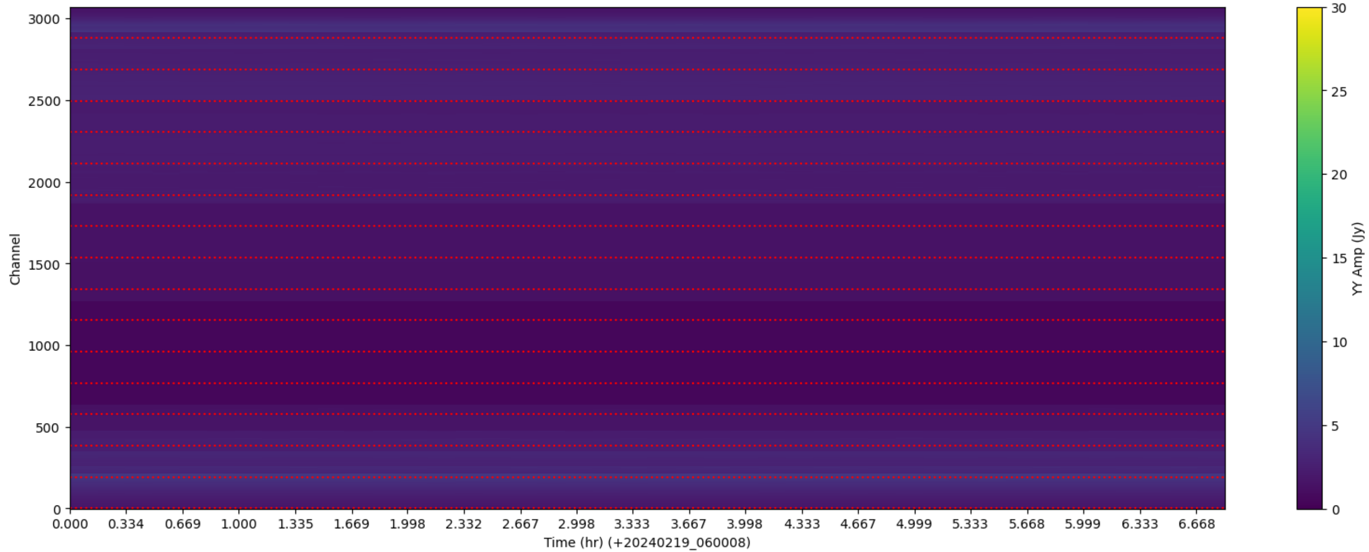
LWA334 - Correlator# 156 - YY - FLAGS: LowFlux
