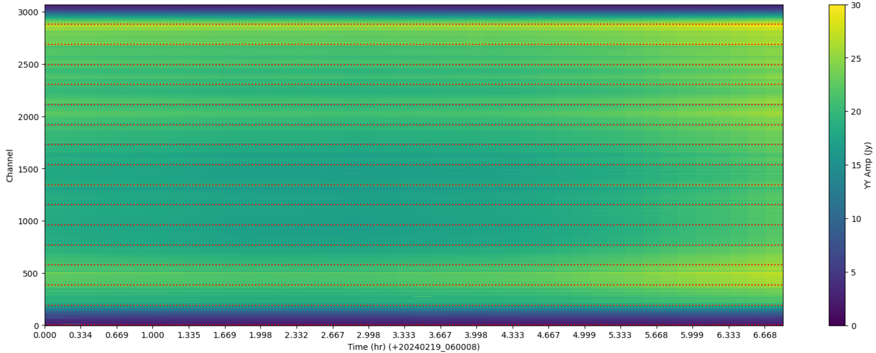
LWA004 - Correlator# 066 - YY - FLAGS: Good
