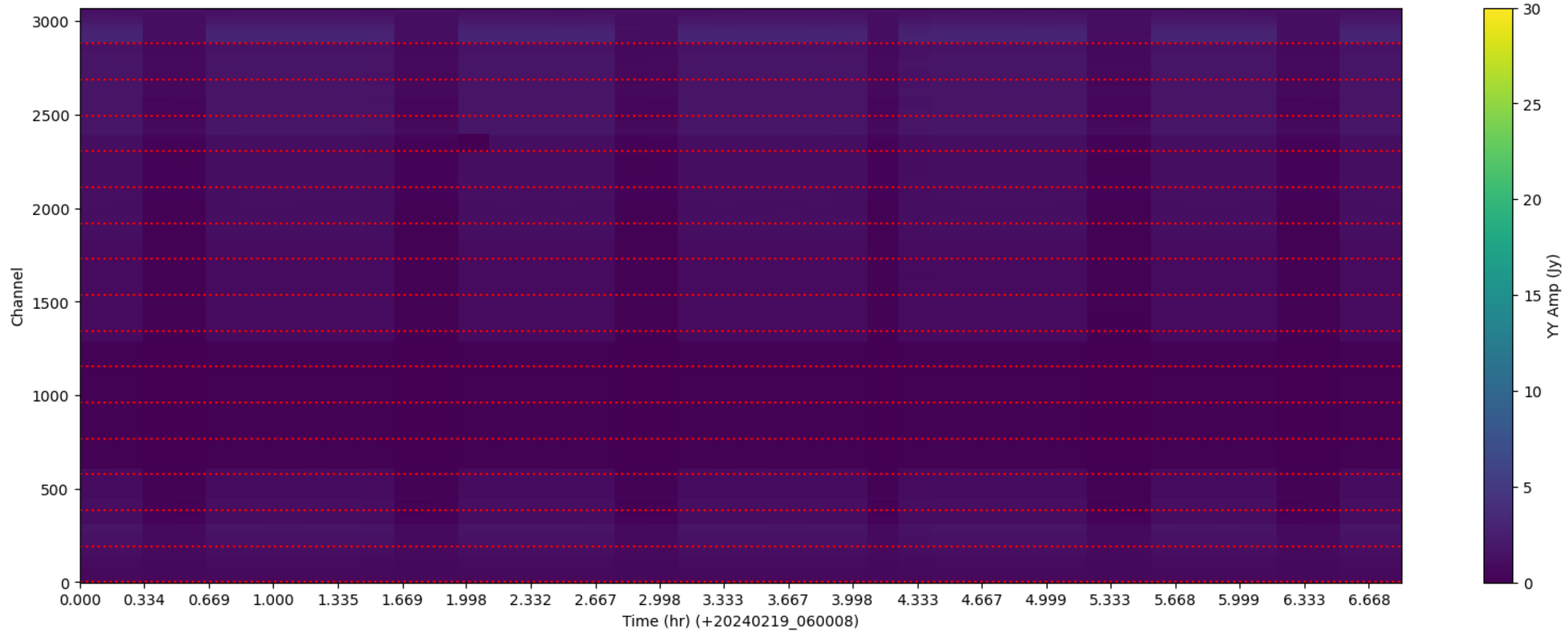
LWA058 - Correlator# 137 - YY - FLAGS: LowFlux
