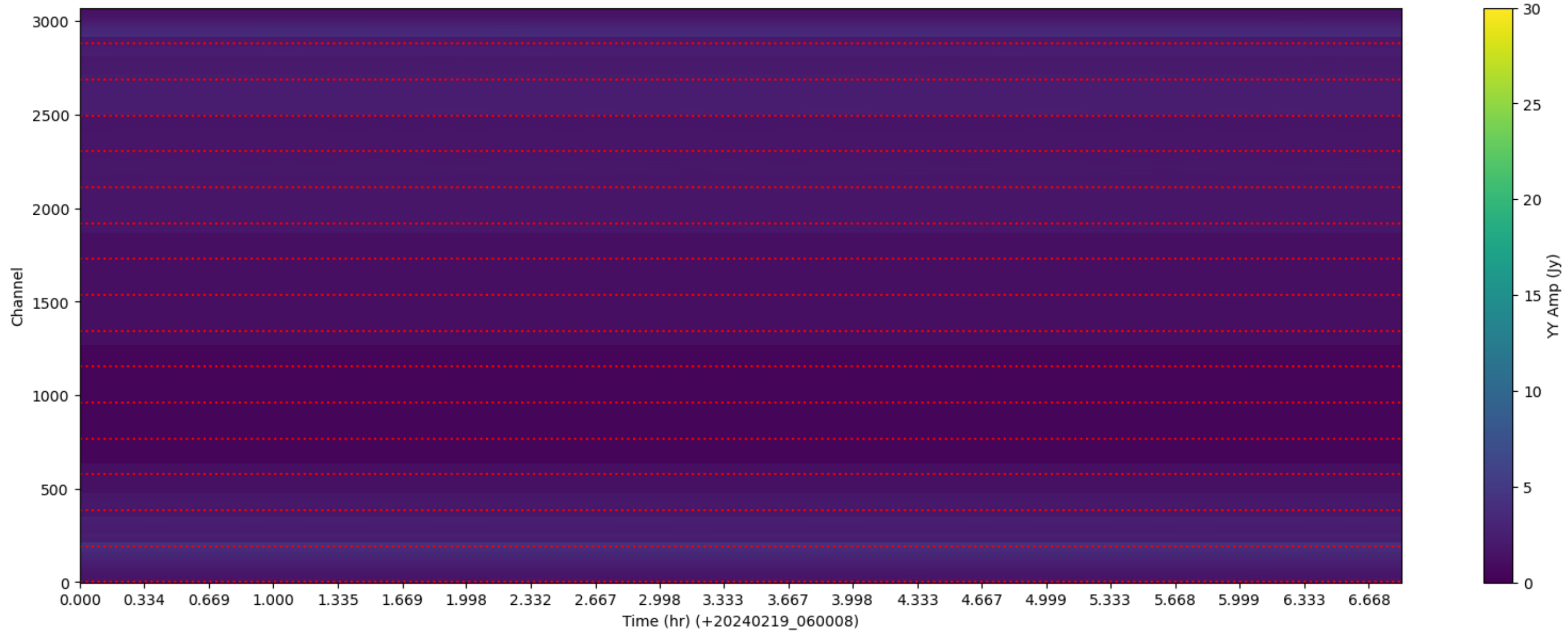
LWA351 - Correlator# 060 - YY - FLAGS: LowFlux
