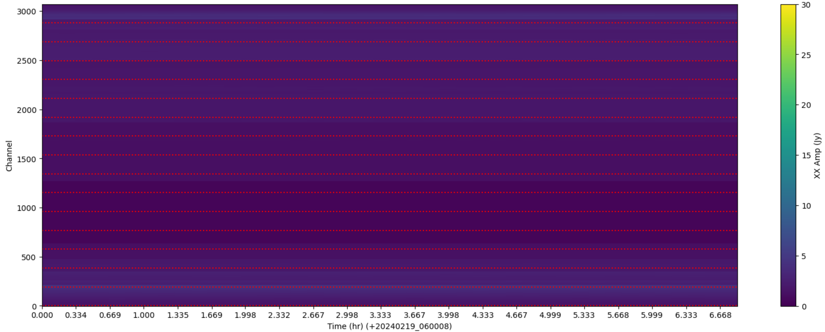
LWA268 - Correlator# 002 - XX - FLAGS: LowFlux
