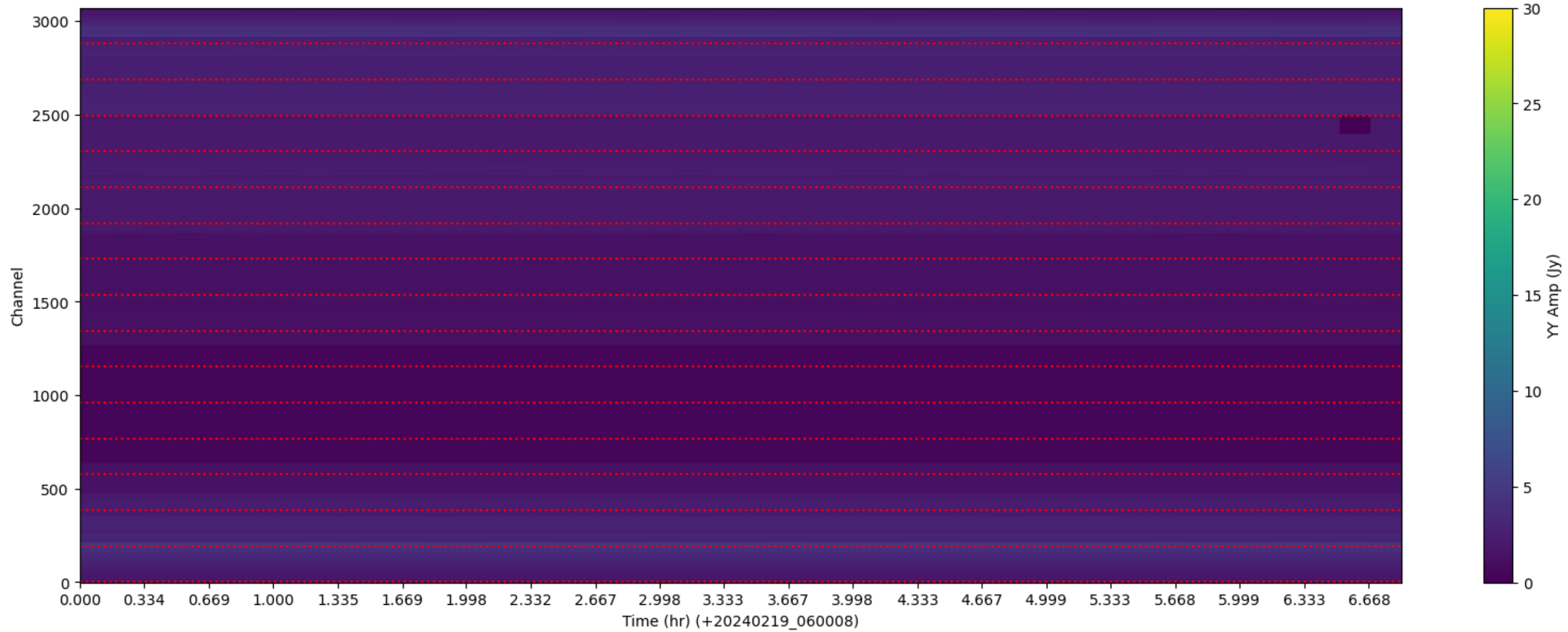
LWA331 - Correlator# 125 - YY - FLAGS: LowFlux
