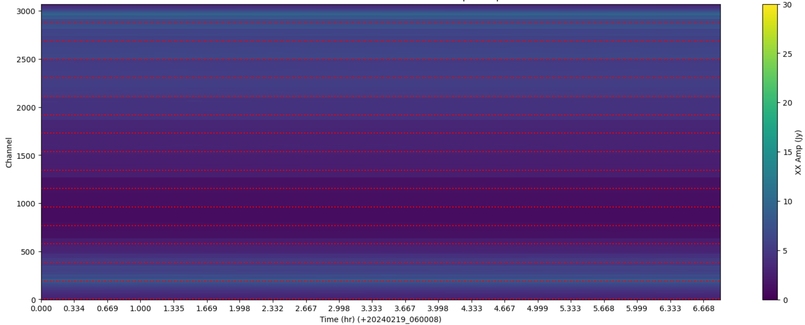
LWA316 - Correlator# 155 - XX - FLAGS: BadSpecShape
