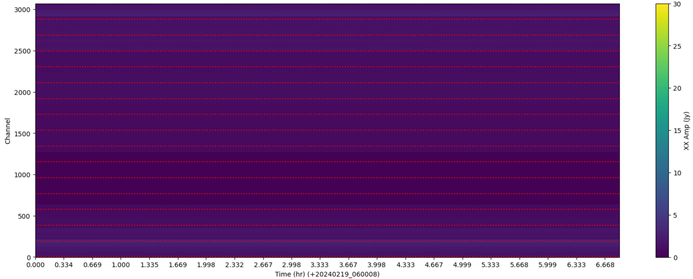
LWA322 - Correlator# 251 - XX - FLAGS: LowFlux
