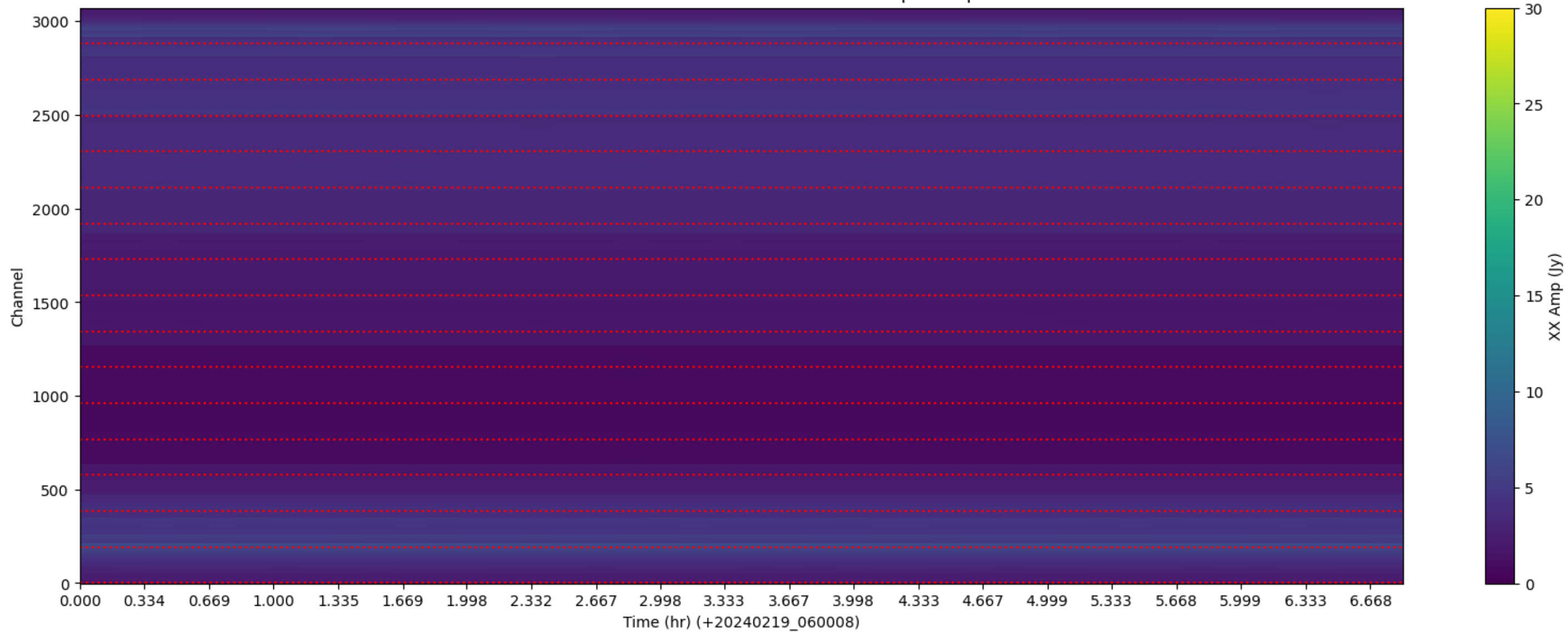
LWA275 - Correlator# 090 - XX - FLAGS: BadSpecShape
