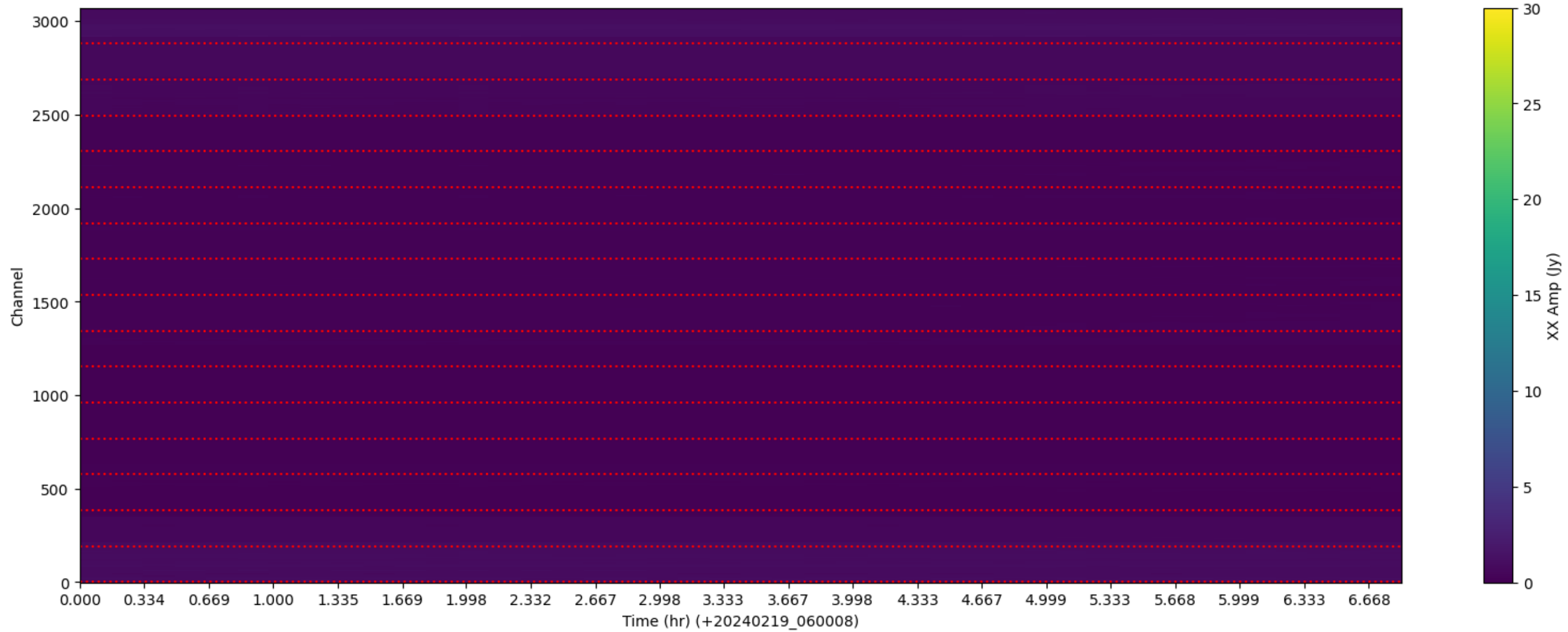
LWA255 - Correlator# 033 - XX - FLAGS: LowFlux
