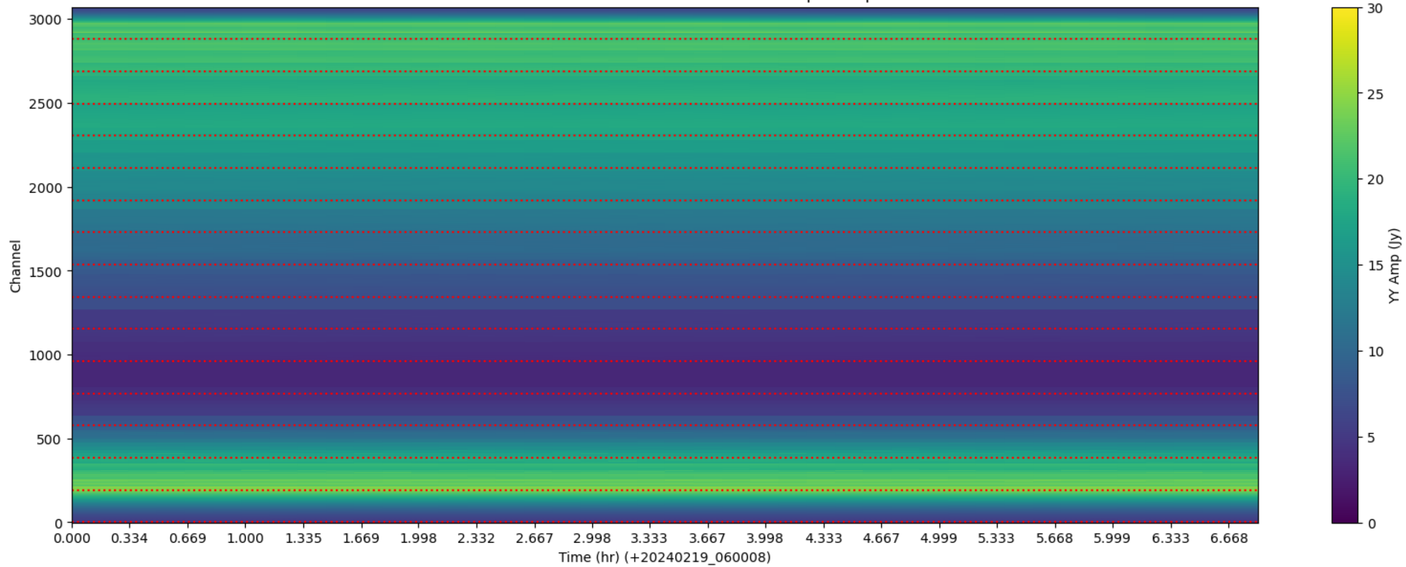
LWA354 - Correlator# 063 - YY - FLAGS: BadSpecShape
