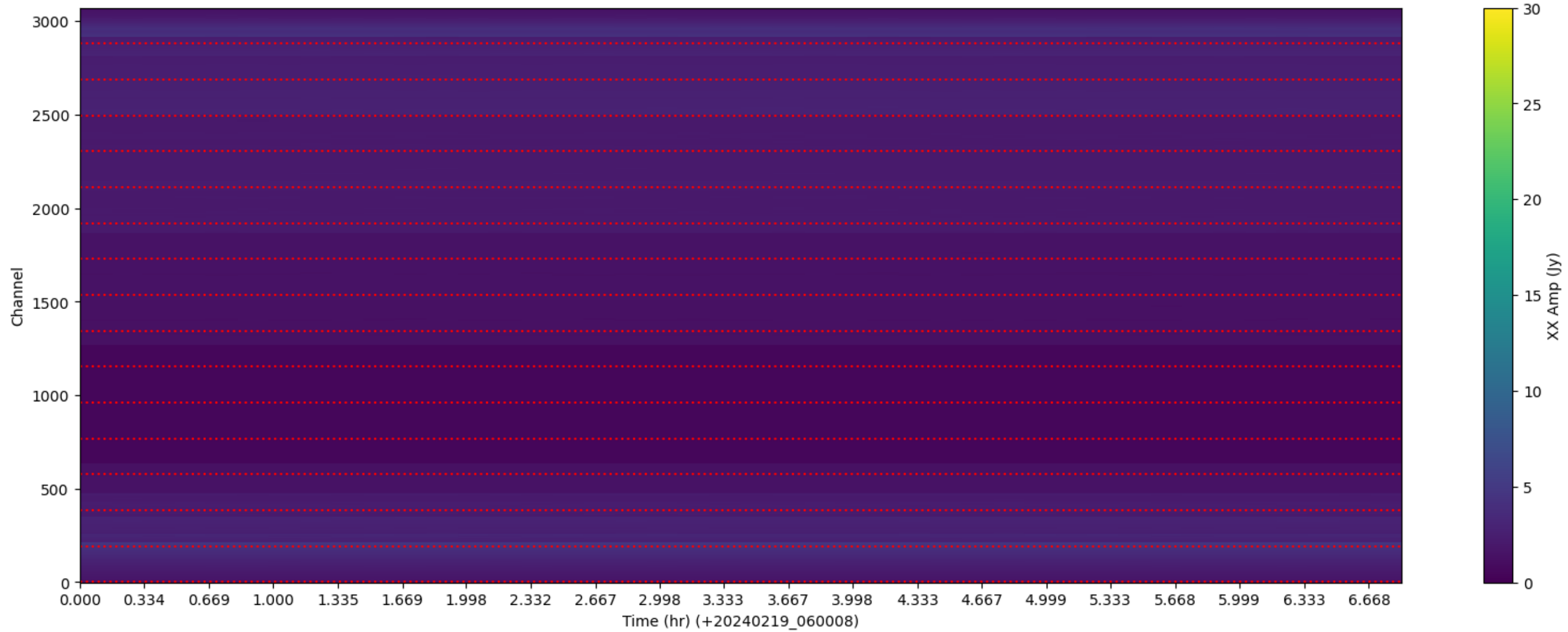
LWA337 - Correlator# 059 - XX - FLAGS: LowFlux
