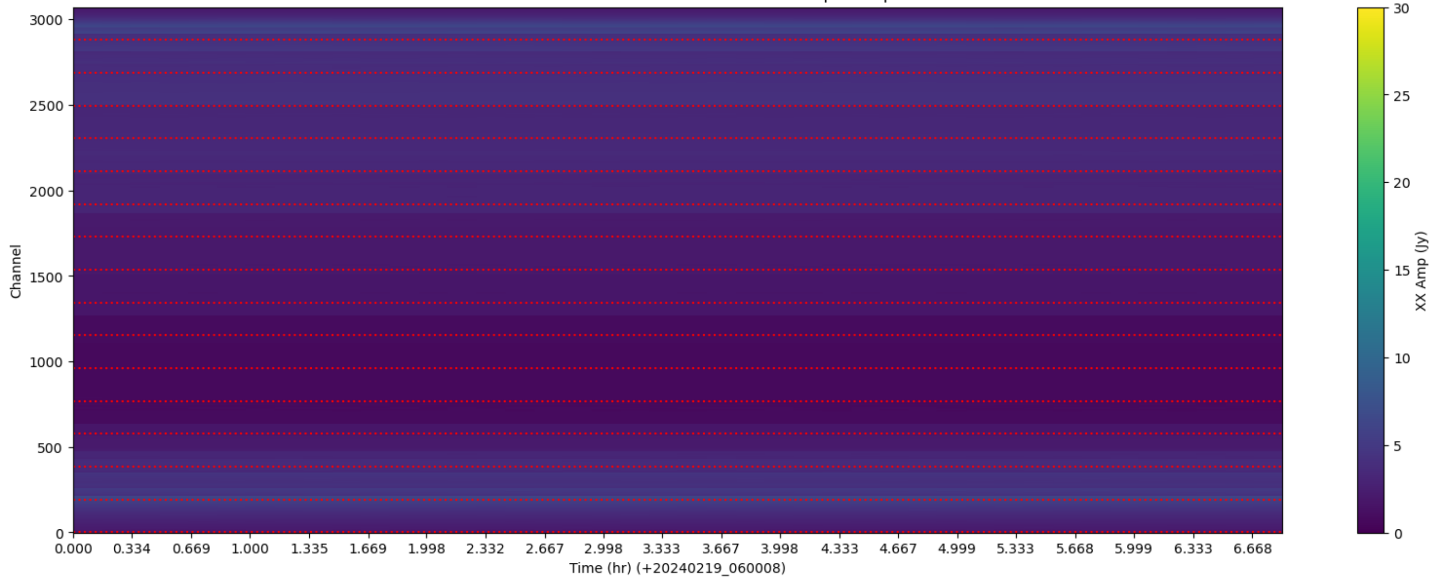
LWA312 - Correlator# 019 - XX - FLAGS: BadSpecShape
