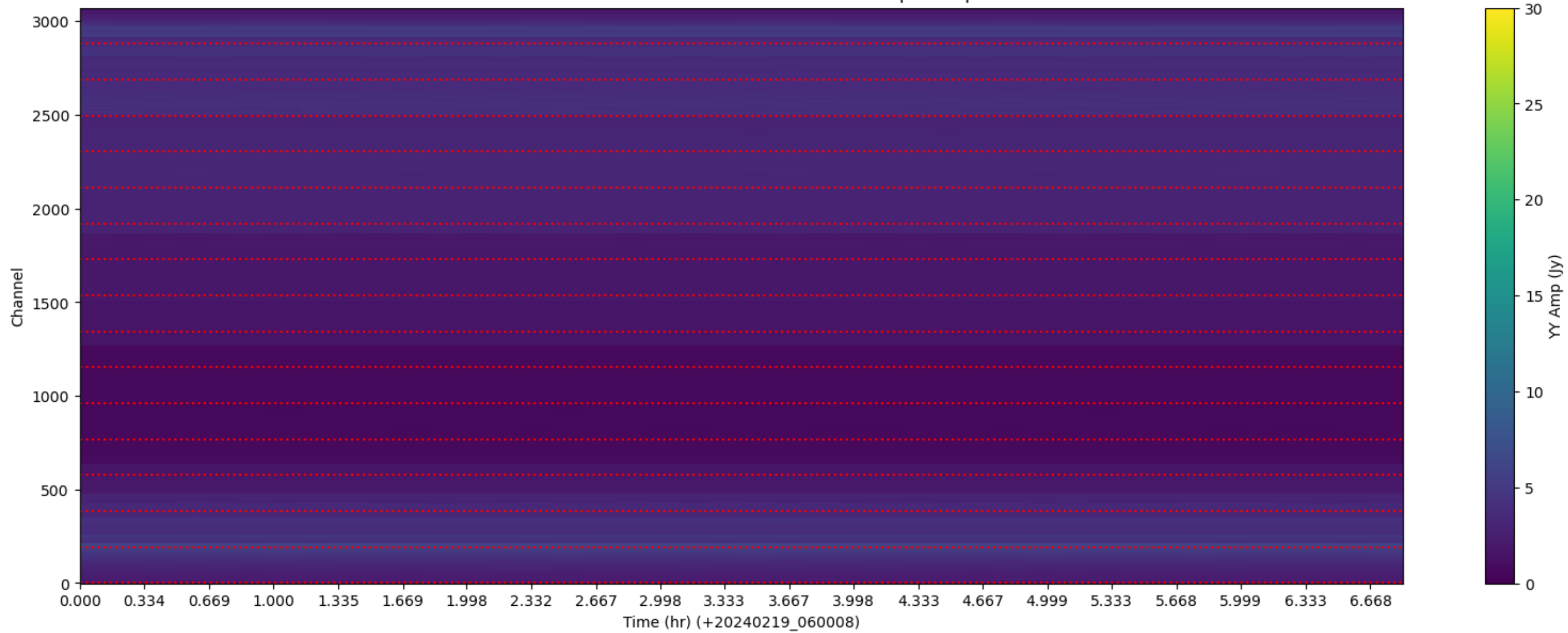
LWA279 - Correlator# 220 - YY - FLAGS: BadSpecShape
