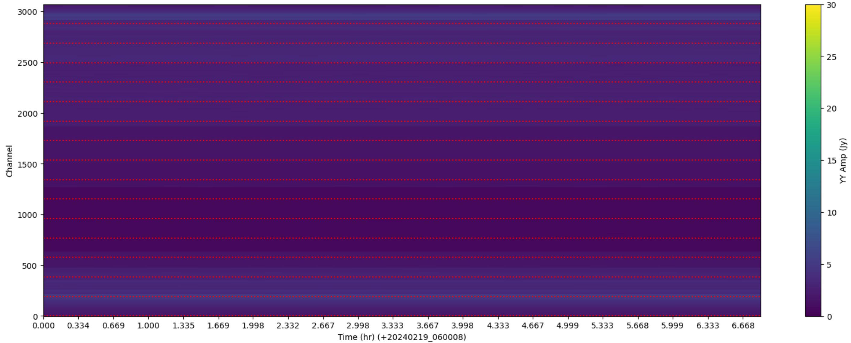
LWA270 - Correlator# 039 - YY - FLAGS: LowFlux
