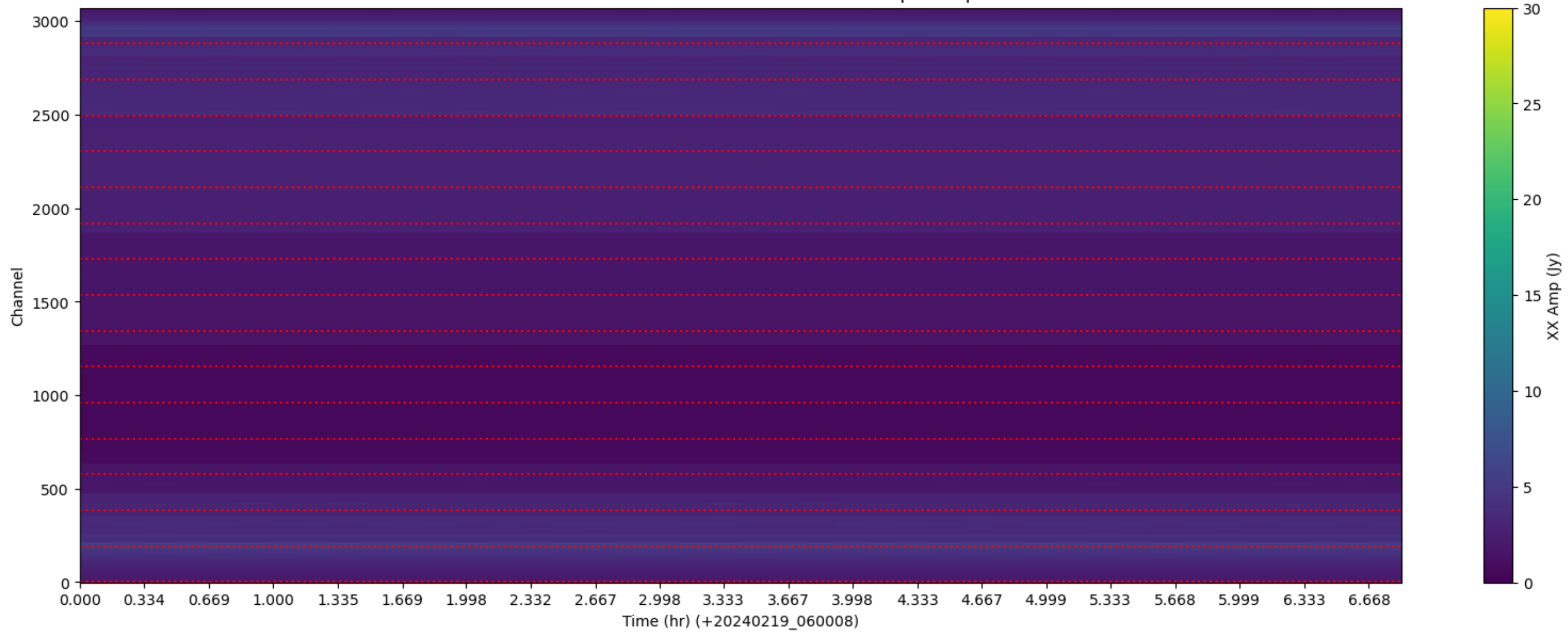
LWA350 - Correlator# 319 - XX - FLAGS: BadSpecShape
