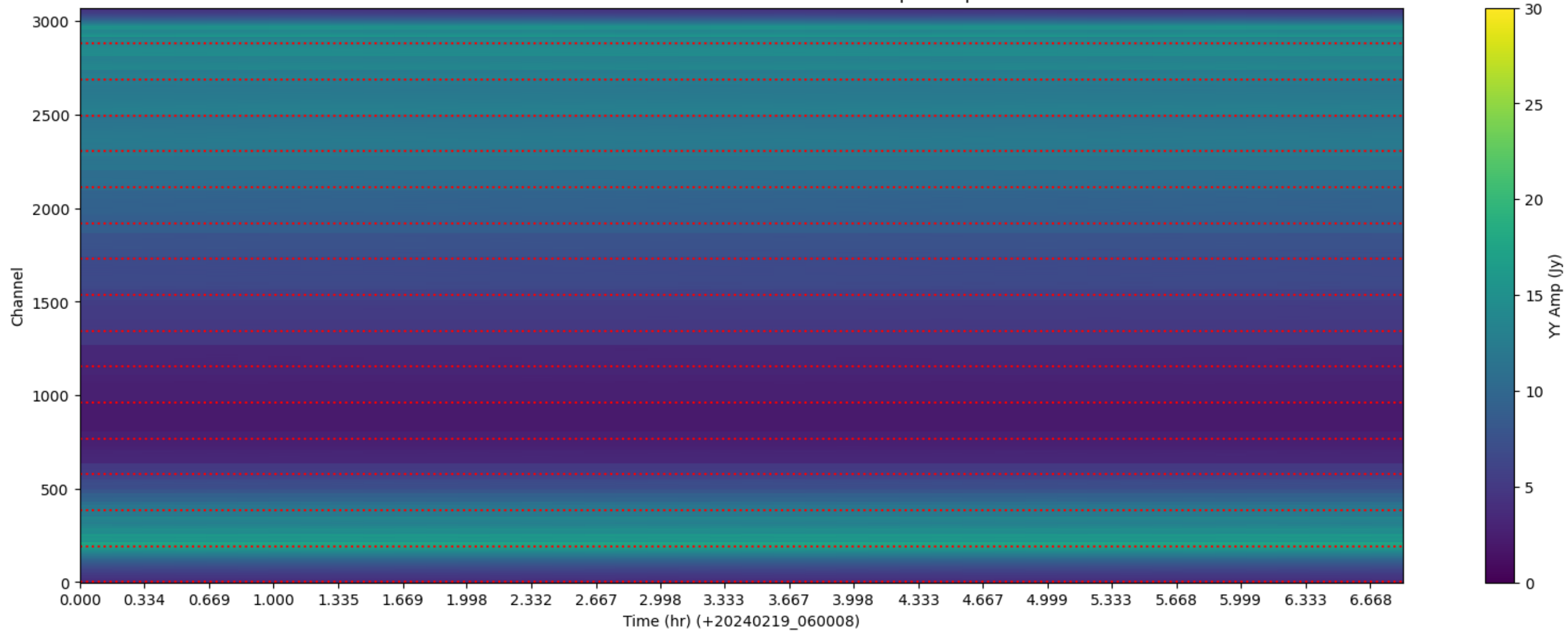
LWA328 - Correlator# 157 - YY - FLAGS: BadSpecShape
