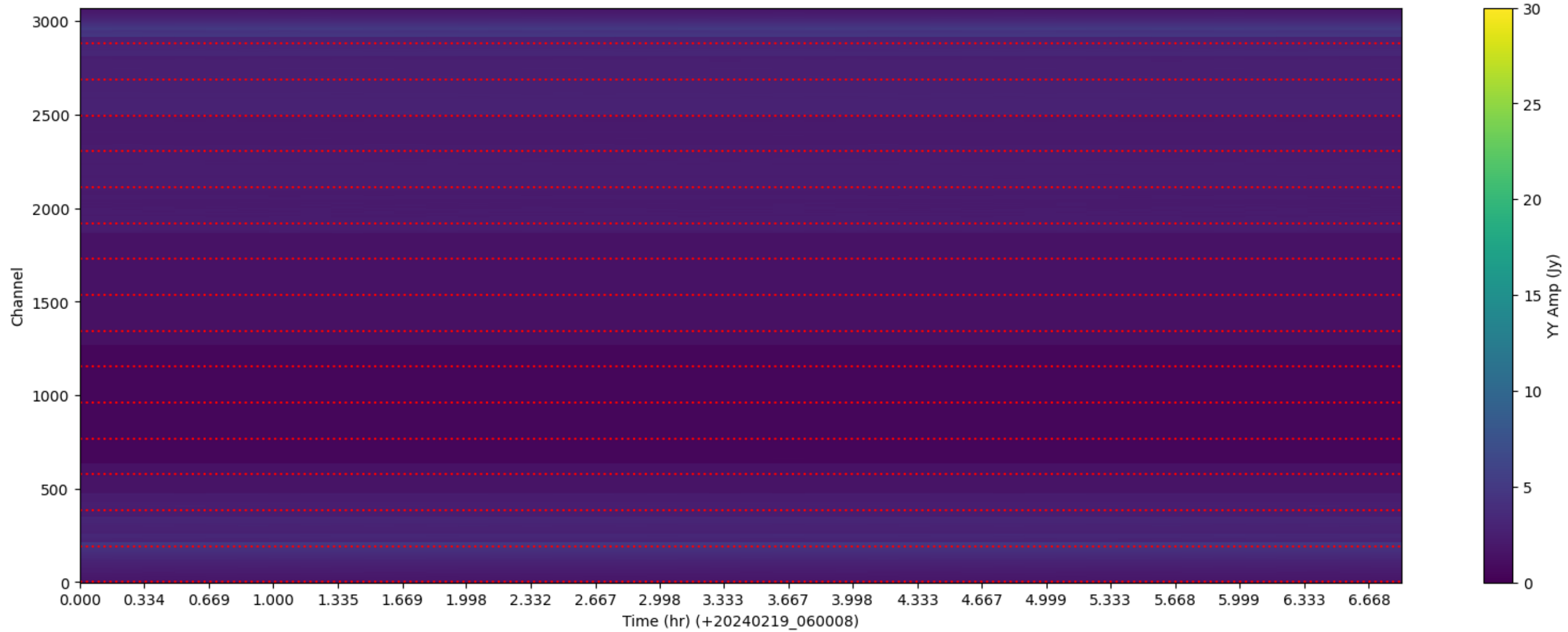
LWA264 - Correlator# 349 - YY - FLAGS: LowFlux
