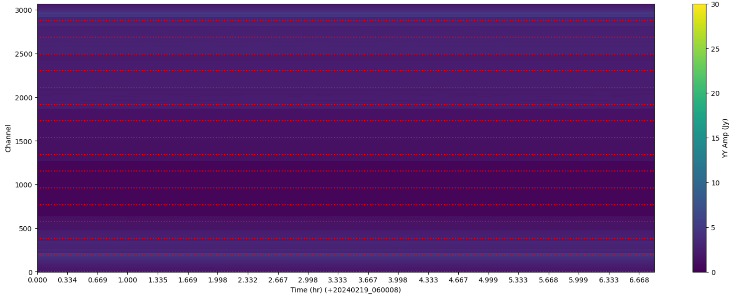
LWA329 - Correlator# 287 - YY - FLAGS: LowFlux
