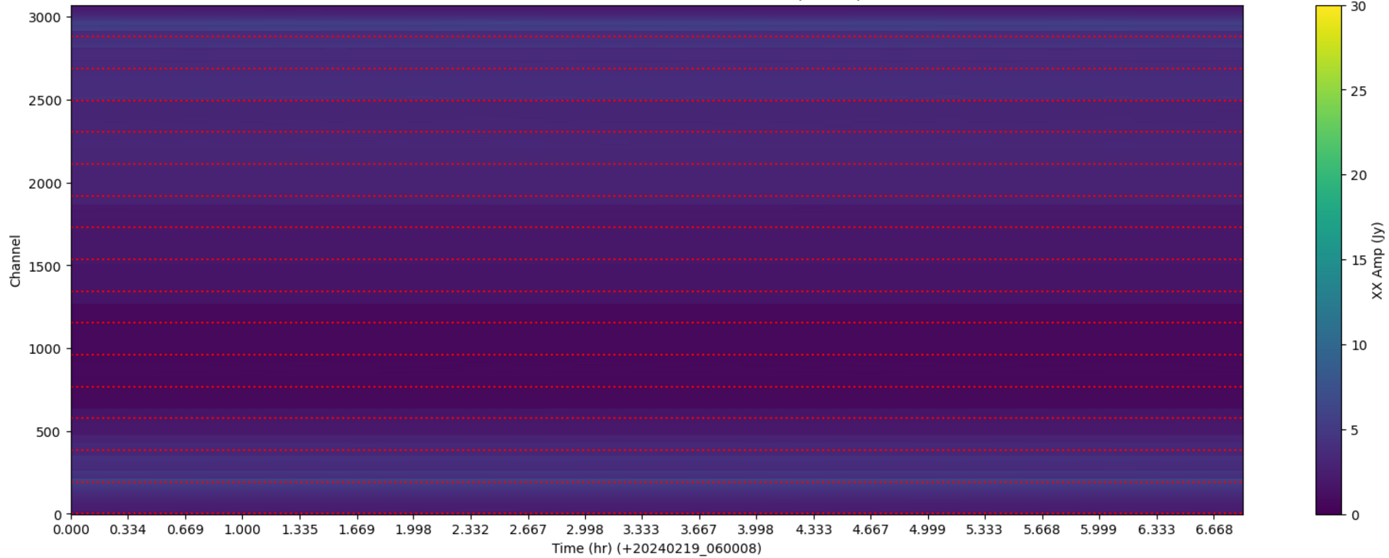
LWA287 - Correlator# 223 - XX - FLAGS: BadSpecShape
