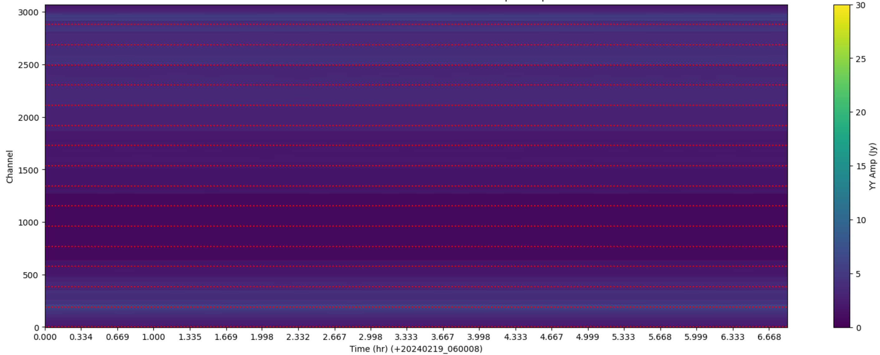
LWA266 - Correlator# 000 - YY - FLAGS: BadSpecShape
