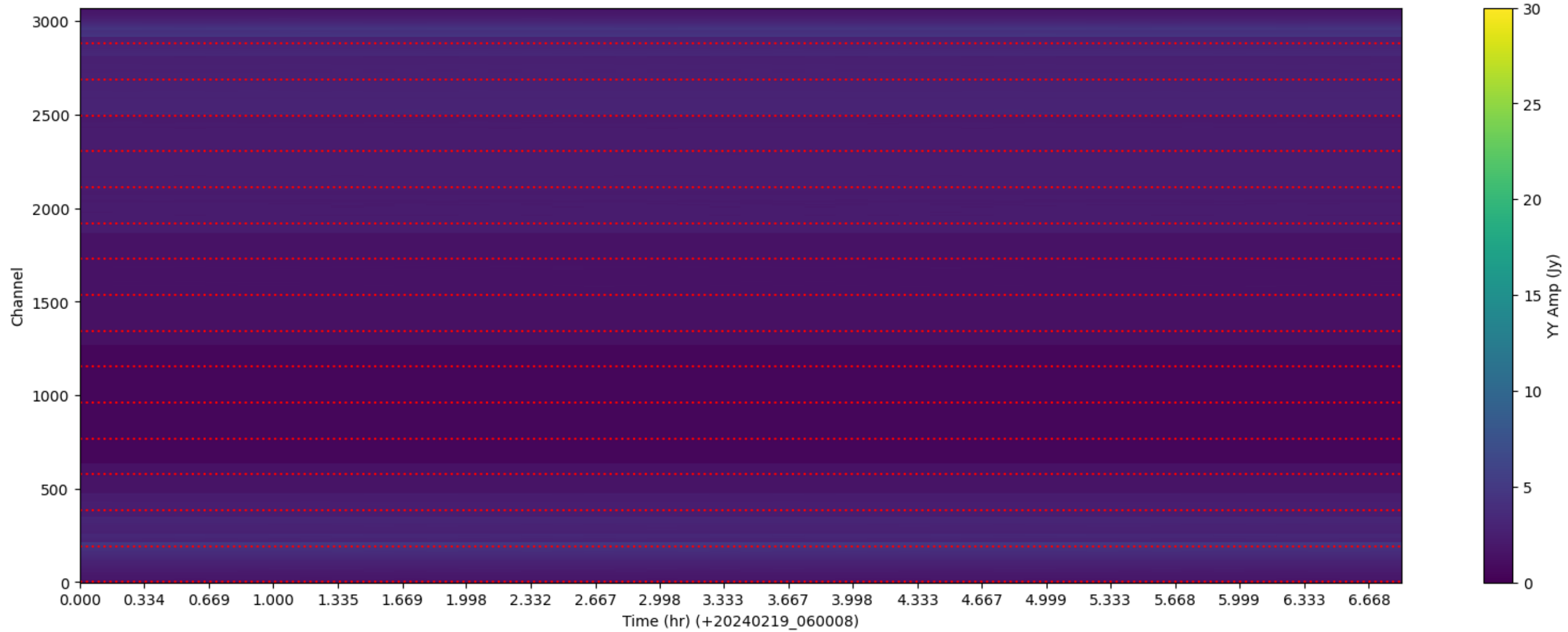
LWA320 - Correlator# 054 - YY - FLAGS: LowFlux
