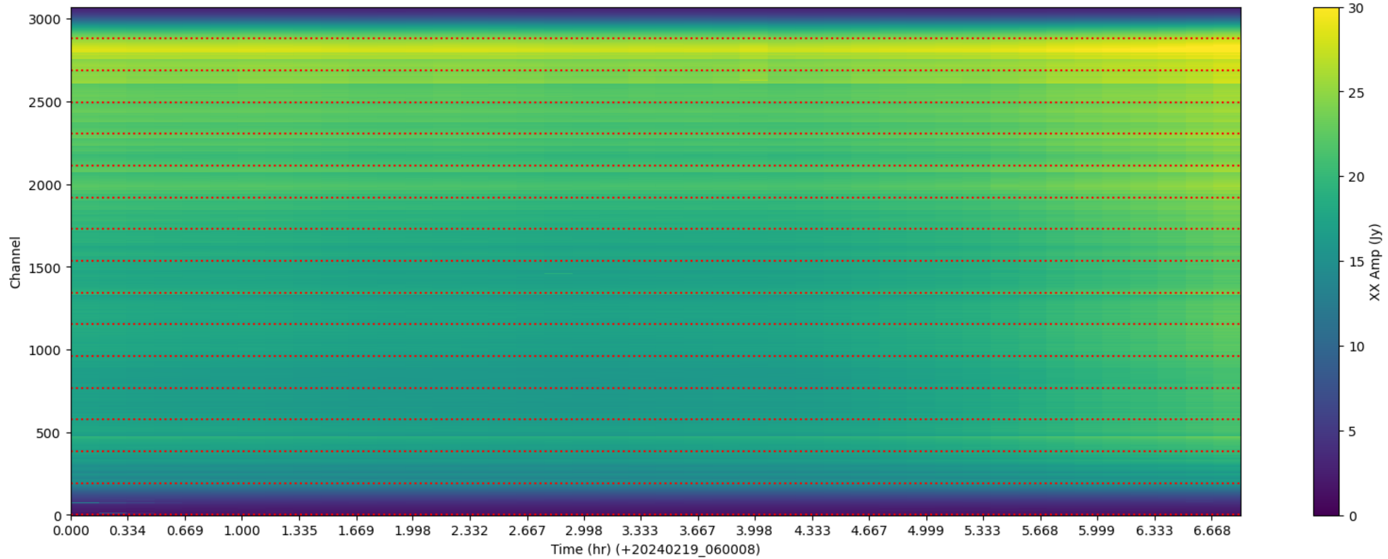
LWA003 - Correlator# 067 - XX - FLAGS: Good
