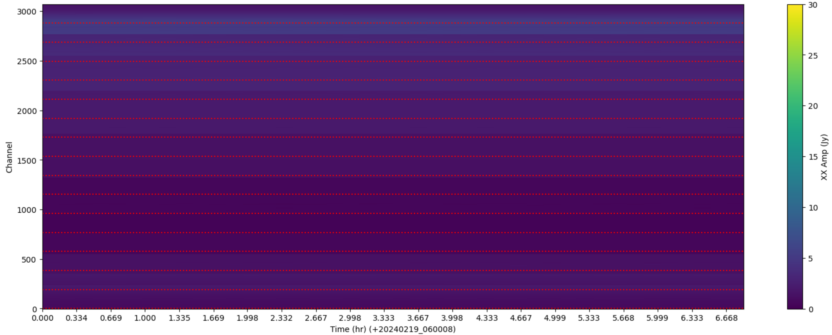
LWA138 - Correlator# 261 - XX - FLAGS: LowFlux
