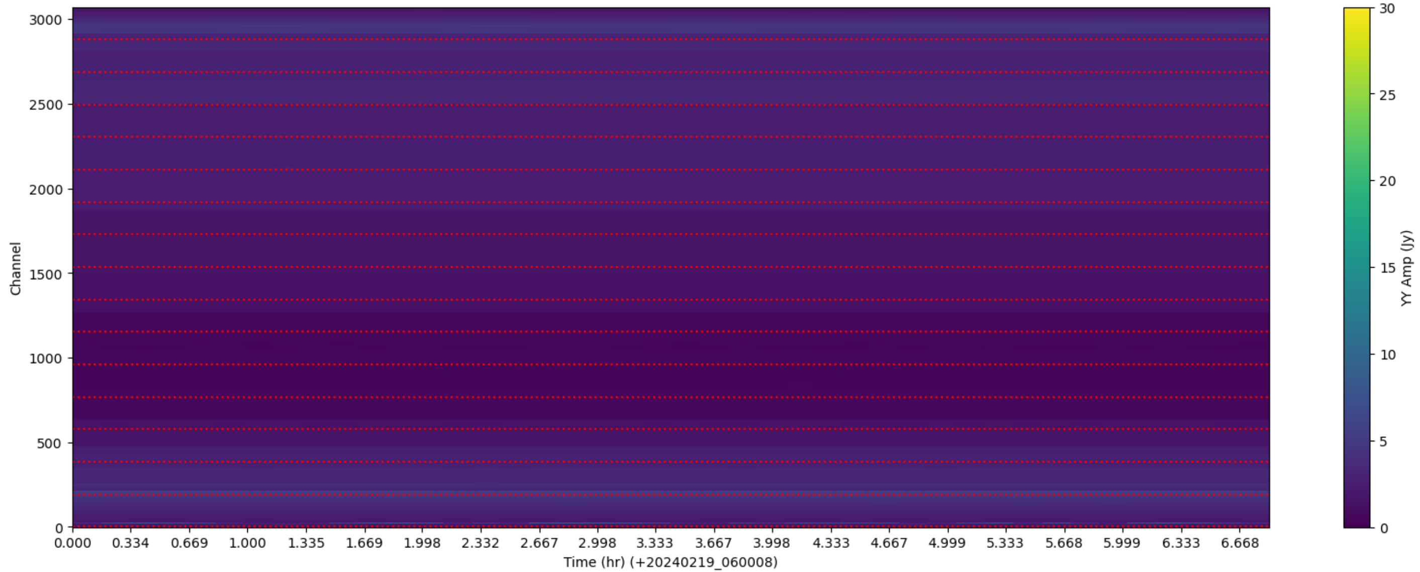
LWA343 - Correlator# 058 - YY - FLAGS: LowFlux
