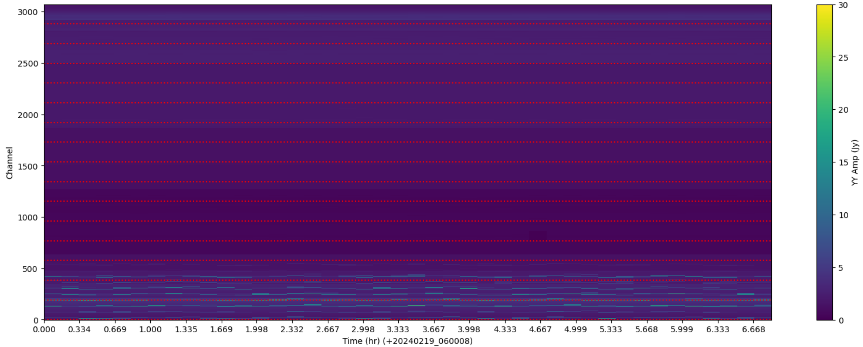
LWA319 - Correlator# 190 - YY - FLAGS: LowFlux
