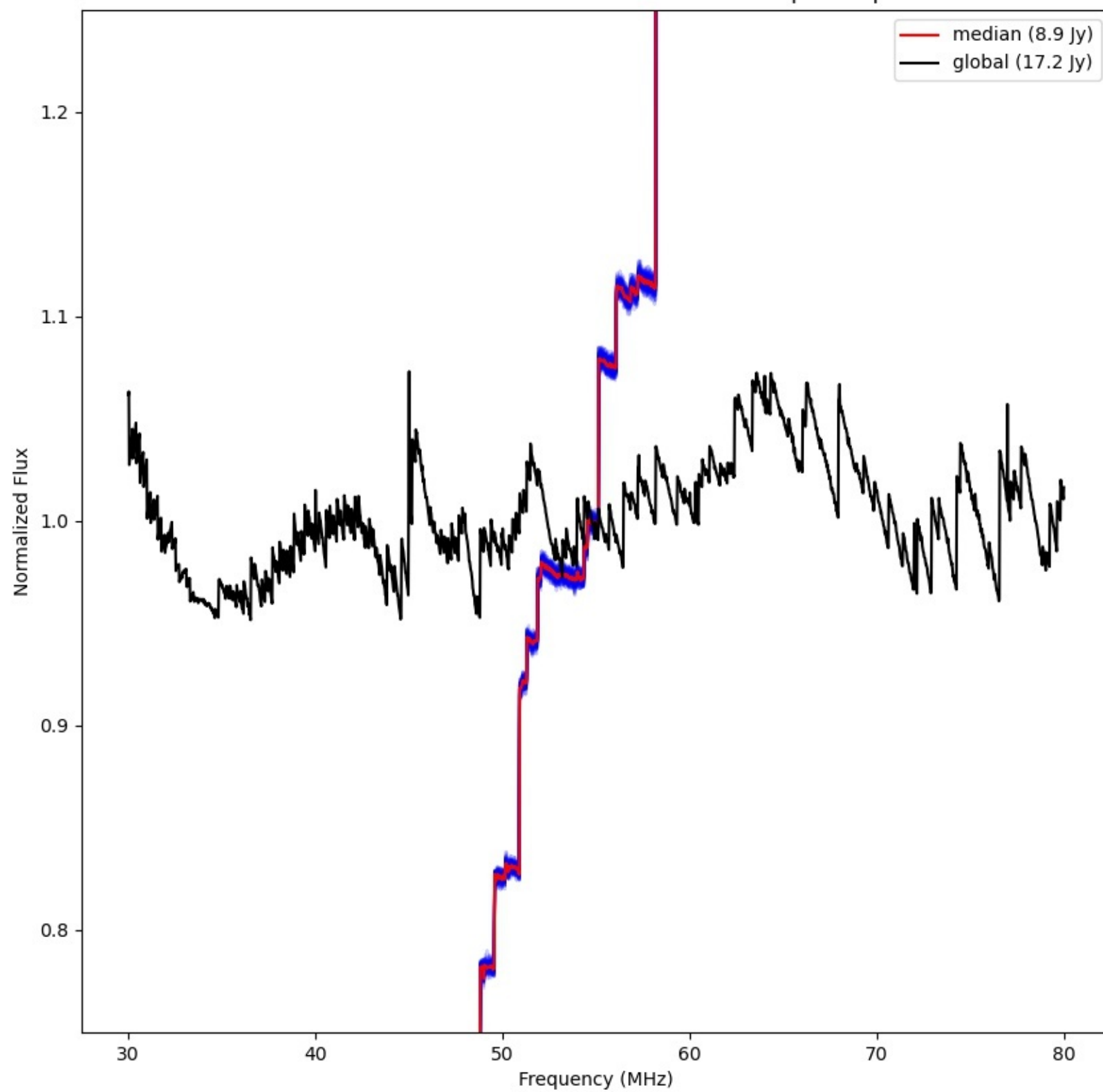
LWA313 - Correlator# 018 - XX - FLAGS:BadSpecShape
