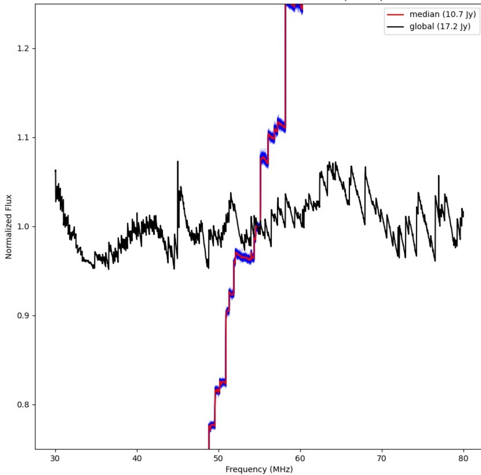
LWA277 - Correlator# 009 - XX - FLAGS:BadSpecShape
