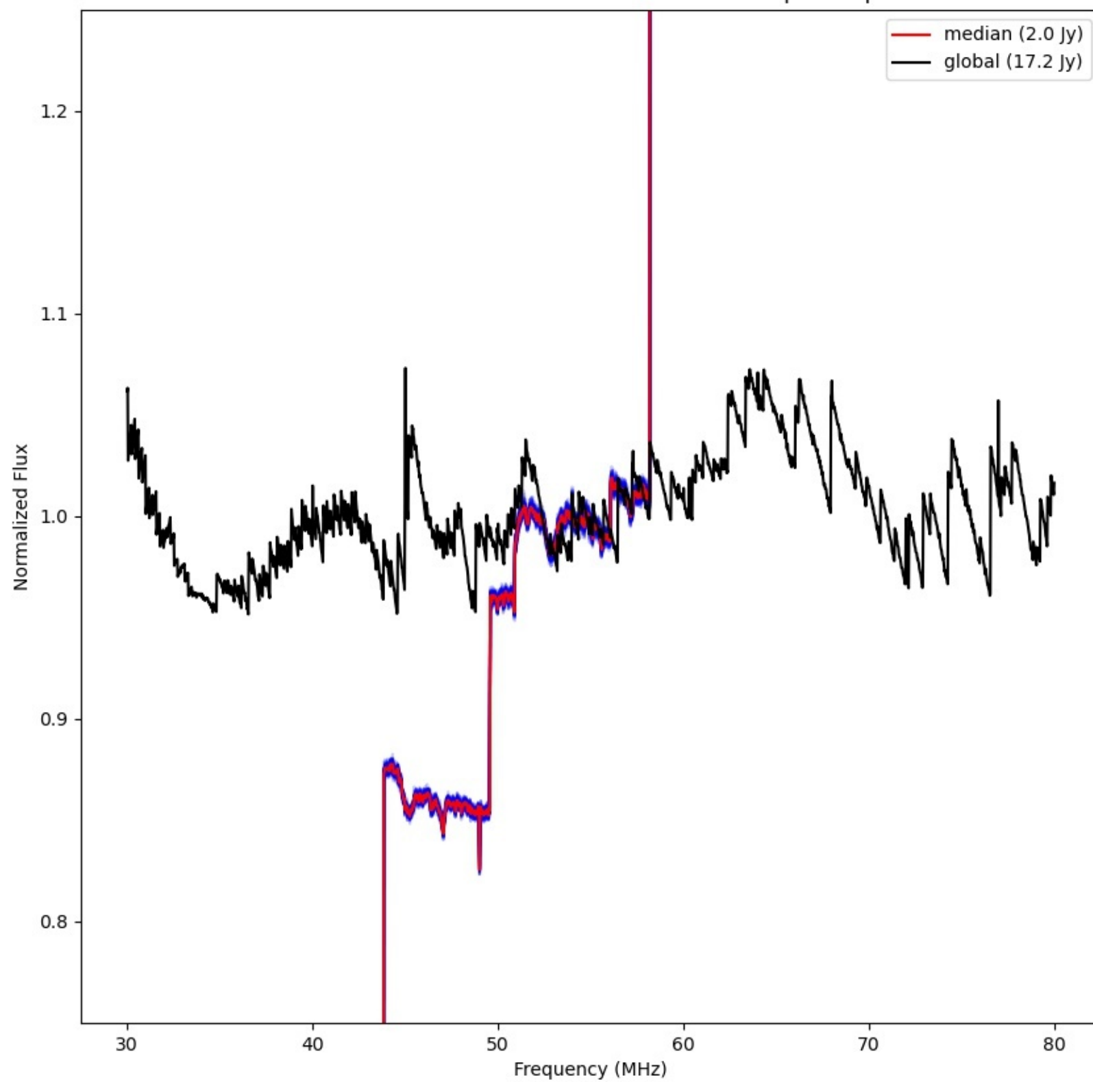
LWA327 - Correlator# 023 - XX - FLAGS:BadSpecShape
