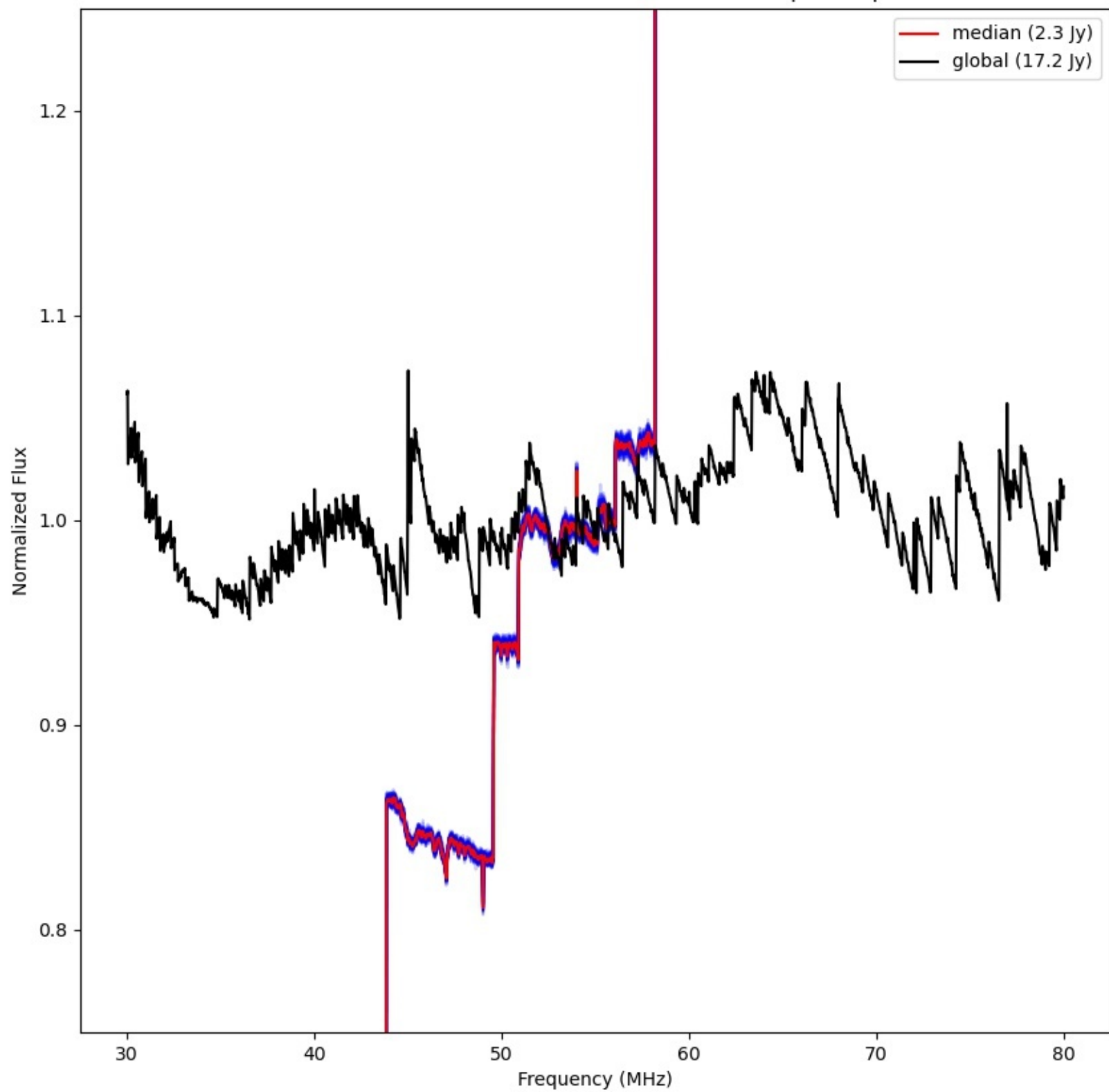
LWA329 - Correlator# 287 - XX - FLAGS:BadSpecShape
