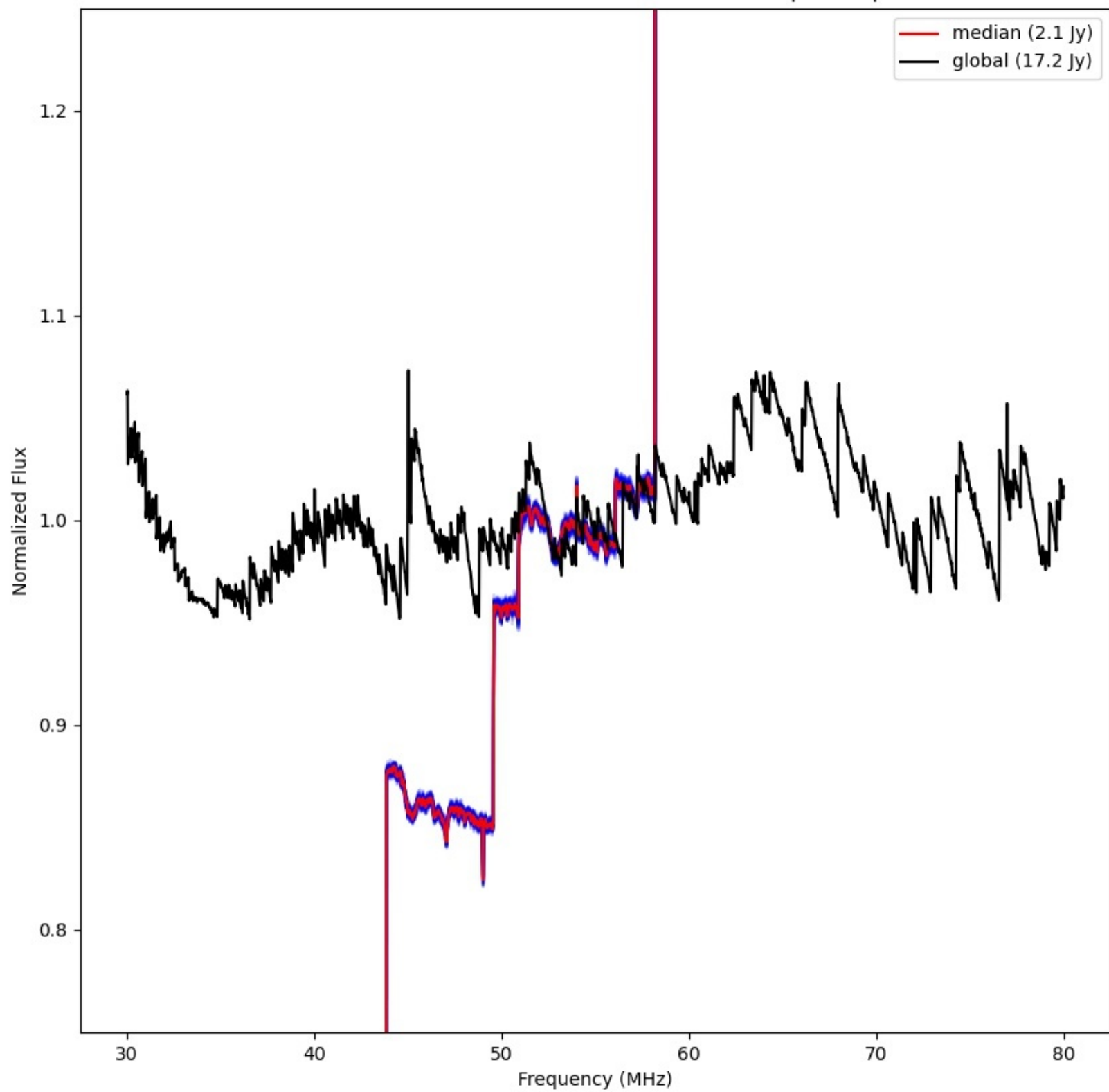
LWA320 - Correlator# 054 - XX - FLAGS:BadSpecShape
