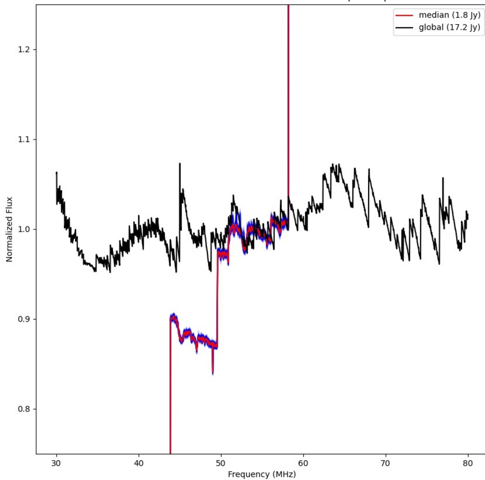
LWA309 - Correlator# 014 - XX - FLAGS:BadSpecShape
