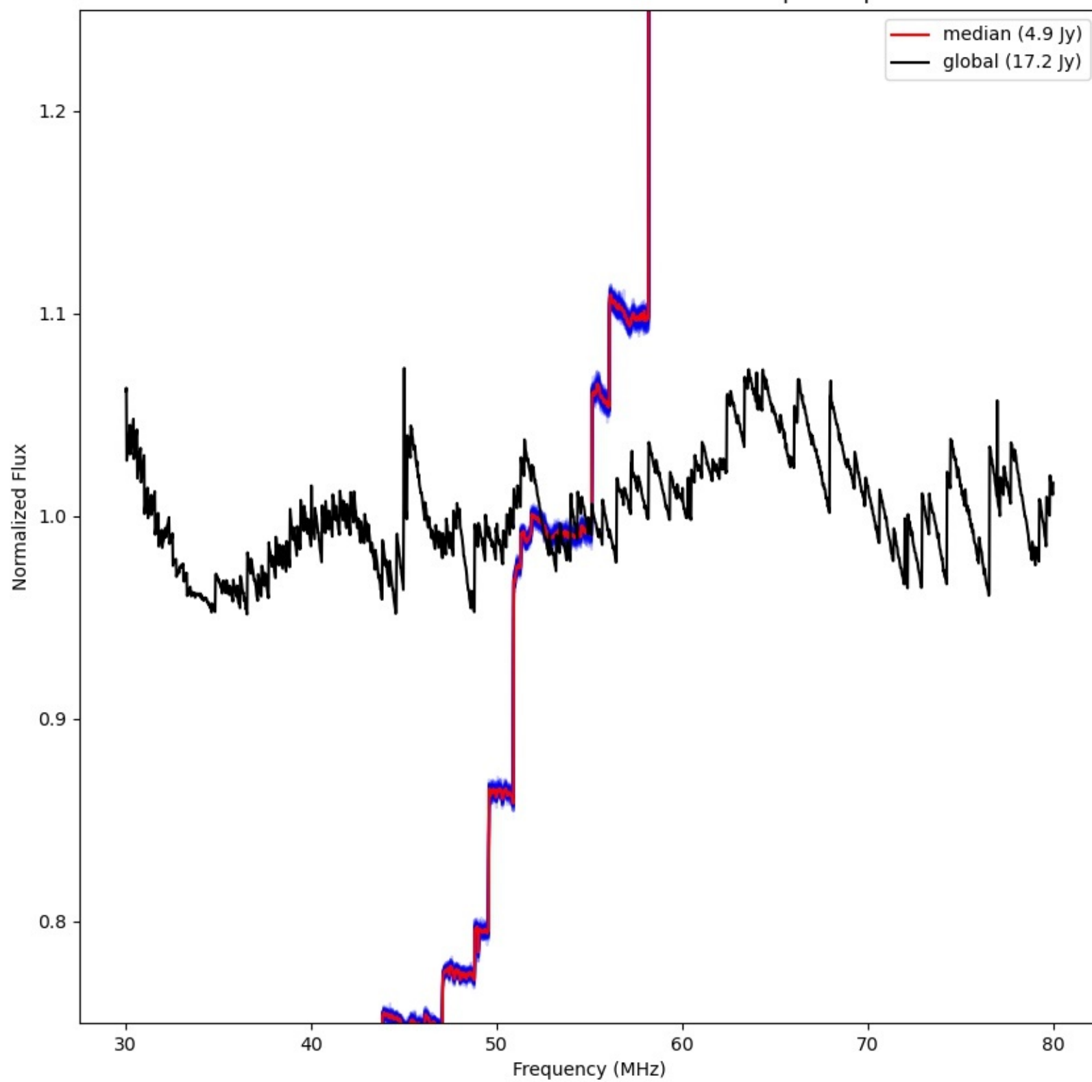
LWA321 - Correlator# 020 - XX - FLAGS:BadSpecShape
