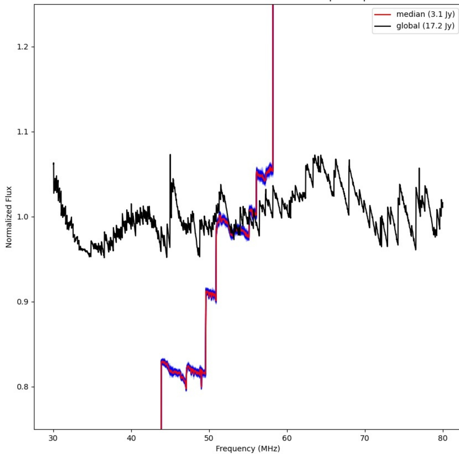
LWA316 - Correlator# 155 - XX - FLAGS:BadSpecShape
