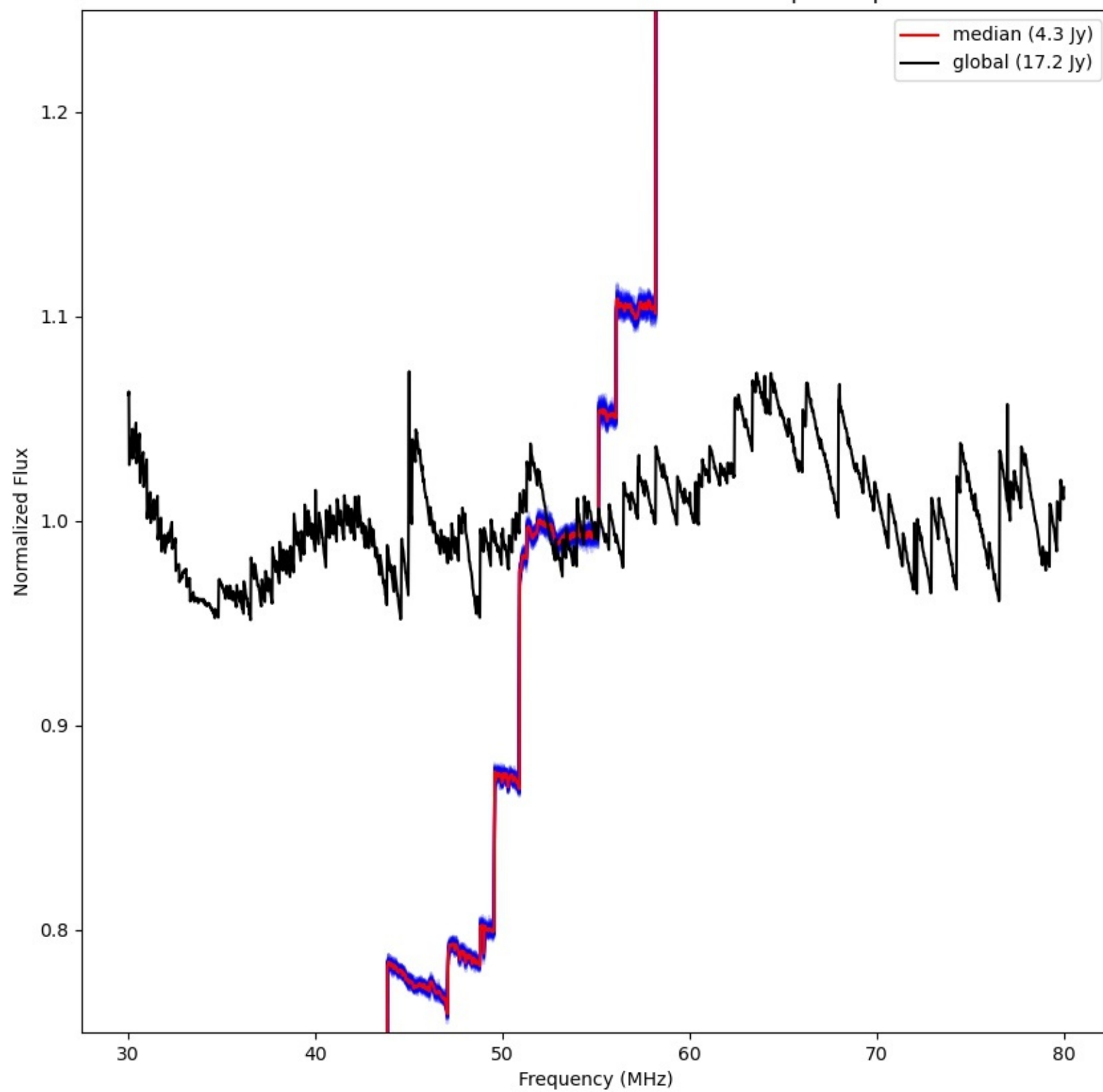
LWA264 - Correlator# 349 - XX - FLAGS:BadSpecShape
