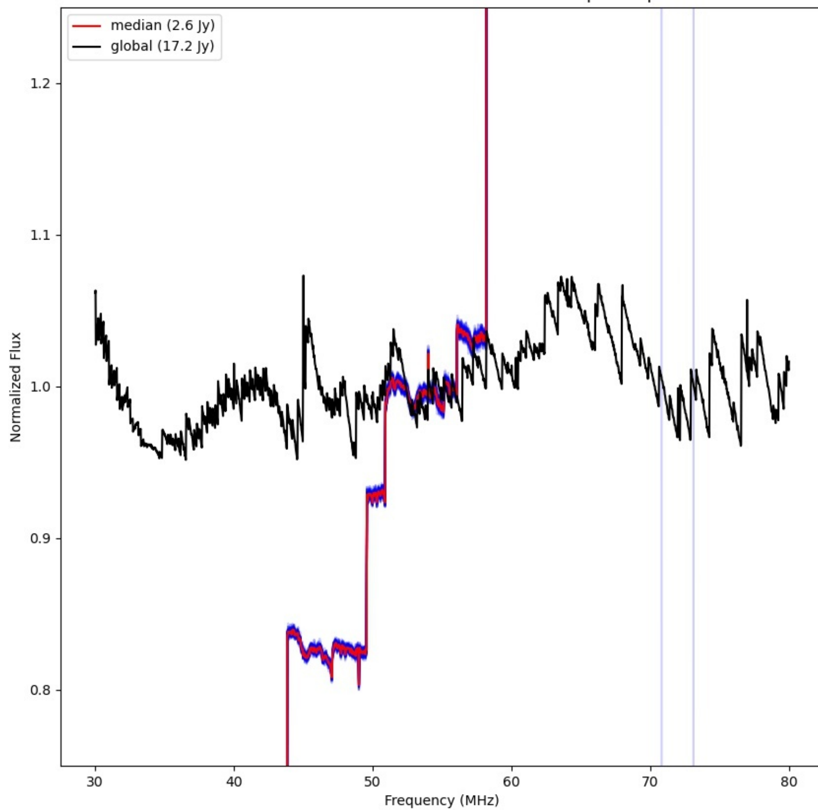
LWA338 - Correlator# 024 - XX - FLAGS:BadSpecShape
