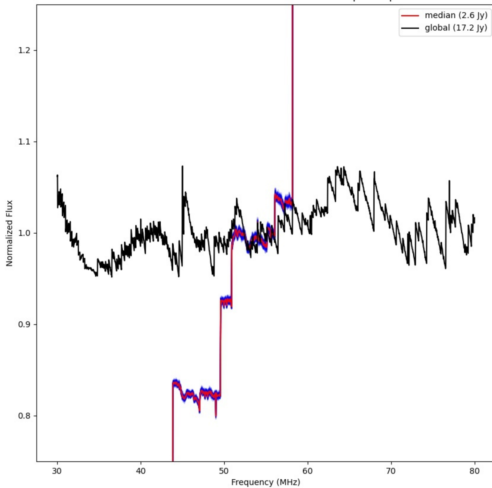
LWA330 - Correlator# 022 - XX - FLAGS:BadSpecShape
