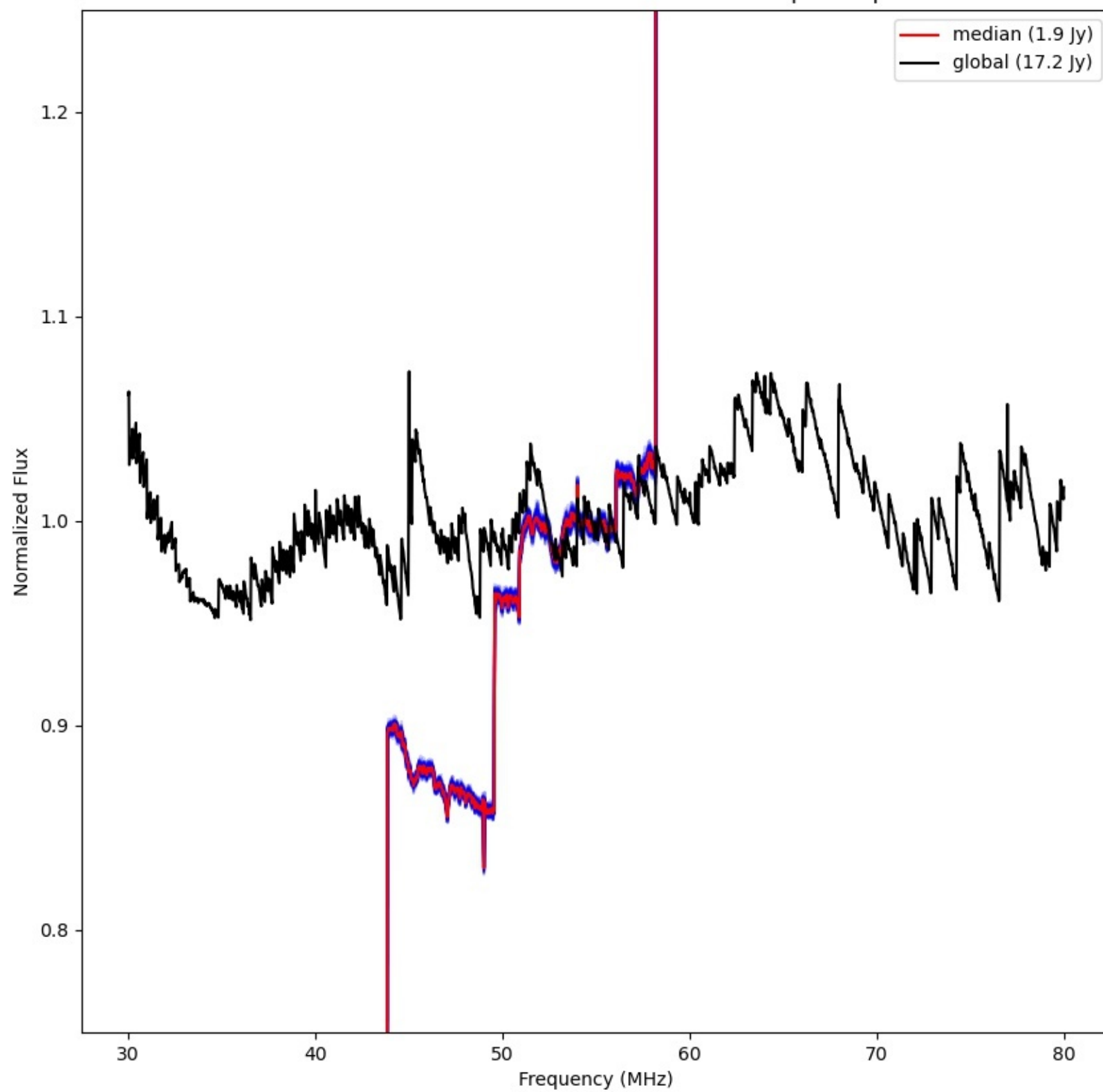
LWA272 - Correlator# 038 - XX - FLAGS:BadSpecShape
