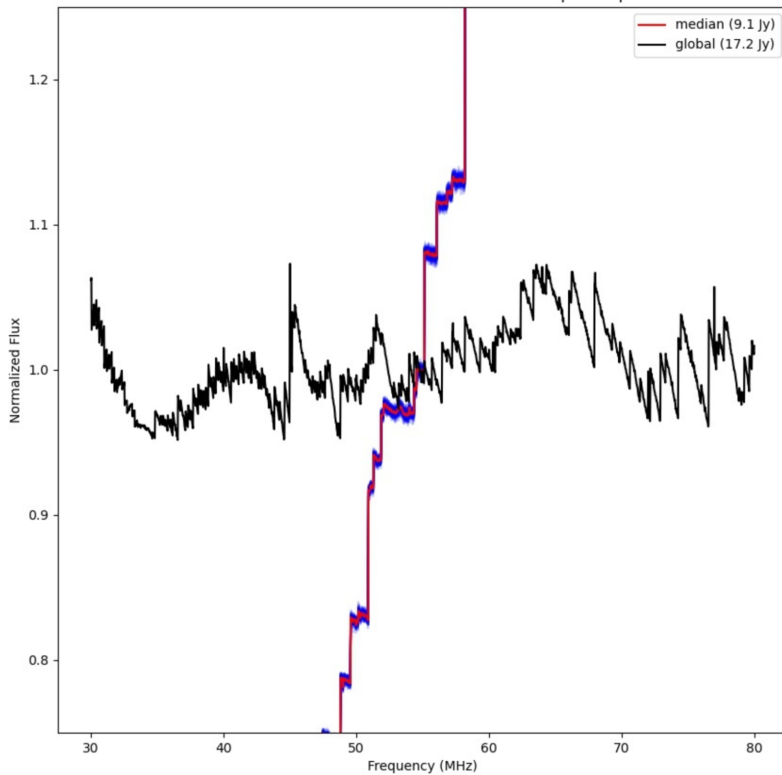
LWA315 - Correlator# 350 - XX - FLAGS:BadSpecShape
