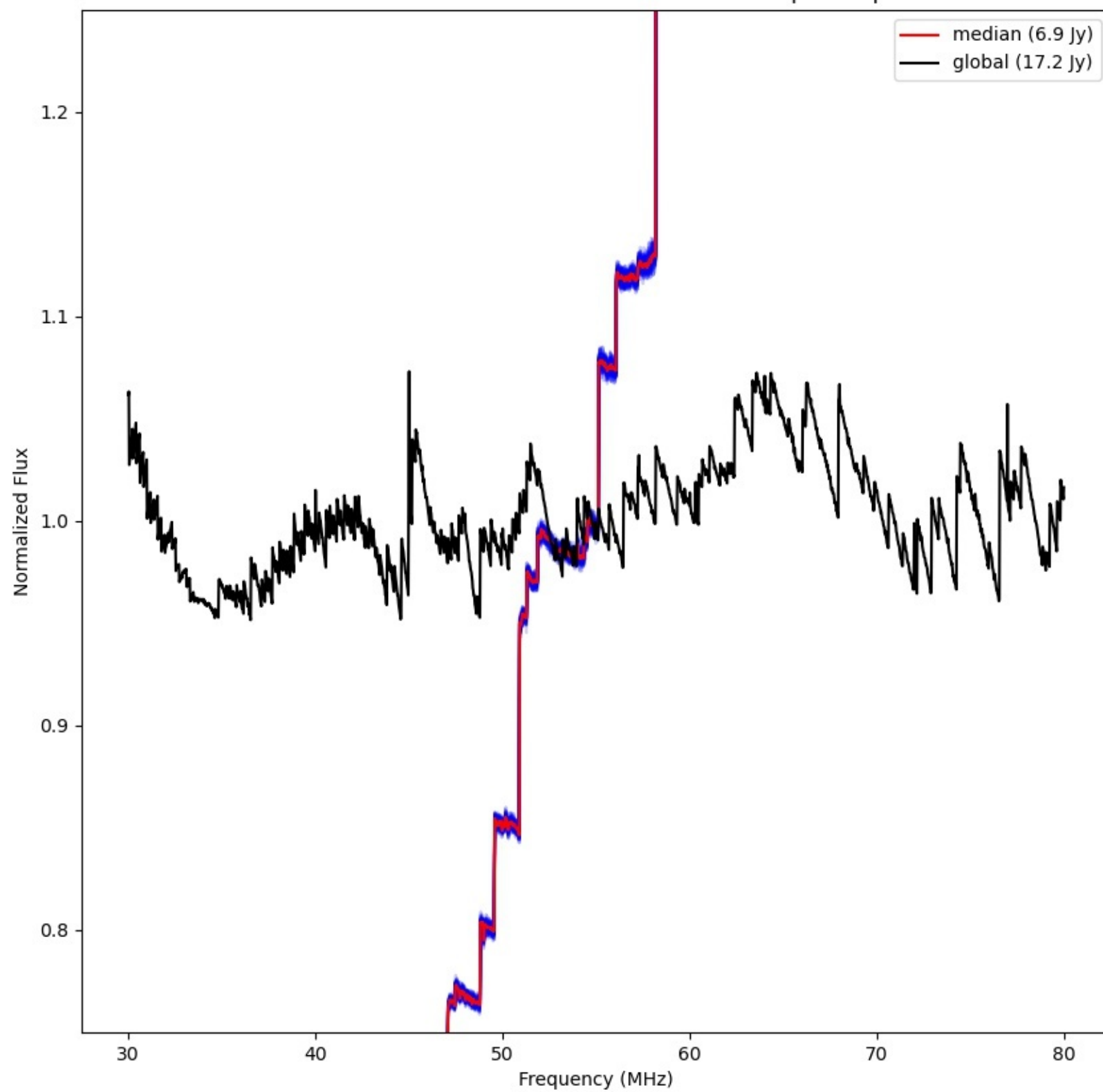
LWA286 - Correlator# 093 - XX - FLAGS:BadSpecShape
