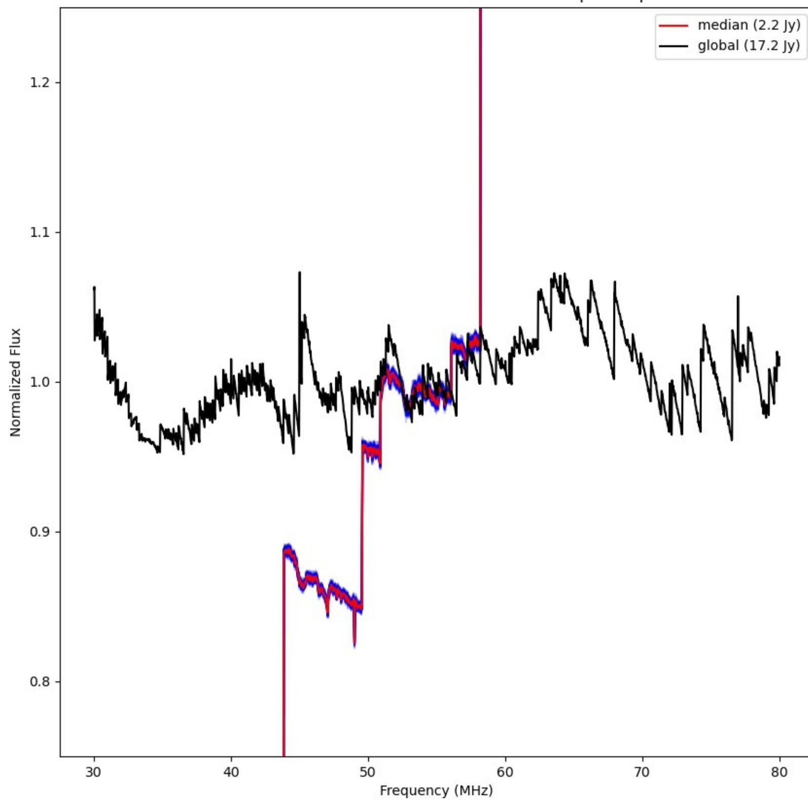
LWA275 - Correlator# 090 - XX - FLAGS:BadSpecShape
