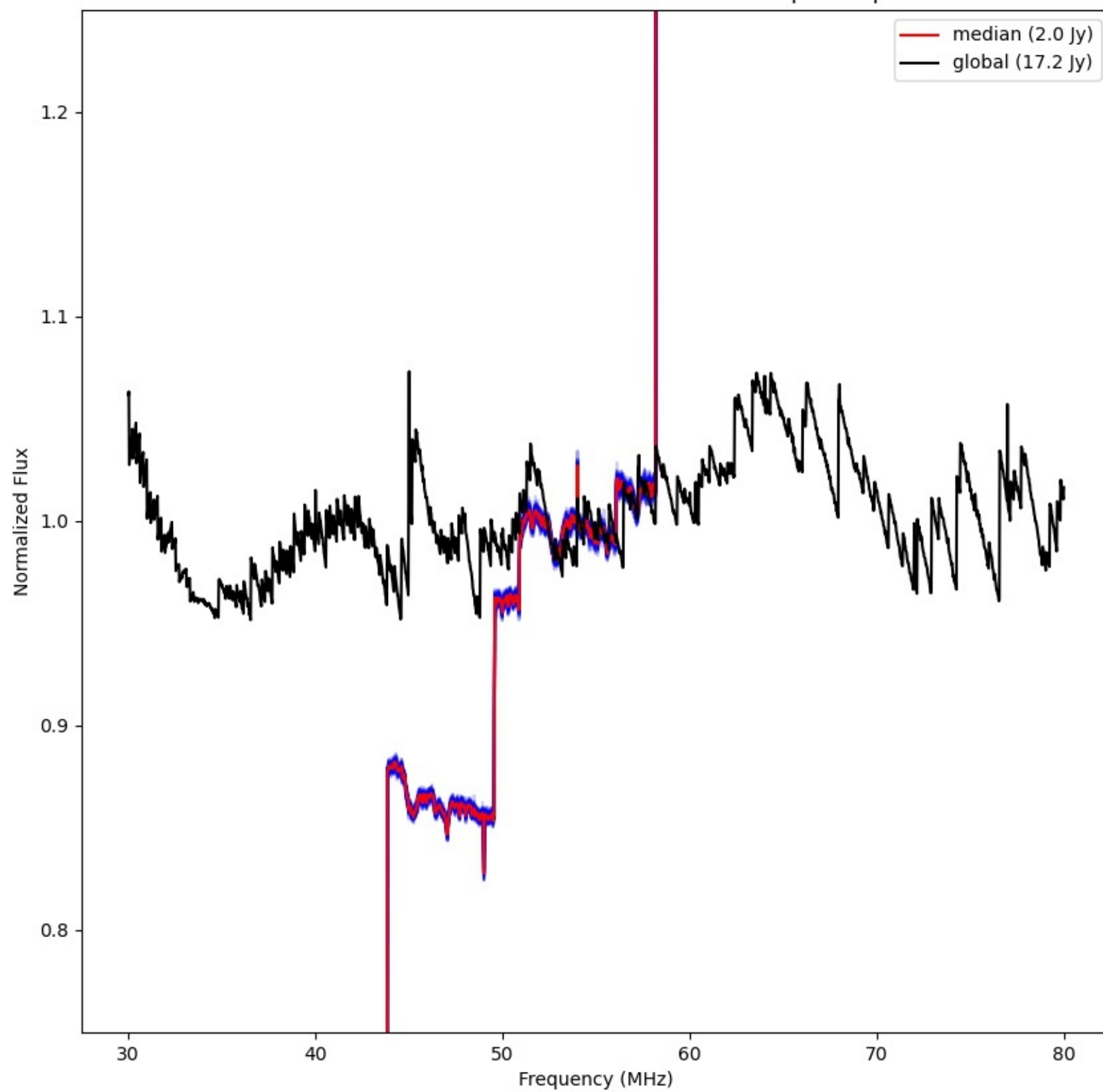
LWA287 - Correlator# 223 - XX - FLAGS:BadSpecShape
