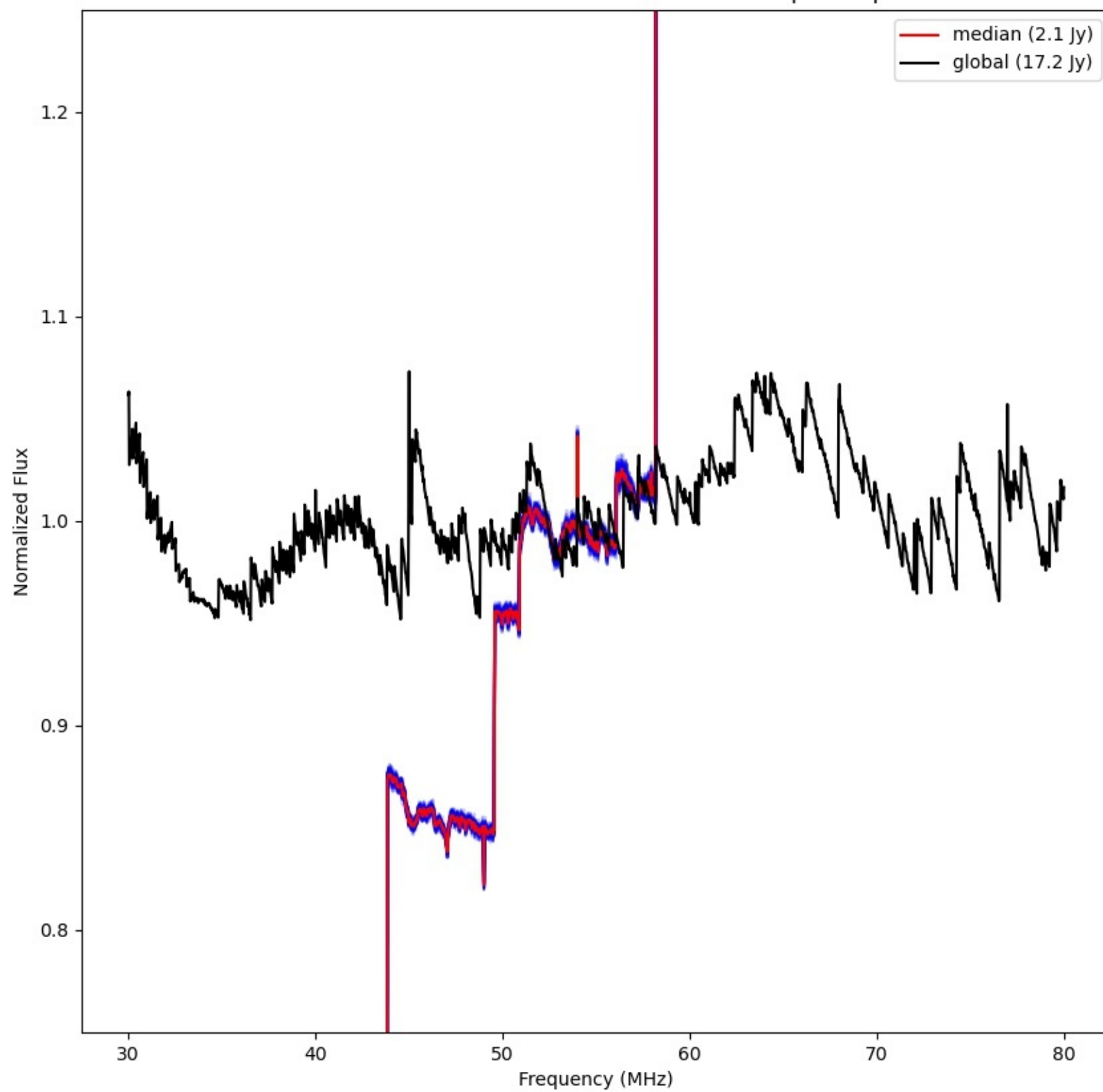
LWA276 - Correlator# 006 - XX - FLAGS:BadSpecShape
