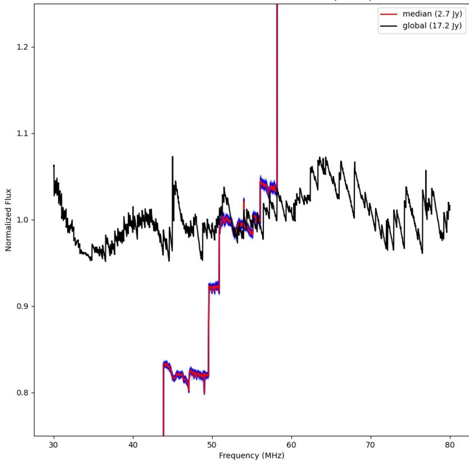
LWA283 - Correlator# 040 - XX - FLAGS:BadSpecShape
