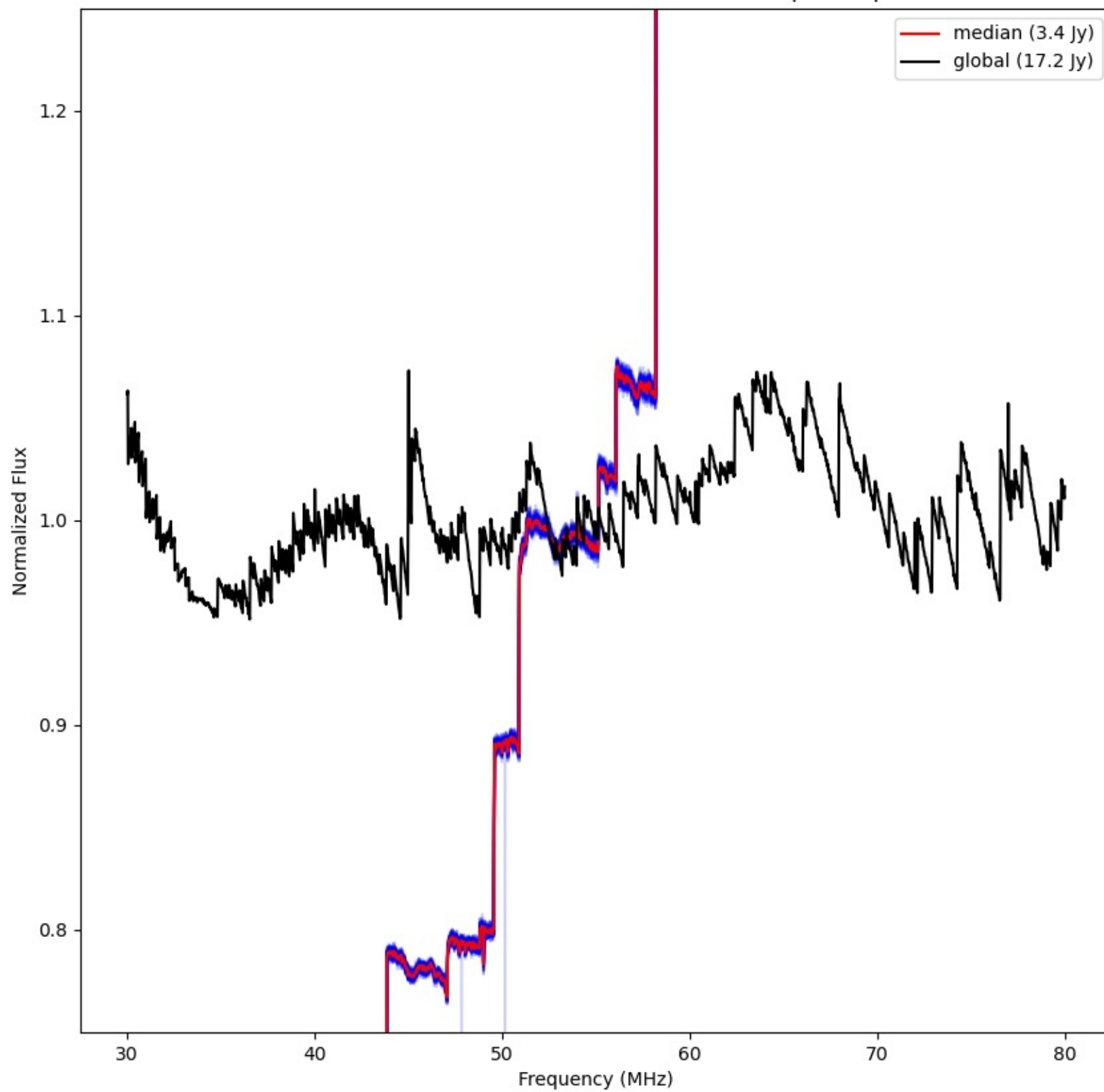
LWA339 - Correlator# 027 - XX - FLAGS:BadSpecShape
