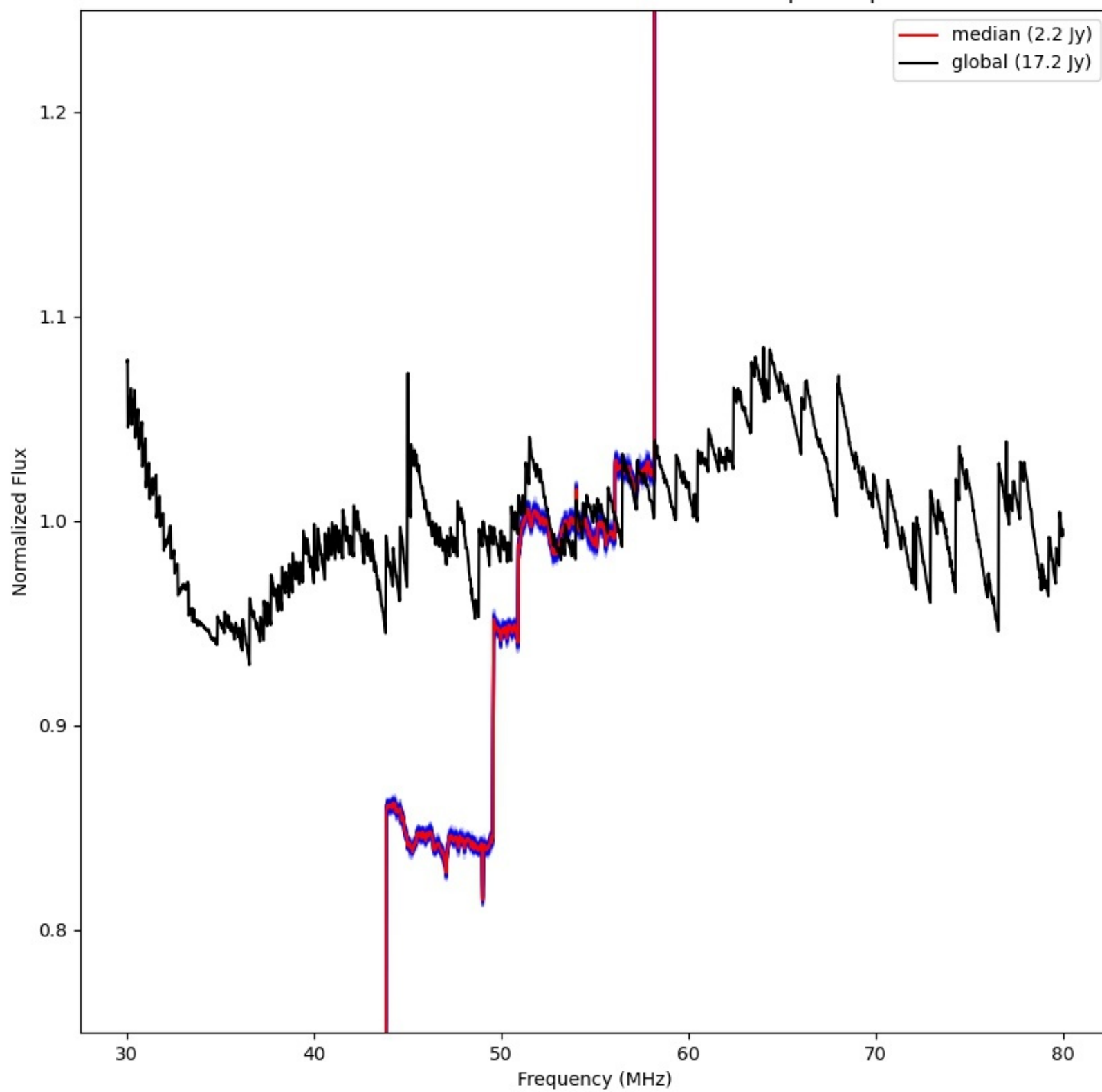
LWA327 - Correlator# 023 - YY - FLAGS:BadSpecShape
