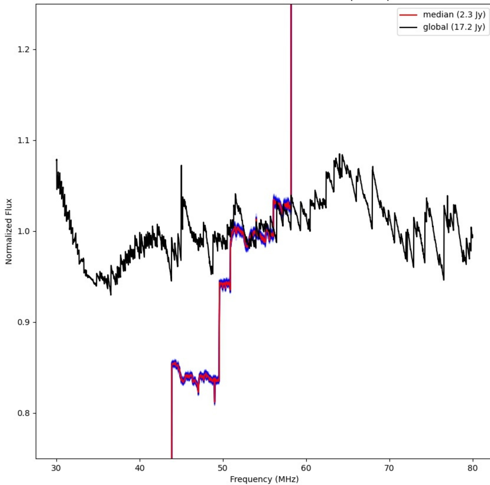
LWA276 - Correlator# 006 - YY - FLAGS:BadSpecShape
