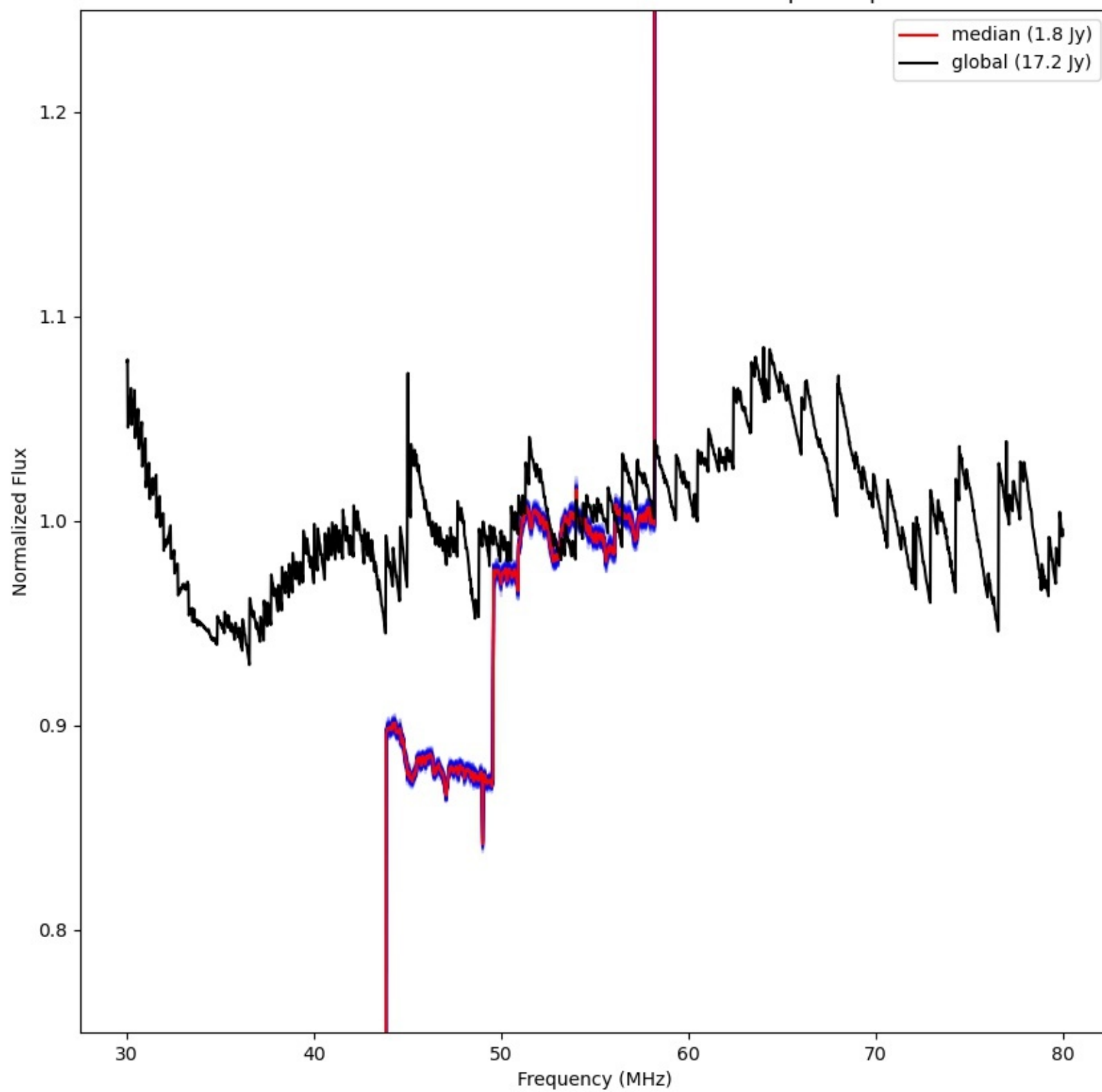
LWA296 - Correlator# 046 - YY - FLAGS:BadSpecShape
