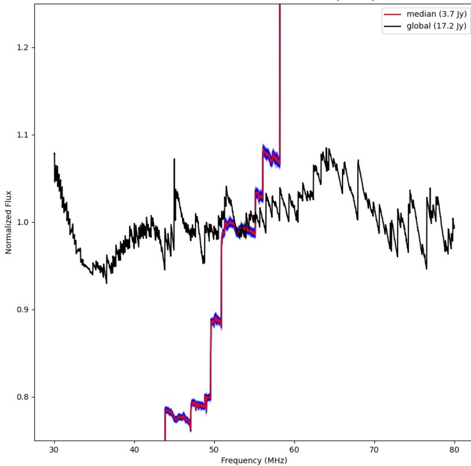
LWA344 - Correlator# 061 - YY - FLAGS:BadSpecShape
