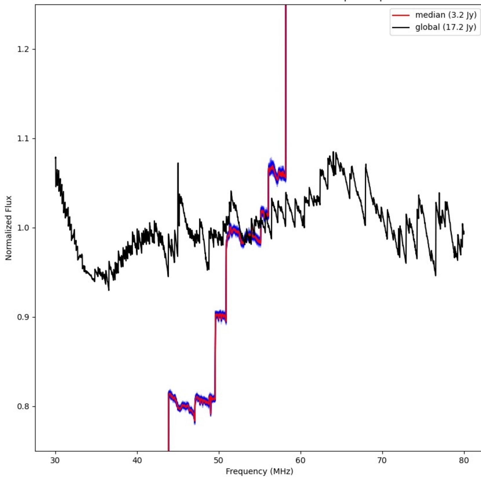
LWA311 - Correlator# 016 - YY - FLAGS:BadSpecShape
