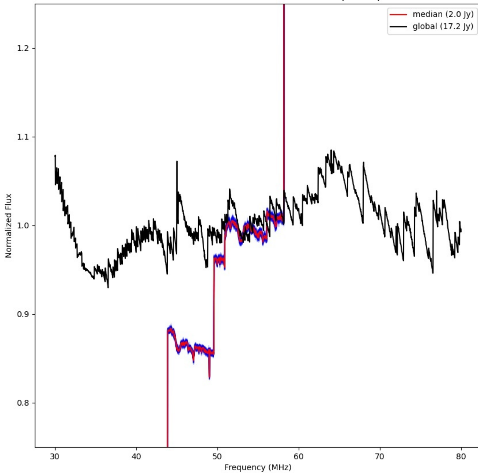
LWA271 - Correlator# 004 - YY - FLAGS:BadSpecShape
