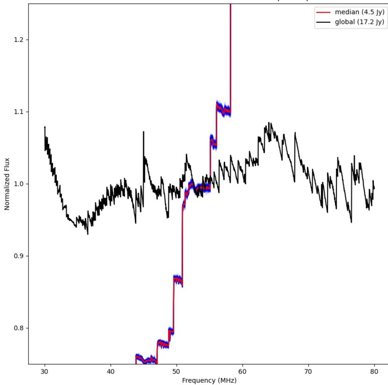
LWA269 - Correlator# 005 - YY - FLAGS:BadSpecShape
