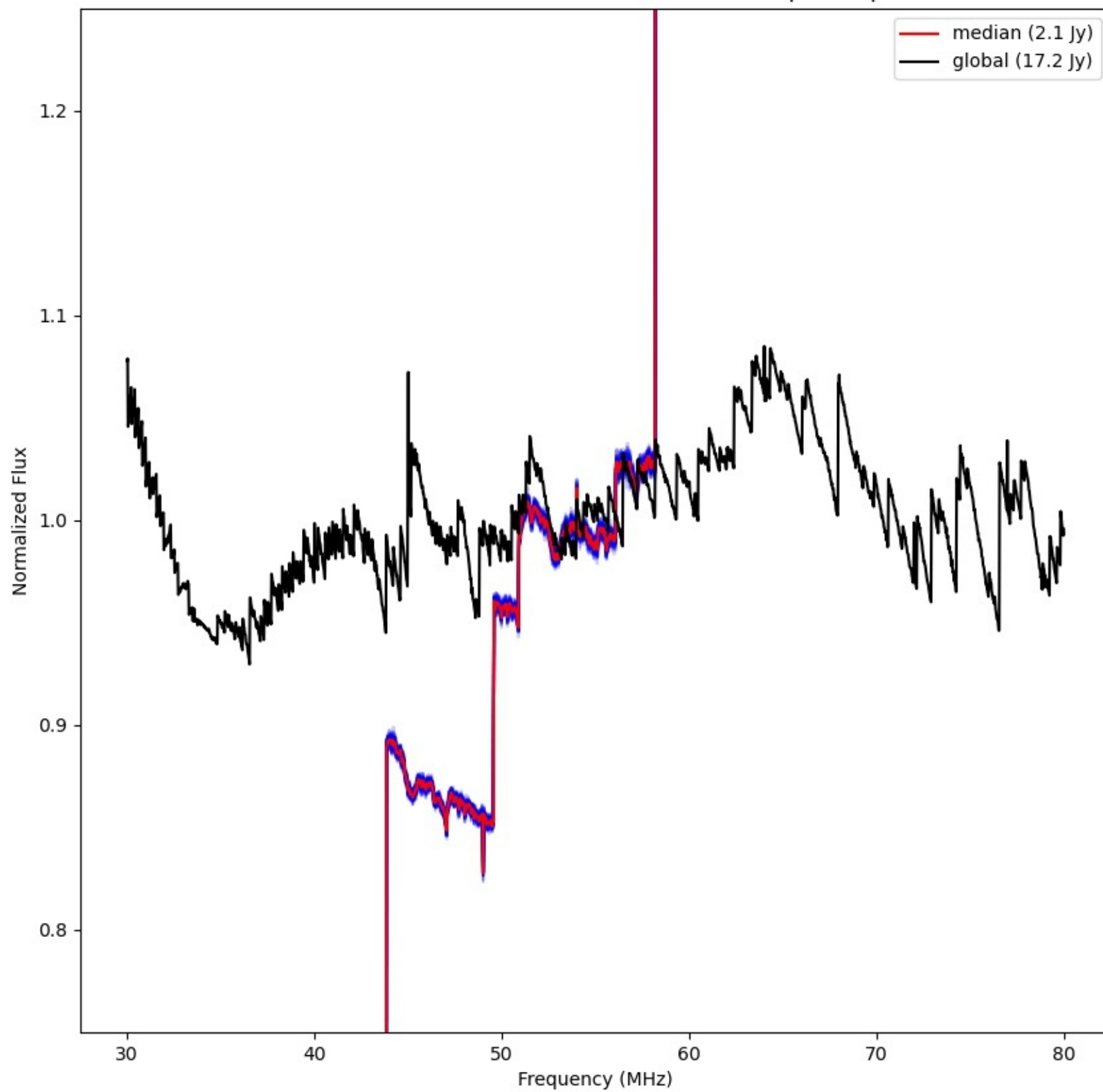
LWA348 - Correlator# 124 - YY - FLAGS:BadSpecShape
