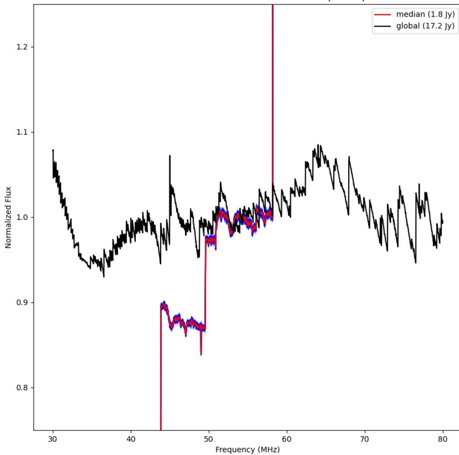
LWA282 - Correlator# 010 - YY - FLAGS:BadSpecShape
