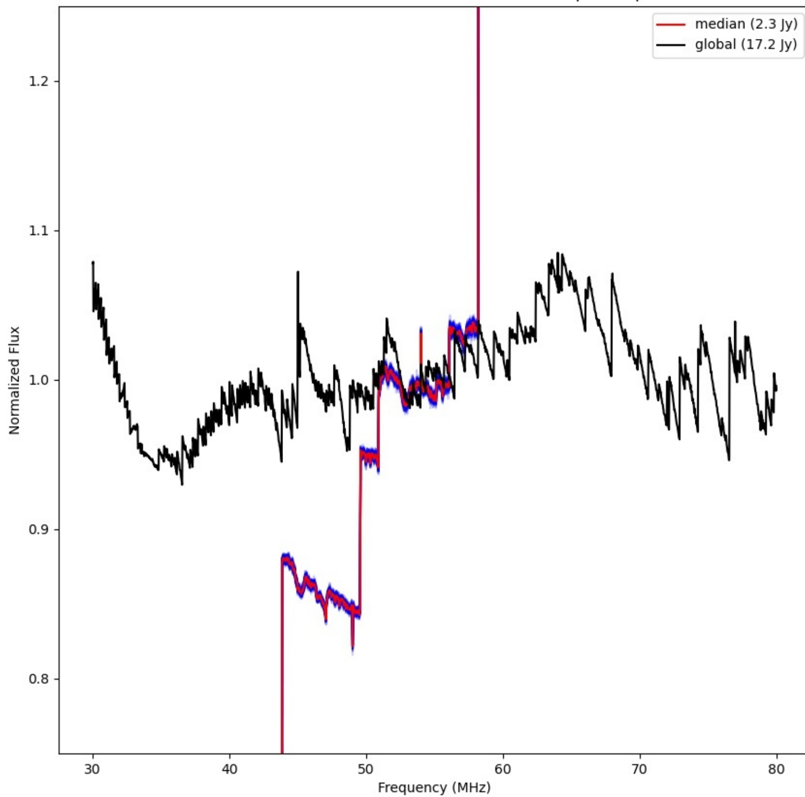
LWA333 - Correlator# 253 - YY - FLAGS:BadSpecShape
