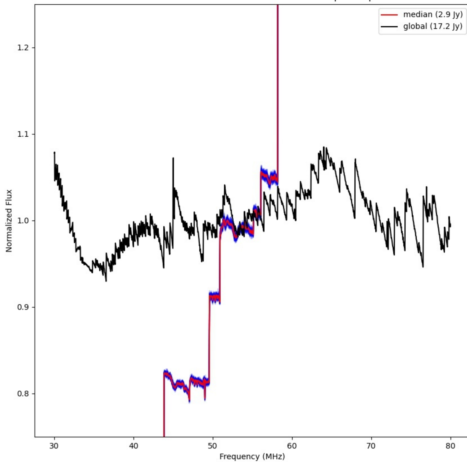
LWA308 - Correlator# 015 - YY - FLAGS:BadSpecShape
