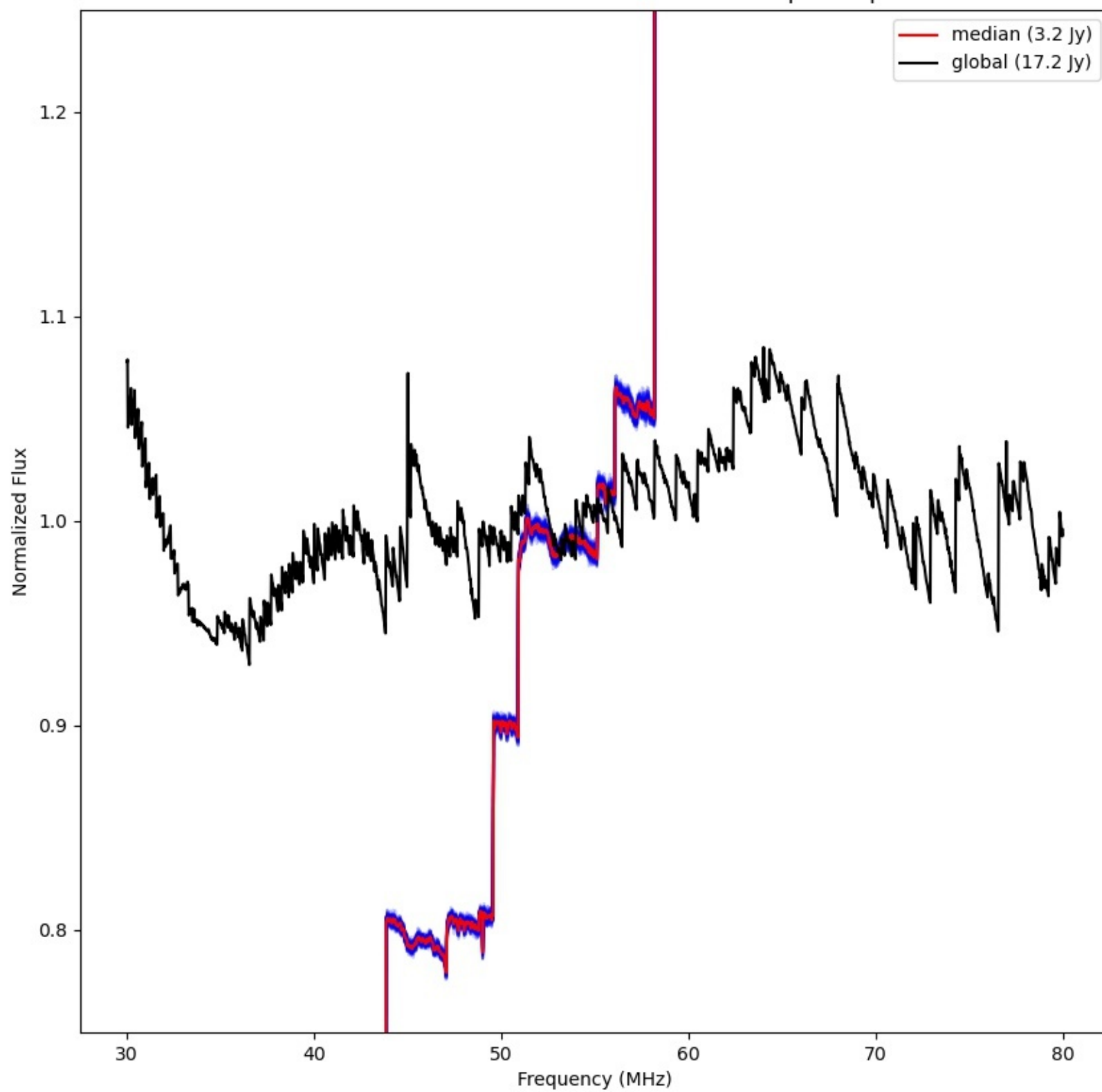
LWA272 - Correlator# 038 - YY - FLAGS:BadSpecShape
