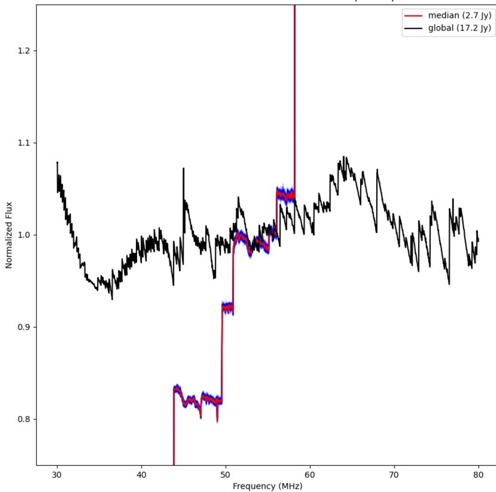
LWA259 - Correlator# 001 - YY - FLAGS:BadSpecShape
