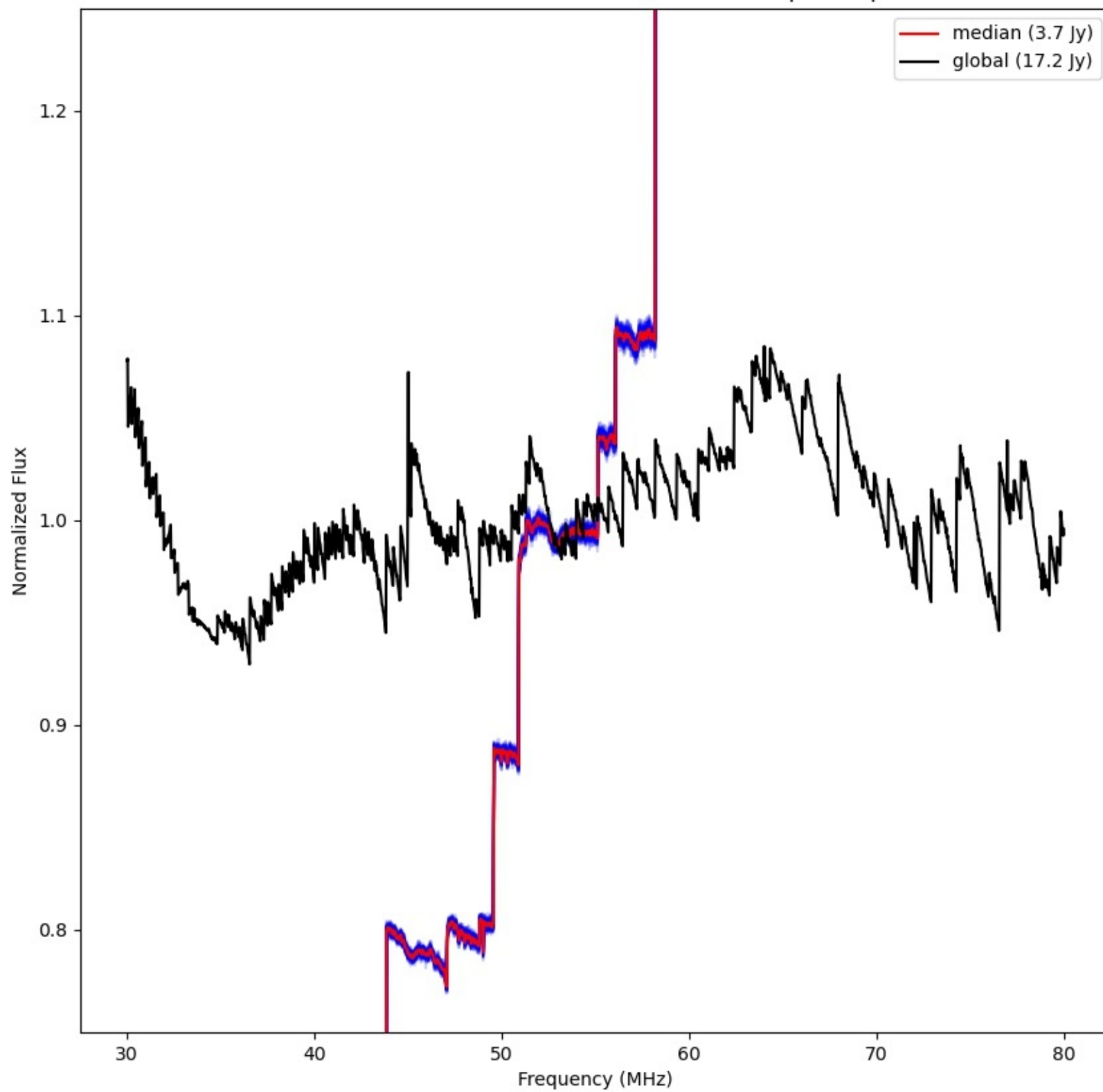
LWA342 - Correlator# 317 - YY - FLAGS:BadSpecShape
