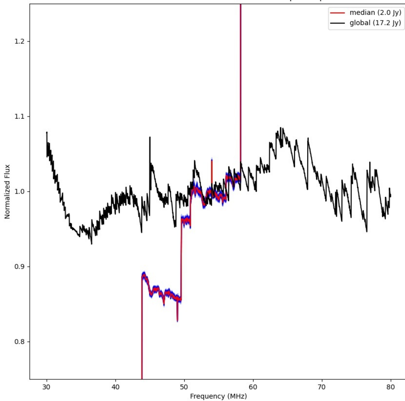
LWA298 - Correlator# 049 - YY - FLAGS:BadSpecShape
