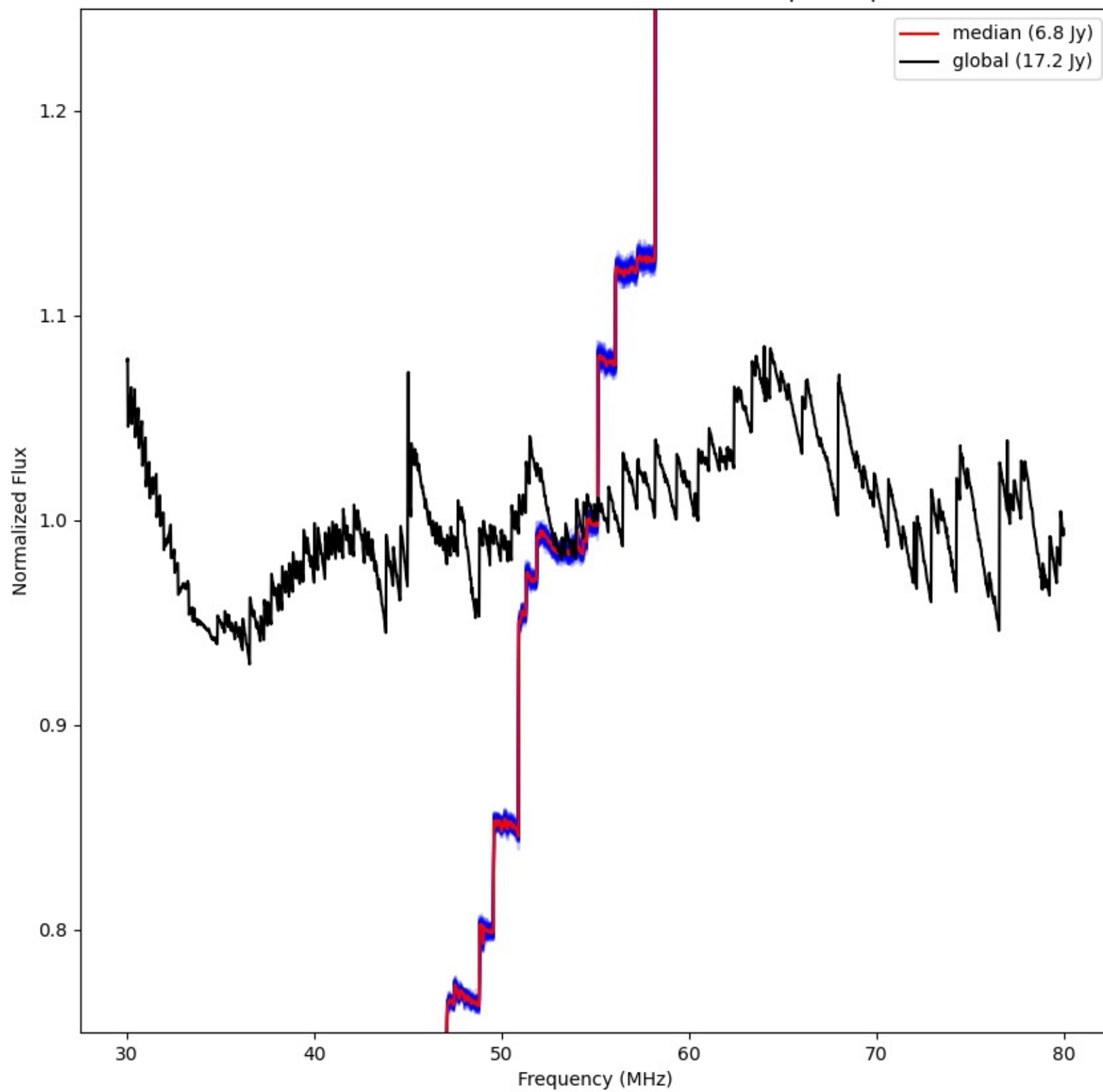
LWA328 - Correlator# 157 - YY - FLAGS:BadSpecShape
