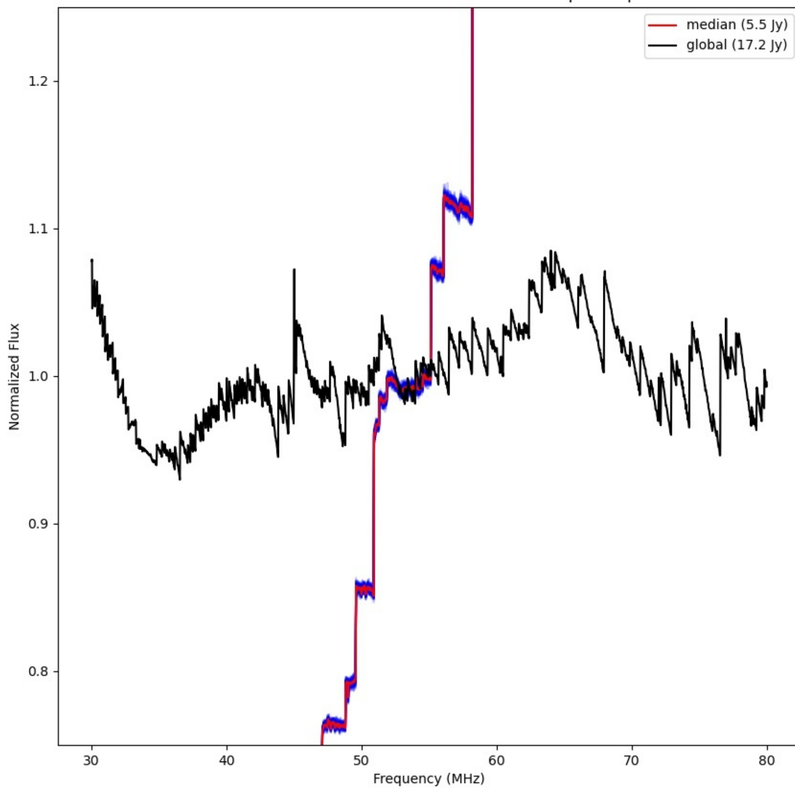
LWA277 - Correlator# 009 - YY - FLAGS:BadSpecShape
