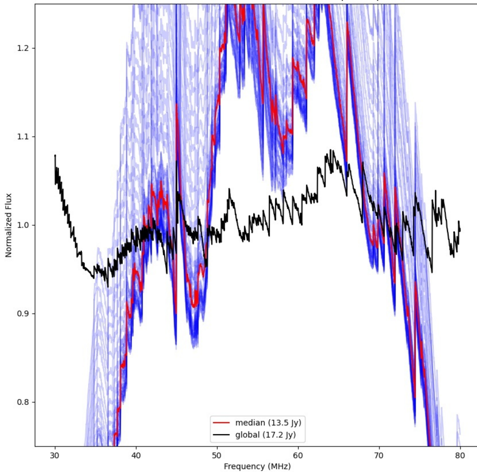
LWA142 - Correlator# 211 - YY - FLAGS:BadSpecShape
