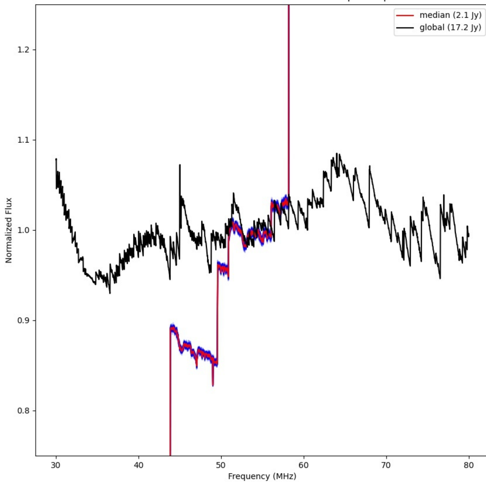
LWA322 - Correlator# 251 - YY - FLAGS:BadSpecShape
