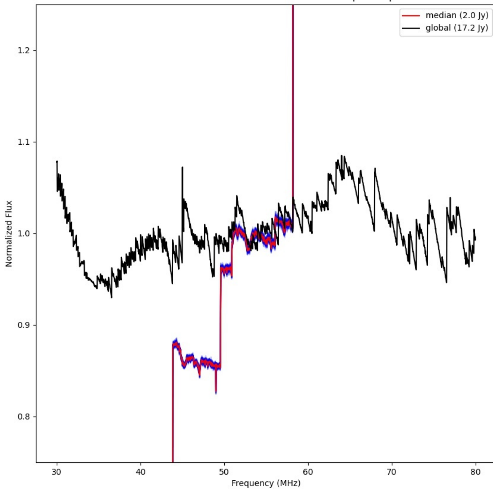
LWA279 - Correlator# 220 - YY - FLAGS:BadSpecShape
