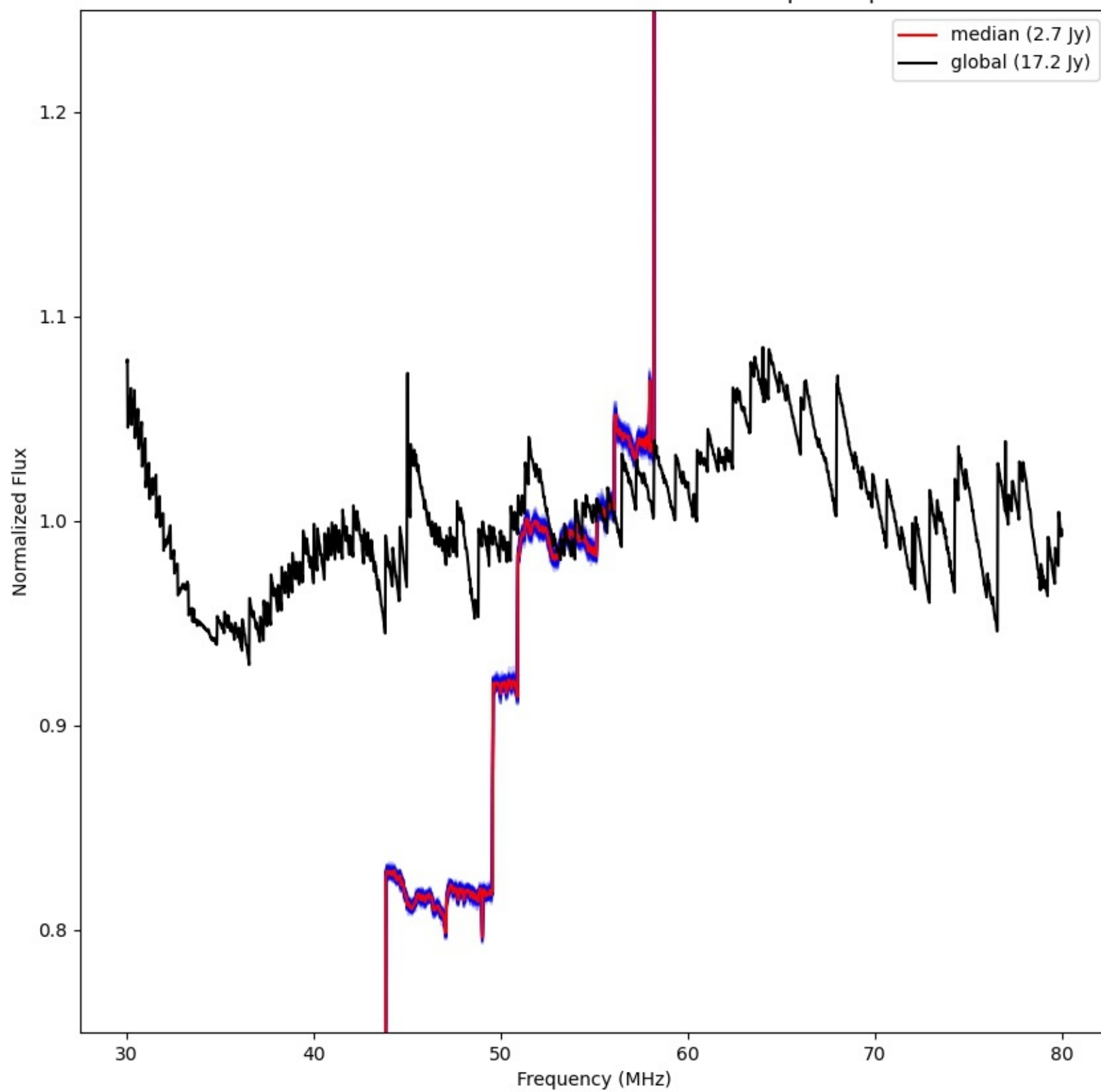
LWA257 - Correlator# 032 - YY - FLAGS:BadSpecShape
