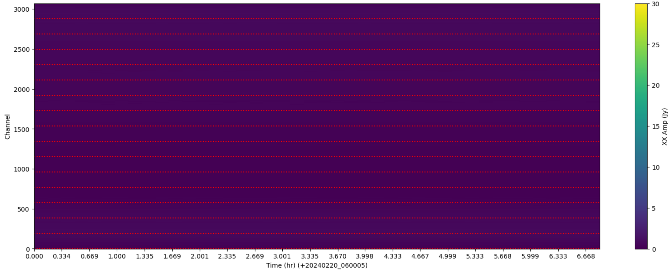
LWA338 - Correlator# 024 - XX - FLAGS: LowFlux
