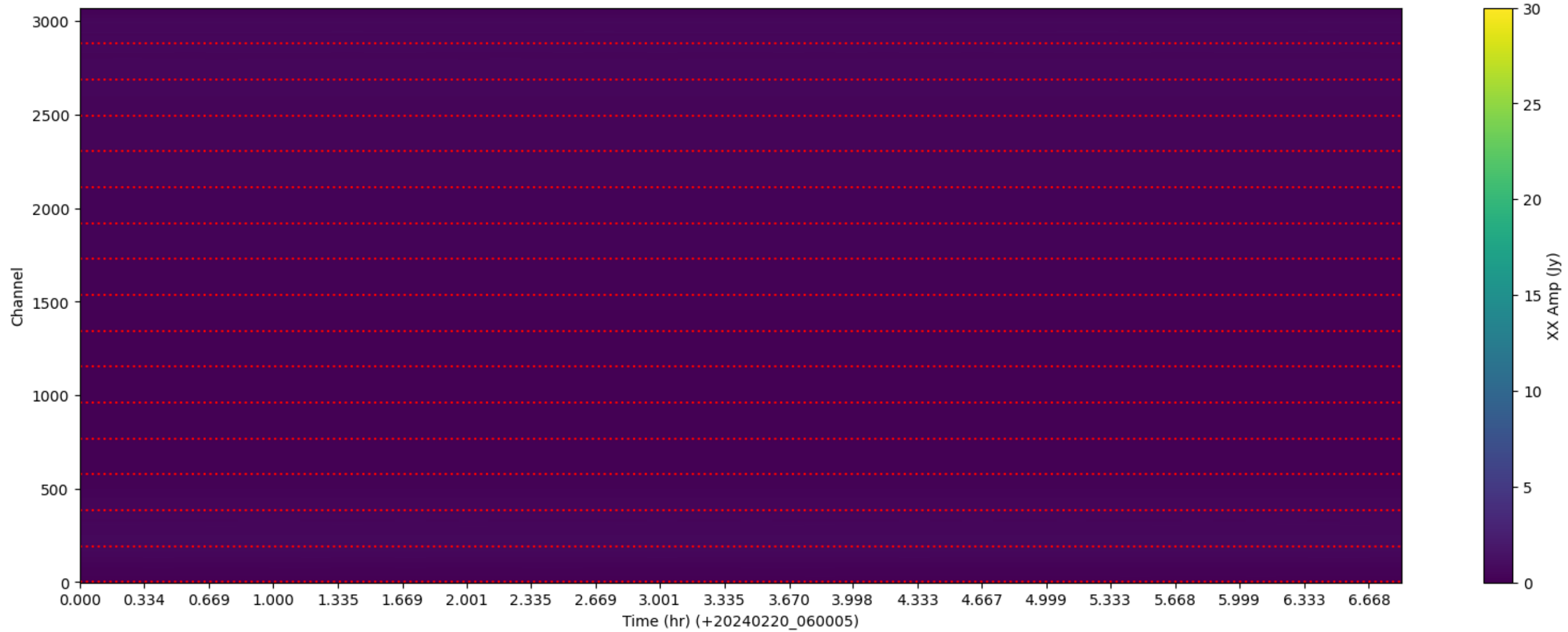
LWA320 - Correlator# 054 - XX - FLAGS: LowFlux
