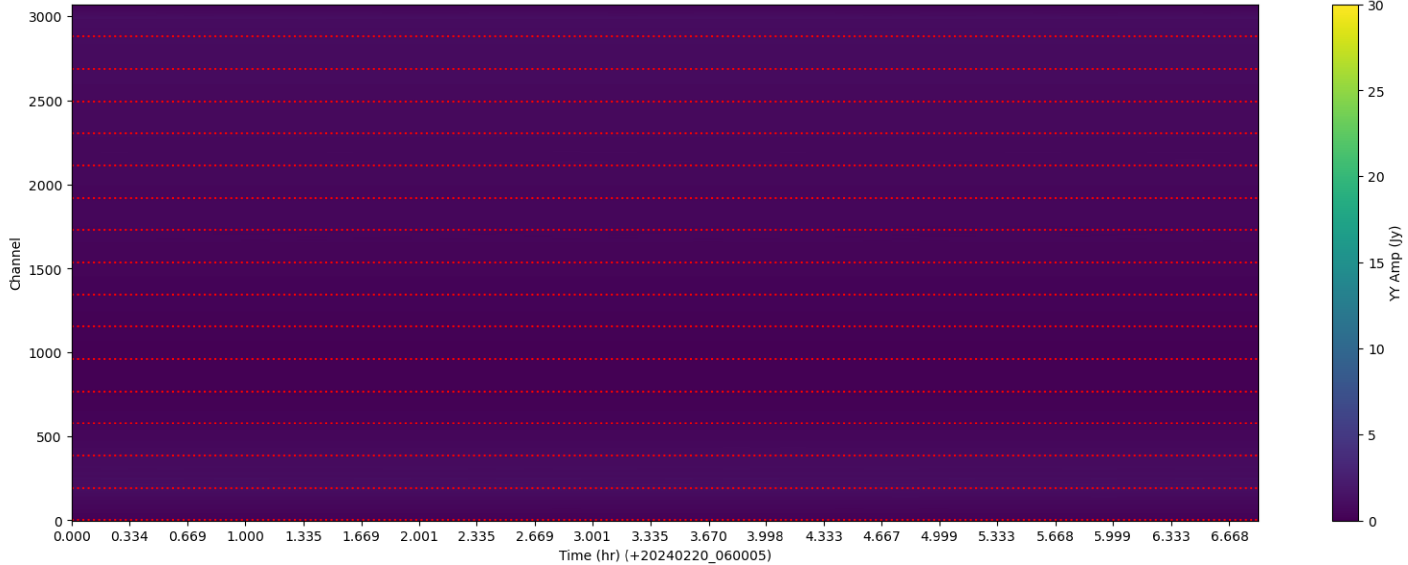
LWA342 - Correlator# 317 - YY - FLAGS: LowFlux
