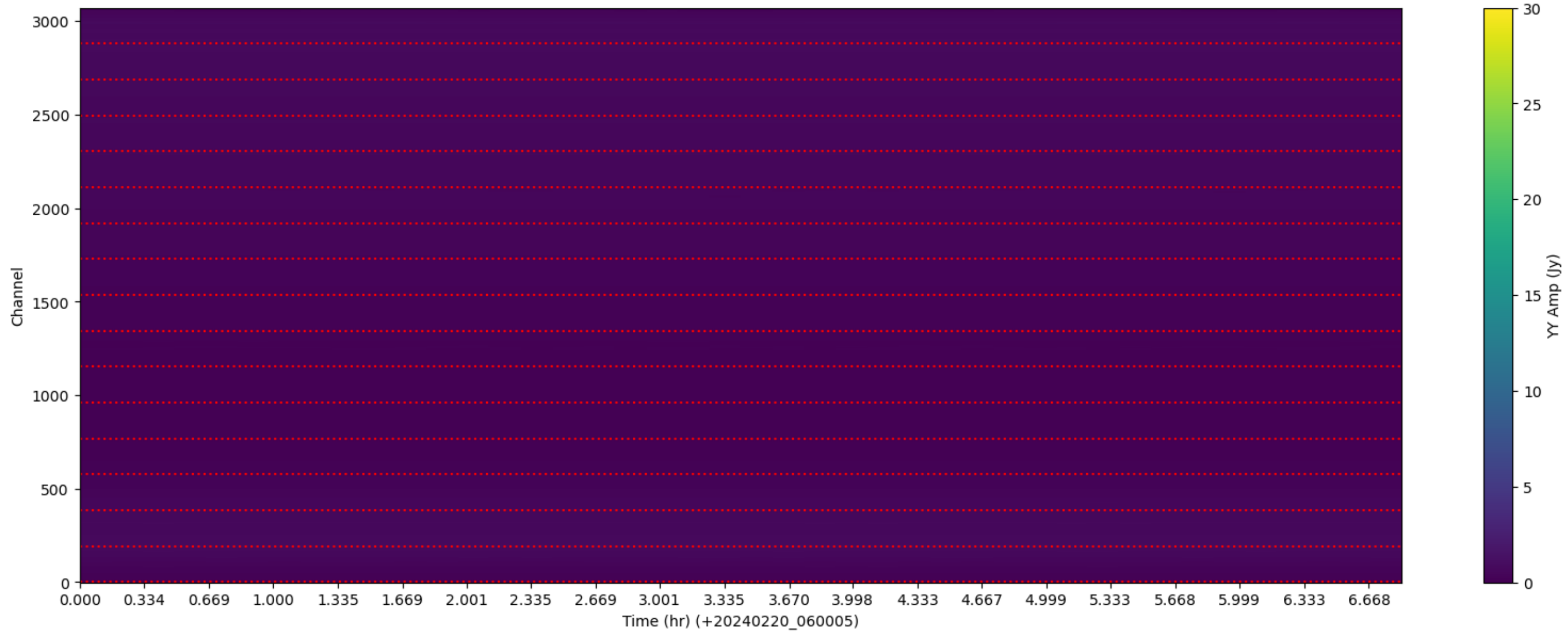
LWA257 - Correlator# 032 - YY - FLAGS: LowFlux
