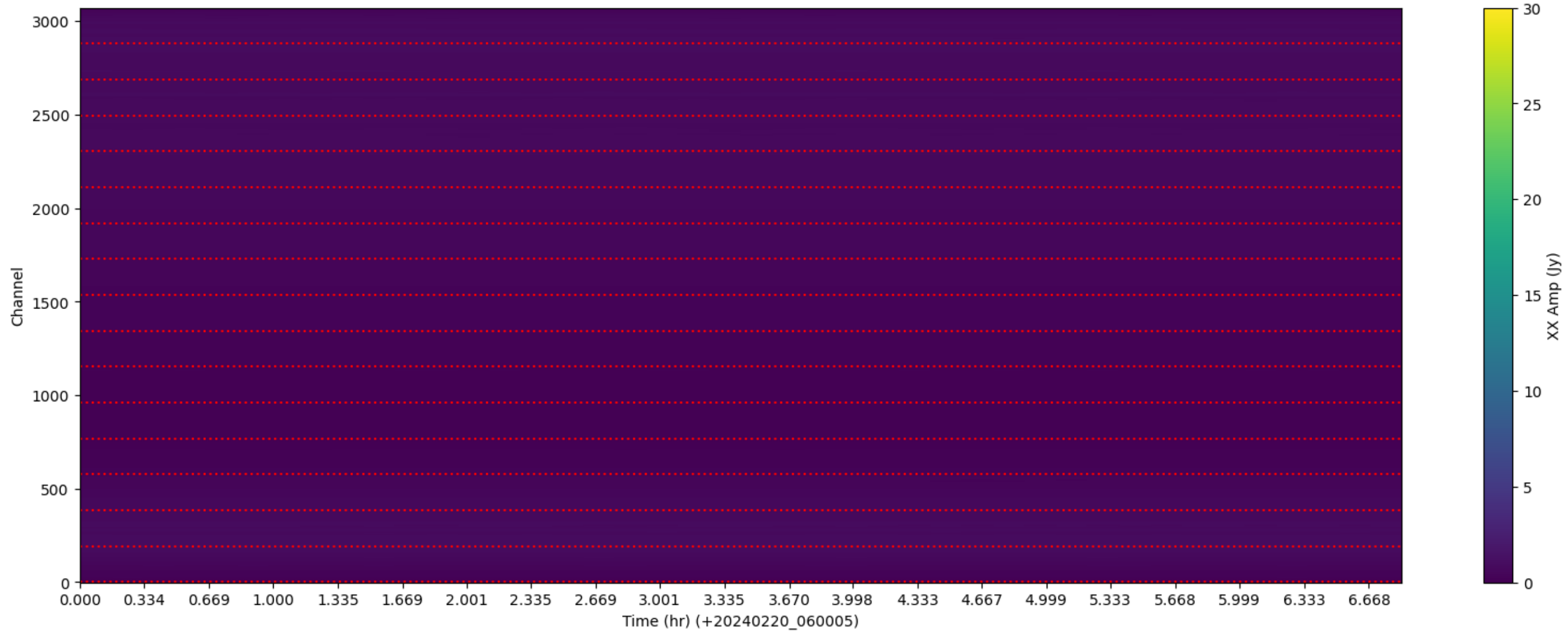
LWA339 - Correlator# 027 - XX - FLAGS: LowFlux
