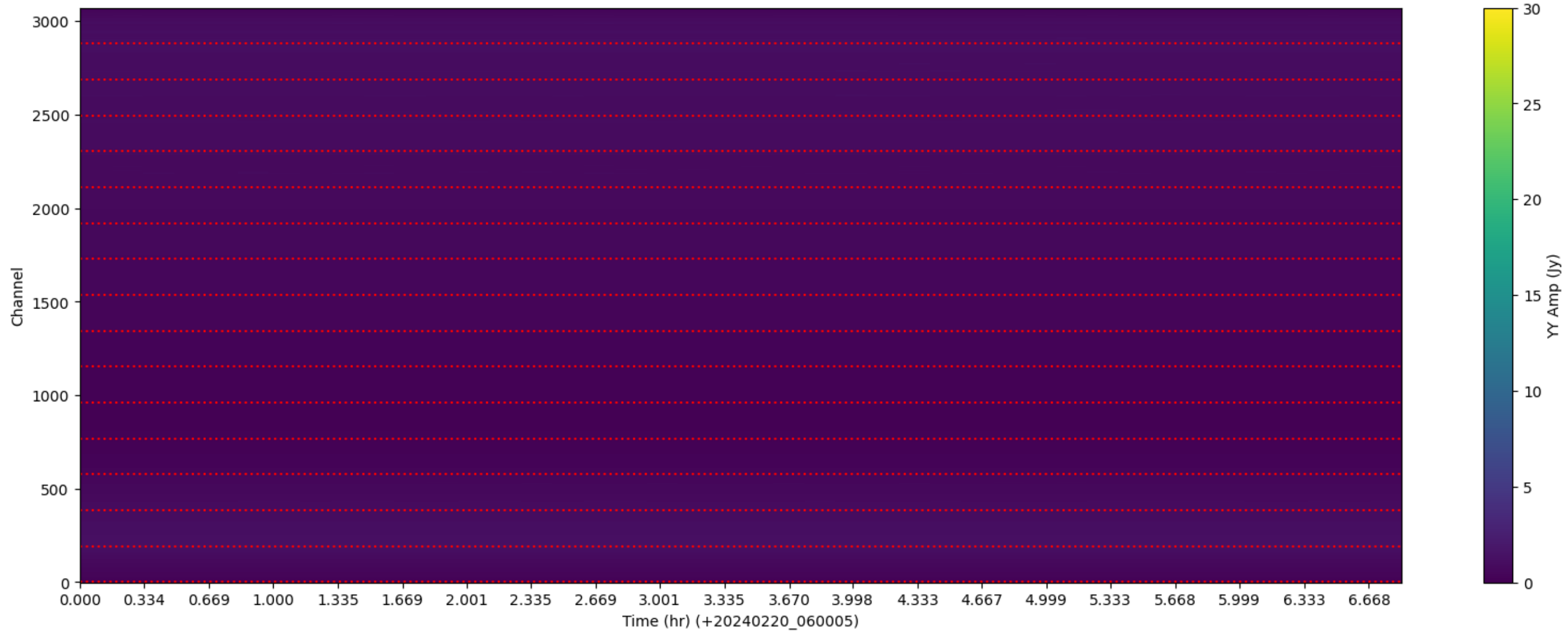
LWA269 - Correlator# 005 - YY - FLAGS: LowFlux
