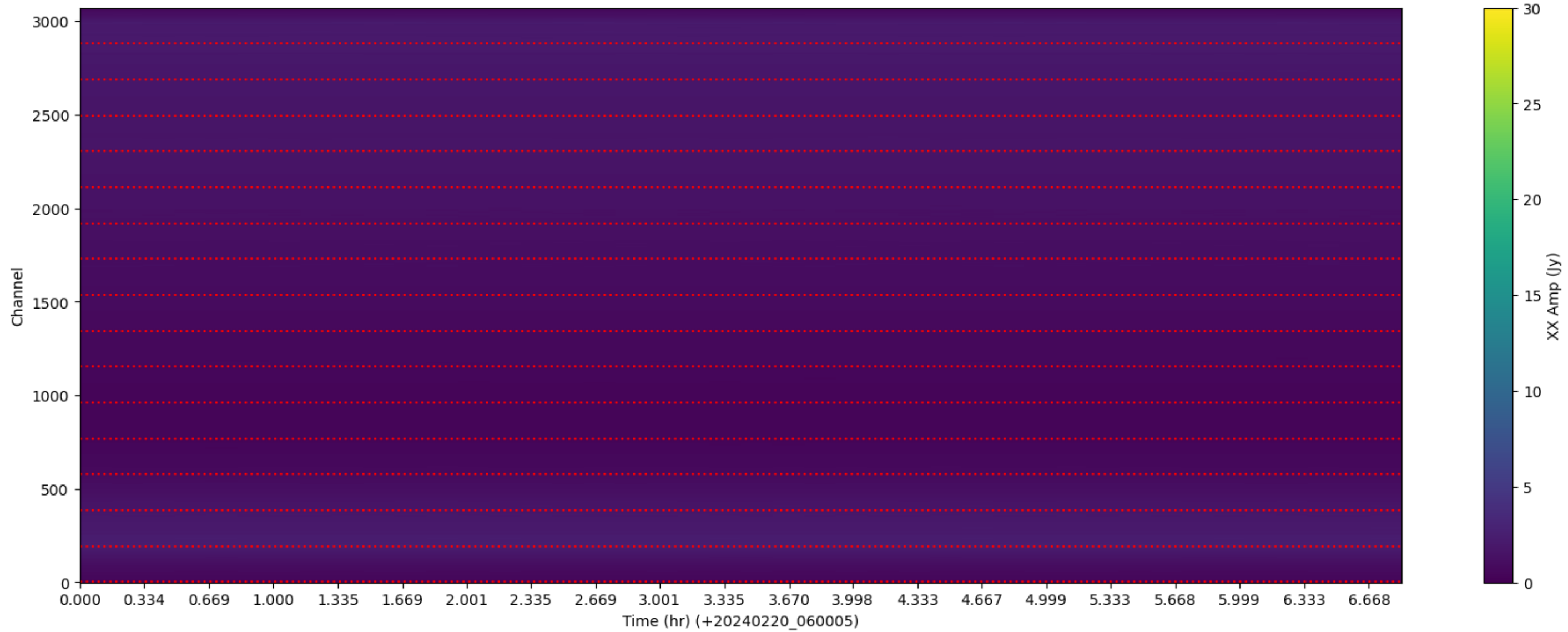
LWA315 - Correlator# 350 - XX - FLAGS: LowFlux
