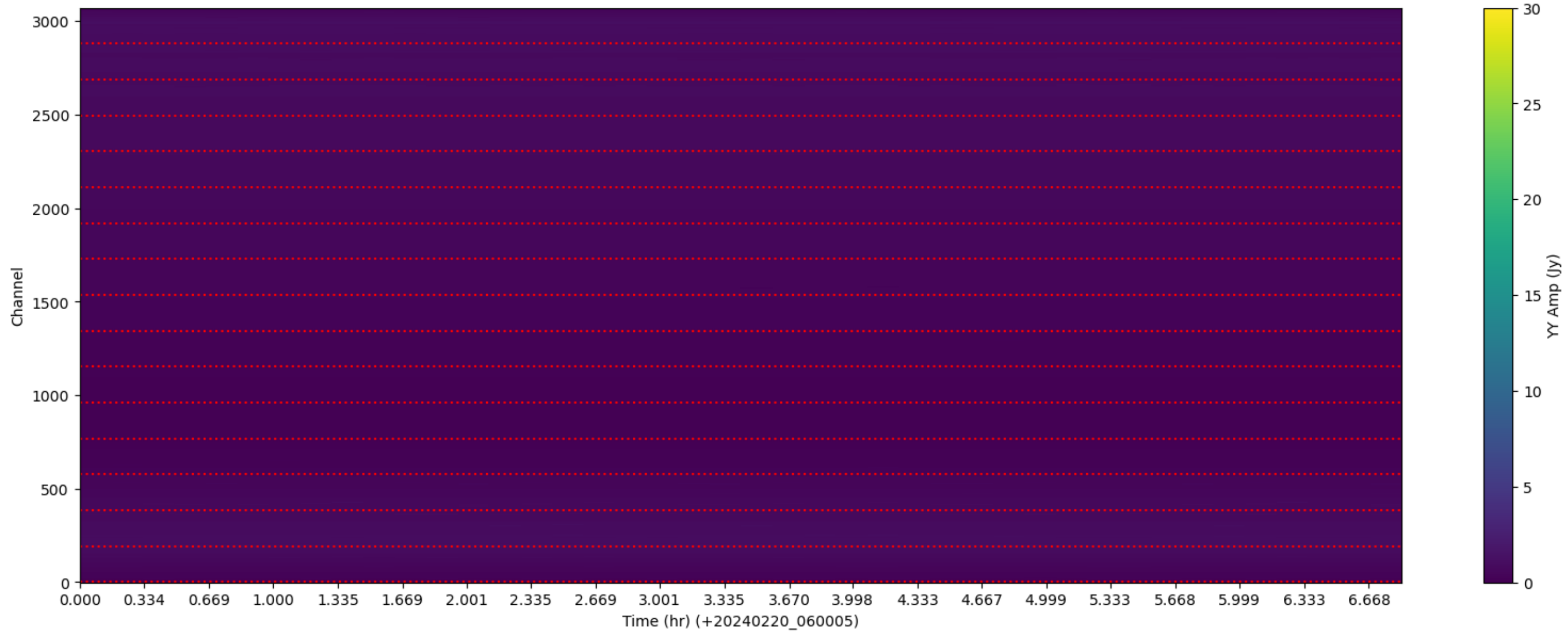
LWA286 - Correlator# 093 - YY - FLAGS: LowFlux
