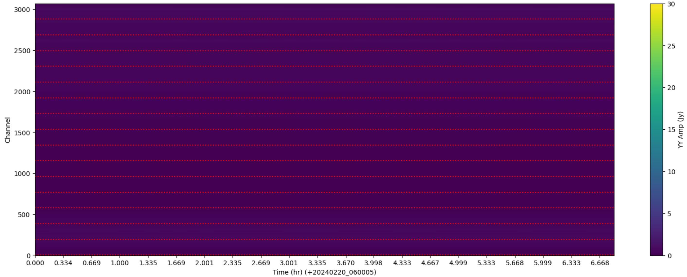
LWA333 - Correlator# 253 - YY - FLAGS: LowFlux
