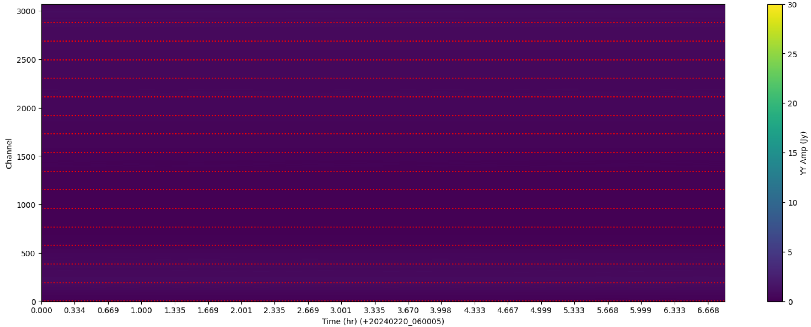
LWA338 - Correlator# 024 - YY - FLAGS: LowFlux
