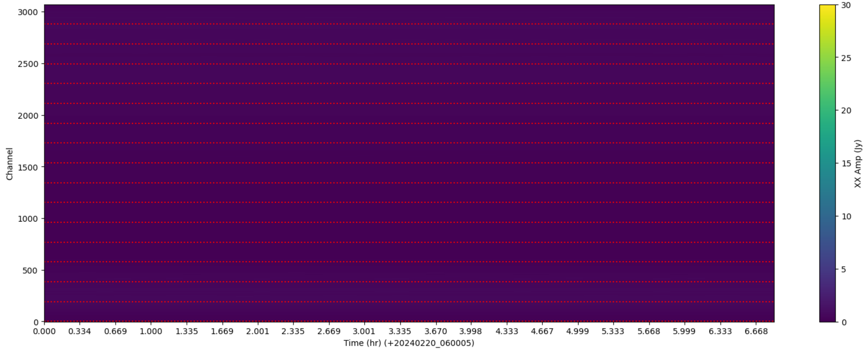
LWA329 - Correlator# 287 - XX - FLAGS: LowFlux
