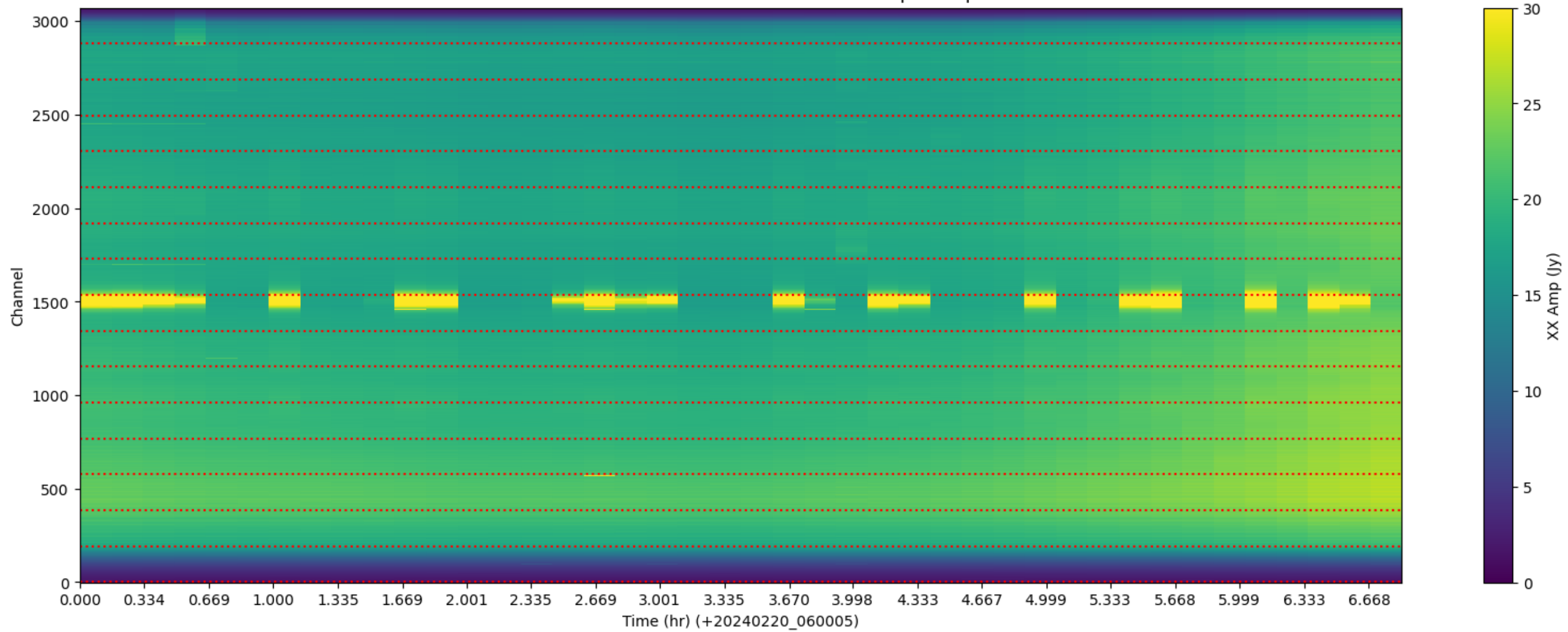
LWA012 - Correlator# 074 - XX - FLAGS: BadSpecShape
