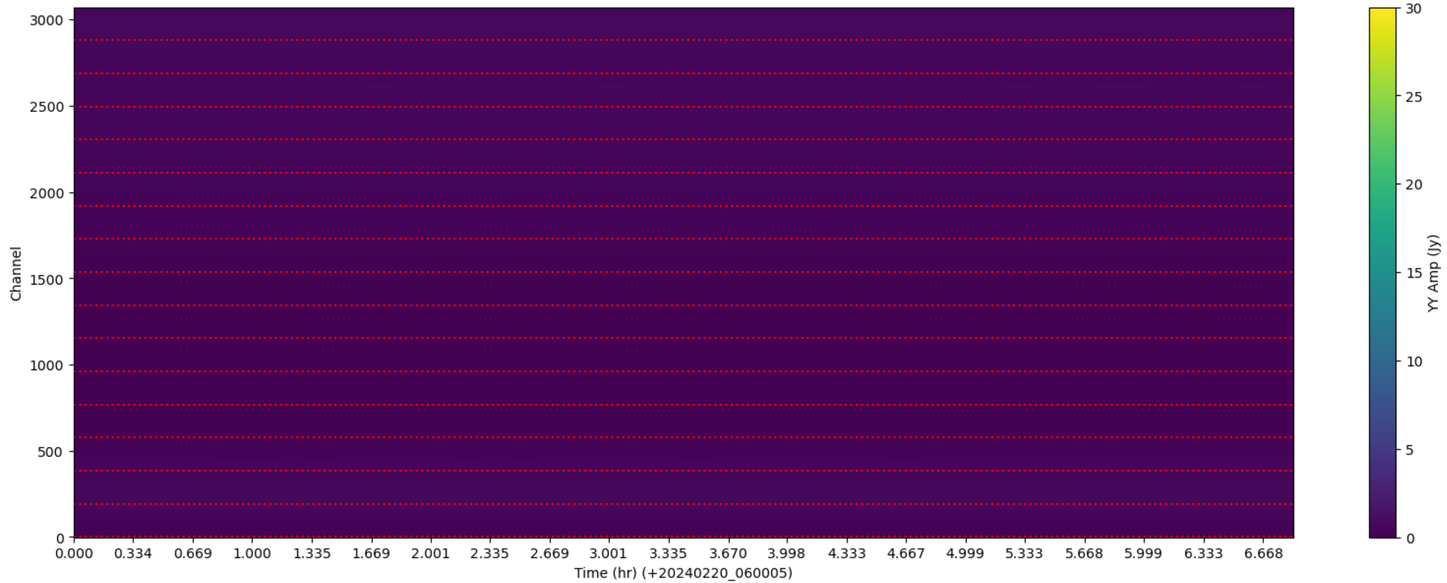
LWA297 - Correlator# 314 - YY - FLAGS: LowFlux
