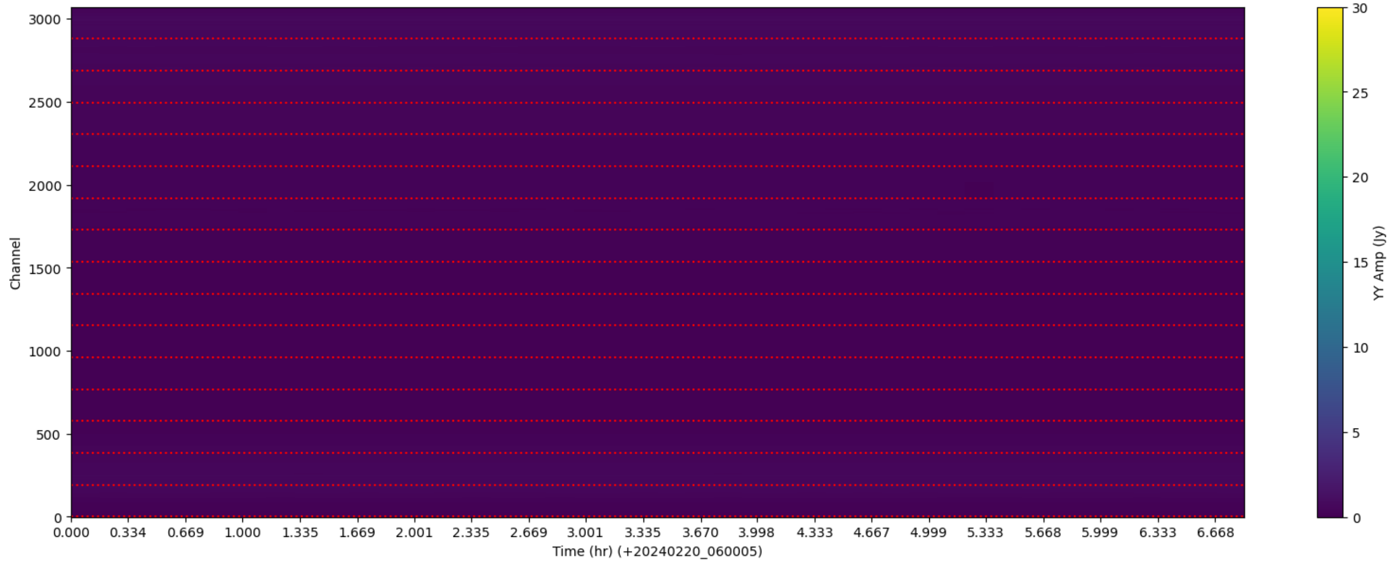
LWA298 - Correlator# 049 - YY - FLAGS: LowFlux
