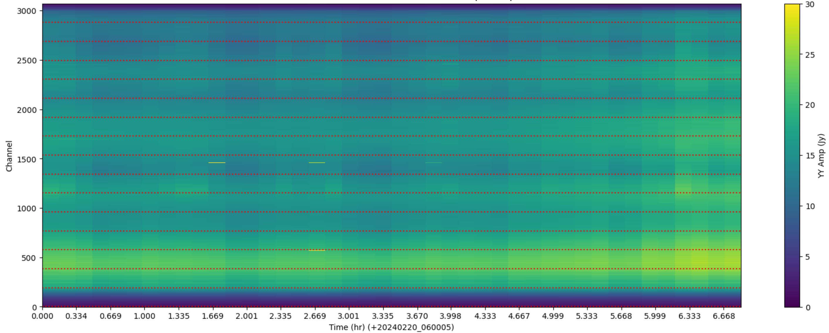
LWA120 - Correlator# 208 - YY - FLAGS: BadSpecShape
