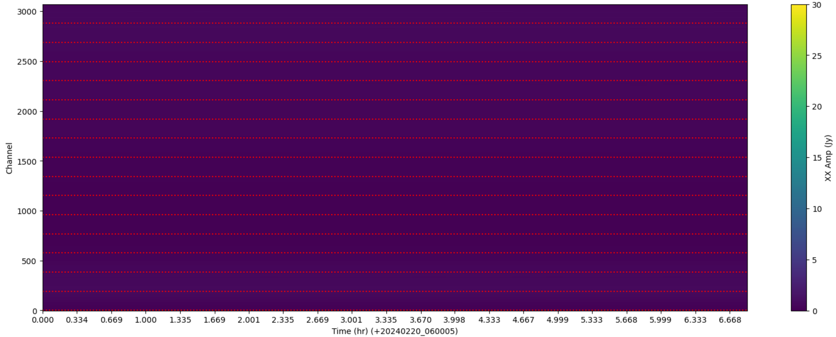
LWA330 - Correlator# 022 - XX - FLAGS: LowFlux
