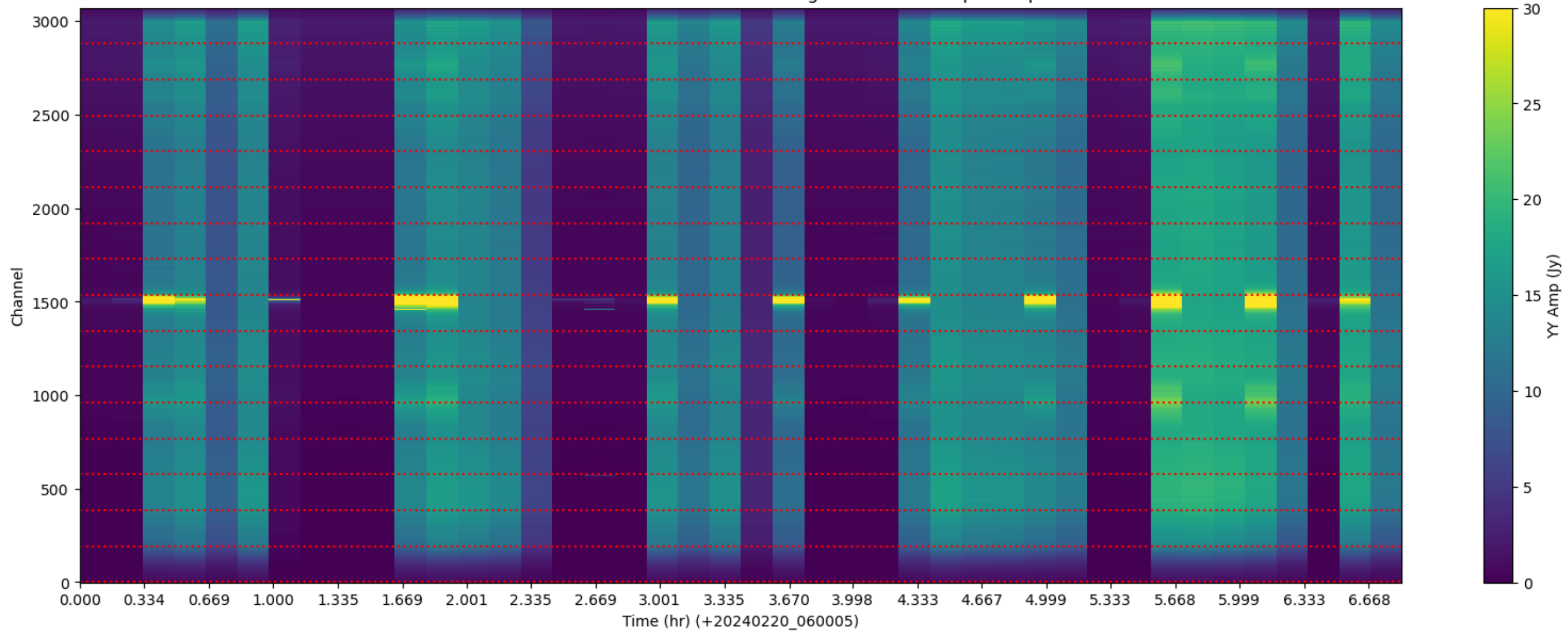
LWA009 - Correlator# 070 - YY - FLAGS: HighTimeVar+BadSpecShape
