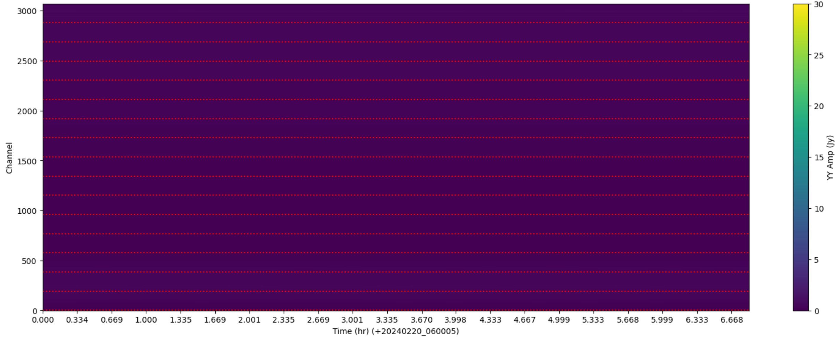
LWA289 - Correlator# 189 - YY - FLAGS: LowFlux
