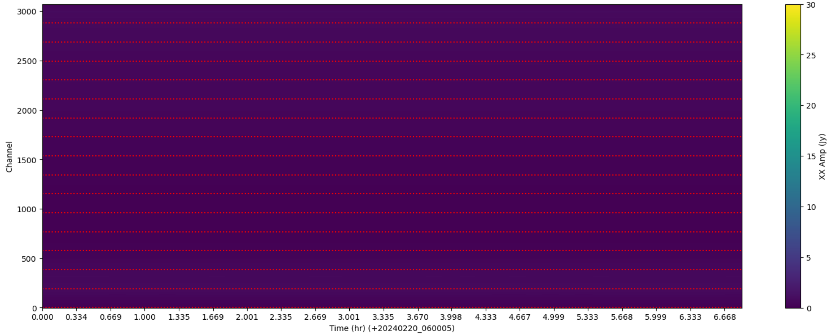
LWA283 - Correlator# 040 - XX - FLAGS: LowFlux
