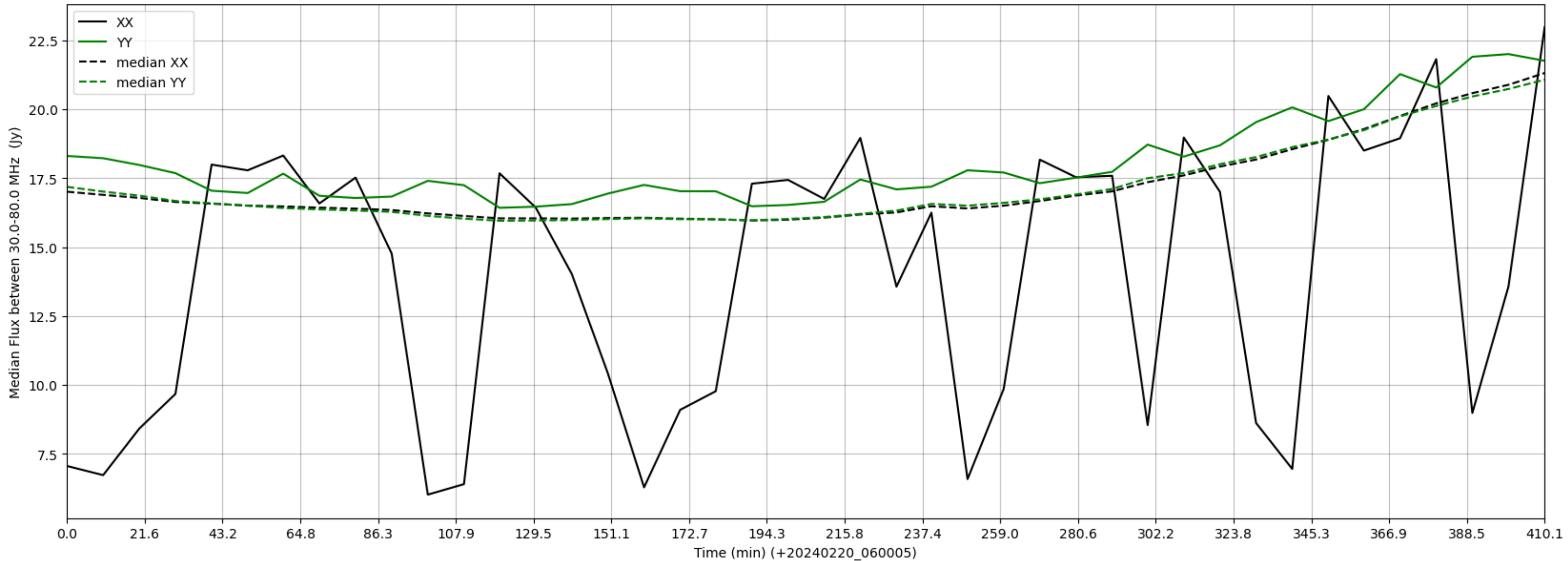
LWA041 - Correlator# 079 - XX FLAGS:HighTimeVar+BadSpecShape - YY FLAGS:BadSpecShape
