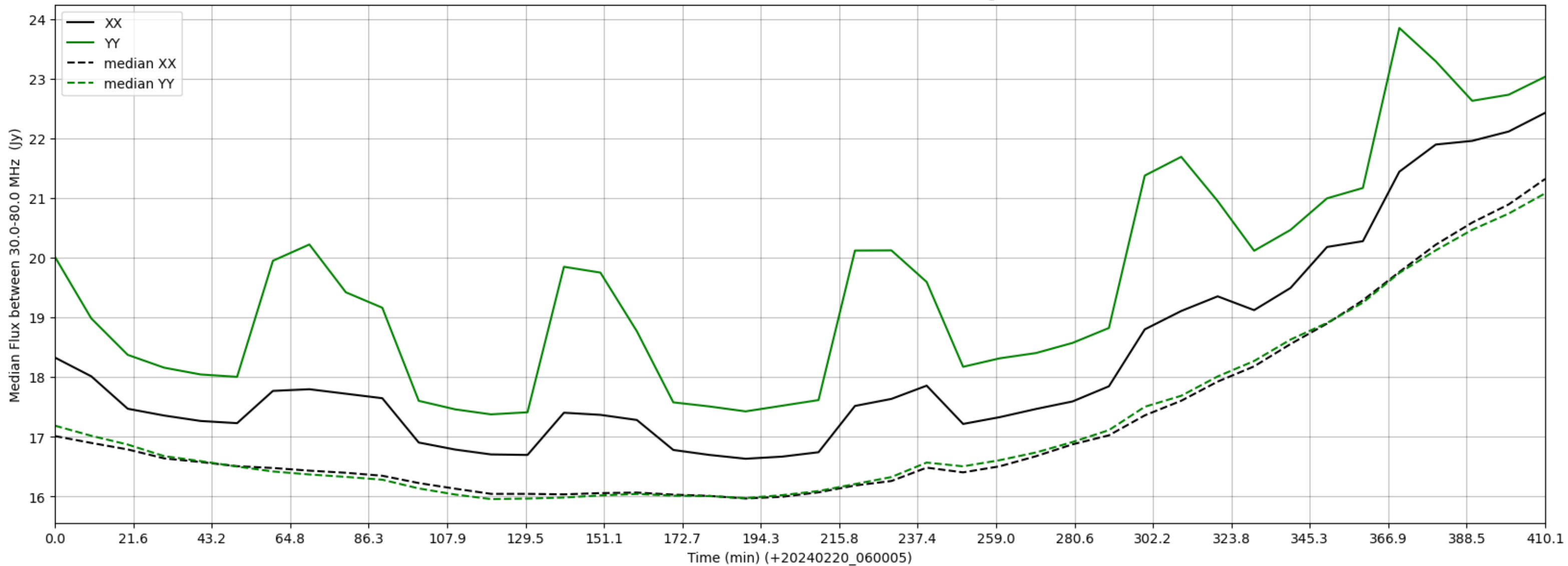
LWA037 - Correlator# 181 - XX FLAGS:Good - YY FLAGS:HighTimeVar
