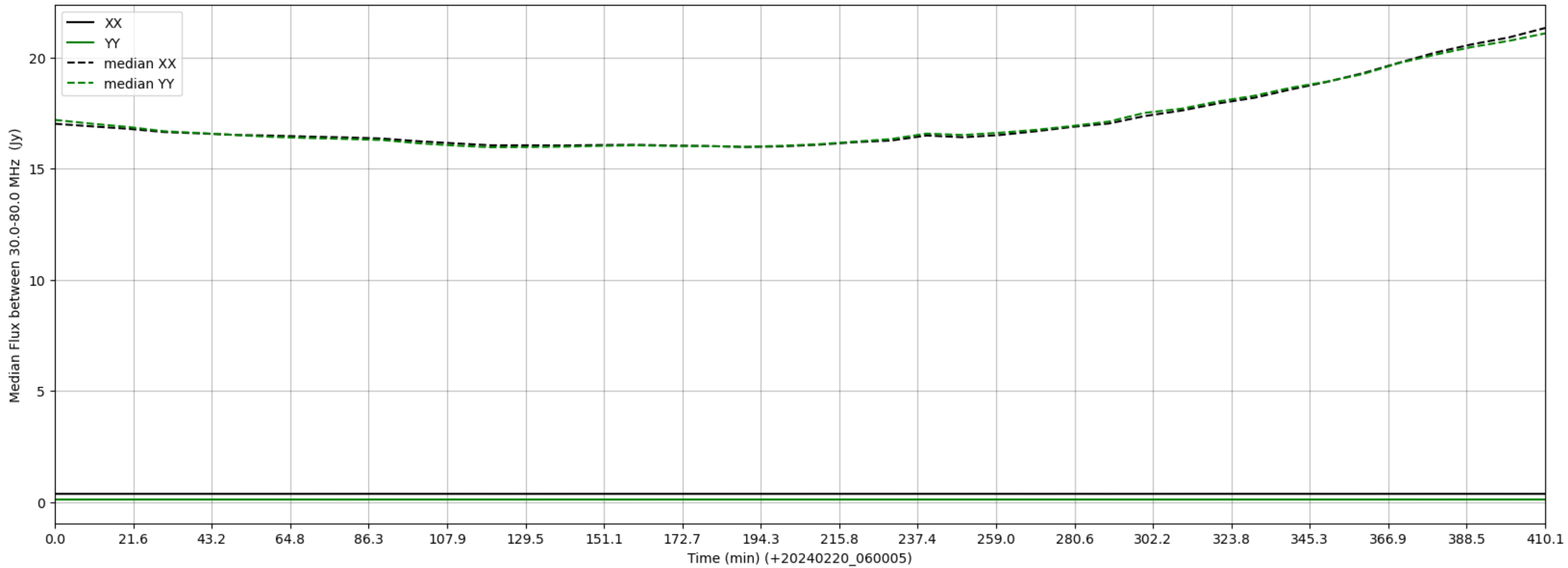
LWA316 - Correlator# 155 - XX FLAGS:LowFlux - YY FLAGS:LowFlux
