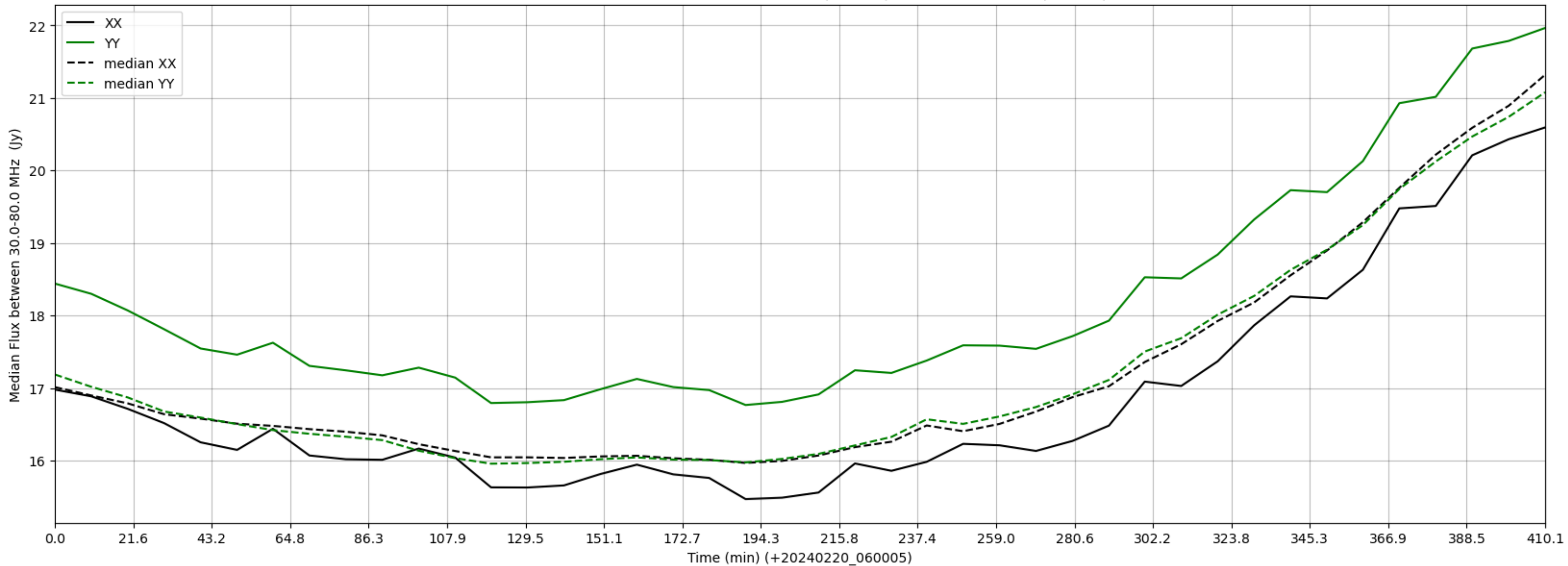
LWA011 - Correlator# 072 - XX FLAGS:BadSpecShape - YY FLAGS:BadSpecShape
