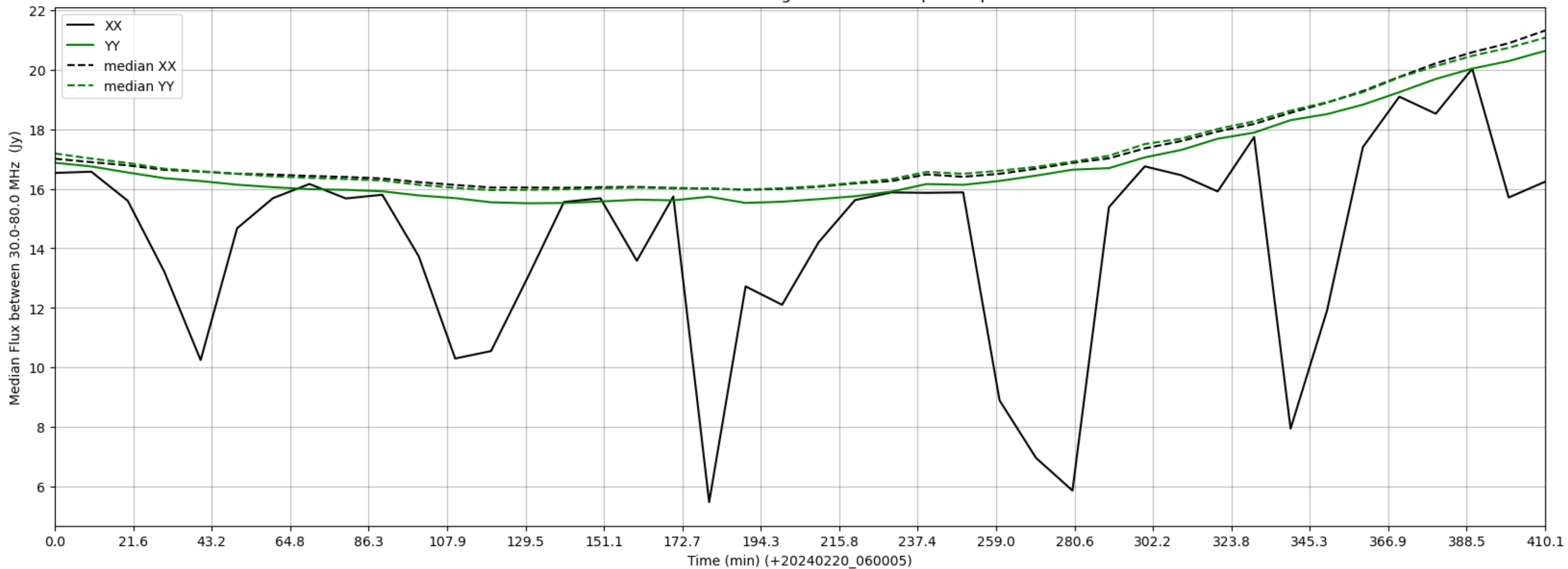
LWA209 - Correlator# 301 - XX FLAGS:HighTimeVar+BadSpecShape - YY FLAGS:Good
