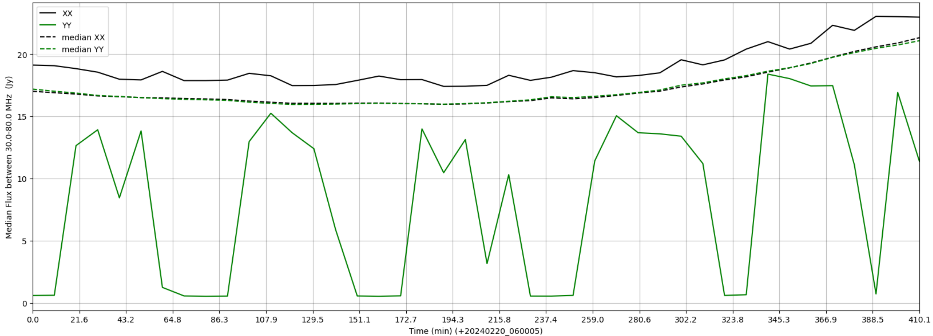
LWA009 - Correlator# 070 - XX FLAGS:BadSpecShape - YY FLAGS:HighTimeVar+BadSpecShape
