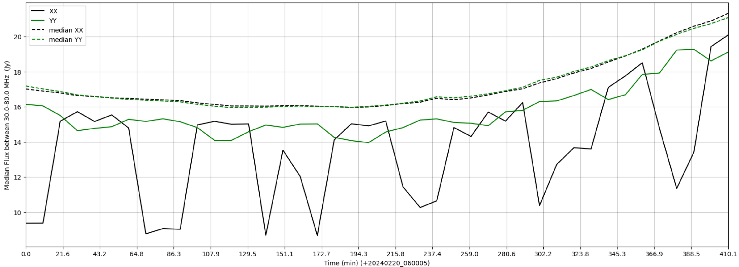
LWA120 - Correlator# 208 - XX FLAGS:HighTimeVar - YY FLAGS:BadSpecShape
