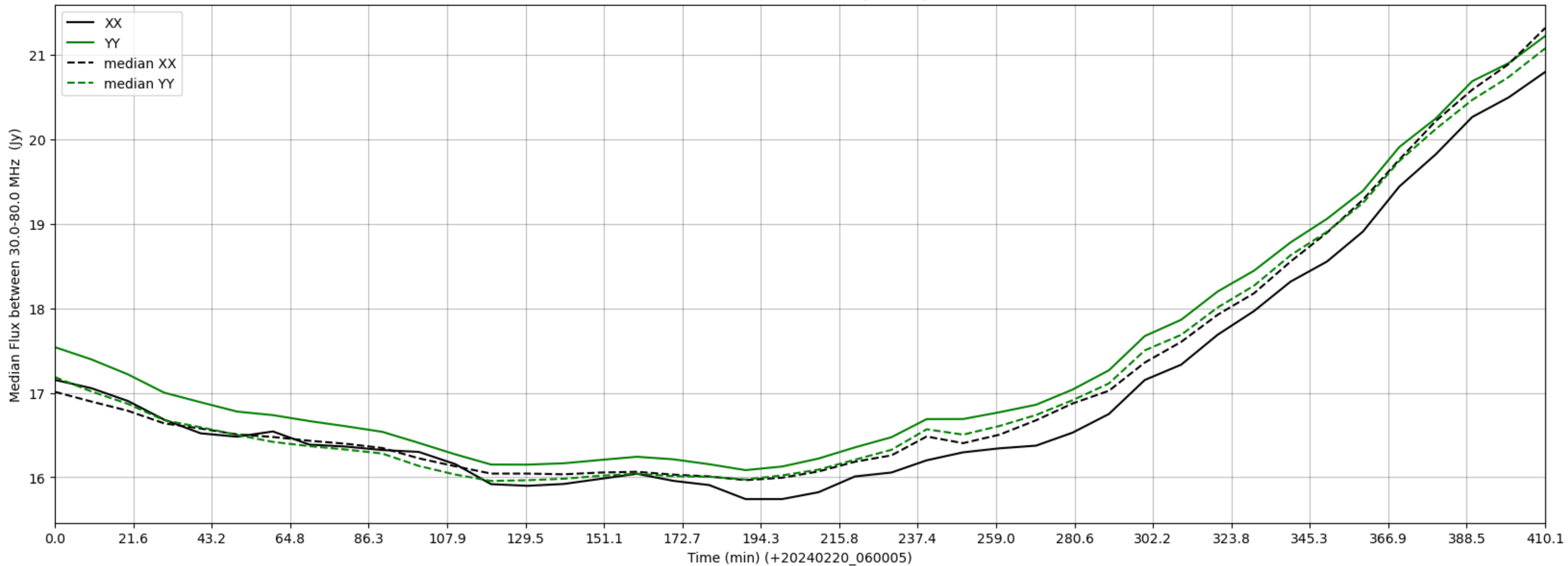
LWA074 - Correlator# 086 - XX FLAGS:BadSpecShape - YY FLAGS:Good
