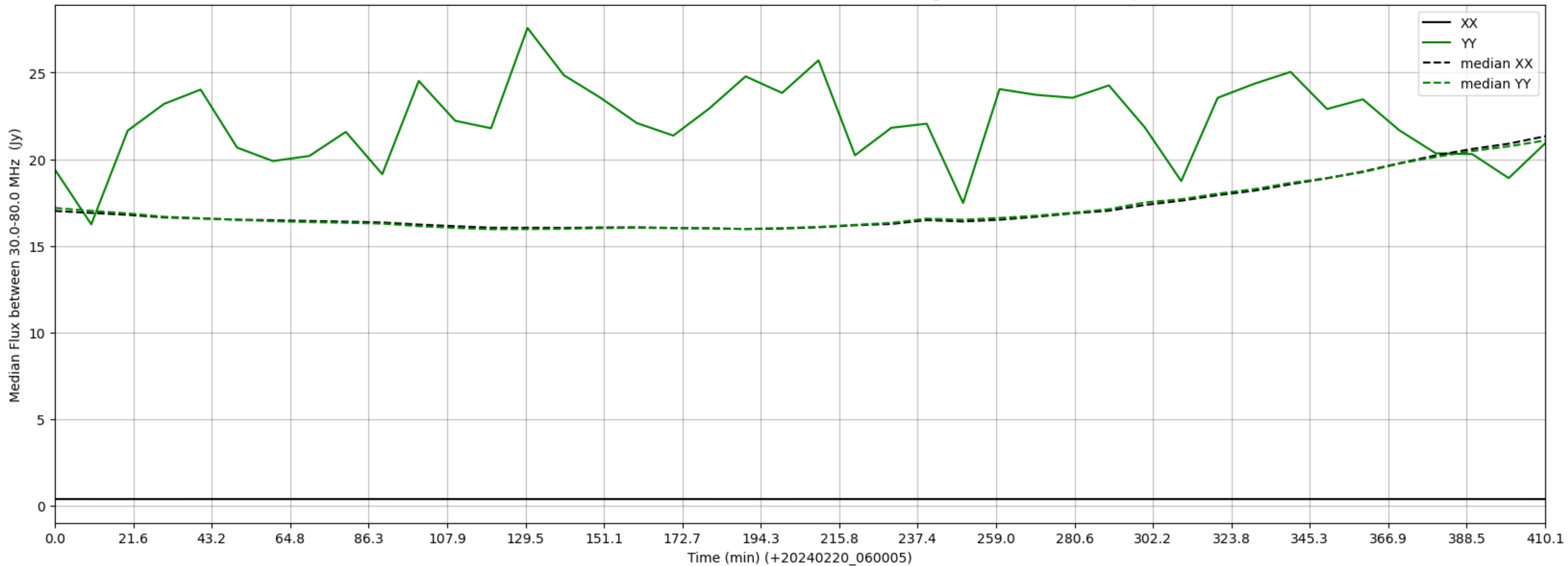
LWA288 - Correlator# 042 - XX FLAGS:LowFlux - YY FLAGS:HighTimeVar+BadSpecShape
