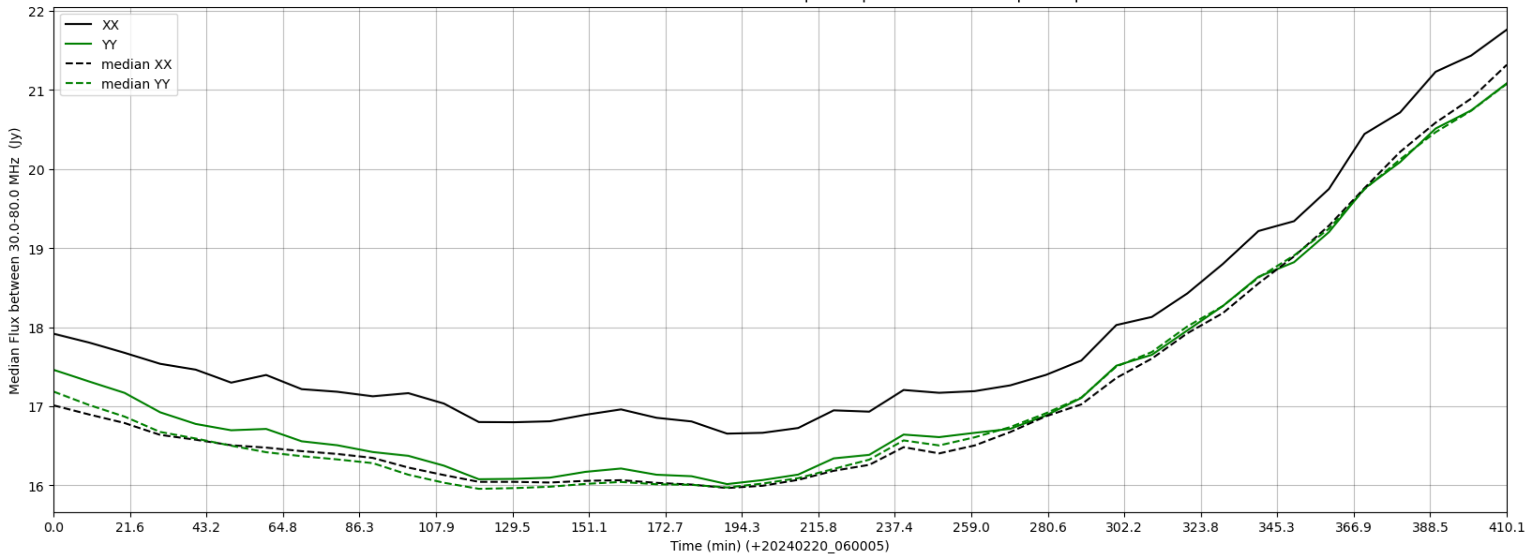
LWA004 - Correlator# 066 - XX FLAGS:BadSpecShape - YY FLAGS:BadSpecShape
