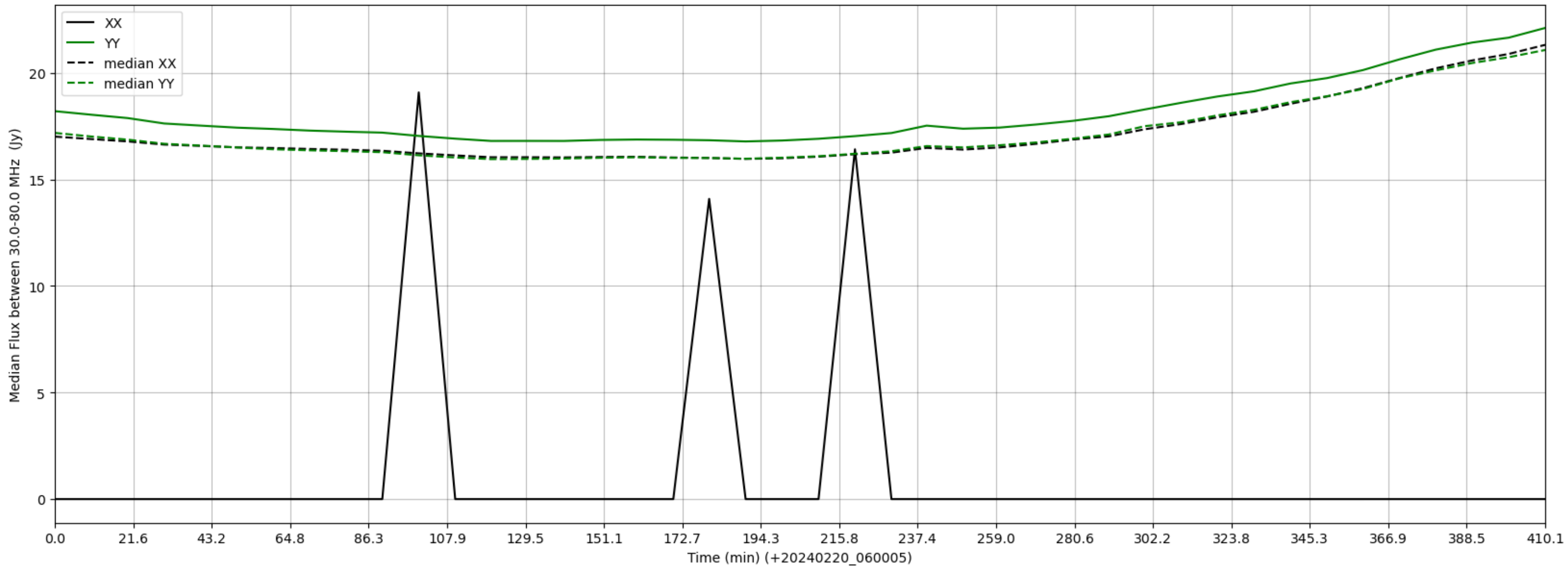
LWA255 - Correlator# 033 - XX FLAGS:LowFlux - YY FLAGS:Good
