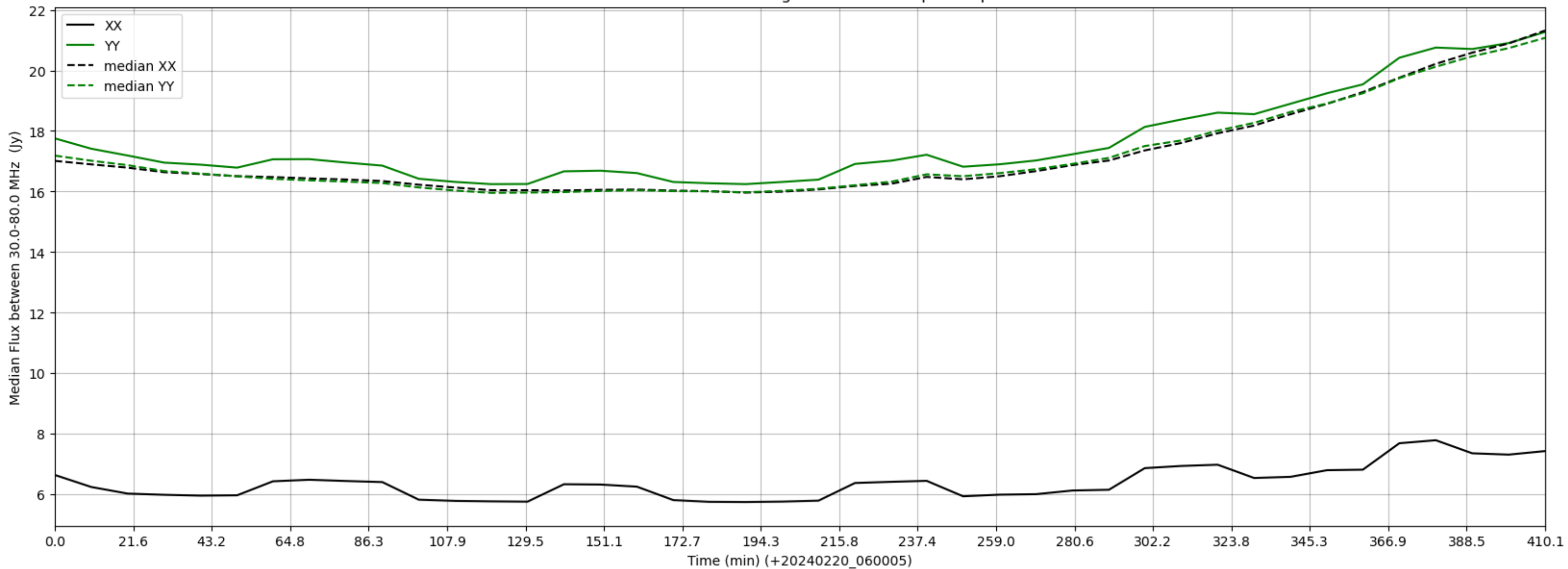
LWA130 - Correlator# 183 - XX FLAGS:HighTimeVar+BadSpecShape - YY FLAGS:Good
