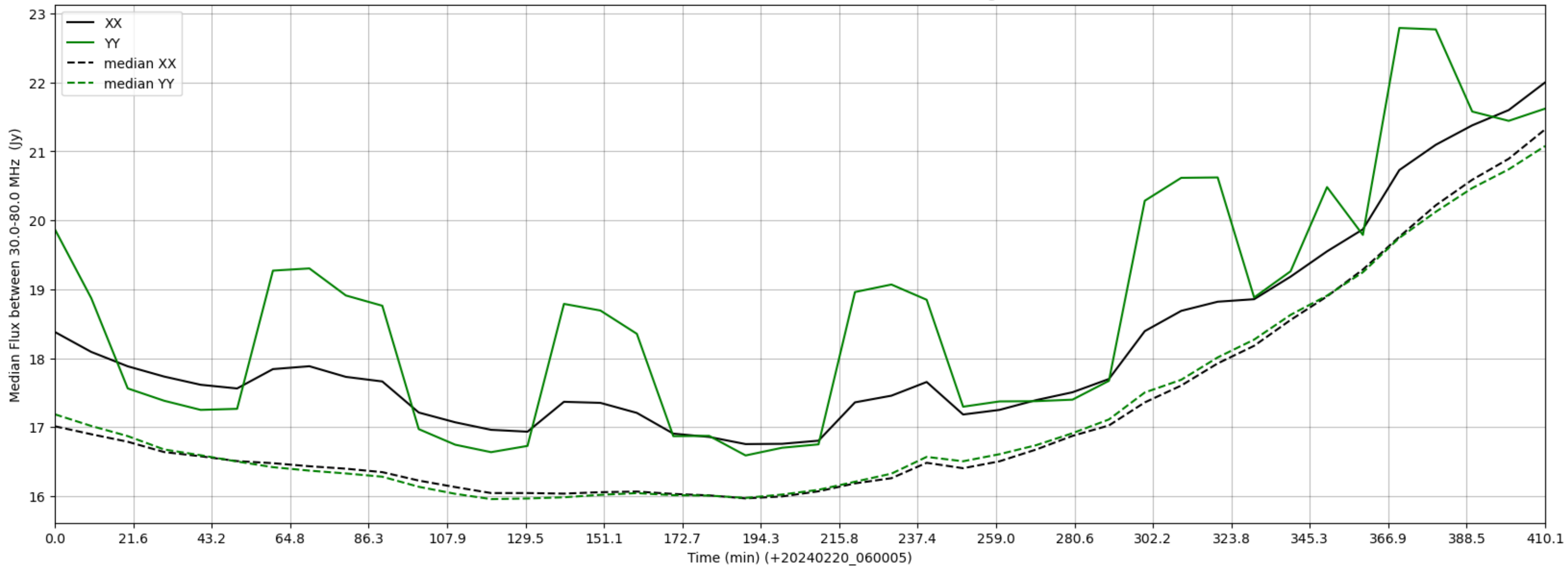
LWA104 - Correlator# 179 - XX FLAGS:Good - YY FLAGS:HighTimeVar
