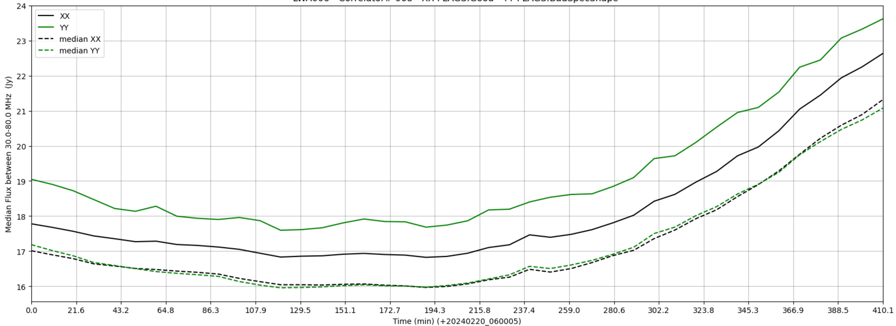
LWA006 - Correlator# 068 - XX FLAGS:Good - YY FLAGS:BadSpecShape
