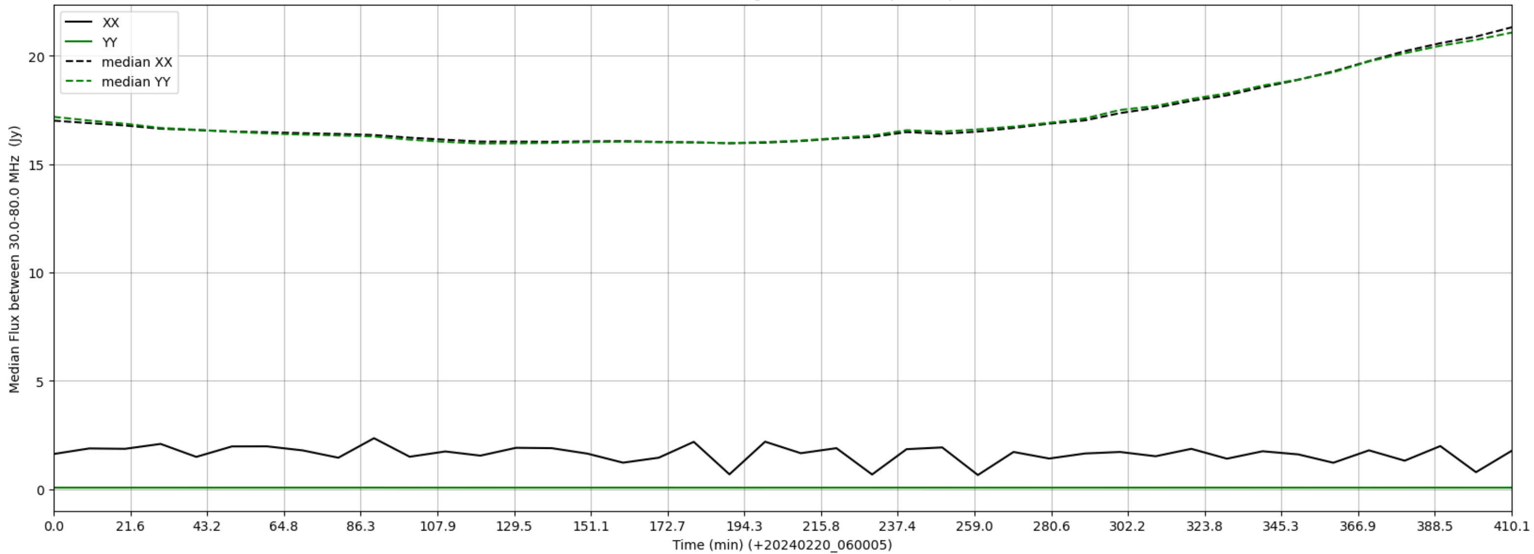
LWA353 - Correlator# 031 - XX FLAGS:HighTimeVar+BadSpecShape - YY FLAGS:LowFlux
