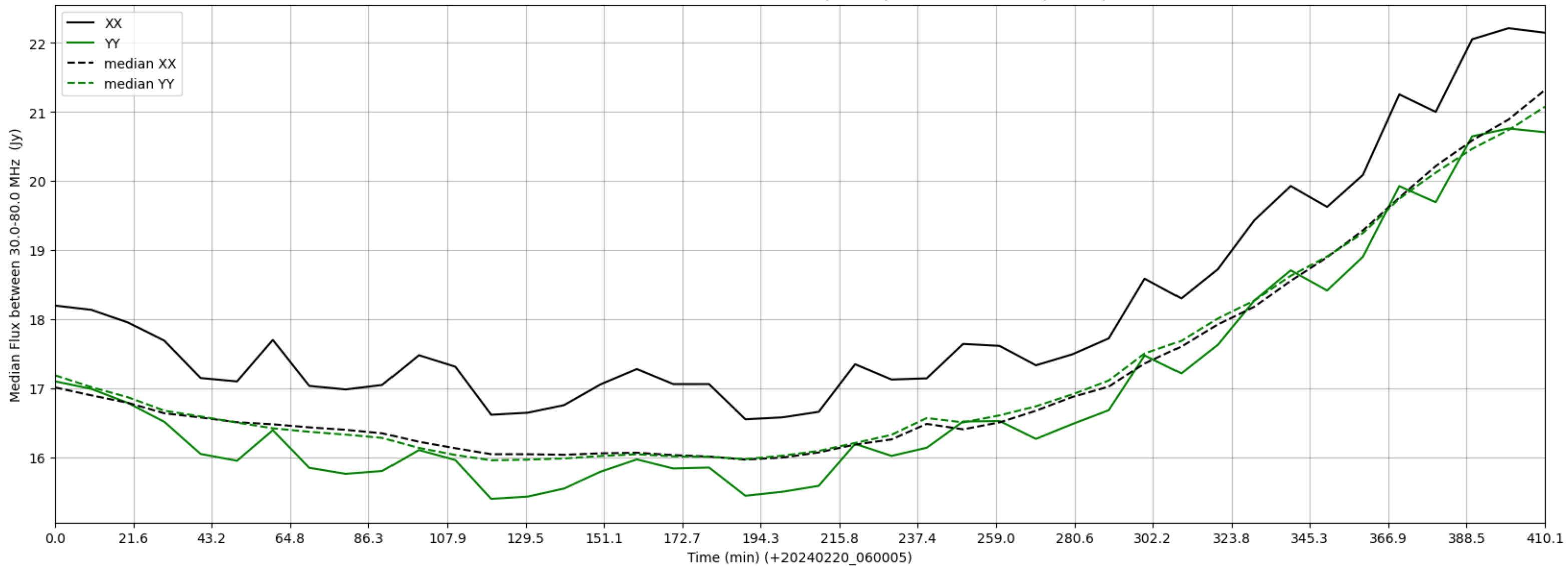
LWA008 - Correlator# 075 - XX FLAGS:BadSpecShape - YY FLAGS:BadSpecShape
