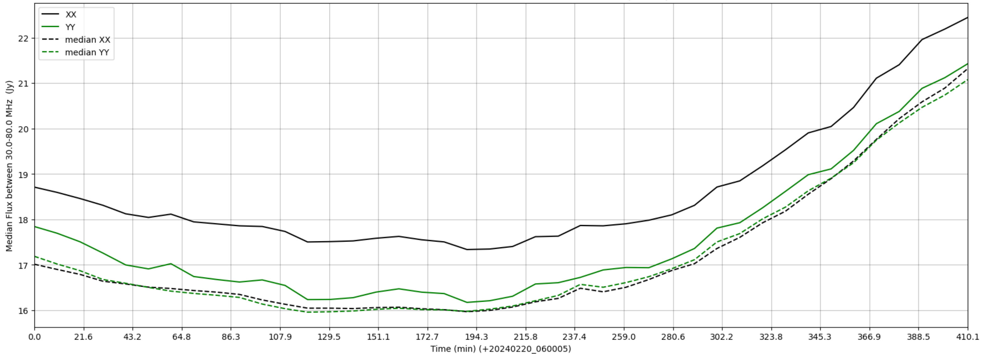
LWA007 - Correlator# 071 - XX FLAGS:Good - YY FLAGS:BadSpecShape
