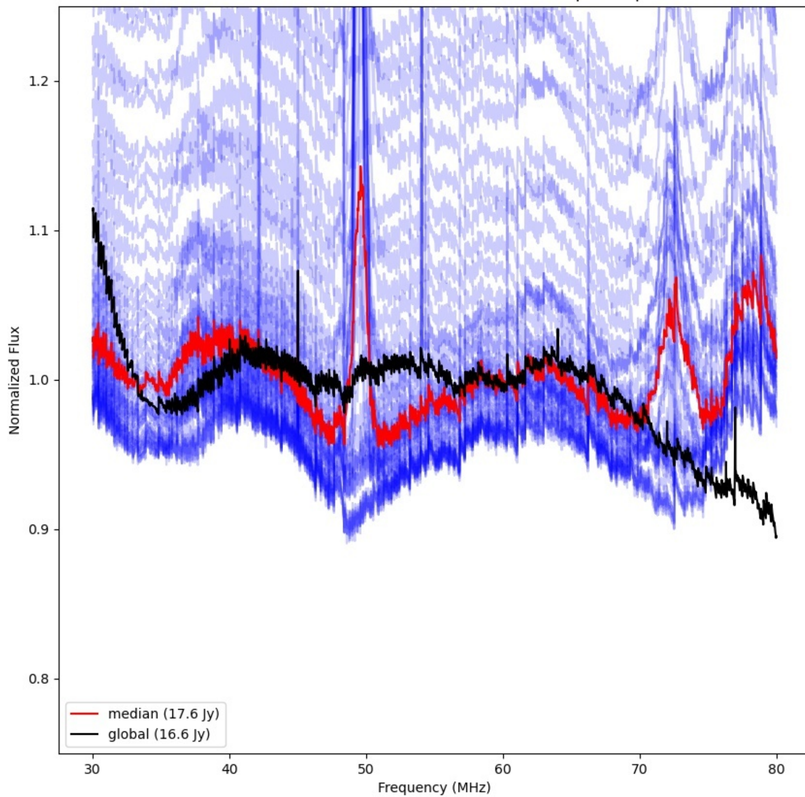
LWA011 - Correlator# 072 - YY - FLAGS:BadSpecShape
