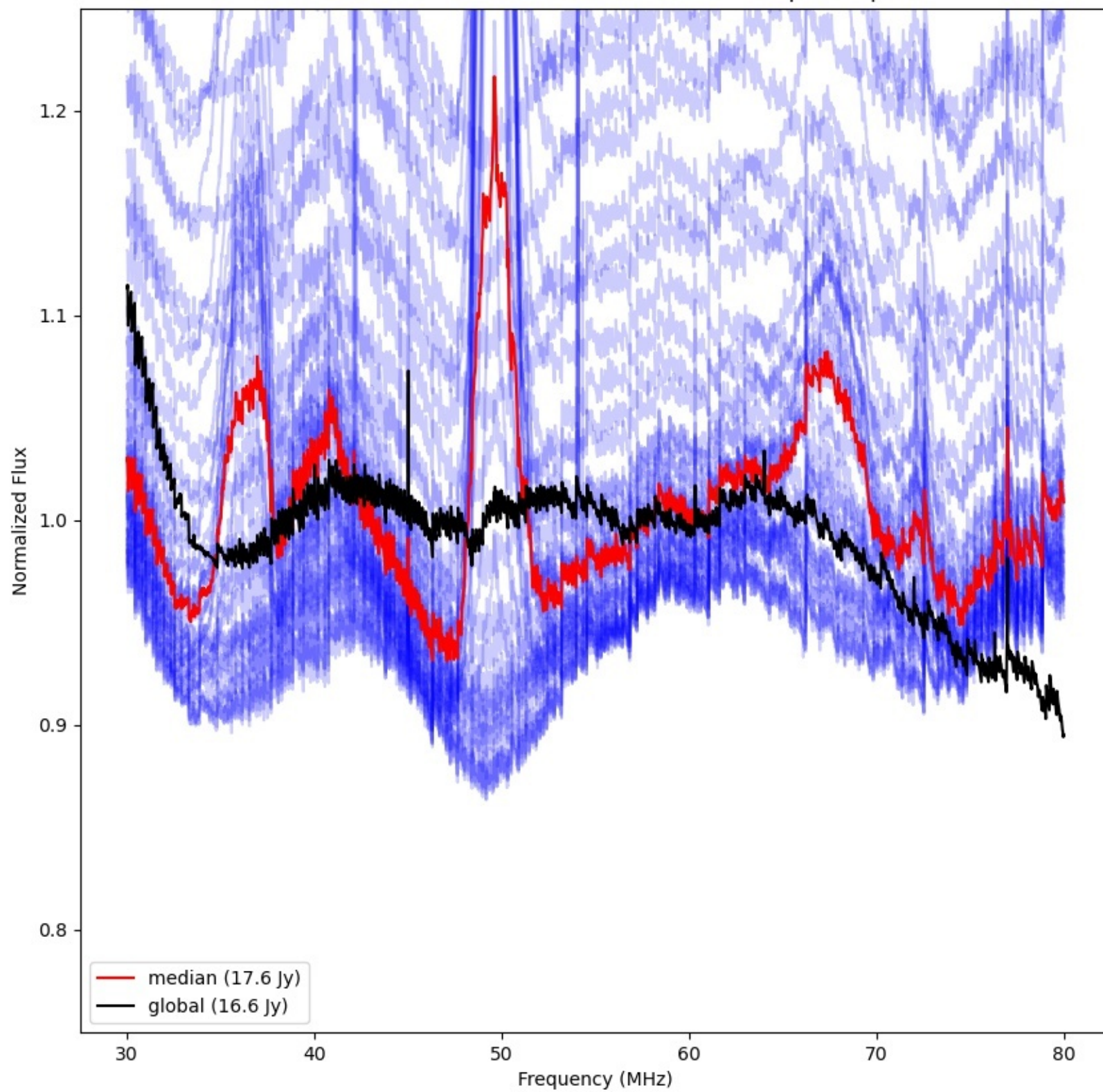
LWA041 - Correlator# 079 - YY - FLAGS:BadSpecShape
