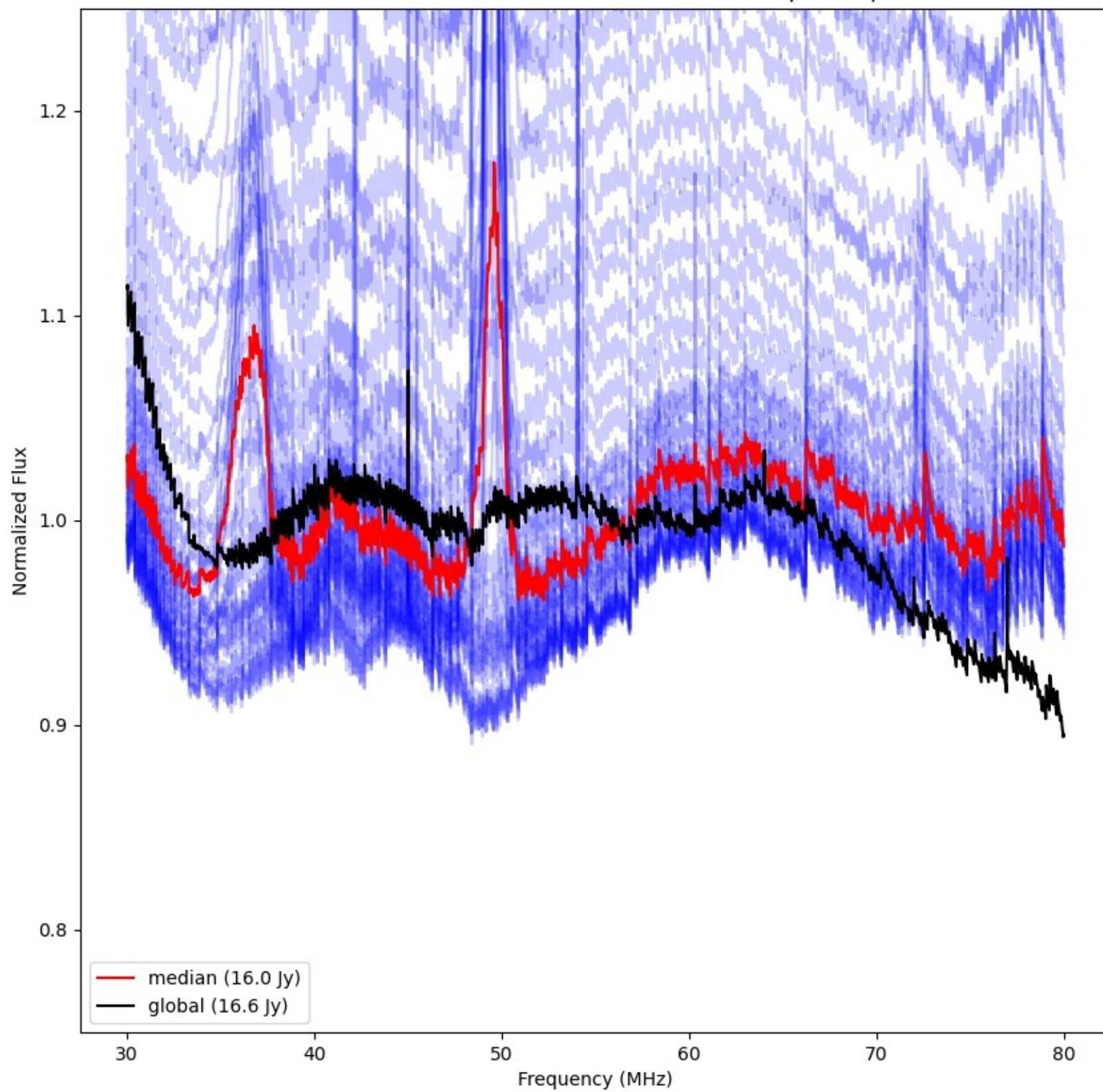
LWA010 - Correlator# 073 - YY - FLAGS:BadSpecShape
