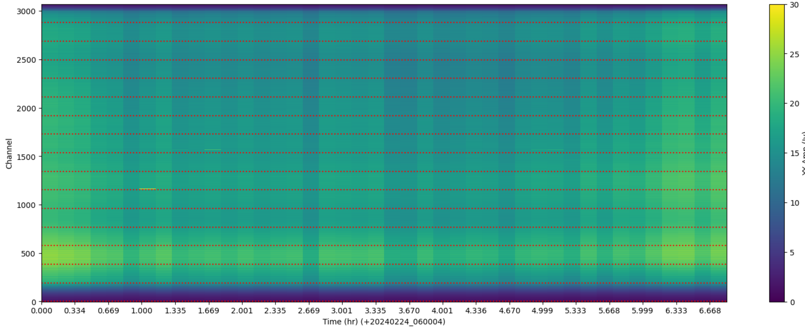
LWA044 - Correlator# 080 - YY - FLAGS: Good
