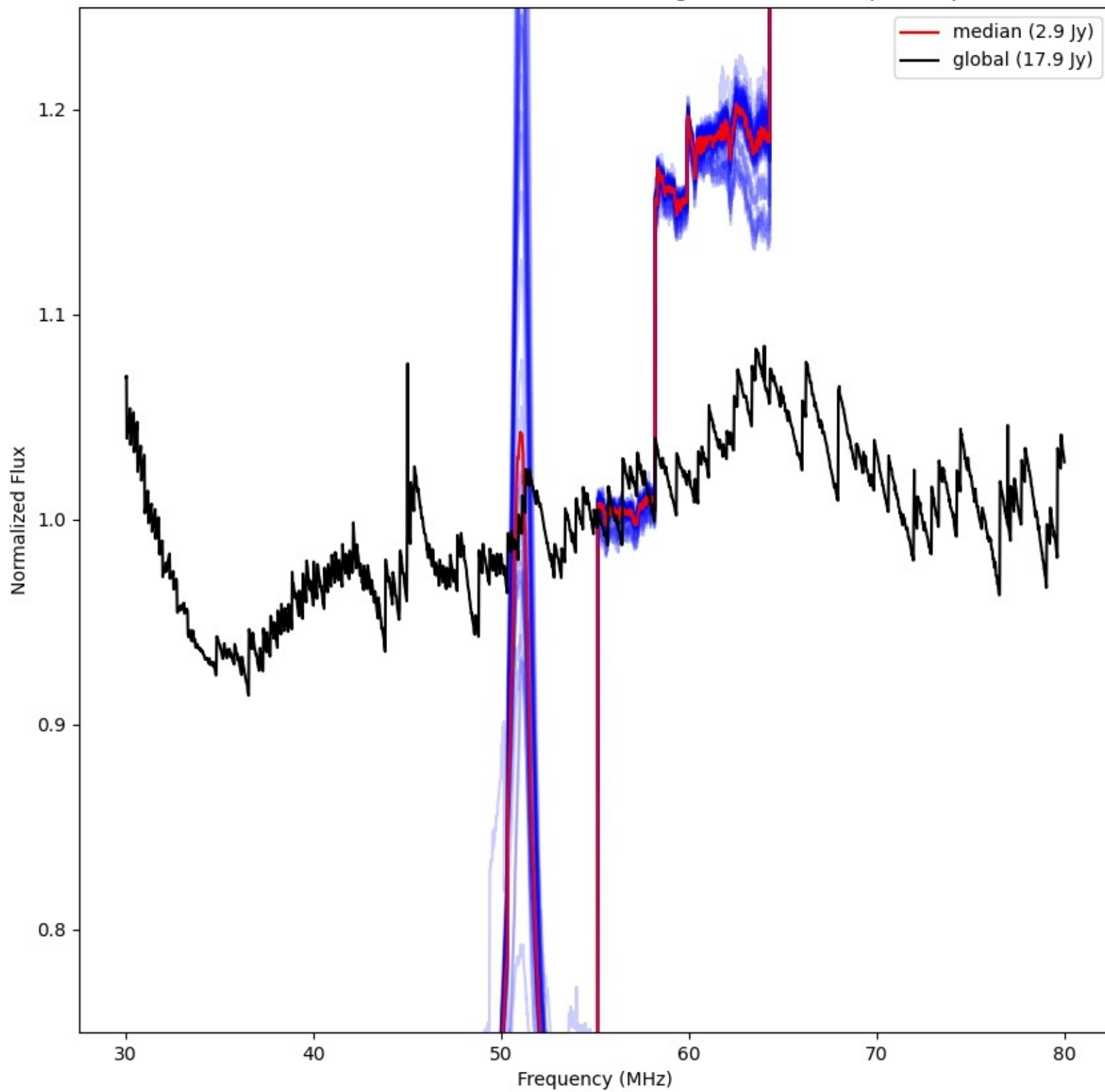
LWA041 - Correlator# 079 - YY - FLAGS:HighTimeVar+BadSpecShape
