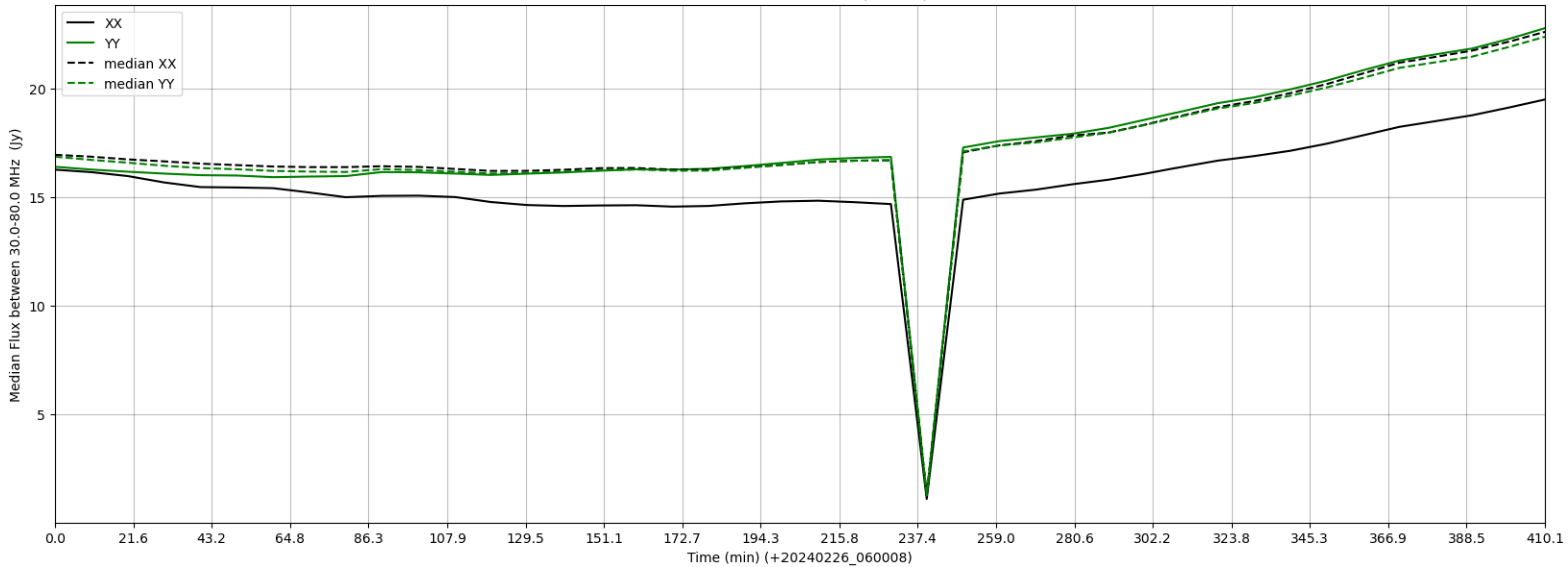
LWA328 - Correlator# 157 - XX FLAGS:BadSpecShape - YY FLAGS:Good
