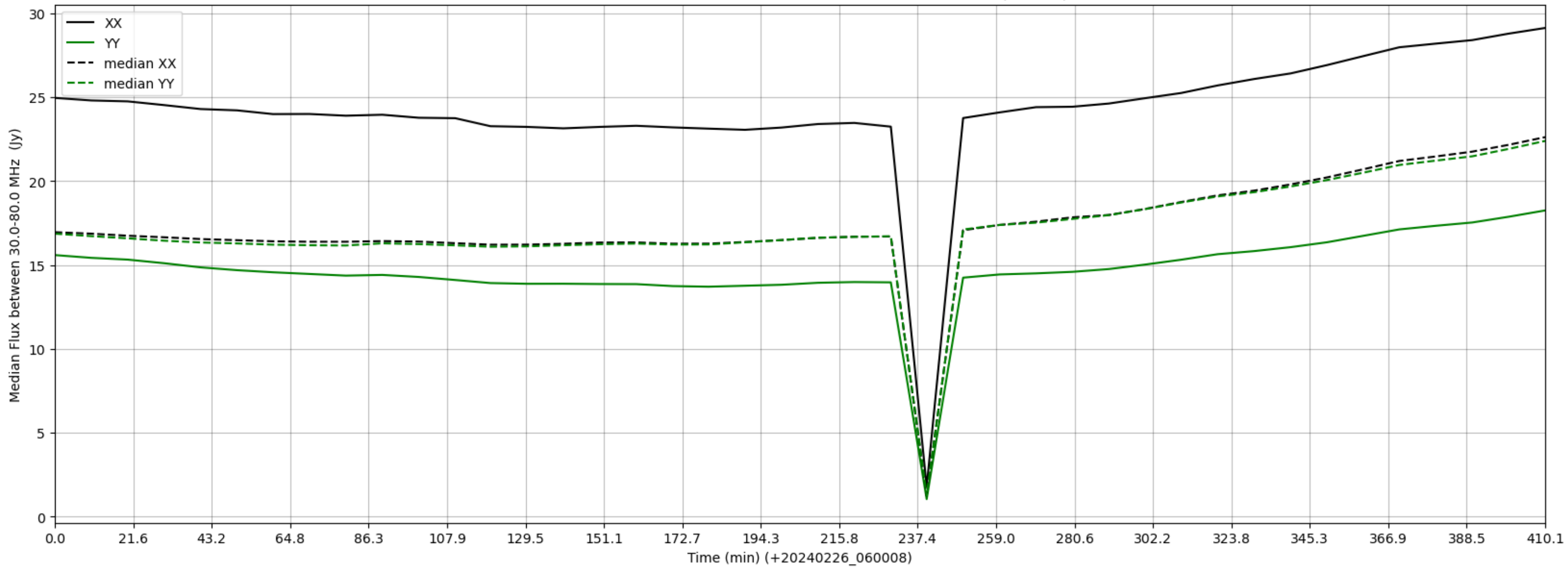
LWA286 - Correlator# 093 - XX FLAGS:Good - YY FLAGS:BadSpecShape
