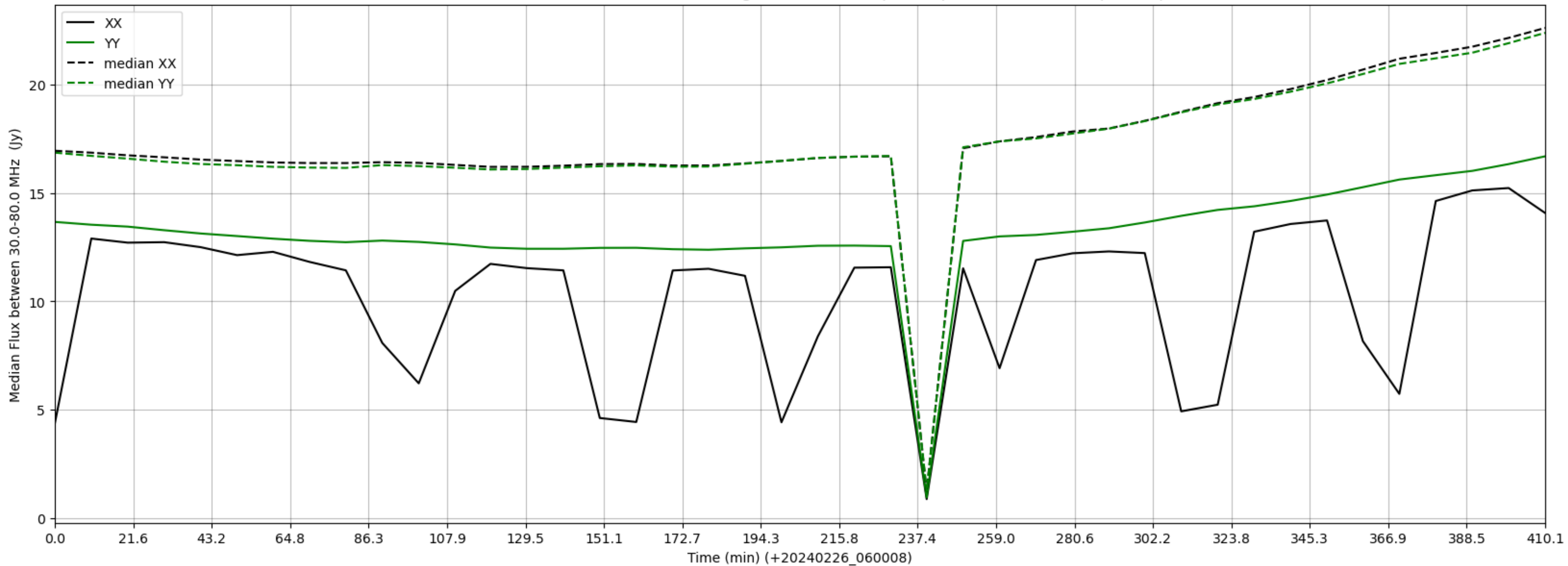
LWA335 - Correlator# 057 - XX FLAGS:HighTimeVar+BadSpecShape - YY FLAGS:BadSpecShape
