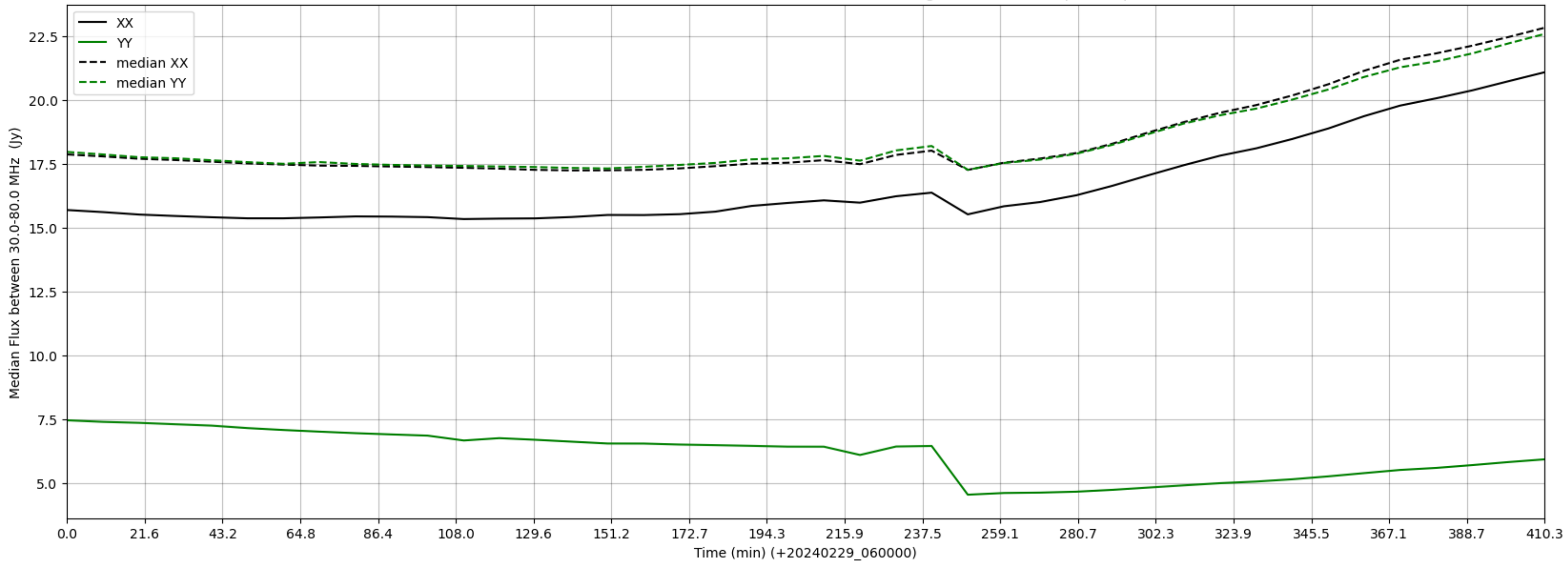
LWA303 - Correlator# 051 - XX FLAGS:Good - YY FLAGS:HighTimeVar+BadSpecShape
