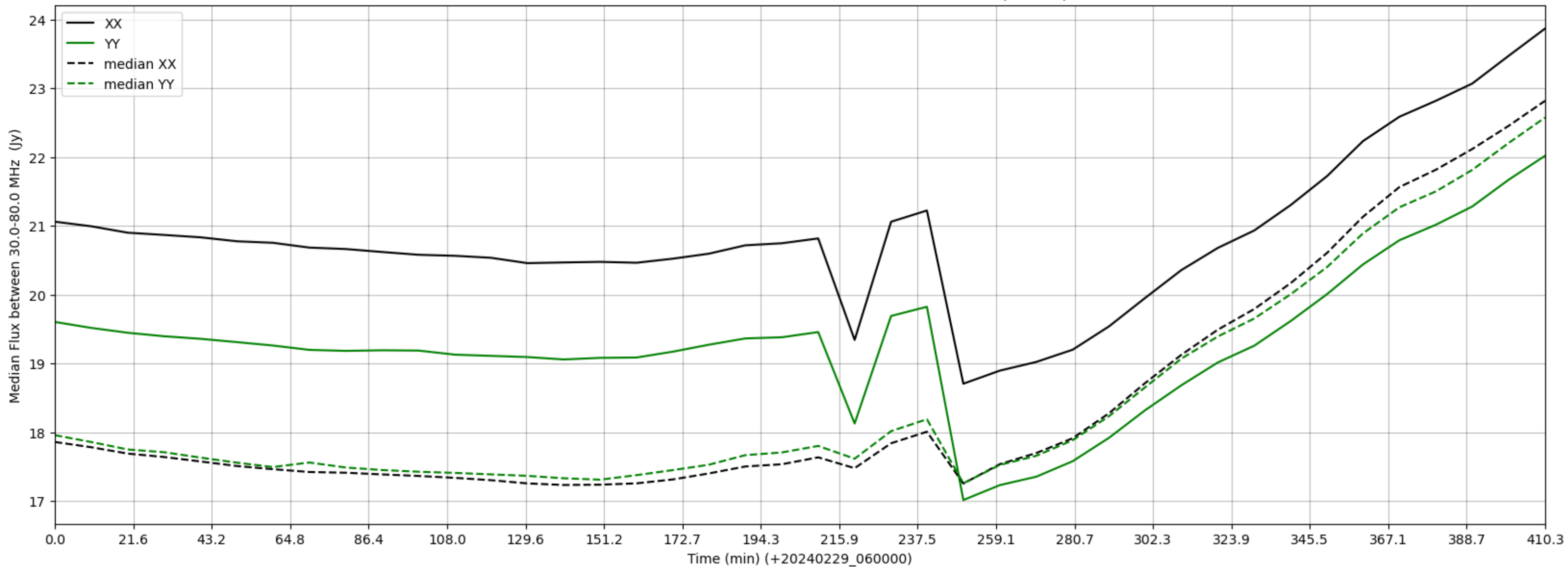
LWA066 - Correlator# 164 - XX FLAGS:Good - YY FLAGS:BadSpecShape
