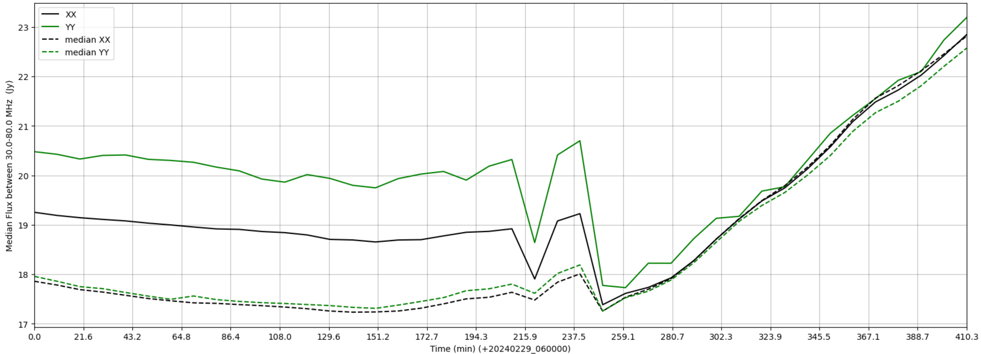
LWA003 - Correlator# 067 - XX FLAGS:Good - YY FLAGS:BadSpecShape
