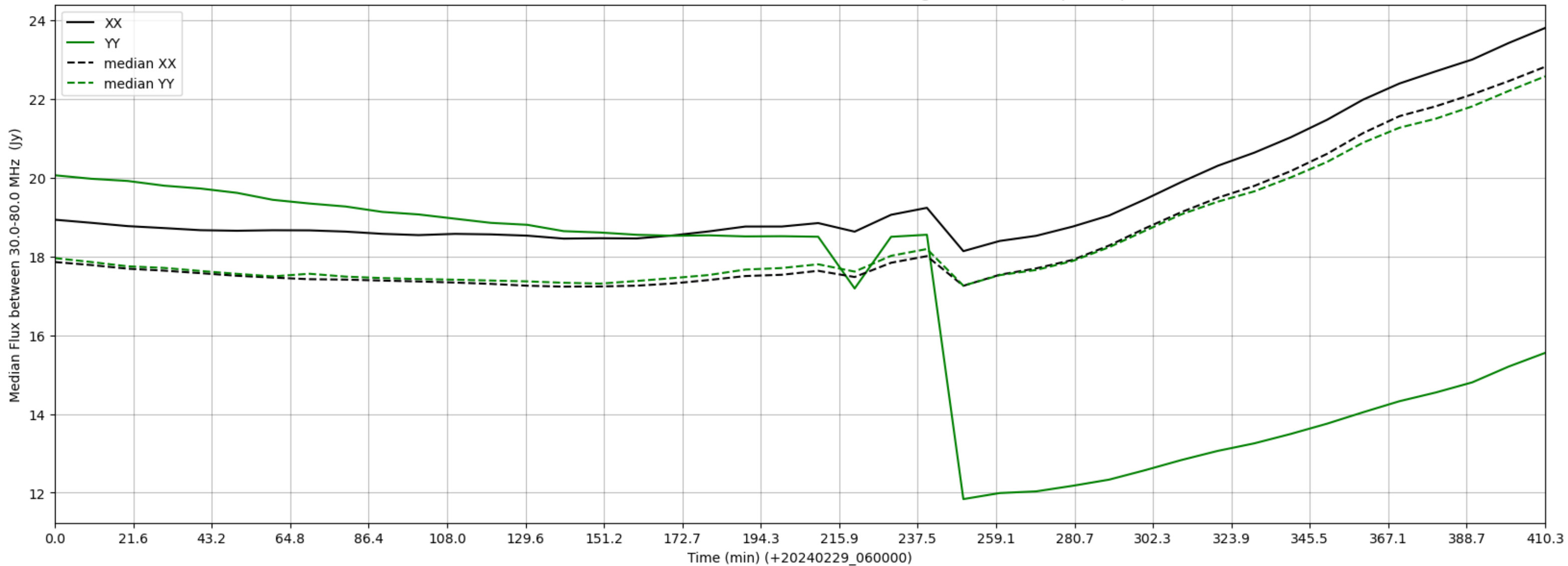
LWA326 - Correlator# 250 - XX FLAGS:Good - YY FLAGS:HighTimeVar+BadSpecShape
