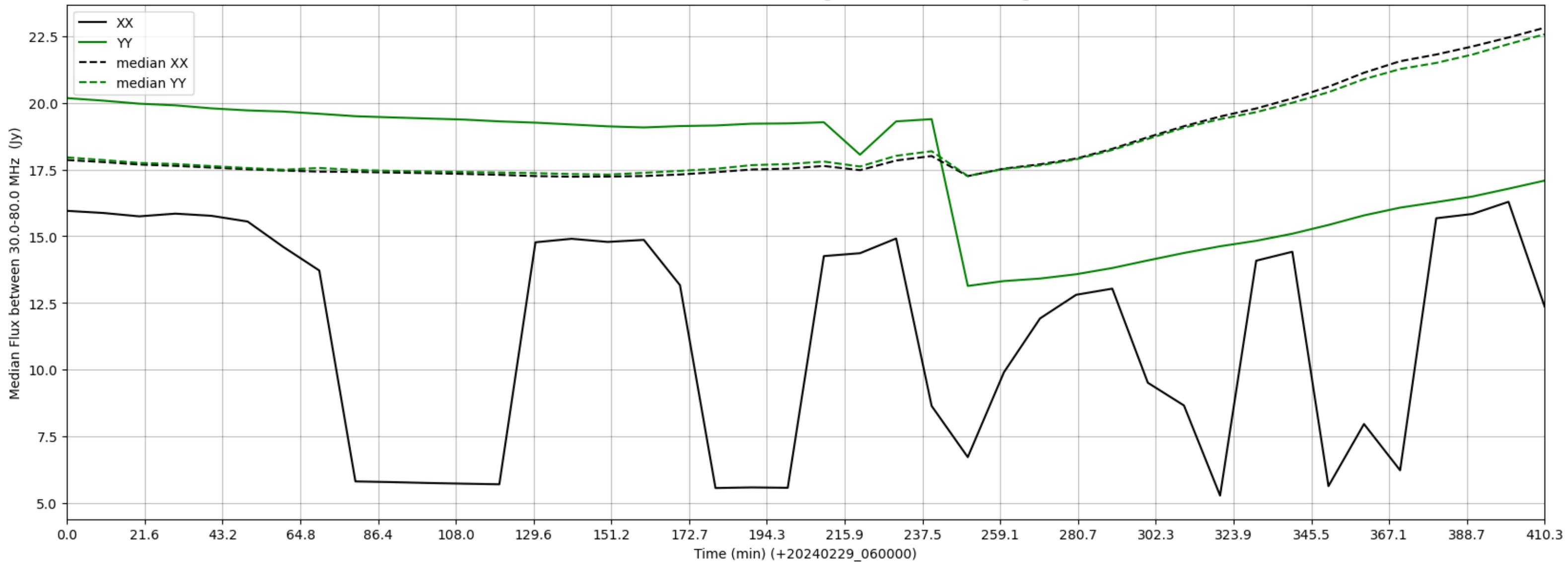
LWA335 - Correlator# 057 - XX FLAGS:HighTimeVar - YY FLAGS:HighTimeVar
