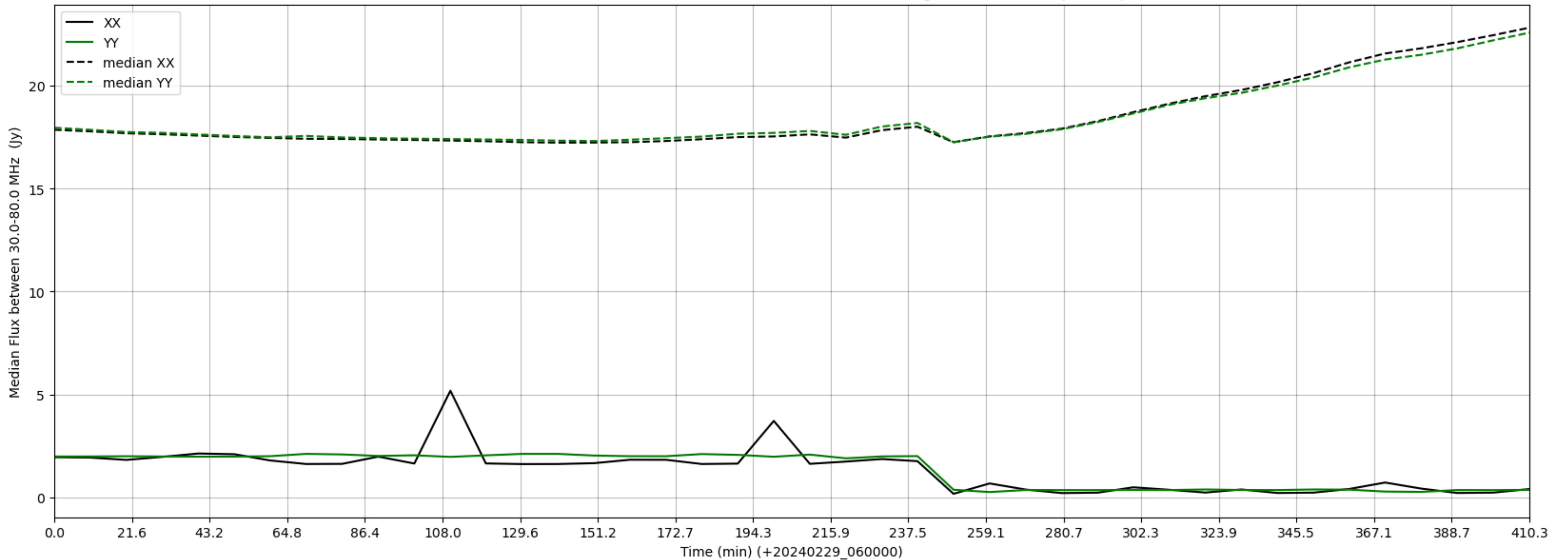
LWA041 - Correlator# 079 - XX FLAGS:LowFlux - YY FLAGS:HighTimeVar+BadSpecShape
