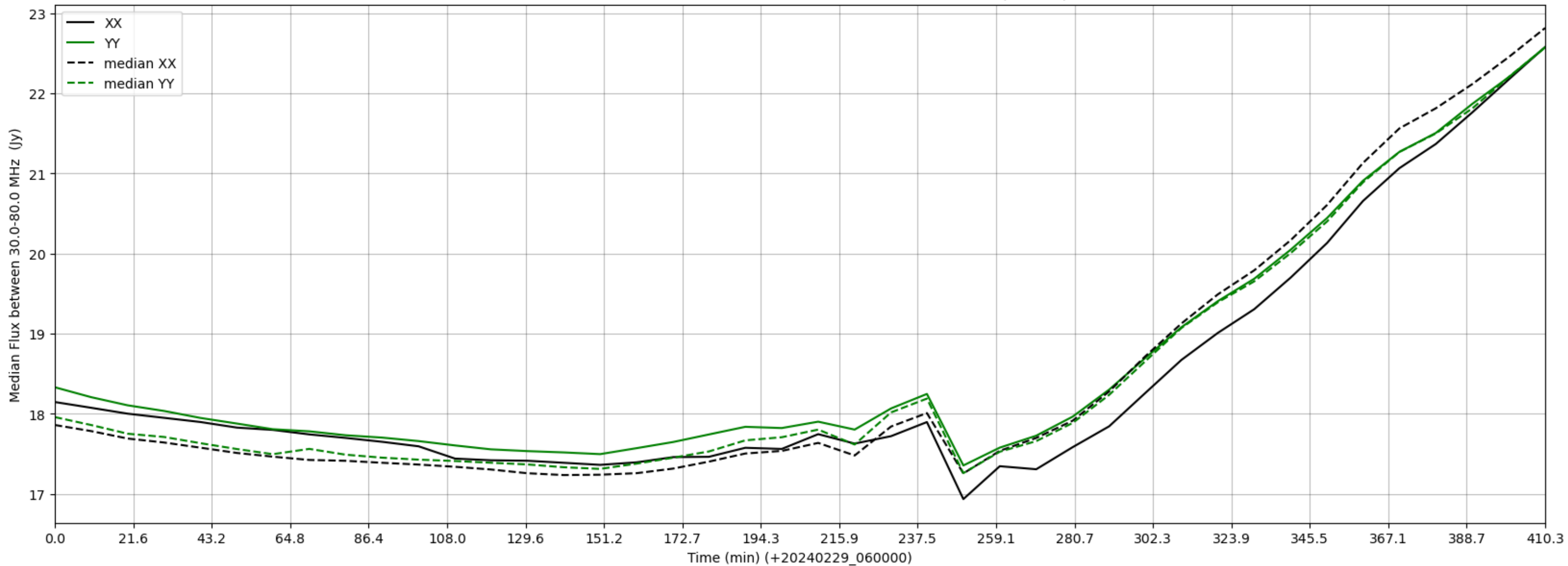
LWA016 - Correlator# 097 - XX FLAGS:Good - YY FLAGS:BadSpecShape
