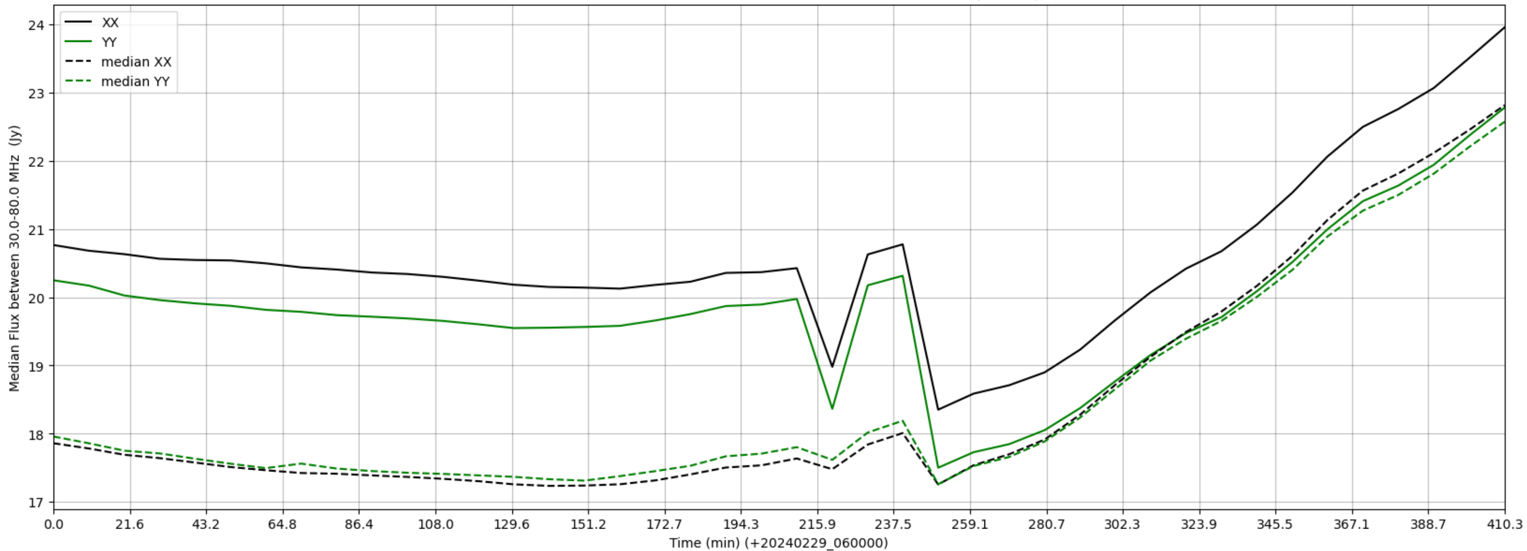
LWA002 - Correlator# 064 - XX FLAGS:Good - YY FLAGS:BadSpecShape
