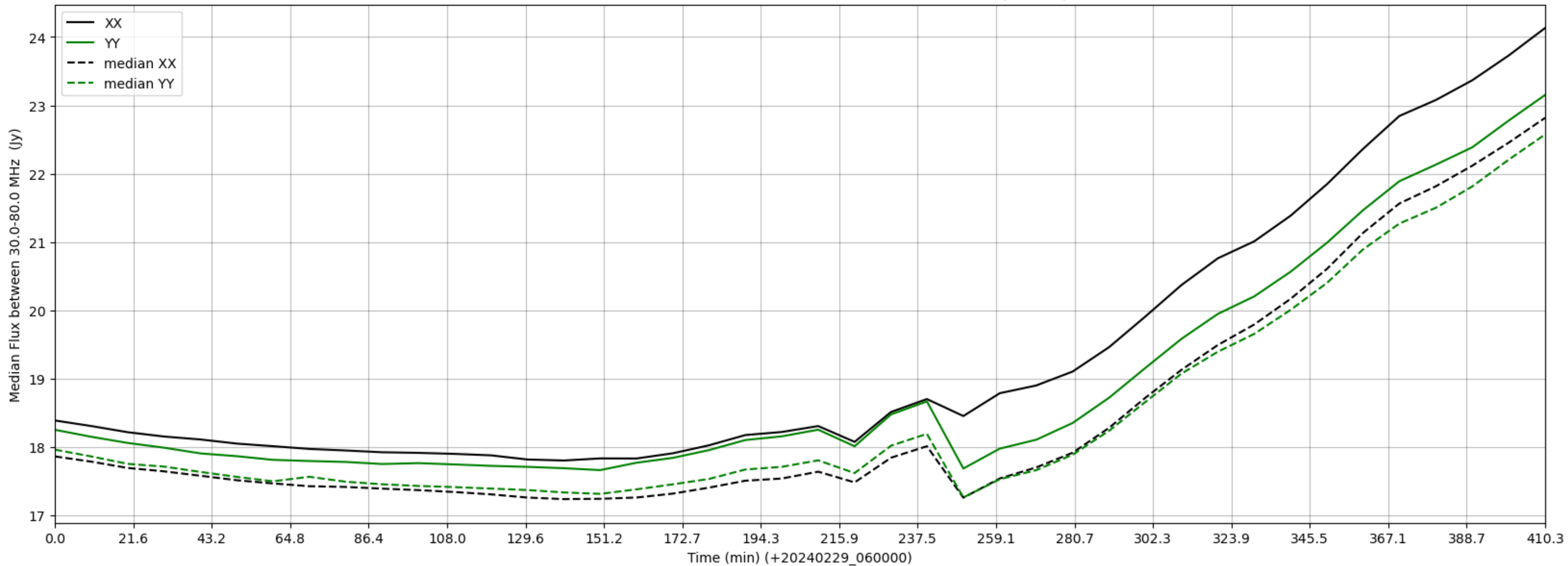
LWA242 - Correlator# 339 - XX FLAGS:Good - YY FLAGS:BadSpecShape
