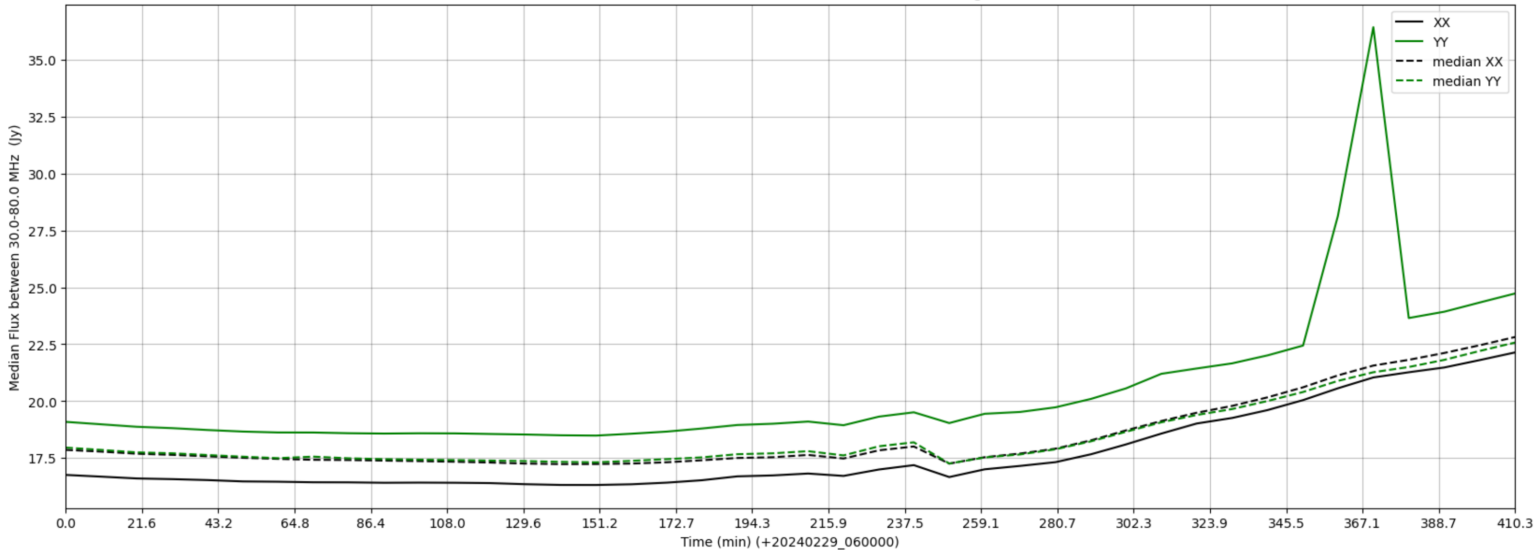
LWA173 - Correlator# 290 - XX FLAGS:Good - YY FLAGS:HighTimeVar
