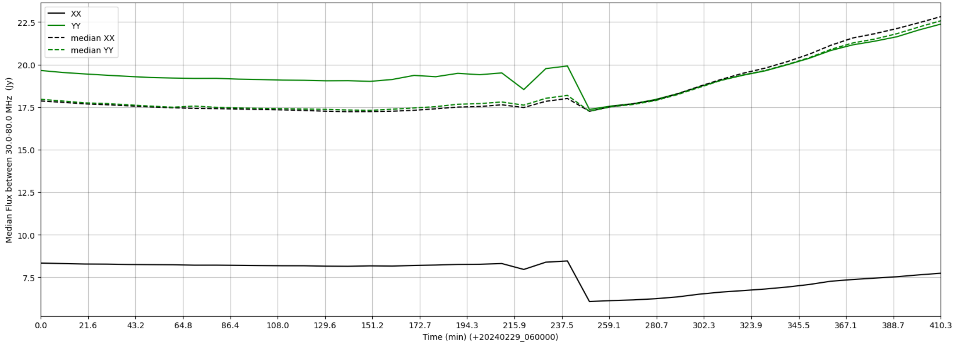
LWA130 - Correlator# 183 - XX FLAGS:HighTimeVar+BadSpecShape - YY FLAGS:BadSpecShape
