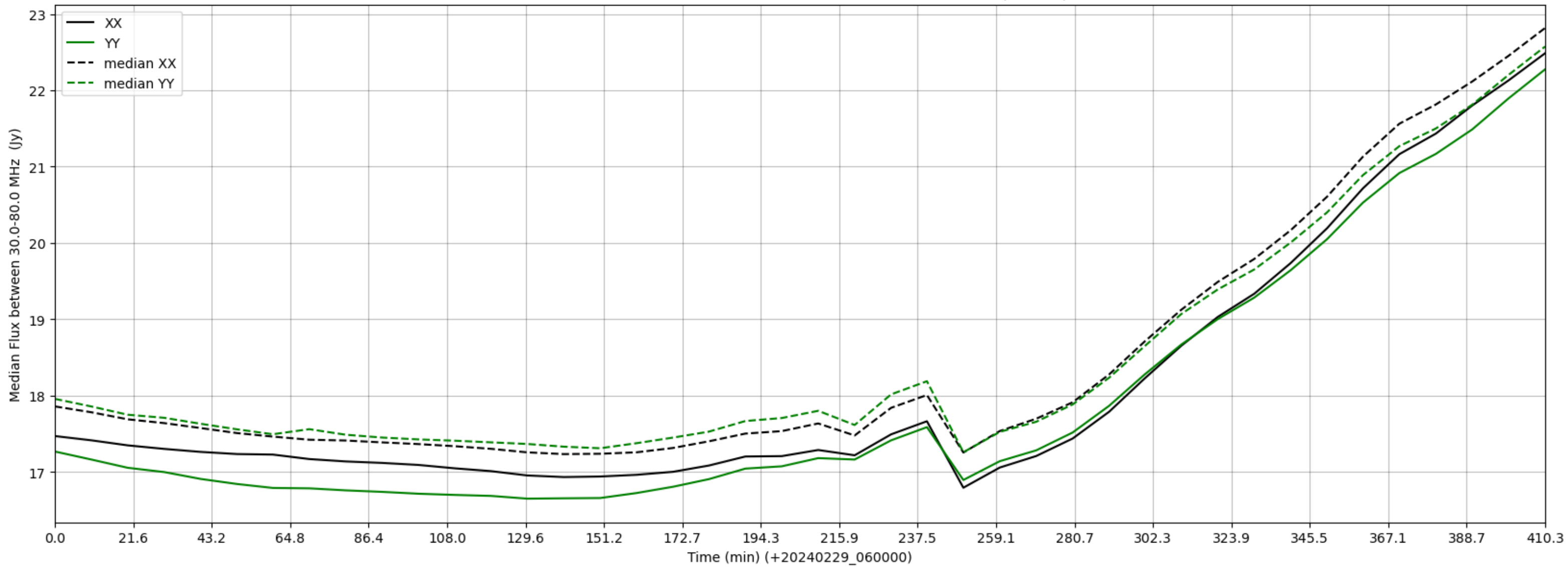
LWA020 - Correlator# 102 - XX FLAGS:Good - YY FLAGS:BadSpecShape
