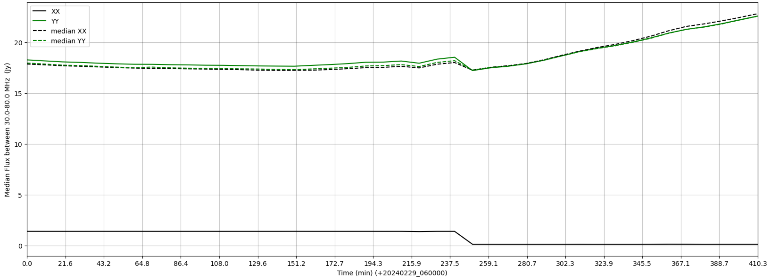
LWA138 - Correlator# 261 - XX FLAGS:LowFlux - YY FLAGS:BadSpecShape
