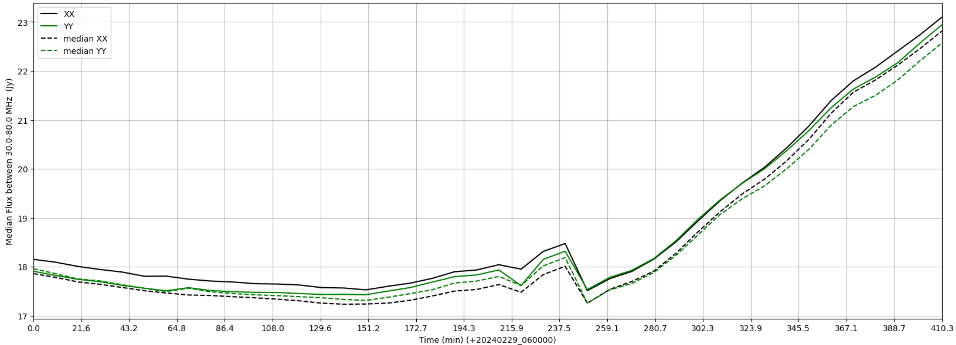
LWA048 - Correlator# 113 - XX FLAGS:Good - YY FLAGS:BadSpecShape
