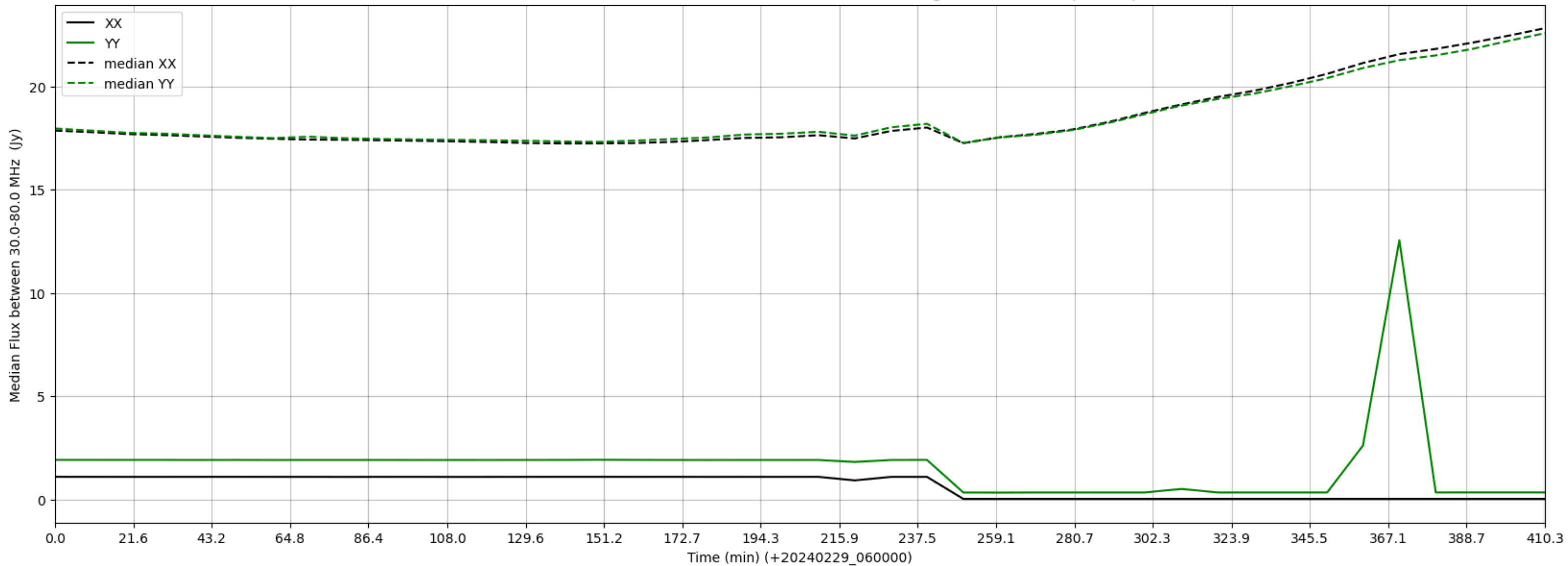
LWA232 - Correlator# 307 - XX FLAGS:LowFlux - YY FLAGS:HighTimeVar+BadSpecShape
