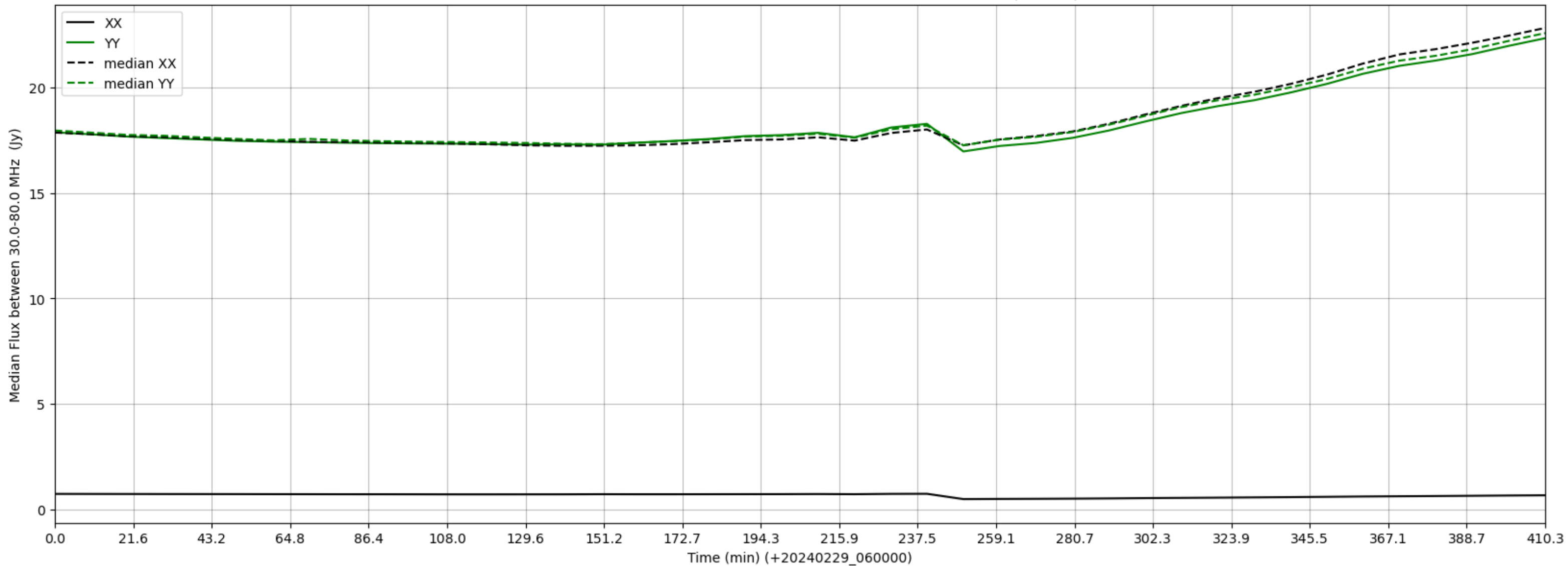
LWA234 - Correlator# 289 - XX FLAGS:LowFlux - YY FLAGS:BadSpecShape
