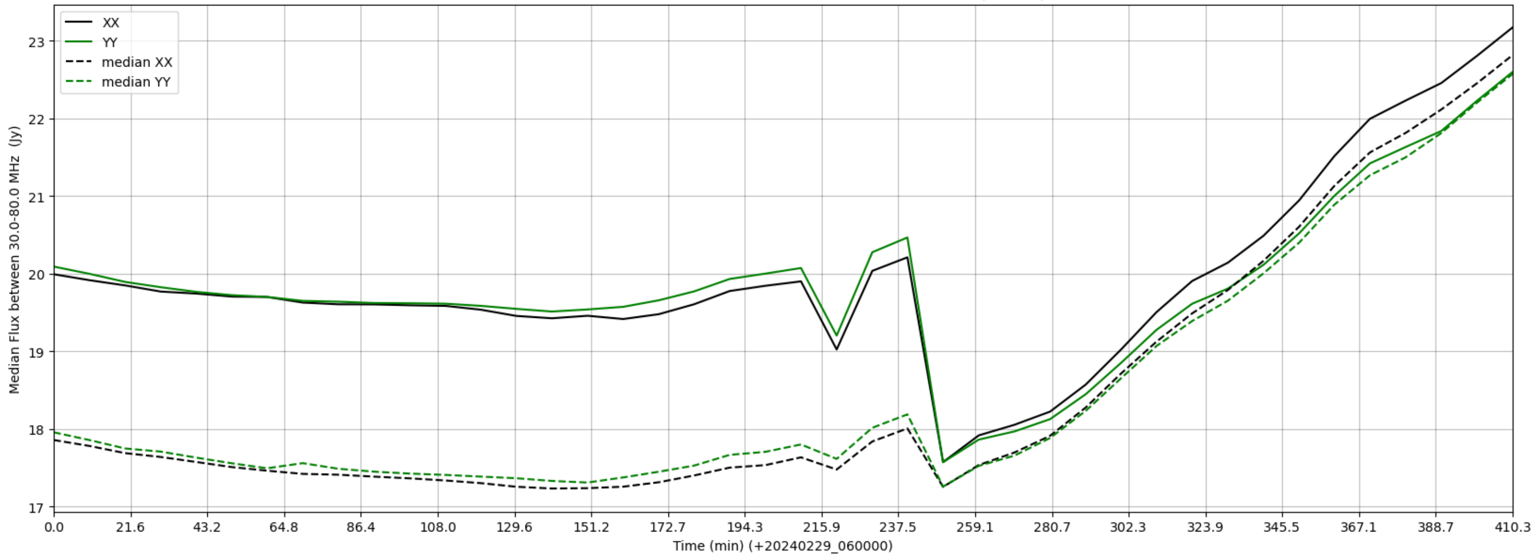
LWA193 - Correlator# 270 - XX FLAGS:Good - YY FLAGS:BadSpecShape
