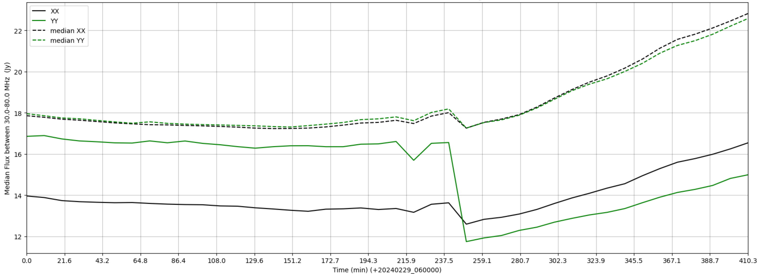
LWA302 - Correlator# 092 - XX FLAGS:Good - YY FLAGS:HighTimeVar
