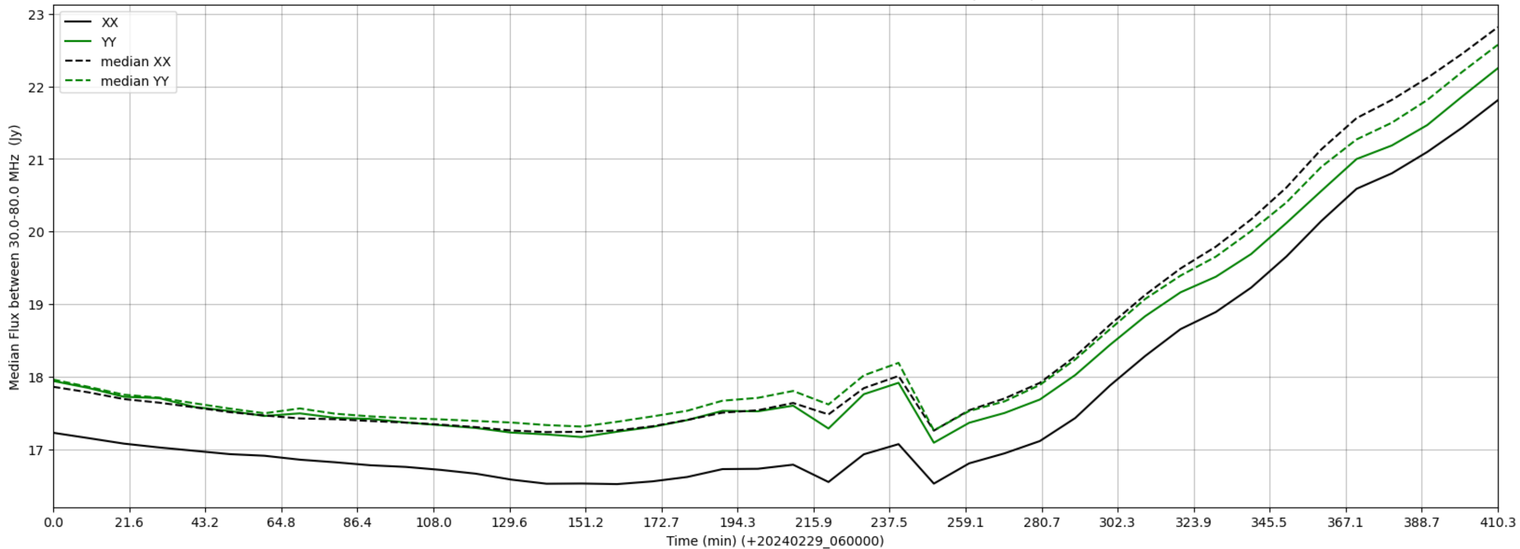
LWA074 - Correlator# 086 - XX FLAGS:Good - YY FLAGS:BadSpecShape
