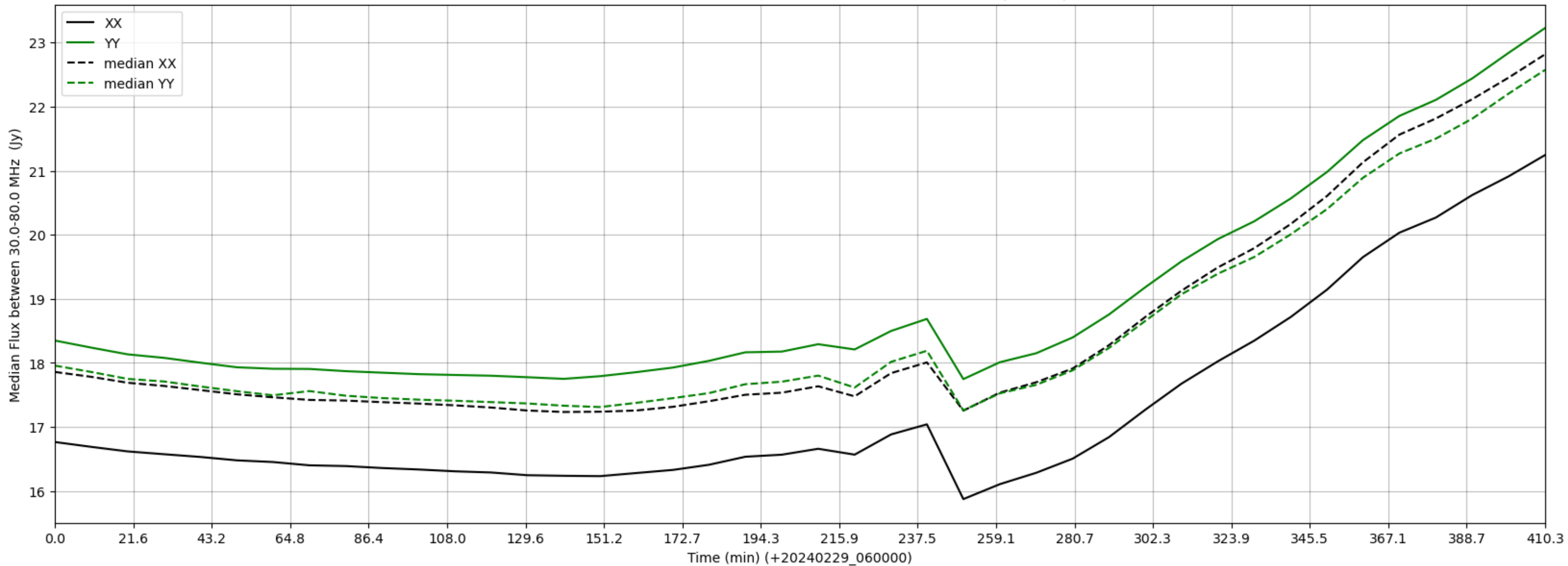
LWA046 - Correlator# 082 - XX FLAGS:Good - YY FLAGS:BadSpecShape
