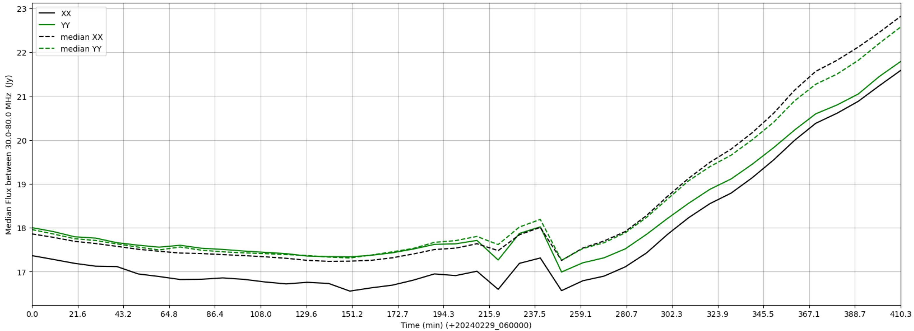
LWA077 - Correlator# 088 - XX FLAGS:Good - YY FLAGS:BadSpecShape
