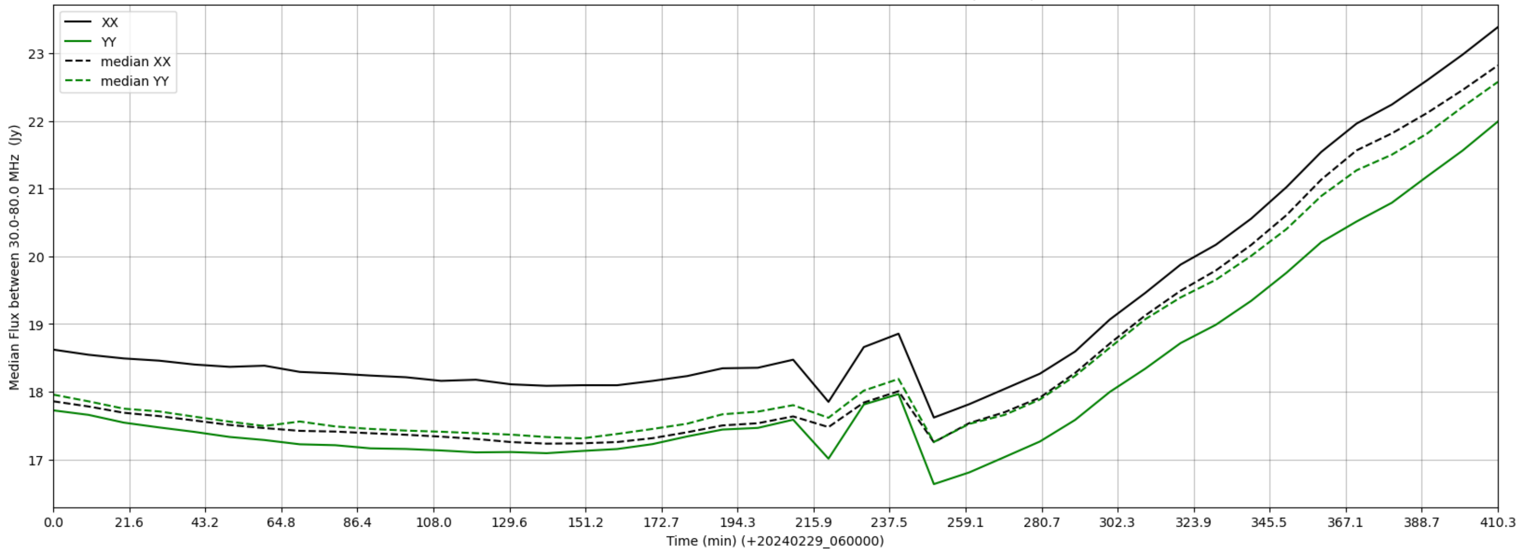
LWA008 - Correlator# 075 - XX FLAGS:Good - YY FLAGS:BadSpecShape
