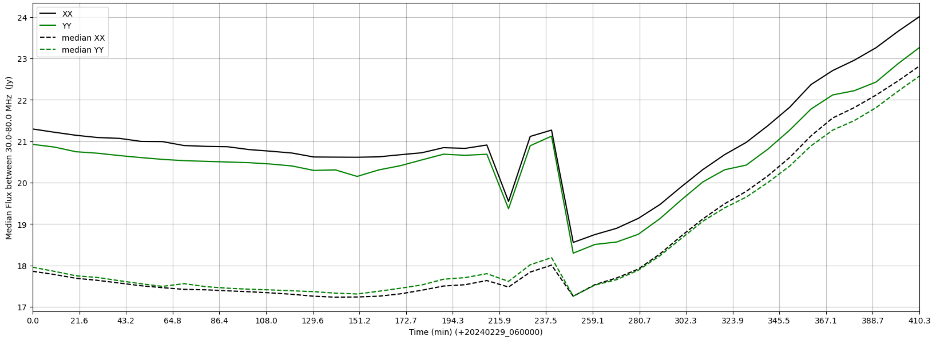
LWA065 - Correlator# 165 - XX FLAGS:Good - YY FLAGS:BadSpecShape
