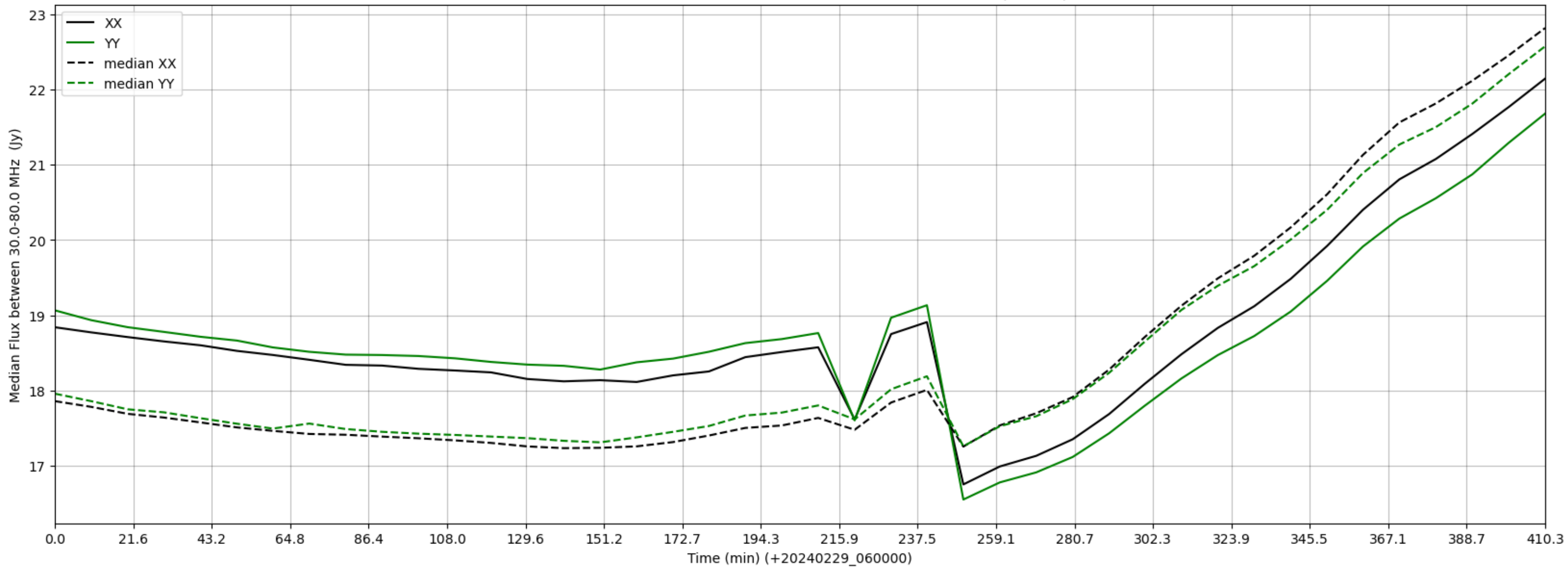
LWA005 - Correlator# 069 - XX FLAGS:Good - YY FLAGS:BadSpecShape
