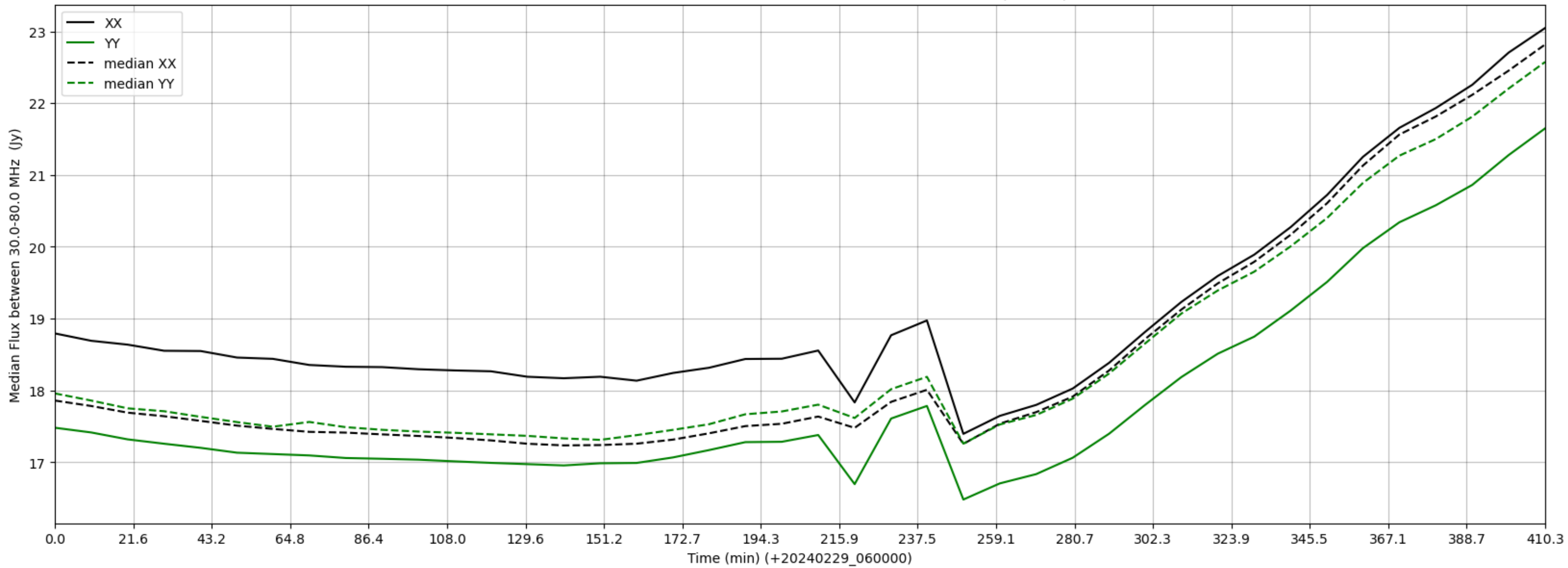
LWA099 - Correlator# 172 - XX FLAGS:Good - YY FLAGS:BadSpecShape
