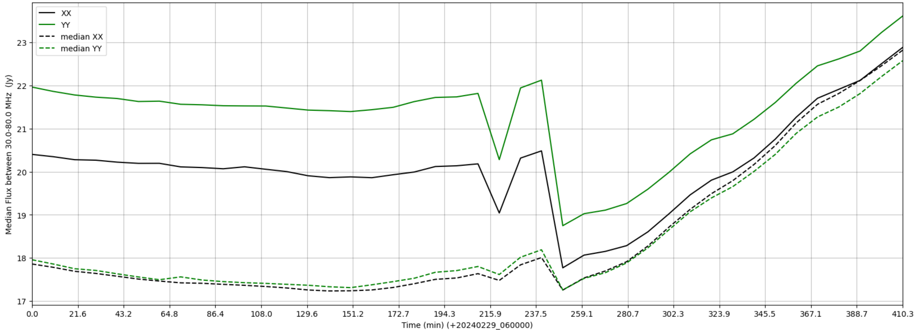
LWA161 - Correlator# 262 - XX FLAGS:Good - YY FLAGS:BadSpecShape
