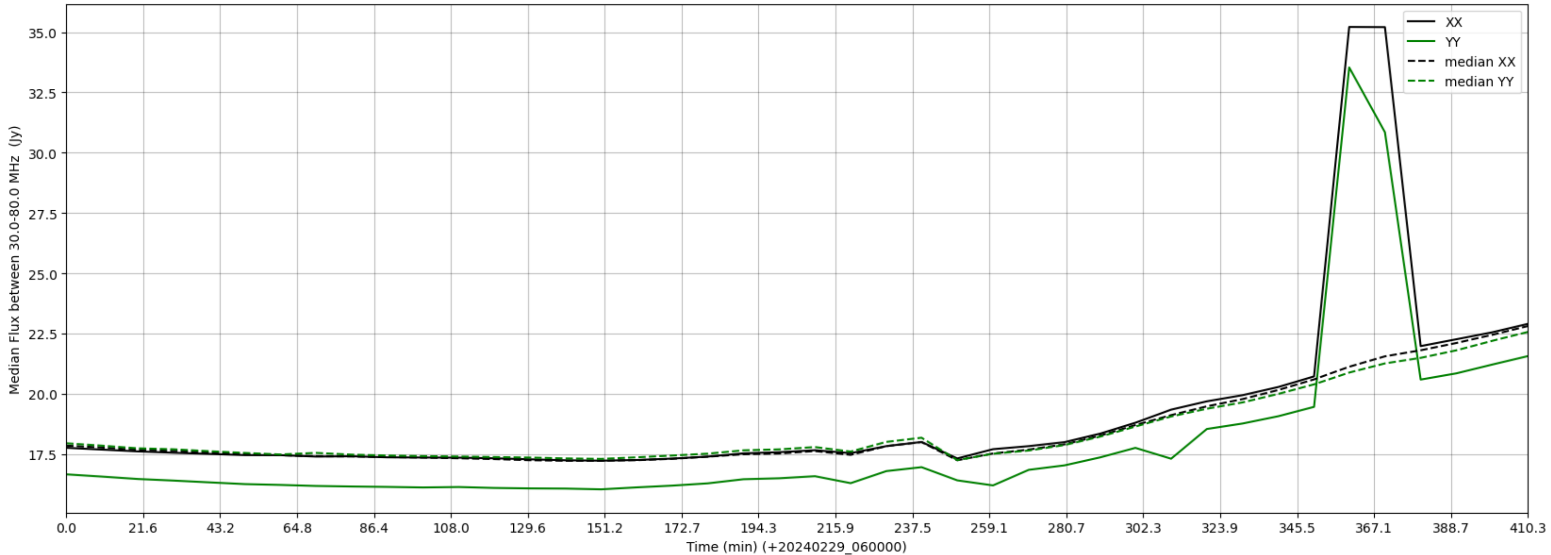
LWA208 - Correlator# 298 - XX FLAGS:HighTimeVar - YY FLAGS:HighTimeVar+BadSpecShape
