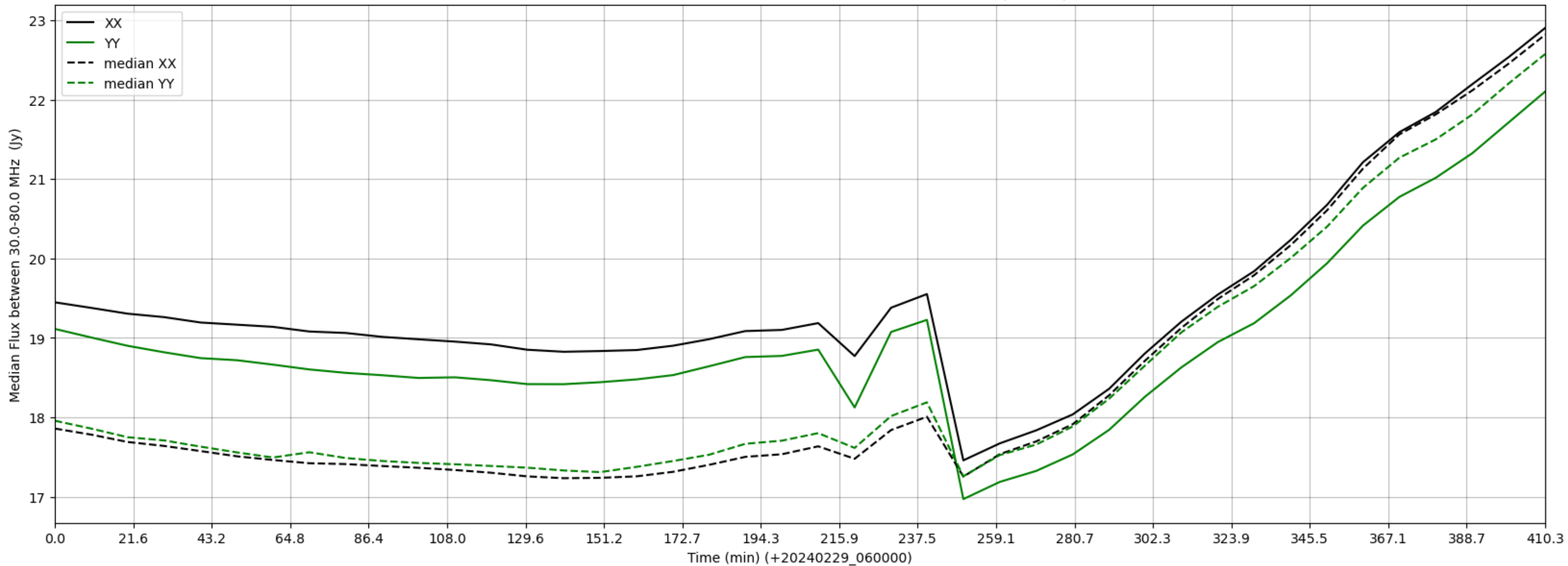
LWA004 - Correlator# 066 - XX FLAGS:Good - YY FLAGS:BadSpecShape
