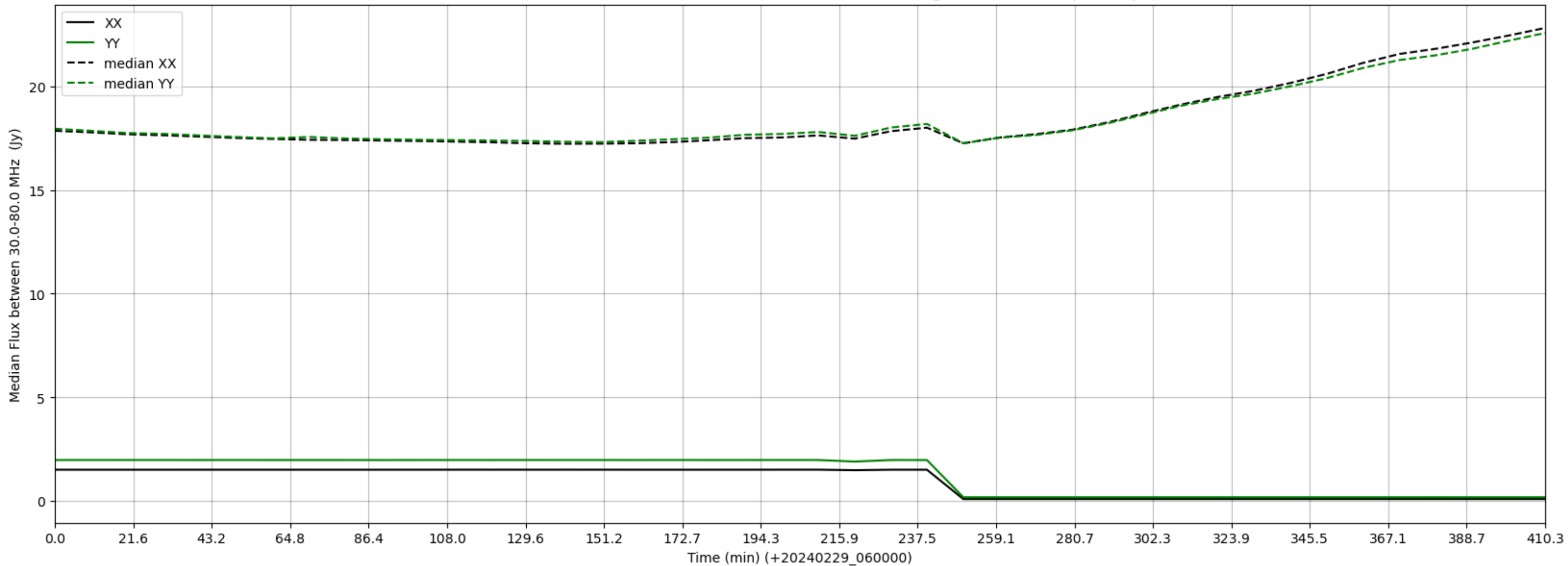
LWA298 - Correlator# 049 - XX FLAGS:LowFlux - YY FLAGS:HighTimeVar+BadSpecShape
