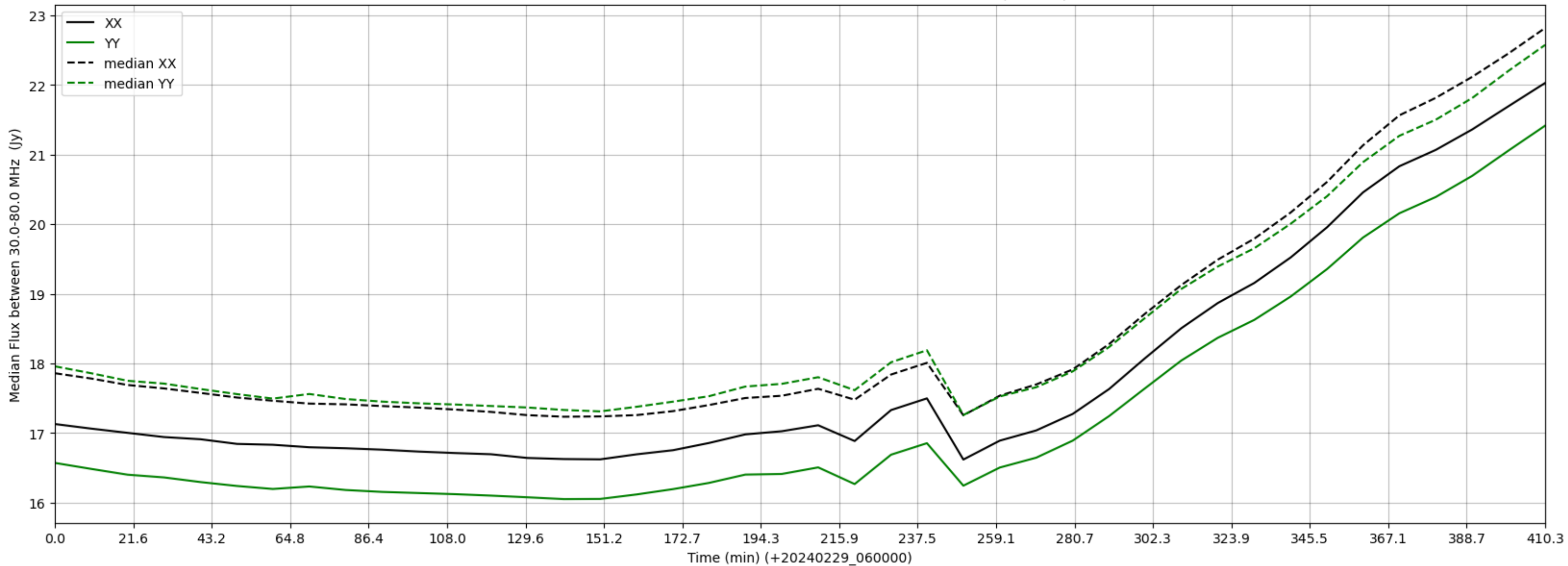
LWA170 - Correlator# 288 - XX FLAGS:Good - YY FLAGS:BadSpecShape
