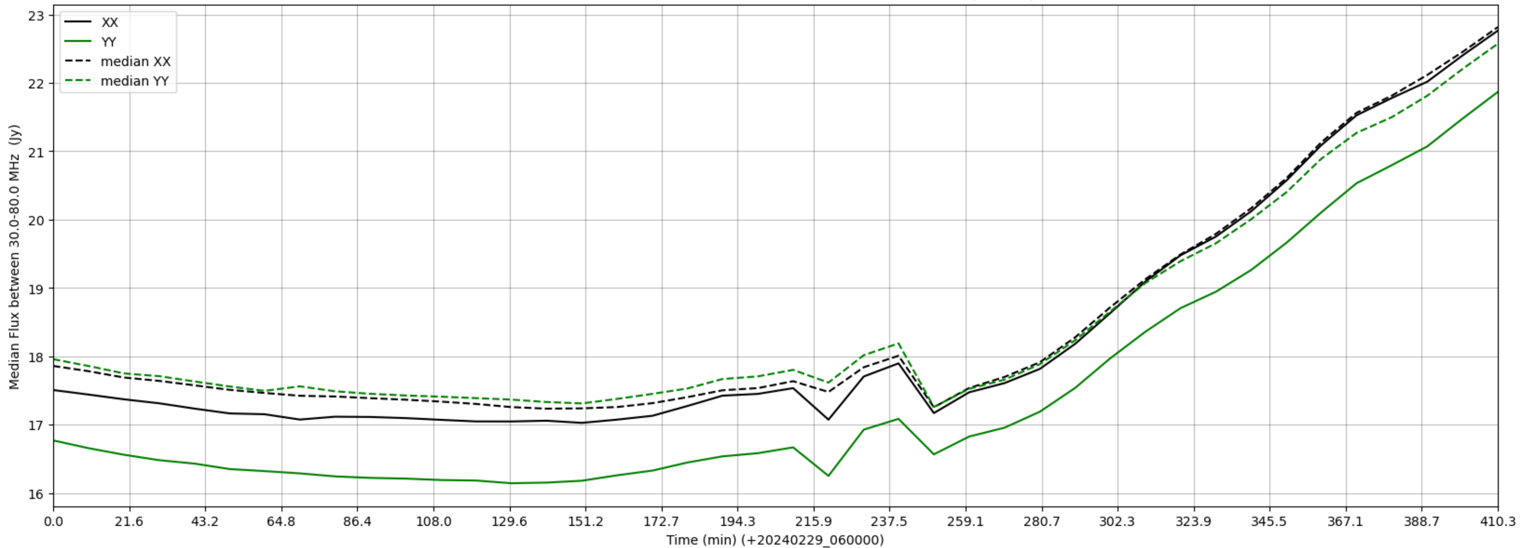
LWA210 - Correlator# 300 - XX FLAGS:Good - YY FLAGS:BadSpecShape
