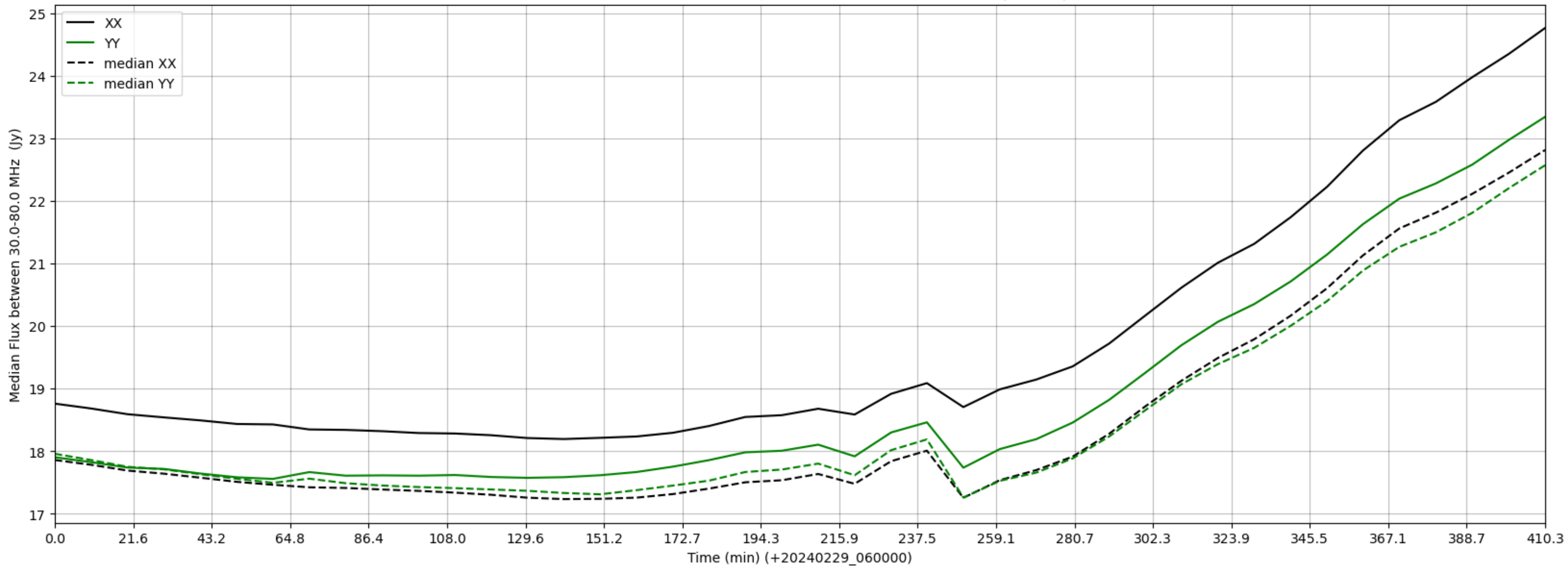
LWA072 - Correlator# 171 - XX FLAGS:Good - YY FLAGS:BadSpecShape
