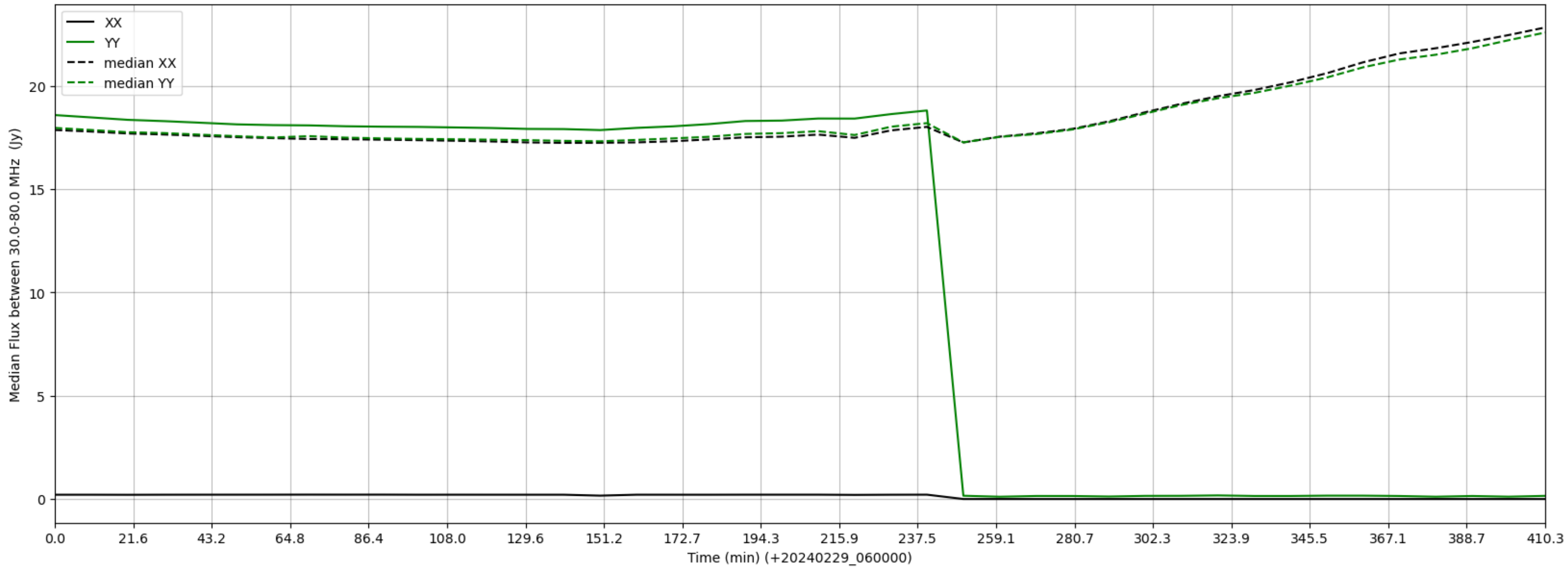
LWA255 - Correlator# 033 - XX FLAGS:LowFlux - YY FLAGS:HighTimeVar
