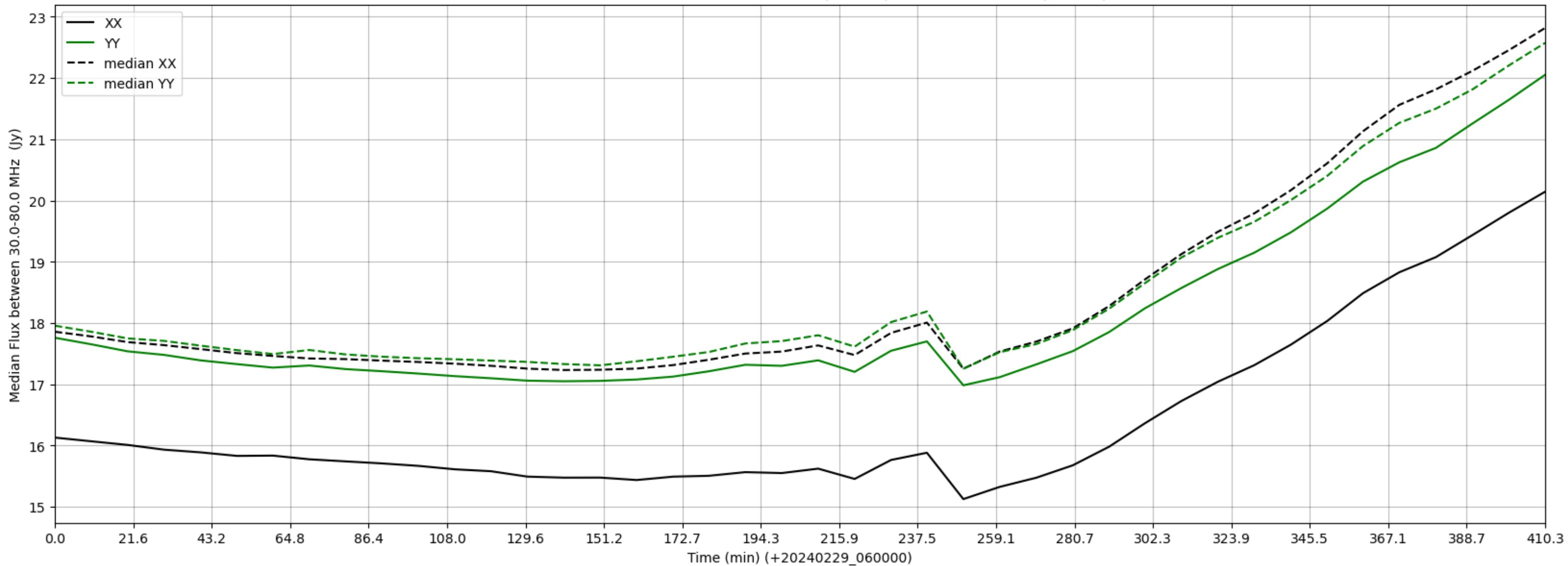
LWA071 - Correlator# 084 - XX FLAGS:BadSpecShape - YY FLAGS:BadSpecShape
