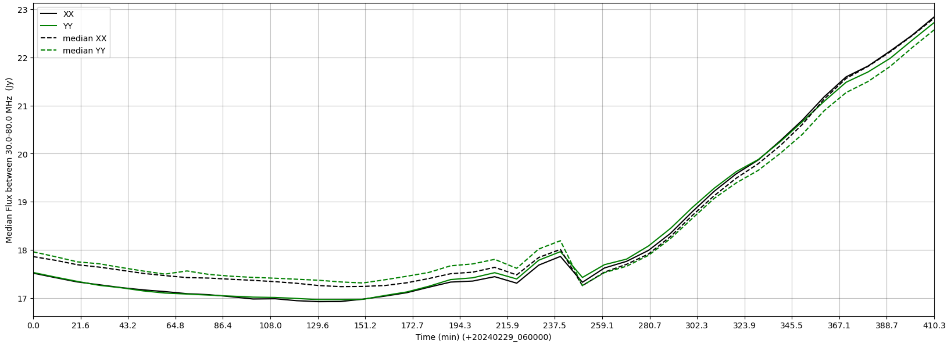
LWA243 - Correlator# 330 - XX FLAGS:Good - YY FLAGS:BadSpecShape
