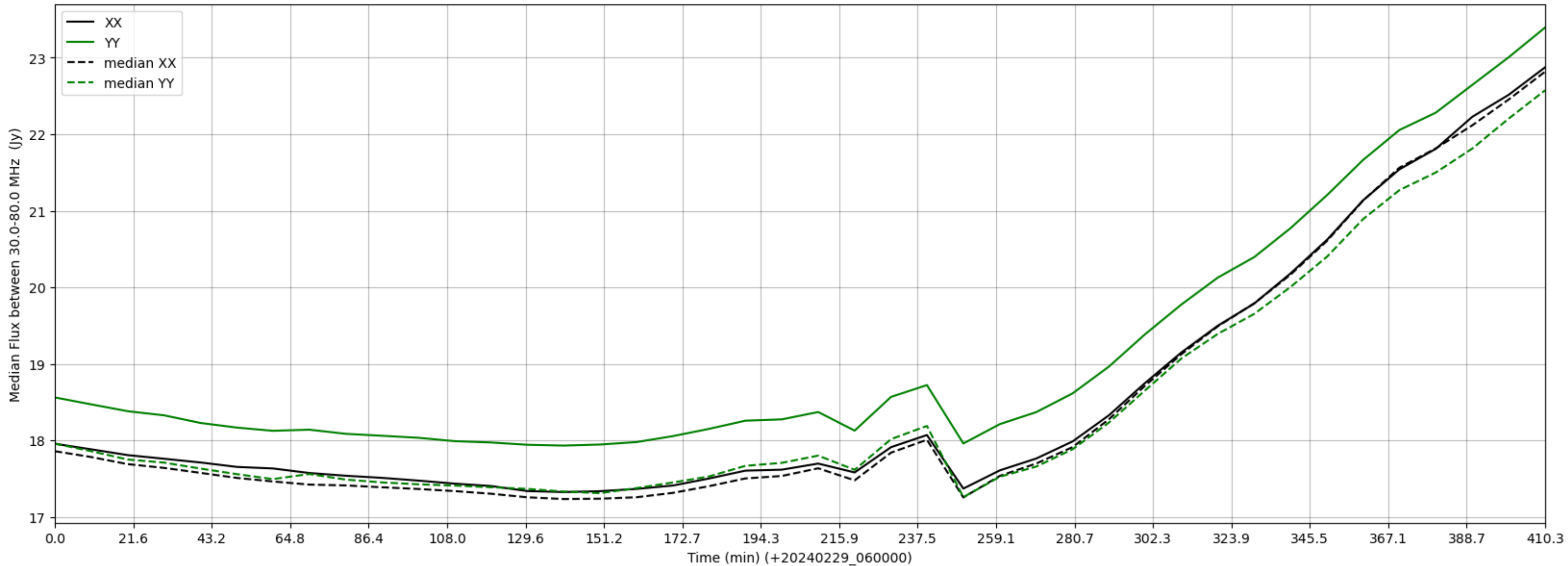
LWA013 - Correlator# 096 - XX FLAGS:Good - YY FLAGS:BadSpecShape
