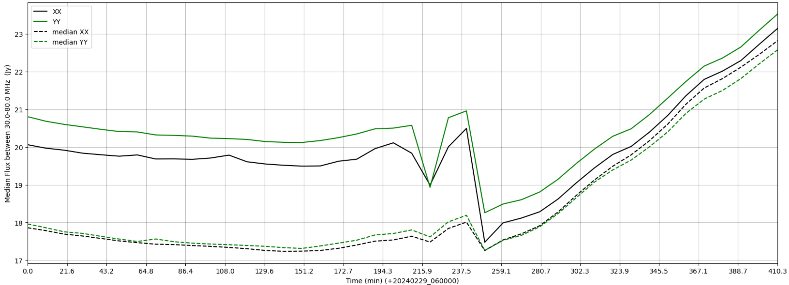
LWA001 - Correlator# 065 - XX FLAGS:Good - YY FLAGS:BadSpecShape
