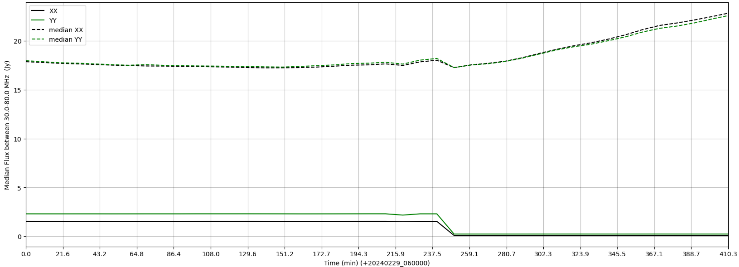
LWA297 - Correlator# 314 - XX FLAGS:LowFlux - YY FLAGS:HighTimeVar+BadSpecShape
