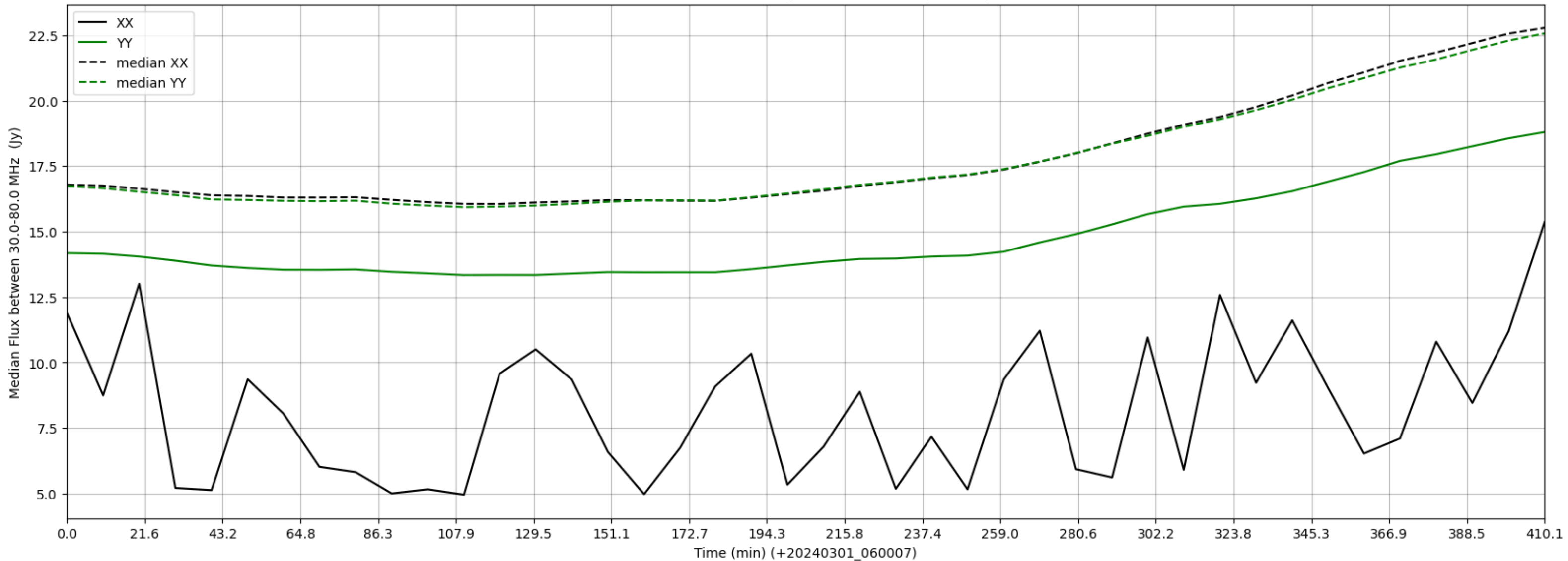
LWA335 - Correlator# 057 - XX FLAGS:HighTimeVar+BadSpecShape - YY FLAGS:Good
