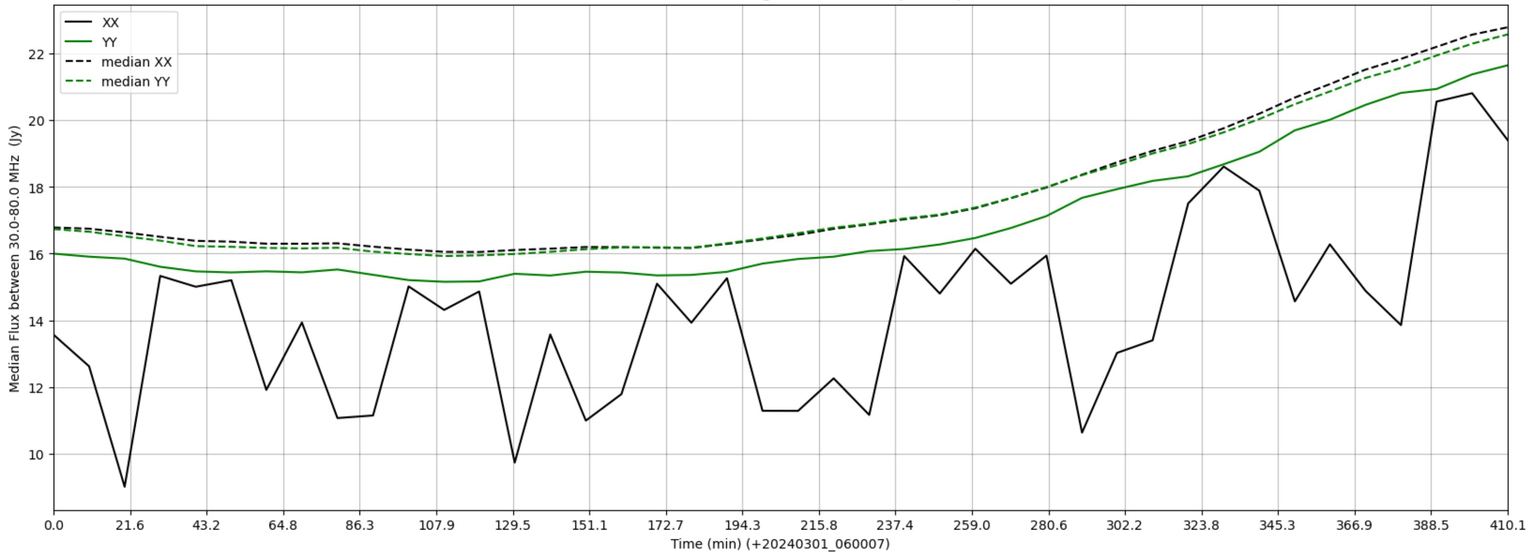
LWA120 - Correlator# 208 - XX FLAGS:HighTimeVar+BadSpecShape - YY FLAGS:Good
