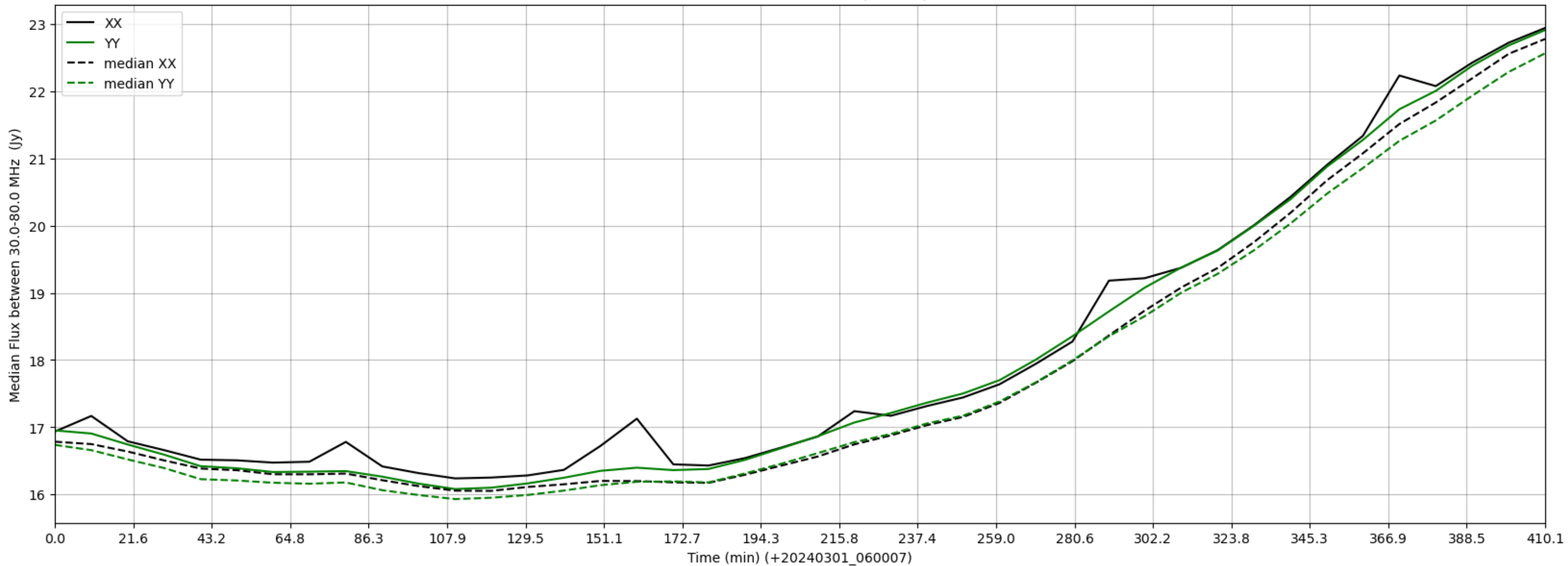
LWA228 - Correlator# 302 - XX FLAGS:BadSpecShape - YY FLAGS:Good
