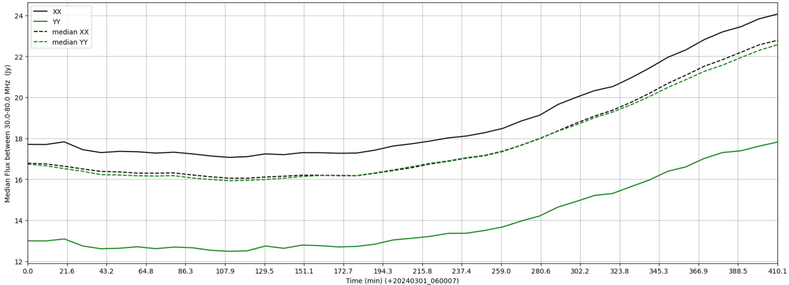
LWA142 - Correlator# 211 - XX FLAGS:Good - YY FLAGS:BadSpecShape
