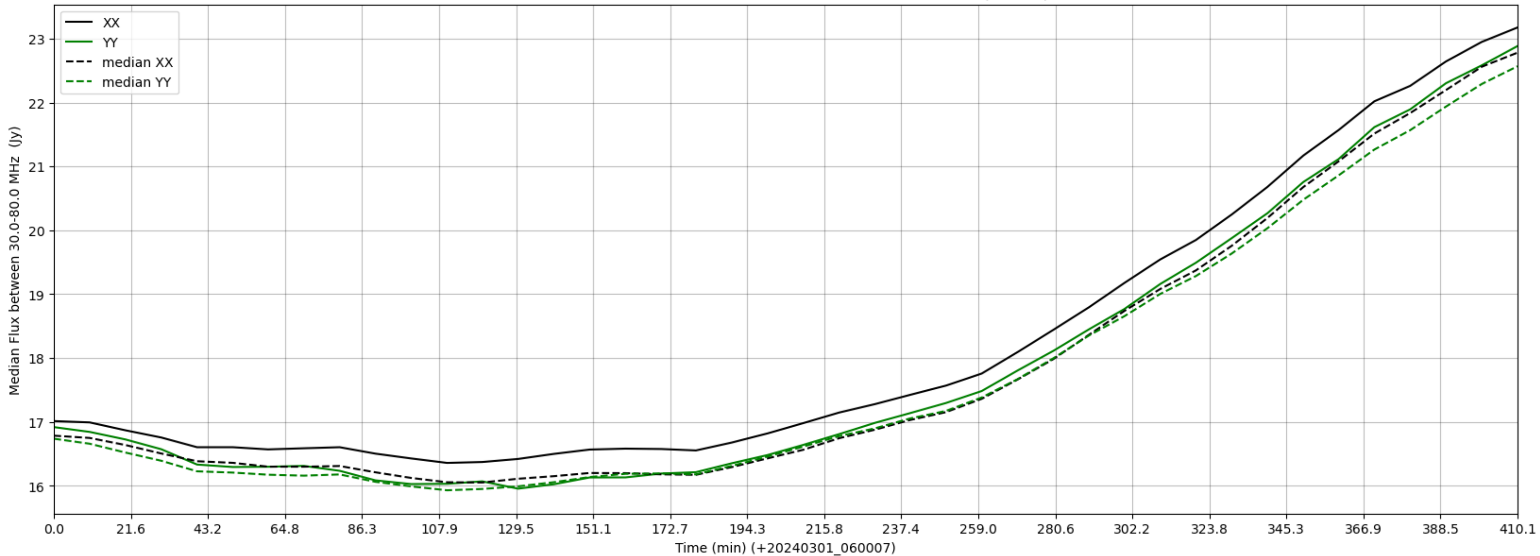
LWA043 - Correlator# 081 - XX FLAGS:Good - YY FLAGS:BadSpecShape
