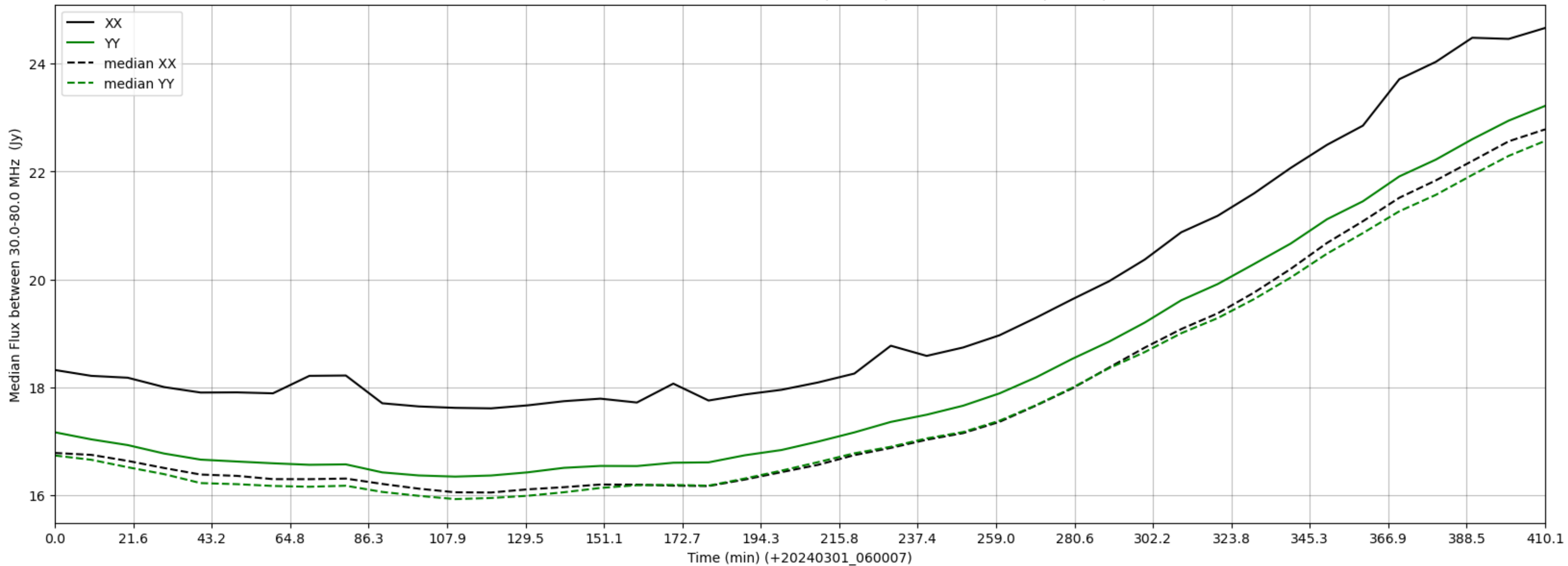
LWA040 - Correlator# 076 - XX FLAGS:BadSpecShape - YY FLAGS:BadSpecShape
