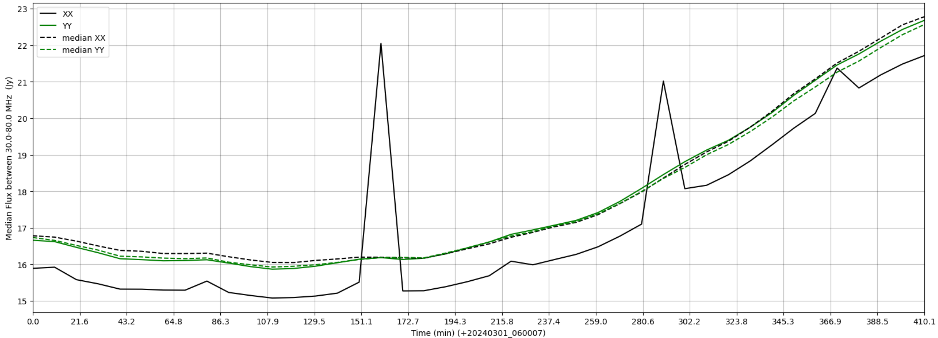
LWA226 - Correlator# 304 - XX FLAGS:BadSpecShape - YY FLAGS:Good
