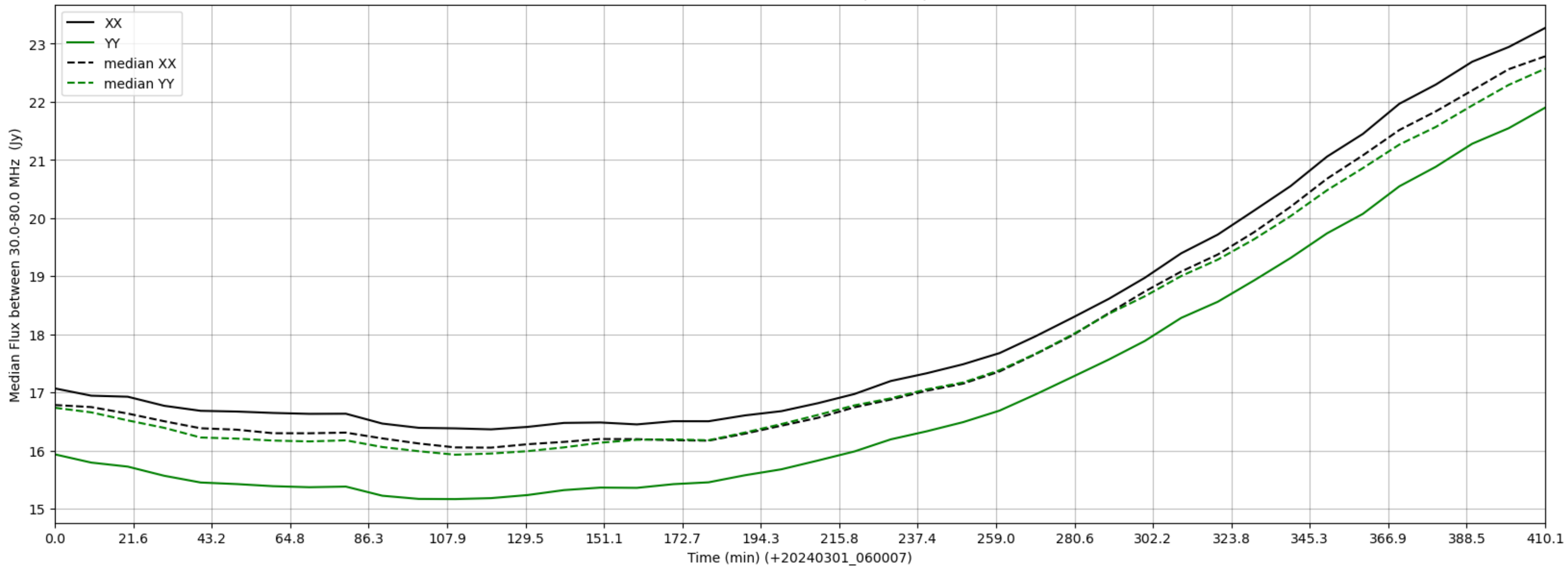
LWA008 - Correlator# 075 - XX FLAGS:BadSpecShape - YY FLAGS:Good
