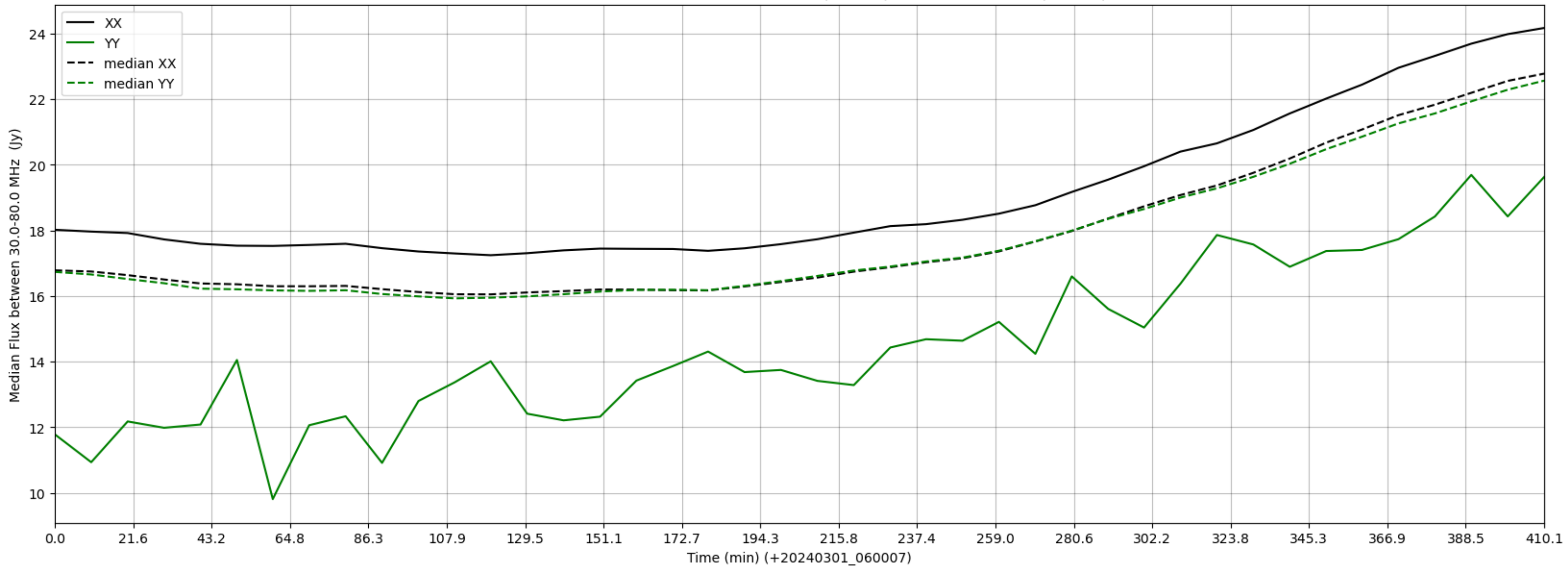
LWA009 - Correlator# 070 - XX FLAGS:BadSpecShape - YY FLAGS:BadSpecShape
