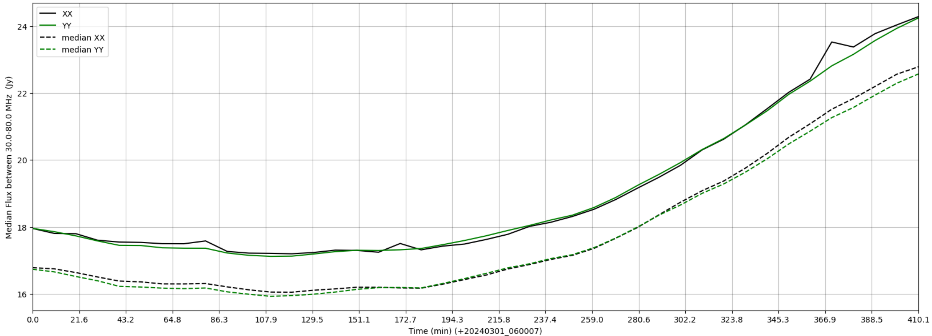
LWA012 - Correlator# 074 - XX FLAGS:BadSpecShape - YY FLAGS:BadSpecShape
