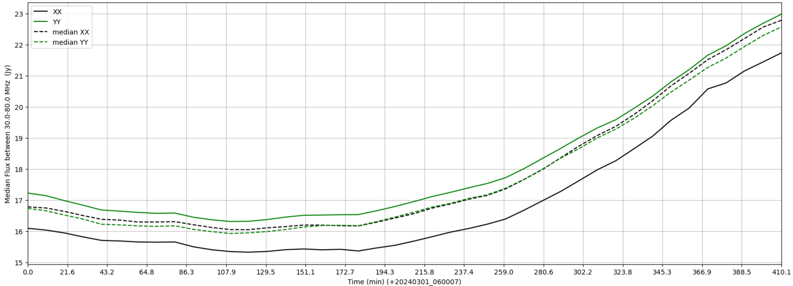
LWA011 - Correlator# 072 - XX FLAGS:BadSpecShape - YY FLAGS:Good
