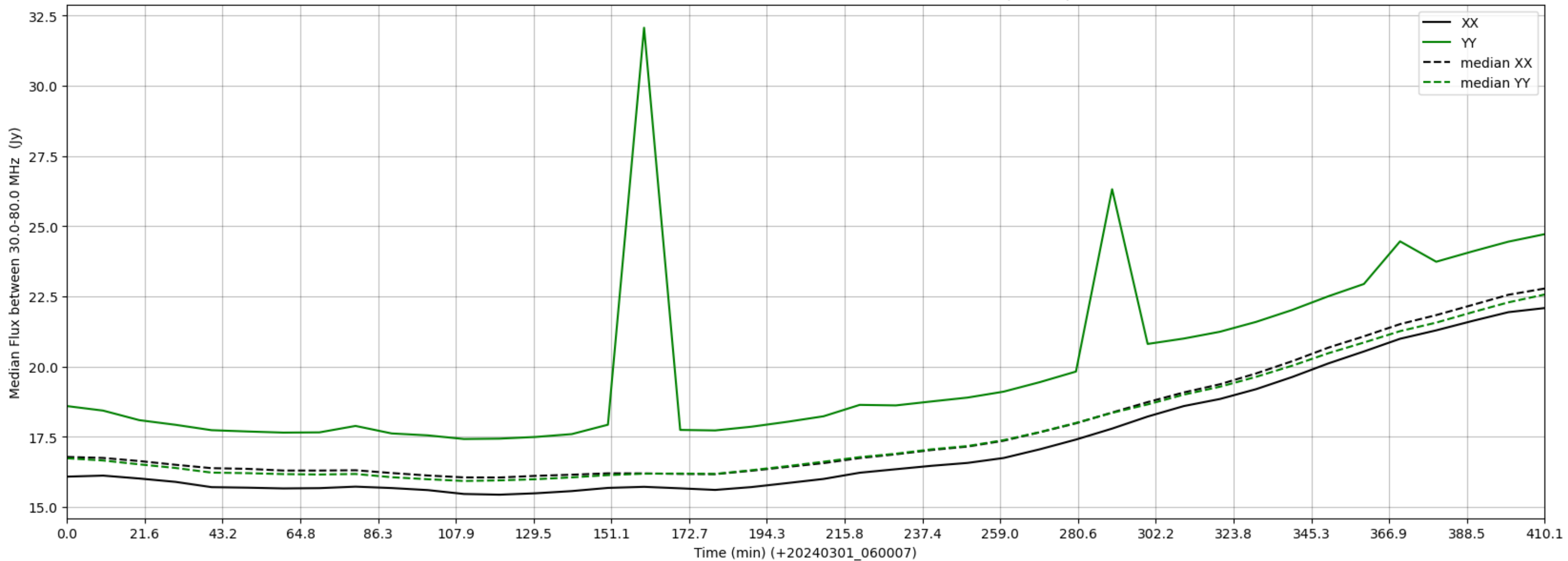
LWA173 - Correlator# 290 - XX FLAGS:Good - YY FLAGS:BadSpecShape
