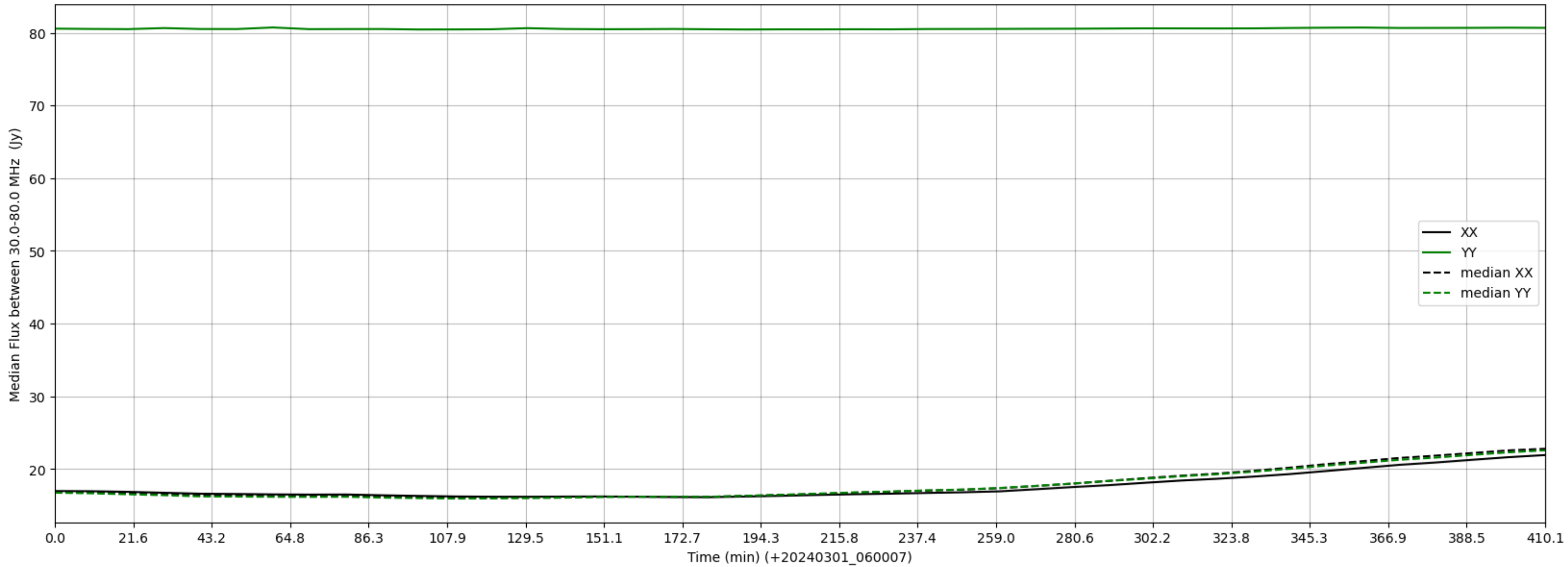
LWA280 - Correlator# 041 - XX FLAGS:BadSpecShape - YY FLAGS:BadSpecShape
