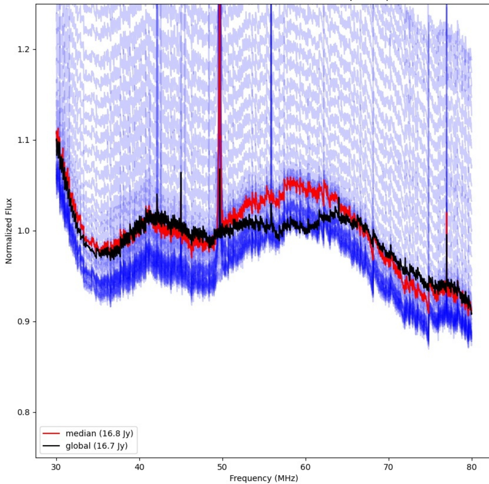
LWA043 - Correlator# 081 - YY - FLAGS:BadSpecShape
