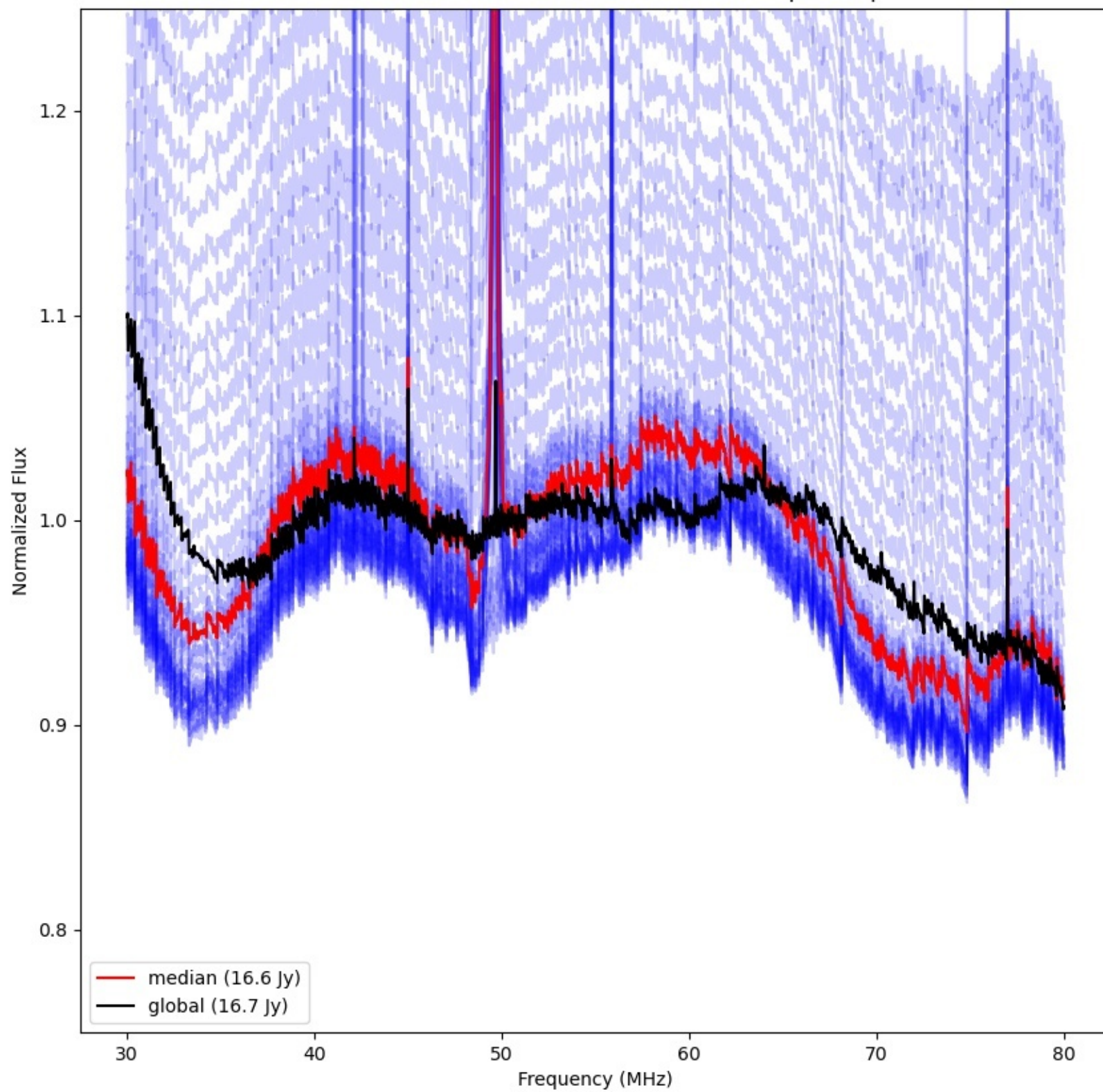
LWA071 - Correlator# 084 - YY - FLAGS:BadSpecShape
