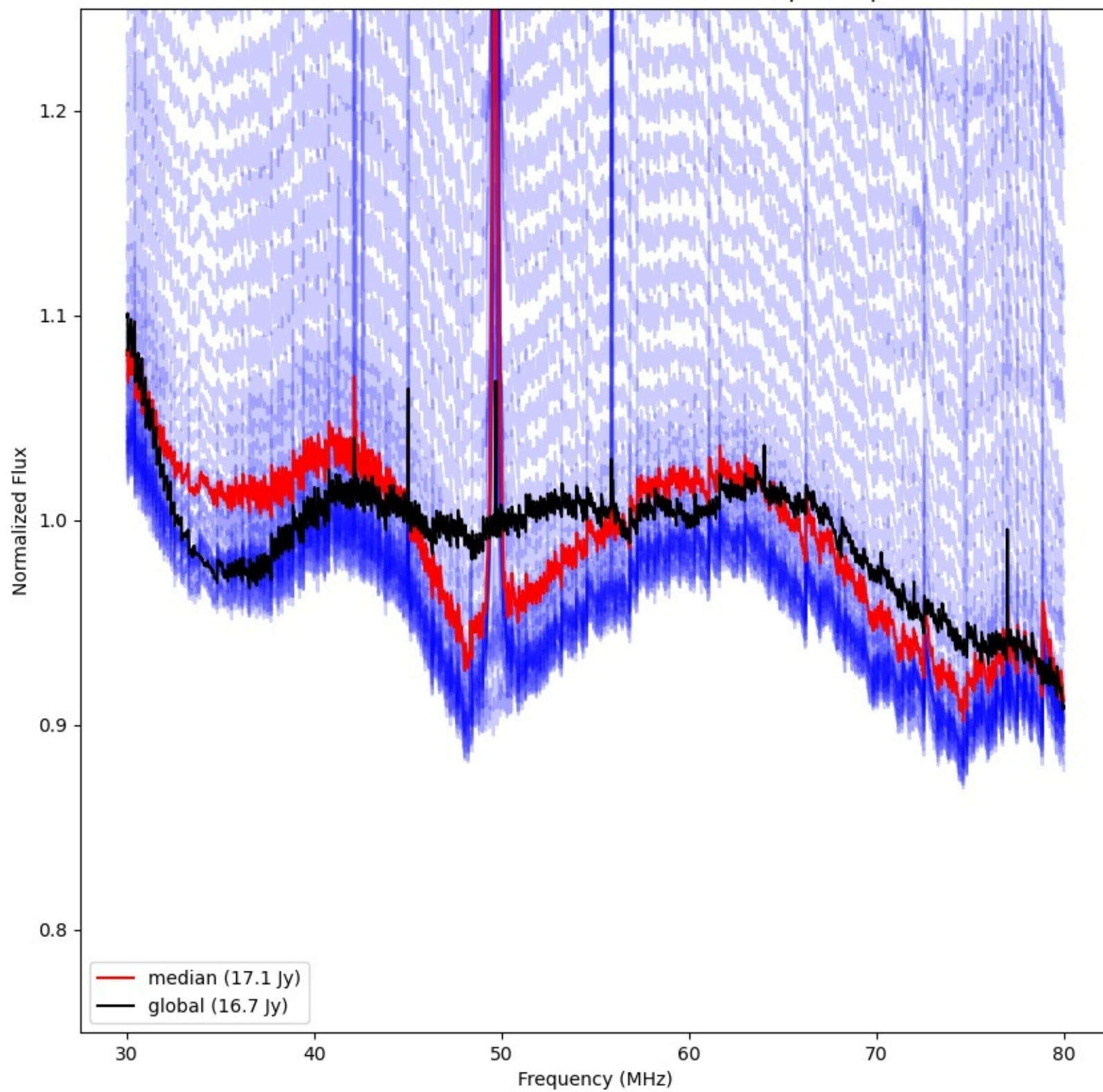
LWA040 - Correlator# 076 - YY - FLAGS:BadSpecShape
